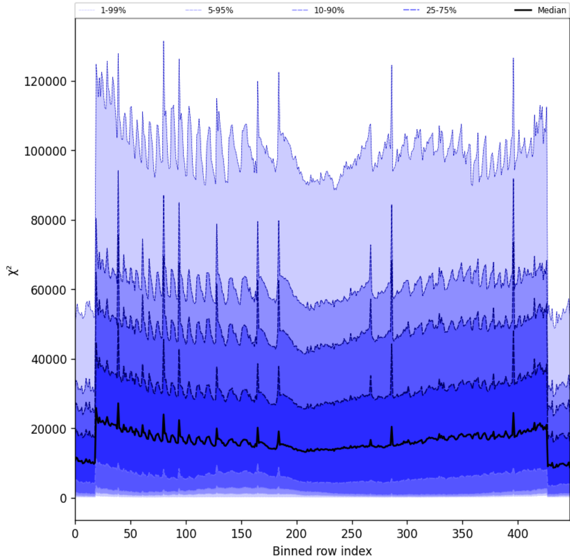
Figure 53: Along track statistics of “ \chi^2 ” for 2025-03-29 to 2025-03-30
