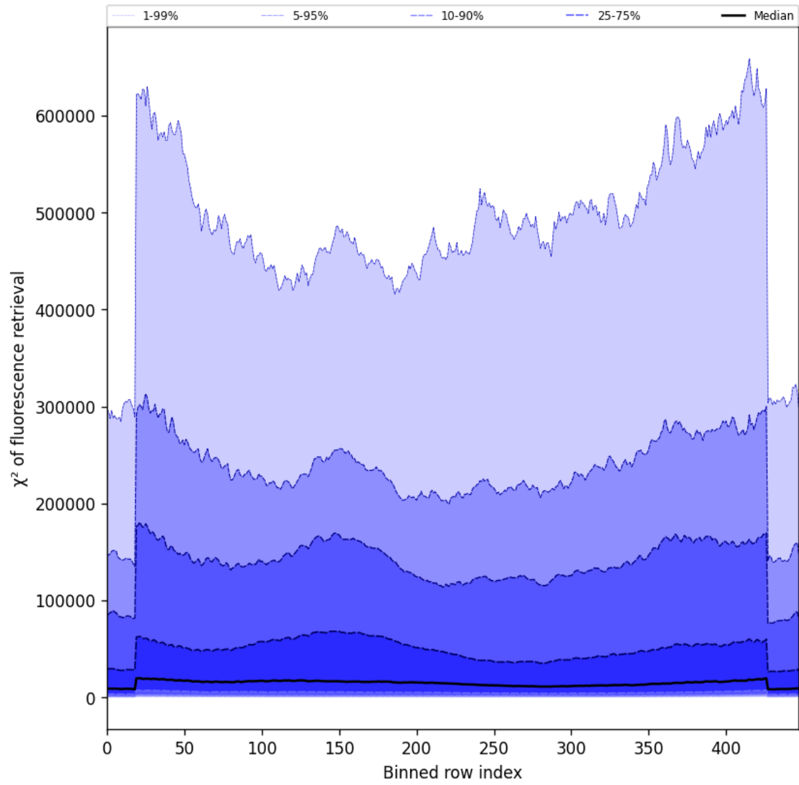
Figure 57: Along track statistics of “ \chi^2 of fluorescence retrieval” for 2025-03-29 to 2025-03-30
