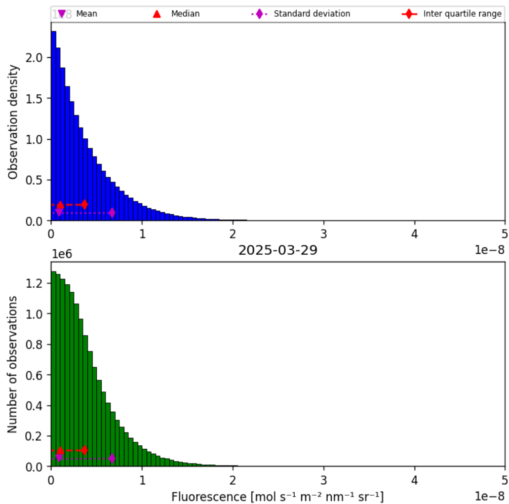
Figure 38: Histogram of “Fluorescence” for 2025-03-29 to 2025-03-30
