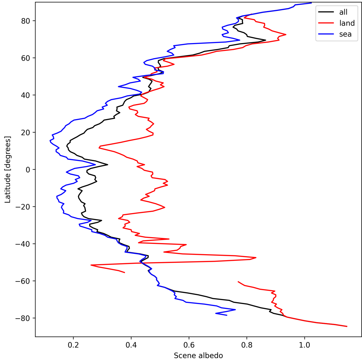
Figure 15: Zonal average of “Scene albedo” for 2025-03-29 to 2025-03-30.
