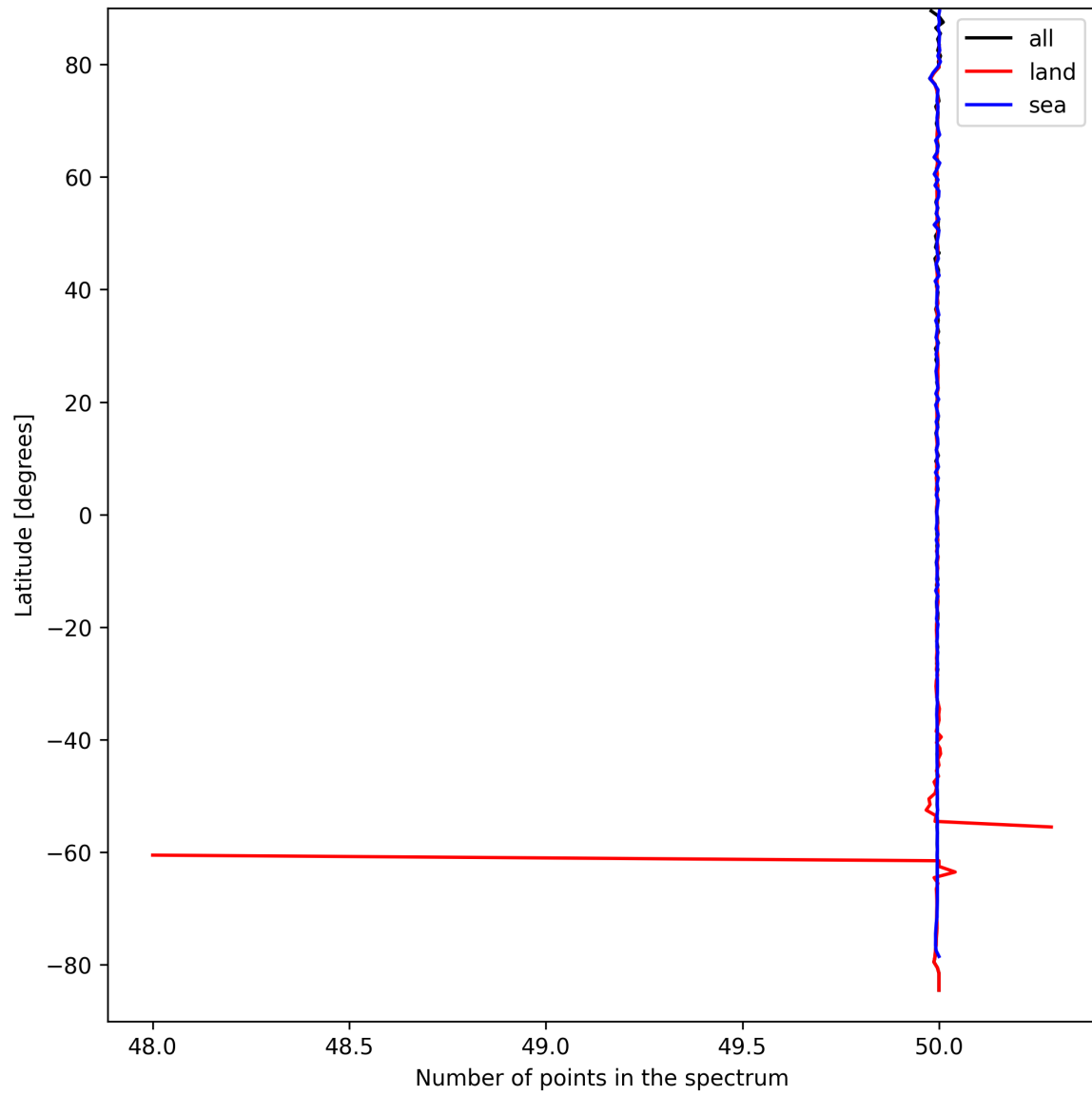
Figure 25: Zonal average of “Number of points in the spectrum” for 2025-03-29 to 2025-03-30.
