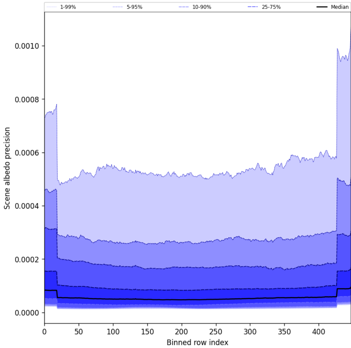
Figure 50: Along track statistics of “Scene albedo precision” for 2025-03-29 to 2025-03-30
