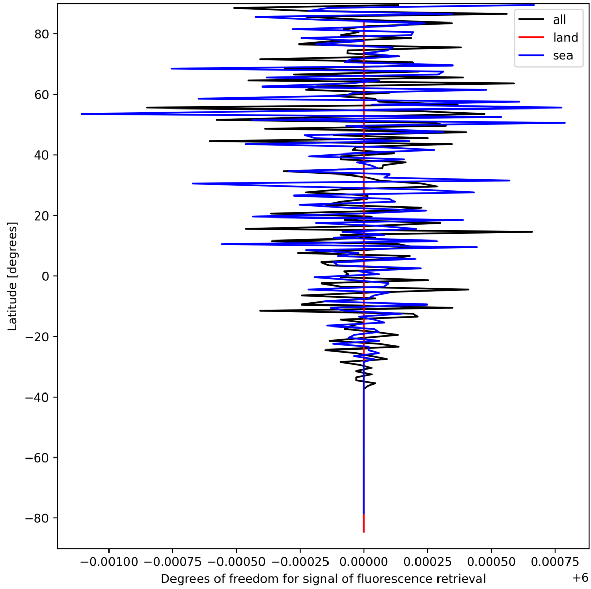
Figure 24: Zonal average of “Degrees of freedom for signal of fluorescence retrieval” for 2025-03-29 to 2025-03-30.
