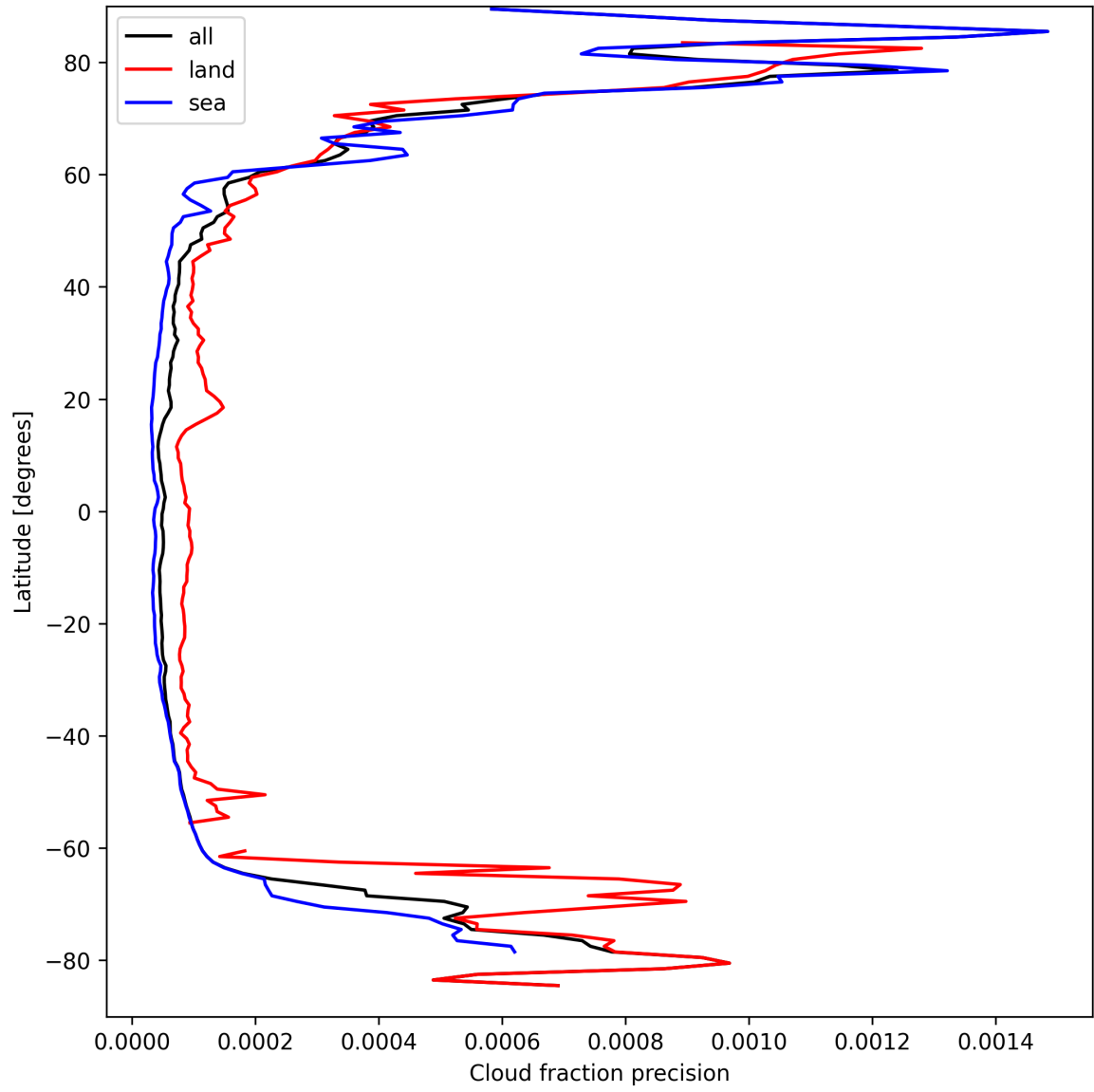
Figure 14: Zonal average of “Cloud fraction precision” for 2025-03-29 to 2025-03-30.
