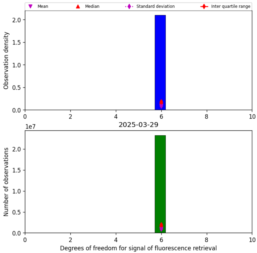
Figure 41: Histogram of “Degrees of freedom for signal of fluorescence retrieval” for 2025-03-29 to 2025-03-30
