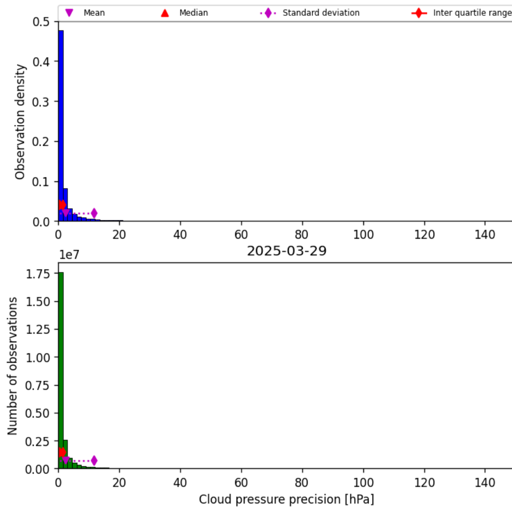
Figure 29: Histogram of “Cloud pressure precision” for 2025-03-29 to 2025-03-30
