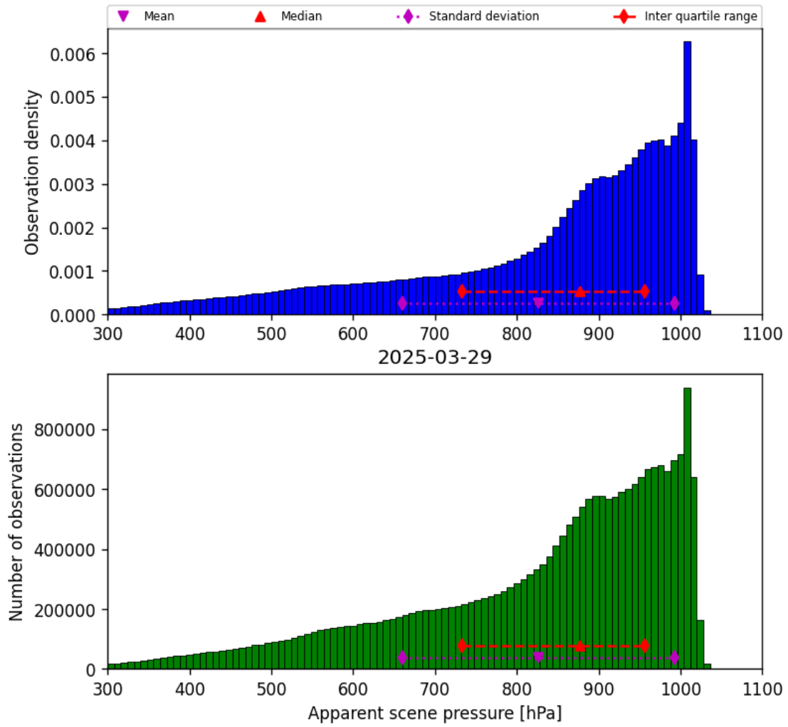
Figure 34: Histogram of “Apparent scene pressure” for 2025-03-29 to 2025-03-30
