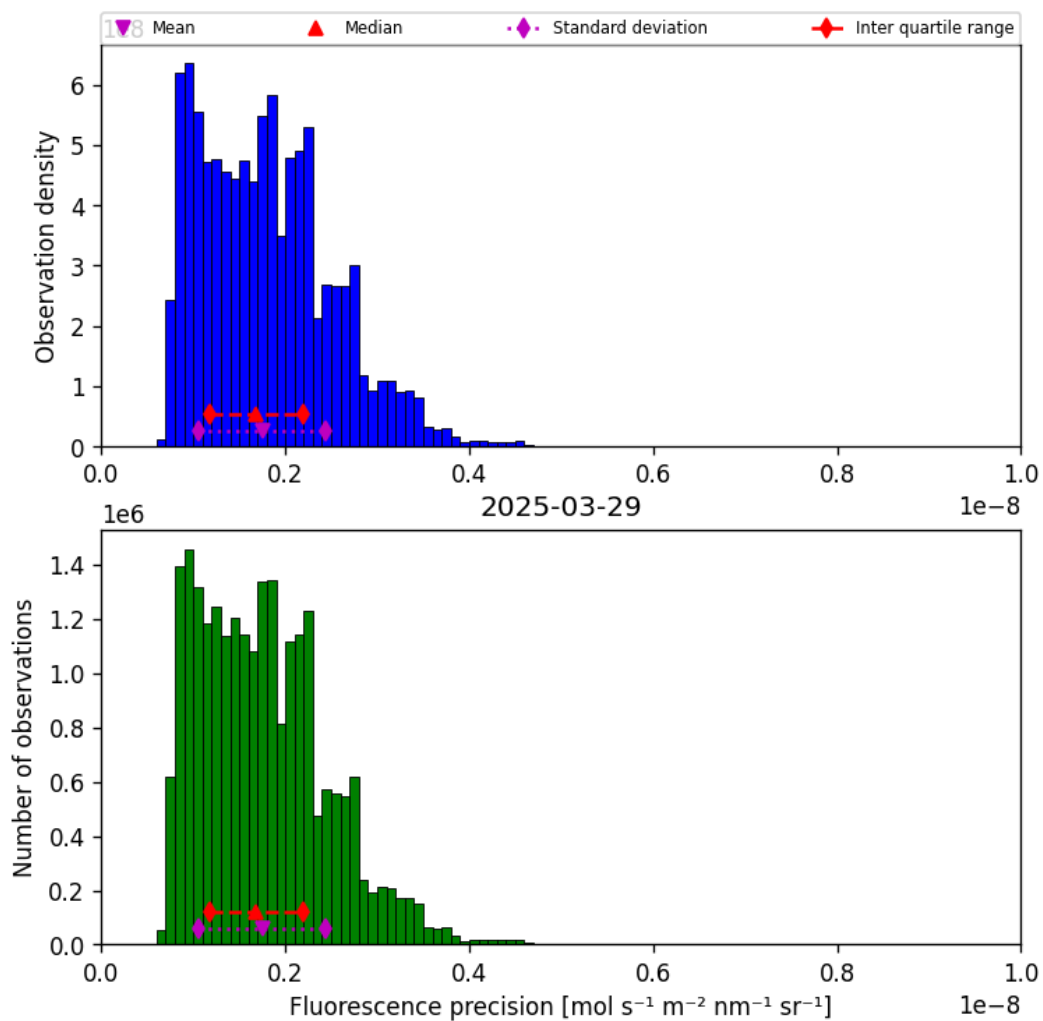
Figure 39: Histogram of “Fluorescence precision” for 2025-03-29 to 2025-03-30
