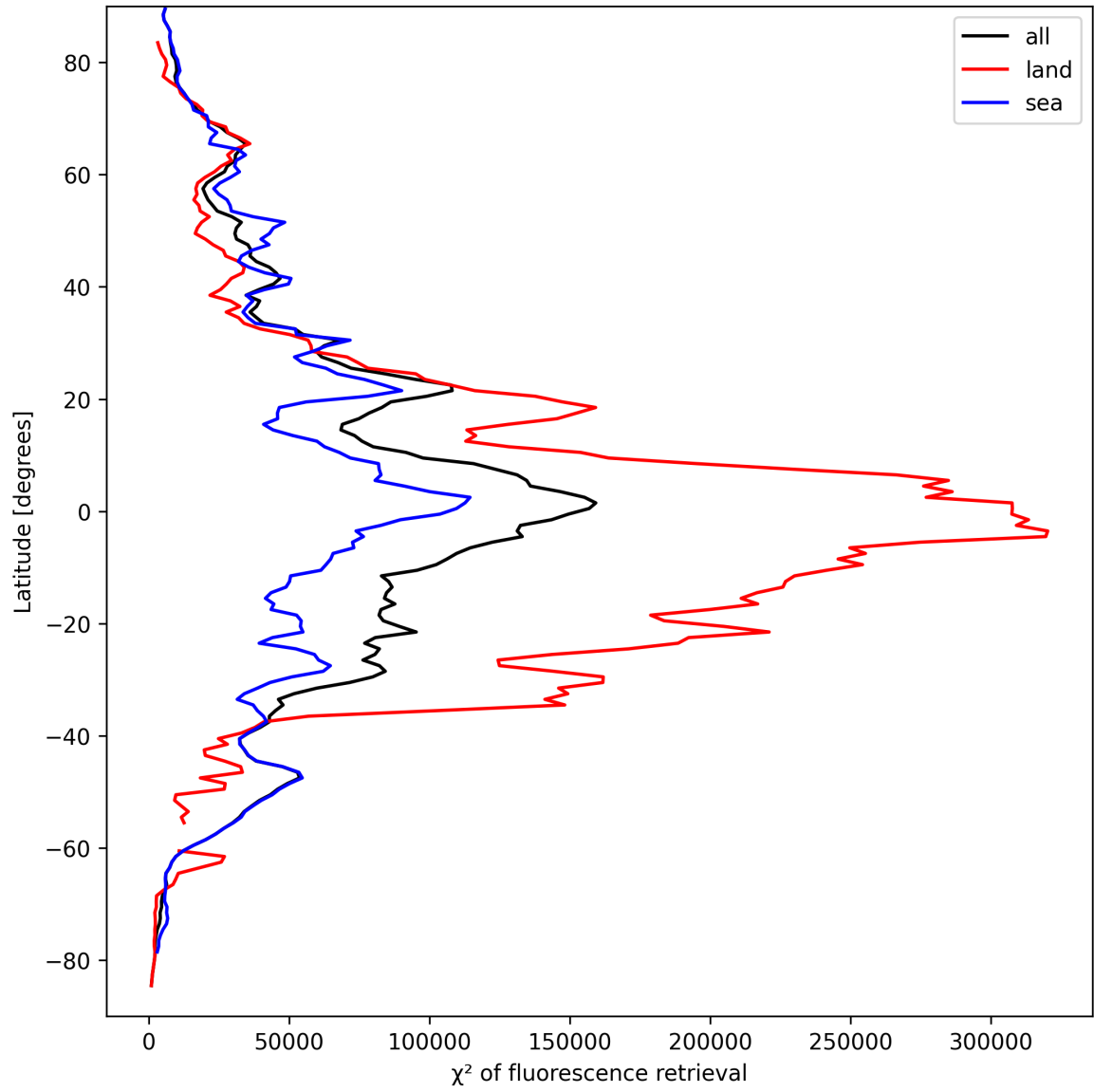
Figure 23: Zonal average of “ \chi^2 of fluorescence retrieval” for 2025-03-29 to 2025-03-30.
