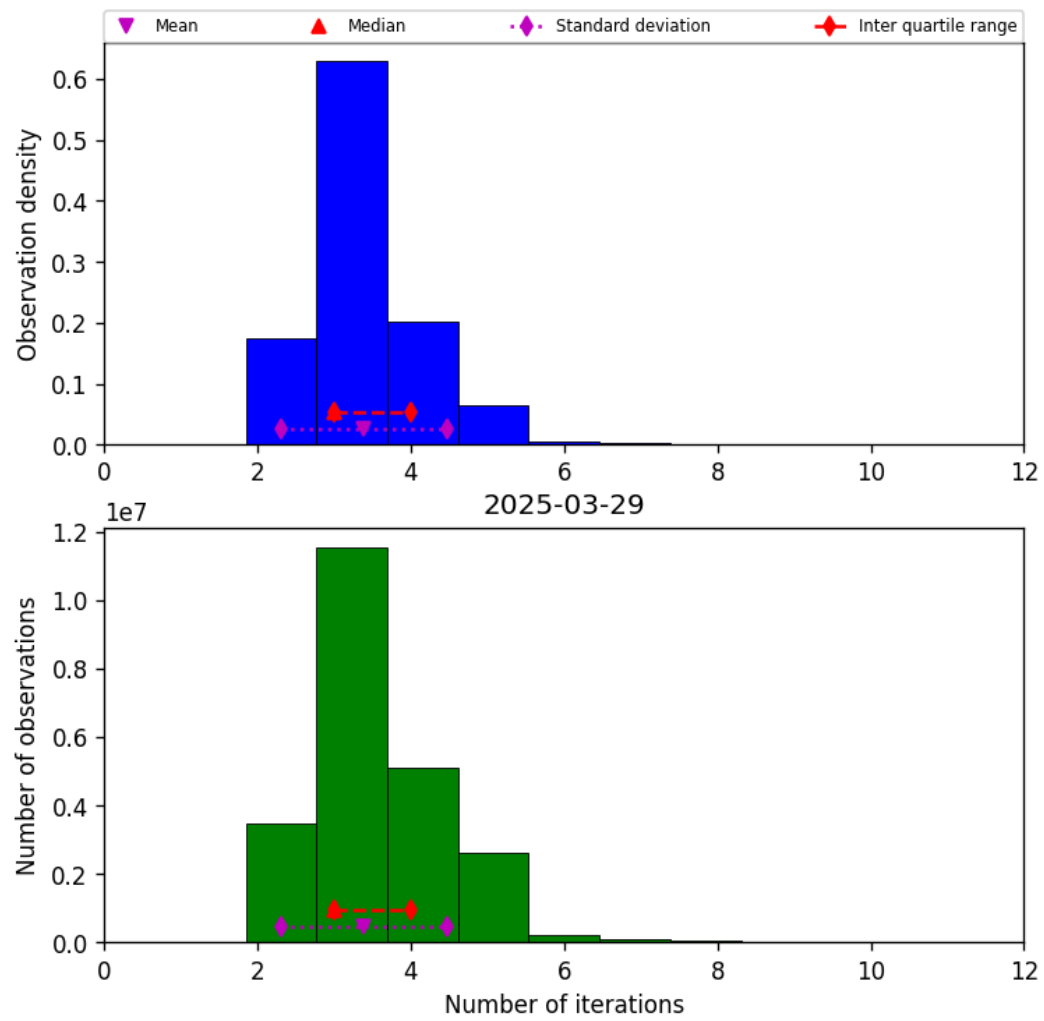
Figure 37: Histogram of “Number of iterations” for 2025-03-29 to 2025-03-30
