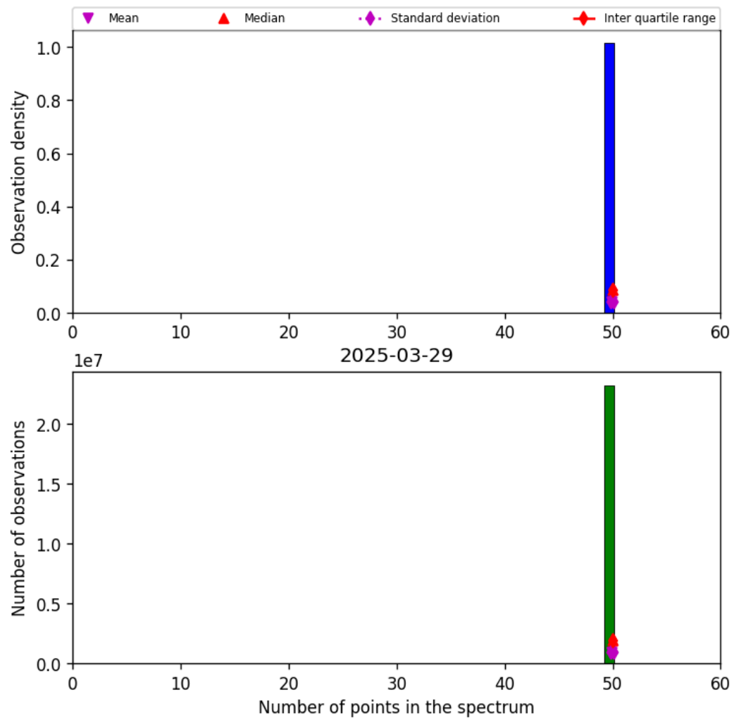
Figure 42: Histogram of “Number of points in the spectrum” for 2025-03-29 to 2025-03-30
