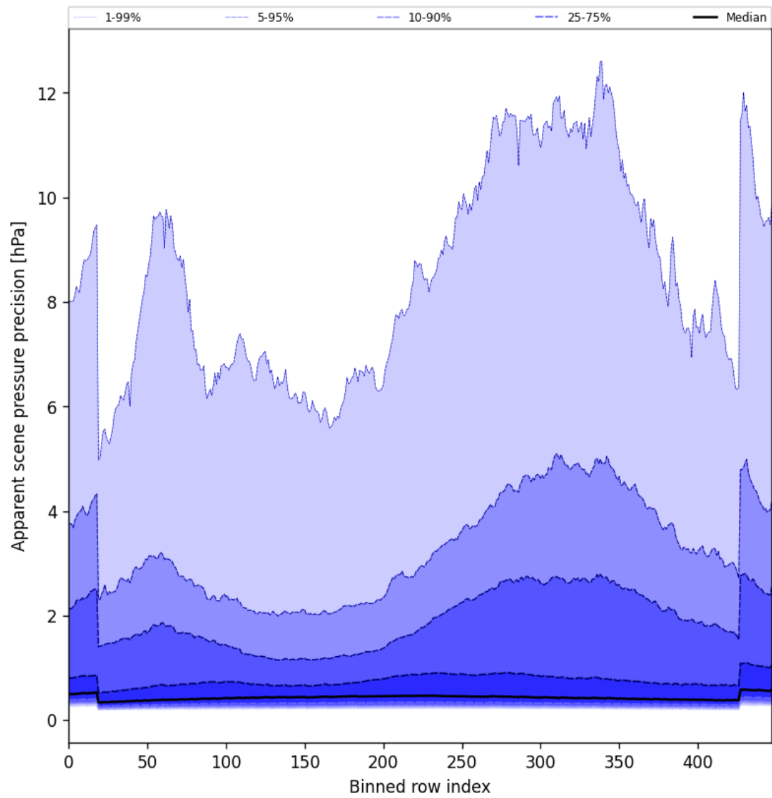
Figure 52: Along track statistics of “Apparent scene pressure precision” for 2025-03-29 to 2025-03-30
