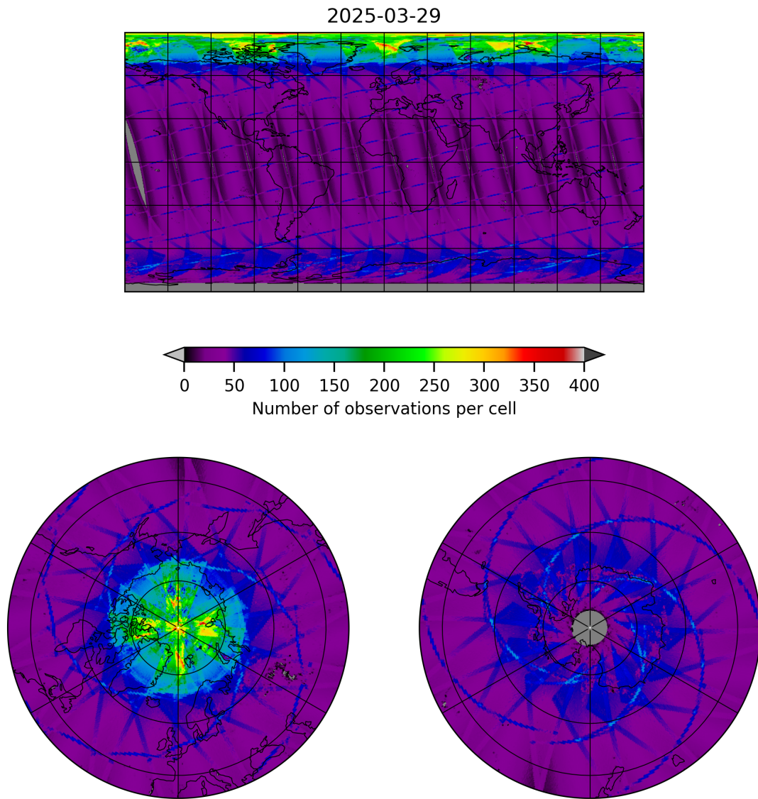
Figure 9: Map of the number of observations for 2025-03-29 to 2025-03-30
