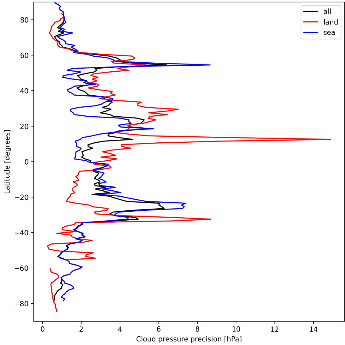
Figure 12: Zonal average of "Cloud pressure precision" for 2025-03-29 to 2025-03-30.
