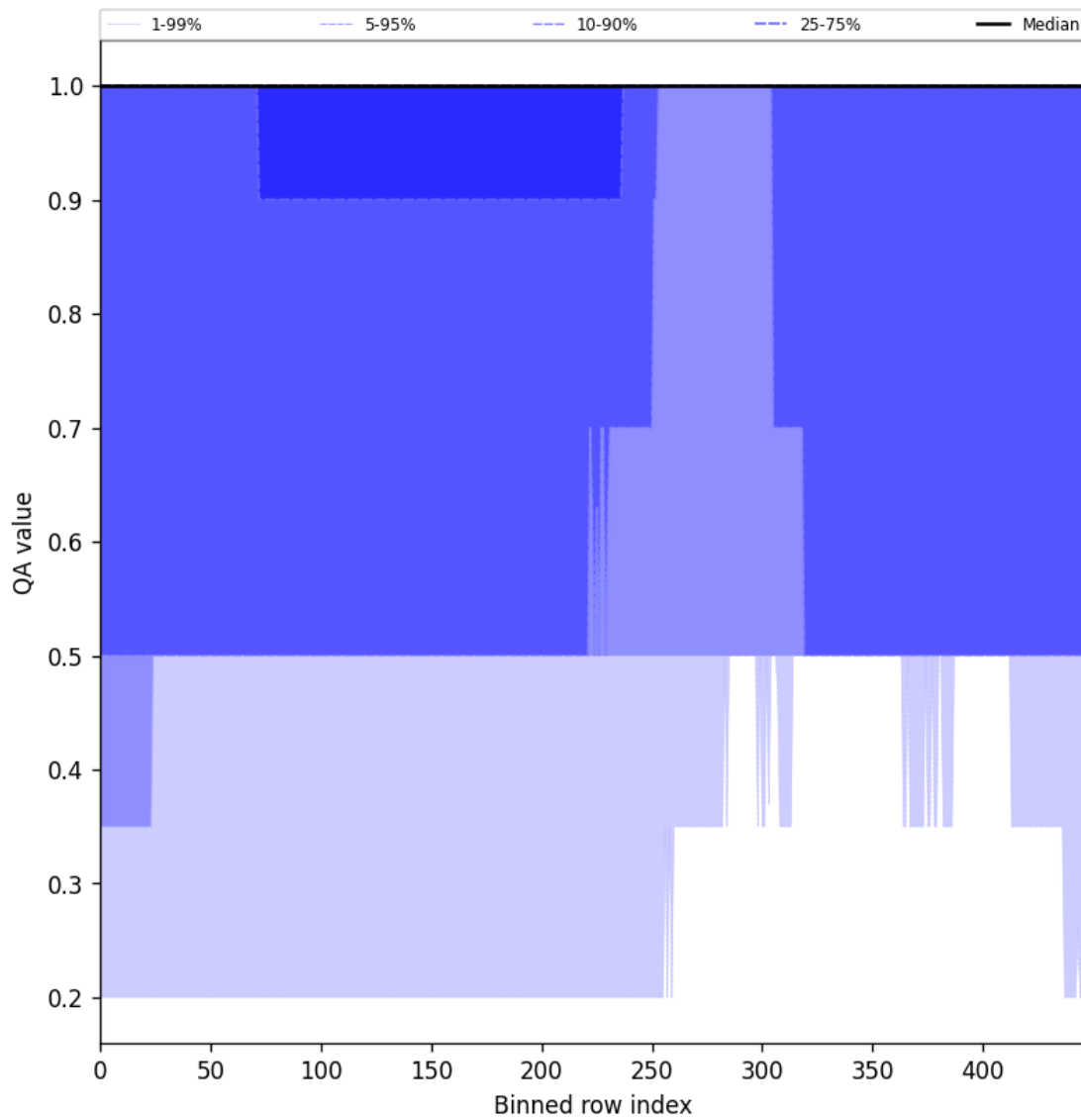
Figure 44: Along track statistics of “QA value” for 2025-03-29 to 2025-03-30
