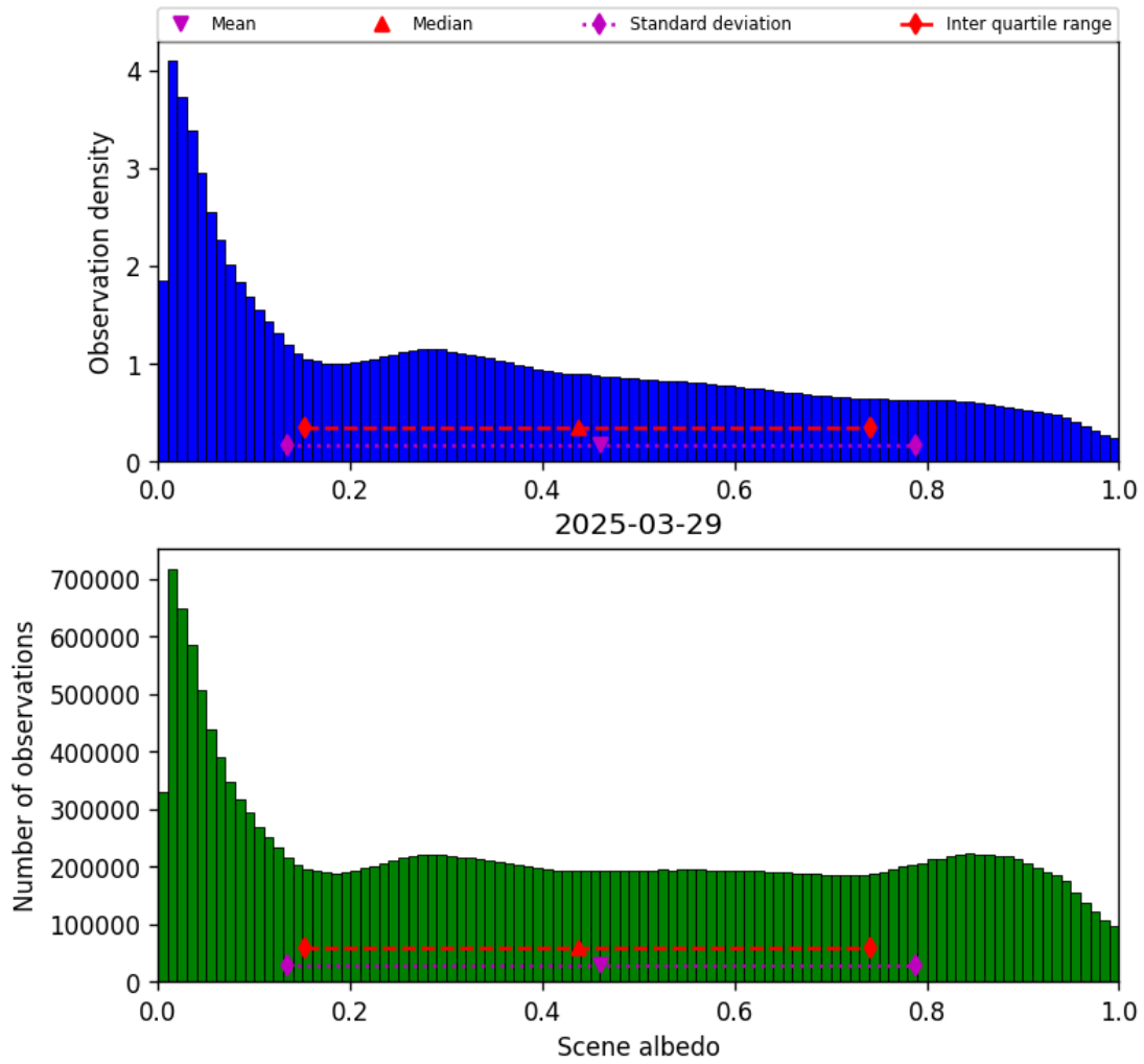
Figure 32: Histogram of “Scene albedo” for 2025-03-29 to 2025-03-30
