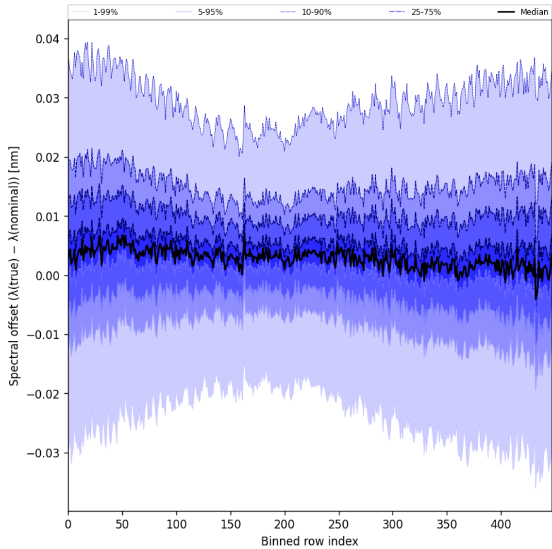
Figure 60: Along track statistics of “Spectral offset ( \lambda_{\text{true}} - \lambda_{\text{nominal}} )” for 2025-03-29 to 2025-03-30
