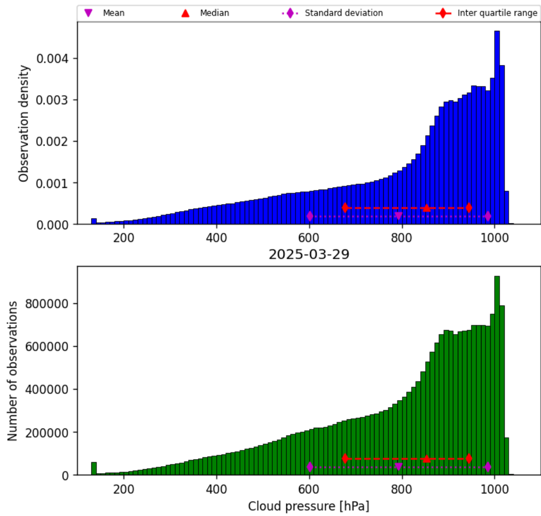
Figure 28: Histogram of “Cloud pressure” for 2025-03-29 to 2025-03-30
