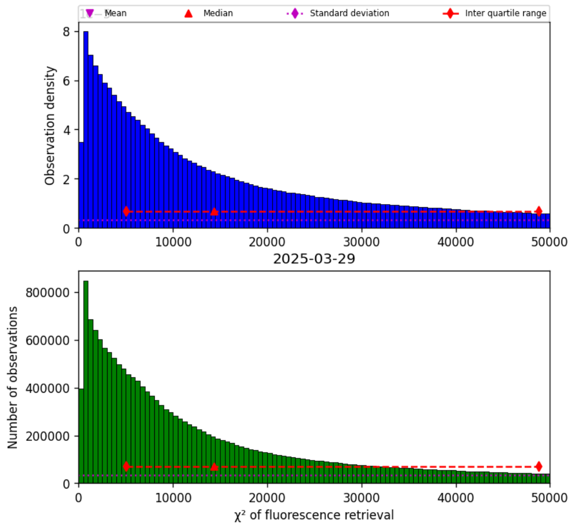
Figure 40: Histogram of “ \chi^2 of fluorescence retrieval” for 2025-03-29 to 2025-03-30
