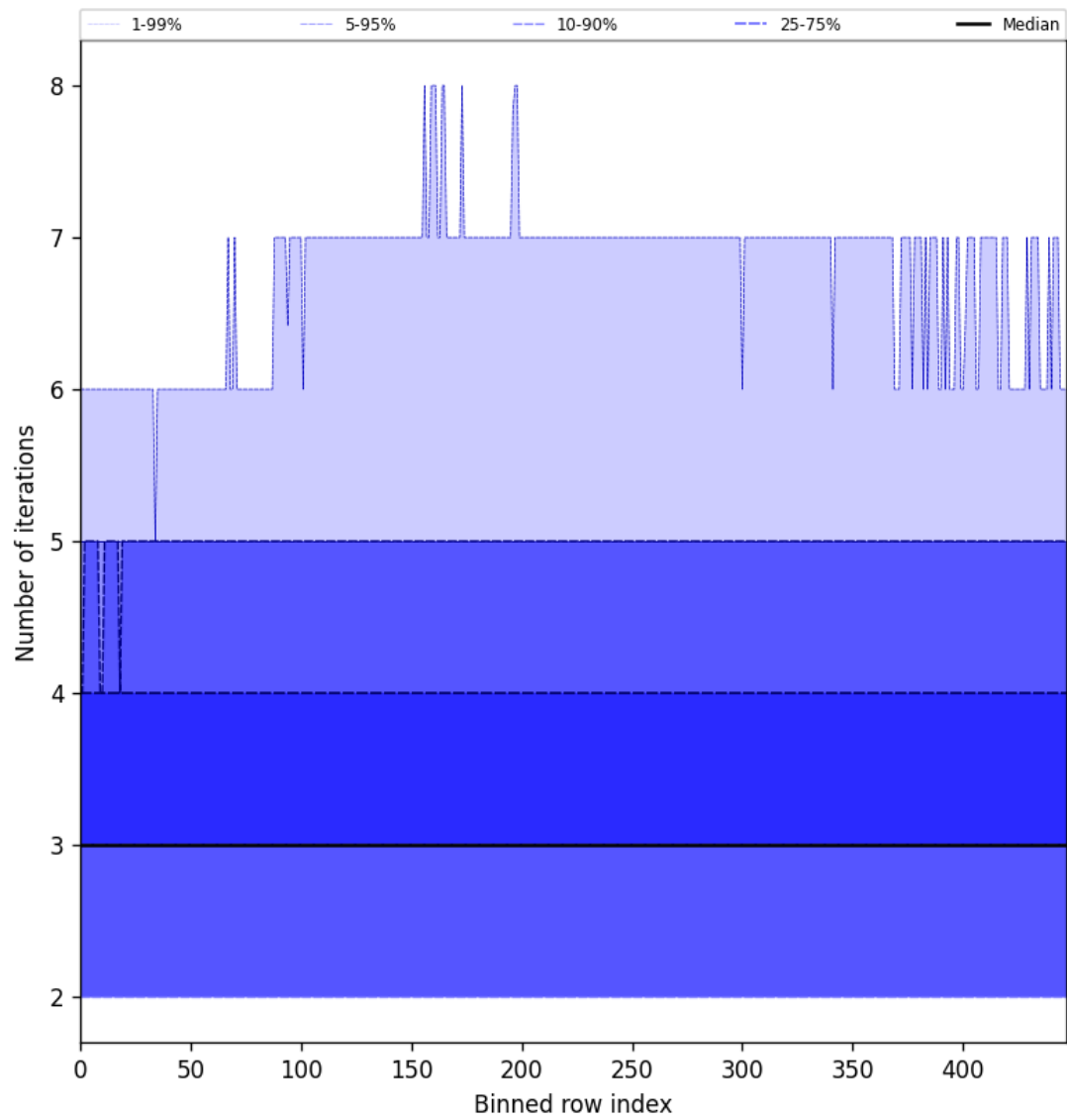
Figure 54: Along track statistics of “Number of iterations” for 2025-03-29 to 2025-03-30
