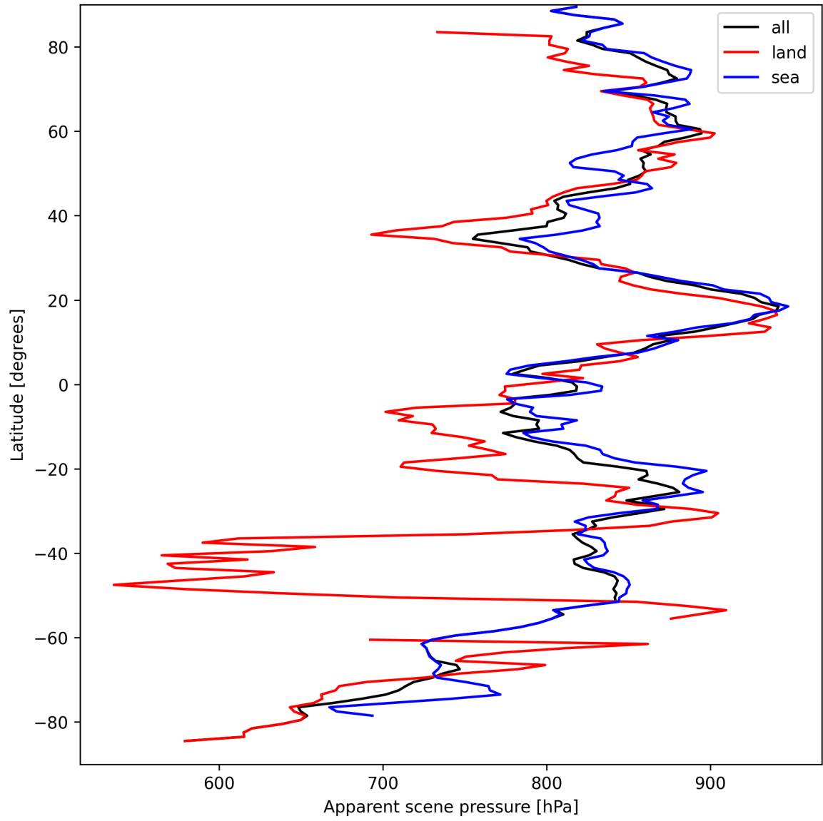
Figure 17: Zonal average of “Apparent scene pressure” for 2025-03-29 to 2025-03-30.
