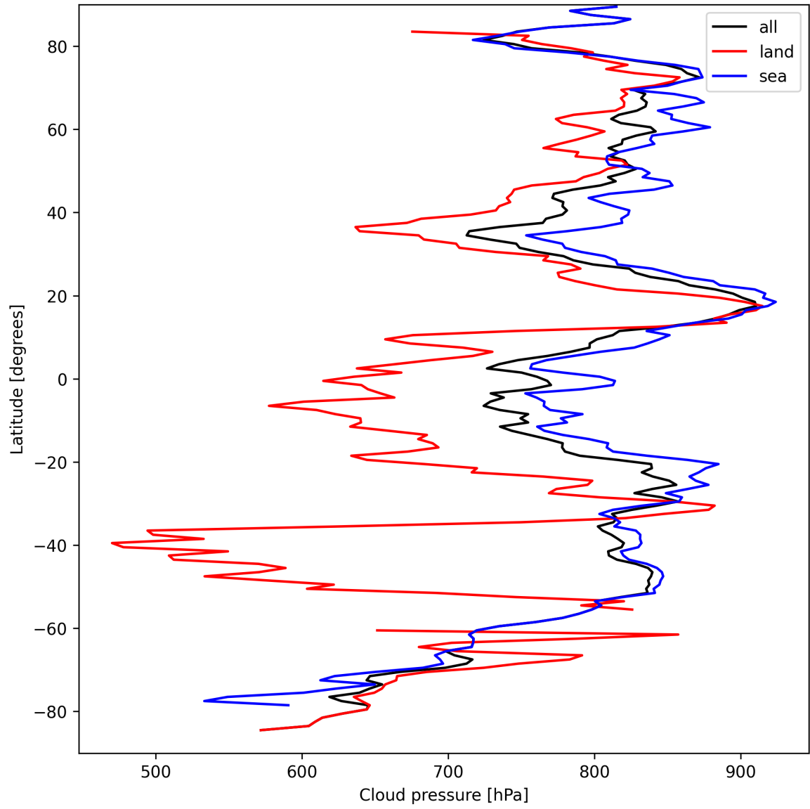
Figure 11: Zonal average of “Cloud pressure” for 2025-03-29 to 2025-03-30.
