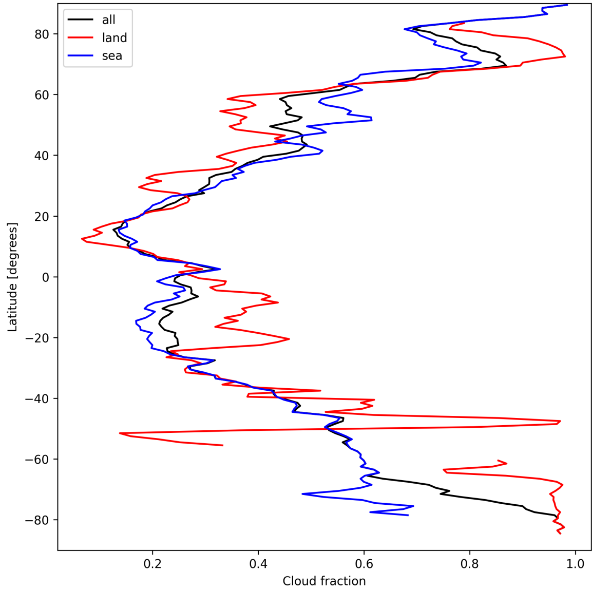
Figure 13: Zonal average of “Cloud fraction” for 2025-03-29 to 2025-03-30.
