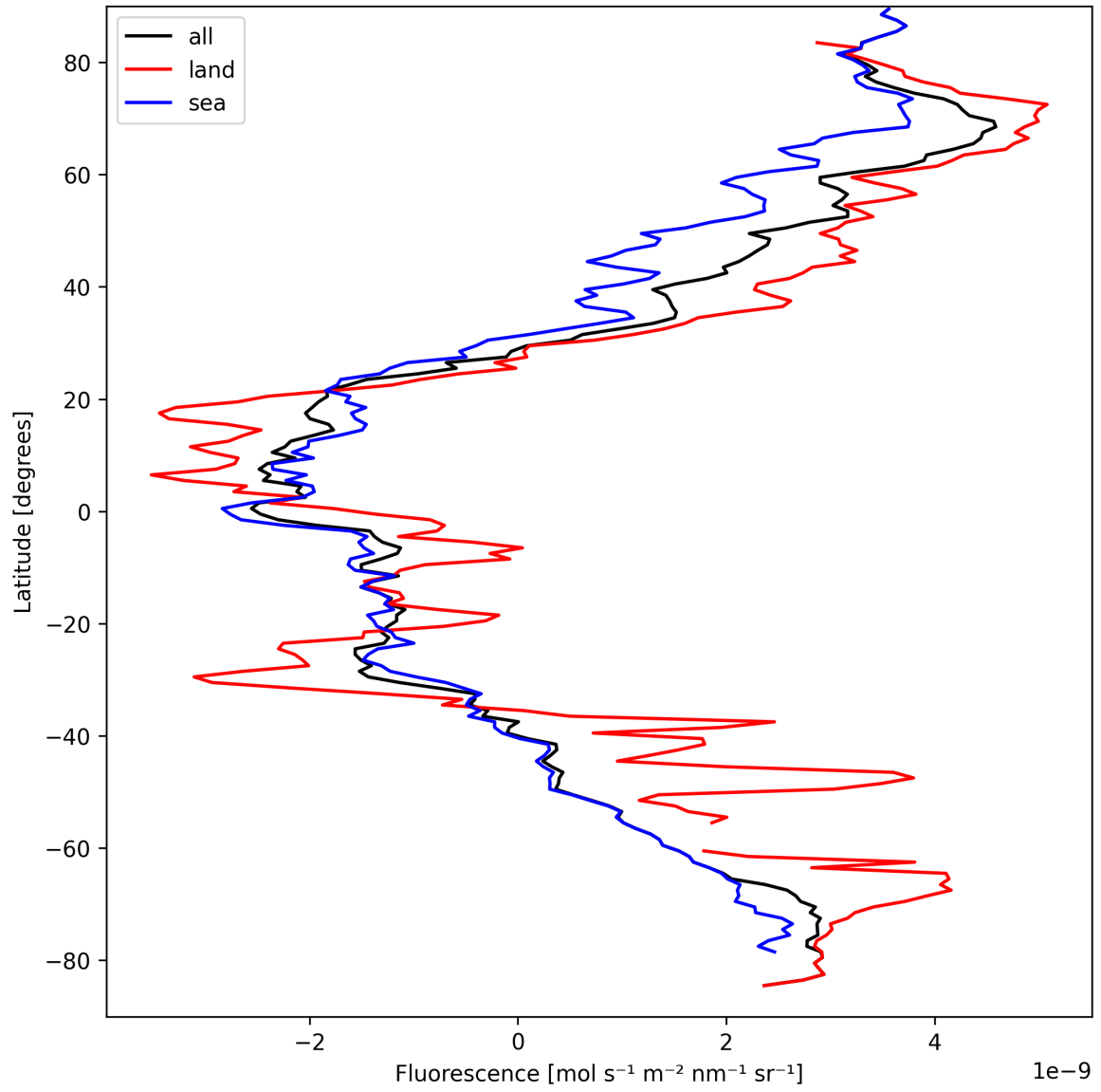
Figure 21: Zonal average of “Fluorescence” for 2025-03-29 to 2025-03-30.
