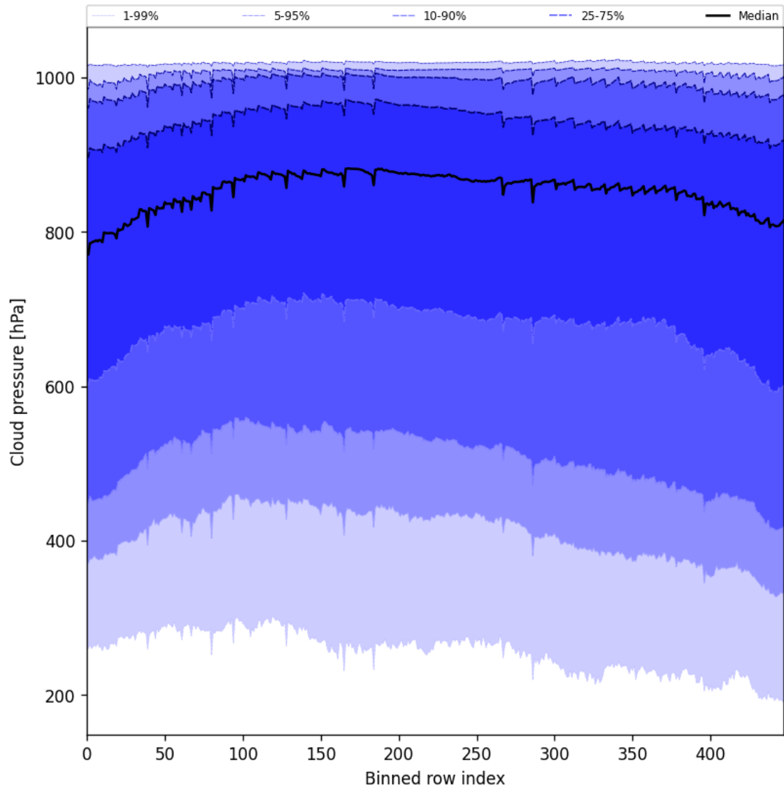
Figure 45: Along track statistics of “Cloud pressure” for 2025-03-29 to 2025-03-30
