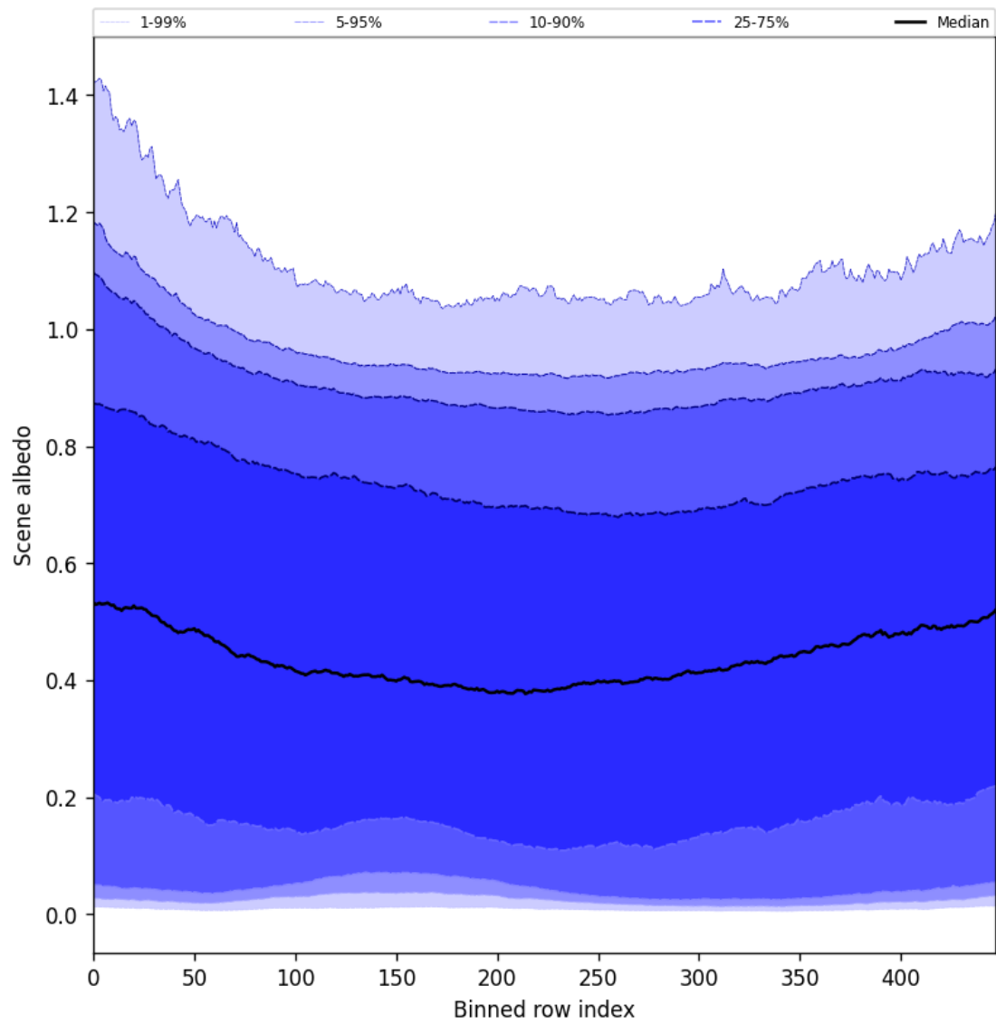
Figure 49: Along track statistics of “Scene albedo” for 2025-03-29 to 2025-03-30
