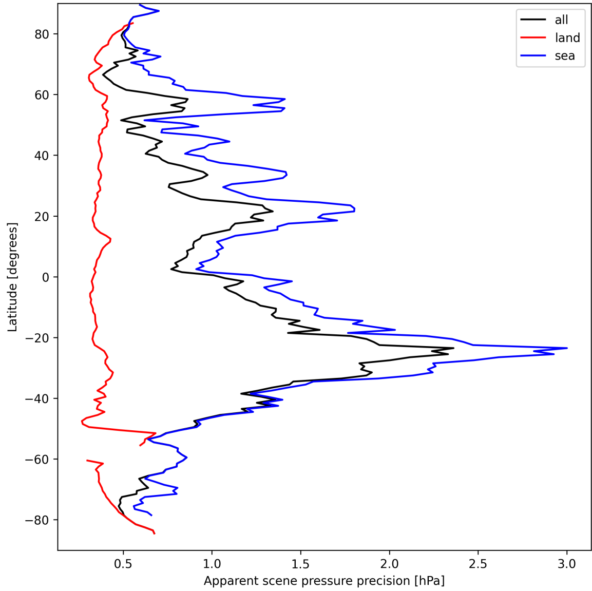
Figure 18: Zonal average of “Apparent scene pressure precision” for 2025-03-29 to 2025-03-30.
