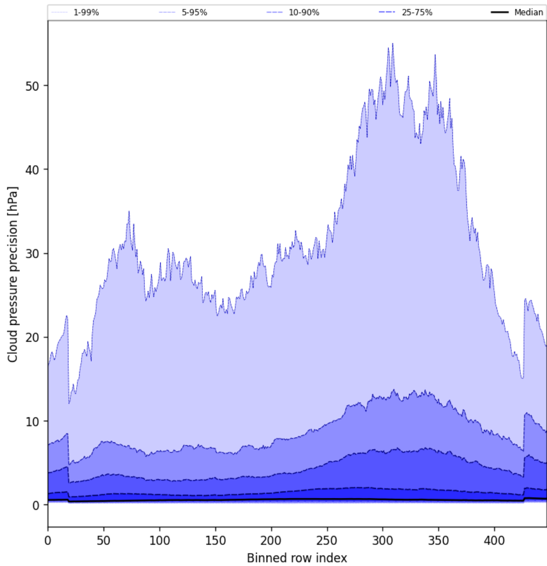
Figure 46: Along track statistics of “Cloud pressure precision” for 2025-03-29 to 2025-03-30
