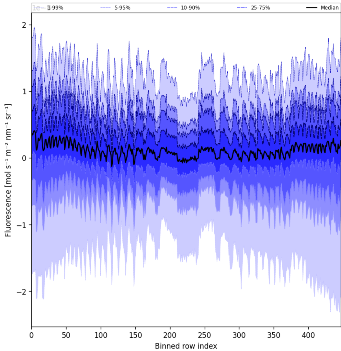
Figure 55: Along track statistics of “Fluorescence” for 2025-03-29 to 2025-03-30
