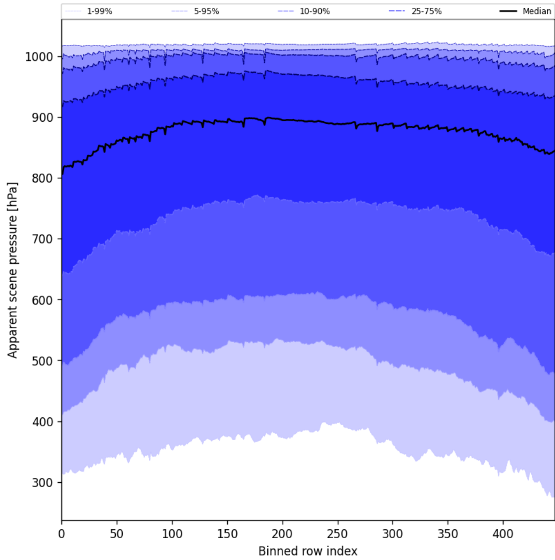
Figure 51: Along track statistics of “Apparent scene pressure” for 2025-03-29 to 2025-03-30
