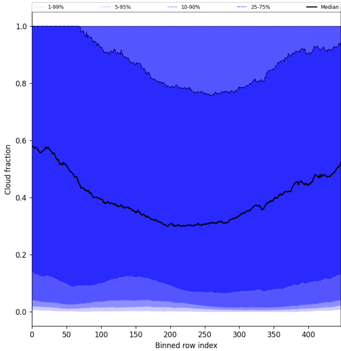
Figure 47: Along track statistics of “Cloud fraction” for 2025-03-29 to 2025-03-30
