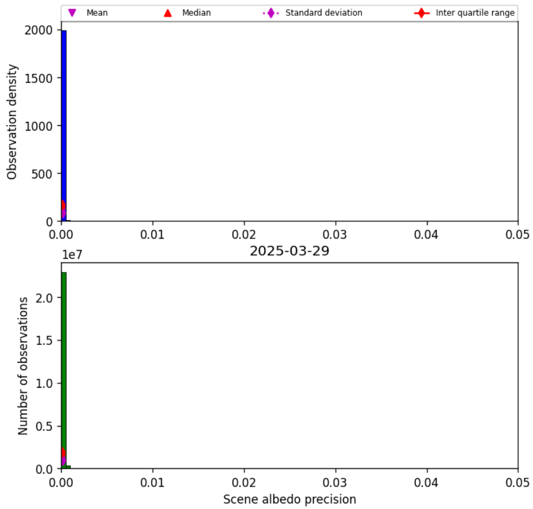
Figure 33: Histogram of “Scene albedo precision” for 2025-03-29 to 2025-03-30
