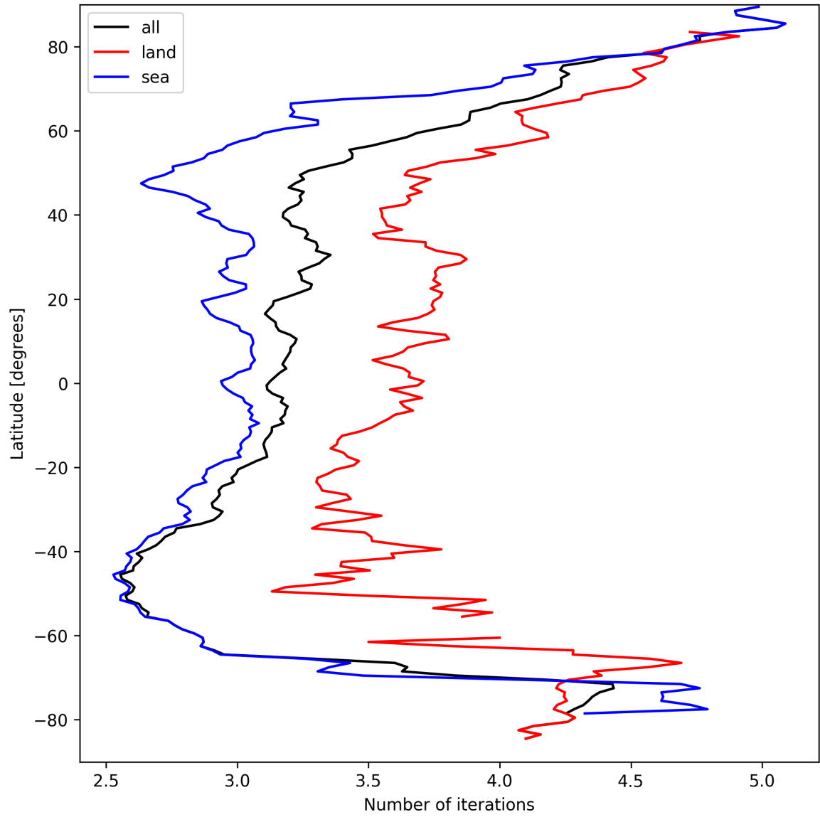
Figure 20: Zonal average of “Number of iterations” for 2025-03-29 to 2025-03-30.
