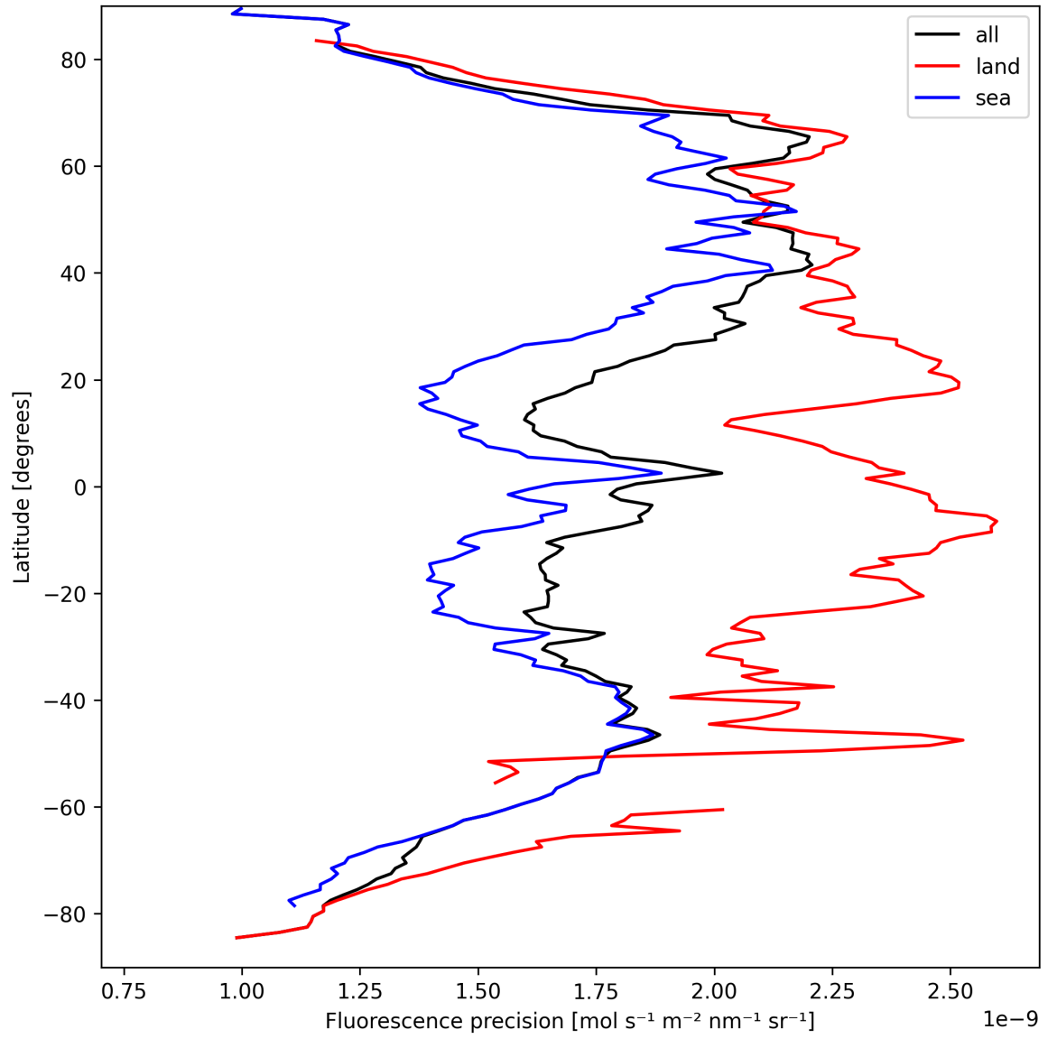
Figure 22: Zonal average of “Fluorescence precision” for 2025-03-29 to 2025-03-30.
