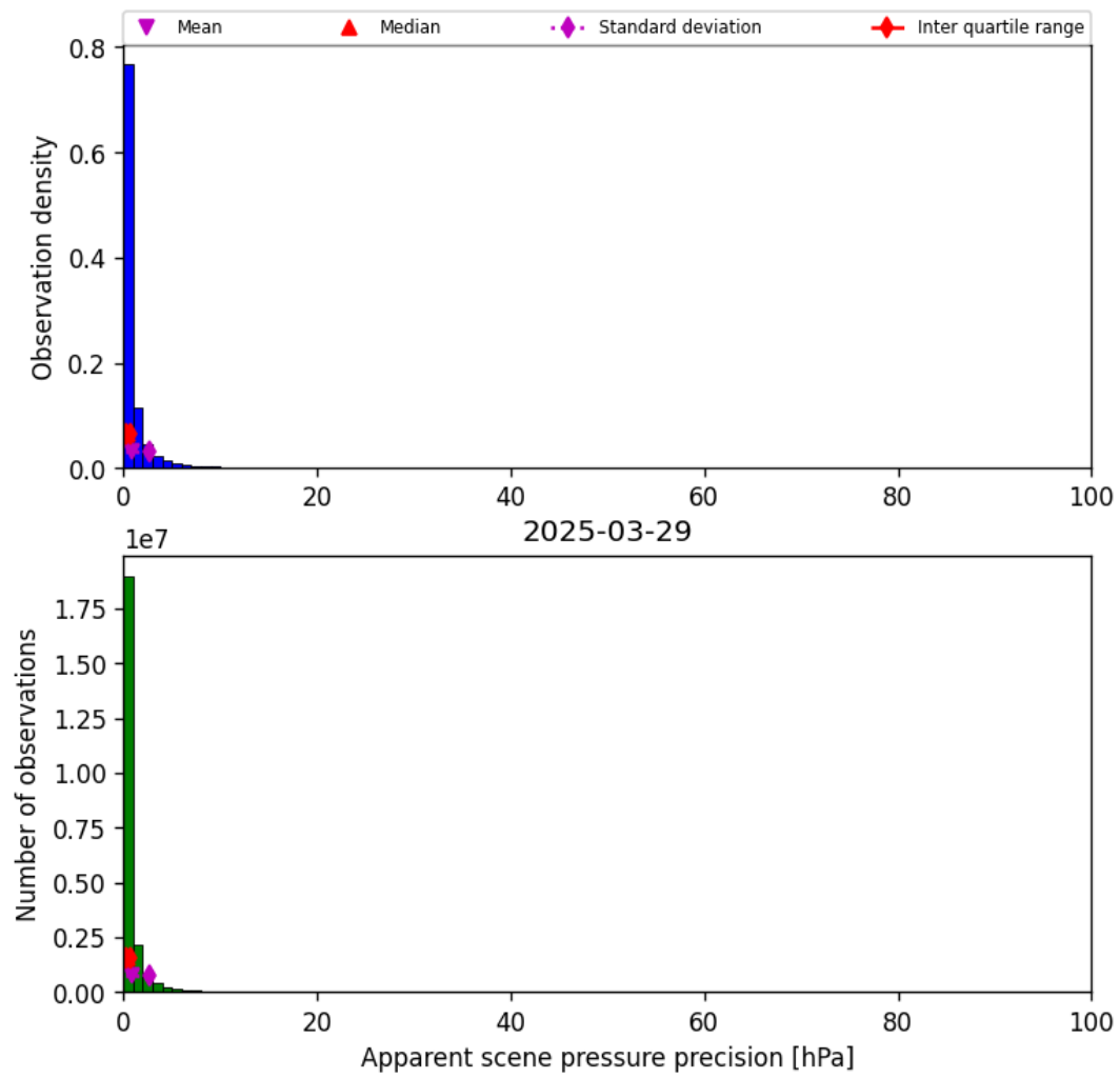
Figure 35: Histogram of “Apparent scene pressure precision” for 2025-03-29 to 2025-03-30
