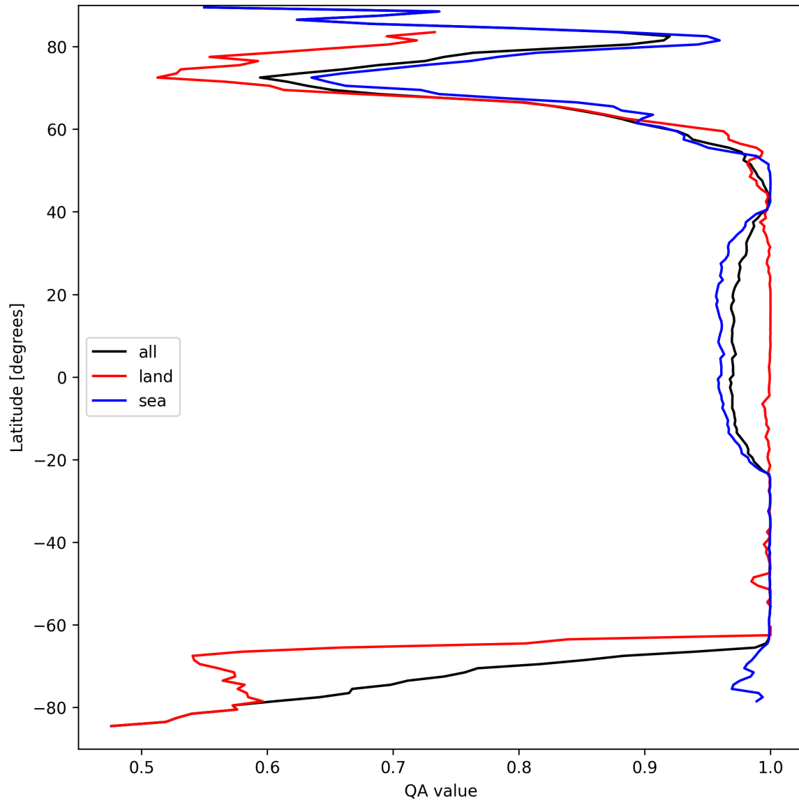
Figure 10: Zonal average of “QA value” for 2025-03-29 to 2025-03-30.
