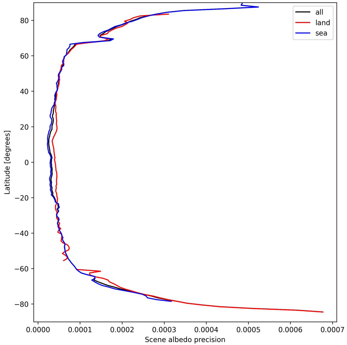
Figure 16: Zonal average of “Scene albedo precision” for 2025-03-29 to 2025-03-30.
