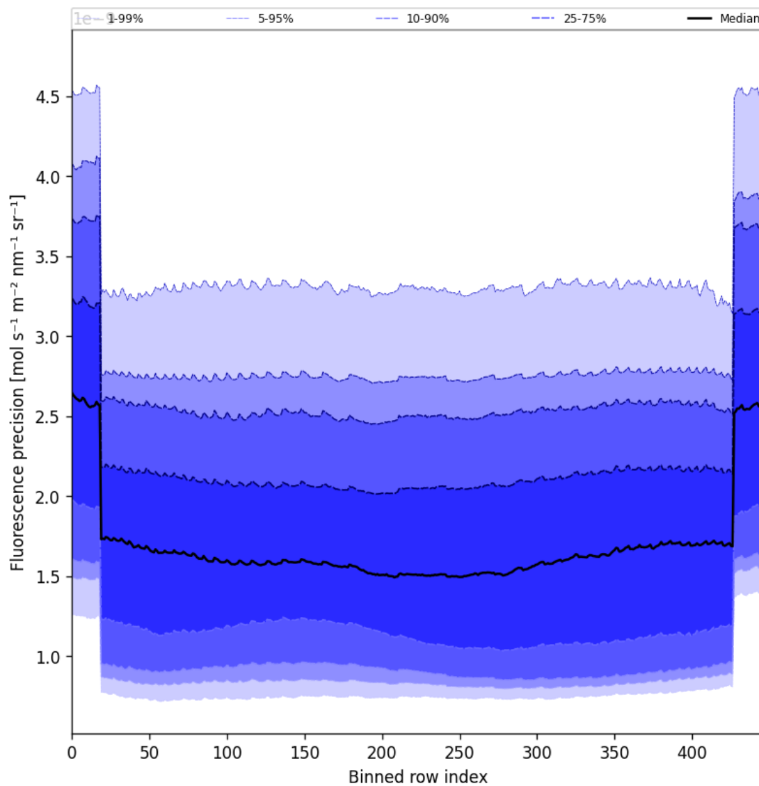
Figure 56: Along track statistics of “Fluorescence precision” for 2025-03-29 to 2025-03-30
