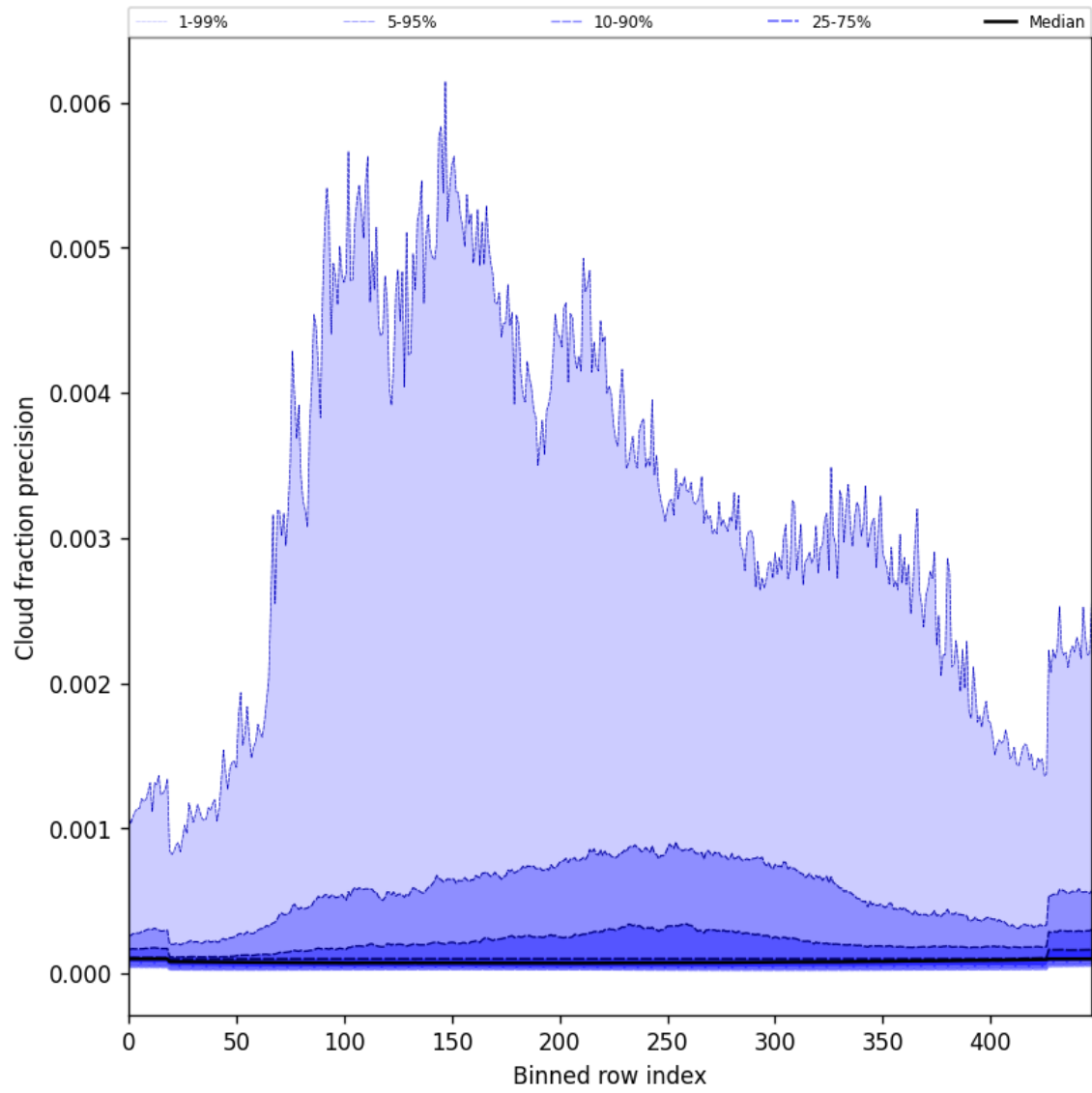
Figure 48: Along track statistics of “Cloud fraction precision” for 2025-03-29 to 2025-03-30
