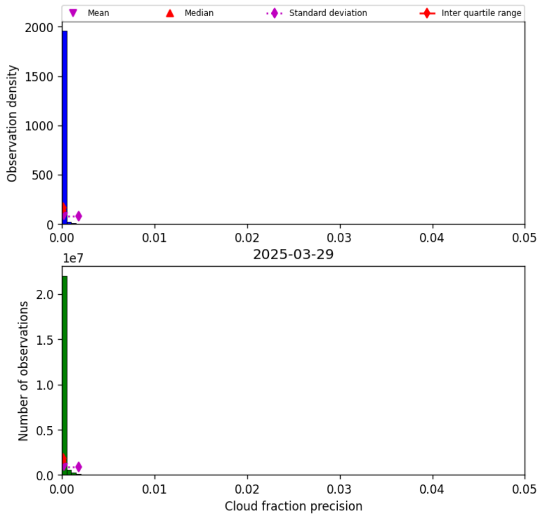
Figure 31: Histogram of “Cloud fraction precision” for 2025-03-29 to 2025-03-30
