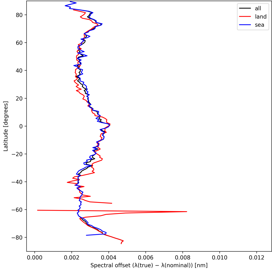
Figure 26: Zonal average of “Spectral offset ( \lambda_{\text{true}} - \lambda_{\text{nominal}} )” for 2025-03-29 to 2025-03-30.
