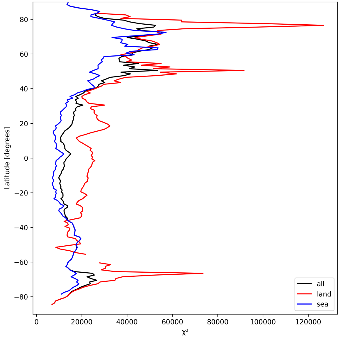
Figure 19: Zonal average of “ \chi^2 ” for 2025-03-29 to 2025-03-30.
