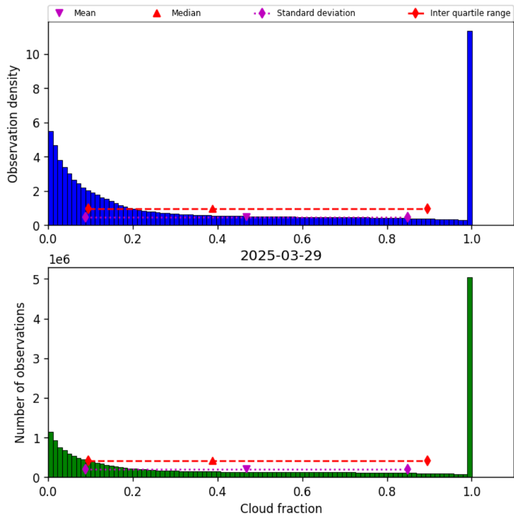
Figure 30: Histogram of “Cloud fraction” for 2025-03-29 to 2025-03-30
