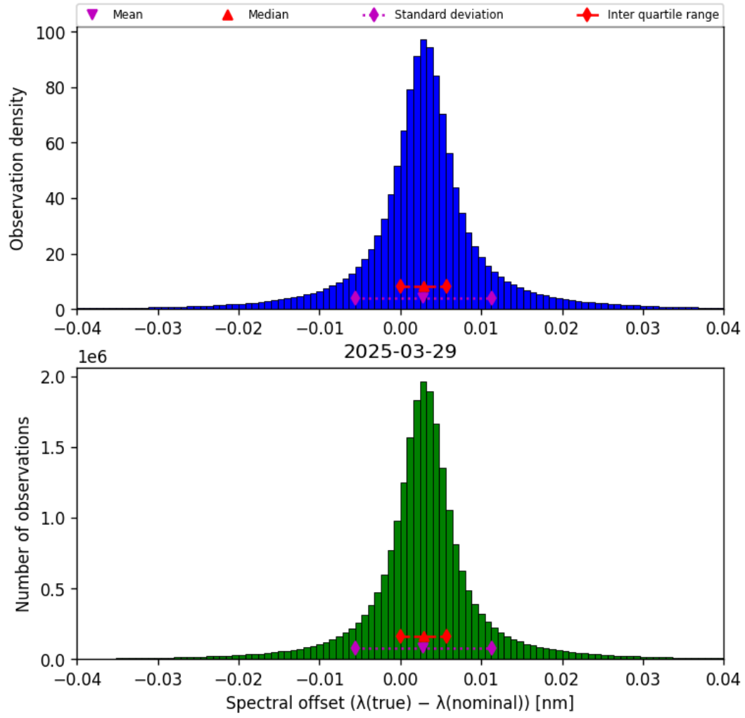
Figure 43: Histogram of “Spectral offset ( \lambda_{\text{true}} - \lambda_{\text{nominal}} )” for 2025-03-29 to 2025-03-30
