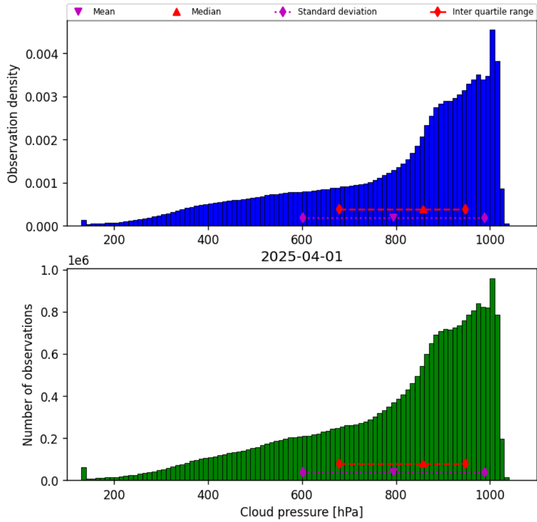
Figure 28: Histogram of “Cloud pressure” for 2025-04-01 to 2025-04-02
