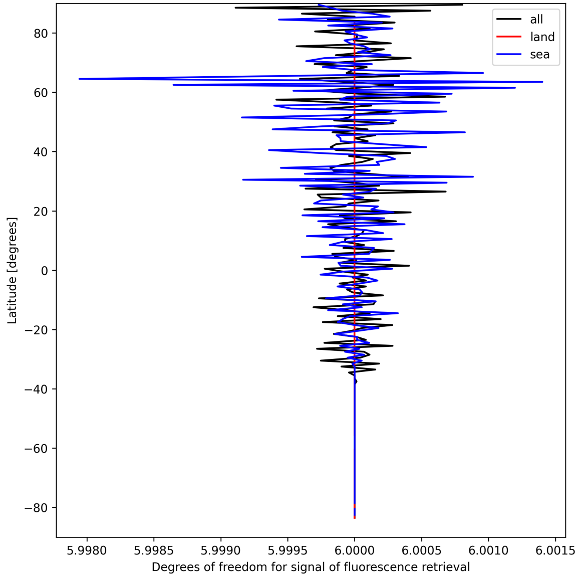
Figure 24: Zonal average of “Degrees of freedom for signal of fluorescence retrieval” for 2025-04-01 to 2025-04-02.
