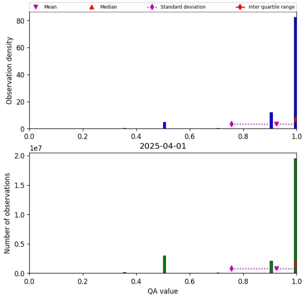
Figure 27: Histogram of “QA value” for 2025-04-01 to 2025-04-02
