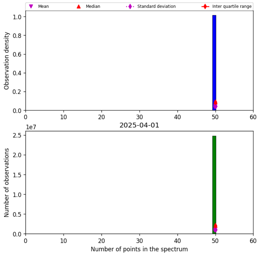
Figure 42: Histogram of “Number of points in the spectrum” for 2025-04-01 to 2025-04-02
