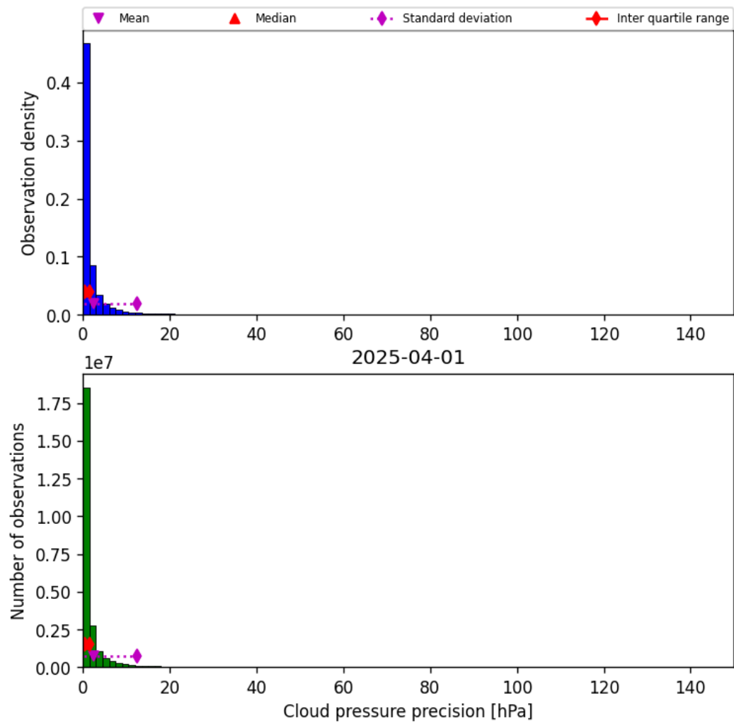
Figure 29: Histogram of “Cloud pressure precision” for 2025-04-01 to 2025-04-02
