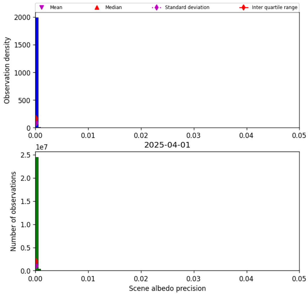
Figure 33: Histogram of “Scene albedo precision” for 2025-04-01 to 2025-04-02
