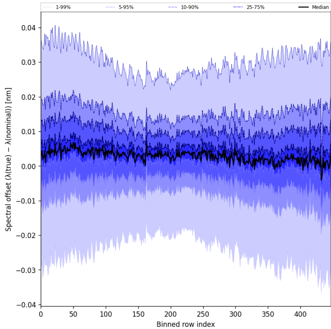
Figure 60: Along track statistics of “Spectral offset ( \lambda_{\text{true}} - \lambda_{\text{nominal}} )” for 2025-04-01 to 2025-04-02
