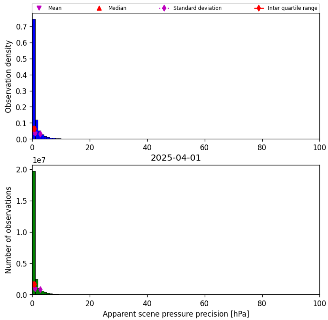
Figure 35: Histogram of “Apparent scene pressure precision” for 2025-04-01 to 2025-04-02
