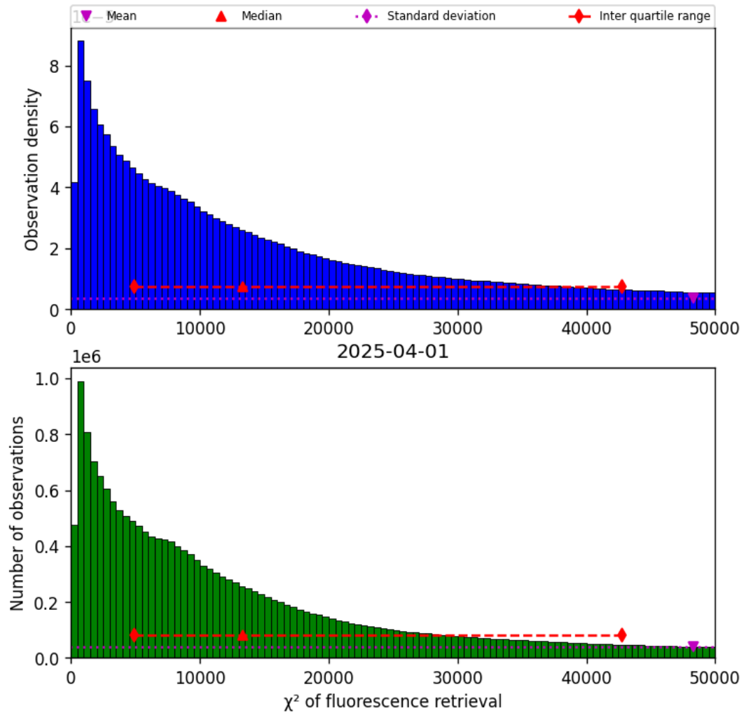
Figure 40: Histogram of “ \chi^2 of fluorescence retrieval” for 2025-04-01 to 2025-04-02
