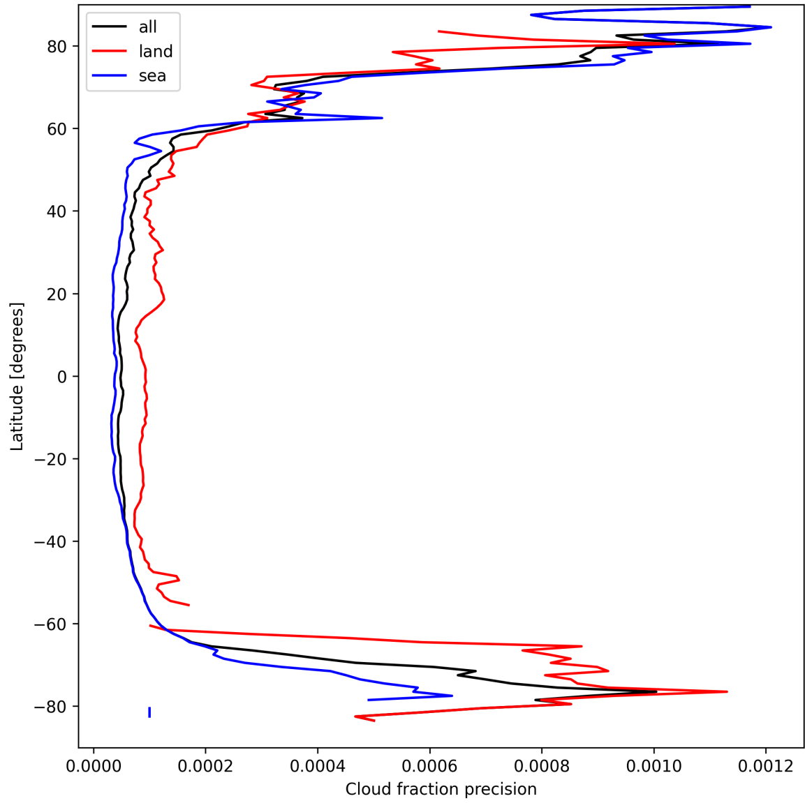
Figure 14: Zonal average of “Cloud fraction precision” for 2025-04-01 to 2025-04-02.
