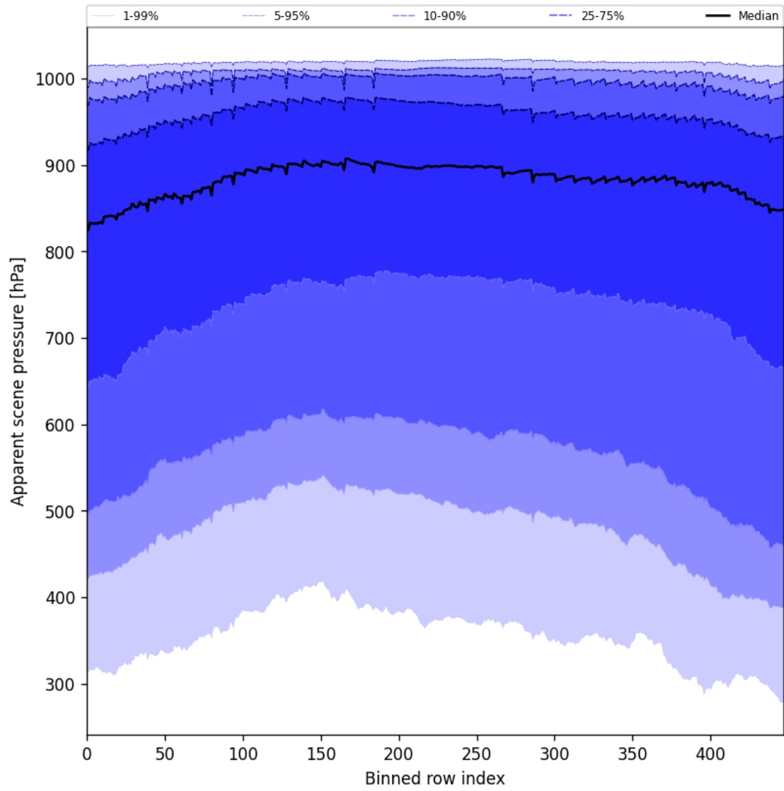
Figure 51: Along track statistics of “Apparent scene pressure” for 2025-04-01 to 2025-04-02
