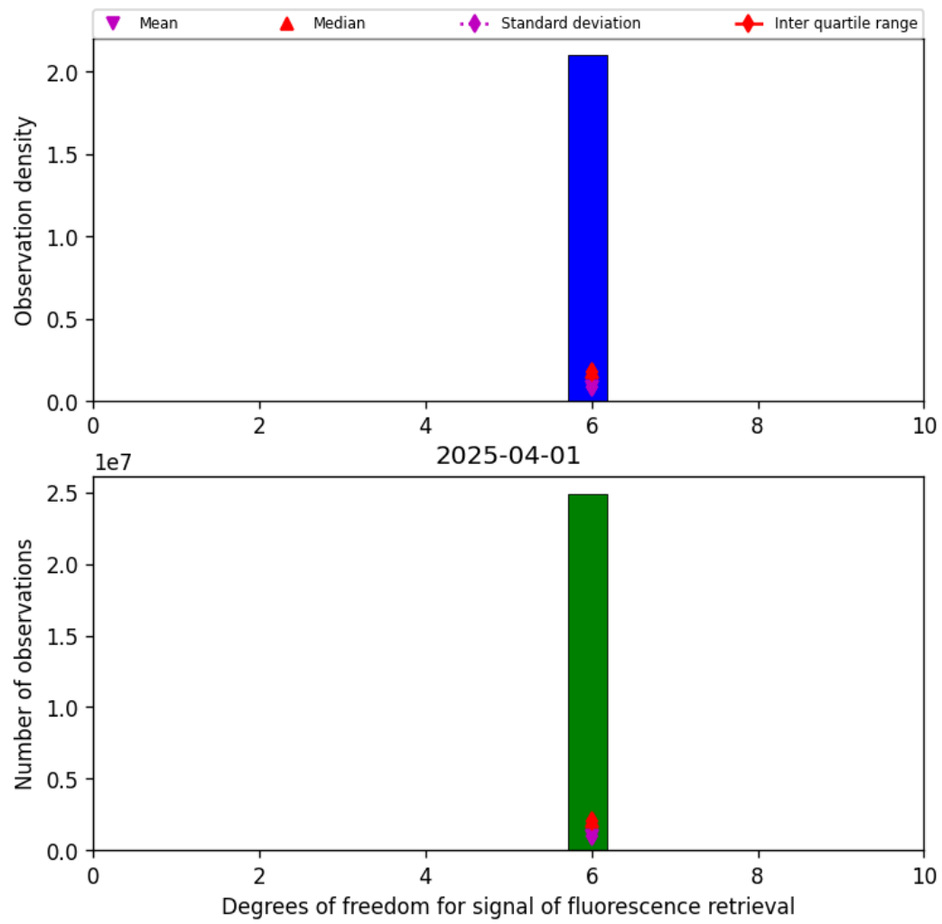
Figure 41: Histogram of “Degrees of freedom for signal of fluorescence retrieval” for 2025-04-01 to 2025-04-02
