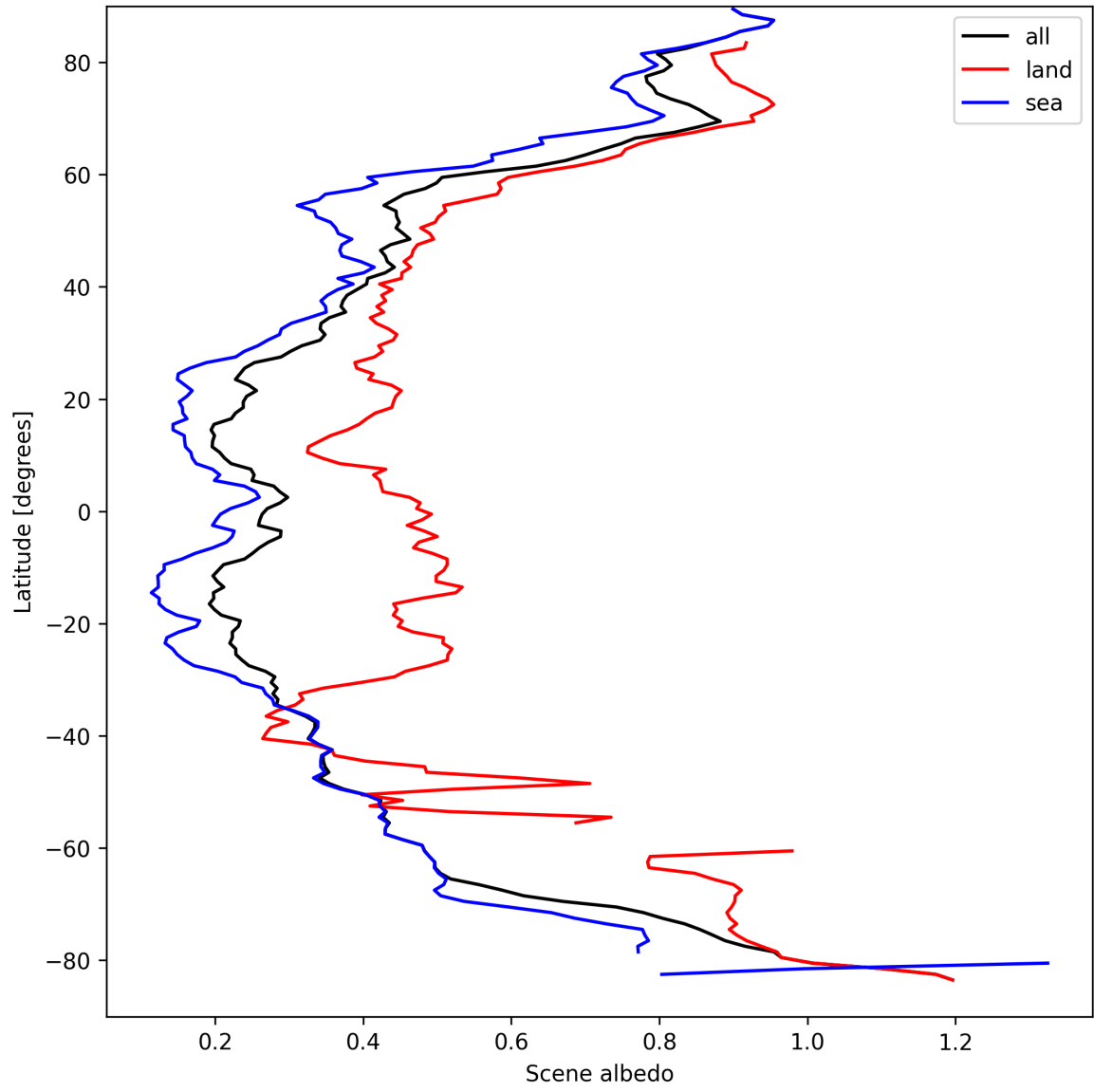
Figure 15: Zonal average of “Scene albedo” for 2025-04-01 to 2025-04-02.
