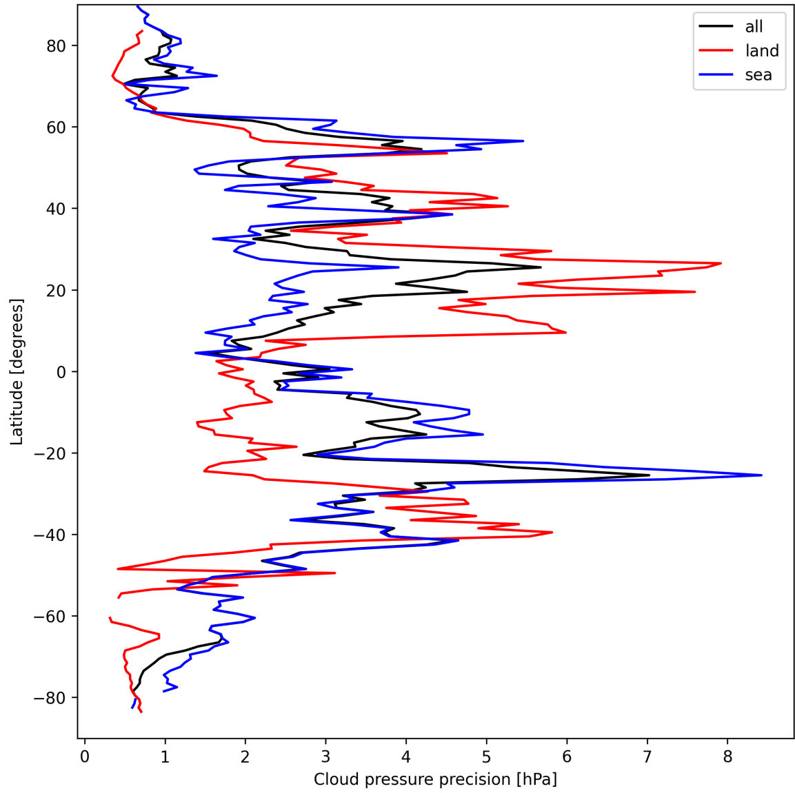
Figure 12: Zonal average of “Cloud pressure precision” for 2025-04-01 to 2025-04-02.
