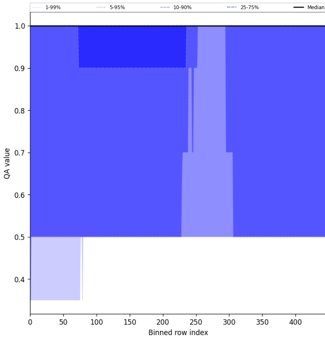
Figure 44: Along track statistics of “QA value” for 2025-04-01 to 2025-04-02
