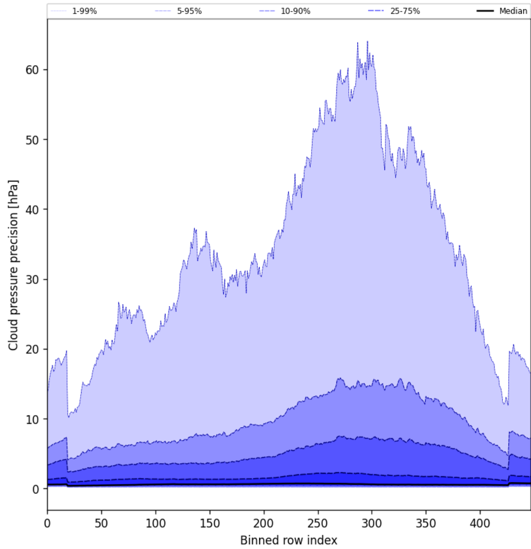
Figure 46: Along track statistics of “Cloud pressure precision” for 2025-04-01 to 2025-04-02
