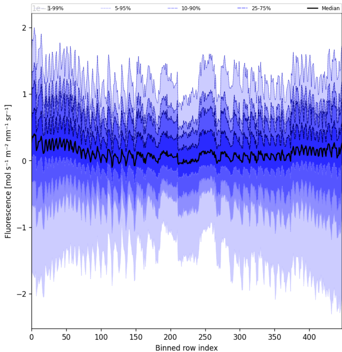
Figure 55: Along track statistics of “Fluorescence” for 2025-04-01 to 2025-04-02
