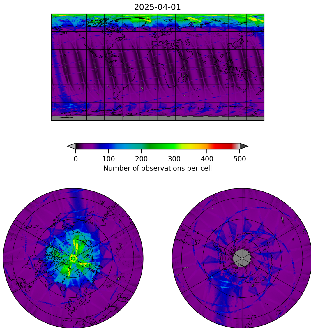
Figure 9: Map of the number of observations for 2025-04-01 to 2025-04-02
