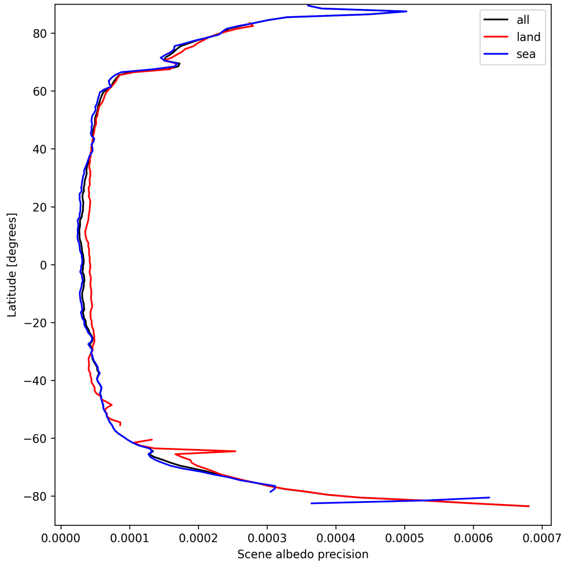
Figure 16: Zonal average of “Scene albedo precision” for 2025-04-01 to 2025-04-02.
