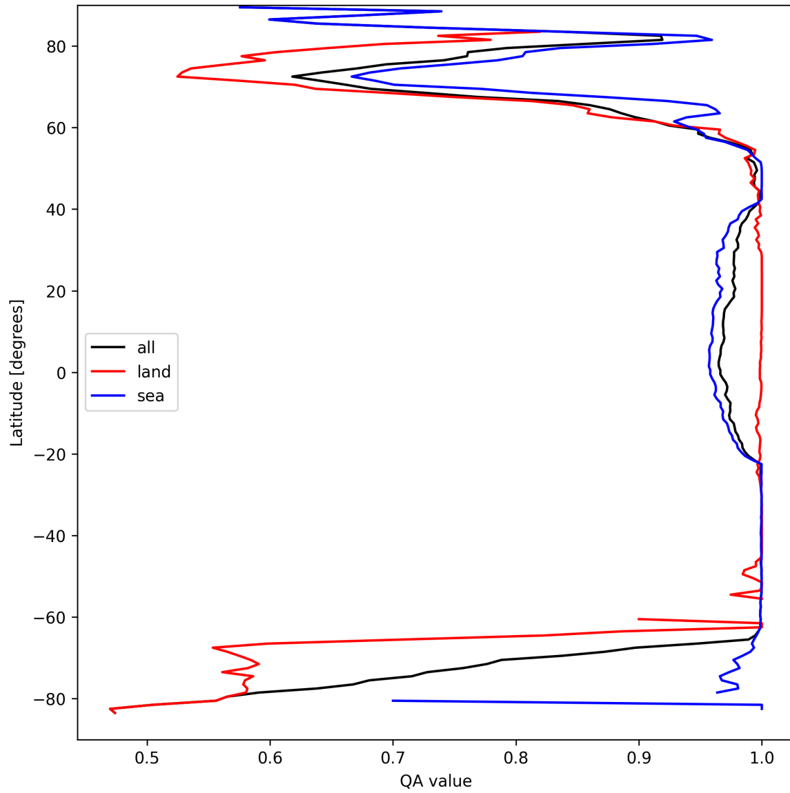
Figure 10: Zonal average of “QA value” for 2025-04-01 to 2025-04-02.
