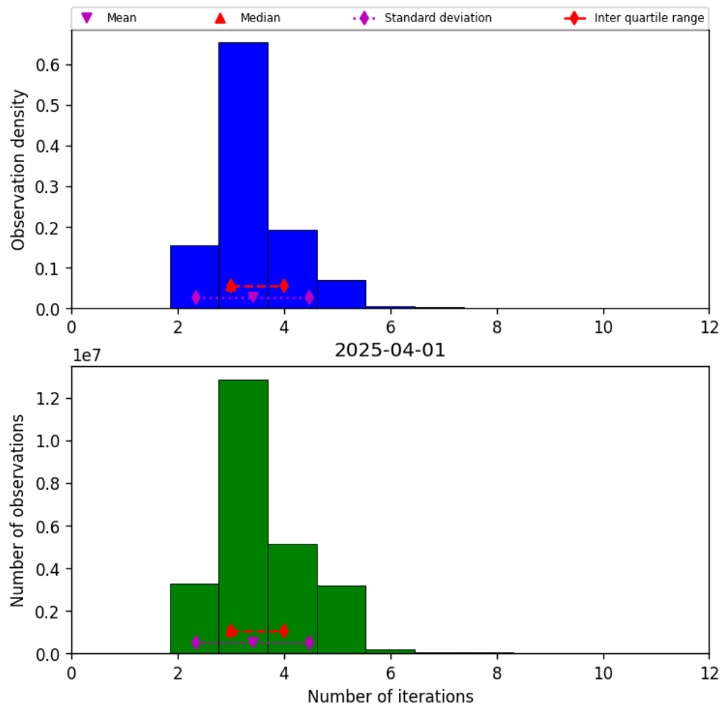
Figure 37: Histogram of “Number of iterations” for 2025-04-01 to 2025-04-02
