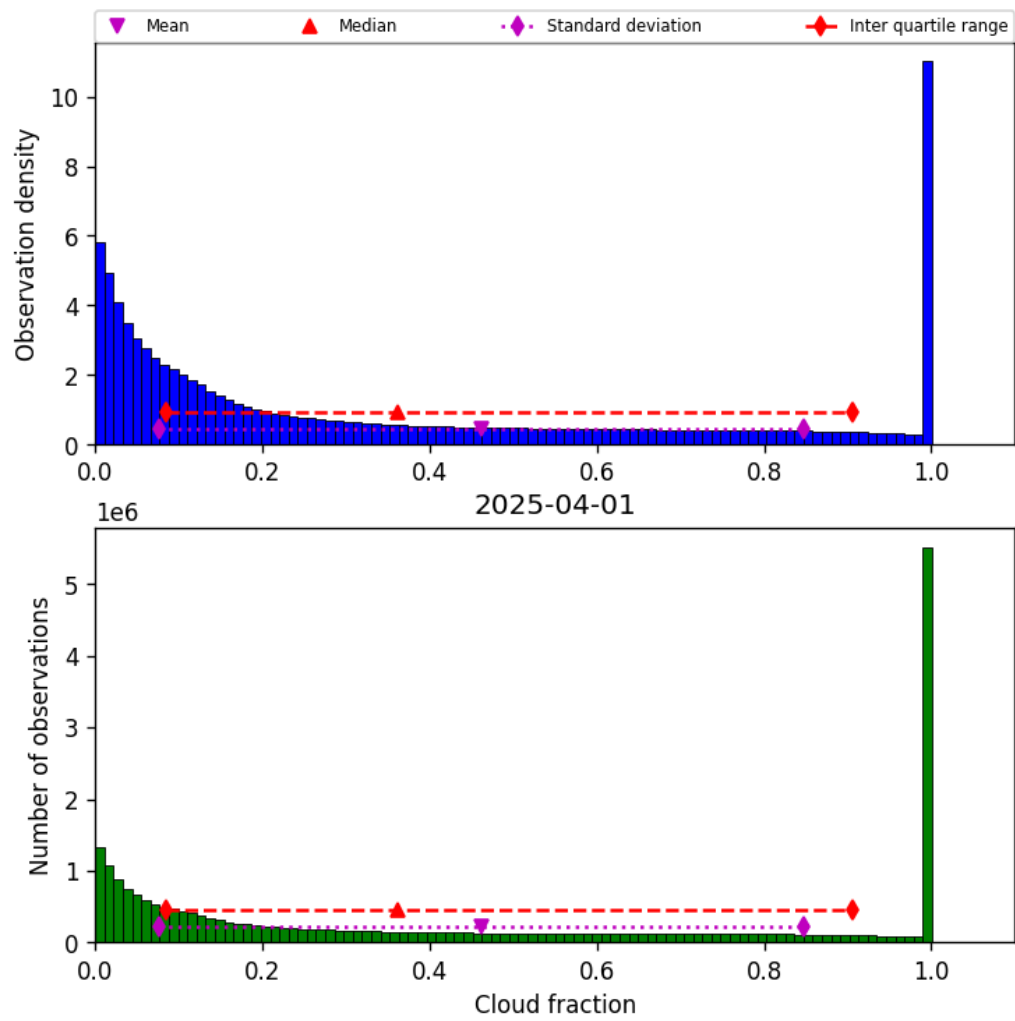
Figure 30: Histogram of “Cloud fraction” for 2025-04-01 to 2025-04-02
