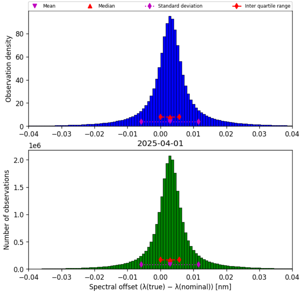
Figure 43: Histogram of “Spectral offset ( \lambda_{\text{true}} - \lambda_{\text{nominal}} )” for 2025-04-01 to 2025-04-02
