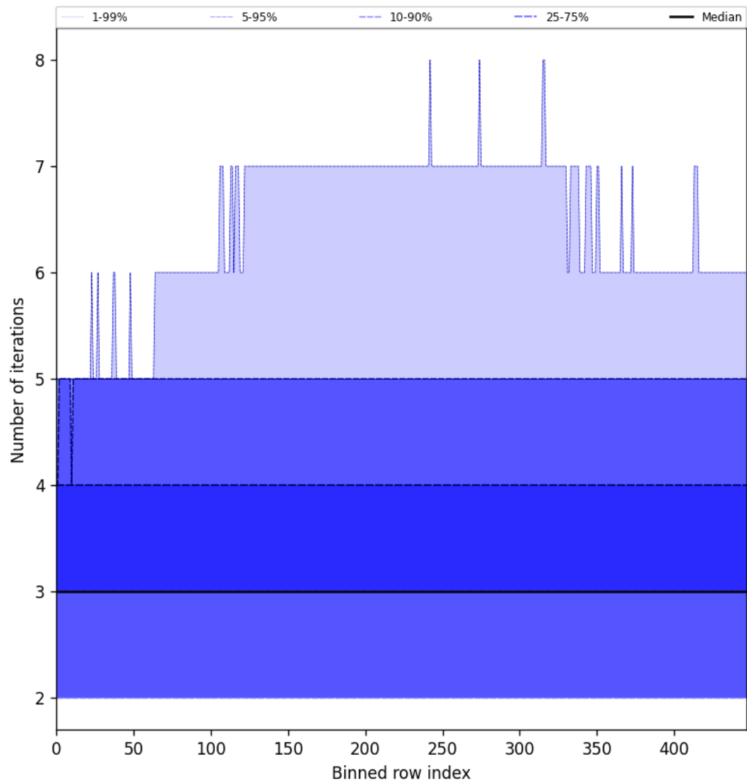
Figure 54: Along track statistics of “Number of iterations” for 2025-04-01 to 2025-04-02
