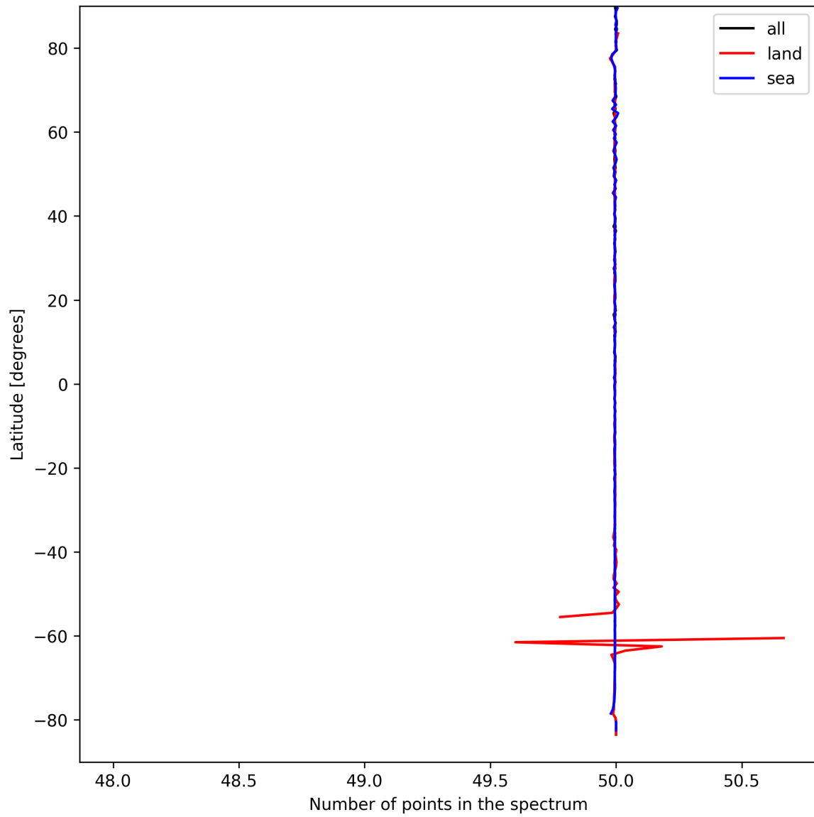
Figure 25: Zonal average of “Number of points in the spectrum” for 2025-04-01 to 2025-04-02.
