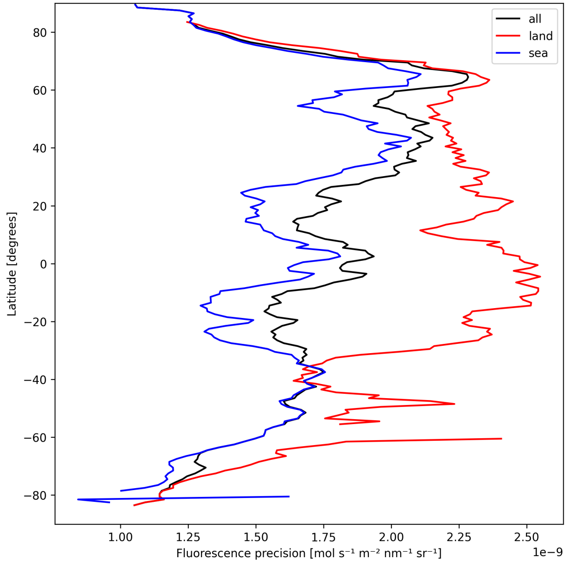
Figure 22: Zonal average of “Fluorescence precision” for 2025-04-01 to 2025-04-02.
