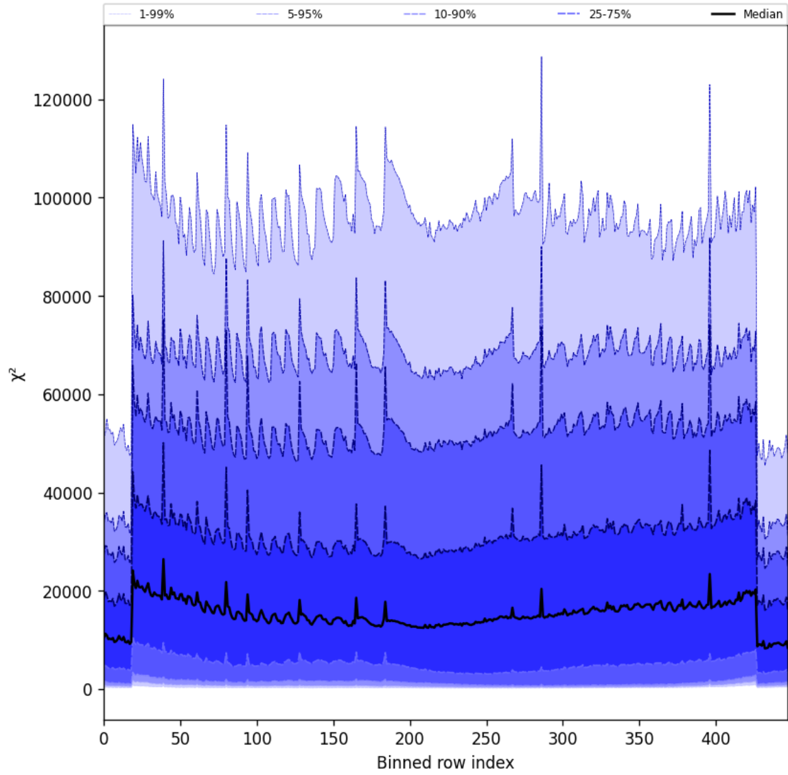
Figure 53: Along track statistics of “ \chi^2 ” for 2025-04-01 to 2025-04-02
