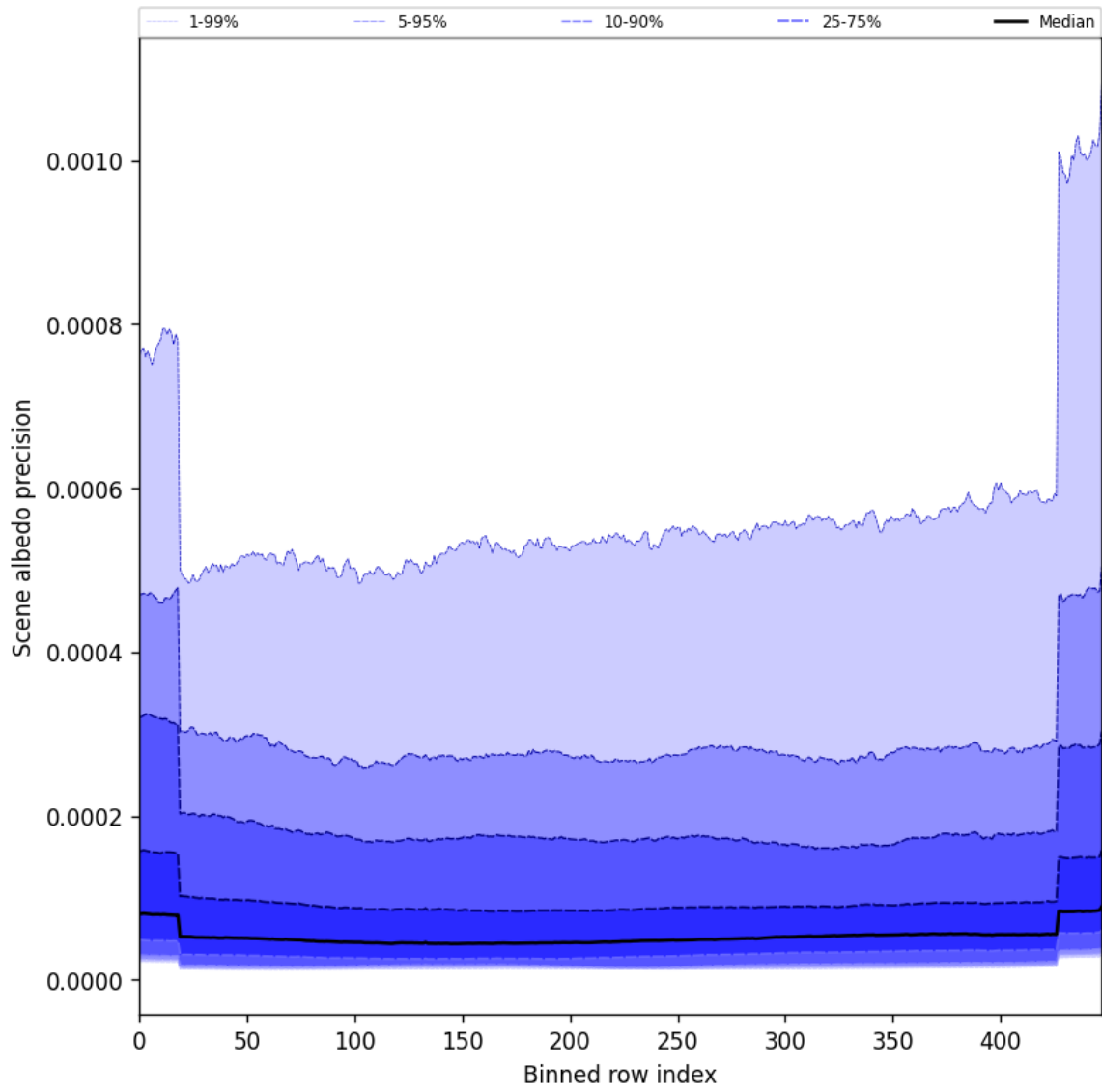
Figure 50: Along track statistics of “Scene albedo precision” for 2025-04-01 to 2025-04-02
