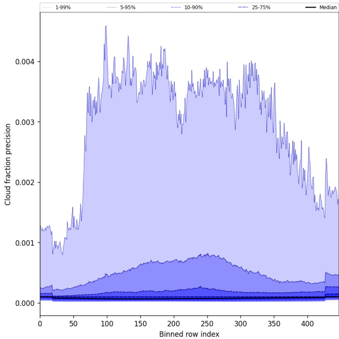
Figure 48: Along track statistics of “Cloud fraction precision” for 2025-04-01 to 2025-04-02
