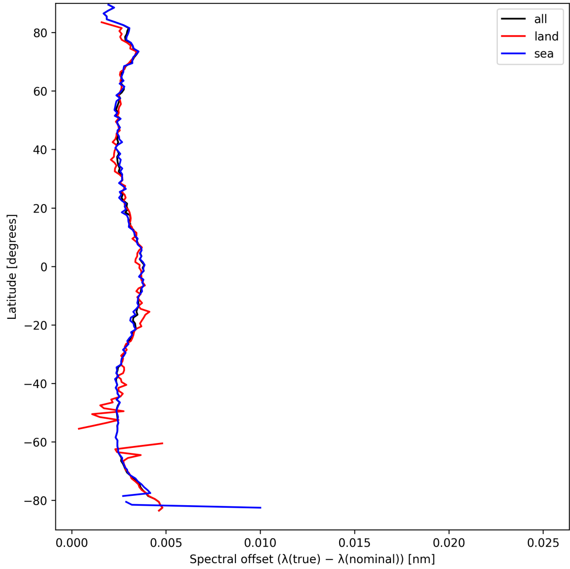
Figure 26: Zonal average of “Spectral offset ( \lambda_{\text{true}} - \lambda_{\text{nominal}} )” for 2025-04-01 to 2025-04-02.
