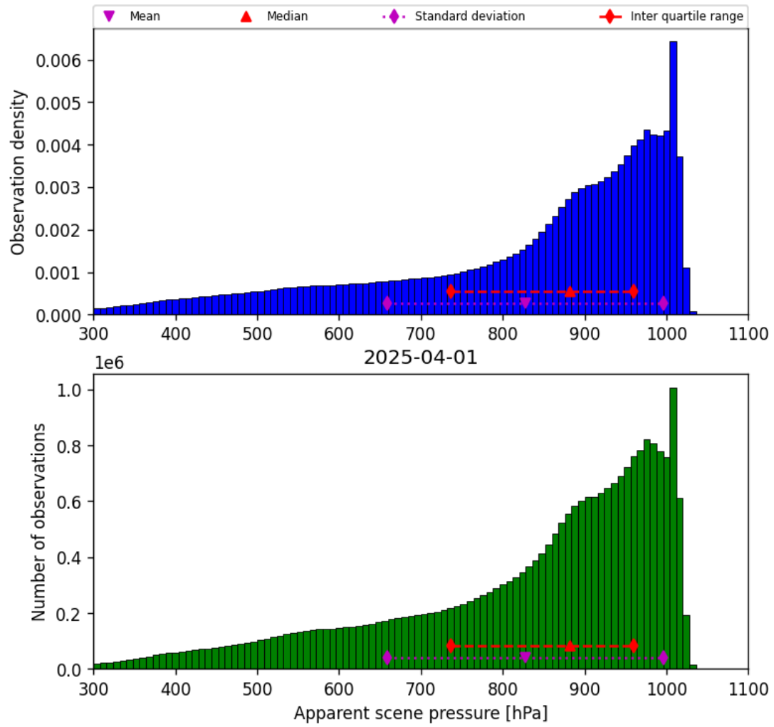
Figure 34: Histogram of “Apparent scene pressure” for 2025-04-01 to 2025-04-02
