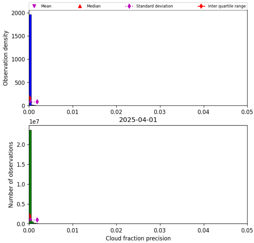
Figure 31: Histogram of “Cloud fraction precision” for 2025-04-01 to 2025-04-02
