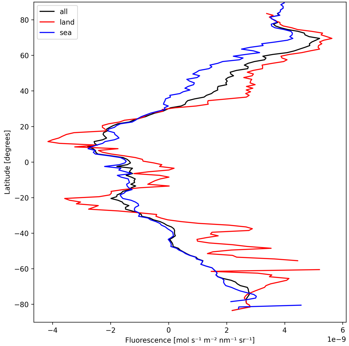
Figure 21: Zonal average of “Fluorescence” for 2025-04-01 to 2025-04-02.
