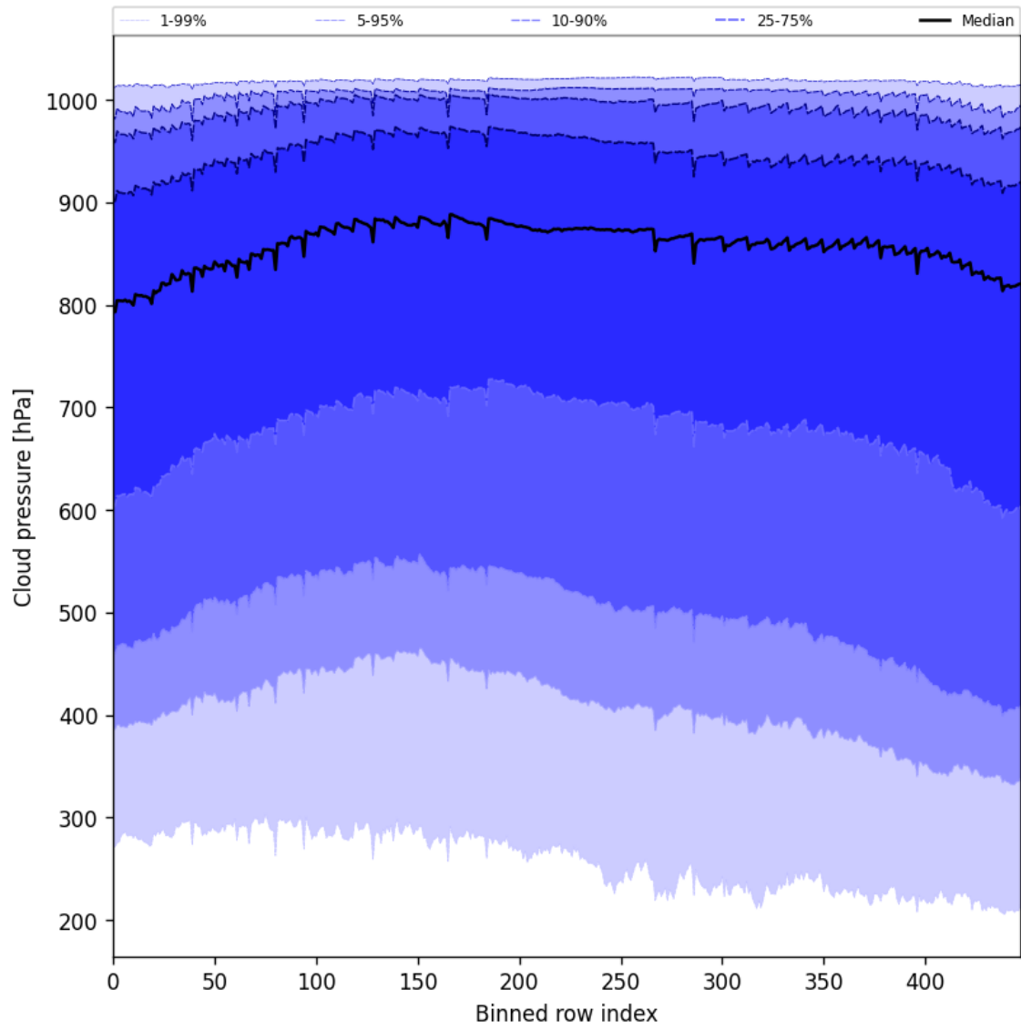
Figure 45: Along track statistics of “Cloud pressure” for 2025-04-01 to 2025-04-02
