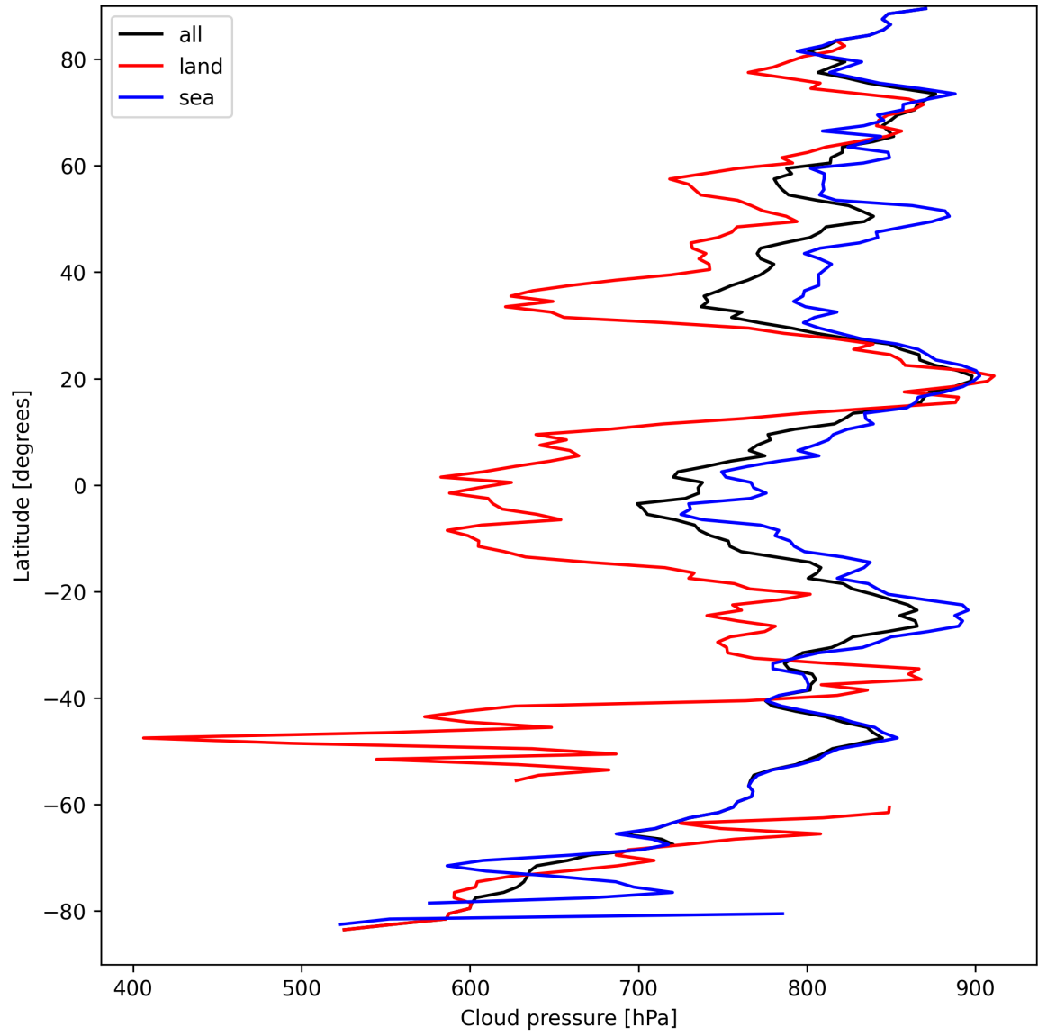
Figure 11: Zonal average of “Cloud pressure” for 2025-04-01 to 2025-04-02.
