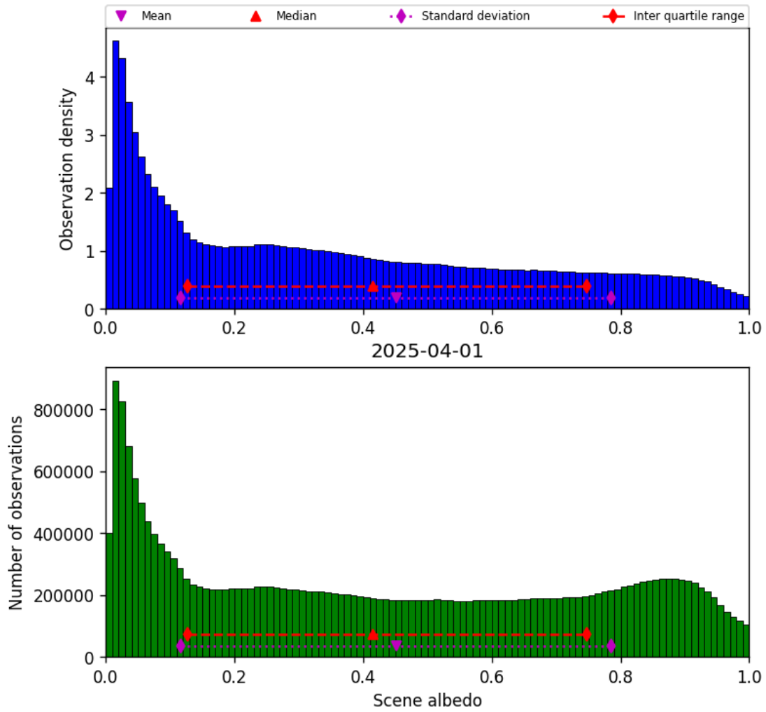
Figure 32: Histogram of “Scene albedo” for 2025-04-01 to 2025-04-02
