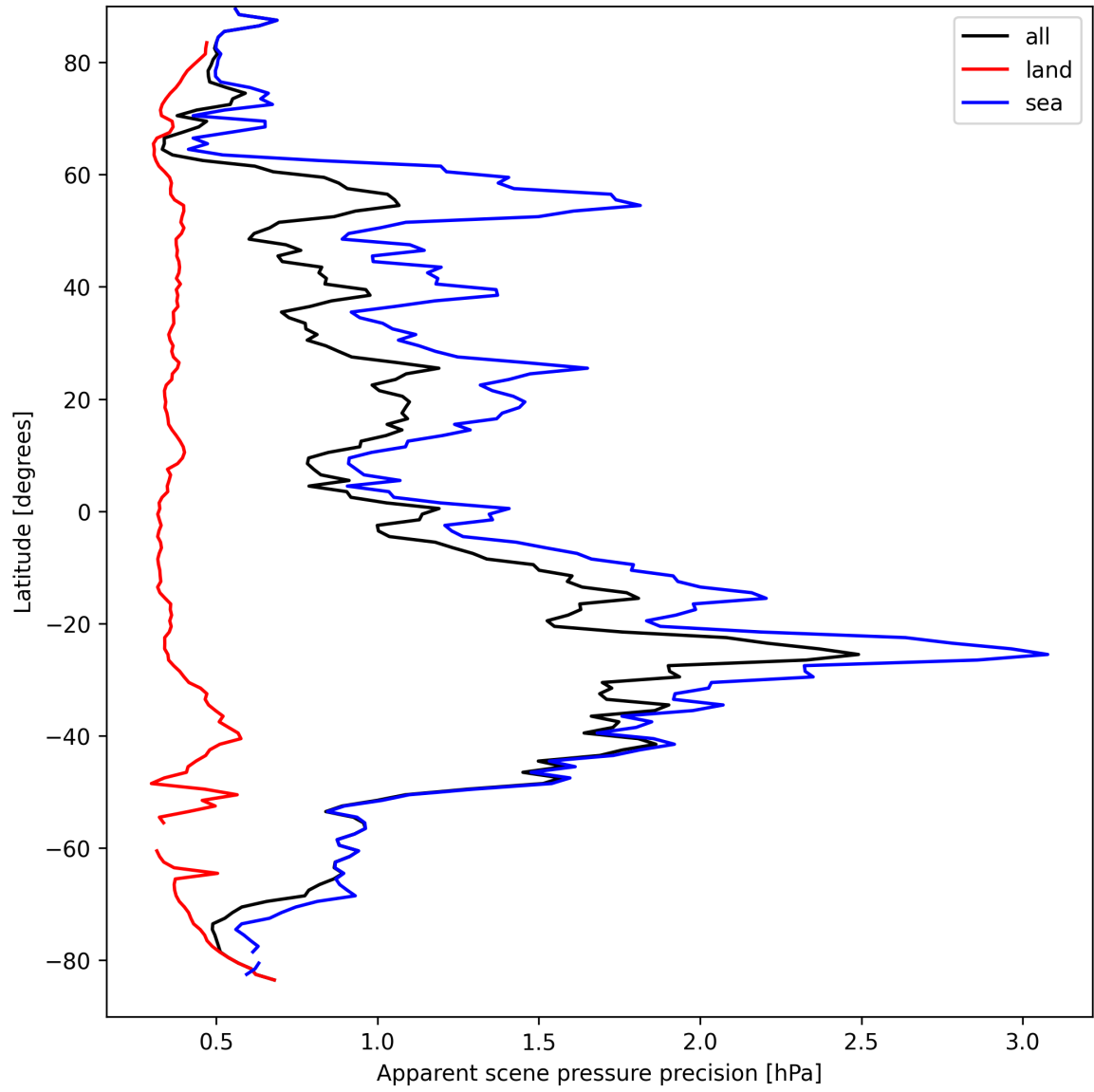
Figure 18: Zonal average of “Apparent scene pressure precision” for 2025-04-01 to 2025-04-02.
