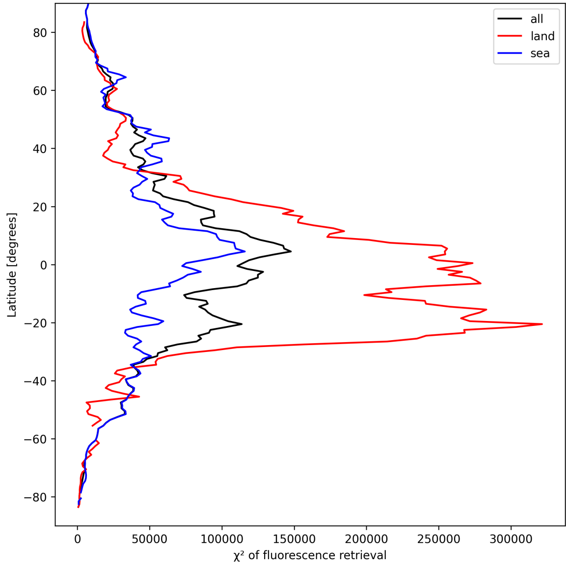
Figure 23: Zonal average of “ \chi^2 of fluorescence retrieval” for 2025-04-01 to 2025-04-02.
