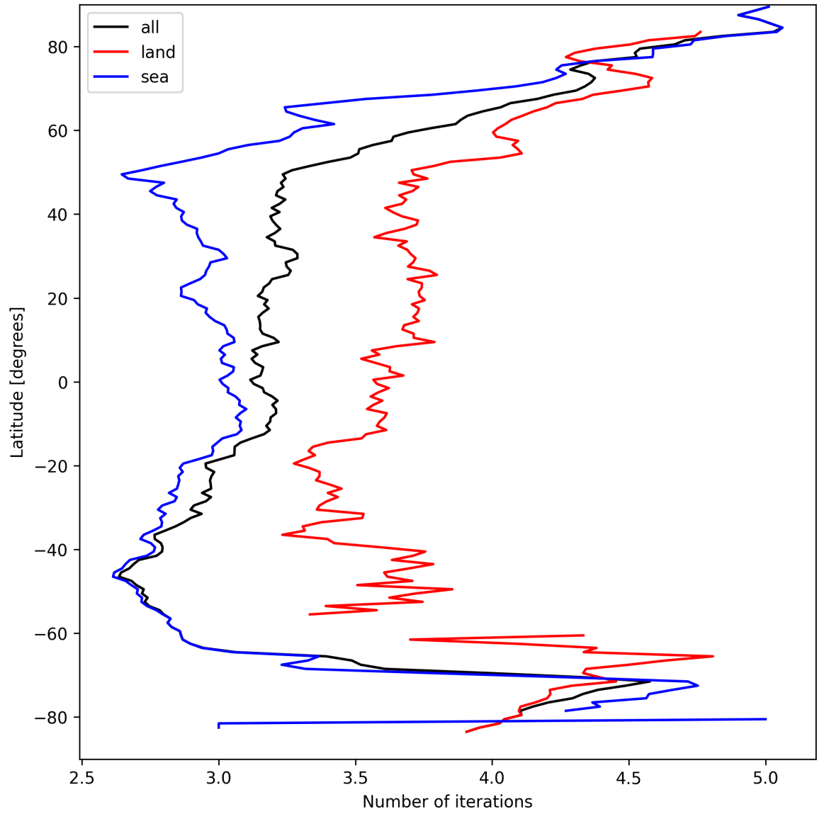
Figure 20: Zonal average of “Number of iterations” for 2025-04-01 to 2025-04-02.
