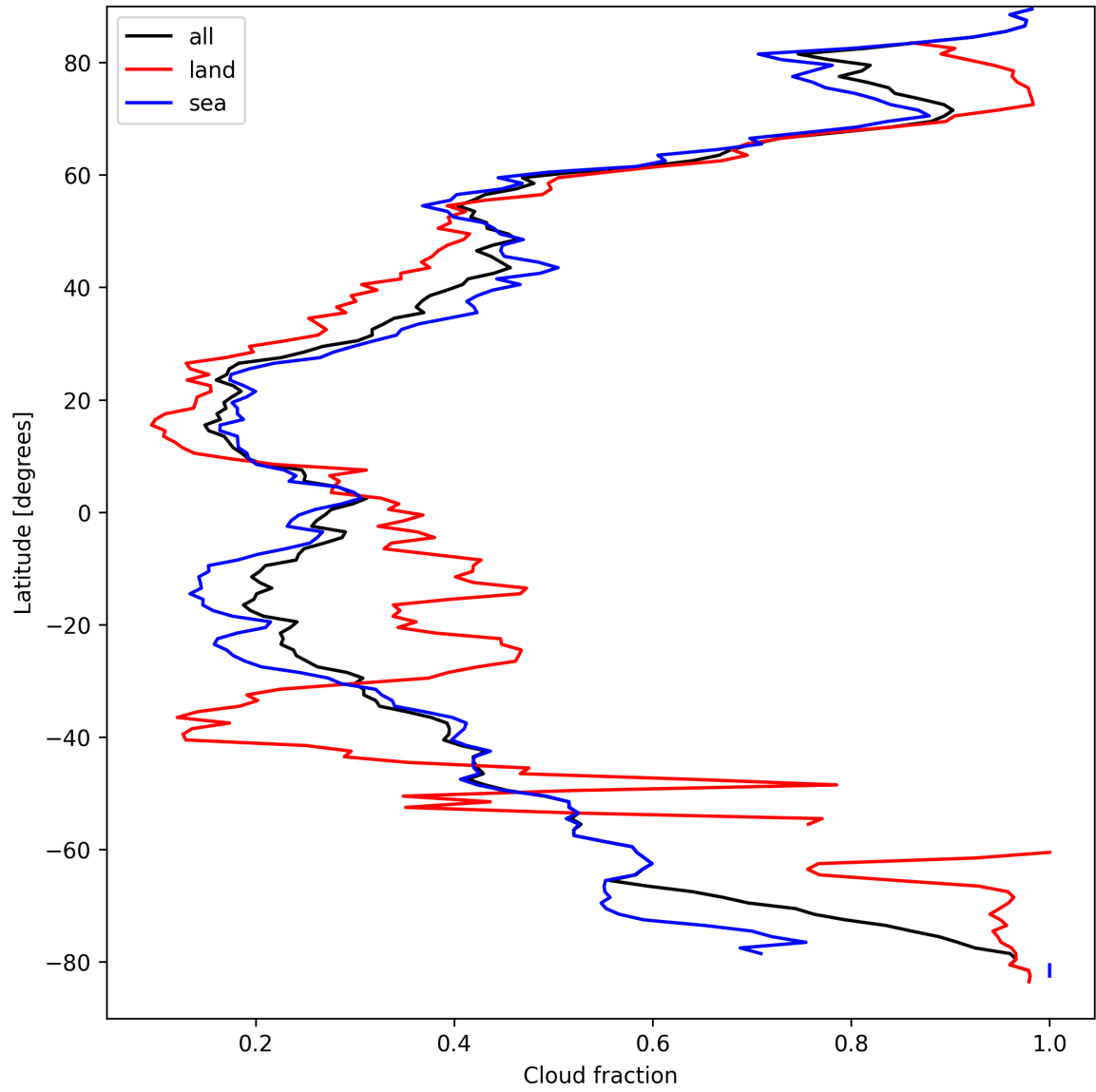
Figure 13: Zonal average of “Cloud fraction” for 2025-04-01 to 2025-04-02.
