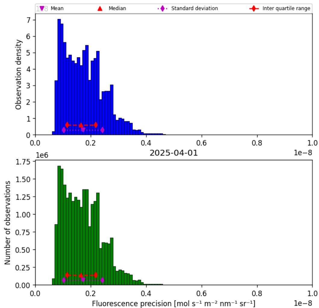
Figure 39: Histogram of “Fluorescence precision” for 2025-04-01 to 2025-04-02
