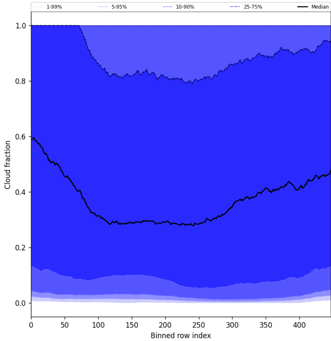
Figure 47: Along track statistics of “Cloud fraction” for 2025-04-01 to 2025-04-02
