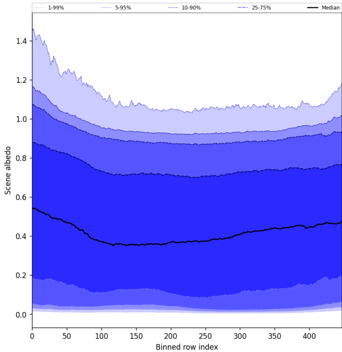
Figure 49: Along track statistics of “Scene albedo” for 2025-04-01 to 2025-04-02
