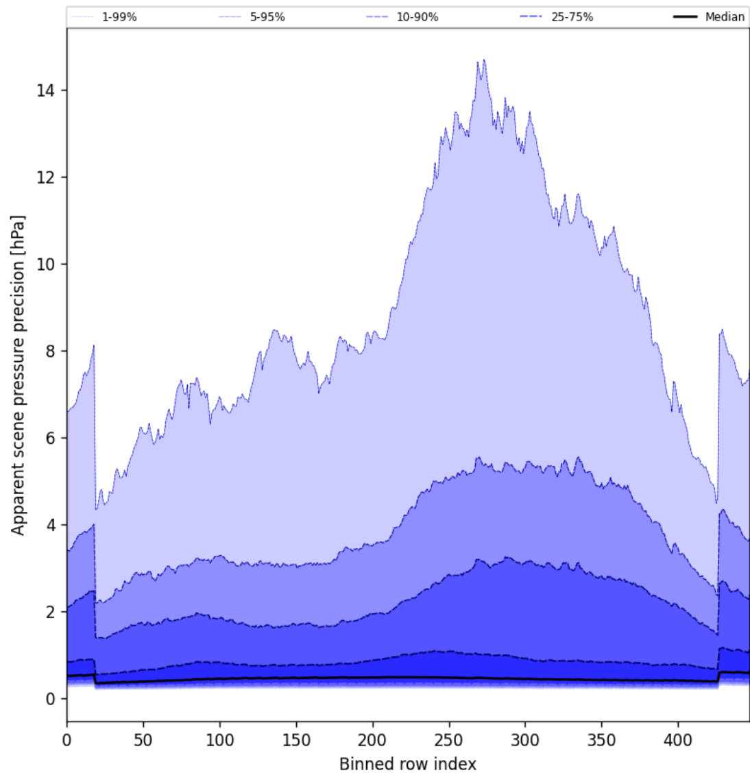
Figure 52: Along track statistics of “Apparent scene pressure precision” for 2025-04-01 to 2025-04-02
