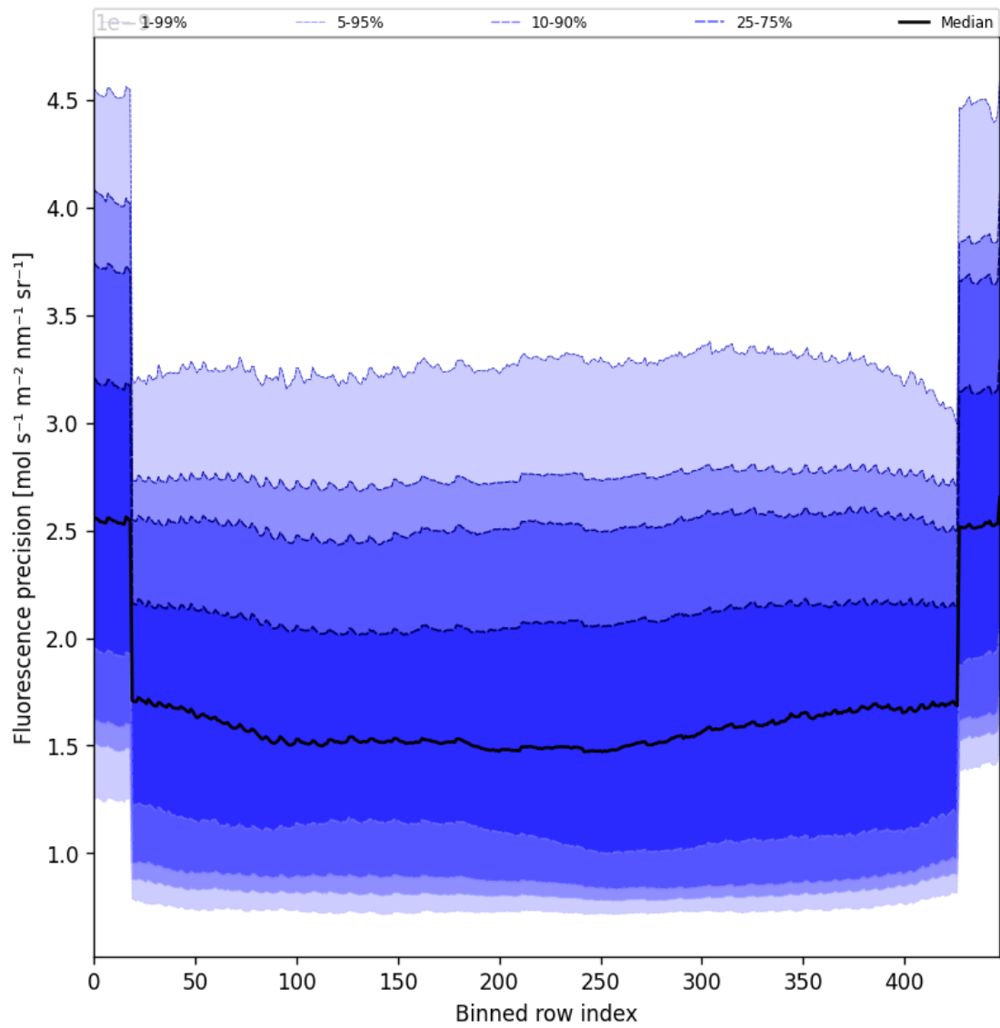
Figure 56: Along track statistics of “Fluorescence precision” for 2025-04-01 to 2025-04-02
