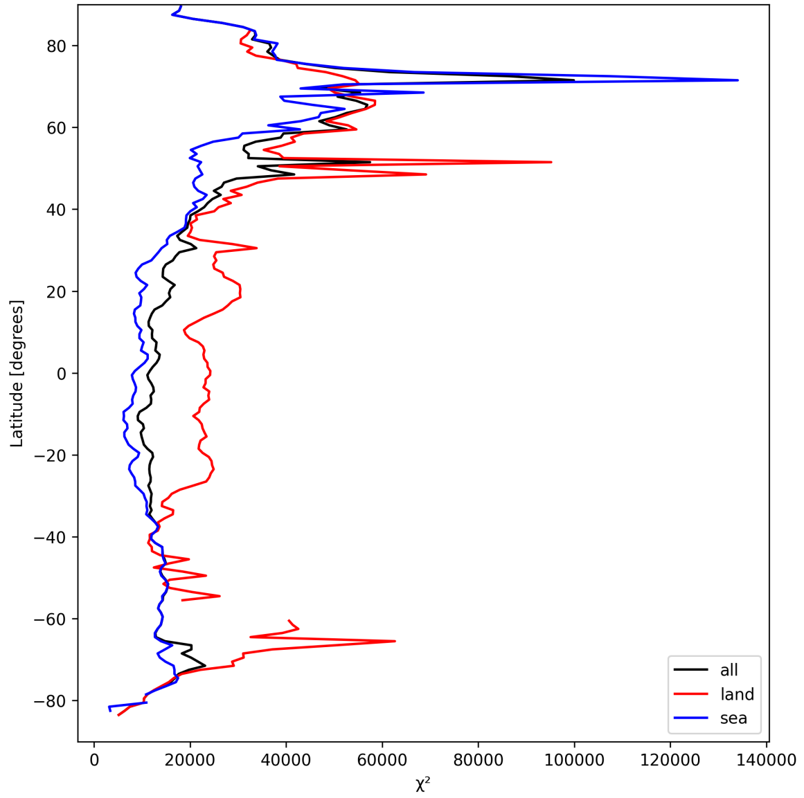
Figure 19: Zonal average of “ \chi^2 ” for 2025-04-01 to 2025-04-02.
