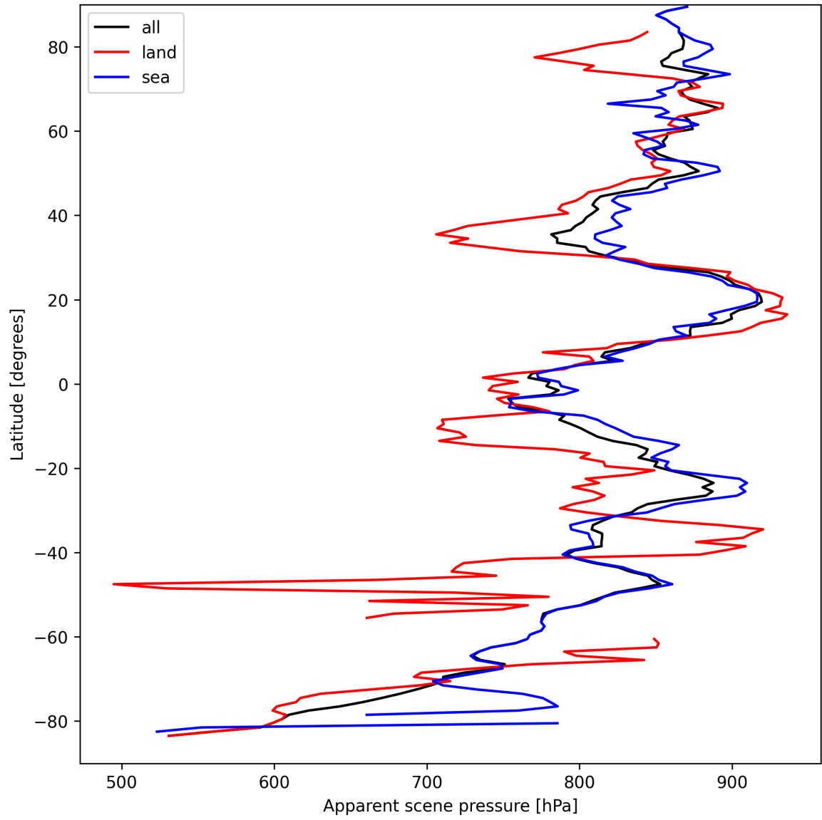
Figure 17: Zonal average of “Apparent scene pressure” for 2025-04-01 to 2025-04-02.
