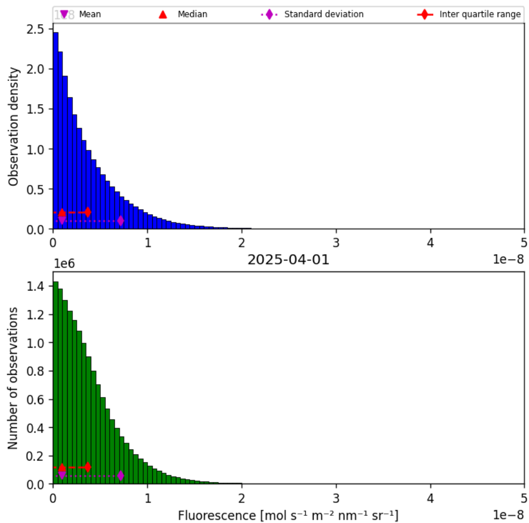
Figure 38: Histogram of “Fluorescence” for 2025-04-01 to 2025-04-02
