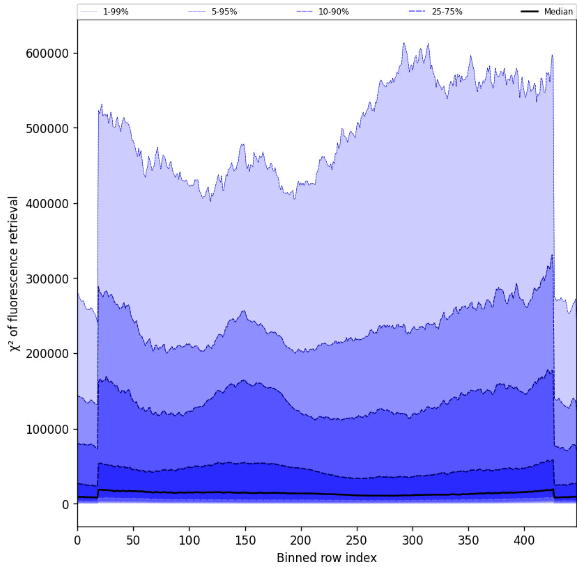
Figure 57: Along track statistics of “ \chi^2 of fluorescence retrieval” for 2025-04-01 to 2025-04-02
