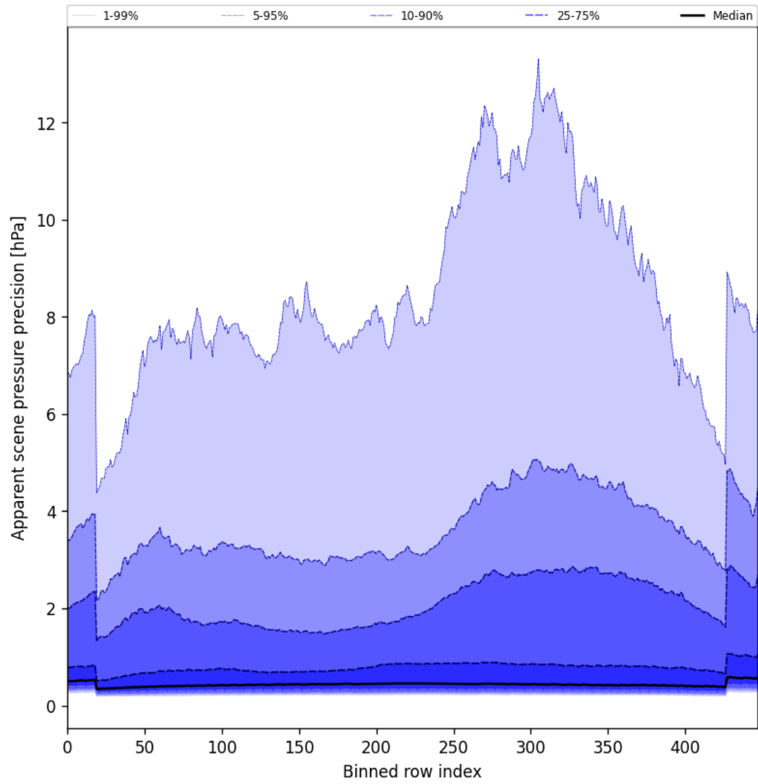
Figure 52: Along track statistics of “Apparent scene pressure precision” for 2025-04-02 to 2025-04-03
