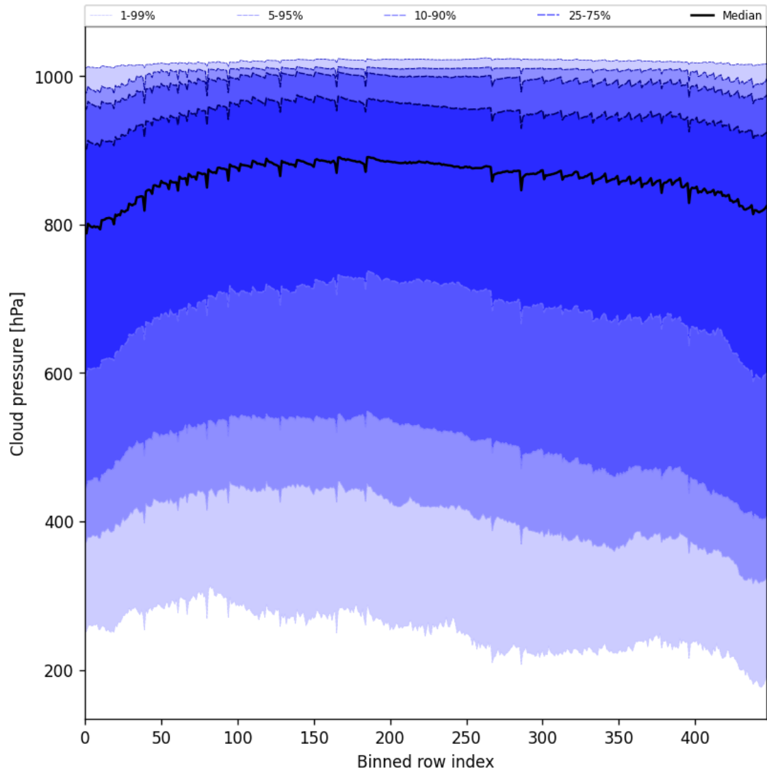
Figure 45: Along track statistics of “Cloud pressure” for 2025-04-02 to 2025-04-03
