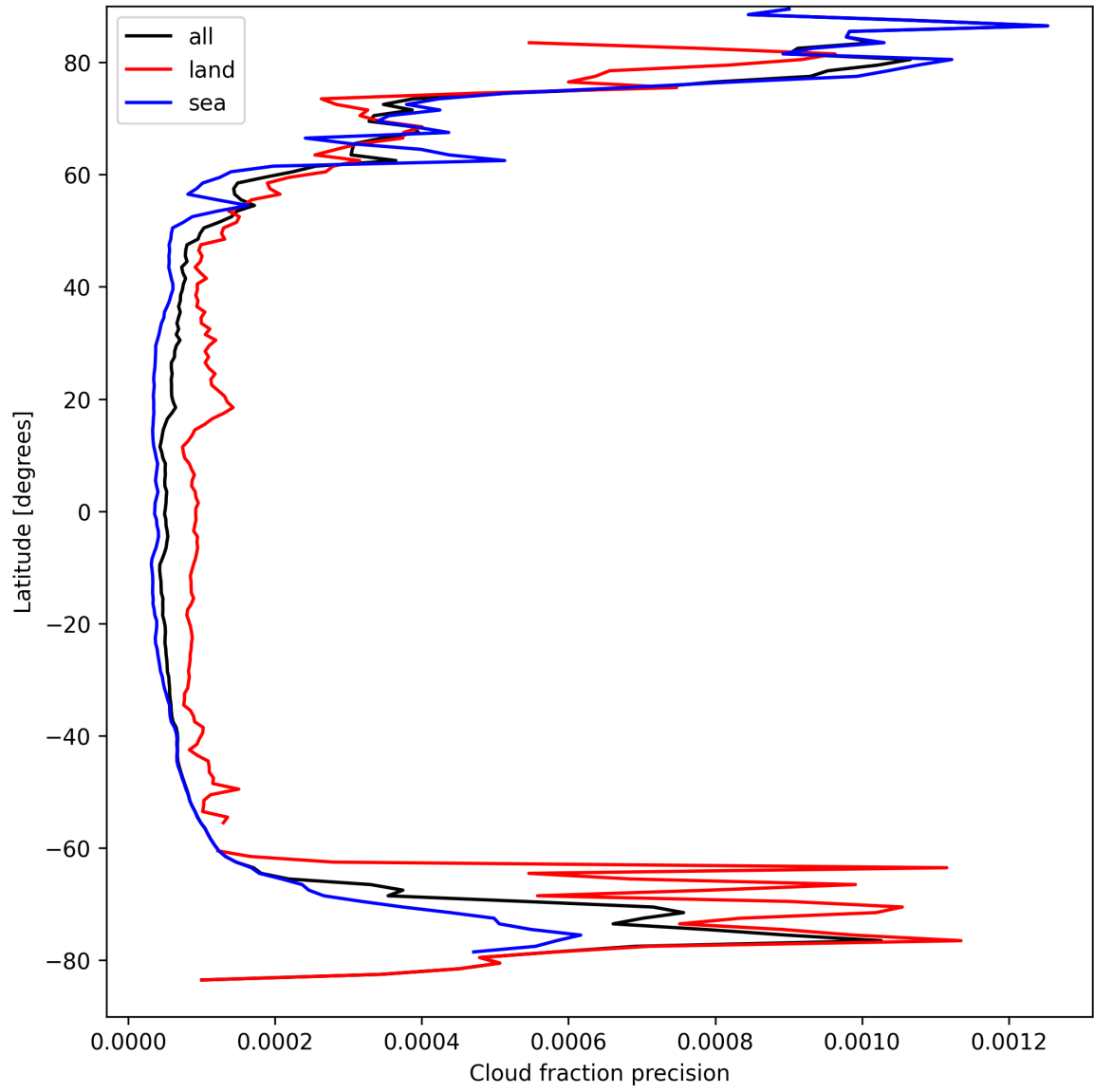
Figure 14: Zonal average of “Cloud fraction precision” for 2025-04-02 to 2025-04-03.
