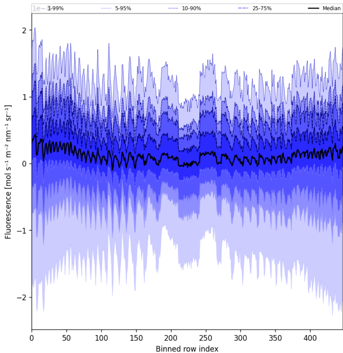
Figure 55: Along track statistics of “Fluorescence” for 2025-04-02 to 2025-04-03
