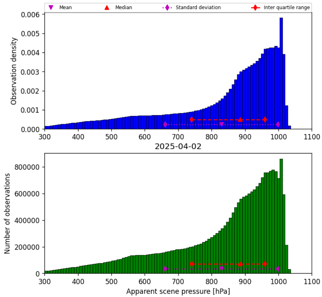
Figure 34: Histogram of “Apparent scene pressure” for 2025-04-02 to 2025-04-03
