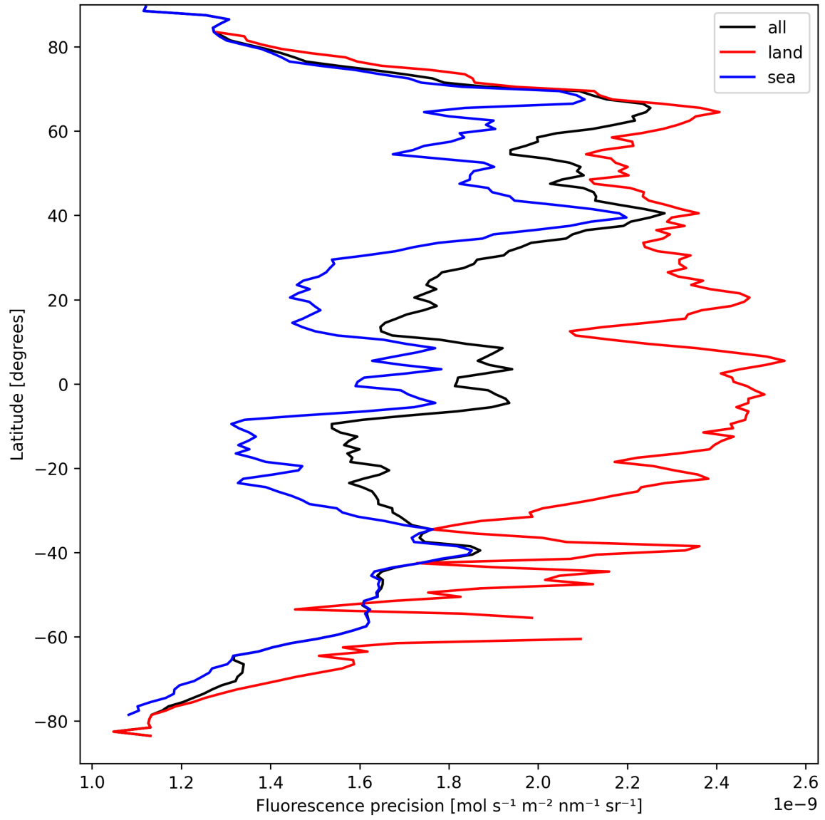
Figure 22: Zonal average of “Fluorescence precision” for 2025-04-02 to 2025-04-03.
