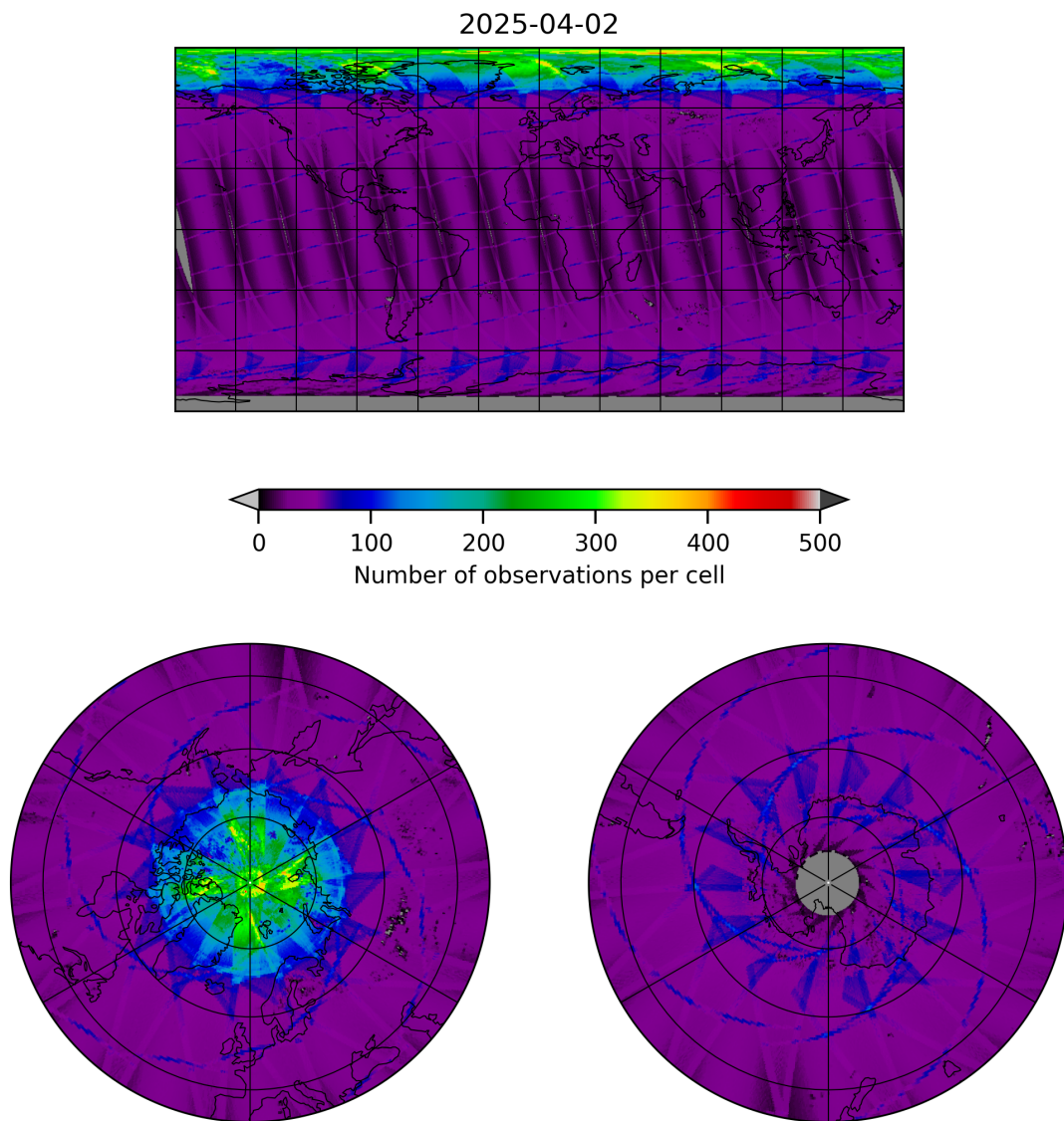
Figure 9: Map of the number of observations for 2025-04-02 to 2025-04-03
