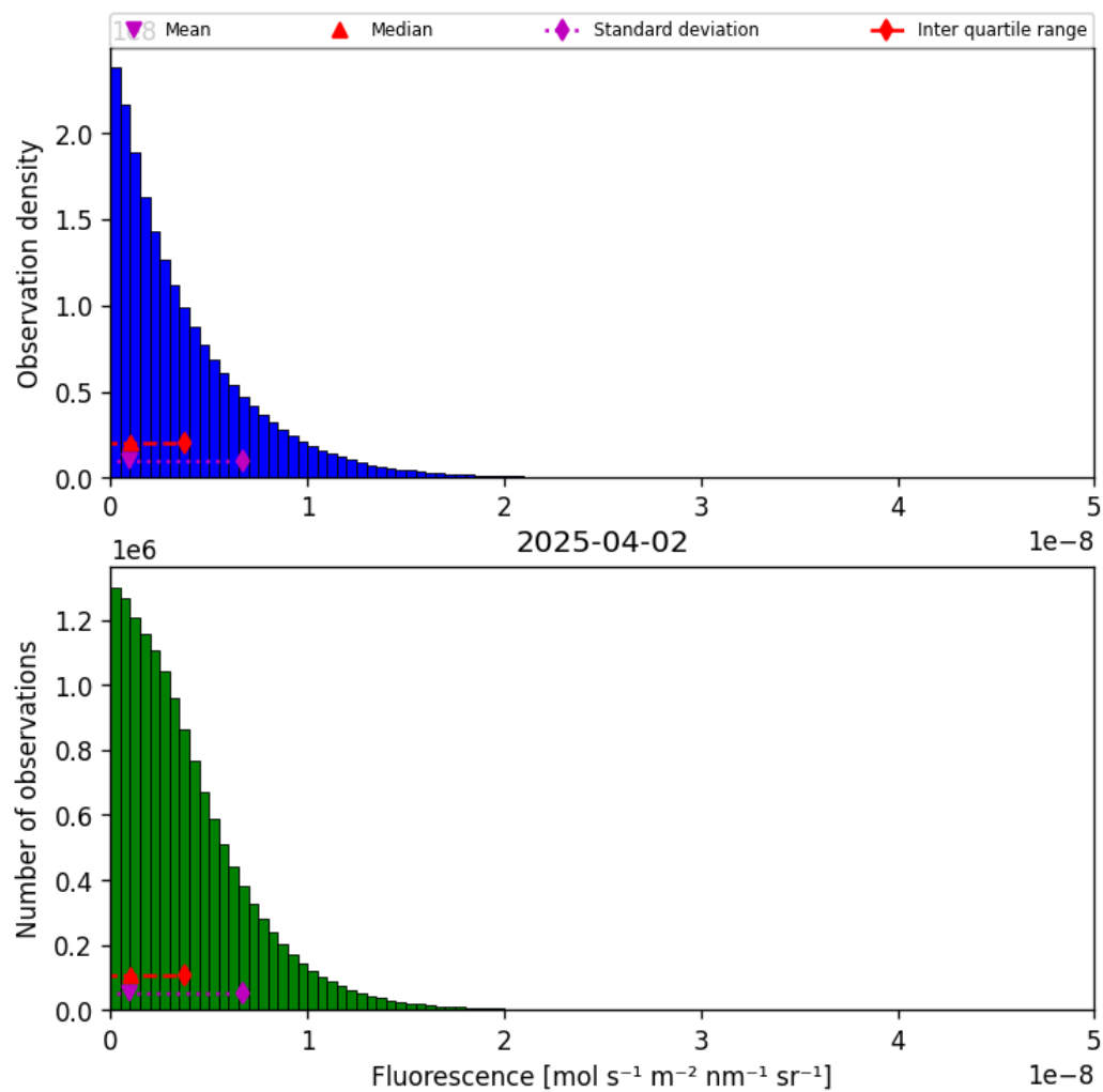
Figure 38: Histogram of “Fluorescence” for 2025-04-02 to 2025-04-03
