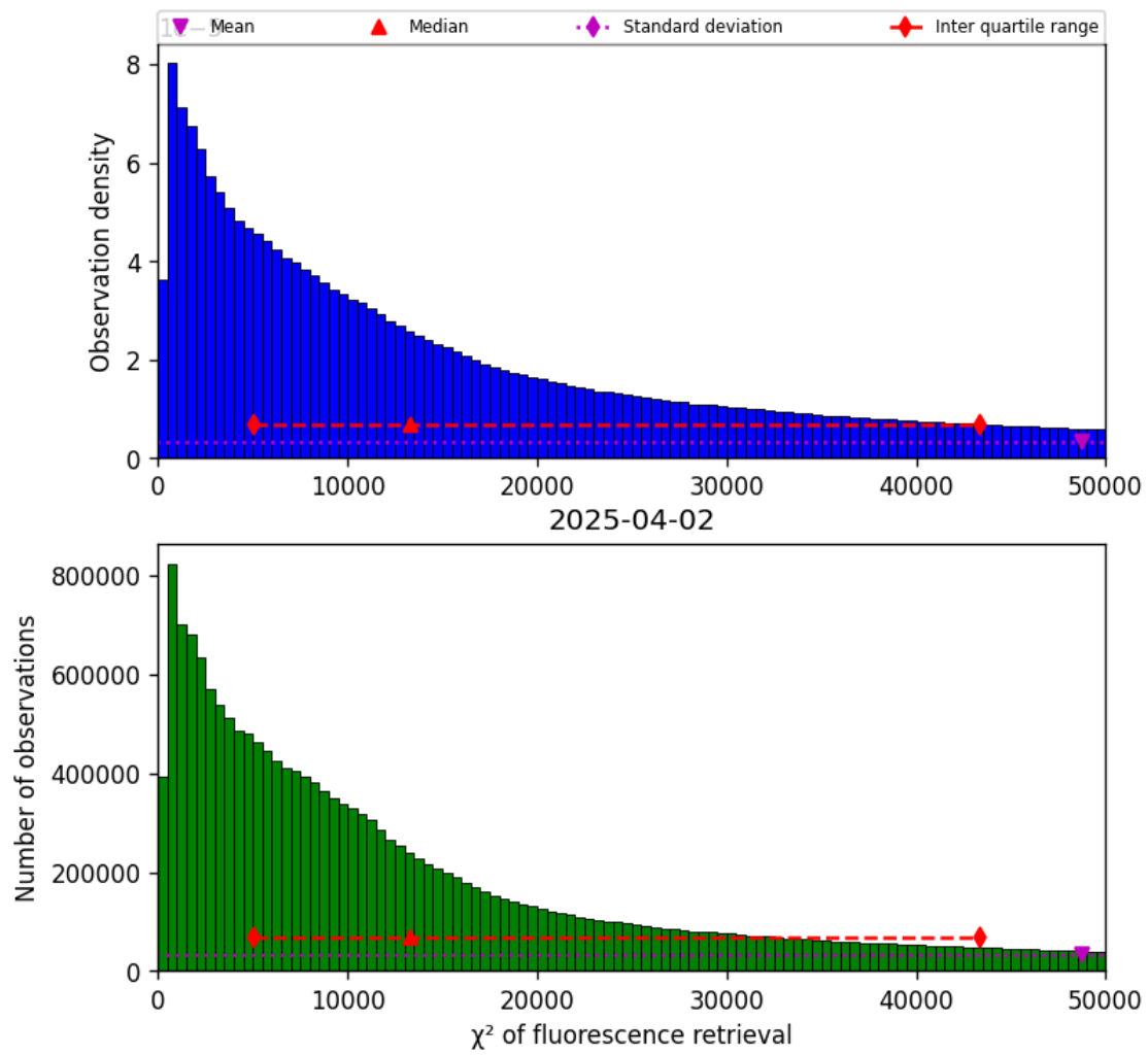
Figure 40: Histogram of “ \chi^2 of fluorescence retrieval” for 2025-04-02 to 2025-04-03
