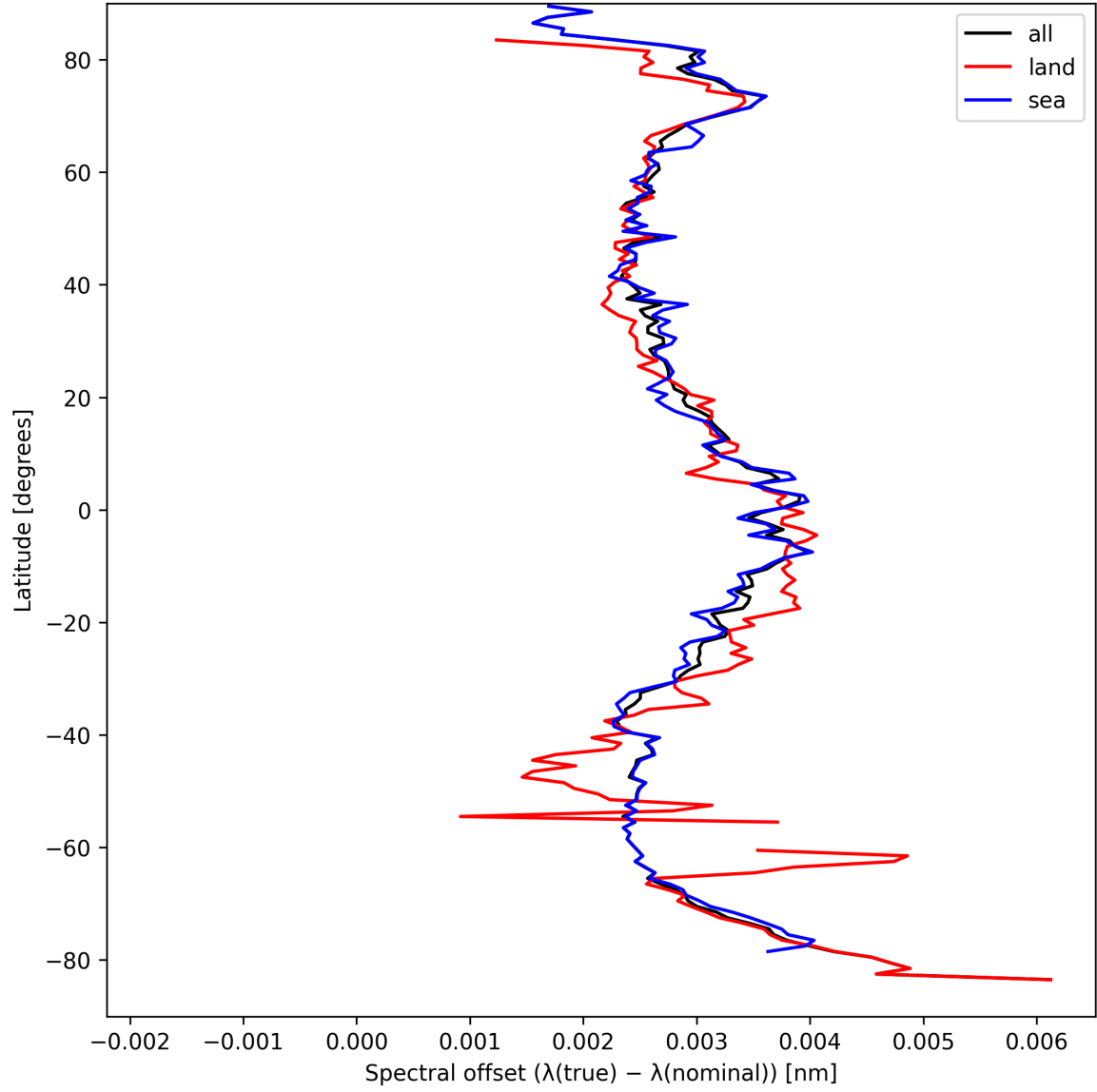
Figure 26: Zonal average of “Spectral offset ( \lambda_{\text{true}} - \lambda_{\text{nominal}} )” for 2025-04-02 to 2025-04-03.
