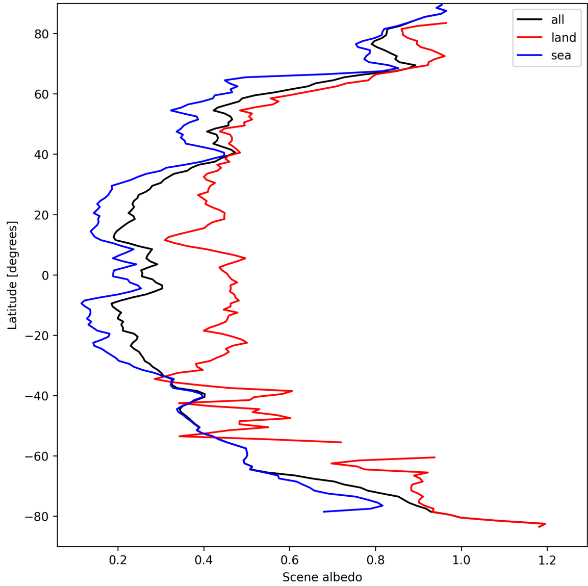
Figure 15: Zonal average of “Scene albedo” for 2025-04-02 to 2025-04-03.
