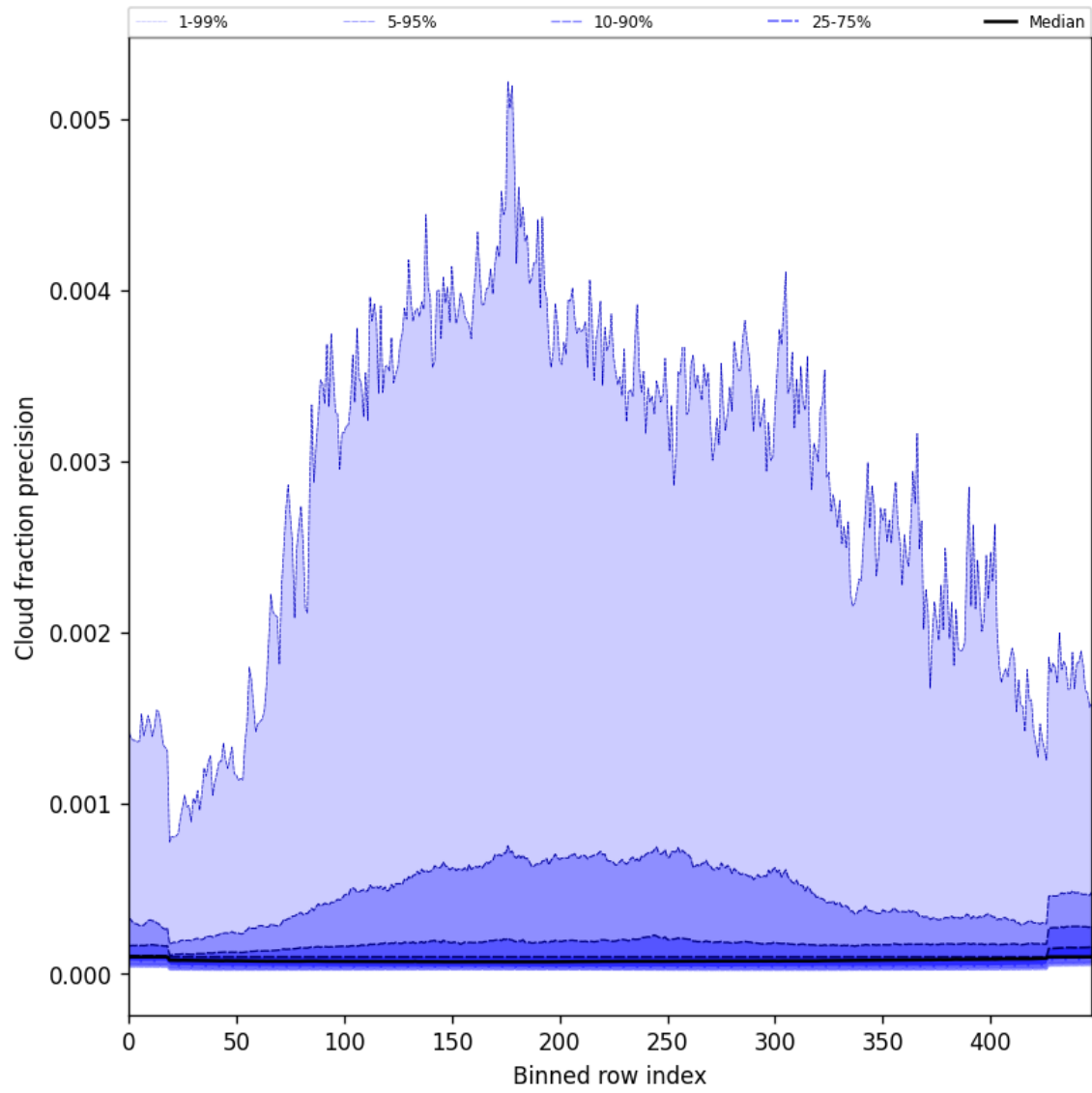
Figure 48: Along track statistics of “Cloud fraction precision” for 2025-04-02 to 2025-04-03
