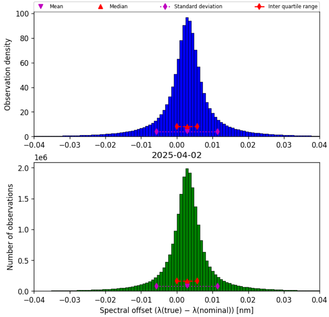
Figure 43: Histogram of “Spectral offset ( \lambda_{\text{true}} - \lambda_{\text{nominal}} )” for 2025-04-02 to 2025-04-03
