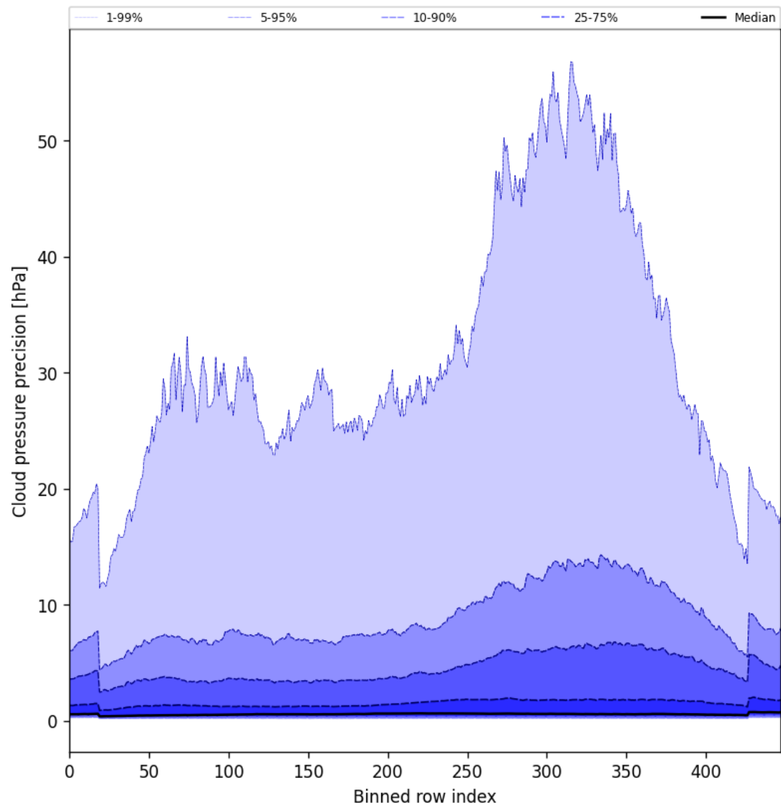
Figure 46: Along track statistics of “Cloud pressure precision” for 2025-04-02 to 2025-04-03
