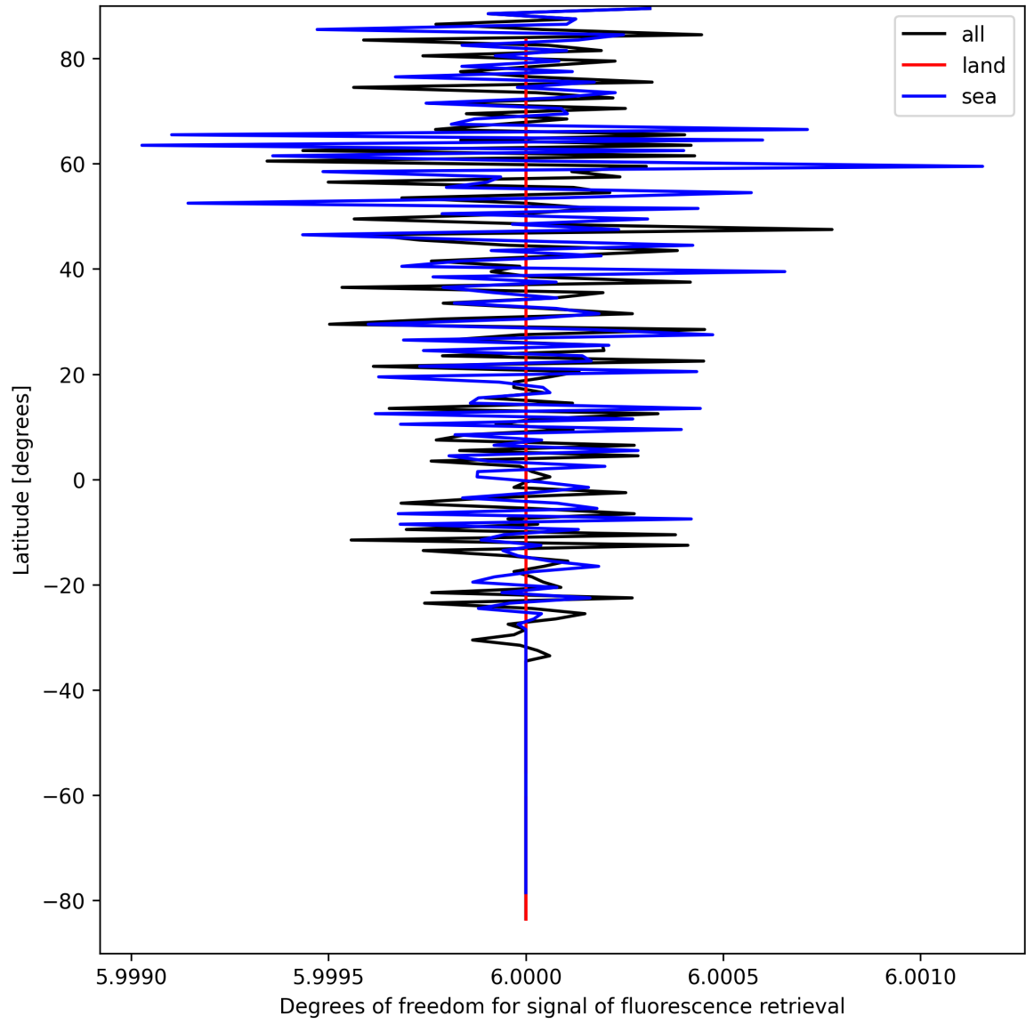
Figure 24: Zonal average of “Degrees of freedom for signal of fluorescence retrieval” for 2025-04-02 to 2025-04-03.
