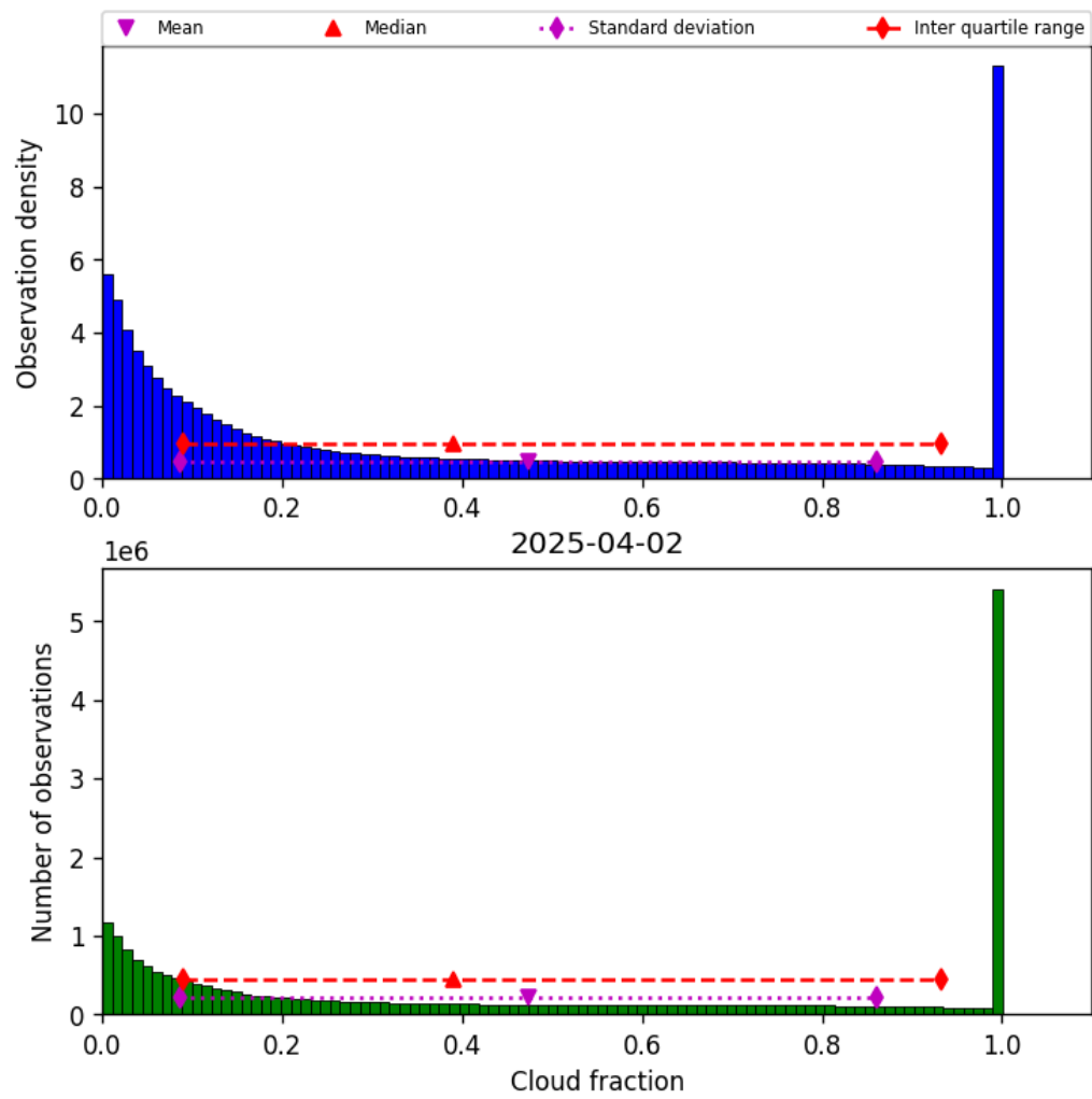
Figure 30: Histogram of “Cloud fraction” for 2025-04-02 to 2025-04-03
