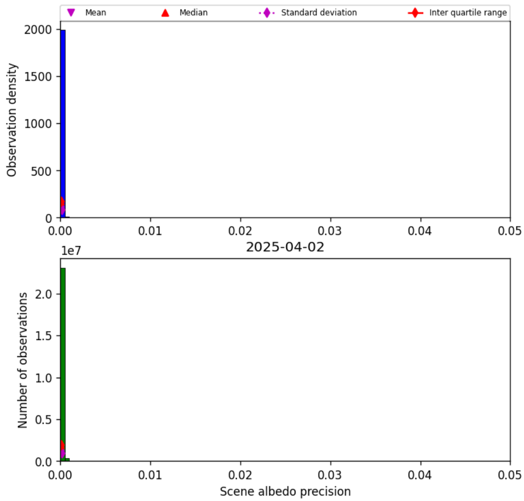
Figure 33: Histogram of “Scene albedo precision” for 2025-04-02 to 2025-04-03
