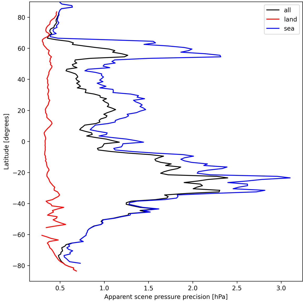
Figure 18: Zonal average of “Apparent scene pressure precision” for 2025-04-02 to 2025-04-03.
