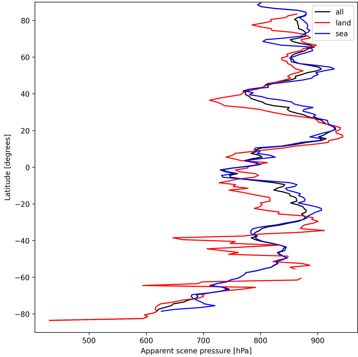
Figure 17: Zonal average of “Apparent scene pressure” for 2025-04-02 to 2025-04-03.
