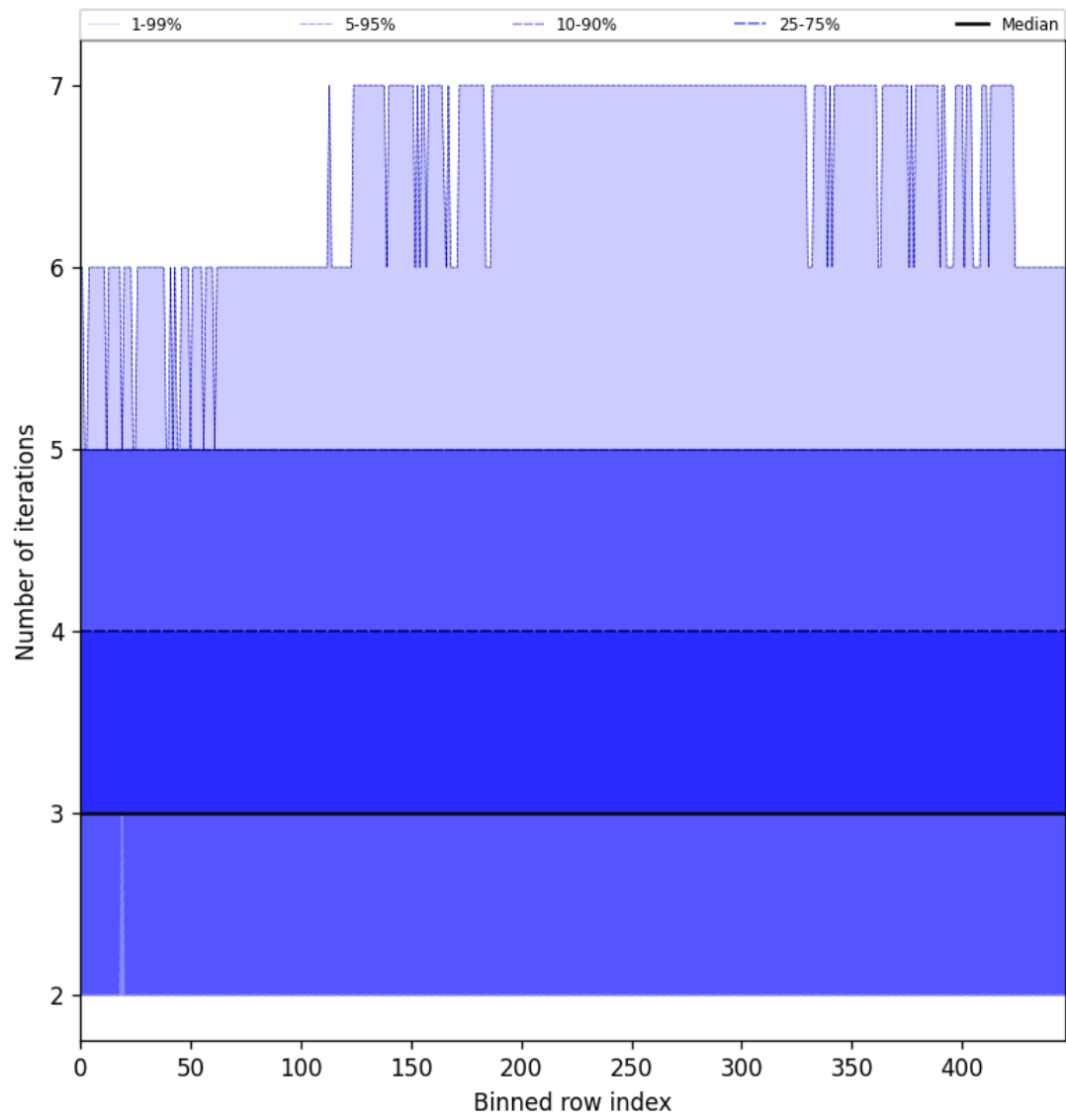
Figure 54: Along track statistics of “Number of iterations” for 2025-04-02 to 2025-04-03
