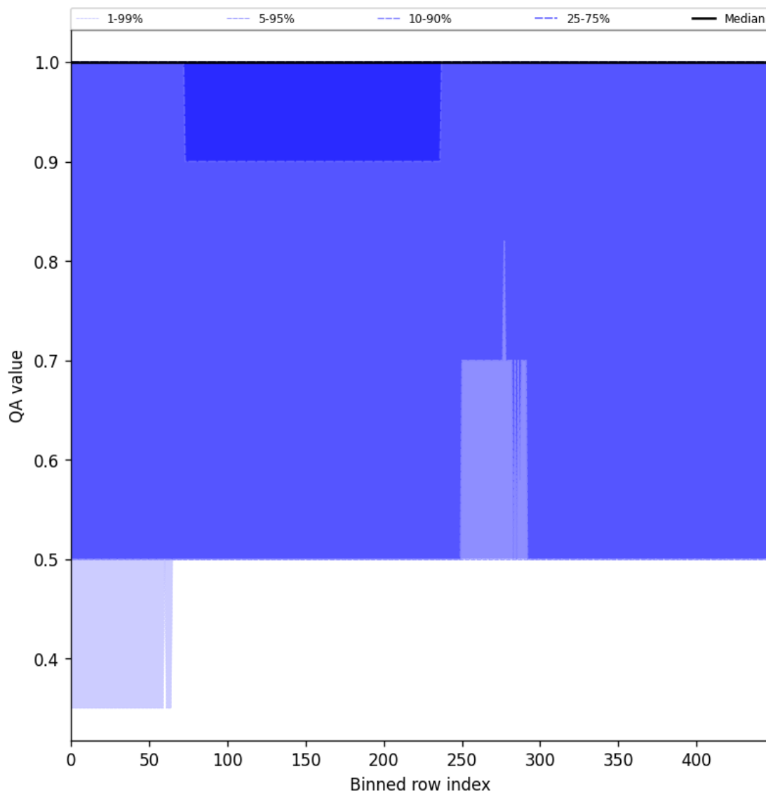
Figure 44: Along track statistics of “QA value” for 2025-04-02 to 2025-04-03
