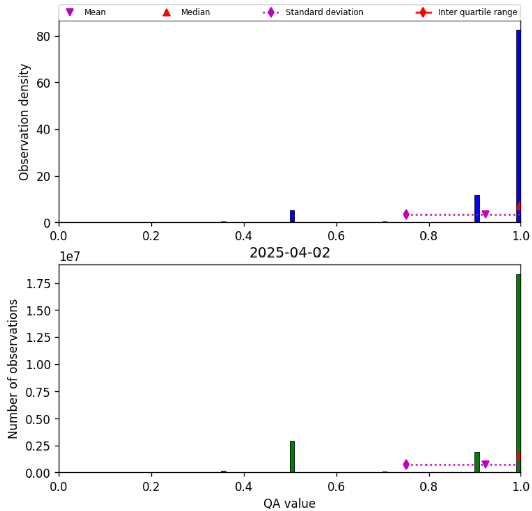
Figure 27: Histogram of “QA value” for 2025-04-02 to 2025-04-03
