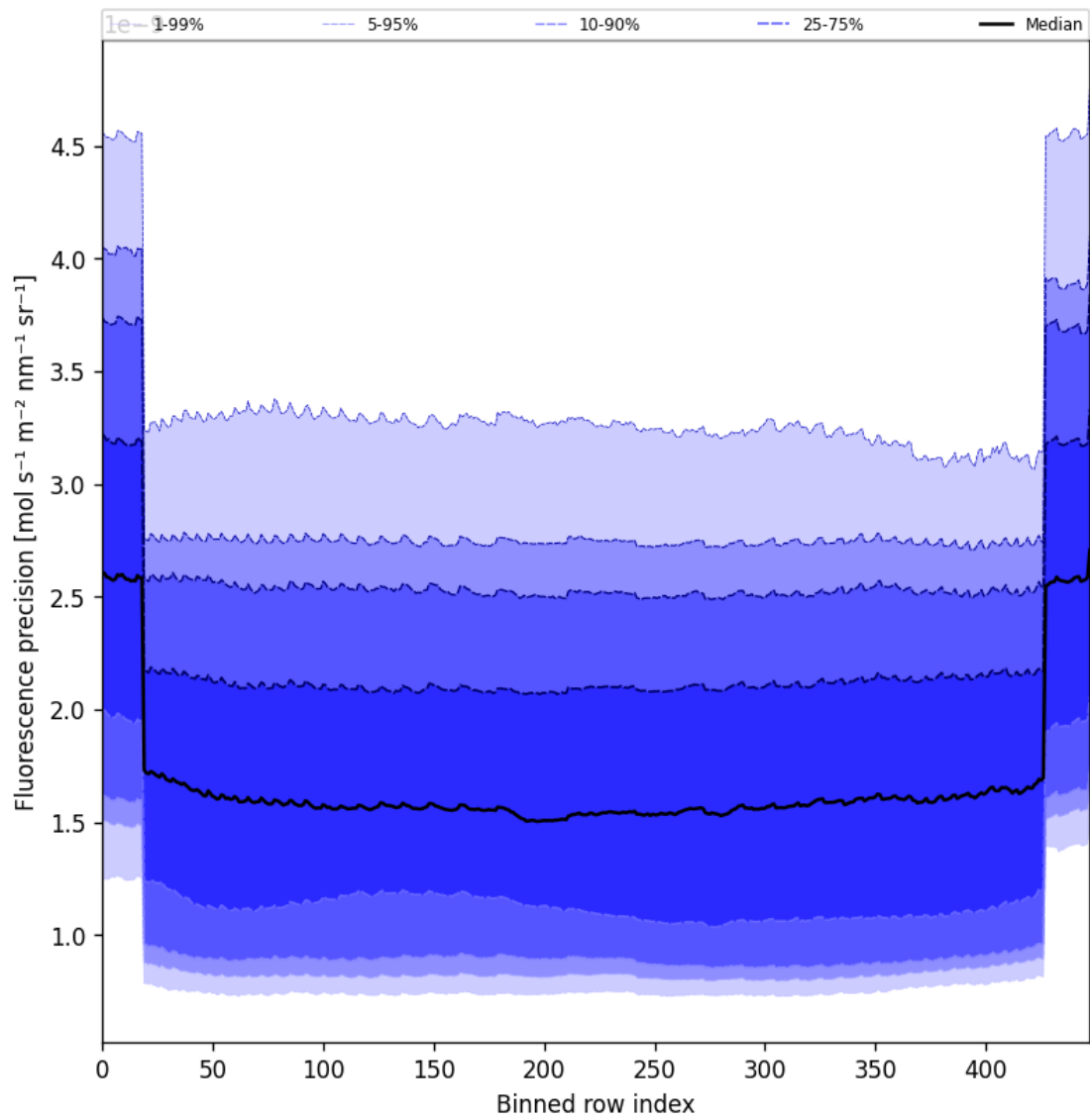
Figure 56: Along track statistics of "Fluorescence precision" for 2025-04-02 to 2025-04-03
