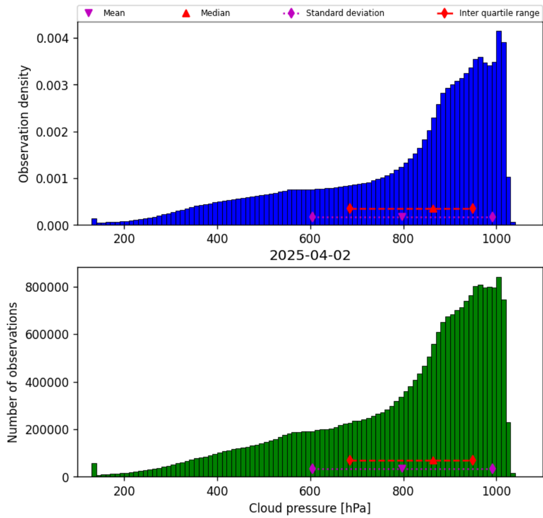
Figure 28: Histogram of “Cloud pressure” for 2025-04-02 to 2025-04-03
