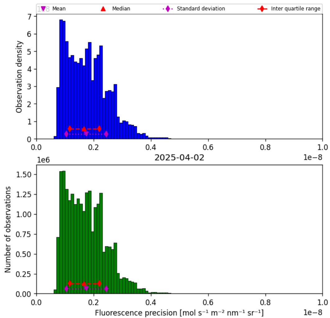
Figure 39: Histogram of “Fluorescence precision” for 2025-04-02 to 2025-04-03
