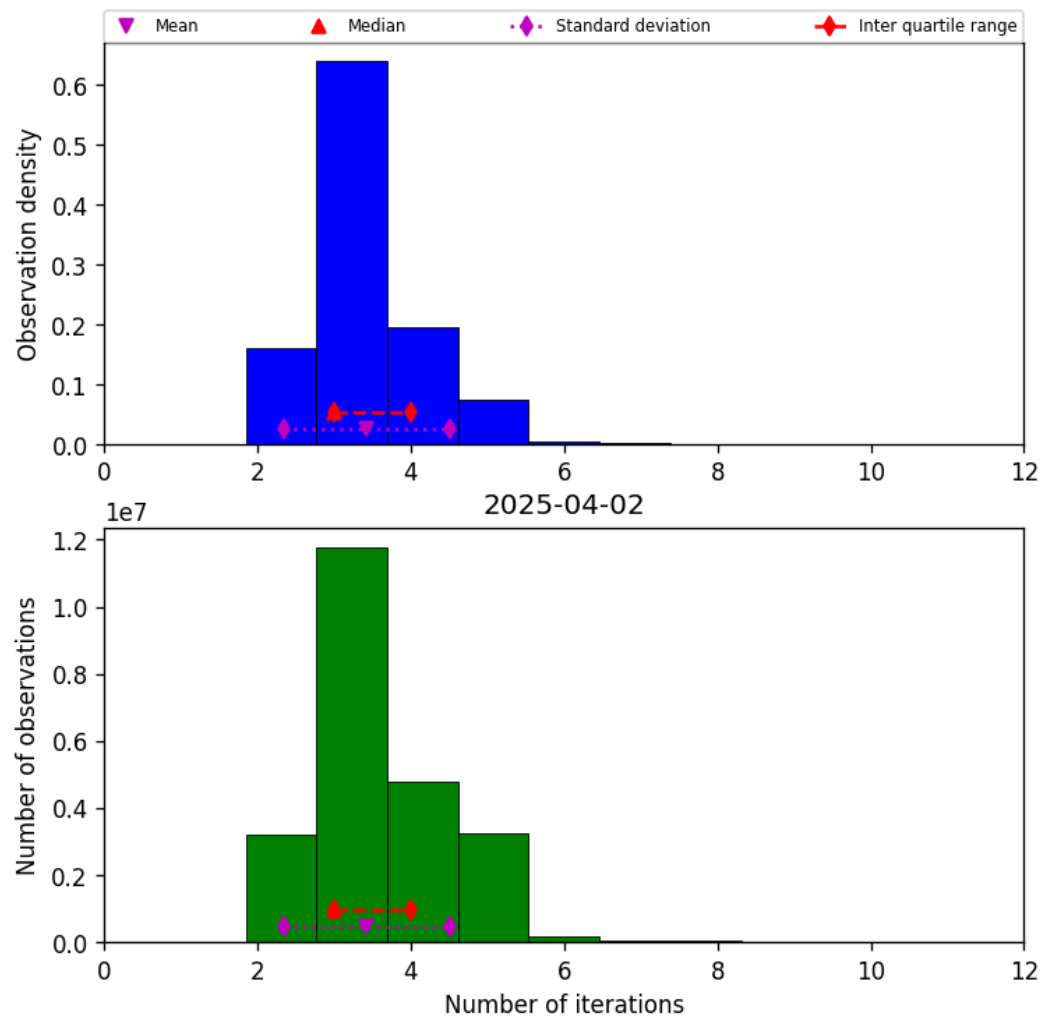
Figure 37: Histogram of “Number of iterations” for 2025-04-02 to 2025-04-03
