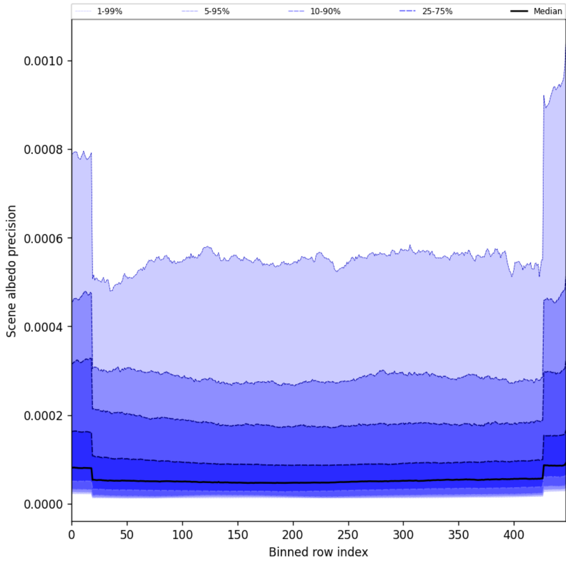
Figure 50: Along track statistics of “Scene albedo precision” for 2025-04-02 to 2025-04-03
