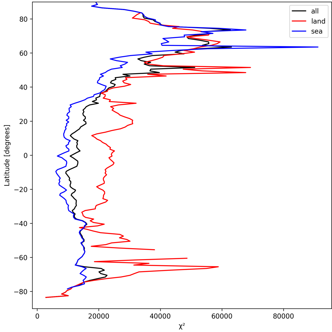
Figure 19: Zonal average of “ \chi^2 ” for 2025-04-02 to 2025-04-03.
