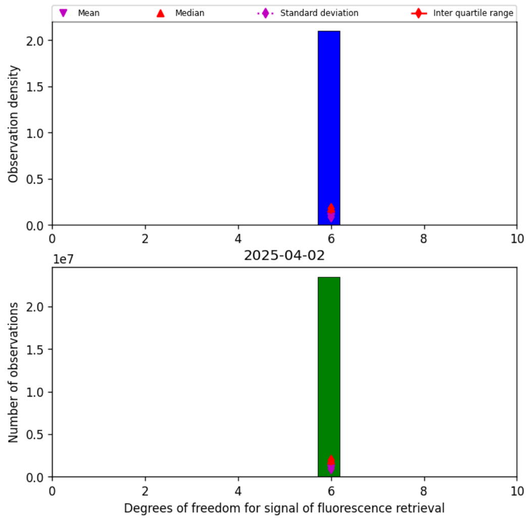
Figure 41: Histogram of “Degrees of freedom for signal of fluorescence retrieval” for 2025-04-02 to 2025-04-03
