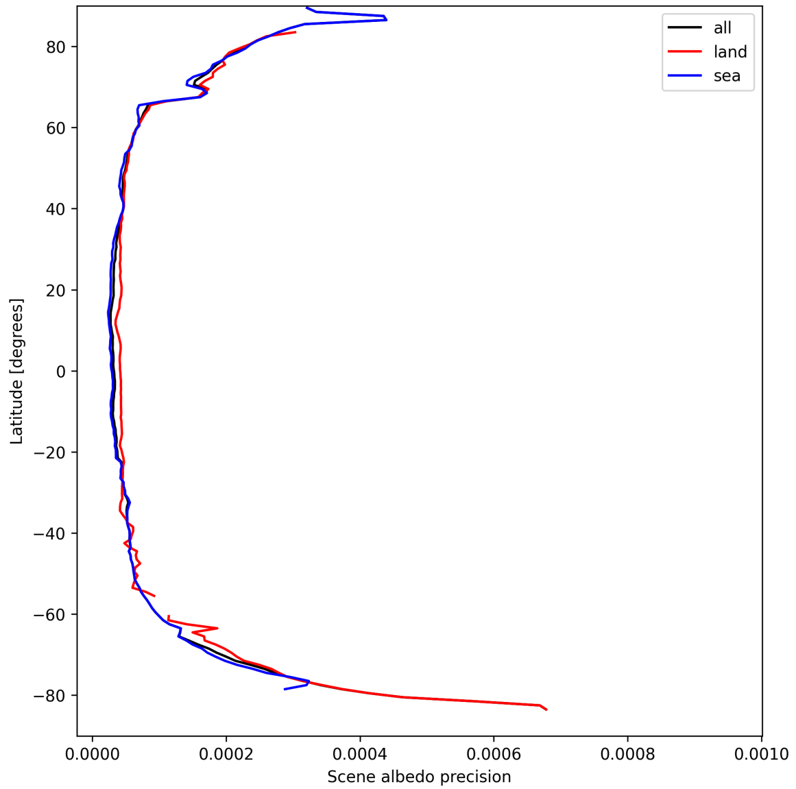
Figure 16: Zonal average of “Scene albedo precision” for 2025-04-02 to 2025-04-03.
