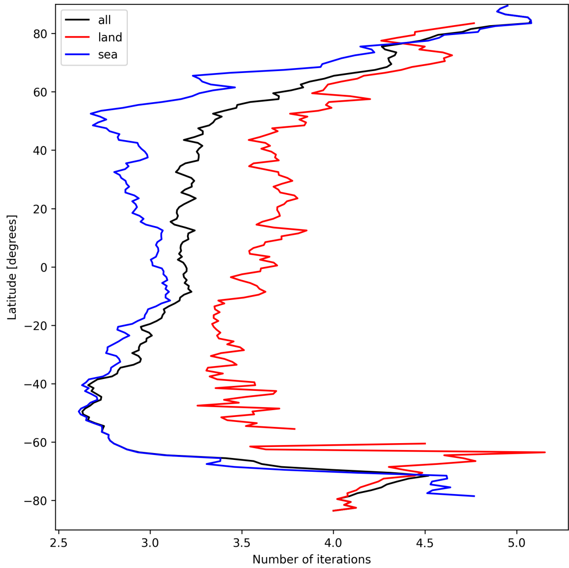
Figure 20: Zonal average of “Number of iterations” for 2025-04-02 to 2025-04-03.
