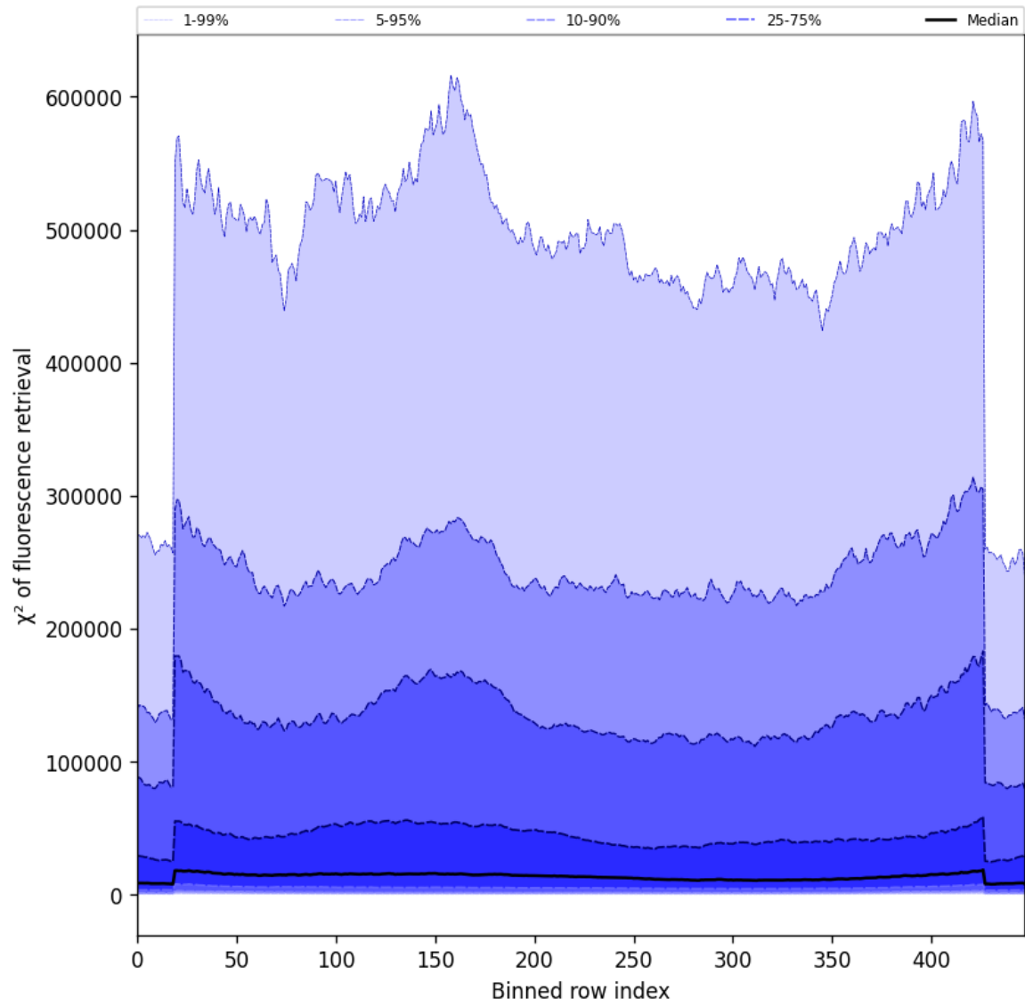
Figure 57: Along track statistics of “ \chi^2 of fluorescence retrieval” for 2025-04-02 to 2025-04-03
