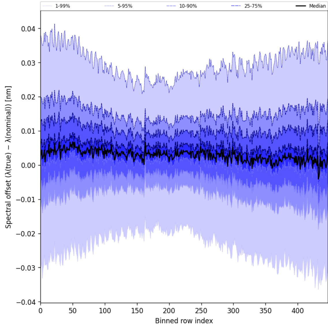
Figure 60: Along track statistics of “Spectral offset ( \lambda_{\text{true}} - \lambda_{\text{nominal}} )” for 2025-04-02 to 2025-04-03
