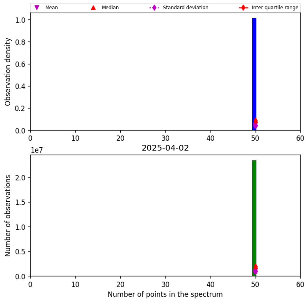
Figure 42: Histogram of “Number of points in the spectrum” for 2025-04-02 to 2025-04-03
