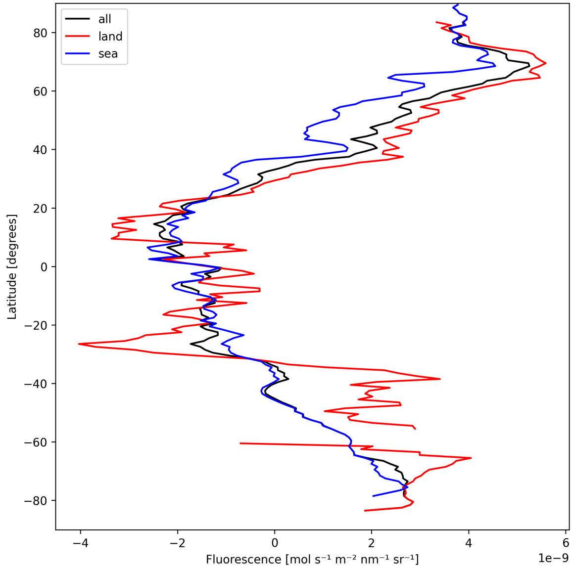
Figure 21: Zonal average of “Fluorescence” for 2025-04-02 to 2025-04-03.
