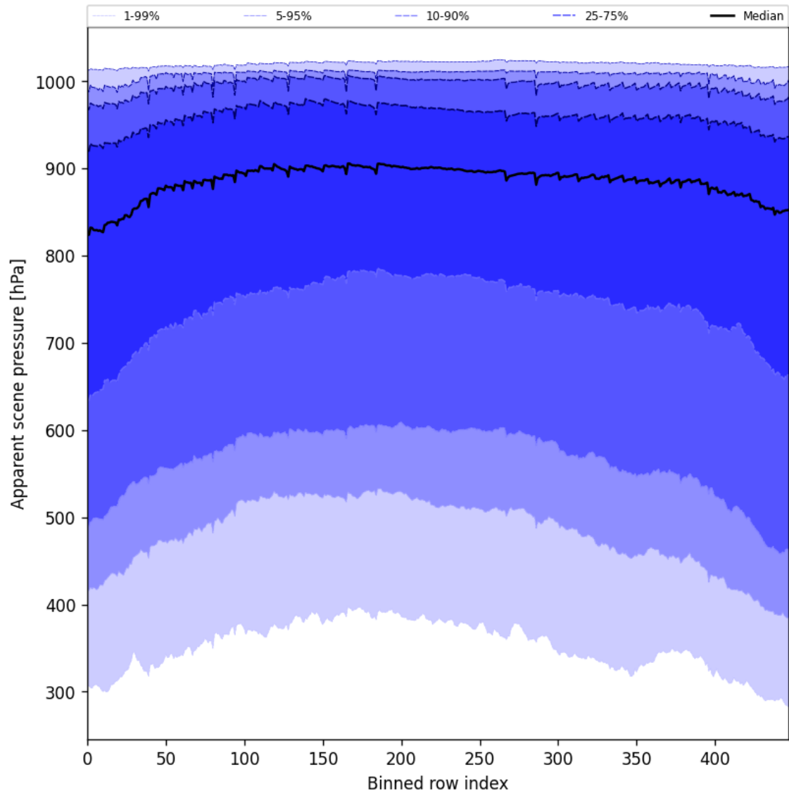
Figure 51: Along track statistics of “Apparent scene pressure” for 2025-04-02 to 2025-04-03
