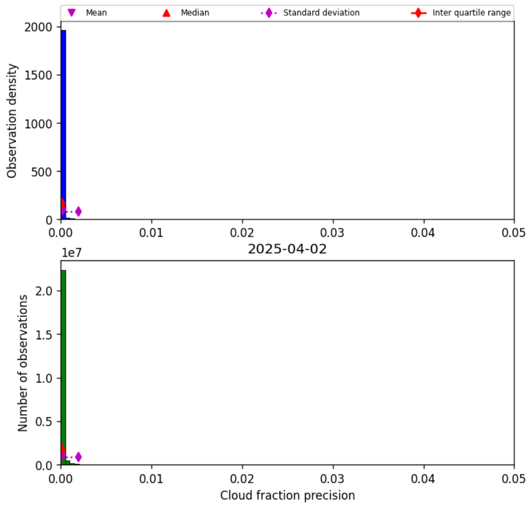
Figure 31: Histogram of “Cloud fraction precision” for 2025-04-02 to 2025-04-03
