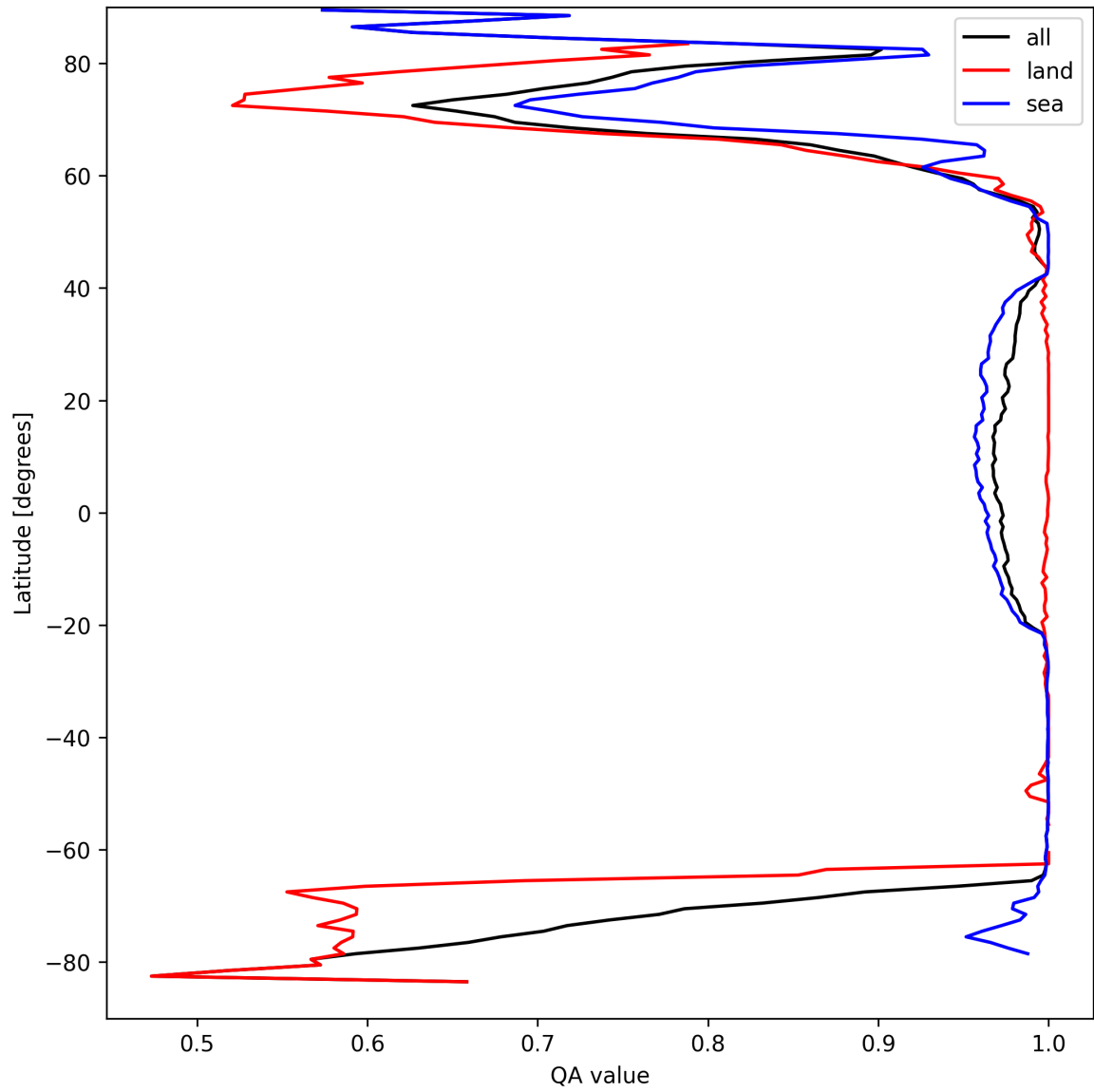
Figure 10: Zonal average of “QA value” for 2025-04-02 to 2025-04-03.
