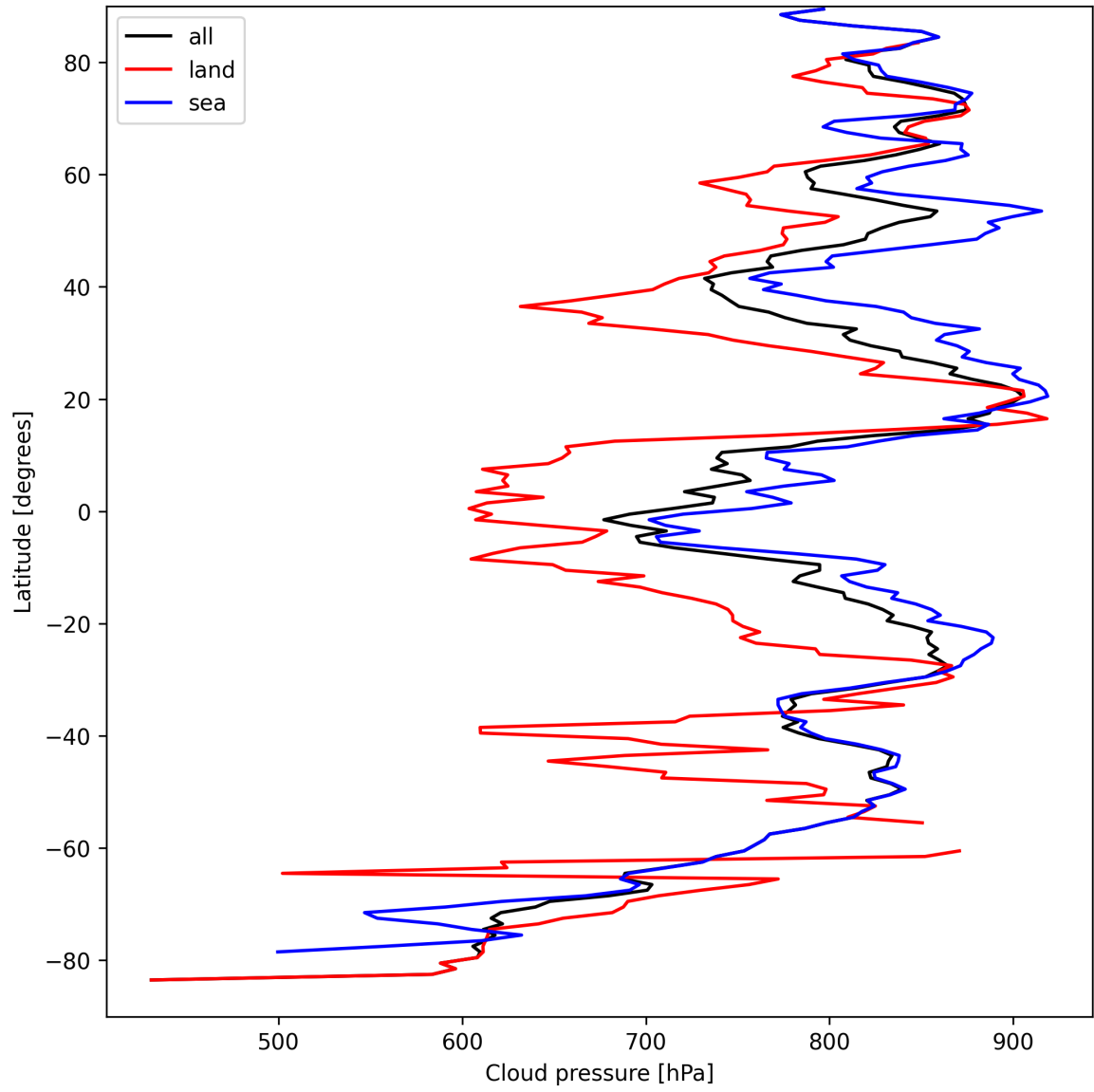
Figure 11: Zonal average of “Cloud pressure” for 2025-04-02 to 2025-04-03.
