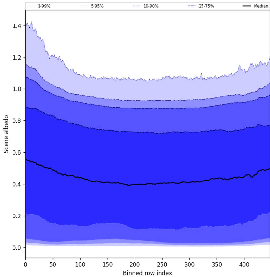
Figure 49: Along track statistics of “Scene albedo” for 2025-04-02 to 2025-04-03
