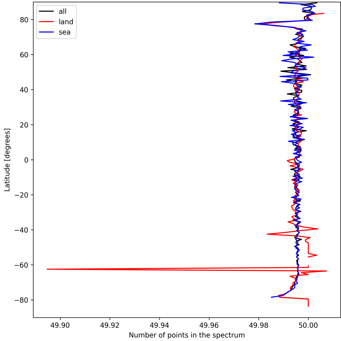
Figure 25: Zonal average of “Number of points in the spectrum” for 2025-04-02 to 2025-04-03.
