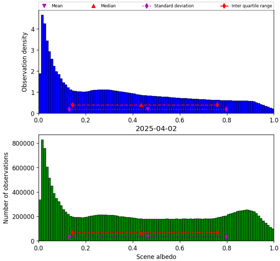
Figure 32: Histogram of “Scene albedo” for 2025-04-02 to 2025-04-03
