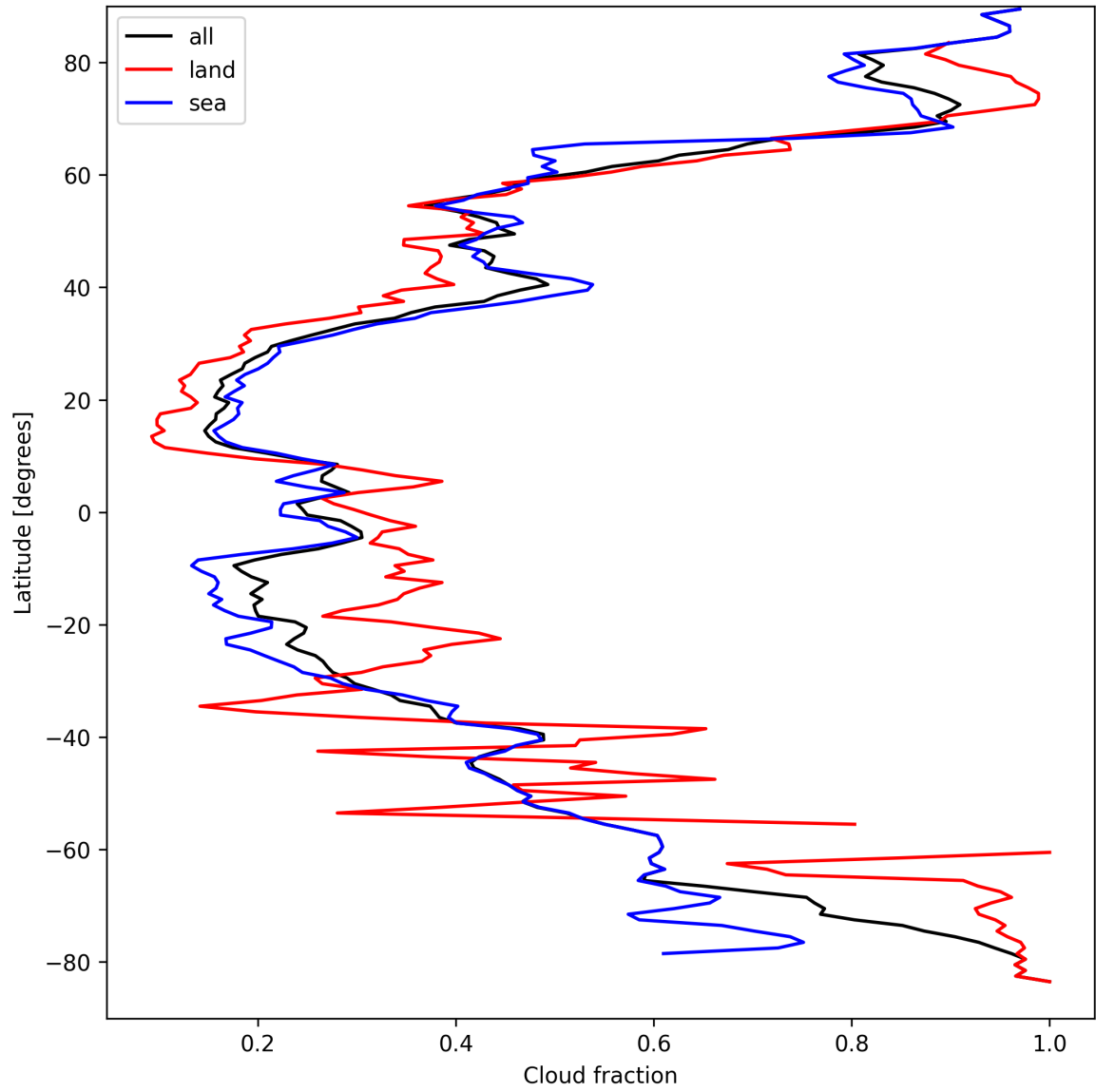
Figure 13: Zonal average of “Cloud fraction” for 2025-04-02 to 2025-04-03.
