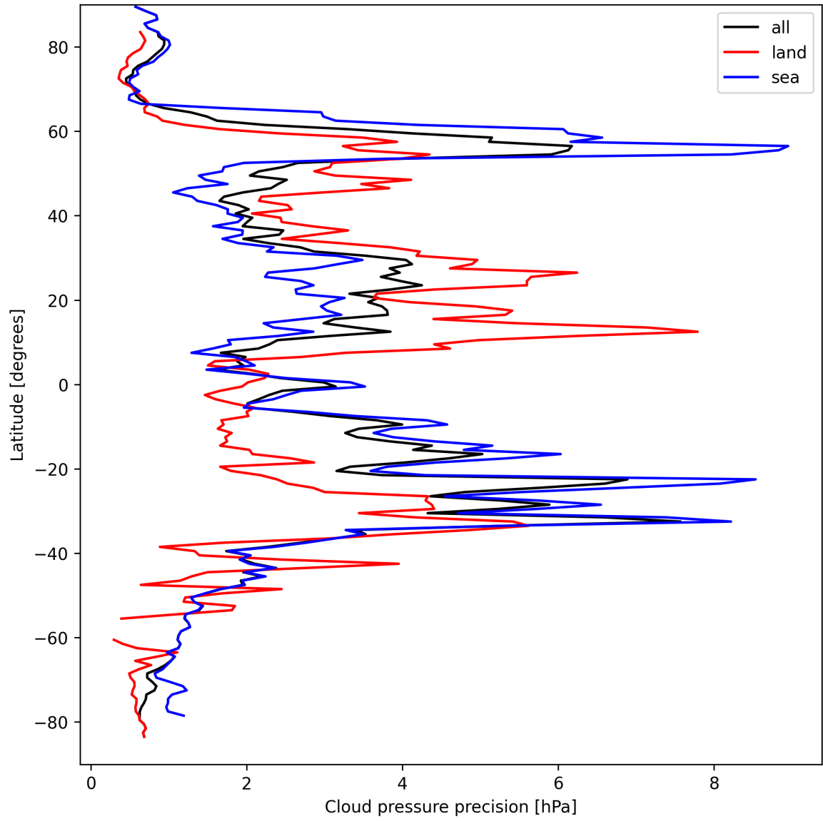
Figure 12: Zonal average of “Cloud pressure precision” for 2025-04-02 to 2025-04-03.
