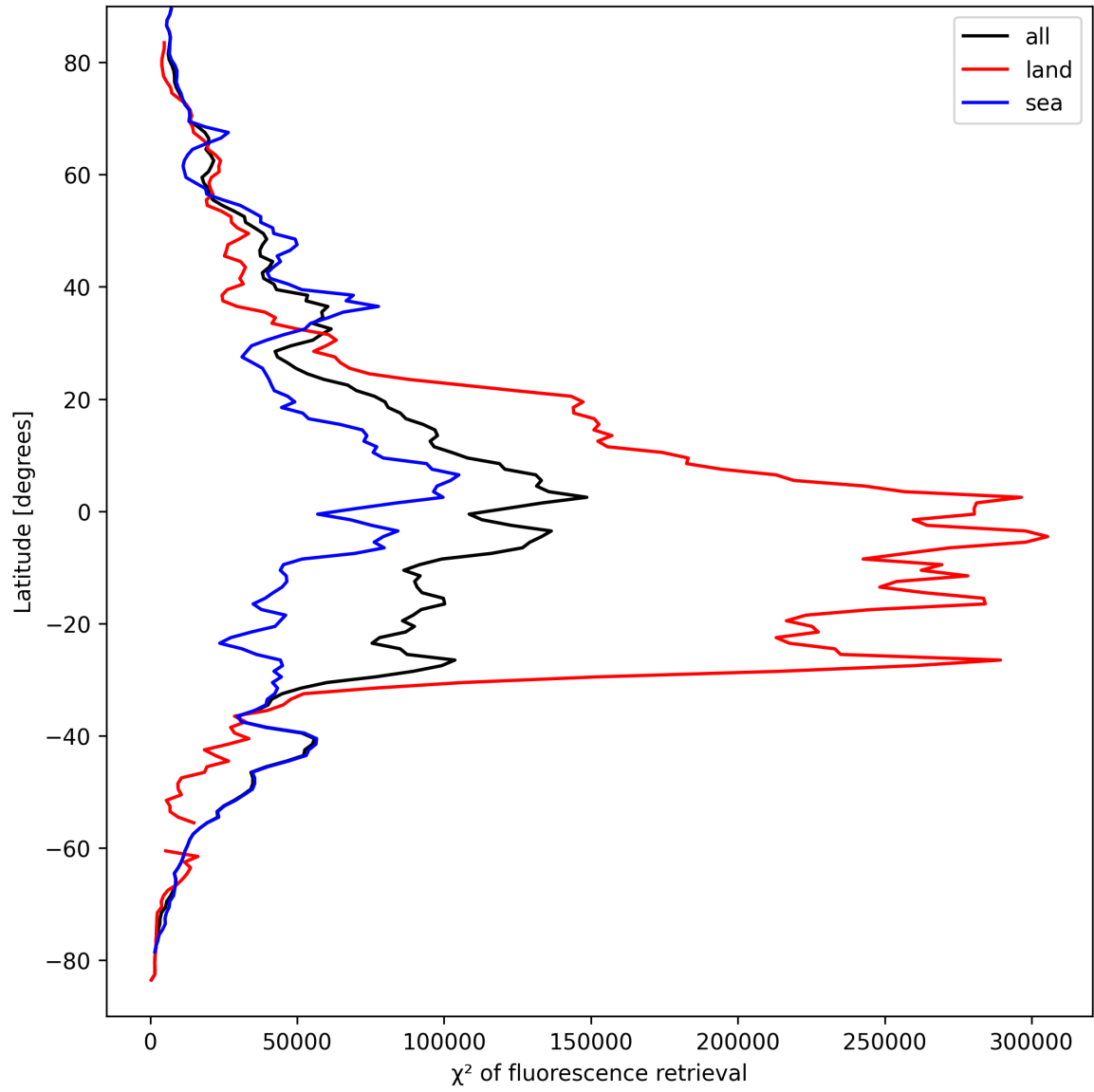
Figure 23: Zonal average of “ \chi^2 of fluorescence retrieval” for 2025-04-02 to 2025-04-03.
