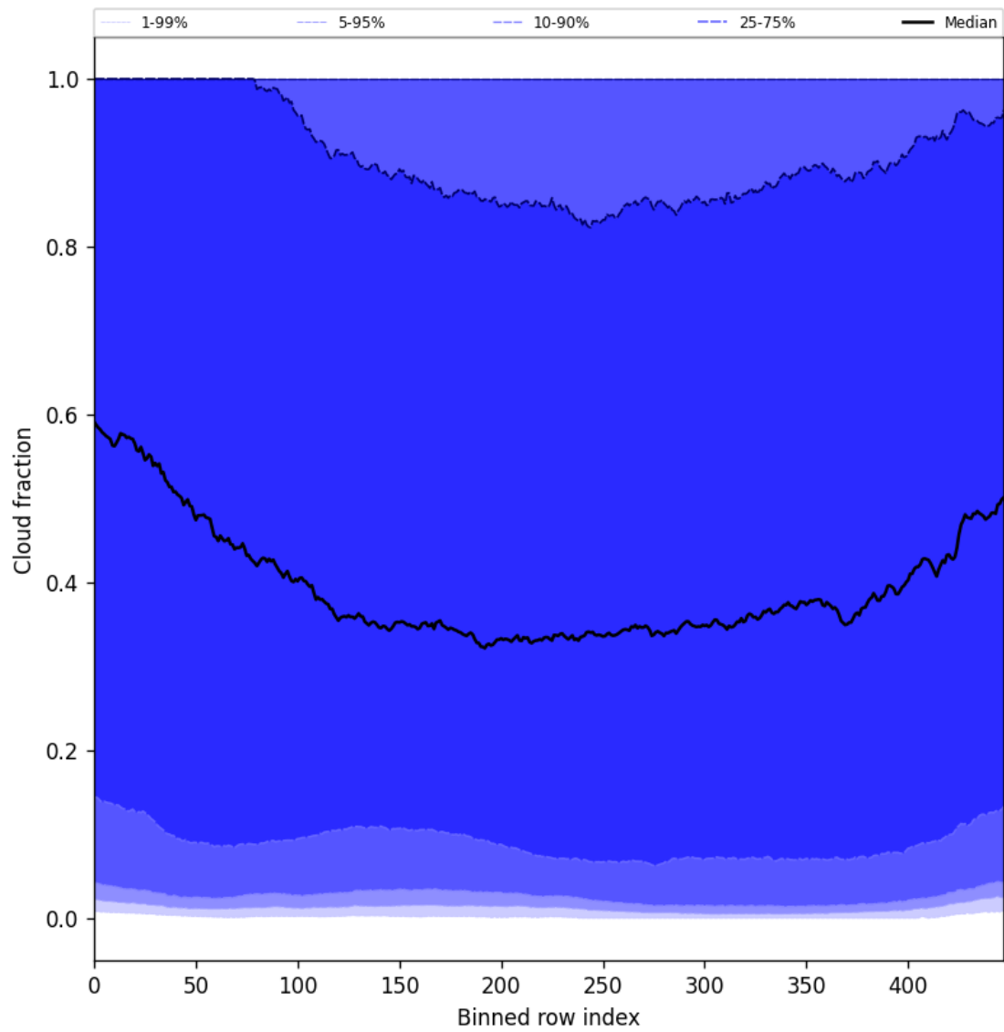
Figure 47: Along track statistics of “Cloud fraction” for 2025-04-02 to 2025-04-03
