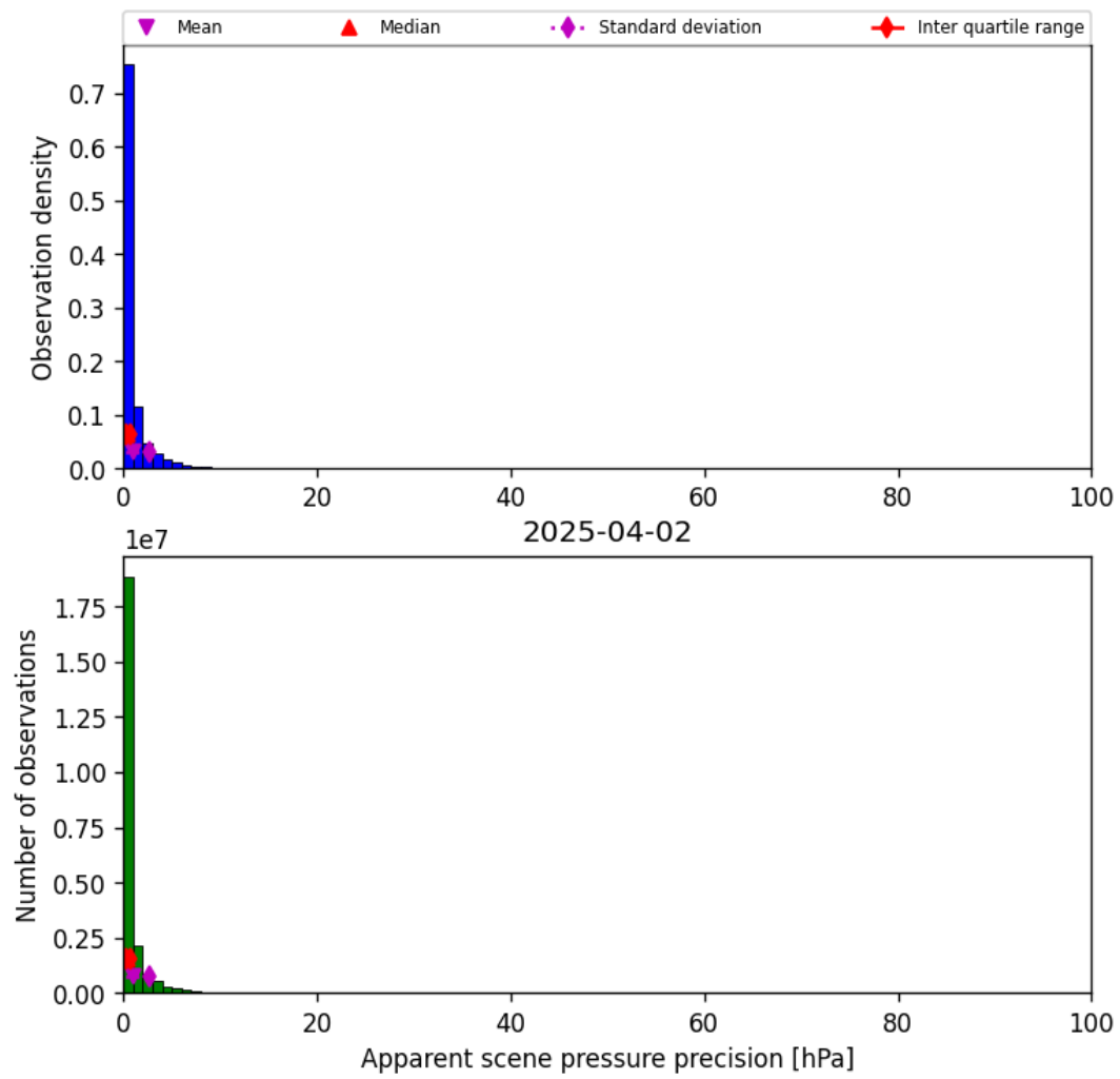
Figure 35: Histogram of “Apparent scene pressure precision” for 2025-04-02 to 2025-04-03
