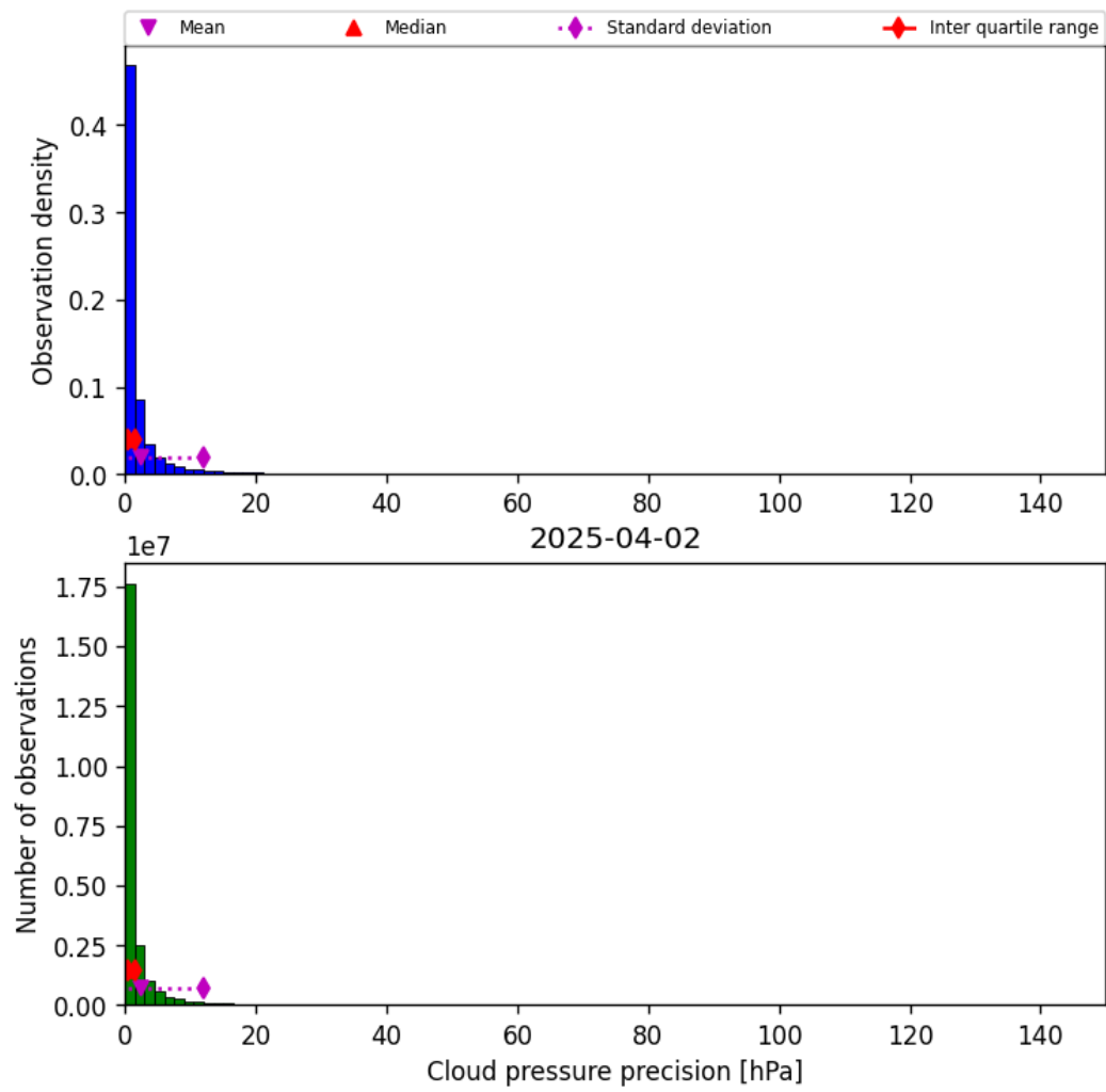
Figure 29: Histogram of “Cloud pressure precision” for 2025-04-02 to 2025-04-03
