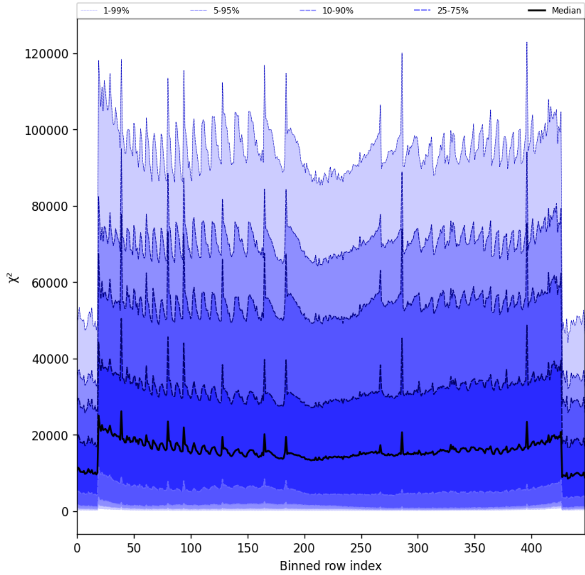
Figure 53: Along track statistics of “ \chi^2 ” for 2025-04-02 to 2025-04-03
