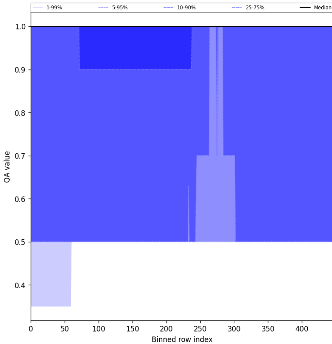
Figure 44: Along track statistics of “QA value” for 2025-04-03 to 2025-04-04
