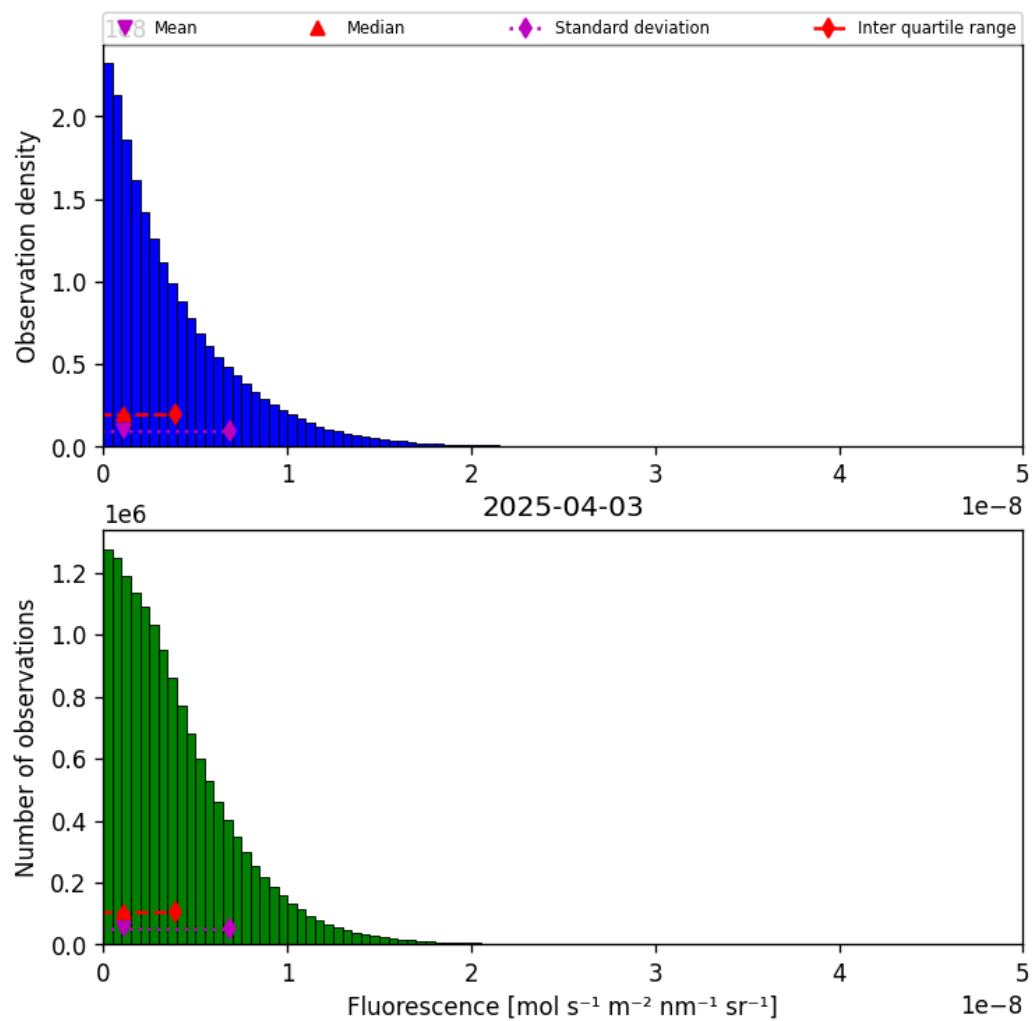
Figure 38: Histogram of “Fluorescence” for 2025-04-03 to 2025-04-04
