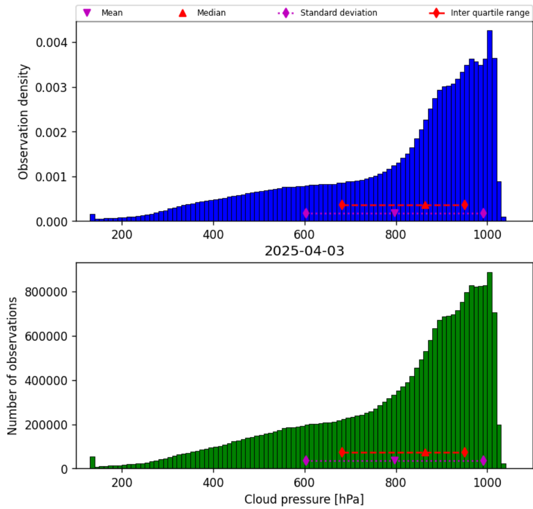
Figure 28: Histogram of “Cloud pressure” for 2025-04-03 to 2025-04-04
