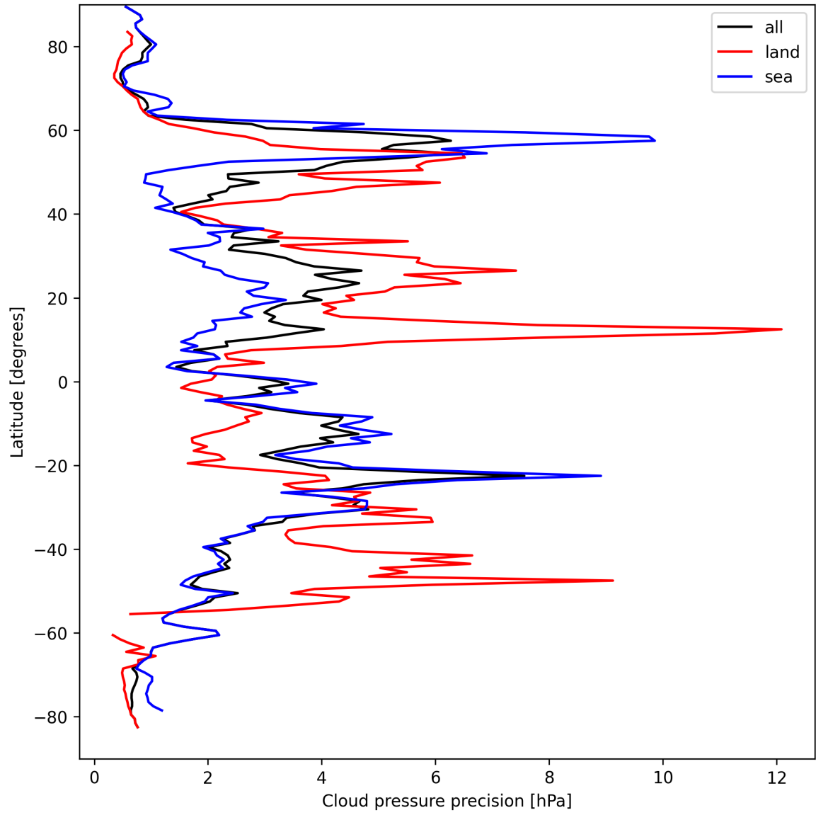
Figure 12: Zonal average of "Cloud pressure precision" for 2025-04-03 to 2025-04-04.
