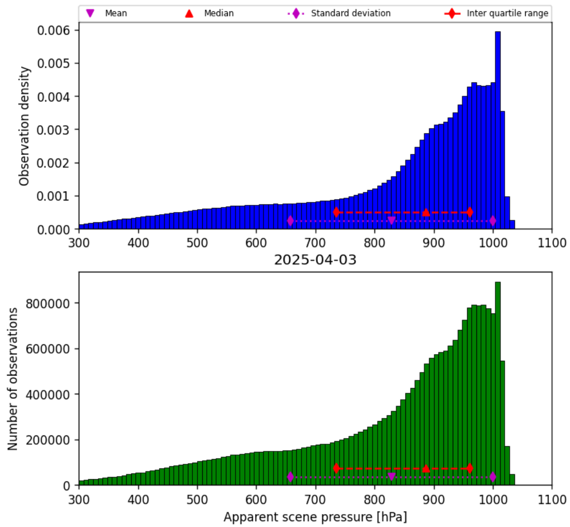
Figure 34: Histogram of “Apparent scene pressure” for 2025-04-03 to 2025-04-04
