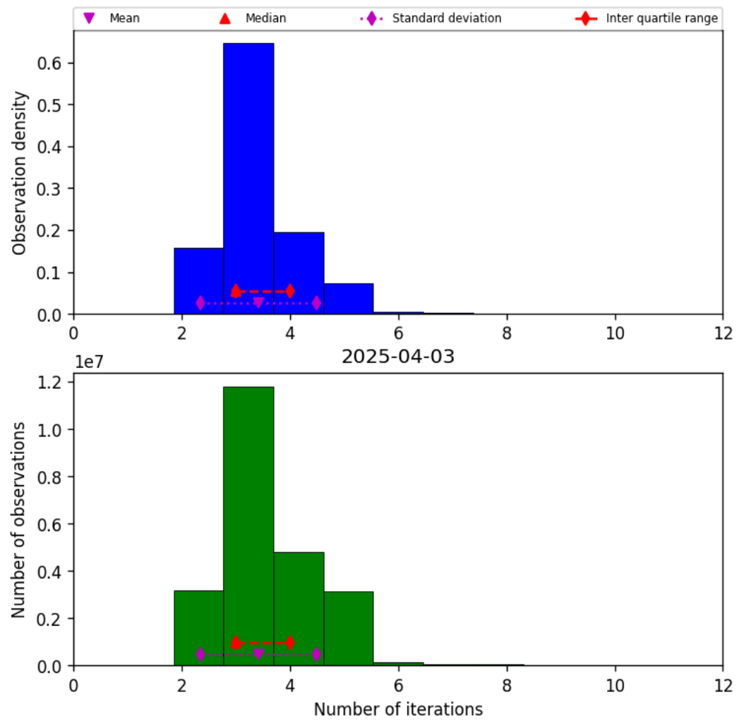
Figure 37: Histogram of “Number of iterations” for 2025-04-03 to 2025-04-04
