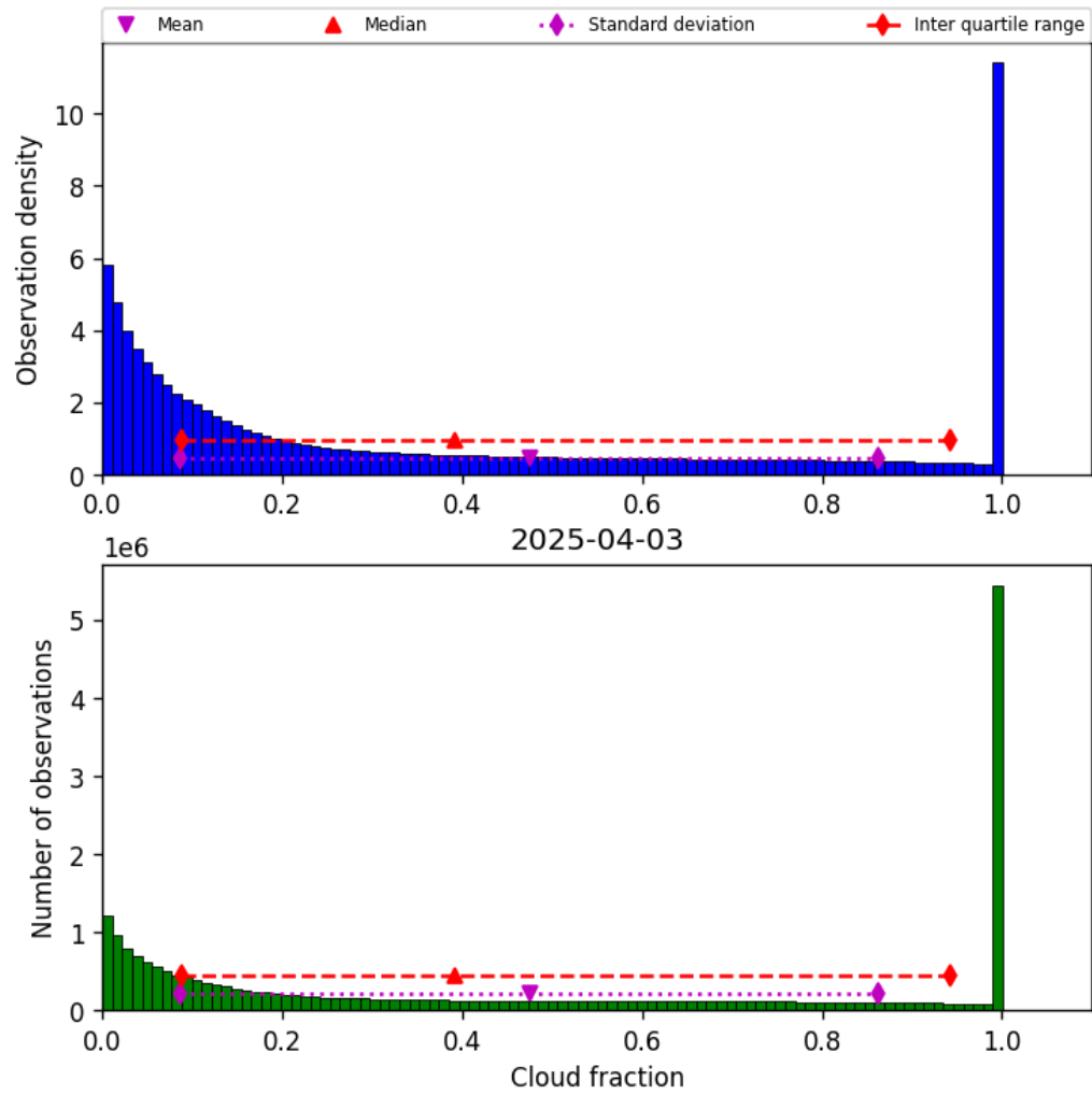
Figure 30: Histogram of “Cloud fraction” for 2025-04-03 to 2025-04-04
