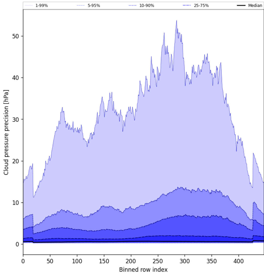
Figure 46: Along track statistics of “Cloud pressure precision” for 2025-04-03 to 2025-04-04
