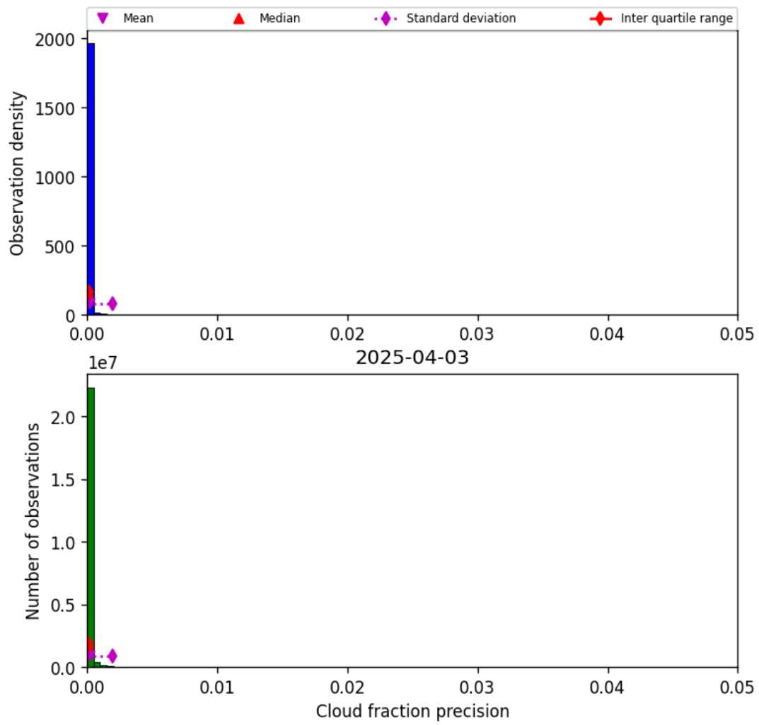
Figure 31: Histogram of “Cloud fraction precision” for 2025-04-03 to 2025-04-04
