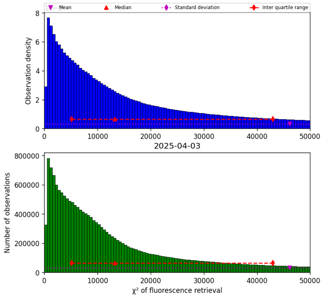
Figure 40: Histogram of “ \chi^2 of fluorescence retrieval” for 2025-04-03 to 2025-04-04
