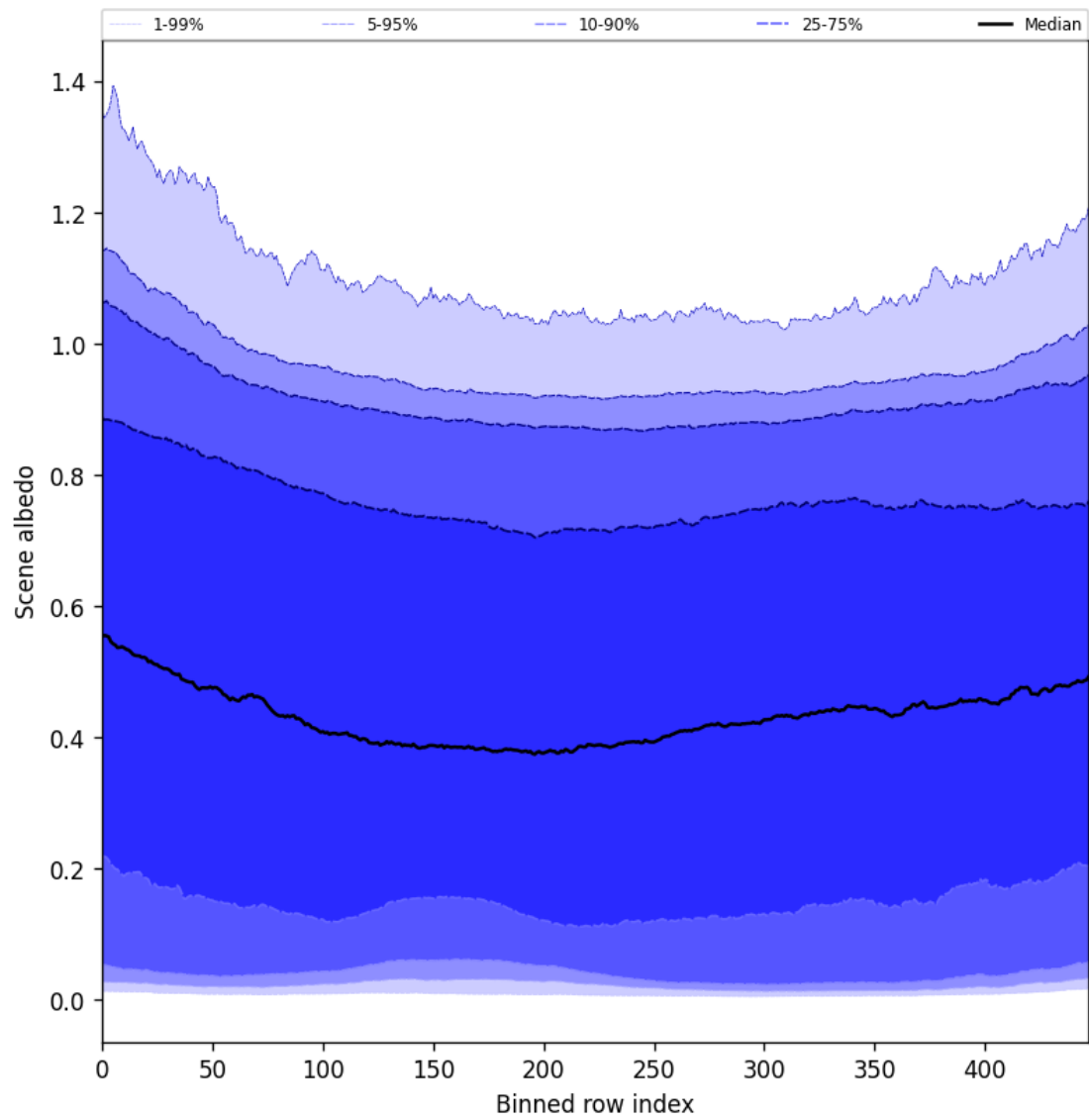
Figure 49: Along track statistics of “Scene albedo” for 2025-04-03 to 2025-04-04
