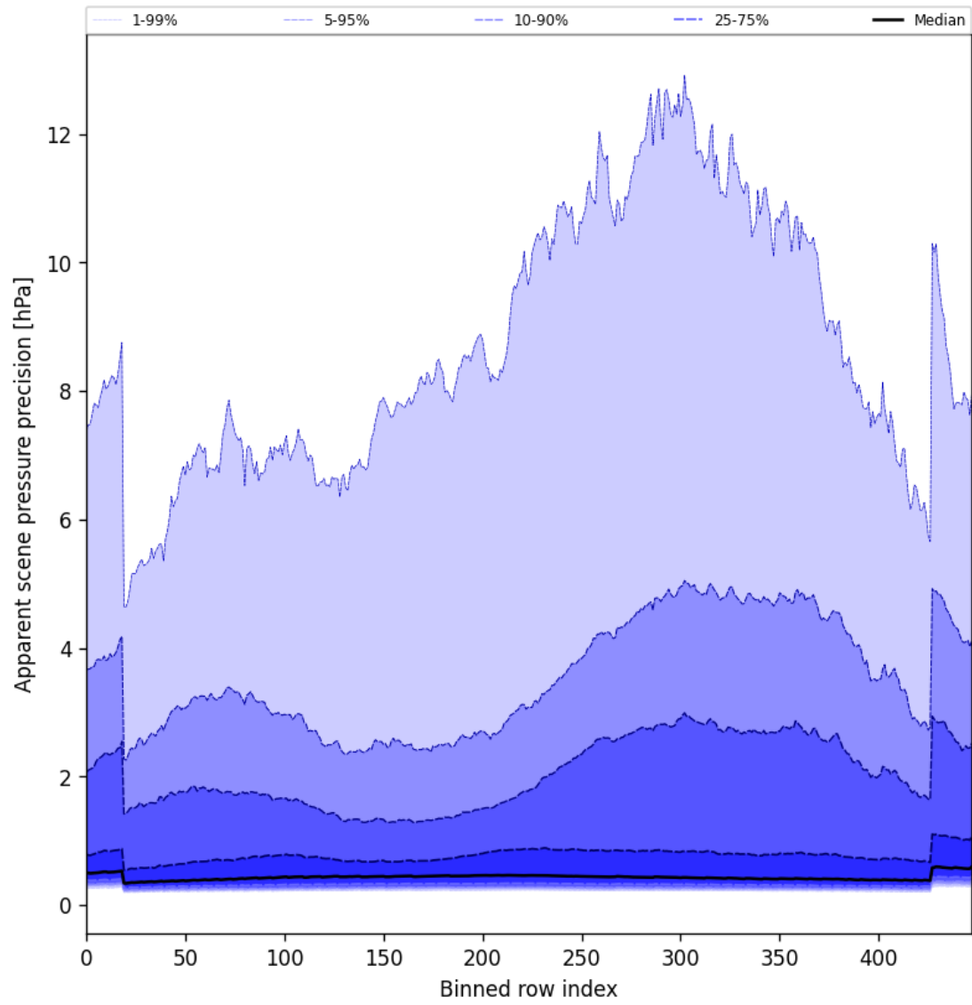
Figure 52: Along track statistics of “Apparent scene pressure precision” for 2025-04-03 to 2025-04-04
