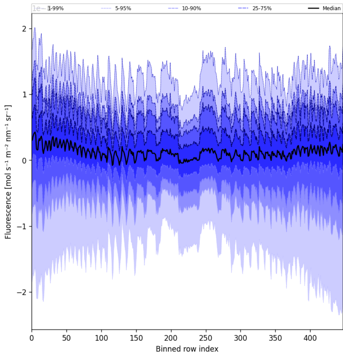
Figure 55: Along track statistics of “Fluorescence” for 2025-04-03 to 2025-04-04
