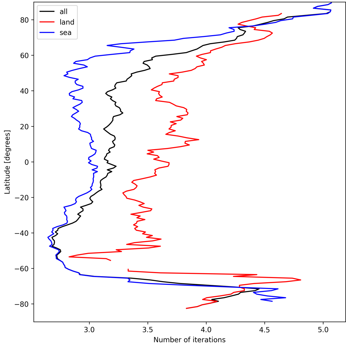
Figure 20: Zonal average of “Number of iterations” for 2025-04-03 to 2025-04-04.
