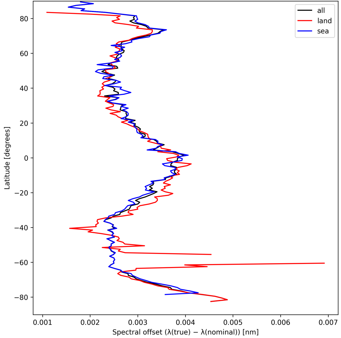
Figure 26: Zonal average of “Spectral offset ( \lambda_{\text{true}} - \lambda_{\text{nominal}} )” for 2025-04-03 to 2025-04-04.
