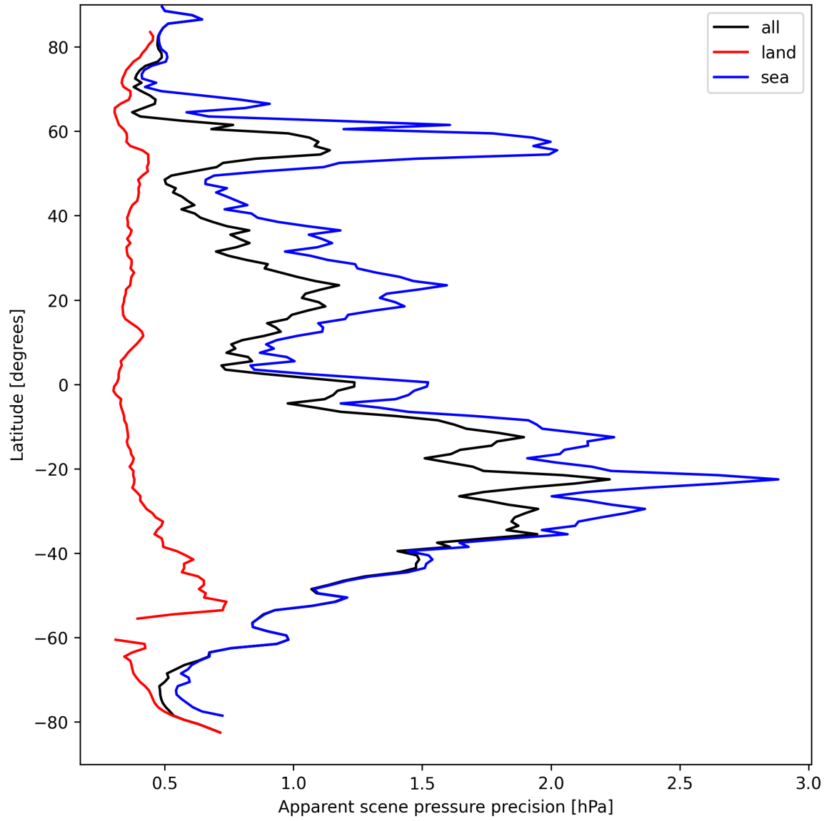
Figure 18: Zonal average of “Apparent scene pressure precision” for 2025-04-03 to 2025-04-04.
