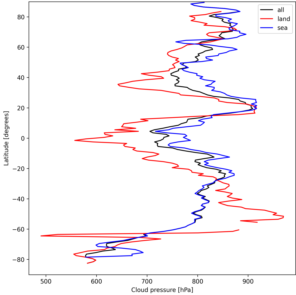
Figure 11: Zonal average of “Cloud pressure” for 2025-04-03 to 2025-04-04.
