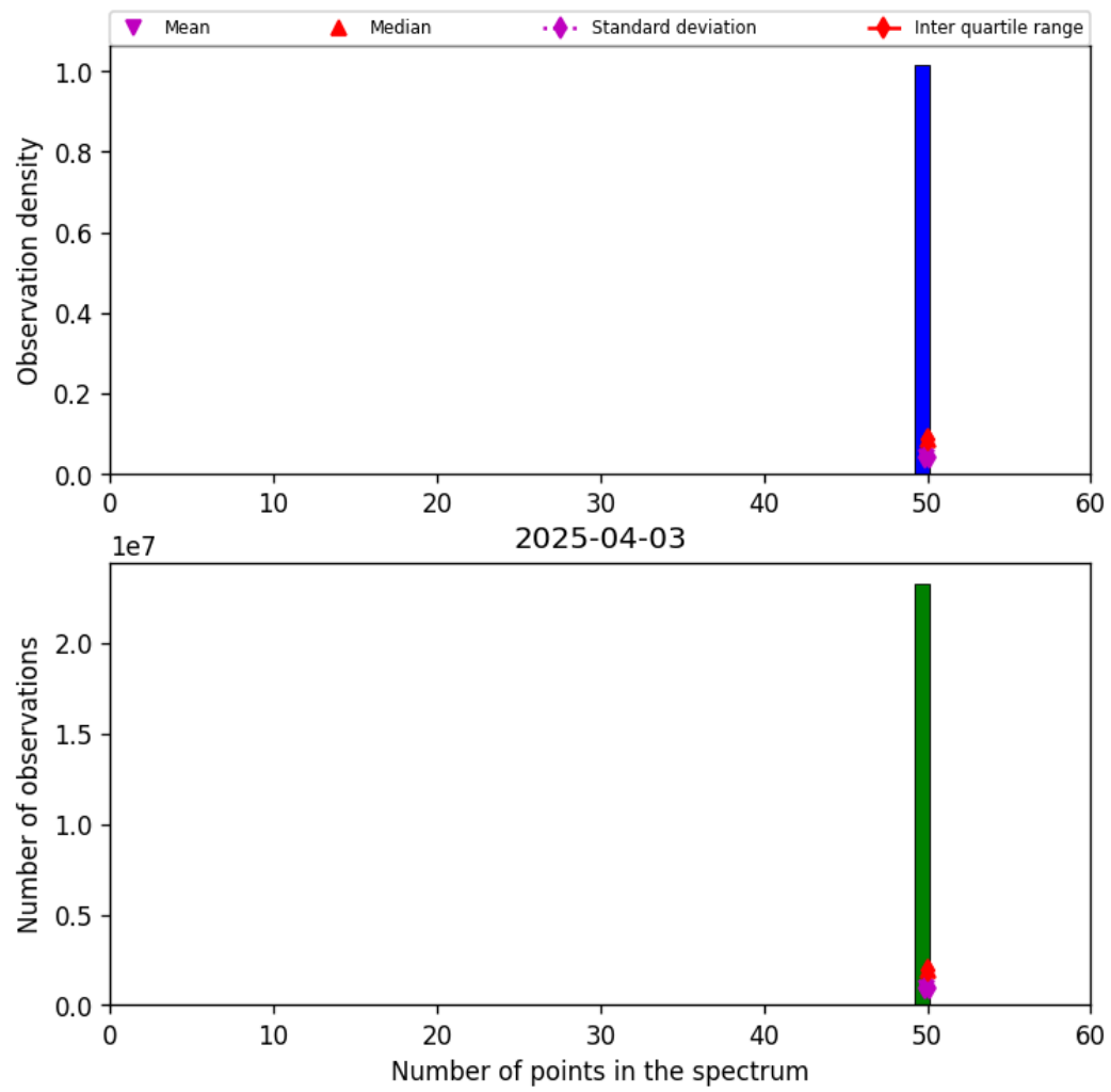
Figure 42: Histogram of “Number of points in the spectrum” for 2025-04-03 to 2025-04-04
