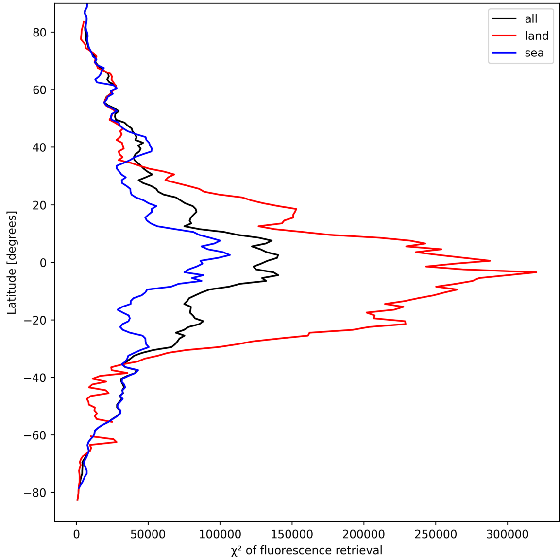
Figure 23: Zonal average of “ \chi^2 of fluorescence retrieval” for 2025-04-03 to 2025-04-04.
