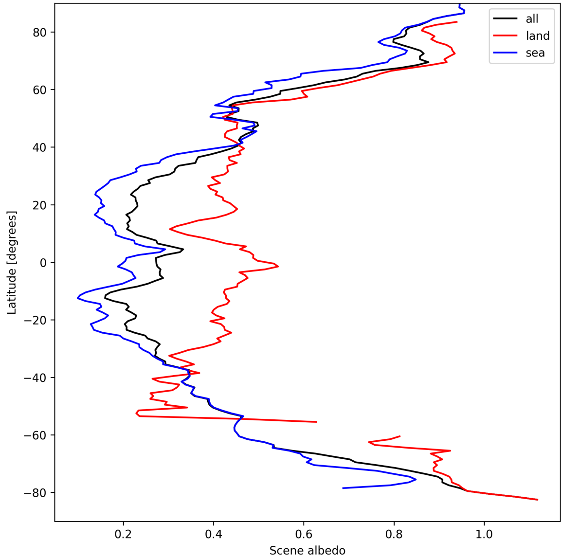
Figure 15: Zonal average of “Scene albedo” for 2025-04-03 to 2025-04-04.
