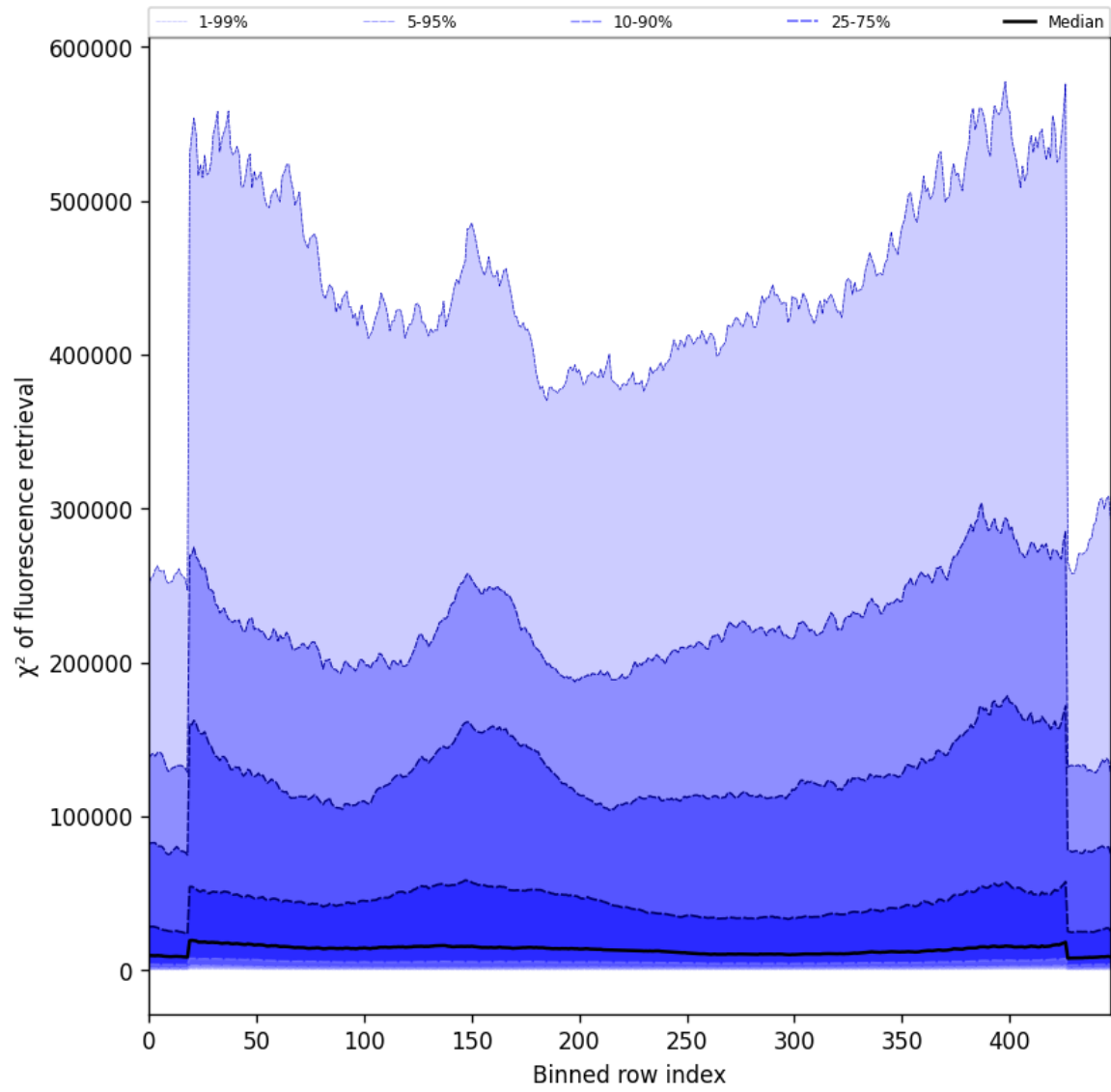
Figure 57: Along track statistics of “ \chi^2 of fluorescence retrieval” for 2025-04-03 to 2025-04-04
