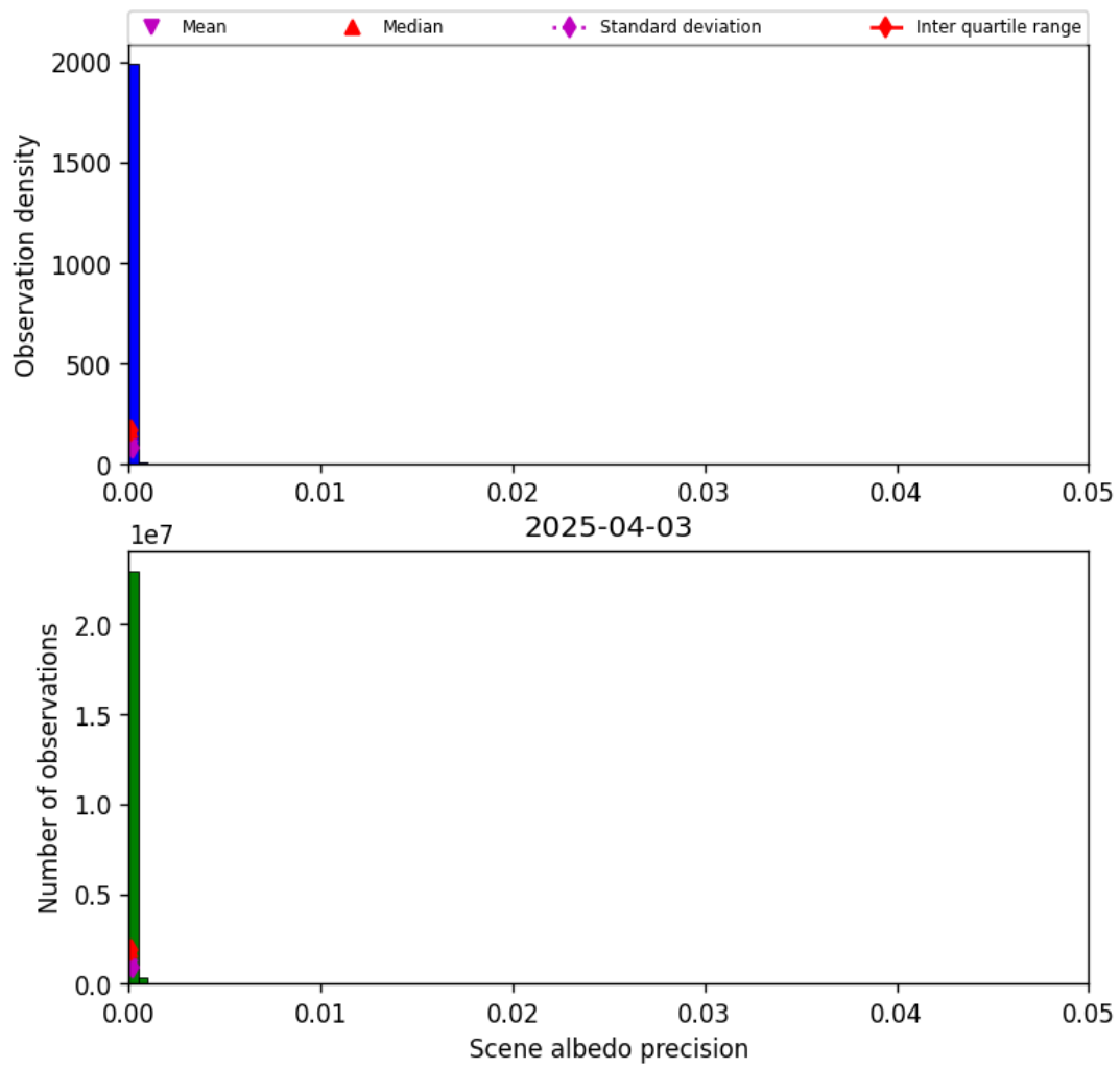
Figure 33: Histogram of “Scene albedo precision” for 2025-04-03 to 2025-04-04
