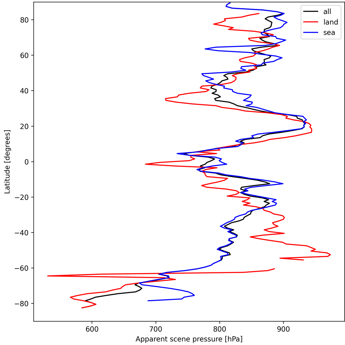
Figure 17: Zonal average of “Apparent scene pressure” for 2025-04-03 to 2025-04-04.
