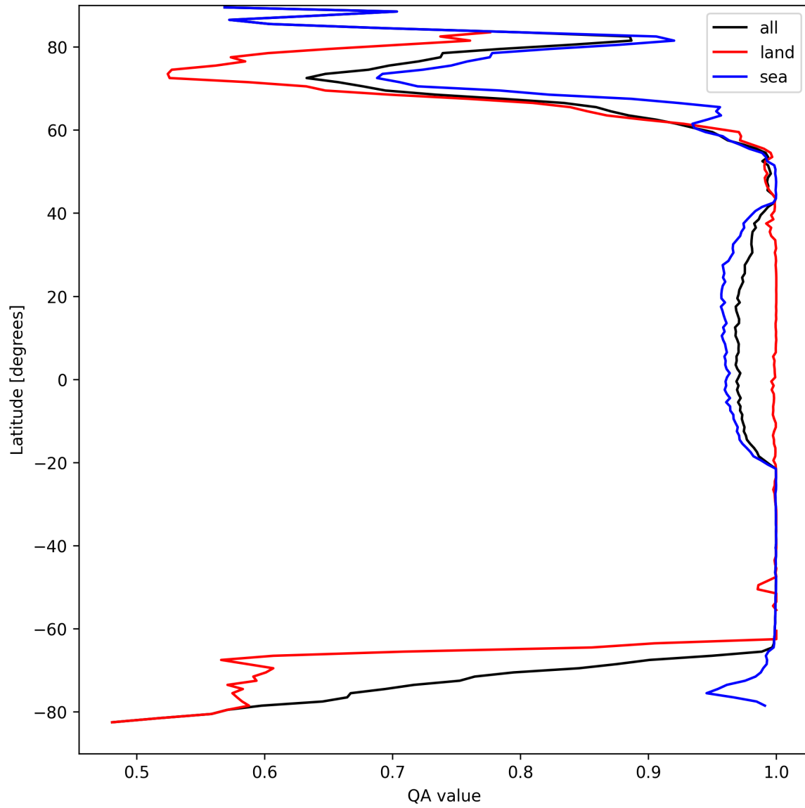
Figure 10: Zonal average of “QA value” for 2025-04-03 to 2025-04-04.
