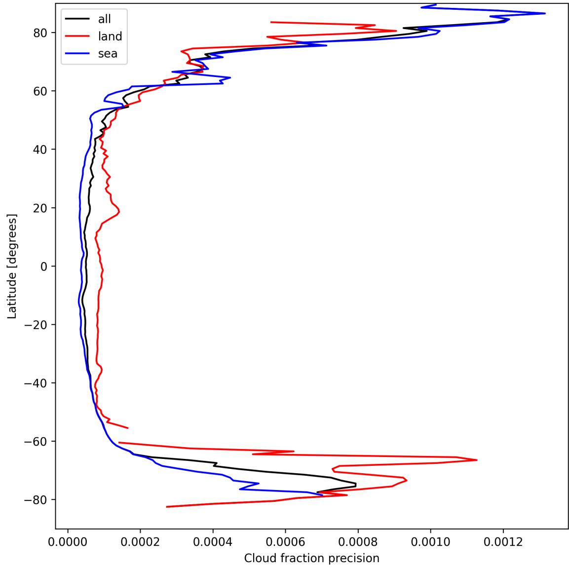
Figure 14: Zonal average of “Cloud fraction precision” for 2025-04-03 to 2025-04-04.
