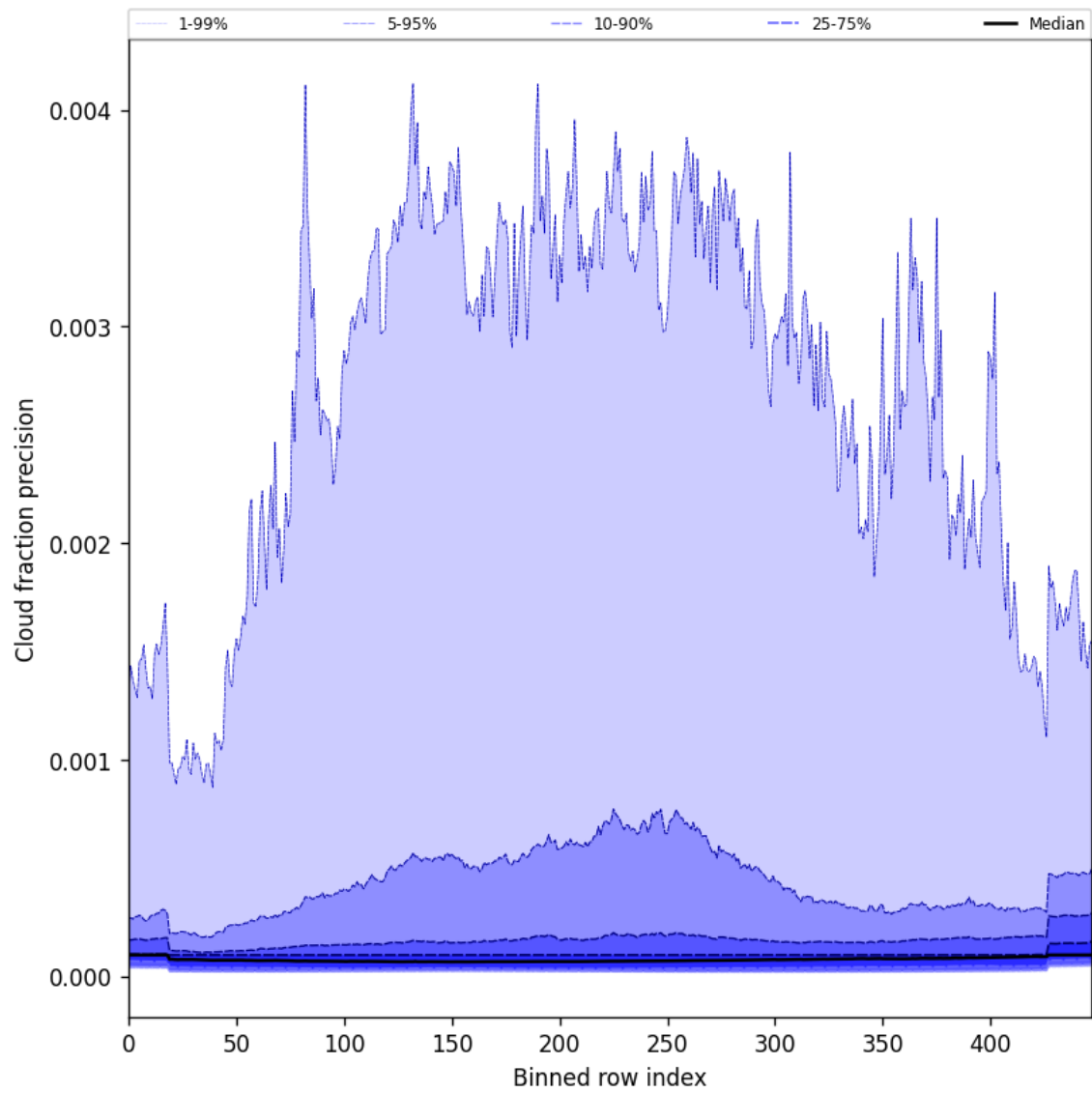
Figure 48: Along track statistics of “Cloud fraction precision” for 2025-04-03 to 2025-04-04
