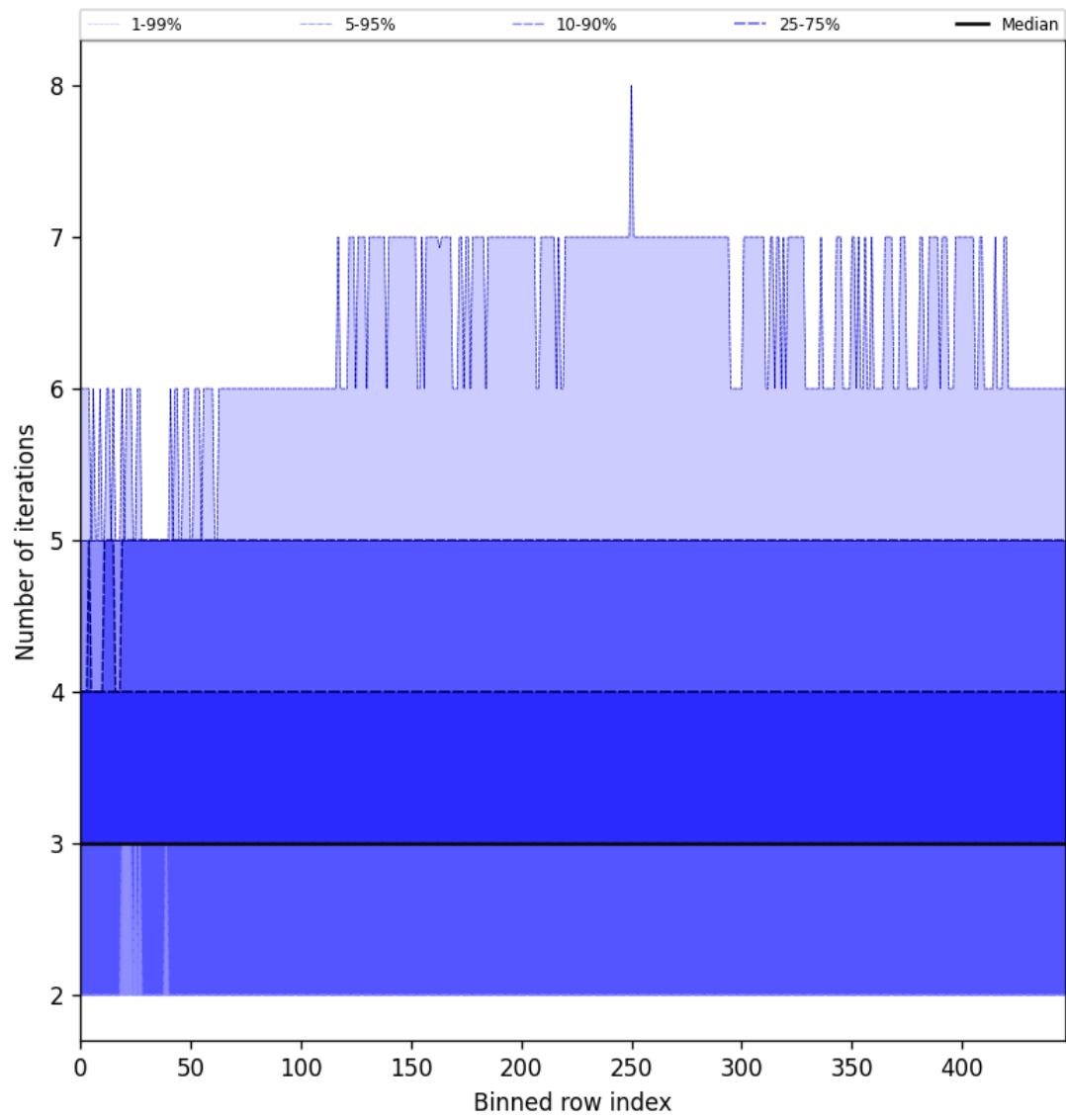
Figure 54: Along track statistics of “Number of iterations” for 2025-04-03 to 2025-04-04
