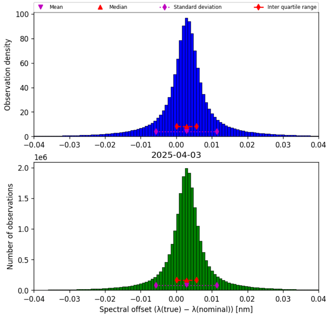
Figure 43: Histogram of “Spectral offset ( \lambda_{\text{true}} - \lambda_{\text{nominal}} )” for 2025-04-03 to 2025-04-04
