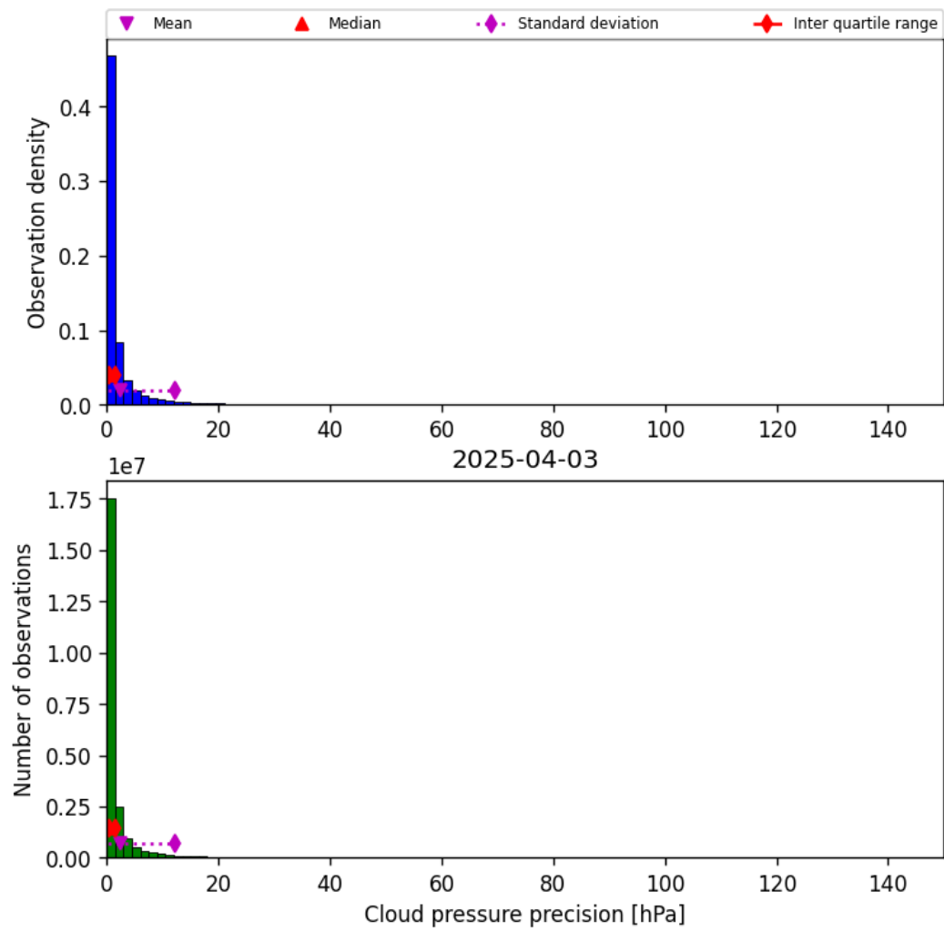
Figure 29: Histogram of “Cloud pressure precision” for 2025-04-03 to 2025-04-04
