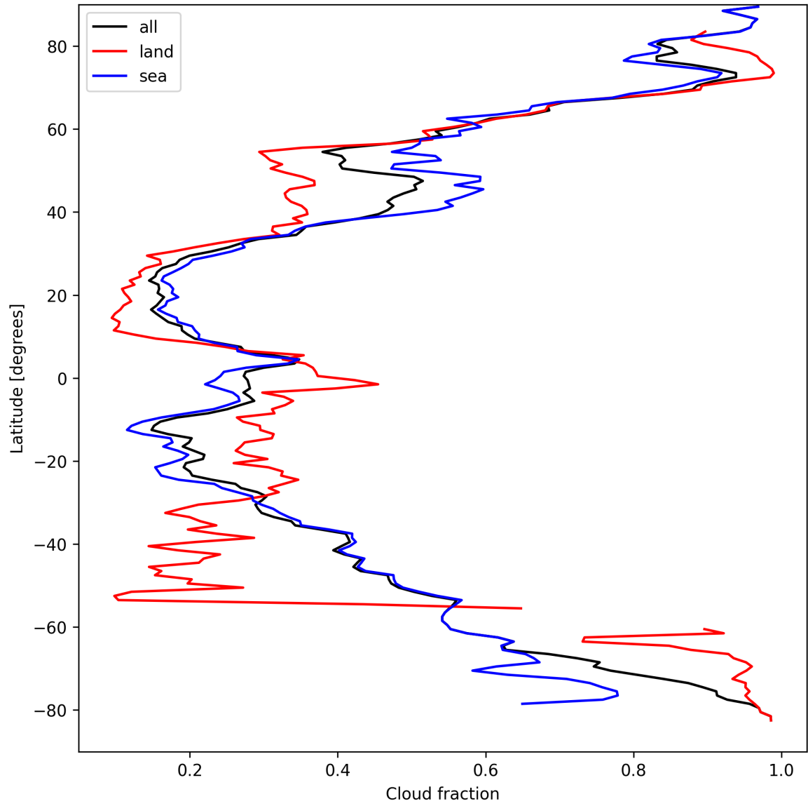
Figure 13: Zonal average of “Cloud fraction” for 2025-04-03 to 2025-04-04.
