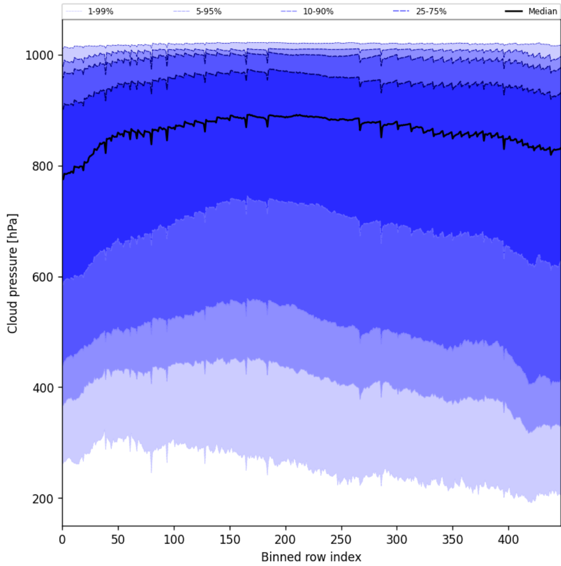
Figure 45: Along track statistics of “Cloud pressure” for 2025-04-03 to 2025-04-04
