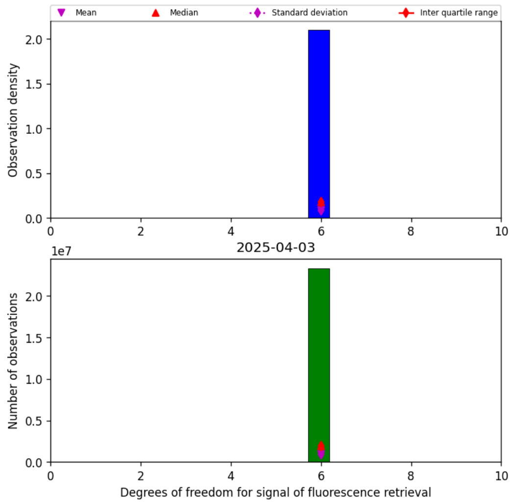
Figure 41: Histogram of “Degrees of freedom for signal of fluorescence retrieval” for 2025-04-03 to 2025-04-04
