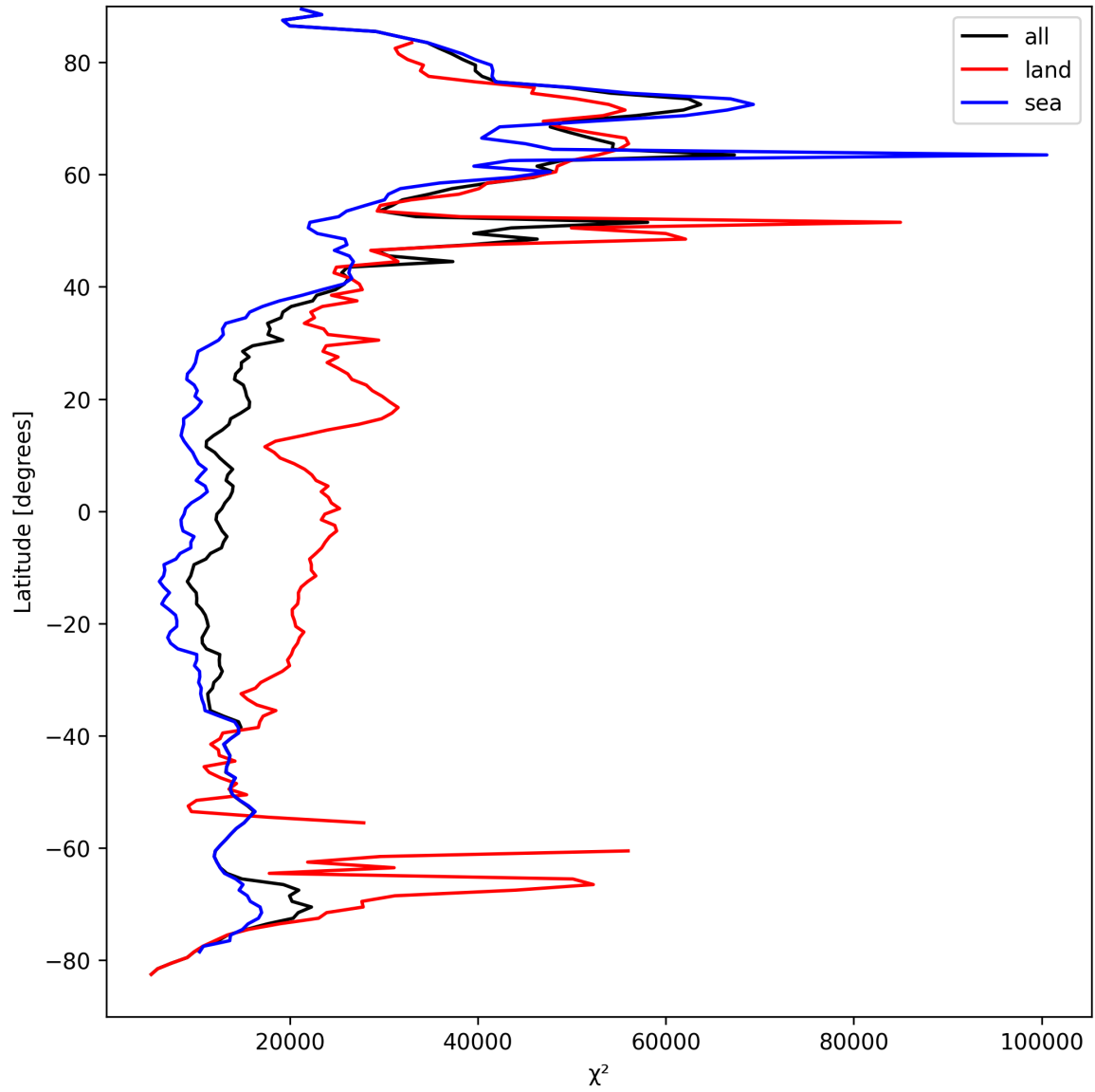
Figure 19: Zonal average of “ \chi^2 ” for 2025-04-03 to 2025-04-04.
