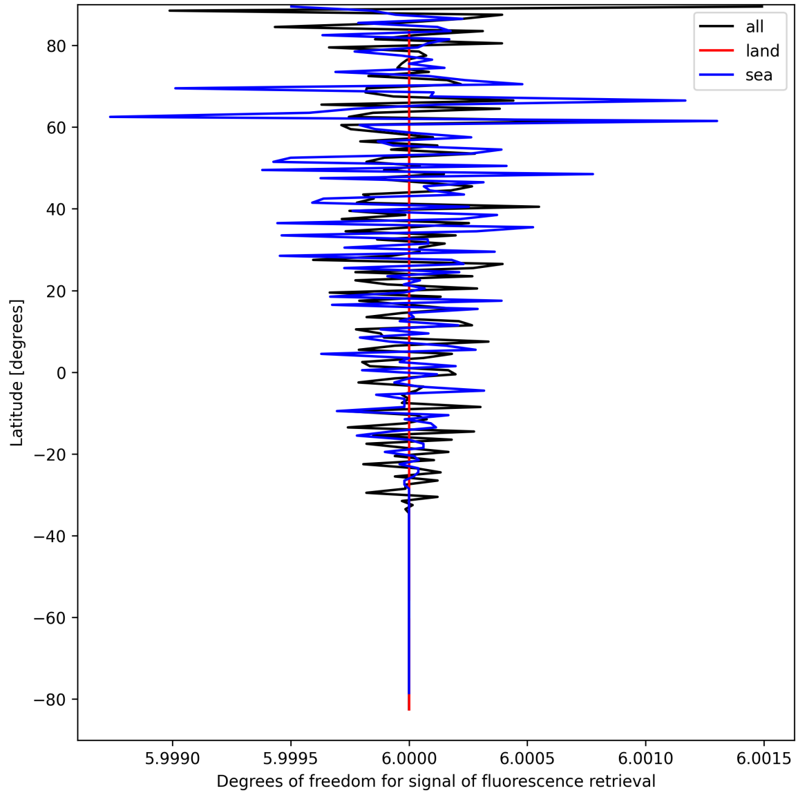
Figure 24: Zonal average of “Degrees of freedom for signal of fluorescence retrieval” for 2025-04-03 to 2025-04-04.
