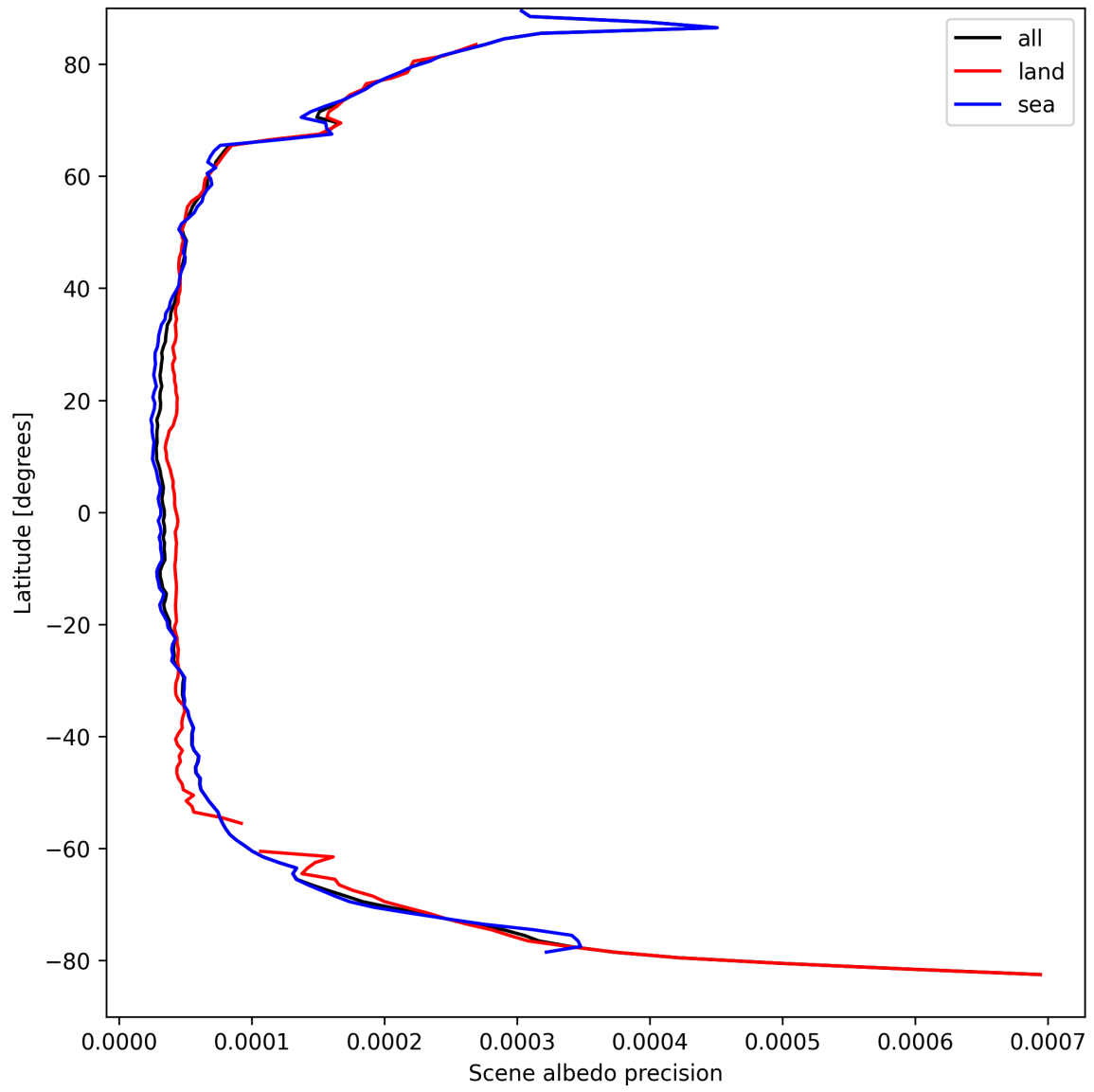
Figure 16: Zonal average of “Scene albedo precision” for 2025-04-03 to 2025-04-04.
