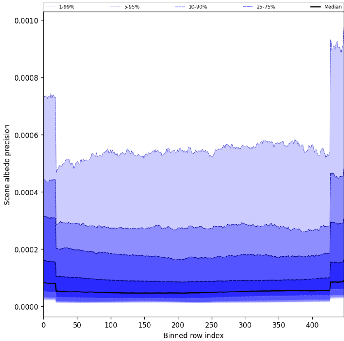
Figure 50: Along track statistics of “Scene albedo precision” for 2025-04-03 to 2025-04-04
