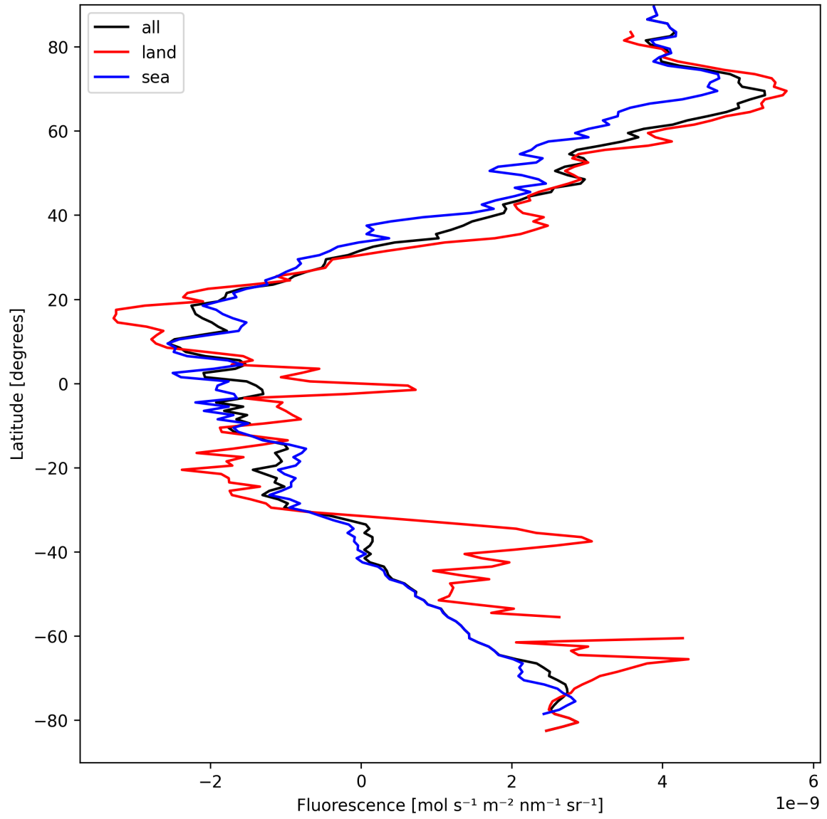
Figure 21: Zonal average of “Fluorescence” for 2025-04-03 to 2025-04-04.
