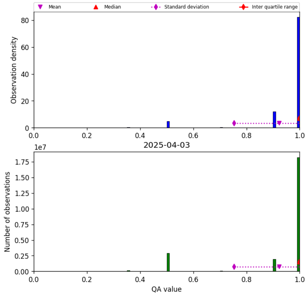
Figure 27: Histogram of “QA value” for 2025-04-03 to 2025-04-04
