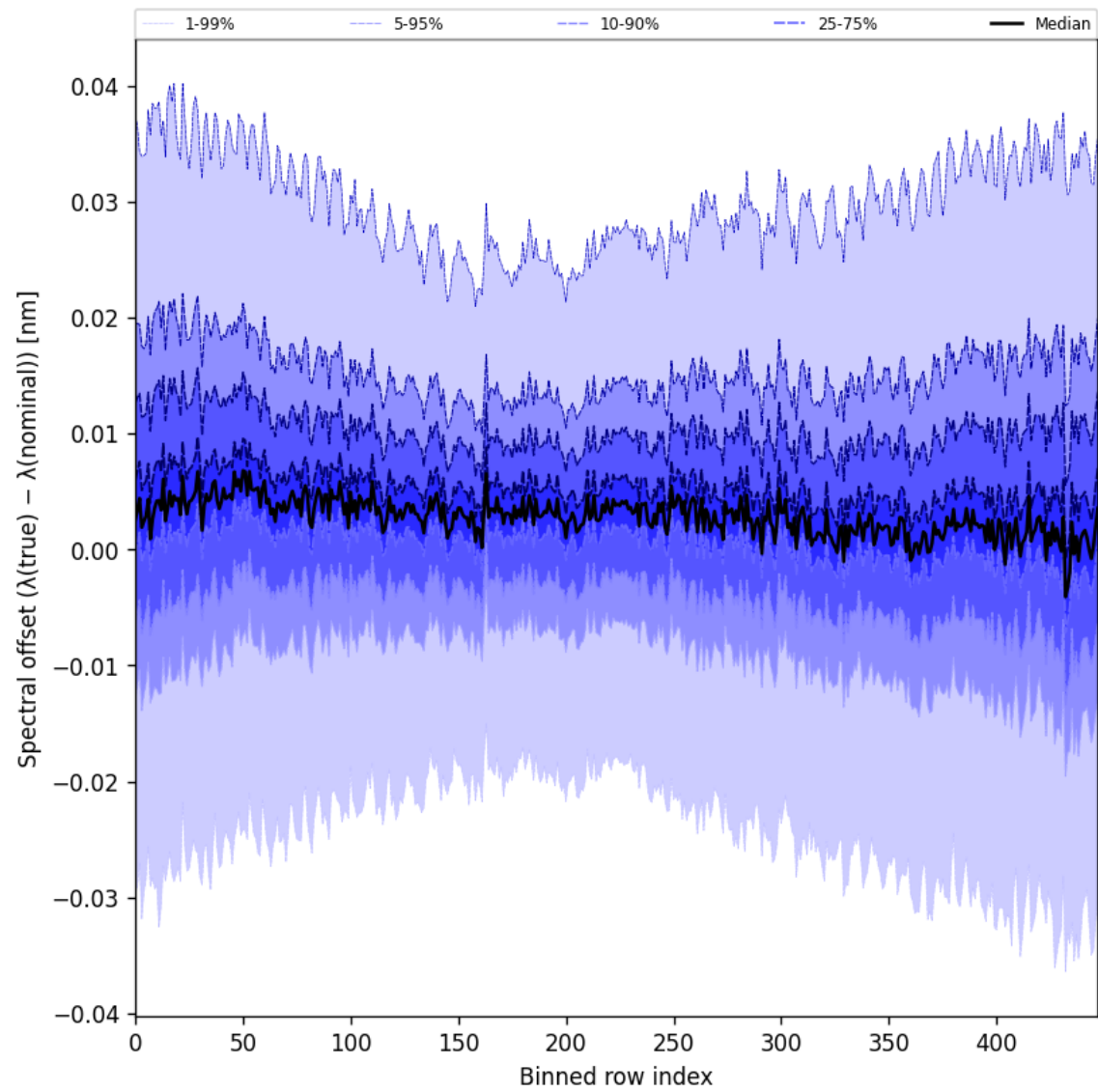
Figure 60: Along track statistics of “Spectral offset ( \lambda_{\text{true}} - \lambda_{\text{nominal}} )” for 2025-04-03 to 2025-04-04
