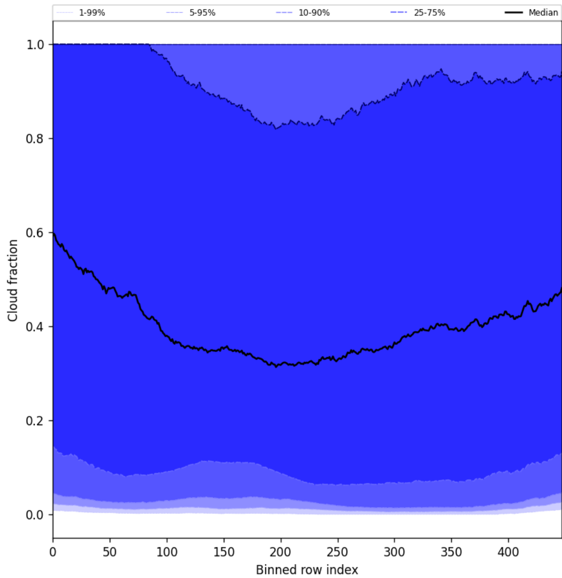
Figure 47: Along track statistics of “Cloud fraction” for 2025-04-03 to 2025-04-04
