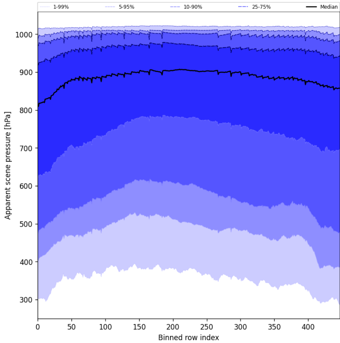
Figure 51: Along track statistics of “Apparent scene pressure” for 2025-04-03 to 2025-04-04
