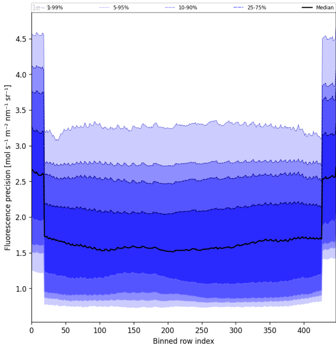
Figure 56: Along track statistics of “Fluorescence precision” for 2025-04-03 to 2025-04-04
