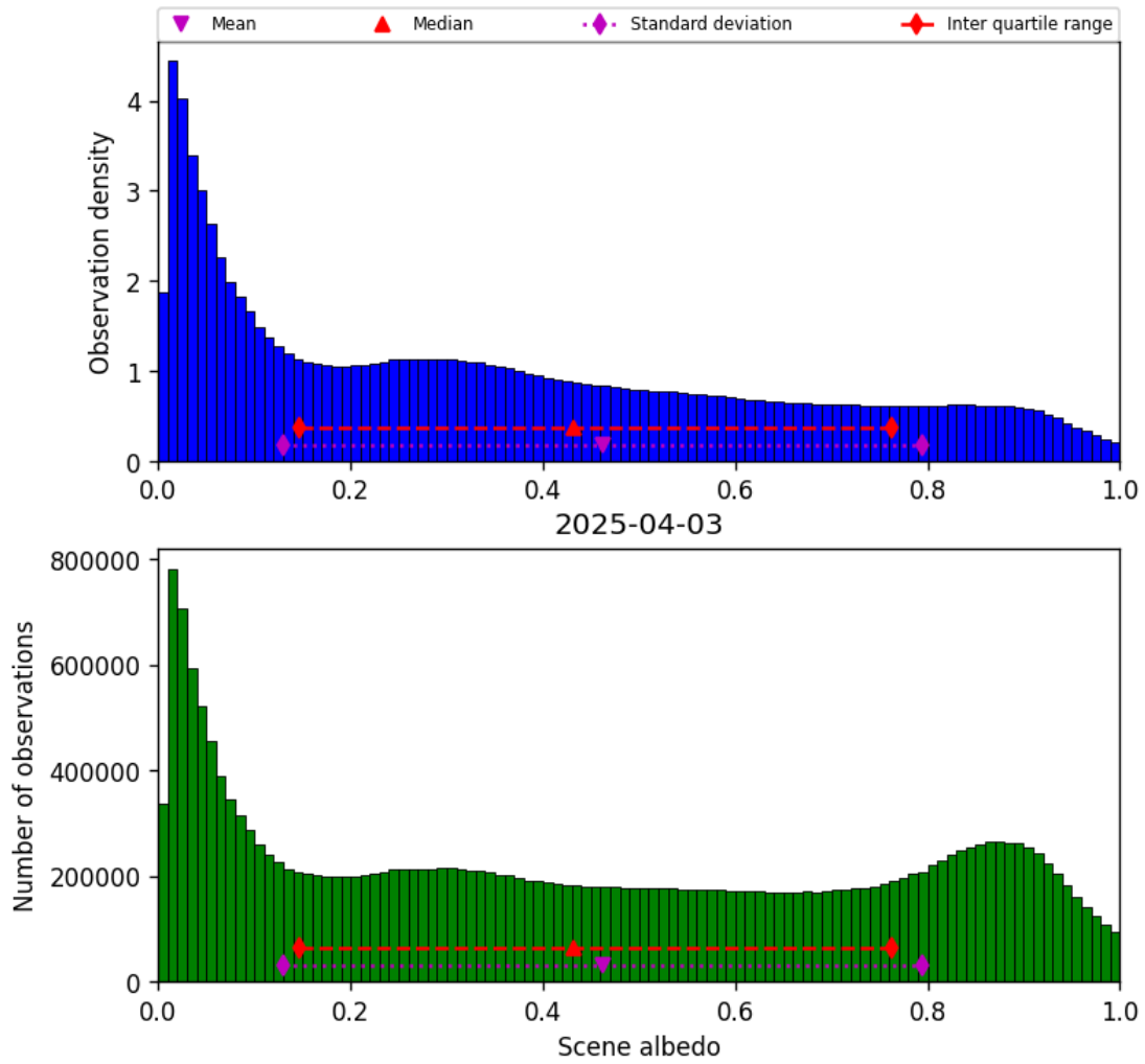
Figure 32: Histogram of “Scene albedo” for 2025-04-03 to 2025-04-04
