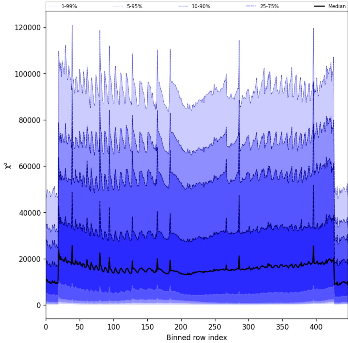
Figure 53: Along track statistics of “ \chi^2 ” for 2025-04-03 to 2025-04-04
