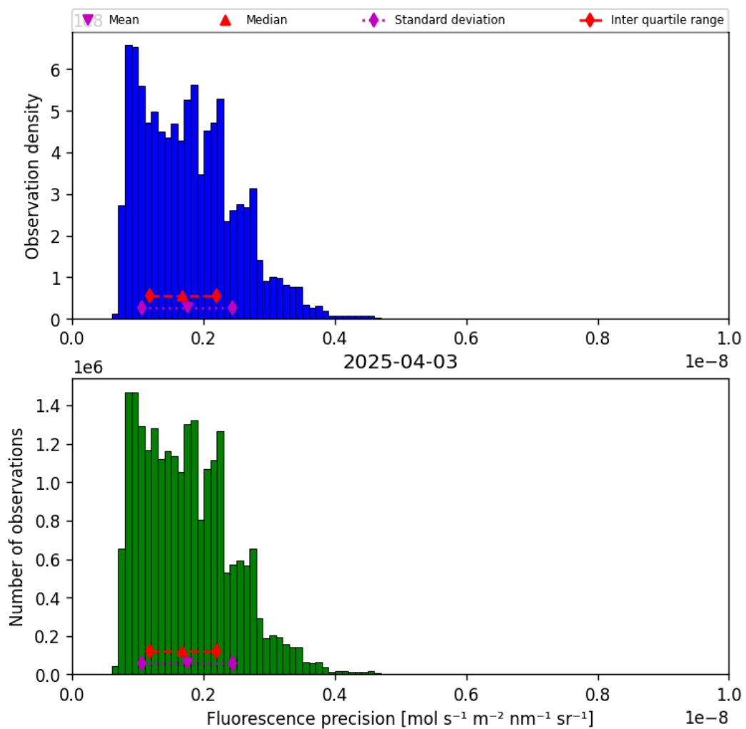
Figure 39: Histogram of “Fluorescence precision” for 2025-04-03 to 2025-04-04
