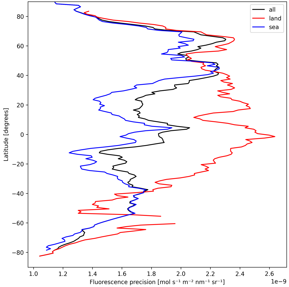
Figure 22: Zonal average of “Fluorescence precision” for 2025-04-03 to 2025-04-04.
