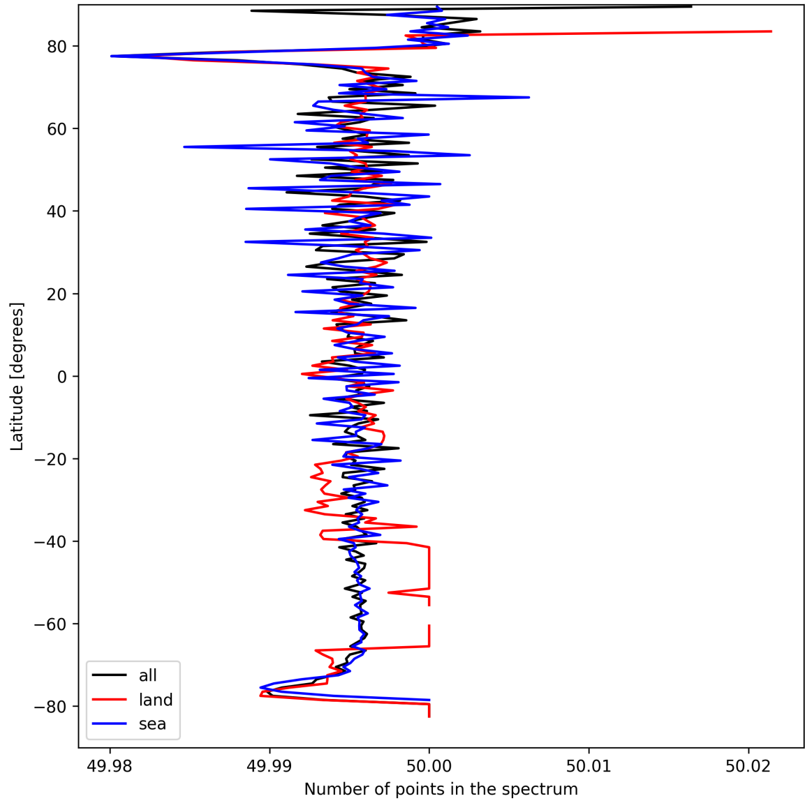
Figure 25: Zonal average of “Number of points in the spectrum” for 2025-04-03 to 2025-04-04.
