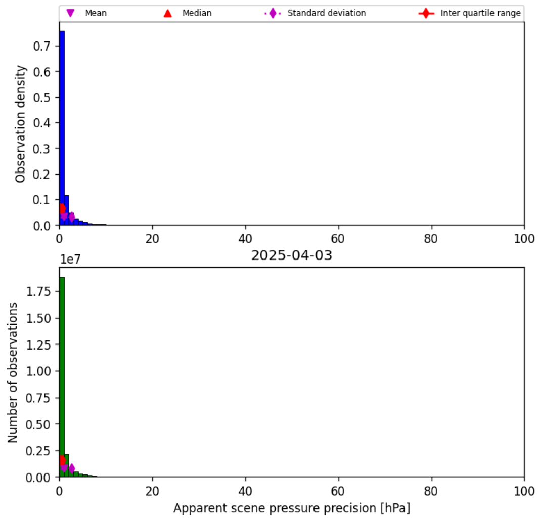
Figure 35: Histogram of “Apparent scene pressure precision” for 2025-04-03 to 2025-04-04
