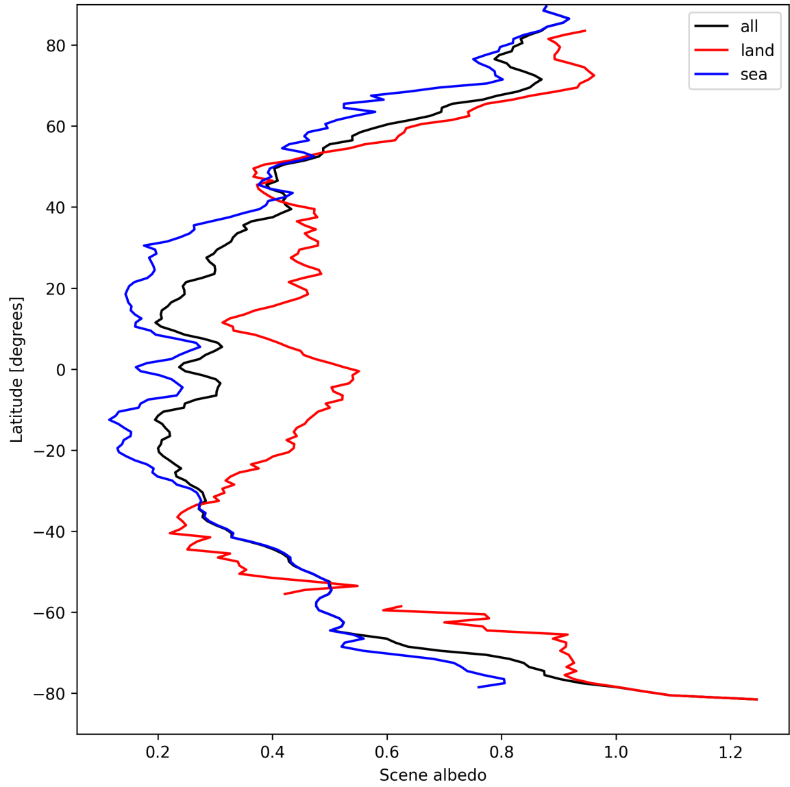
Figure 15: Zonal average of “Scene albedo” for 2025-04-05 to 2025-04-06.
