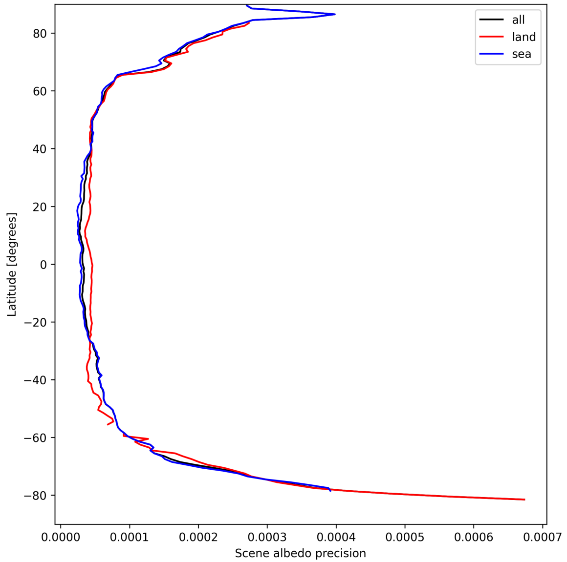
Figure 16: Zonal average of “Scene albedo precision” for 2025-04-05 to 2025-04-06.
