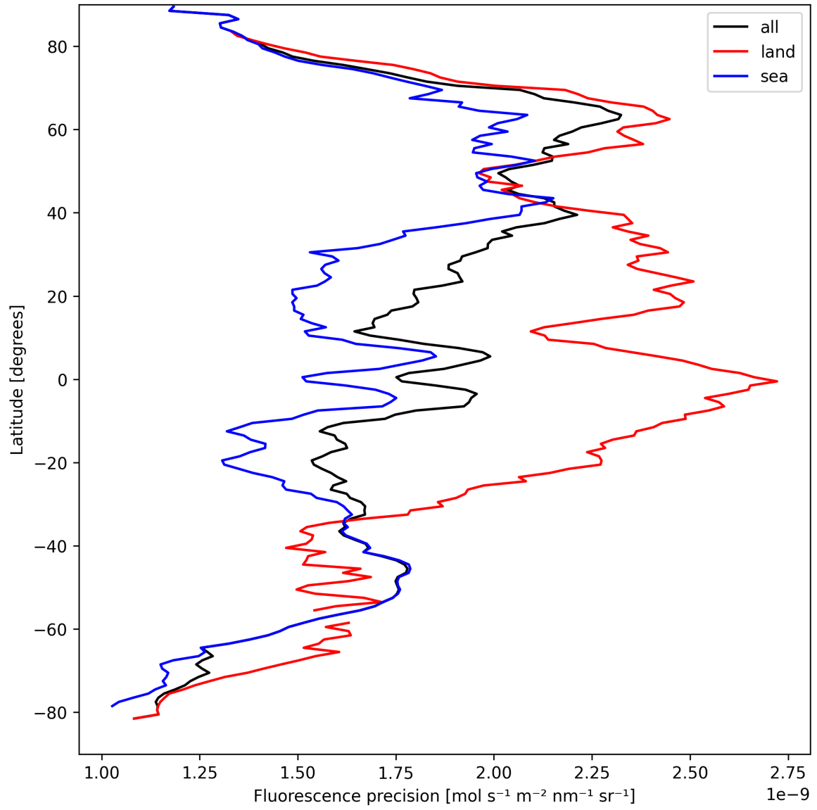
Figure 22: Zonal average of “Fluorescence precision” for 2025-04-05 to 2025-04-06.
