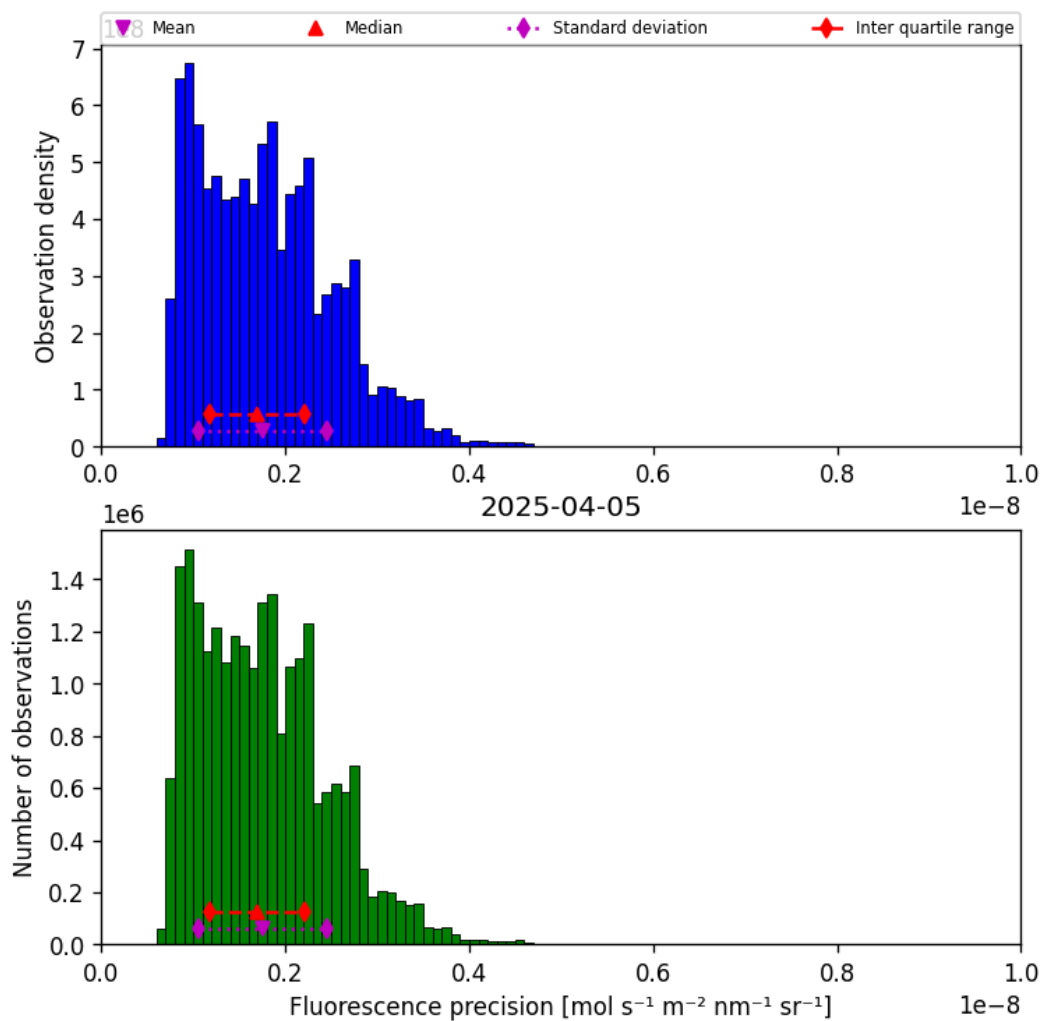
Figure 39: Histogram of “Fluorescence precision” for 2025-04-05 to 2025-04-06
