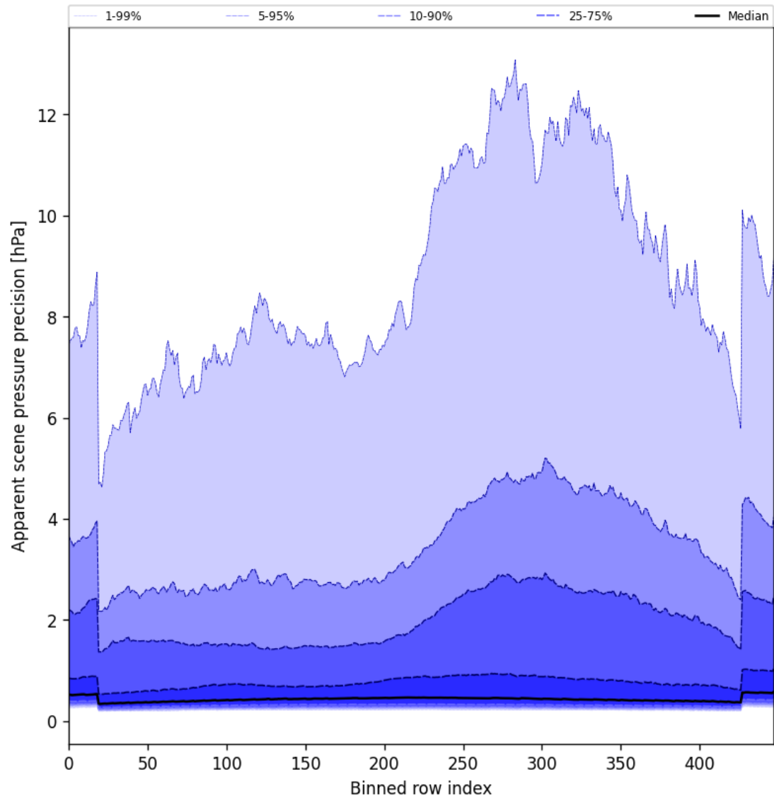
Figure 52: Along track statistics of “Apparent scene pressure precision” for 2025-04-05 to 2025-04-06
