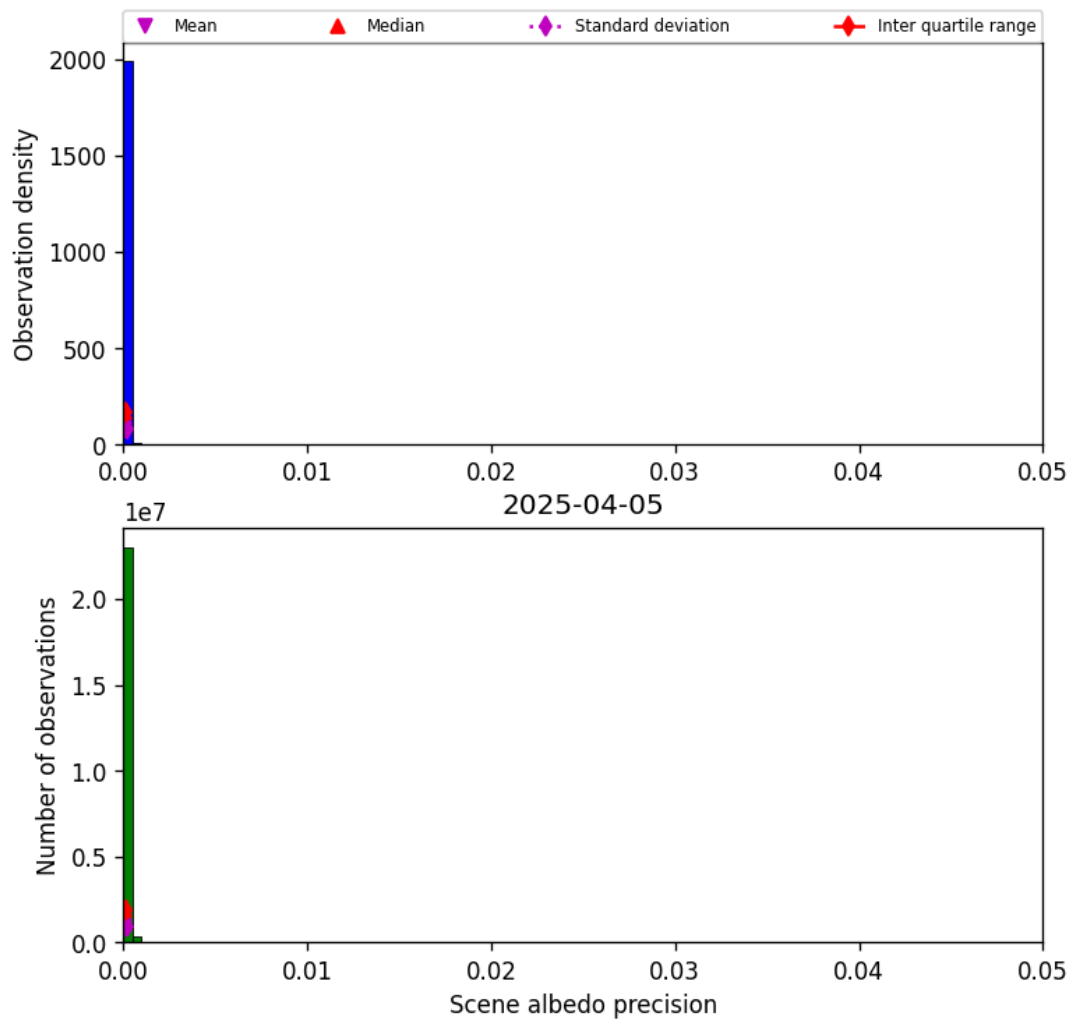
Figure 33: Histogram of “Scene albedo precision” for 2025-04-05 to 2025-04-06
