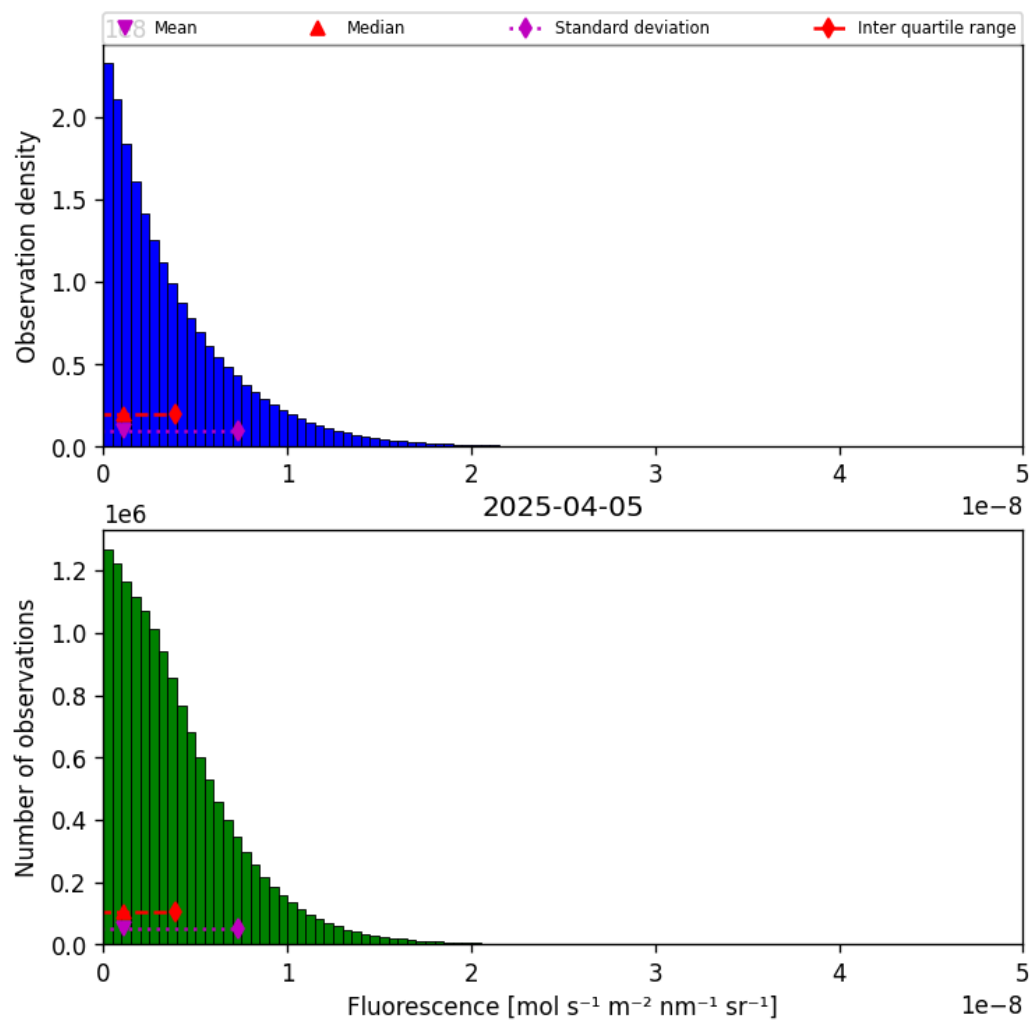
Figure 38: Histogram of “Fluorescence” for 2025-04-05 to 2025-04-06
