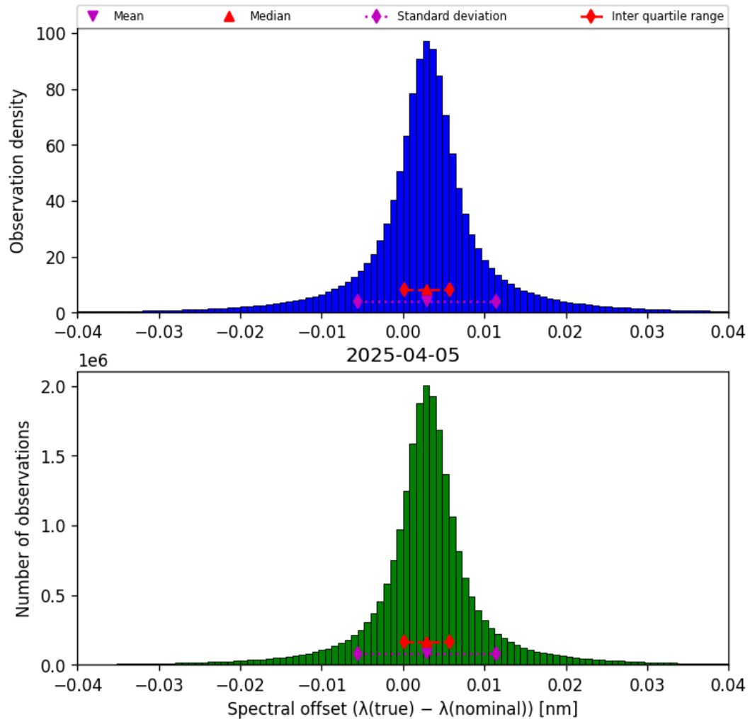
Figure 43: Histogram of “Spectral offset ( \lambda_{\text{true}} - \lambda_{\text{nominal}} )” for 2025-04-05 to 2025-04-06
