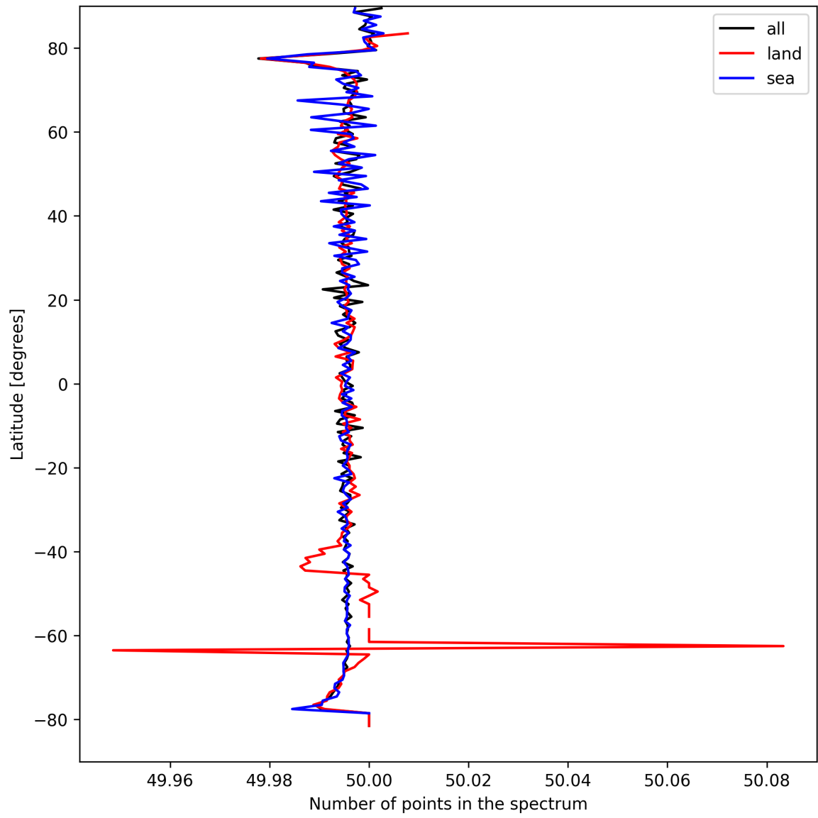
Figure 25: Zonal average of “Number of points in the spectrum” for 2025-04-05 to 2025-04-06.
