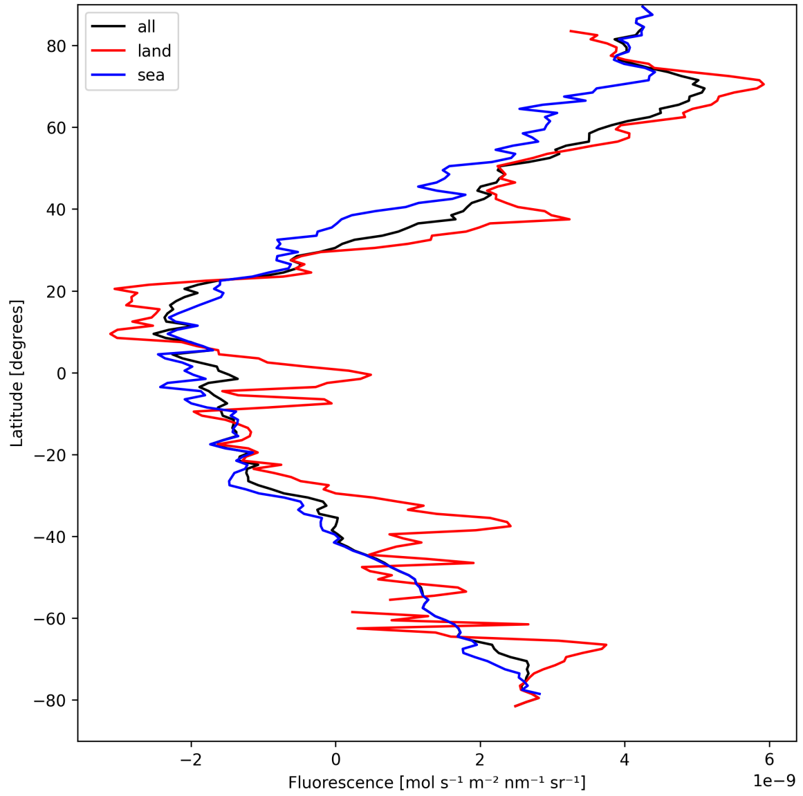
Figure 21: Zonal average of “Fluorescence” for 2025-04-05 to 2025-04-06.
