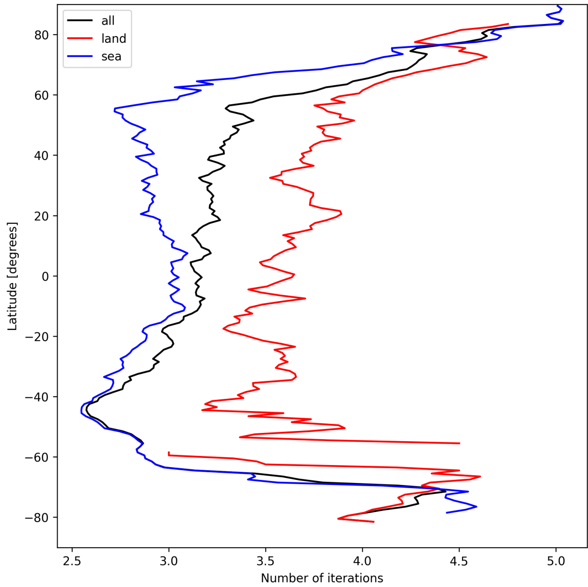
Figure 20: Zonal average of “Number of iterations” for 2025-04-05 to 2025-04-06.
