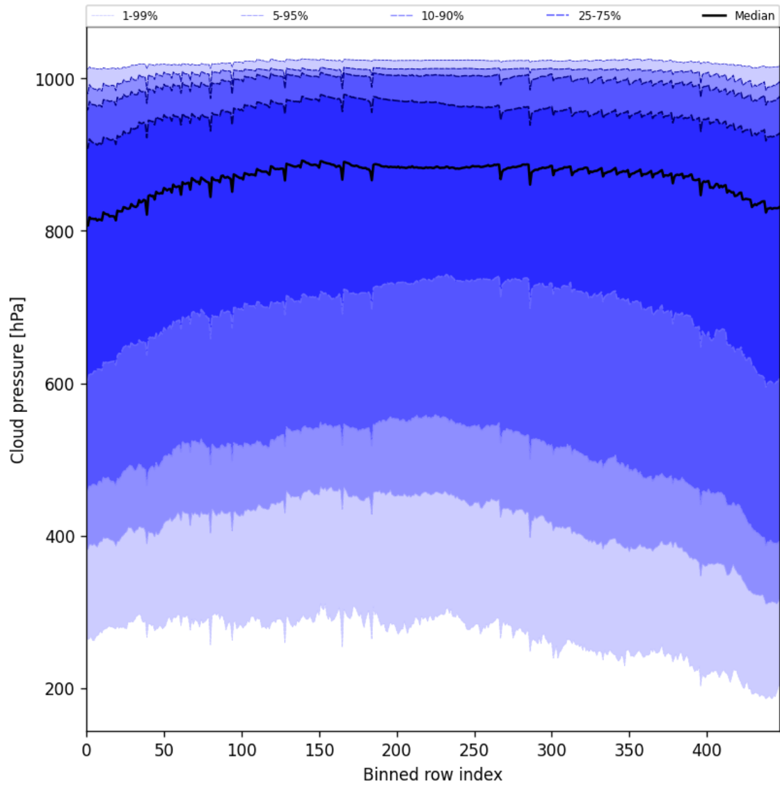
Figure 45: Along track statistics of “Cloud pressure” for 2025-04-05 to 2025-04-06
