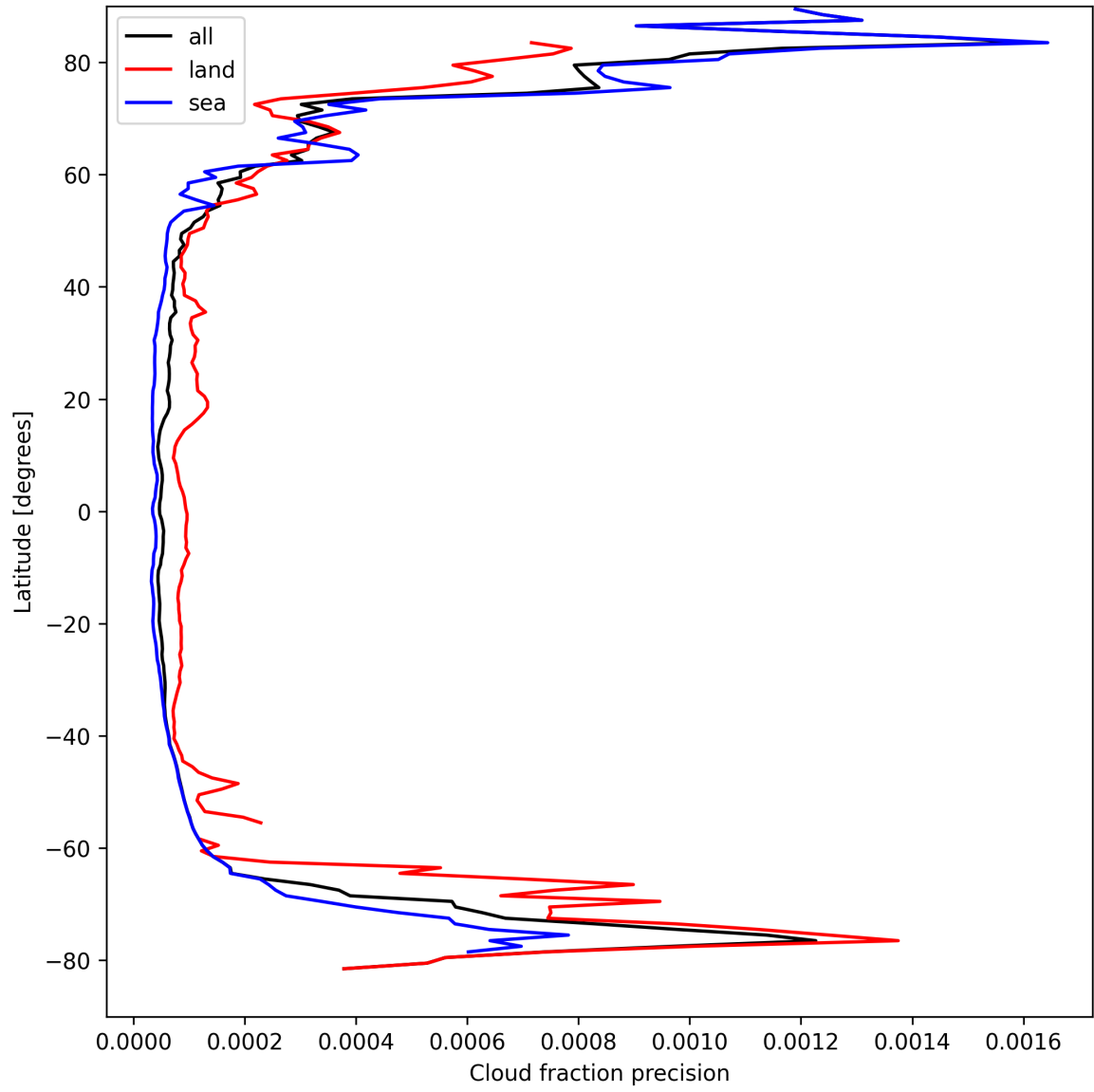
Figure 14: Zonal average of “Cloud fraction precision” for 2025-04-05 to 2025-04-06.
