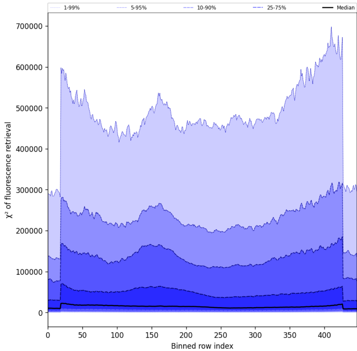
Figure 57: Along track statistics of “ \chi^2 of fluorescence retrieval” for 2025-04-05 to 2025-04-06
