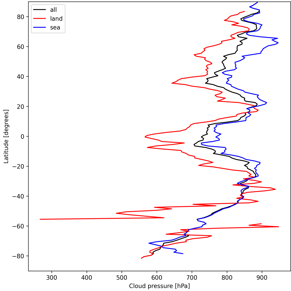
Figure 11: Zonal average of “Cloud pressure” for 2025-04-05 to 2025-04-06.
