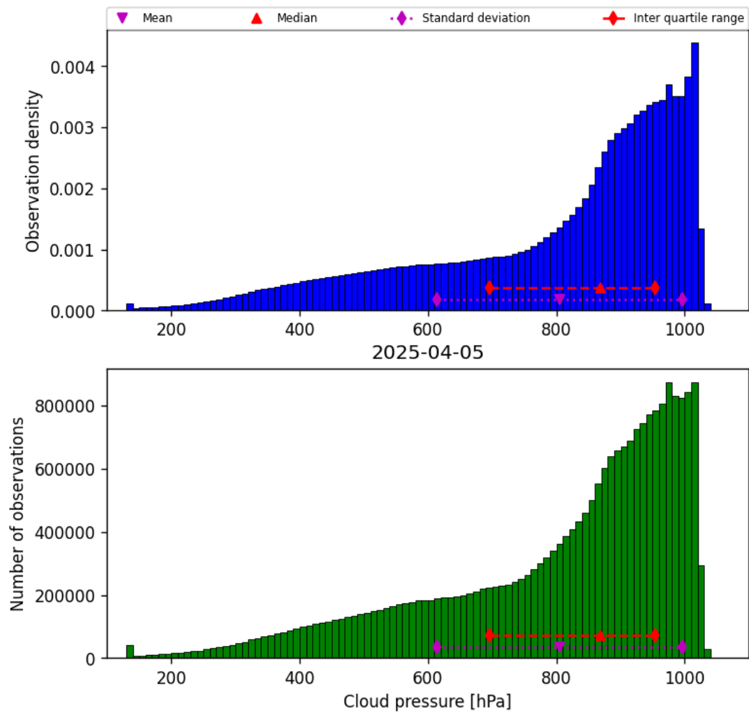
Figure 28: Histogram of “Cloud pressure” for 2025-04-05 to 2025-04-06
