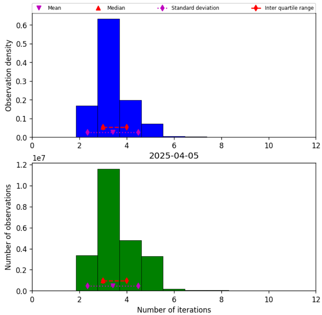
Figure 37: Histogram of “Number of iterations” for 2025-04-05 to 2025-04-06
