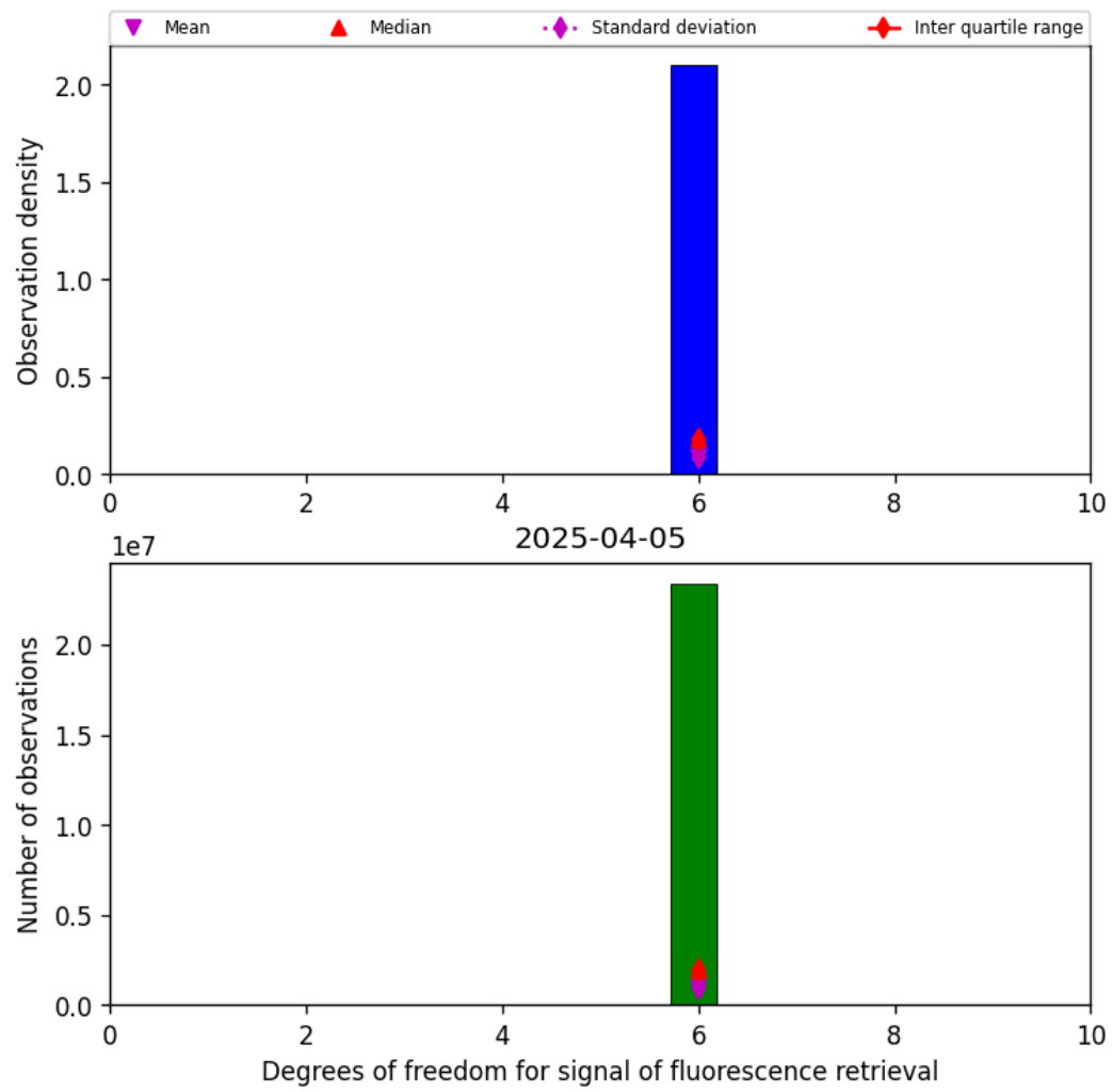
Figure 41: Histogram of “Degrees of freedom for signal of fluorescence retrieval” for 2025-04-05 to 2025-04-06
