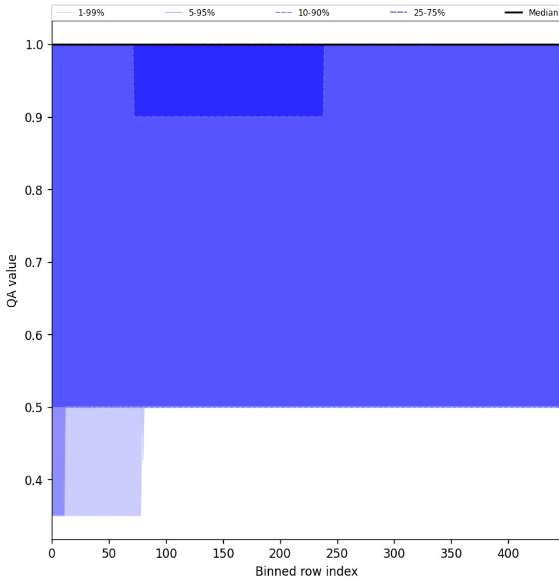
Figure 44: Along track statistics of “QA value” for 2025-04-05 to 2025-04-06
