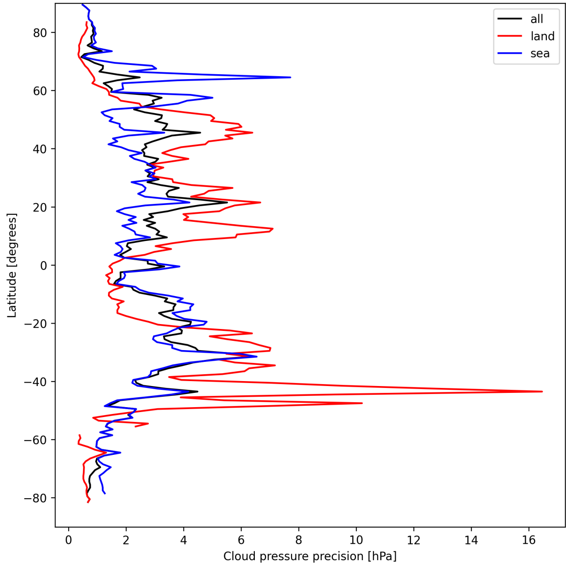
Figure 12: Zonal average of “Cloud pressure precision” for 2025-04-05 to 2025-04-06.
