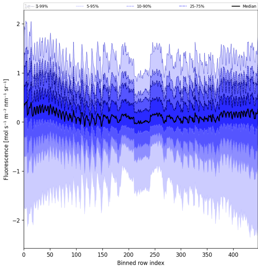
Figure 55: Along track statistics of “Fluorescence” for 2025-04-05 to 2025-04-06
