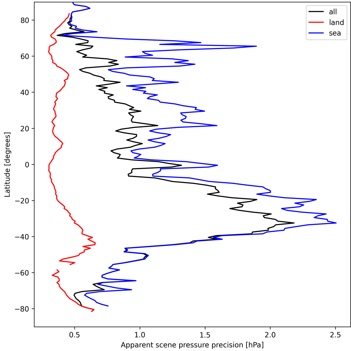
Figure 18: Zonal average of “Apparent scene pressure precision” for 2025-04-05 to 2025-04-06.
