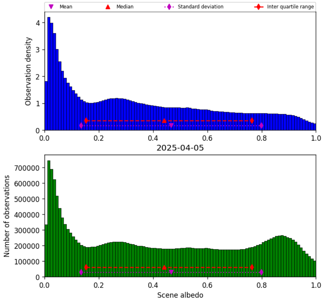
Figure 32: Histogram of “Scene albedo” for 2025-04-05 to 2025-04-06
