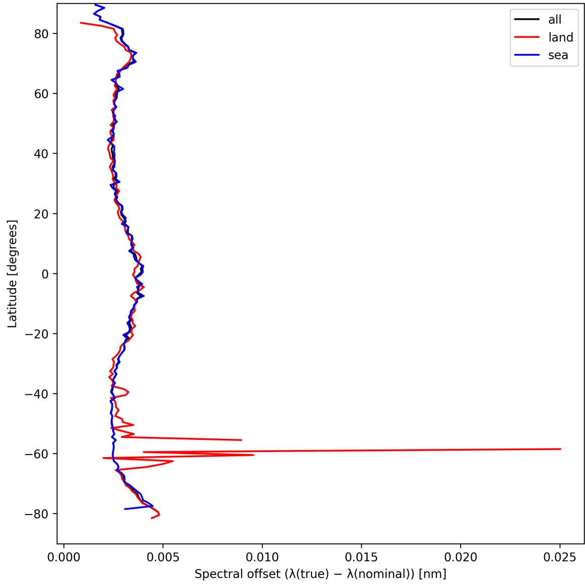
Figure 26: Zonal average of “Spectral offset ( \lambda_{\text{true}} - \lambda_{\text{nominal}} )” for 2025-04-05 to 2025-04-06.
