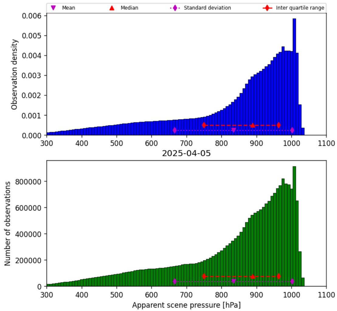
Figure 34: Histogram of “Apparent scene pressure” for 2025-04-05 to 2025-04-06
