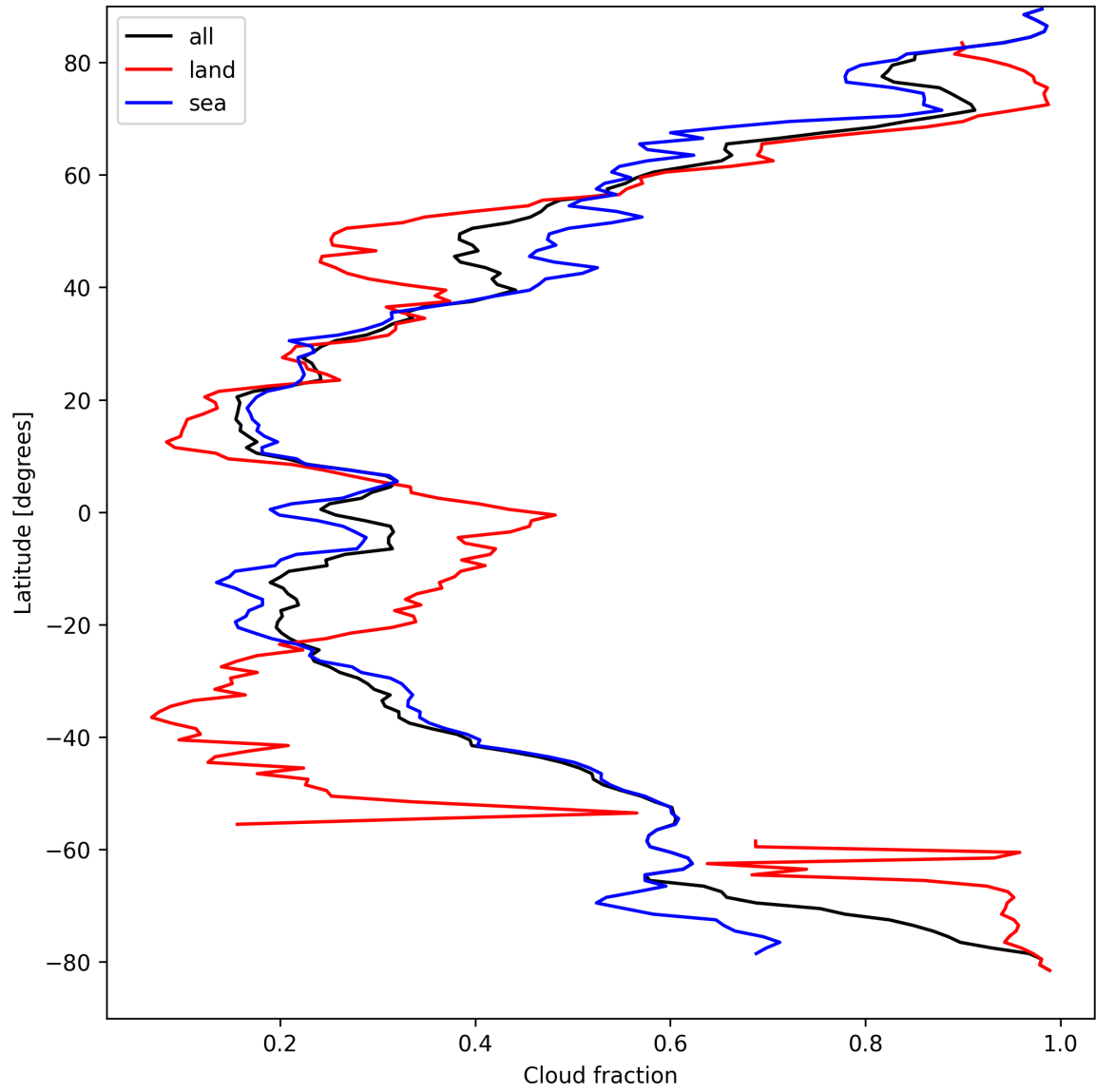
Figure 13: Zonal average of “Cloud fraction” for 2025-04-05 to 2025-04-06.
