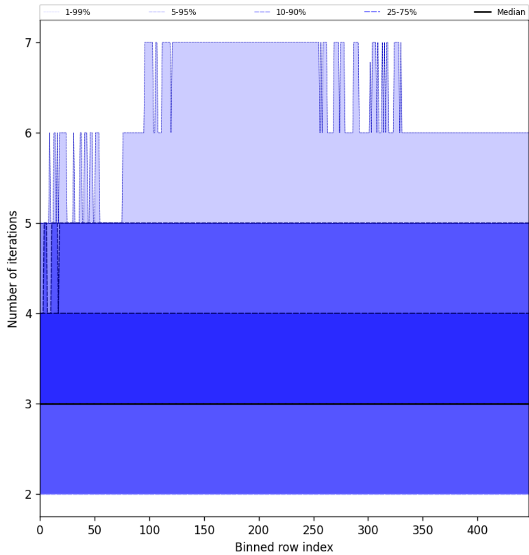
Figure 54: Along track statistics of “Number of iterations” for 2025-04-05 to 2025-04-06
