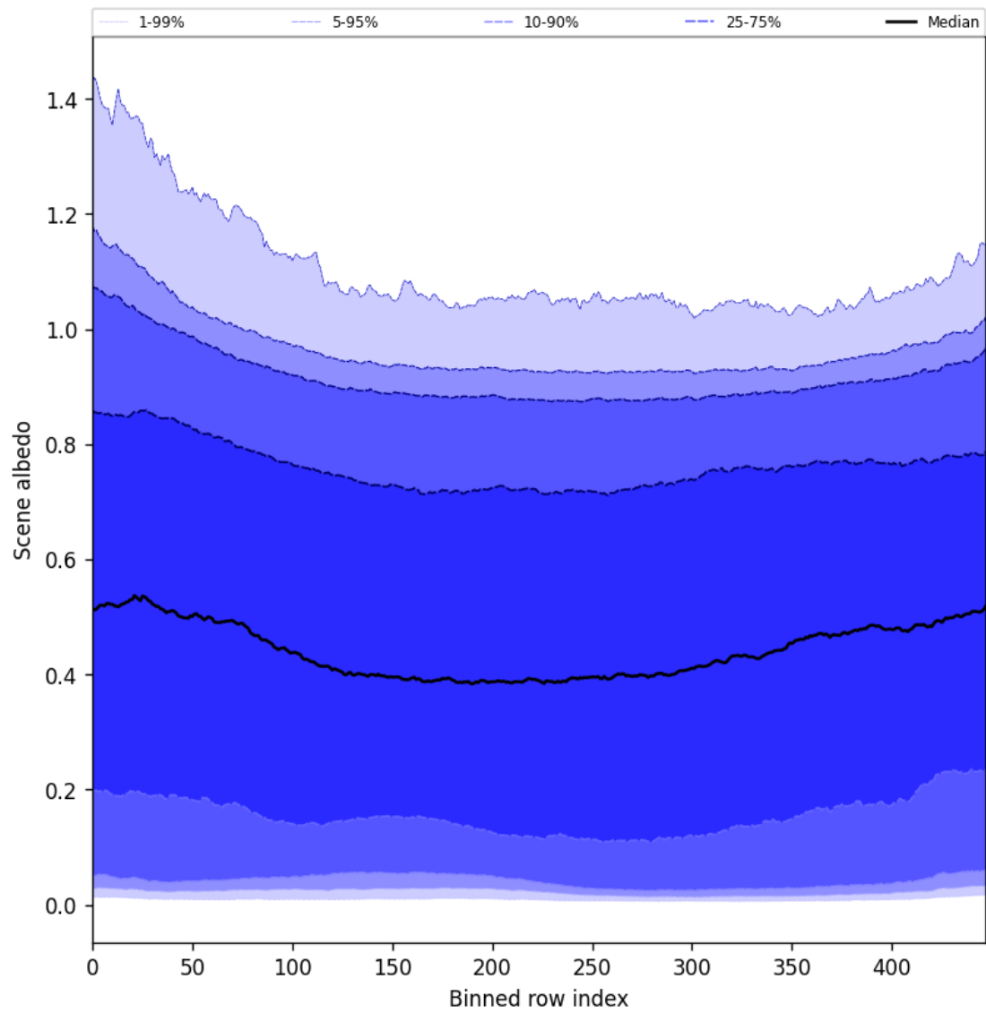
Figure 49: Along track statistics of “Scene albedo” for 2025-04-05 to 2025-04-06
