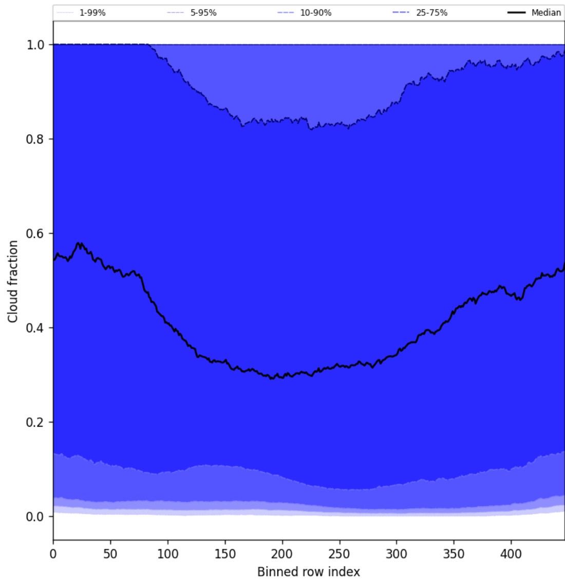
Figure 47: Along track statistics of “Cloud fraction” for 2025-04-05 to 2025-04-06
