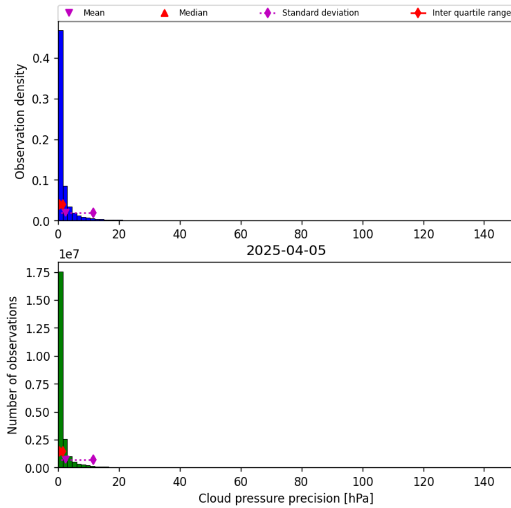
Figure 29: Histogram of “Cloud pressure precision” for 2025-04-05 to 2025-04-06
