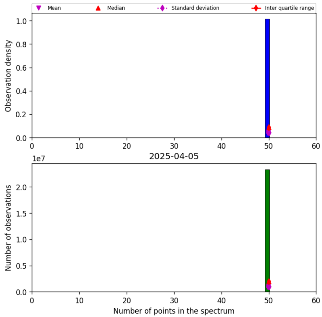
Figure 42: Histogram of “Number of points in the spectrum” for 2025-04-05 to 2025-04-06
