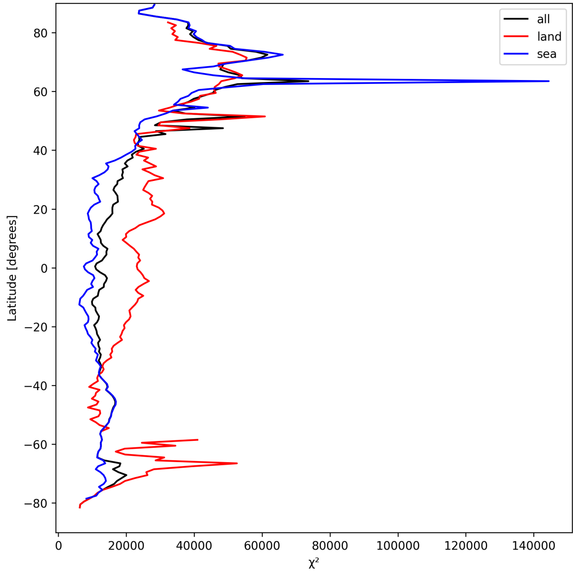
Figure 19: Zonal average of “ \chi^2 ” for 2025-04-05 to 2025-04-06.
