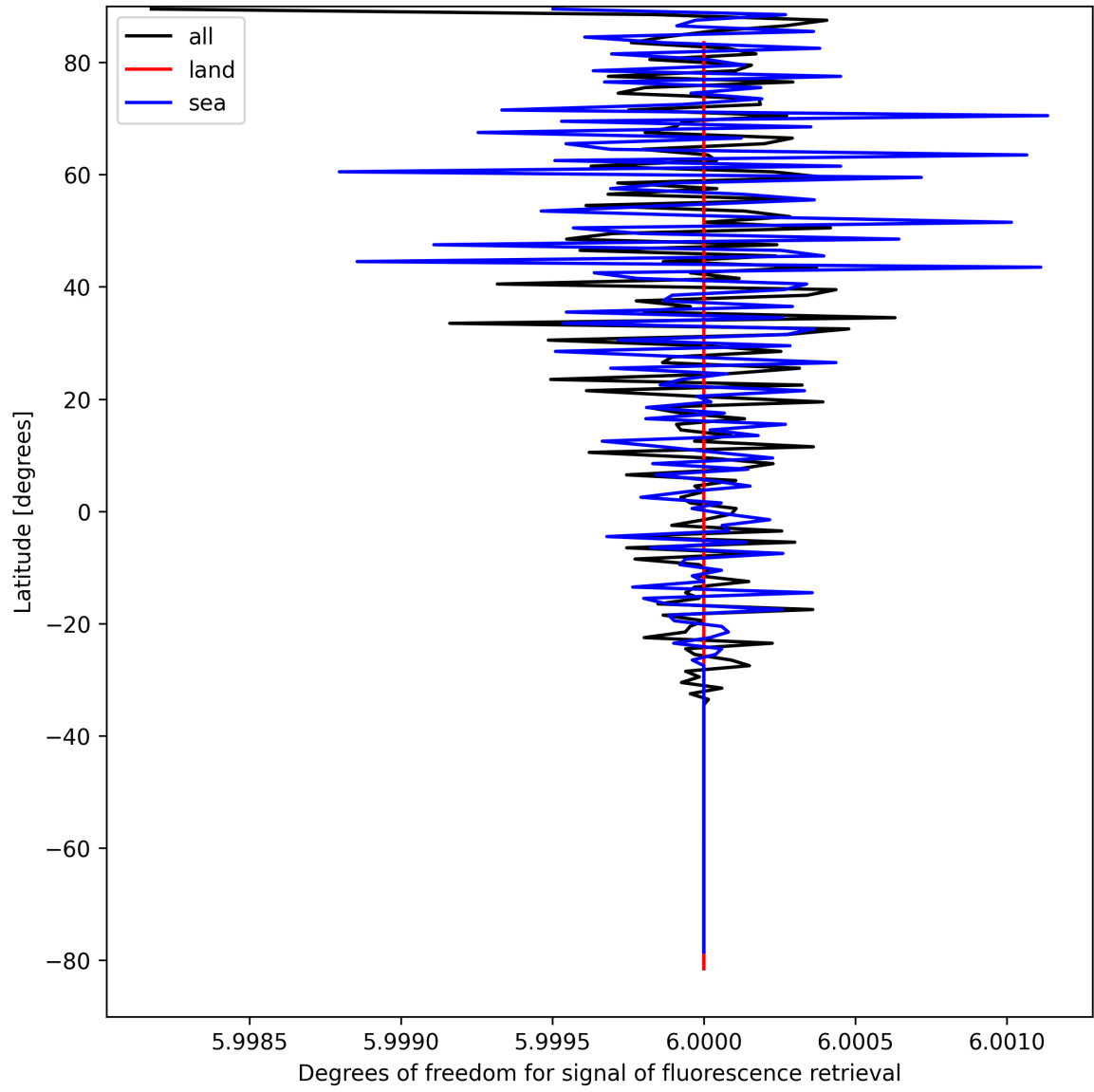
Figure 24: Zonal average of “Degrees of freedom for signal of fluorescence retrieval” for 2025-04-05 to 2025-04-06.
