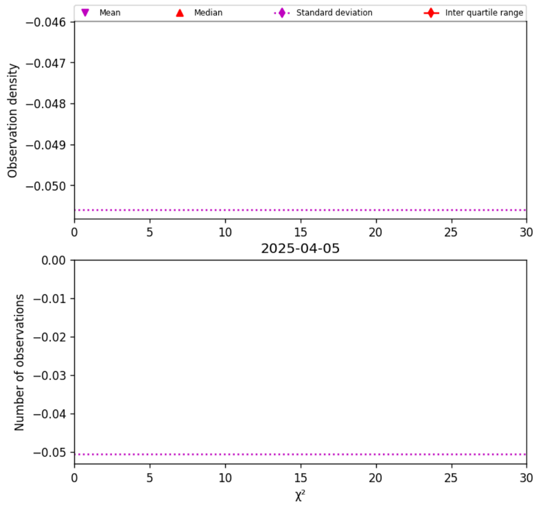
Figure 36: Histogram of “ \chi^2 ” for 2025-04-05 to 2025-04-06
