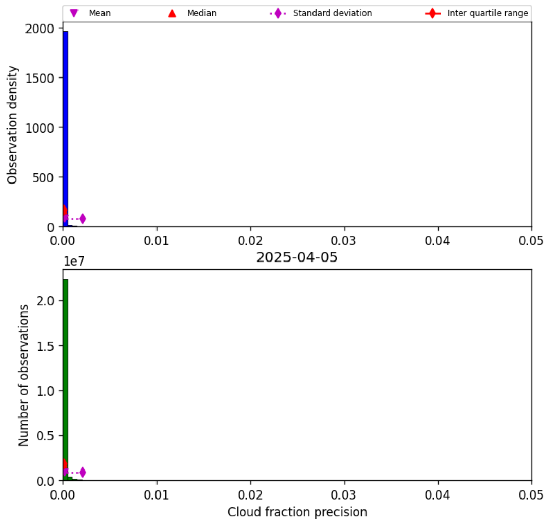
Figure 31: Histogram of “Cloud fraction precision” for 2025-04-05 to 2025-04-06
