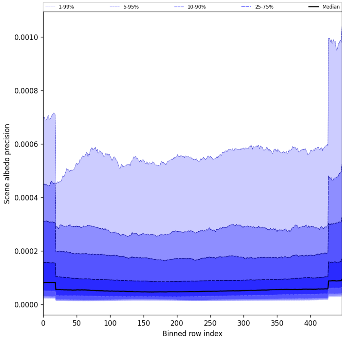
Figure 50: Along track statistics of “Scene albedo precision” for 2025-04-05 to 2025-04-06
