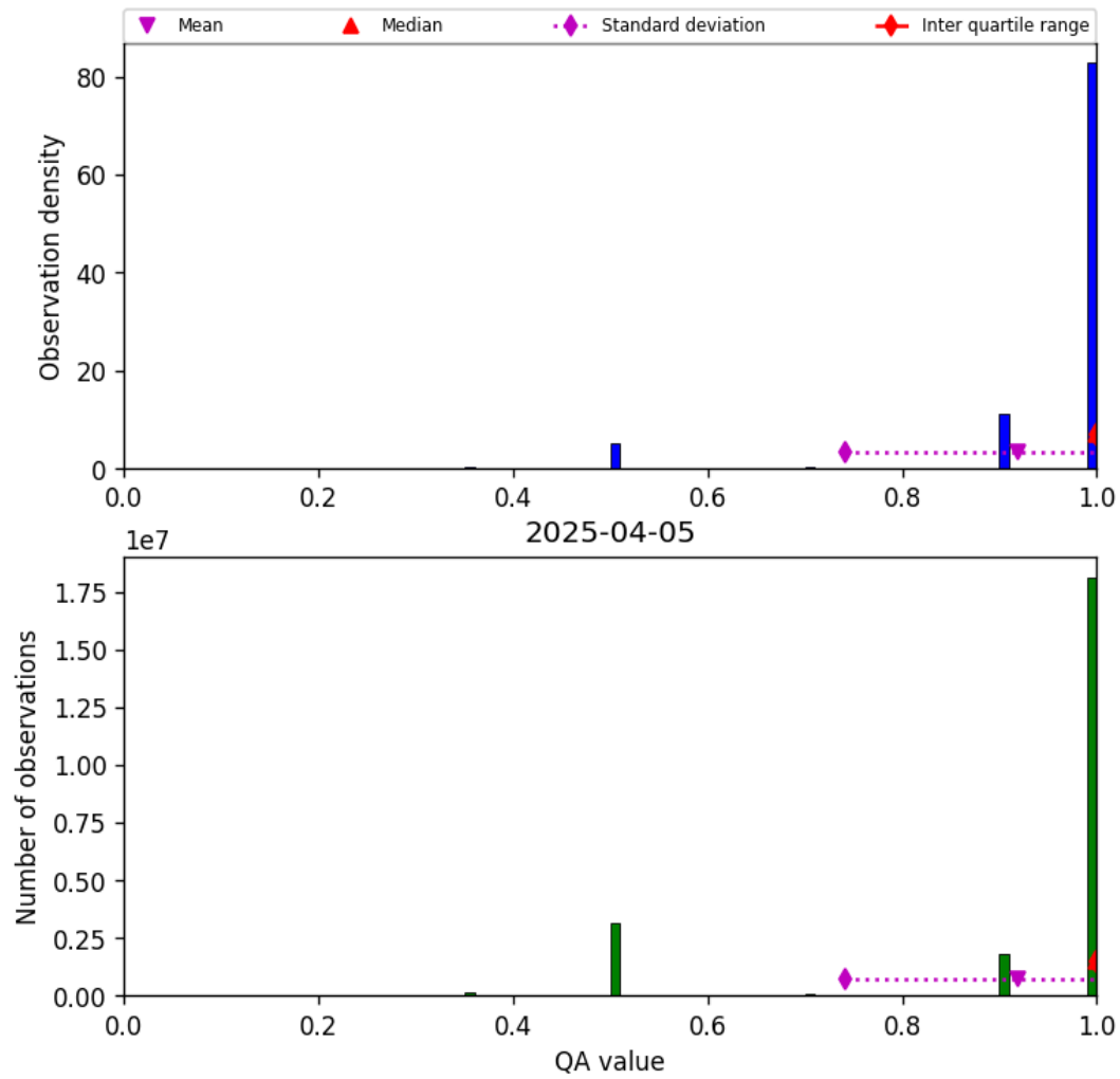
Figure 27: Histogram of “QA value” for 2025-04-05 to 2025-04-06
