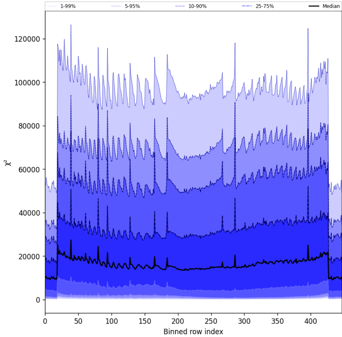
Figure 53: Along track statistics of “ \chi^2 ” for 2025-04-05 to 2025-04-06
