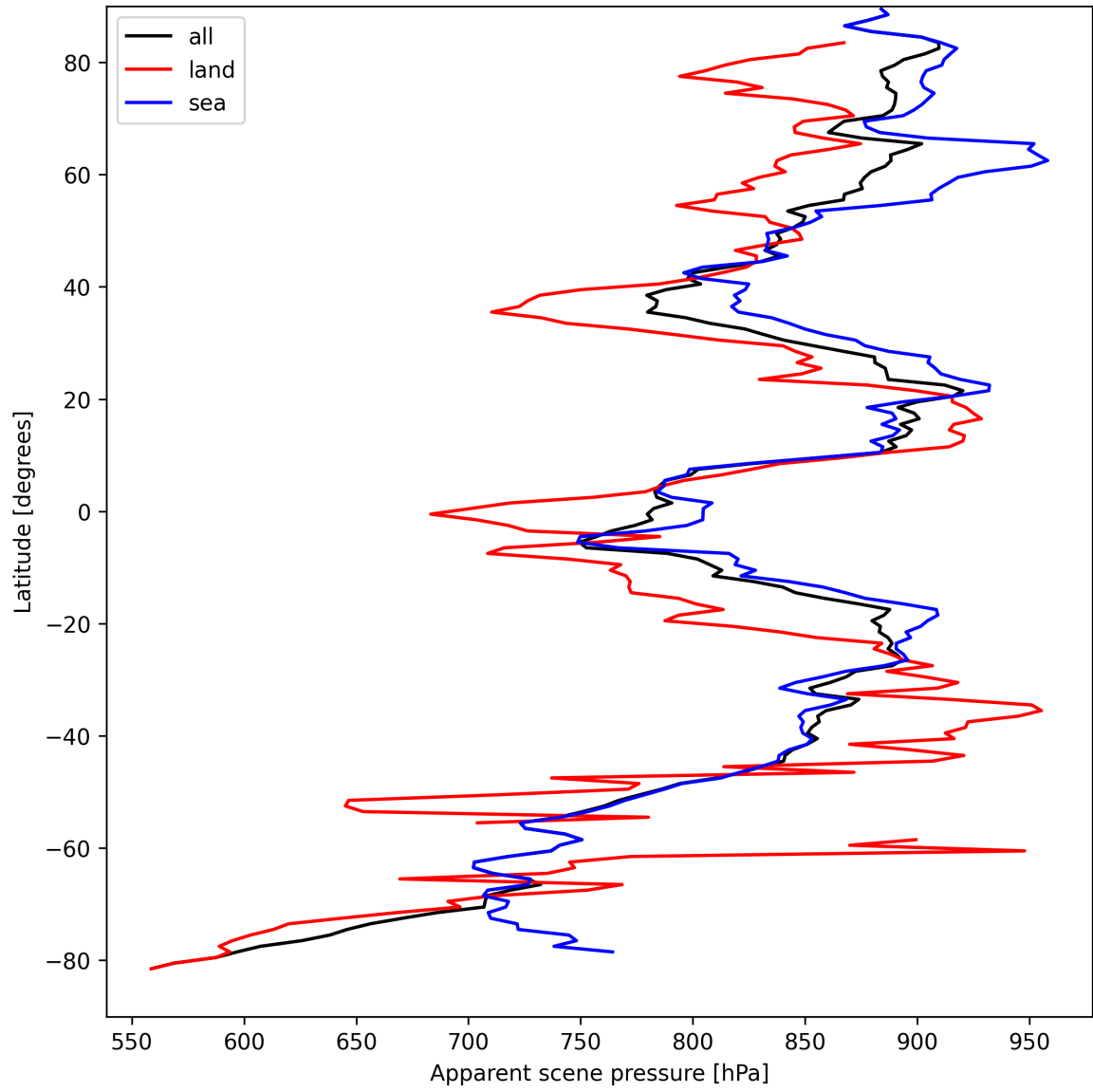
Figure 17: Zonal average of “Apparent scene pressure” for 2025-04-05 to 2025-04-06.
