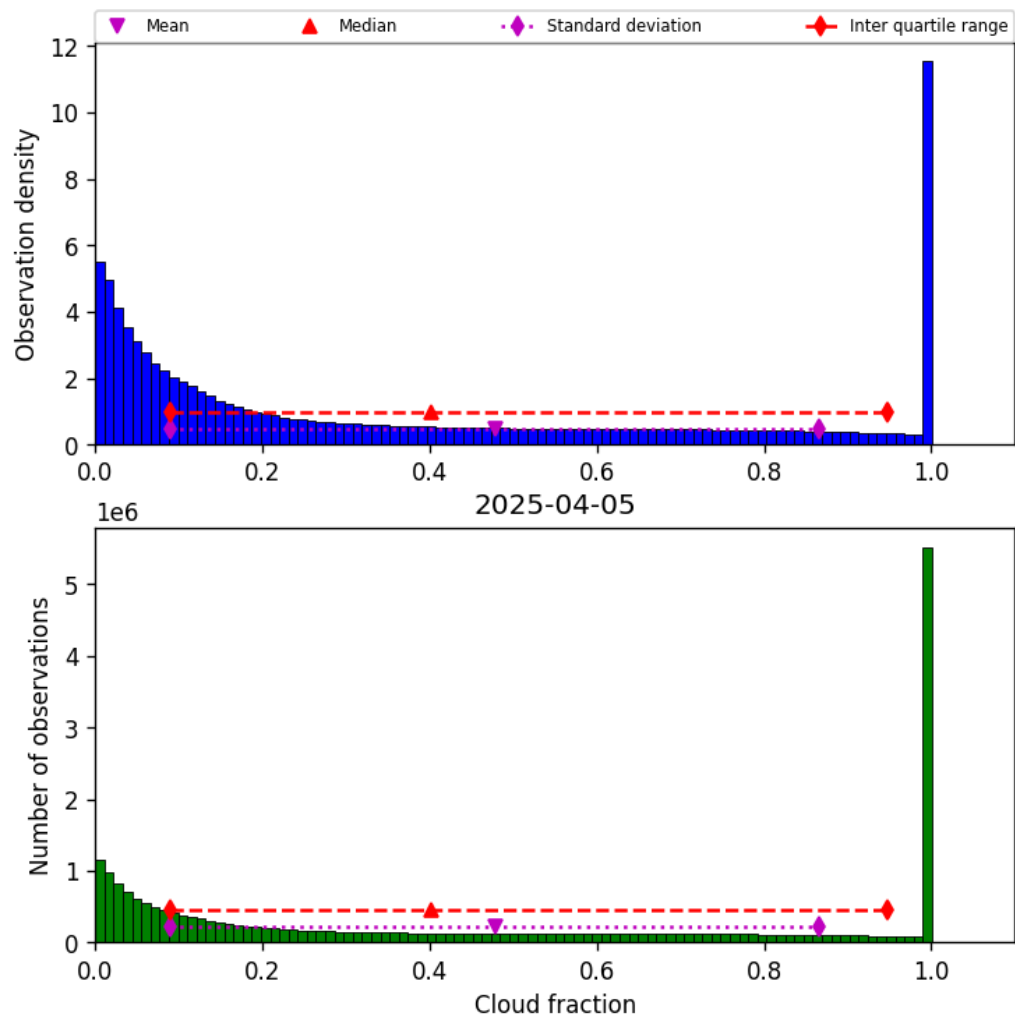
Figure 30: Histogram of “Cloud fraction” for 2025-04-05 to 2025-04-06
