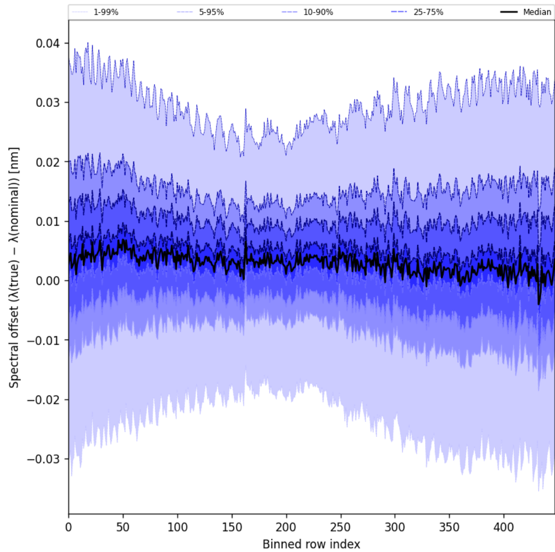
Figure 60: Along track statistics of “Spectral offset ( \lambda_{\text{true}} - \lambda_{\text{nominal}} )” for 2025-04-05 to 2025-04-06
