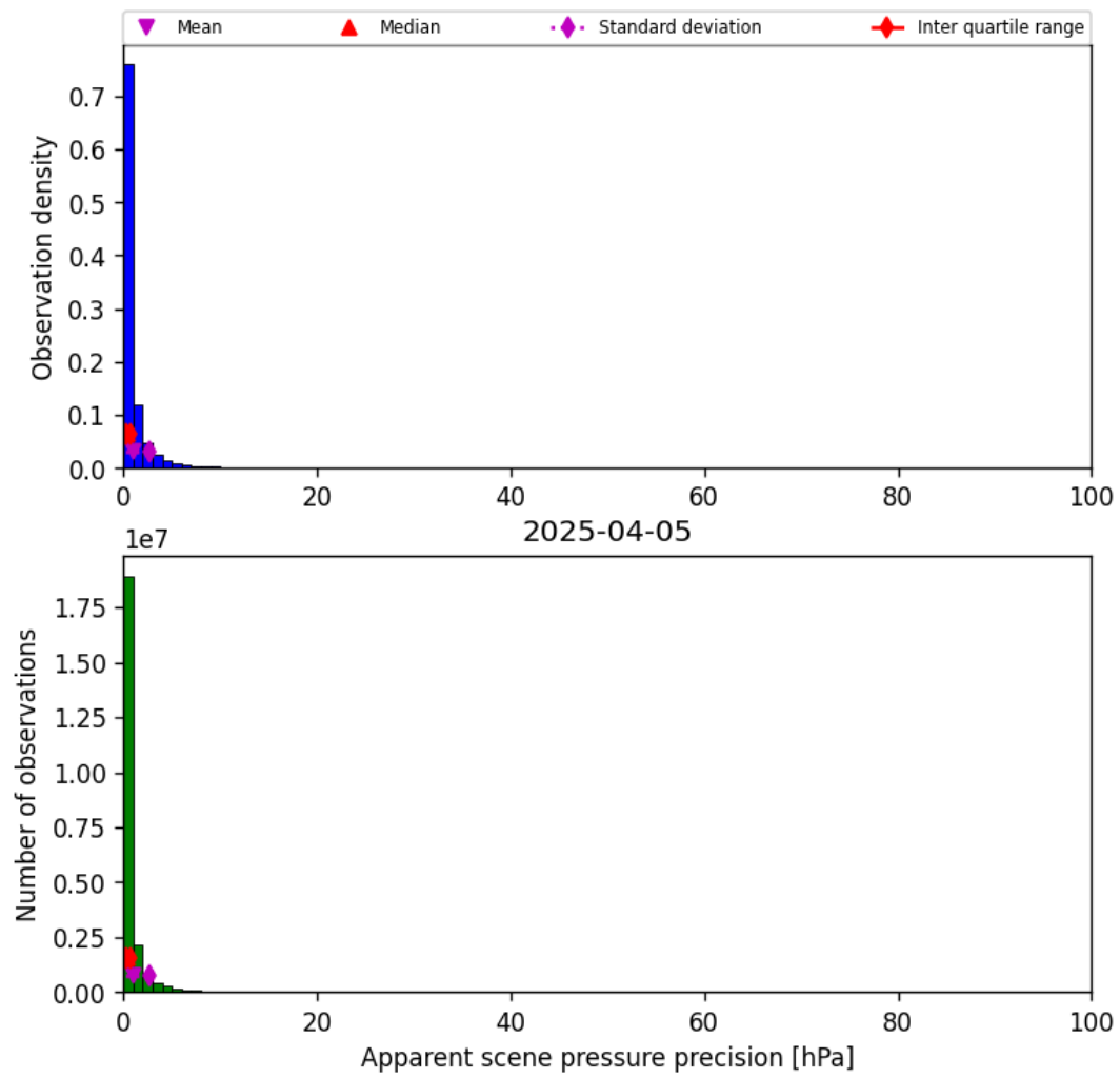
Figure 35: Histogram of “Apparent scene pressure precision” for 2025-04-05 to 2025-04-06
