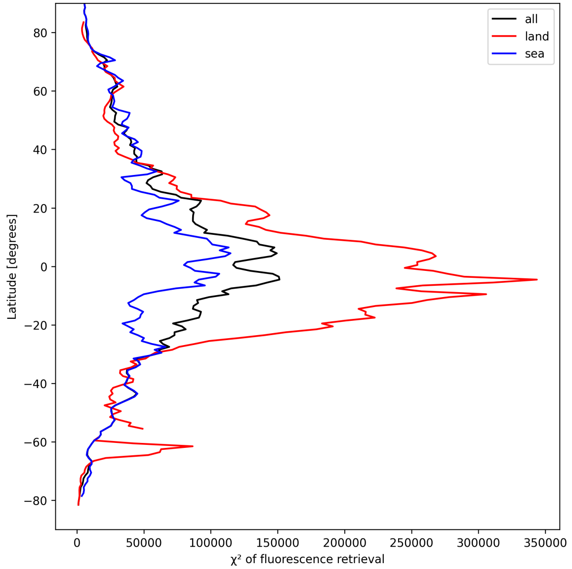
Figure 23: Zonal average of “ \chi^2 of fluorescence retrieval” for 2025-04-05 to 2025-04-06.
