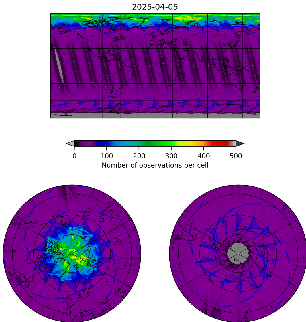
Figure 9: Map of the number of observations for 2025-04-05 to 2025-04-06
