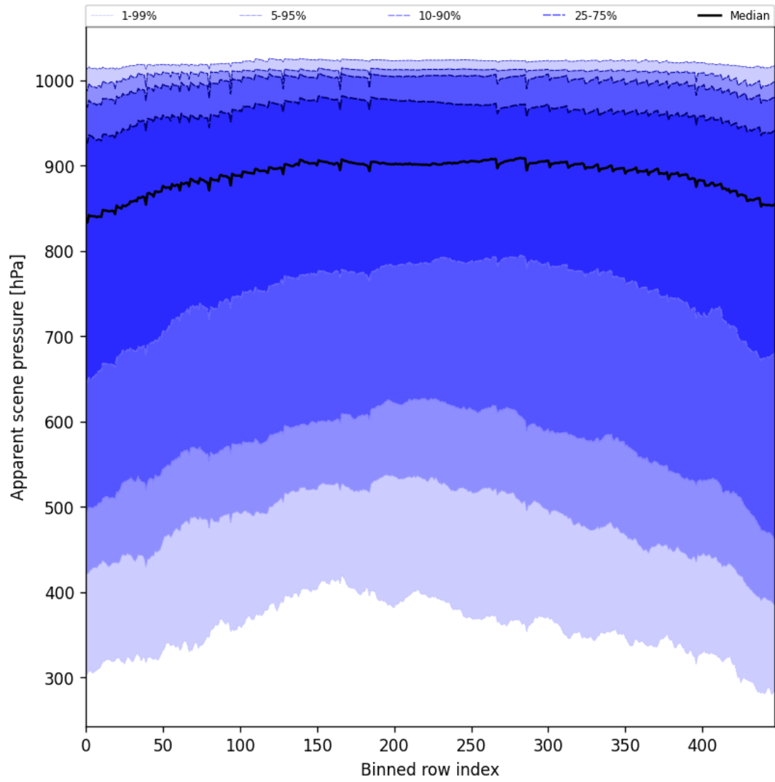
Figure 51: Along track statistics of “Apparent scene pressure” for 2025-04-05 to 2025-04-06
