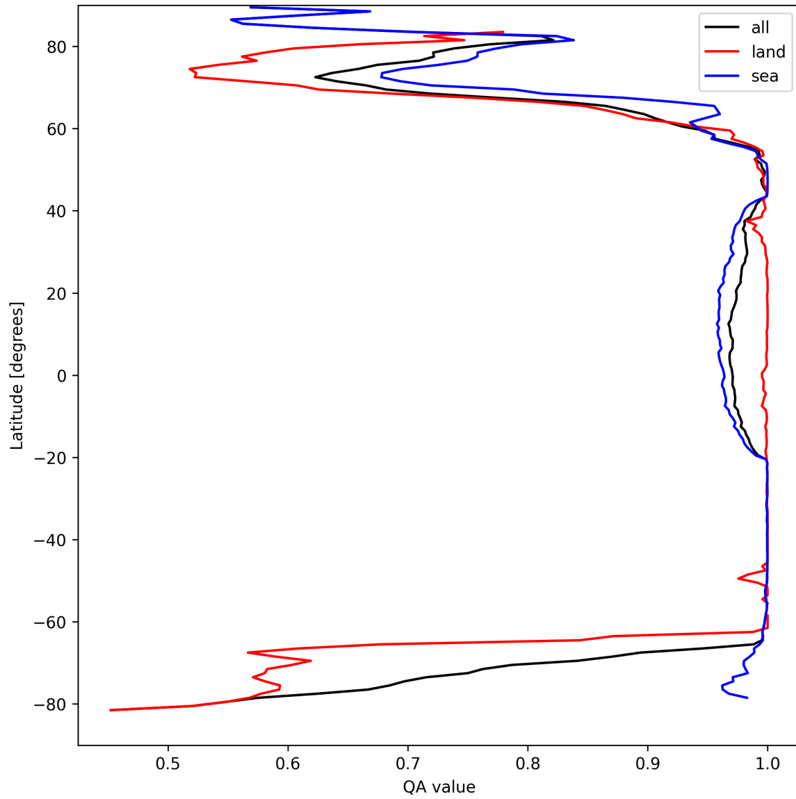
Figure 10: Zonal average of “QA value” for 2025-04-05 to 2025-04-06.
