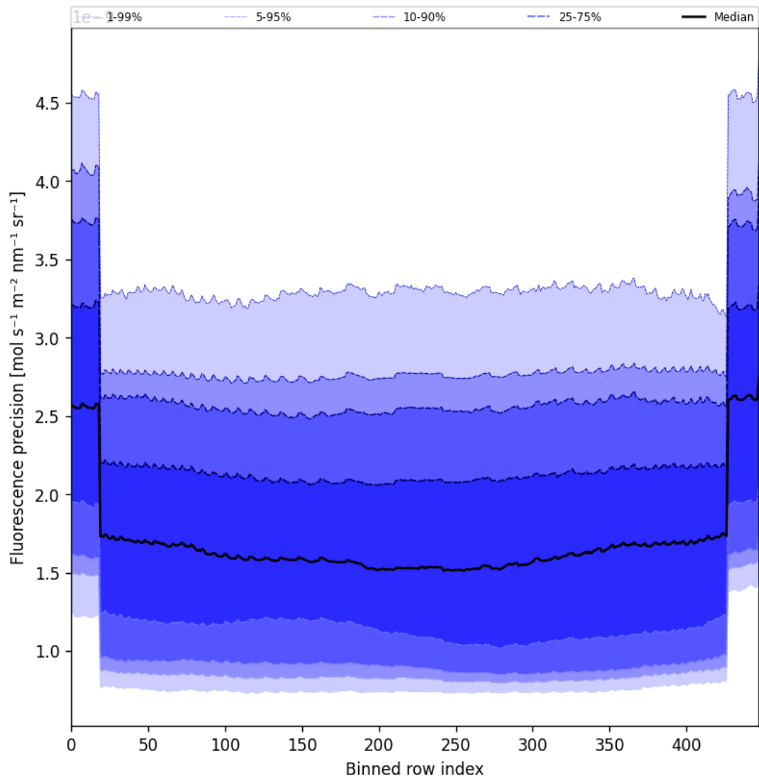
Figure 56: Along track statistics of “Fluorescence precision” for 2025-04-05 to 2025-04-06
