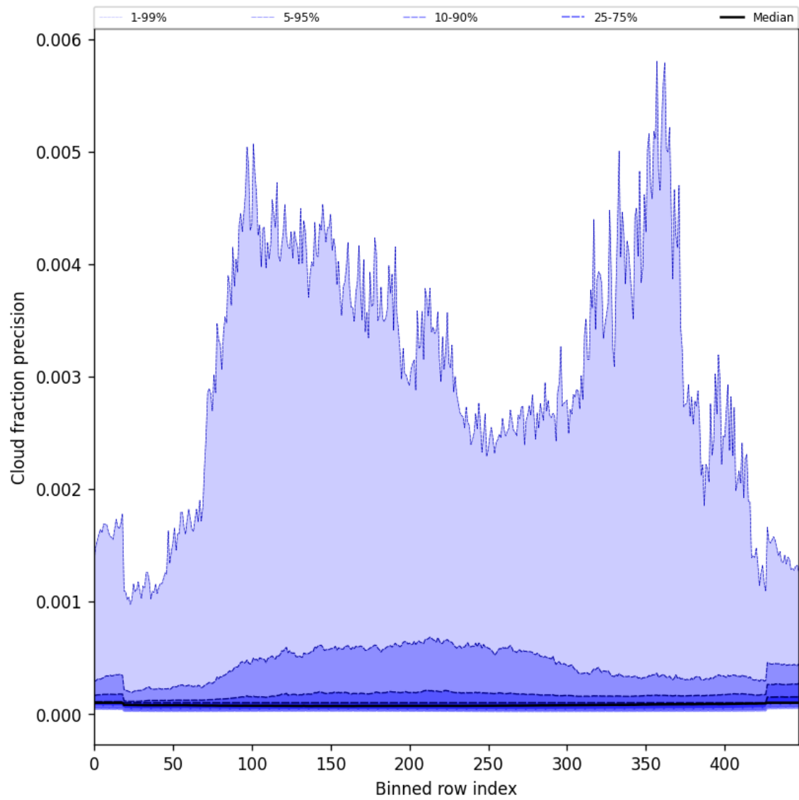
Figure 48: Along track statistics of “Cloud fraction precision” for 2025-04-05 to 2025-04-06
