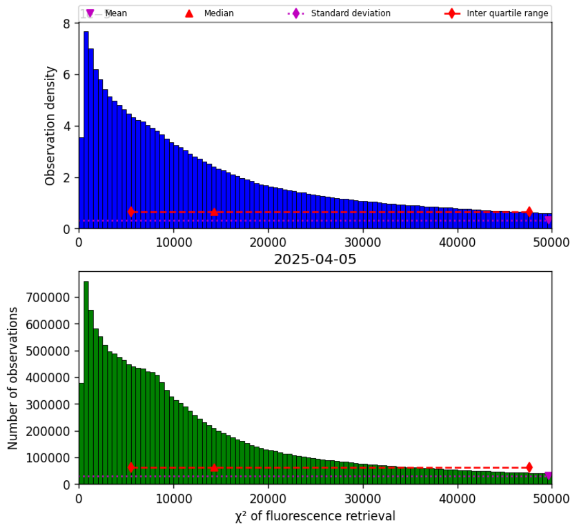
Figure 40: Histogram of “ \chi^2 of fluorescence retrieval” for 2025-04-05 to 2025-04-06
