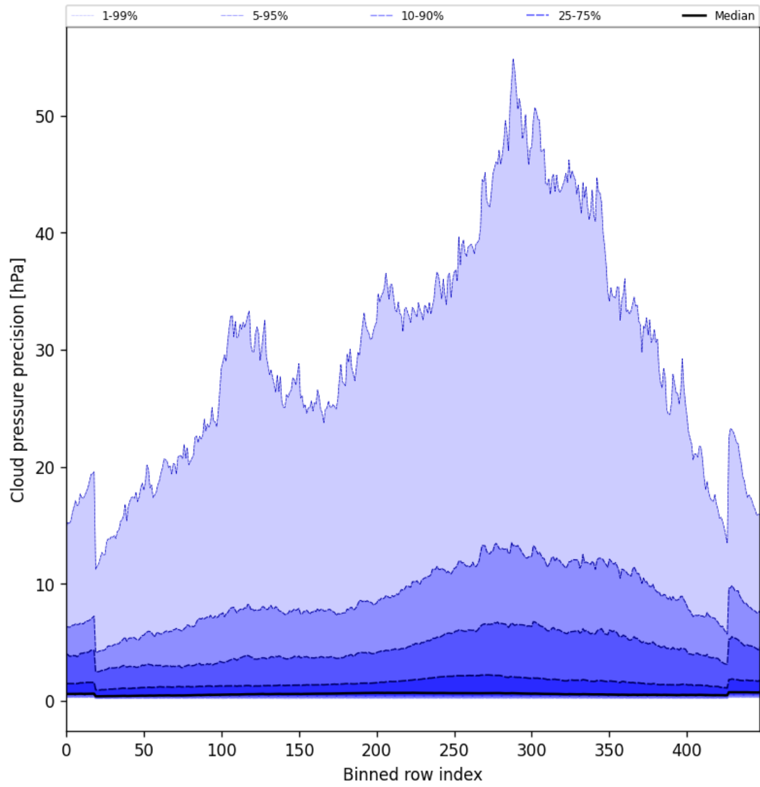
Figure 46: Along track statistics of “Cloud pressure precision” for 2025-04-05 to 2025-04-06
