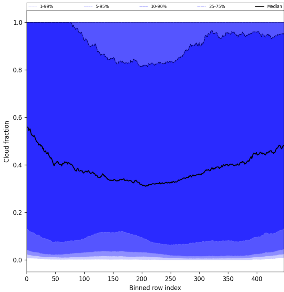
Figure 47: Along track statistics of “Cloud fraction” for 2025-04-09 to 2025-04-10
