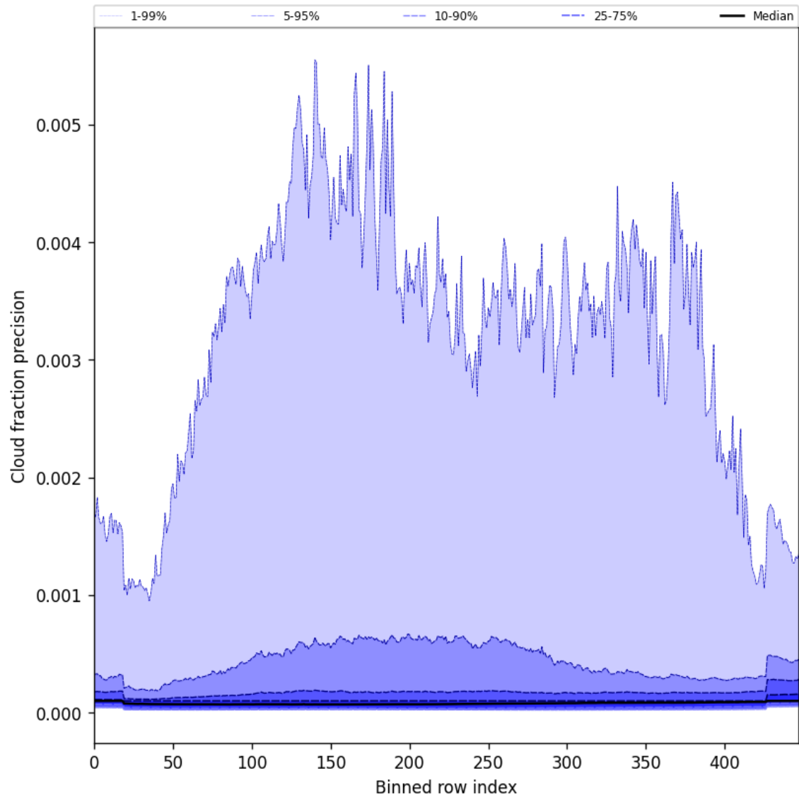
Figure 48: Along track statistics of “Cloud fraction precision” for 2025-04-09 to 2025-04-10
