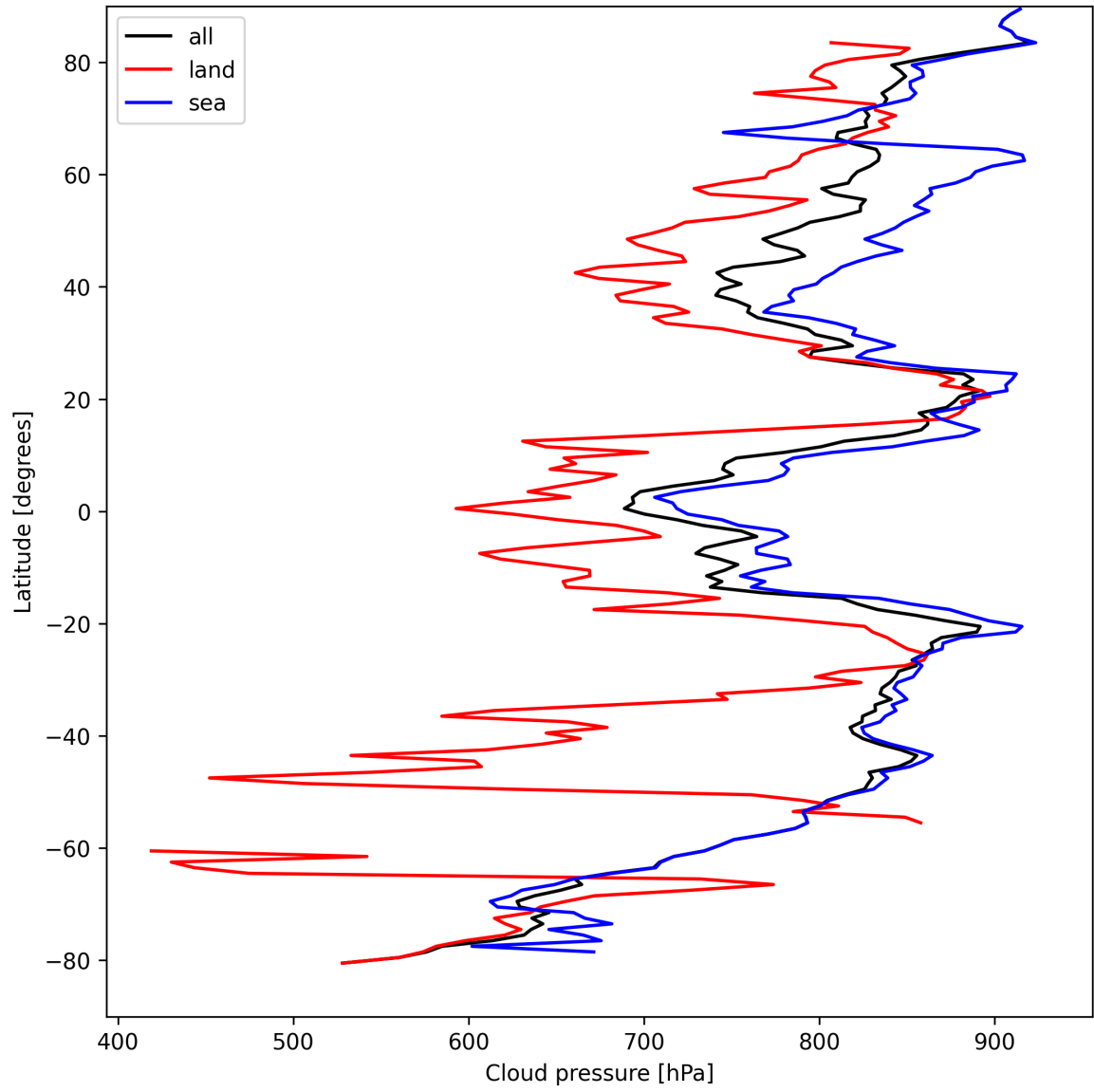
Figure 11: Zonal average of “Cloud pressure” for 2025-04-09 to 2025-04-10.
