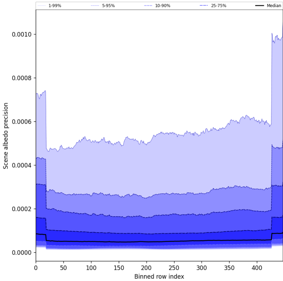
Figure 50: Along track statistics of “Scene albedo precision” for 2025-04-09 to 2025-04-10
