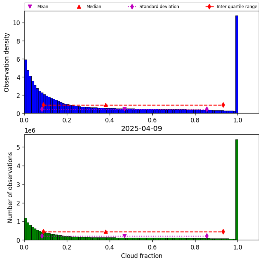
Figure 30: Histogram of “Cloud fraction” for 2025-04-09 to 2025-04-10
