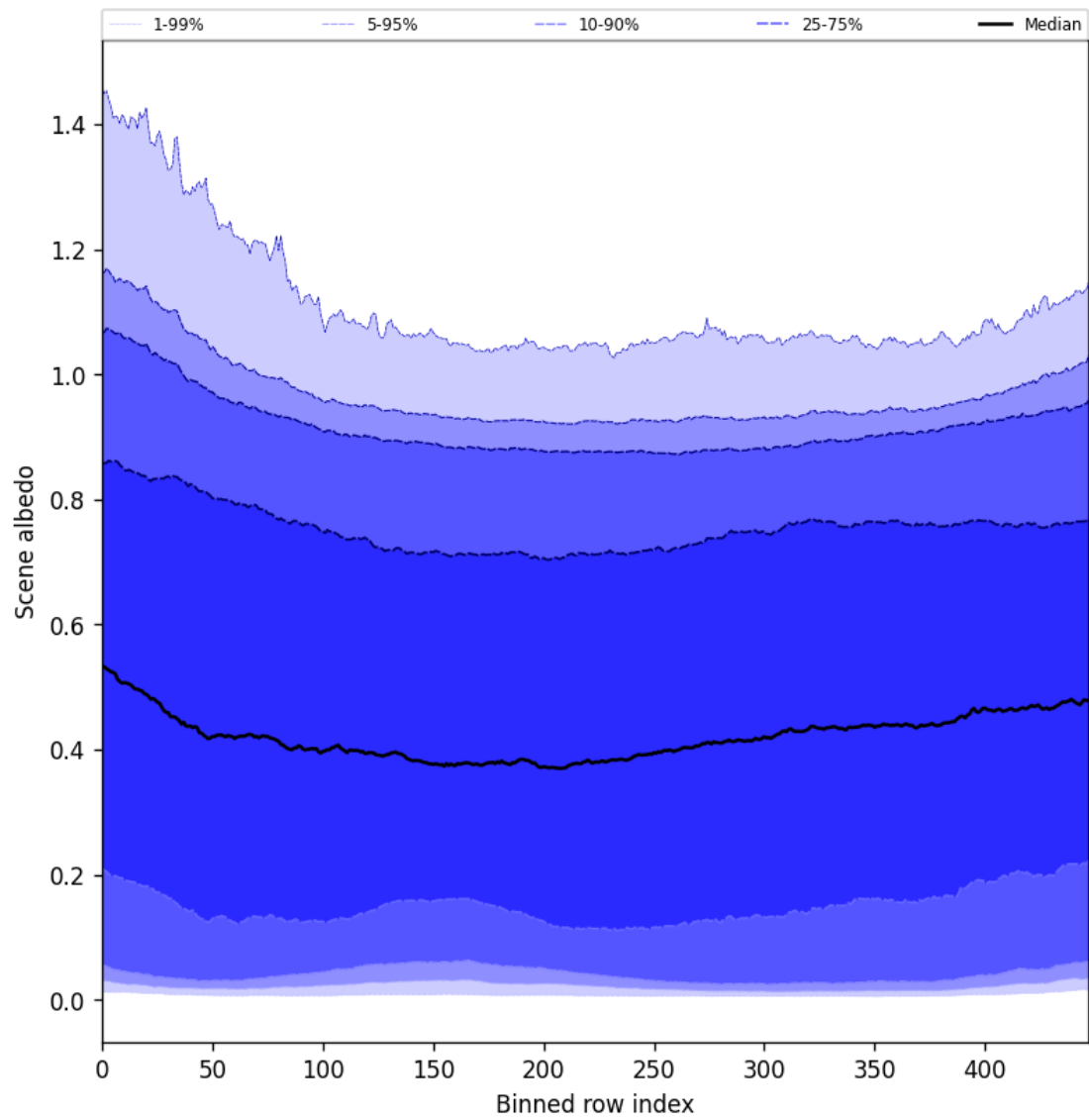
Figure 49: Along track statistics of “Scene albedo” for 2025-04-09 to 2025-04-10
