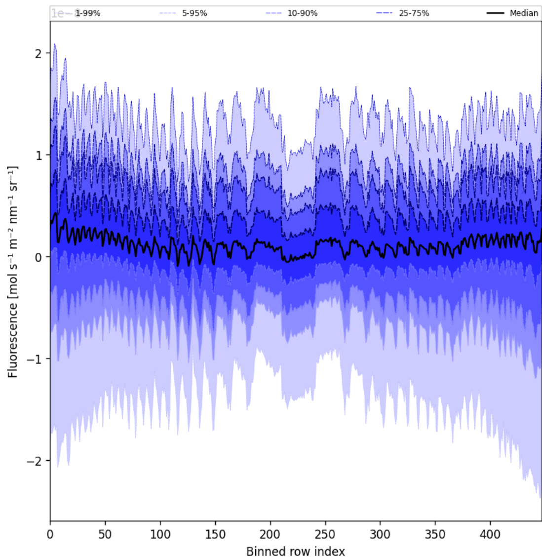
Figure 55: Along track statistics of “Fluorescence” for 2025-04-09 to 2025-04-10
