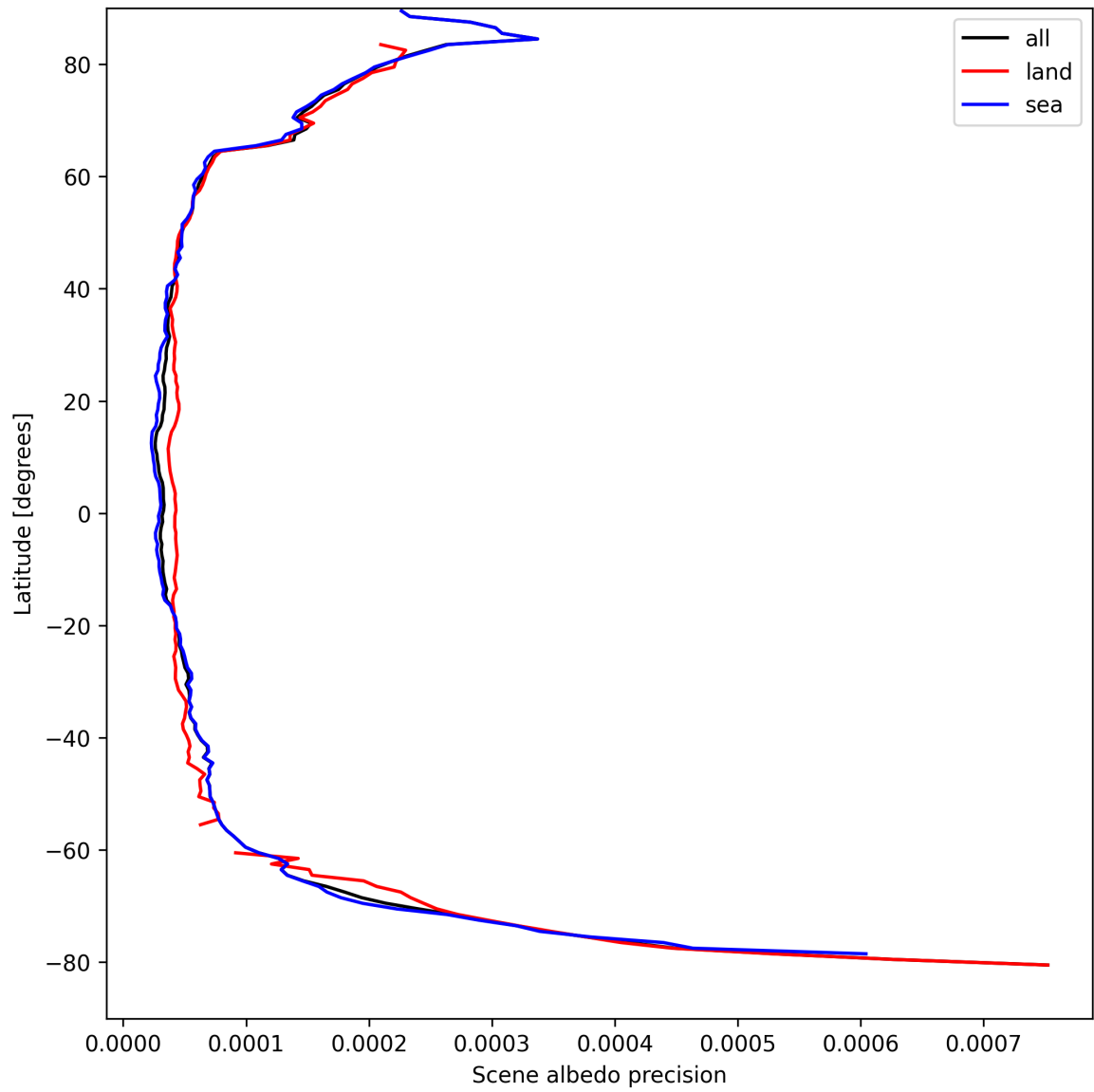
Figure 16: Zonal average of “Scene albedo precision” for 2025-04-09 to 2025-04-10.
