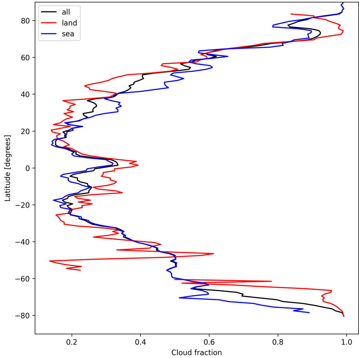
Figure 13: Zonal average of “Cloud fraction” for 2025-04-09 to 2025-04-10.
