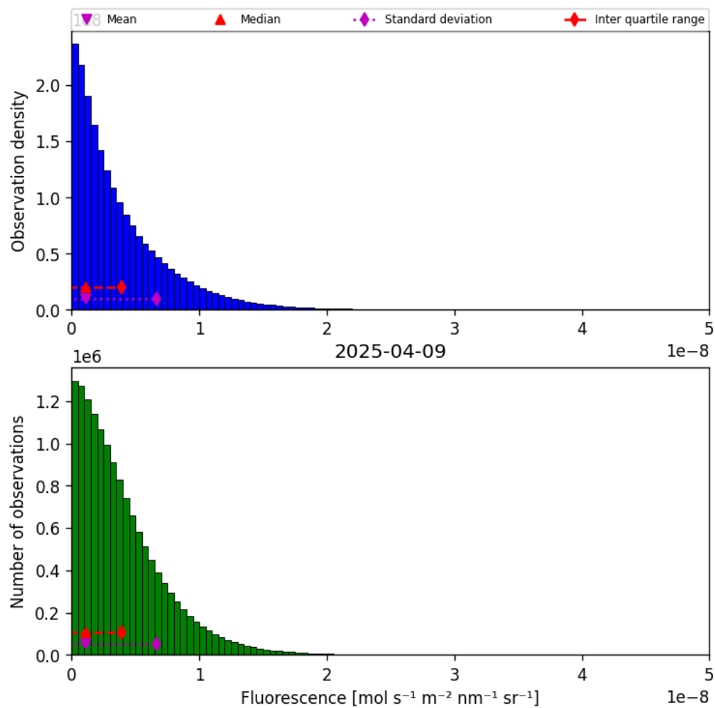
Figure 38: Histogram of “Fluorescence” for 2025-04-09 to 2025-04-10
