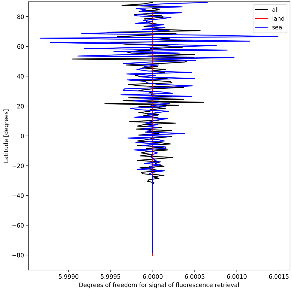
Figure 24: Zonal average of “Degrees of freedom for signal of fluorescence retrieval” for 2025-04-09 to 2025-04-10.
