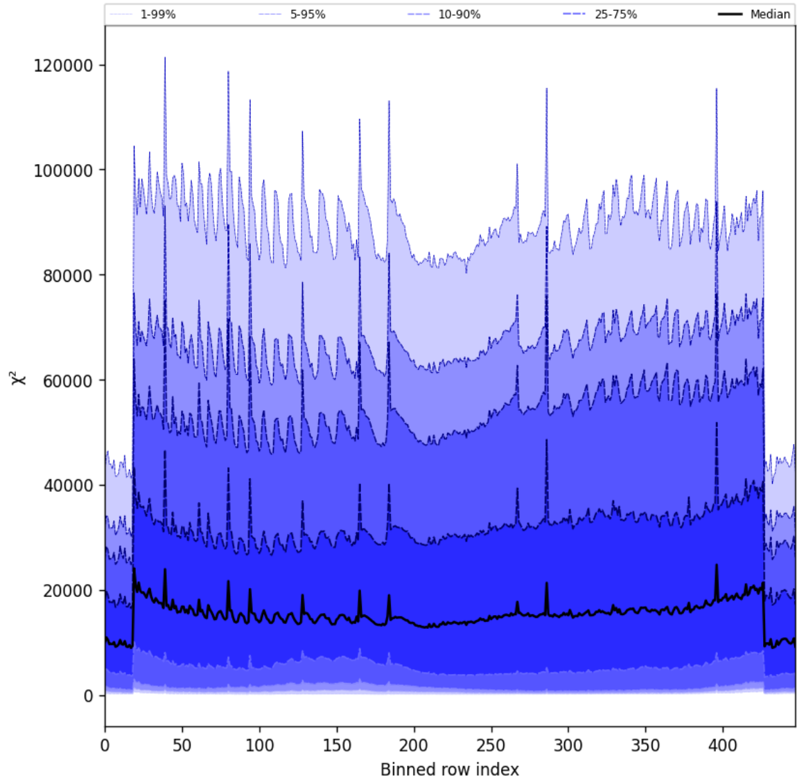
Figure 53: Along track statistics of “ \chi^2 ” for 2025-04-09 to 2025-04-10
