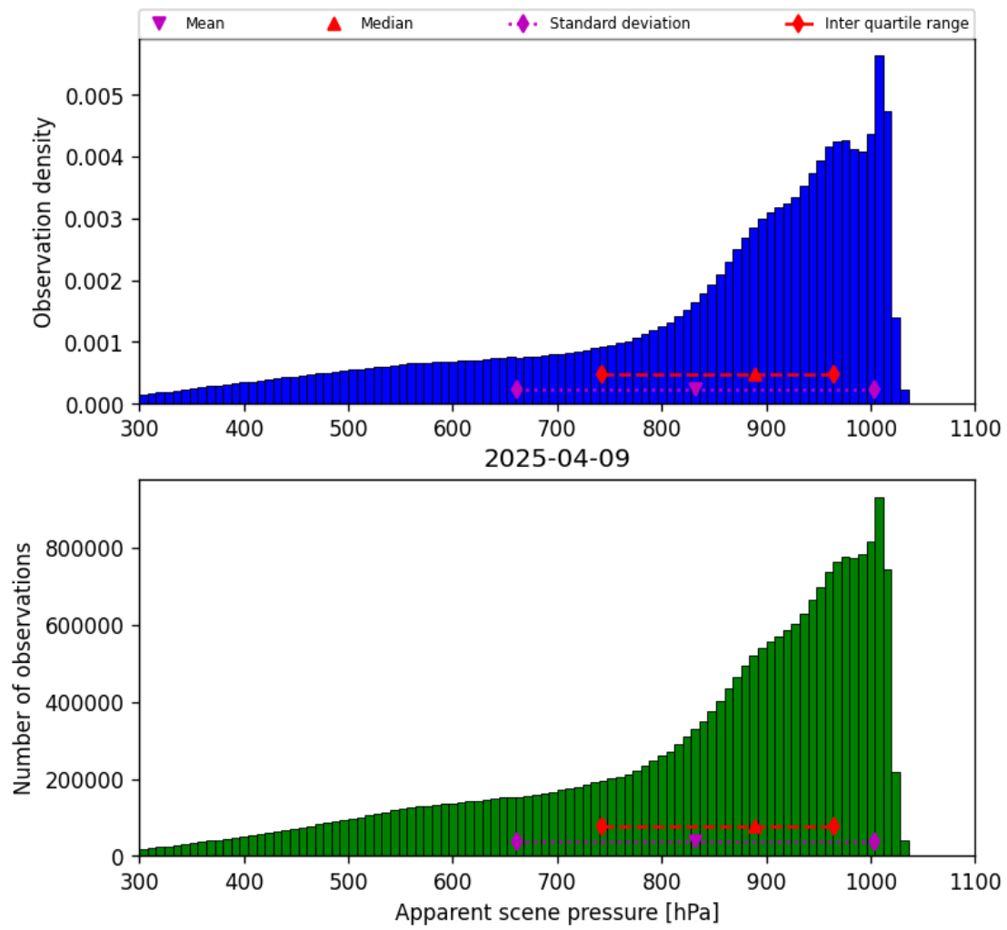
Figure 34: Histogram of “Apparent scene pressure” for 2025-04-09 to 2025-04-10
