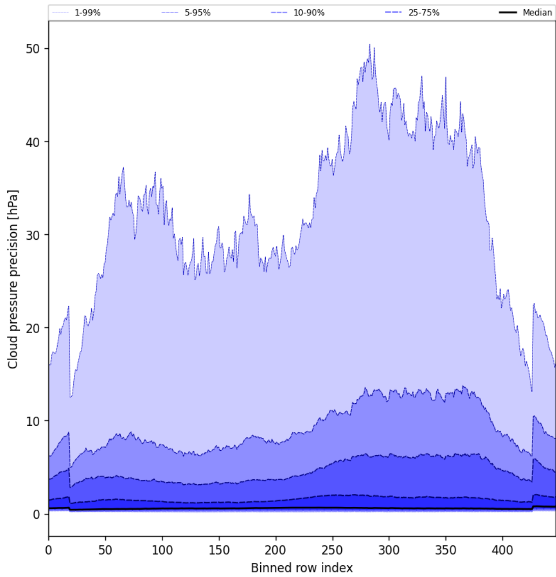
Figure 46: Along track statistics of “Cloud pressure precision” for 2025-04-09 to 2025-04-10
