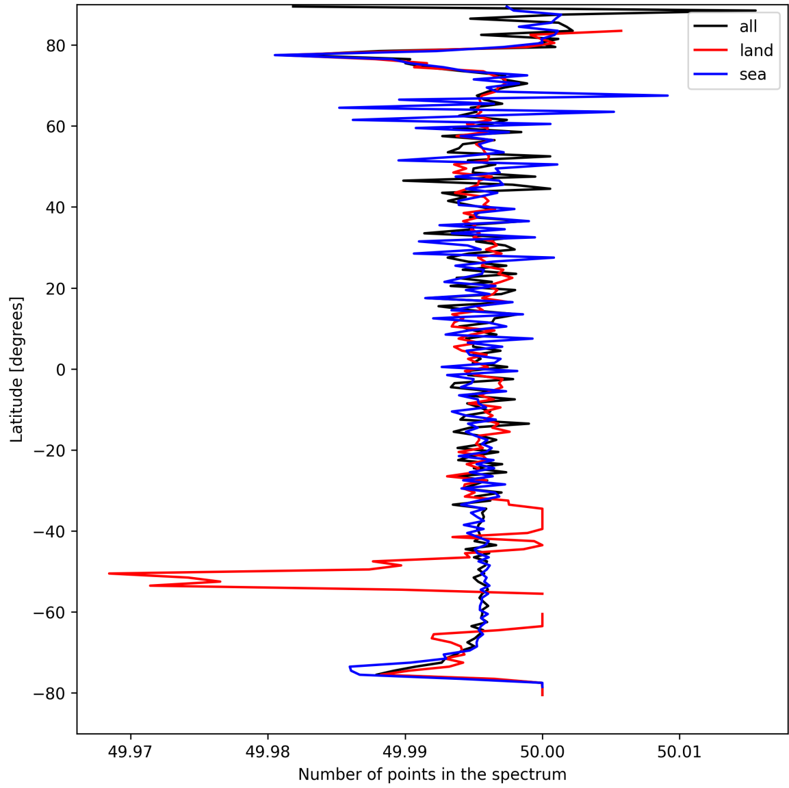
Figure 25: Zonal average of “Number of points in the spectrum” for 2025-04-09 to 2025-04-10.
