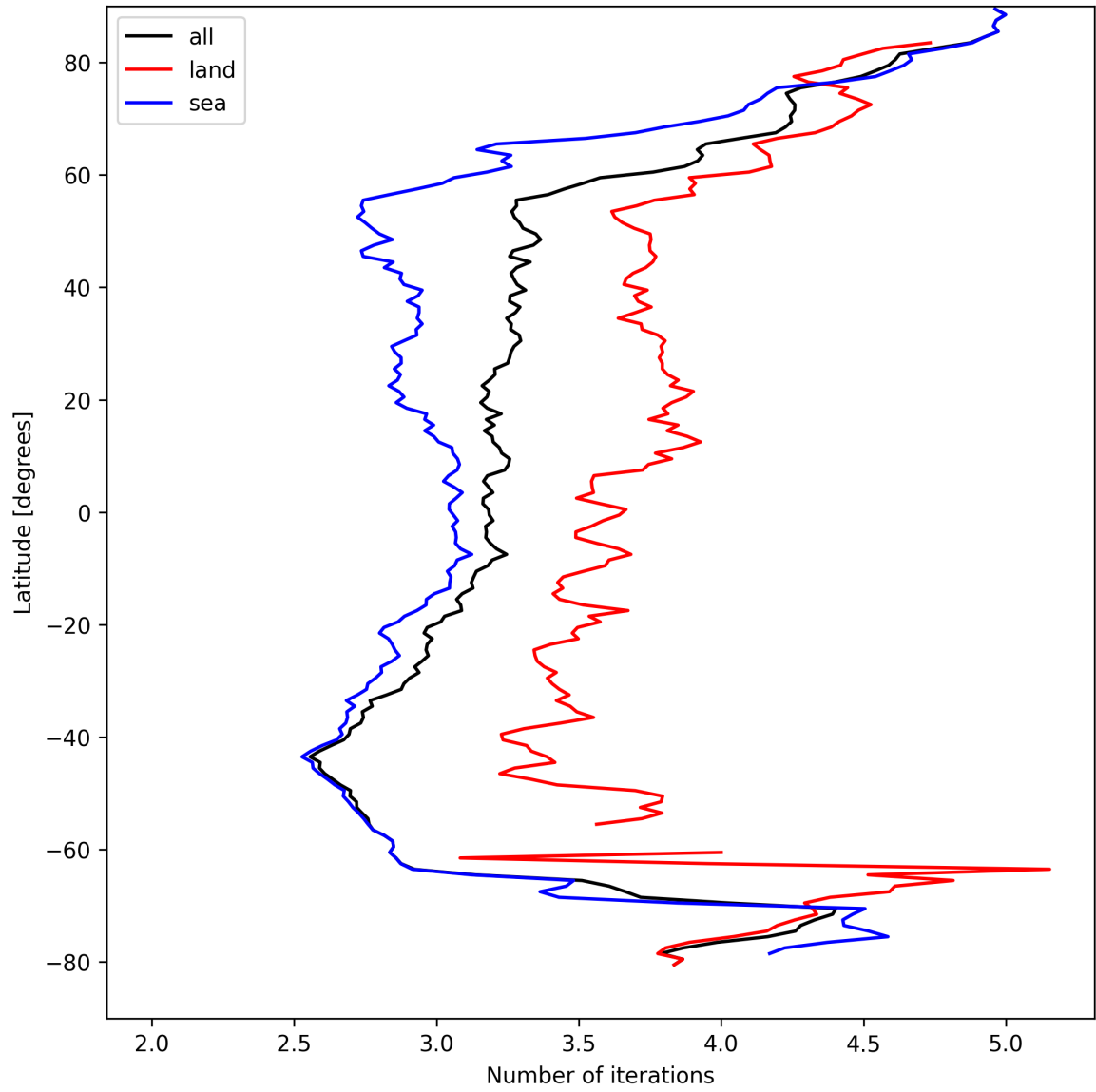
Figure 20: Zonal average of “Number of iterations” for 2025-04-09 to 2025-04-10.
