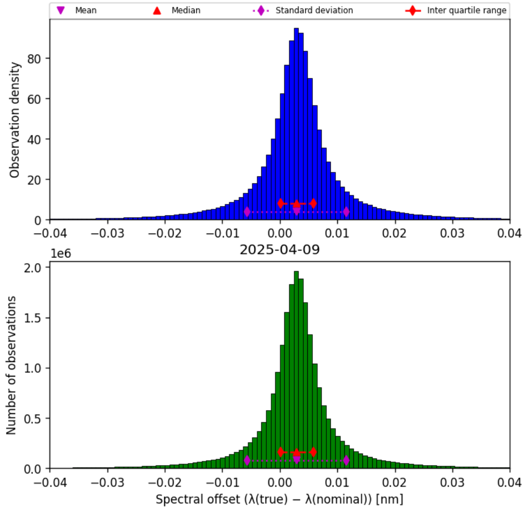
Figure 43: Histogram of “Spectral offset ( \lambda_{\text{true}} - \lambda_{\text{nominal}} )” for 2025-04-09 to 2025-04-10
