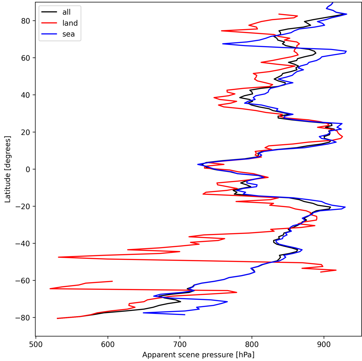
Figure 17: Zonal average of “Apparent scene pressure” for 2025-04-09 to 2025-04-10.
