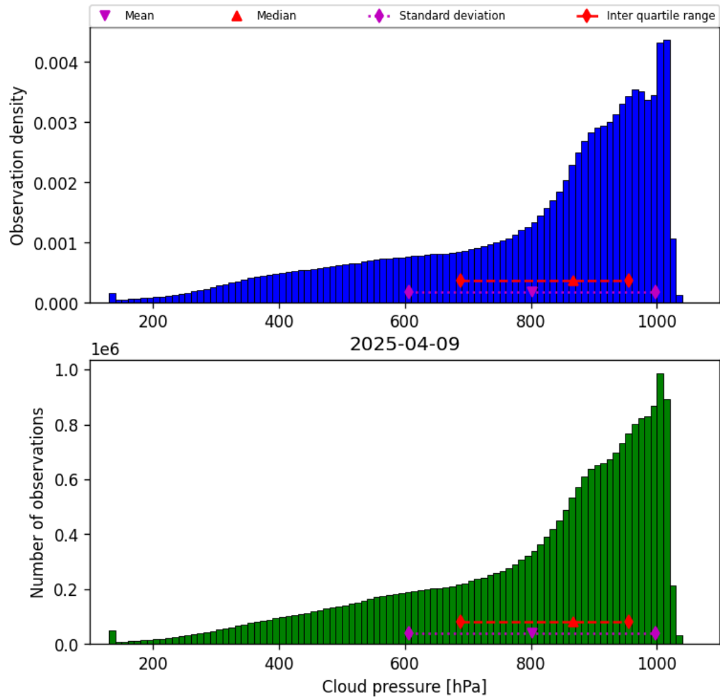
Figure 28: Histogram of “Cloud pressure” for 2025-04-09 to 2025-04-10
