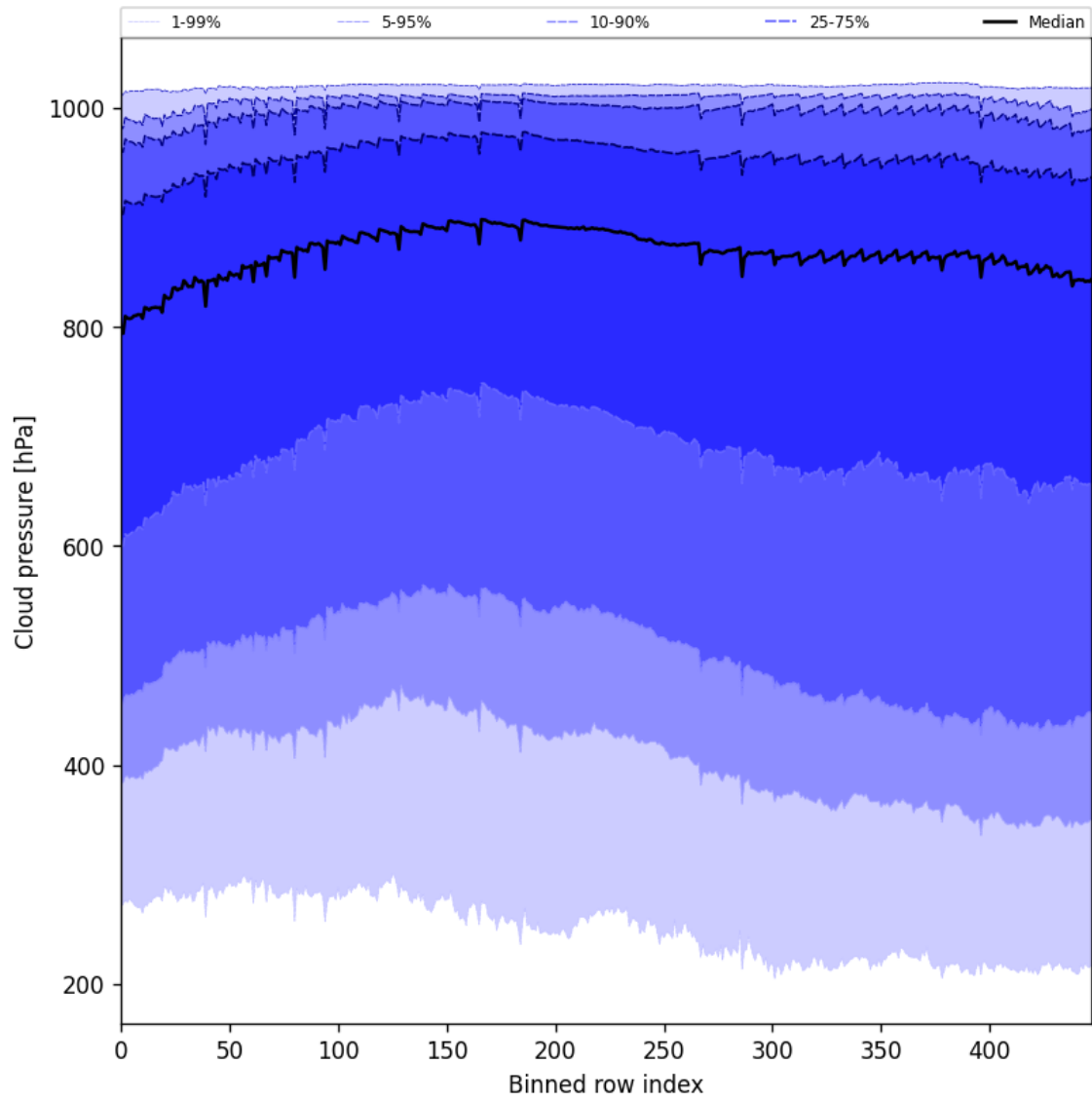
Figure 45: Along track statistics of “Cloud pressure” for 2025-04-09 to 2025-04-10
