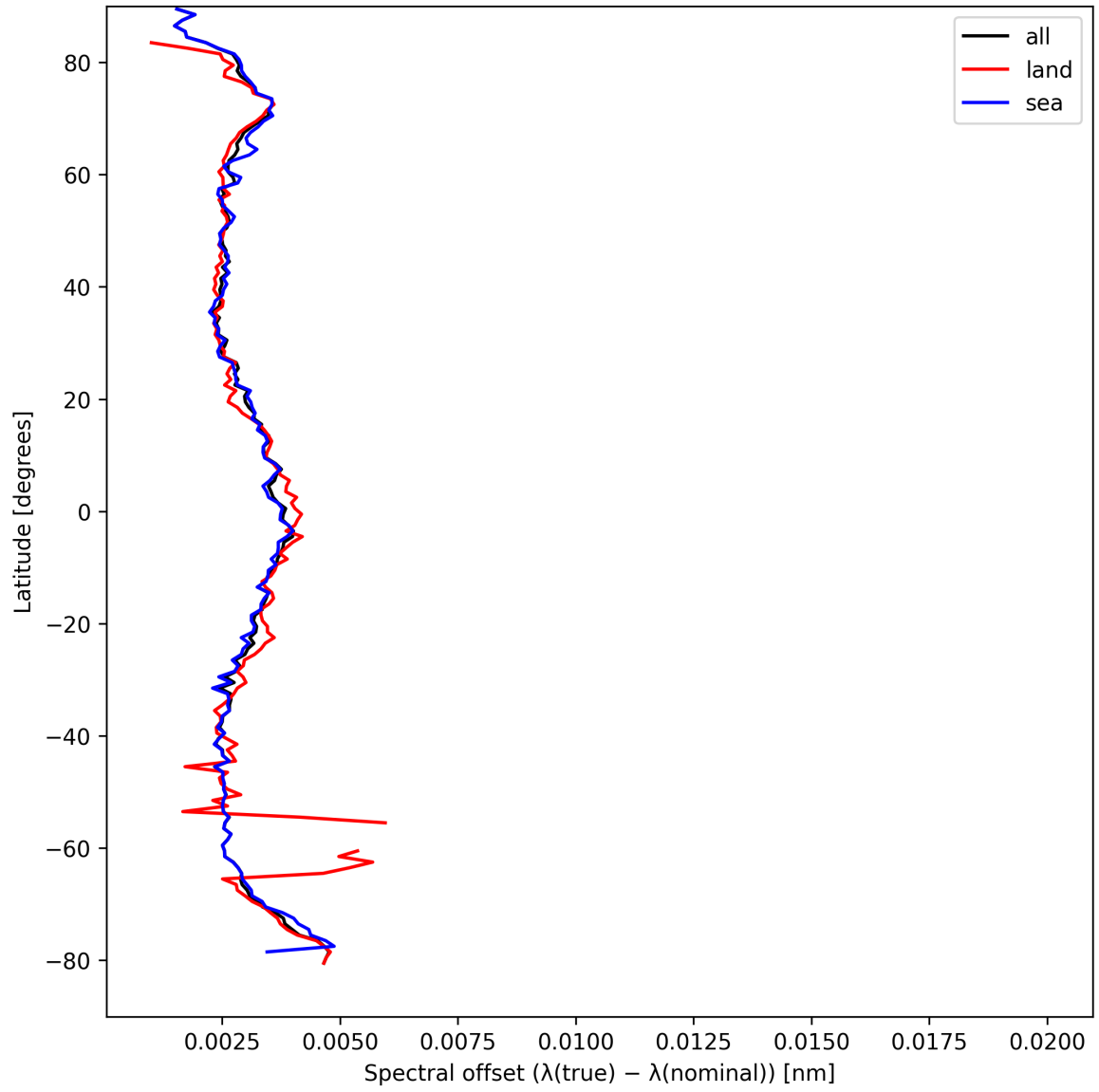
Figure 26: Zonal average of “Spectral offset ( \lambda_{\text{true}} - \lambda_{\text{nominal}} )” for 2025-04-09 to 2025-04-10.
