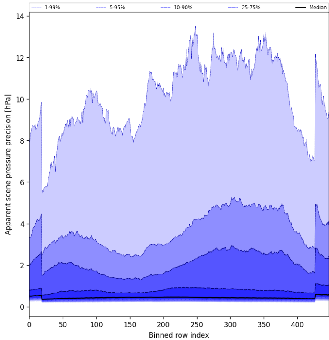
Figure 52: Along track statistics of “Apparent scene pressure precision” for 2025-04-09 to 2025-04-10
