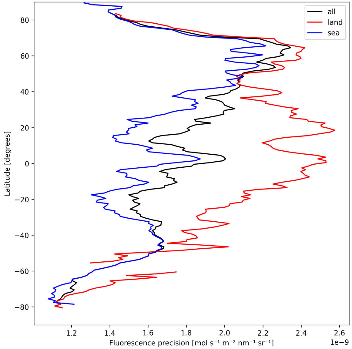
Figure 22: Zonal average of “Fluorescence precision” for 2025-04-09 to 2025-04-10.
