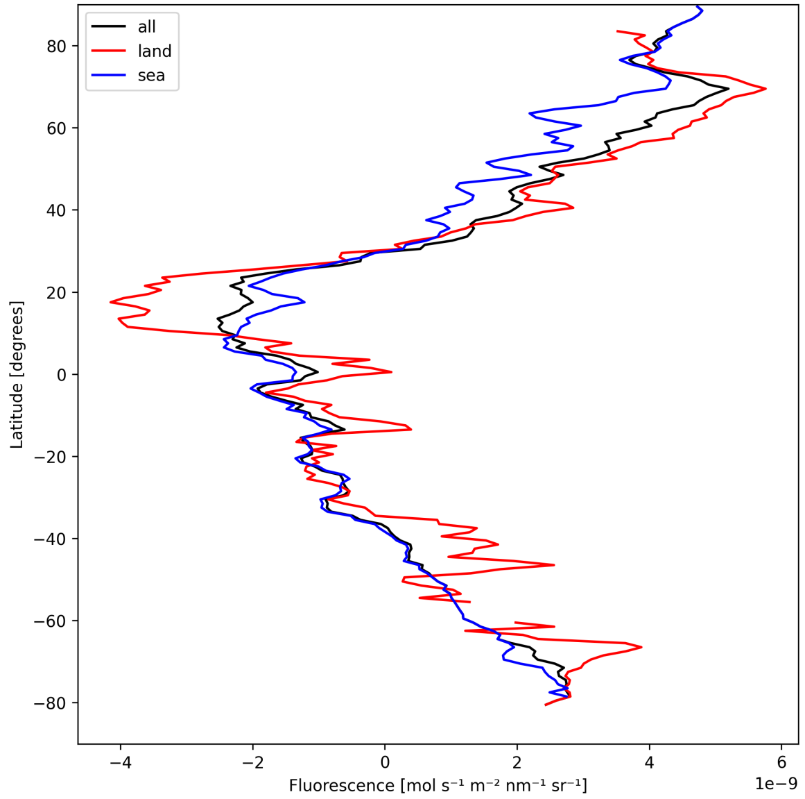
Figure 21: Zonal average of “Fluorescence” for 2025-04-09 to 2025-04-10.
