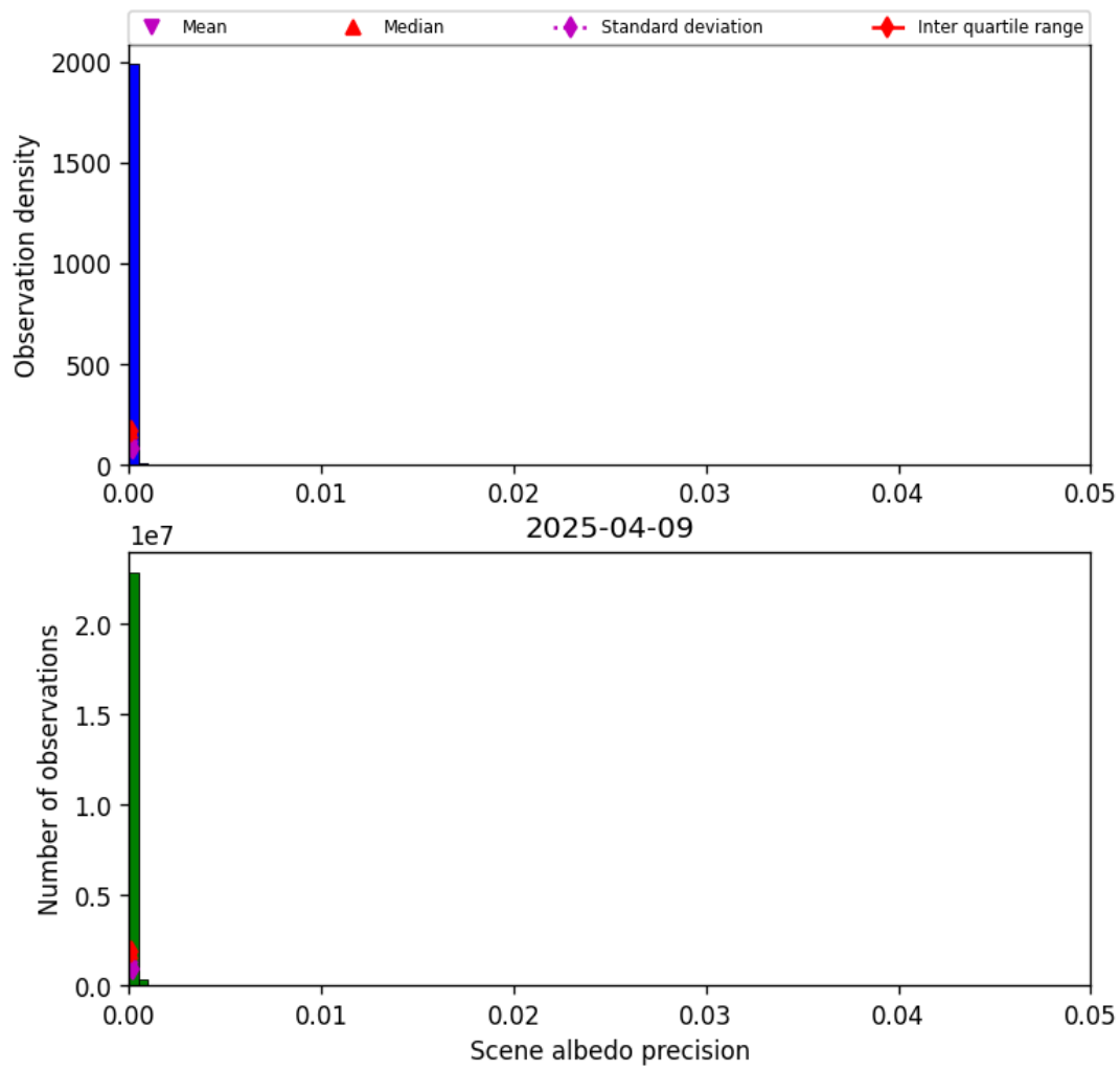
Figure 33: Histogram of “Scene albedo precision” for 2025-04-09 to 2025-04-10
