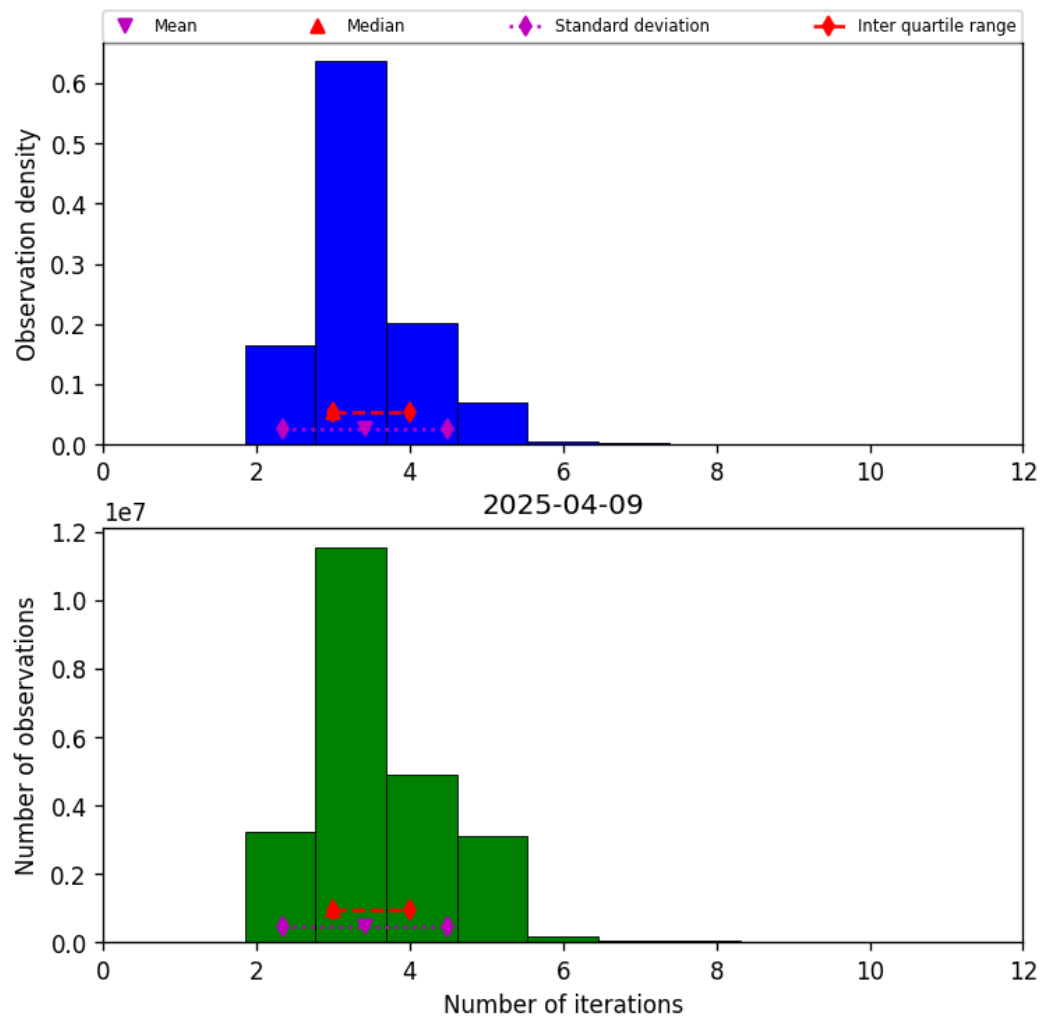
Figure 37: Histogram of “Number of iterations” for 2025-04-09 to 2025-04-10
