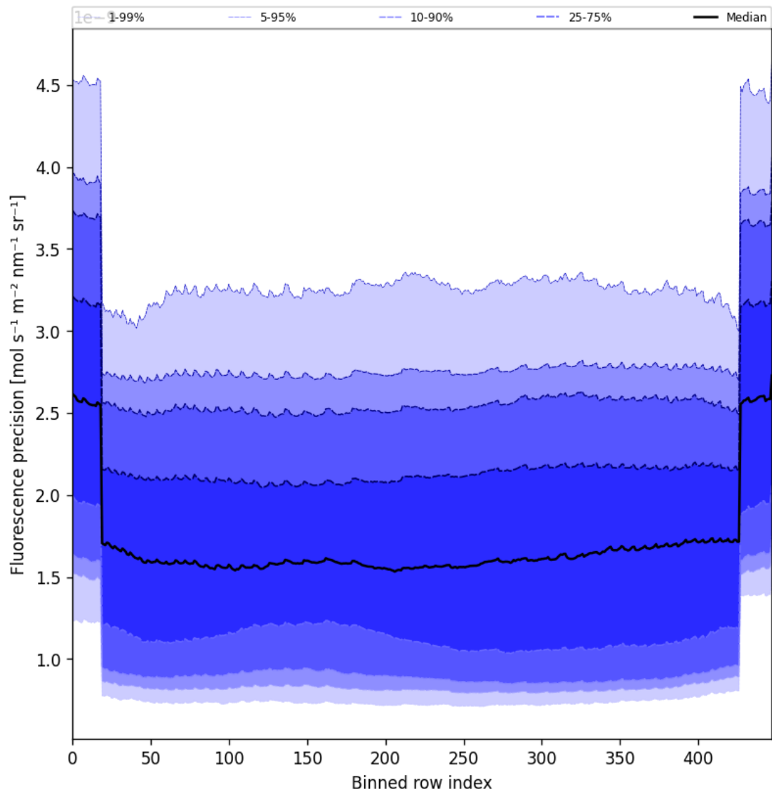
Figure 56: Along track statistics of “Fluorescence precision” for 2025-04-09 to 2025-04-10
