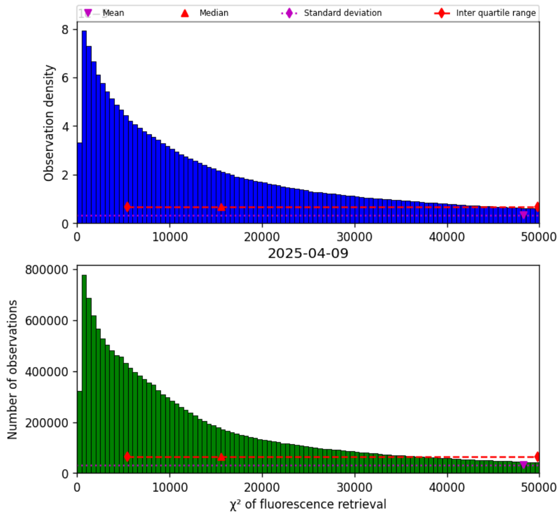
Figure 40: Histogram of “ \chi^2 of fluorescence retrieval” for 2025-04-09 to 2025-04-10
