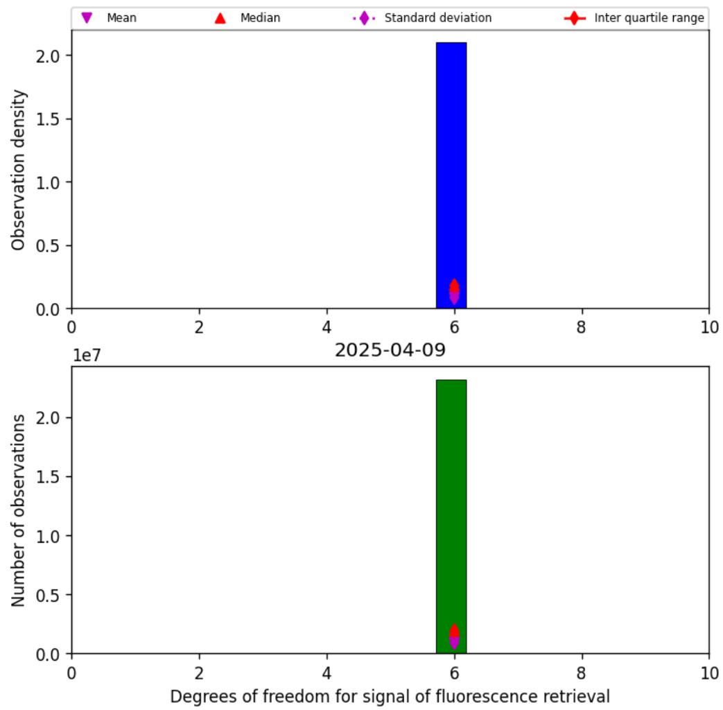
Figure 41: Histogram of “Degrees of freedom for signal of fluorescence retrieval” for 2025-04-09 to 2025-04-10
