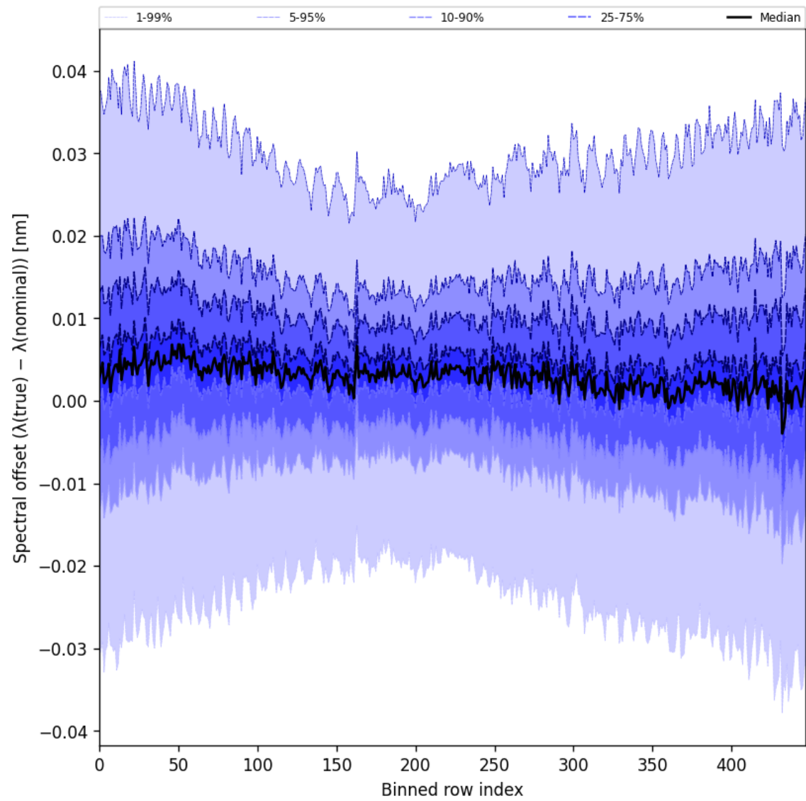
Figure 60: Along track statistics of “Spectral offset ( \lambda_{\text{true}} - \lambda_{\text{nominal}} )” for 2025-04-09 to 2025-04-10
