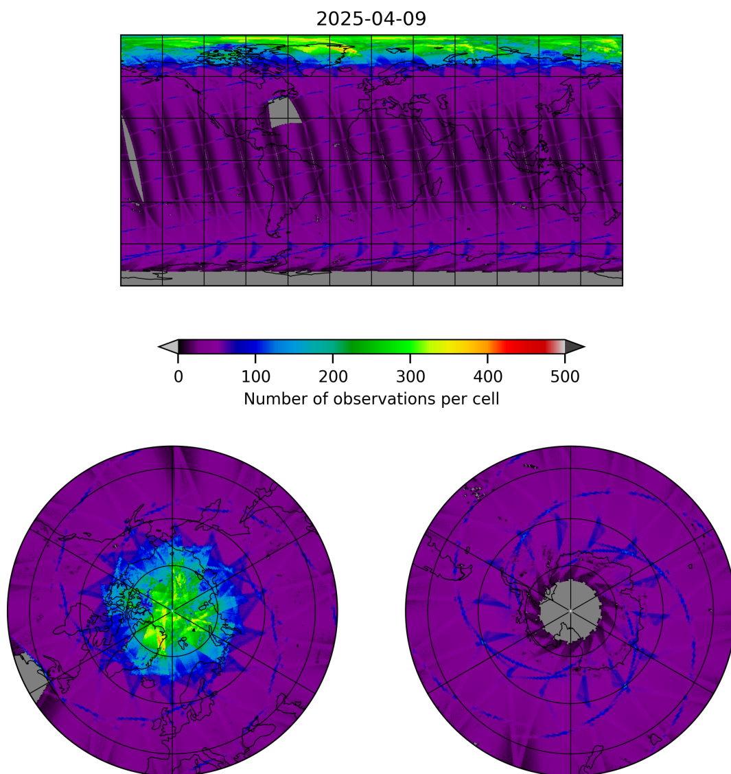
Figure 9: Map of the number of observations for 2025-04-09 to 2025-04-10
