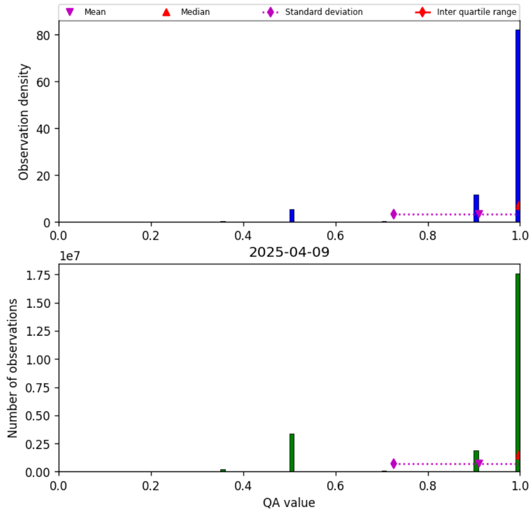
Figure 27: Histogram of “QA value” for 2025-04-09 to 2025-04-10
