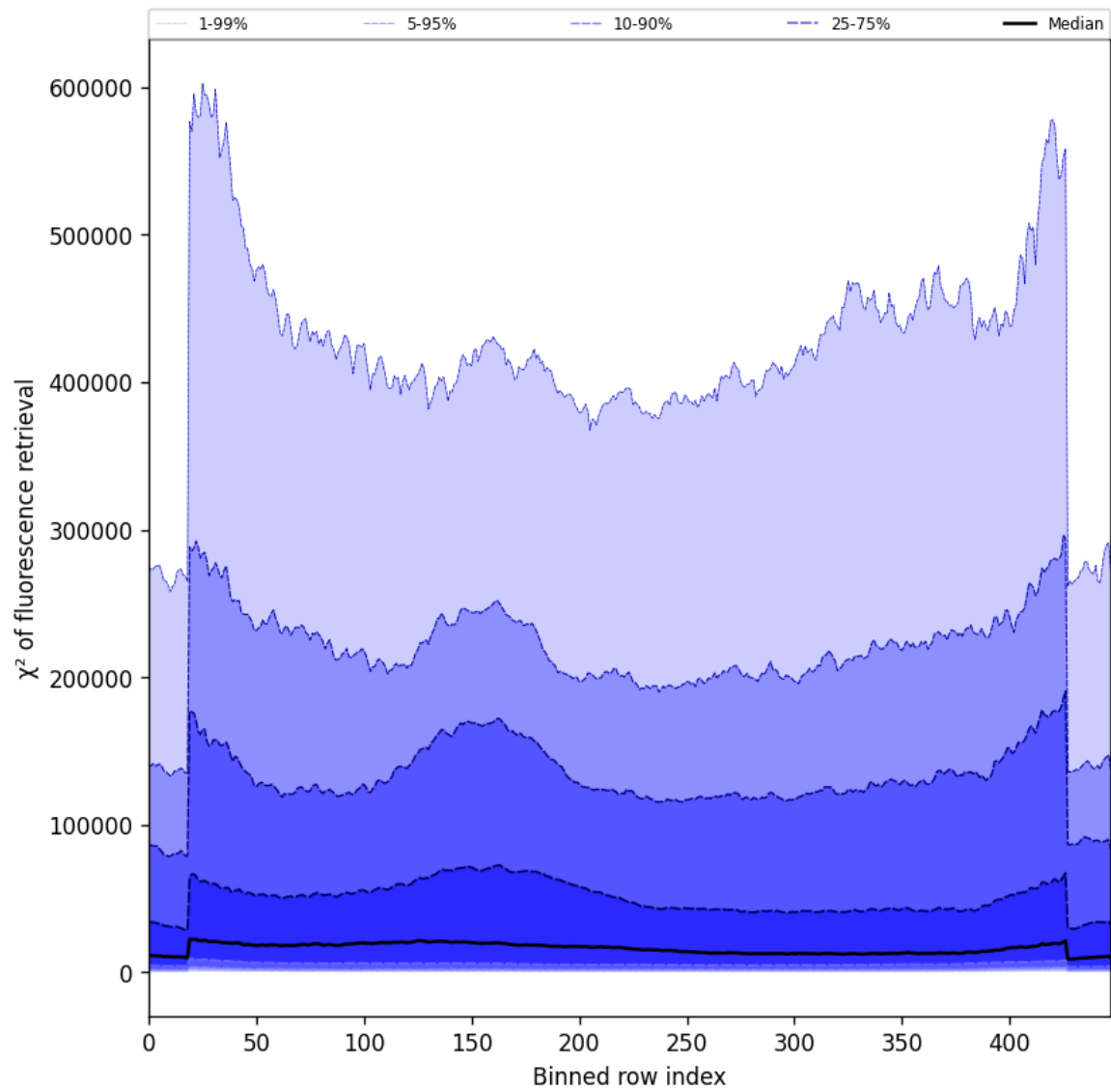
Figure 57: Along track statistics of “ \chi^2 of fluorescence retrieval” for 2025-04-09 to 2025-04-10
