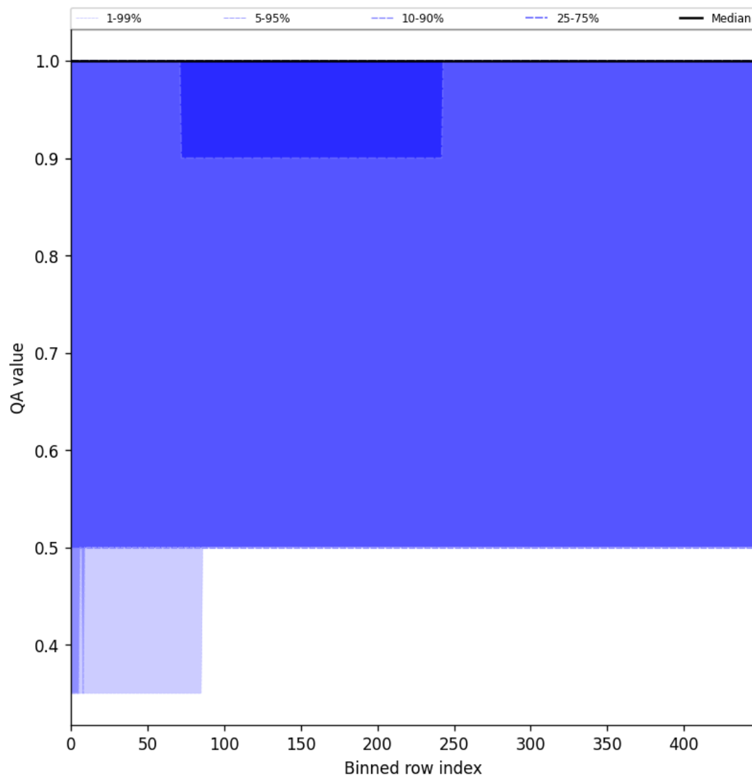
Figure 44: Along track statistics of “QA value” for 2025-04-09 to 2025-04-10
