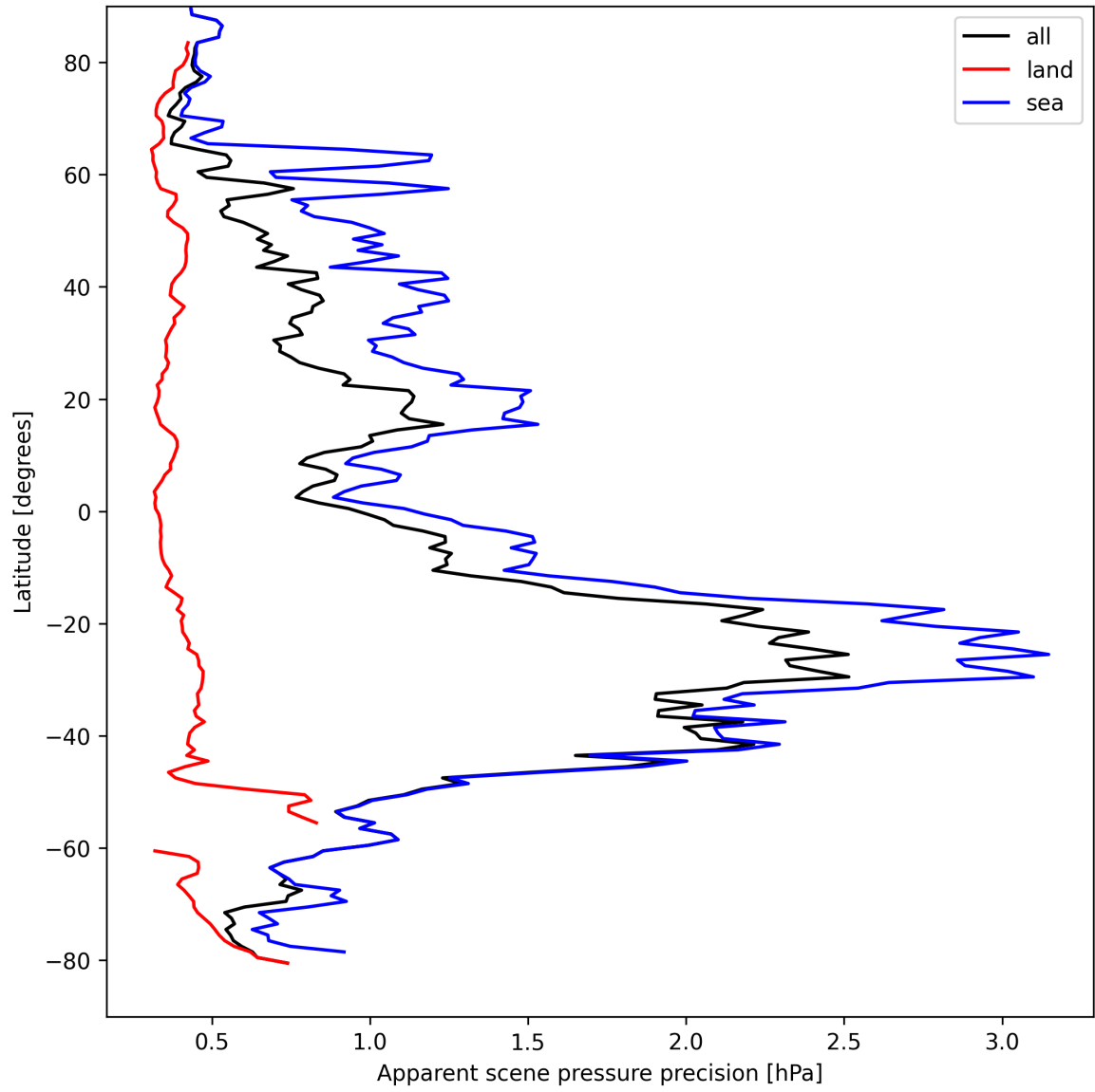
Figure 18: Zonal average of “Apparent scene pressure precision” for 2025-04-09 to 2025-04-10.
