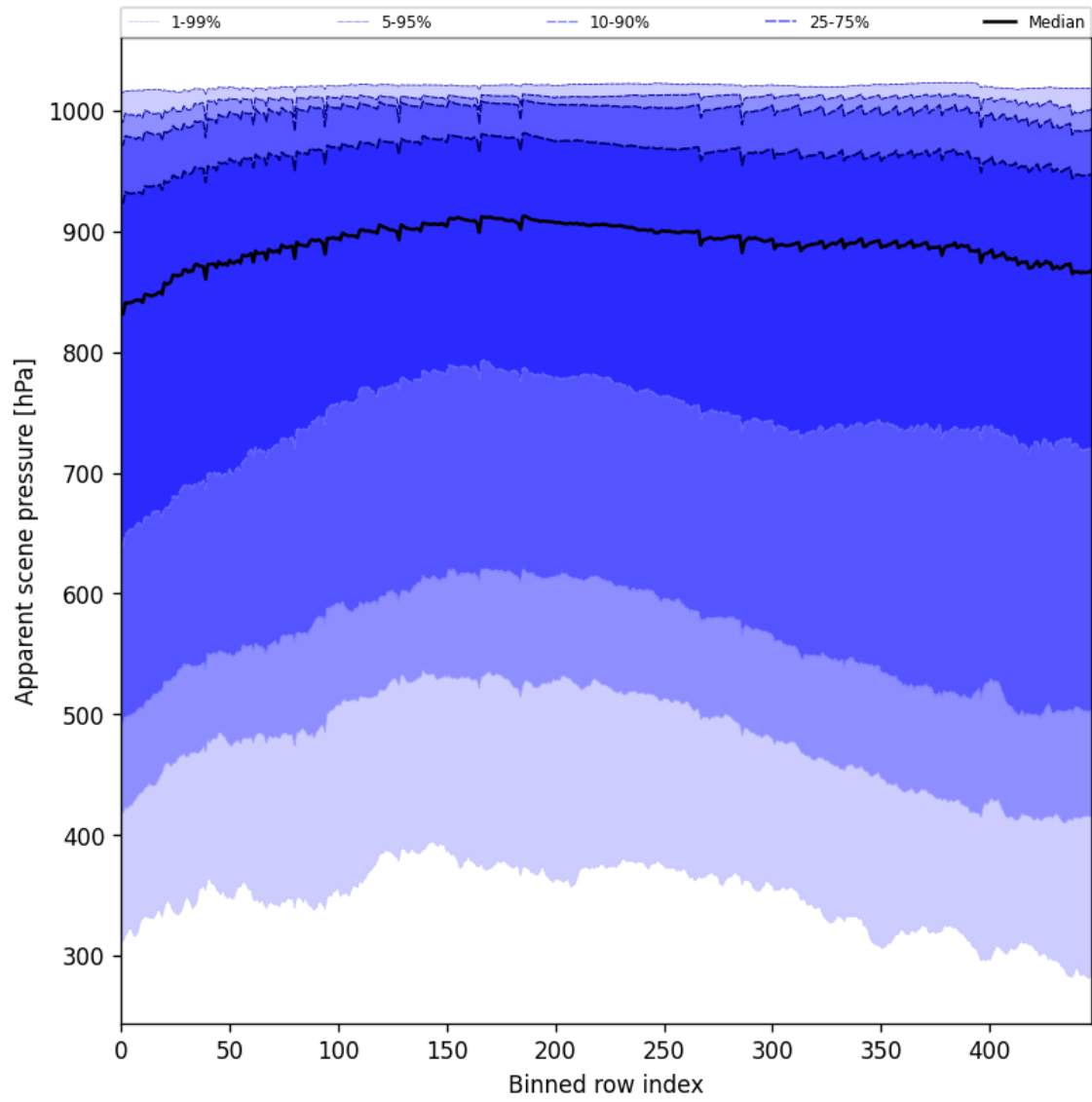
Figure 51: Along track statistics of “Apparent scene pressure” for 2025-04-09 to 2025-04-10
