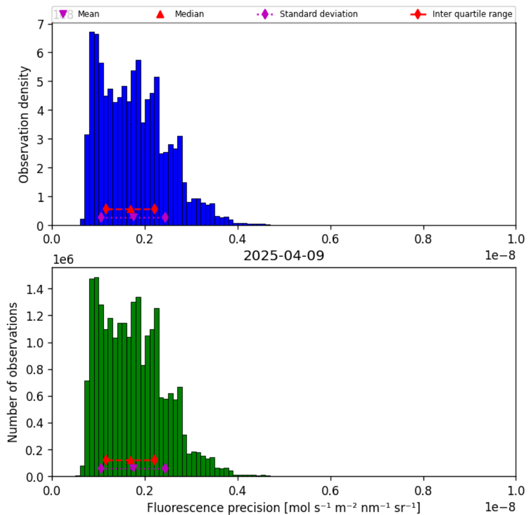
Figure 39: Histogram of “Fluorescence precision” for 2025-04-09 to 2025-04-10
