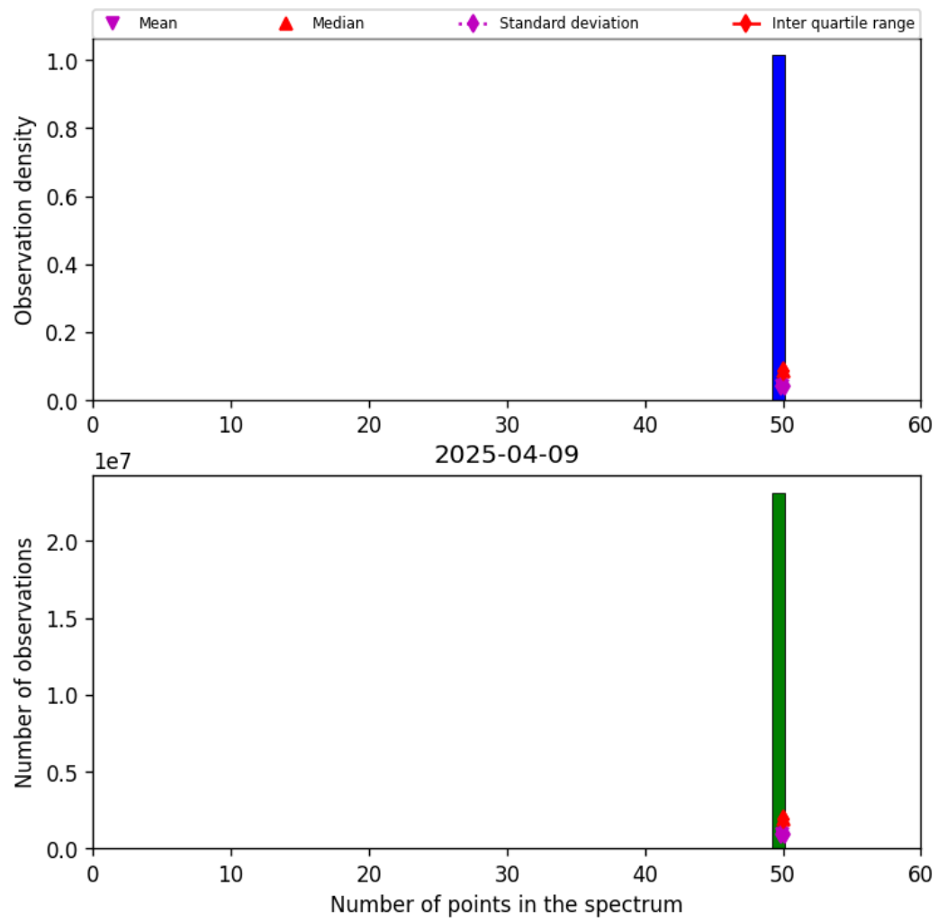
Figure 42: Histogram of “Number of points in the spectrum” for 2025-04-09 to 2025-04-10
