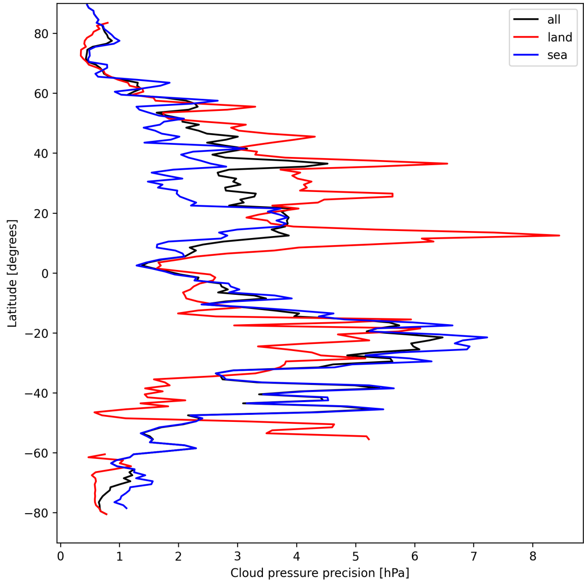
Figure 12: Zonal average of "Cloud pressure precision" for 2025-04-09 to 2025-04-10.
