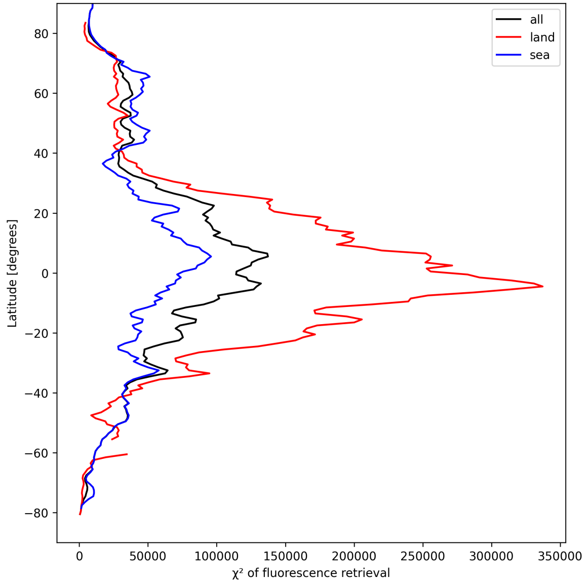
Figure 23: Zonal average of “ \chi^2 of fluorescence retrieval” for 2025-04-09 to 2025-04-10.
