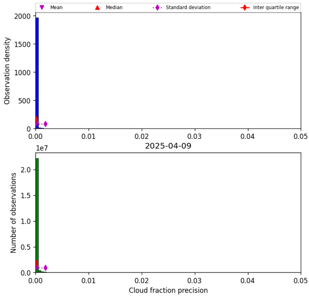
Figure 31: Histogram of “Cloud fraction precision” for 2025-04-09 to 2025-04-10
