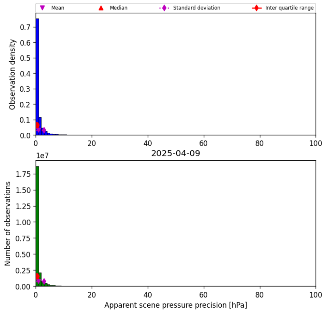
Figure 35: Histogram of “Apparent scene pressure precision” for 2025-04-09 to 2025-04-10
