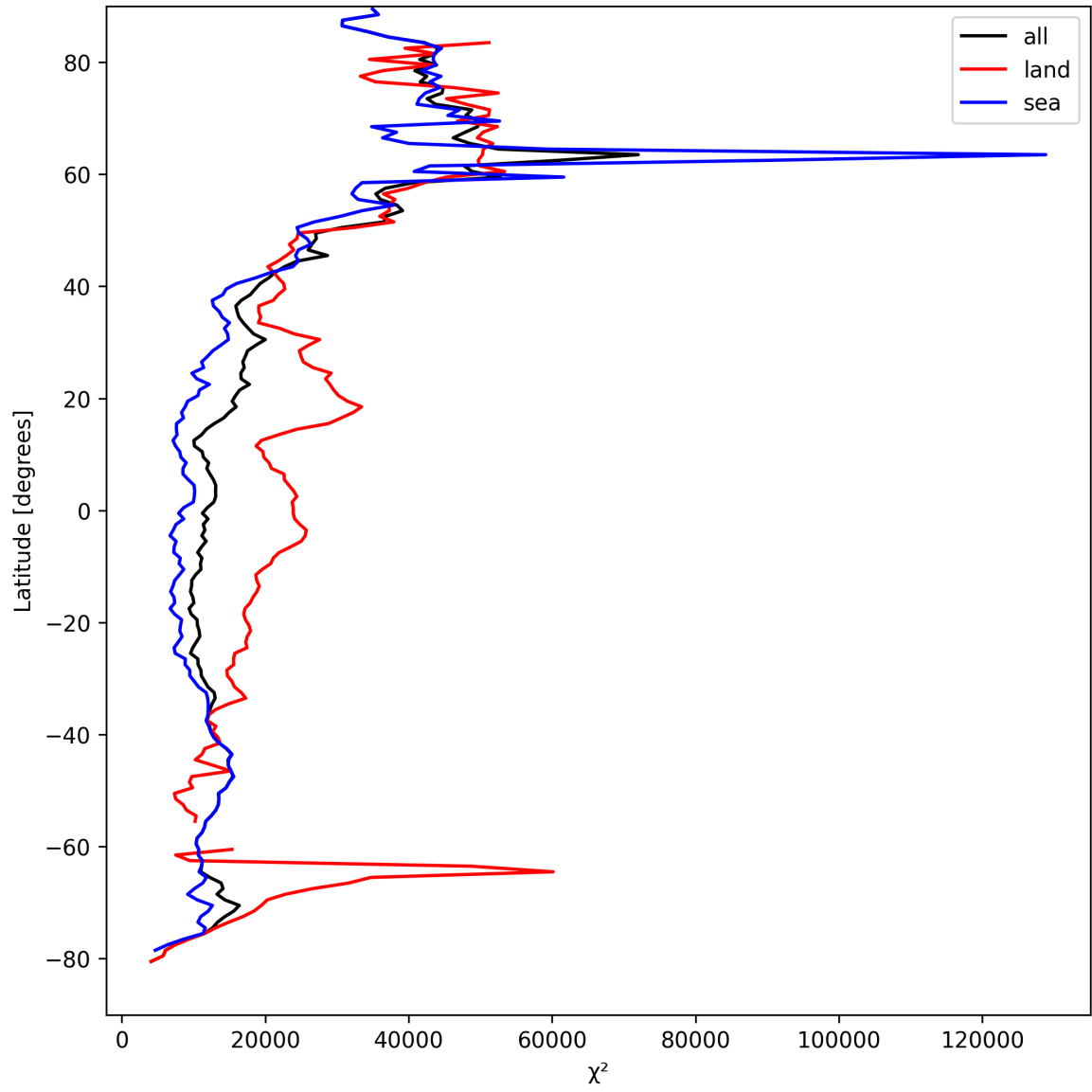
Figure 19: Zonal average of “ \chi^2 ” for 2025-04-09 to 2025-04-10.
