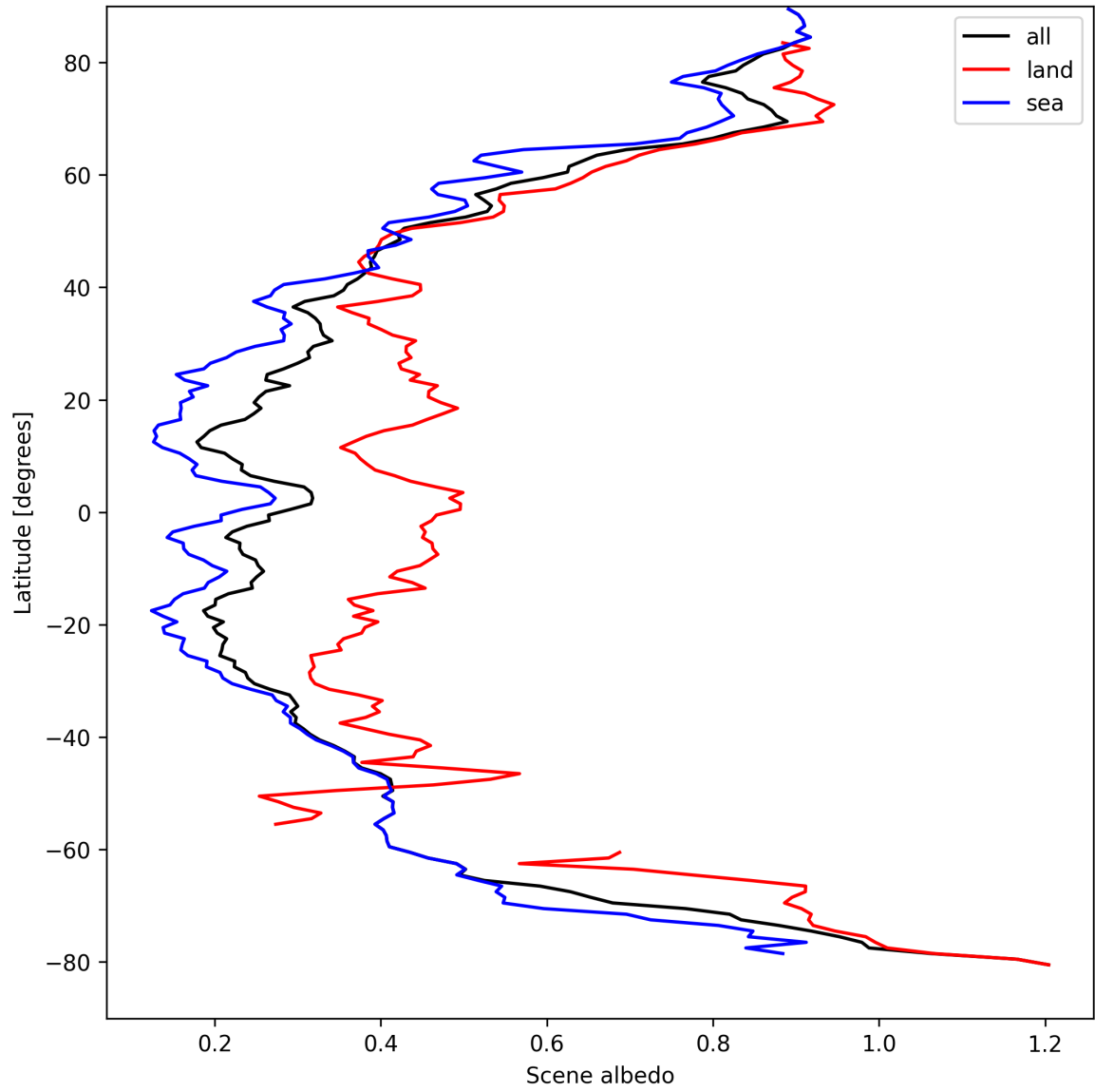
Figure 15: Zonal average of “Scene albedo” for 2025-04-09 to 2025-04-10.
