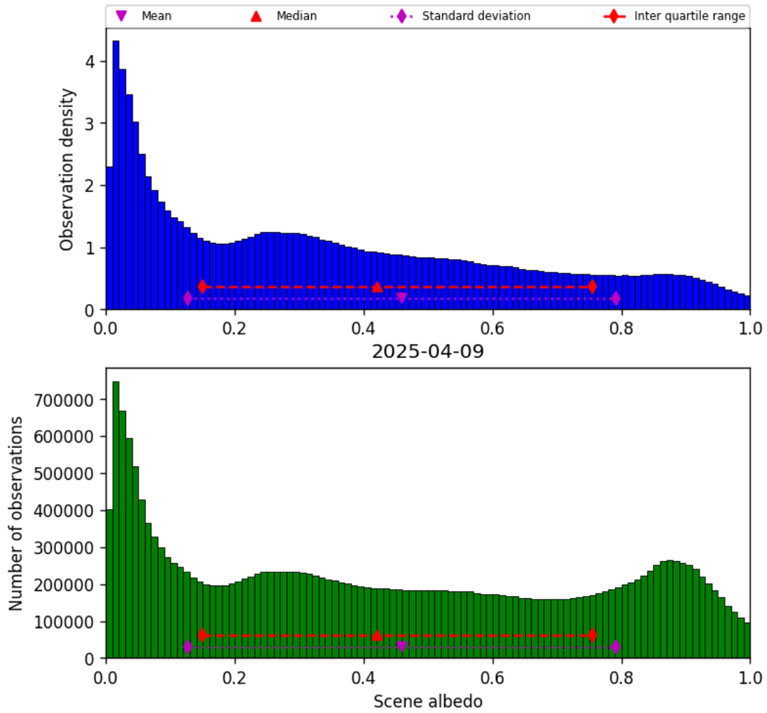
Figure 32: Histogram of “Scene albedo” for 2025-04-09 to 2025-04-10
