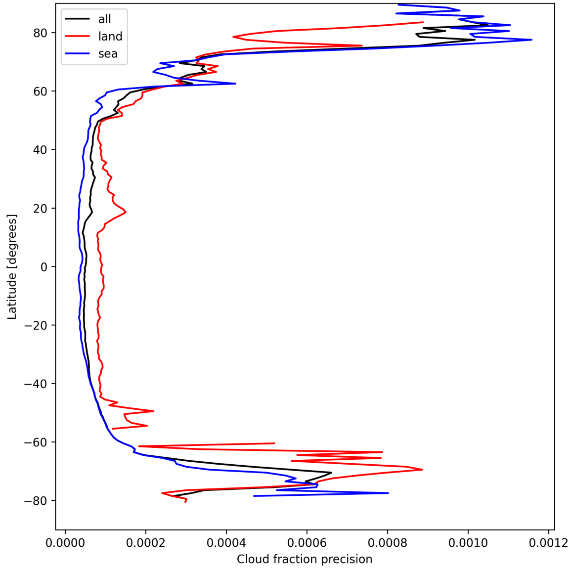
Figure 14: Zonal average of “Cloud fraction precision” for 2025-04-09 to 2025-04-10.
