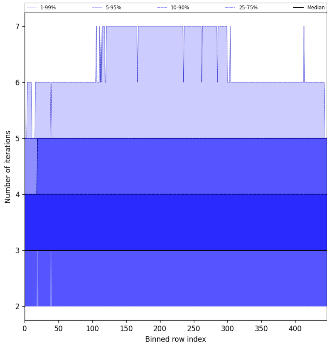
Figure 54: Along track statistics of “Number of iterations” for 2025-04-09 to 2025-04-10
