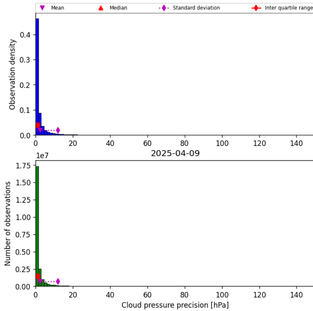
Figure 29: Histogram of “Cloud pressure precision” for 2025-04-09 to 2025-04-10
