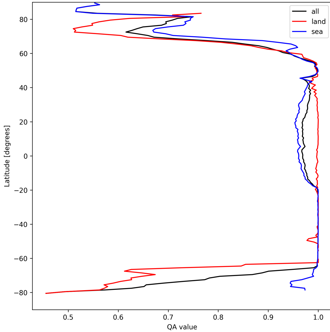
Figure 10: Zonal average of “QA value” for 2025-04-09 to 2025-04-10.
