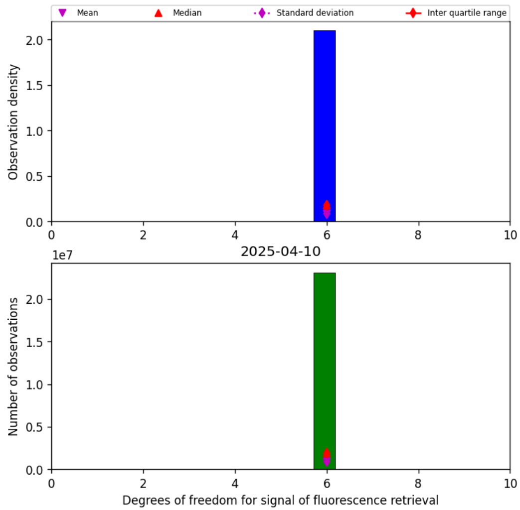
Figure 41: Histogram of “Degrees of freedom for signal of fluorescence retrieval” for 2025-04-10 to 2025-04-11
