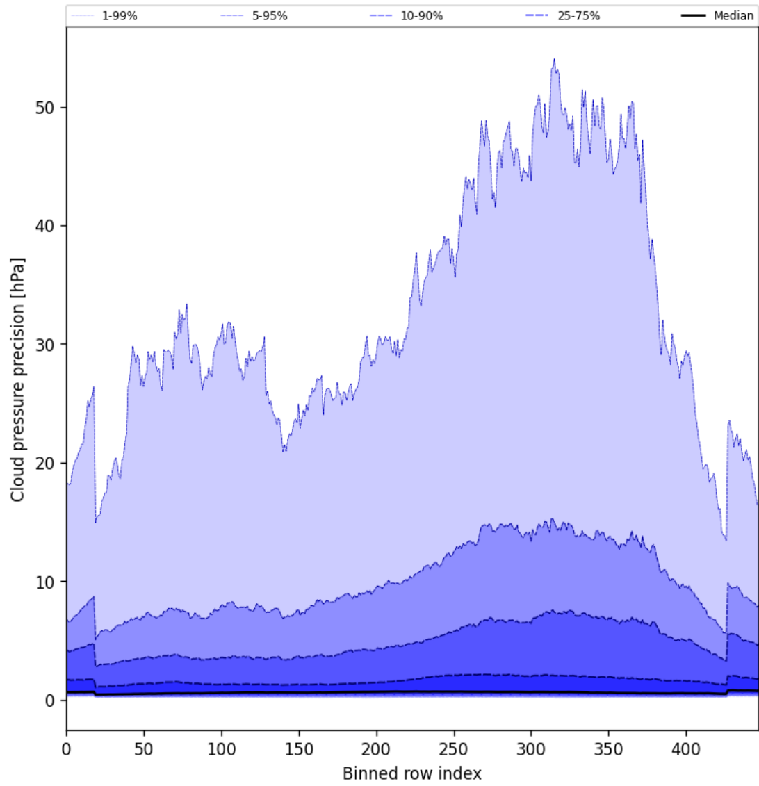
Figure 46: Along track statistics of “Cloud pressure precision” for 2025-04-10 to 2025-04-11
