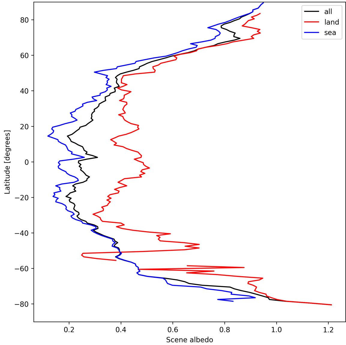
Figure 15: Zonal average of “Scene albedo” for 2025-04-10 to 2025-04-11.
