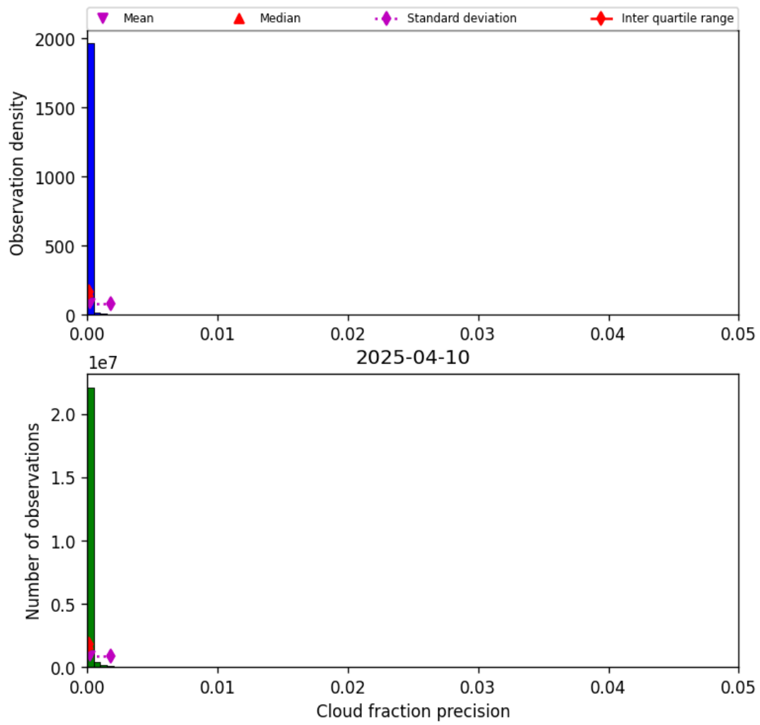
Figure 31: Histogram of “Cloud fraction precision” for 2025-04-10 to 2025-04-11
