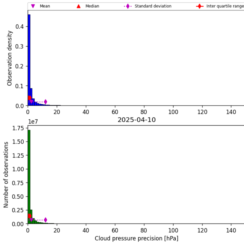
Figure 29: Histogram of "Cloud pressure precision" for 2025-04-10 to 2025-04-11
