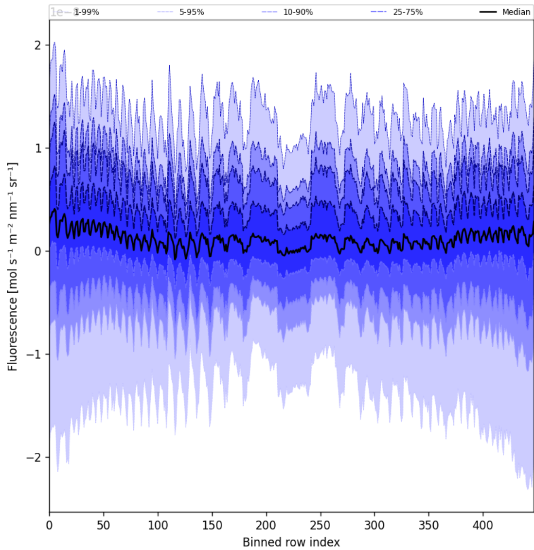
Figure 55: Along track statistics of “Fluorescence” for 2025-04-10 to 2025-04-11
