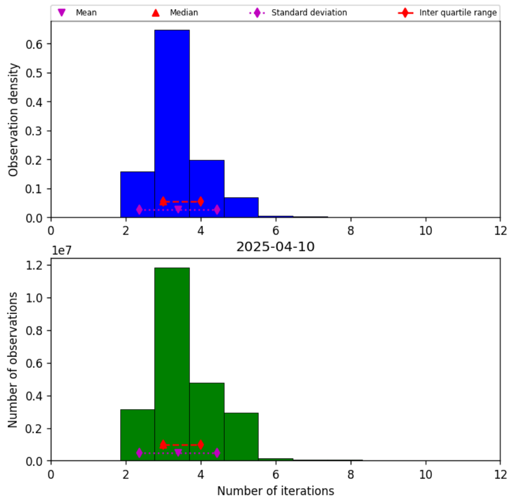
Figure 37: Histogram of “Number of iterations” for 2025-04-10 to 2025-04-11
