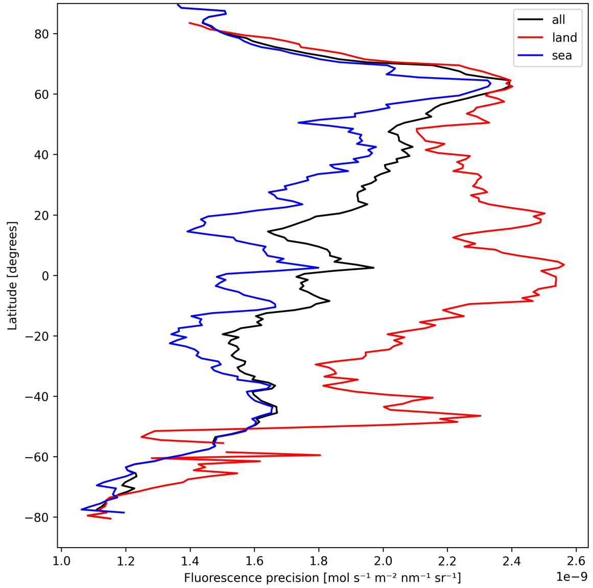
Figure 22: Zonal average of “Fluorescence precision” for 2025-04-10 to 2025-04-11.
