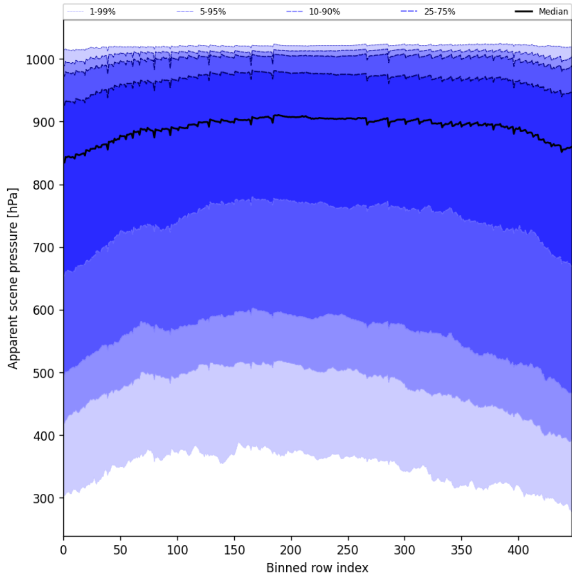
Figure 51: Along track statistics of “Apparent scene pressure” for 2025-04-10 to 2025-04-11
