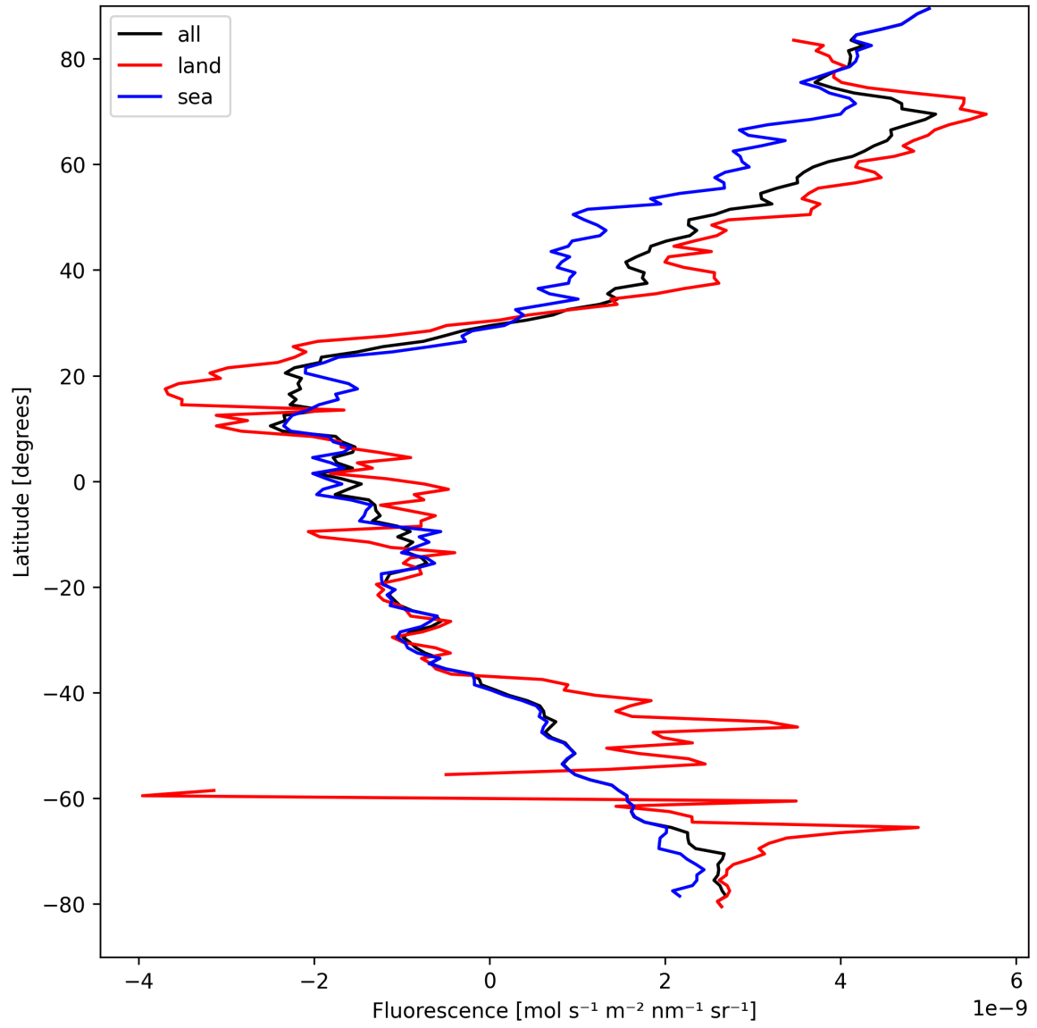
Figure 21: Zonal average of “Fluorescence” for 2025-04-10 to 2025-04-11.
