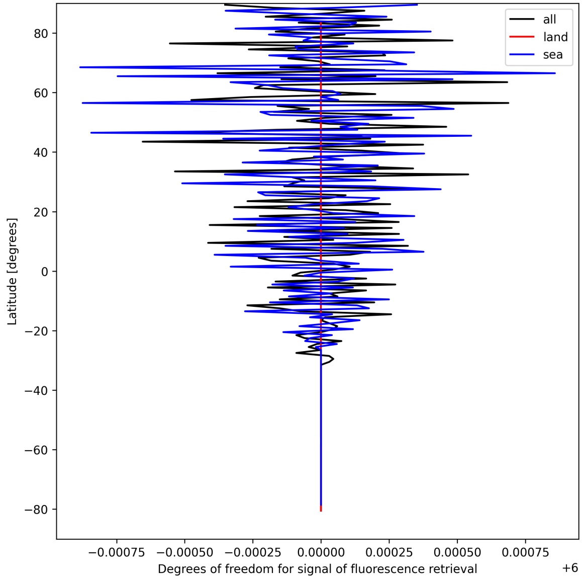
Figure 24: Zonal average of “Degrees of freedom for signal of fluorescence retrieval” for 2025-04-10 to 2025-04-11.
