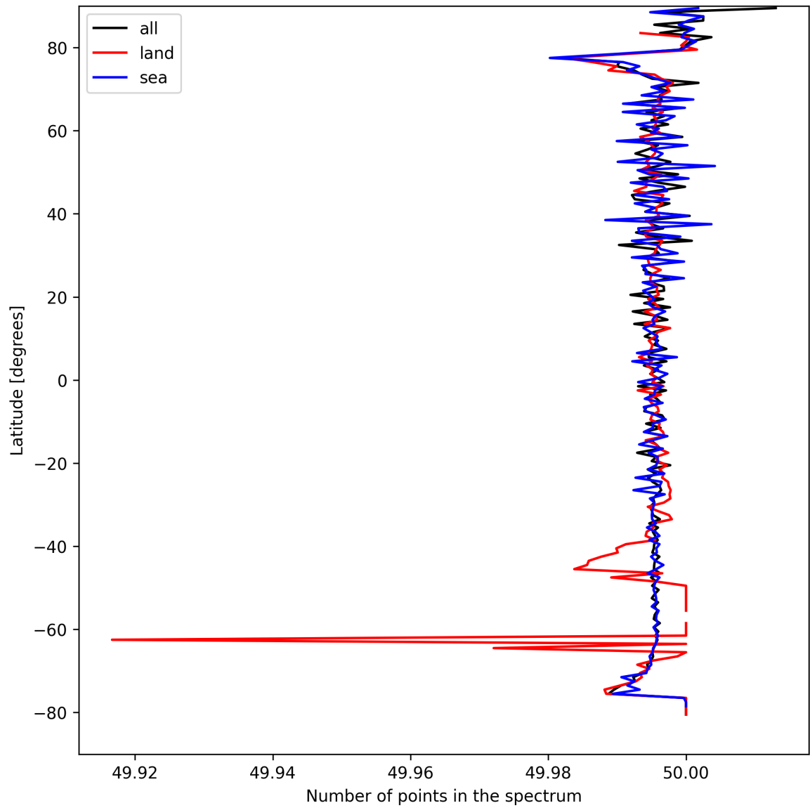
Figure 25: Zonal average of “Number of points in the spectrum” for 2025-04-10 to 2025-04-11.
