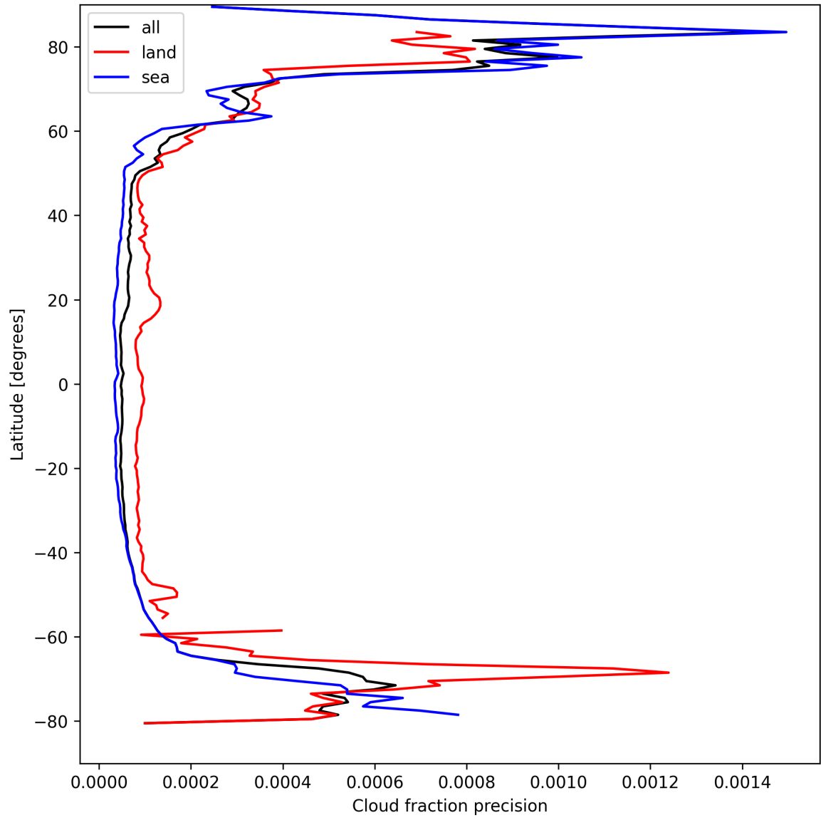
Figure 14: Zonal average of “Cloud fraction precision” for 2025-04-10 to 2025-04-11.
