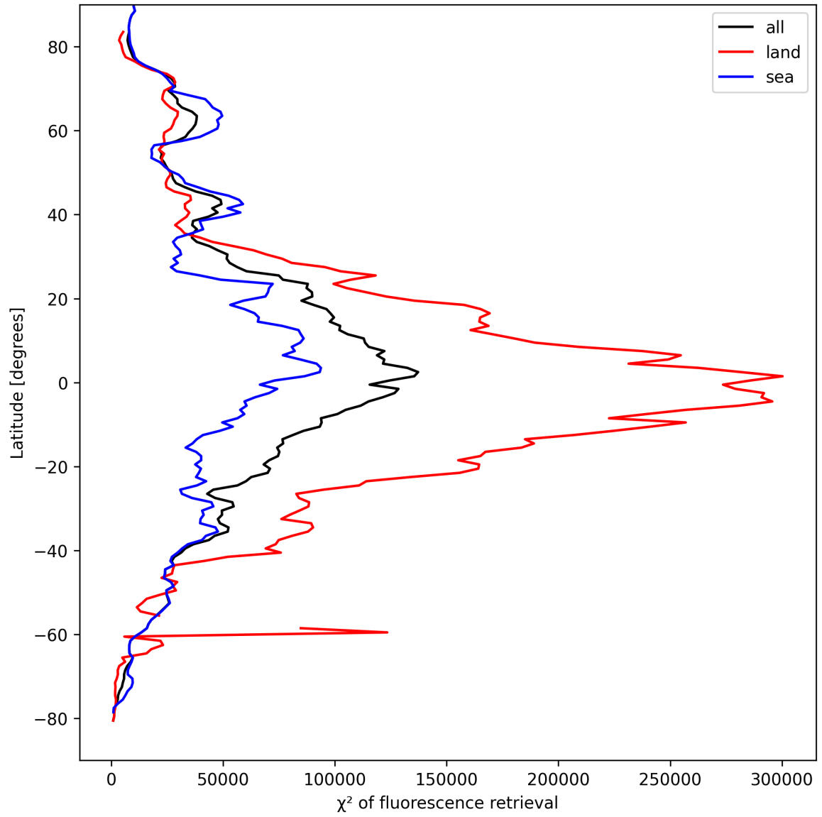
Figure 23: Zonal average of “ \chi^2 of fluorescence retrieval” for 2025-04-10 to 2025-04-11.
