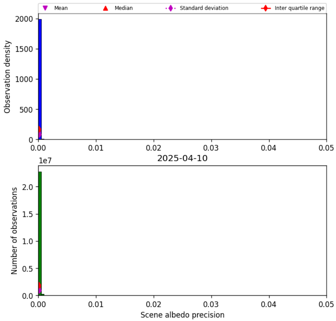
Figure 33: Histogram of “Scene albedo precision” for 2025-04-10 to 2025-04-11
