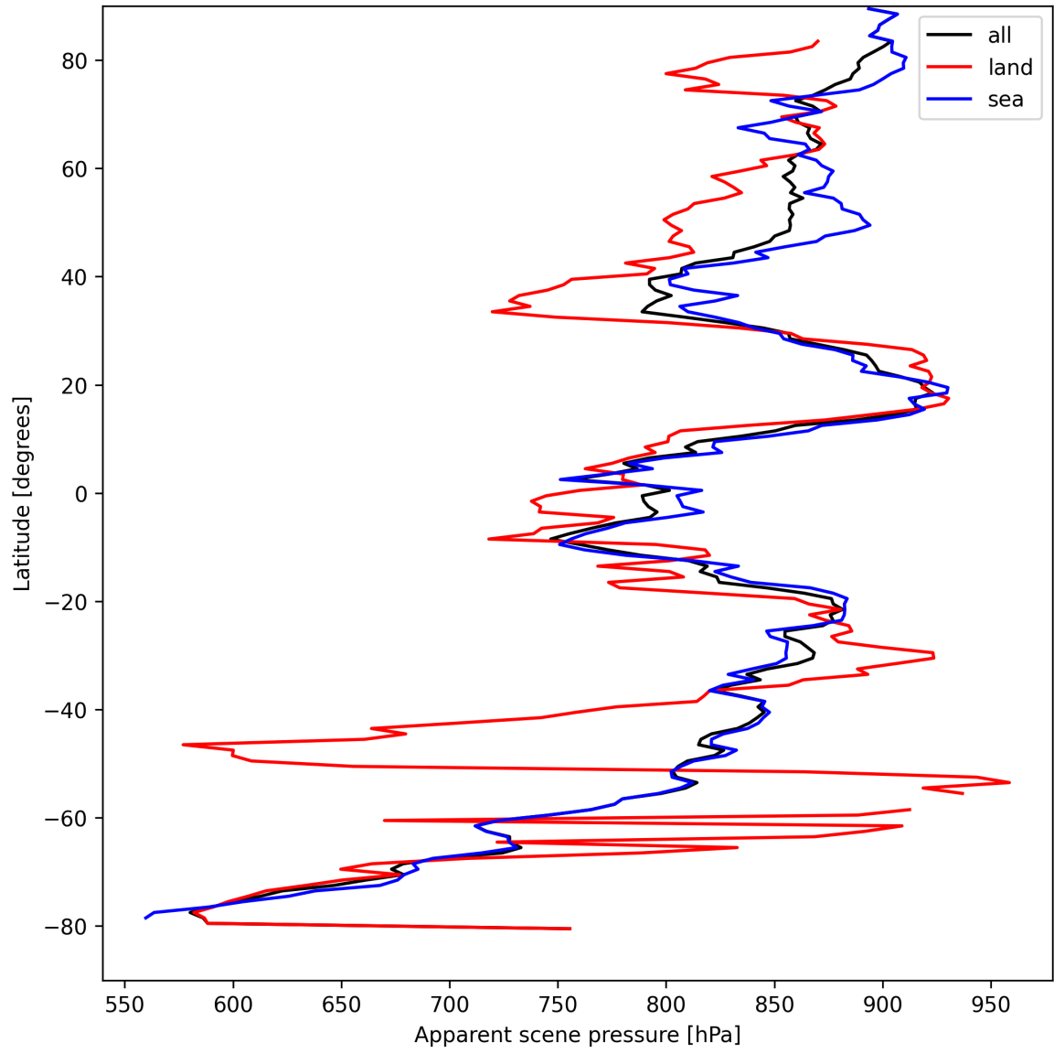
Figure 17: Zonal average of “Apparent scene pressure” for 2025-04-10 to 2025-04-11.
