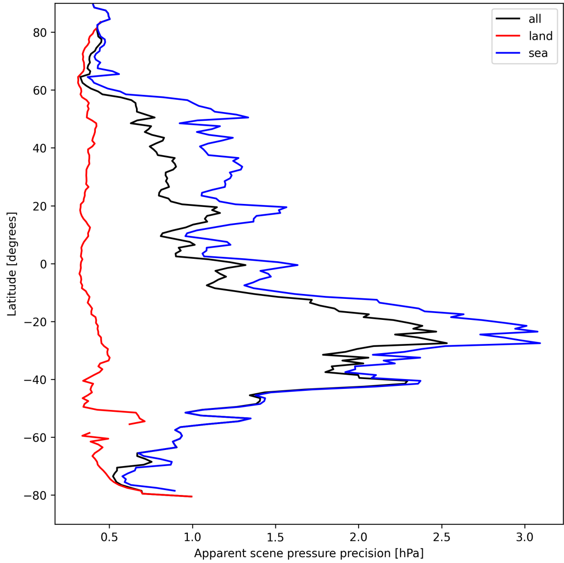
Figure 18: Zonal average of “Apparent scene pressure precision” for 2025-04-10 to 2025-04-11.
