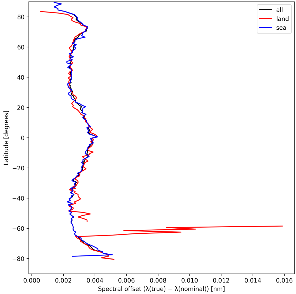
Figure 26: Zonal average of “Spectral offset ( \lambda_{\text{true}} - \lambda_{\text{nominal}} )” for 2025-04-10 to 2025-04-11.
