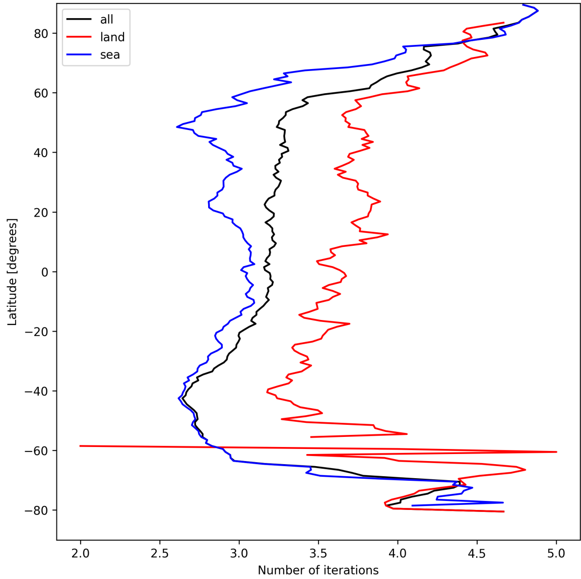
Figure 20: Zonal average of “Number of iterations” for 2025-04-10 to 2025-04-11.
