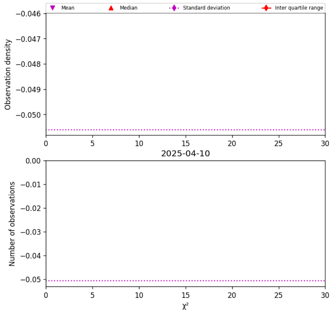
Figure 36: Histogram of “ \chi^2 ” for 2025-04-10 to 2025-04-11
