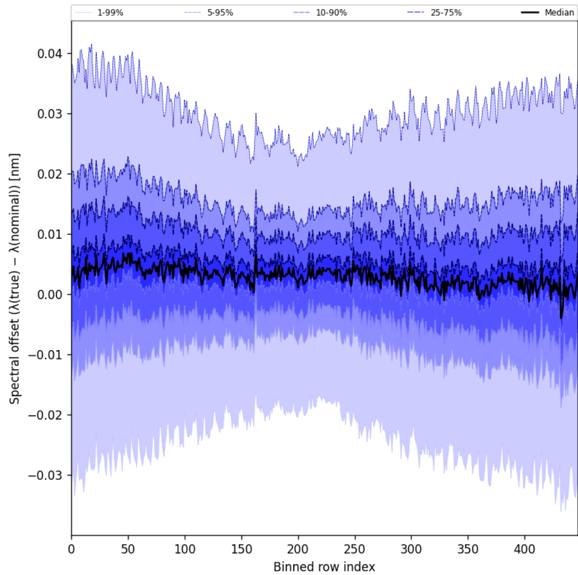
Figure 60: Along track statistics of “Spectral offset ( \lambda_{\text{true}} - \lambda_{\text{nominal}} )” for 2025-04-10 to 2025-04-11
