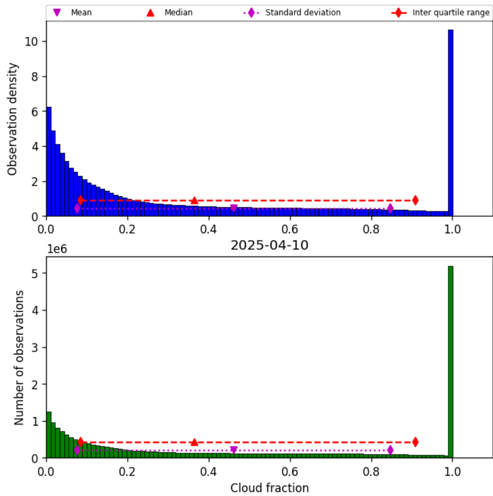
Figure 30: Histogram of “Cloud fraction” for 2025-04-10 to 2025-04-11
