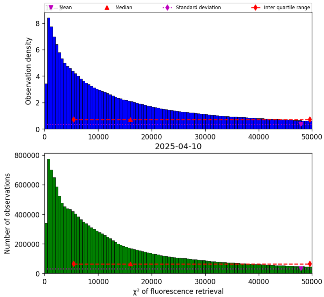
Figure 40: Histogram of “ \chi^2 of fluorescence retrieval” for 2025-04-10 to 2025-04-11
