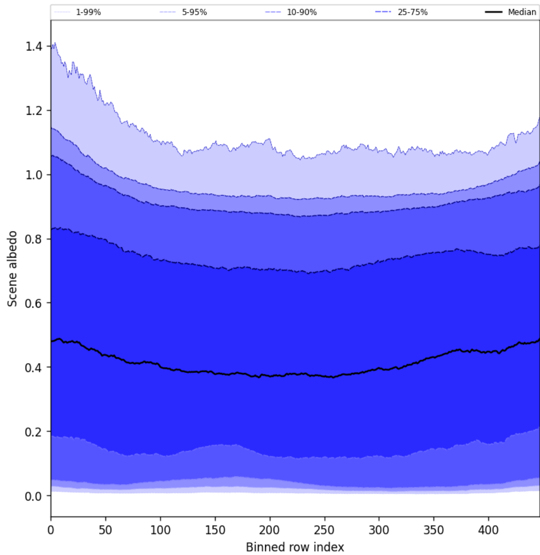
Figure 49: Along track statistics of “Scene albedo” for 2025-04-10 to 2025-04-11
