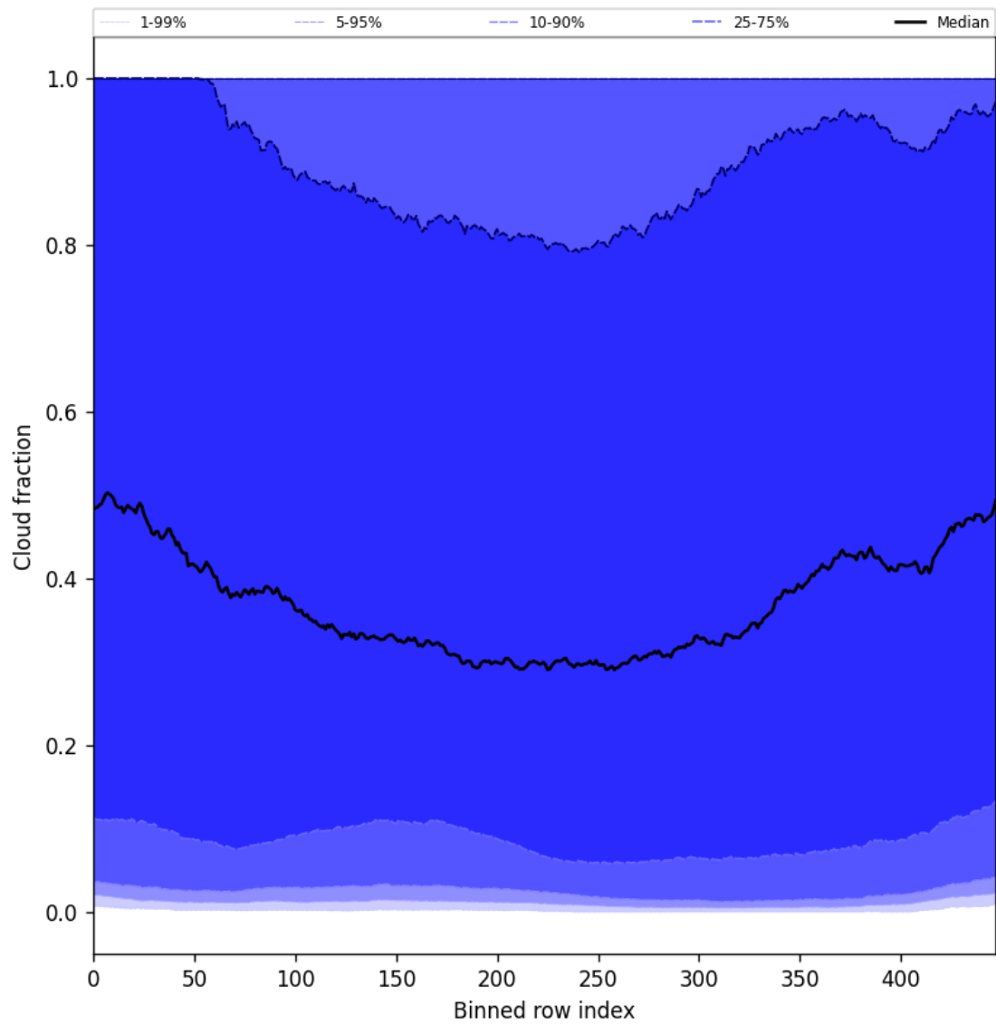
Figure 47: Along track statistics of “Cloud fraction” for 2025-04-10 to 2025-04-11
