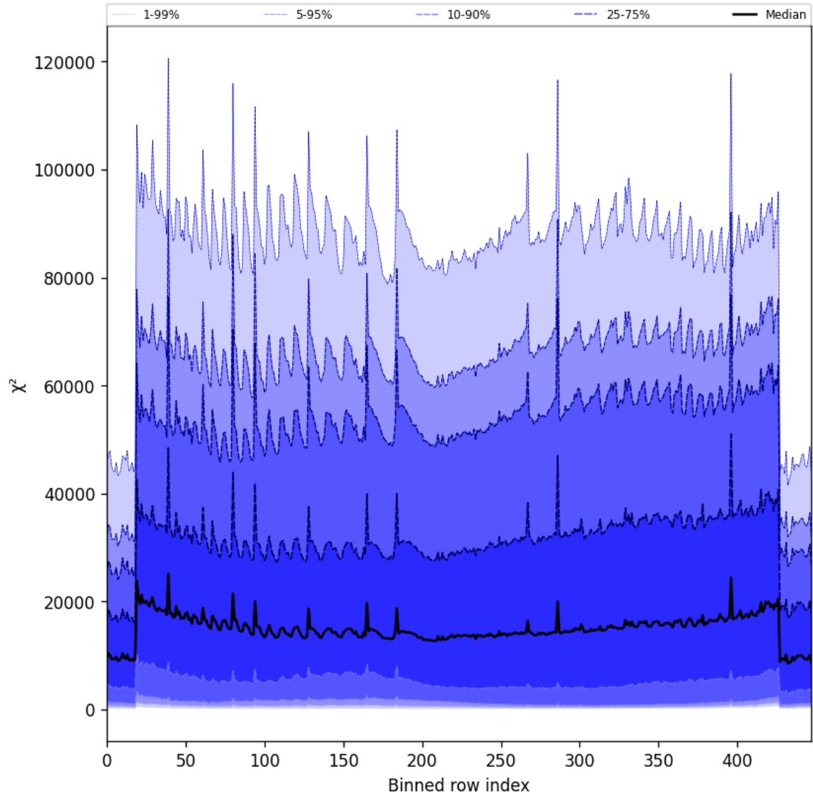
Figure 53: Along track statistics of “ \chi^2 ” for 2025-04-10 to 2025-04-11
