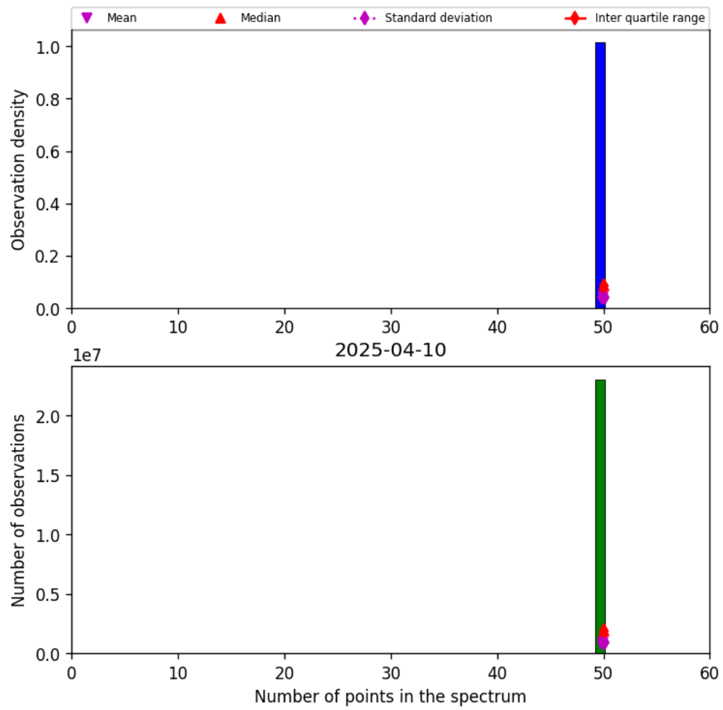
Figure 42: Histogram of “Number of points in the spectrum” for 2025-04-10 to 2025-04-11
