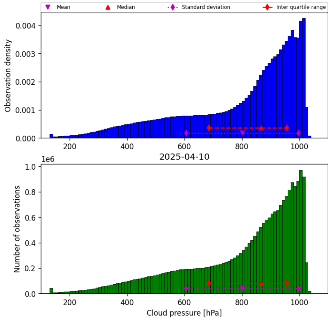
Figure 28: Histogram of “Cloud pressure” for 2025-04-10 to 2025-04-11
