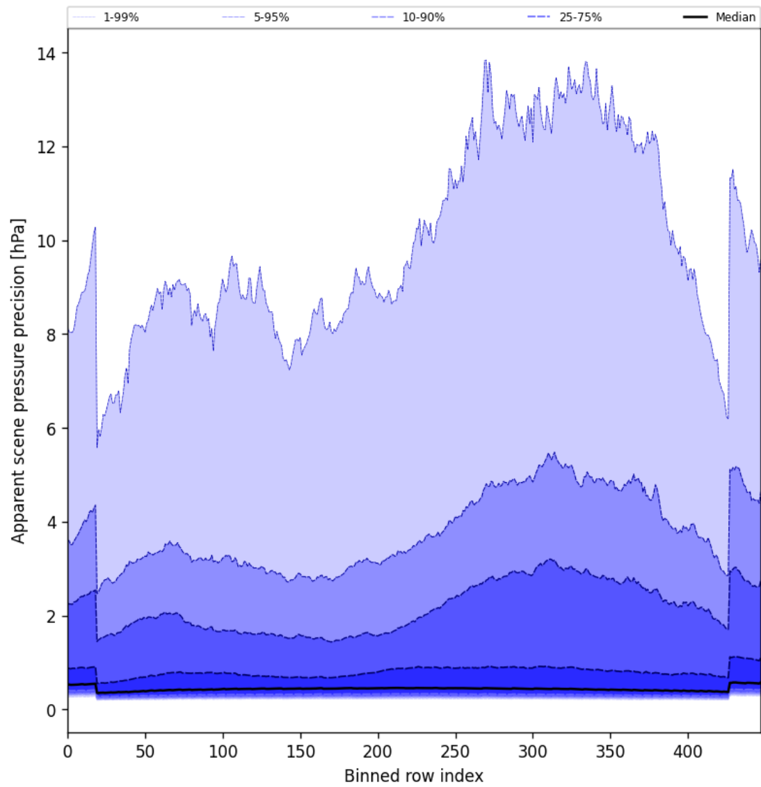
Figure 52: Along track statistics of “Apparent scene pressure precision” for 2025-04-10 to 2025-04-11
