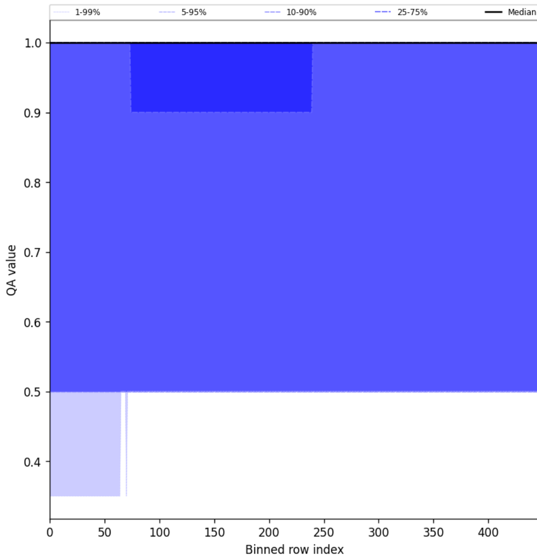
Figure 44: Along track statistics of “QA value” for 2025-04-10 to 2025-04-11
