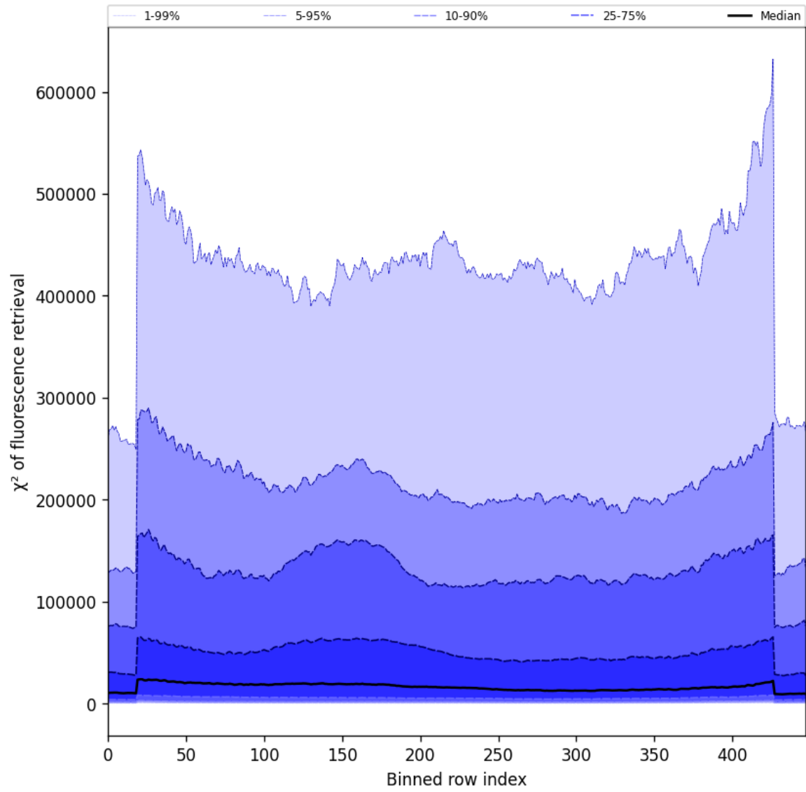
Figure 57: Along track statistics of " \chi^2 of fluorescence retrieval" for 2025-04-10 to 2025-04-11
