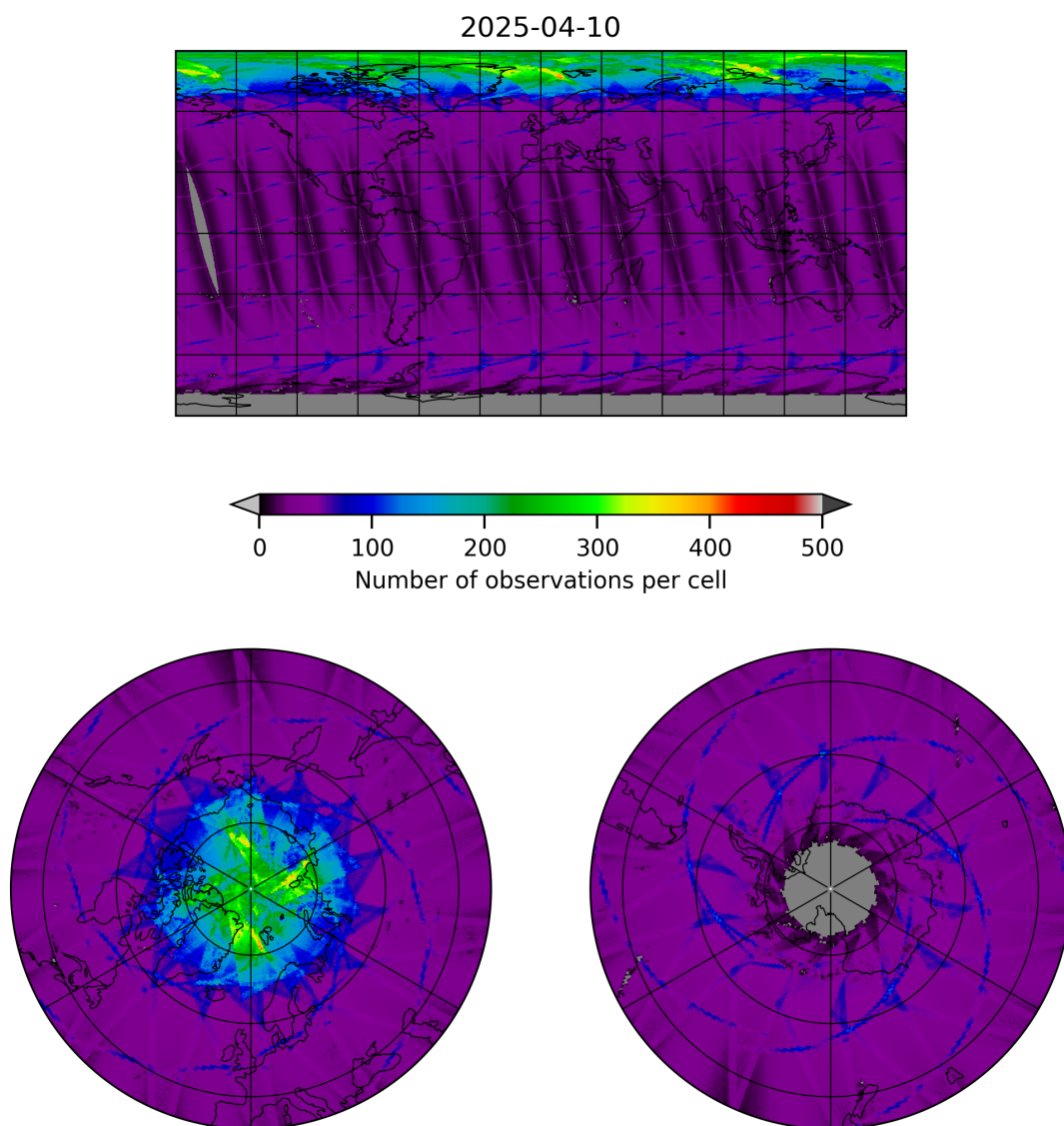
Figure 9: Map of the number of observations for 2025-04-10 to 2025-04-11
