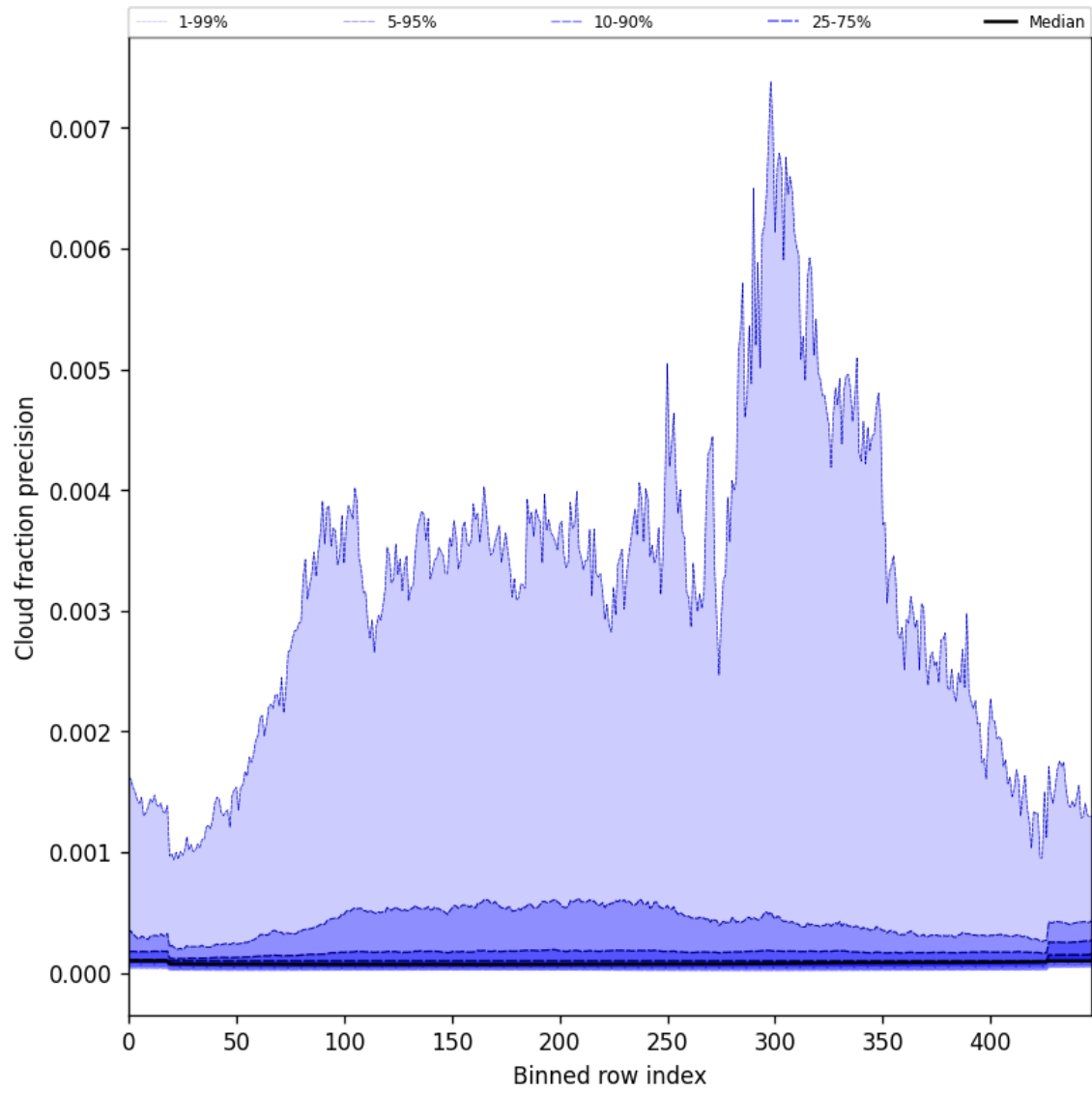
Figure 48: Along track statistics of “Cloud fraction precision” for 2025-04-10 to 2025-04-11
