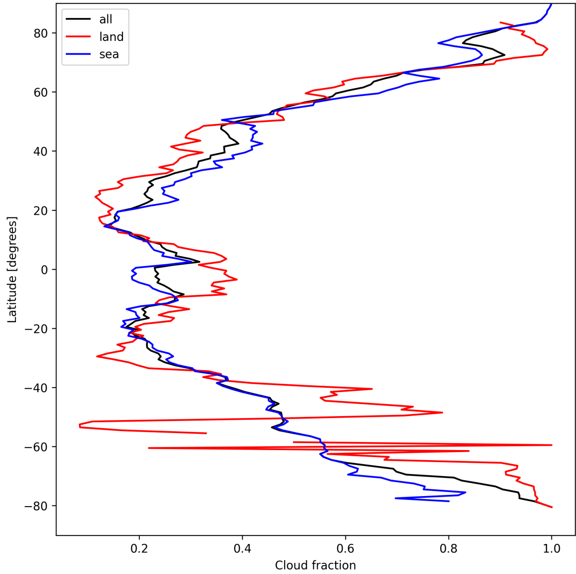
Figure 13: Zonal average of “Cloud fraction” for 2025-04-10 to 2025-04-11.
