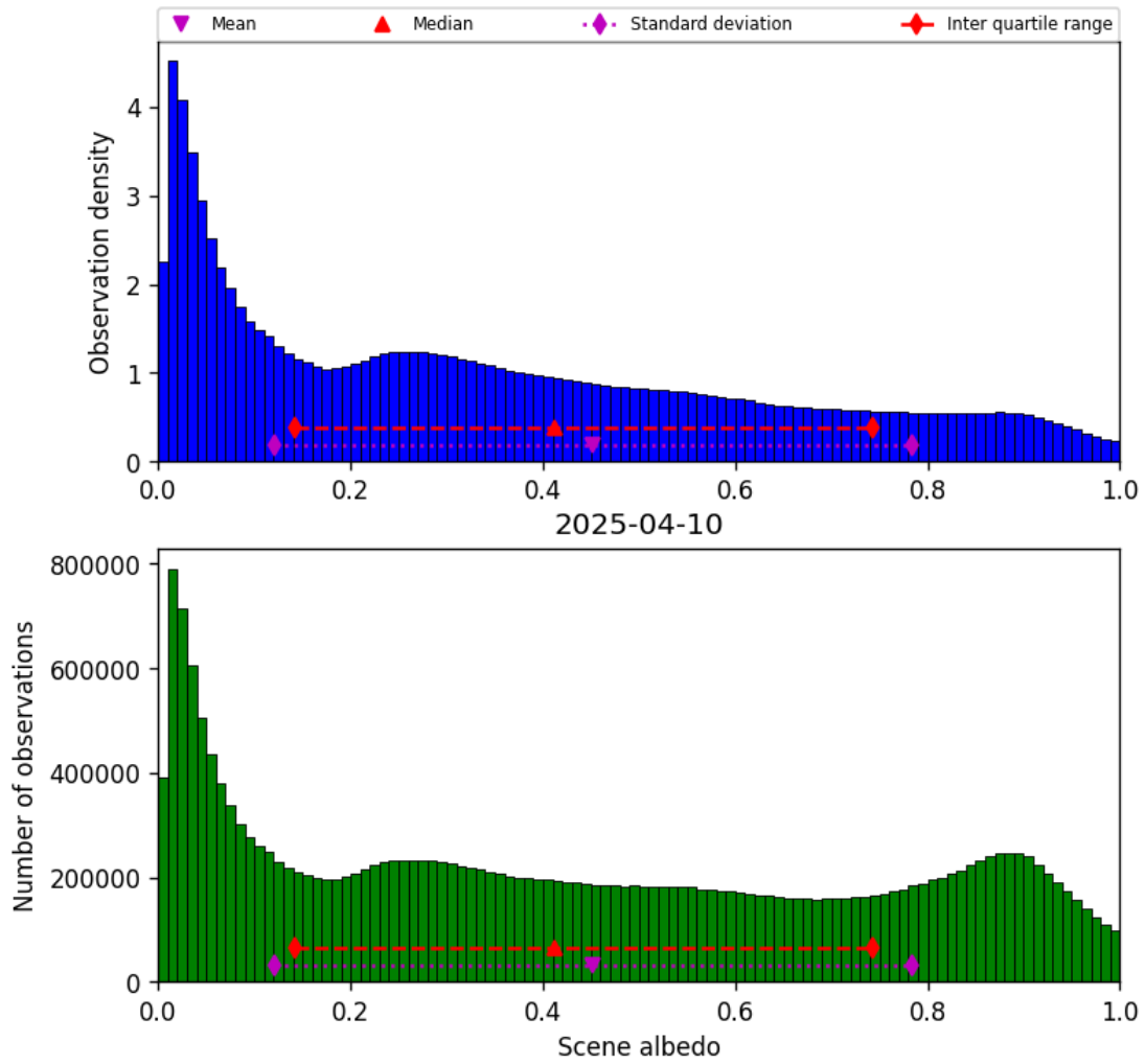
Figure 32: Histogram of “Scene albedo” for 2025-04-10 to 2025-04-11
