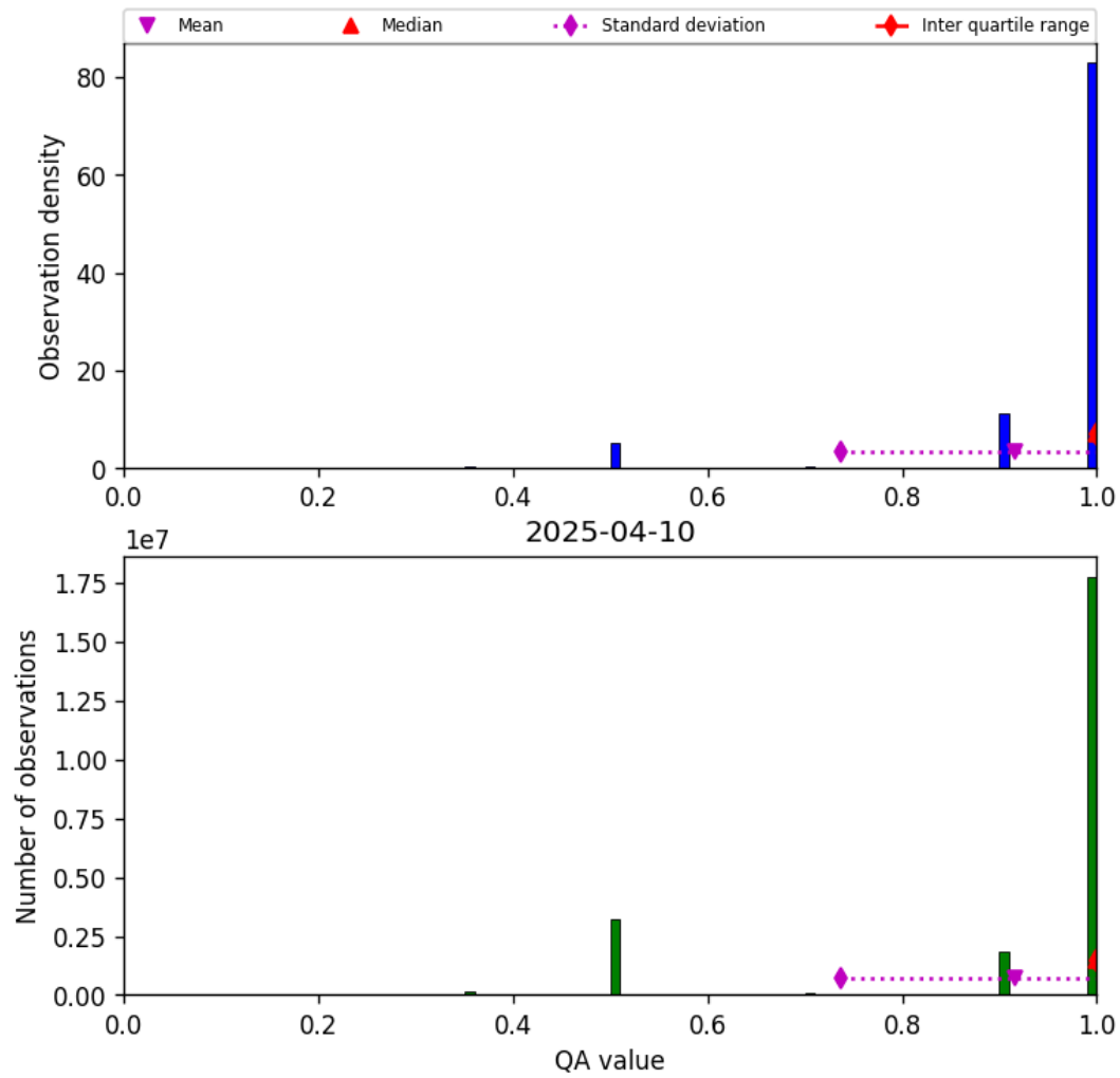
Figure 27: Histogram of “QA value” for 2025-04-10 to 2025-04-11
