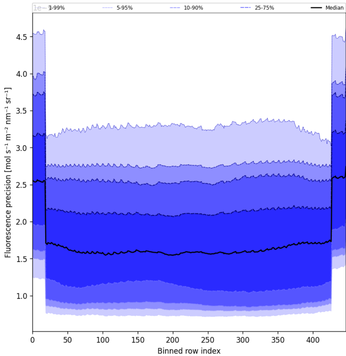
Figure 56: Along track statistics of “Fluorescence precision” for 2025-04-10 to 2025-04-11
