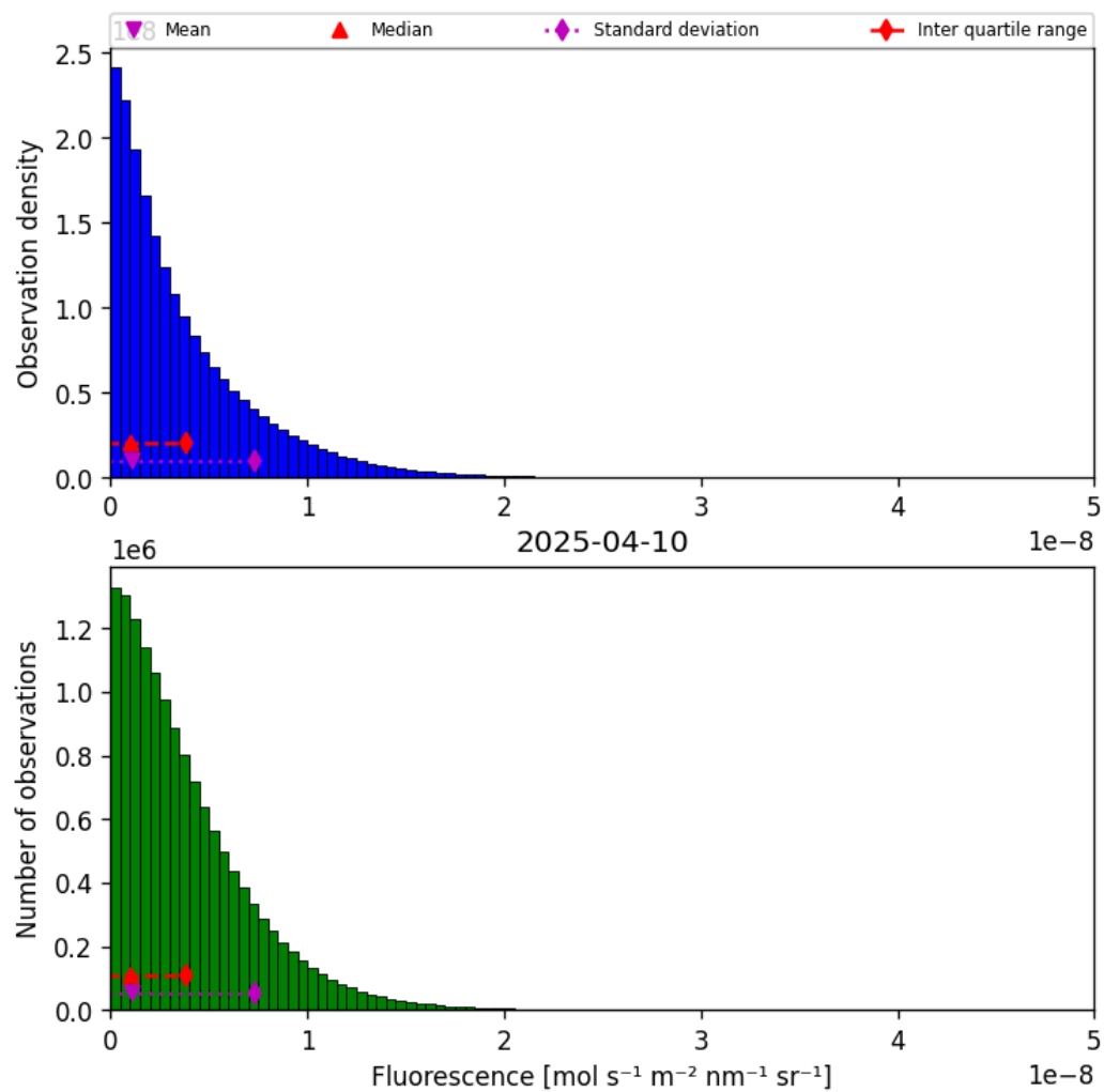
Figure 38: Histogram of “Fluorescence” for 2025-04-10 to 2025-04-11
