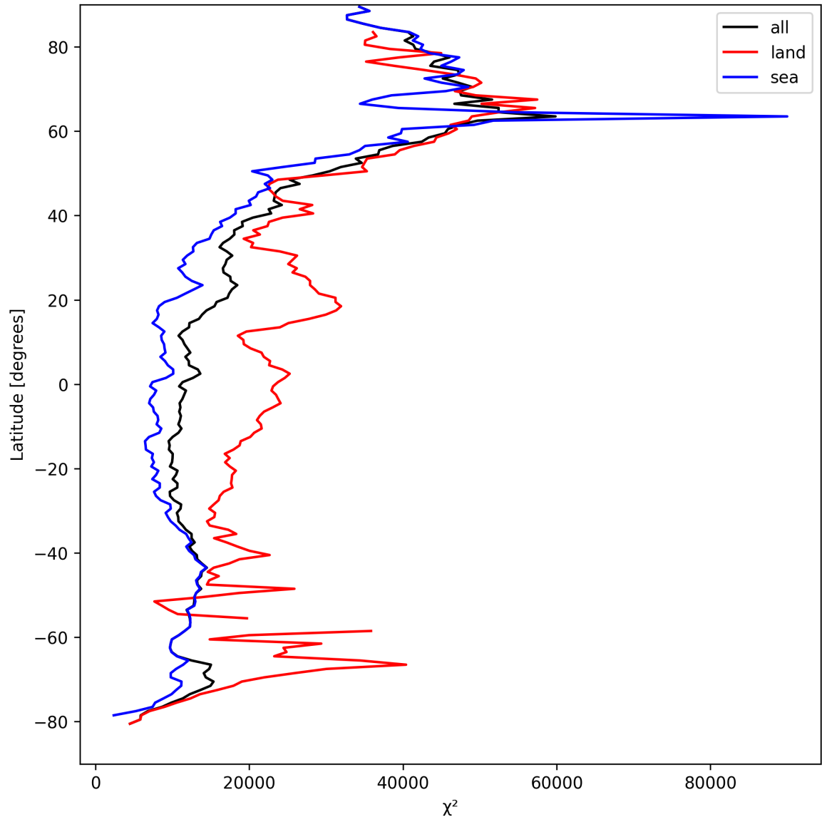
Figure 19: Zonal average of “ \chi^2 ” for 2025-04-10 to 2025-04-11.
