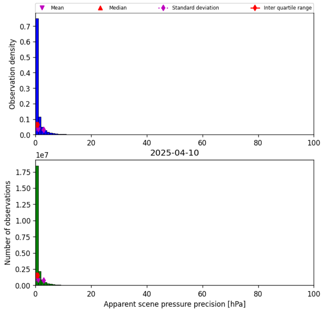
Figure 35: Histogram of “Apparent scene pressure precision” for 2025-04-10 to 2025-04-11
