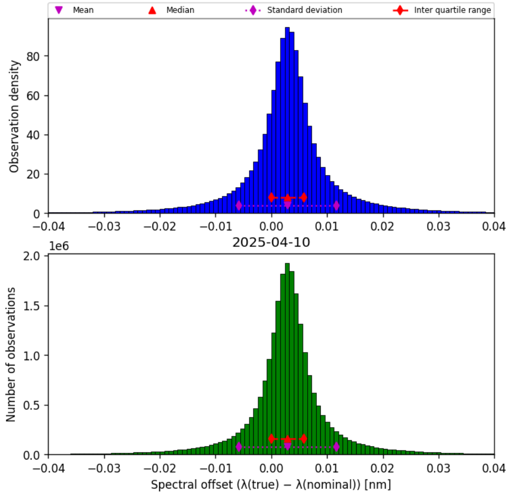
Figure 43: Histogram of “Spectral offset ( \lambda_{\text{true}} - \lambda_{\text{nominal}} )” for 2025-04-10 to 2025-04-11
