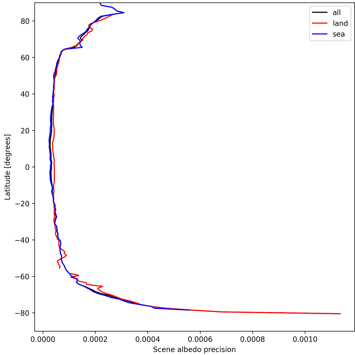
Figure 16: Zonal average of “Scene albedo precision” for 2025-04-10 to 2025-04-11.
