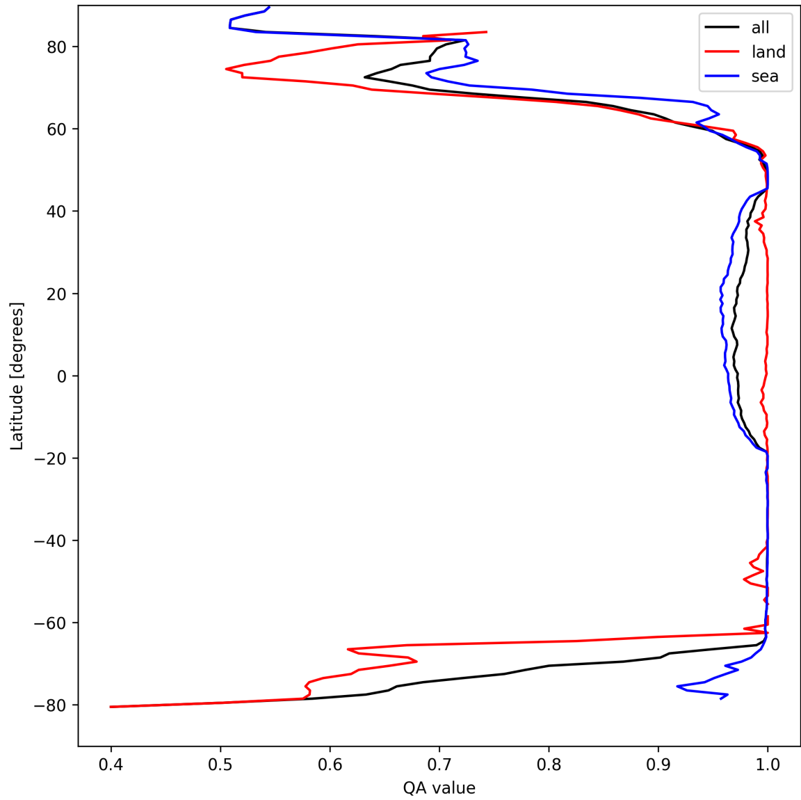
Figure 10: Zonal average of “QA value” for 2025-04-10 to 2025-04-11.
