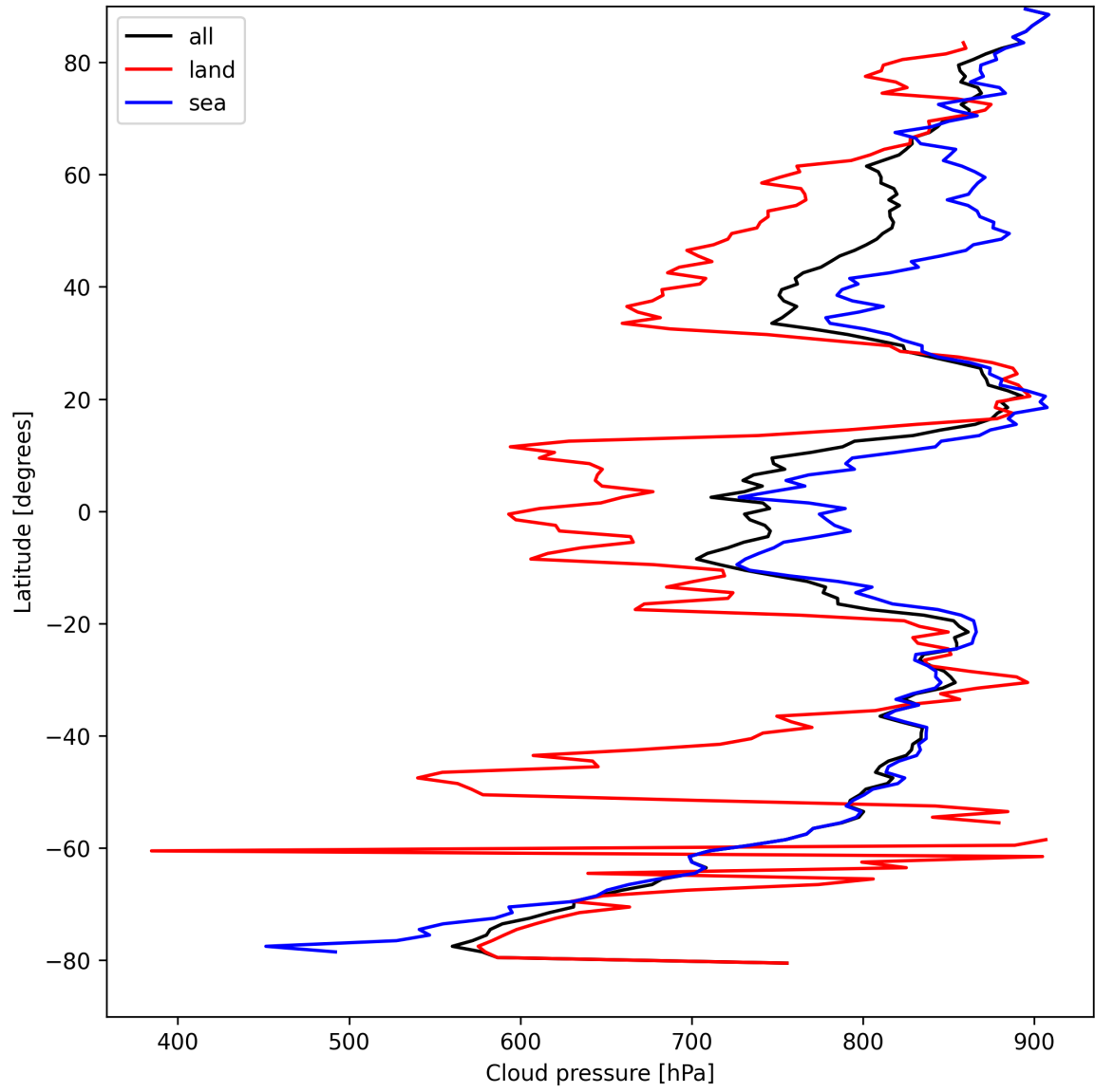
Figure 11: Zonal average of “Cloud pressure” for 2025-04-10 to 2025-04-11.
