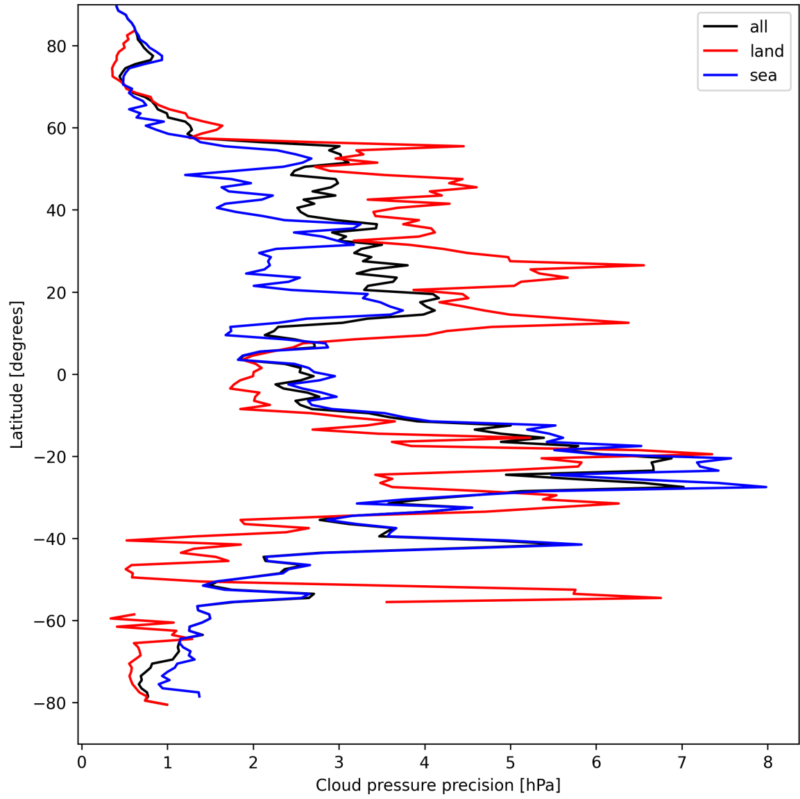
Figure 12: Zonal average of “Cloud pressure precision” for 2025-04-10 to 2025-04-11.
