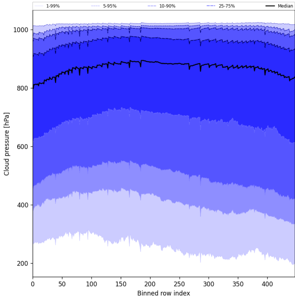
Figure 45: Along track statistics of “Cloud pressure” for 2025-04-10 to 2025-04-11
