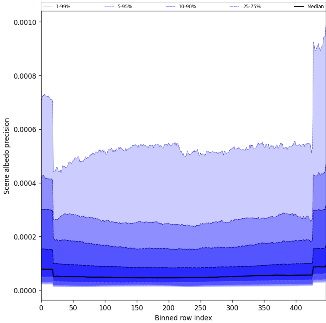
Figure 50: Along track statistics of “Scene albedo precision” for 2025-04-10 to 2025-04-11
