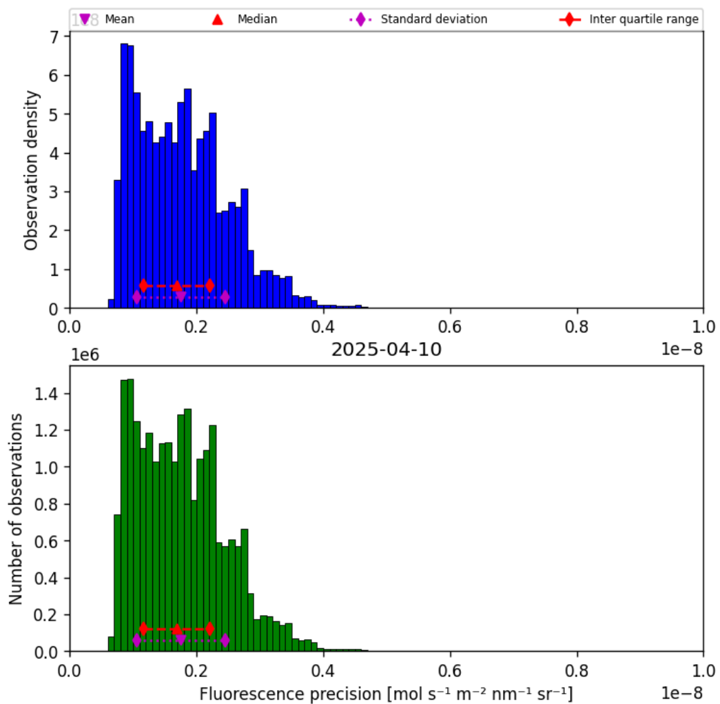
Figure 39: Histogram of “Fluorescence precision” for 2025-04-10 to 2025-04-11
