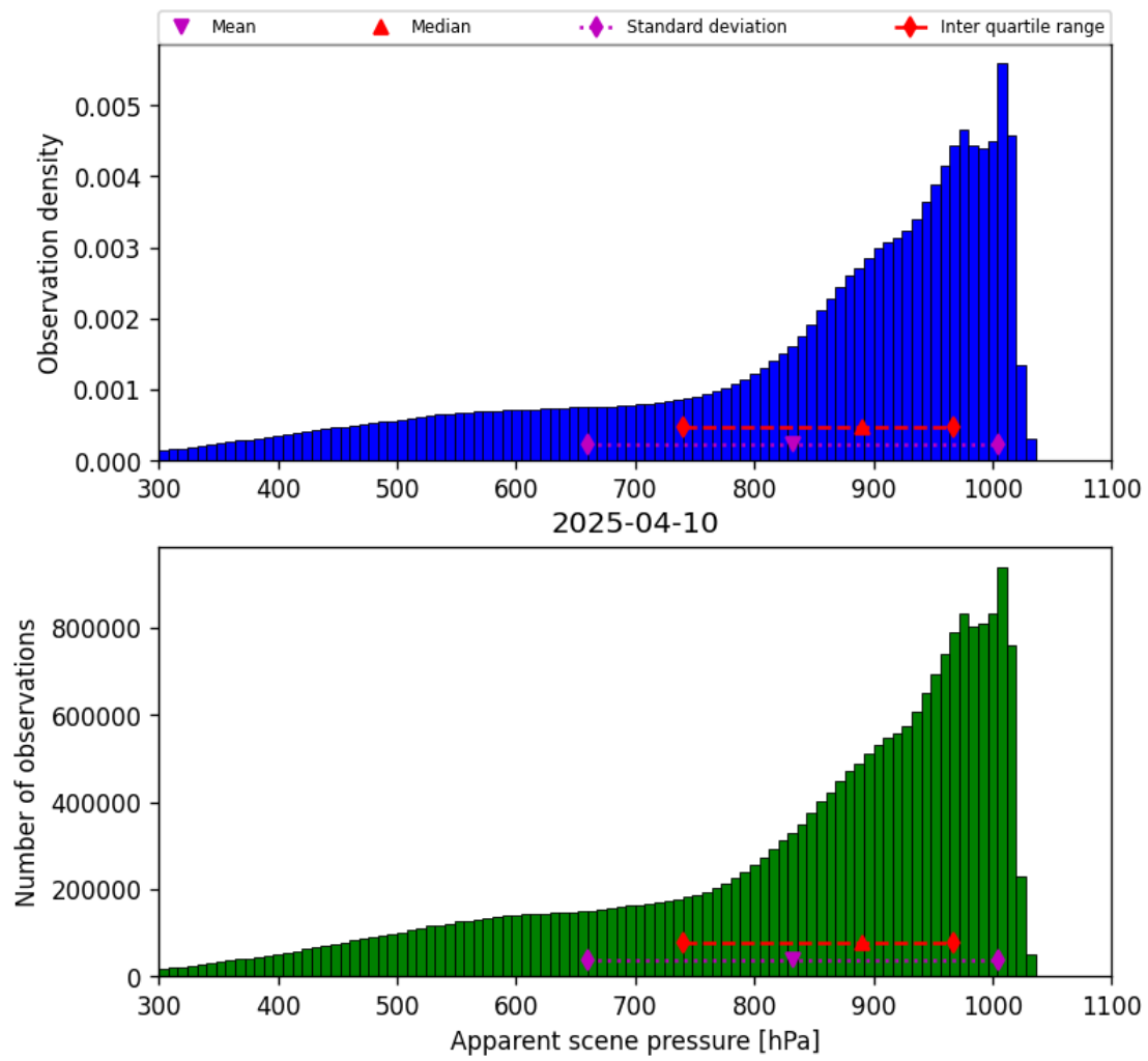
Figure 34: Histogram of “Apparent scene pressure” for 2025-04-10 to 2025-04-11
