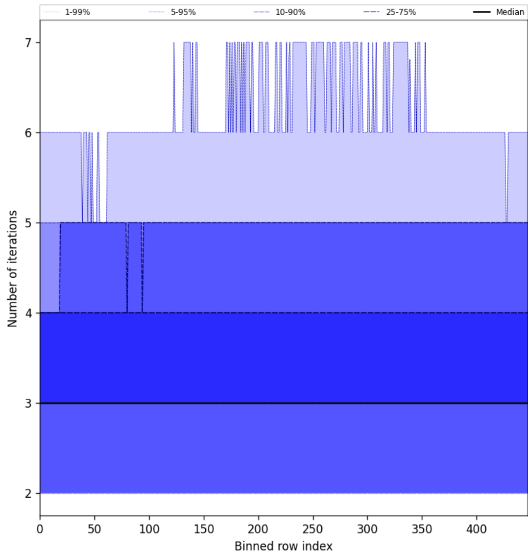
Figure 54: Along track statistics of “Number of iterations” for 2025-04-10 to 2025-04-11
