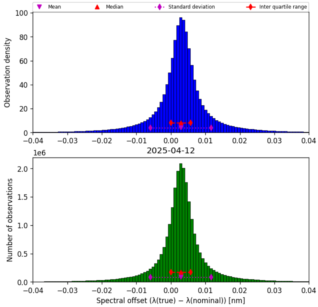
Figure 43: Histogram of “Spectral offset ( \lambda_{\text{true}} - \lambda_{\text{nominal}} )” for 2025-04-12 to 2025-04-13
