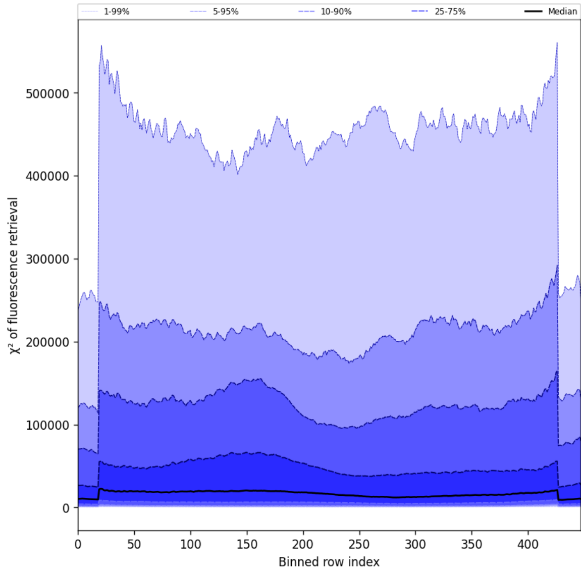
Figure 57: Along track statistics of " \chi^2 of fluorescence retrieval" for 2025-04-12 to 2025-04-13
