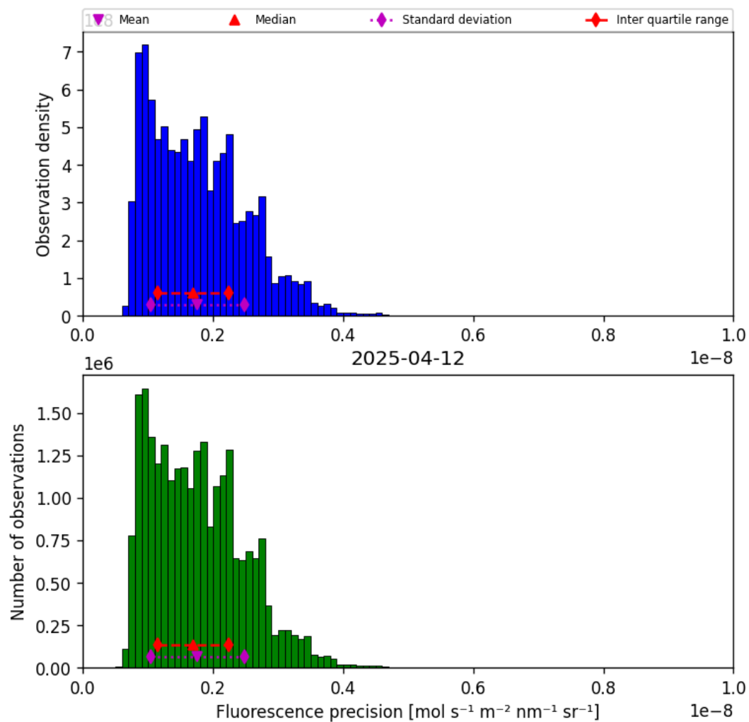
Figure 39: Histogram of “Fluorescence precision” for 2025-04-12 to 2025-04-13
