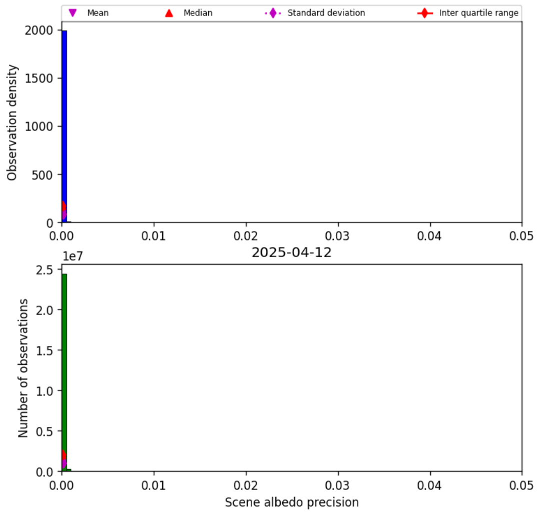
Figure 33: Histogram of “Scene albedo precision” for 2025-04-12 to 2025-04-13
