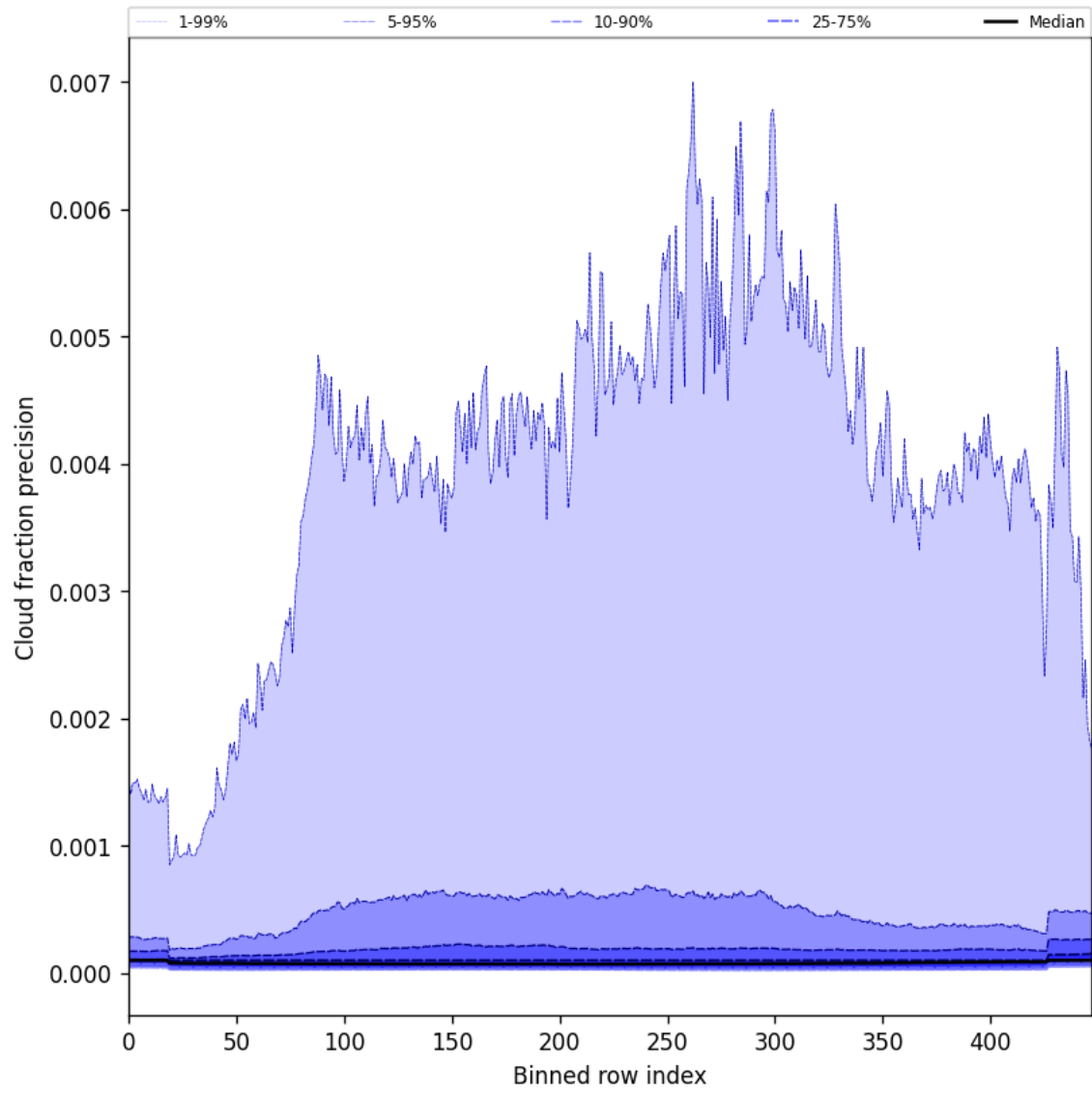
Figure 48: Along track statistics of “Cloud fraction precision” for 2025-04-12 to 2025-04-13
