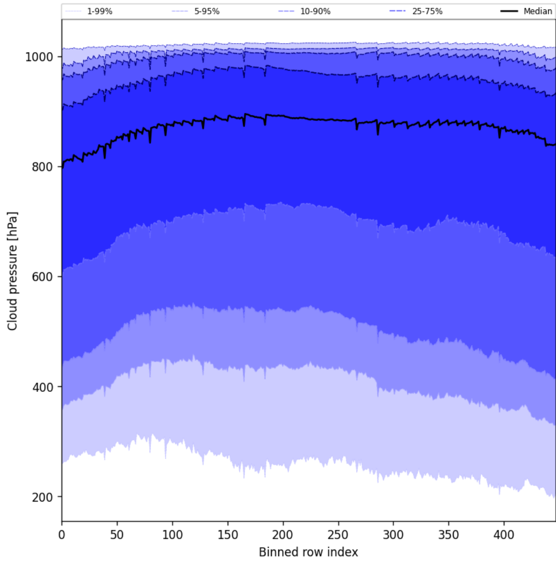
Figure 45: Along track statistics of “Cloud pressure” for 2025-04-12 to 2025-04-13
