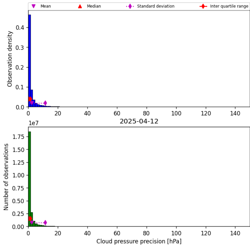
Figure 29: Histogram of “Cloud pressure precision” for 2025-04-12 to 2025-04-13
