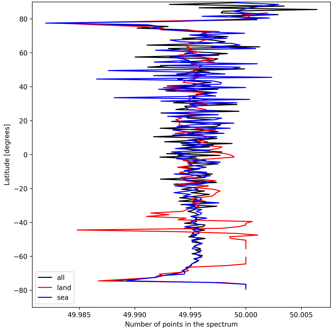
Figure 25: Zonal average of “Number of points in the spectrum” for 2025-04-12 to 2025-04-13.
