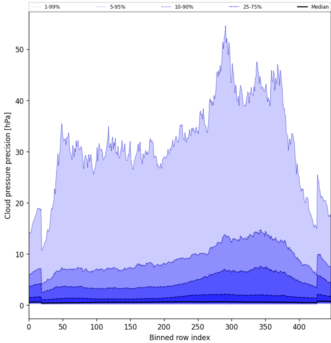
Figure 46: Along track statistics of “Cloud pressure precision” for 2025-04-12 to 2025-04-13
