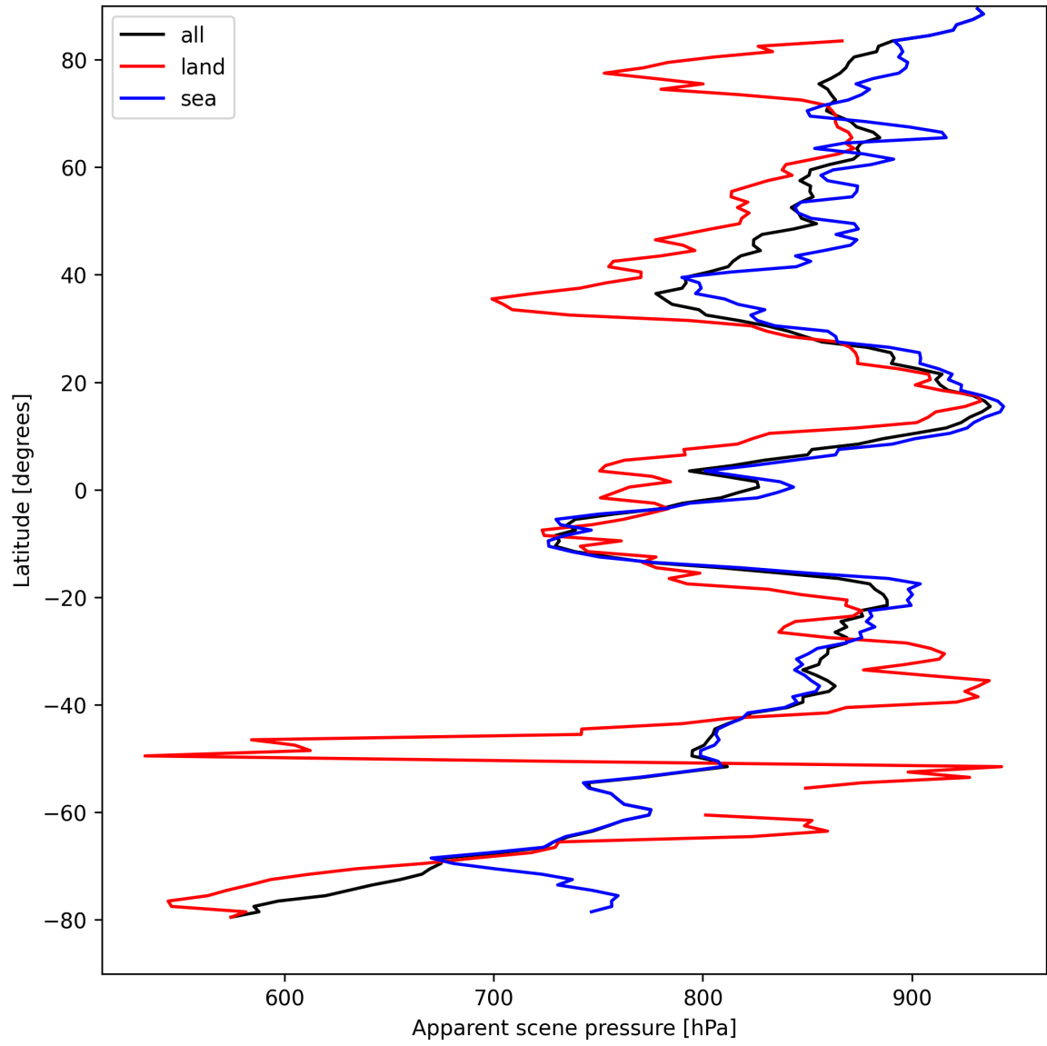
Figure 17: Zonal average of “Apparent scene pressure” for 2025-04-12 to 2025-04-13.
