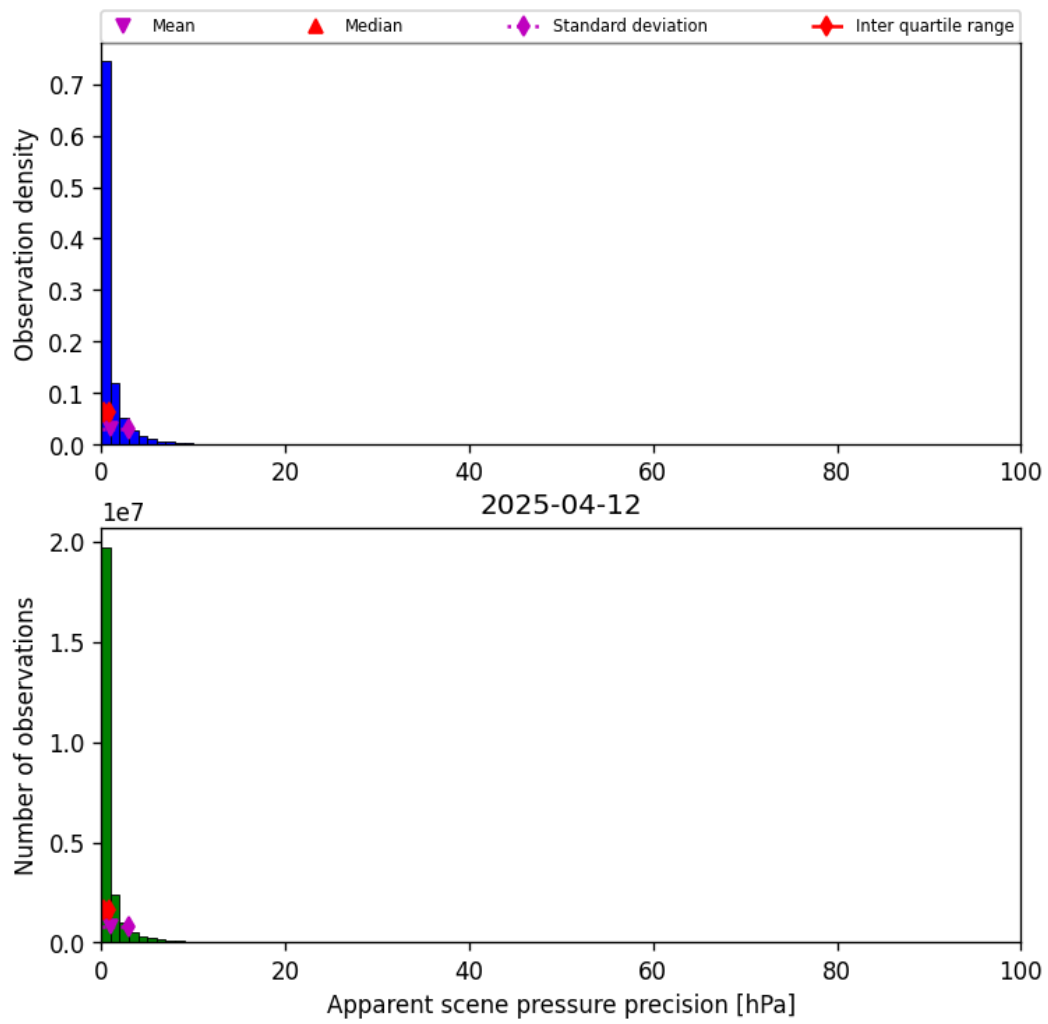
Figure 35: Histogram of “Apparent scene pressure precision” for 2025-04-12 to 2025-04-13
