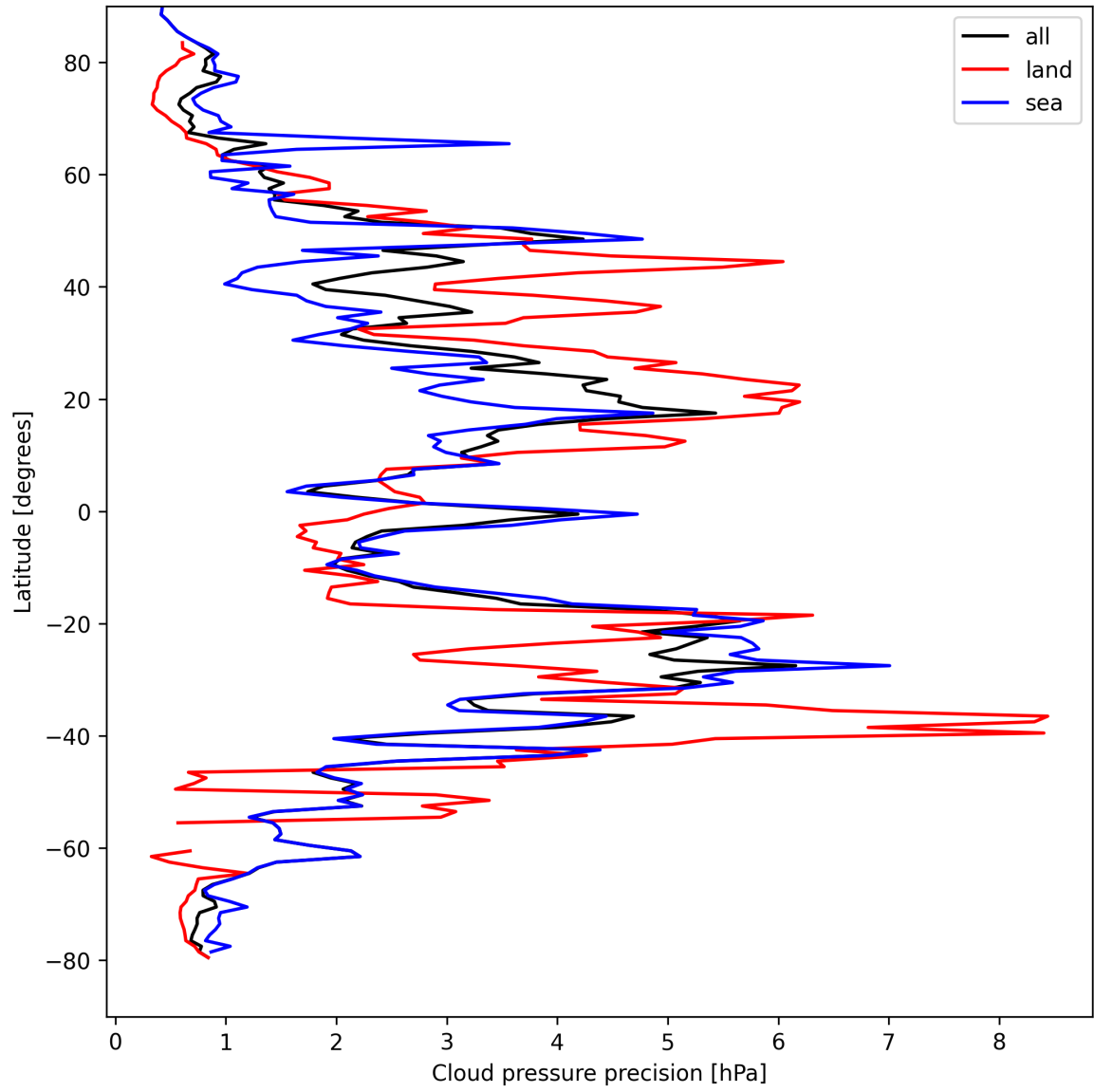
Figure 12: Zonal average of “Cloud pressure precision” for 2025-04-12 to 2025-04-13.
