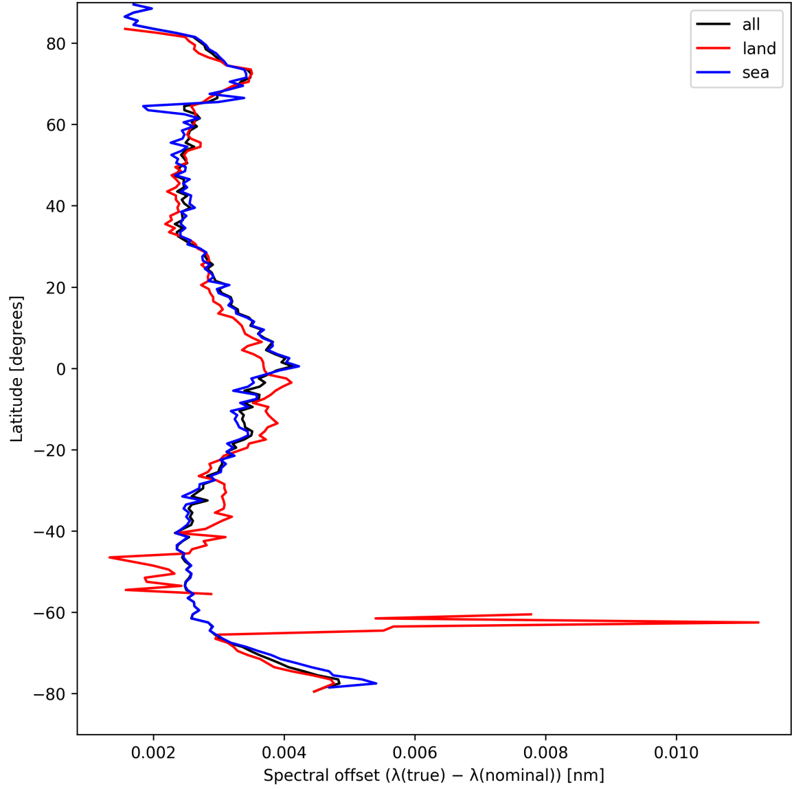
Figure 26: Zonal average of “Spectral offset ( \lambda_{\text{true}} - \lambda_{\text{nominal}} )” for 2025-04-12 to 2025-04-13.
