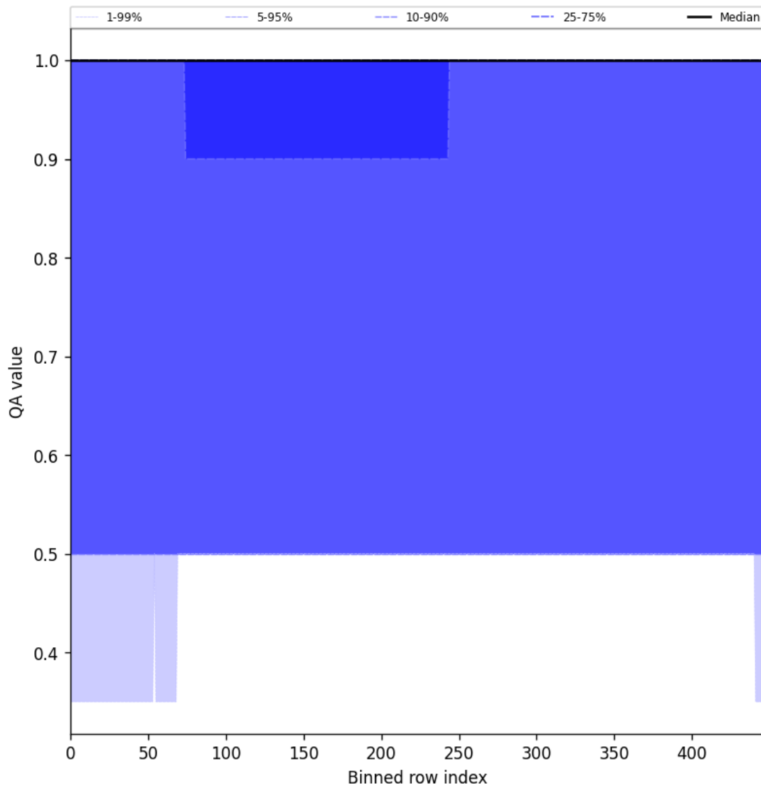
Figure 44: Along track statistics of “QA value” for 2025-04-12 to 2025-04-13
