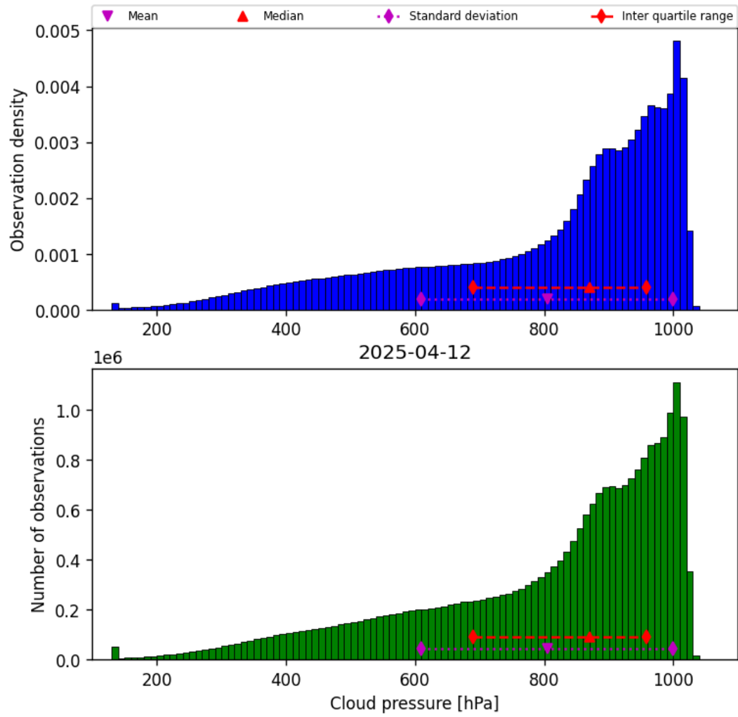
Figure 28: Histogram of “Cloud pressure” for 2025-04-12 to 2025-04-13
