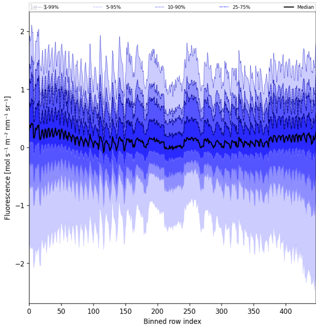
Figure 55: Along track statistics of “Fluorescence” for 2025-04-12 to 2025-04-13
