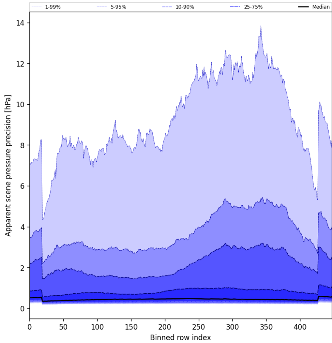
Figure 52: Along track statistics of “Apparent scene pressure precision” for 2025-04-12 to 2025-04-13
