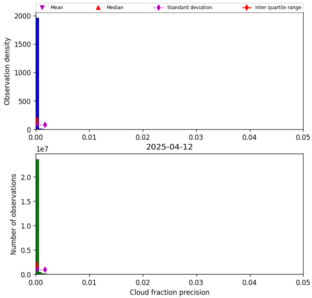
Figure 31: Histogram of “Cloud fraction precision” for 2025-04-12 to 2025-04-13
