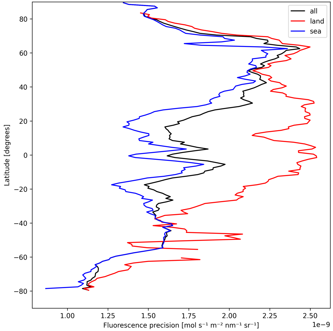
Figure 22: Zonal average of “Fluorescence precision” for 2025-04-12 to 2025-04-13.
