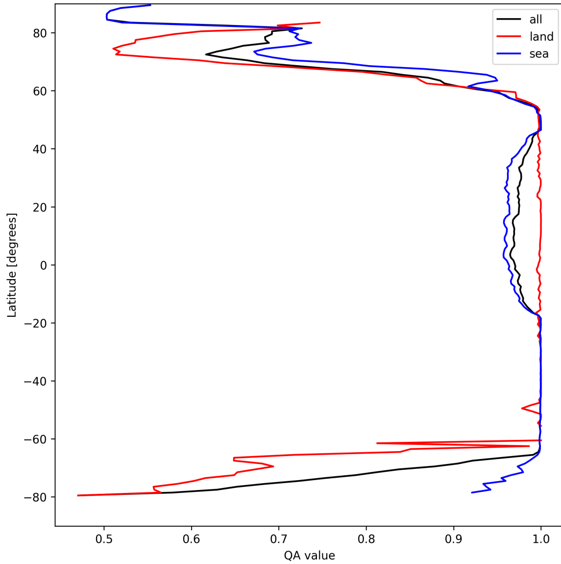
Figure 10: Zonal average of “QA value” for 2025-04-12 to 2025-04-13.
