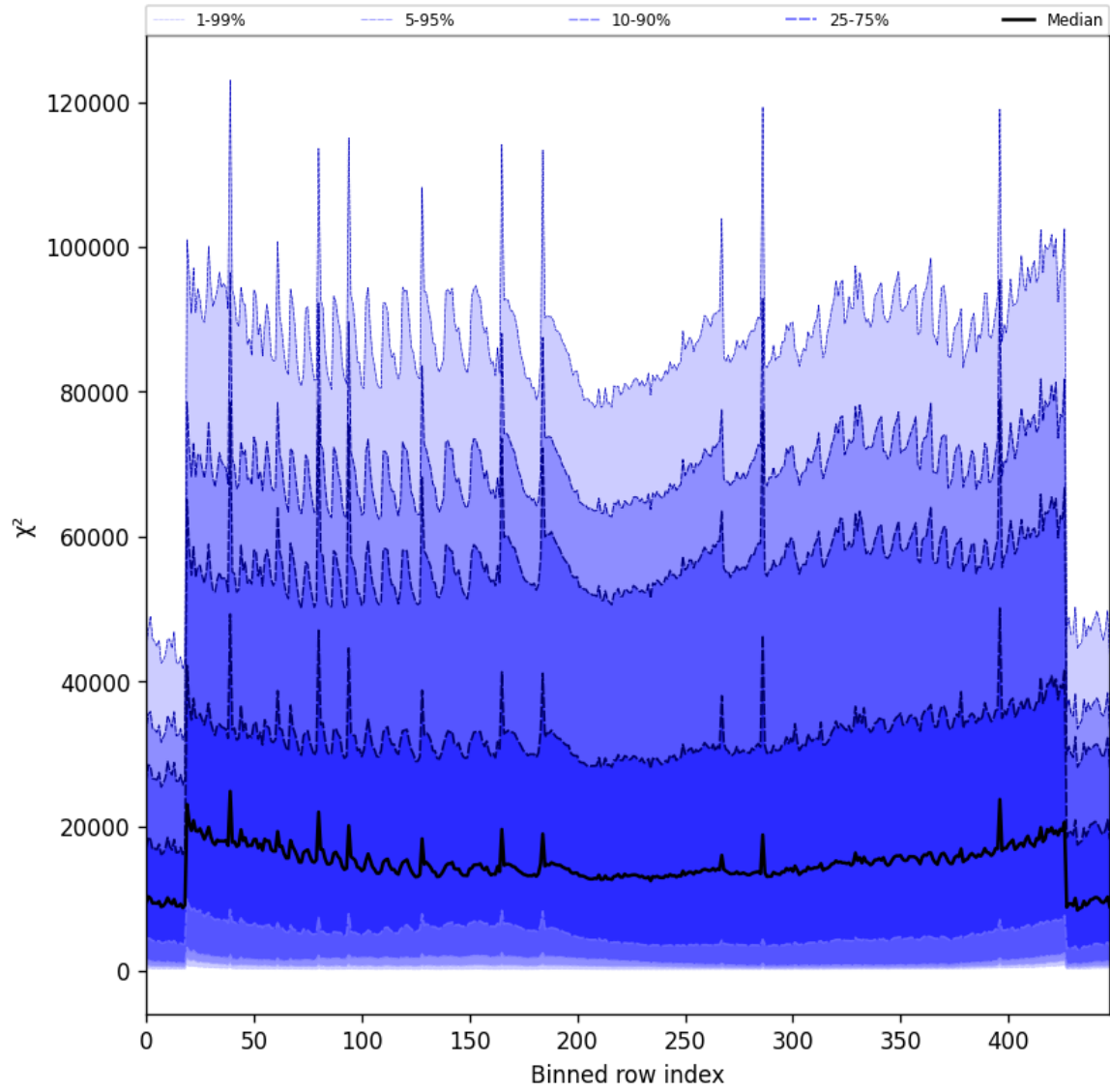
Figure 53: Along track statistics of “ \chi^2 ” for 2025-04-12 to 2025-04-13
