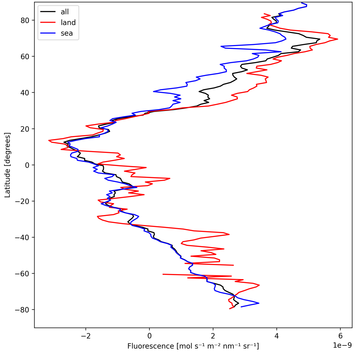
Figure 21: Zonal average of “Fluorescence” for 2025-04-12 to 2025-04-13.
