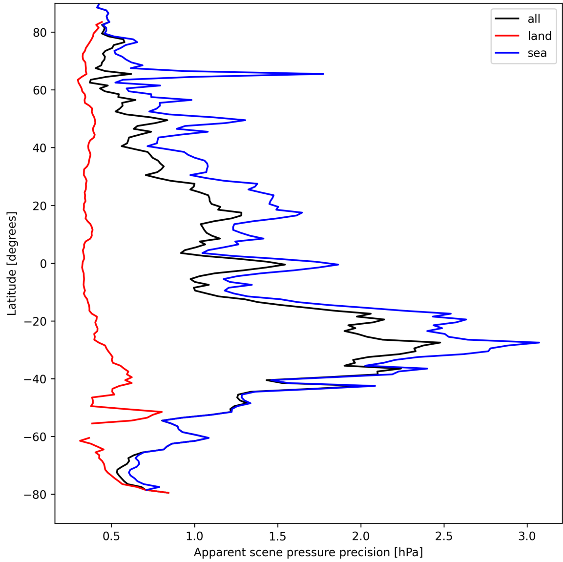
Figure 18: Zonal average of “Apparent scene pressure precision” for 2025-04-12 to 2025-04-13.
