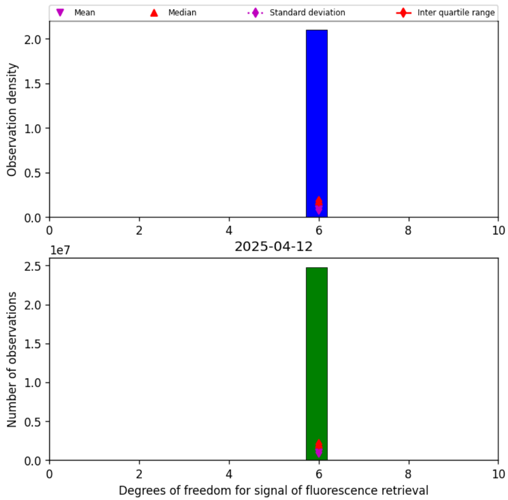
Figure 41: Histogram of “Degrees of freedom for signal of fluorescence retrieval” for 2025-04-12 to 2025-04-13
