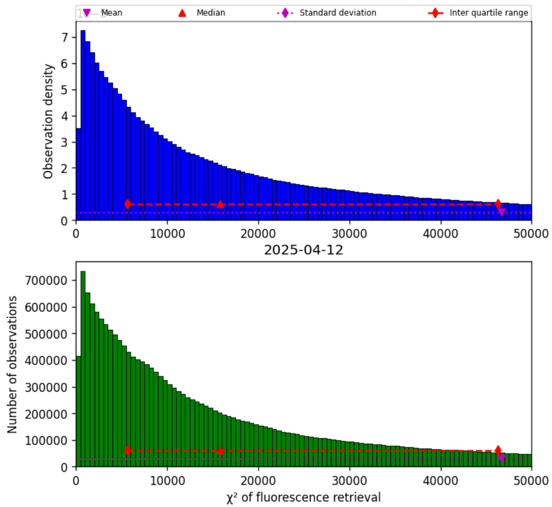
Figure 40: Histogram of “ \chi^2 of fluorescence retrieval” for 2025-04-12 to 2025-04-13
