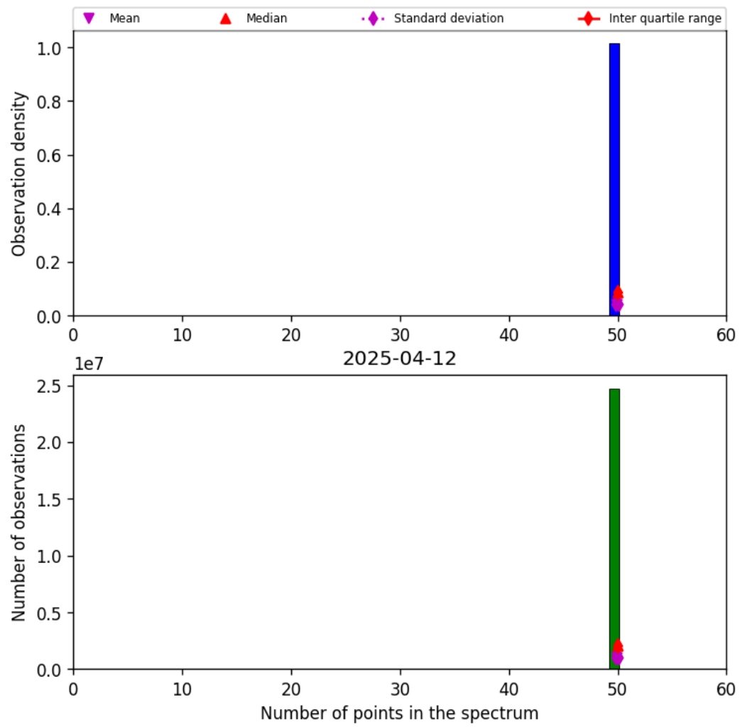
Figure 42: Histogram of "Number of points in the spectrum" for 2025-04-12 to 2025-04-13
