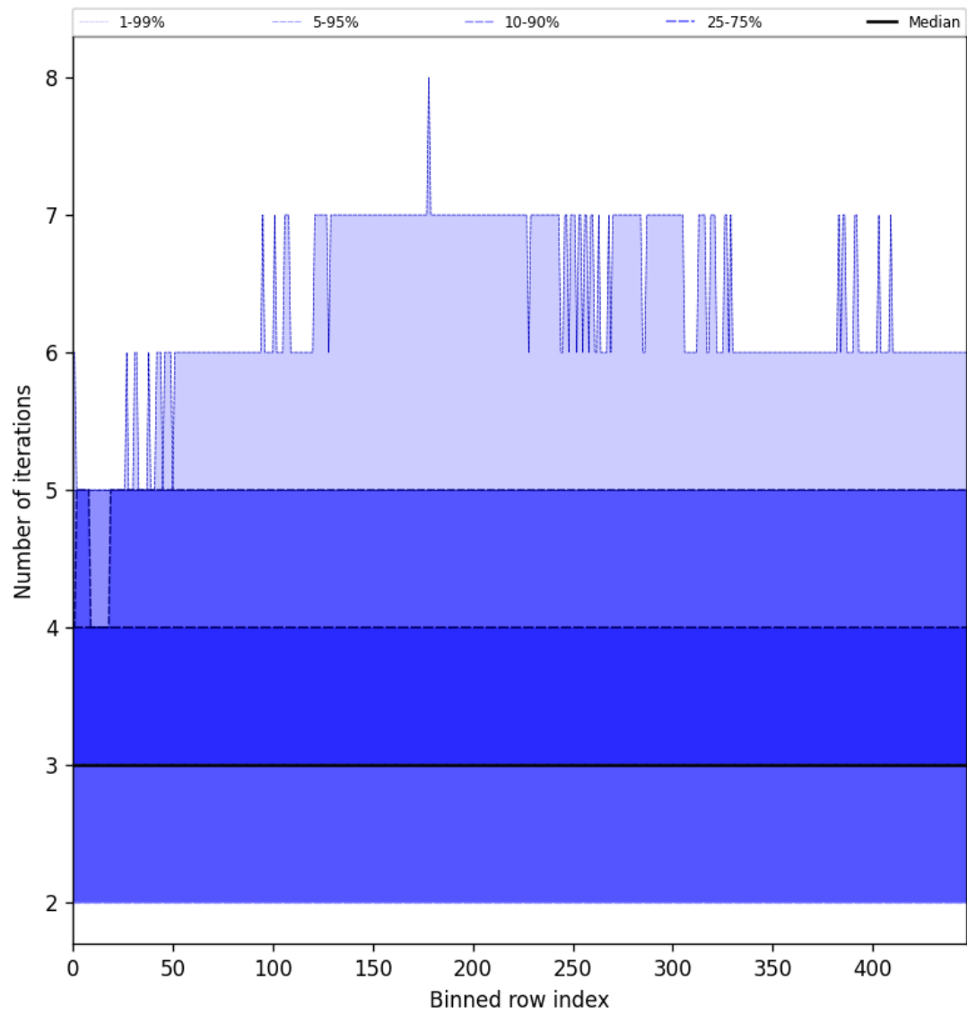
Figure 54: Along track statistics of “Number of iterations” for 2025-04-12 to 2025-04-13
