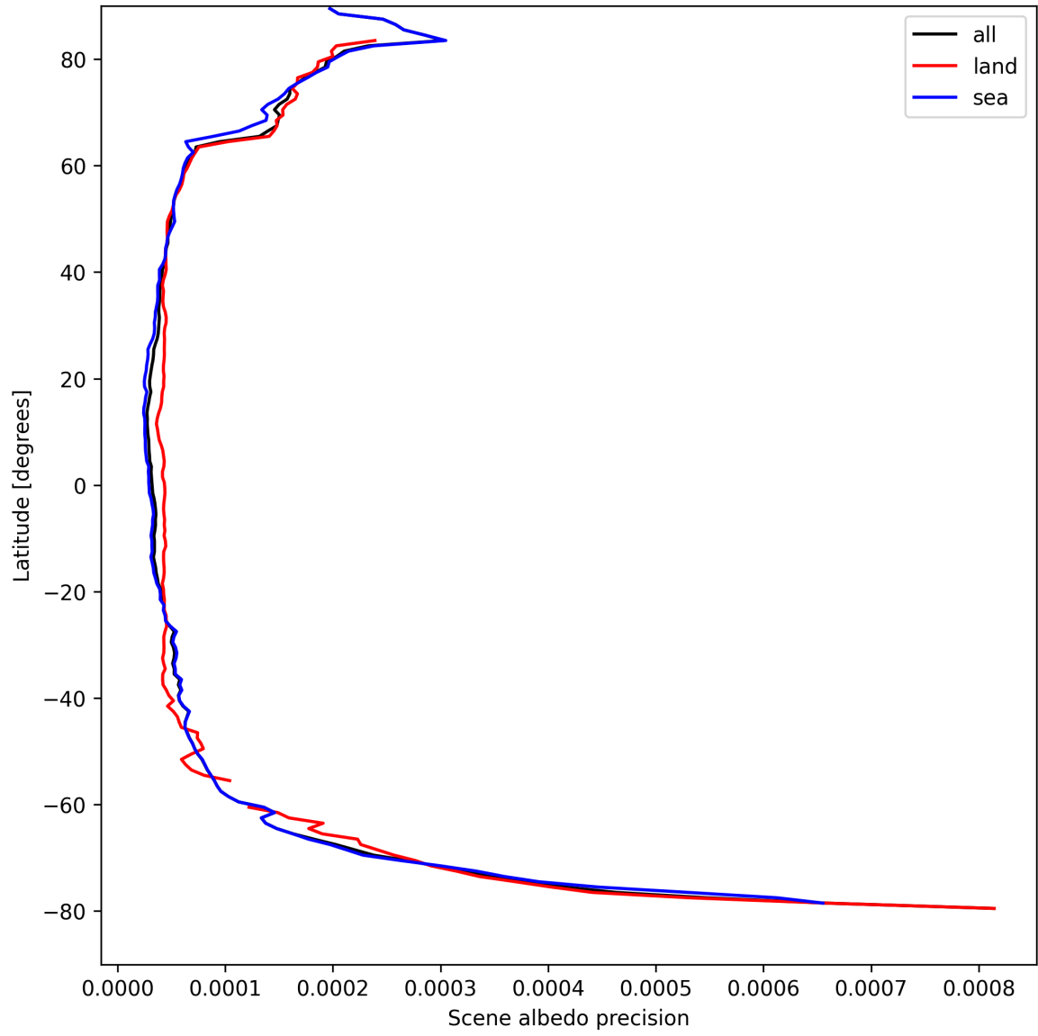
Figure 16: Zonal average of “Scene albedo precision” for 2025-04-12 to 2025-04-13.
