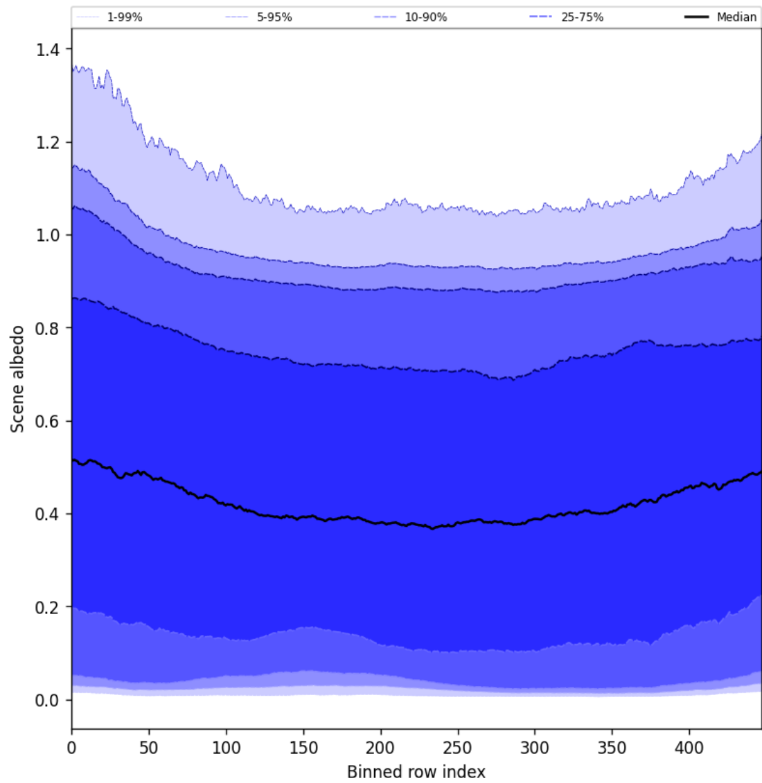
Figure 49: Along track statistics of “Scene albedo” for 2025-04-12 to 2025-04-13
