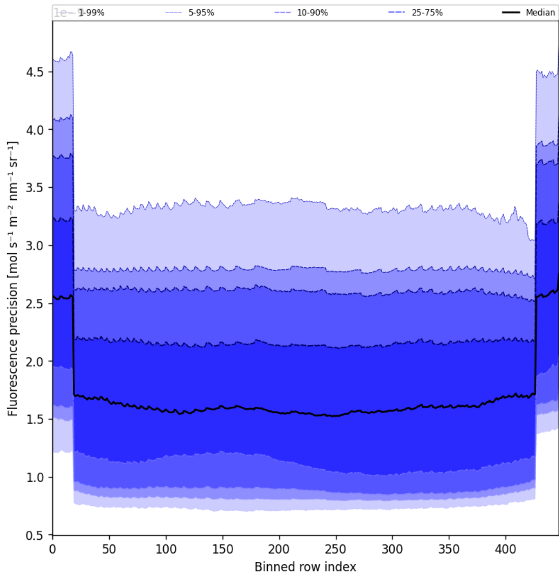
Figure 56: Along track statistics of “Fluorescence precision” for 2025-04-12 to 2025-04-13
