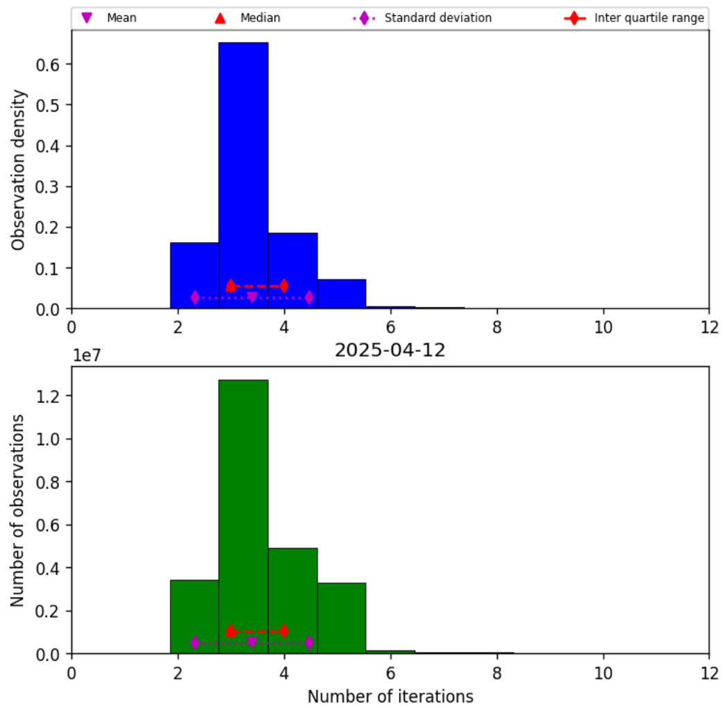
Figure 37: Histogram of “Number of iterations” for 2025-04-12 to 2025-04-13
