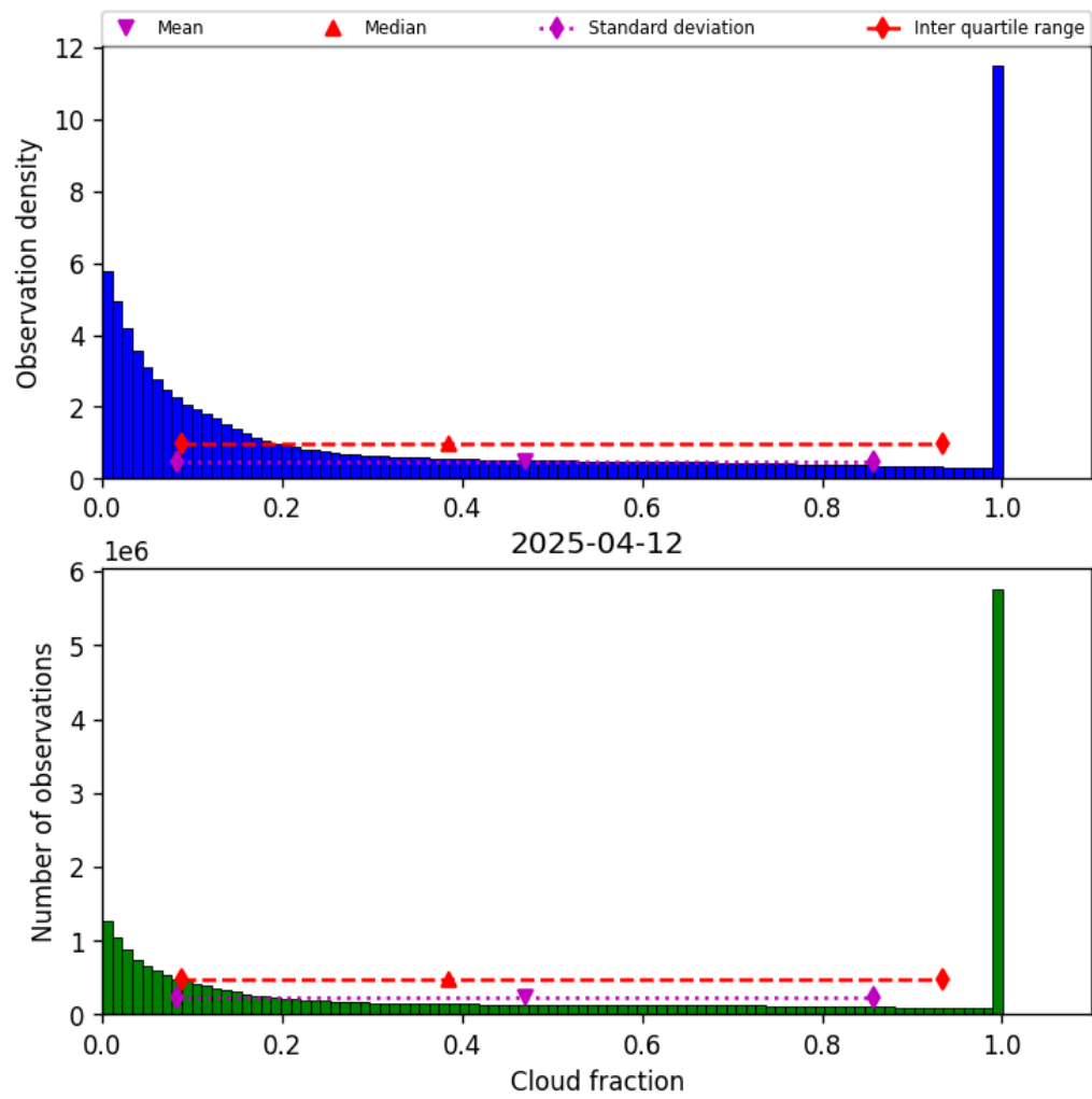
Figure 30: Histogram of “Cloud fraction” for 2025-04-12 to 2025-04-13
