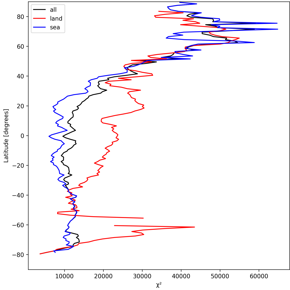
Figure 19: Zonal average of “ \chi^2 ” for 2025-04-12 to 2025-04-13.
