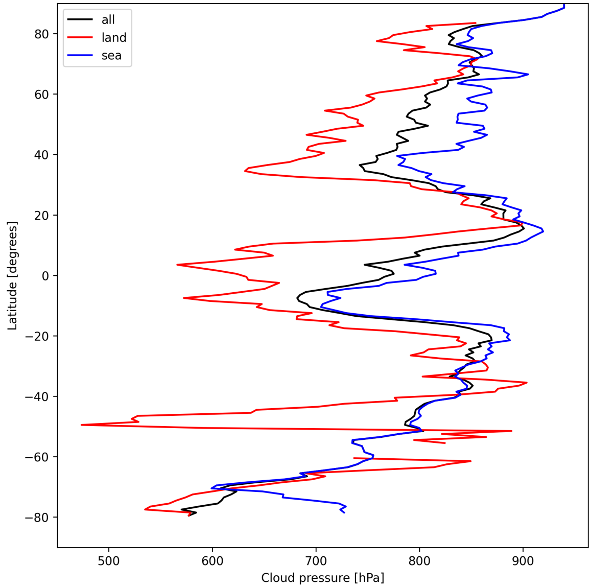
Figure 11: Zonal average of “Cloud pressure” for 2025-04-12 to 2025-04-13.
