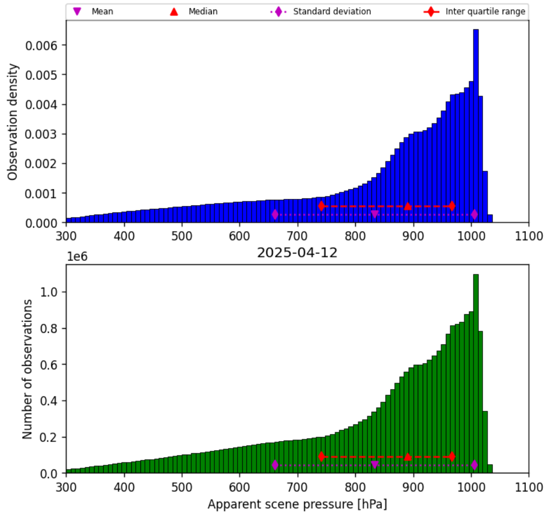
Figure 34: Histogram of “Apparent scene pressure” for 2025-04-12 to 2025-04-13
