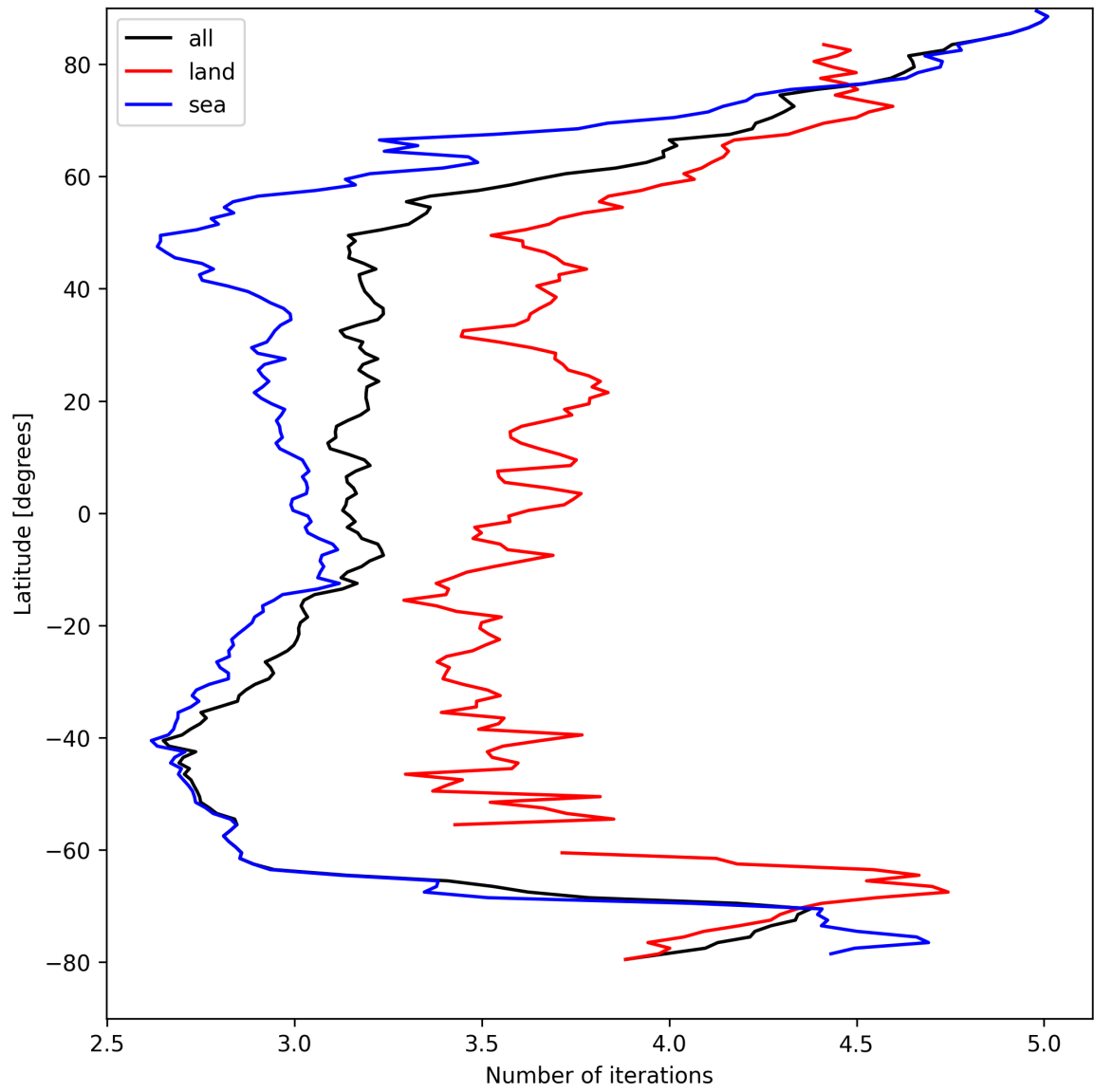
Figure 20: Zonal average of “Number of iterations” for 2025-04-12 to 2025-04-13.
