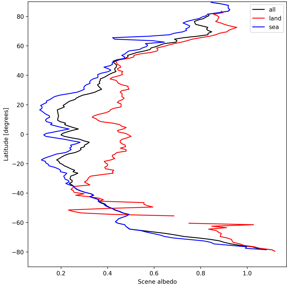
Figure 15: Zonal average of “Scene albedo” for 2025-04-12 to 2025-04-13.
