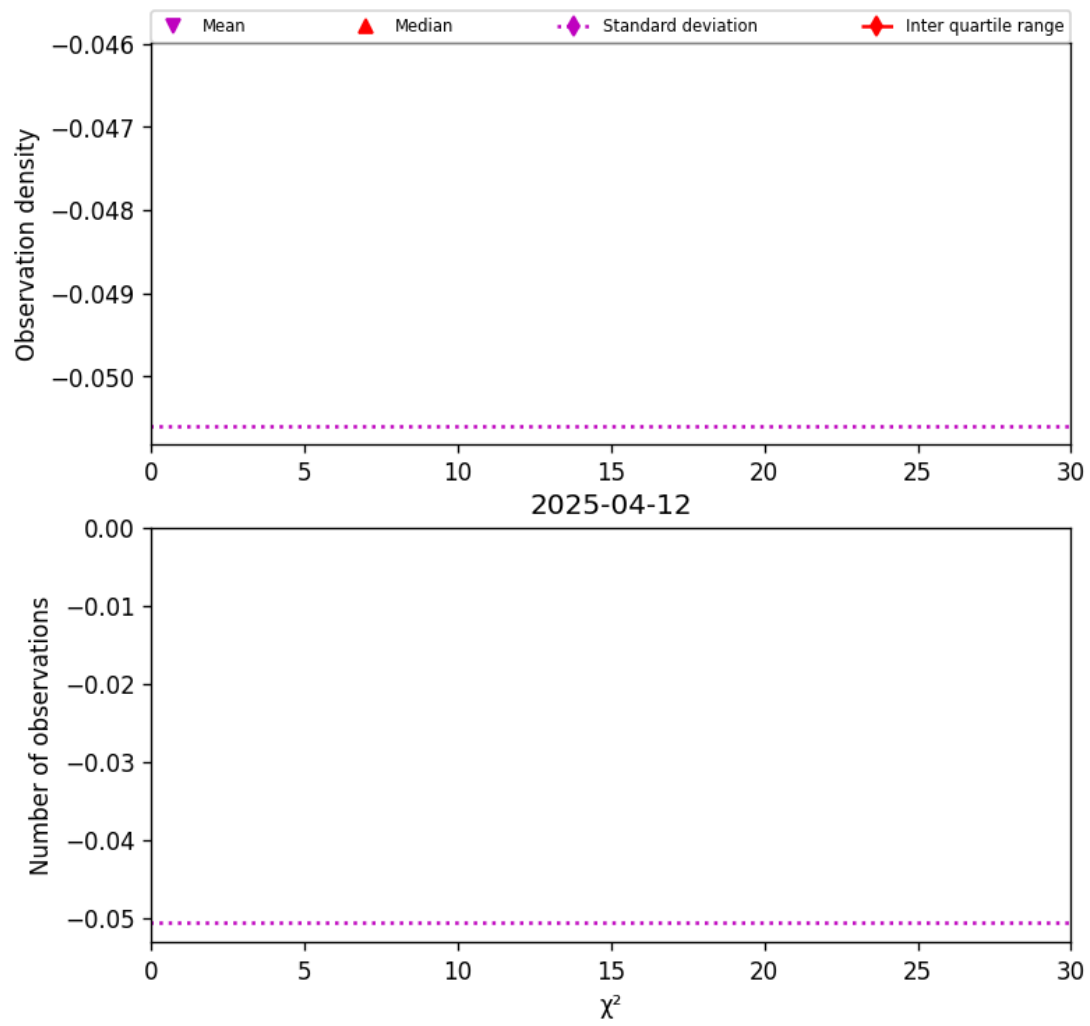
Figure 36: Histogram of “ \chi^2 ” for 2025-04-12 to 2025-04-13
