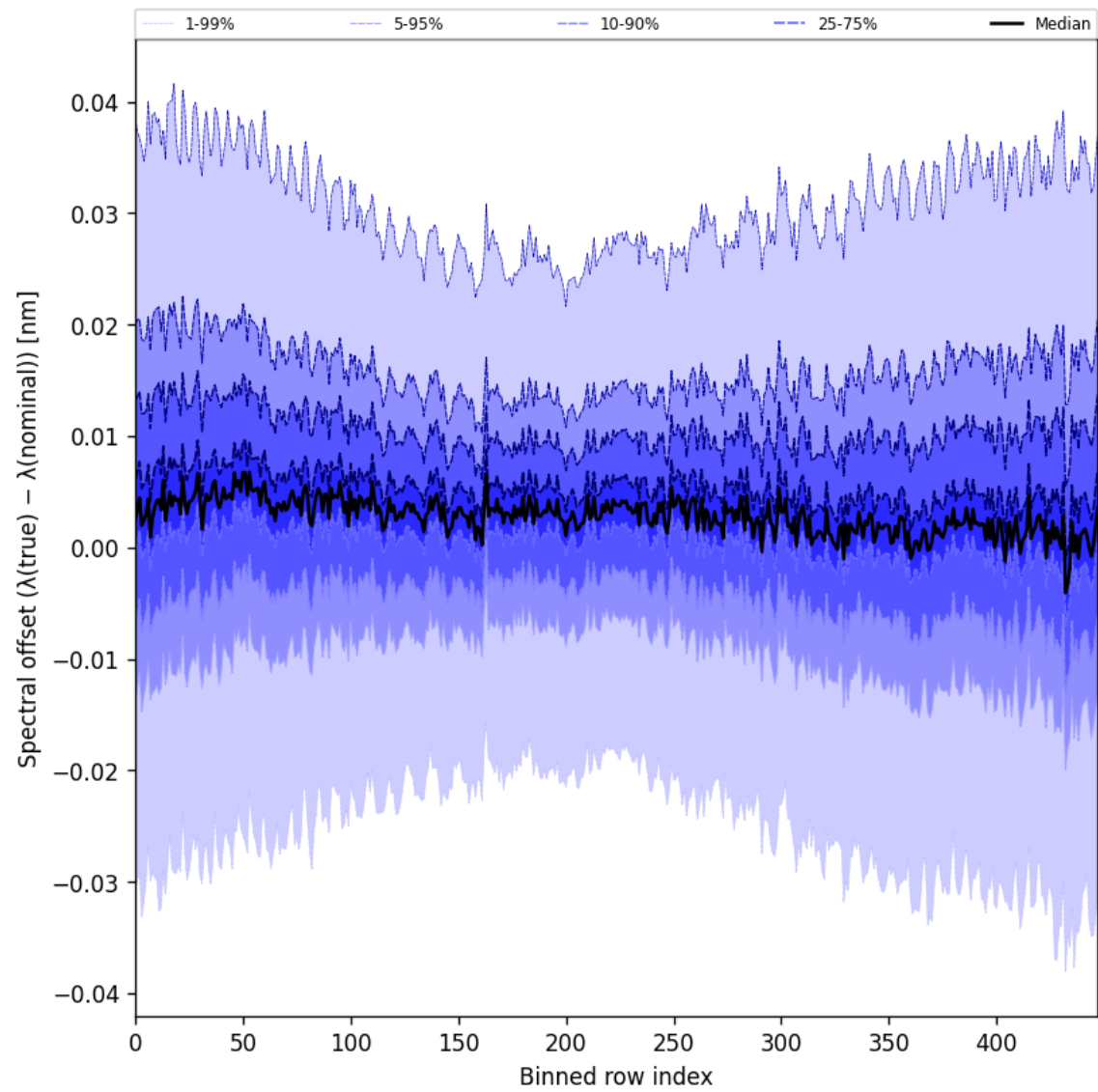
Figure 60: Along track statistics of “Spectral offset ( \lambda_{\text{true}} - \lambda_{\text{nominal}} )” for 2025-04-12 to 2025-04-13
