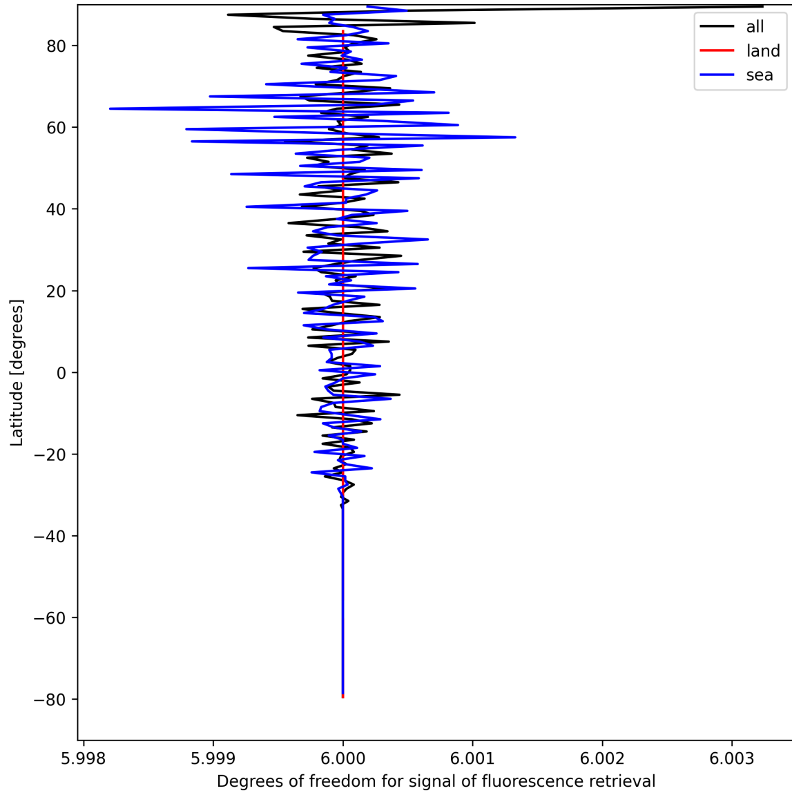
Figure 24: Zonal average of “Degrees of freedom for signal of fluorescence retrieval” for 2025-04-12 to 2025-04-13.
