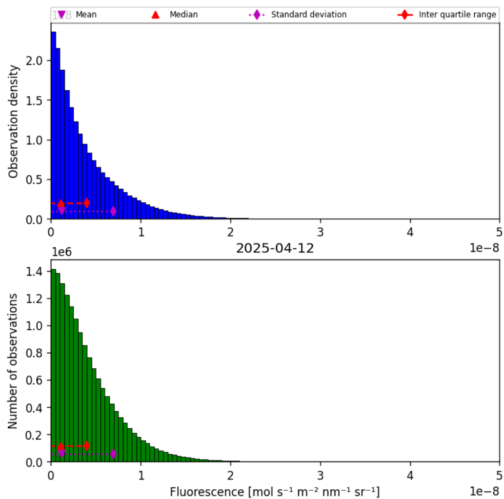
Figure 38: Histogram of “Fluorescence” for 2025-04-12 to 2025-04-13
