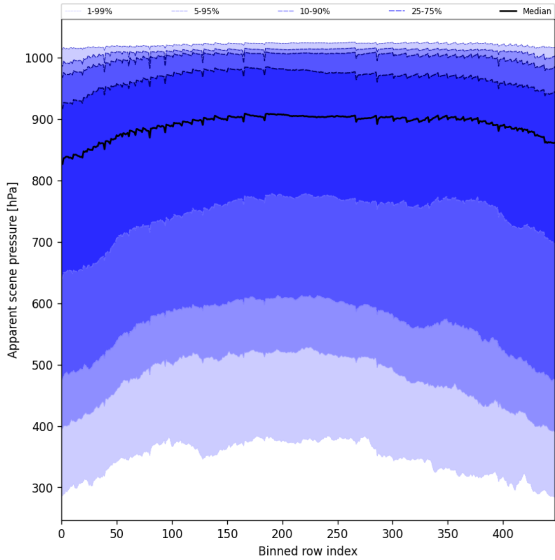
Figure 51: Along track statistics of “Apparent scene pressure” for 2025-04-12 to 2025-04-13
