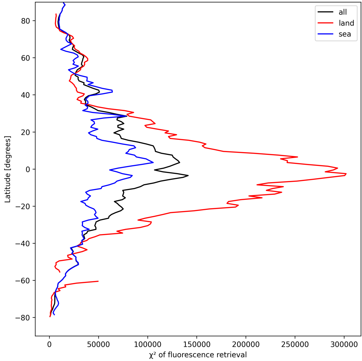
Figure 23: Zonal average of “ \chi^2 of fluorescence retrieval” for 2025-04-12 to 2025-04-13.
