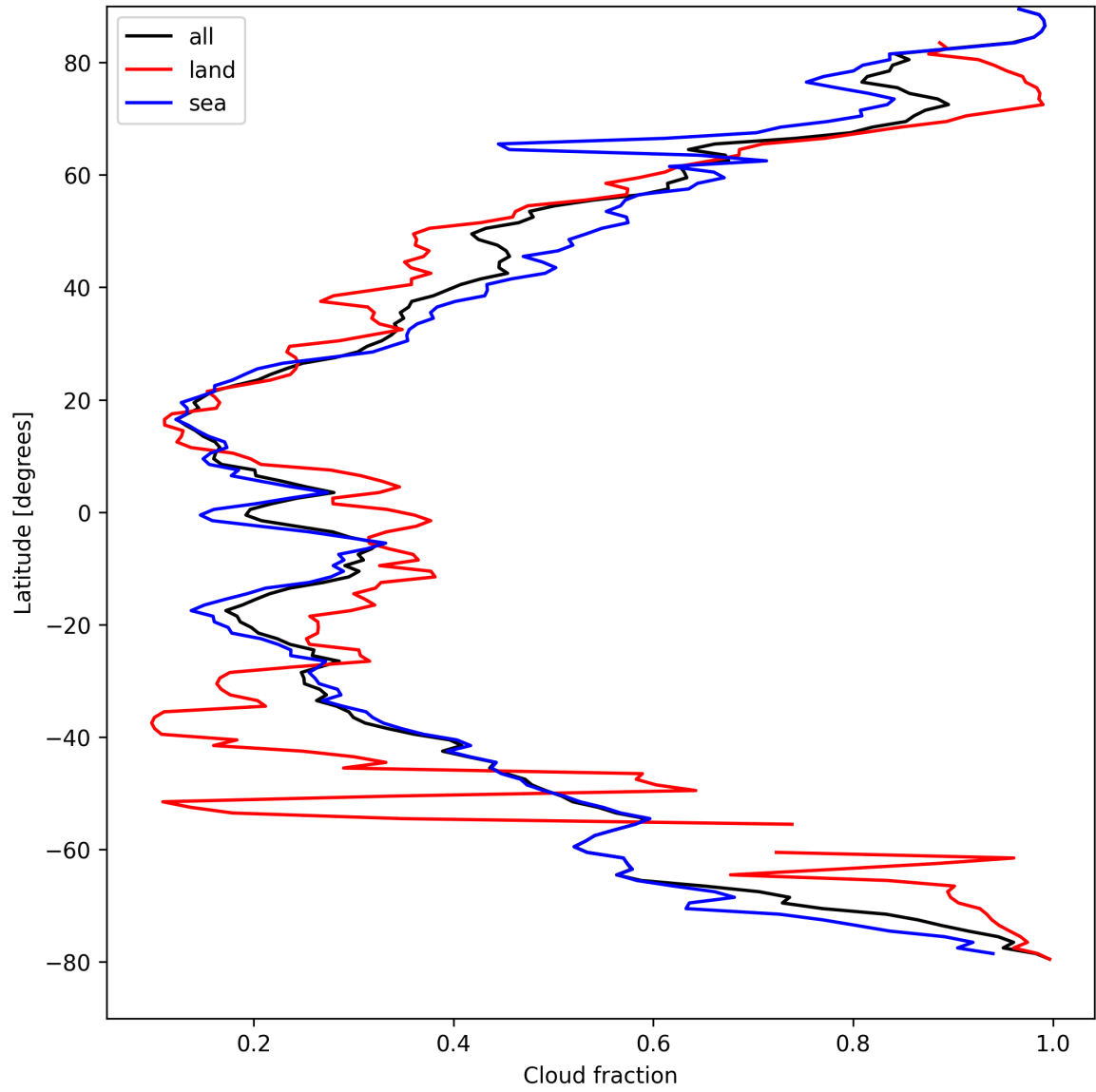
Figure 13: Zonal average of “Cloud fraction” for 2025-04-12 to 2025-04-13.
