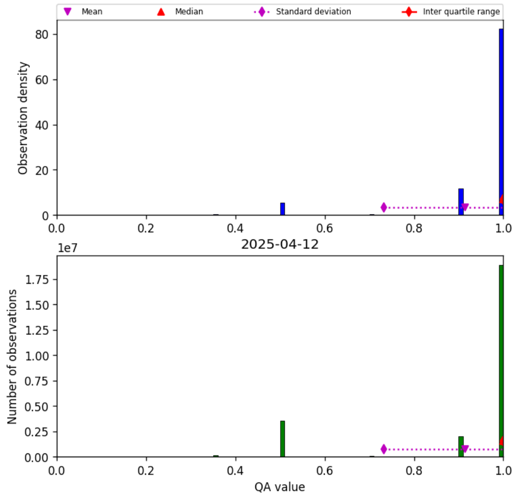
Figure 27: Histogram of “QA value” for 2025-04-12 to 2025-04-13
