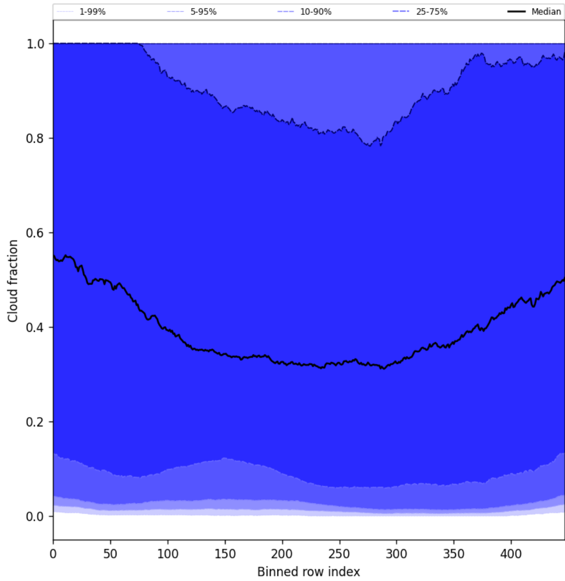
Figure 47: Along track statistics of “Cloud fraction” for 2025-04-12 to 2025-04-13
