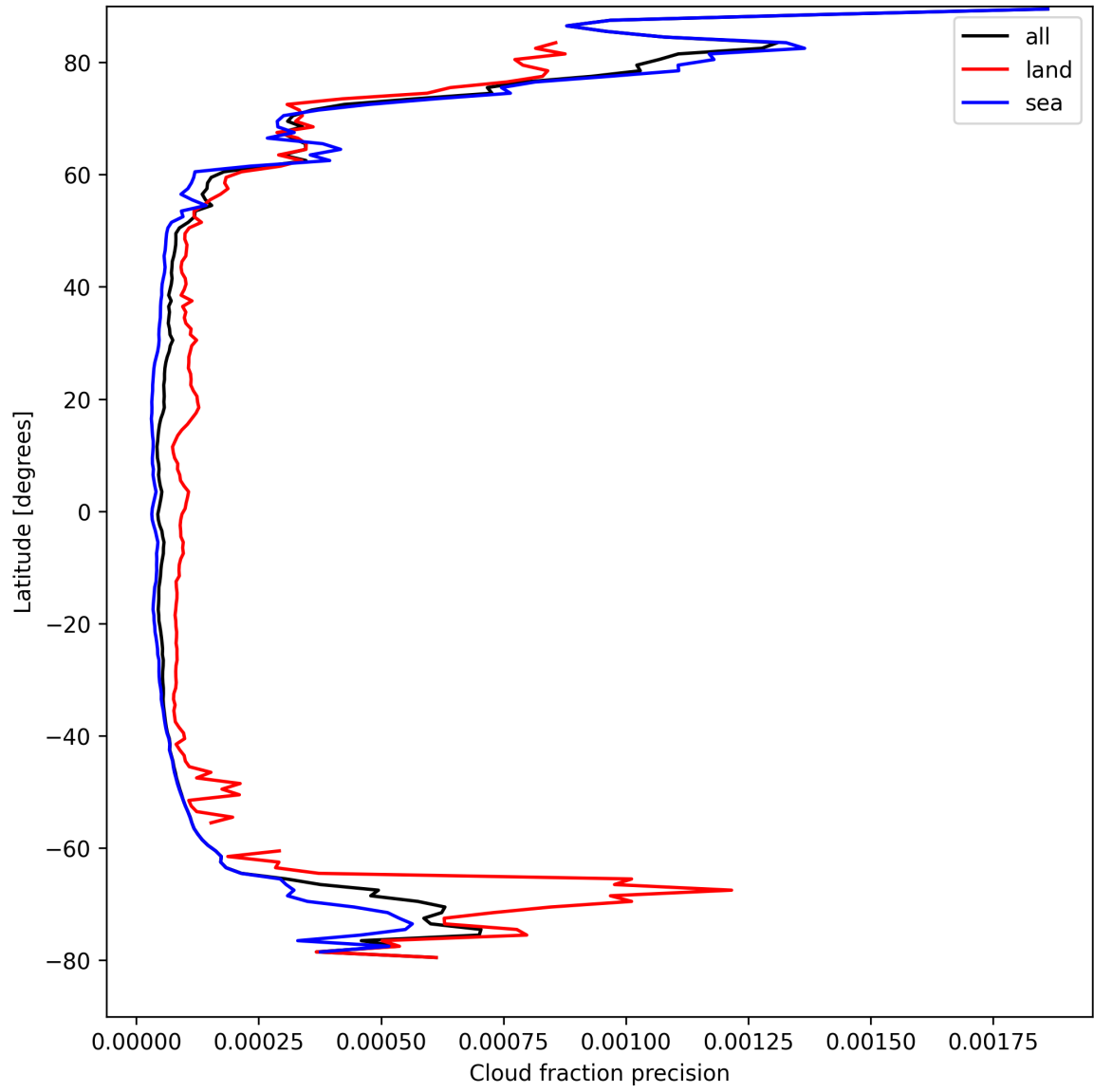
Figure 14: Zonal average of “Cloud fraction precision” for 2025-04-12 to 2025-04-13.
