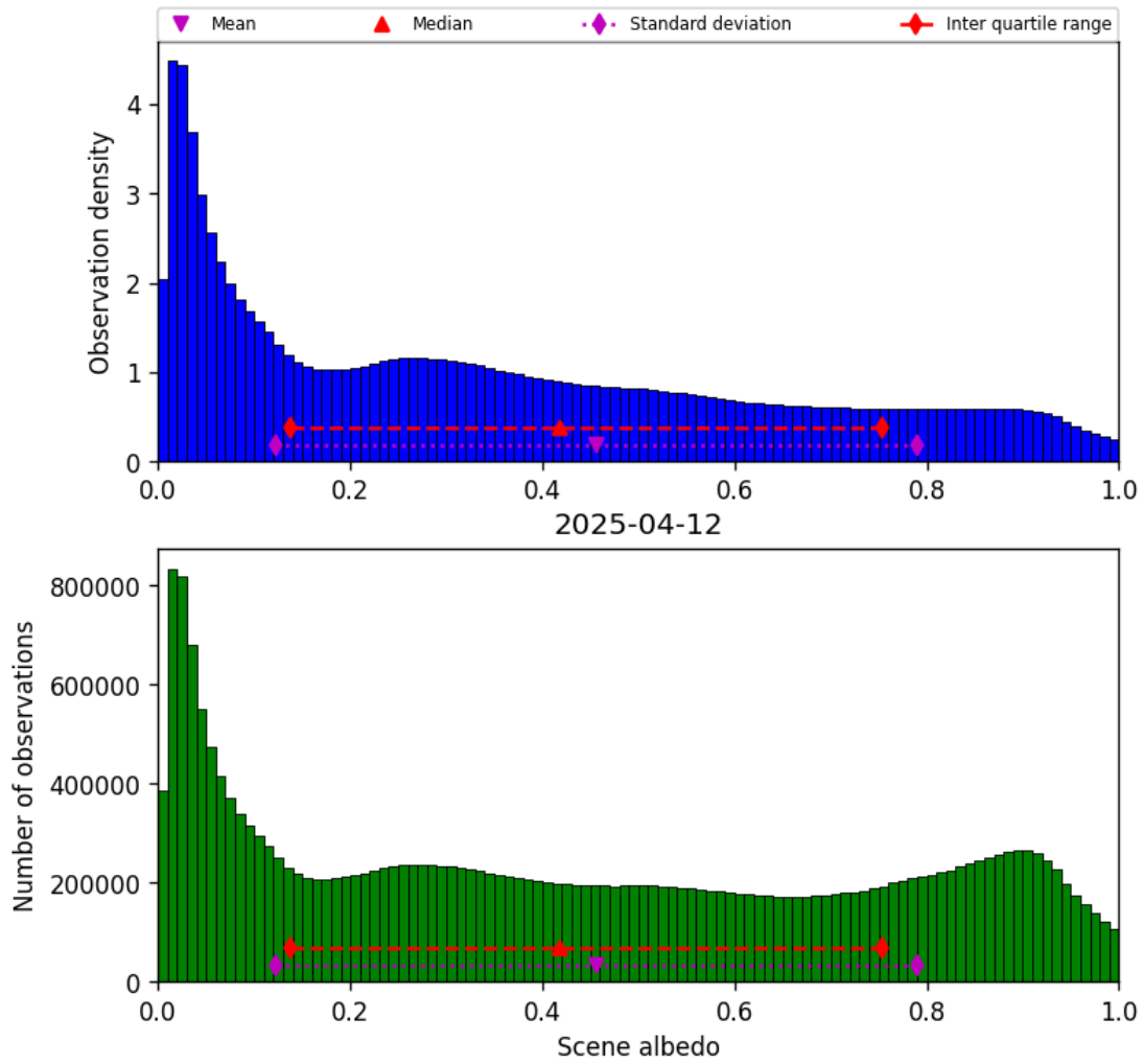
Figure 32: Histogram of “Scene albedo” for 2025-04-12 to 2025-04-13
