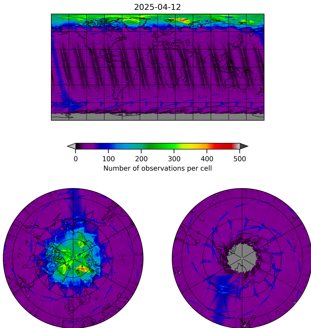
Figure 9: Map of the number of observations for 2025-04-12 to 2025-04-13
