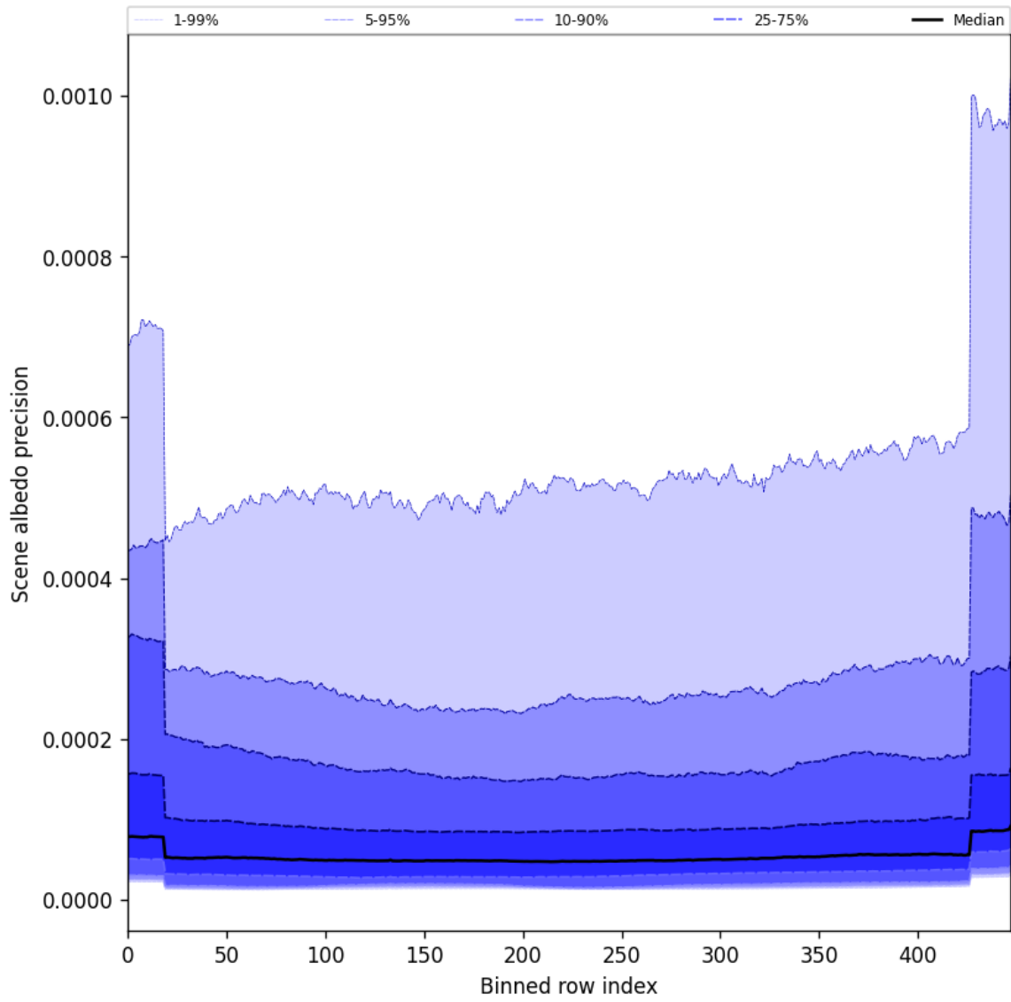
Figure 50: Along track statistics of “Scene albedo precision” for 2025-04-12 to 2025-04-13
