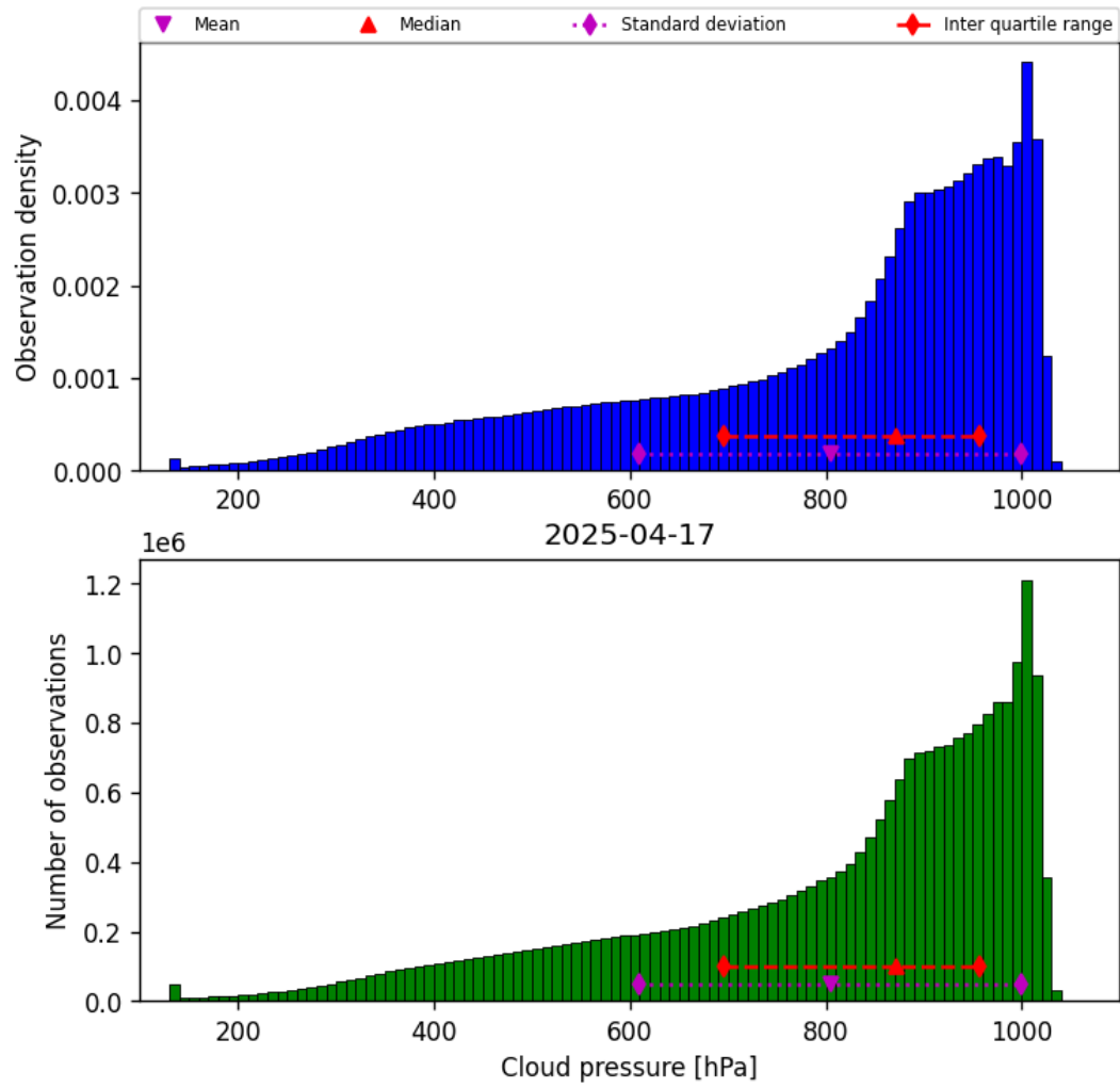
Figure 28: Histogram of “Cloud pressure” for 2025-04-17 to 2025-04-18
