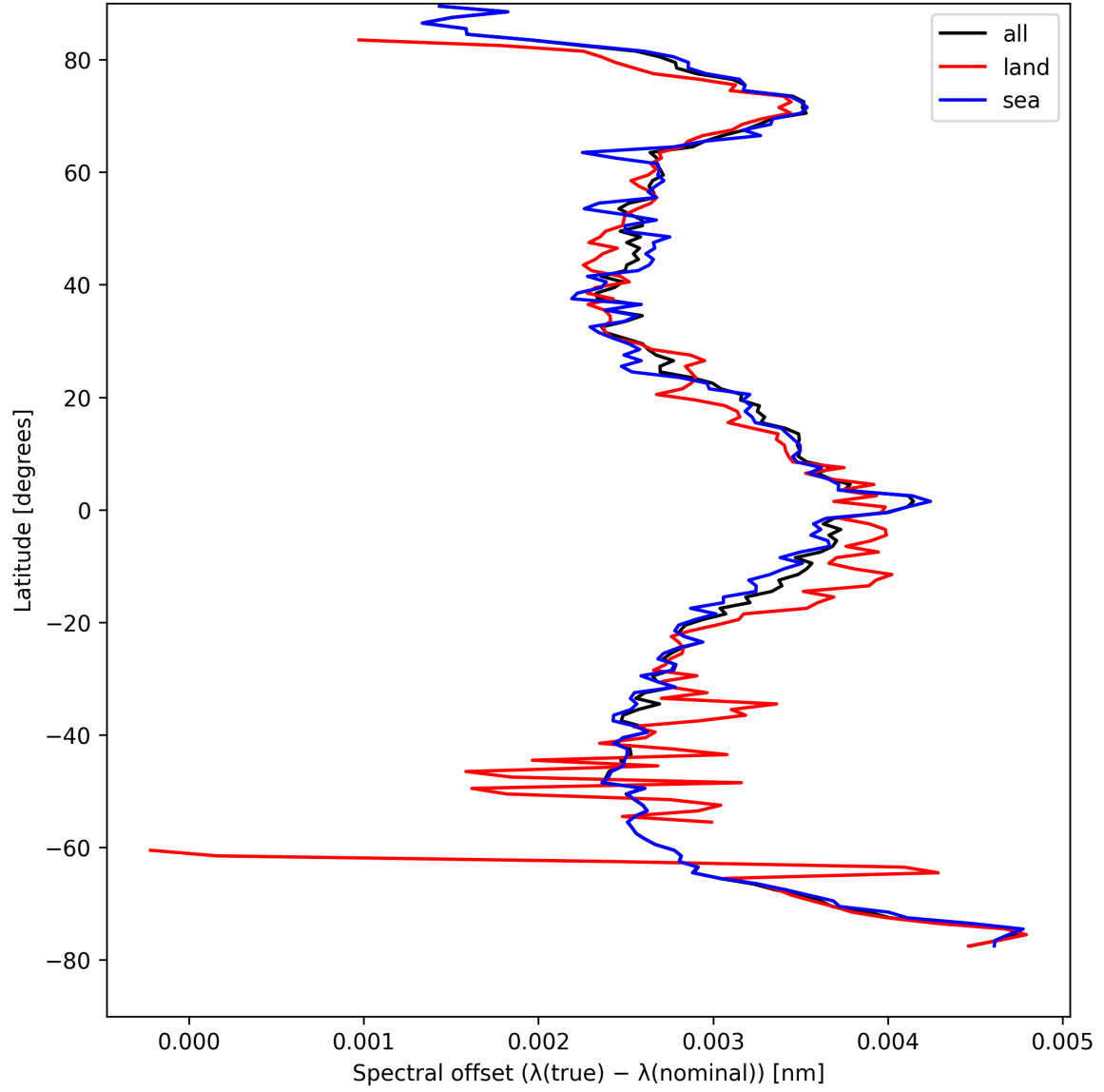
Figure 26: Zonal average of “Spectral offset ( \lambda_{\text{true}} - \lambda_{\text{nominal}} )” for 2025-04-17 to 2025-04-18.
