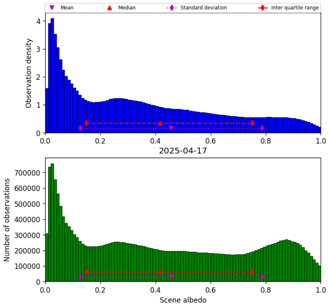
Figure 32: Histogram of “Scene albedo” for 2025-04-17 to 2025-04-18
