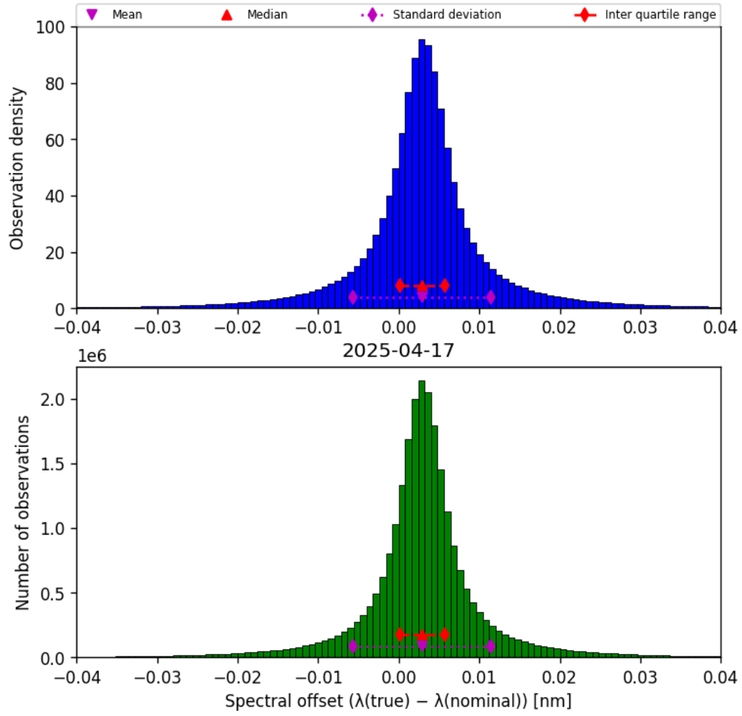
Figure 43: Histogram of “Spectral offset ( \lambda_{\text{true}} - \lambda_{\text{nominal}} )” for 2025-04-17 to 2025-04-18
