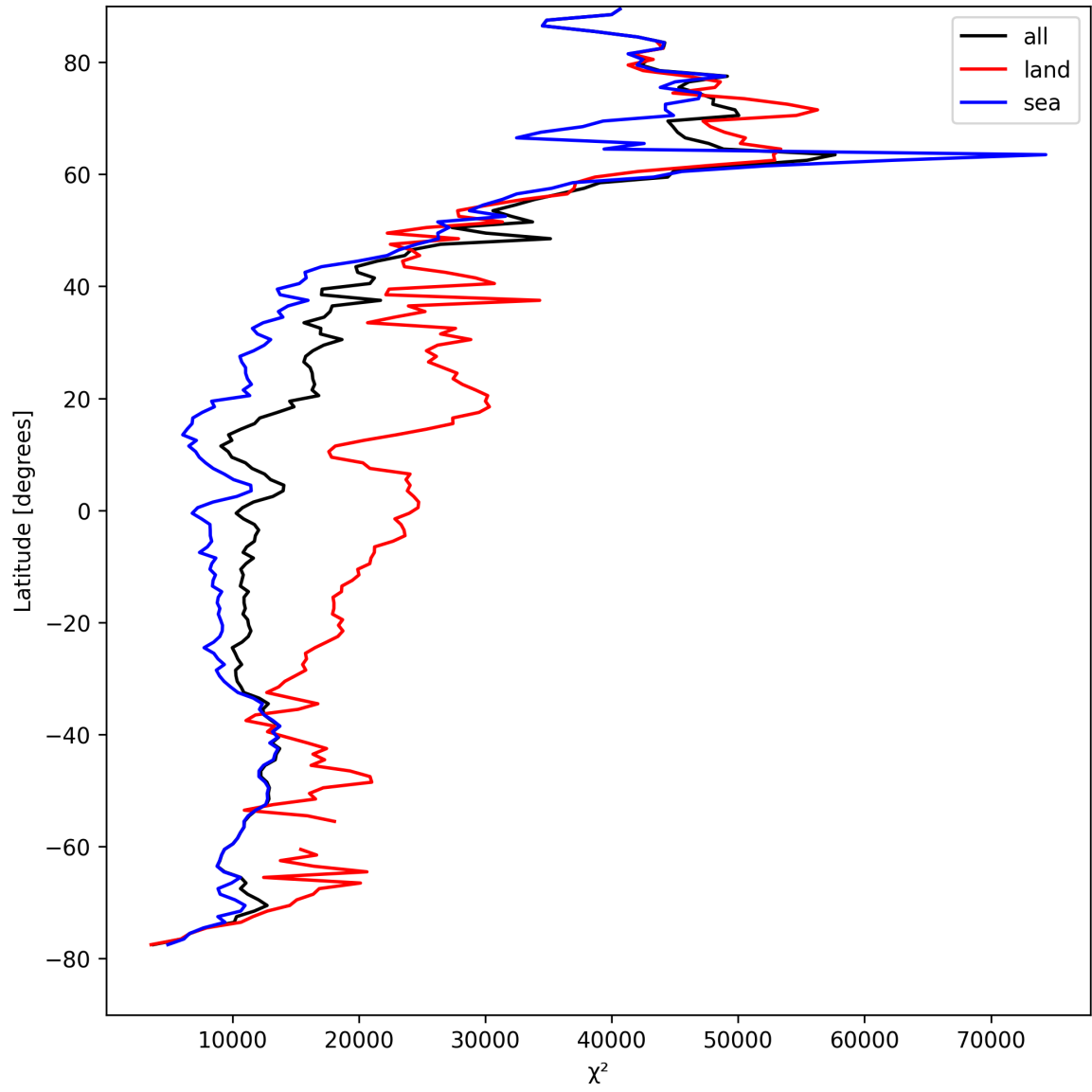
Figure 19: Zonal average of “ \chi^2 ” for 2025-04-17 to 2025-04-18.
