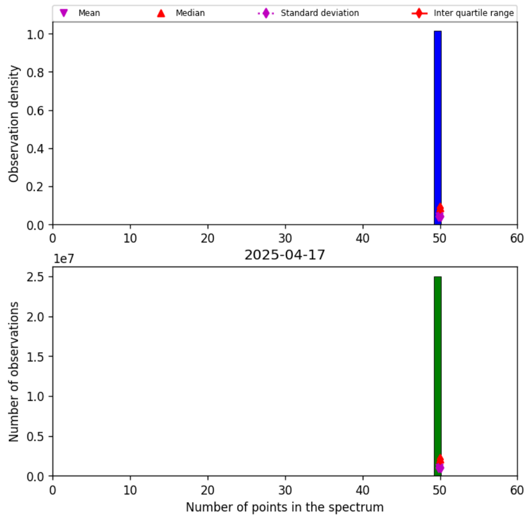
Figure 42: Histogram of “Number of points in the spectrum” for 2025-04-17 to 2025-04-18
