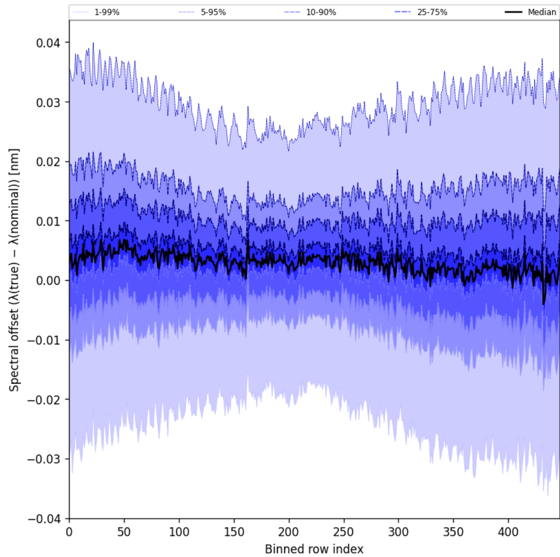
Figure 60: Along track statistics of “Spectral offset ( \lambda_{\text{true}} - \lambda_{\text{nominal}} )” for 2025-04-17 to 2025-04-18
