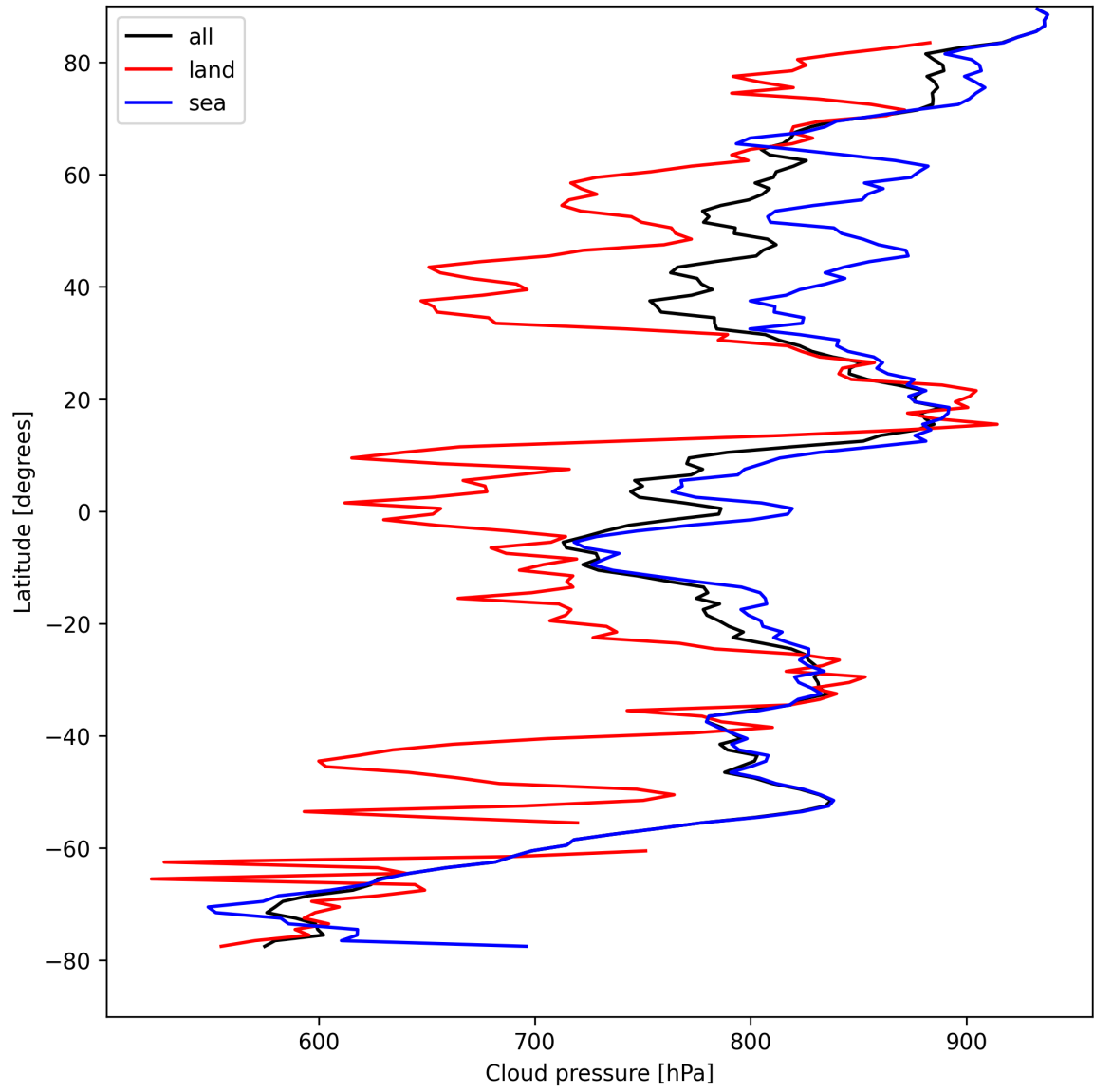
Figure 11: Zonal average of “Cloud pressure” for 2025-04-17 to 2025-04-18.
