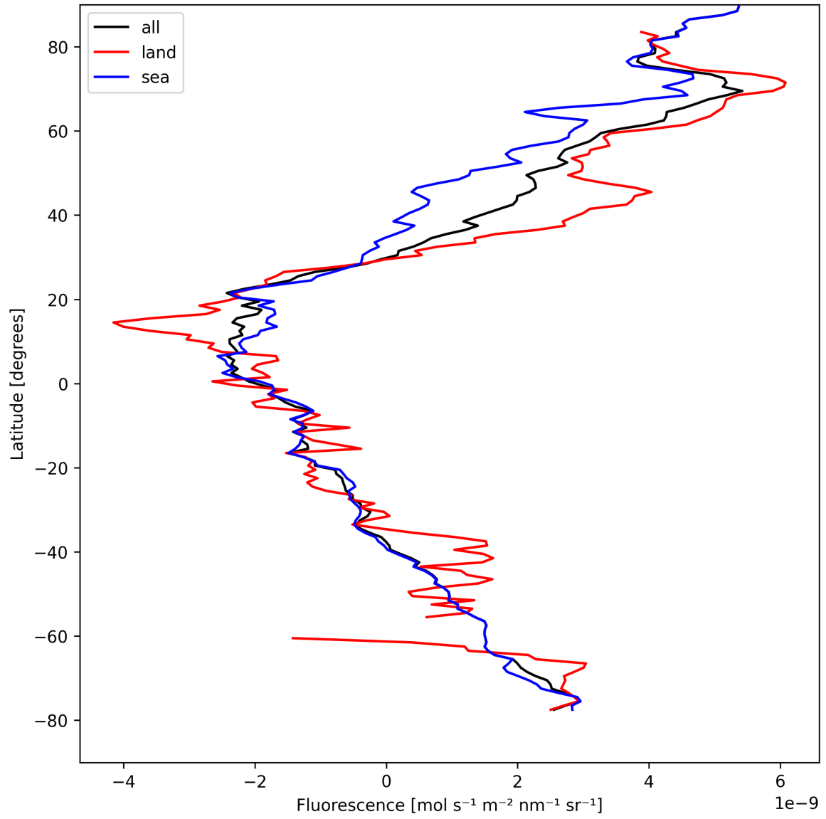
Figure 21: Zonal average of “Fluorescence” for 2025-04-17 to 2025-04-18.
