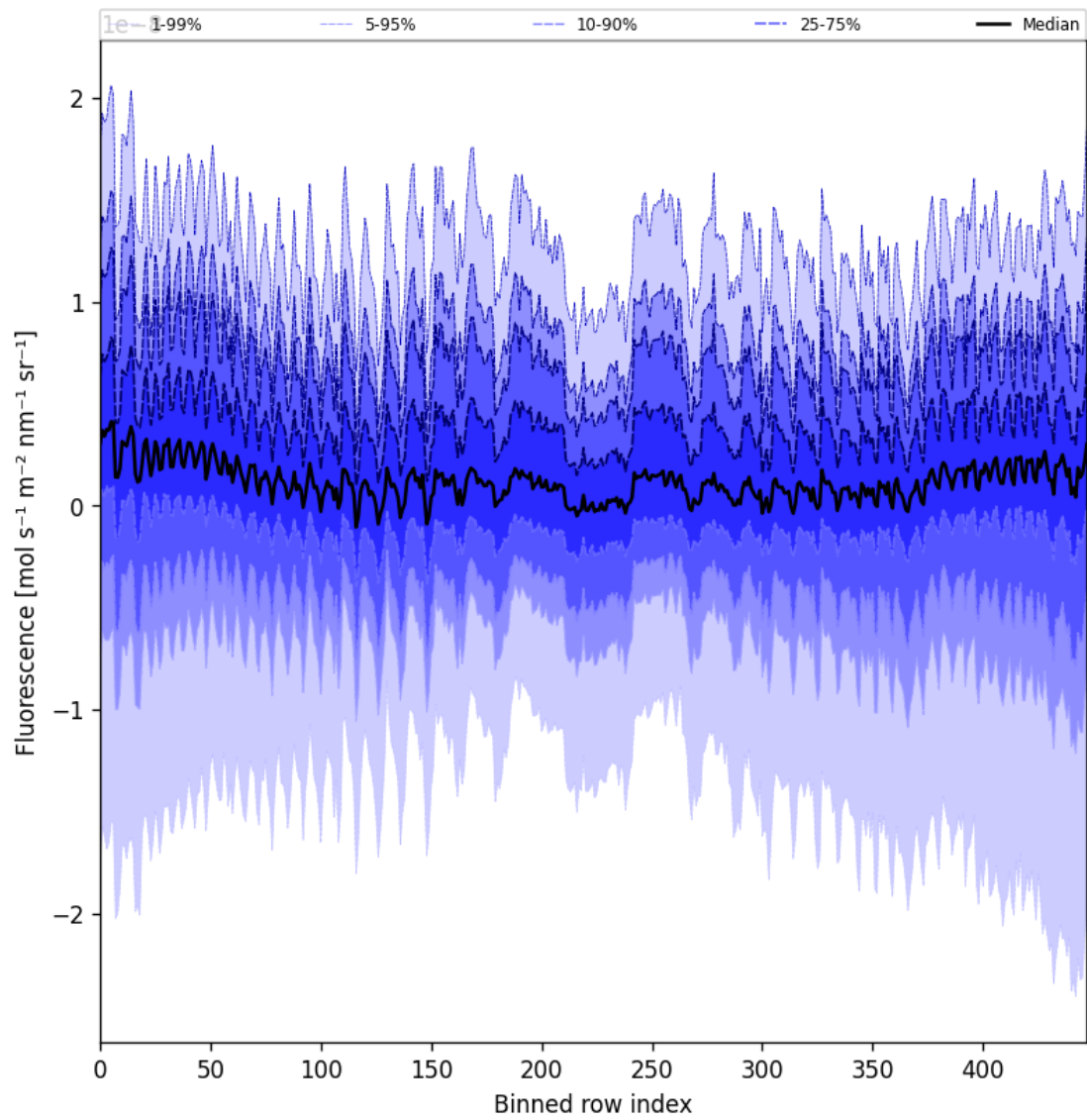
Figure 55: Along track statistics of “Fluorescence” for 2025-04-17 to 2025-04-18
