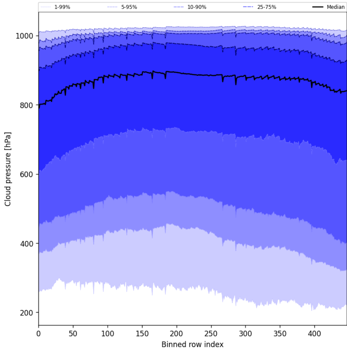
Figure 45: Along track statistics of “Cloud pressure” for 2025-04-17 to 2025-04-18
