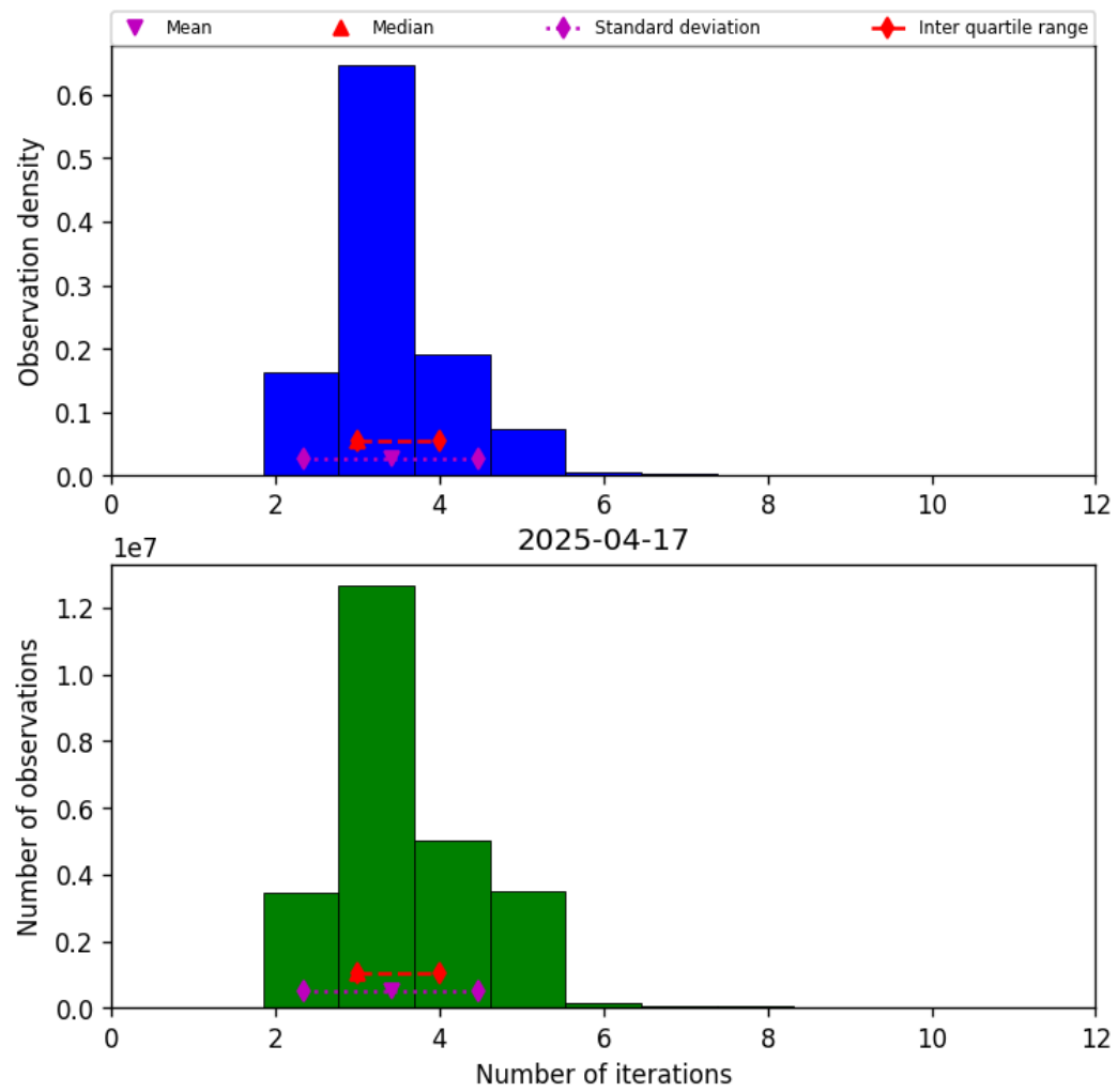
Figure 37: Histogram of “Number of iterations” for 2025-04-17 to 2025-04-18
