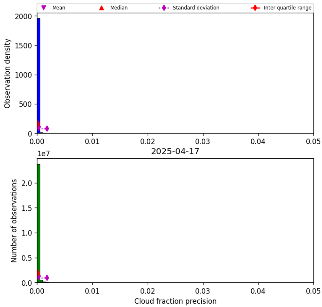
Figure 31: Histogram of “Cloud fraction precision” for 2025-04-17 to 2025-04-18
