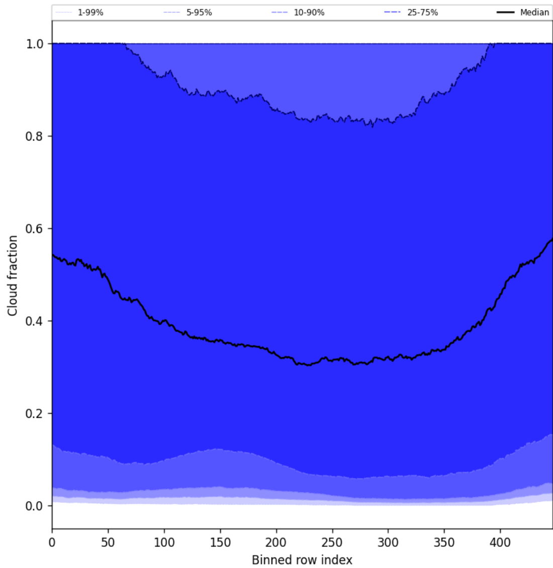
Figure 47: Along track statistics of “Cloud fraction” for 2025-04-17 to 2025-04-18
