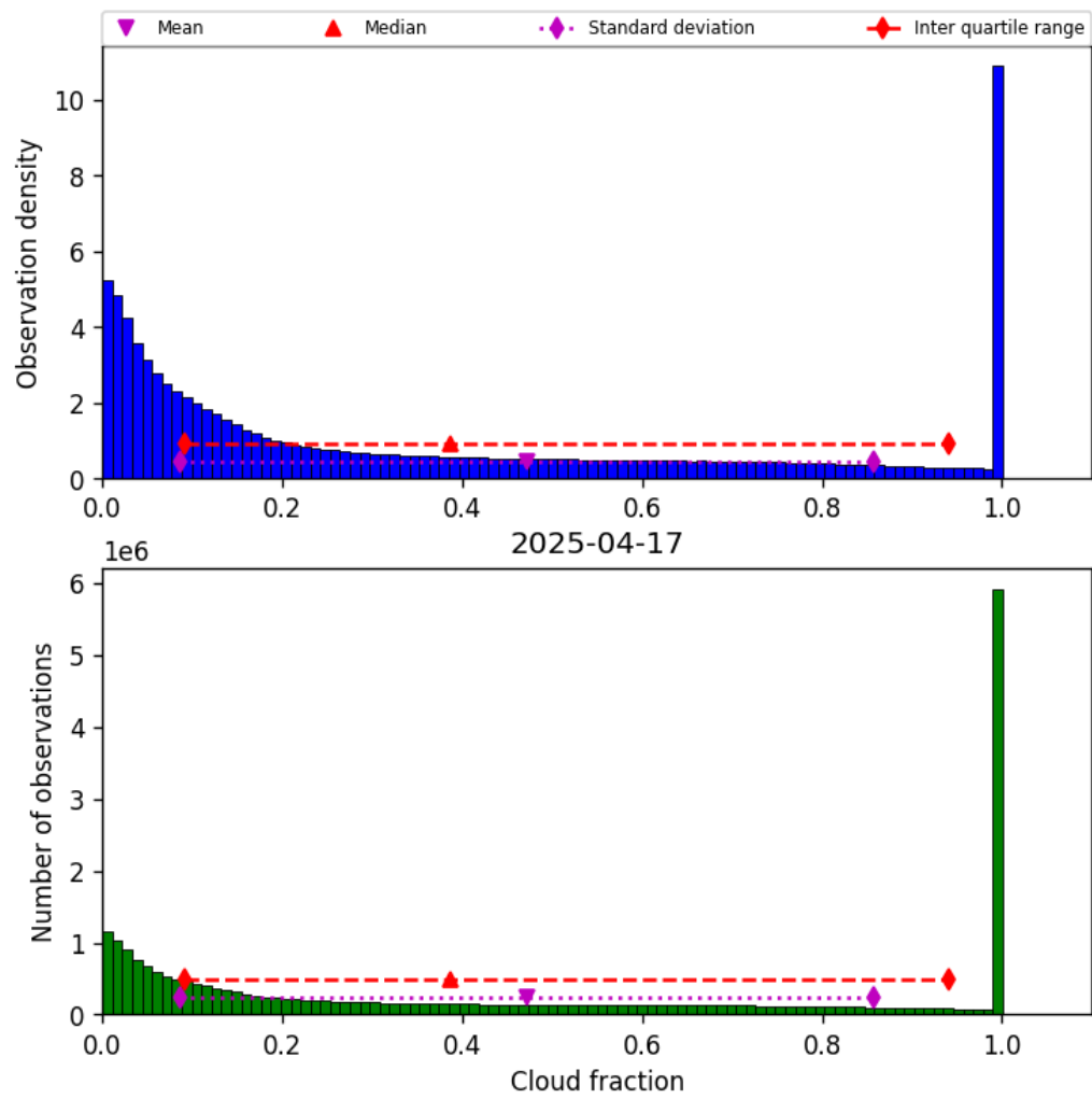
Figure 30: Histogram of “Cloud fraction” for 2025-04-17 to 2025-04-18
