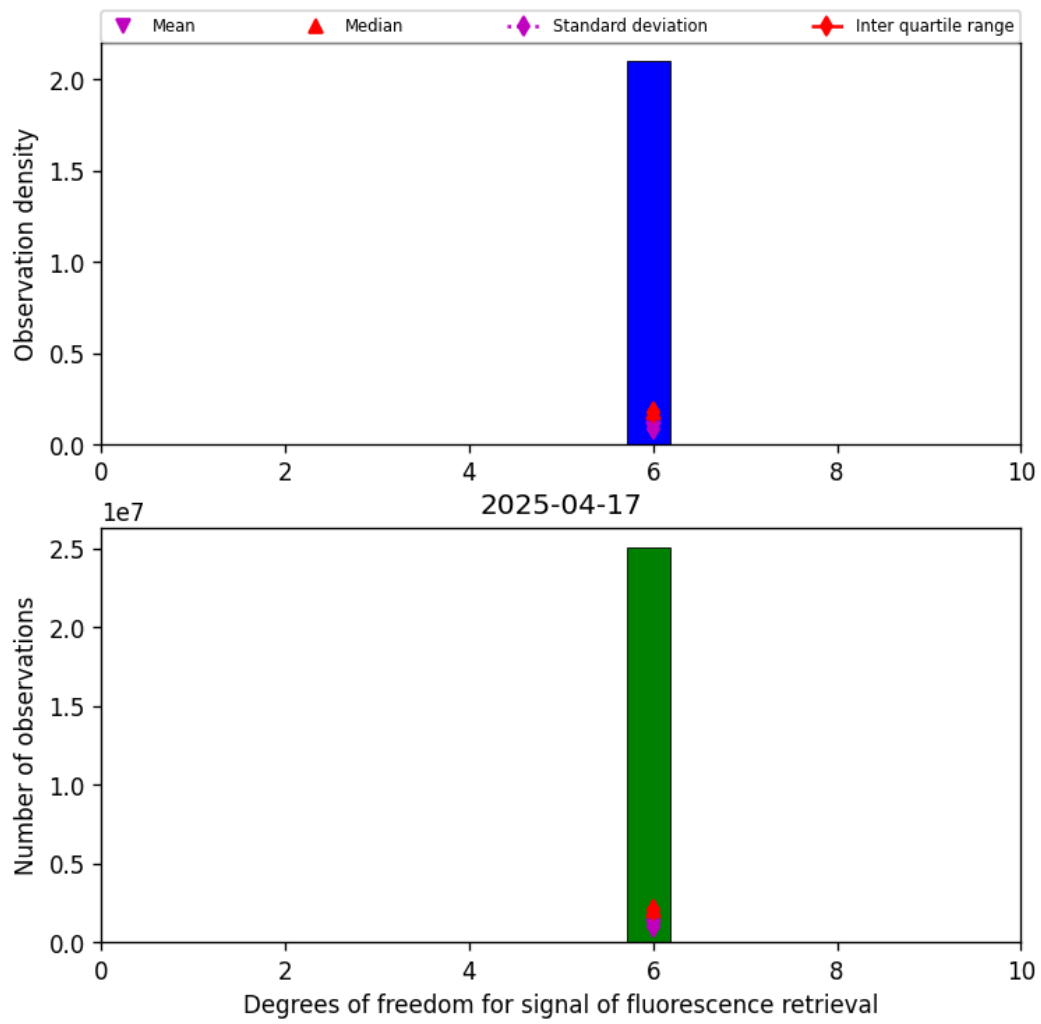
Figure 41: Histogram of “Degrees of freedom for signal of fluorescence retrieval” for 2025-04-17 to 2025-04-18
