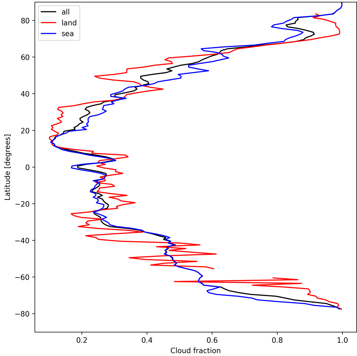
Figure 13: Zonal average of “Cloud fraction” for 2025-04-17 to 2025-04-18.
