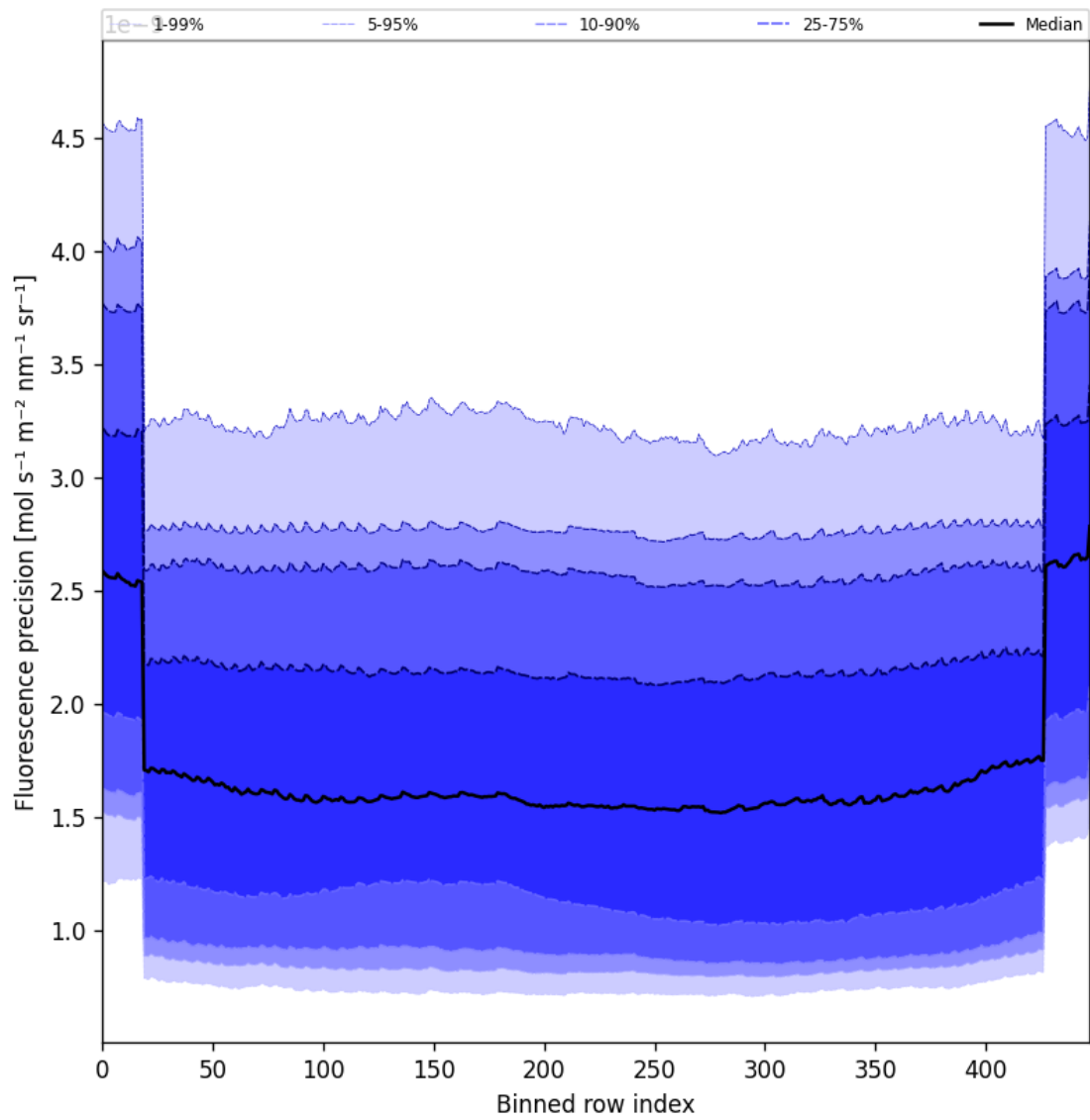
Figure 56: Along track statistics of “Fluorescence precision” for 2025-04-17 to 2025-04-18
