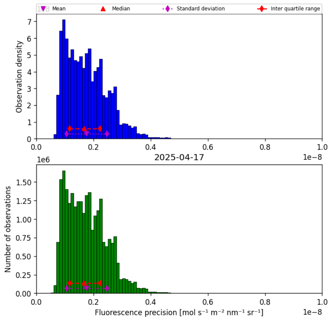
Figure 39: Histogram of “Fluorescence precision” for 2025-04-17 to 2025-04-18
