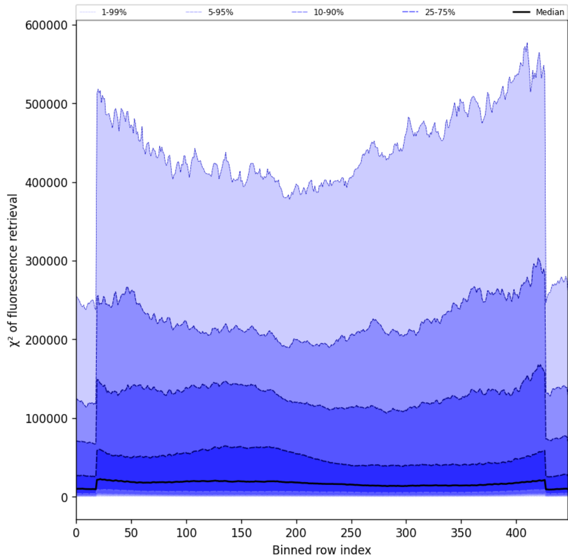
Figure 57: Along track statistics of “ \chi^2 of fluorescence retrieval” for 2025-04-17 to 2025-04-18
