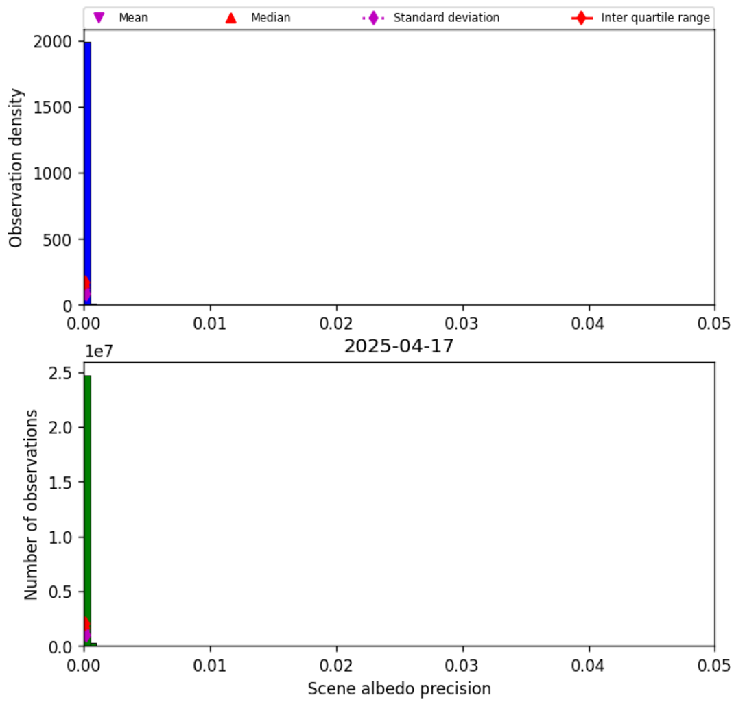
Figure 33: Histogram of “Scene albedo precision” for 2025-04-17 to 2025-04-18
