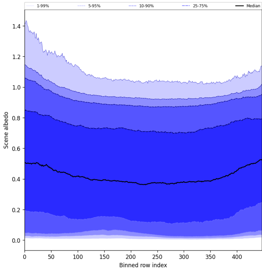
Figure 49: Along track statistics of “Scene albedo” for 2025-04-17 to 2025-04-18
