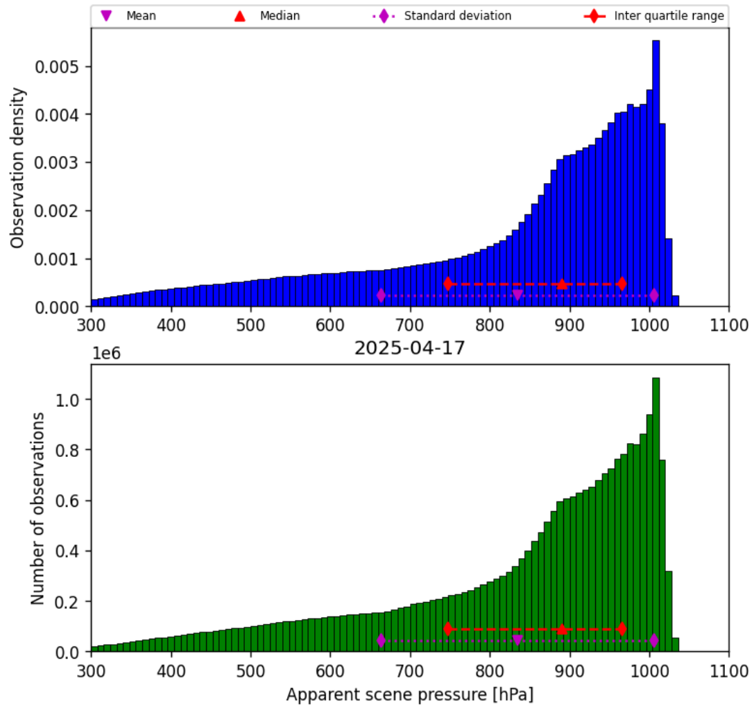
Figure 34: Histogram of “Apparent scene pressure” for 2025-04-17 to 2025-04-18
