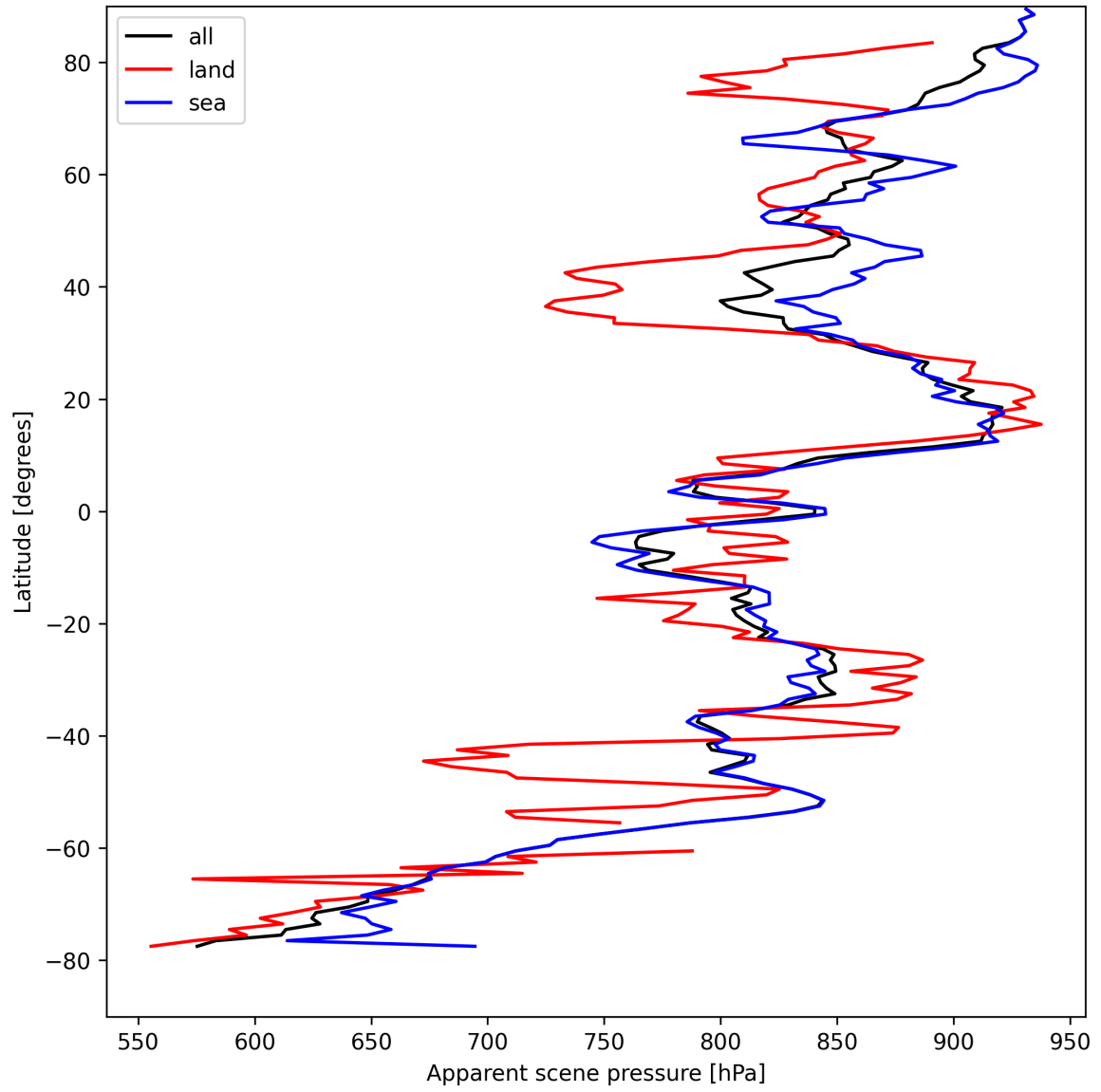
Figure 17: Zonal average of “Apparent scene pressure” for 2025-04-17 to 2025-04-18.
