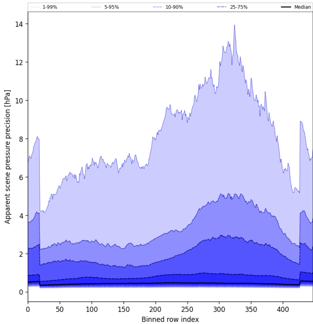
Figure 52: Along track statistics of “Apparent scene pressure precision” for 2025-04-17 to 2025-04-18
