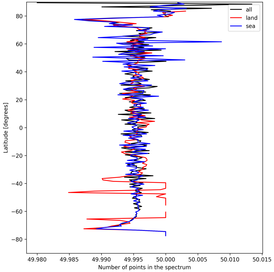
Figure 25: Zonal average of “Number of points in the spectrum” for 2025-04-17 to 2025-04-18.
