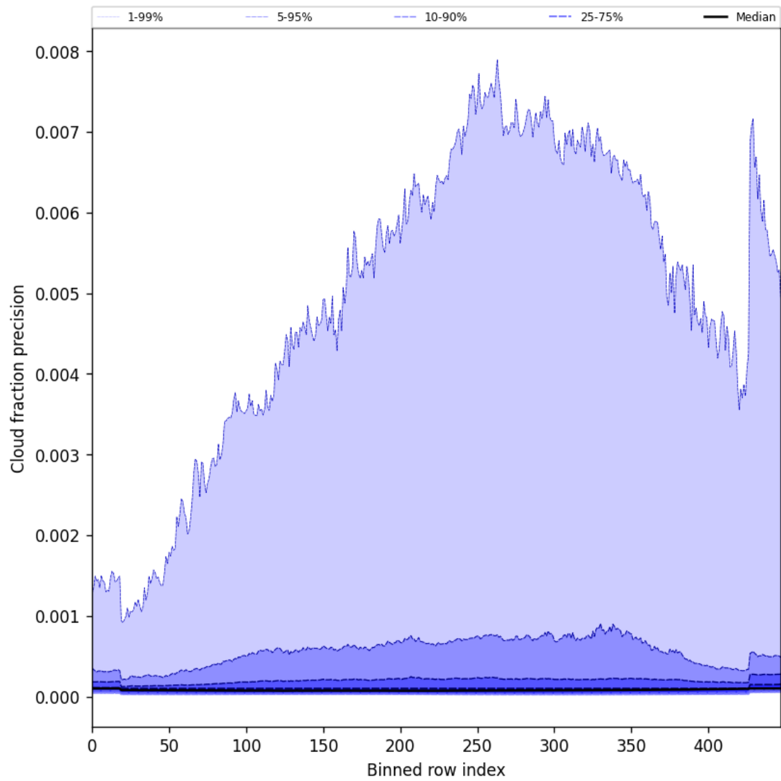
Figure 48: Along track statistics of “Cloud fraction precision” for 2025-04-17 to 2025-04-18
