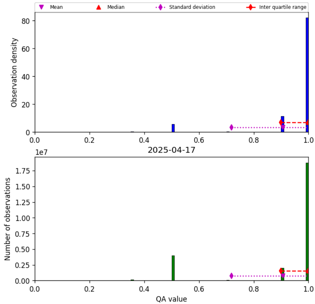
Figure 27: Histogram of “QA value” for 2025-04-17 to 2025-04-18
