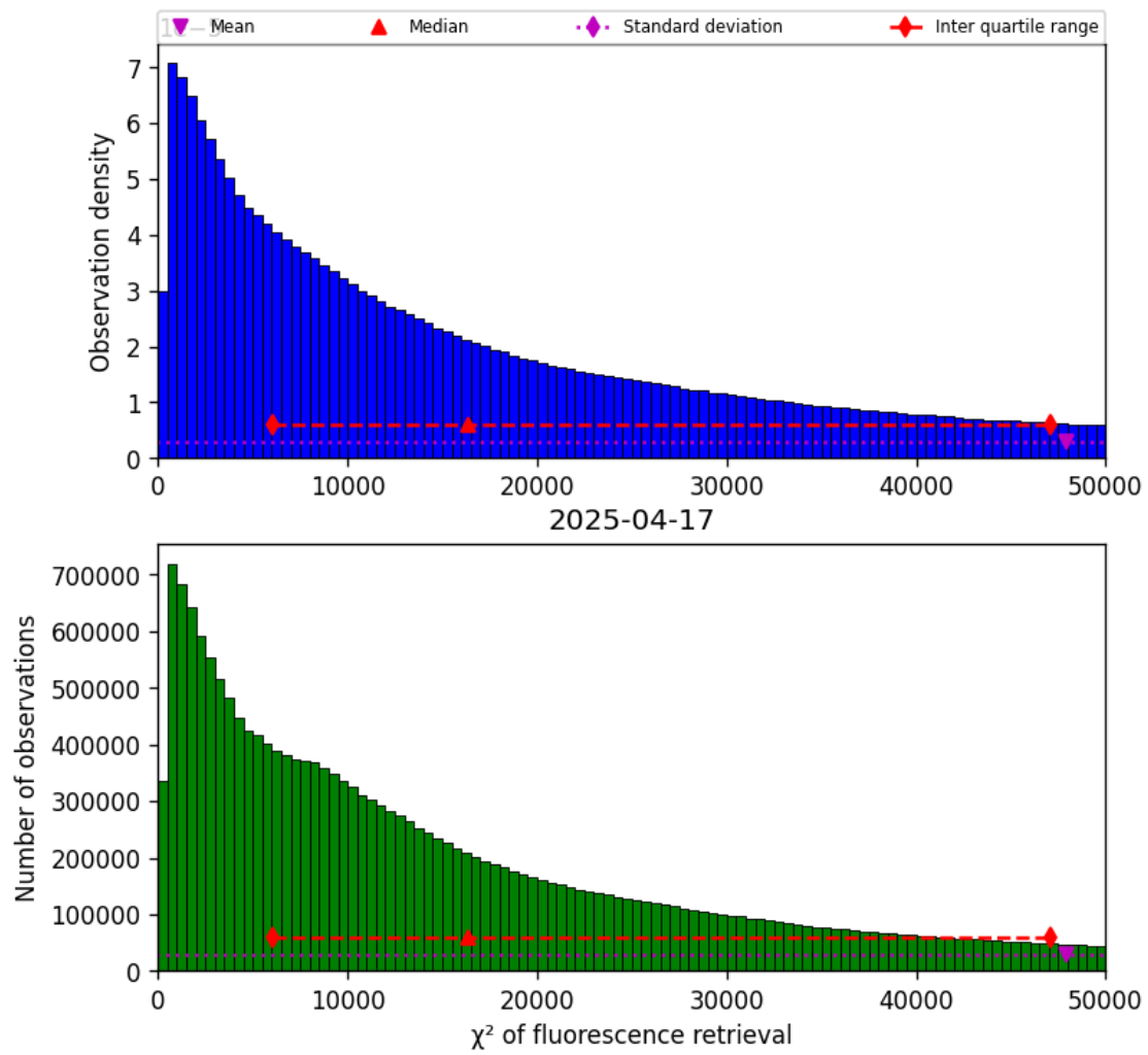
Figure 40: Histogram of “ \chi^2 of fluorescence retrieval” for 2025-04-17 to 2025-04-18
