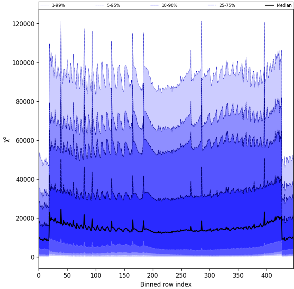
Figure 53: Along track statistics of “ \chi^2 ” for 2025-04-17 to 2025-04-18
