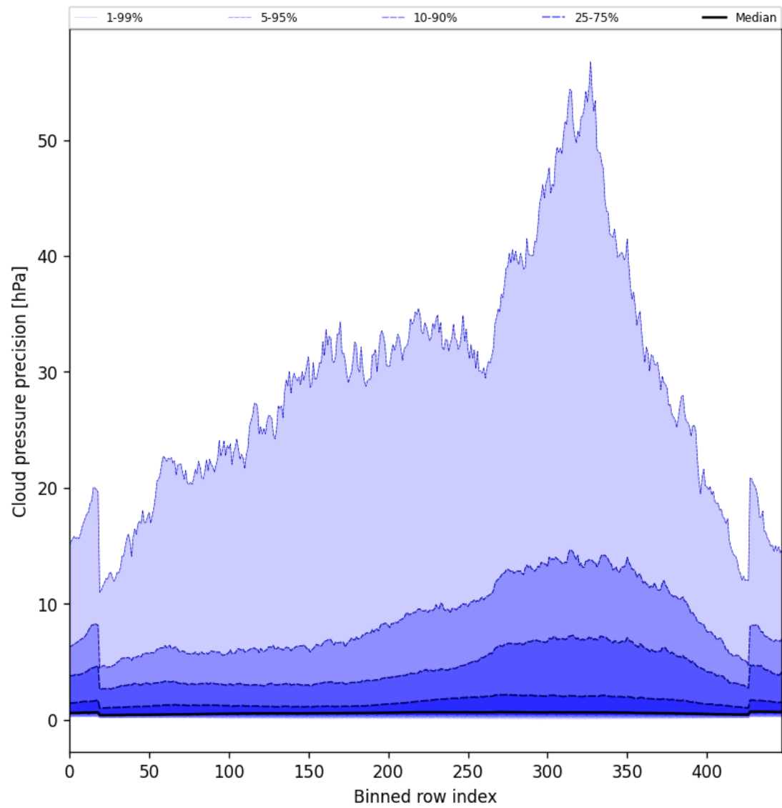
Figure 46: Along track statistics of “Cloud pressure precision” for 2025-04-17 to 2025-04-18
