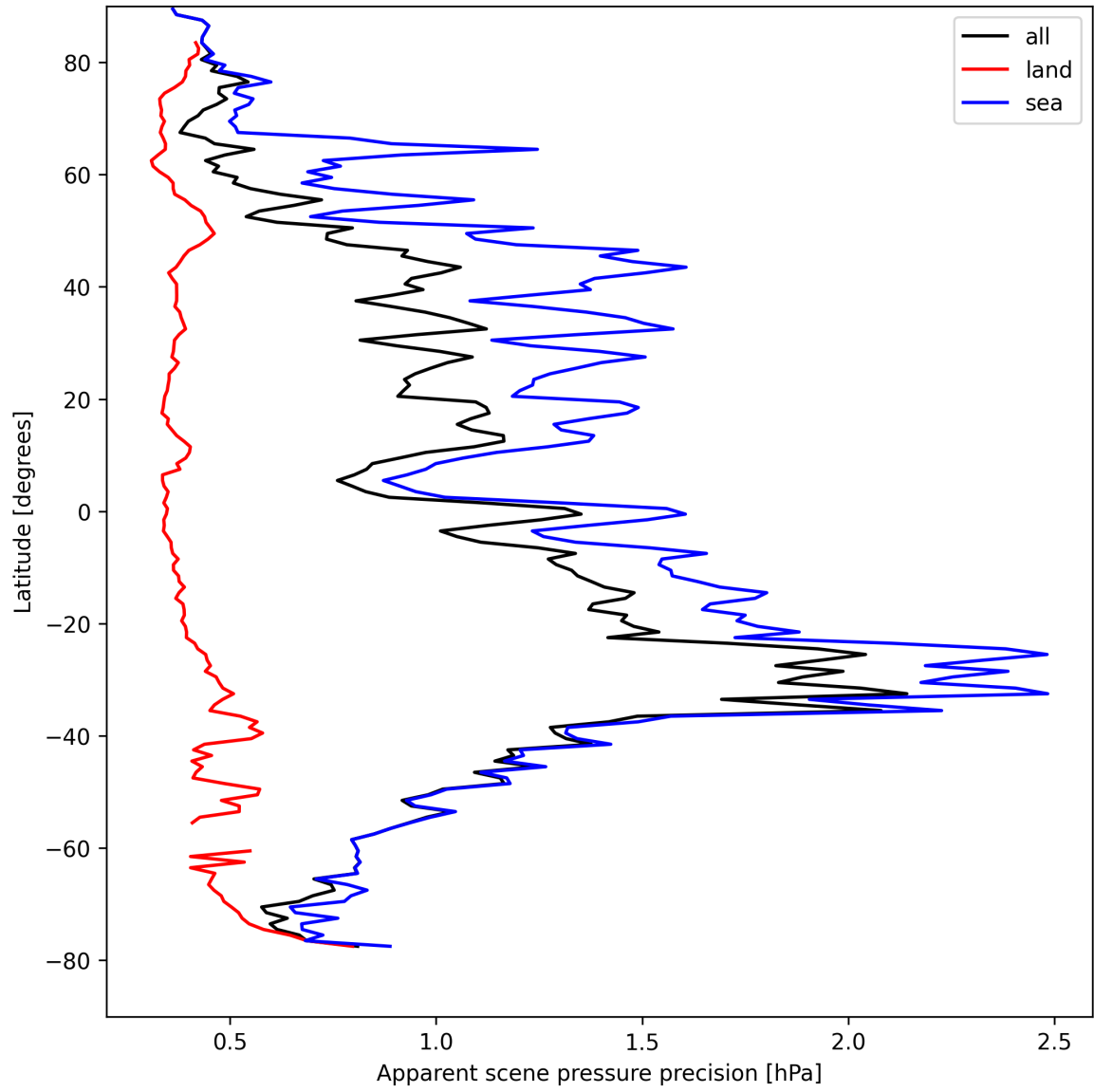
Figure 18: Zonal average of “Apparent scene pressure precision” for 2025-04-17 to 2025-04-18.
