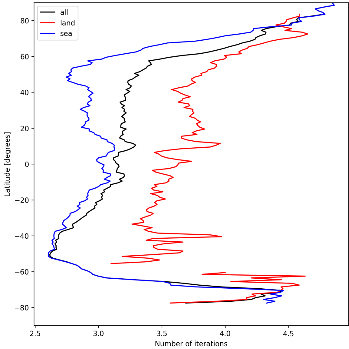
Figure 20: Zonal average of “Number of iterations” for 2025-04-17 to 2025-04-18.
