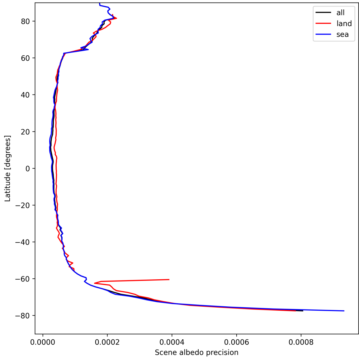
Figure 16: Zonal average of “Scene albedo precision” for 2025-04-17 to 2025-04-18.
