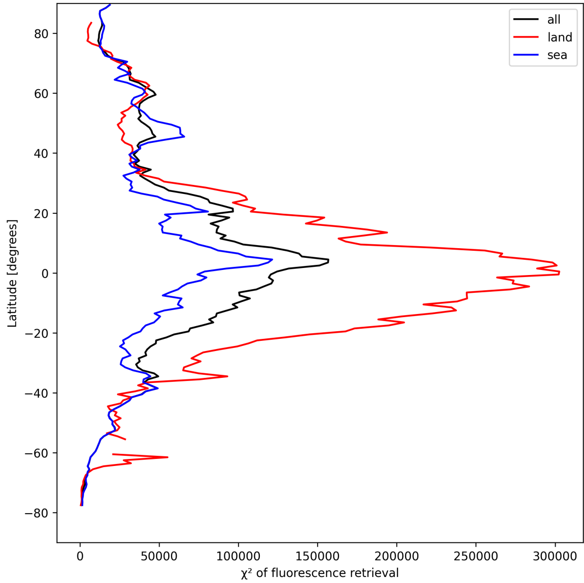
Figure 23: Zonal average of “ \chi^2 of fluorescence retrieval” for 2025-04-17 to 2025-04-18.
