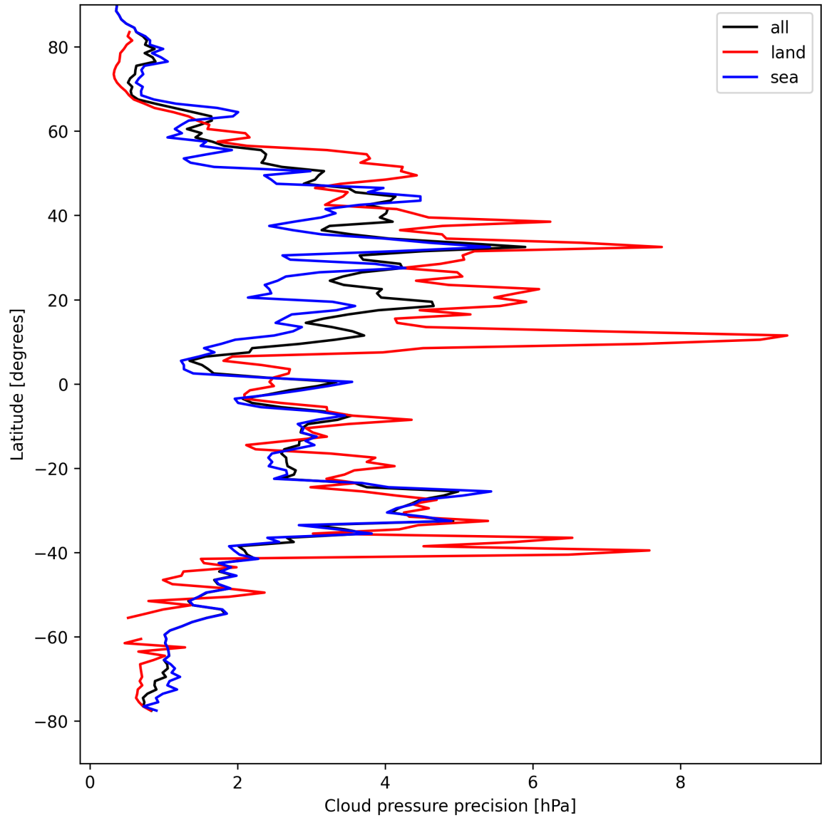
Figure 12: Zonal average of "Cloud pressure precision" for 2025-04-17 to 2025-04-18.
