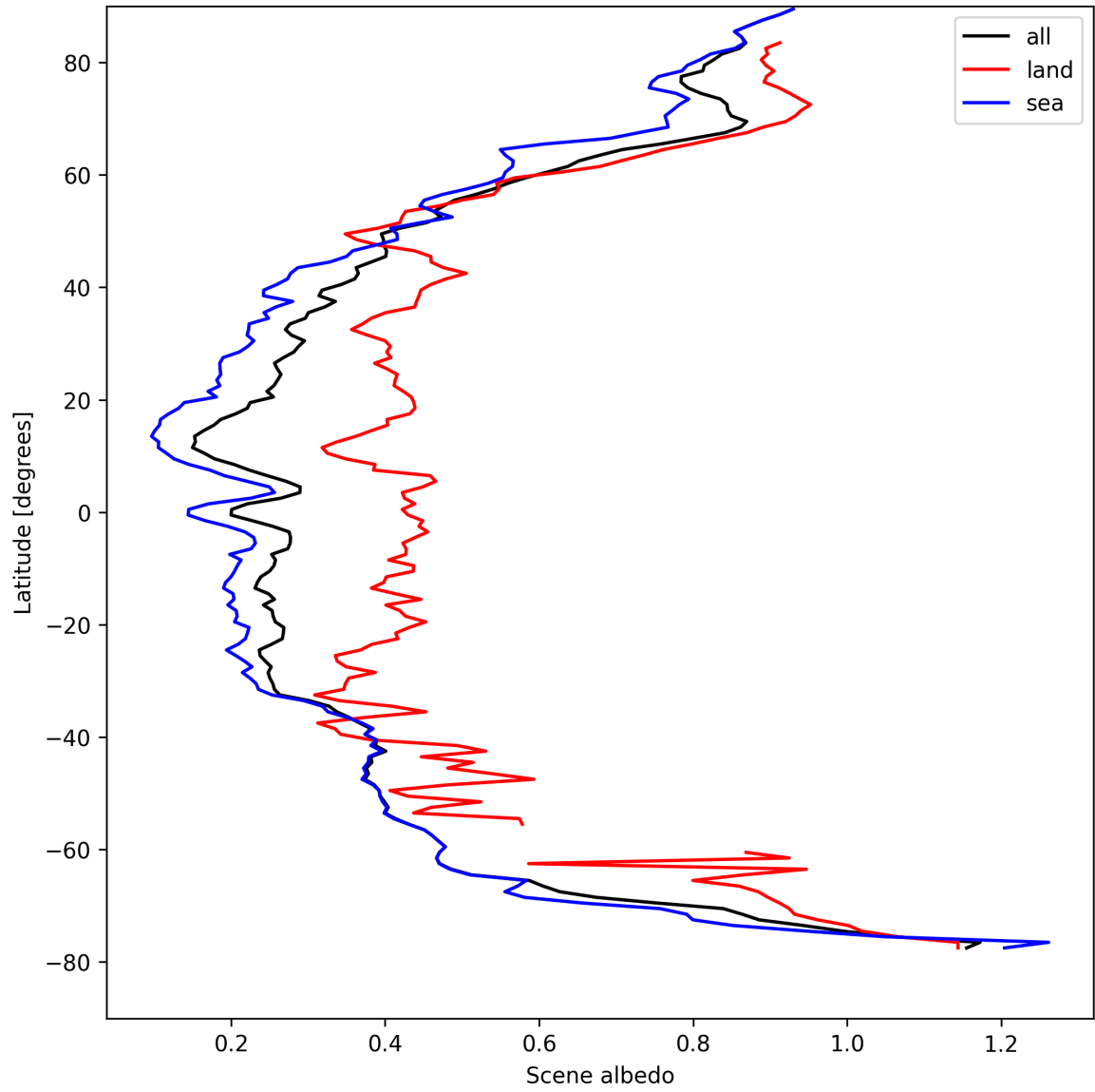
Figure 15: Zonal average of “Scene albedo” for 2025-04-17 to 2025-04-18.
