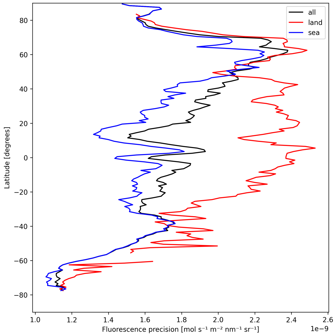
Figure 22: Zonal average of “Fluorescence precision” for 2025-04-17 to 2025-04-18.
