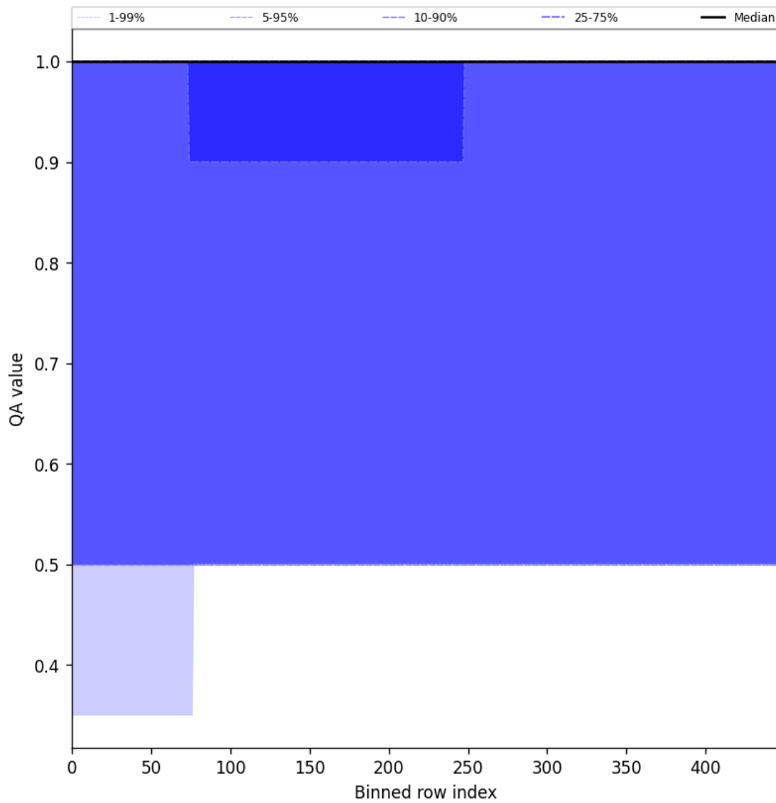
Figure 44: Along track statistics of “QA value” for 2025-04-17 to 2025-04-18
