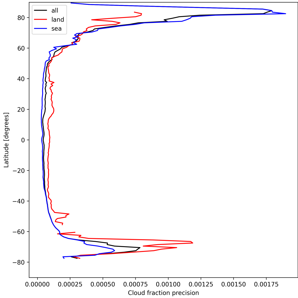
Figure 14: Zonal average of “Cloud fraction precision” for 2025-04-17 to 2025-04-18.
