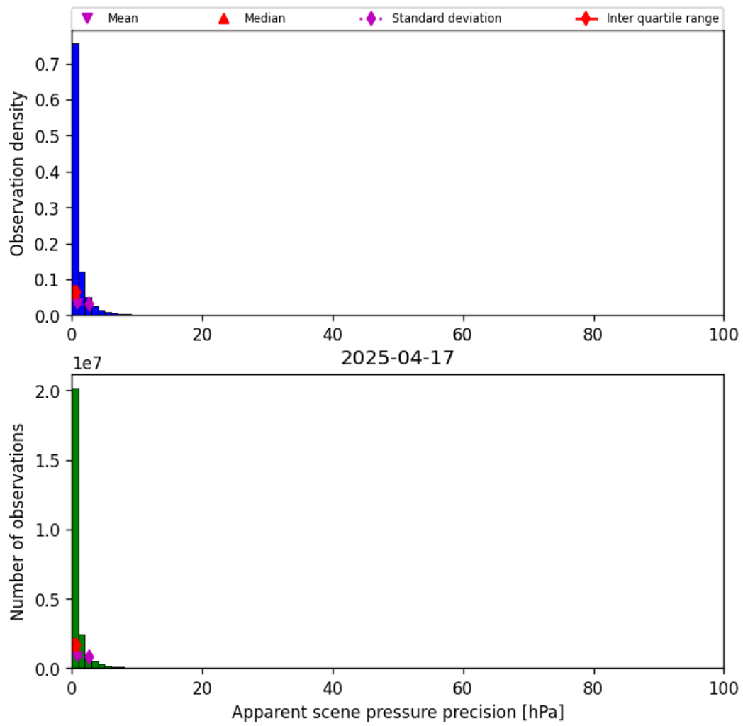
Figure 35: Histogram of “Apparent scene pressure precision” for 2025-04-17 to 2025-04-18
