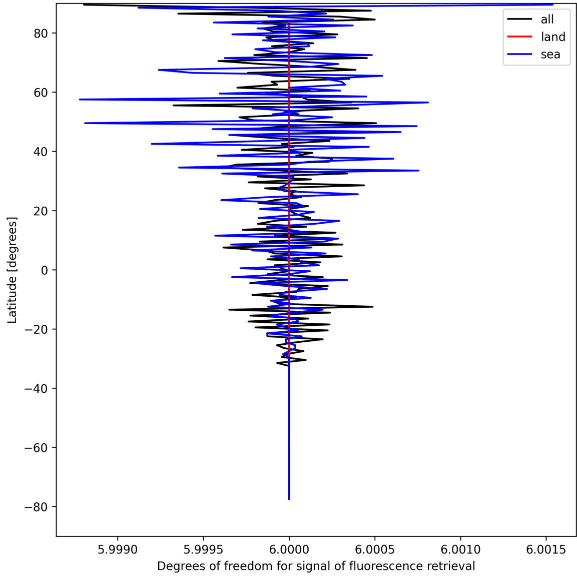
Figure 24: Zonal average of “Degrees of freedom for signal of fluorescence retrieval” for 2025-04-17 to 2025-04-18.
