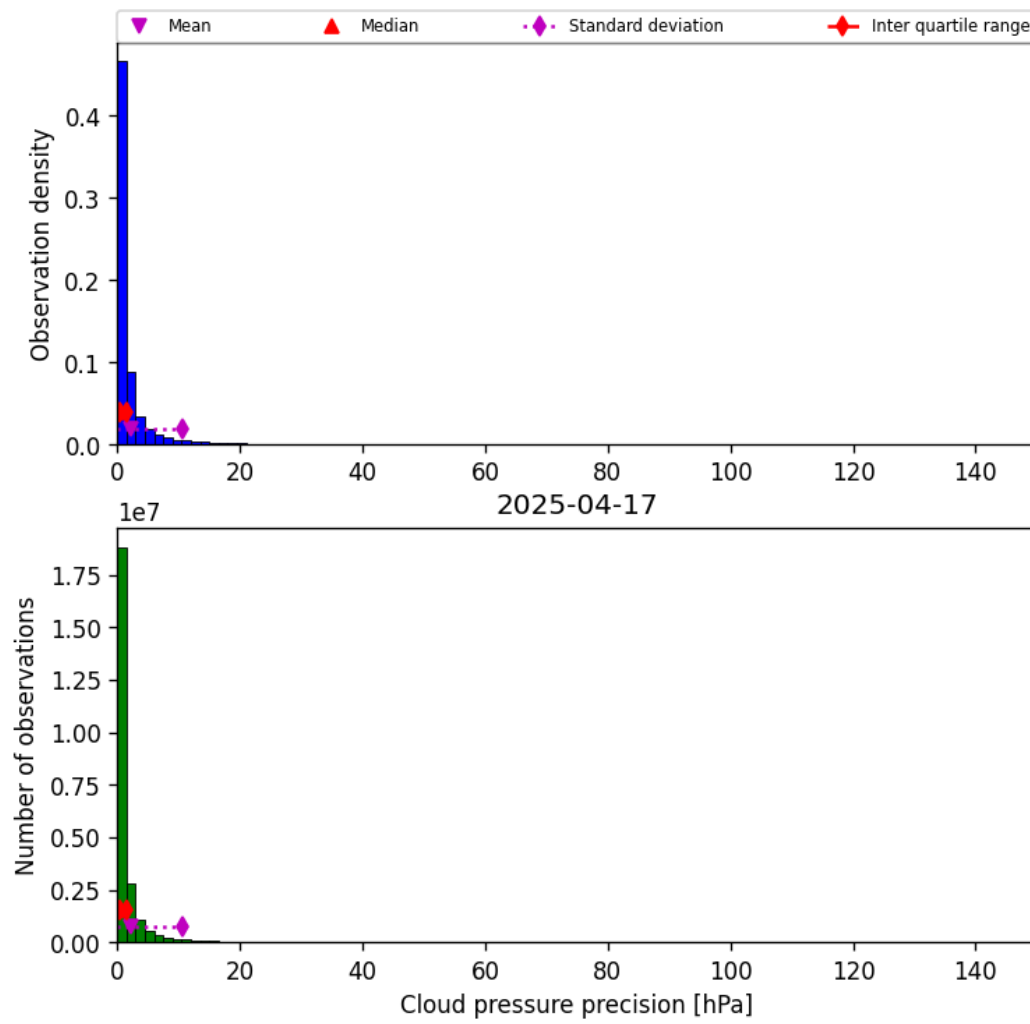
Figure 29: Histogram of “Cloud pressure precision” for 2025-04-17 to 2025-04-18
