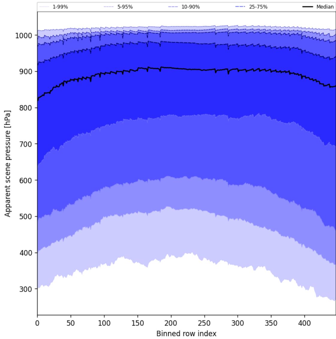
Figure 51: Along track statistics of “Apparent scene pressure” for 2025-04-17 to 2025-04-18
