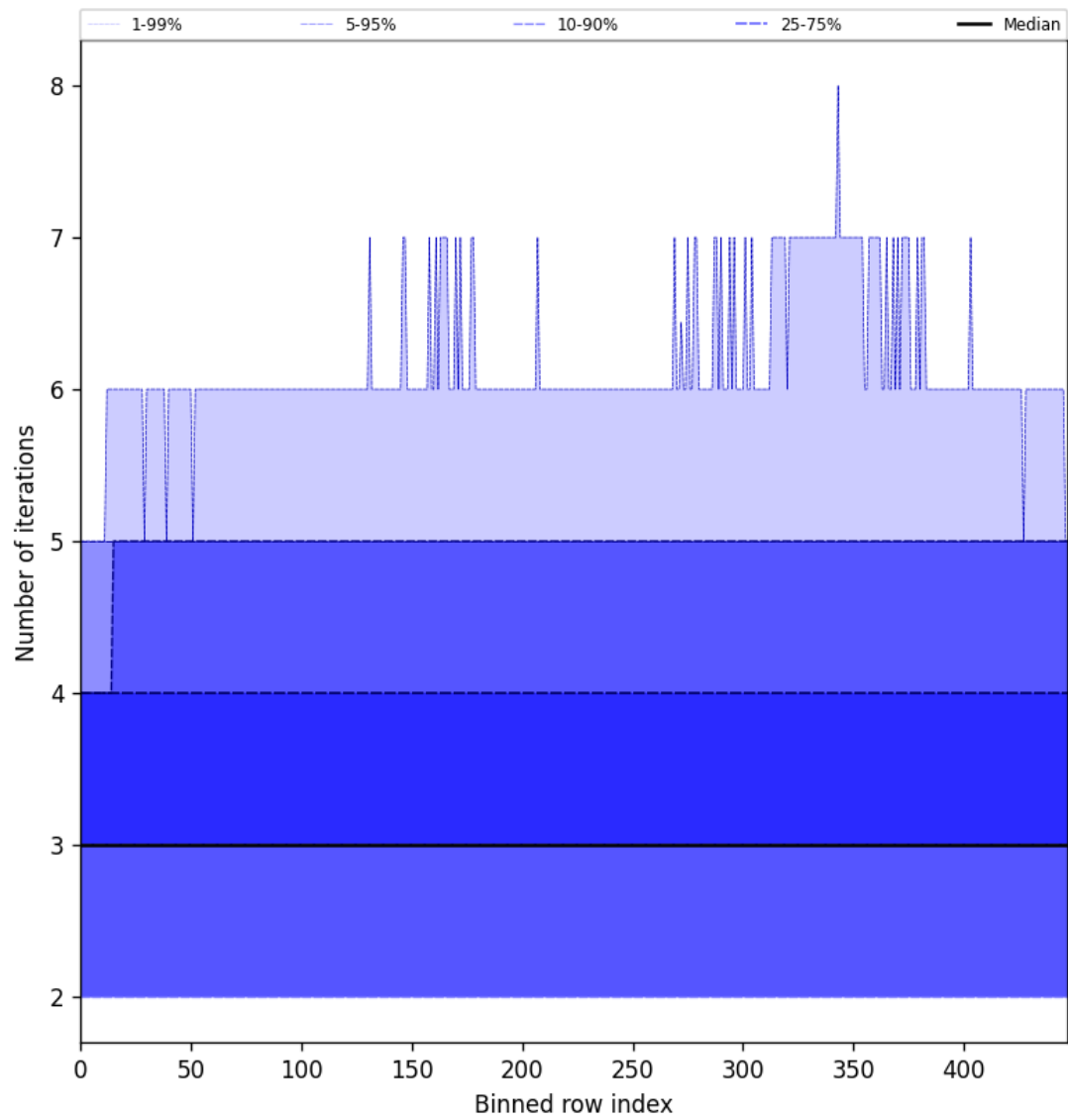
Figure 54: Along track statistics of “Number of iterations” for 2025-04-17 to 2025-04-18
