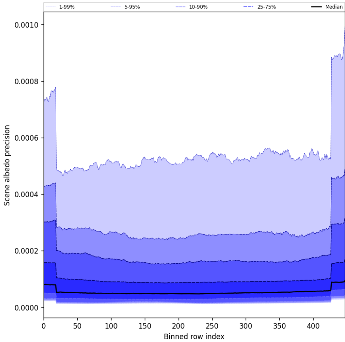
Figure 50: Along track statistics of “Scene albedo precision” for 2025-04-17 to 2025-04-18
