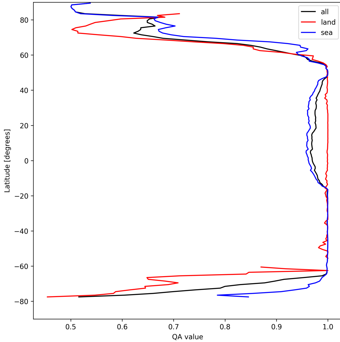
Figure 10: Zonal average of “QA value” for 2025-04-17 to 2025-04-18.
