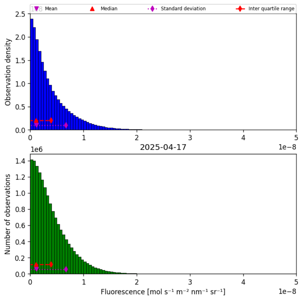
Figure 38: Histogram of “Fluorescence” for 2025-04-17 to 2025-04-18
