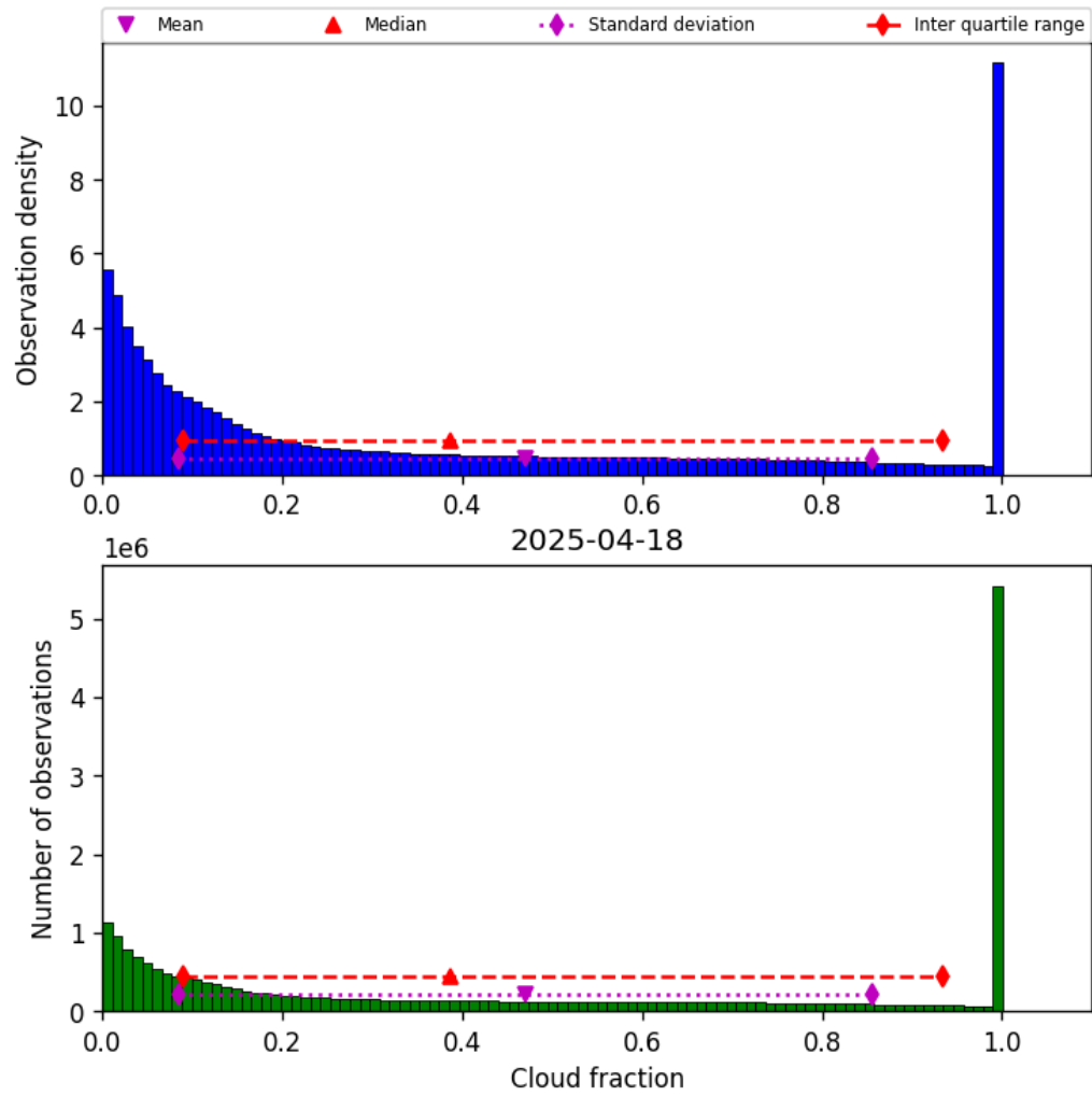
Figure 30: Histogram of “Cloud fraction” for 2025-04-18 to 2025-04-19
