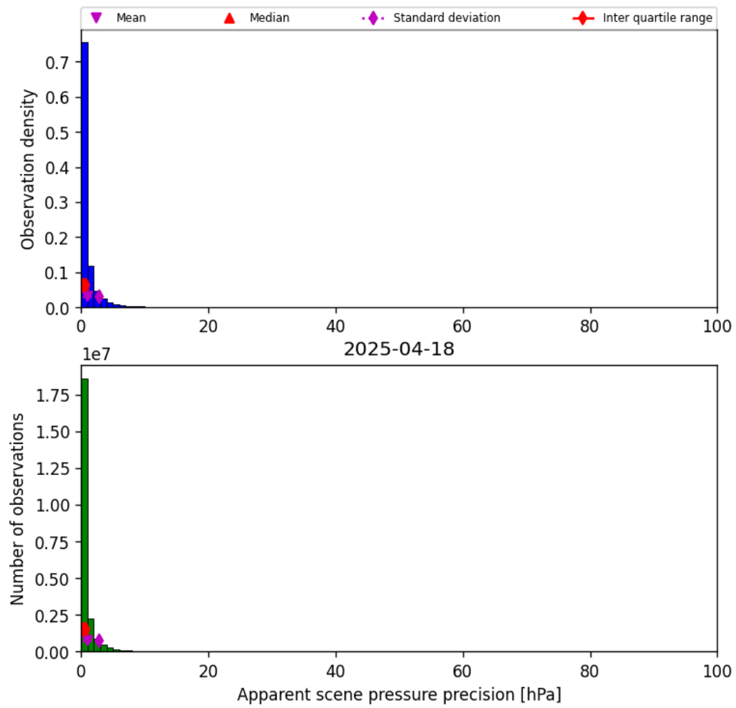
Figure 35: Histogram of “Apparent scene pressure precision” for 2025-04-18 to 2025-04-19
