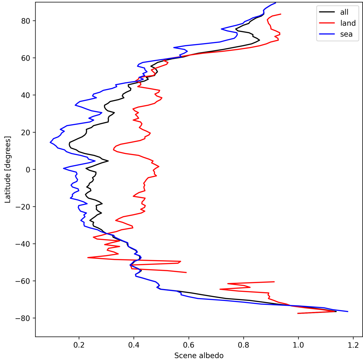
Figure 15: Zonal average of “Scene albedo” for 2025-04-18 to 2025-04-19.
