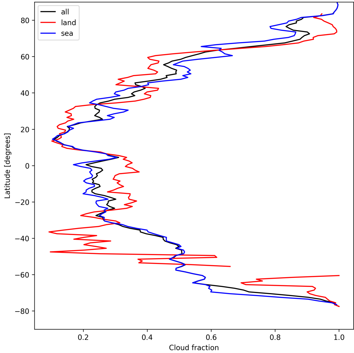
Figure 13: Zonal average of “Cloud fraction” for 2025-04-18 to 2025-04-19.
