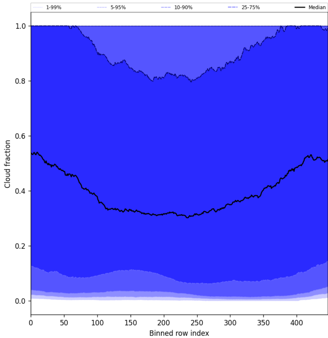
Figure 47: Along track statistics of “Cloud fraction” for 2025-04-18 to 2025-04-19
