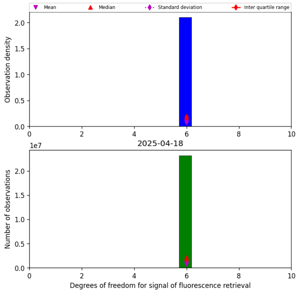
Figure 41: Histogram of “Degrees of freedom for signal of fluorescence retrieval” for 2025-04-18 to 2025-04-19
