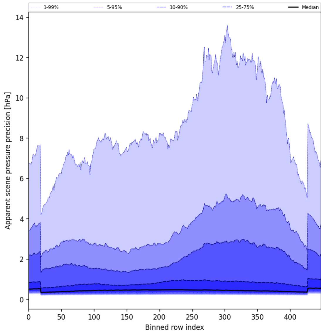
Figure 52: Along track statistics of “Apparent scene pressure precision” for 2025-04-18 to 2025-04-19
