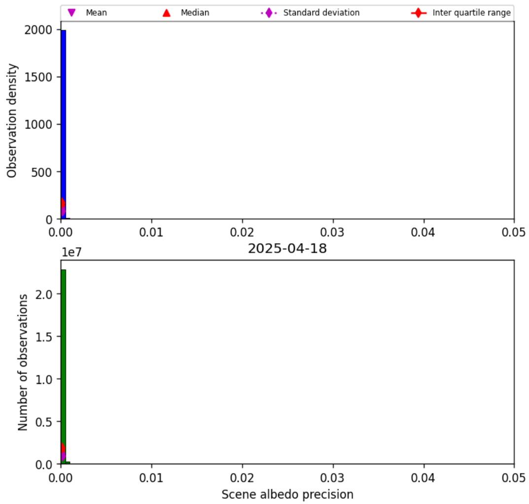
Figure 33: Histogram of “Scene albedo precision” for 2025-04-18 to 2025-04-19
