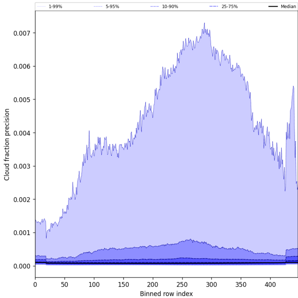
Figure 48: Along track statistics of “Cloud fraction precision” for 2025-04-18 to 2025-04-19
