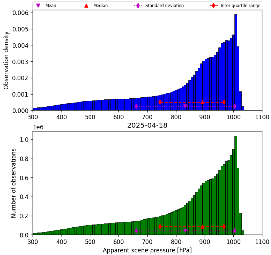
Figure 34: Histogram of “Apparent scene pressure” for 2025-04-18 to 2025-04-19
