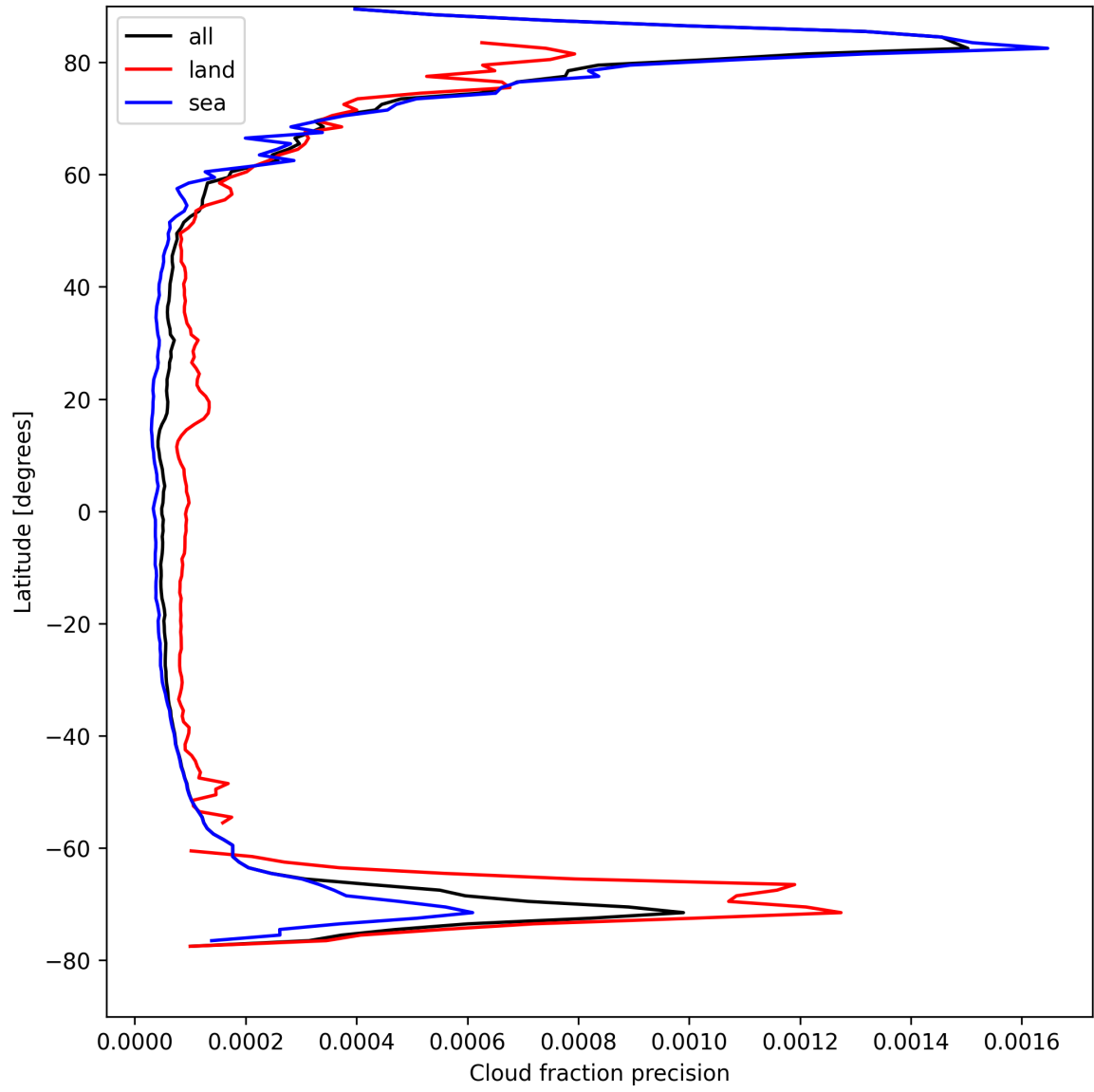
Figure 14: Zonal average of “Cloud fraction precision” for 2025-04-18 to 2025-04-19.
