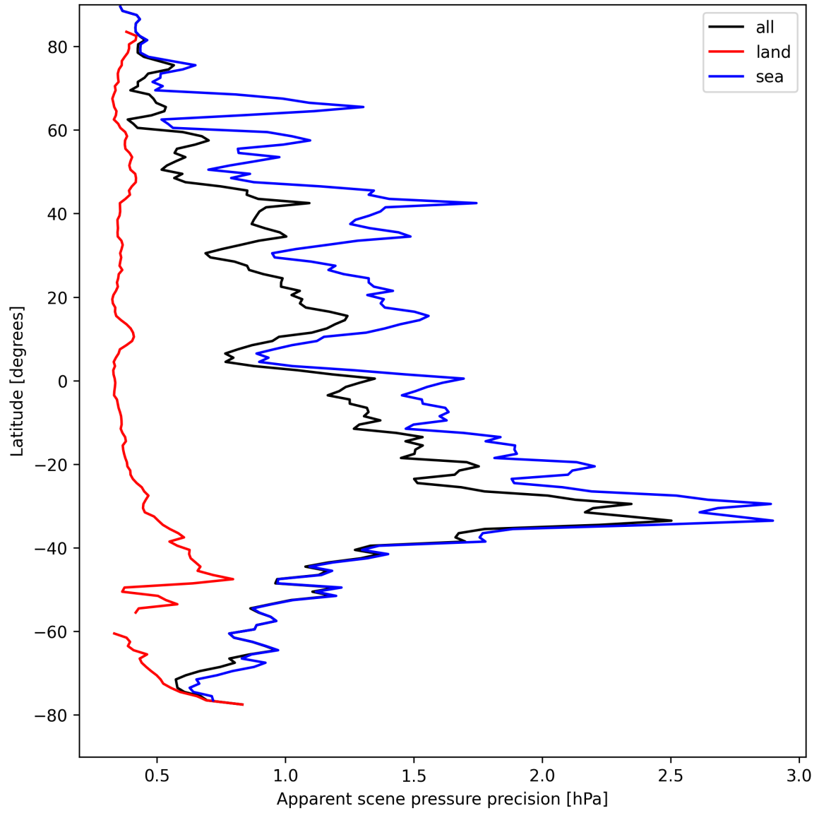
Figure 18: Zonal average of “Apparent scene pressure precision” for 2025-04-18 to 2025-04-19.
