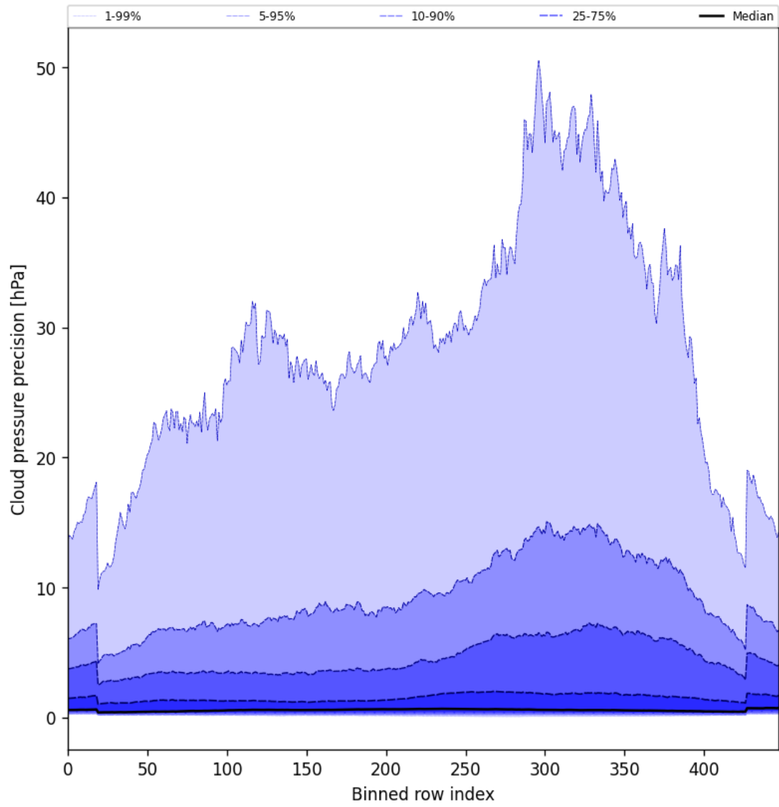
Figure 46: Along track statistics of “Cloud pressure precision” for 2025-04-18 to 2025-04-19
