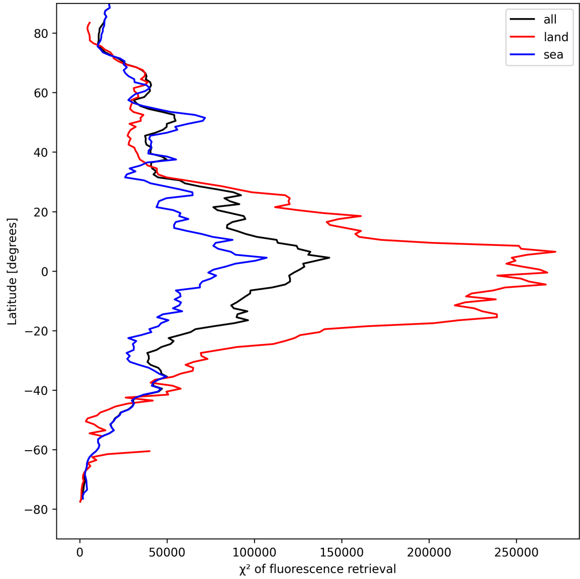
Figure 23: Zonal average of “ \chi^2 of fluorescence retrieval” for 2025-04-18 to 2025-04-19.
