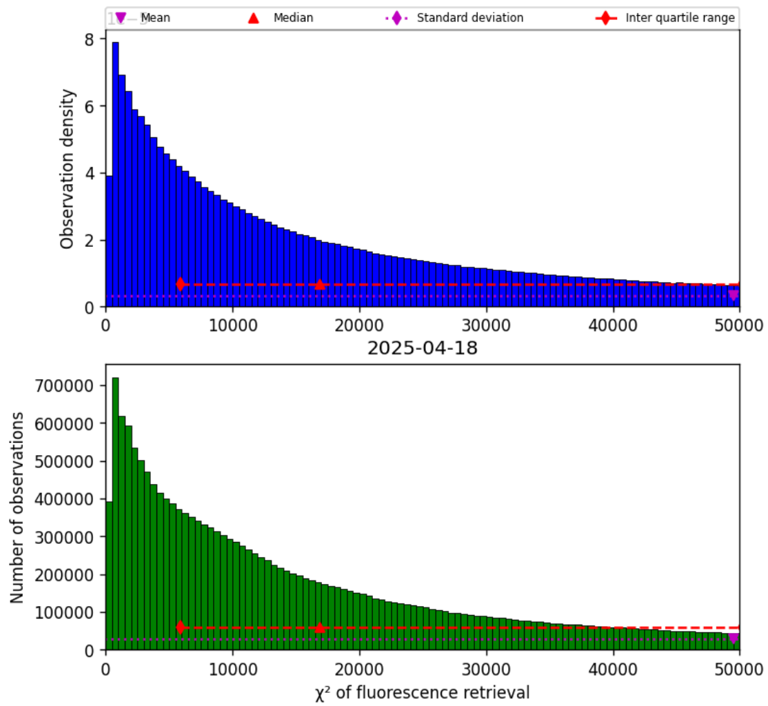
Figure 40: Histogram of “ \chi^2 of fluorescence retrieval” for 2025-04-18 to 2025-04-19
