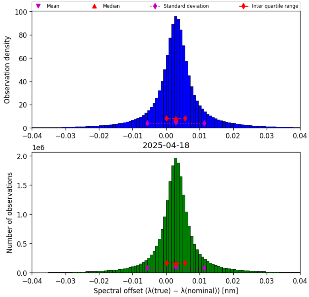
Figure 43: Histogram of “Spectral offset ( \lambda_{\text{true}} - \lambda_{\text{nominal}} )” for 2025-04-18 to 2025-04-19
