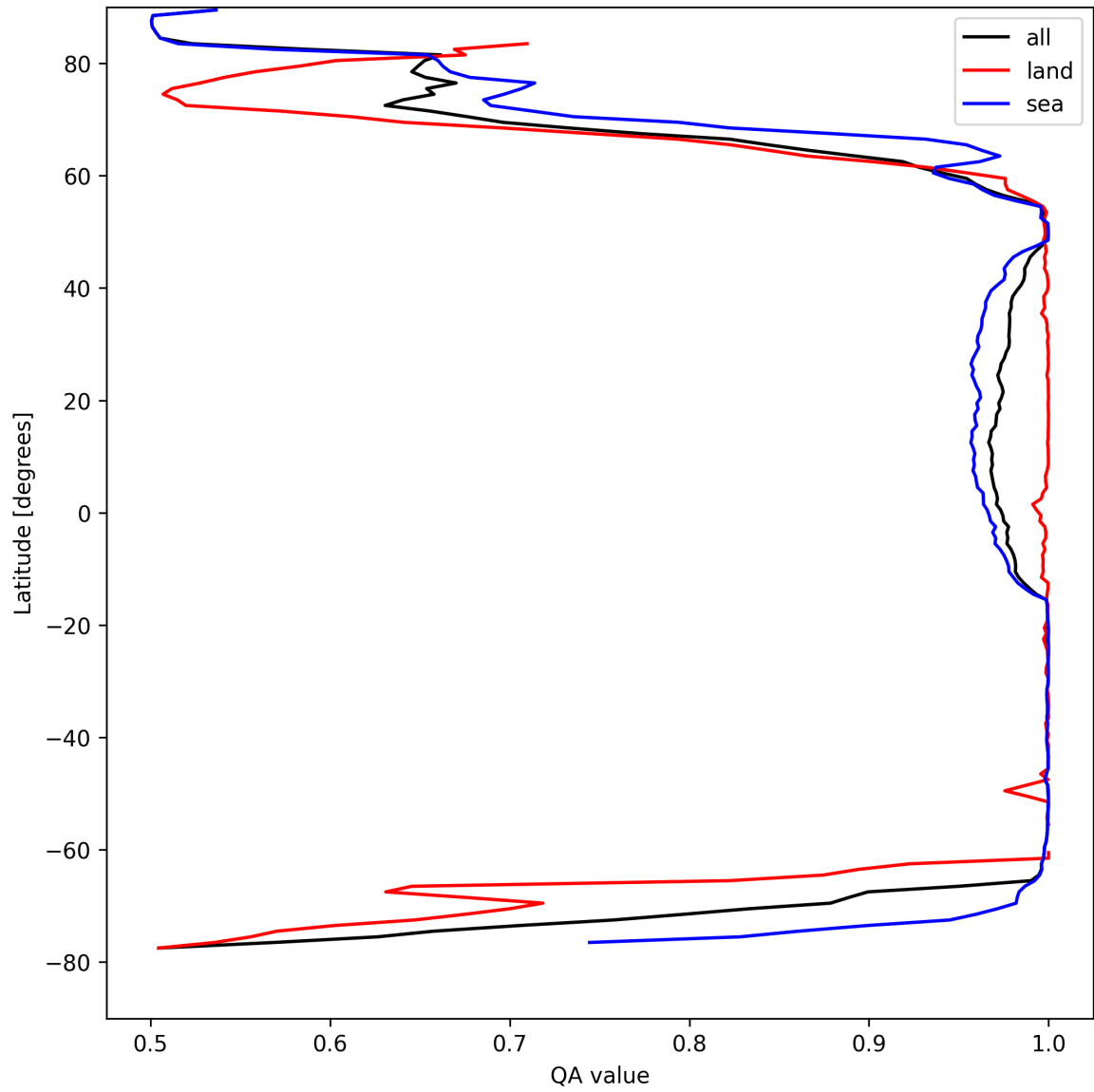
Figure 10: Zonal average of “QA value” for 2025-04-18 to 2025-04-19.
