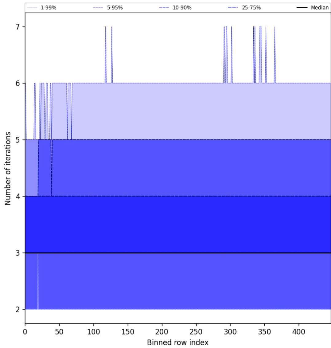
Figure 54: Along track statistics of “Number of iterations” for 2025-04-18 to 2025-04-19
