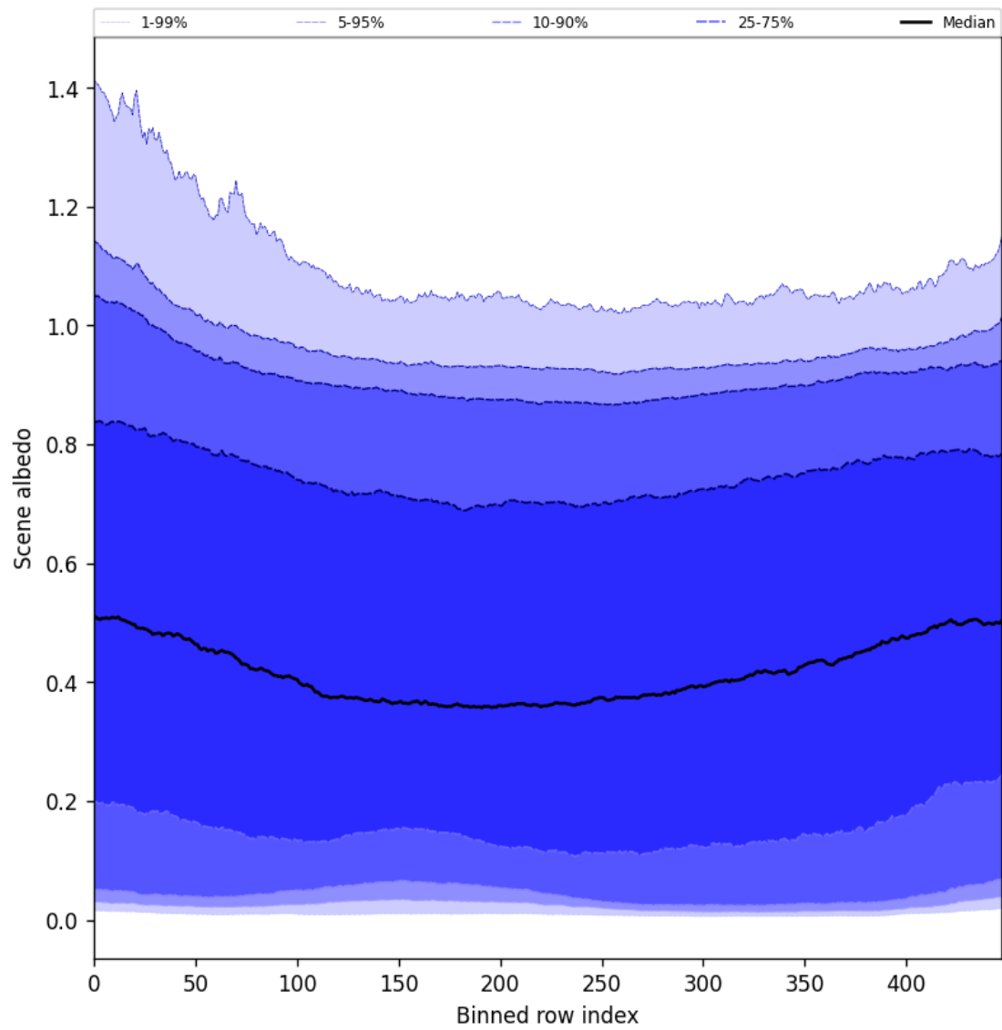
Figure 49: Along track statistics of “Scene albedo” for 2025-04-18 to 2025-04-19
