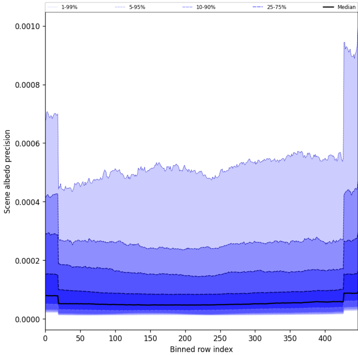
Figure 50: Along track statistics of “Scene albedo precision” for 2025-04-18 to 2025-04-19
