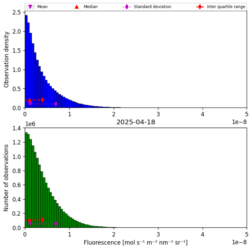
Figure 38: Histogram of “Fluorescence” for 2025-04-18 to 2025-04-19
