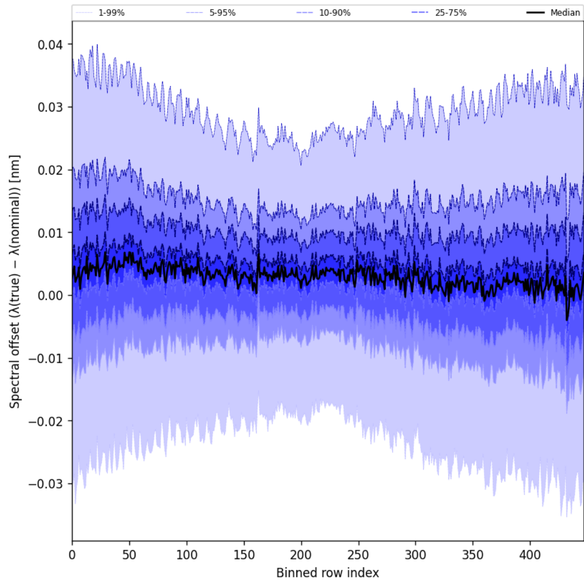
Figure 60: Along track statistics of “Spectral offset ( \lambda_{\text{true}} - \lambda_{\text{nominal}} )” for 2025-04-18 to 2025-04-19
