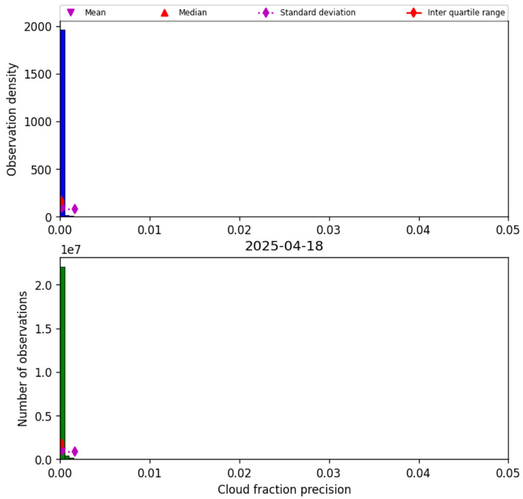
Figure 31: Histogram of “Cloud fraction precision” for 2025-04-18 to 2025-04-19
