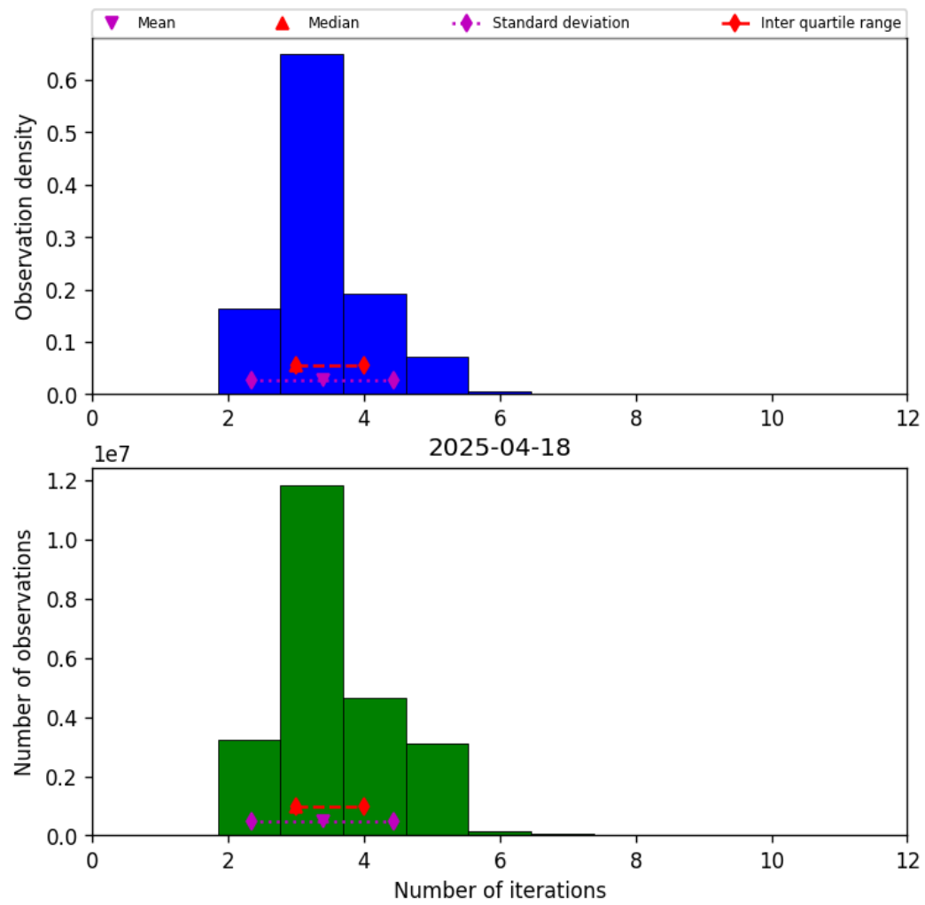
Figure 37: Histogram of “Number of iterations” for 2025-04-18 to 2025-04-19
