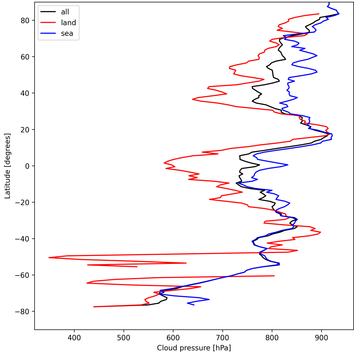
Figure 11: Zonal average of “Cloud pressure” for 2025-04-18 to 2025-04-19.
