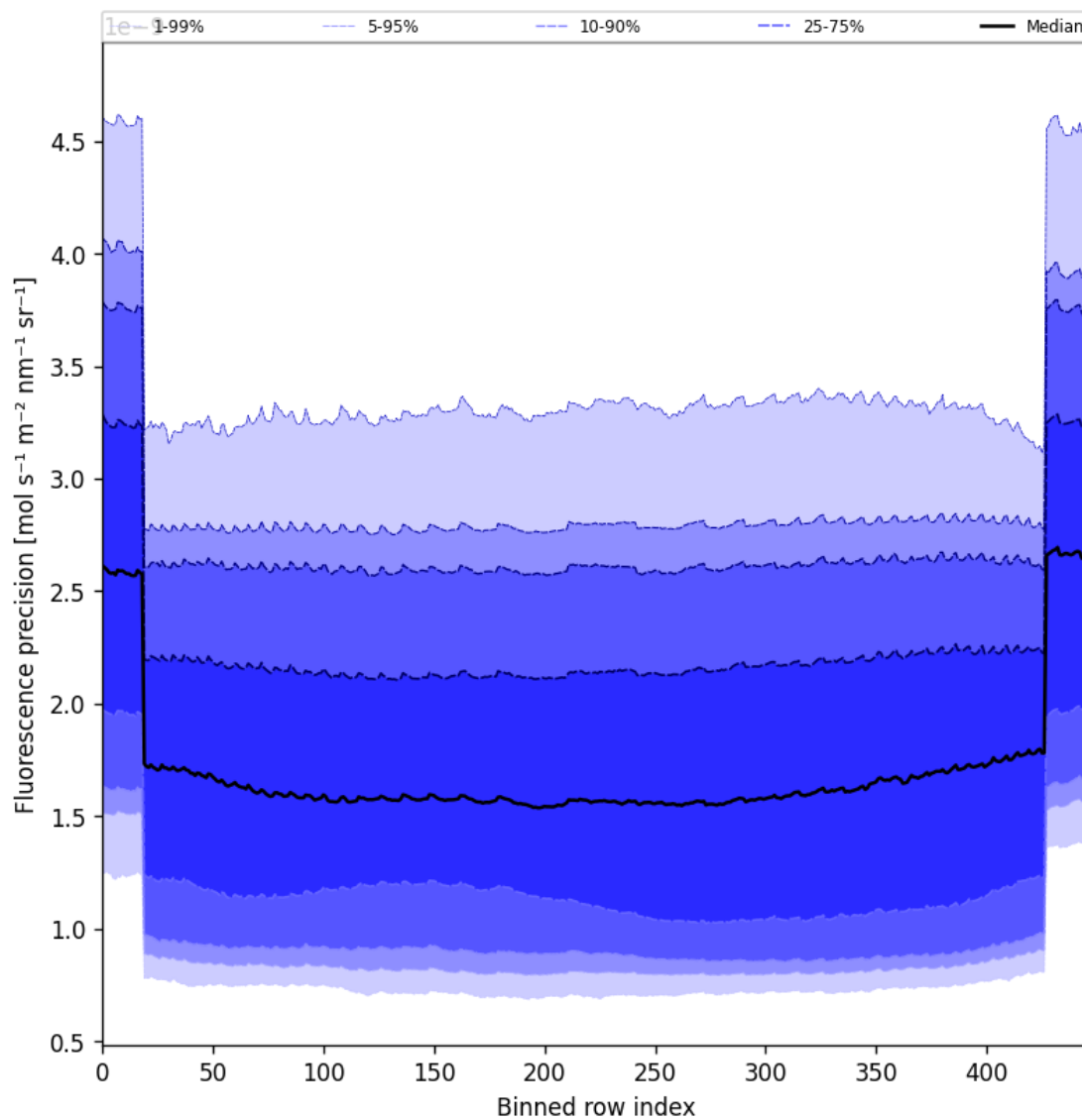
Figure 56: Along track statistics of “Fluorescence precision” for 2025-04-18 to 2025-04-19
