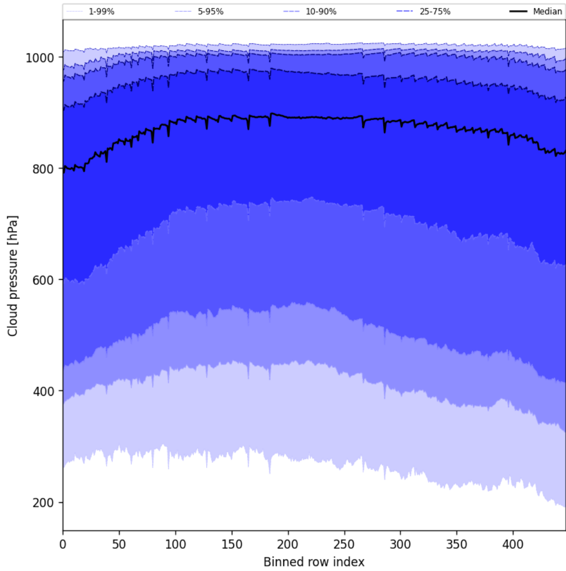
Figure 45: Along track statistics of “Cloud pressure” for 2025-04-18 to 2025-04-19
