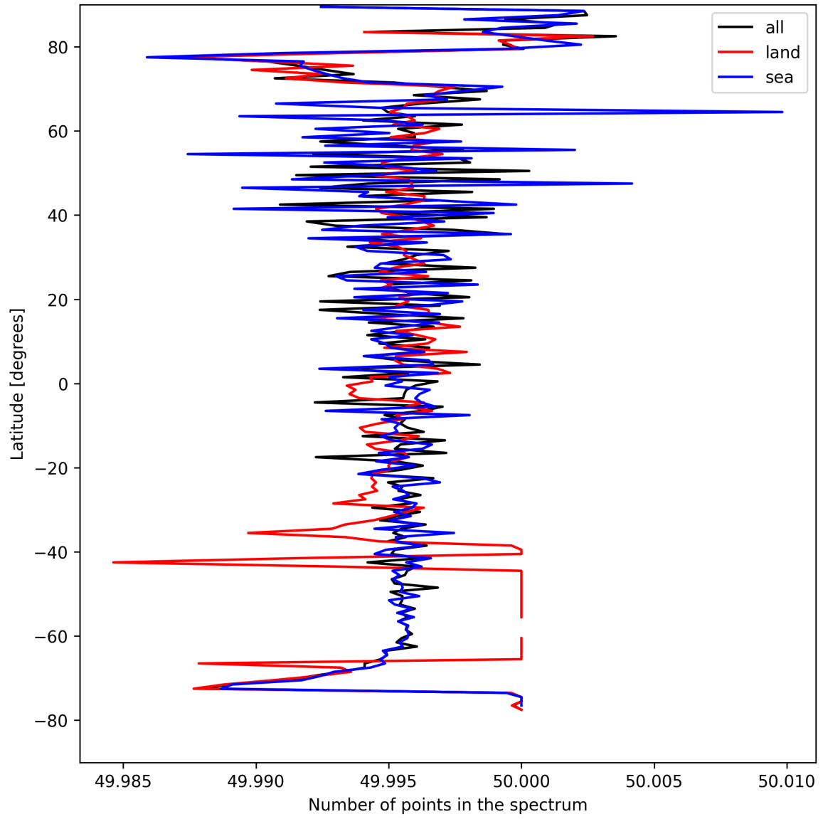
Figure 25: Zonal average of “Number of points in the spectrum” for 2025-04-18 to 2025-04-19.
