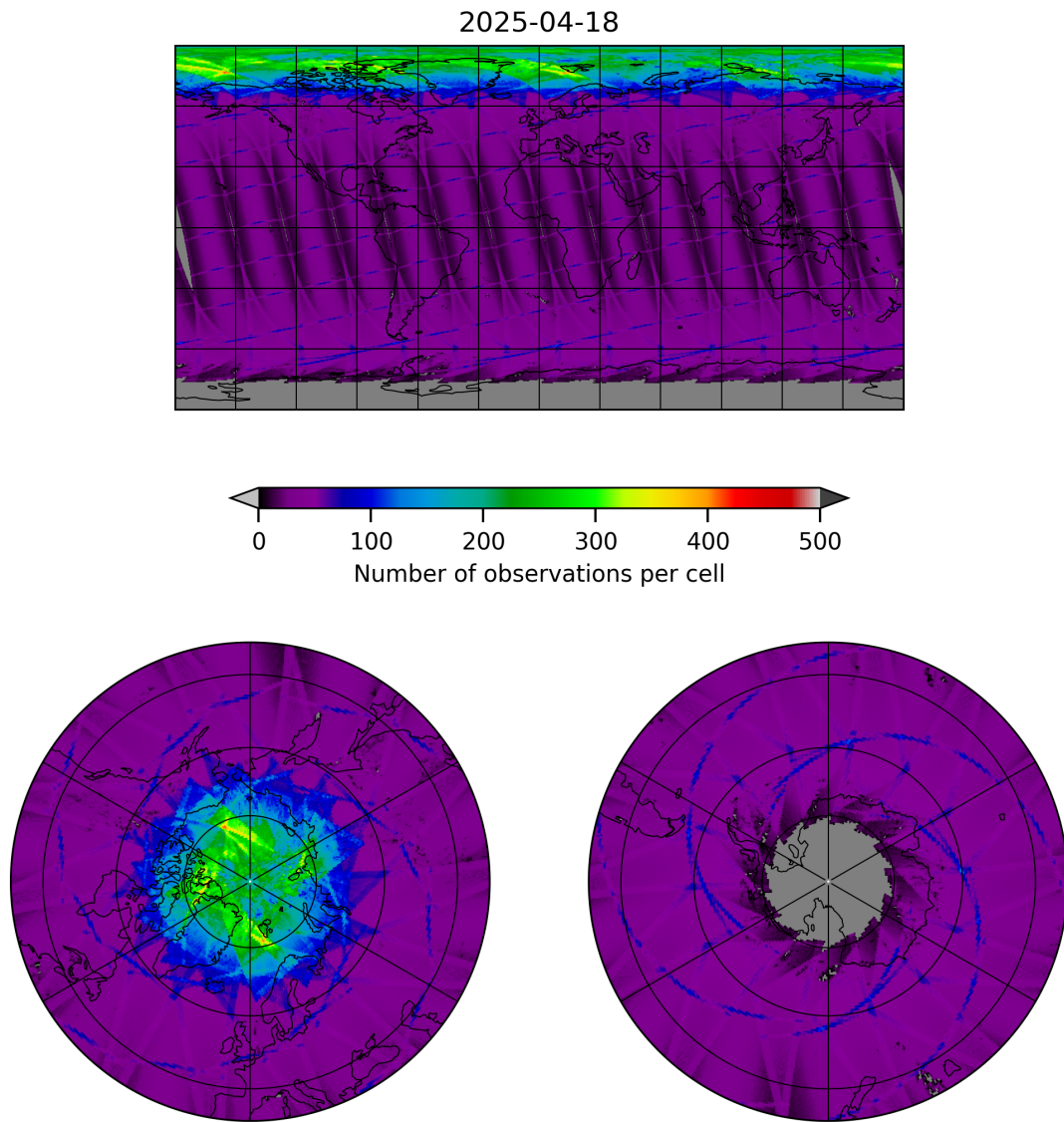
Figure 9: Map of the number of observations for 2025-04-18 to 2025-04-19
