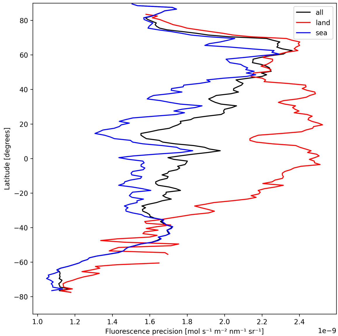
Figure 22: Zonal average of “Fluorescence precision” for 2025-04-18 to 2025-04-19.
