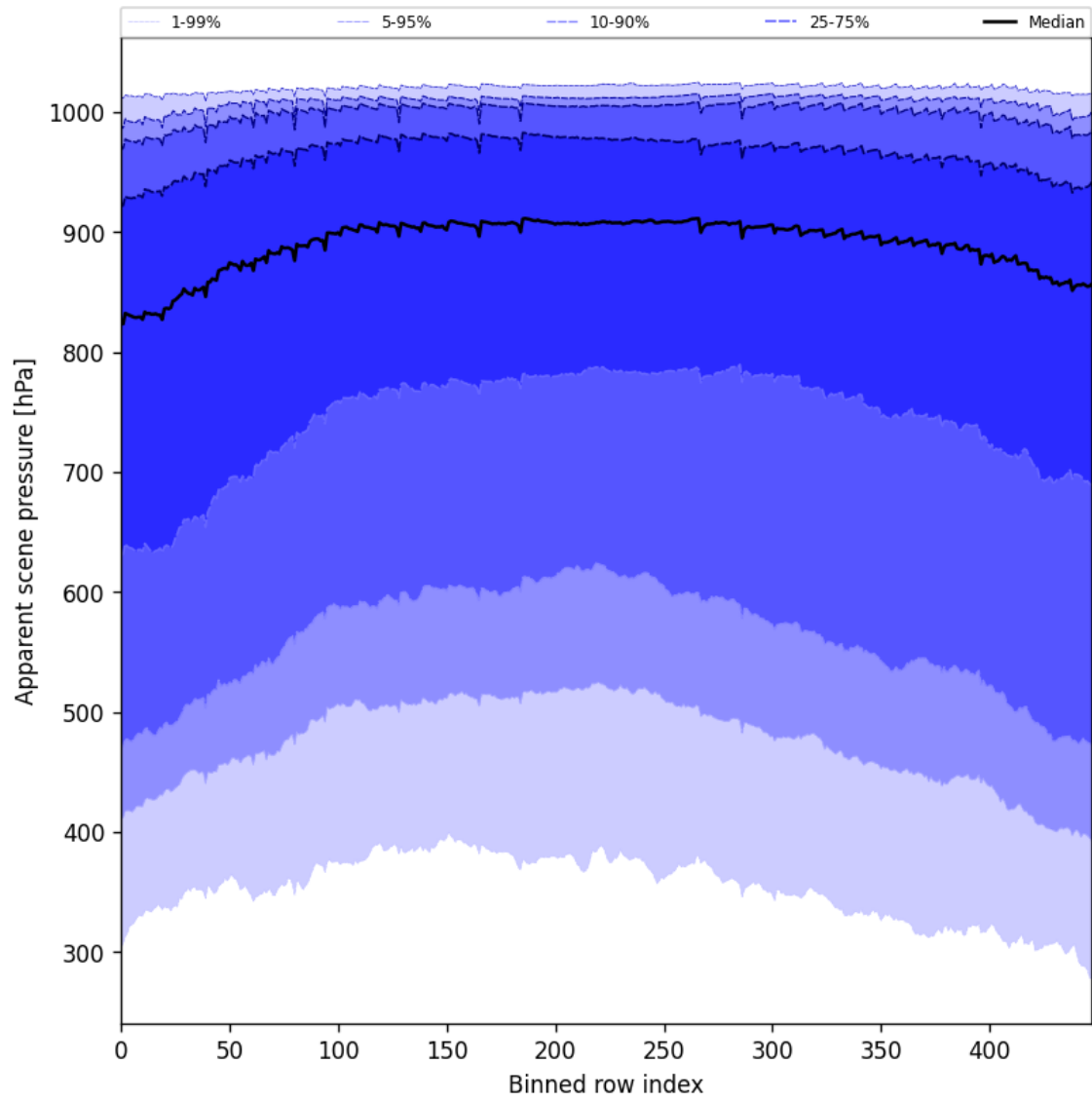
Figure 51: Along track statistics of “Apparent scene pressure” for 2025-04-18 to 2025-04-19
