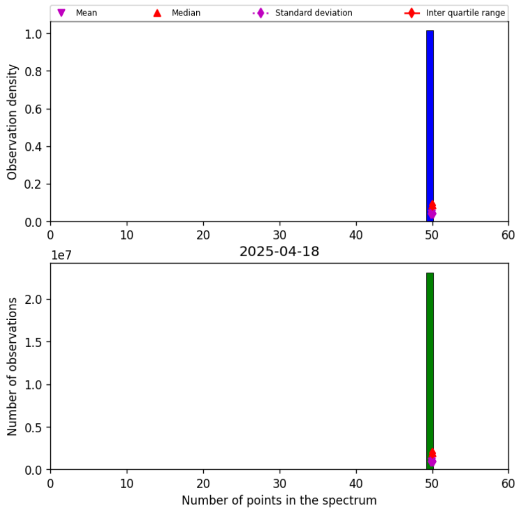
Figure 42: Histogram of “Number of points in the spectrum” for 2025-04-18 to 2025-04-19
