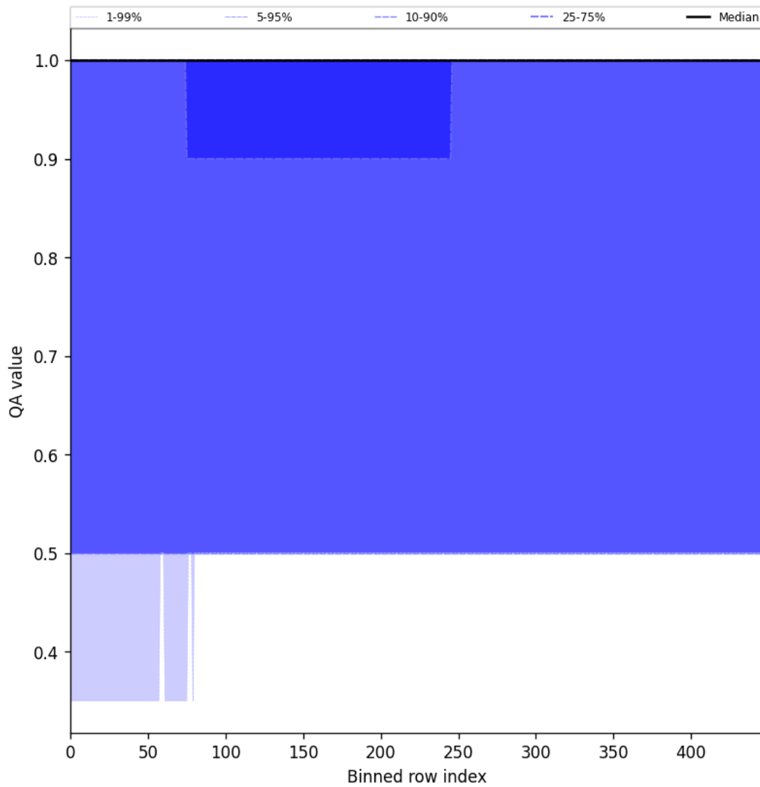
Figure 44: Along track statistics of “QA value” for 2025-04-18 to 2025-04-19
