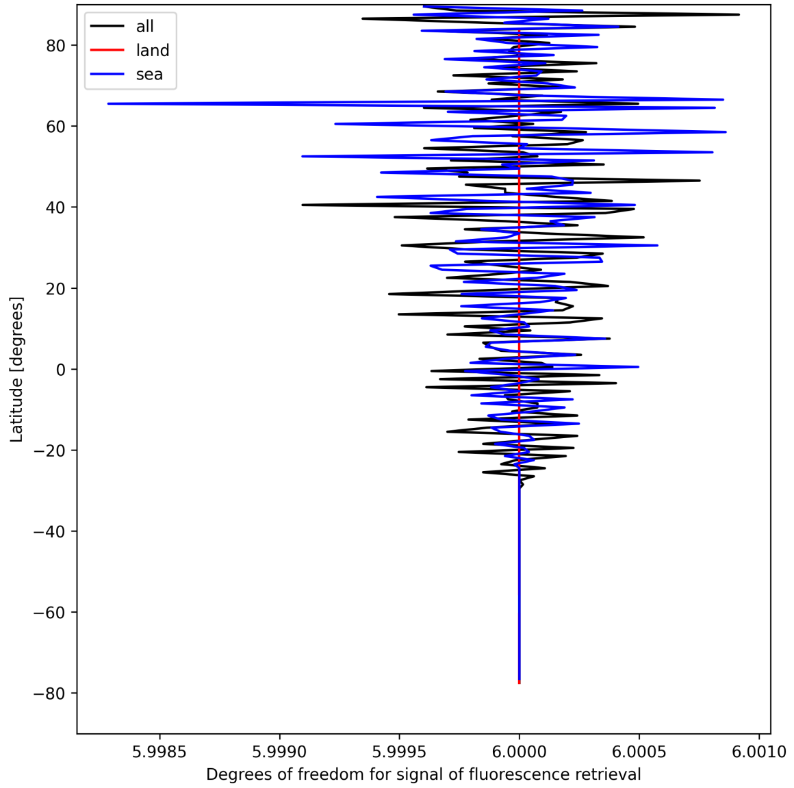
Figure 24: Zonal average of “Degrees of freedom for signal of fluorescence retrieval” for 2025-04-18 to 2025-04-19.
