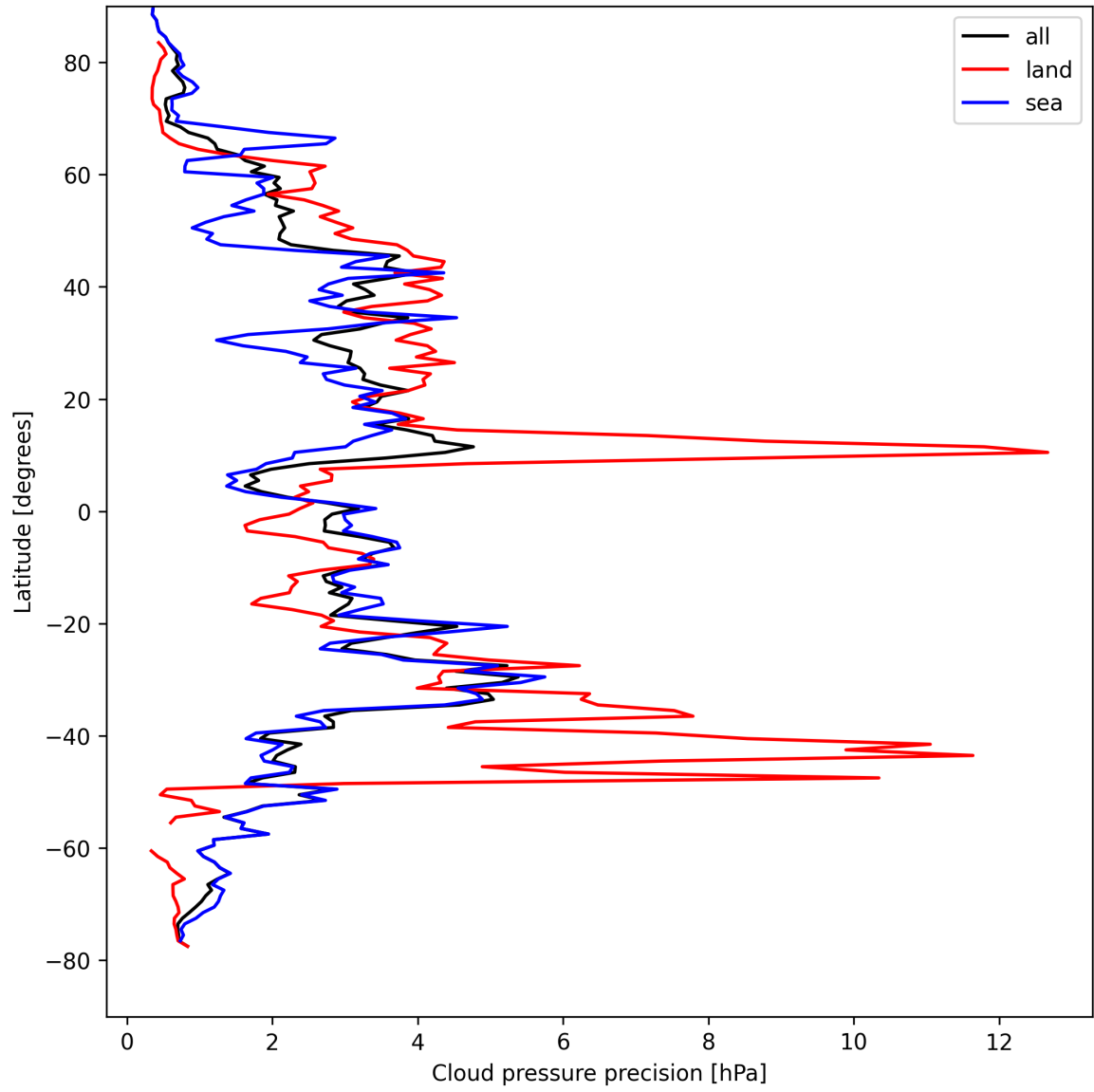
Figure 12: Zonal average of “Cloud pressure precision” for 2025-04-18 to 2025-04-19.
