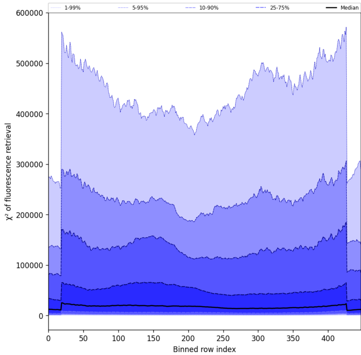
Figure 57: Along track statistics of “ \chi^2 of fluorescence retrieval” for 2025-04-18 to 2025-04-19
