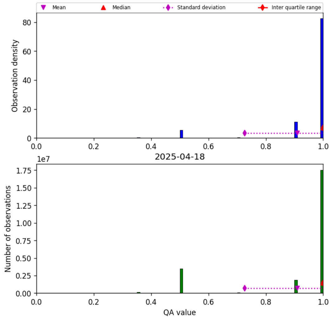
Figure 27: Histogram of “QA value” for 2025-04-18 to 2025-04-19
