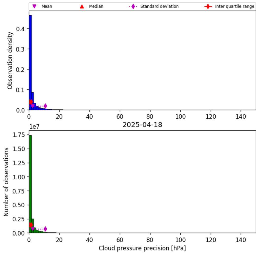
Figure 29: Histogram of “Cloud pressure precision” for 2025-04-18 to 2025-04-19
