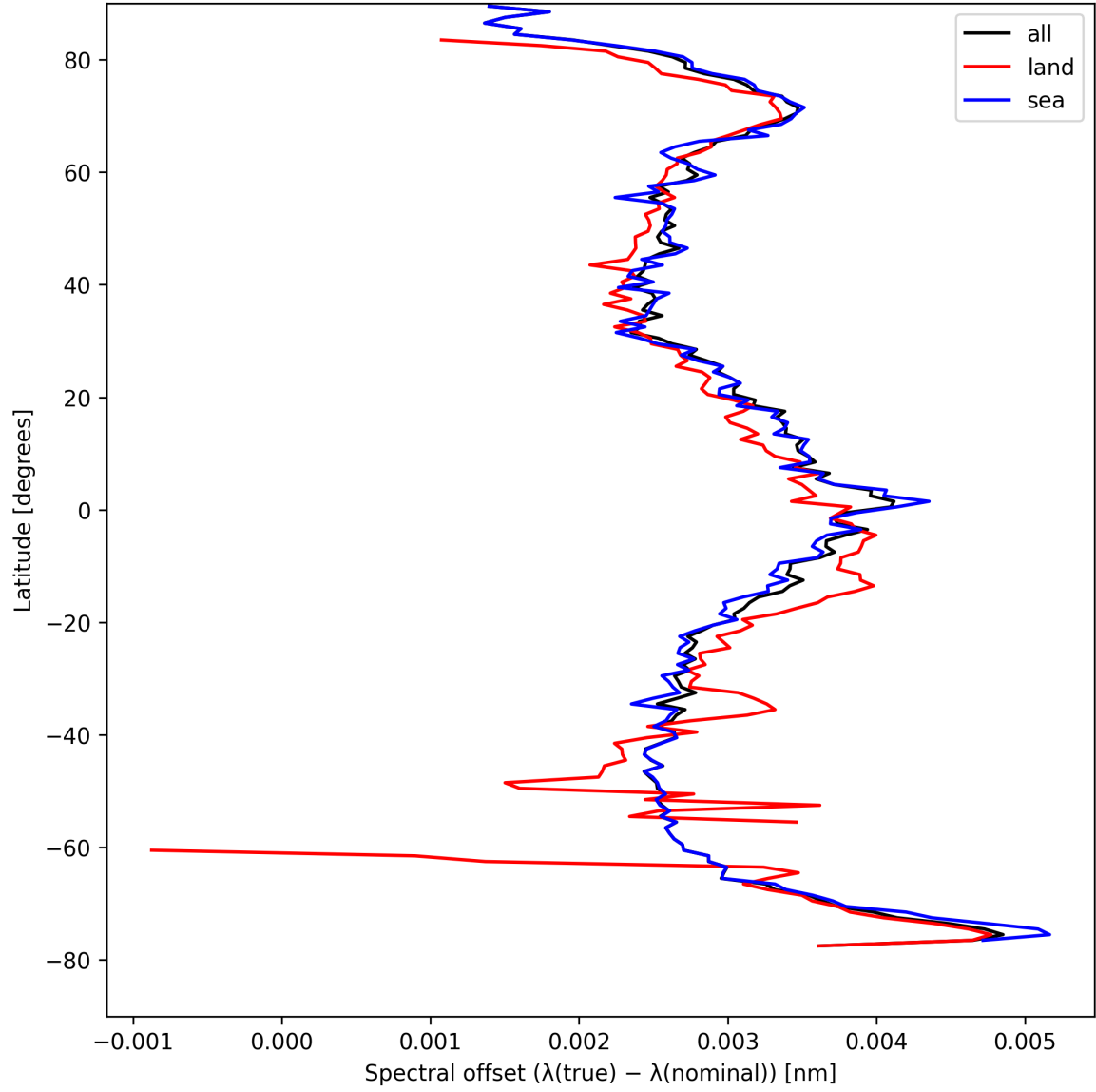
Figure 26: Zonal average of “Spectral offset ( \lambda_{\text{true}} - \lambda_{\text{nominal}} )” for 2025-04-18 to 2025-04-19.
