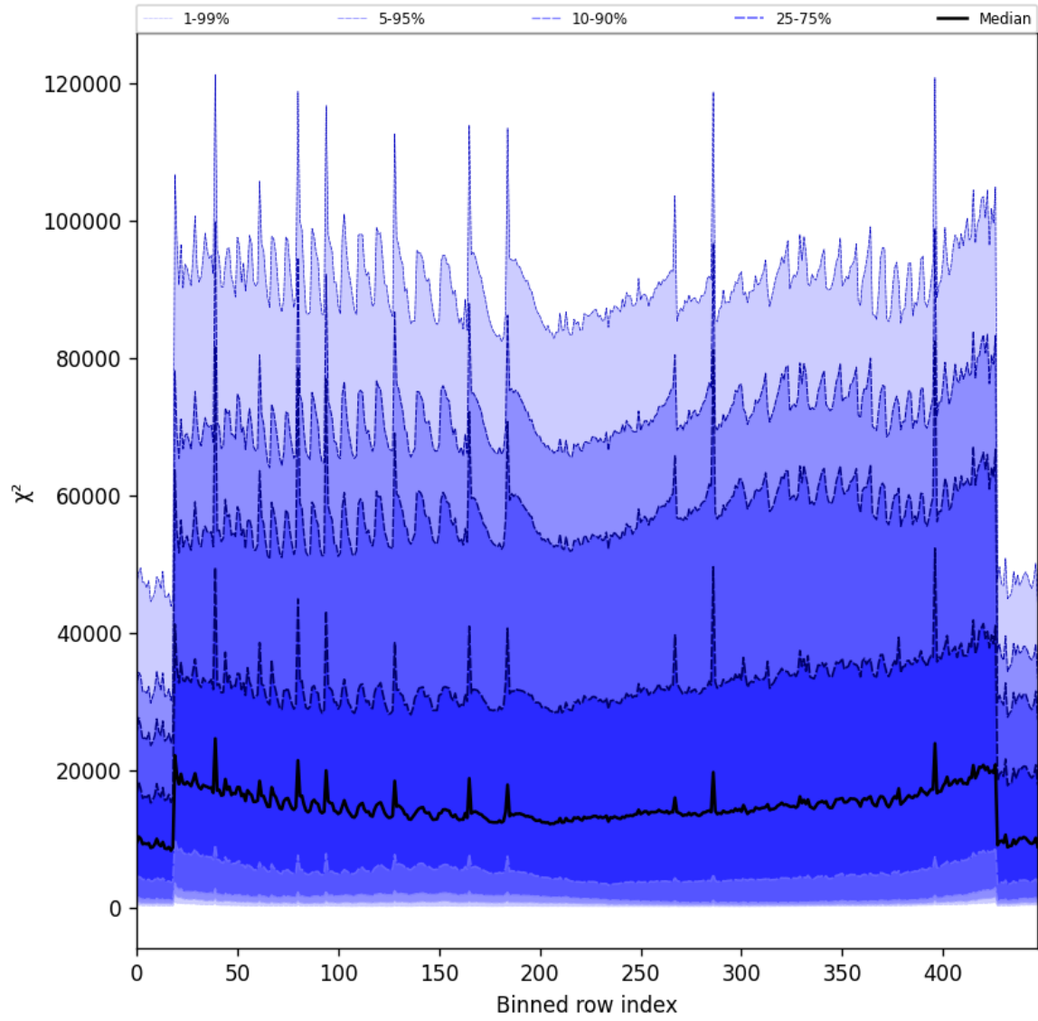
Figure 53: Along track statistics of “ \chi^2 ” for 2025-04-18 to 2025-04-19
