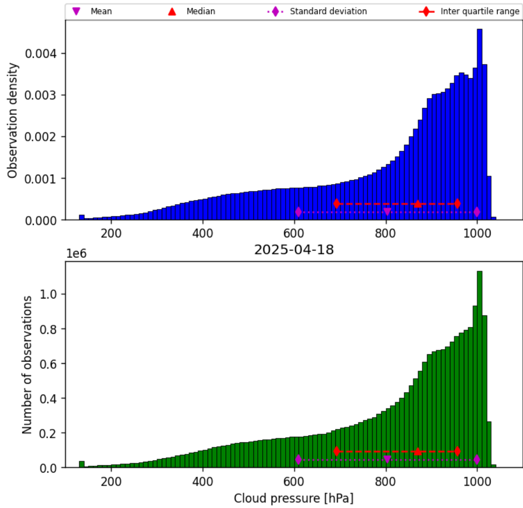
Figure 28: Histogram of “Cloud pressure” for 2025-04-18 to 2025-04-19
