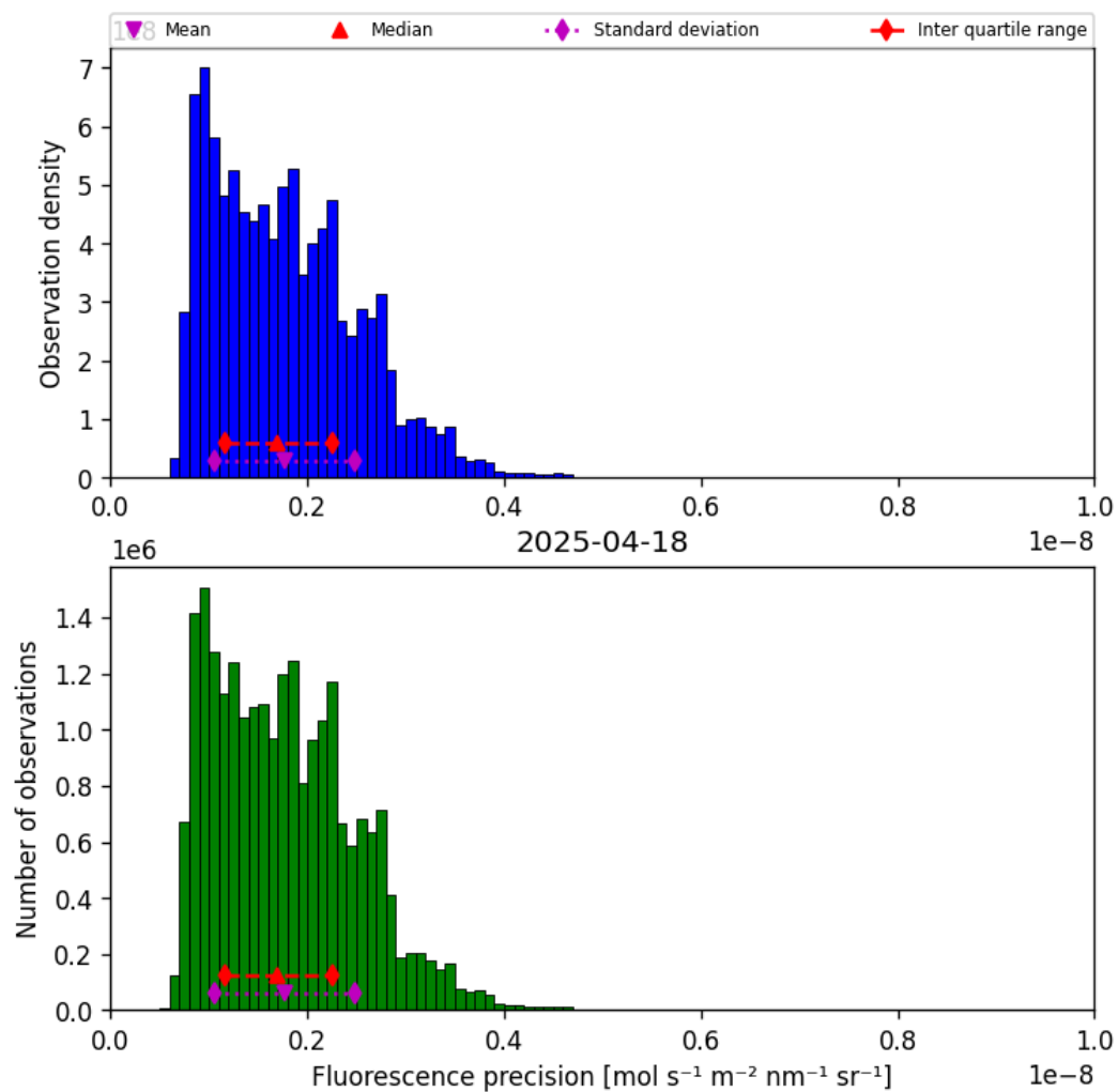
Figure 39: Histogram of “Fluorescence precision” for 2025-04-18 to 2025-04-19
