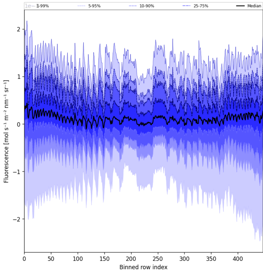
Figure 55: Along track statistics of “Fluorescence” for 2025-04-18 to 2025-04-19
