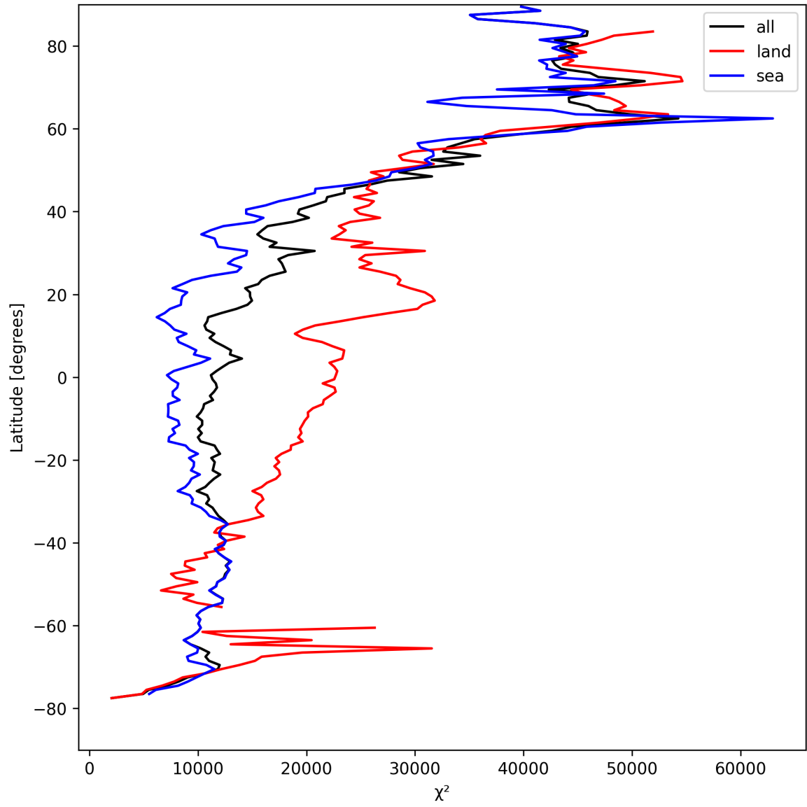
Figure 19: Zonal average of “ \chi^2 ” for 2025-04-18 to 2025-04-19.
