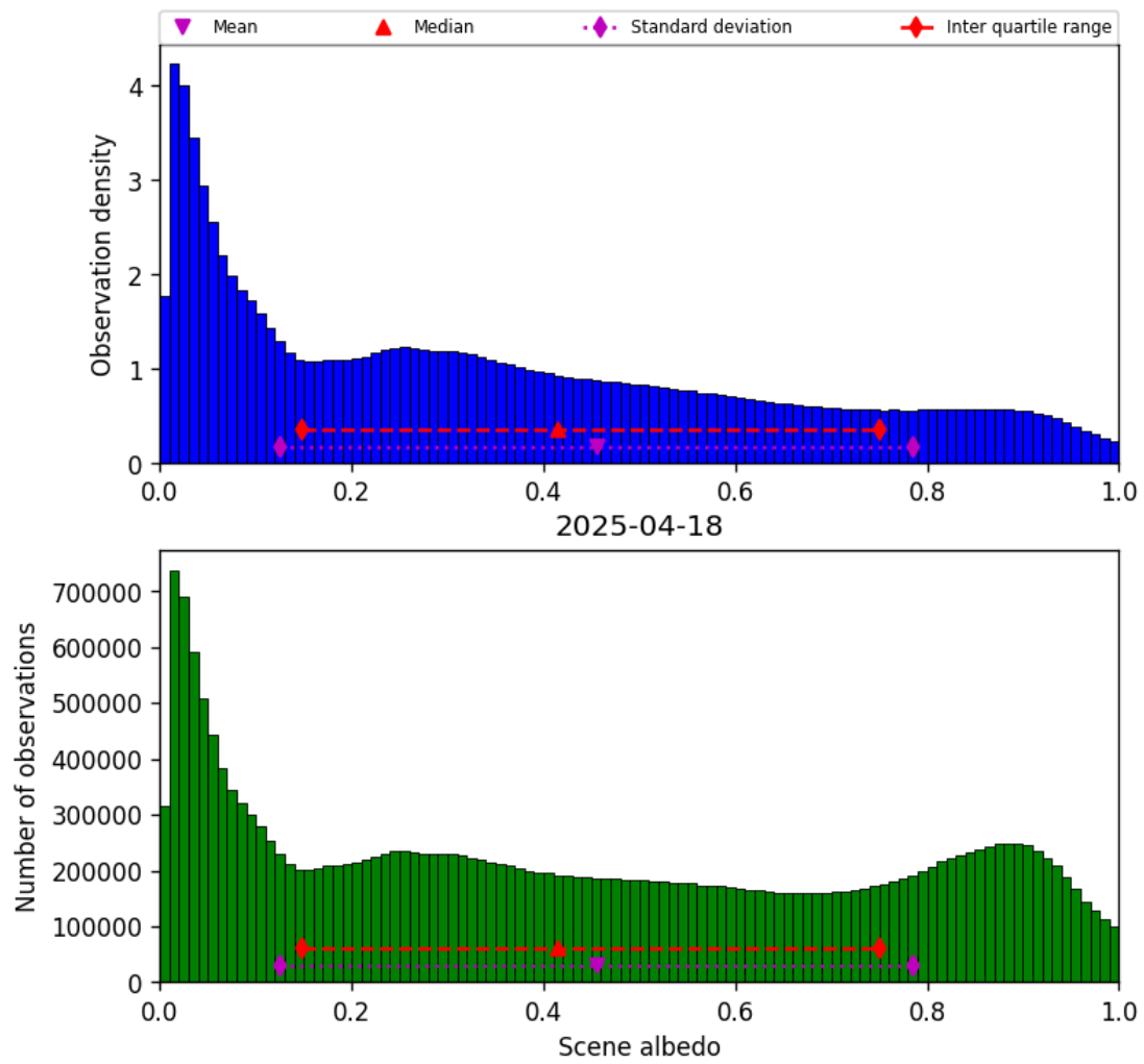
Figure 32: Histogram of “Scene albedo” for 2025-04-18 to 2025-04-19
