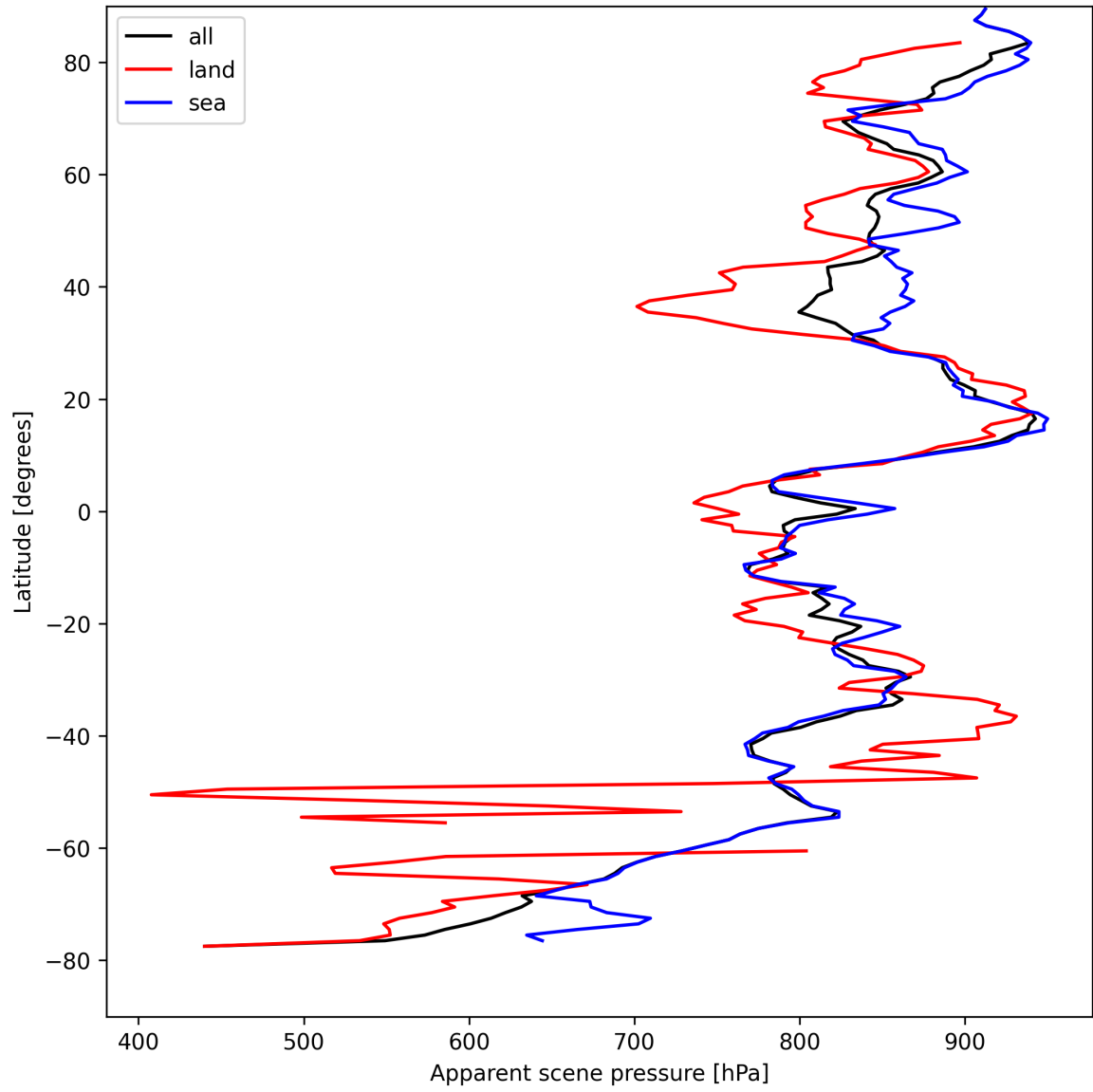
Figure 17: Zonal average of “Apparent scene pressure” for 2025-04-18 to 2025-04-19.
