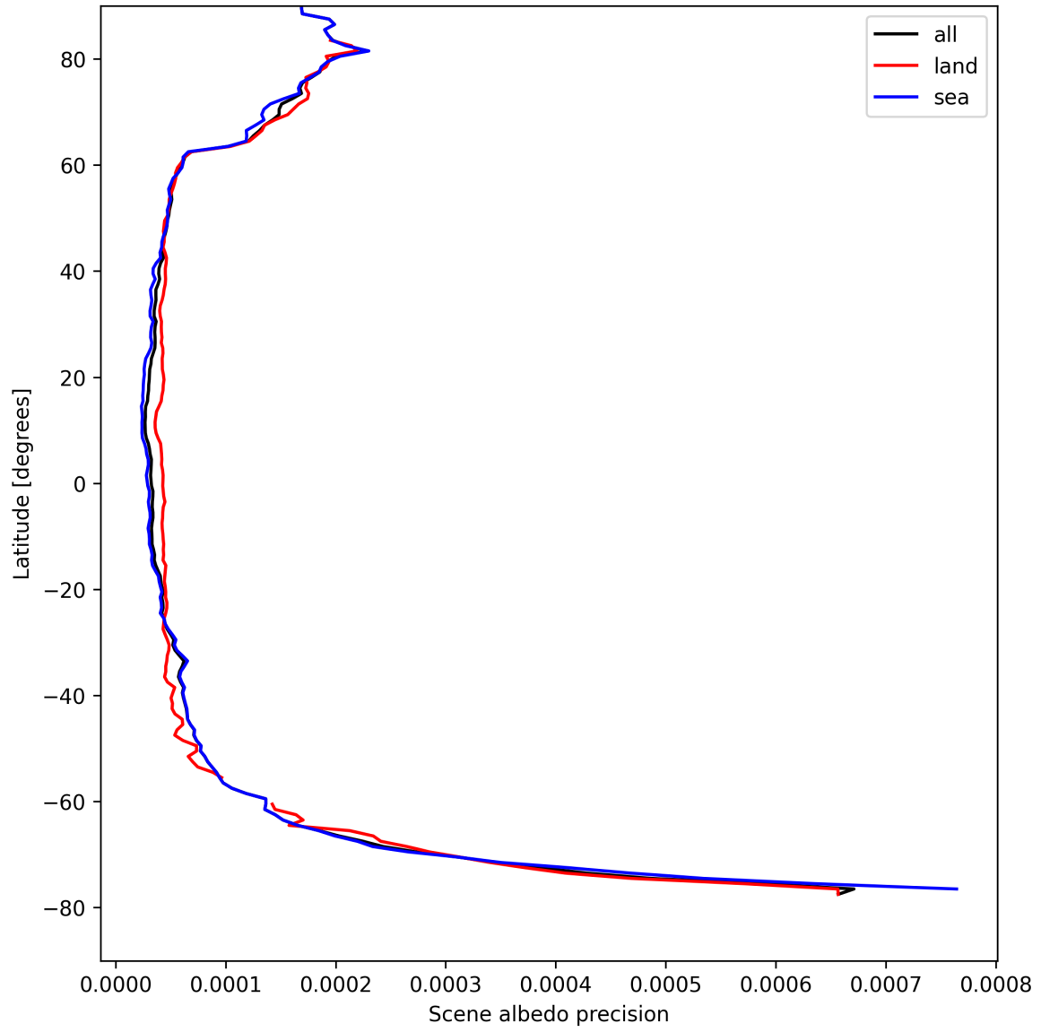
Figure 16: Zonal average of “Scene albedo precision” for 2025-04-18 to 2025-04-19.
