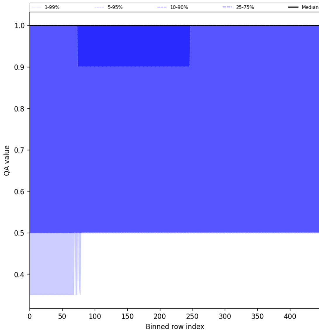
Figure 44: Along track statistics of “QA value” for 2025-04-19 to 2025-04-20
