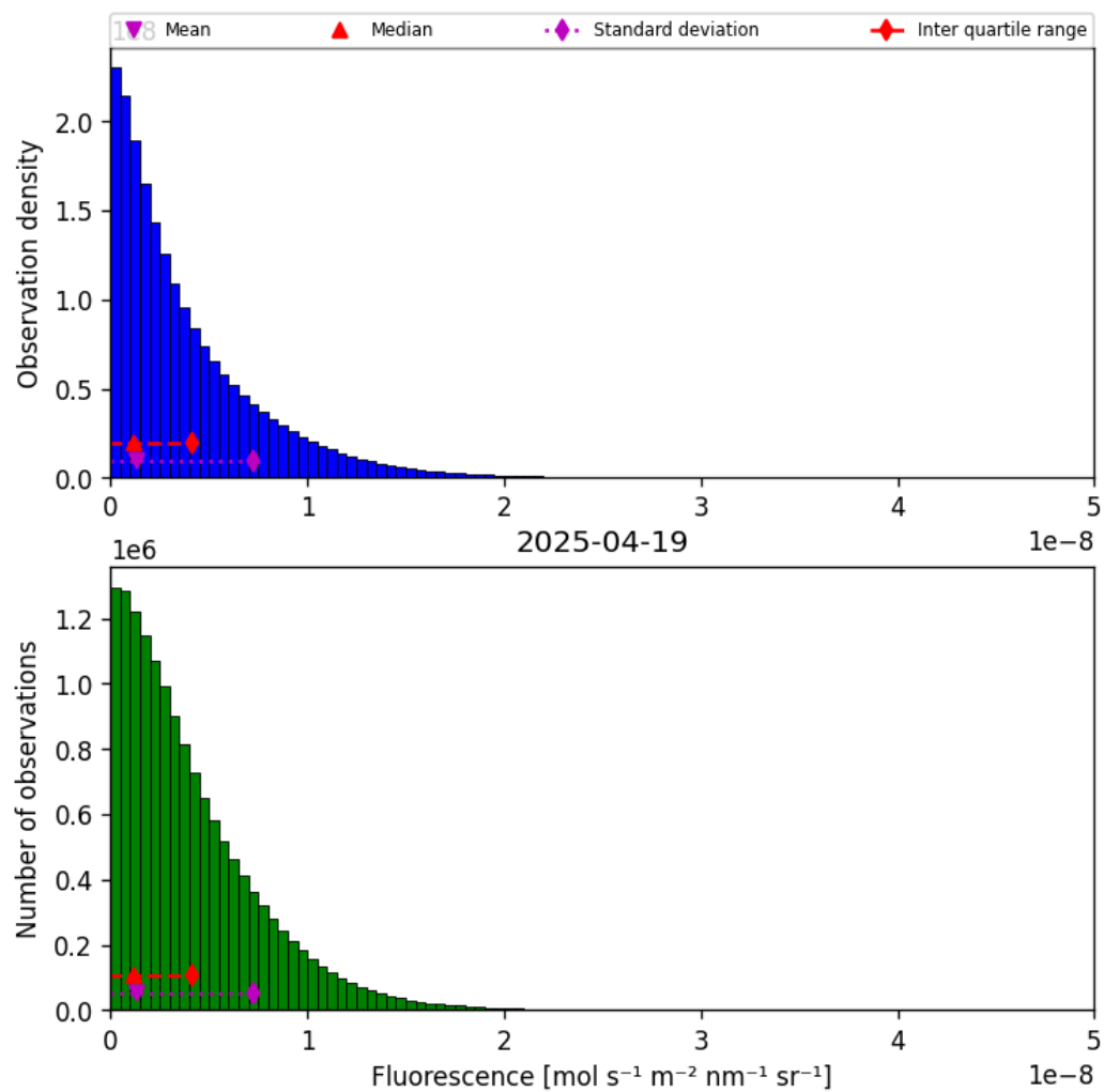
Figure 38: Histogram of “Fluorescence” for 2025-04-19 to 2025-04-20
