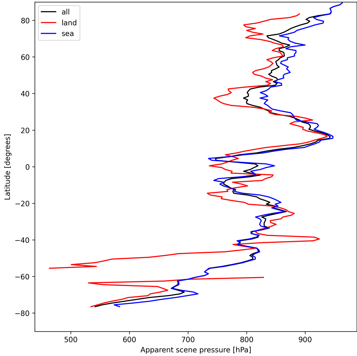
Figure 17: Zonal average of “Apparent scene pressure” for 2025-04-19 to 2025-04-20.
