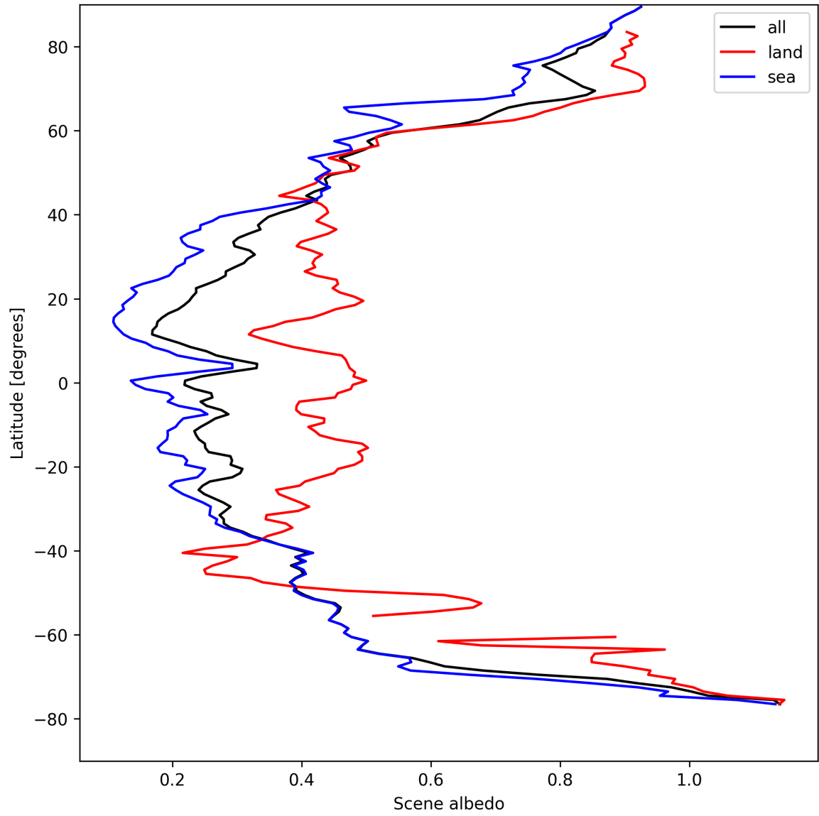
Figure 15: Zonal average of “Scene albedo” for 2025-04-19 to 2025-04-20.
