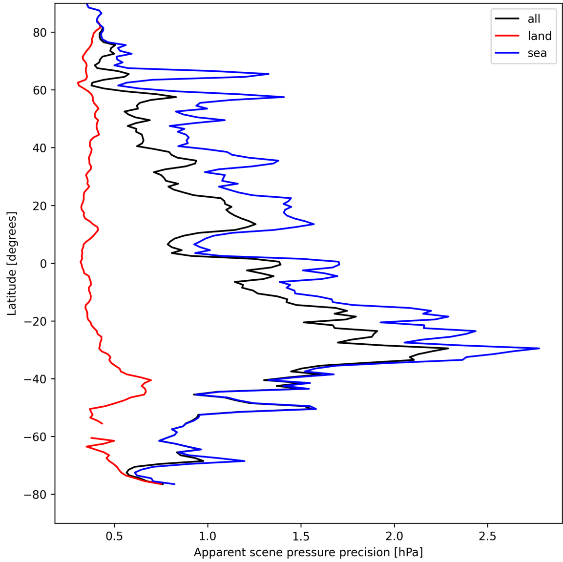
Figure 18: Zonal average of “Apparent scene pressure precision” for 2025-04-19 to 2025-04-20.
