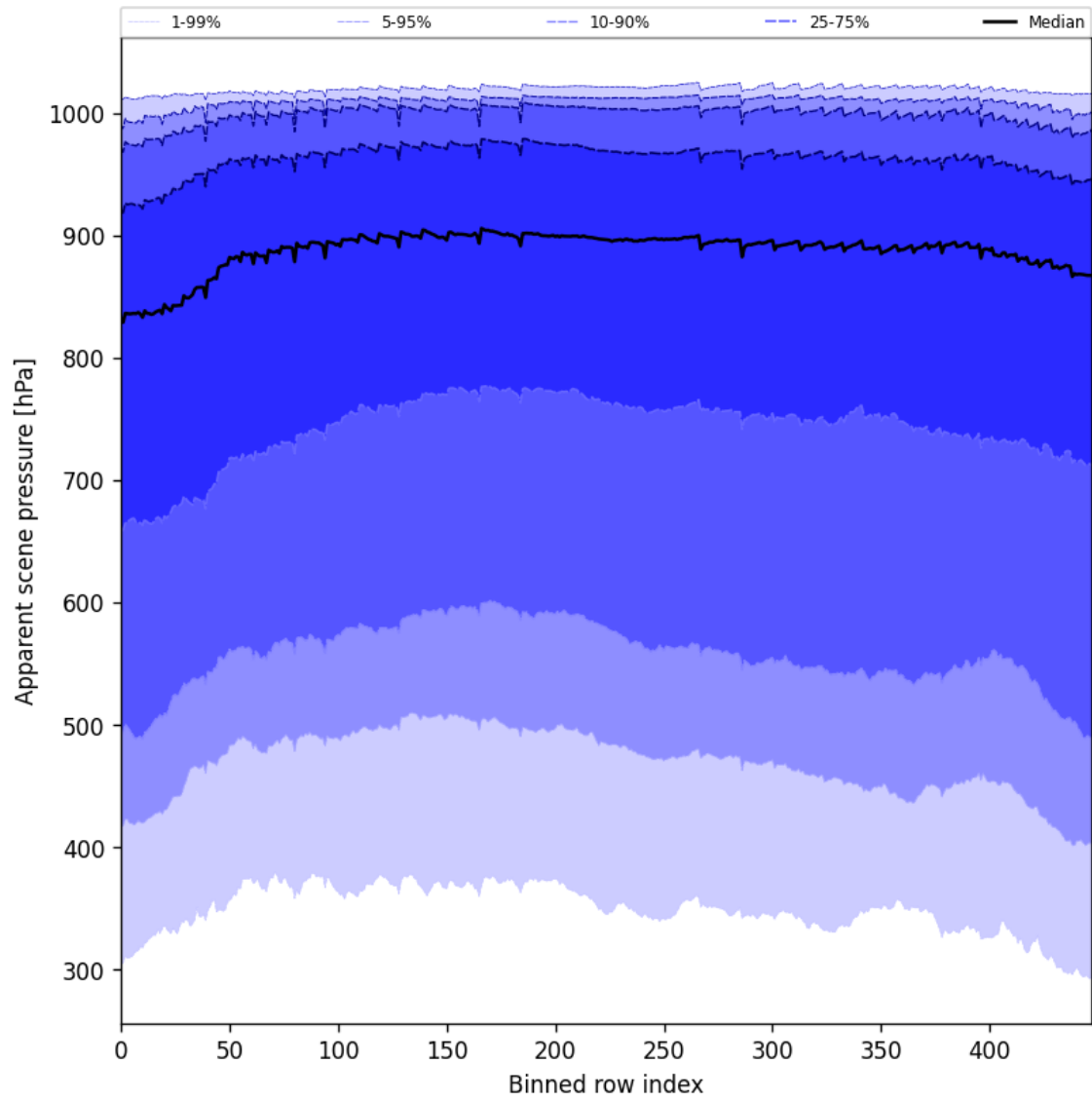
Figure 51: Along track statistics of “Apparent scene pressure” for 2025-04-19 to 2025-04-20
