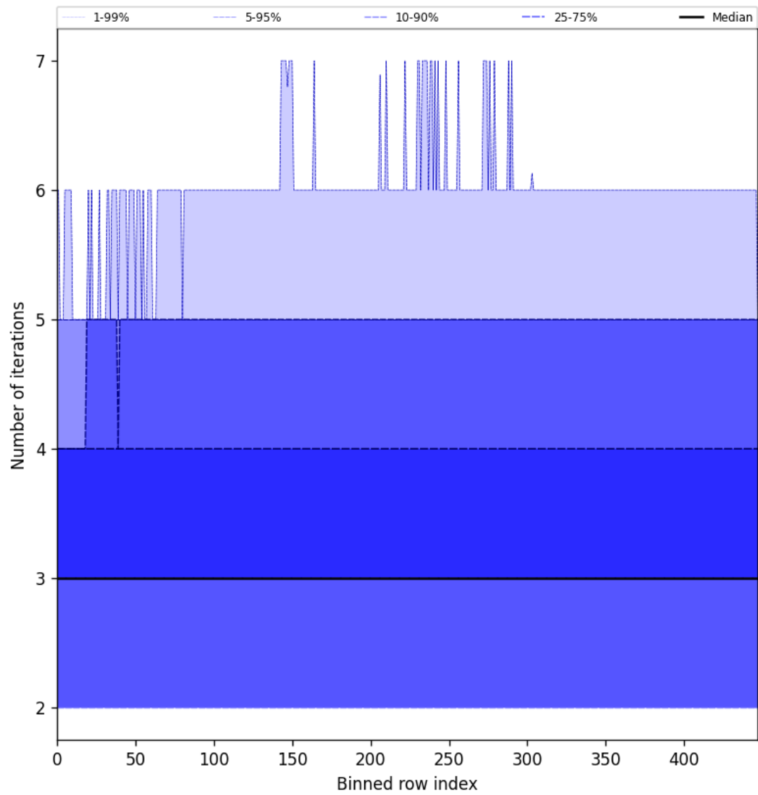
Figure 54: Along track statistics of “Number of iterations” for 2025-04-19 to 2025-04-20
