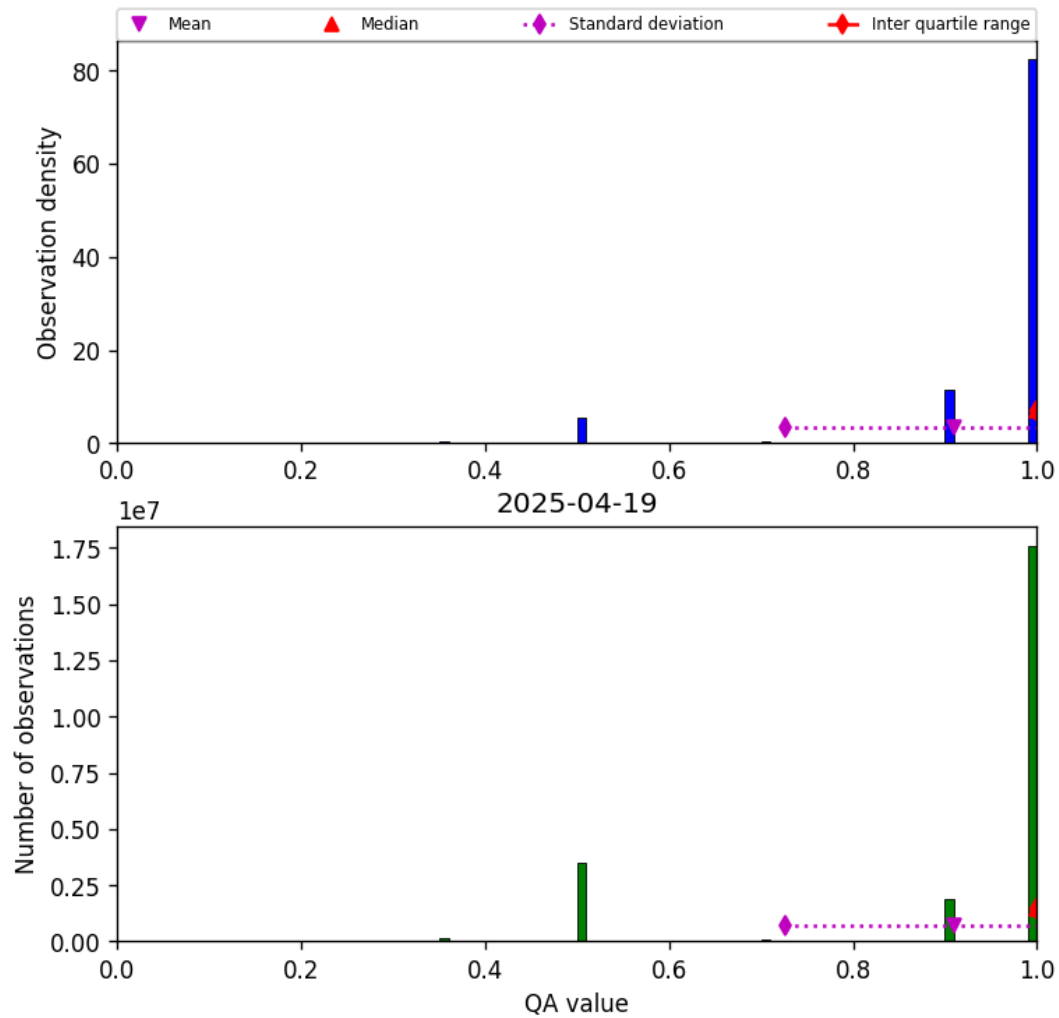
Figure 27: Histogram of “QA value” for 2025-04-19 to 2025-04-20
