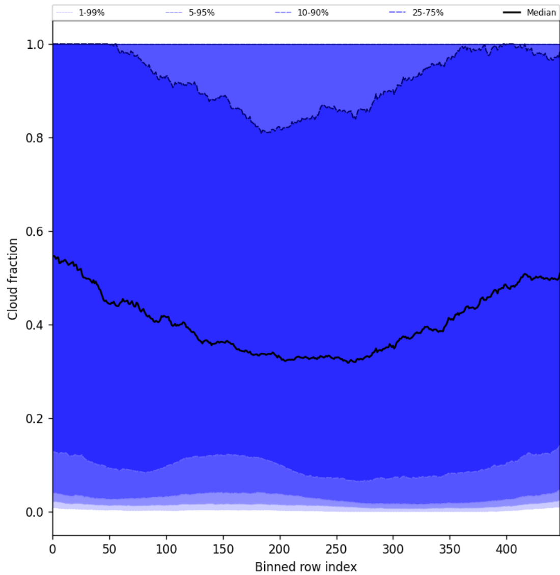
Figure 47: Along track statistics of “Cloud fraction” for 2025-04-19 to 2025-04-20
