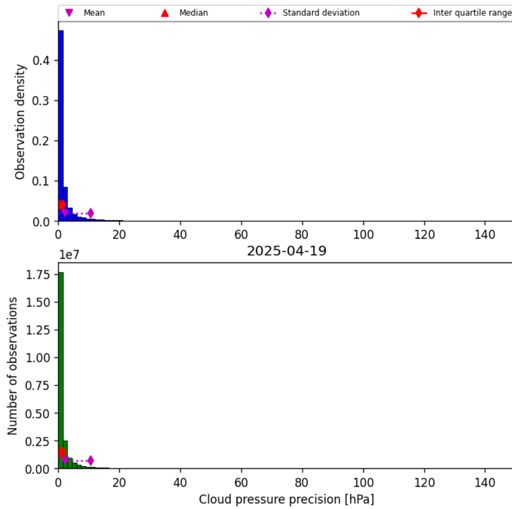
Figure 29: Histogram of “Cloud pressure precision” for 2025-04-19 to 2025-04-20
