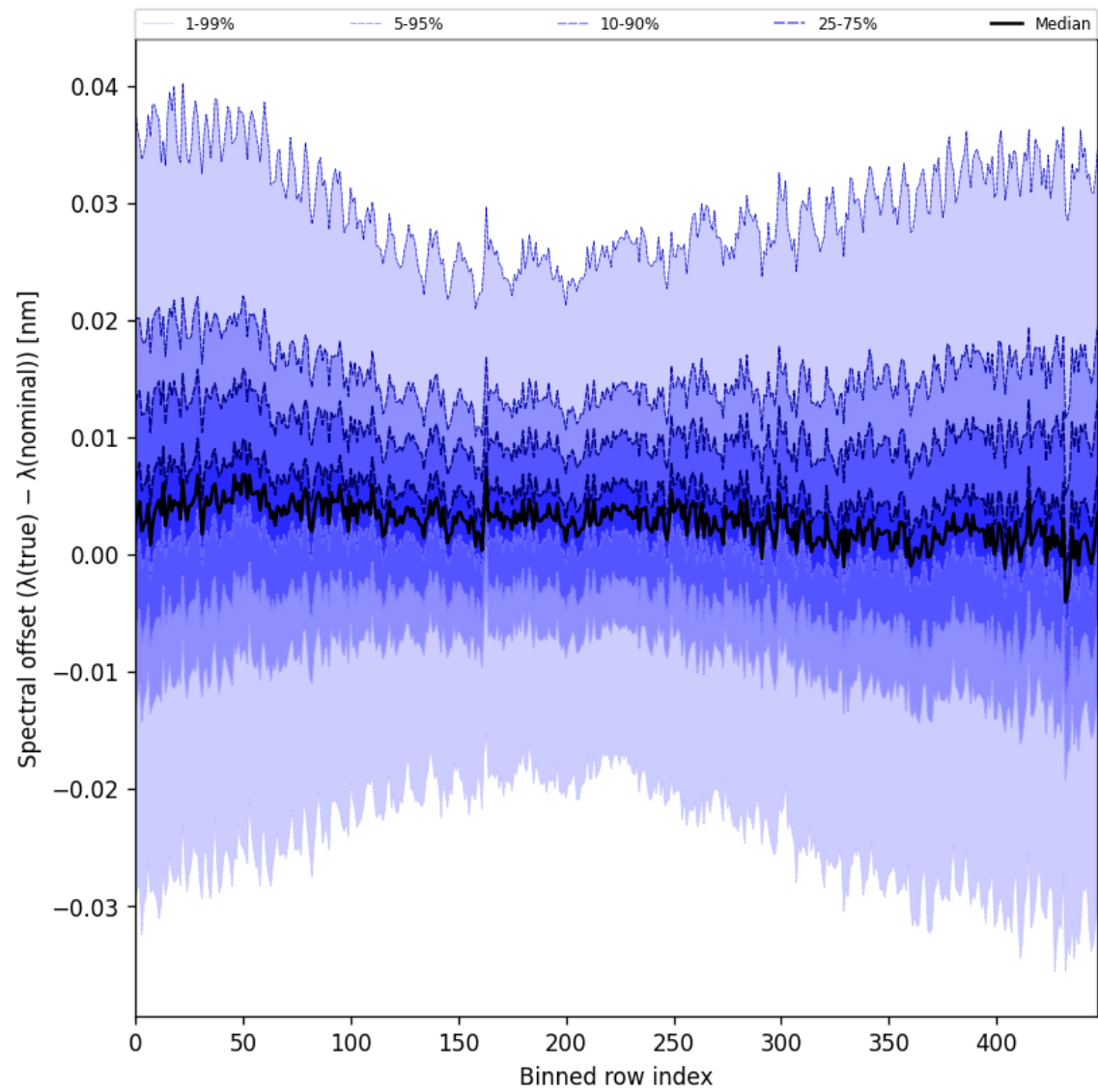
Figure 60: Along track statistics of “Spectral offset ( \lambda_{\text{true}} - \lambda_{\text{nominal}} )” for 2025-04-19 to 2025-04-20
