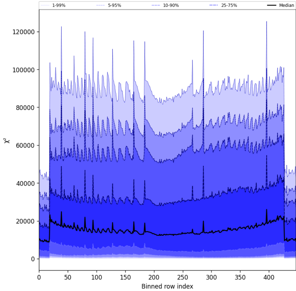
Figure 53: Along track statistics of “ \chi^2 ” for 2025-04-19 to 2025-04-20
