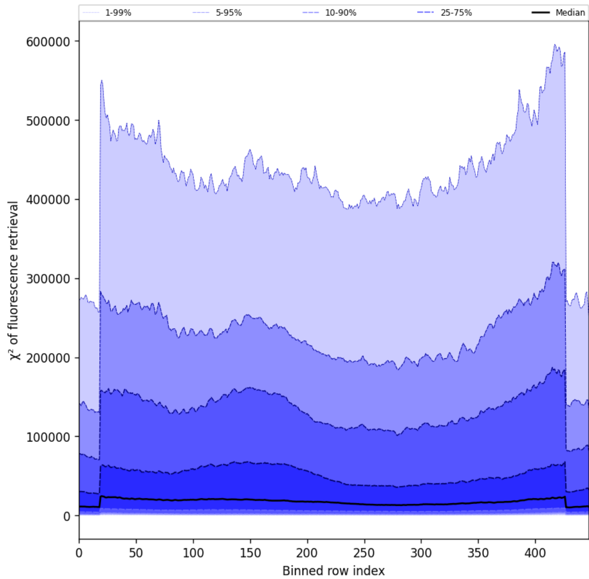
Figure 57: Along track statistics of “ \chi^2 of fluorescence retrieval” for 2025-04-19 to 2025-04-20
