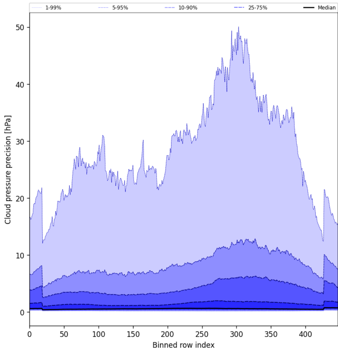
Figure 46: Along track statistics of “Cloud pressure precision” for 2025-04-19 to 2025-04-20
