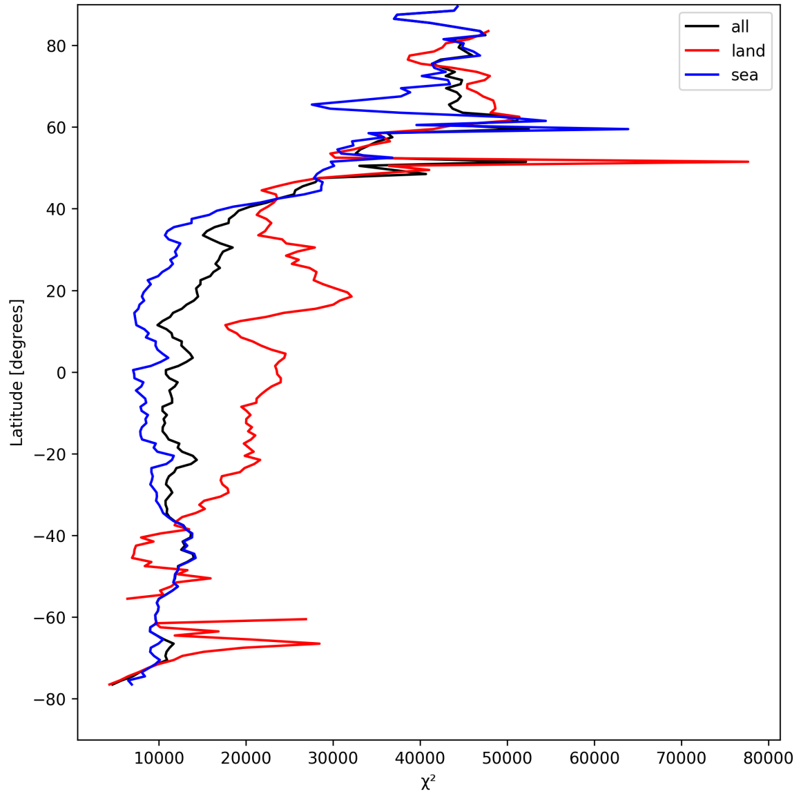
Figure 19: Zonal average of “ \chi^2 ” for 2025-04-19 to 2025-04-20.
