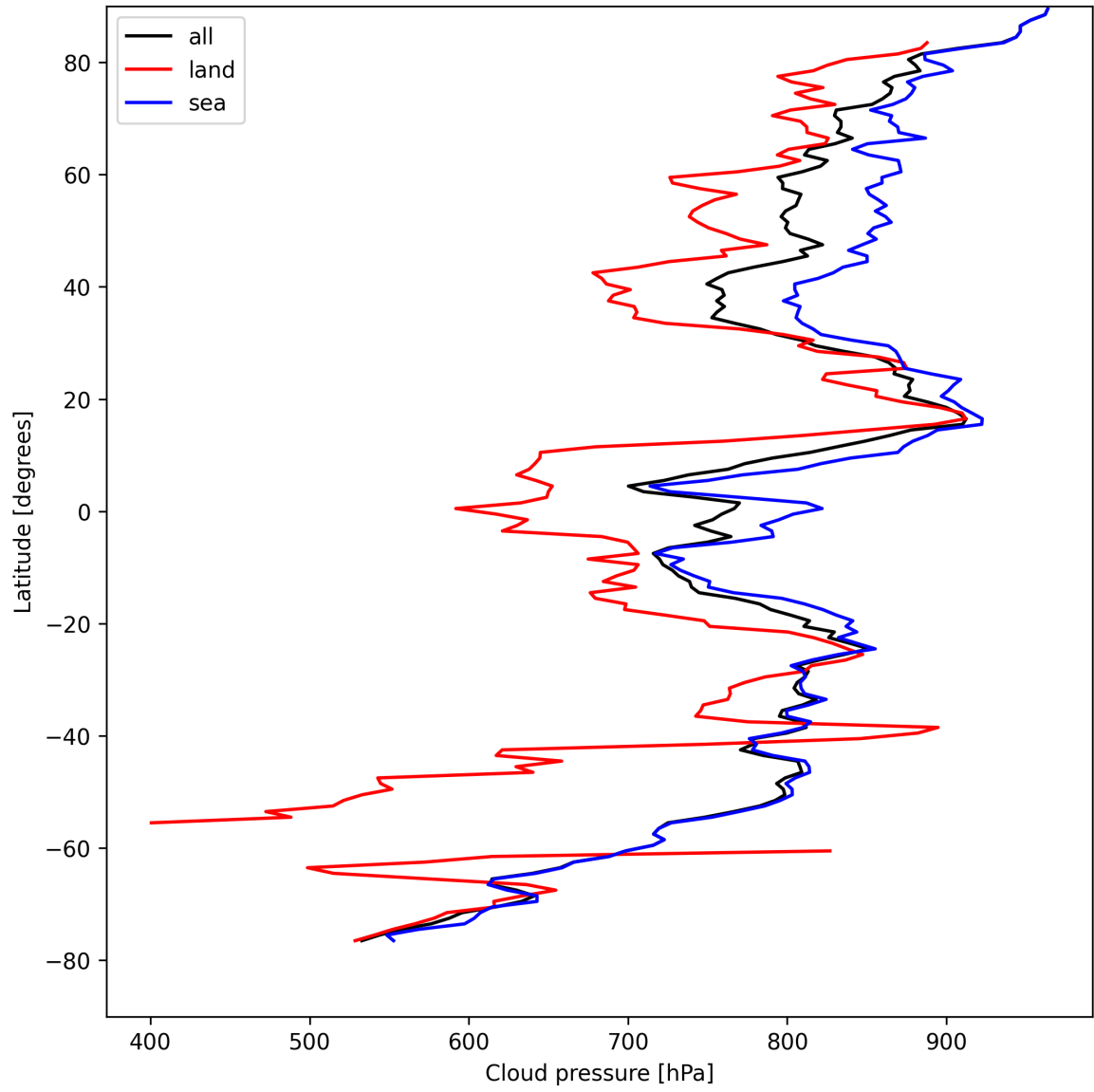
Figure 11: Zonal average of “Cloud pressure” for 2025-04-19 to 2025-04-20.
