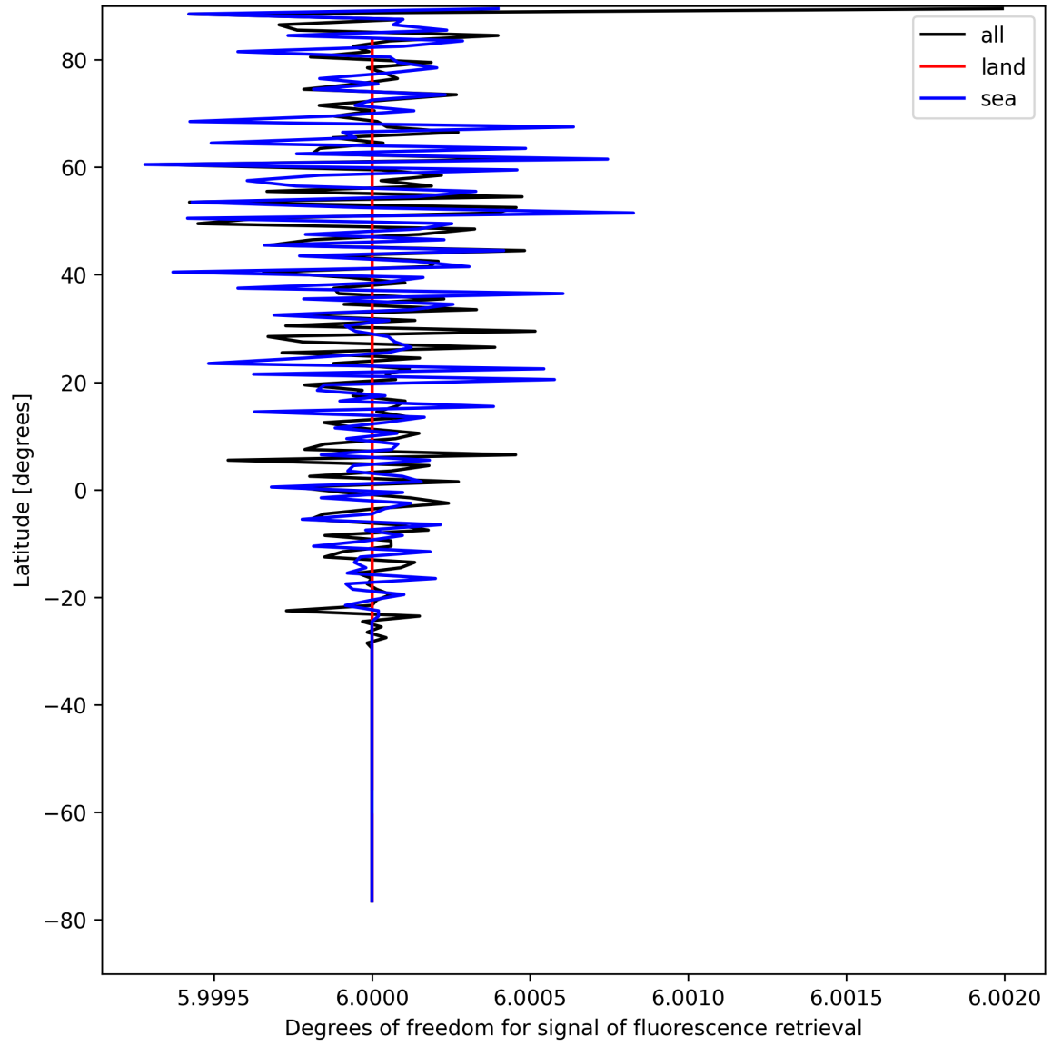
Figure 24: Zonal average of “Degrees of freedom for signal of fluorescence retrieval” for 2025-04-19 to 2025-04-20.
