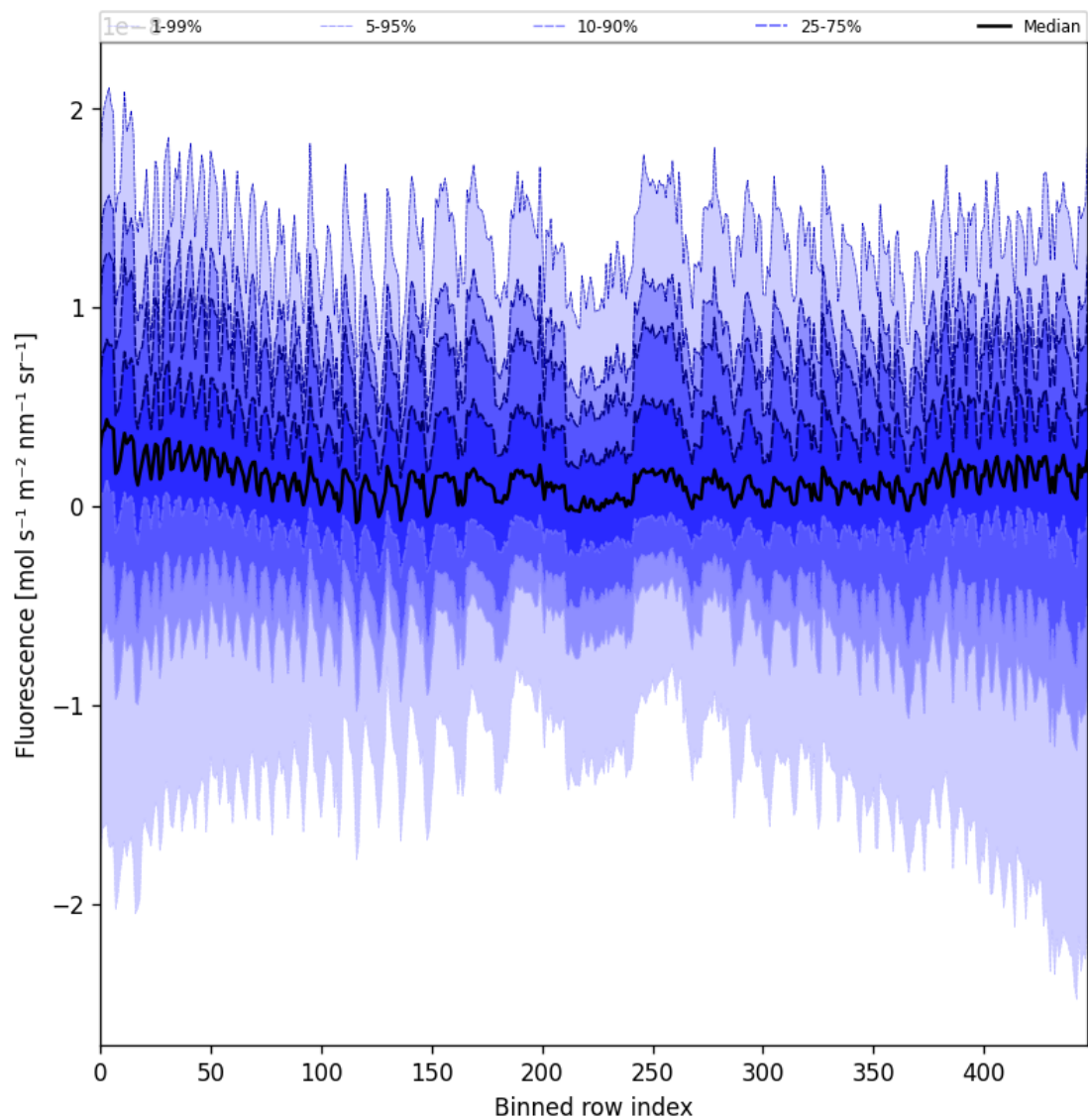
Figure 55: Along track statistics of “Fluorescence” for 2025-04-19 to 2025-04-20
