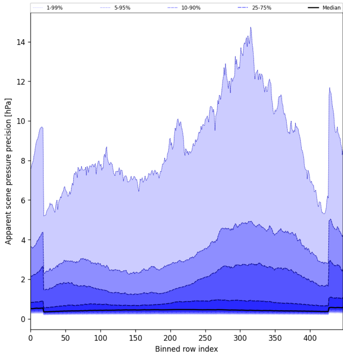
Figure 52: Along track statistics of “Apparent scene pressure precision” for 2025-04-19 to 2025-04-20
