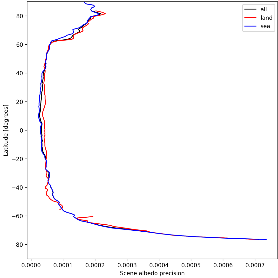
Figure 16: Zonal average of “Scene albedo precision” for 2025-04-19 to 2025-04-20.
