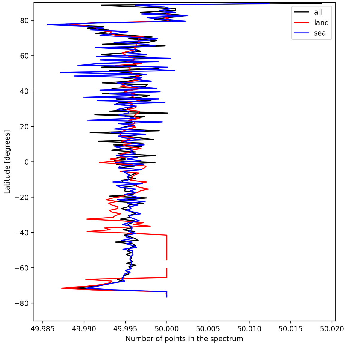
Figure 25: Zonal average of “Number of points in the spectrum” for 2025-04-19 to 2025-04-20.
