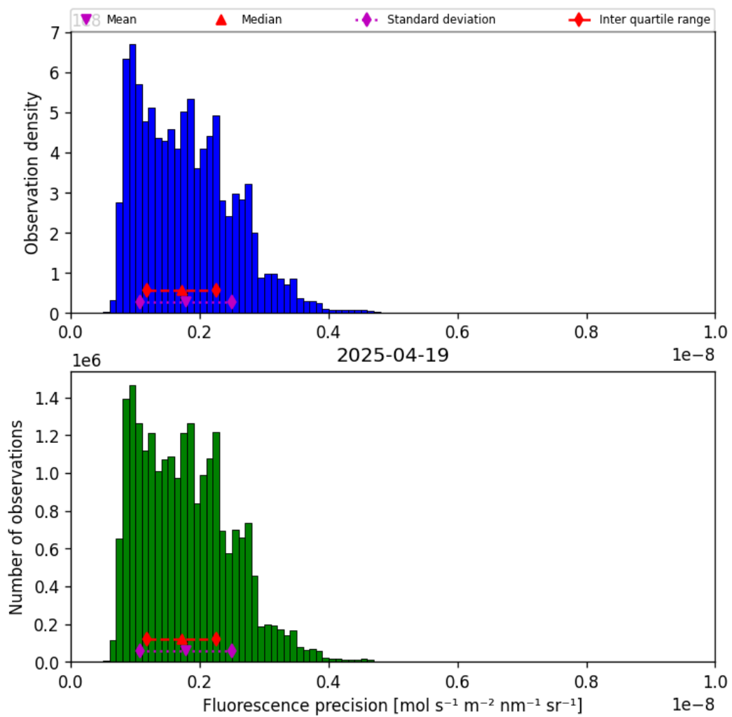
Figure 39: Histogram of “Fluorescence precision” for 2025-04-19 to 2025-04-20
