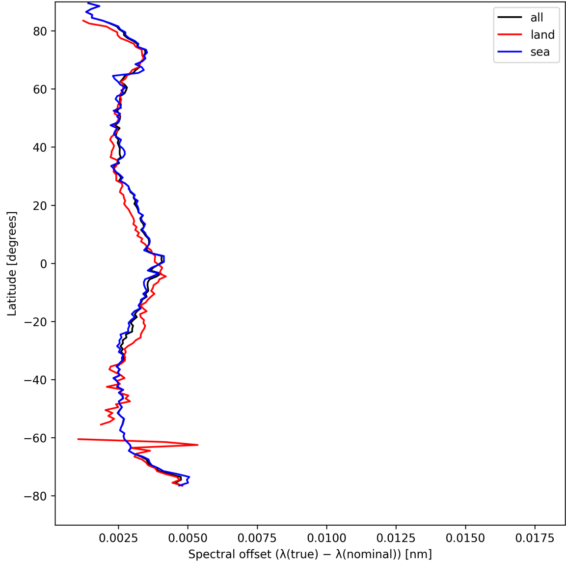
Figure 26: Zonal average of “Spectral offset ( \lambda_{\text{true}} - \lambda_{\text{nominal}} )” for 2025-04-19 to 2025-04-20.
