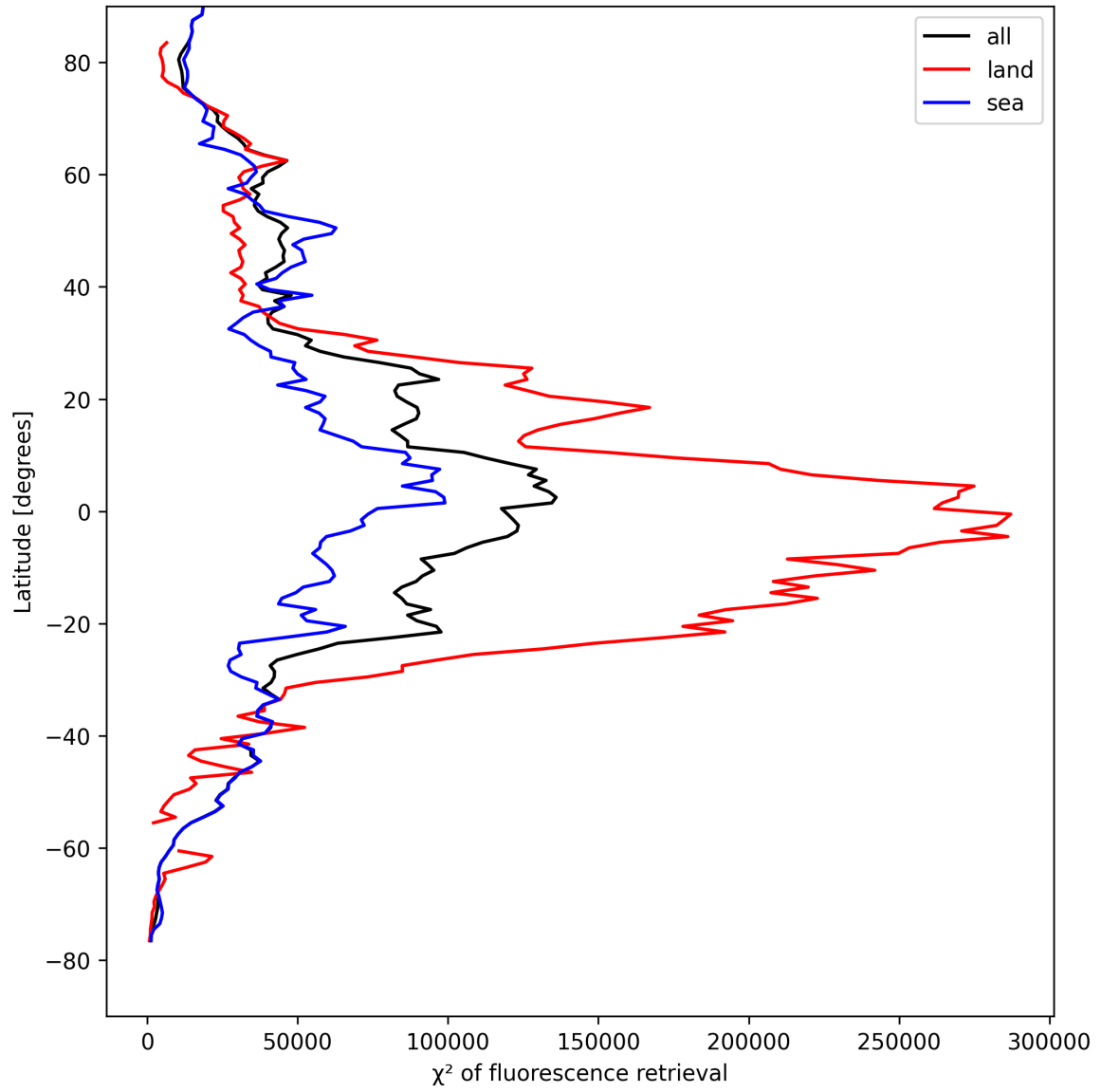
Figure 23: Zonal average of “ \chi^2 of fluorescence retrieval” for 2025-04-19 to 2025-04-20.
