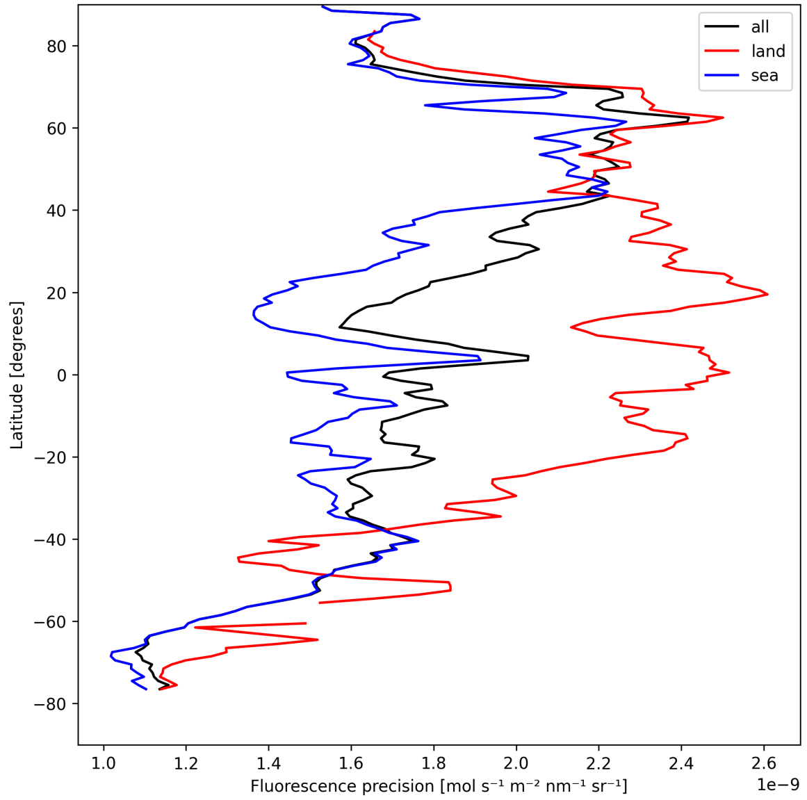
Figure 22: Zonal average of “Fluorescence precision” for 2025-04-19 to 2025-04-20.
