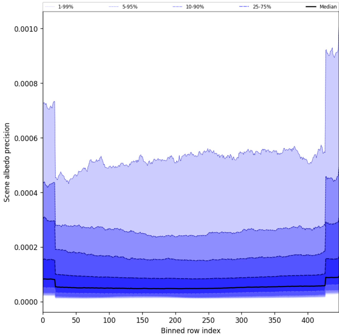
Figure 50: Along track statistics of “Scene albedo precision” for 2025-04-19 to 2025-04-20
