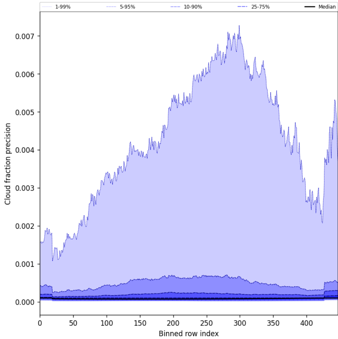
Figure 48: Along track statistics of “Cloud fraction precision” for 2025-04-19 to 2025-04-20
