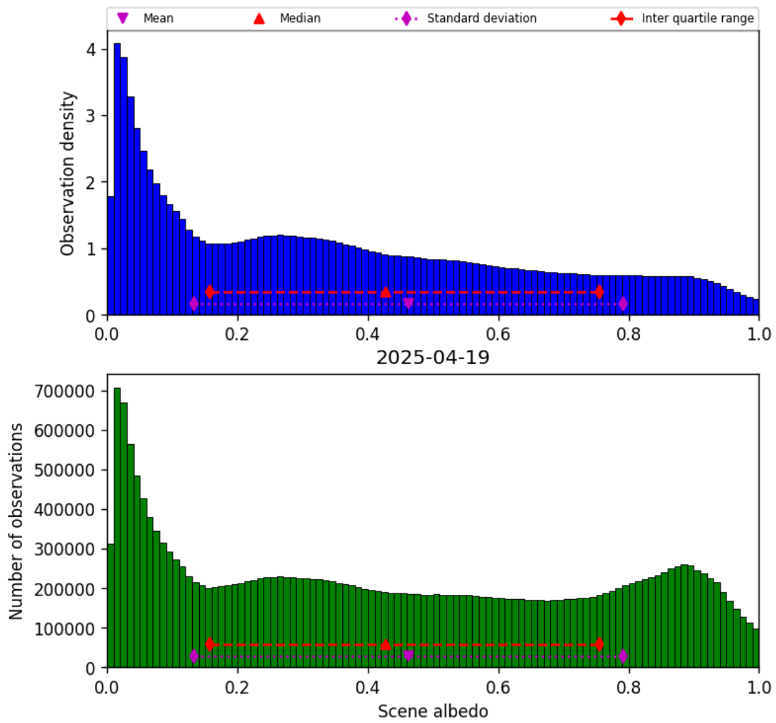
Figure 32: Histogram of “Scene albedo” for 2025-04-19 to 2025-04-20
