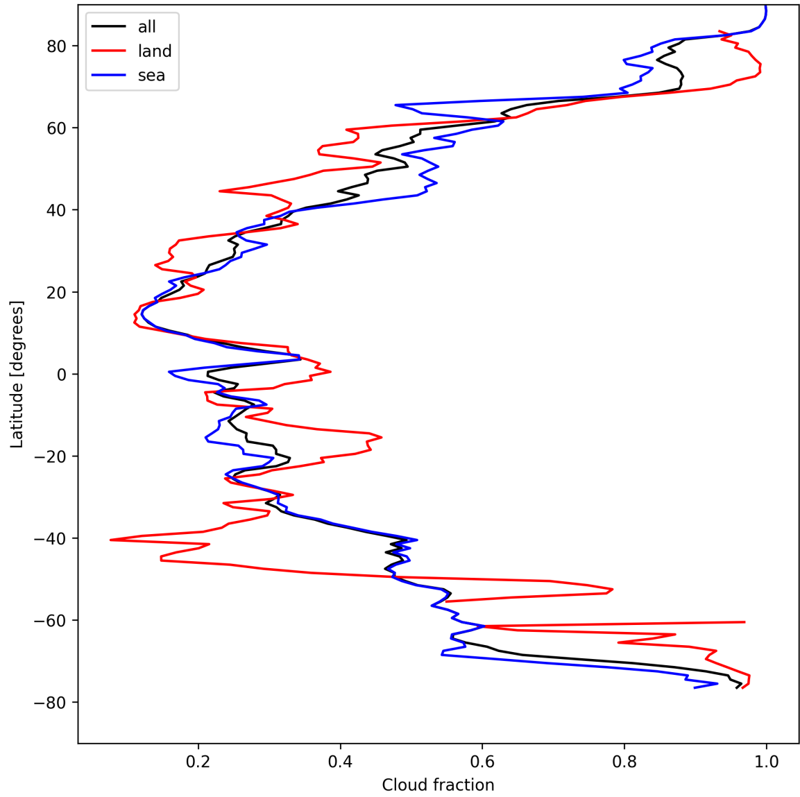
Figure 13: Zonal average of “Cloud fraction” for 2025-04-19 to 2025-04-20.
