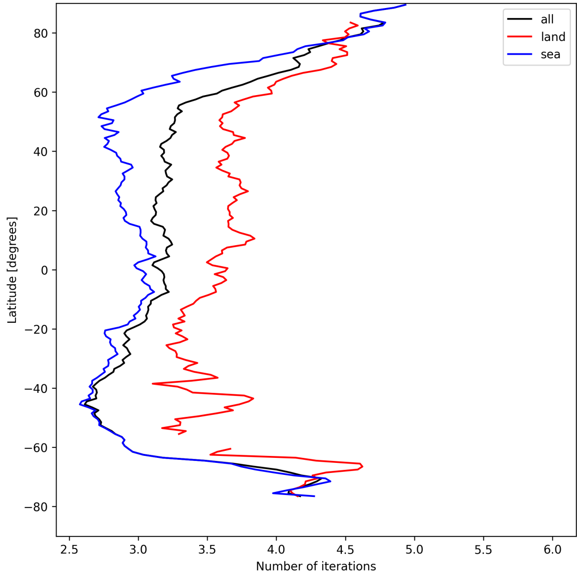
Figure 20: Zonal average of “Number of iterations” for 2025-04-19 to 2025-04-20.
