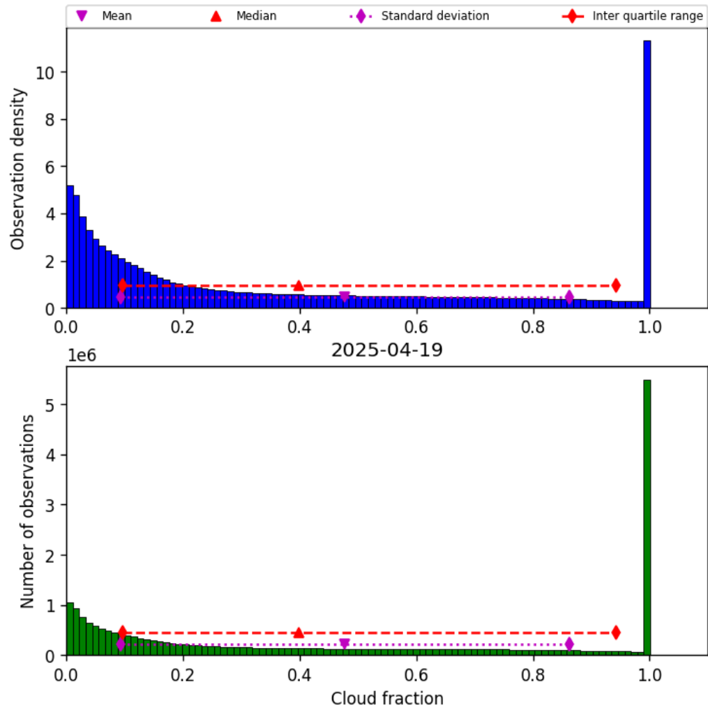
Figure 30: Histogram of “Cloud fraction” for 2025-04-19 to 2025-04-20
