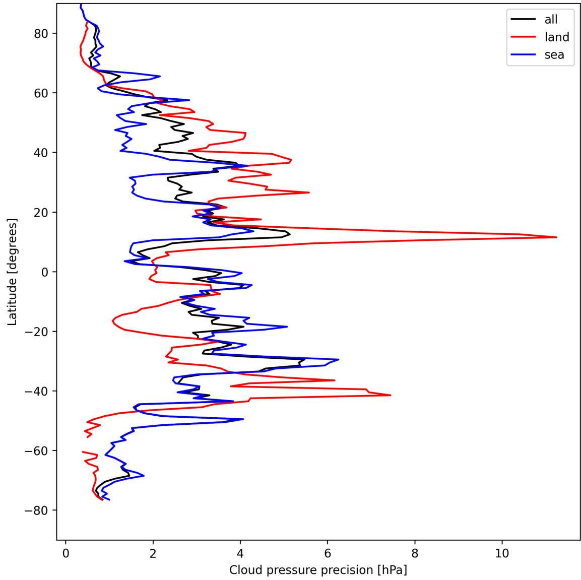
Figure 12: Zonal average of “Cloud pressure precision” for 2025-04-19 to 2025-04-20.
