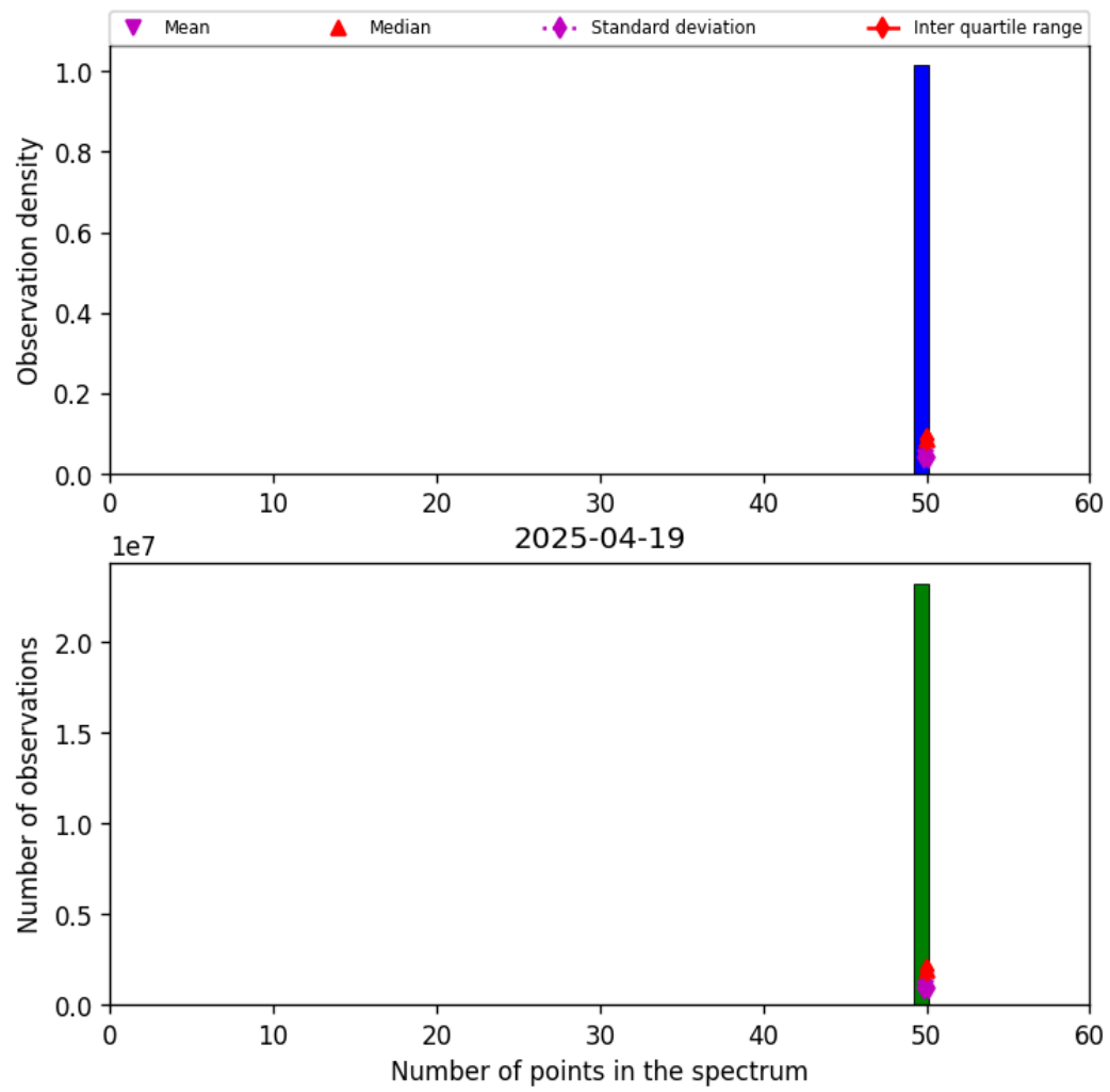
Figure 42: Histogram of “Number of points in the spectrum” for 2025-04-19 to 2025-04-20
