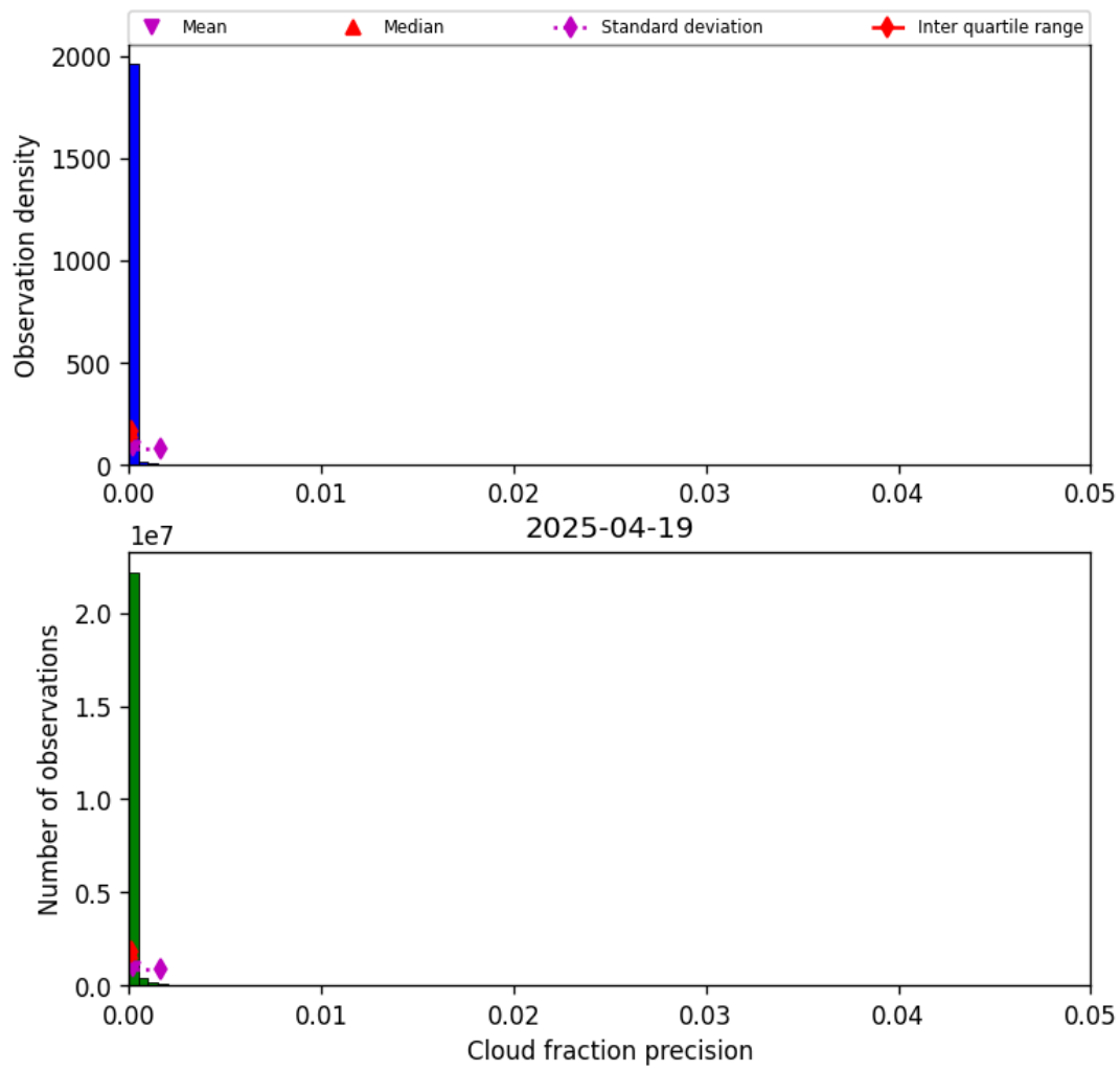
Figure 31: Histogram of “Cloud fraction precision” for 2025-04-19 to 2025-04-20
