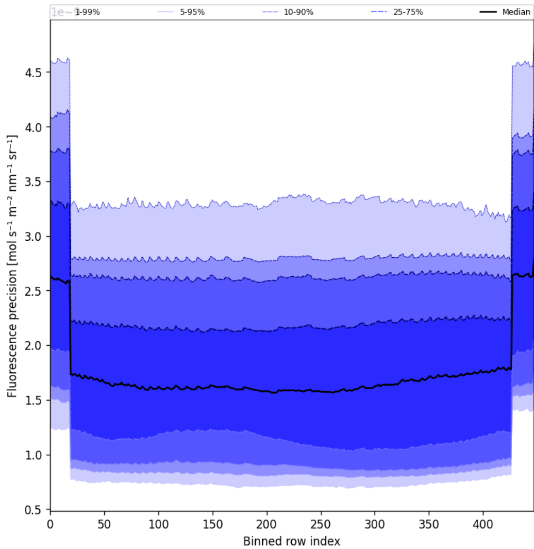
Figure 56: Along track statistics of “Fluorescence precision” for 2025-04-19 to 2025-04-20
