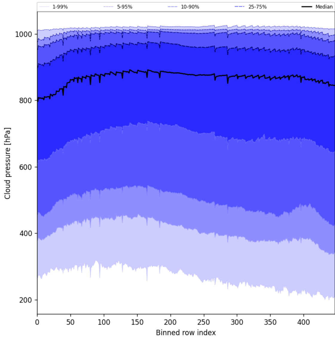
Figure 45: Along track statistics of “Cloud pressure” for 2025-04-19 to 2025-04-20
