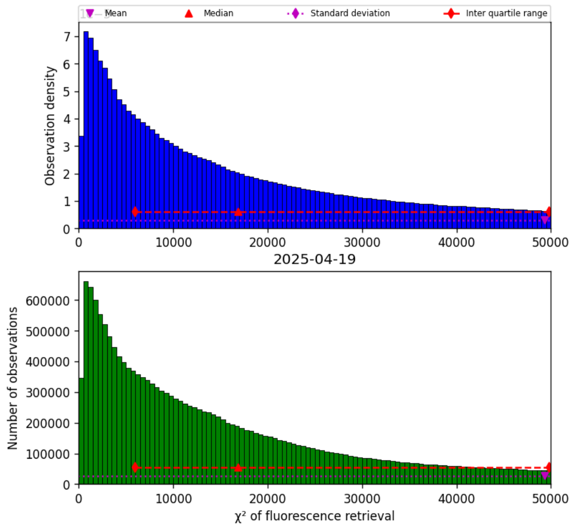
Figure 40: Histogram of “ \chi^2 of fluorescence retrieval” for 2025-04-19 to 2025-04-20
