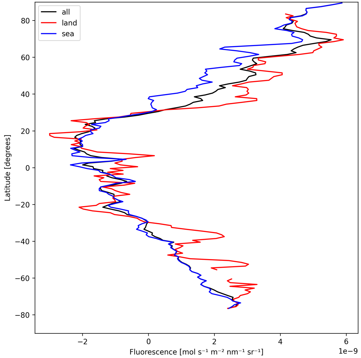
Figure 21: Zonal average of “Fluorescence” for 2025-04-19 to 2025-04-20.
