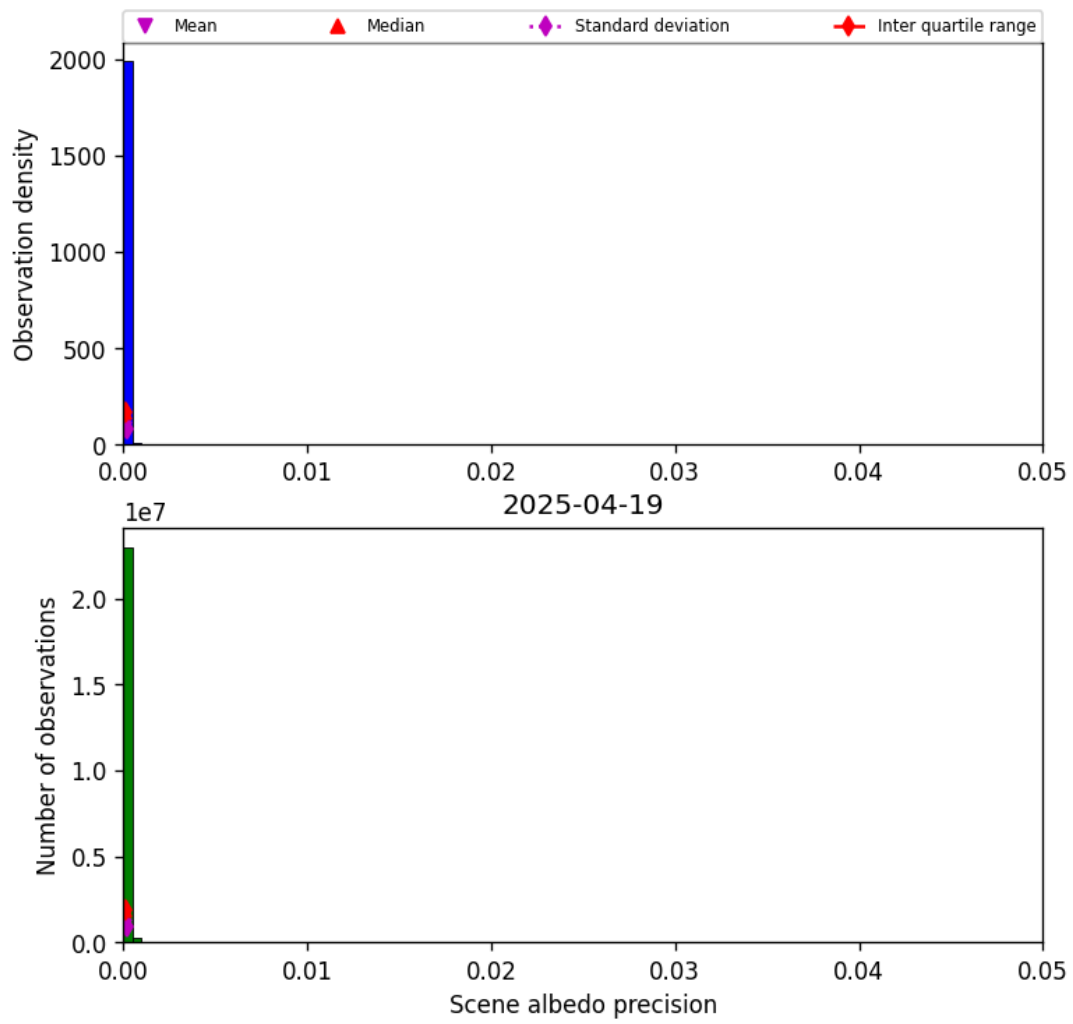
Figure 33: Histogram of “Scene albedo precision” for 2025-04-19 to 2025-04-20
