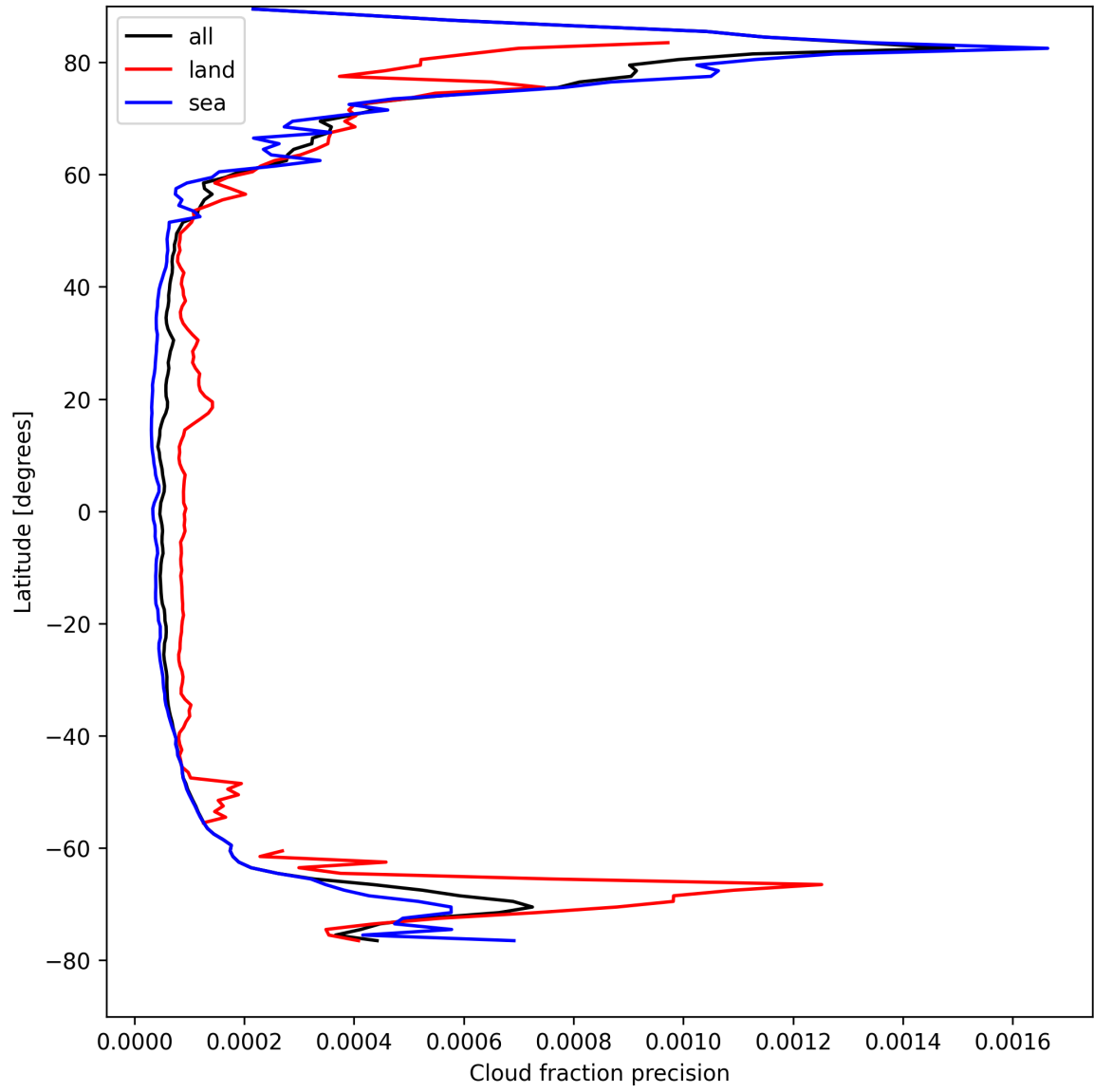
Figure 14: Zonal average of “Cloud fraction precision” for 2025-04-19 to 2025-04-20.
