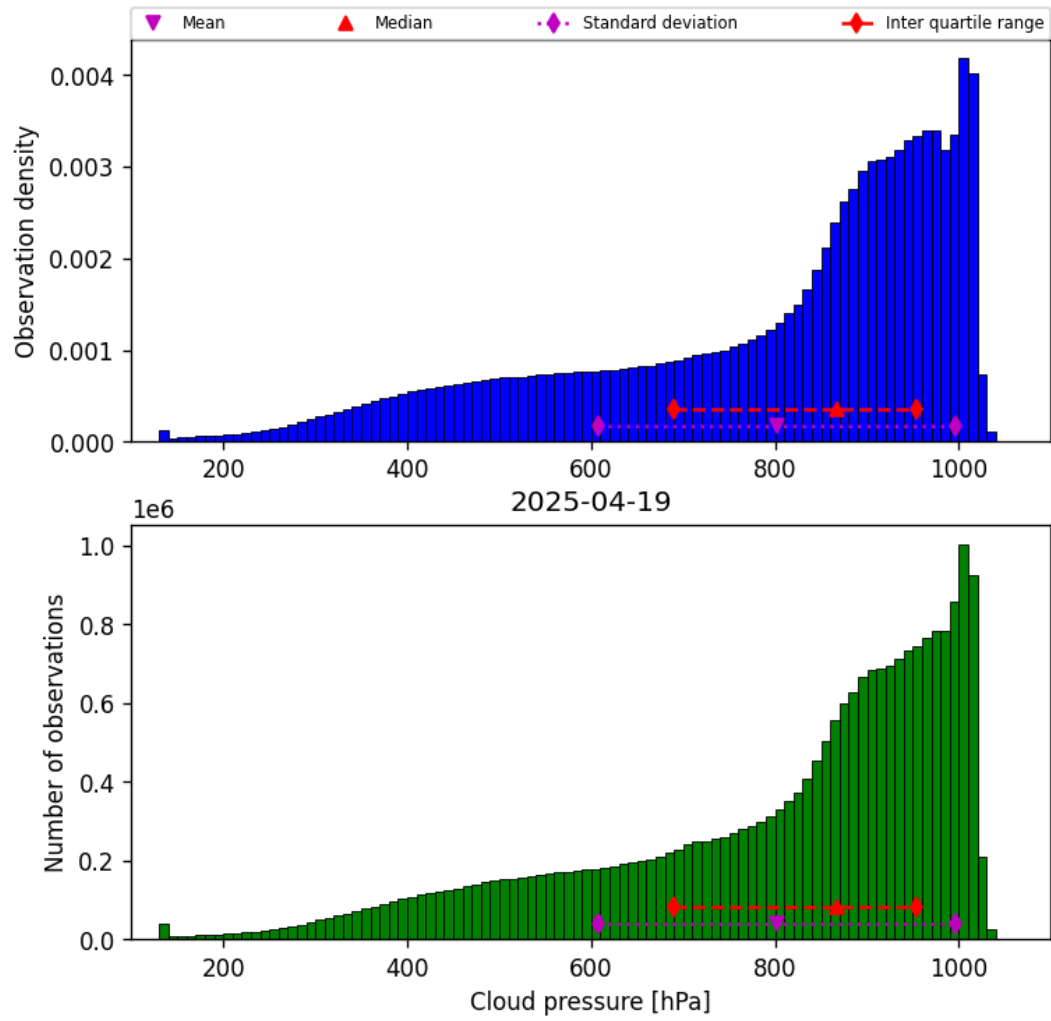
Figure 28: Histogram of “Cloud pressure” for 2025-04-19 to 2025-04-20
