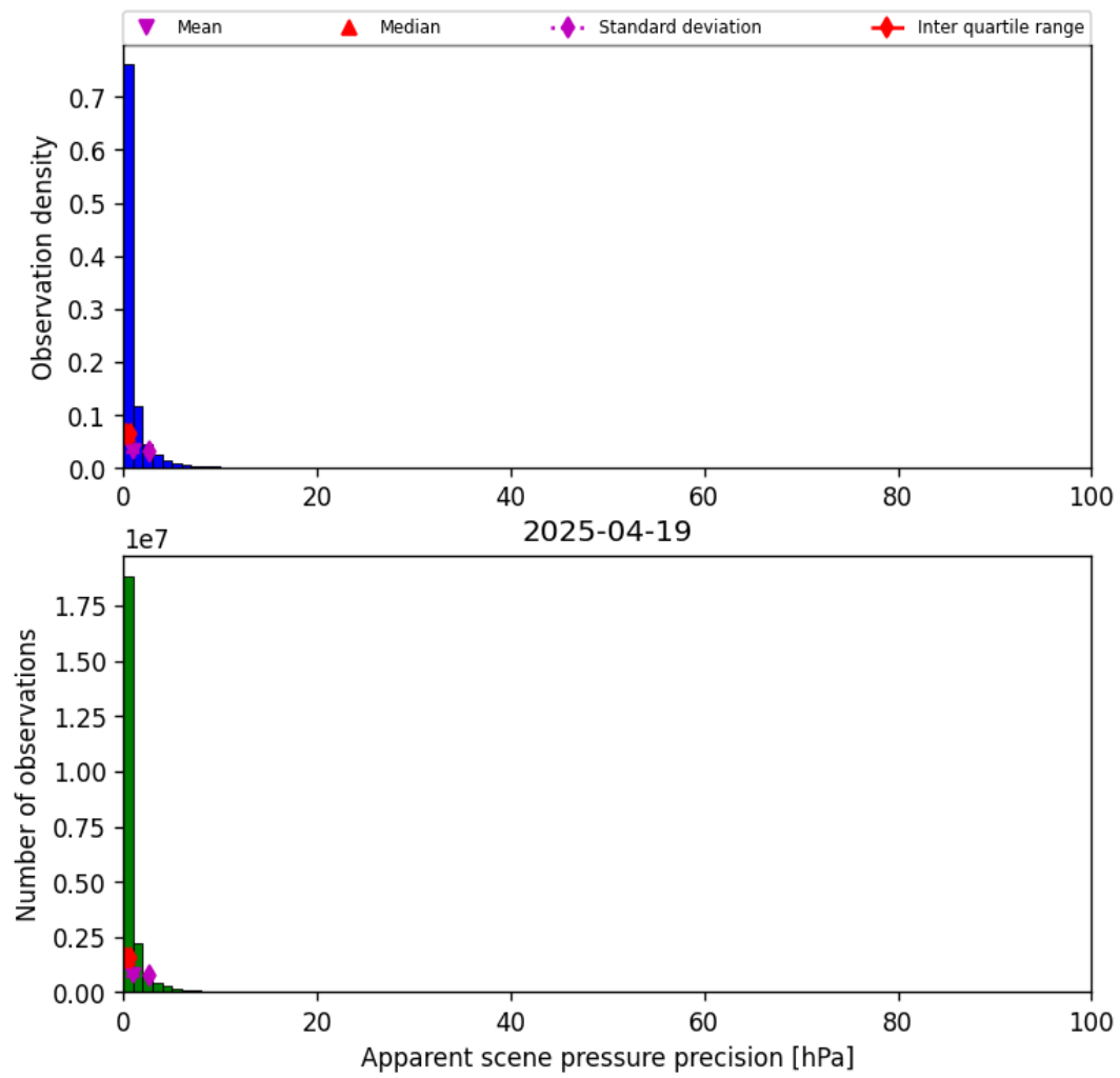
Figure 35: Histogram of “Apparent scene pressure precision” for 2025-04-19 to 2025-04-20
