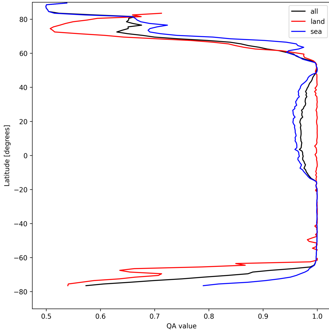
Figure 10: Zonal average of “QA value” for 2025-04-19 to 2025-04-20.
