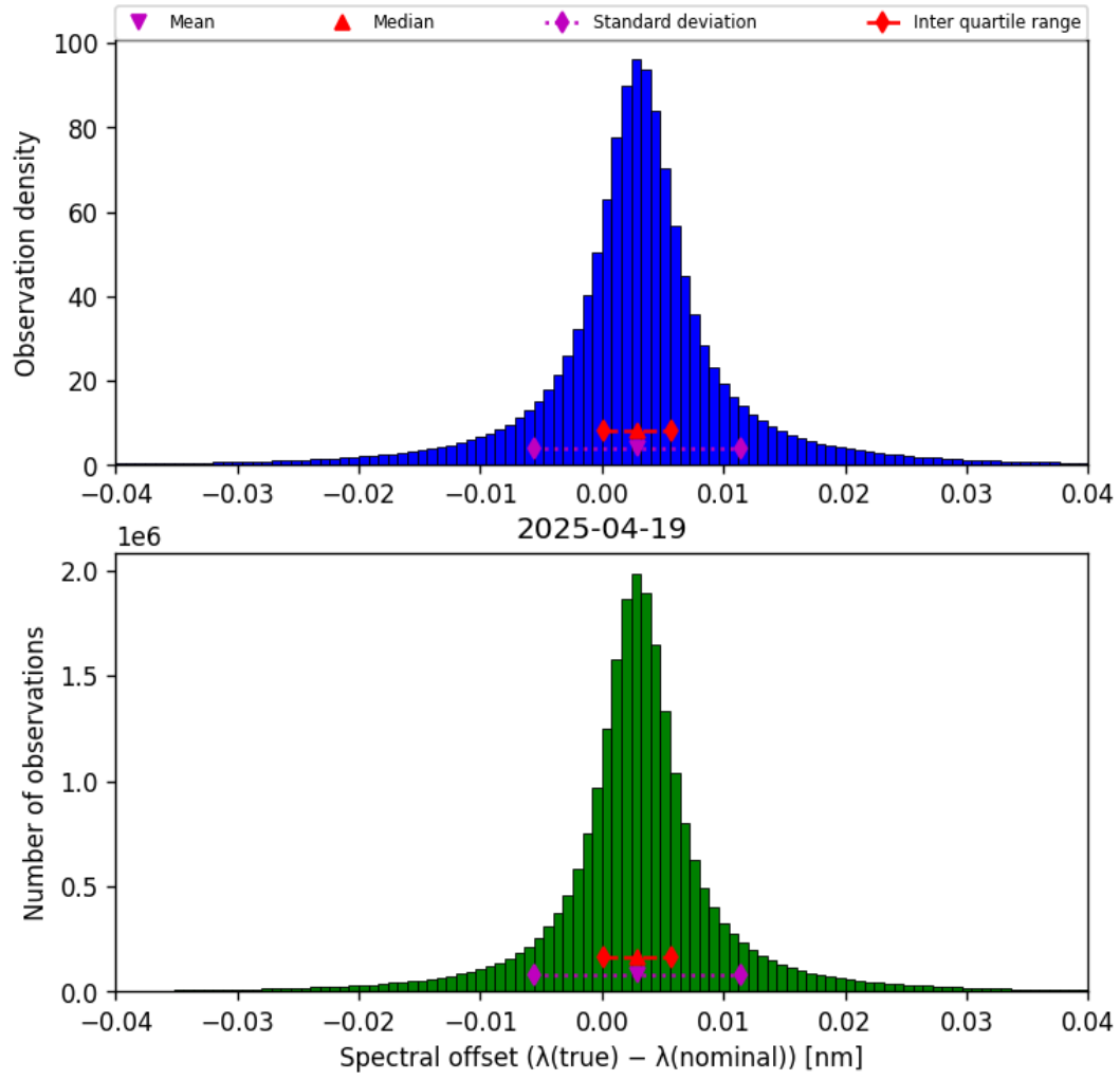
Figure 43: Histogram of “Spectral offset ( \lambda_{\text{true}} - \lambda_{\text{nominal}} )” for 2025-04-19 to 2025-04-20
