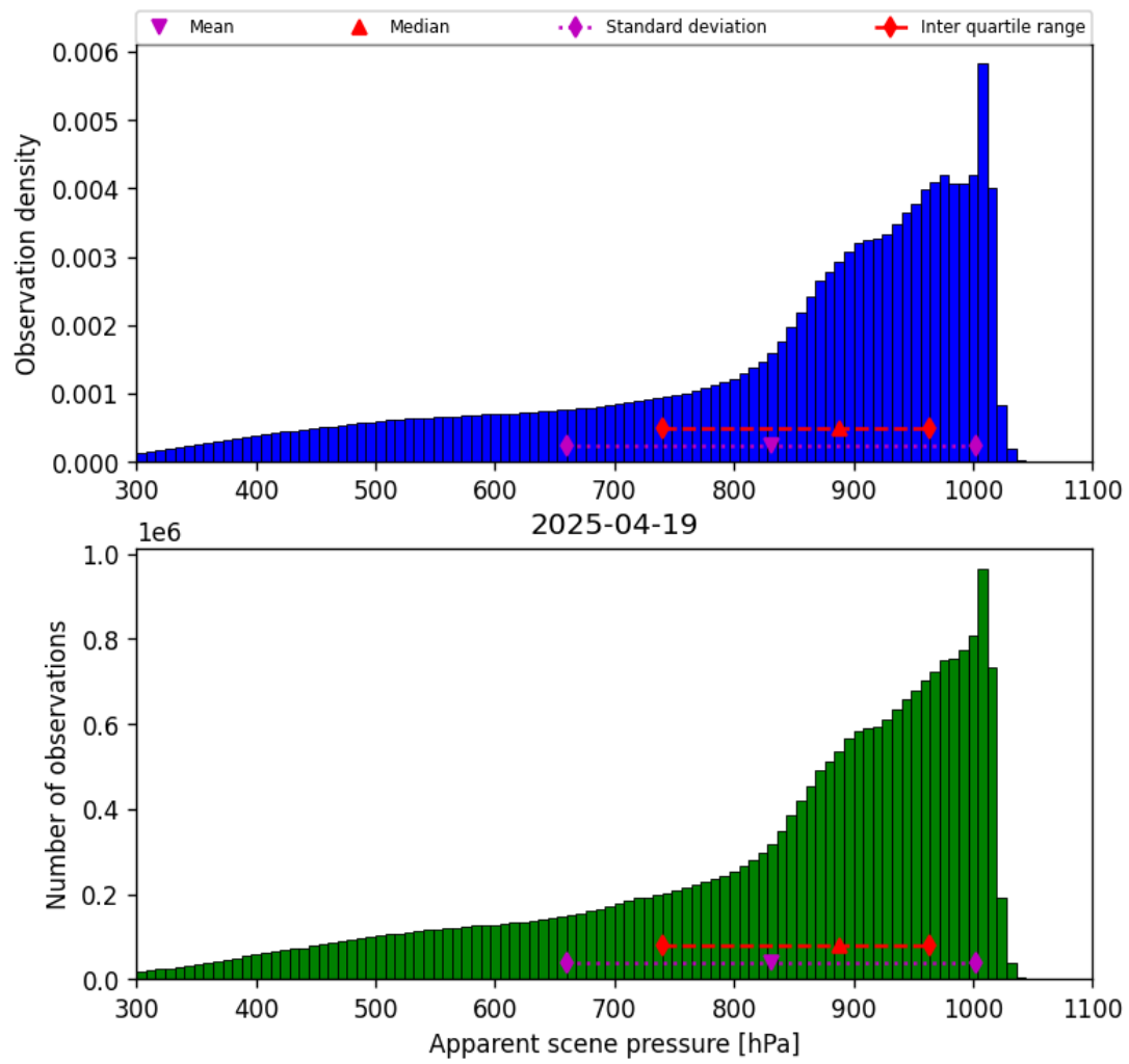
Figure 34: Histogram of “Apparent scene pressure” for 2025-04-19 to 2025-04-20
