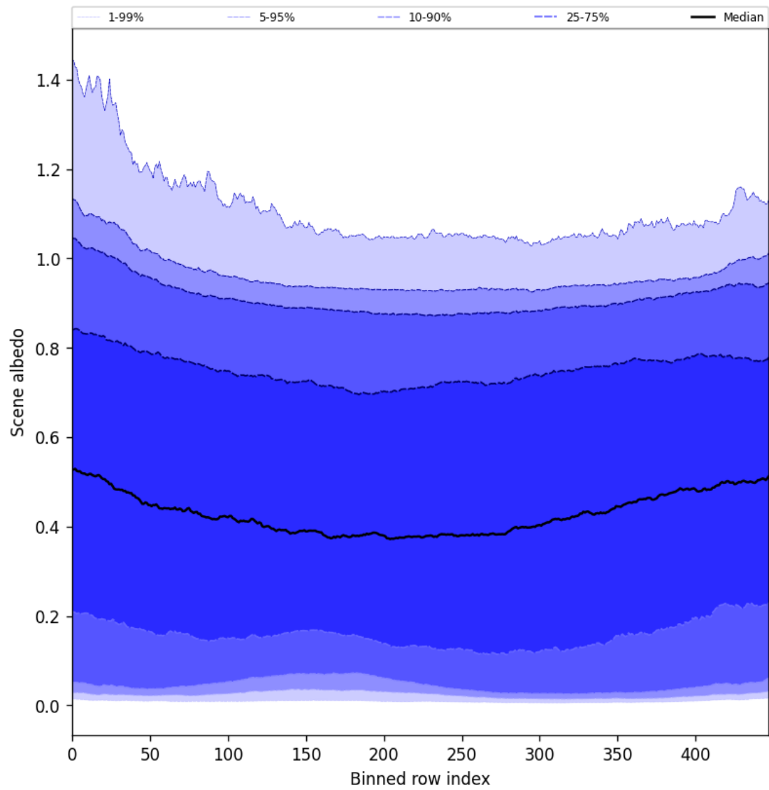
Figure 49: Along track statistics of “Scene albedo” for 2025-04-19 to 2025-04-20
