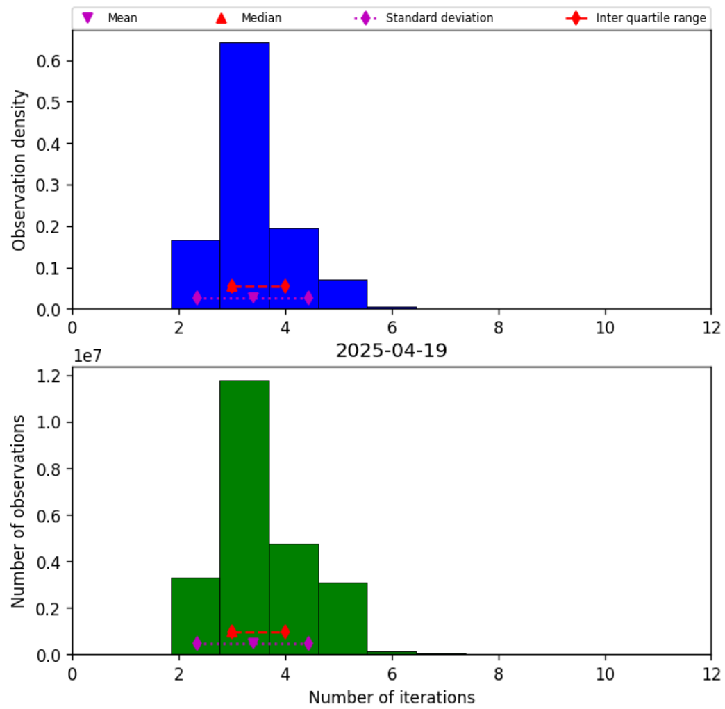
Figure 37: Histogram of “Number of iterations” for 2025-04-19 to 2025-04-20
