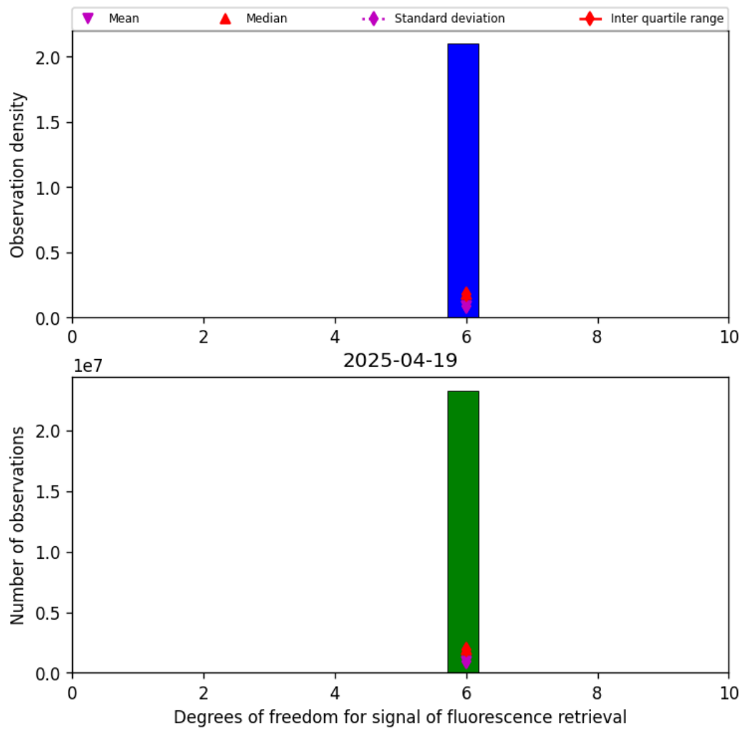
Figure 41: Histogram of “Degrees of freedom for signal of fluorescence retrieval” for 2025-04-19 to 2025-04-20
