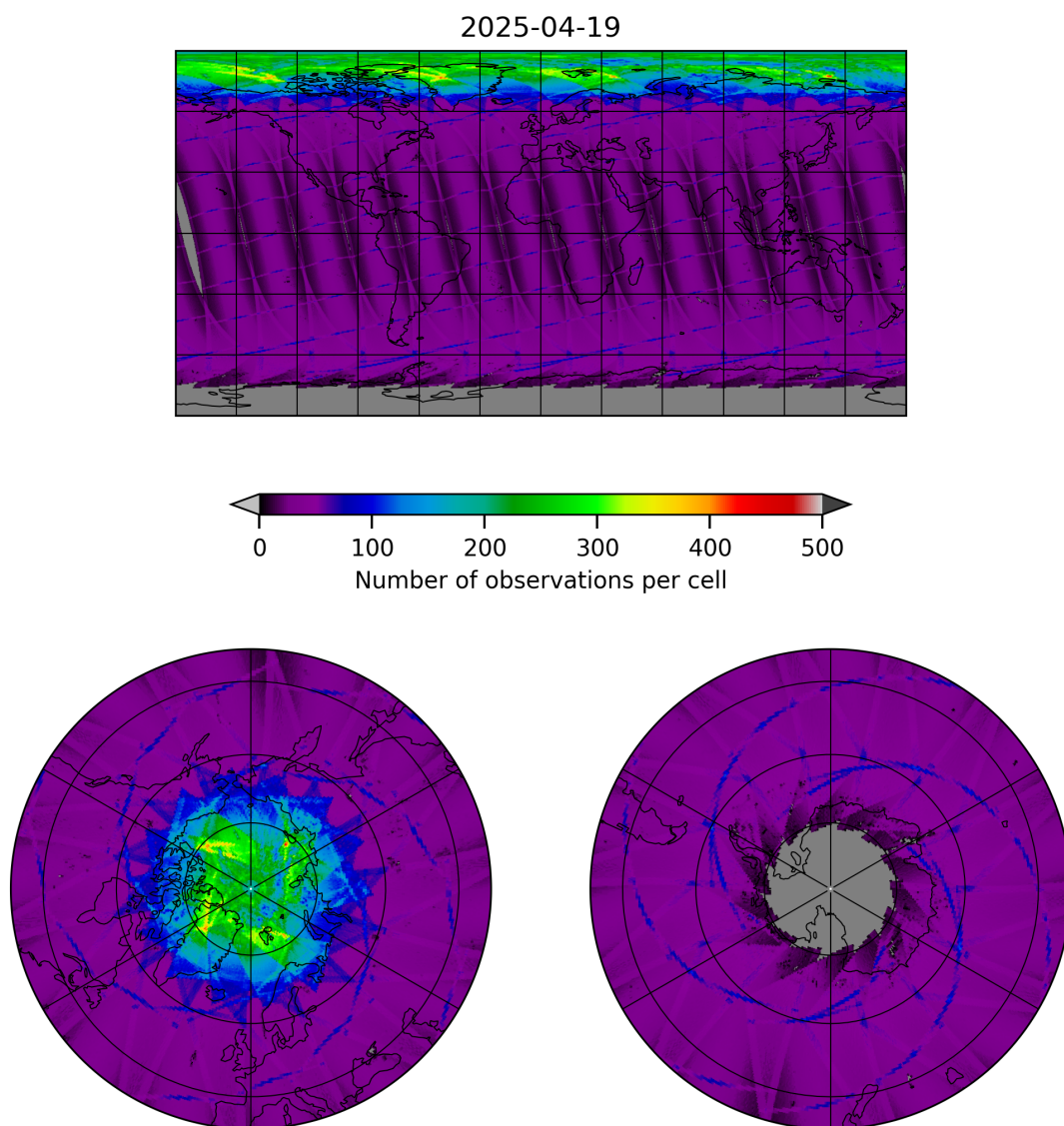
Figure 9: Map of the number of observations for 2025-04-19 to 2025-04-20
