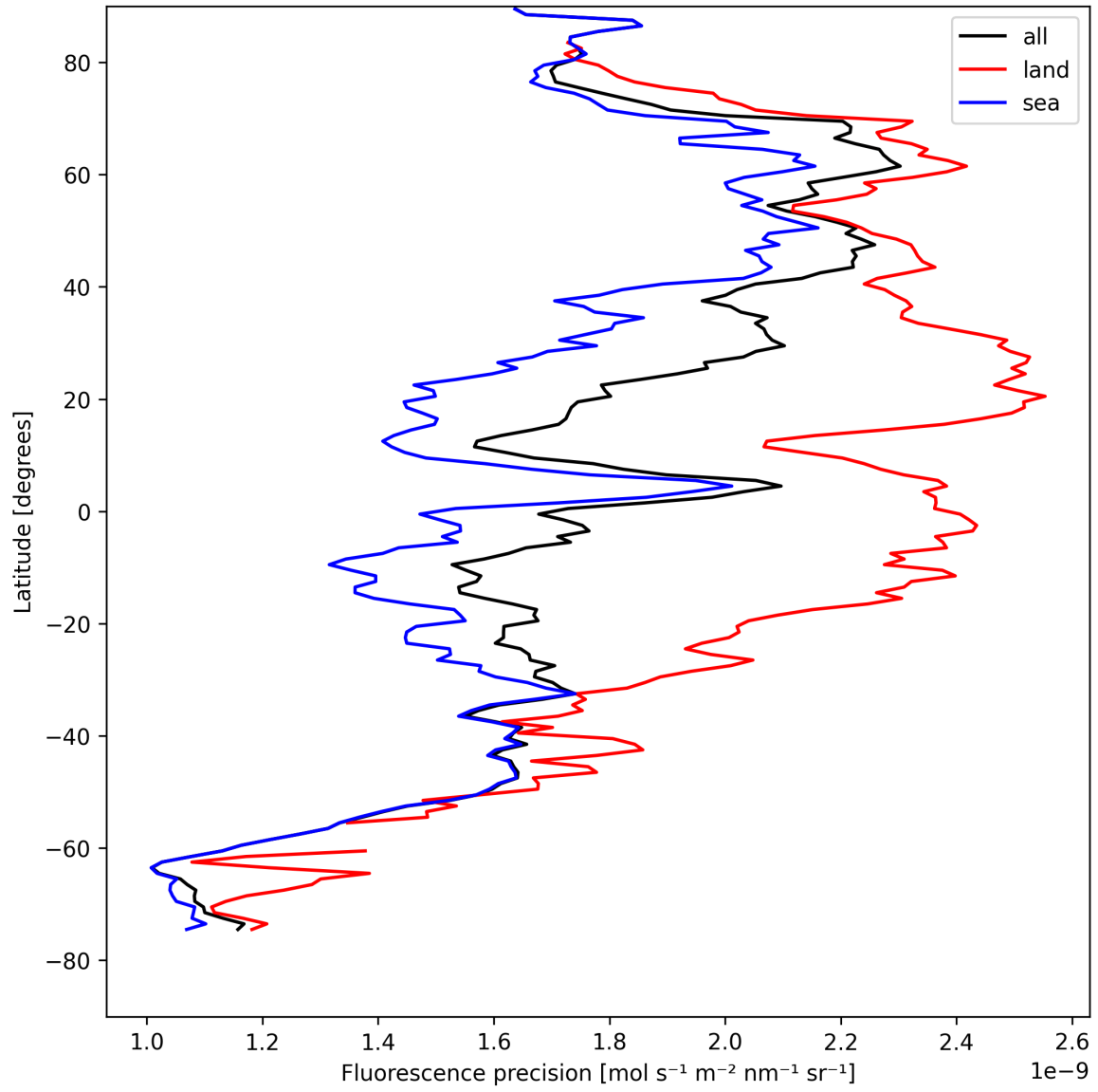
Figure 22: Zonal average of “Fluorescence precision” for 2025-04-24 to 2025-04-25.
