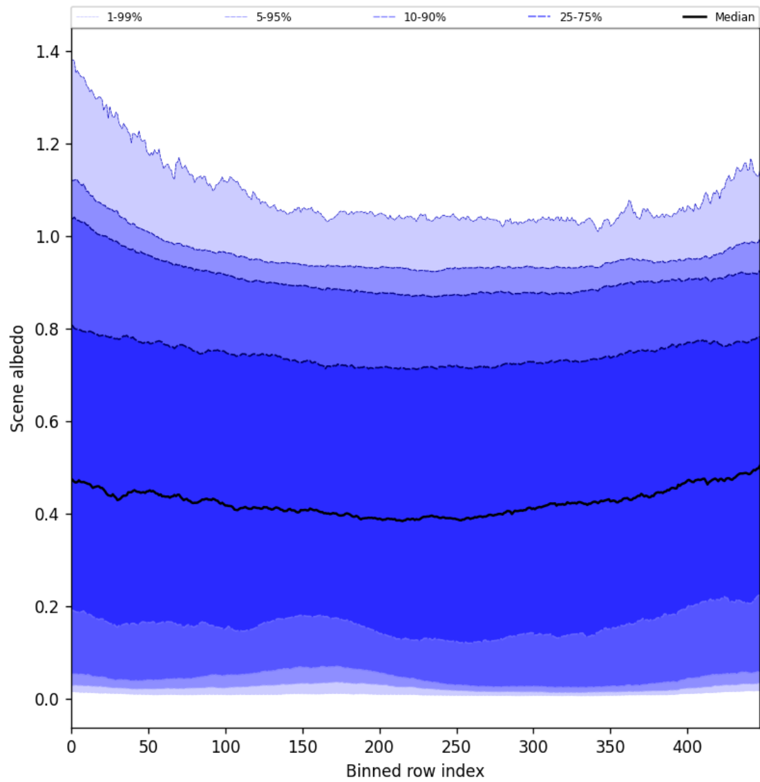
Figure 49: Along track statistics of “Scene albedo” for 2025-04-24 to 2025-04-25
