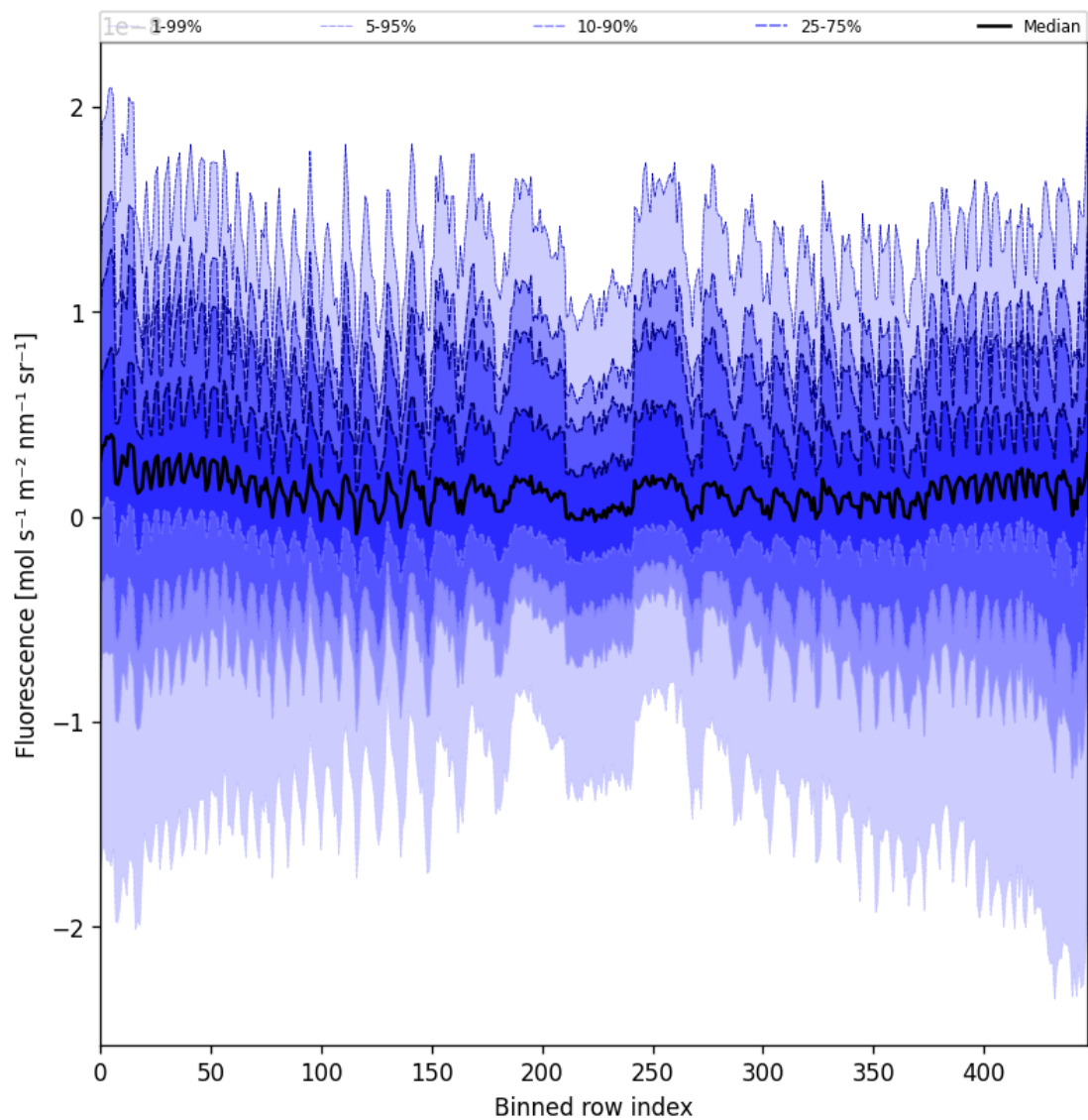
Figure 55: Along track statistics of “Fluorescence” for 2025-04-24 to 2025-04-25
