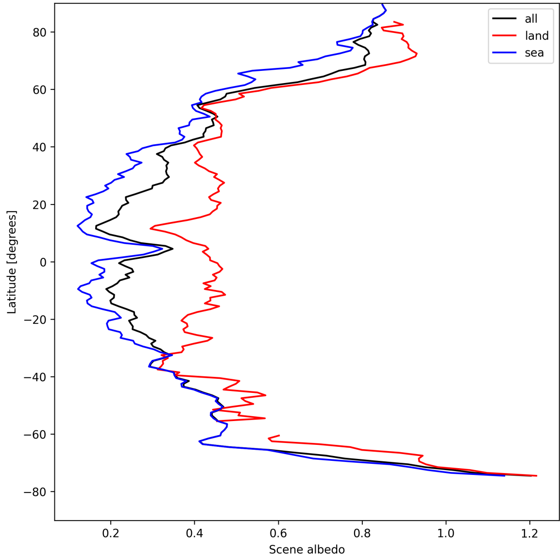
Figure 15: Zonal average of “Scene albedo” for 2025-04-24 to 2025-04-25.
