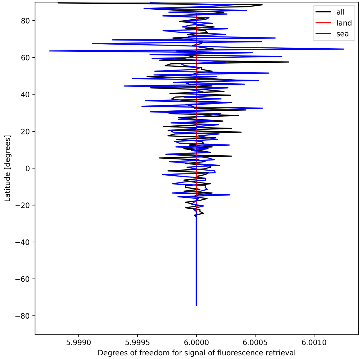
Figure 24: Zonal average of “Degrees of freedom for signal of fluorescence retrieval” for 2025-04-24 to 2025-04-25.
