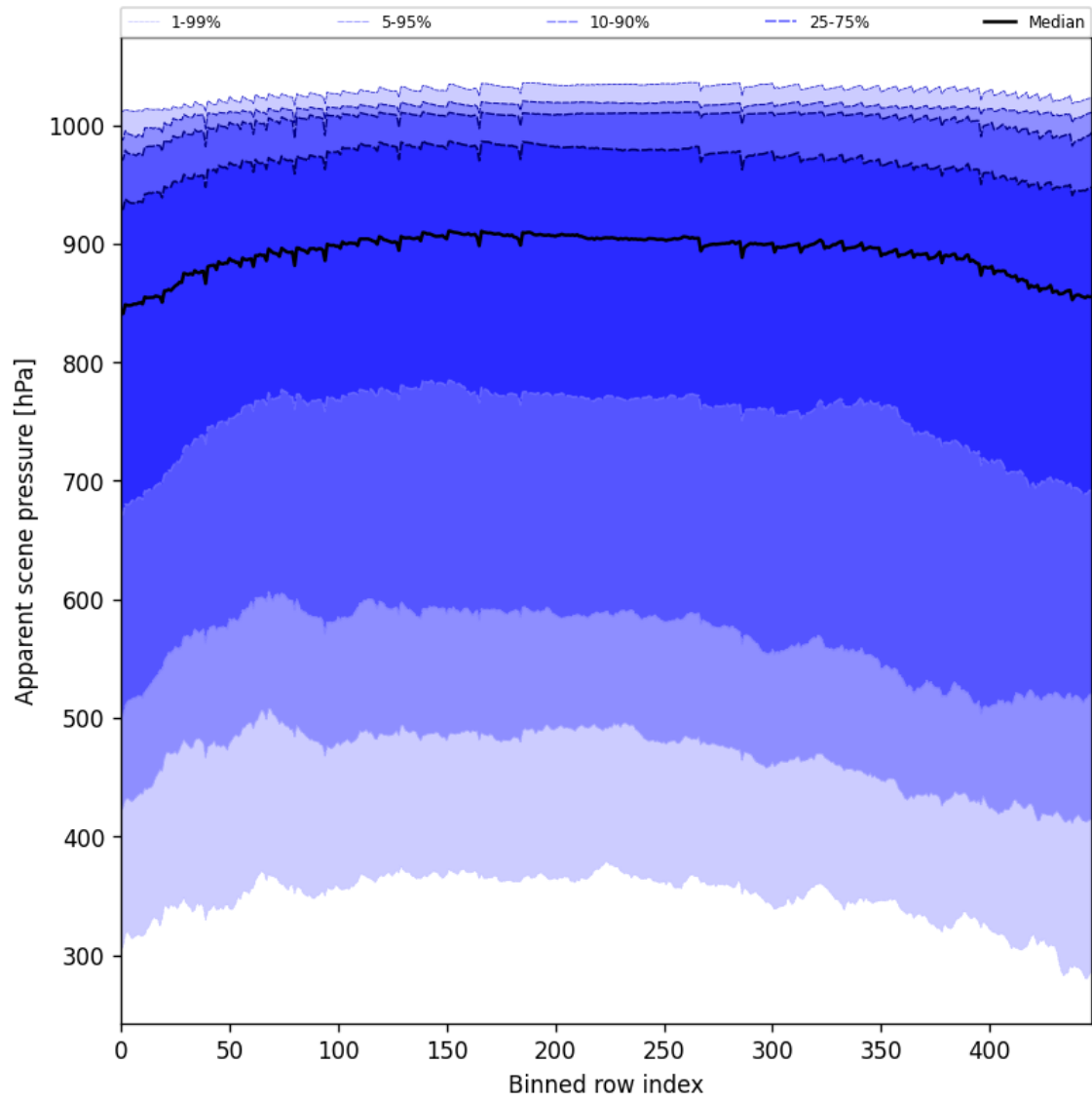
Figure 51: Along track statistics of “Apparent scene pressure” for 2025-04-24 to 2025-04-25
