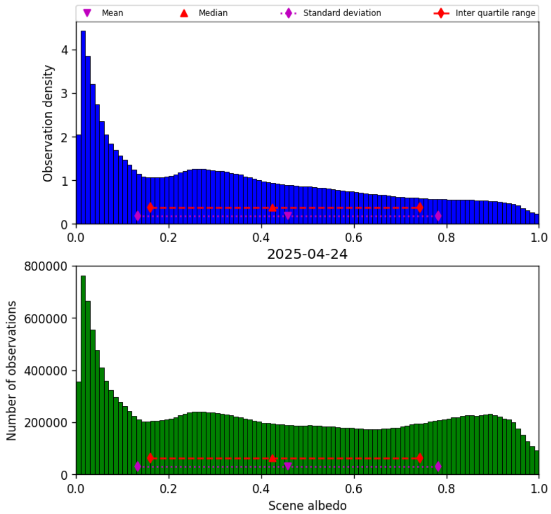
Figure 32: Histogram of “Scene albedo” for 2025-04-24 to 2025-04-25
