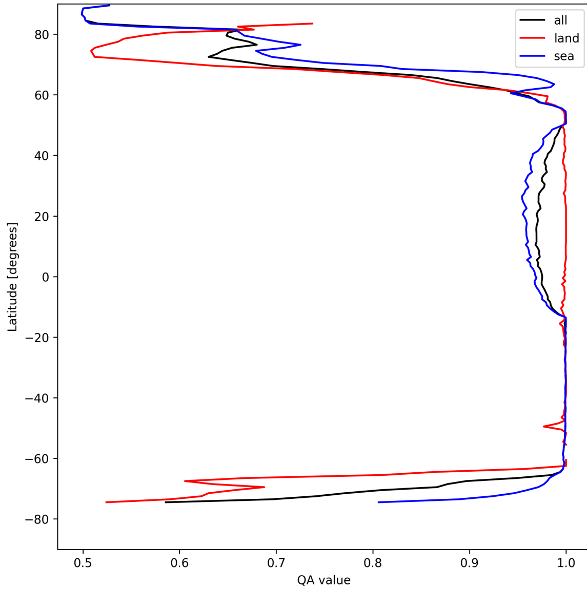
Figure 10: Zonal average of “QA value” for 2025-04-24 to 2025-04-25.
