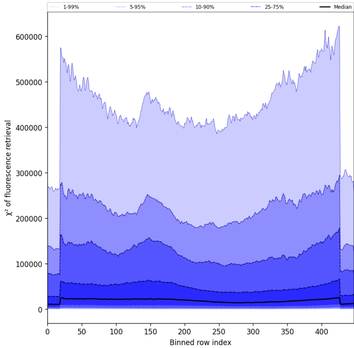
Figure 57: Along track statistics of “ \chi^2 of fluorescence retrieval” for 2025-04-24 to 2025-04-25
