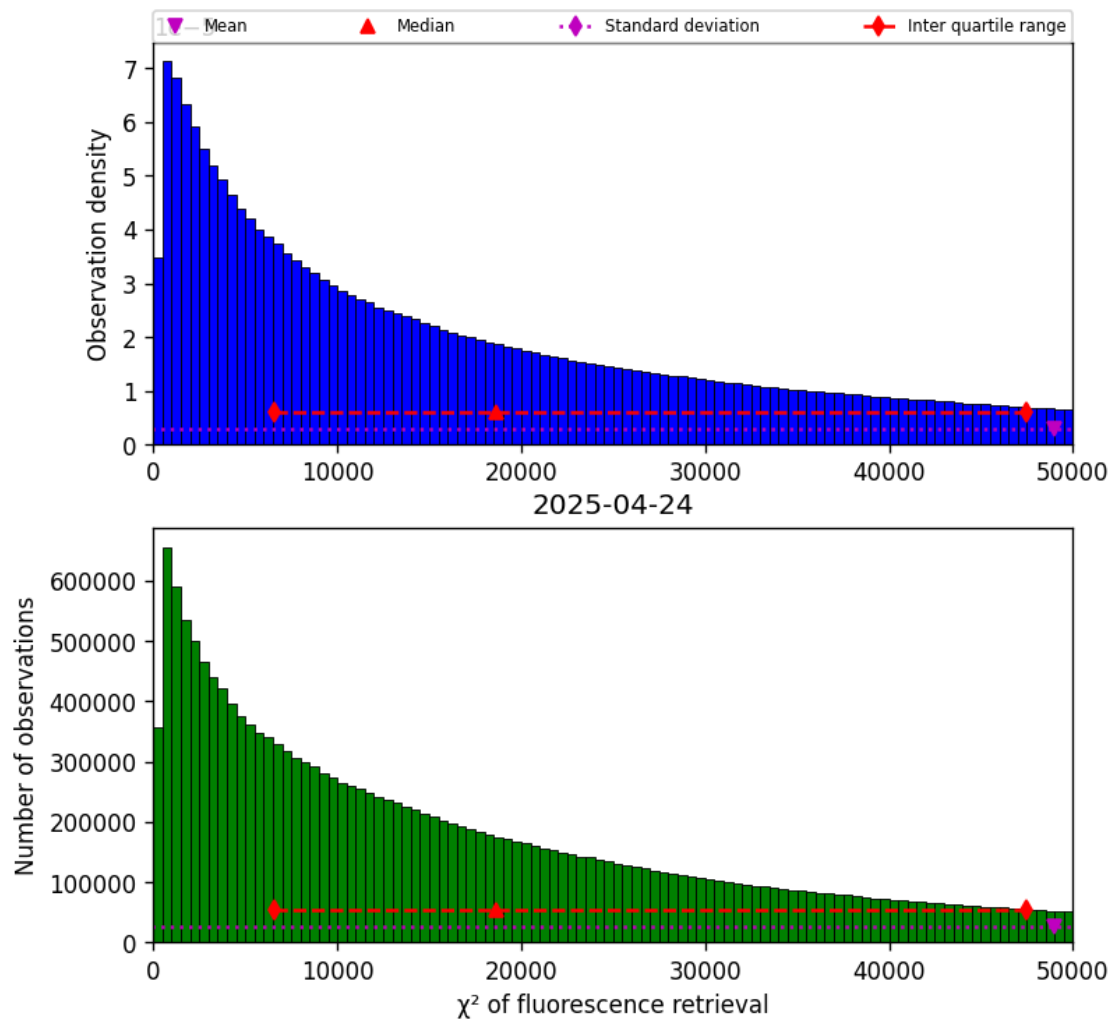
Figure 40: Histogram of “ \chi^2 of fluorescence retrieval” for 2025-04-24 to 2025-04-25
