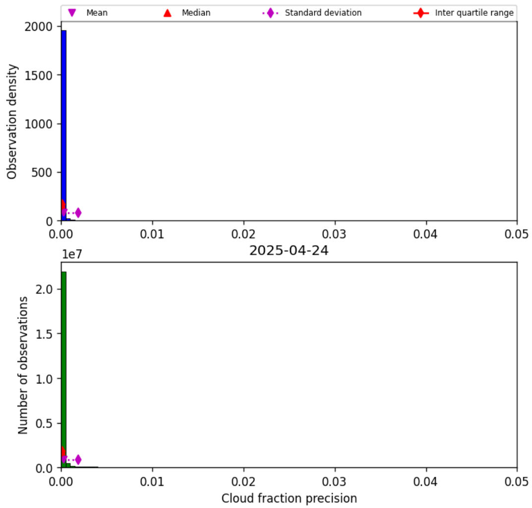
Figure 31: Histogram of “Cloud fraction precision” for 2025-04-24 to 2025-04-25
