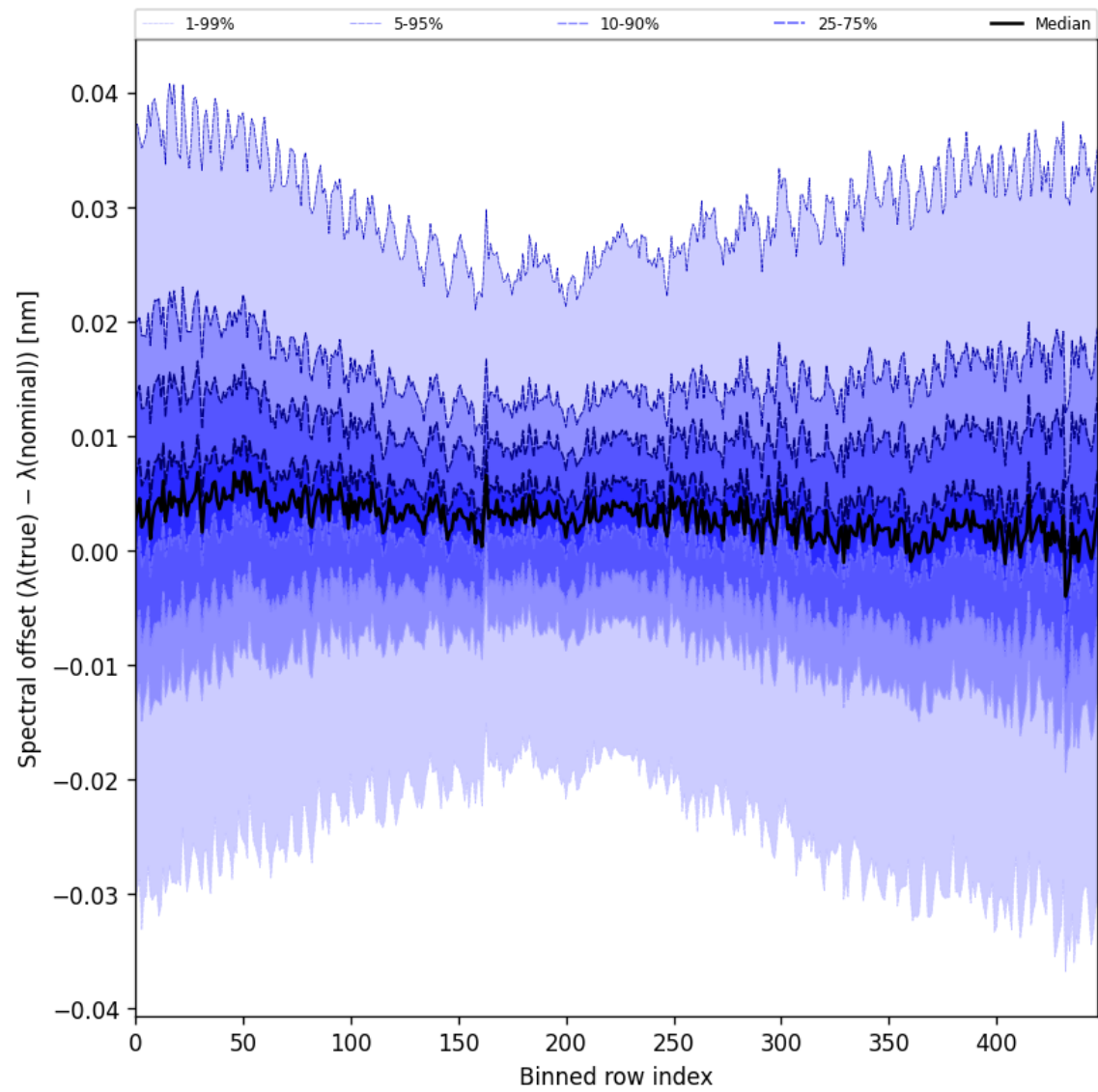
Figure 60: Along track statistics of “Spectral offset ( \lambda_{\text{true}} - \lambda_{\text{nominal}} )” for 2025-04-24 to 2025-04-25
