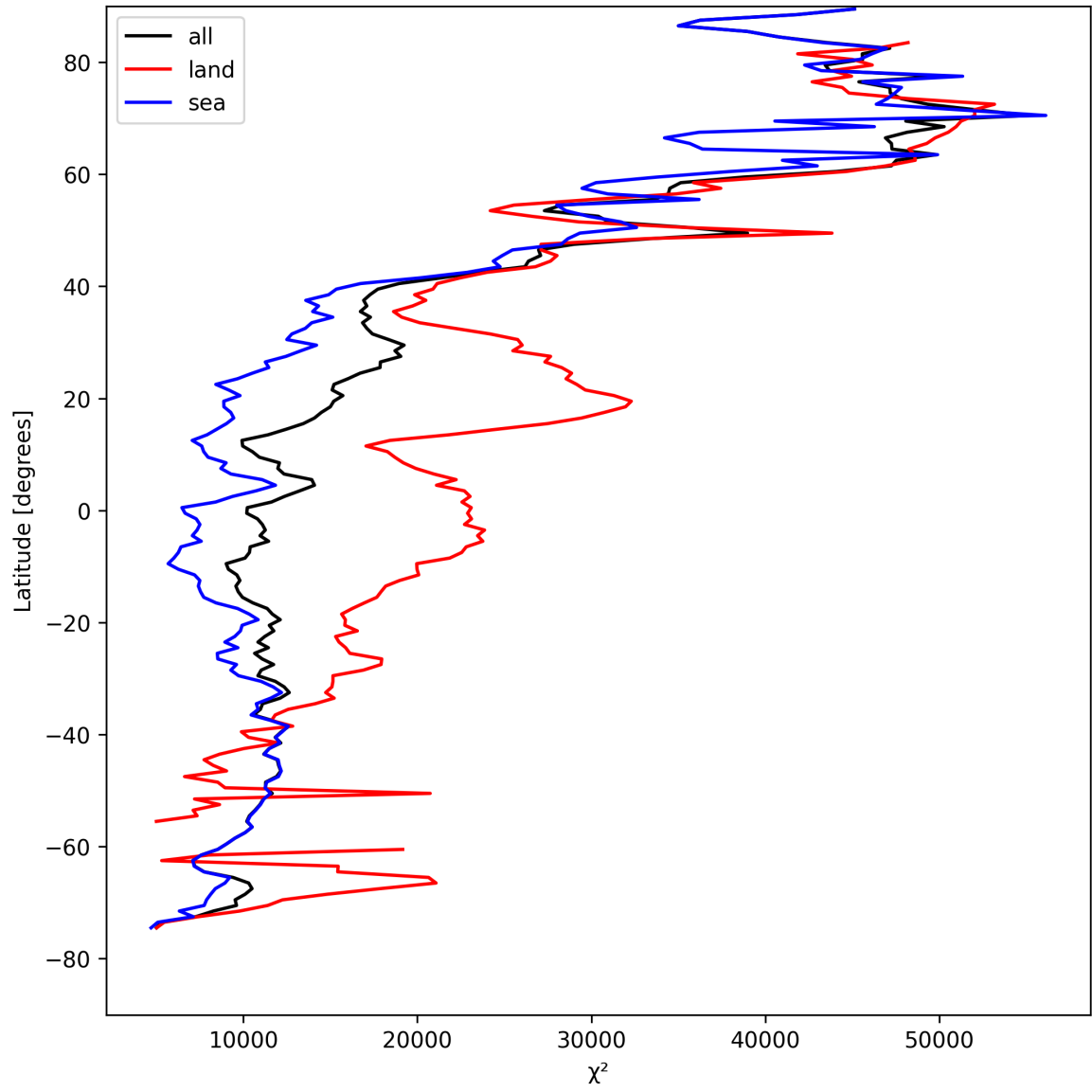
Figure 19: Zonal average of “ \chi^2 ” for 2025-04-24 to 2025-04-25.
