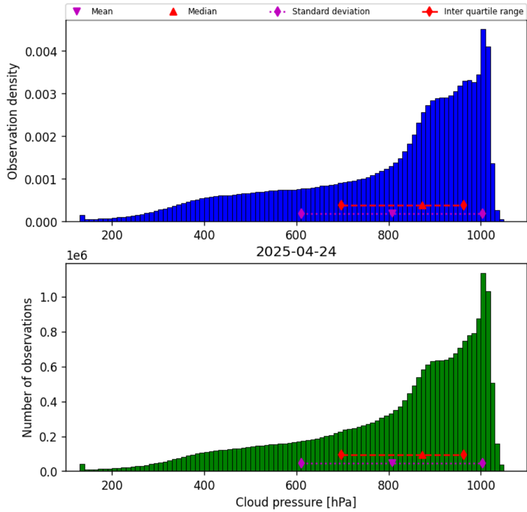
Figure 28: Histogram of “Cloud pressure” for 2025-04-24 to 2025-04-25
