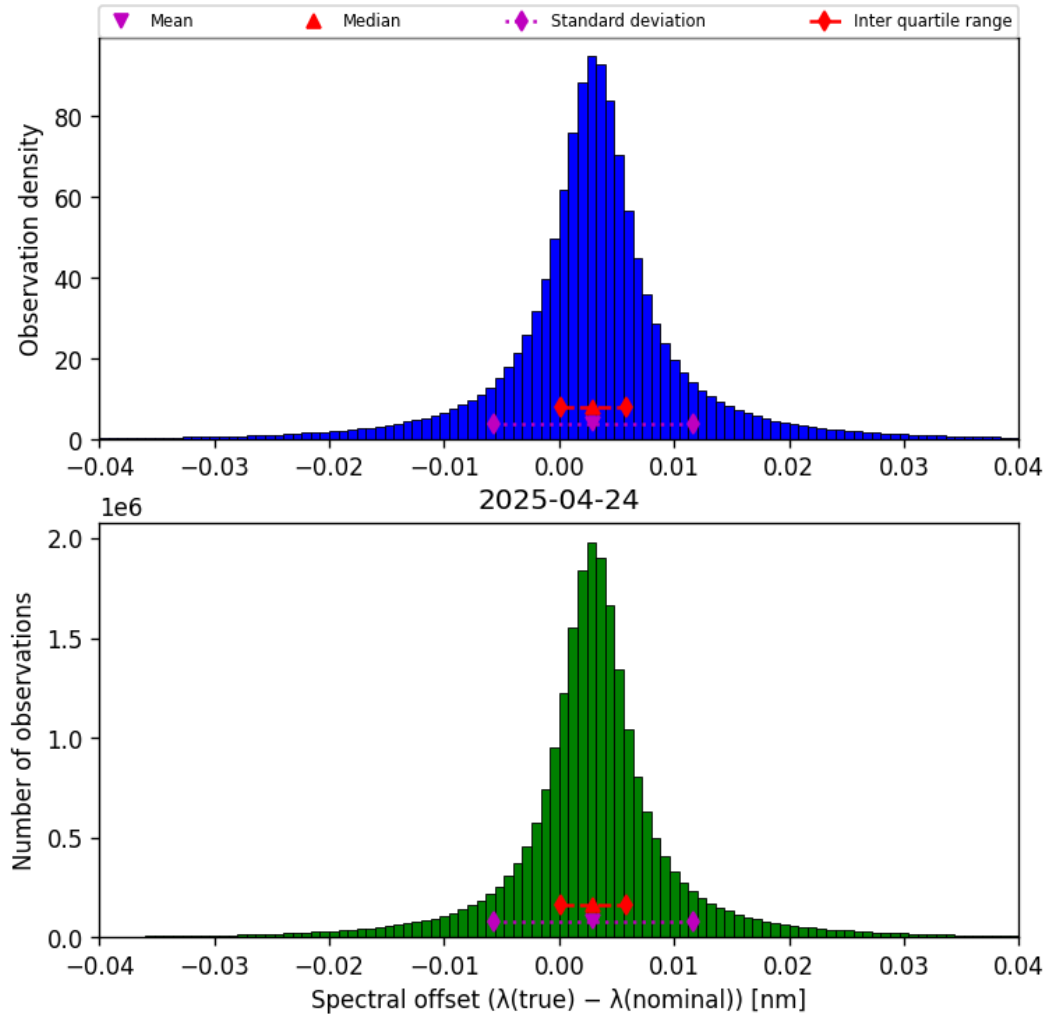
Figure 43: Histogram of “Spectral offset ( \lambda_{\text{true}} - \lambda_{\text{nominal}} )” for 2025-04-24 to 2025-04-25
