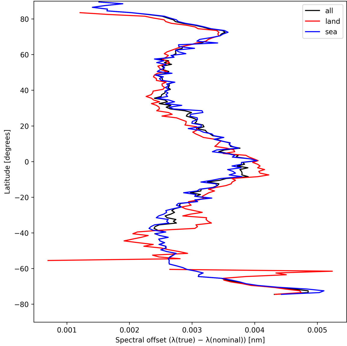
Figure 26: Zonal average of “Spectral offset ( \lambda_{\text{true}} - \lambda_{\text{nominal}} )” for 2025-04-24 to 2025-04-25.
