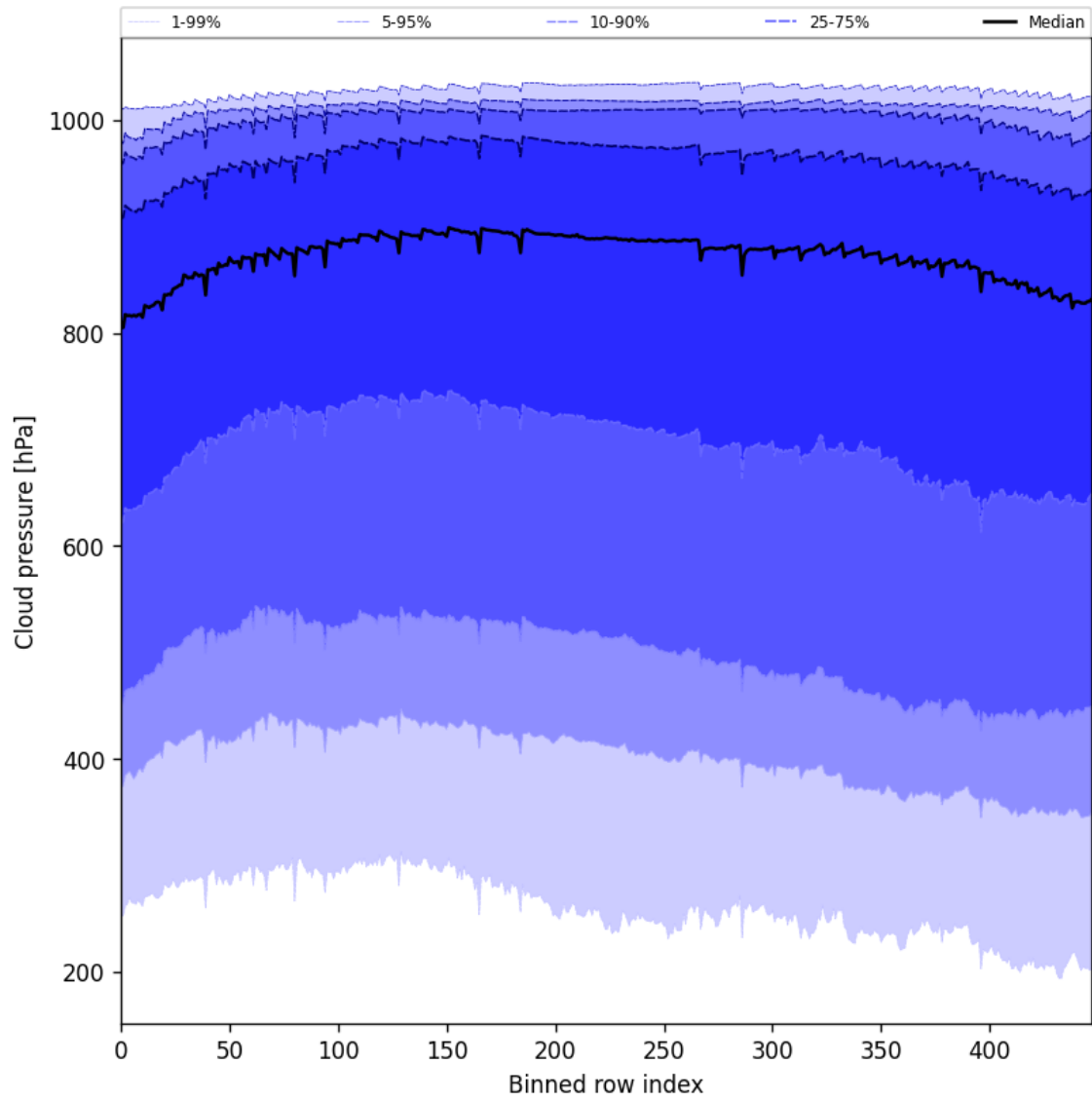
Figure 45: Along track statistics of “Cloud pressure” for 2025-04-24 to 2025-04-25
