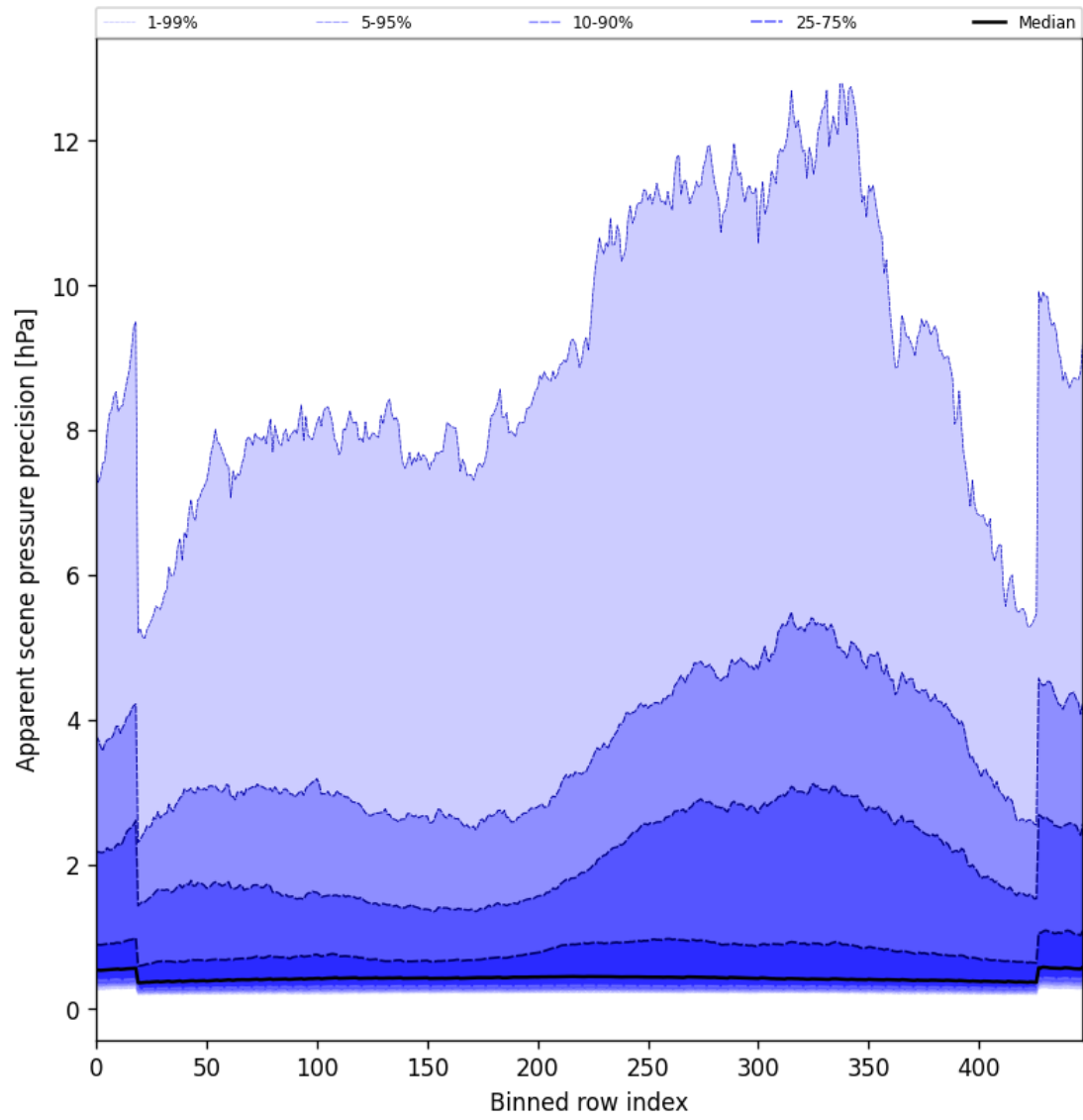
Figure 52: Along track statistics of “Apparent scene pressure precision” for 2025-04-24 to 2025-04-25
