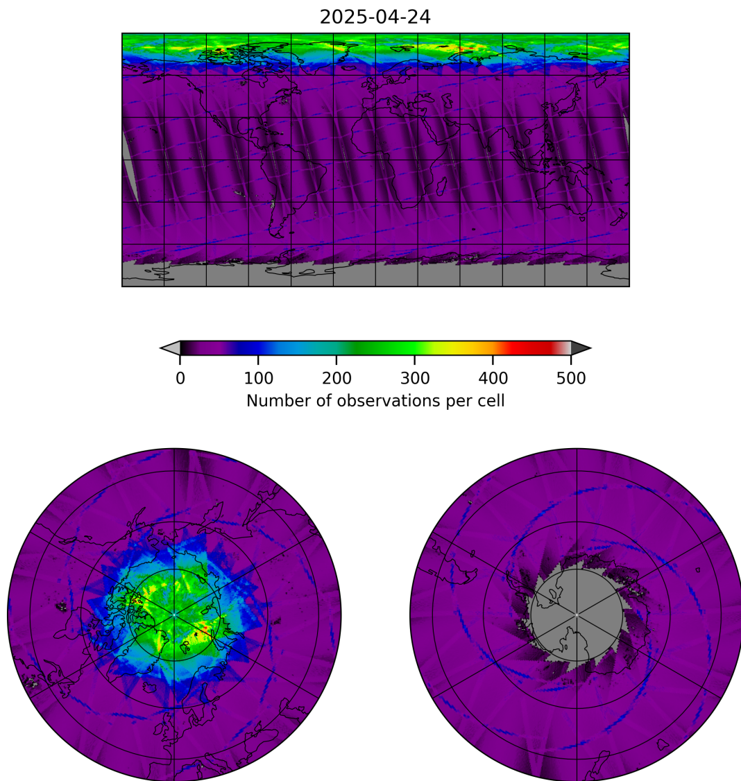
Figure 9: Map of the number of observations for 2025-04-24 to 2025-04-25
