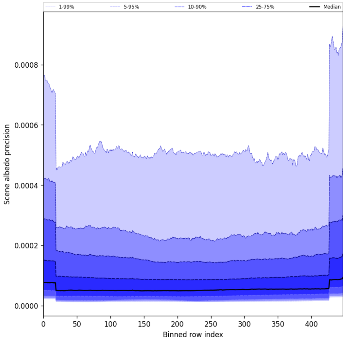
Figure 50: Along track statistics of “Scene albedo precision” for 2025-04-24 to 2025-04-25
