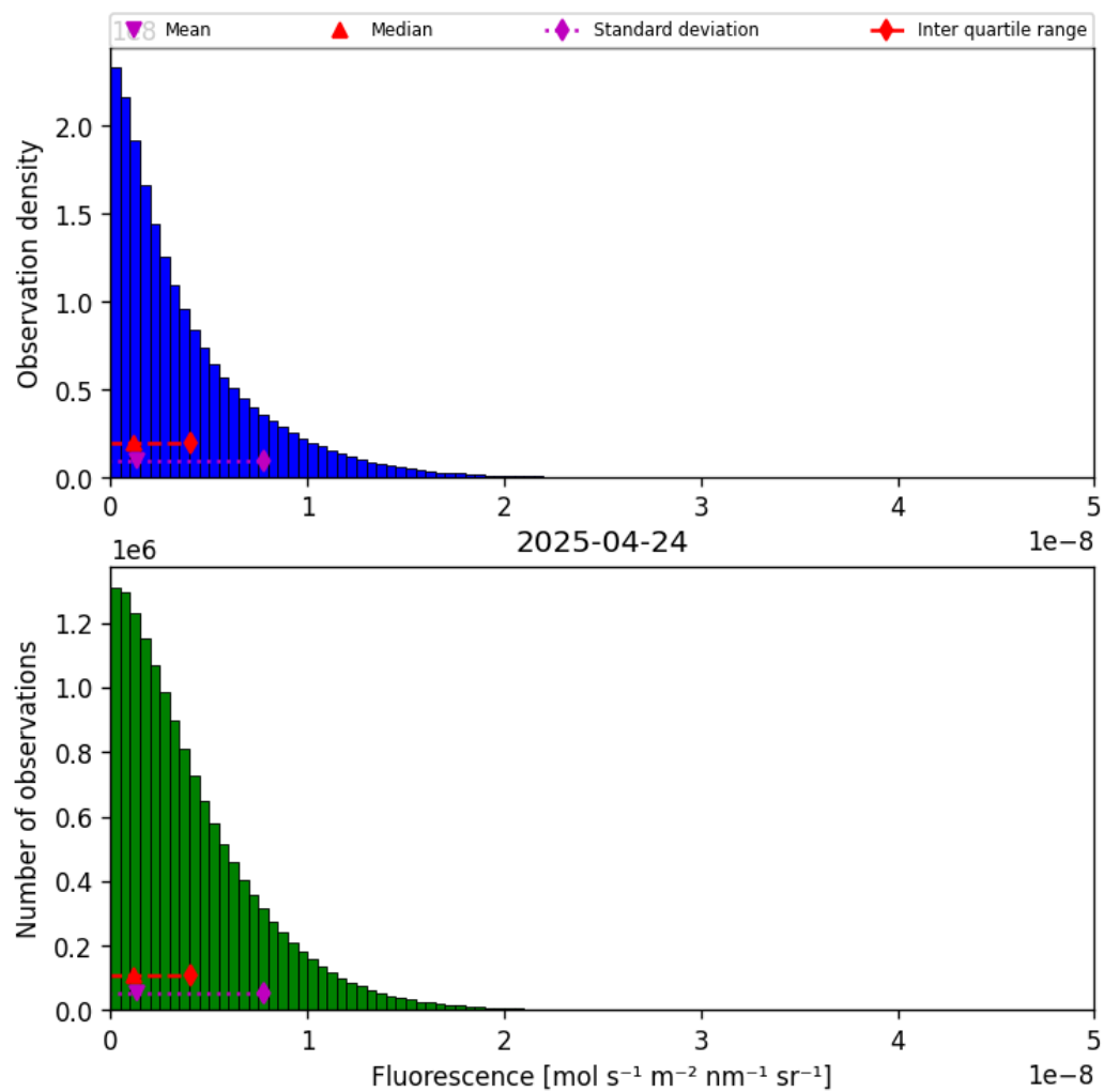
Figure 38: Histogram of “Fluorescence” for 2025-04-24 to 2025-04-25
