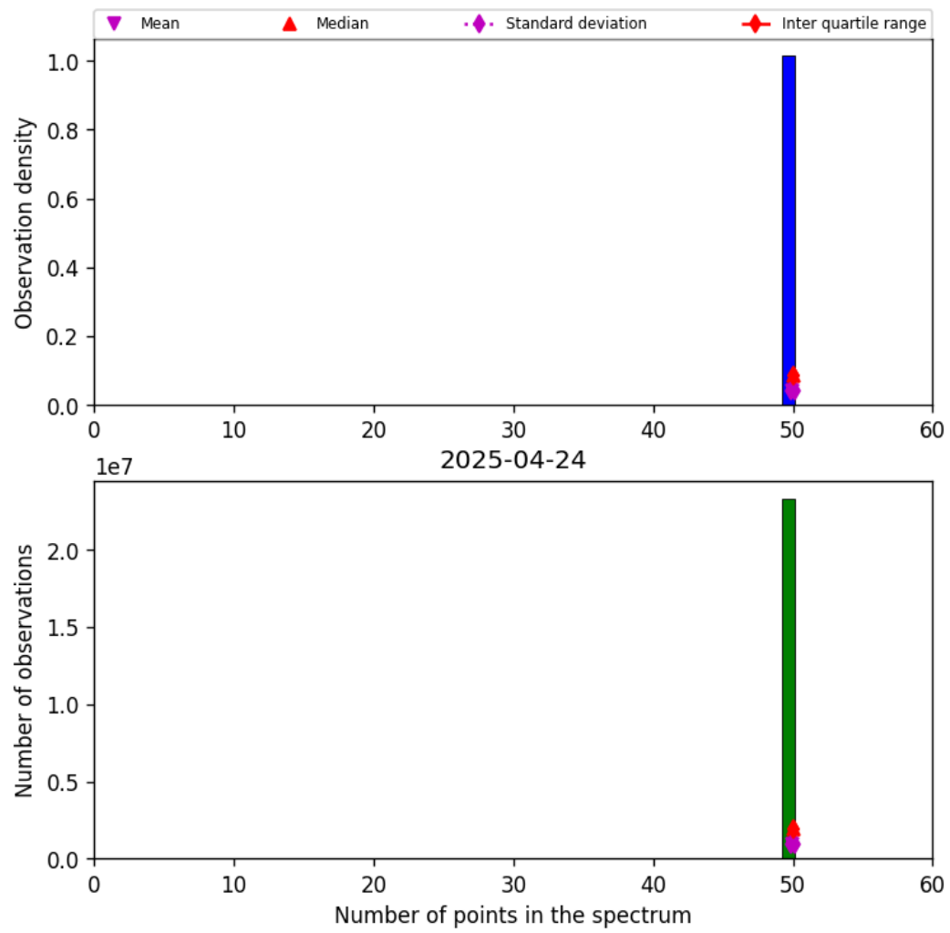
Figure 42: Histogram of “Number of points in the spectrum” for 2025-04-24 to 2025-04-25
