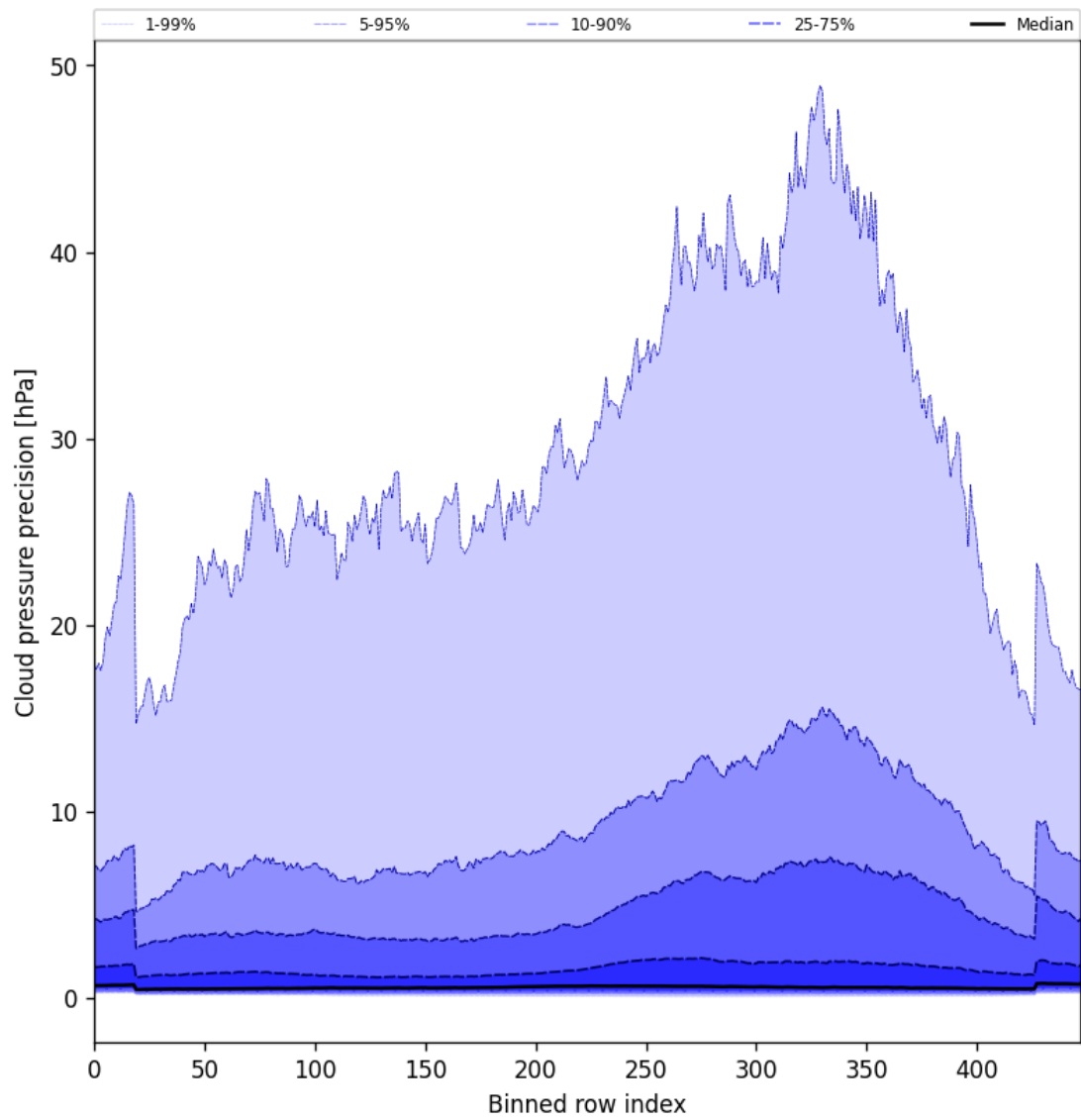
Figure 46: Along track statistics of “Cloud pressure precision” for 2025-04-24 to 2025-04-25
