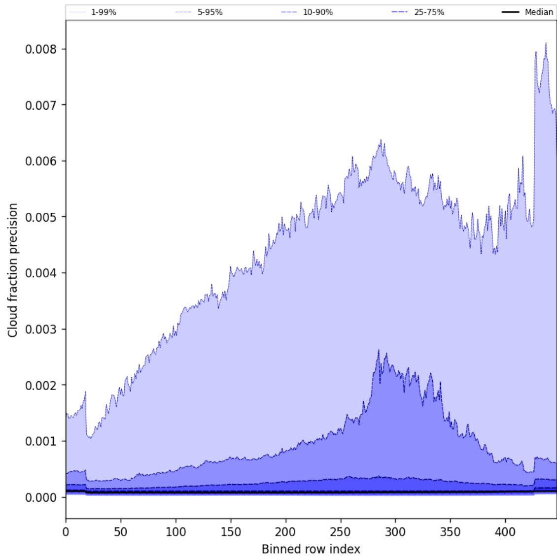
Figure 48: Along track statistics of “Cloud fraction precision” for 2025-04-24 to 2025-04-25
