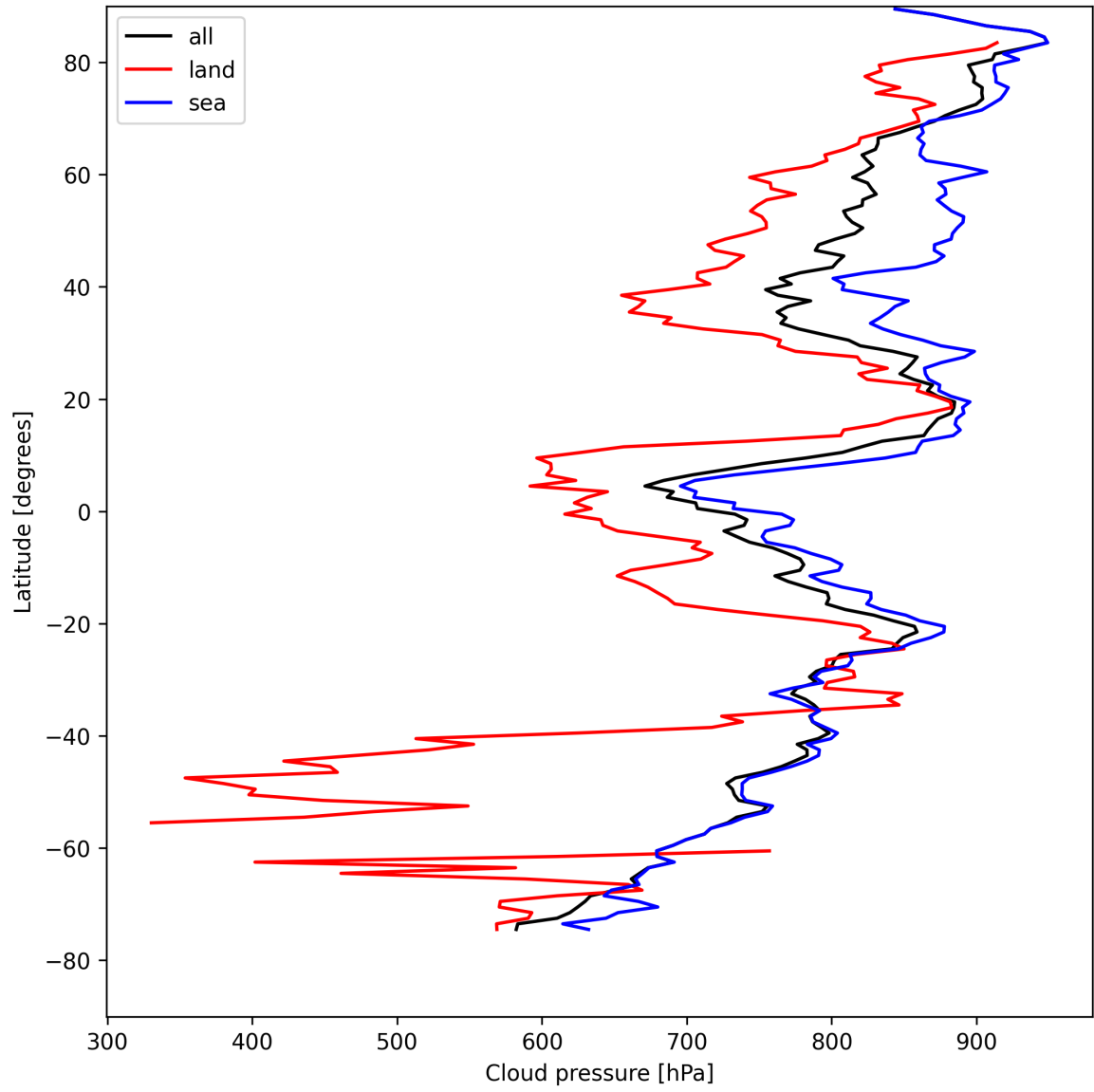
Figure 11: Zonal average of “Cloud pressure” for 2025-04-24 to 2025-04-25.
