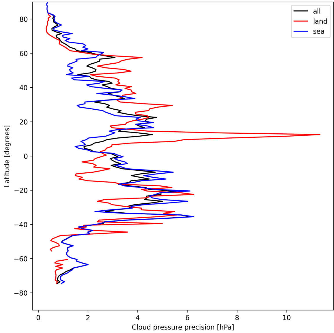
Figure 12: Zonal average of “Cloud pressure precision” for 2025-04-24 to 2025-04-25.
