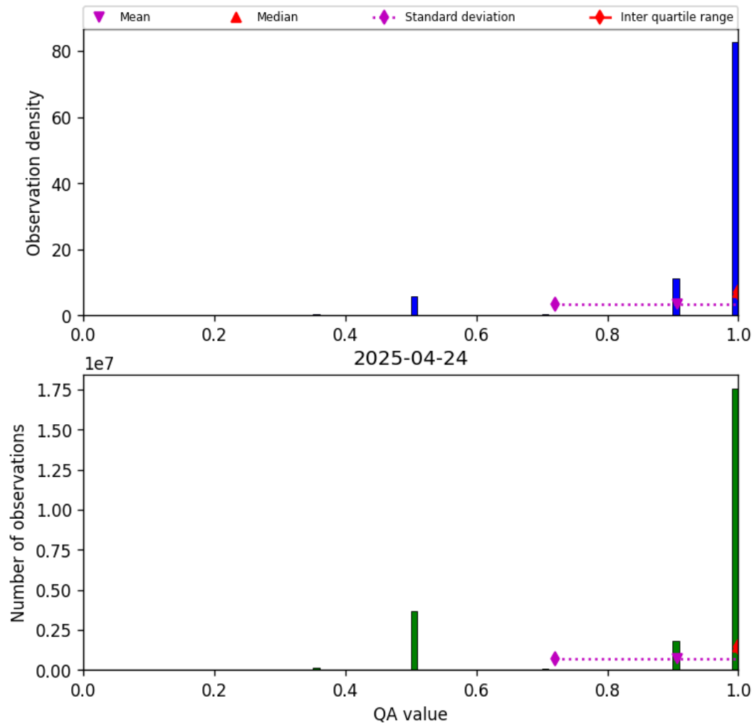
Figure 27: Histogram of “QA value” for 2025-04-24 to 2025-04-25
