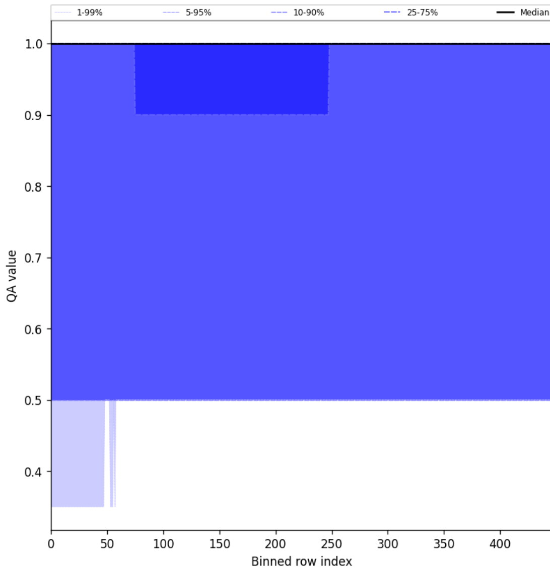
Figure 44: Along track statistics of “QA value” for 2025-04-24 to 2025-04-25
