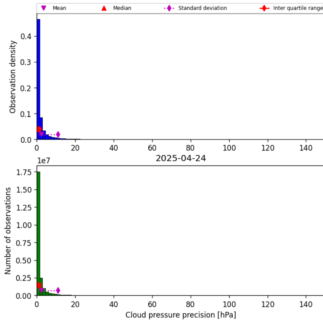
Figure 29: Histogram of “Cloud pressure precision” for 2025-04-24 to 2025-04-25
