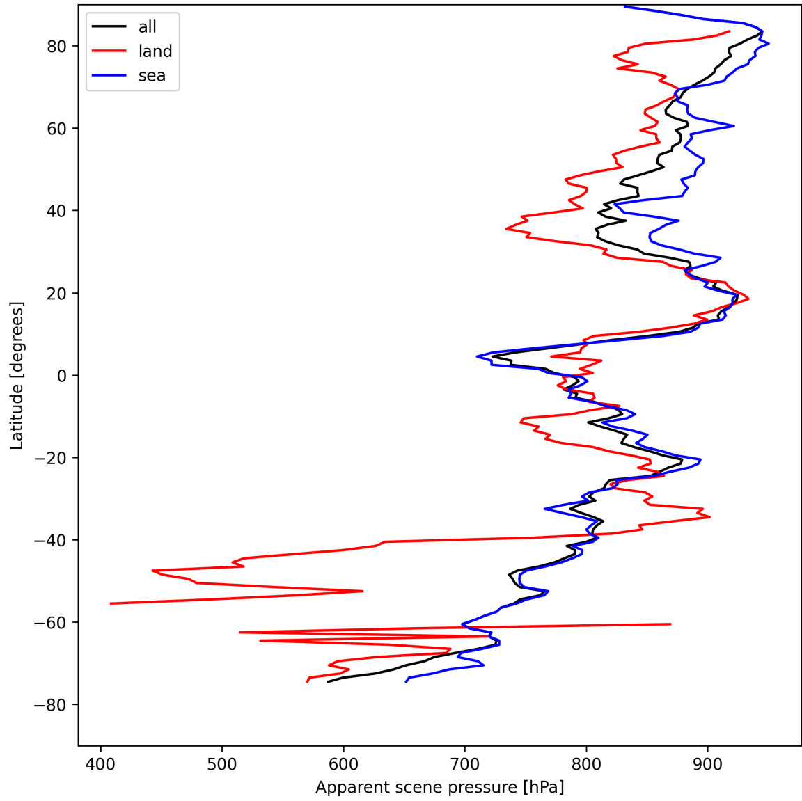
Figure 17: Zonal average of “Apparent scene pressure” for 2025-04-24 to 2025-04-25.
