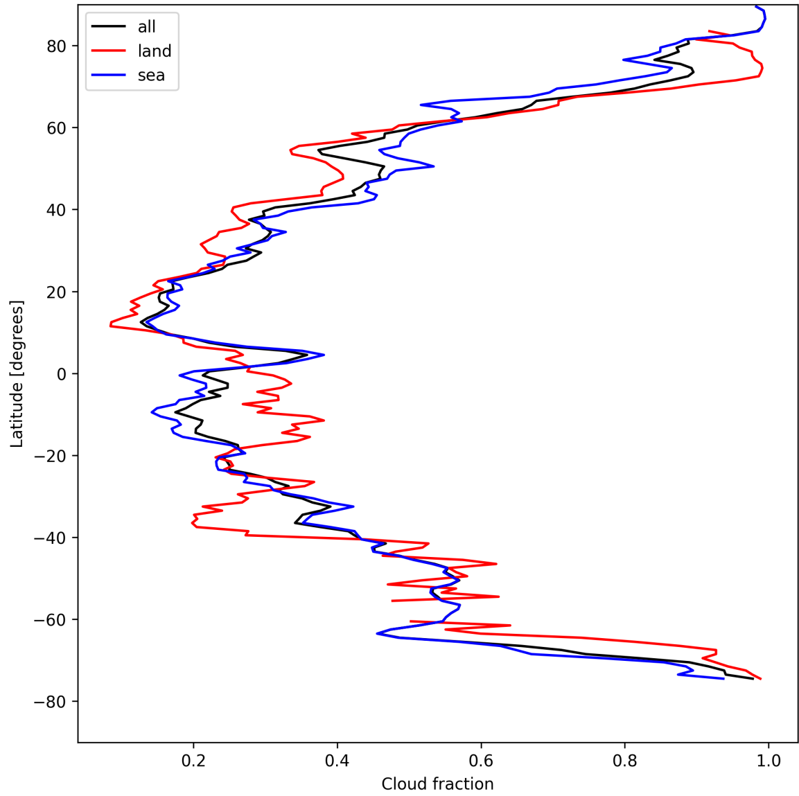
Figure 13: Zonal average of “Cloud fraction” for 2025-04-24 to 2025-04-25.
