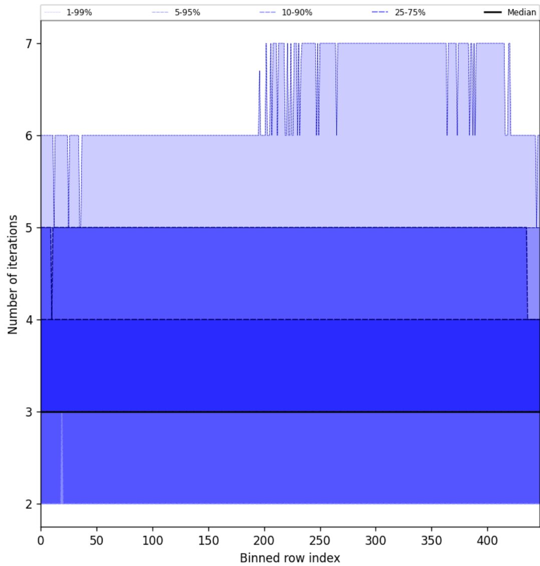
Figure 54: Along track statistics of “Number of iterations” for 2025-04-24 to 2025-04-25
