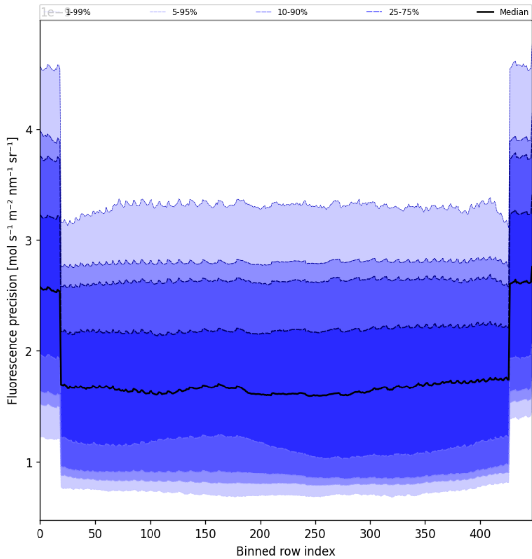
Figure 56: Along track statistics of “Fluorescence precision” for 2025-04-24 to 2025-04-25
