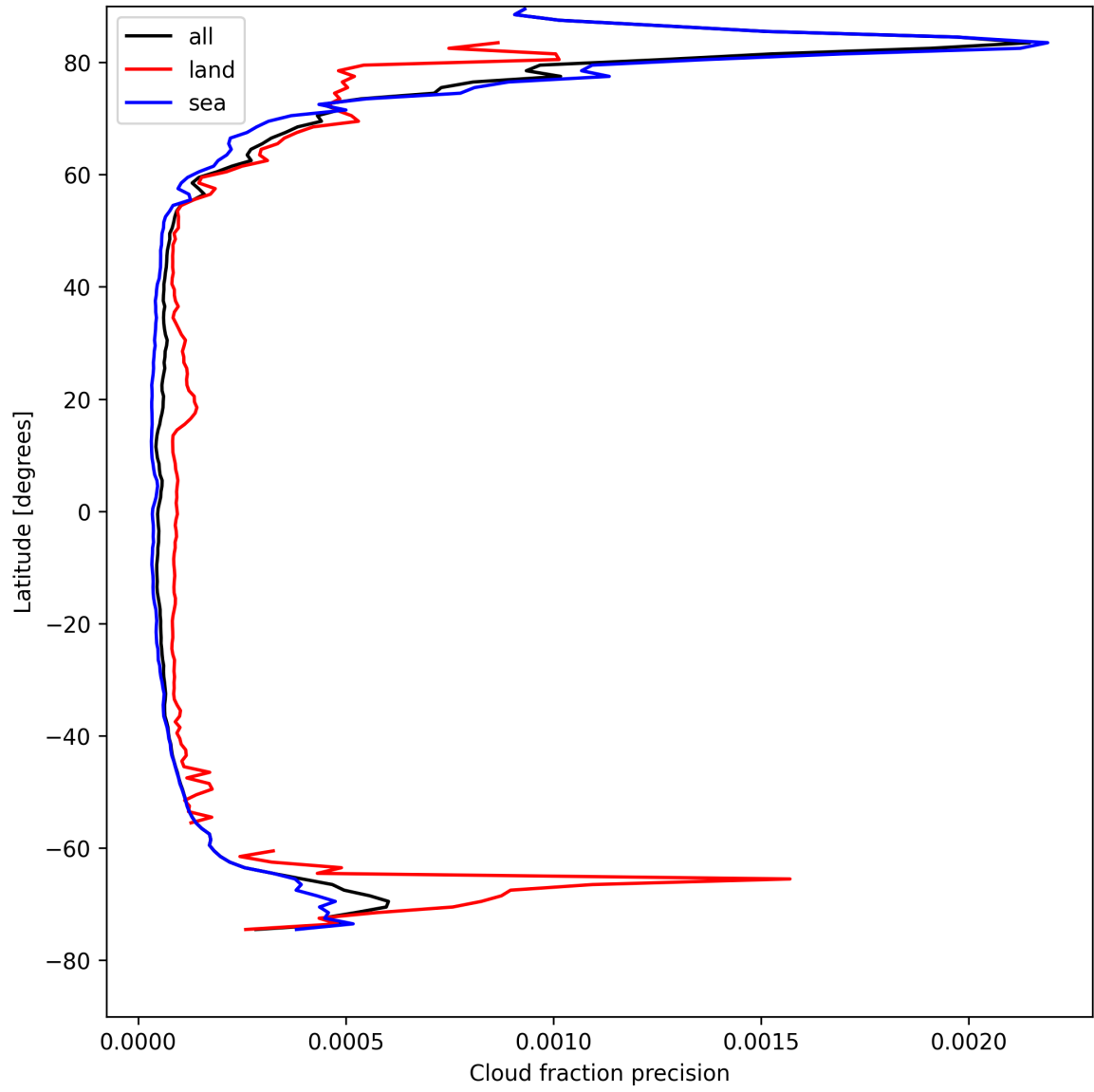
Figure 14: Zonal average of “Cloud fraction precision” for 2025-04-24 to 2025-04-25.
