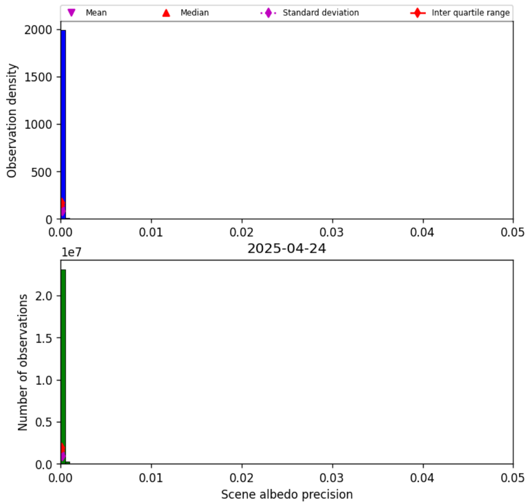
Figure 33: Histogram of “Scene albedo precision” for 2025-04-24 to 2025-04-25
