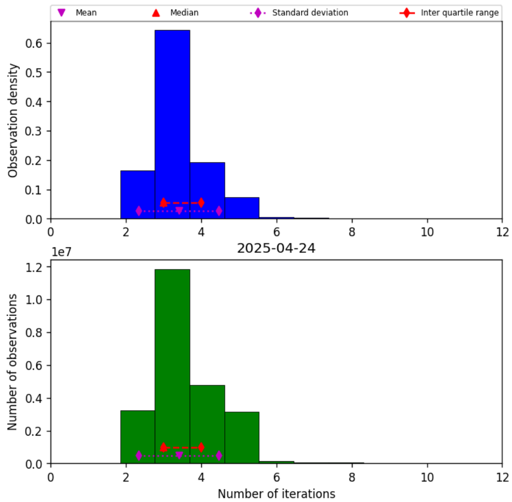
Figure 37: Histogram of “Number of iterations” for 2025-04-24 to 2025-04-25
