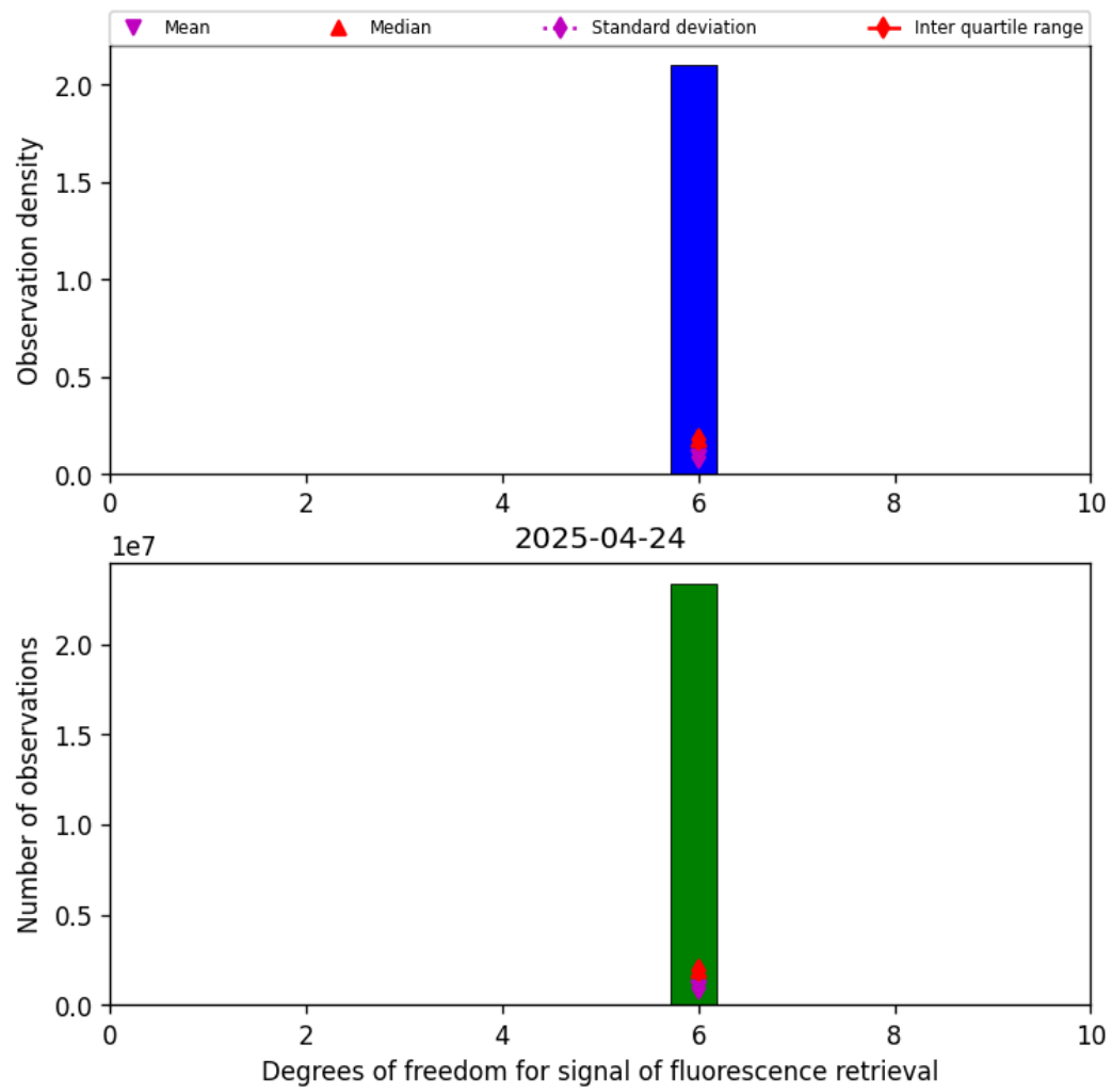
Figure 41: Histogram of “Degrees of freedom for signal of fluorescence retrieval” for 2025-04-24 to 2025-04-25
