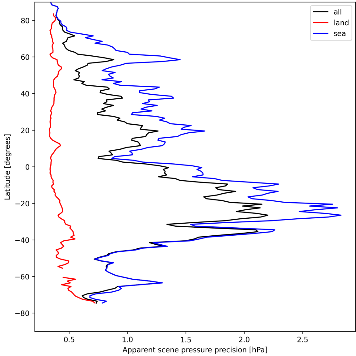
Figure 18: Zonal average of “Apparent scene pressure precision” for 2025-04-24 to 2025-04-25.
