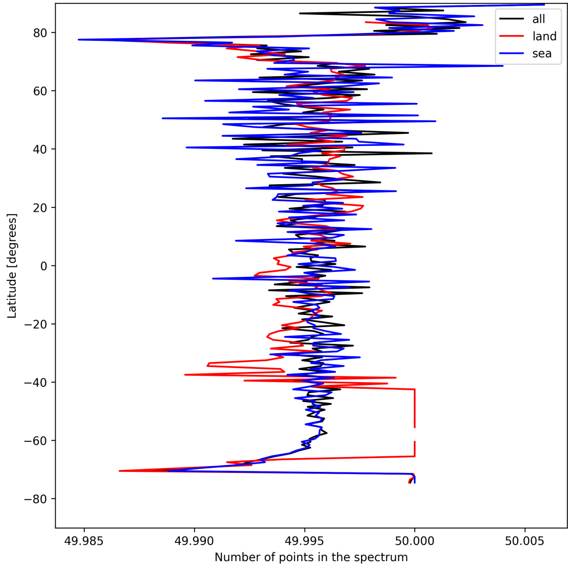
Figure 25: Zonal average of “Number of points in the spectrum” for 2025-04-24 to 2025-04-25.
