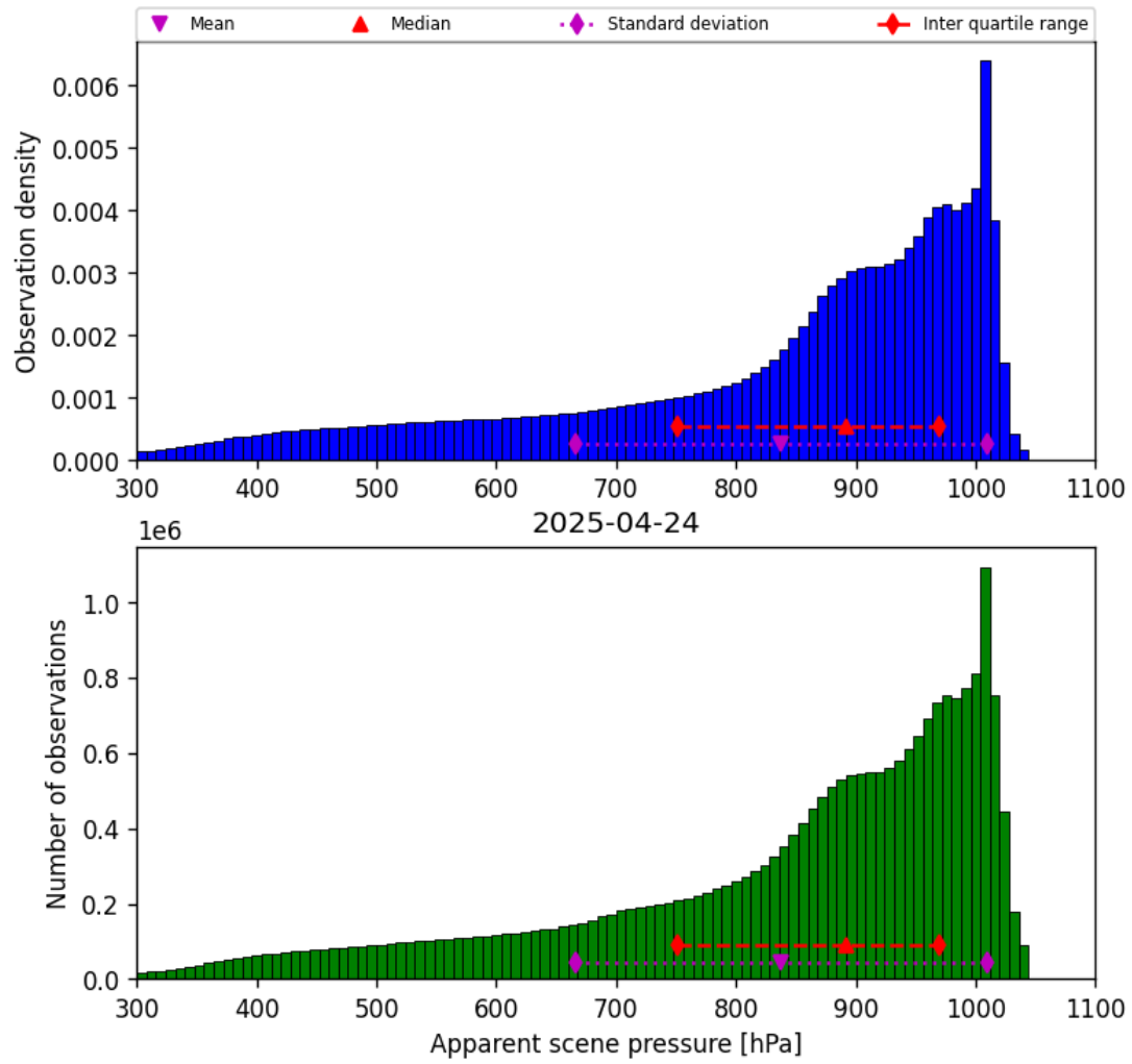
Figure 34: Histogram of “Apparent scene pressure” for 2025-04-24 to 2025-04-25
