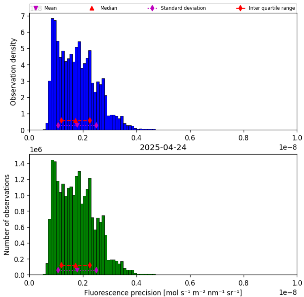
Figure 39: Histogram of “Fluorescence precision” for 2025-04-24 to 2025-04-25
