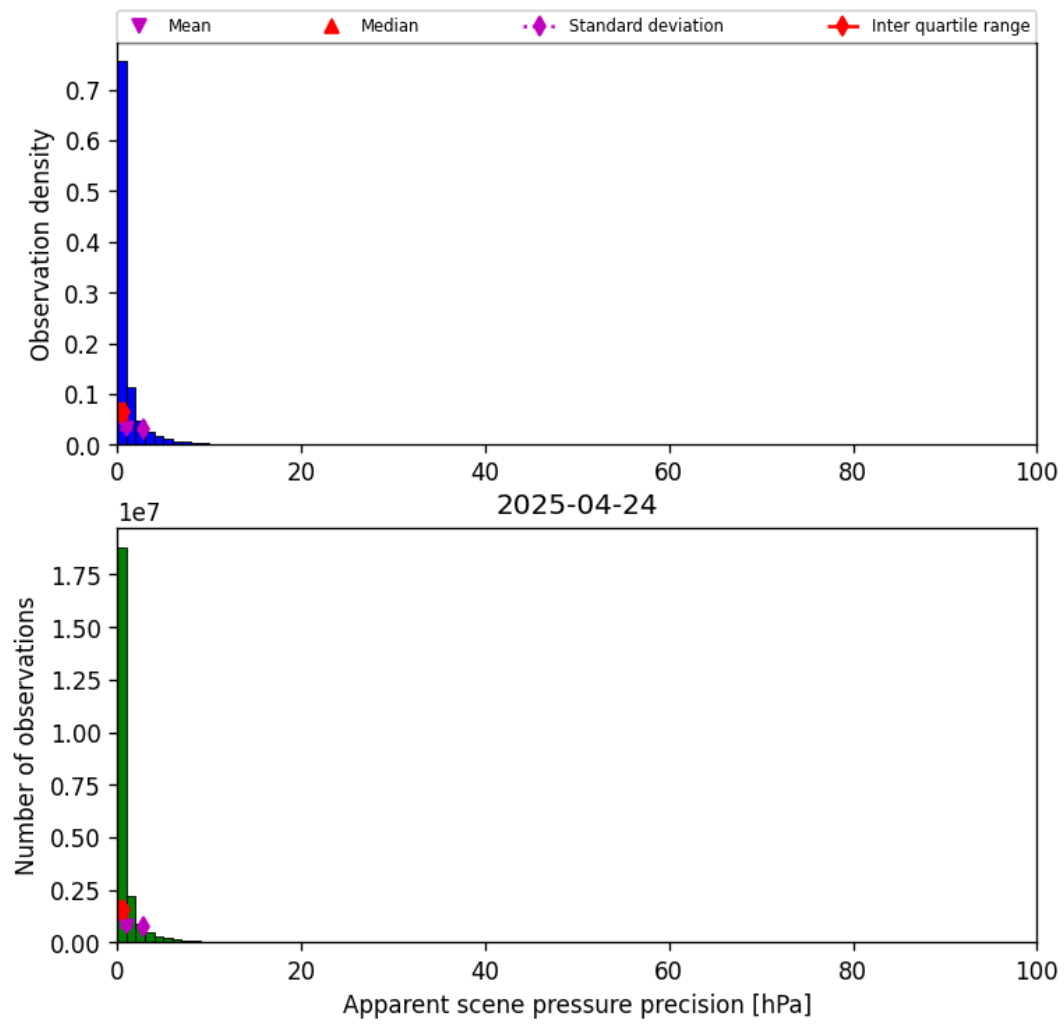
Figure 35: Histogram of “Apparent scene pressure precision” for 2025-04-24 to 2025-04-25
