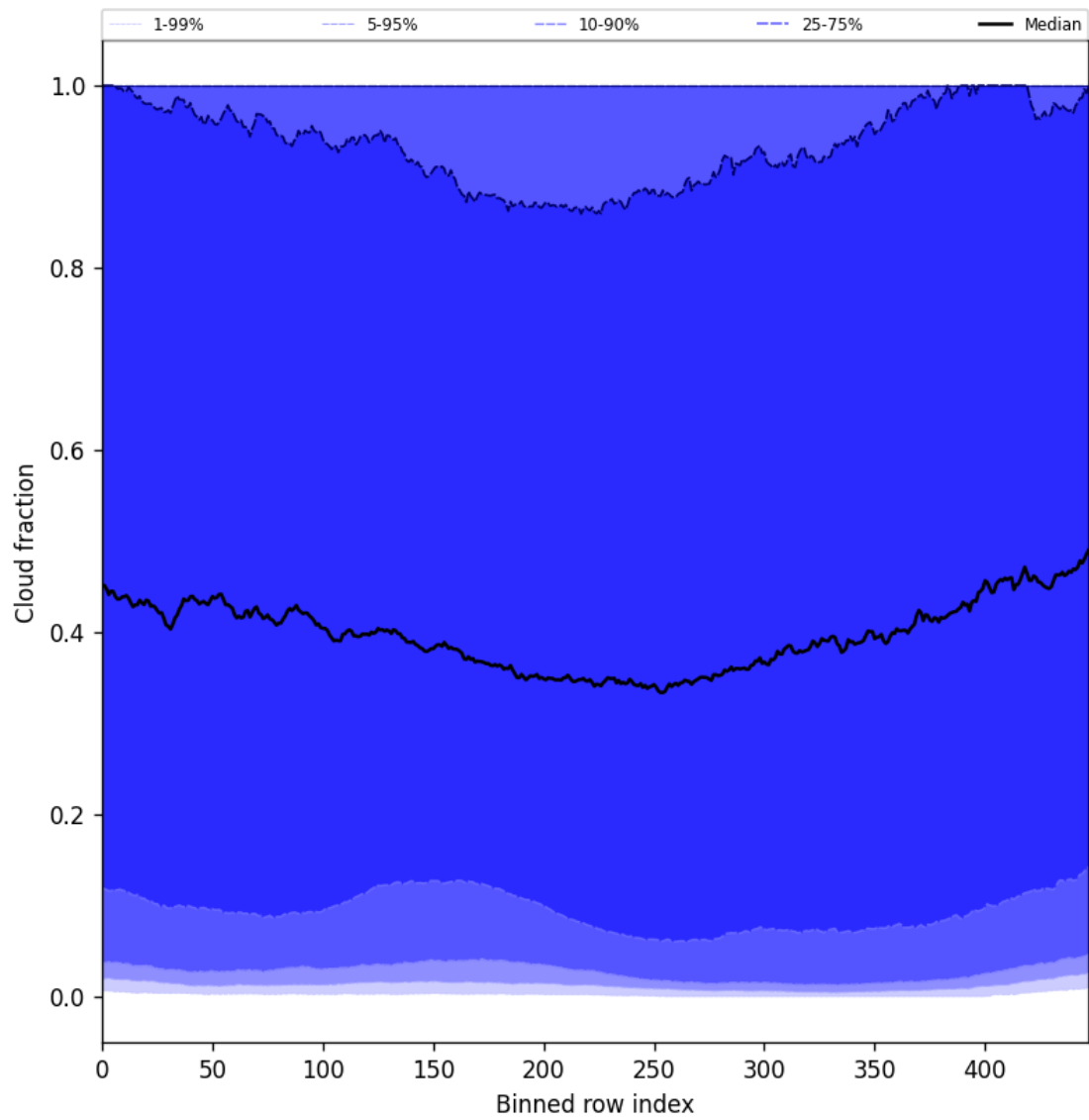
Figure 47: Along track statistics of “Cloud fraction” for 2025-04-24 to 2025-04-25
