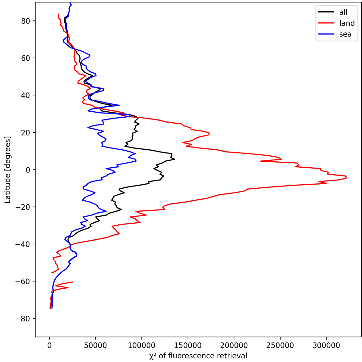
Figure 23: Zonal average of “ \chi^2 of fluorescence retrieval” for 2025-04-24 to 2025-04-25.
