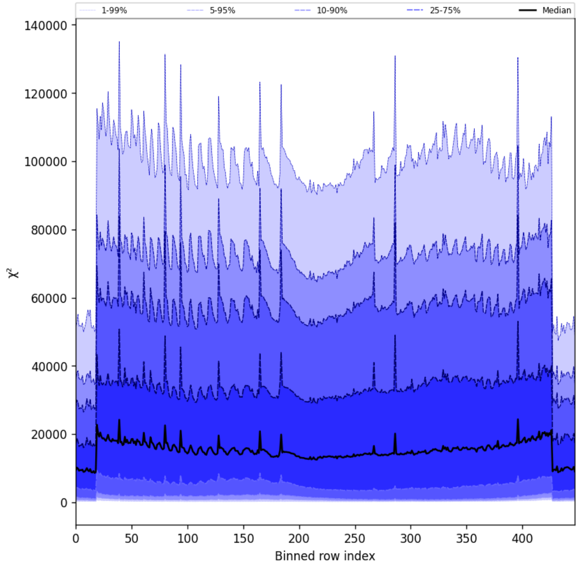
Figure 53: Along track statistics of “ \chi^2 ” for 2025-04-24 to 2025-04-25
