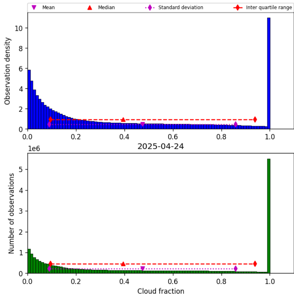
Figure 30: Histogram of “Cloud fraction” for 2025-04-24 to 2025-04-25
