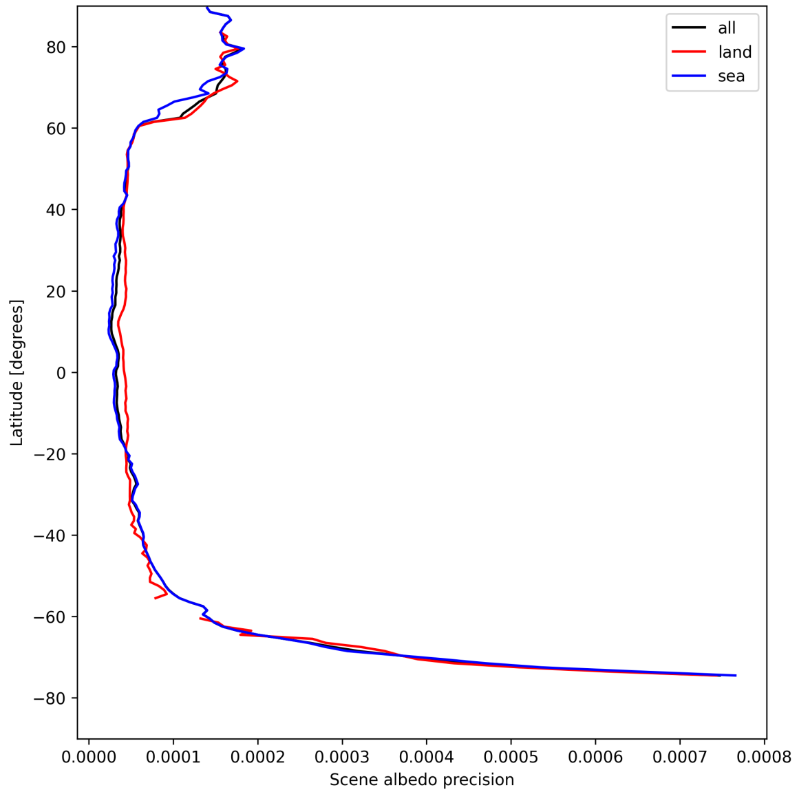
Figure 16: Zonal average of “Scene albedo precision” for 2025-04-24 to 2025-04-25.
