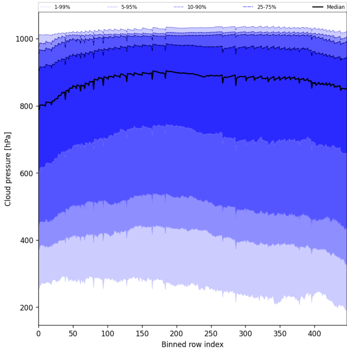
Figure 45: Along track statistics of “Cloud pressure” for 2025-04-26 to 2025-04-27
