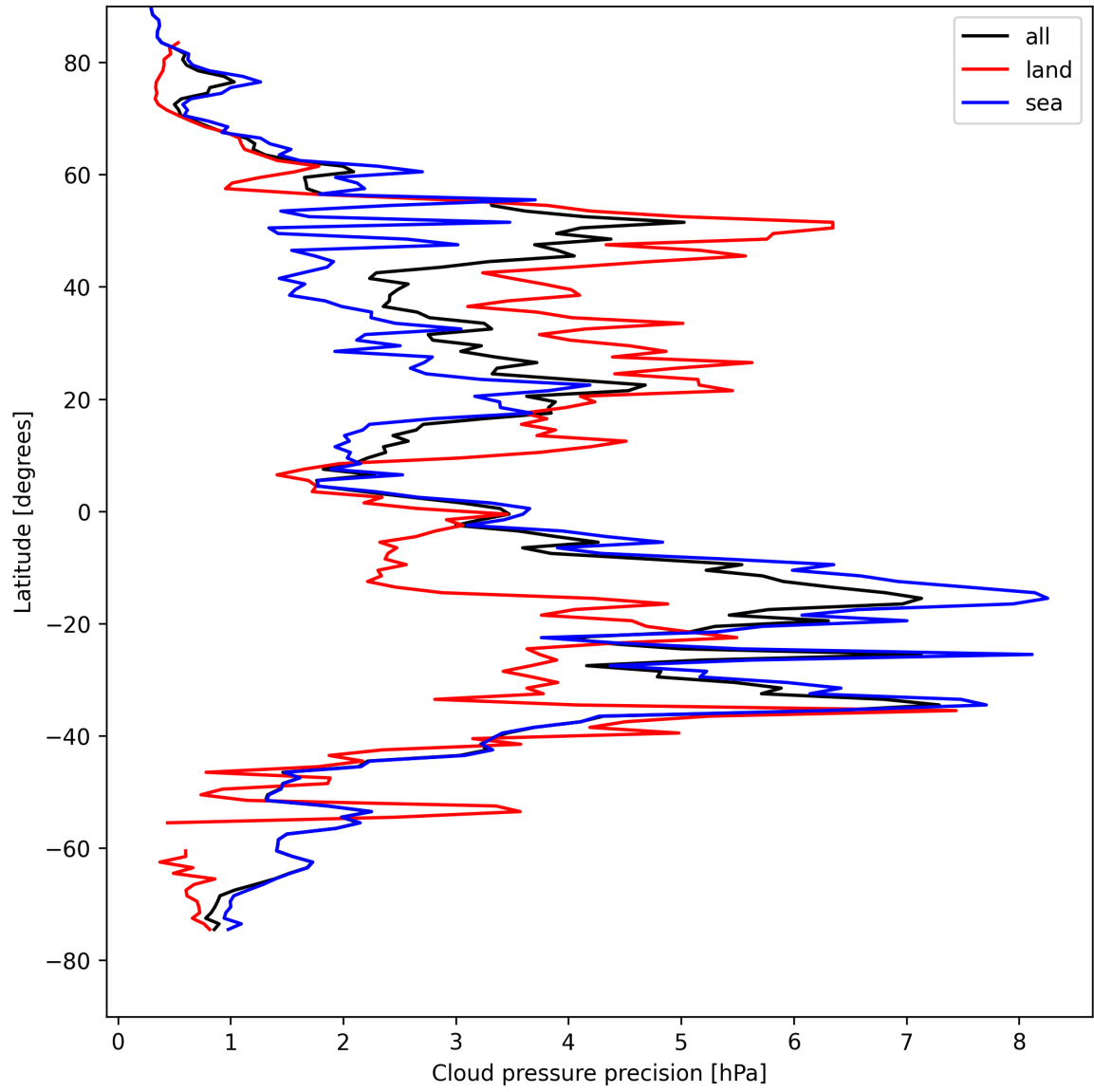
Figure 12: Zonal average of “Cloud pressure precision” for 2025-04-26 to 2025-04-27.
