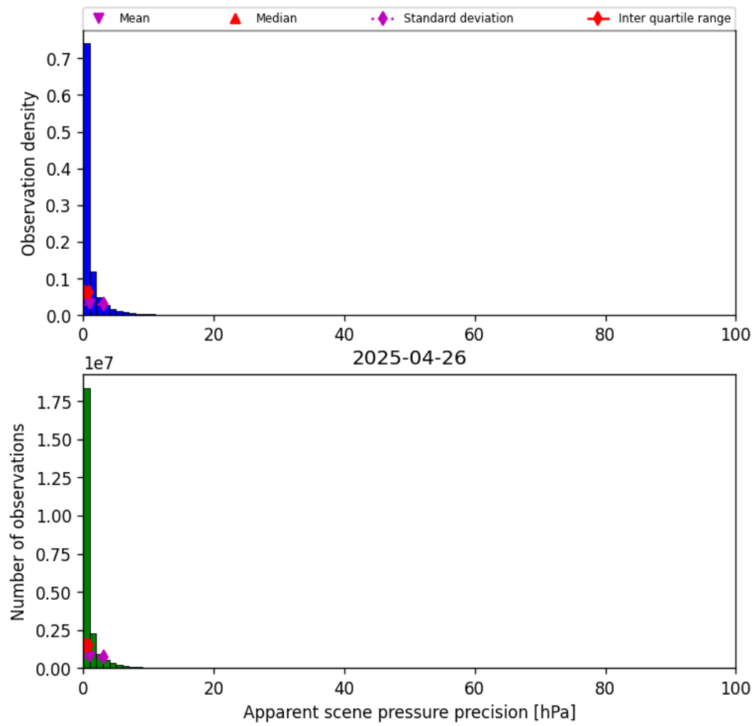
Figure 35: Histogram of “Apparent scene pressure precision” for 2025-04-26 to 2025-04-27
