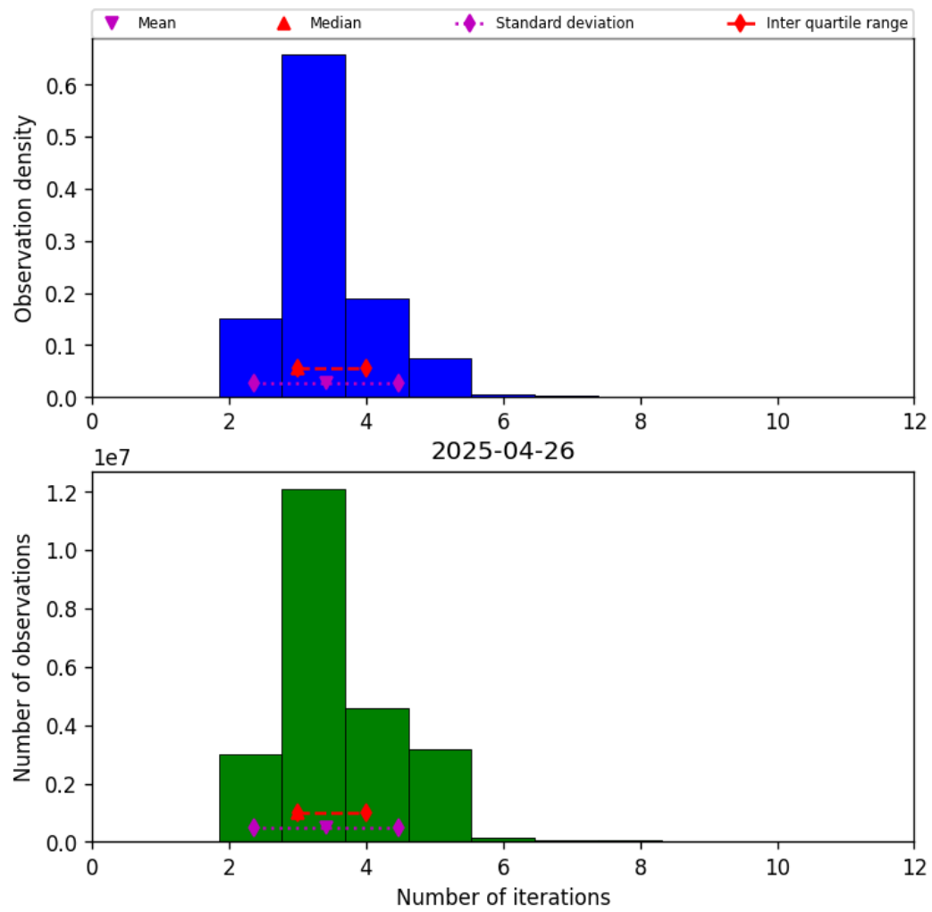
Figure 37: Histogram of “Number of iterations” for 2025-04-26 to 2025-04-27
