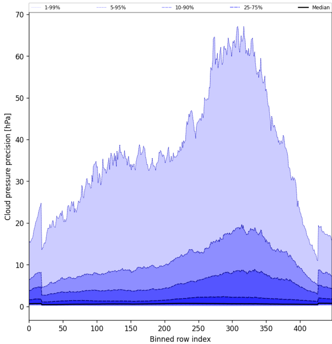
Figure 46: Along track statistics of “Cloud pressure precision” for 2025-04-26 to 2025-04-27
