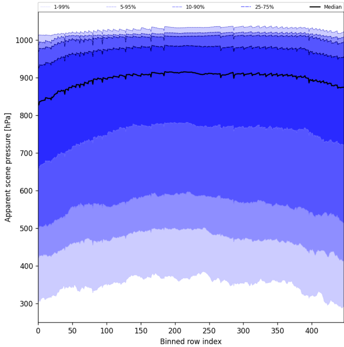
Figure 51: Along track statistics of “Apparent scene pressure” for 2025-04-26 to 2025-04-27
