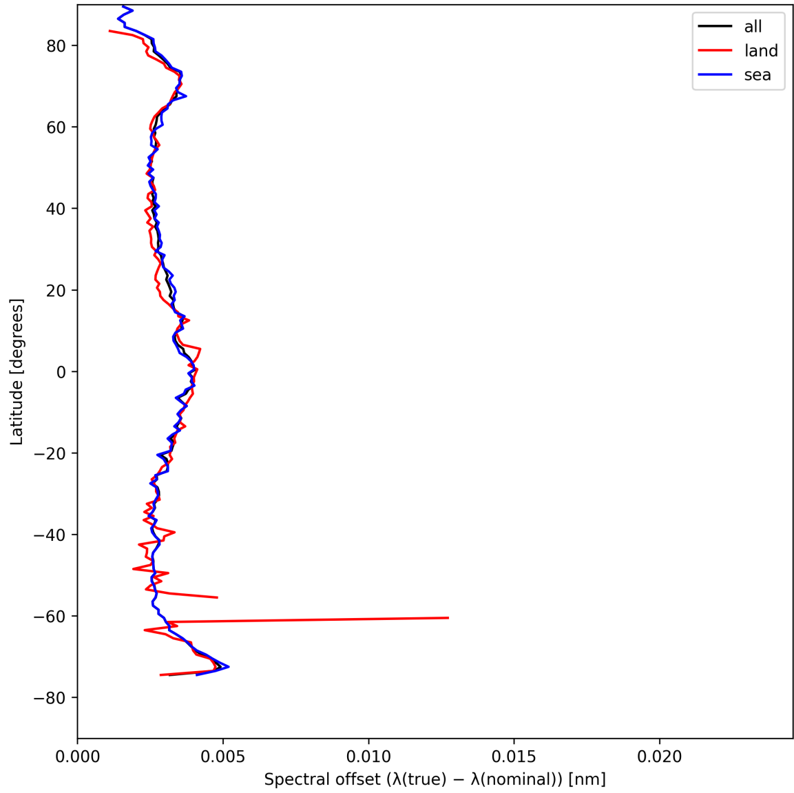
Figure 26: Zonal average of “Spectral offset ( \lambda_{\text{true}} - \lambda_{\text{nominal}} )” for 2025-04-26 to 2025-04-27.
