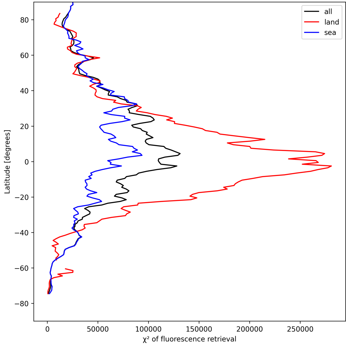
Figure 23: Zonal average of “ \chi^2 of fluorescence retrieval” for 2025-04-26 to 2025-04-27.
