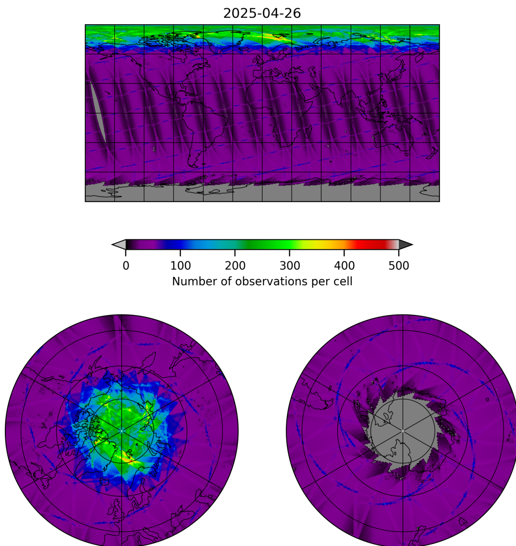
Figure 9: Map of the number of observations for 2025-04-26 to 2025-04-27
