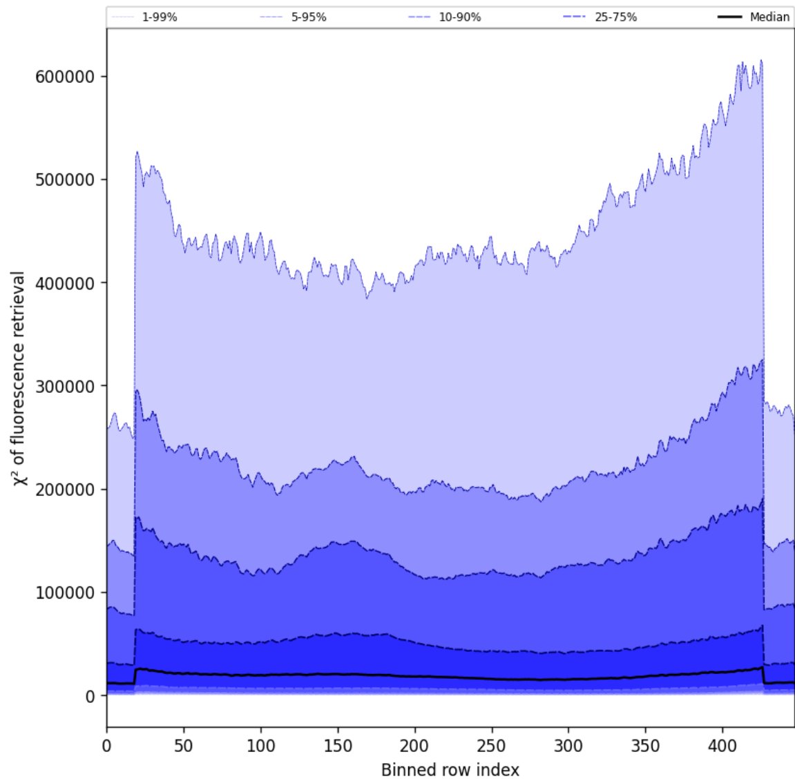
Figure 57: Along track statistics of “ \chi^2 of fluorescence retrieval” for 2025-04-26 to 2025-04-27
