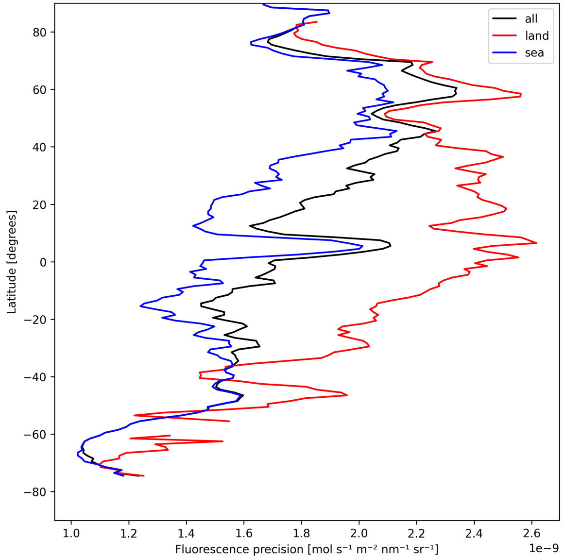
Figure 22: Zonal average of “Fluorescence precision” for 2025-04-26 to 2025-04-27.
