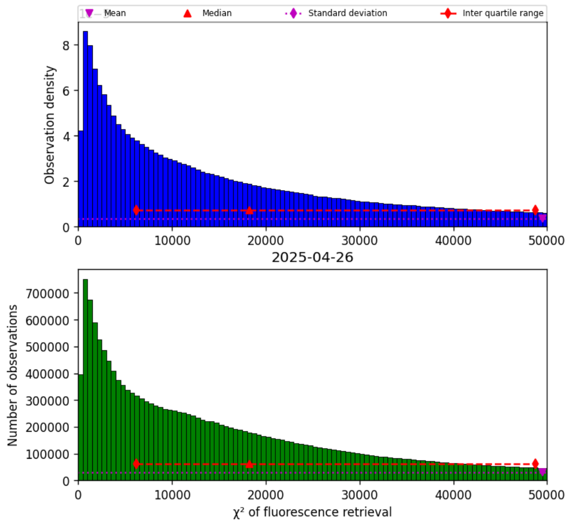
Figure 40: Histogram of “ \chi^2 of fluorescence retrieval” for 2025-04-26 to 2025-04-27
