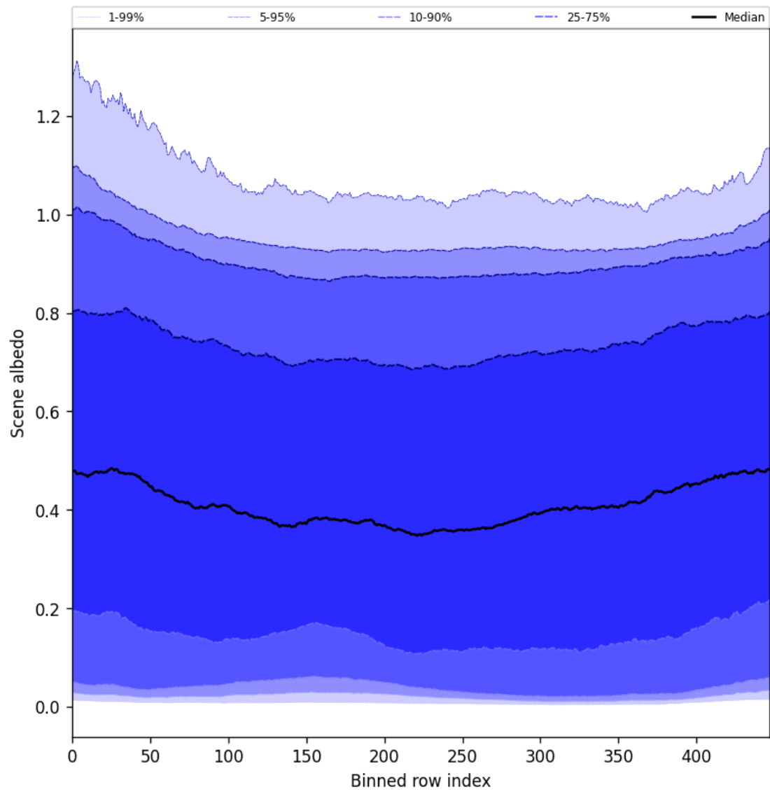
Figure 49: Along track statistics of “Scene albedo” for 2025-04-26 to 2025-04-27
