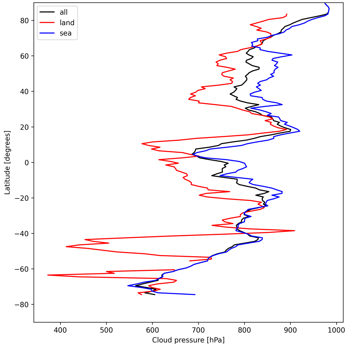
Figure 11: Zonal average of “Cloud pressure” for 2025-04-26 to 2025-04-27.
