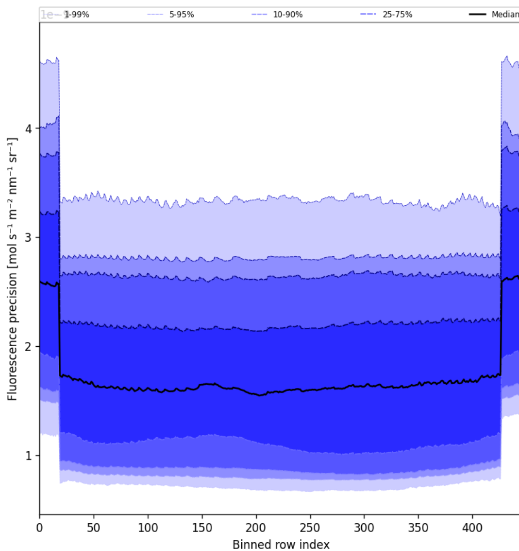
Figure 56: Along track statistics of “Fluorescence precision” for 2025-04-26 to 2025-04-27
