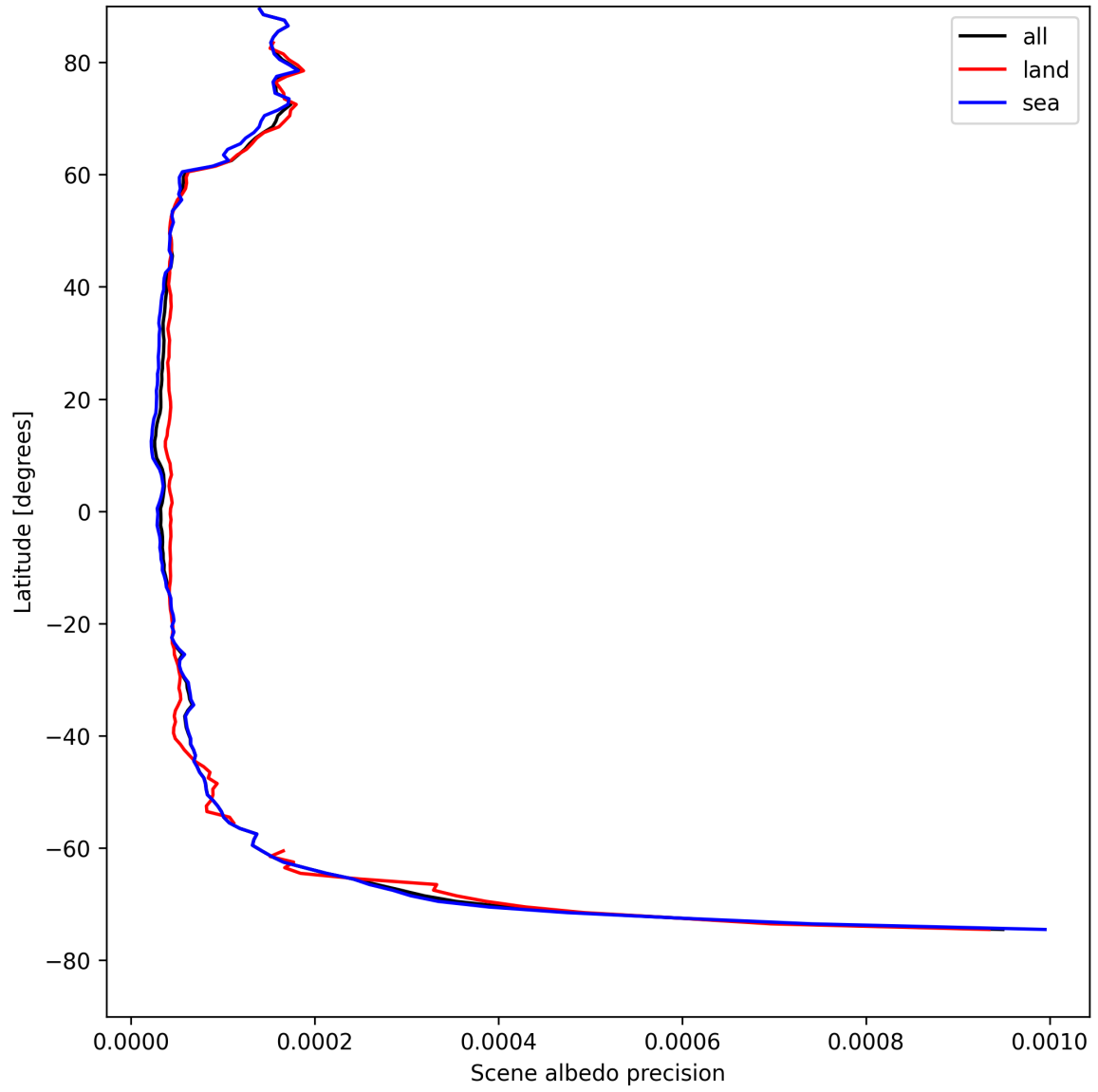
Figure 16: Zonal average of “Scene albedo precision” for 2025-04-26 to 2025-04-27.
