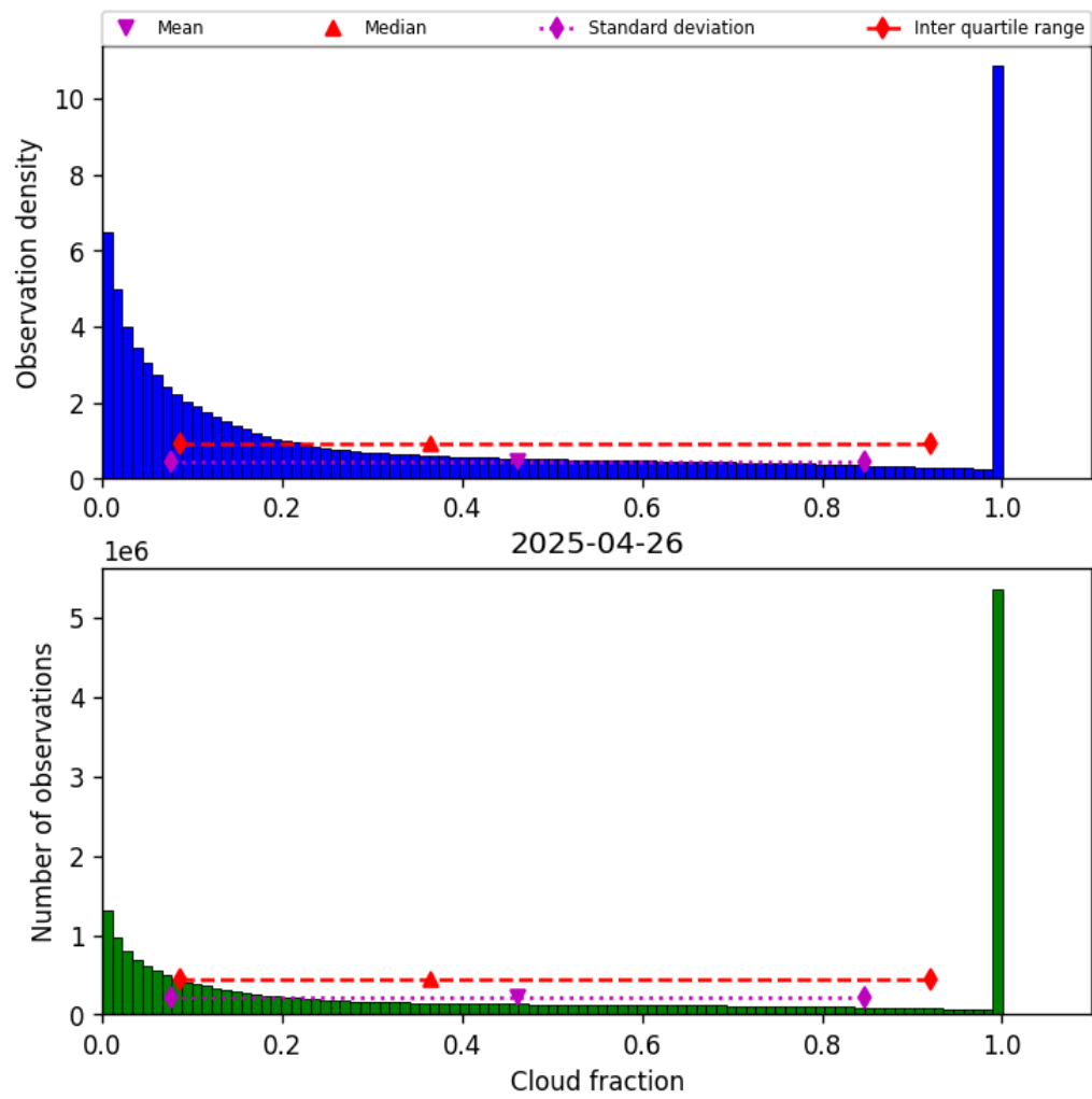
Figure 30: Histogram of “Cloud fraction” for 2025-04-26 to 2025-04-27
