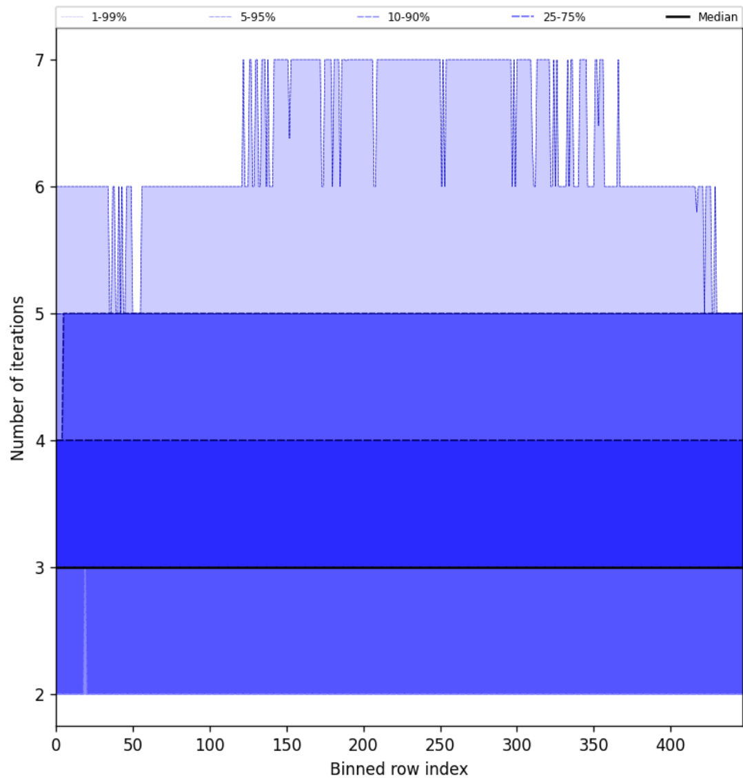
Figure 54: Along track statistics of “Number of iterations” for 2025-04-26 to 2025-04-27
