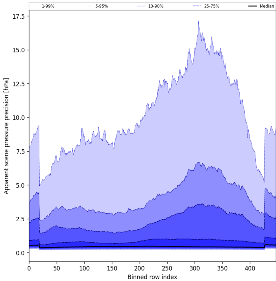
Figure 52: Along track statistics of “Apparent scene pressure precision” for 2025-04-26 to 2025-04-27
