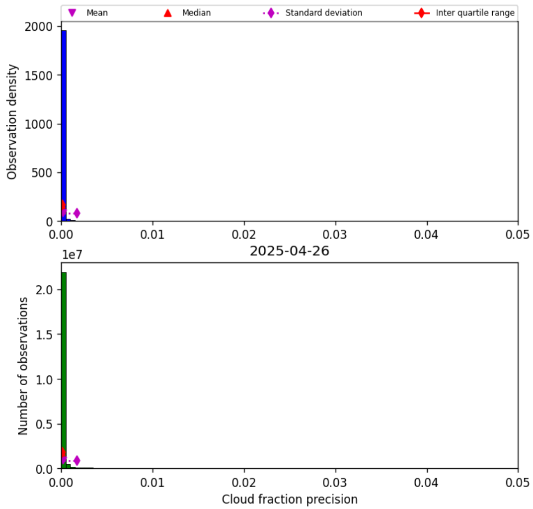
Figure 31: Histogram of “Cloud fraction precision” for 2025-04-26 to 2025-04-27
