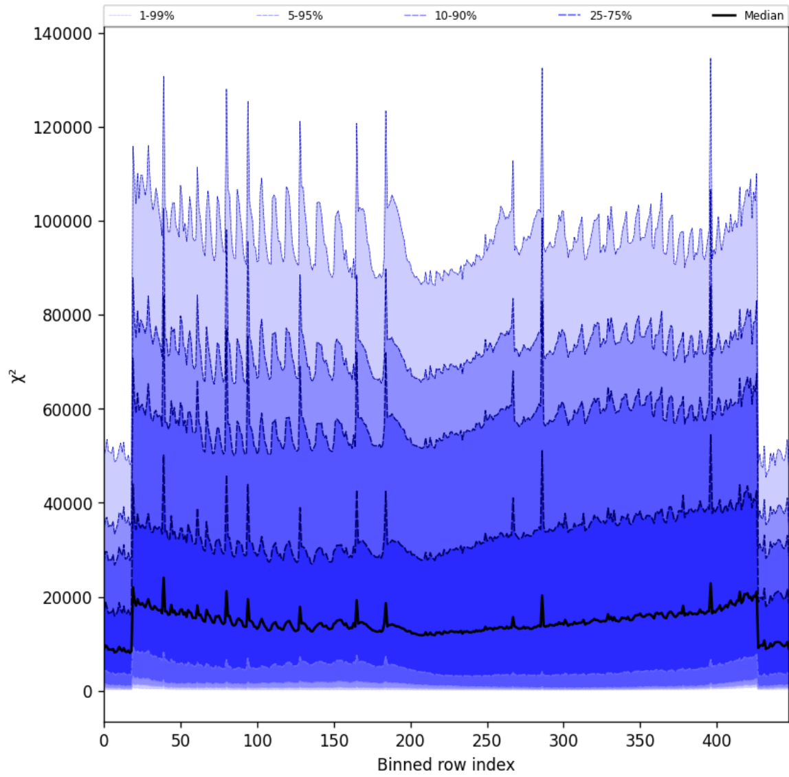
Figure 53: Along track statistics of “ \chi^2 ” for 2025-04-26 to 2025-04-27
