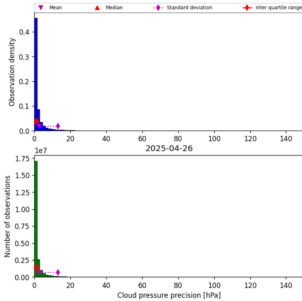
Figure 29: Histogram of “Cloud pressure precision” for 2025-04-26 to 2025-04-27
