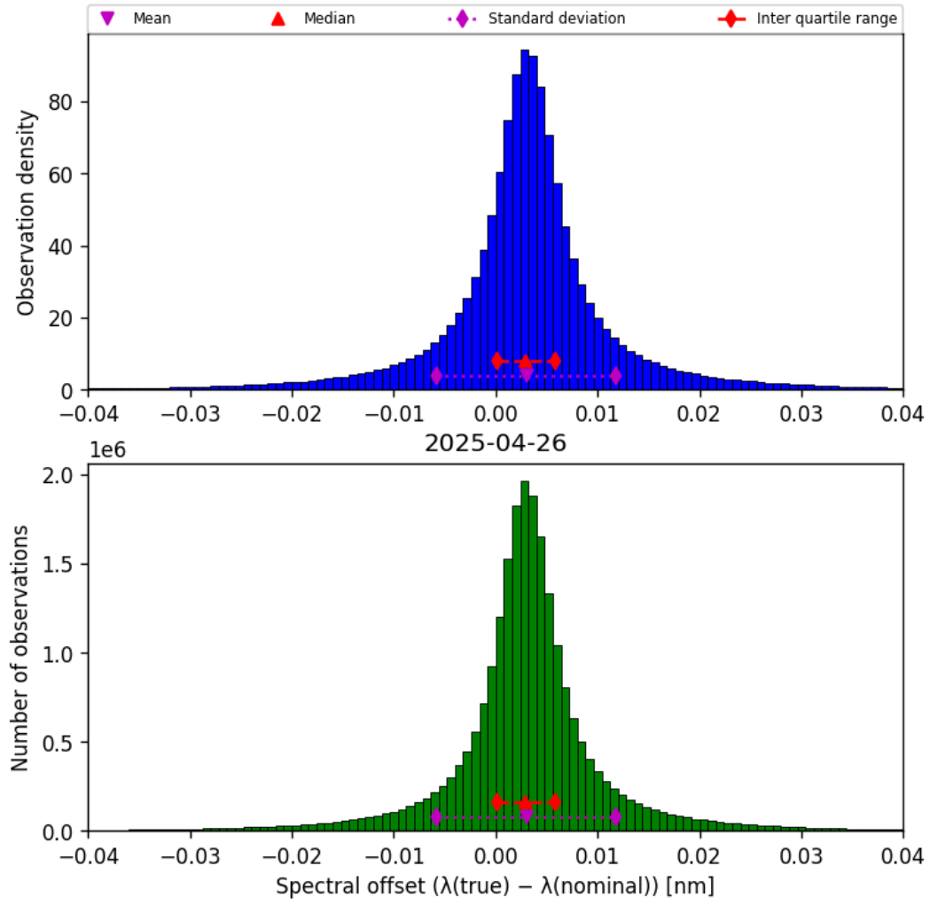
Figure 43: Histogram of “Spectral offset ( \lambda_{\text{true}} - \lambda_{\text{nominal}} )” for 2025-04-26 to 2025-04-27
