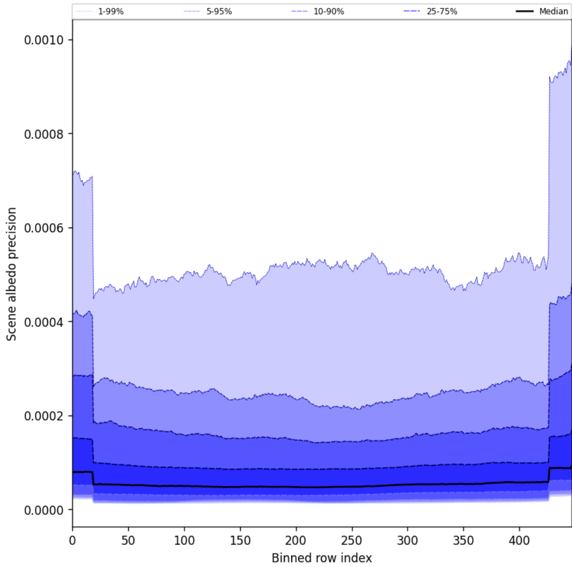
Figure 50: Along track statistics of “Scene albedo precision” for 2025-04-26 to 2025-04-27
