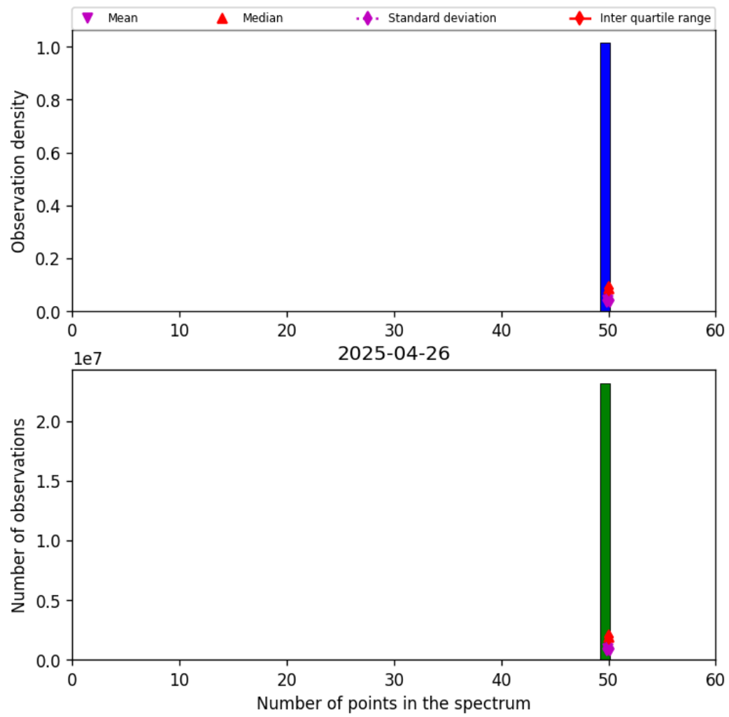
Figure 42: Histogram of “Number of points in the spectrum” for 2025-04-26 to 2025-04-27
