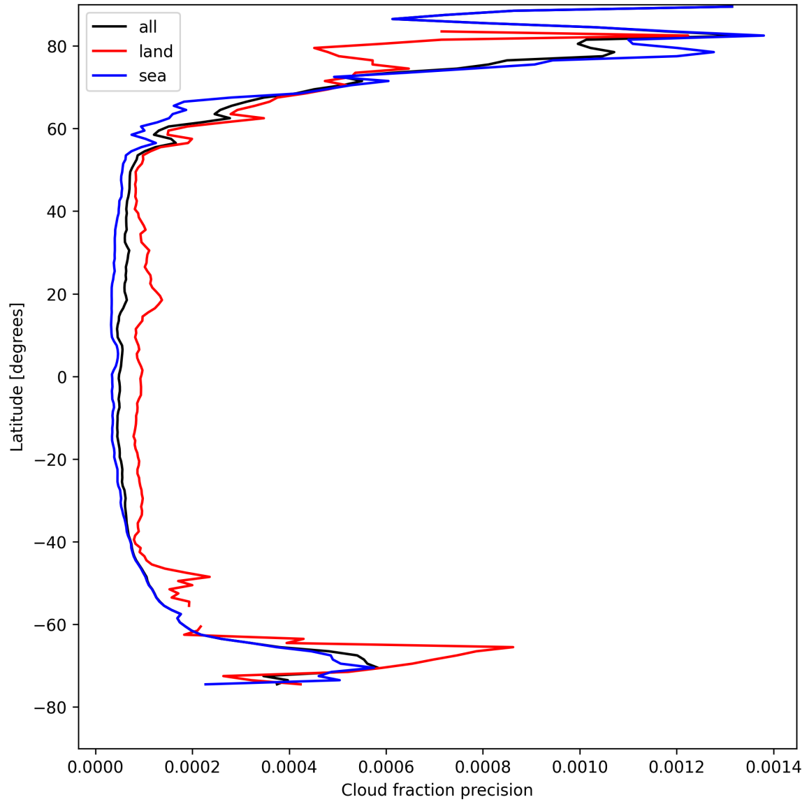
Figure 14: Zonal average of “Cloud fraction precision” for 2025-04-26 to 2025-04-27.
