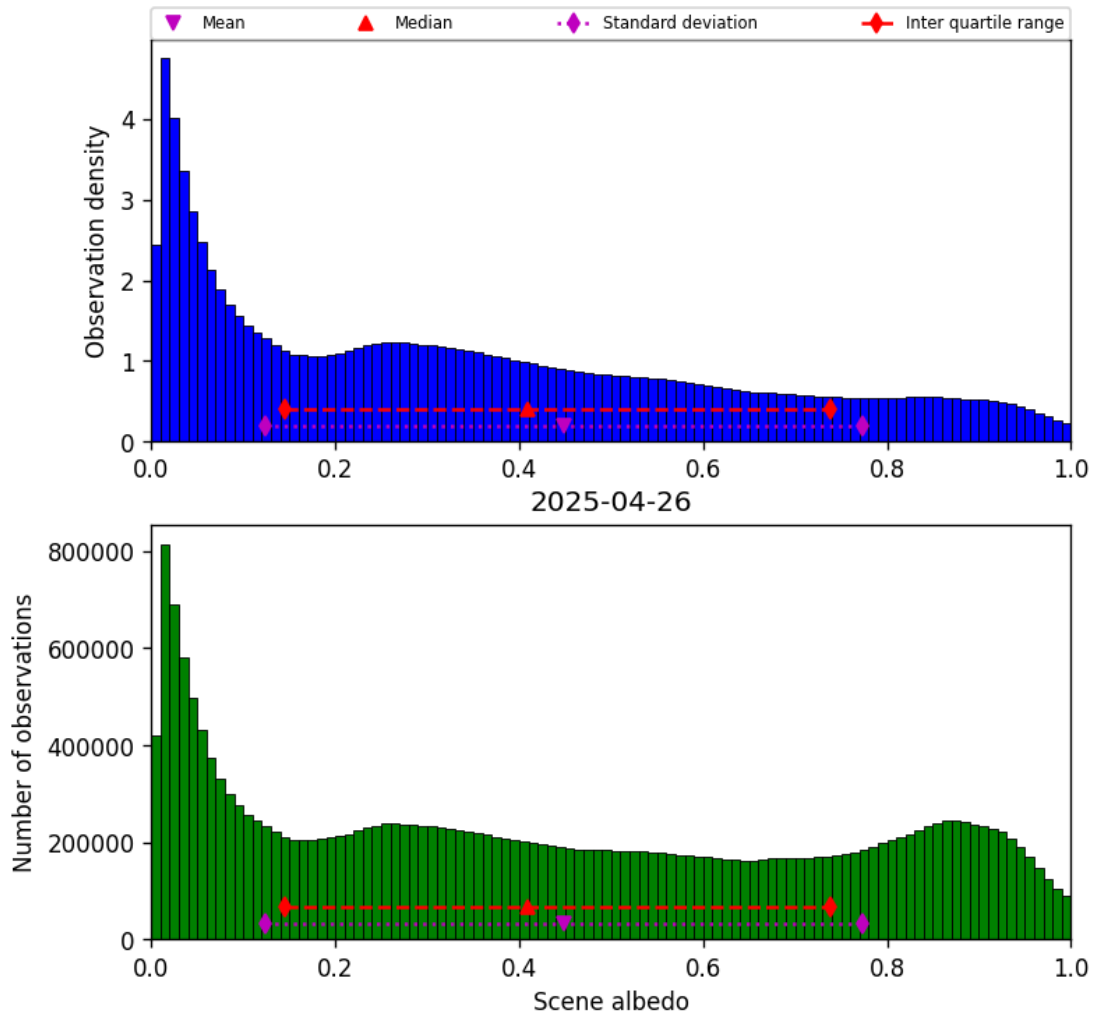
Figure 32: Histogram of “Scene albedo” for 2025-04-26 to 2025-04-27
