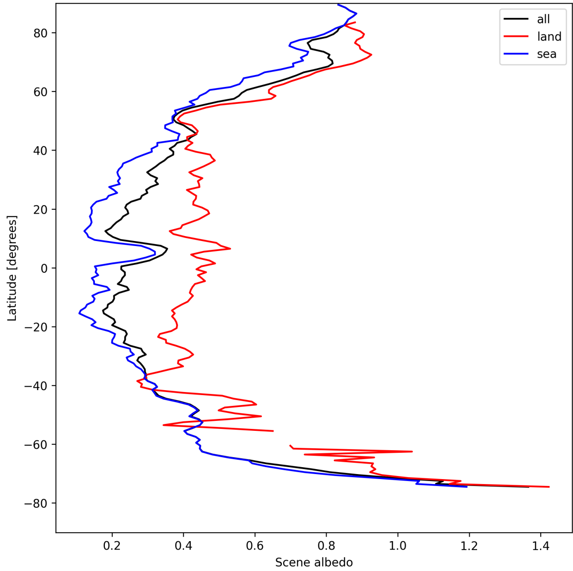
Figure 15: Zonal average of “Scene albedo” for 2025-04-26 to 2025-04-27.
