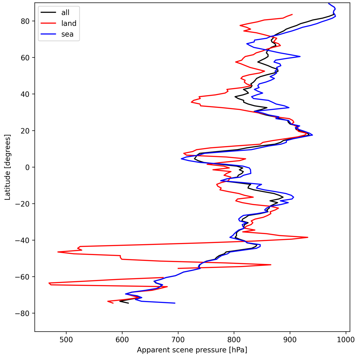
Figure 17: Zonal average of “Apparent scene pressure” for 2025-04-26 to 2025-04-27.
