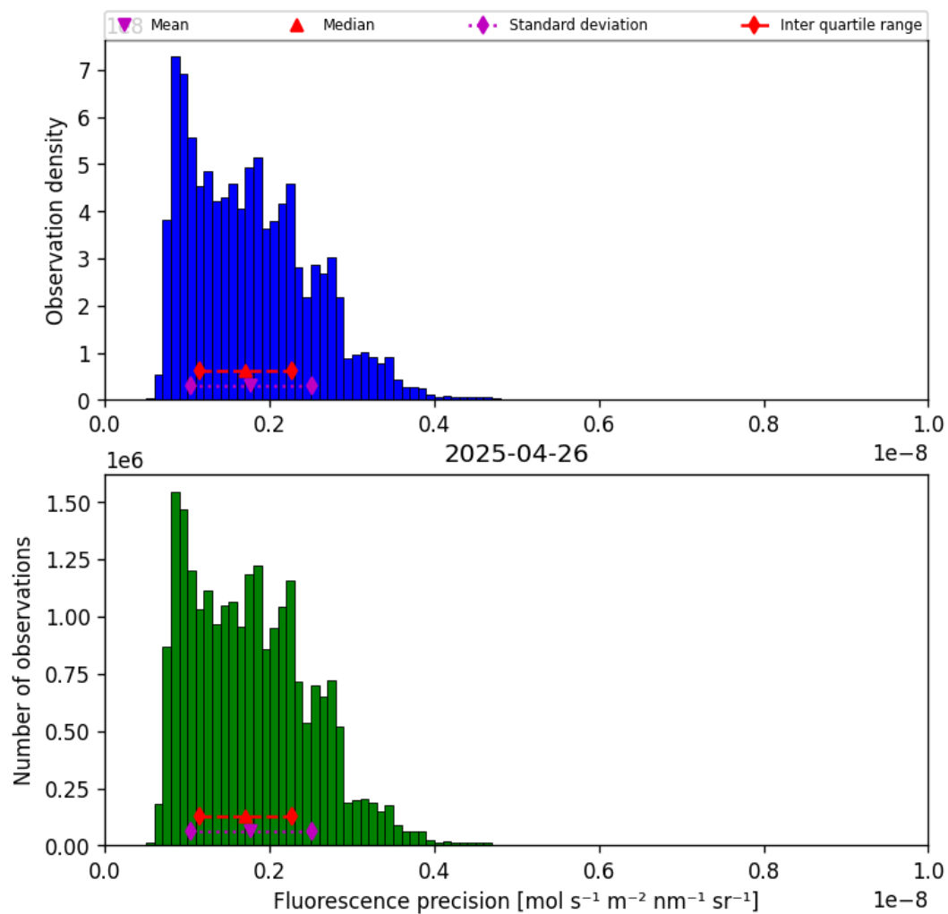
Figure 39: Histogram of “Fluorescence precision” for 2025-04-26 to 2025-04-27
