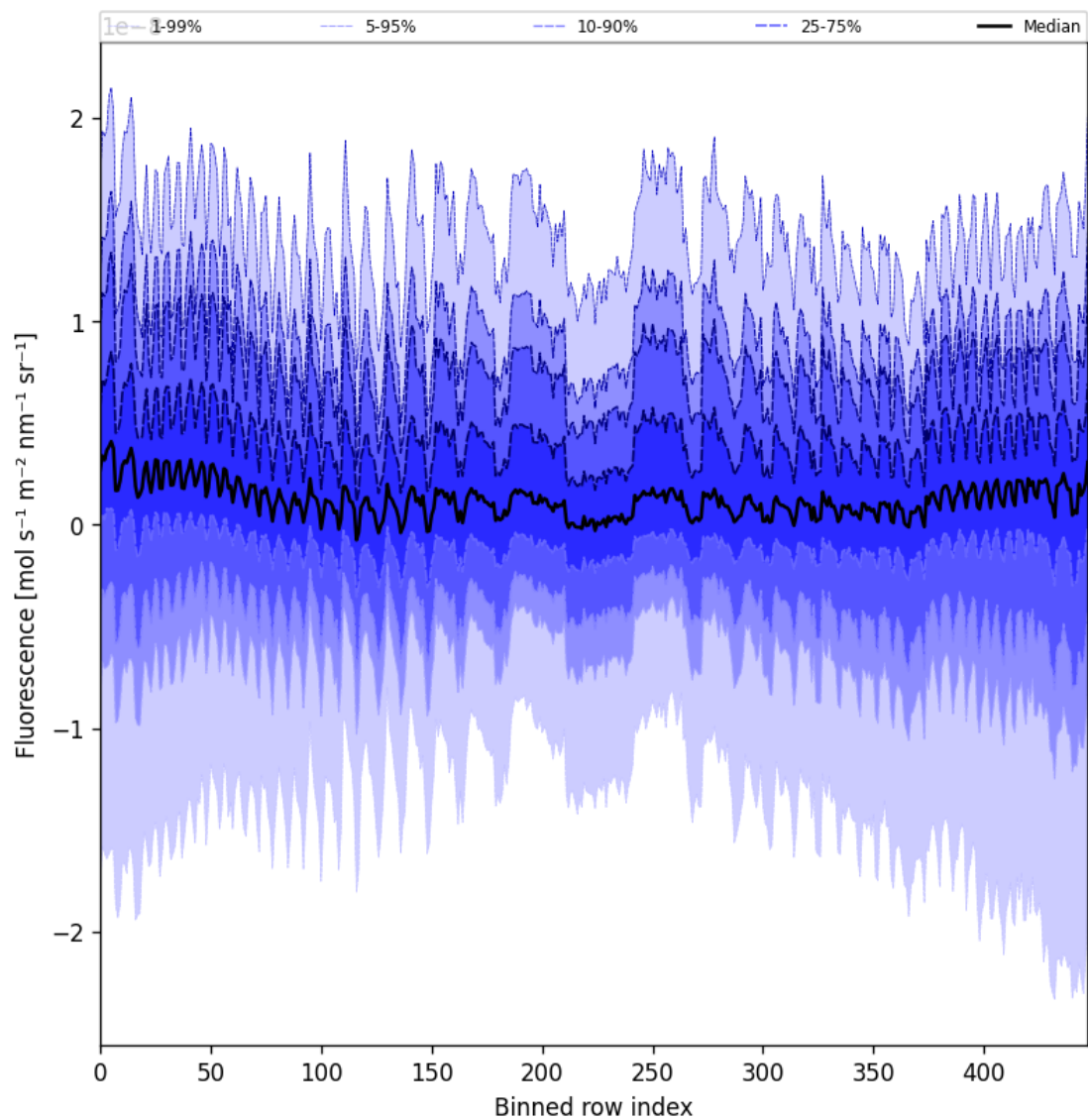
Figure 55: Along track statistics of “Fluorescence” for 2025-04-26 to 2025-04-27
