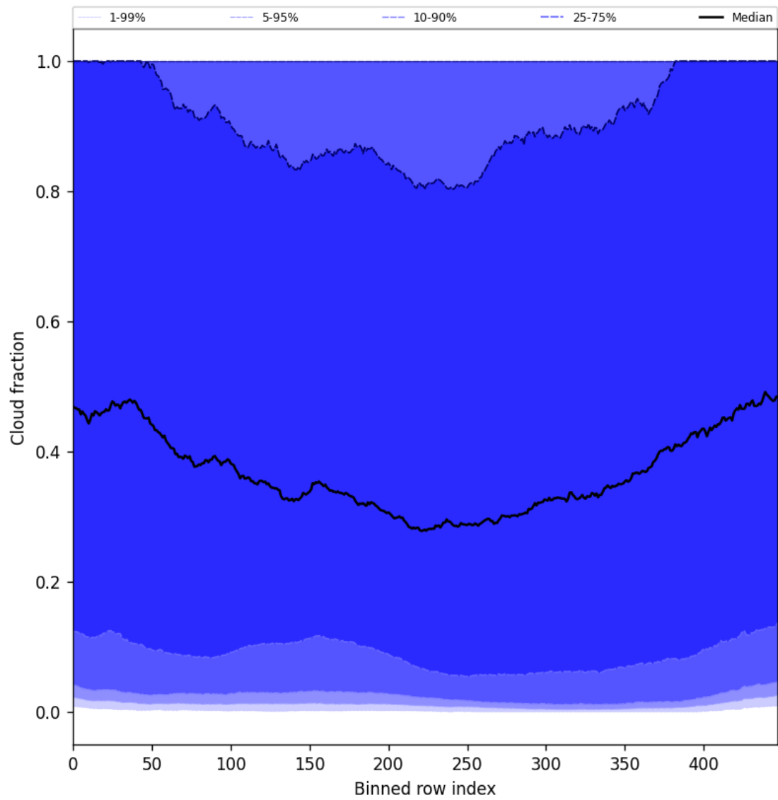
Figure 47: Along track statistics of “Cloud fraction” for 2025-04-26 to 2025-04-27
