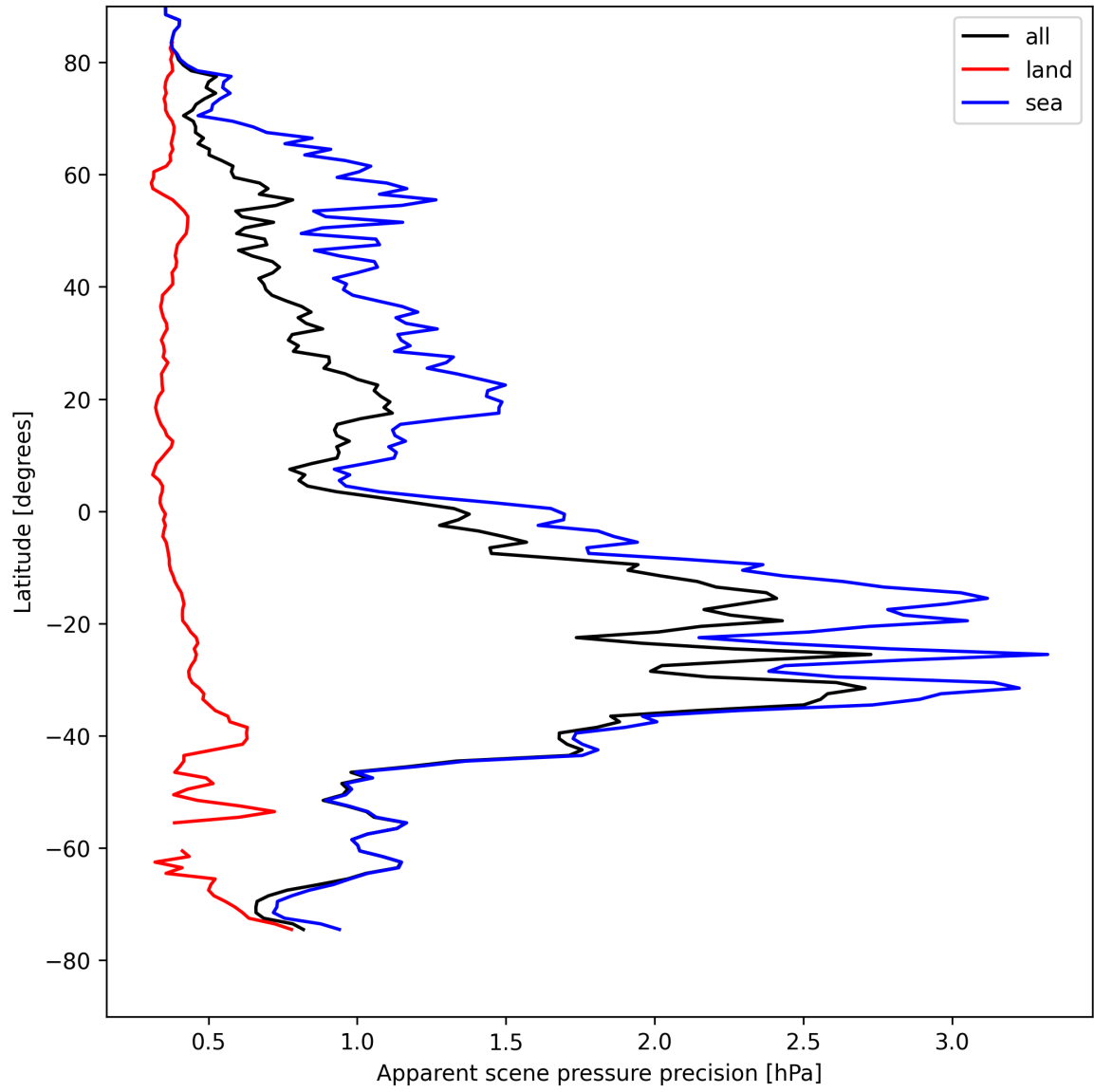
Figure 18: Zonal average of “Apparent scene pressure precision” for 2025-04-26 to 2025-04-27.
