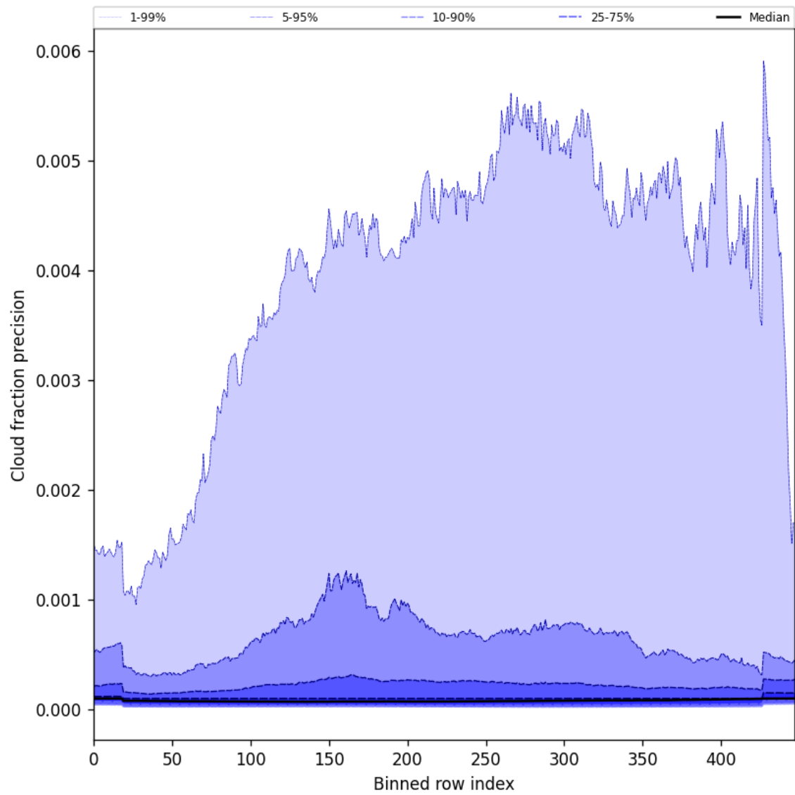
Figure 48: Along track statistics of “Cloud fraction precision” for 2025-04-26 to 2025-04-27
