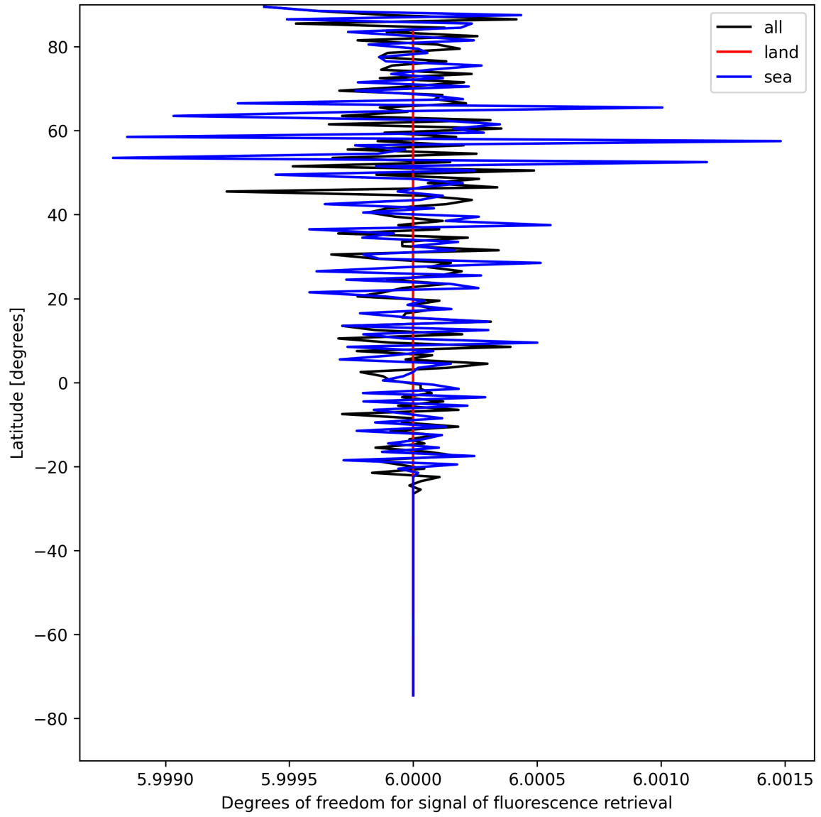
Figure 24: Zonal average of “Degrees of freedom for signal of fluorescence retrieval” for 2025-04-26 to 2025-04-27.
