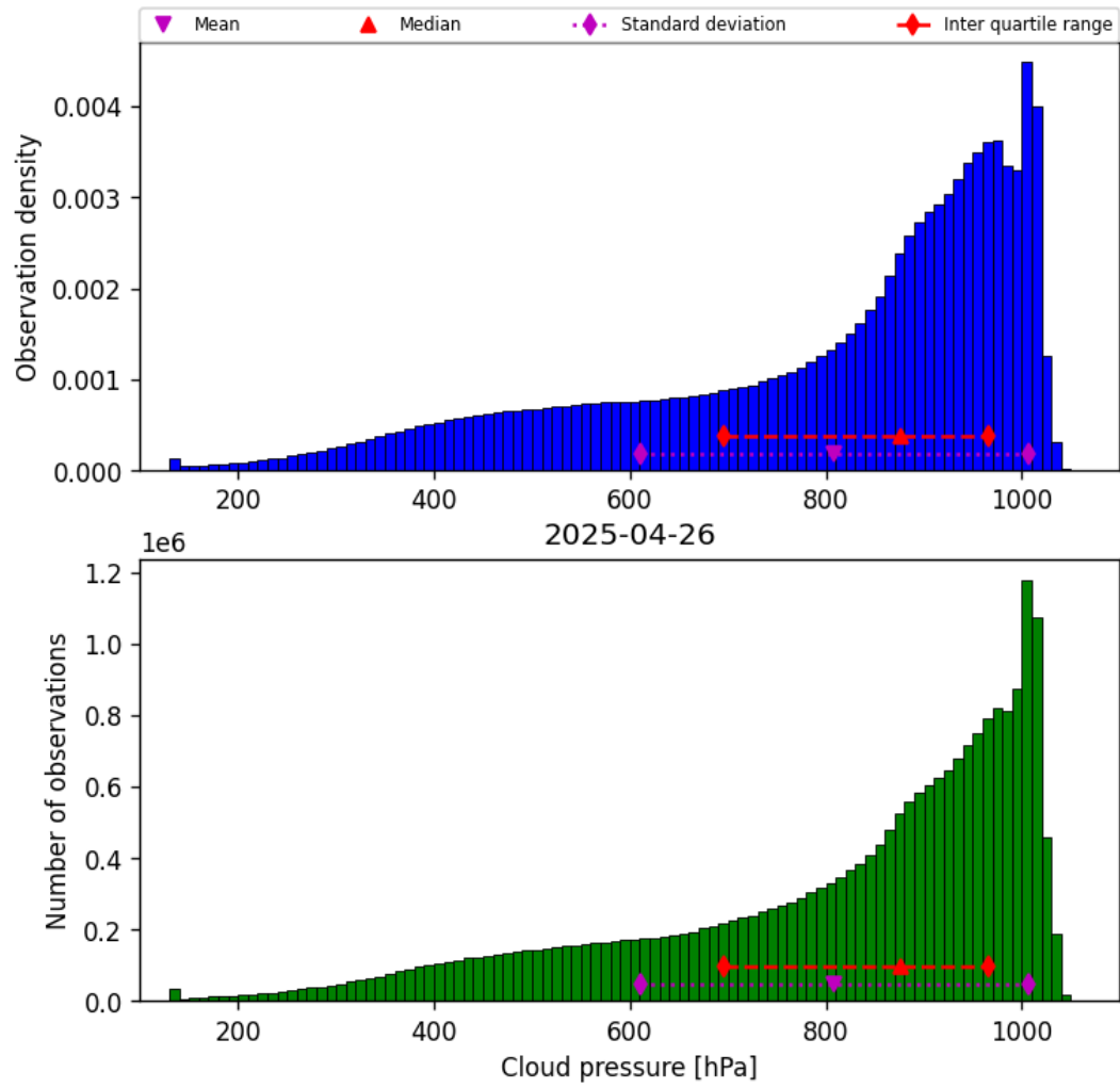
Figure 28: Histogram of “Cloud pressure” for 2025-04-26 to 2025-04-27
