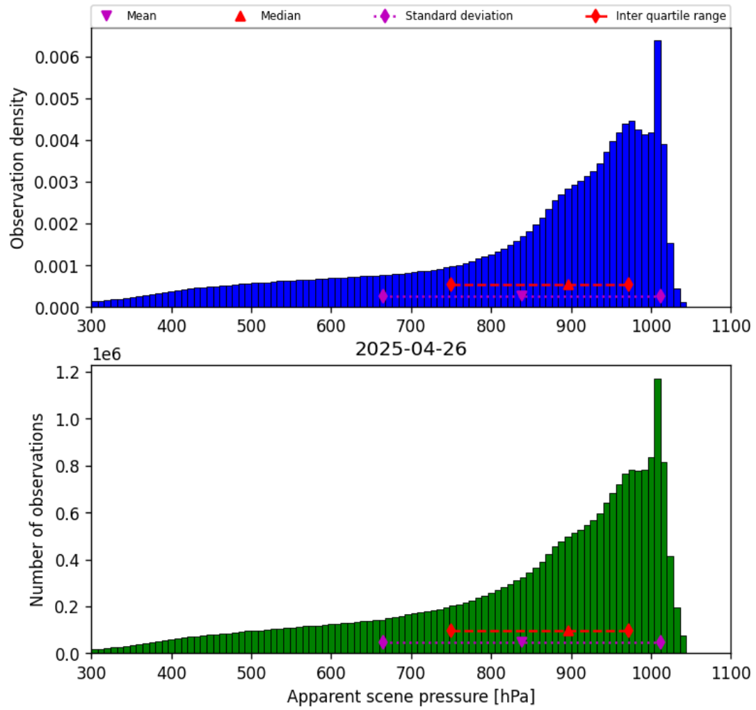
Figure 34: Histogram of “Apparent scene pressure” for 2025-04-26 to 2025-04-27
