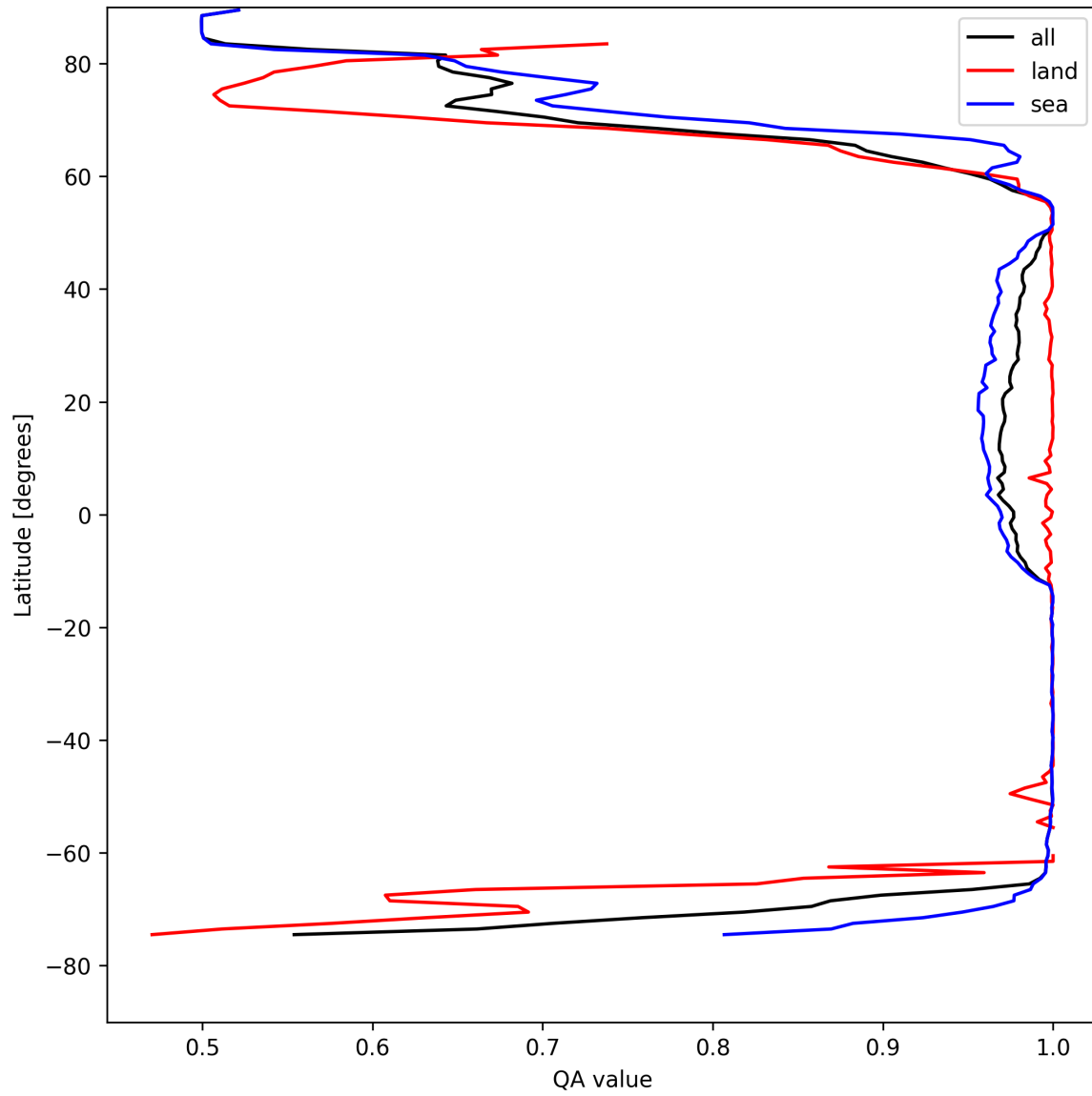
Figure 10: Zonal average of “QA value” for 2025-04-26 to 2025-04-27.
