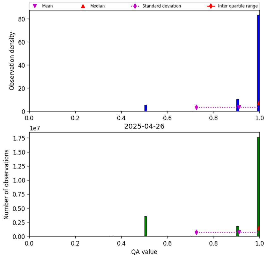
Figure 27: Histogram of “QA value” for 2025-04-26 to 2025-04-27
