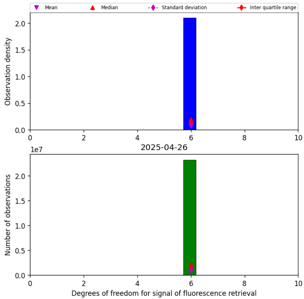
Figure 41: Histogram of “Degrees of freedom for signal of fluorescence retrieval” for 2025-04-26 to 2025-04-27
