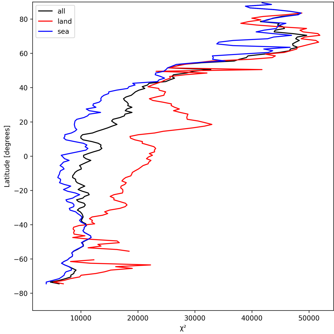
Figure 19: Zonal average of “ \chi^2 ” for 2025-04-26 to 2025-04-27.
