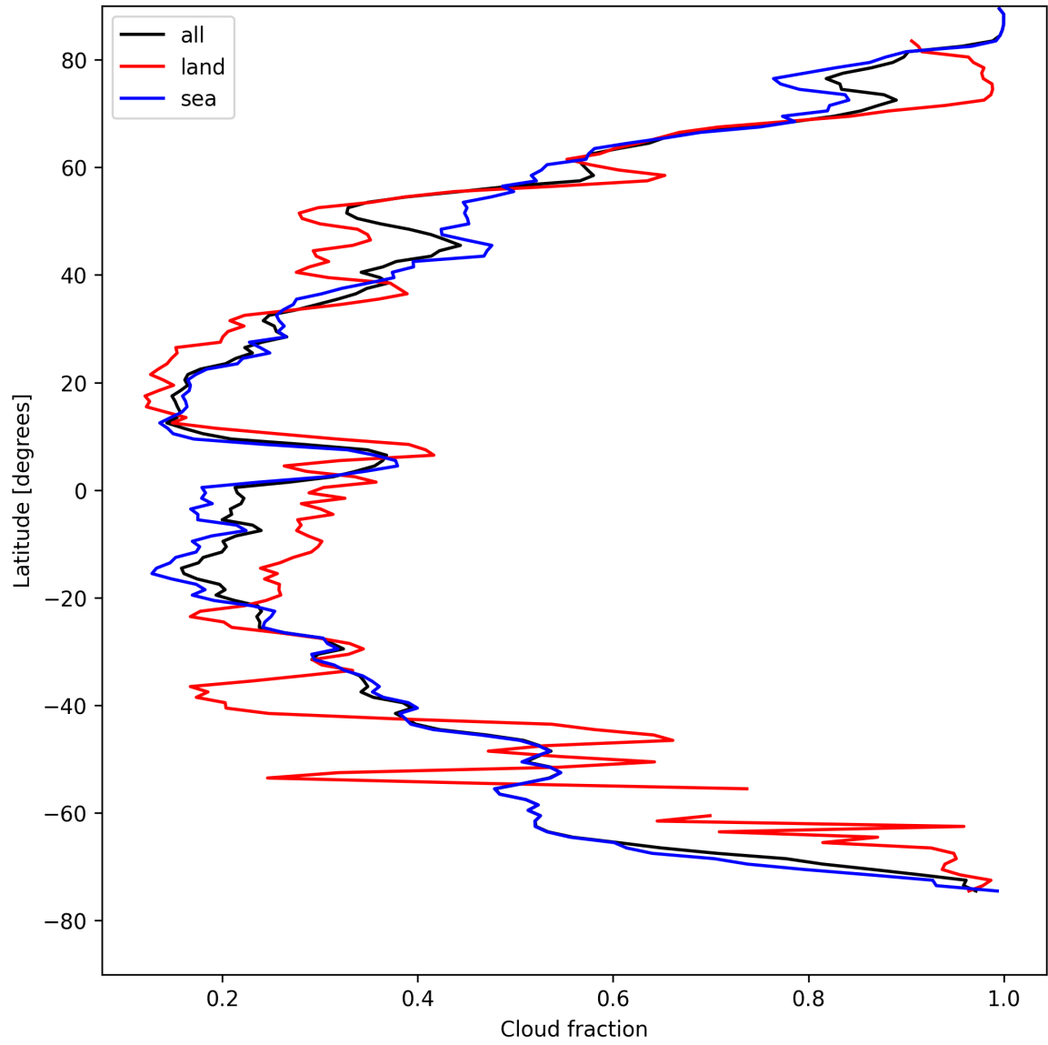
Figure 13: Zonal average of “Cloud fraction” for 2025-04-26 to 2025-04-27.
