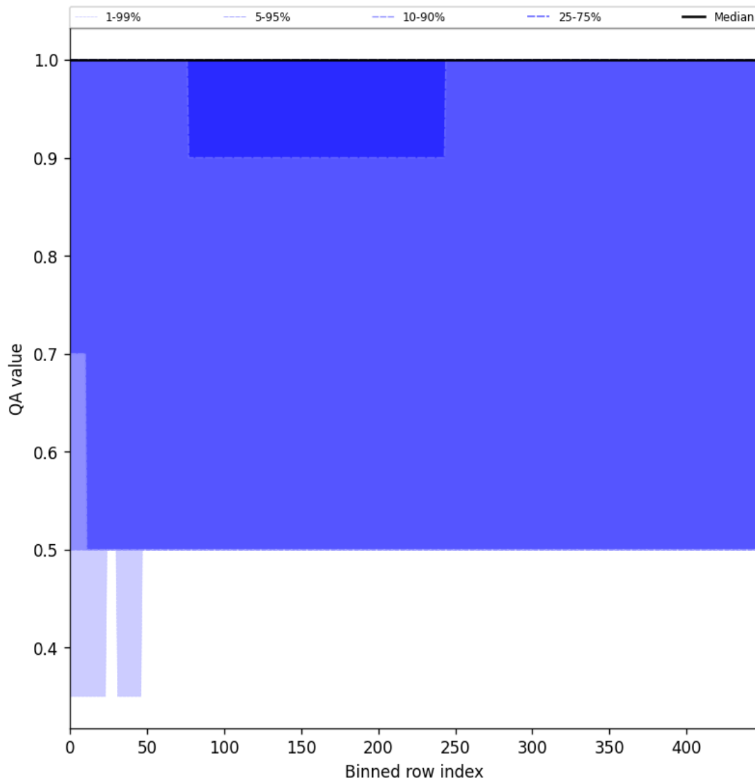
Figure 44: Along track statistics of “QA value” for 2025-04-26 to 2025-04-27
