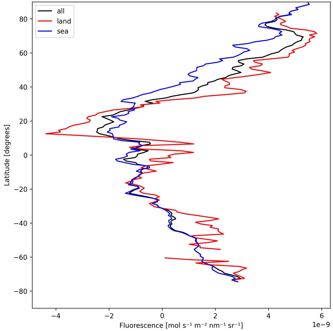
Figure 21: Zonal average of “Fluorescence” for 2025-04-26 to 2025-04-27.
