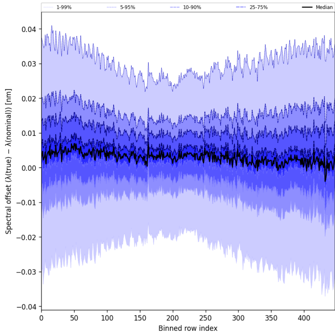
Figure 60: Along track statistics of “Spectral offset ( \lambda_{\text{true}} - \lambda_{\text{nominal}} )” for 2025-04-26 to 2025-04-27
