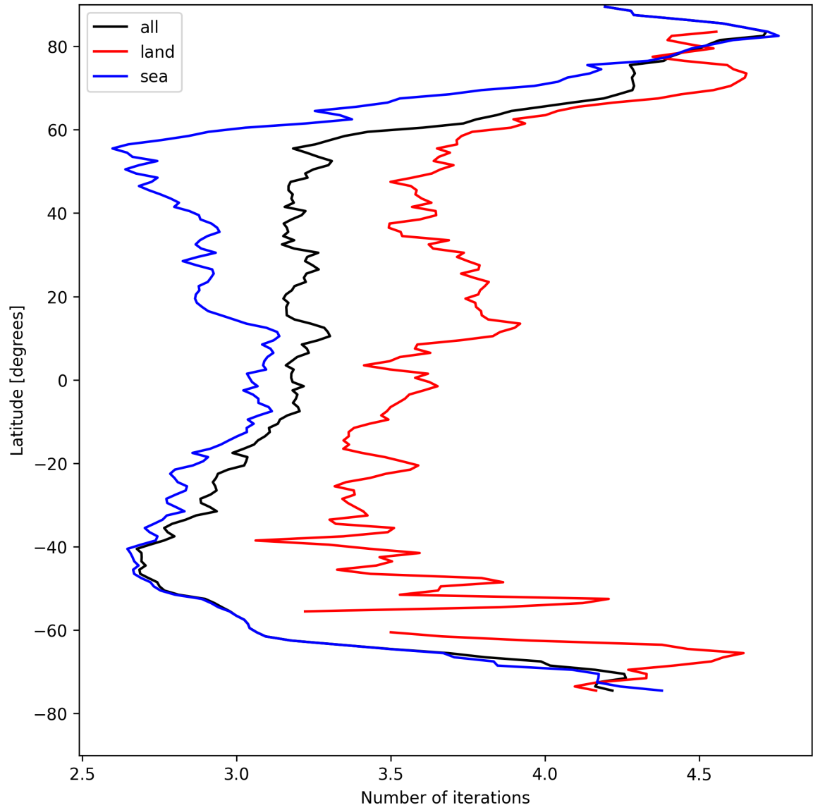
Figure 20: Zonal average of “Number of iterations” for 2025-04-26 to 2025-04-27.
