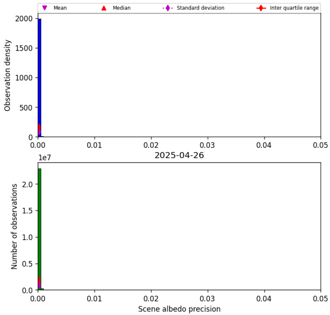
Figure 33: Histogram of “Scene albedo precision” for 2025-04-26 to 2025-04-27
