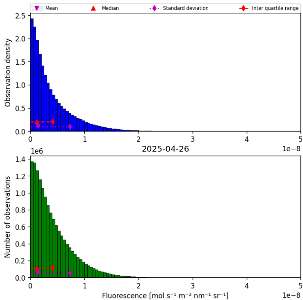
Figure 38: Histogram of “Fluorescence” for 2025-04-26 to 2025-04-27
