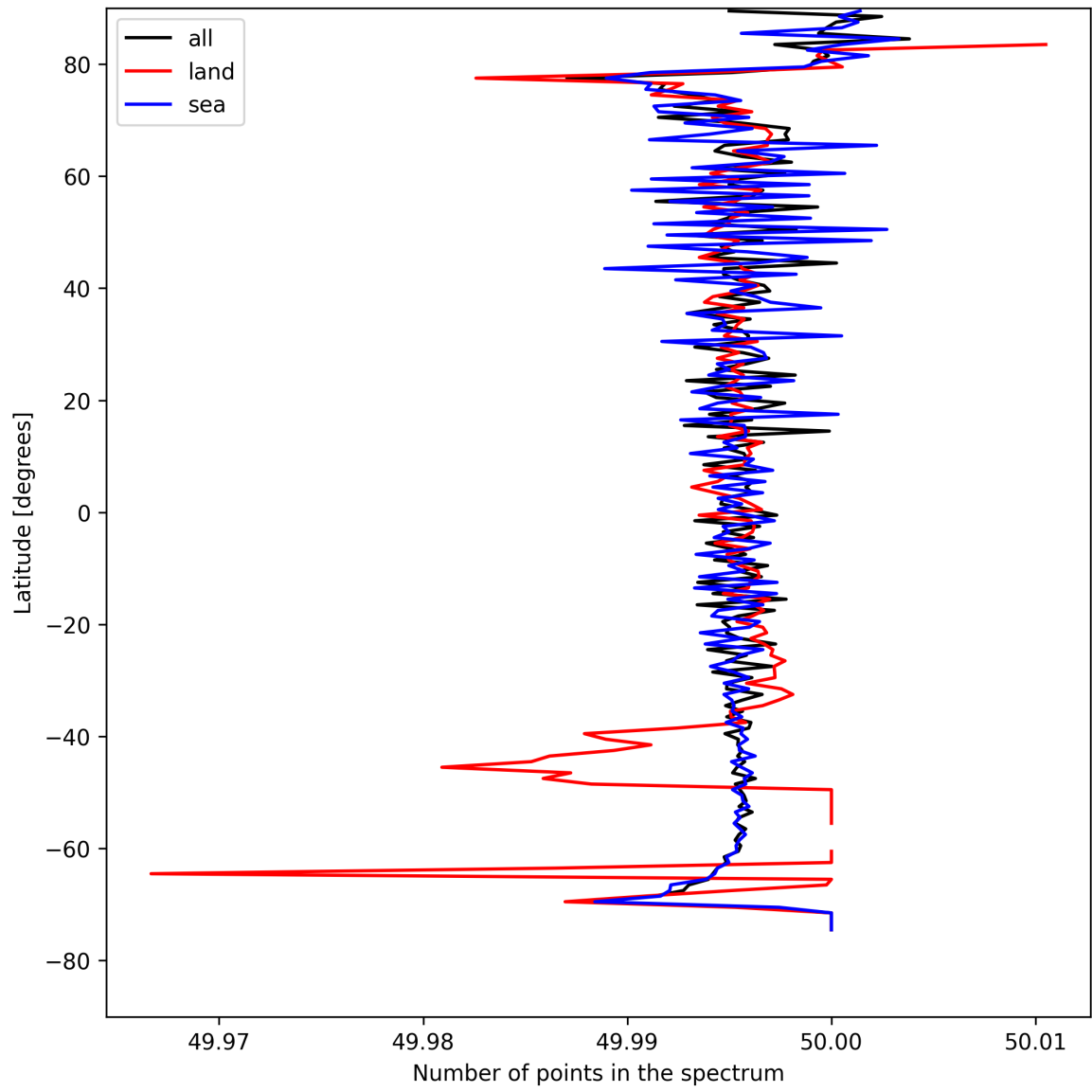
Figure 25: Zonal average of “Number of points in the spectrum” for 2025-04-26 to 2025-04-27.
