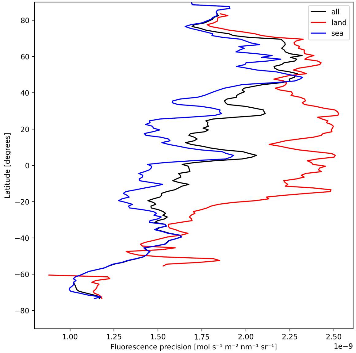
Figure 22: Zonal average of “Fluorescence precision” for 2025-04-28 to 2025-04-29.
