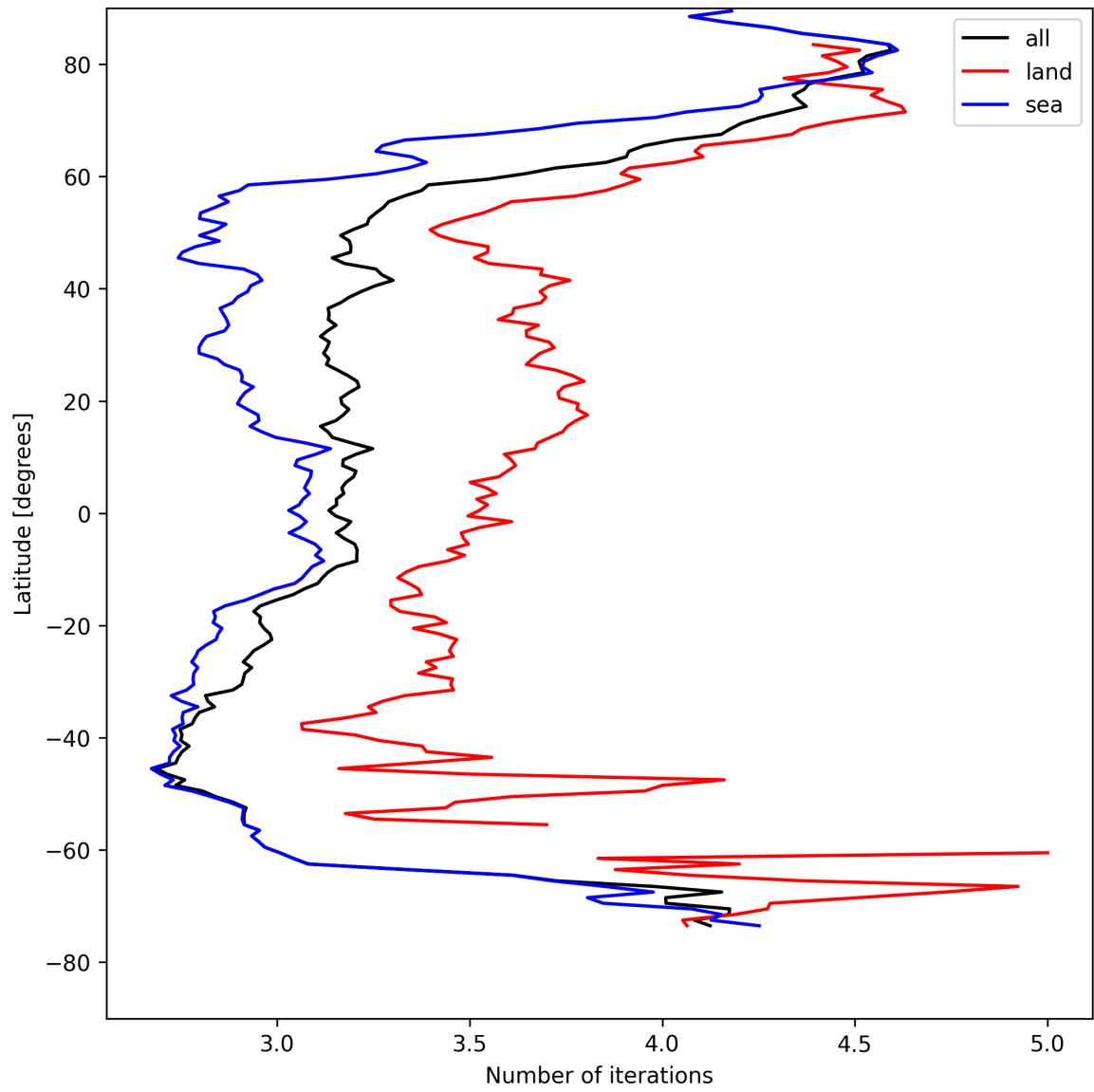
Figure 20: Zonal average of “Number of iterations” for 2025-04-28 to 2025-04-29.
