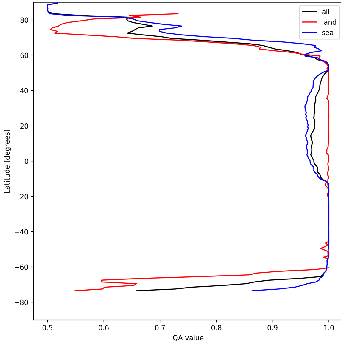
Figure 10: Zonal average of “QA value” for 2025-04-28 to 2025-04-29.
