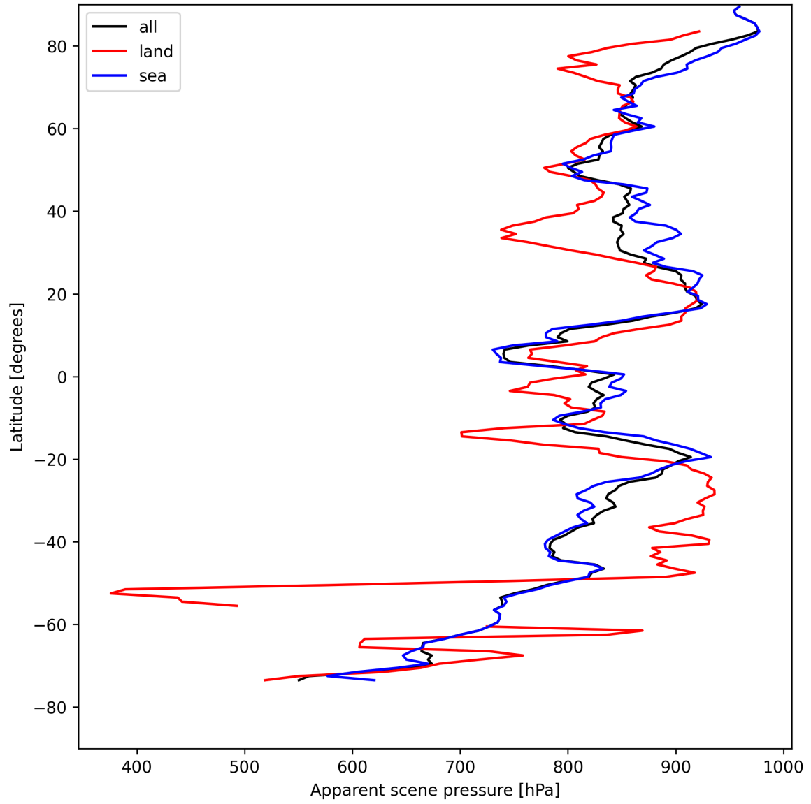
Figure 17: Zonal average of “Apparent scene pressure” for 2025-04-28 to 2025-04-29.
