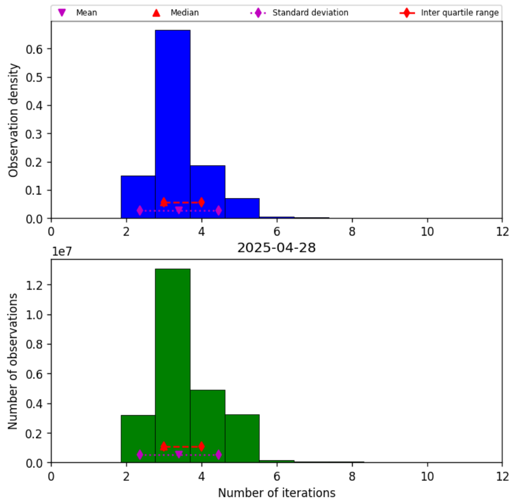
Figure 37: Histogram of “Number of iterations” for 2025-04-28 to 2025-04-29
