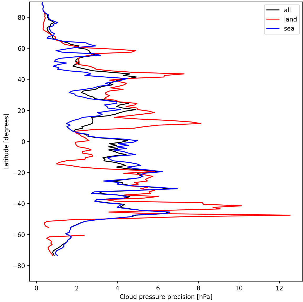
Figure 12: Zonal average of "Cloud pressure precision" for 2025-04-28 to 2025-04-29.
