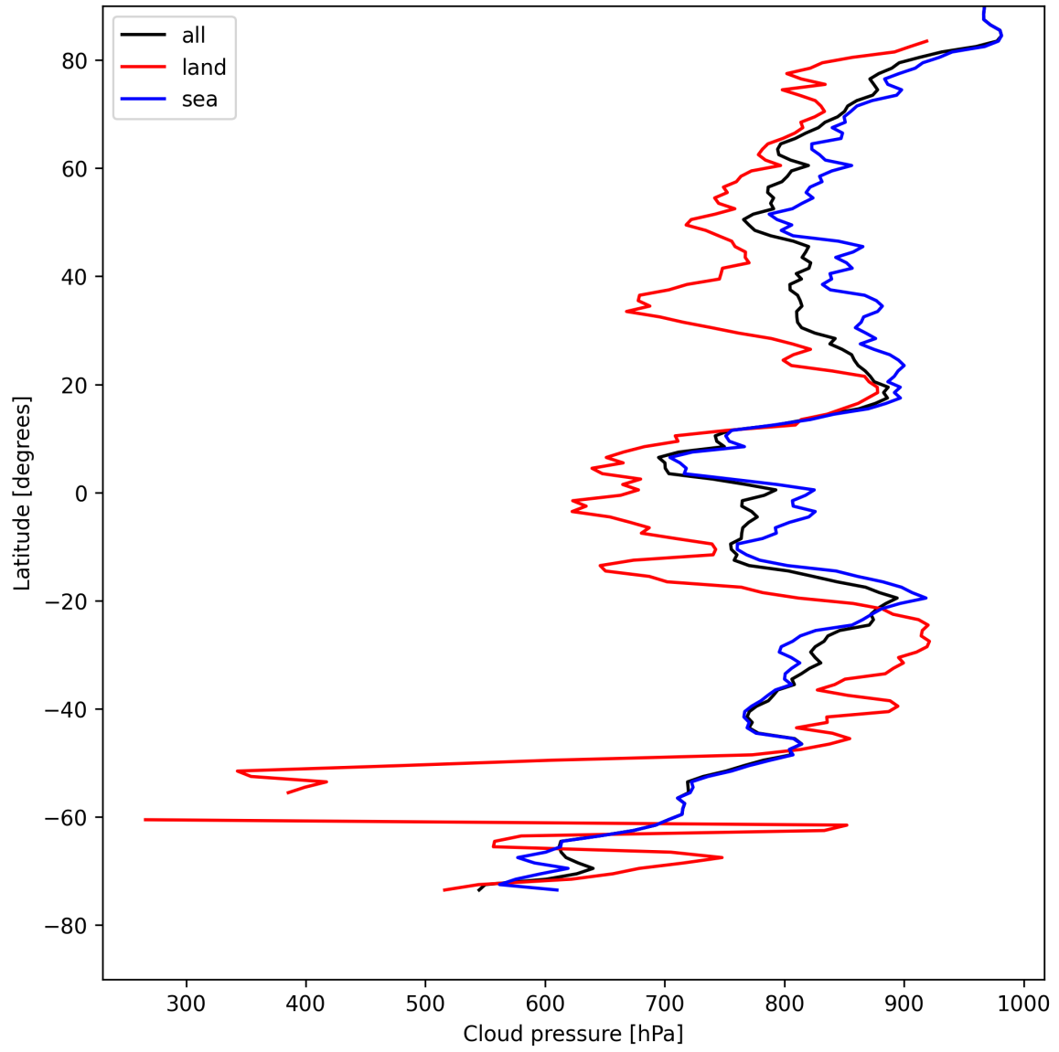
Figure 11: Zonal average of “Cloud pressure” for 2025-04-28 to 2025-04-29.
