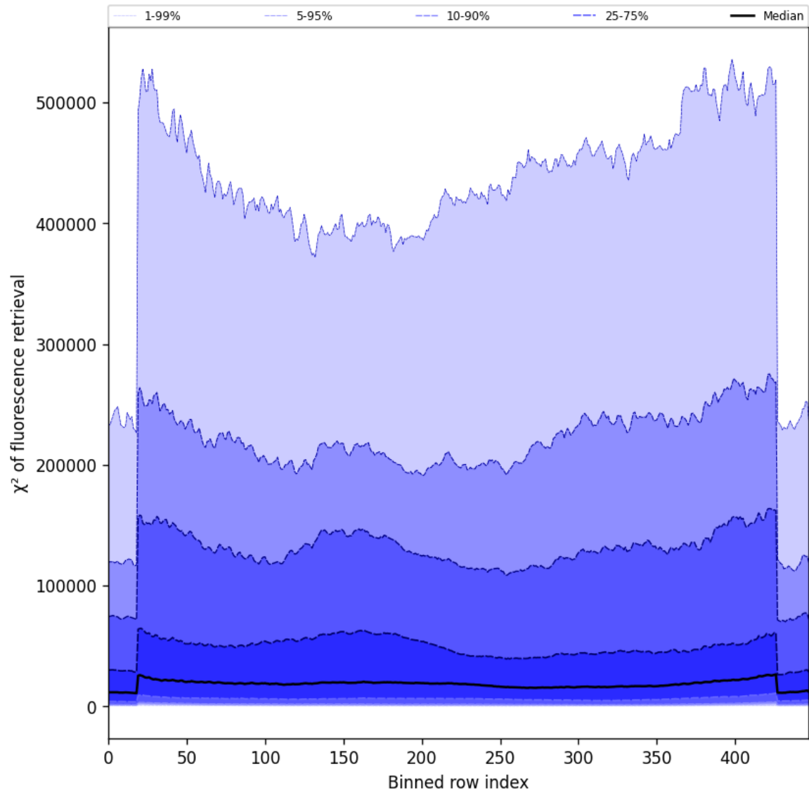
Figure 57: Along track statistics of “ \chi^2 of fluorescence retrieval” for 2025-04-28 to 2025-04-29
