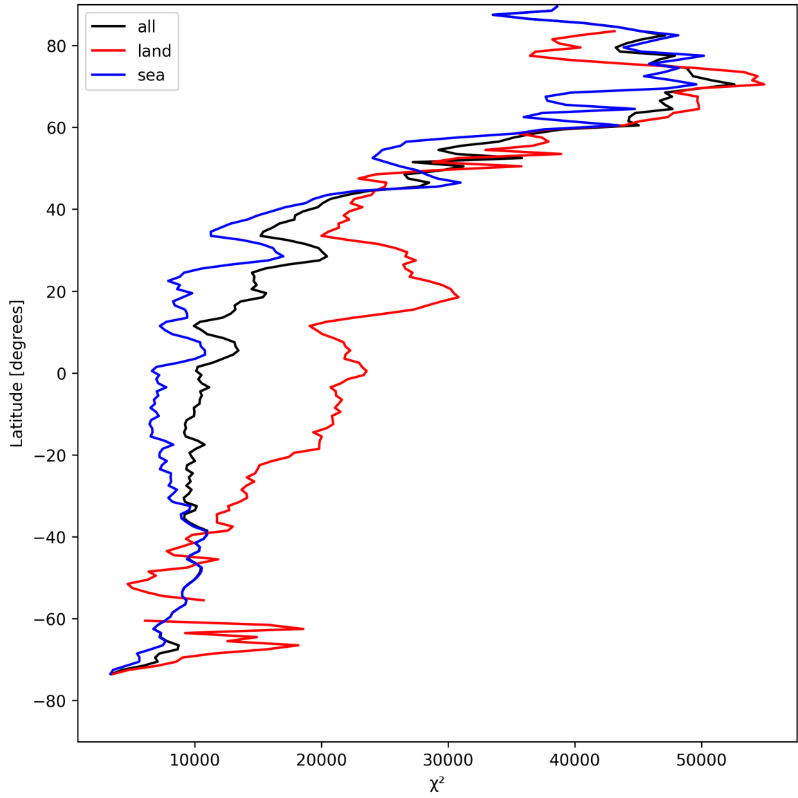
Figure 19: Zonal average of “ \chi^2 ” for 2025-04-28 to 2025-04-29.
