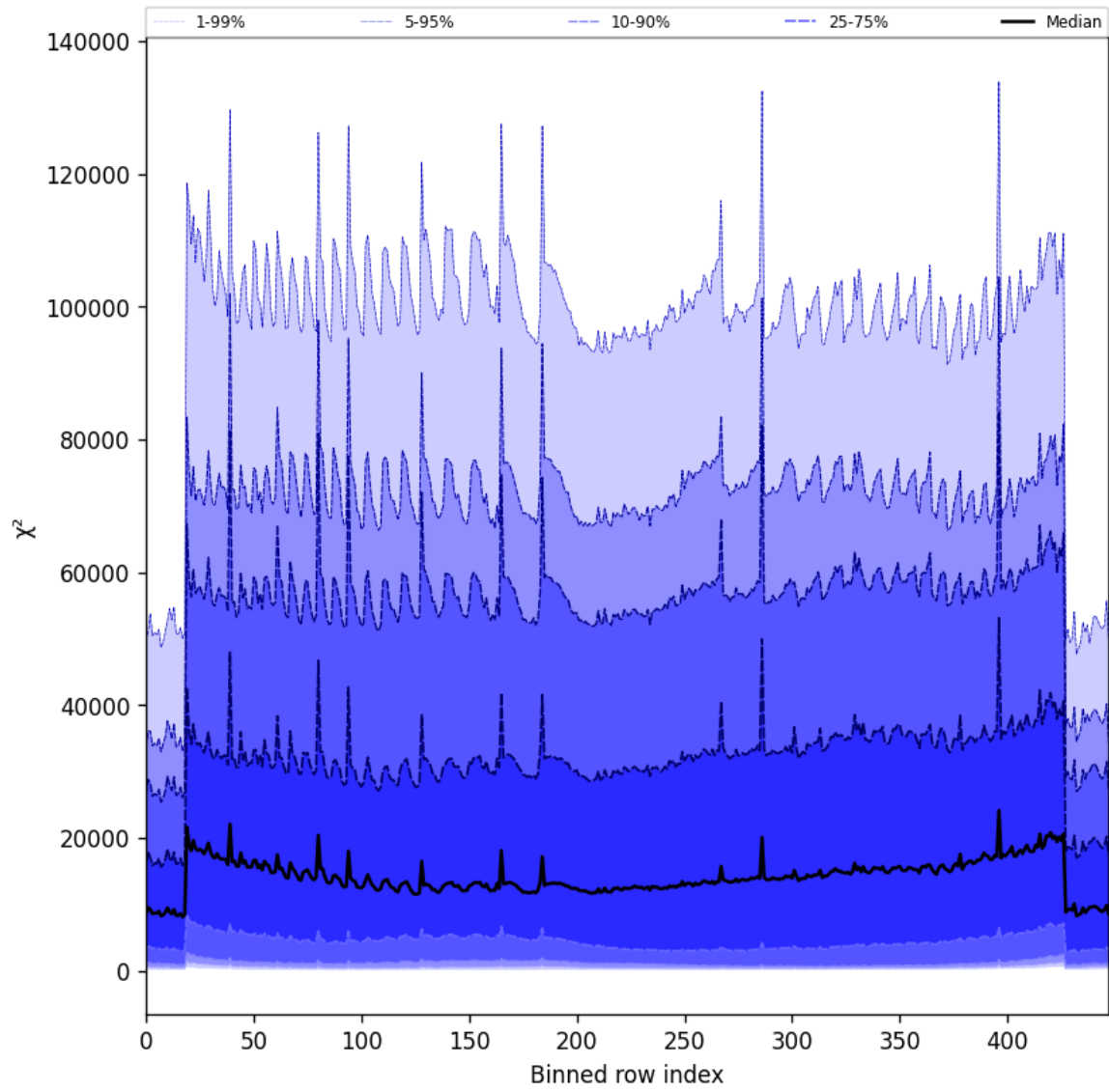
Figure 53: Along track statistics of “ \chi^2 ” for 2025-04-28 to 2025-04-29
