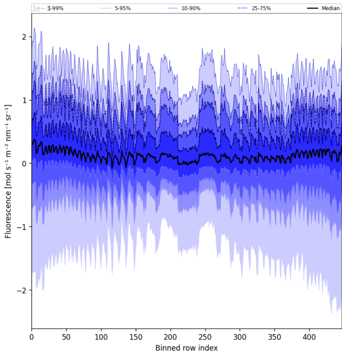
Figure 55: Along track statistics of “Fluorescence” for 2025-04-28 to 2025-04-29
