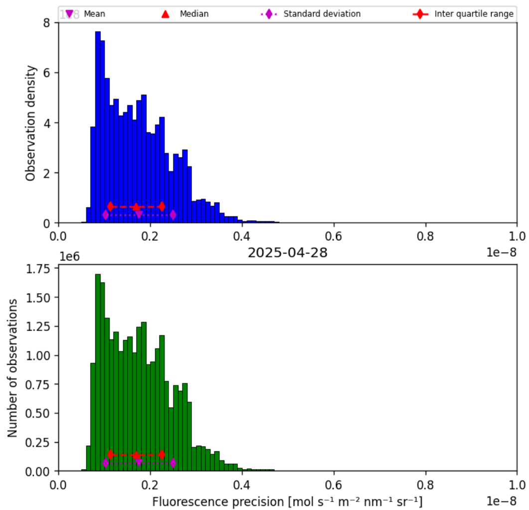
Figure 39: Histogram of “Fluorescence precision” for 2025-04-28 to 2025-04-29
