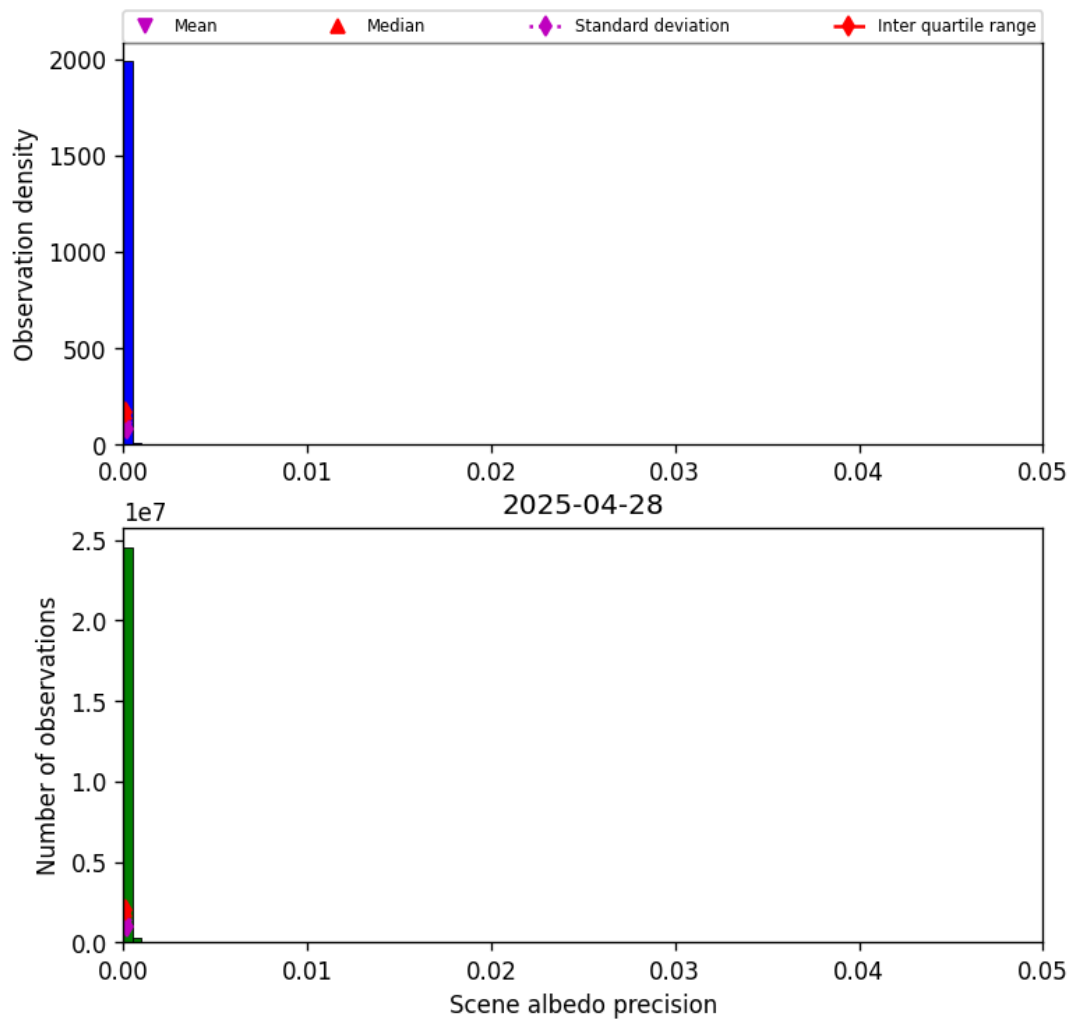
Figure 33: Histogram of “Scene albedo precision” for 2025-04-28 to 2025-04-29
