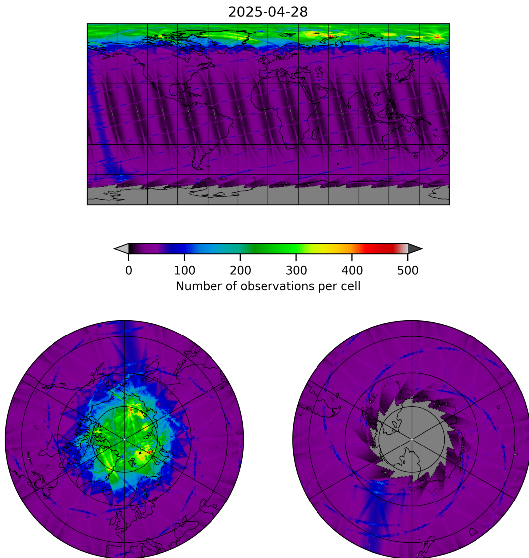
Figure 9: Map of the number of observations for 2025-04-28 to 2025-04-29
