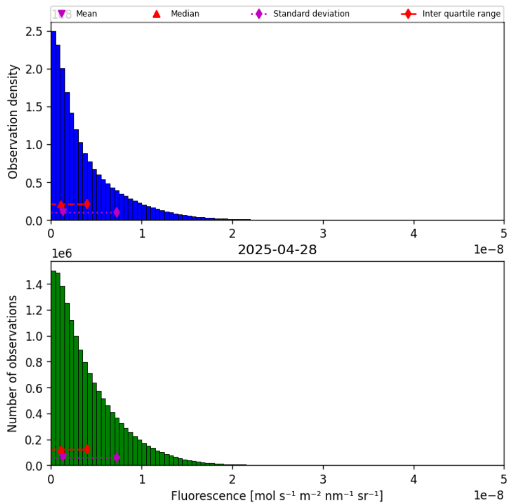
Figure 38: Histogram of “Fluorescence” for 2025-04-28 to 2025-04-29
