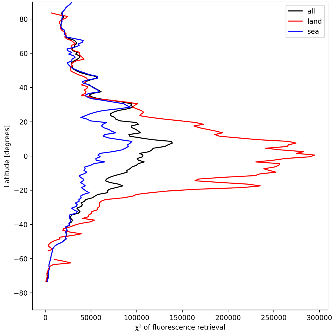
Figure 23: Zonal average of “ \chi^2 of fluorescence retrieval” for 2025-04-28 to 2025-04-29.
