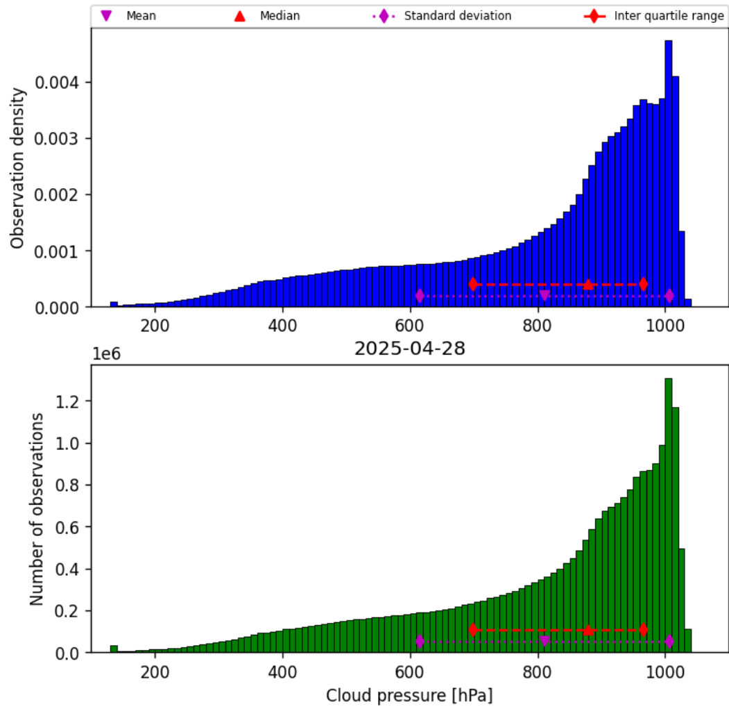
Figure 28: Histogram of “Cloud pressure” for 2025-04-28 to 2025-04-29
