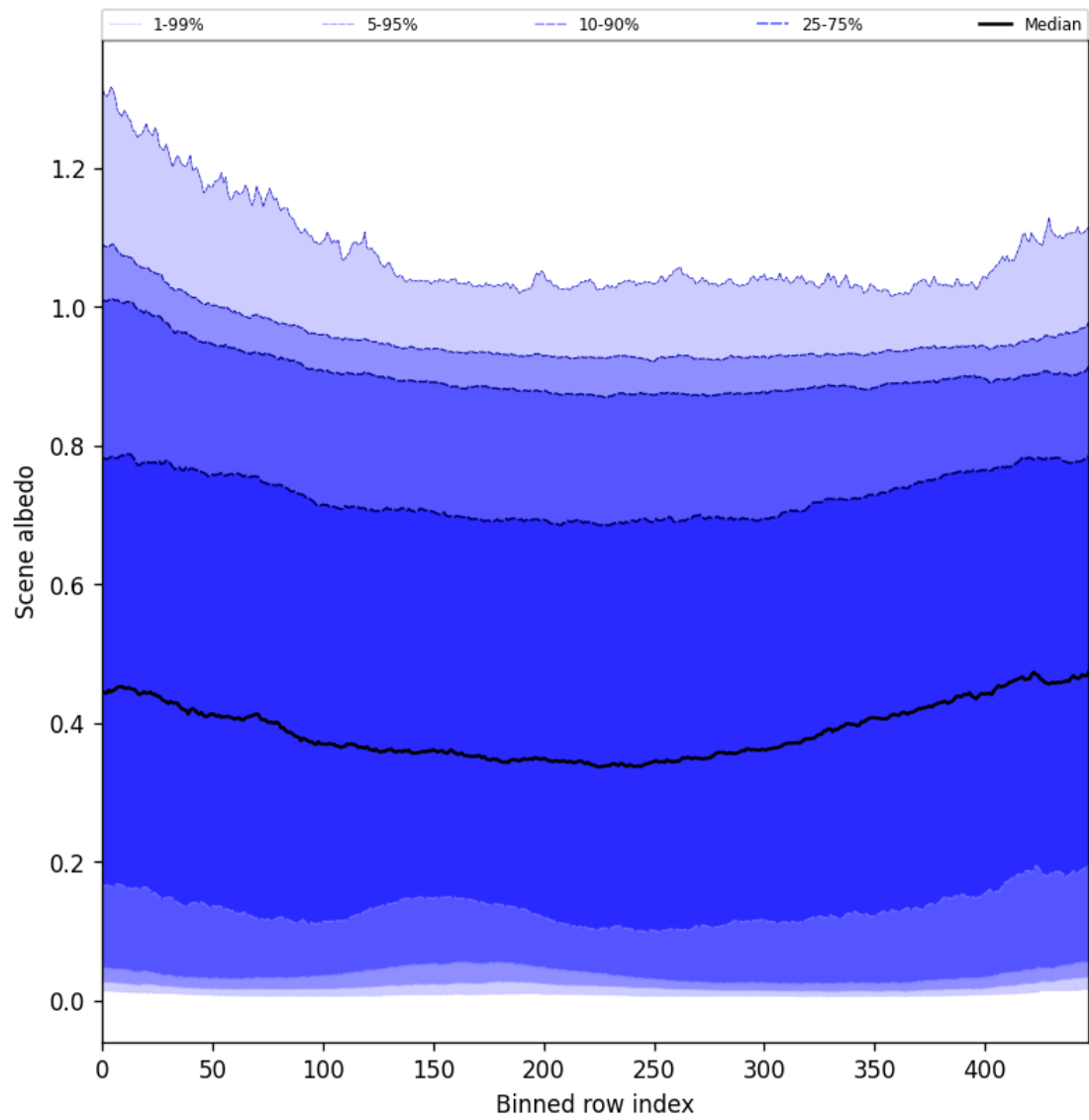
Figure 49: Along track statistics of “Scene albedo” for 2025-04-28 to 2025-04-29
