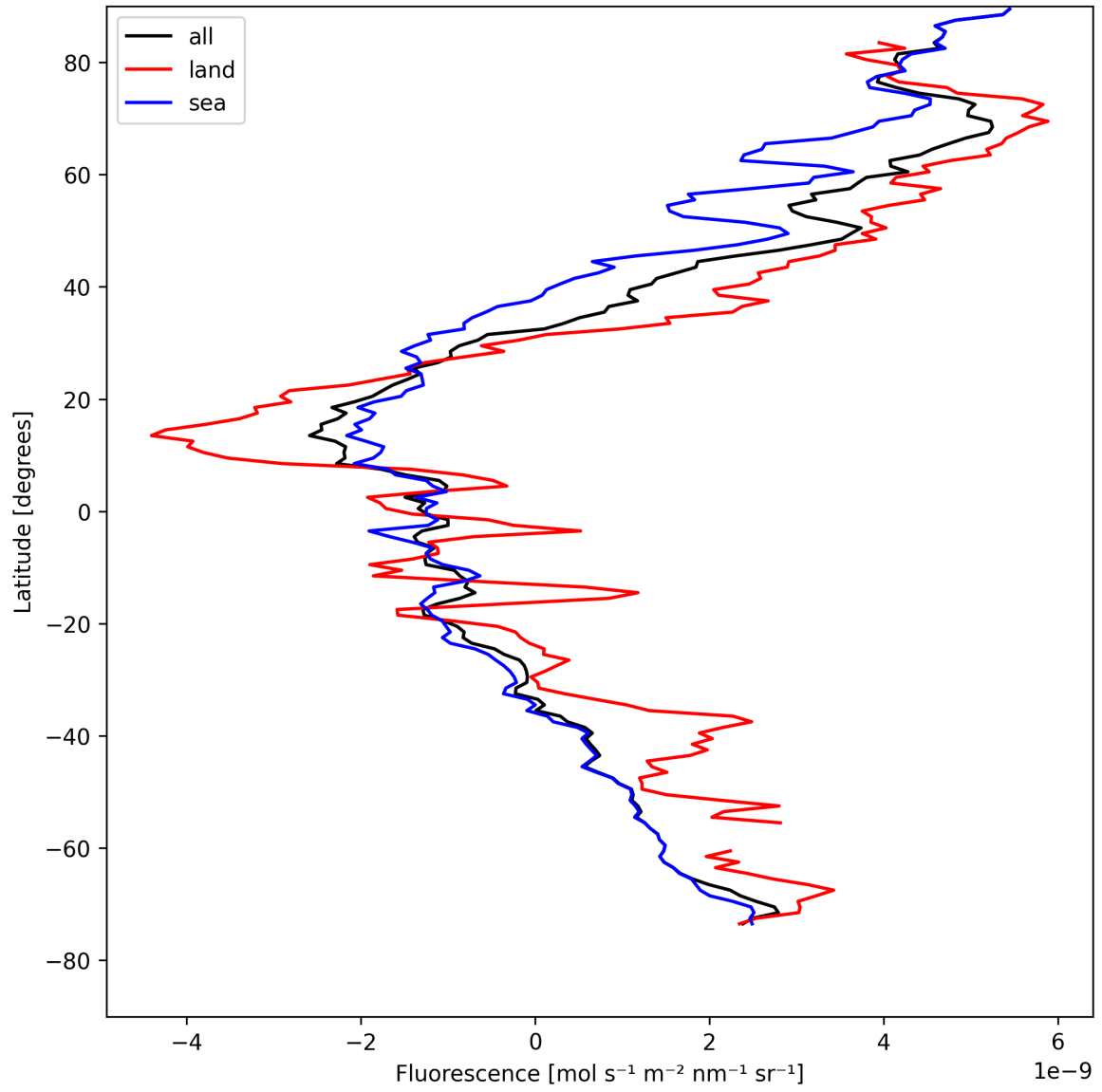
Figure 21: Zonal average of “Fluorescence” for 2025-04-28 to 2025-04-29.
