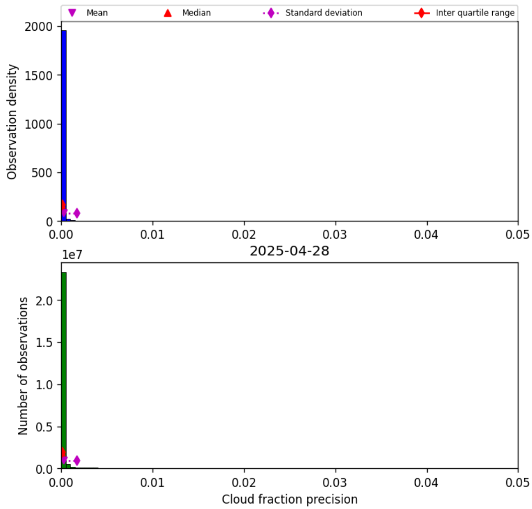
Figure 31: Histogram of “Cloud fraction precision” for 2025-04-28 to 2025-04-29
