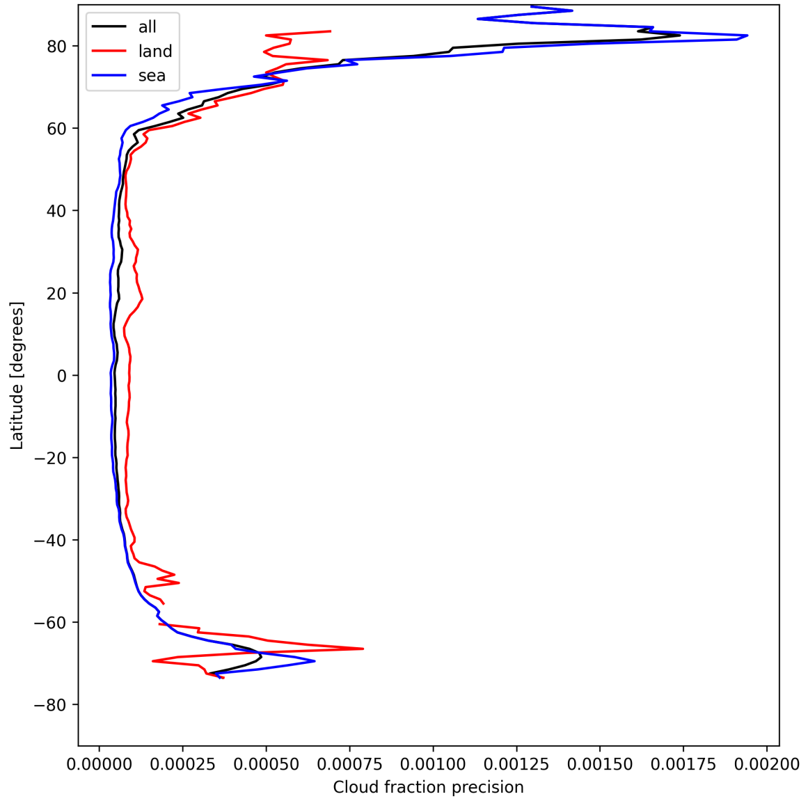
Figure 14: Zonal average of “Cloud fraction precision” for 2025-04-28 to 2025-04-29.
