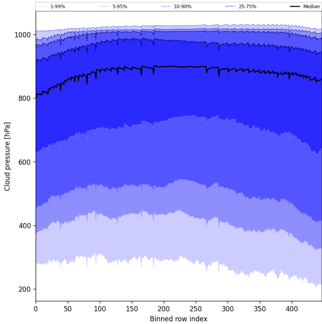
Figure 45: Along track statistics of “Cloud pressure” for 2025-04-28 to 2025-04-29
