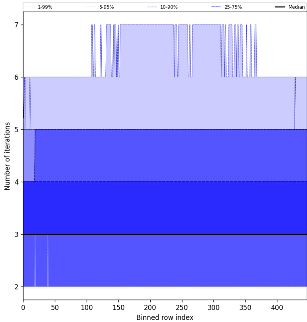
Figure 54: Along track statistics of “Number of iterations” for 2025-04-28 to 2025-04-29
