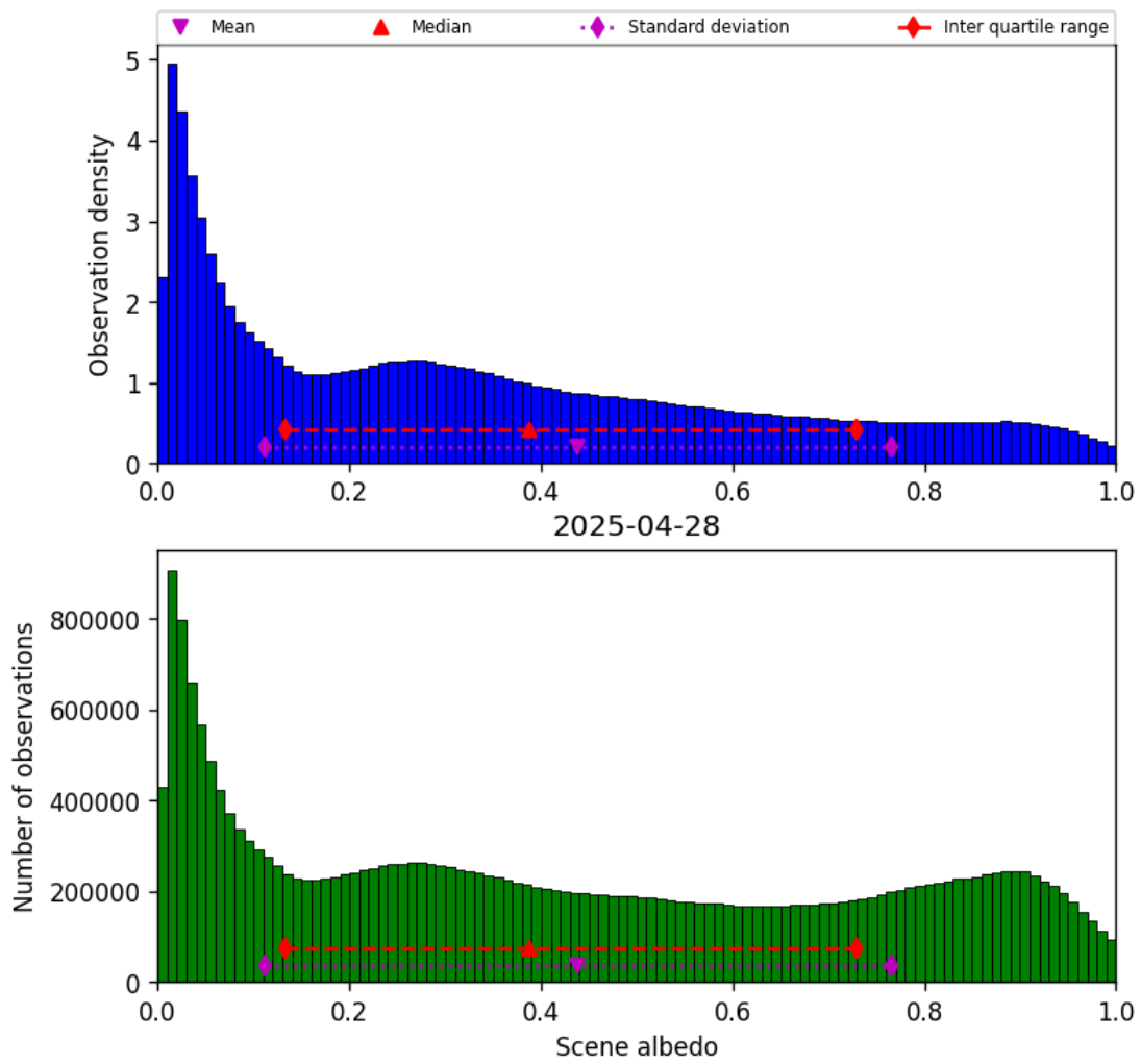
Figure 32: Histogram of “Scene albedo” for 2025-04-28 to 2025-04-29
