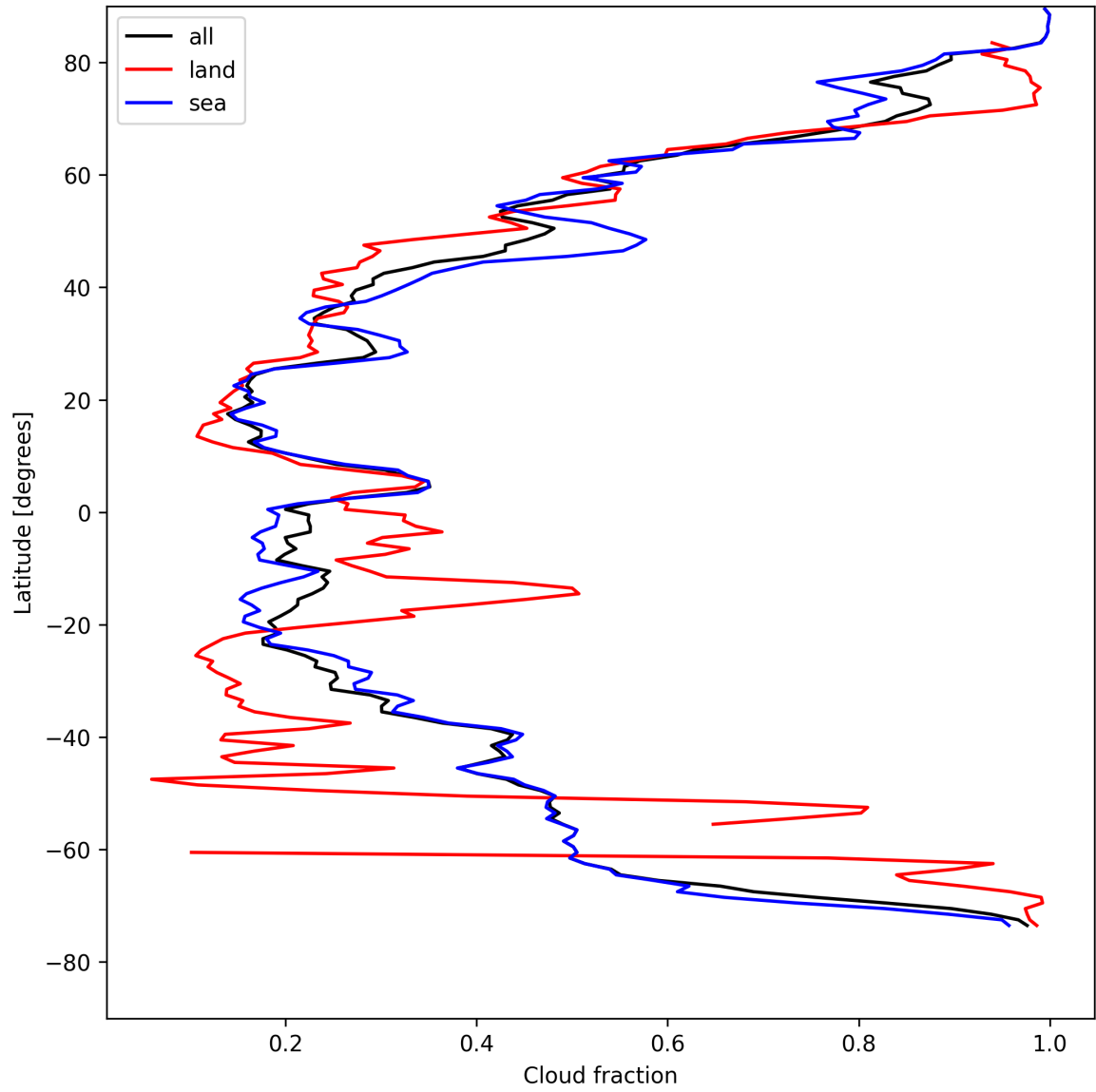
Figure 13: Zonal average of “Cloud fraction” for 2025-04-28 to 2025-04-29.
