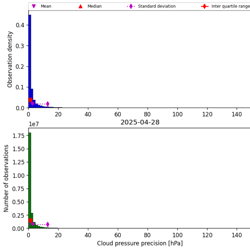
Figure 29: Histogram of “Cloud pressure precision” for 2025-04-28 to 2025-04-29
