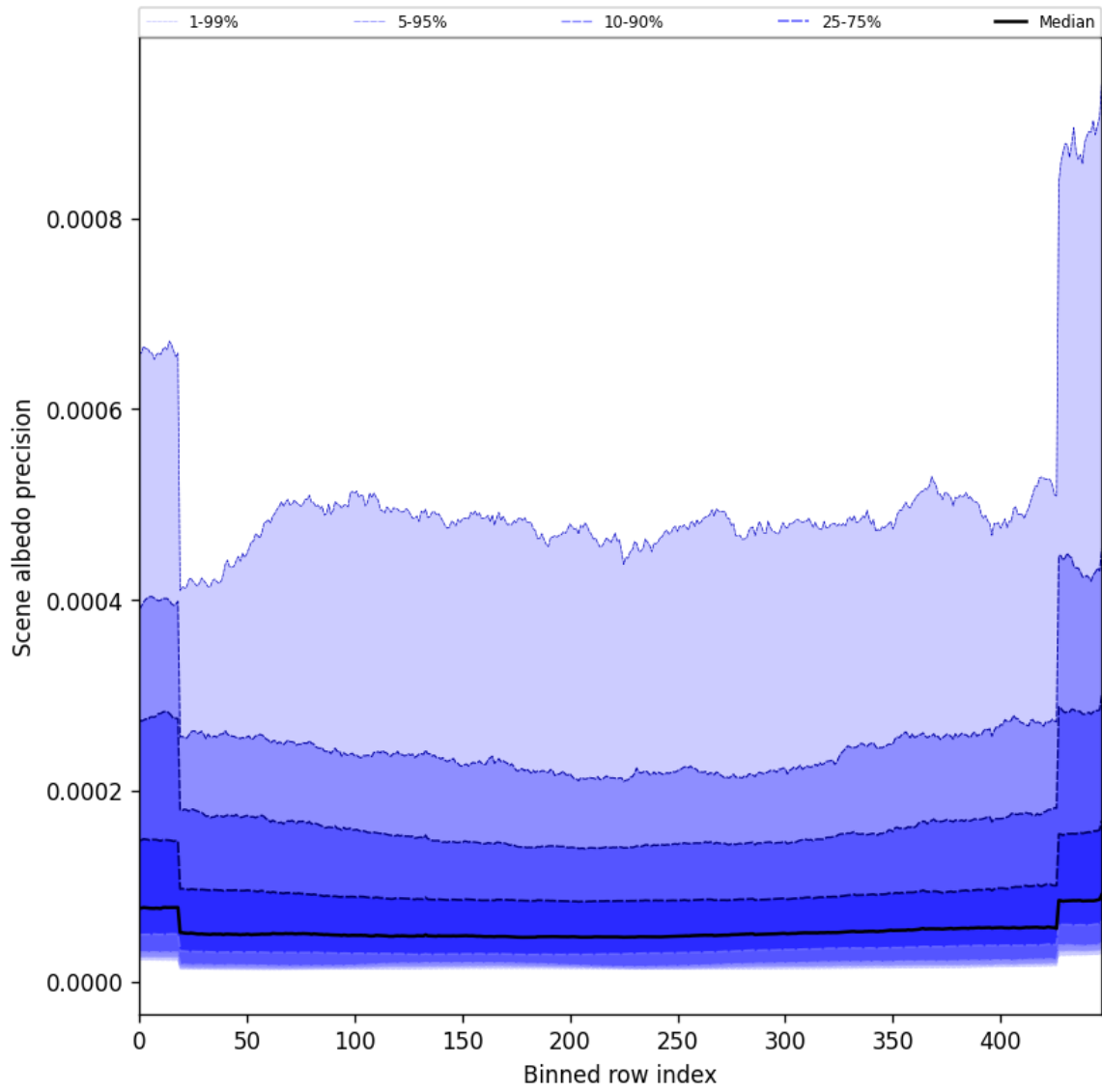
Figure 50: Along track statistics of “Scene albedo precision” for 2025-04-28 to 2025-04-29
