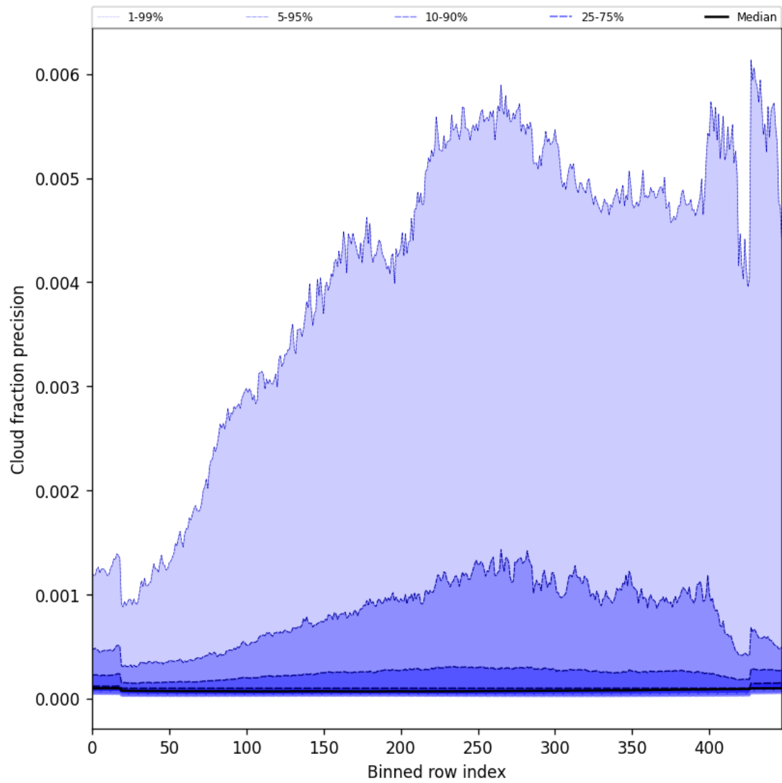
Figure 48: Along track statistics of “Cloud fraction precision” for 2025-04-28 to 2025-04-29
