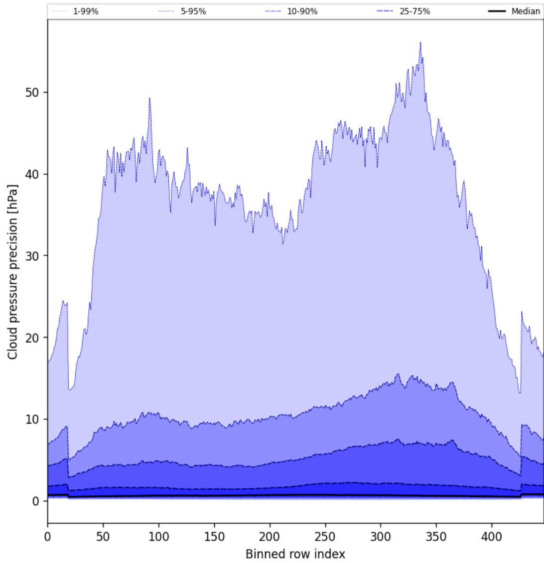
Figure 46: Along track statistics of “Cloud pressure precision” for 2025-04-28 to 2025-04-29
