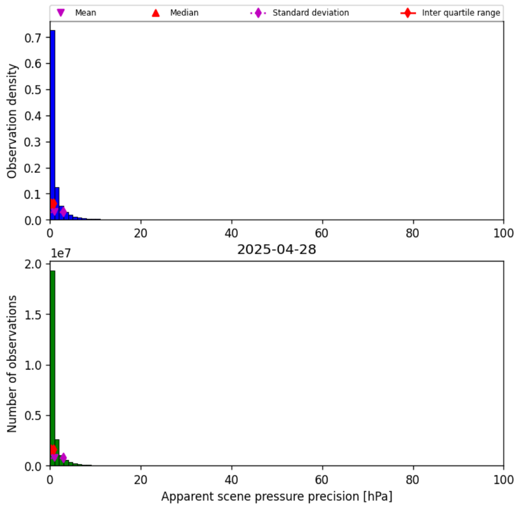
Figure 35: Histogram of “Apparent scene pressure precision” for 2025-04-28 to 2025-04-29
