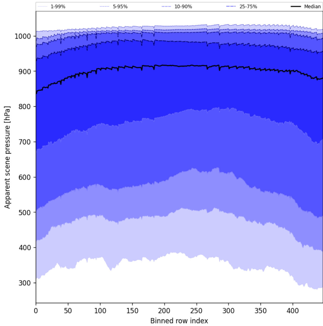
Figure 51: Along track statistics of “Apparent scene pressure” for 2025-04-28 to 2025-04-29
