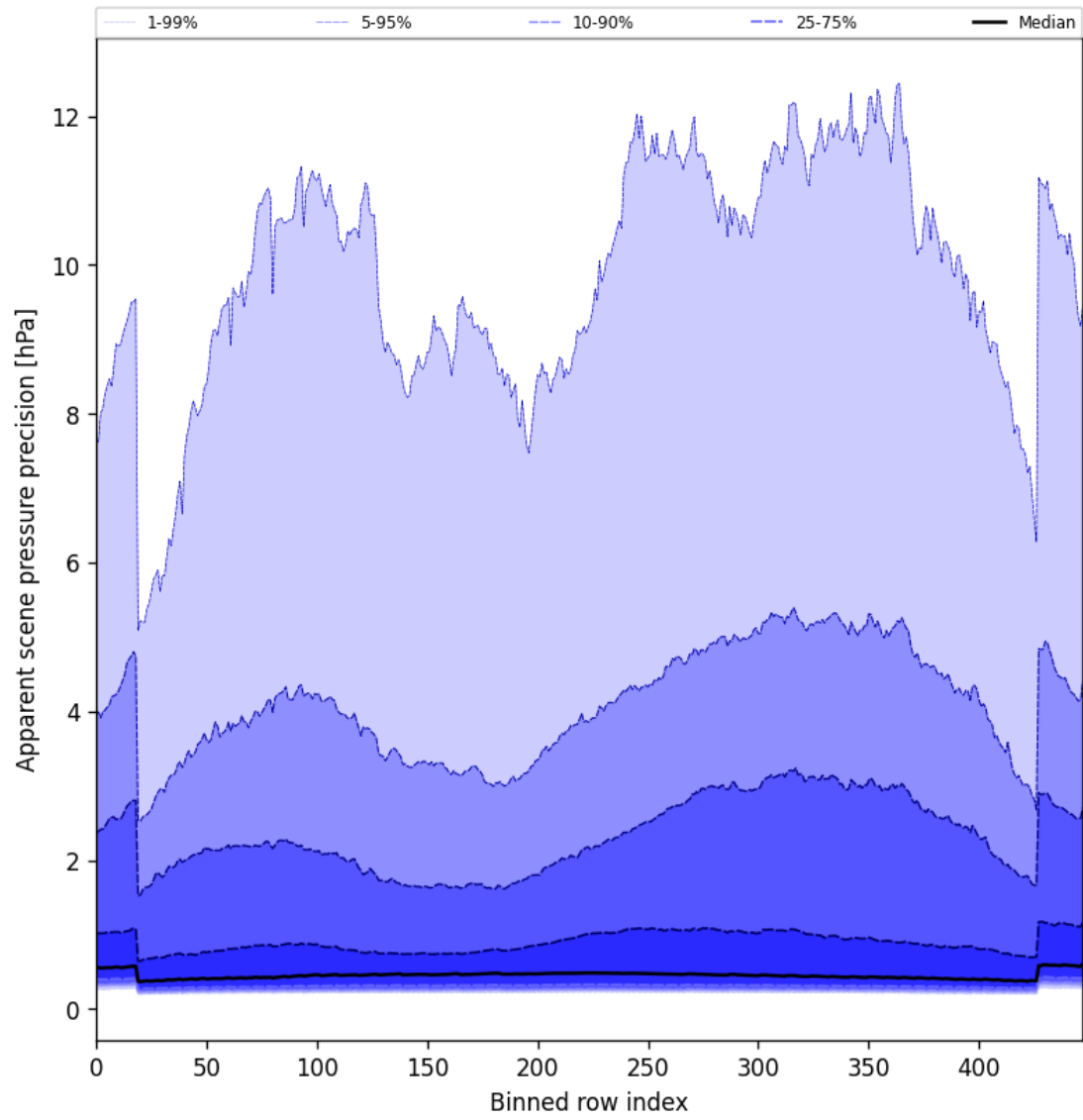
Figure 52: Along track statistics of “Apparent scene pressure precision” for 2025-04-28 to 2025-04-29
