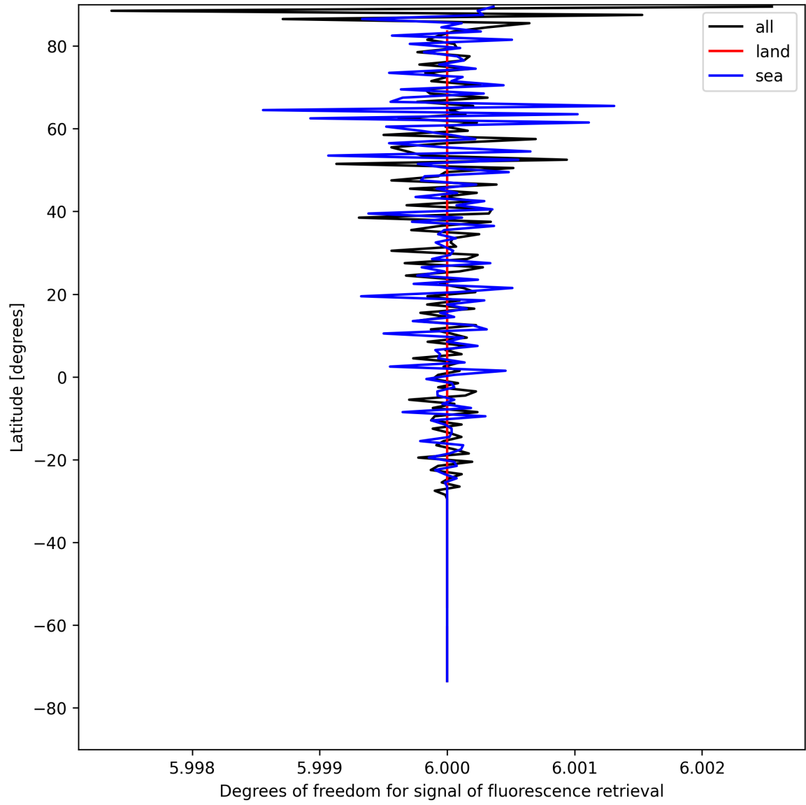
Figure 24: Zonal average of “Degrees of freedom for signal of fluorescence retrieval” for 2025-04-28 to 2025-04-29.
