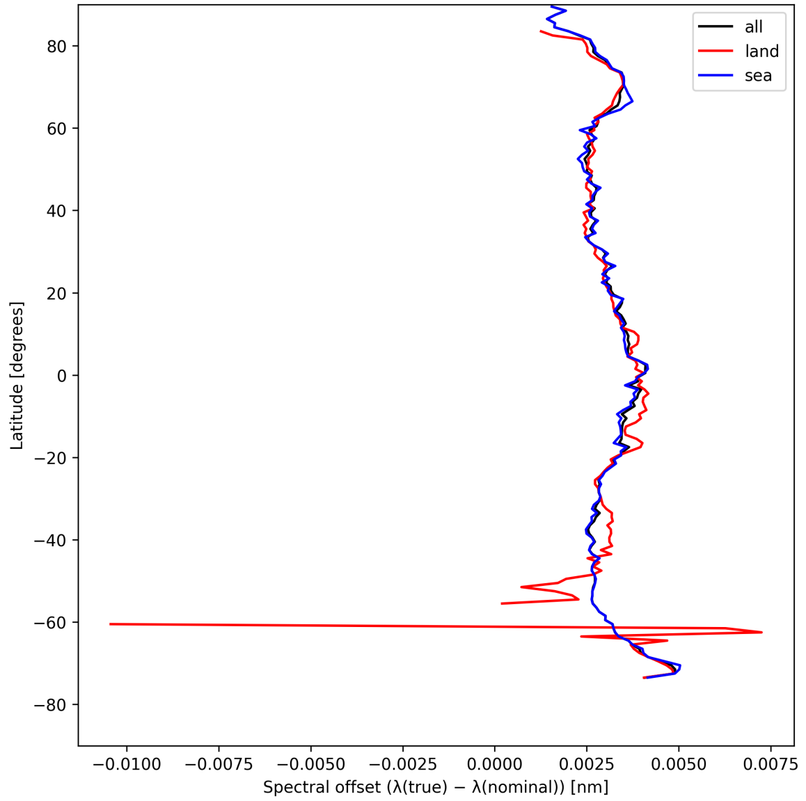
Figure 26: Zonal average of “Spectral offset ( \lambda_{\text{true}} - \lambda_{\text{nominal}} )” for 2025-04-28 to 2025-04-29.
