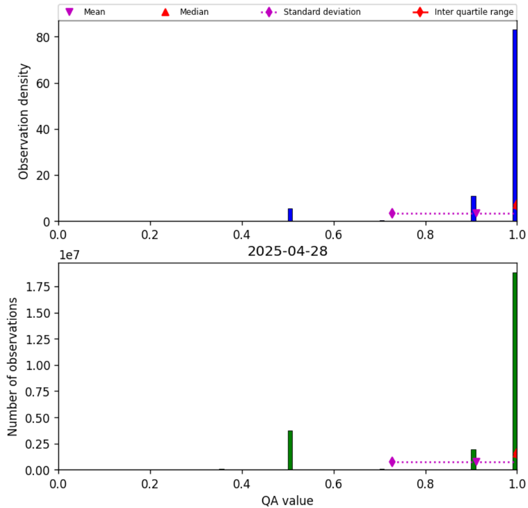
Figure 27: Histogram of “QA value” for 2025-04-28 to 2025-04-29
