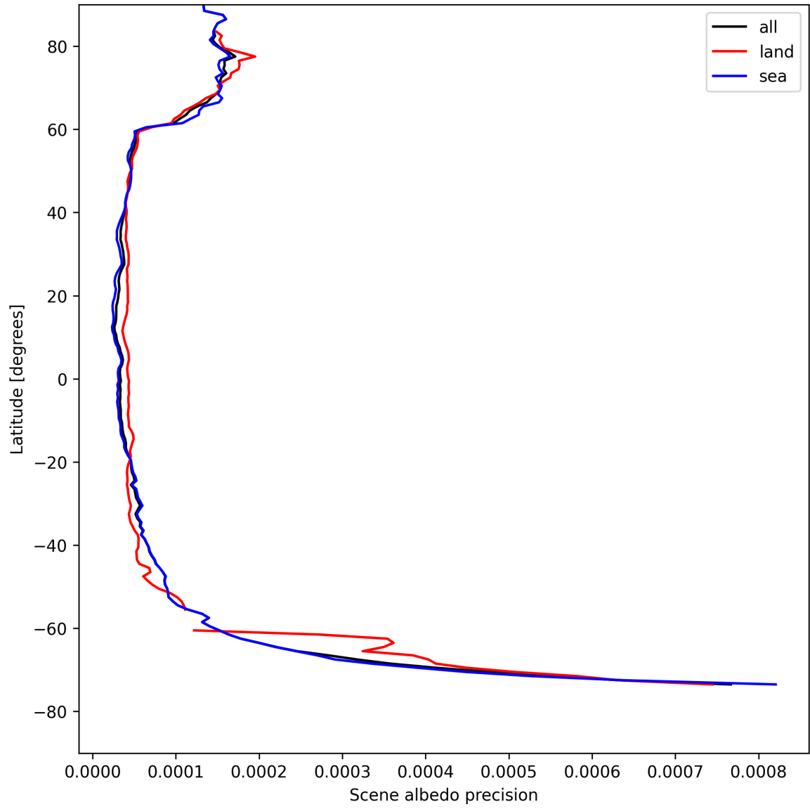
Figure 16: Zonal average of “Scene albedo precision” for 2025-04-28 to 2025-04-29.
