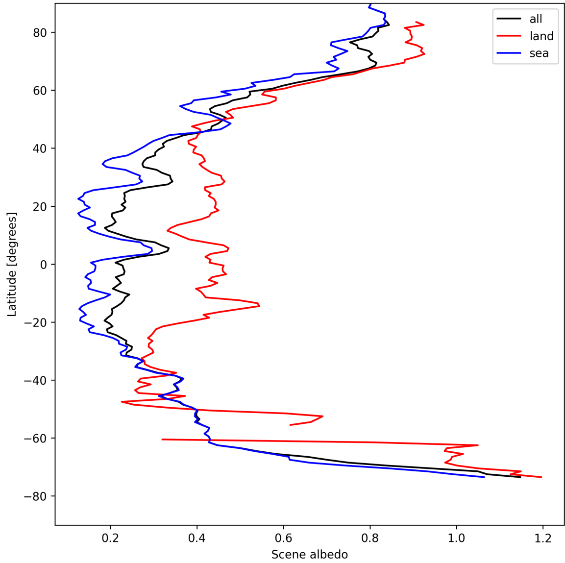
Figure 15: Zonal average of “Scene albedo” for 2025-04-28 to 2025-04-29.
