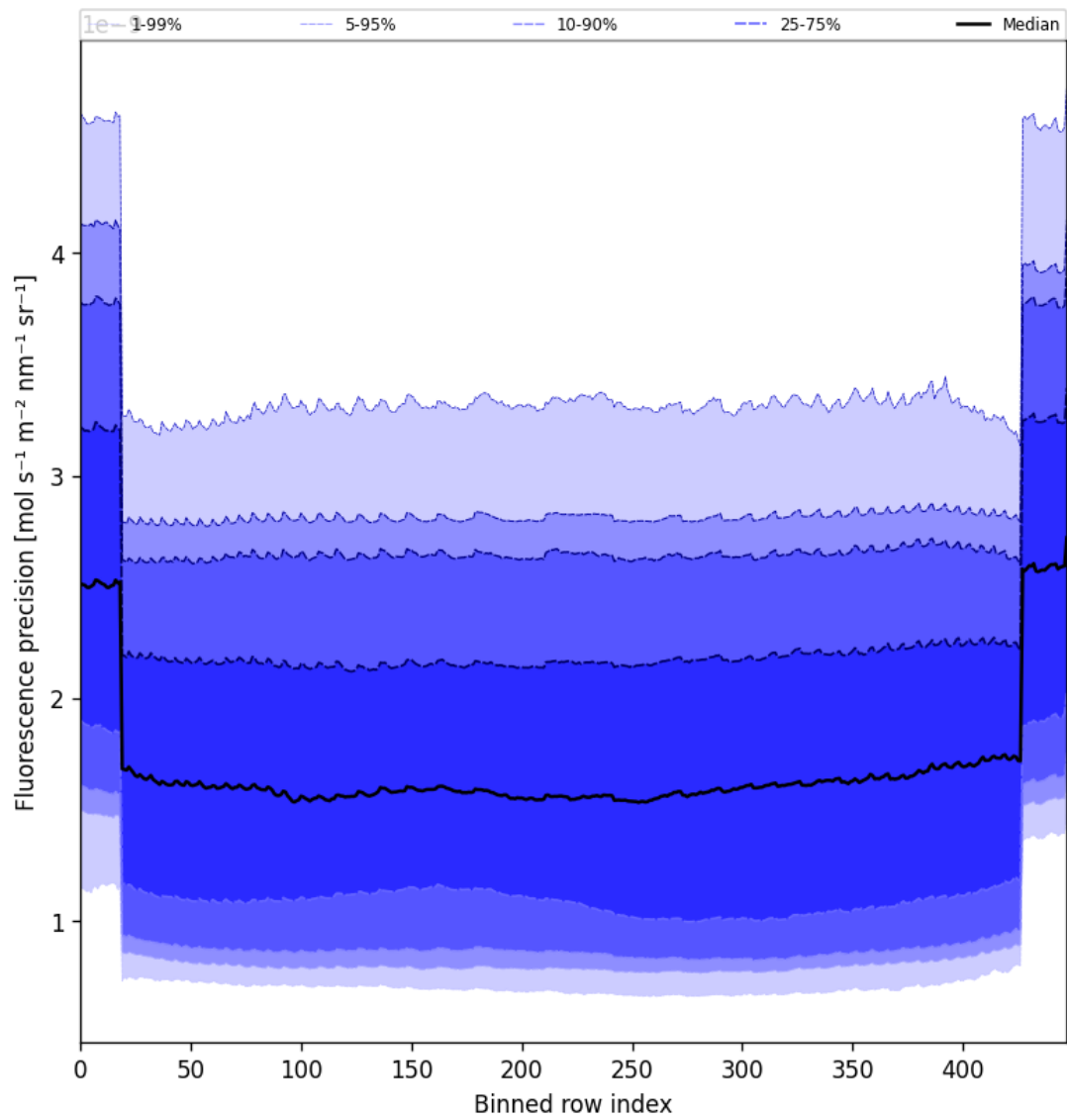
Figure 56: Along track statistics of “Fluorescence precision” for 2025-04-28 to 2025-04-29
