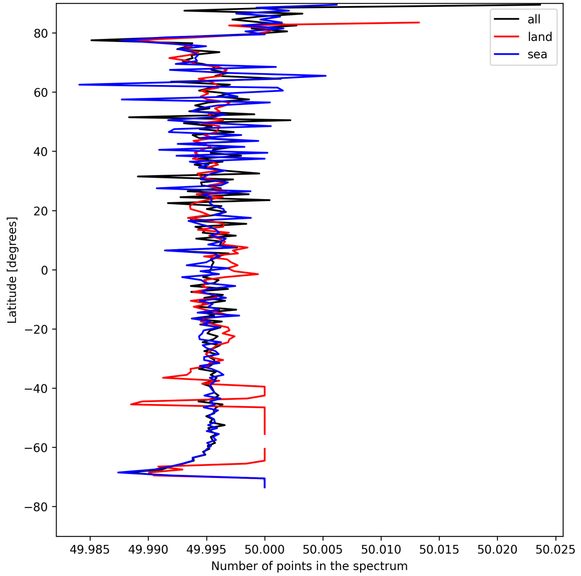
Figure 25: Zonal average of “Number of points in the spectrum” for 2025-04-28 to 2025-04-29.
