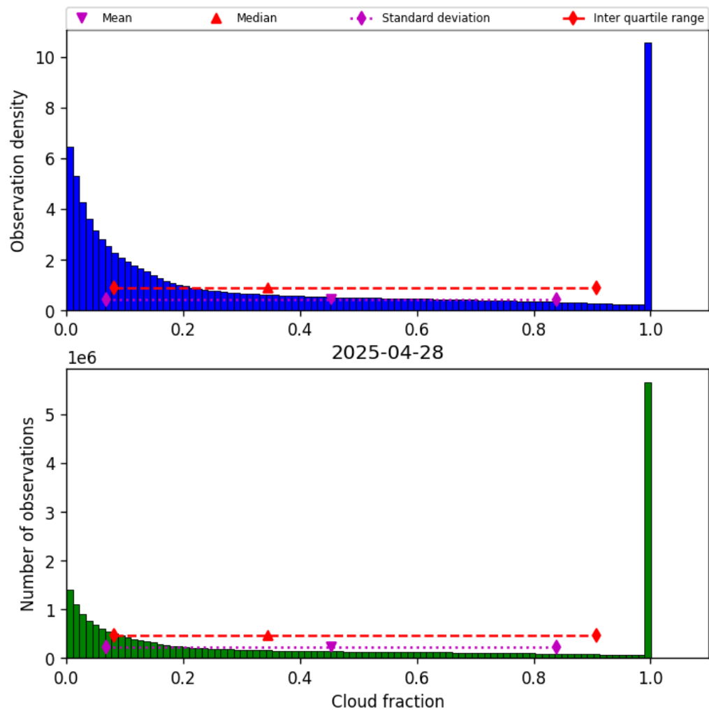
Figure 30: Histogram of “Cloud fraction” for 2025-04-28 to 2025-04-29
