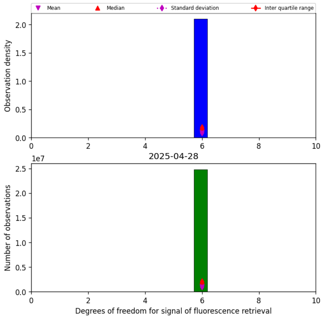
Figure 41: Histogram of “Degrees of freedom for signal of fluorescence retrieval” for 2025-04-28 to 2025-04-29
