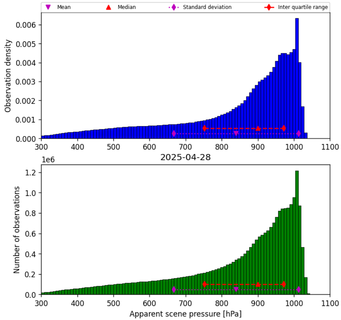
Figure 34: Histogram of “Apparent scene pressure” for 2025-04-28 to 2025-04-29
