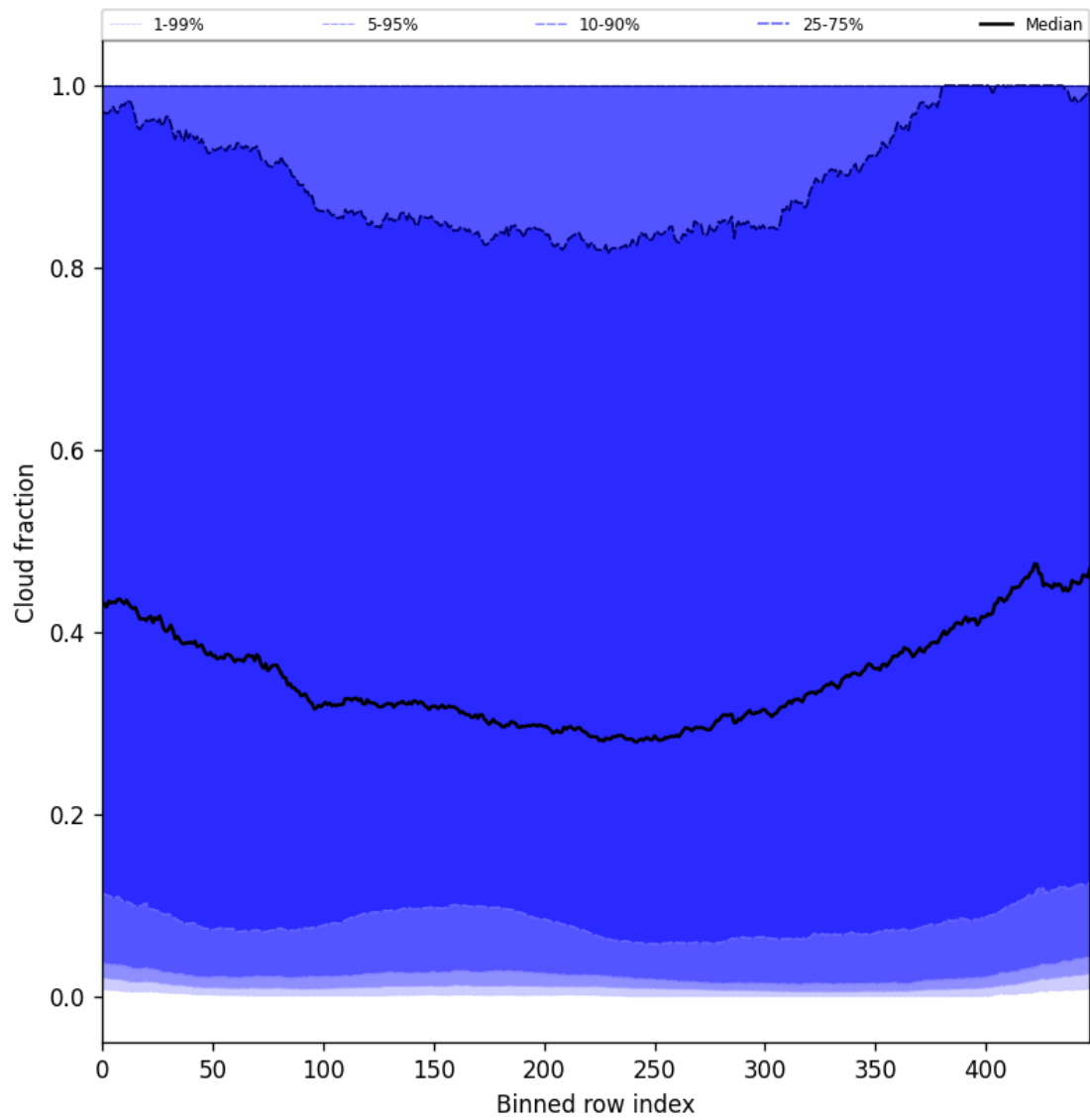
Figure 47: Along track statistics of “Cloud fraction” for 2025-04-28 to 2025-04-29
