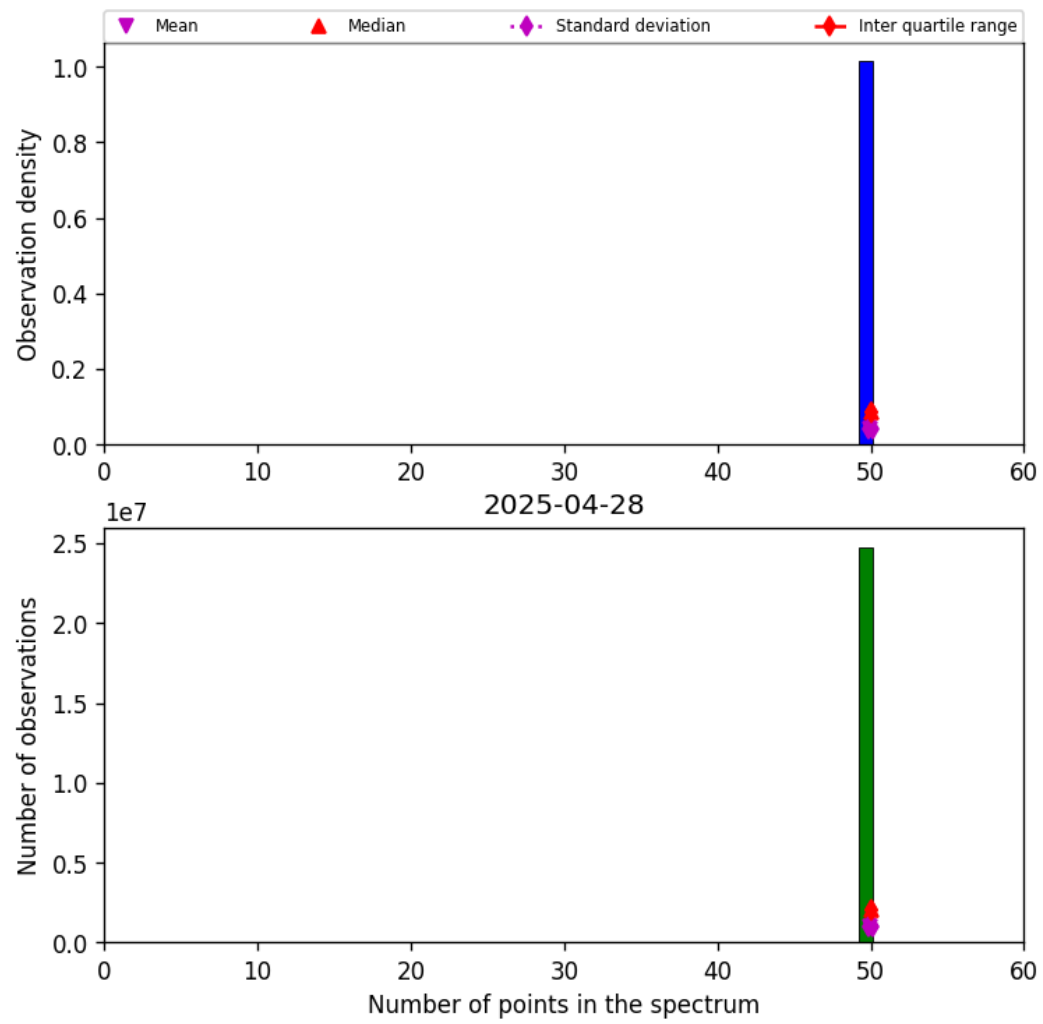
Figure 42: Histogram of “Number of points in the spectrum” for 2025-04-28 to 2025-04-29
