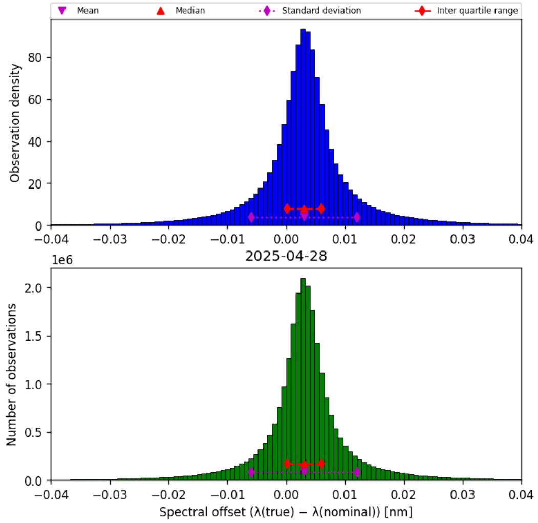
Figure 43: Histogram of “Spectral offset ( \lambda_{\text{true}} - \lambda_{\text{nominal}} )” for 2025-04-28 to 2025-04-29
