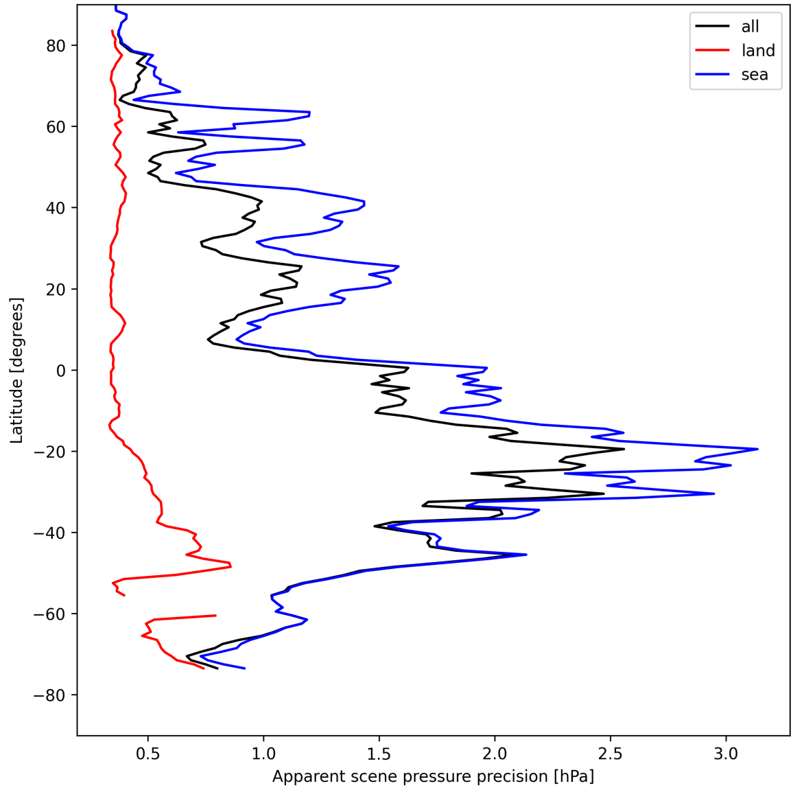
Figure 18: Zonal average of “Apparent scene pressure precision” for 2025-04-28 to 2025-04-29.
