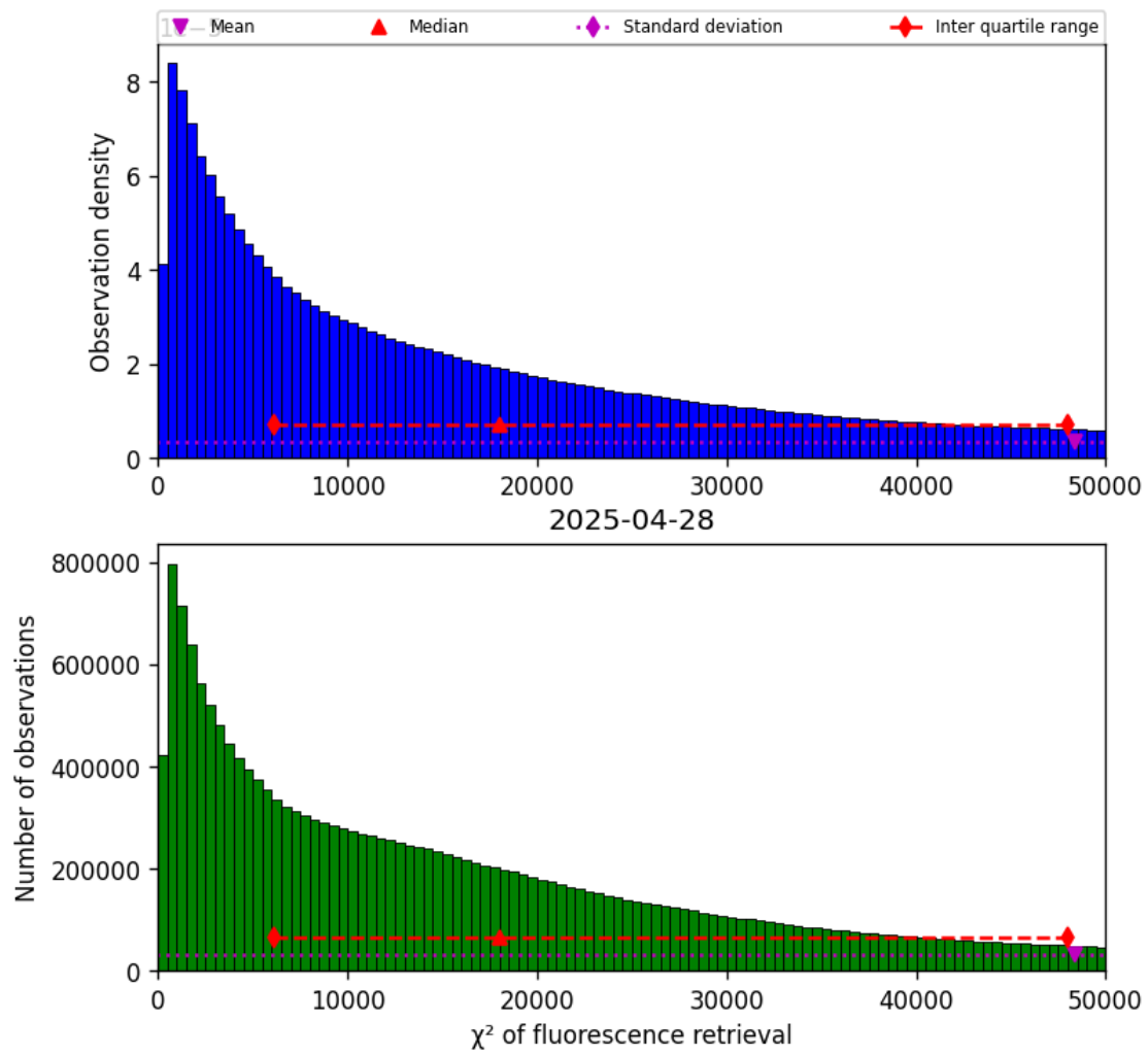
Figure 40: Histogram of “ \chi^2 of fluorescence retrieval” for 2025-04-28 to 2025-04-29
