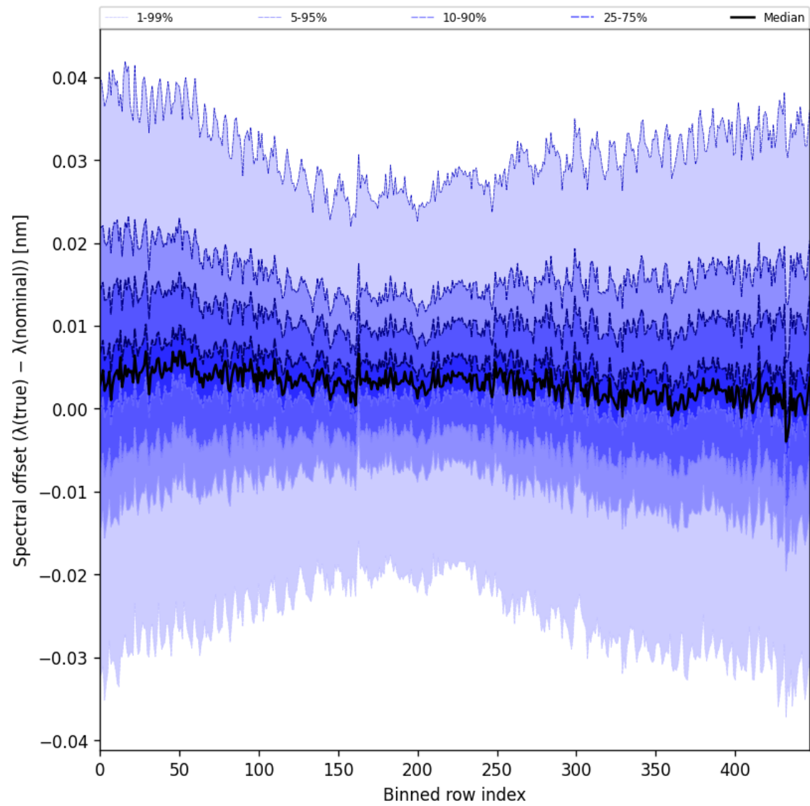
Figure 60: Along track statistics of “Spectral offset ( \lambda_{\text{true}} - \lambda_{\text{nominal}} )” for 2025-04-28 to 2025-04-29
