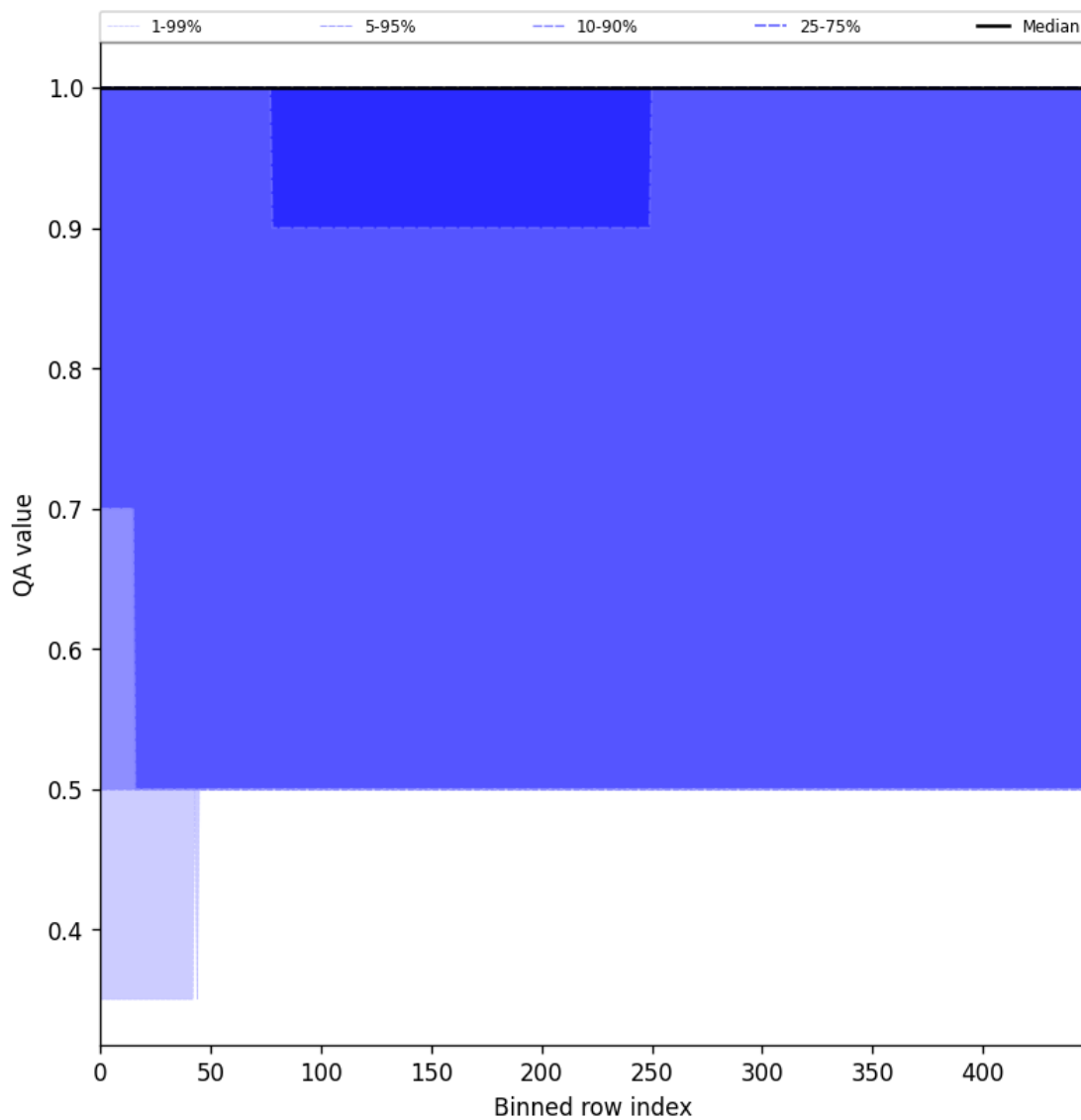
Figure 44: Along track statistics of “QA value” for 2025-04-28 to 2025-04-29
