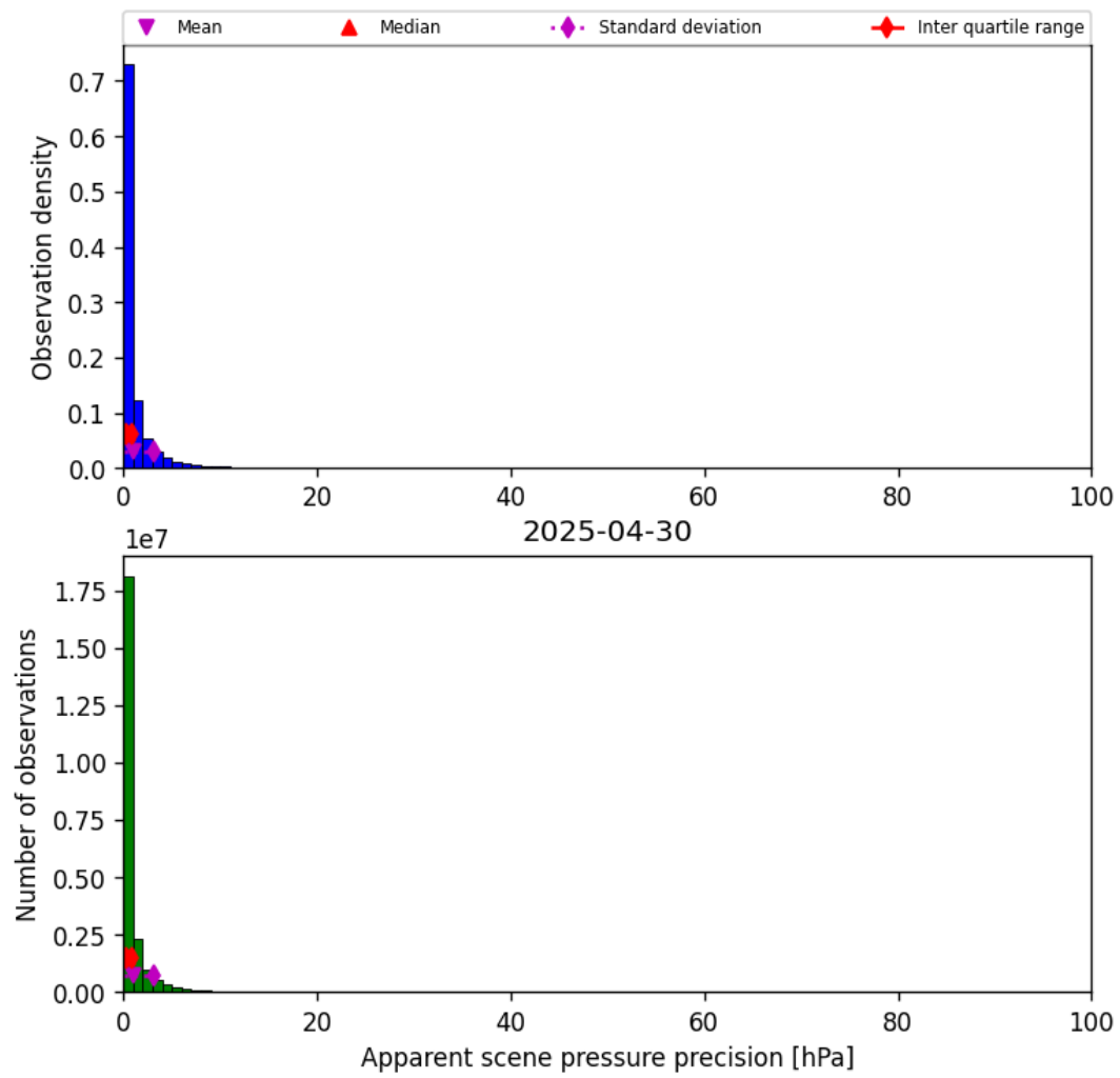
Figure 35: Histogram of “Apparent scene pressure precision” for 2025-04-30 to 2025-05-01
