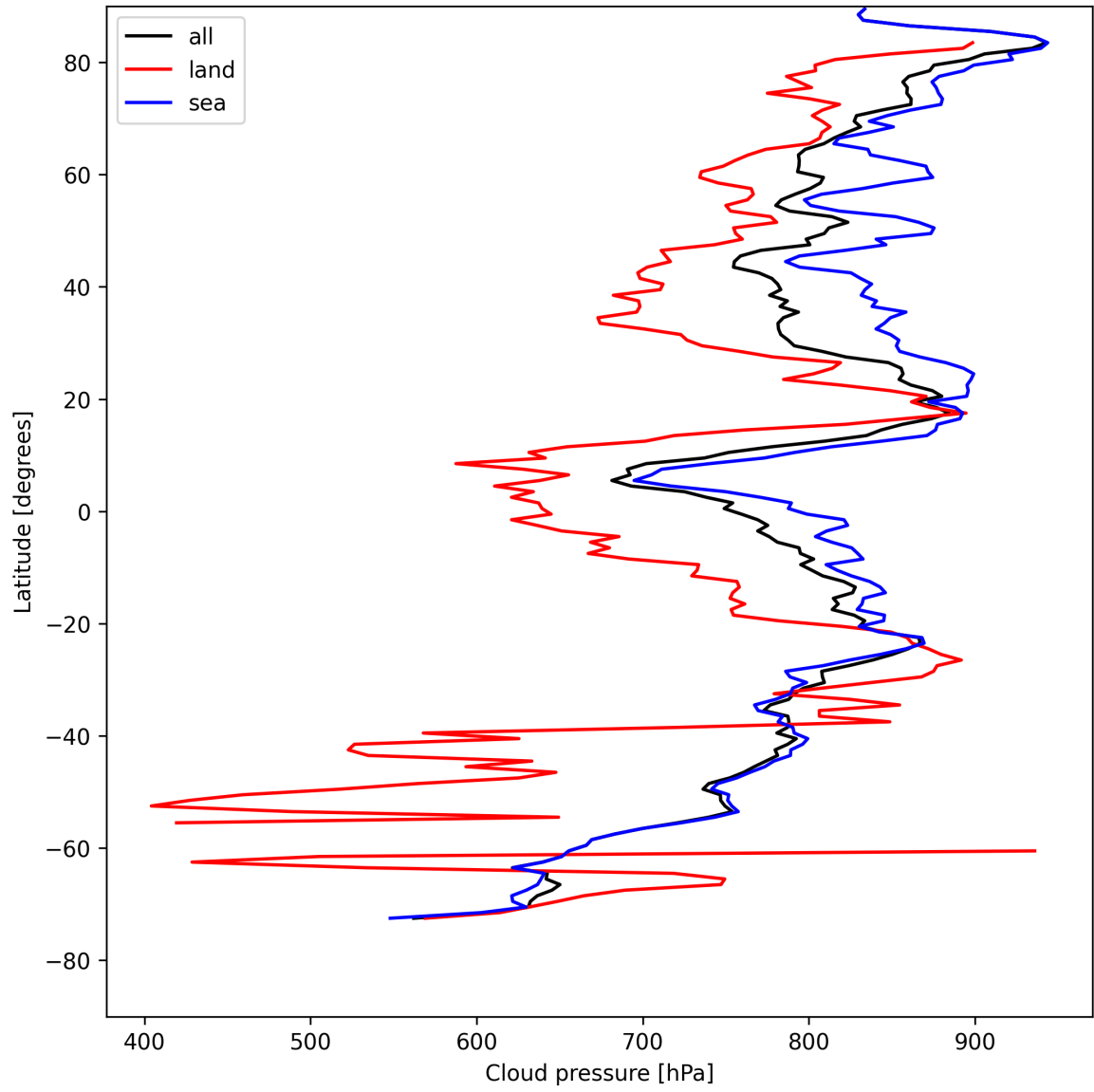
Figure 11: Zonal average of “Cloud pressure” for 2025-04-30 to 2025-05-01.
