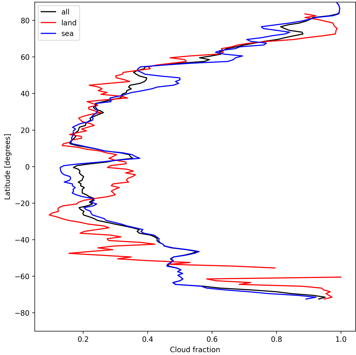
Figure 13: Zonal average of “Cloud fraction” for 2025-04-30 to 2025-05-01.
