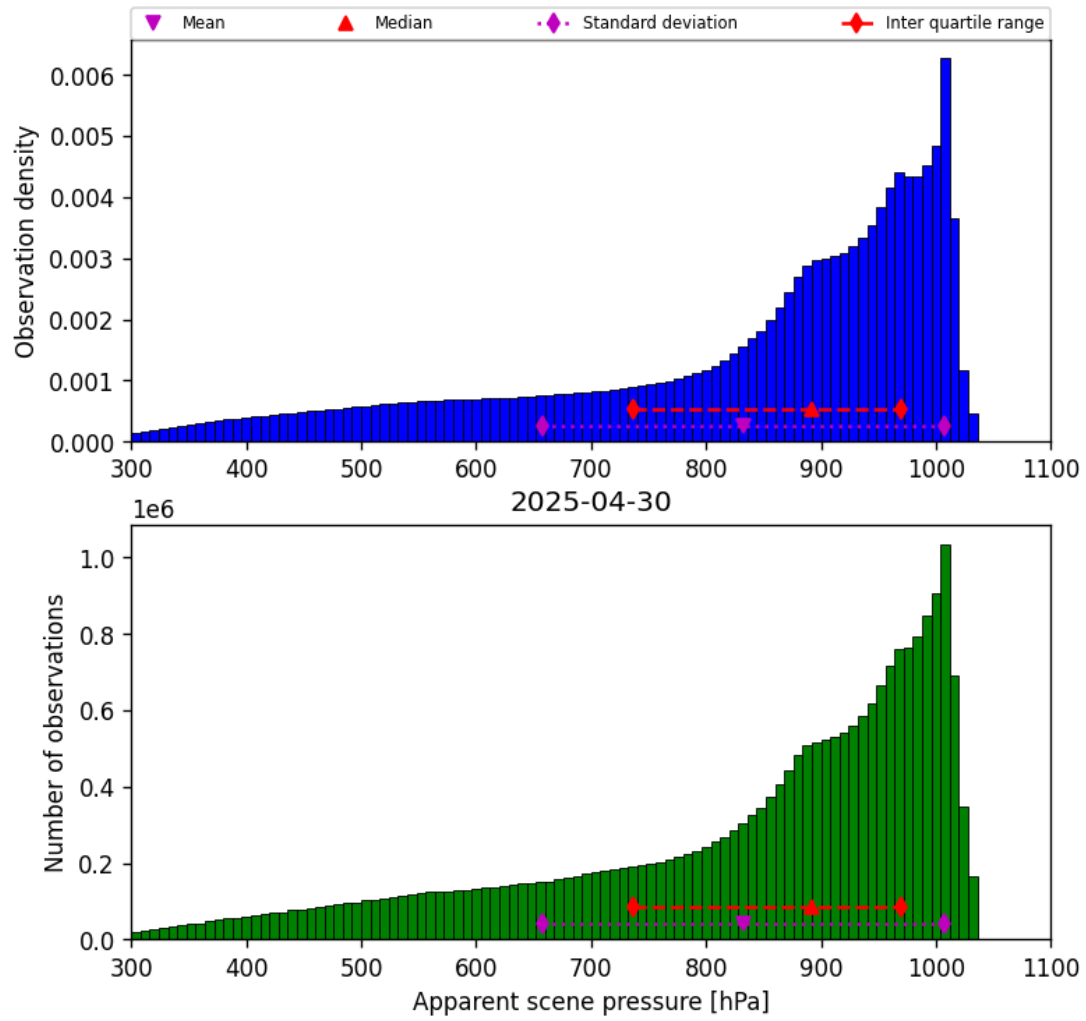
Figure 34: Histogram of “Apparent scene pressure” for 2025-04-30 to 2025-05-01
