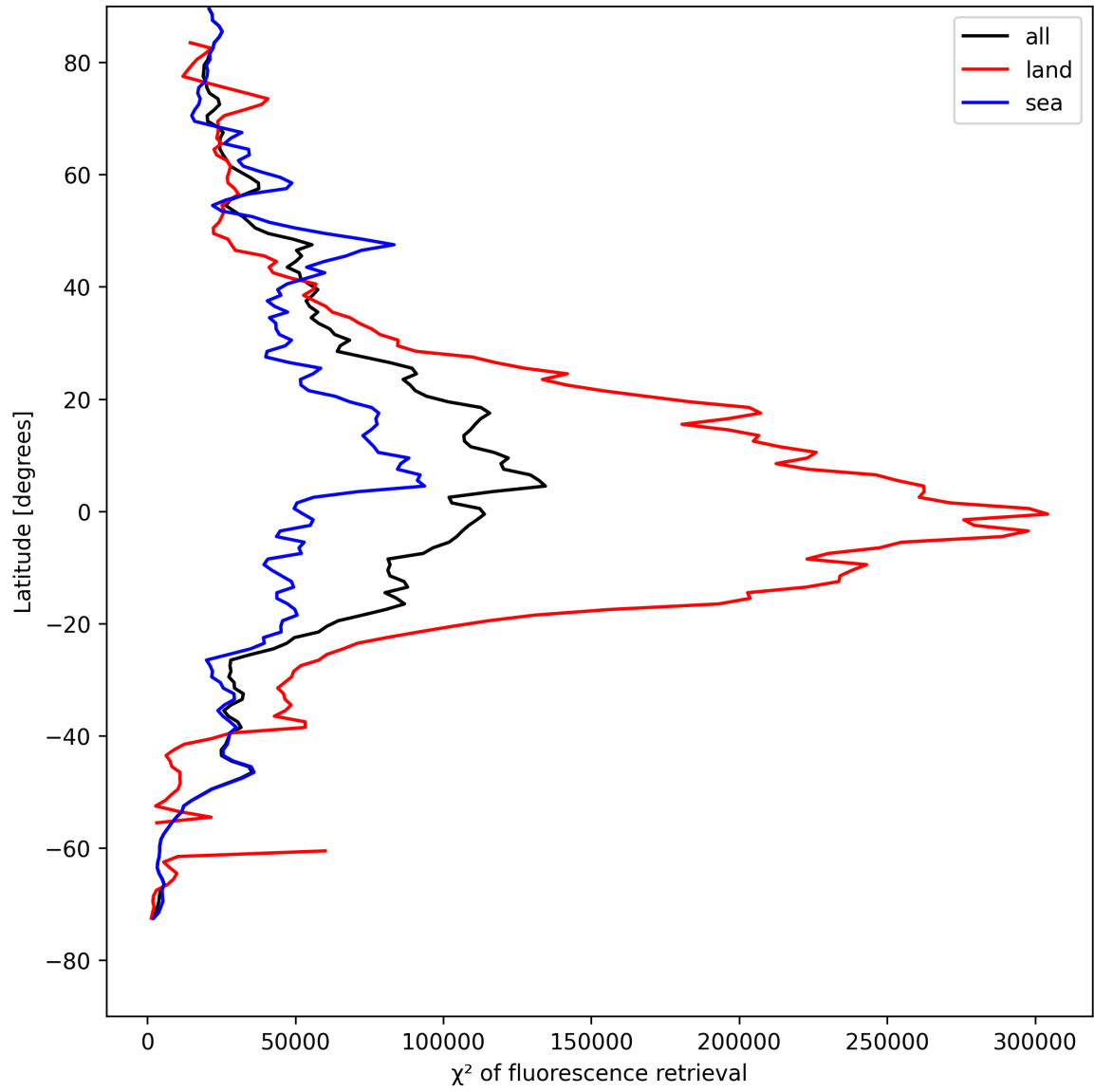
Figure 23: Zonal average of “ \chi^2 of fluorescence retrieval” for 2025-04-30 to 2025-05-01.
