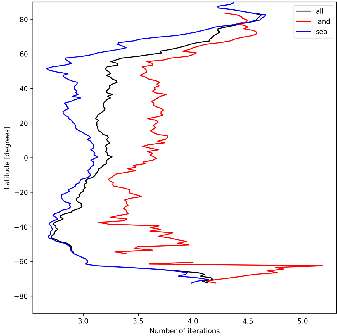
Figure 20: Zonal average of “Number of iterations” for 2025-04-30 to 2025-05-01.
