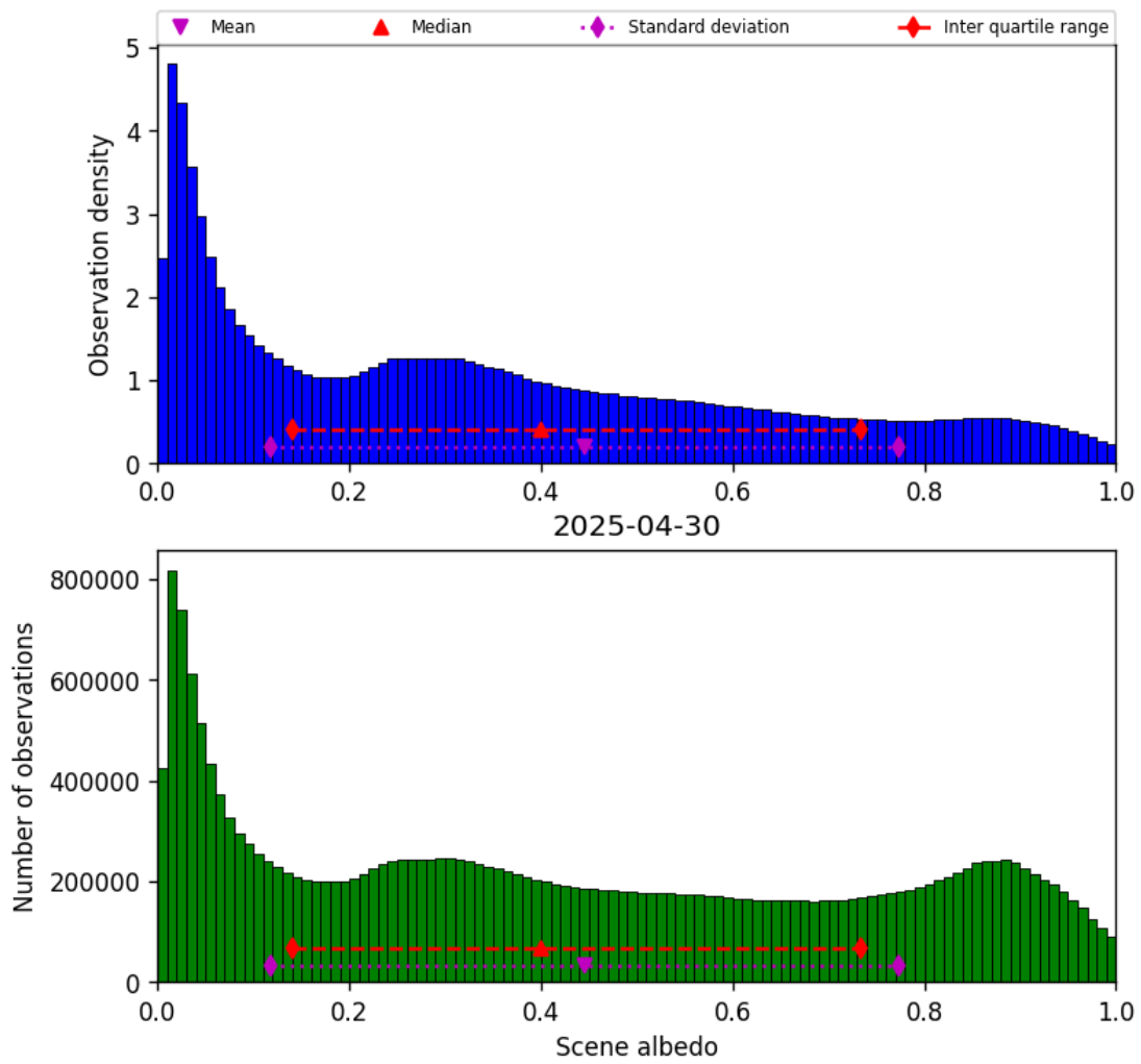
Figure 32: Histogram of “Scene albedo” for 2025-04-30 to 2025-05-01
