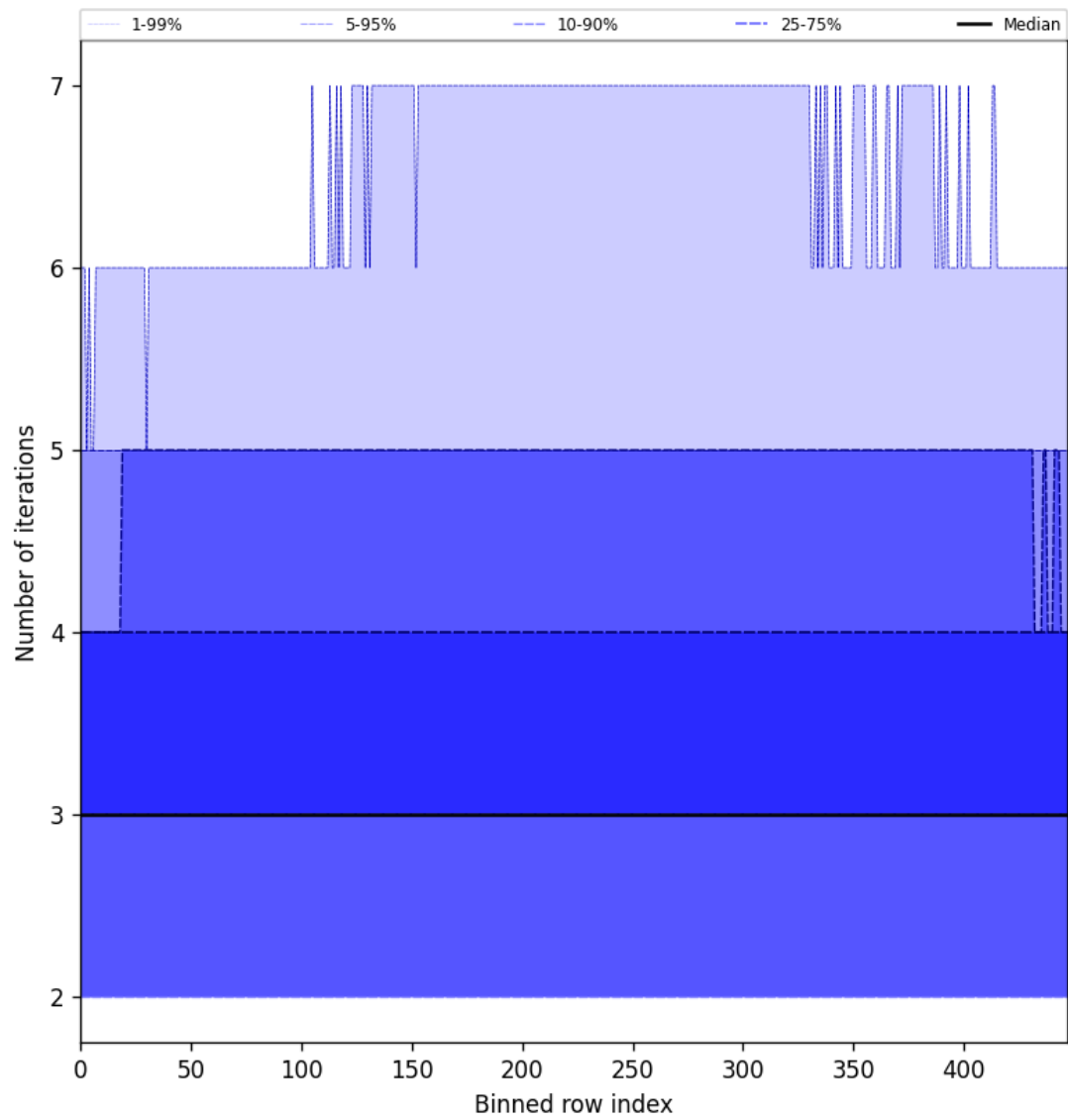
Figure 54: Along track statistics of “Number of iterations” for 2025-04-30 to 2025-05-01
