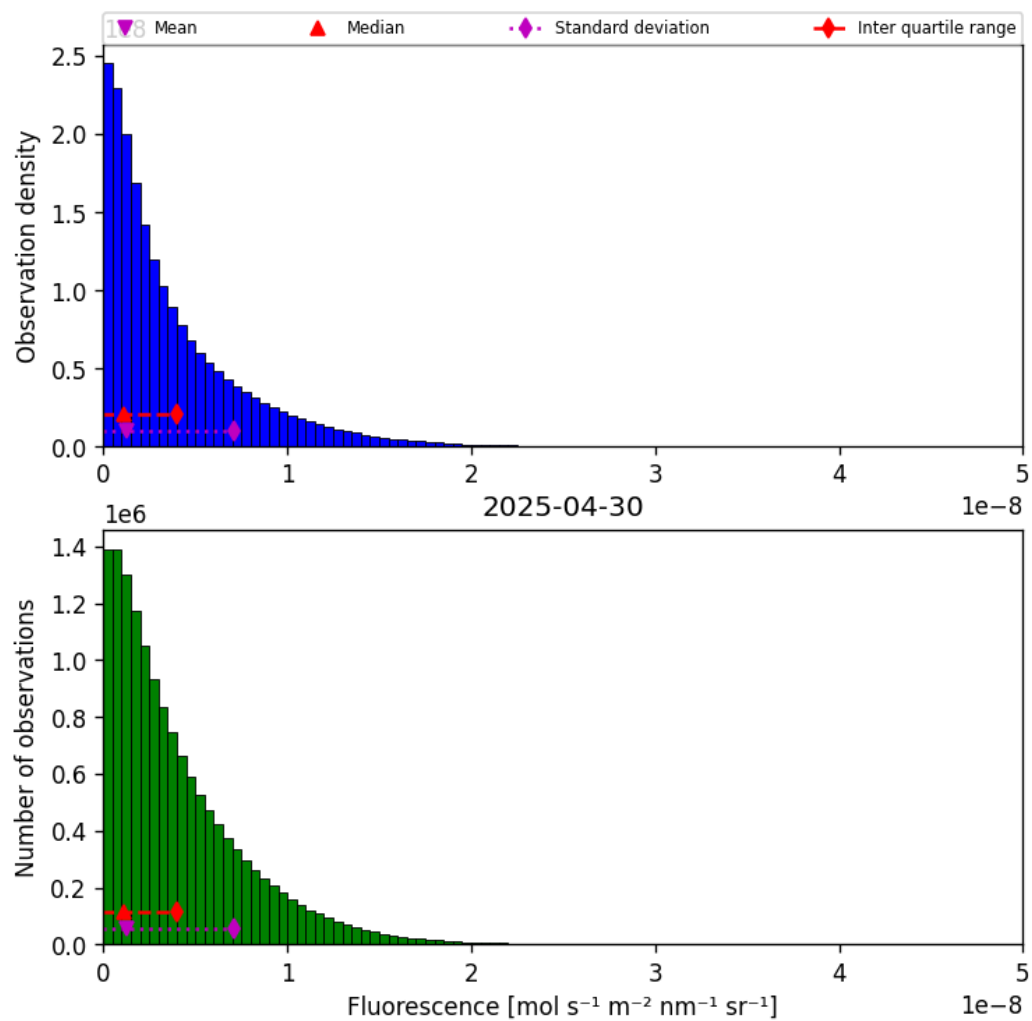
Figure 38: Histogram of “Fluorescence” for 2025-04-30 to 2025-05-01
