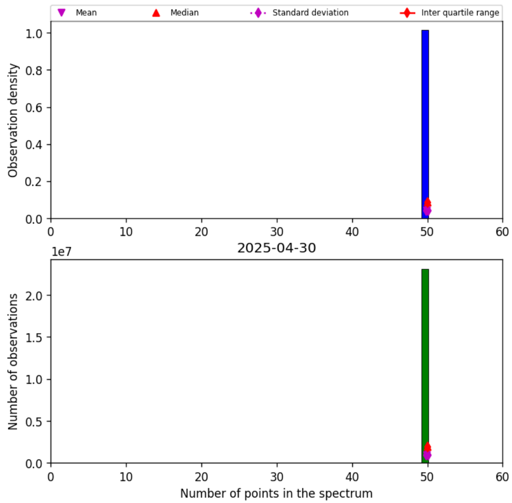
Figure 42: Histogram of "Number of points in the spectrum" for 2025-04-30 to 2025-05-01
