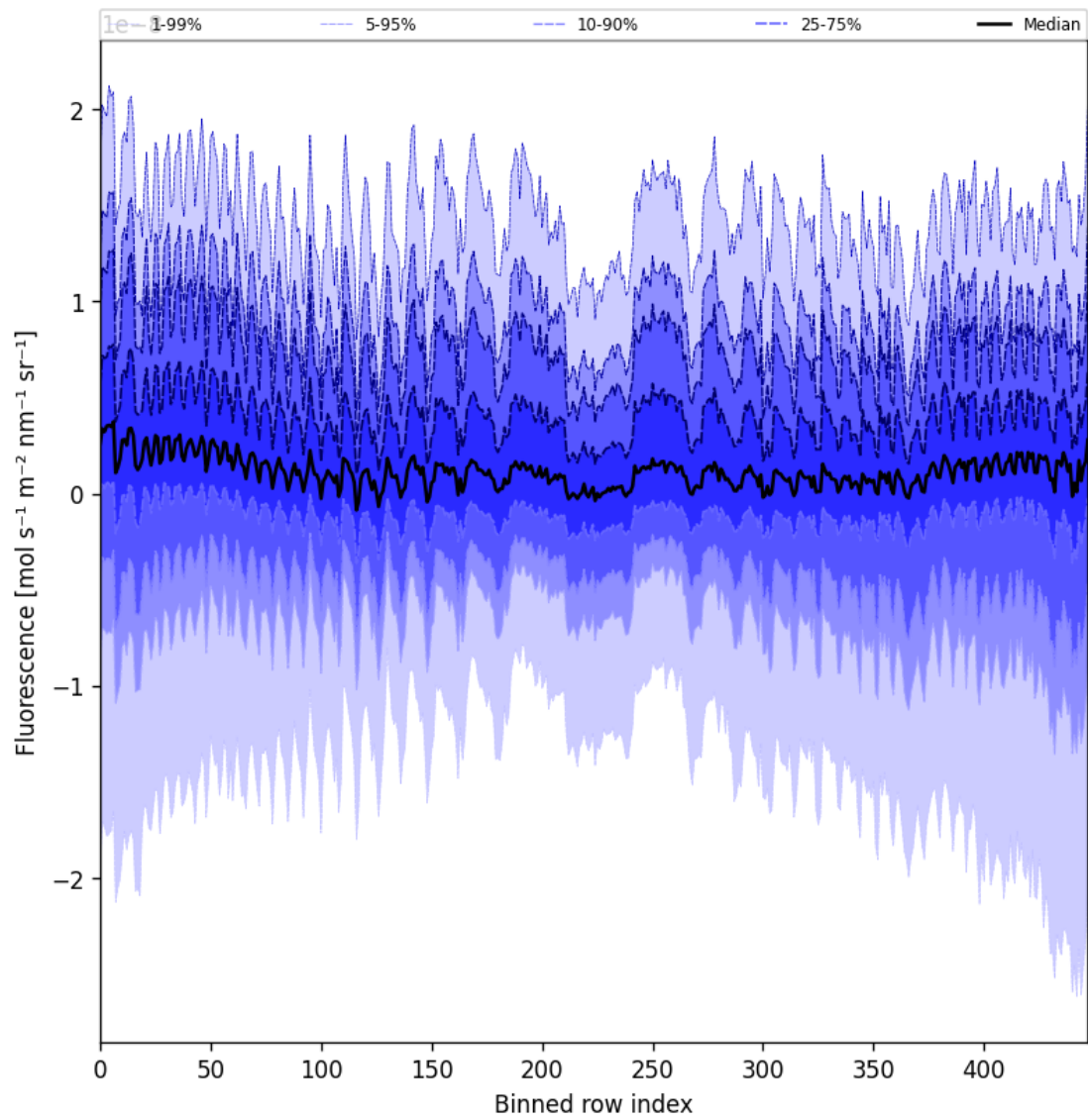
Figure 55: Along track statistics of “Fluorescence” for 2025-04-30 to 2025-05-01
