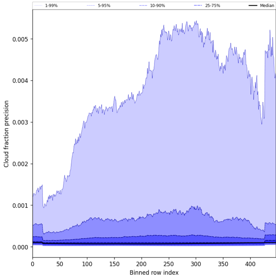
Figure 48: Along track statistics of “Cloud fraction precision” for 2025-04-30 to 2025-05-01
