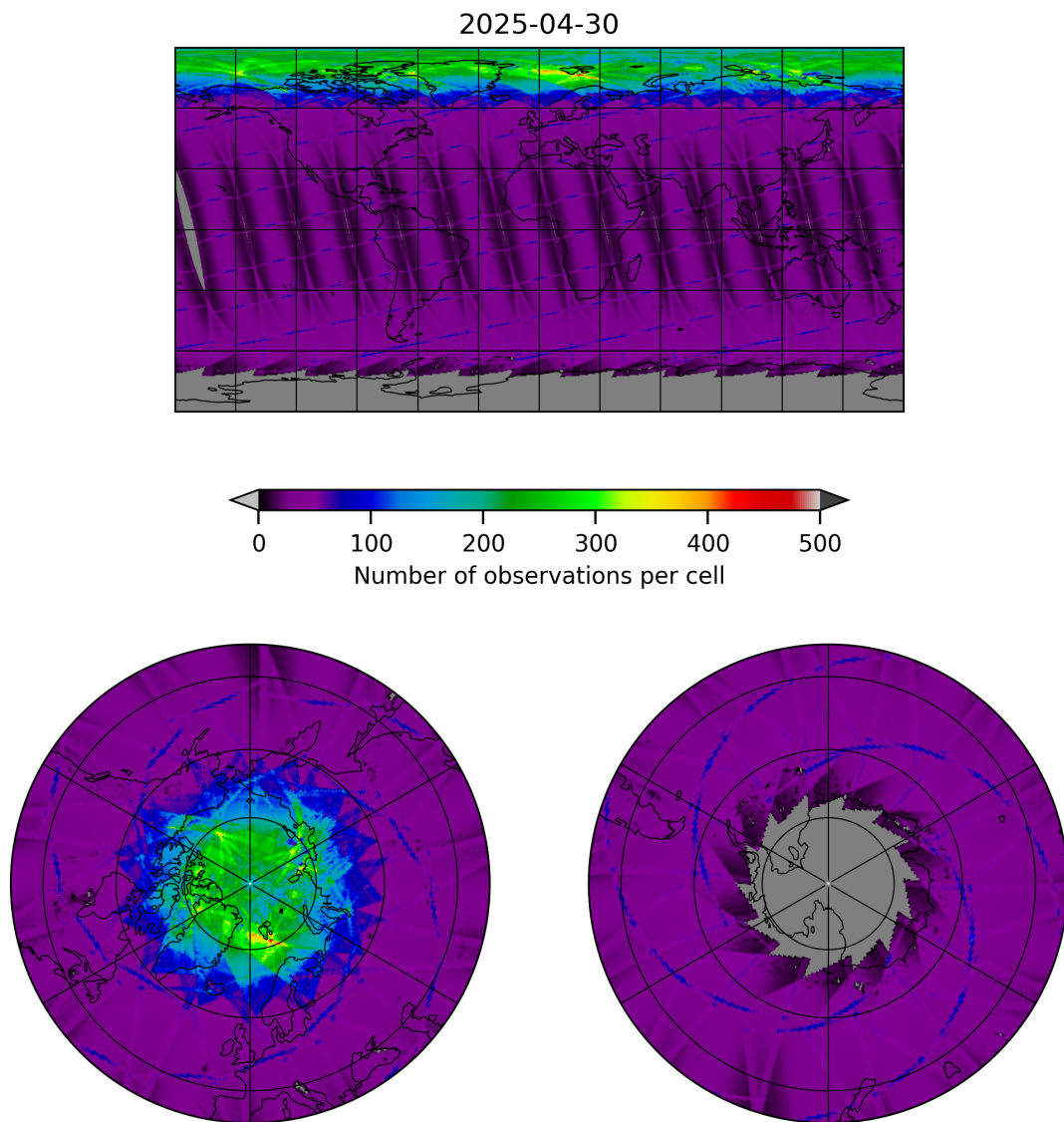
Figure 9: Map of the number of observations for 2025-04-30 to 2025-05-01
