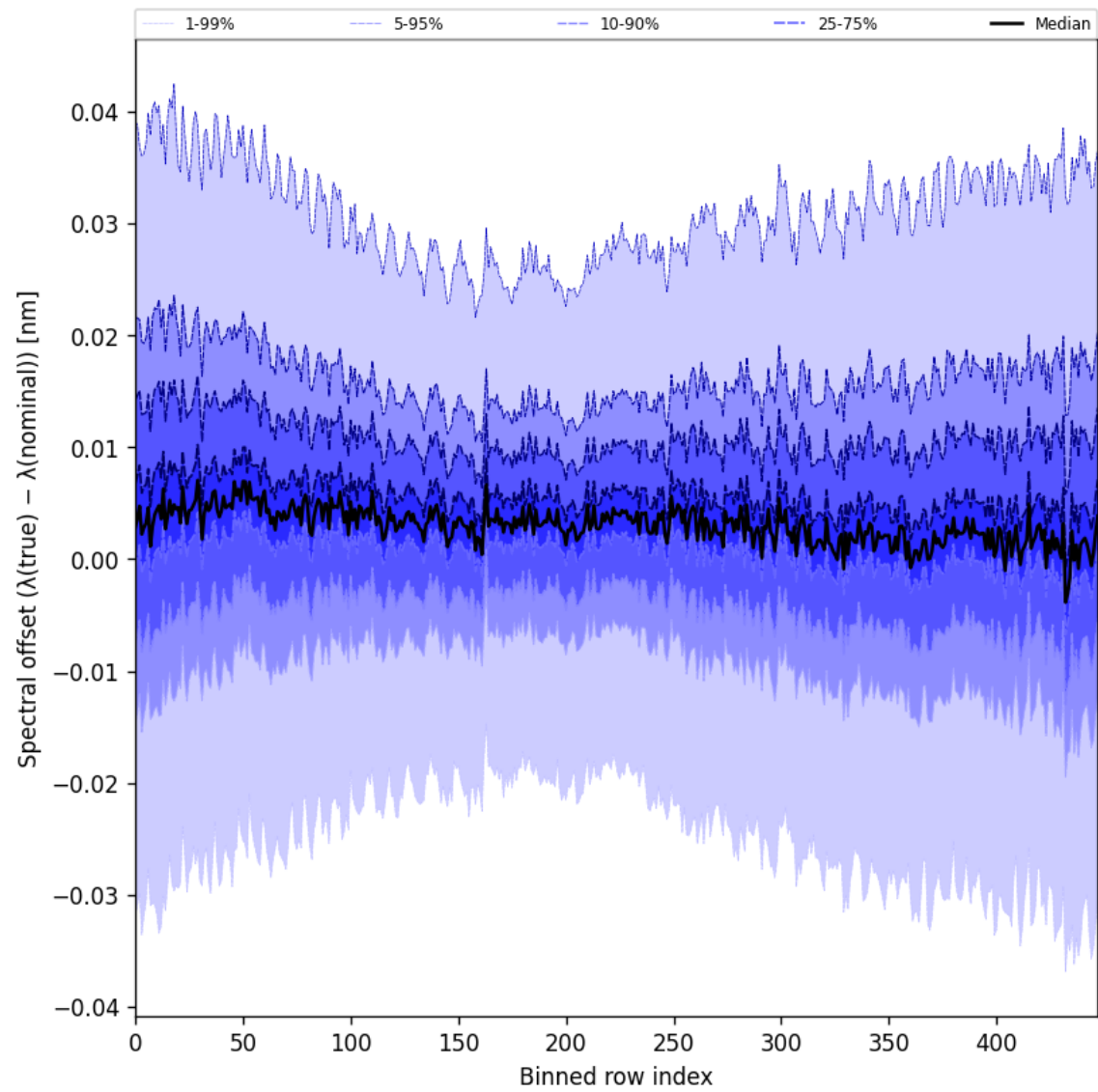
Figure 60: Along track statistics of “Spectral offset ( \lambda_{\text{true}} - \lambda_{\text{nominal}} )” for 2025-04-30 to 2025-05-01
