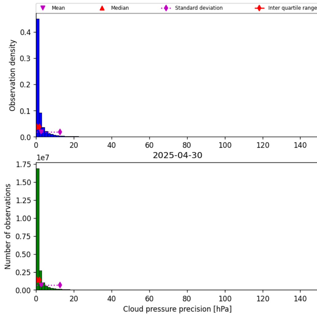
Figure 29: Histogram of “Cloud pressure precision” for 2025-04-30 to 2025-05-01
