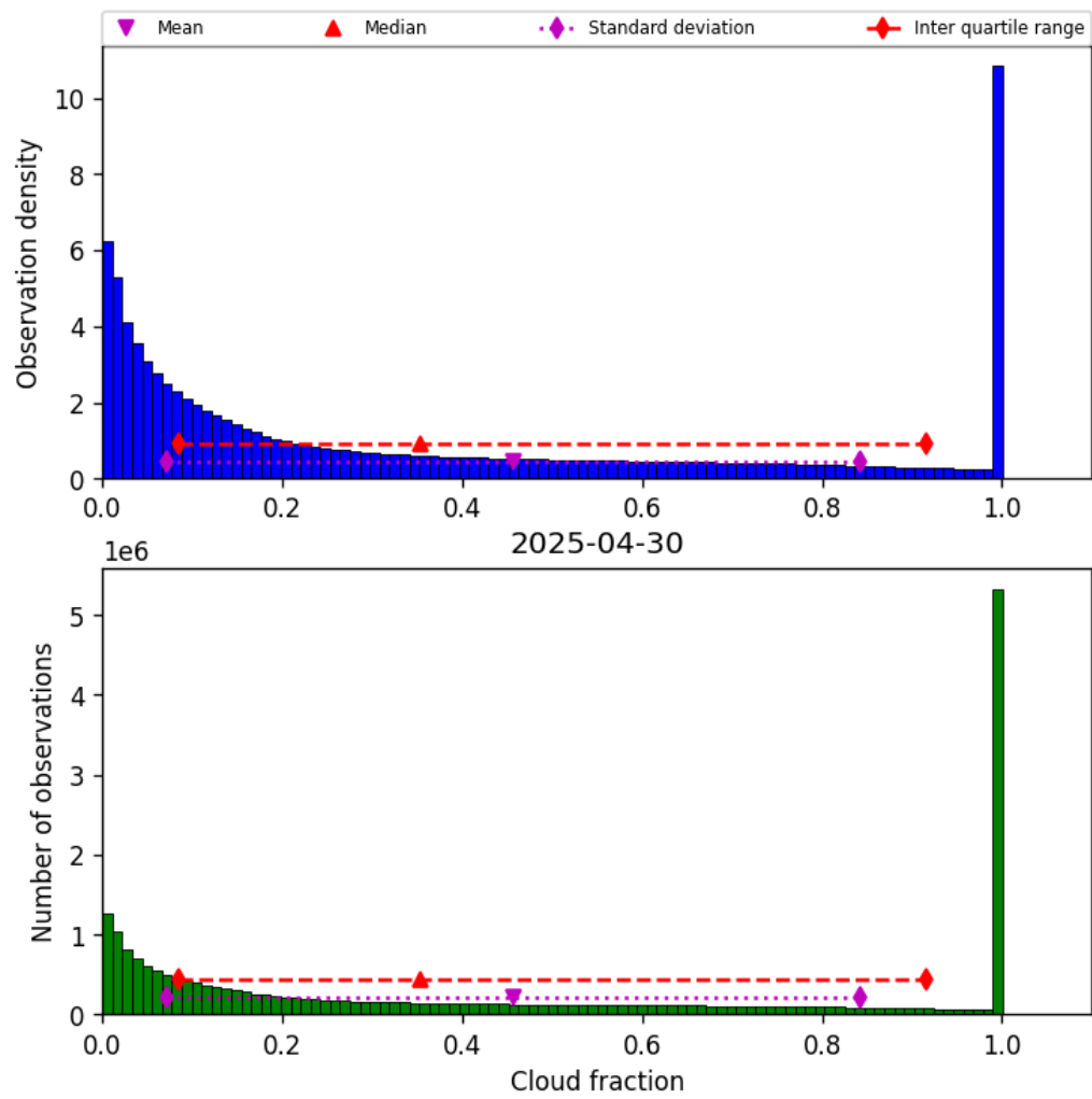
Figure 30: Histogram of “Cloud fraction” for 2025-04-30 to 2025-05-01
