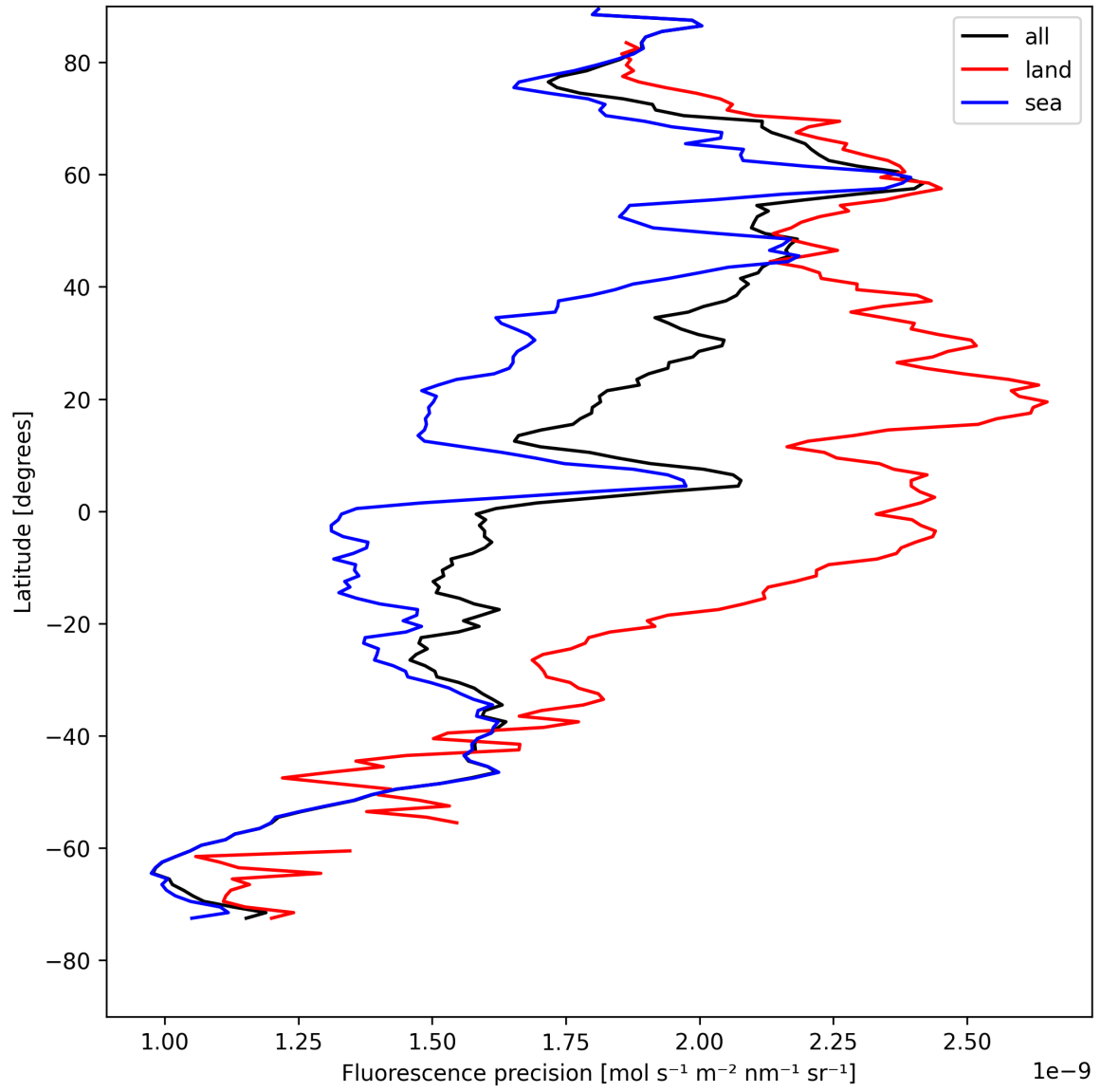
Figure 22: Zonal average of “Fluorescence precision” for 2025-04-30 to 2025-05-01.
