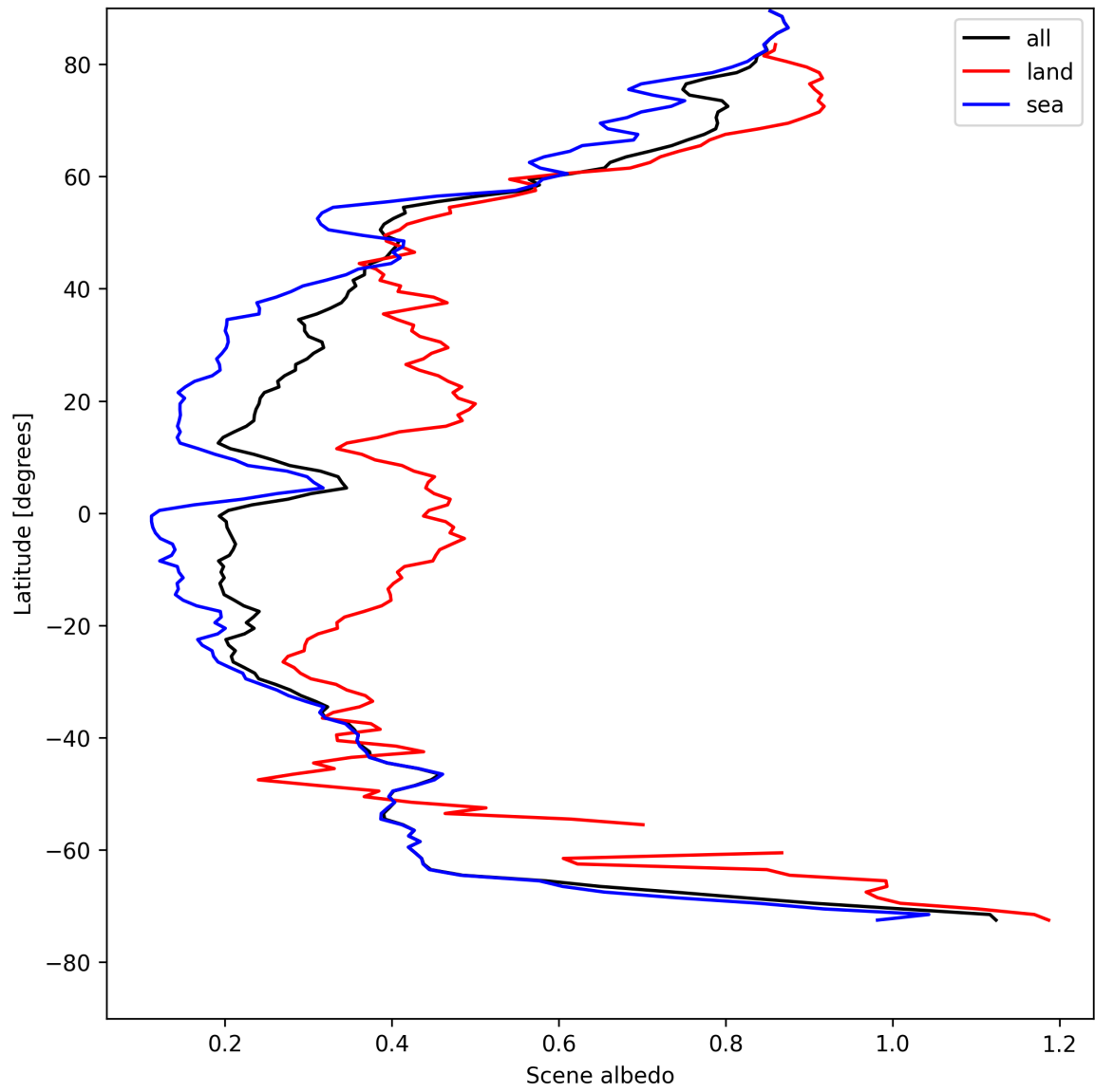
Figure 15: Zonal average of “Scene albedo” for 2025-04-30 to 2025-05-01.
