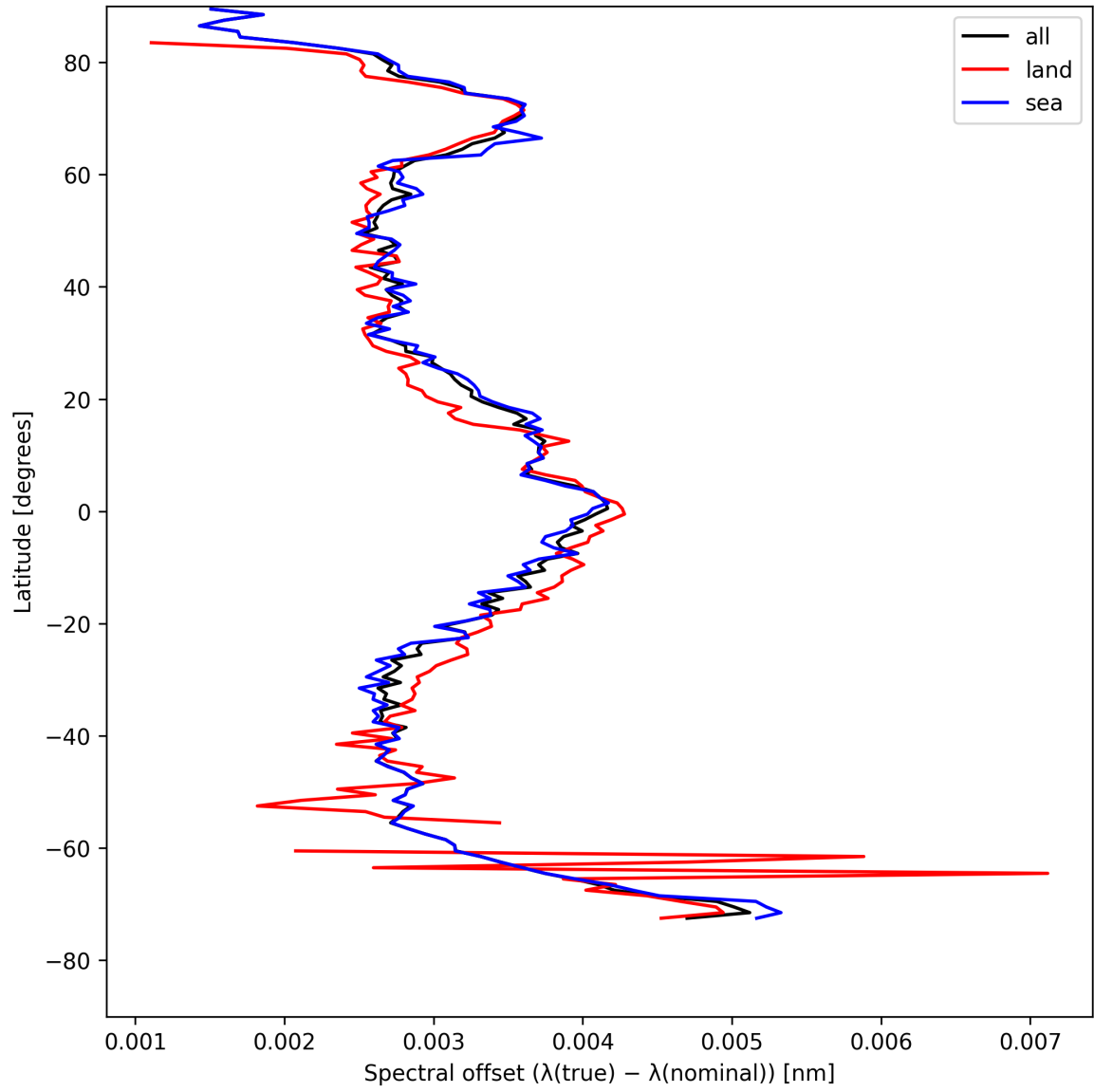
Figure 26: Zonal average of “Spectral offset ( \lambda_{\text{true}} - \lambda_{\text{nominal}} )” for 2025-04-30 to 2025-05-01.
