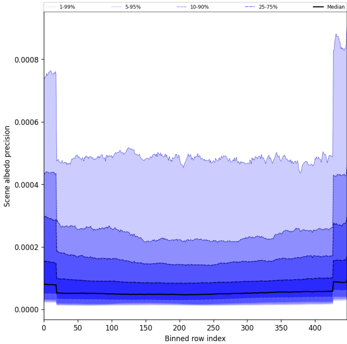
Figure 50: Along track statistics of “Scene albedo precision” for 2025-04-30 to 2025-05-01
