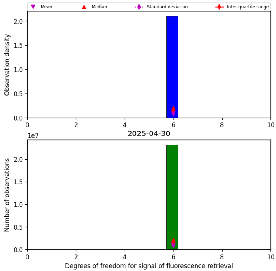
Figure 41: Histogram of “Degrees of freedom for signal of fluorescence retrieval” for 2025-04-30 to 2025-05-01
