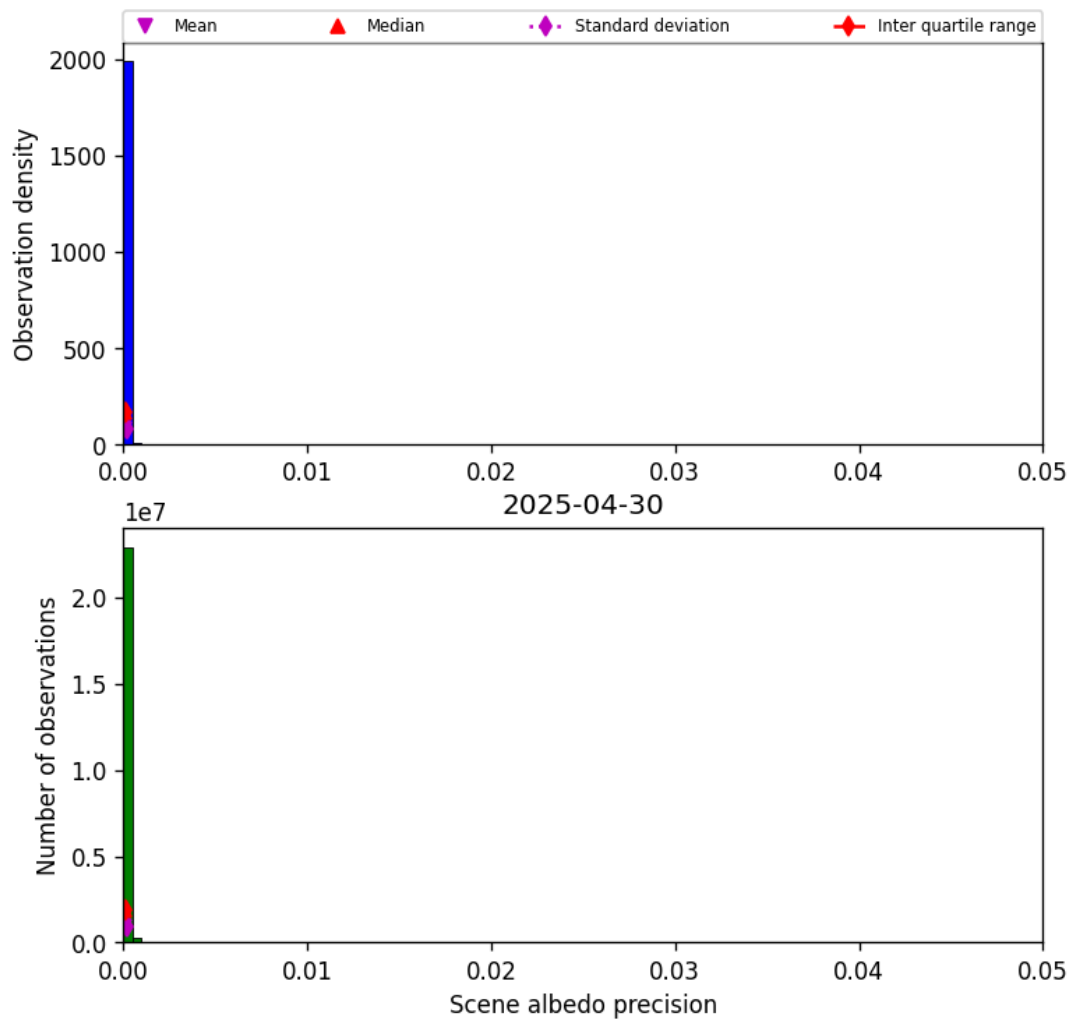
Figure 33: Histogram of “Scene albedo precision” for 2025-04-30 to 2025-05-01
