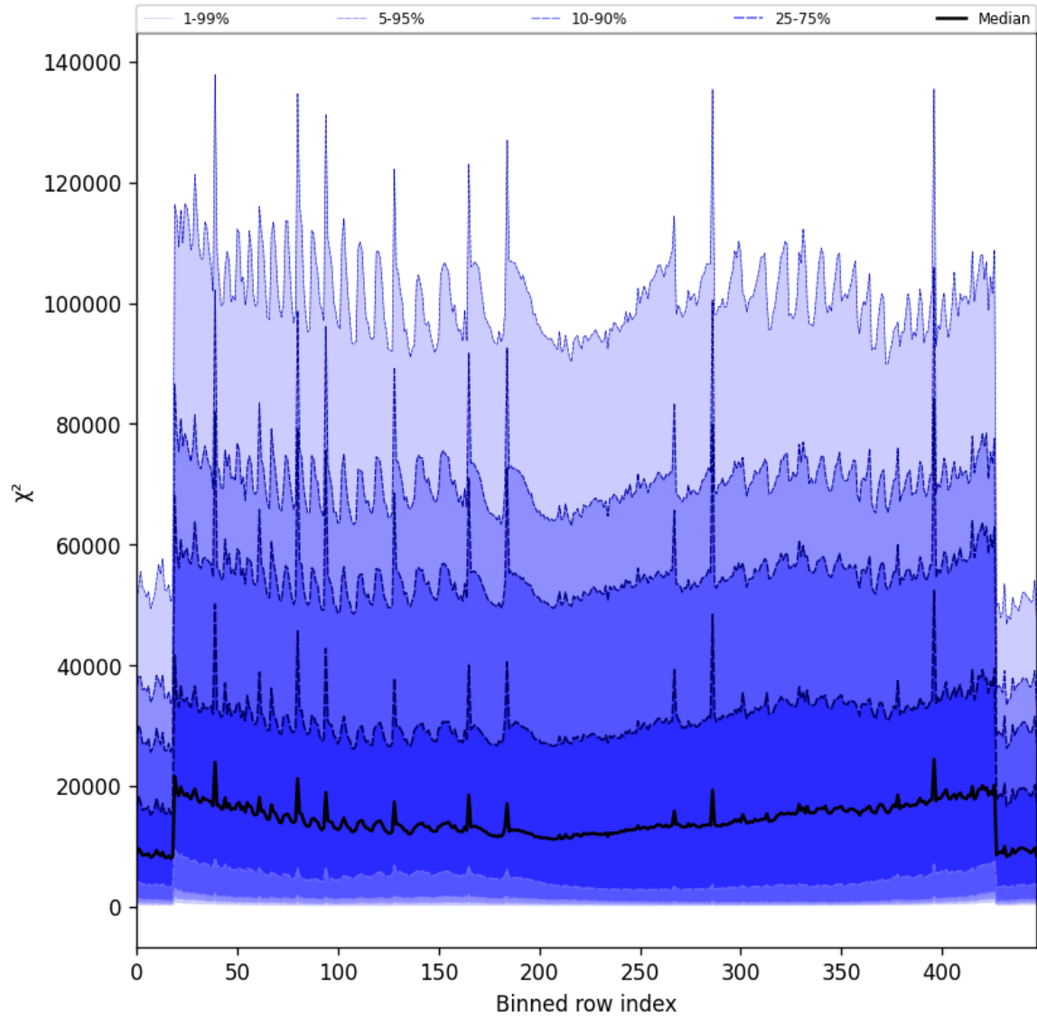
Figure 53: Along track statistics of “ \chi^2 ” for 2025-04-30 to 2025-05-01
