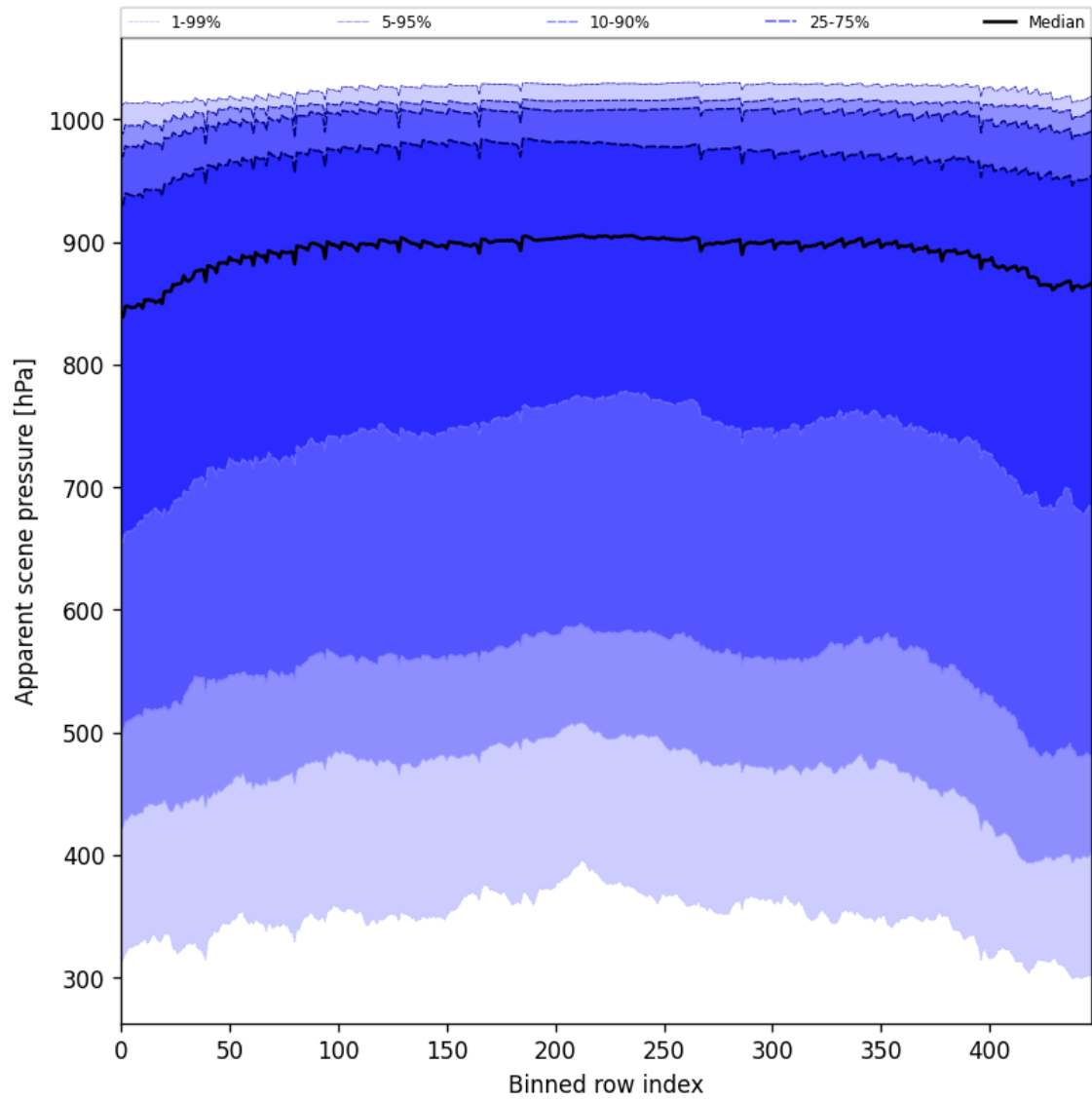
Figure 51: Along track statistics of “Apparent scene pressure” for 2025-04-30 to 2025-05-01
