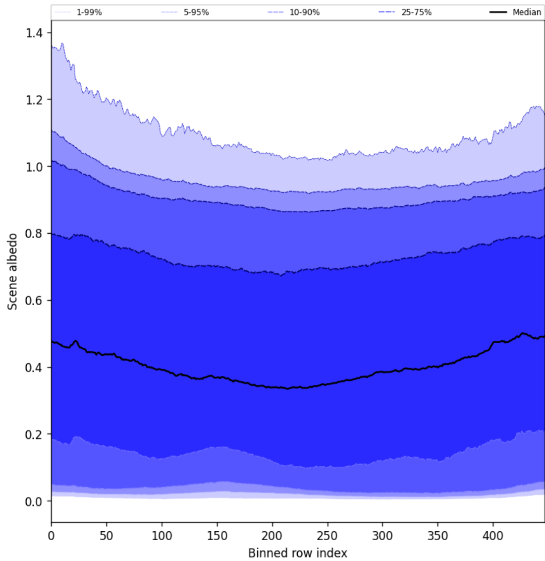
Figure 49: Along track statistics of “Scene albedo” for 2025-04-30 to 2025-05-01
