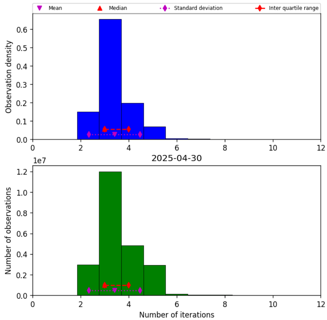
Figure 37: Histogram of “Number of iterations” for 2025-04-30 to 2025-05-01
