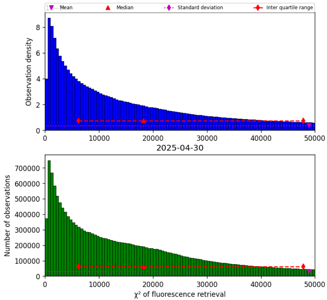
Figure 40: Histogram of “ \chi^2 of fluorescence retrieval” for 2025-04-30 to 2025-05-01
