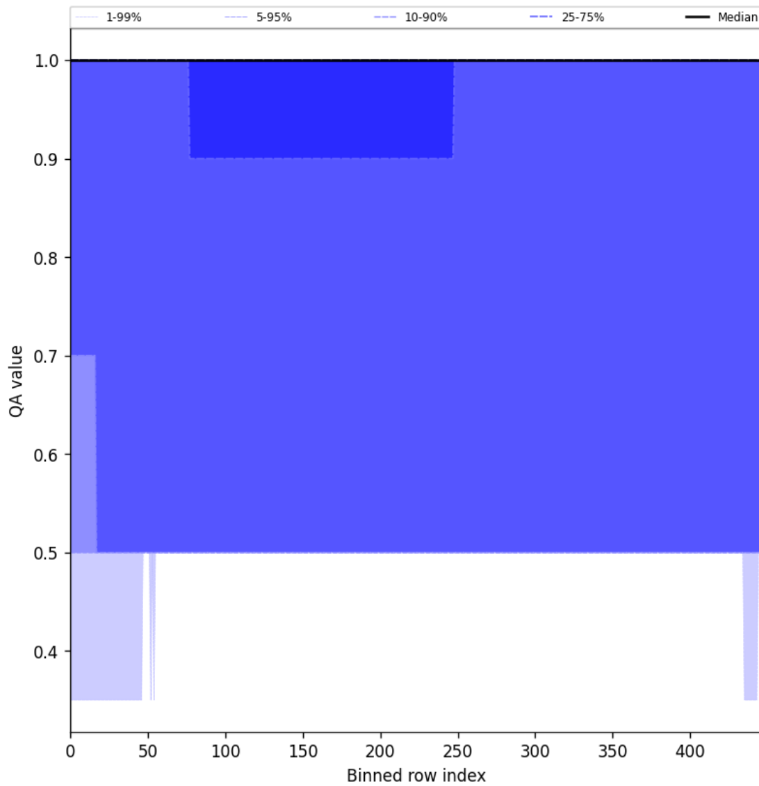
Figure 44: Along track statistics of “QA value” for 2025-04-30 to 2025-05-01
