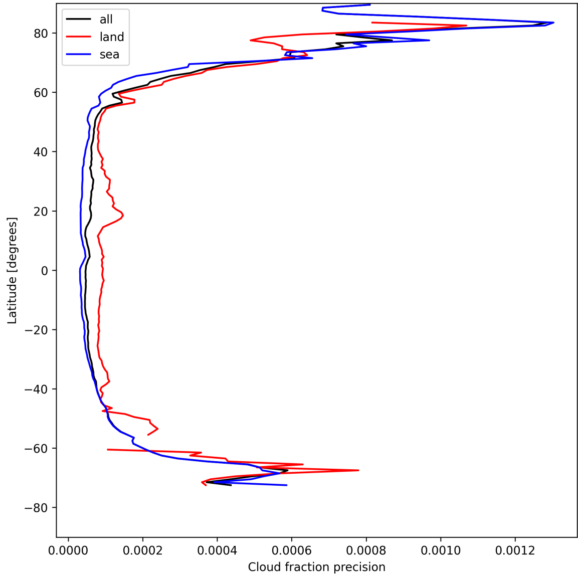
Figure 14: Zonal average of “Cloud fraction precision” for 2025-04-30 to 2025-05-01.
