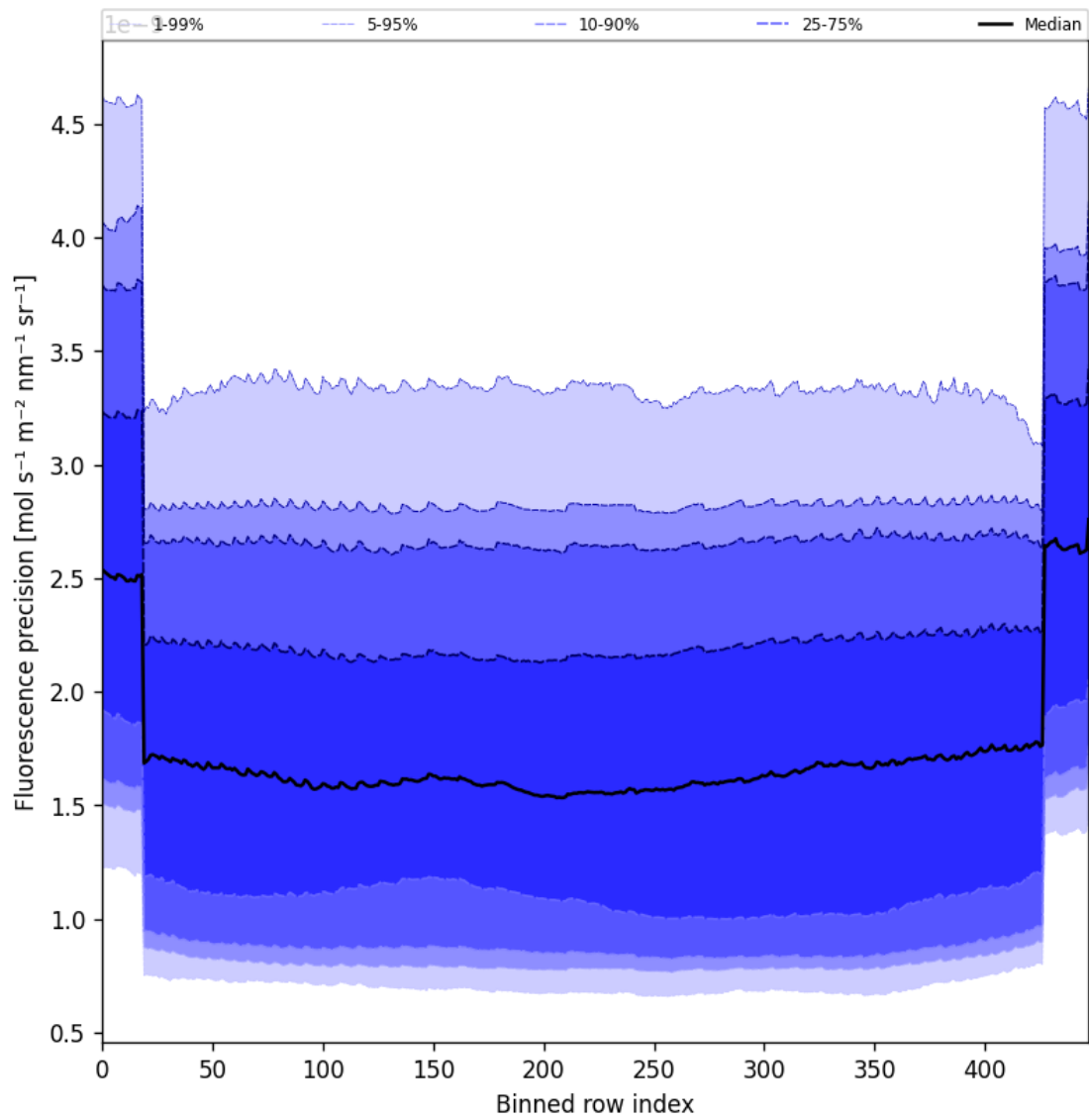
Figure 56: Along track statistics of “Fluorescence precision” for 2025-04-30 to 2025-05-01
