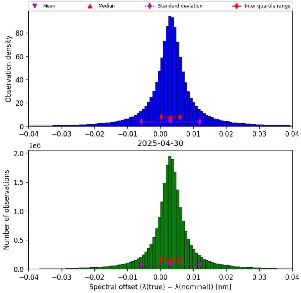
Figure 43: Histogram of “Spectral offset ( \lambda_{\text{true}} - \lambda_{\text{nominal}} )” for 2025-04-30 to 2025-05-01
