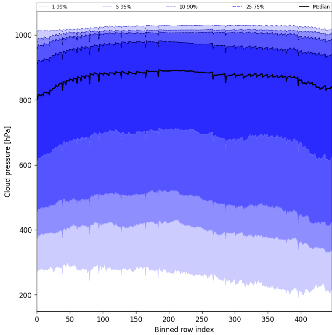
Figure 45: Along track statistics of “Cloud pressure” for 2025-04-30 to 2025-05-01
