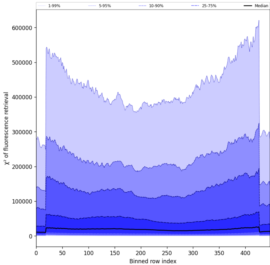
Figure 57: Along track statistics of “ \chi^2 of fluorescence retrieval” for 2025-04-30 to 2025-05-01
