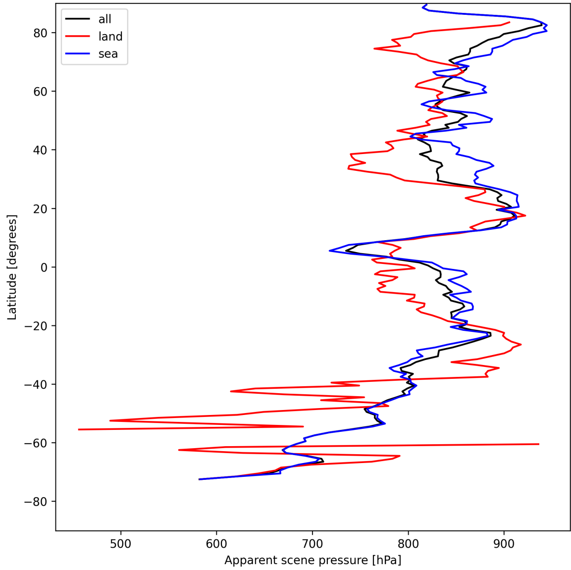
Figure 17: Zonal average of “Apparent scene pressure” for 2025-04-30 to 2025-05-01.
