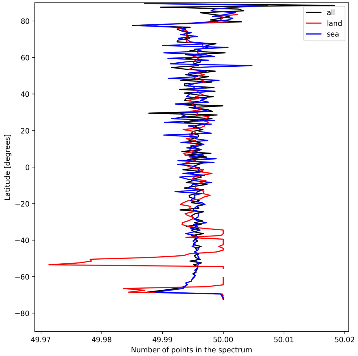
Figure 25: Zonal average of “Number of points in the spectrum” for 2025-04-30 to 2025-05-01.
