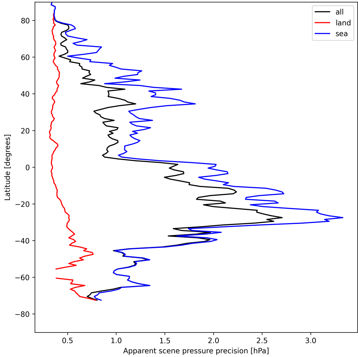
Figure 18: Zonal average of “Apparent scene pressure precision” for 2025-04-30 to 2025-05-01.
