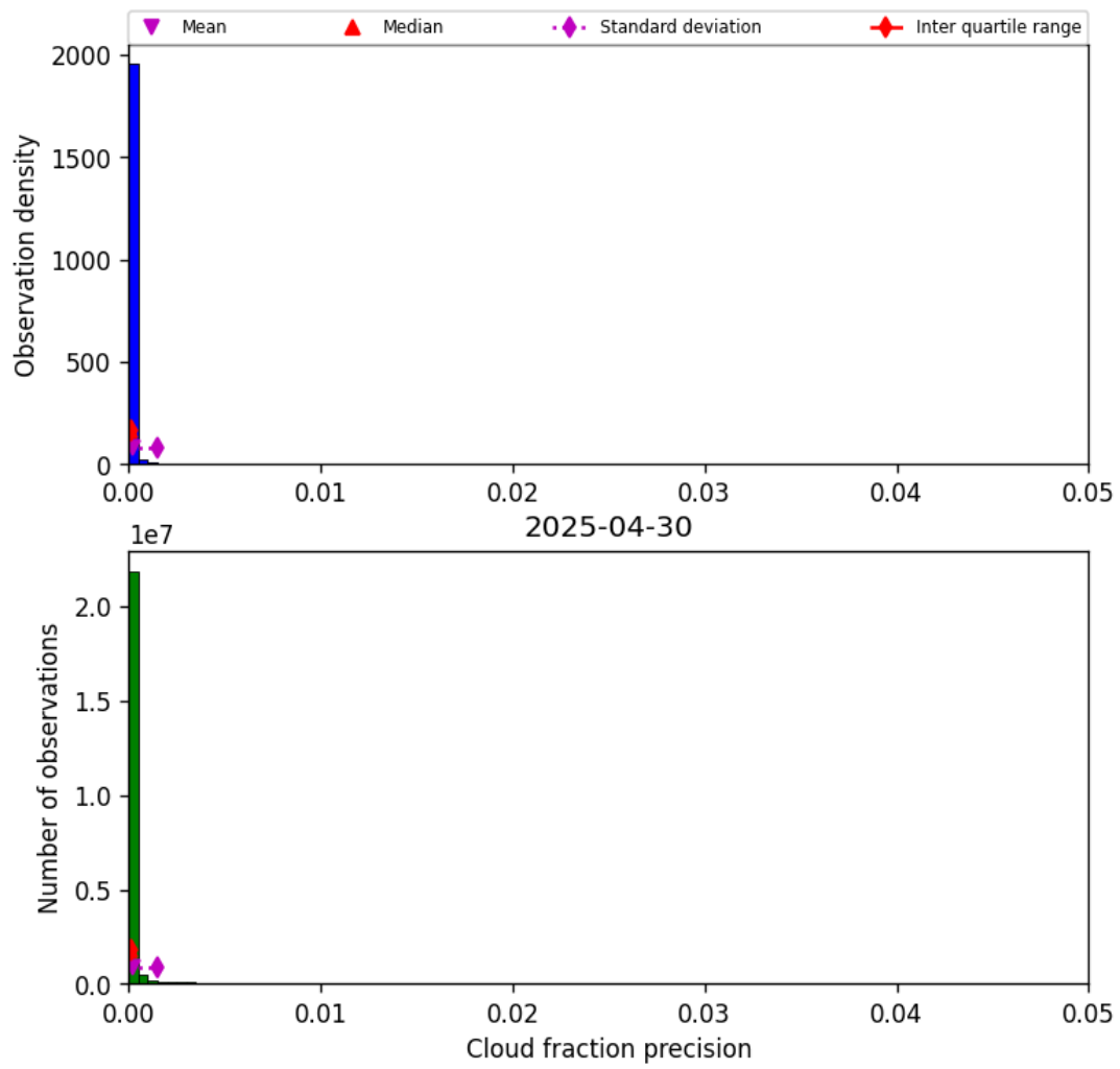
Figure 31: Histogram of “Cloud fraction precision” for 2025-04-30 to 2025-05-01
