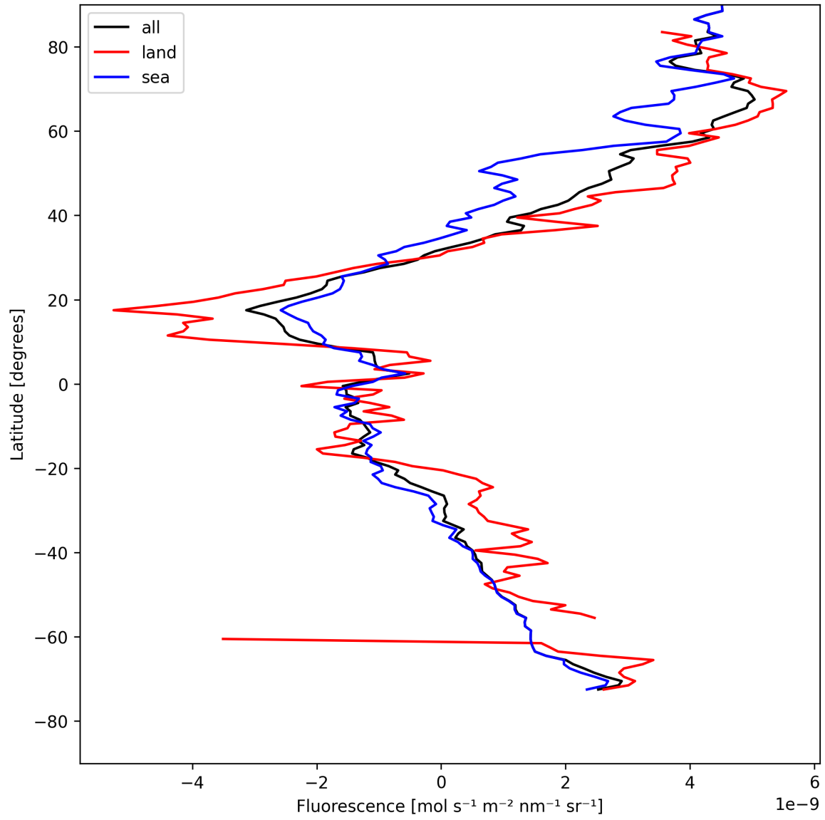
Figure 21: Zonal average of “Fluorescence” for 2025-04-30 to 2025-05-01.
