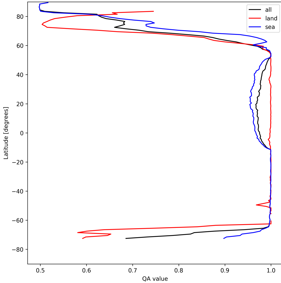
Figure 10: Zonal average of “QA value” for 2025-04-30 to 2025-05-01.
