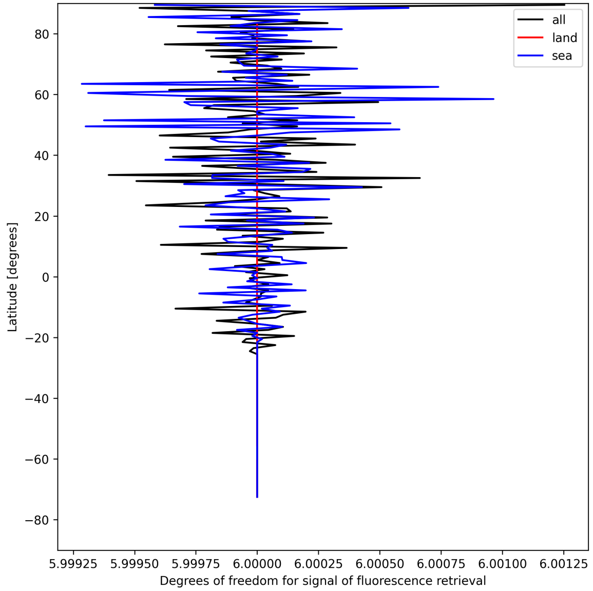
Figure 24: Zonal average of “Degrees of freedom for signal of fluorescence retrieval” for 2025-04-30 to 2025-05-01.
