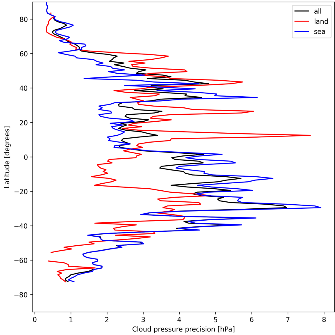
Figure 12: Zonal average of “Cloud pressure precision” for 2025-04-30 to 2025-05-01.
