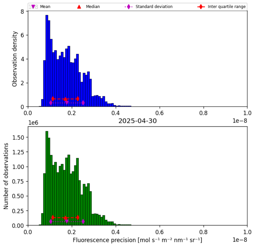
Figure 39: Histogram of “Fluorescence precision” for 2025-04-30 to 2025-05-01
