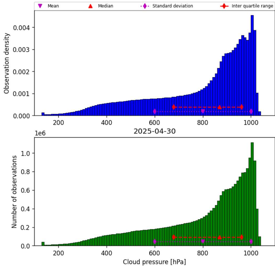
Figure 28: Histogram of “Cloud pressure” for 2025-04-30 to 2025-05-01
