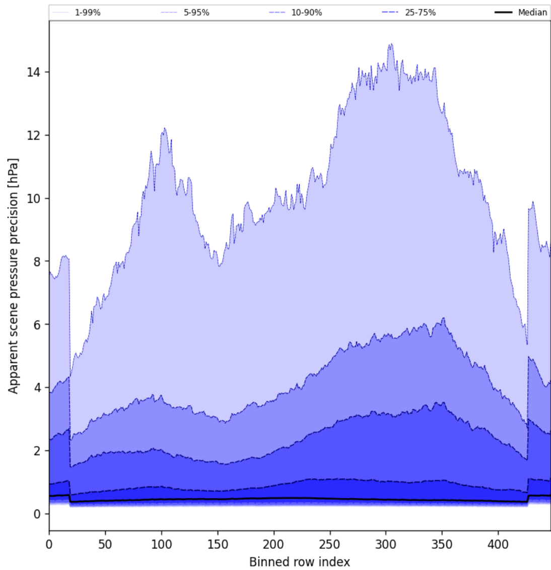
Figure 52: Along track statistics of “Apparent scene pressure precision” for 2025-04-30 to 2025-05-01
