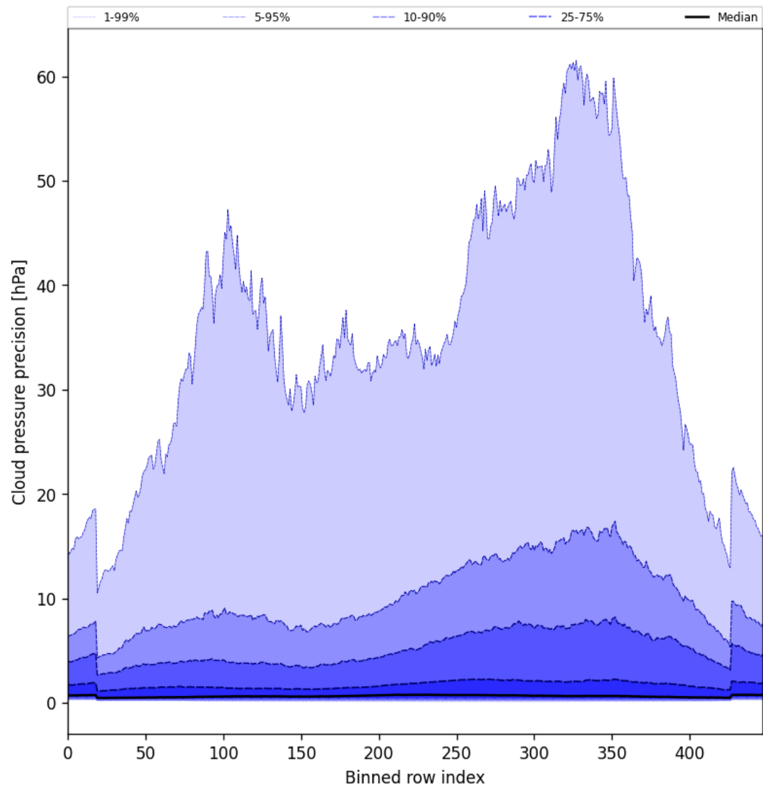
Figure 46: Along track statistics of “Cloud pressure precision” for 2025-04-30 to 2025-05-01
