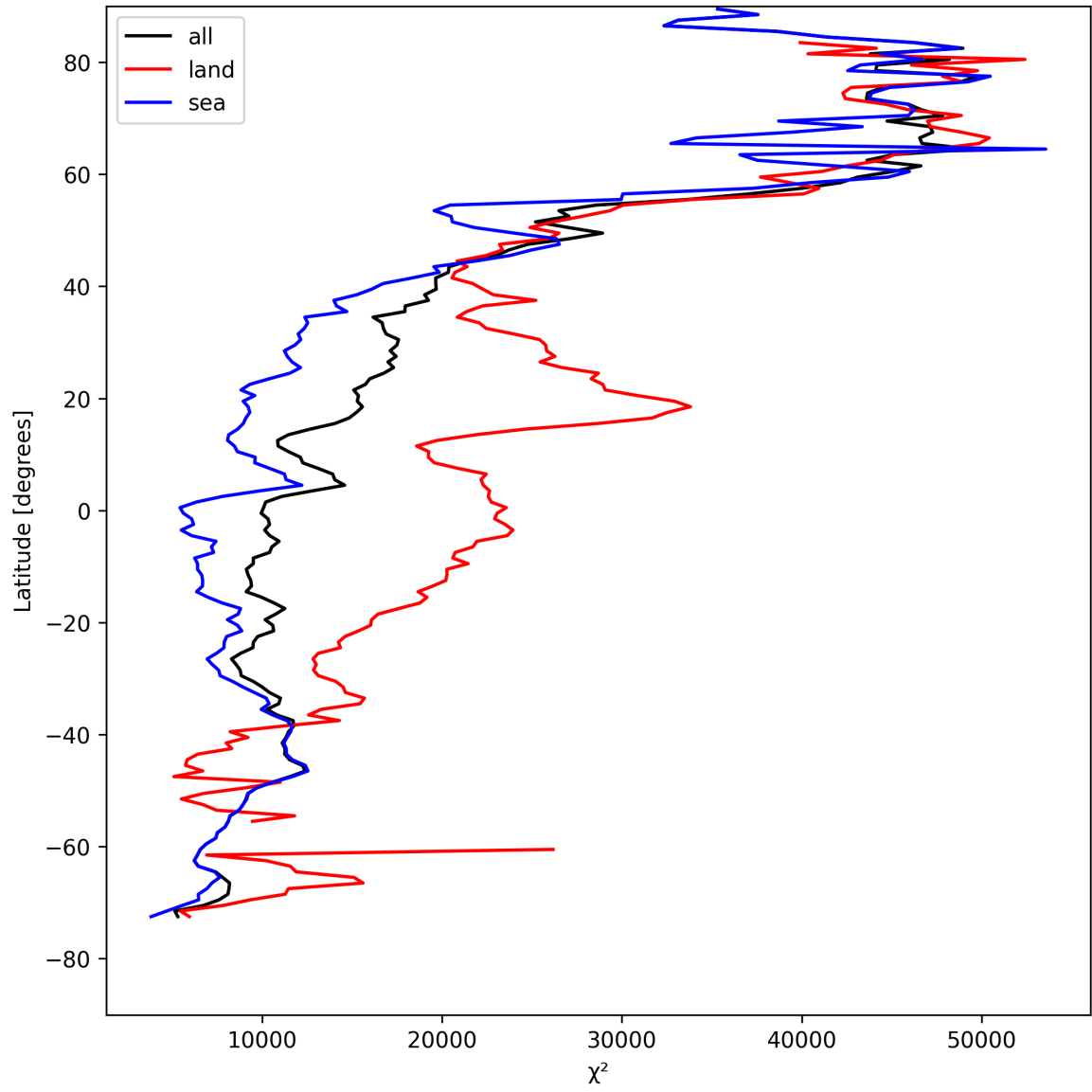
Figure 19: Zonal average of “ \chi^2 ” for 2025-04-30 to 2025-05-01.
