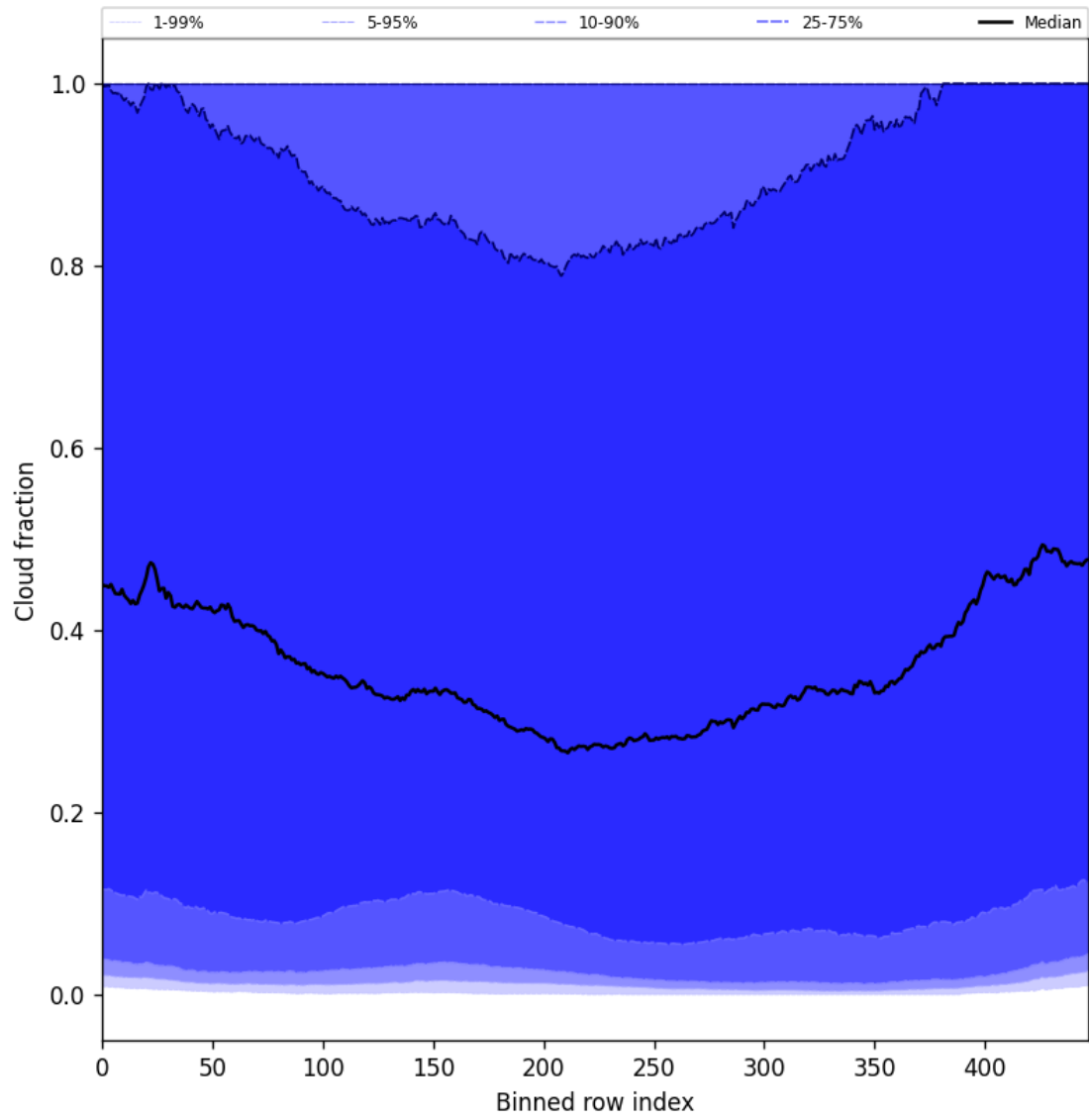
Figure 47: Along track statistics of “Cloud fraction” for 2025-04-30 to 2025-05-01
