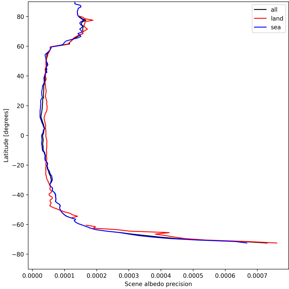
Figure 16: Zonal average of “Scene albedo precision” for 2025-04-30 to 2025-05-01.
