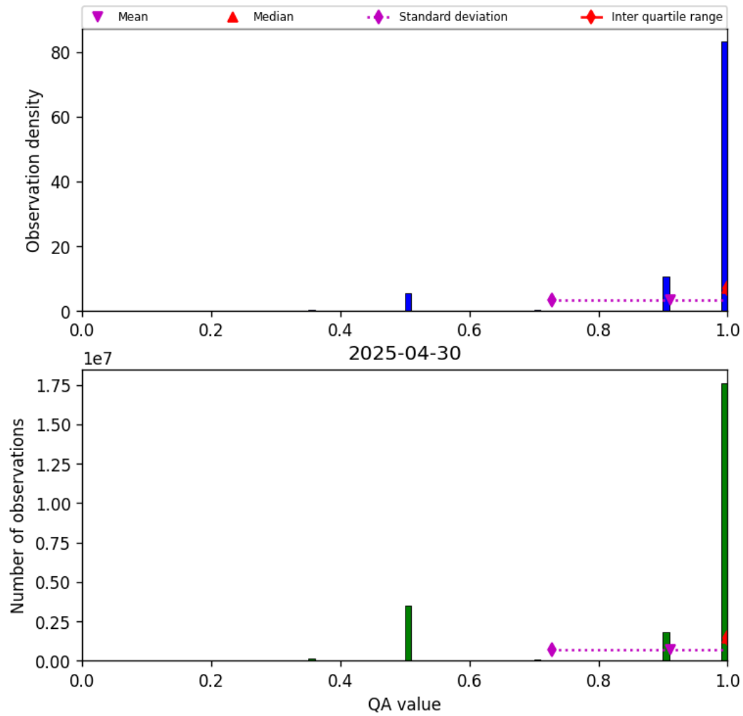
Figure 27: Histogram of “QA value” for 2025-04-30 to 2025-05-01
