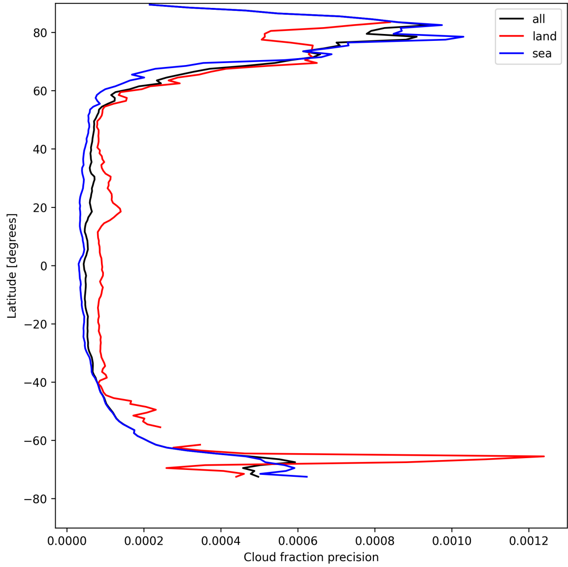
Figure 14: Zonal average of “Cloud fraction precision” for 2025-05-01 to 2025-05-02.
