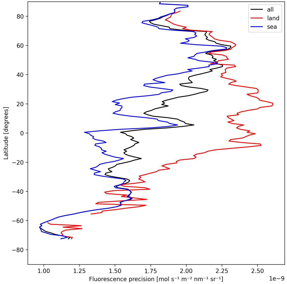
Figure 22: Zonal average of “Fluorescence precision” for 2025-05-01 to 2025-05-02.
