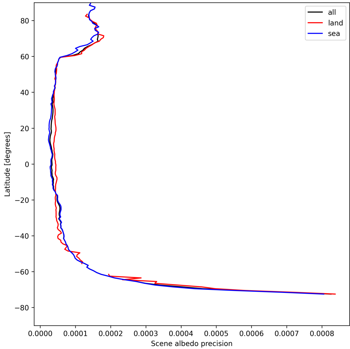
Figure 16: Zonal average of “Scene albedo precision” for 2025-05-01 to 2025-05-02.
