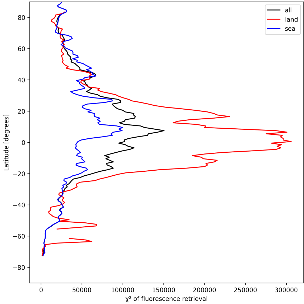
Figure 23: Zonal average of “ \chi^2 of fluorescence retrieval” for 2025-05-01 to 2025-05-02.
