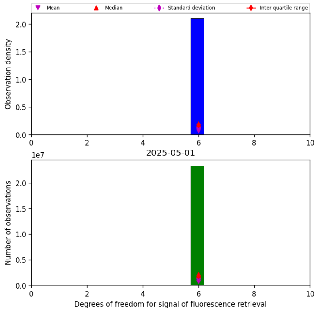
Figure 41: Histogram of “Degrees of freedom for signal of fluorescence retrieval” for 2025-05-01 to 2025-05-02
