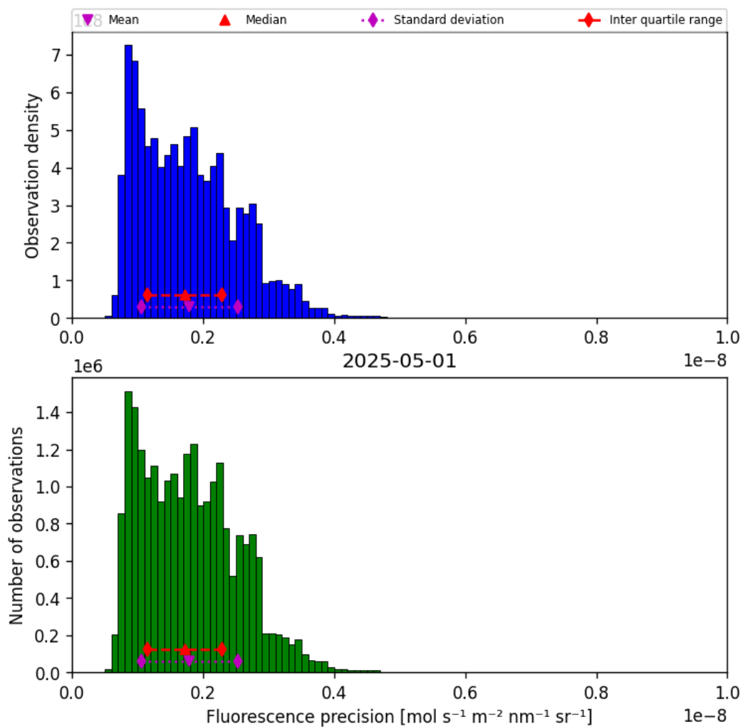
Figure 39: Histogram of “Fluorescence precision” for 2025-05-01 to 2025-05-02
