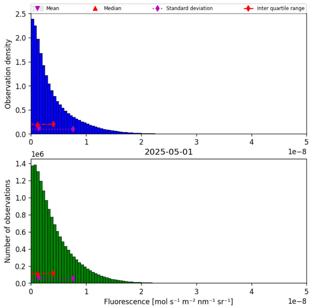
Figure 38: Histogram of “Fluorescence” for 2025-05-01 to 2025-05-02
