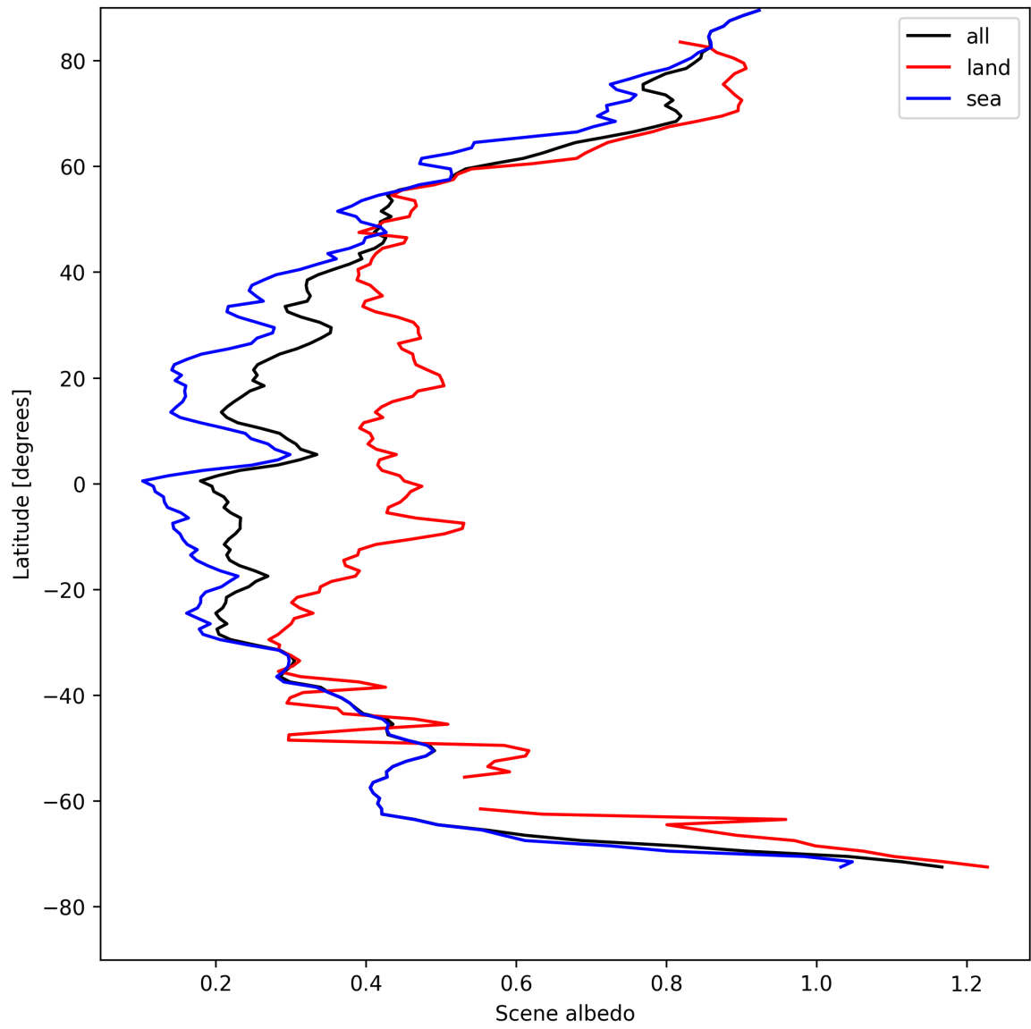
Figure 15: Zonal average of “Scene albedo” for 2025-05-01 to 2025-05-02.
