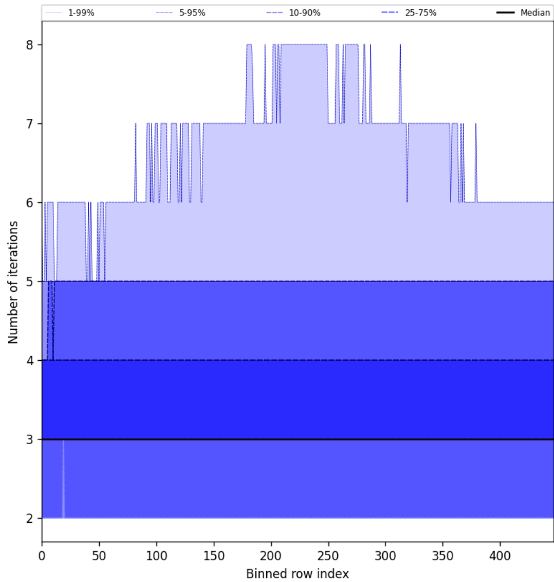
Figure 54: Along track statistics of “Number of iterations” for 2025-05-01 to 2025-05-02
