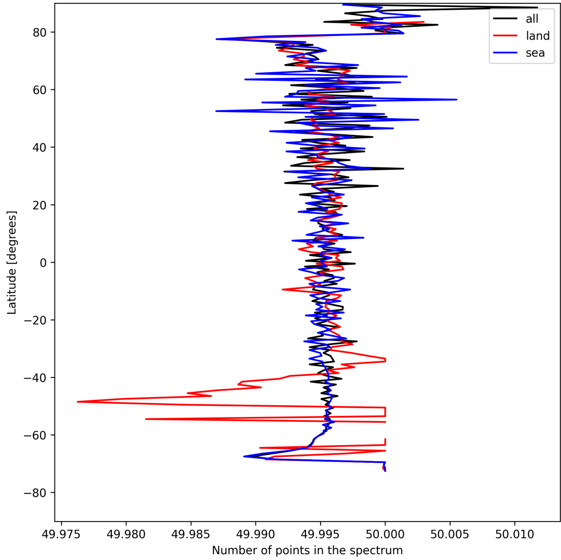
Figure 25: Zonal average of “Number of points in the spectrum” for 2025-05-01 to 2025-05-02.
