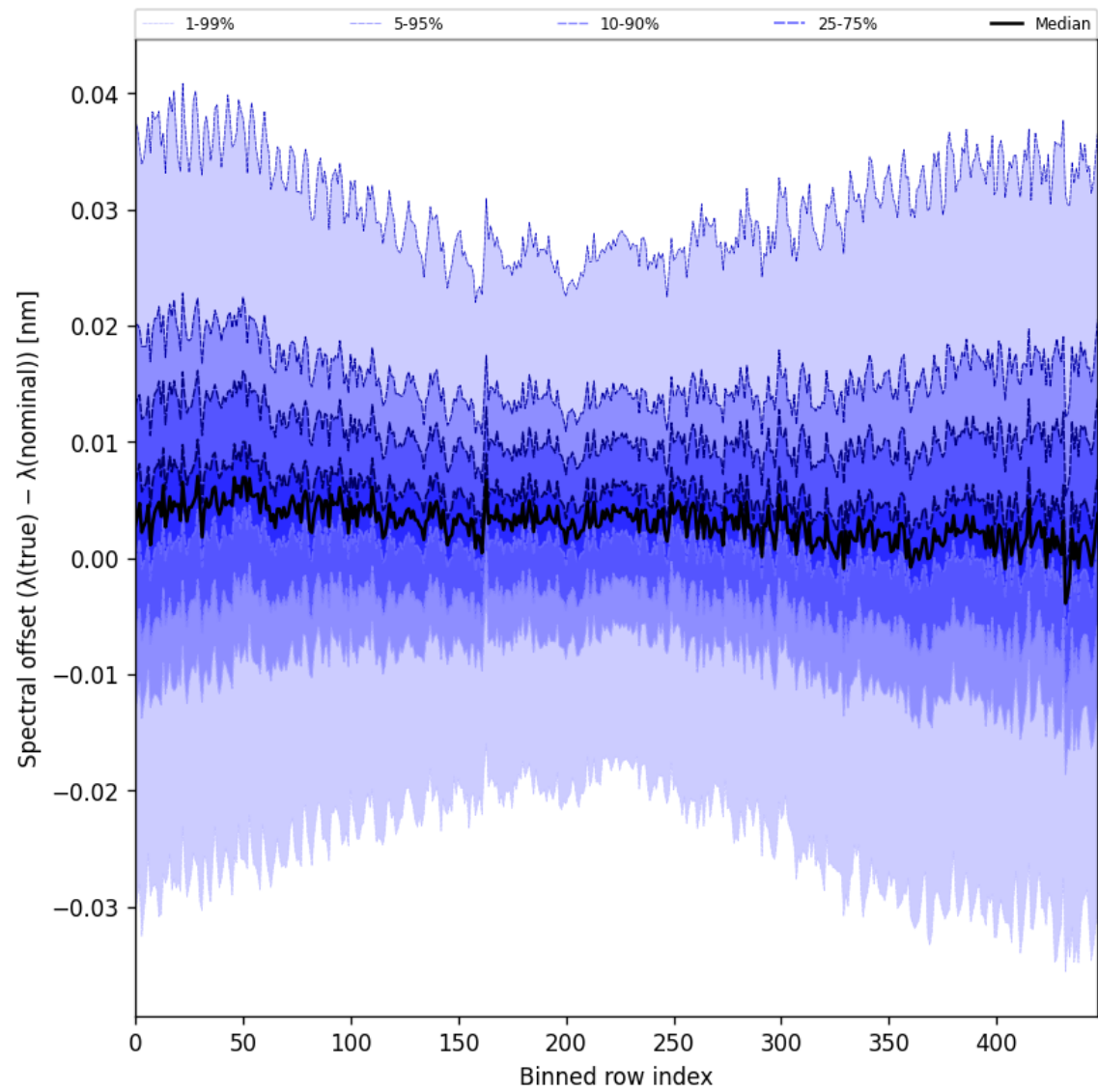
Figure 60: Along track statistics of “Spectral offset ( \lambda_{\text{true}} - \lambda_{\text{nominal}} )” for 2025-05-01 to 2025-05-02
