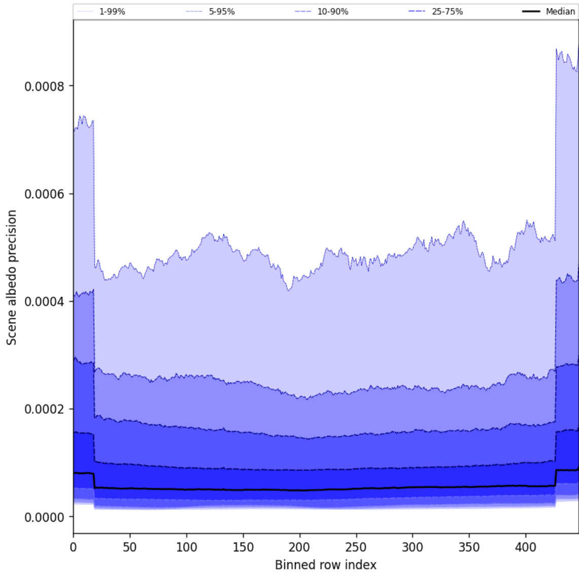
Figure 50: Along track statistics of “Scene albedo precision” for 2025-05-01 to 2025-05-02
