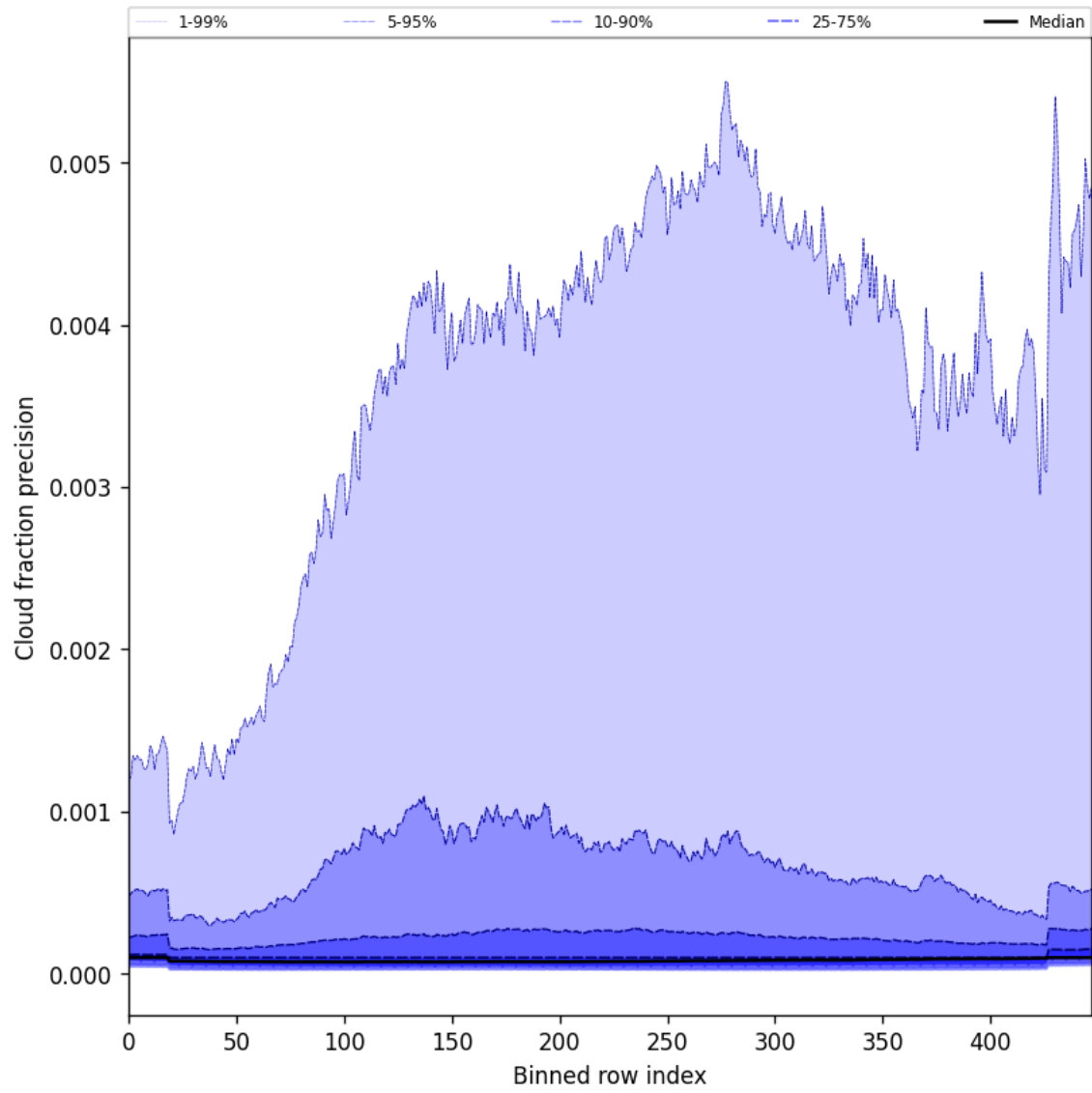
Figure 48: Along track statistics of “Cloud fraction precision” for 2025-05-01 to 2025-05-02
