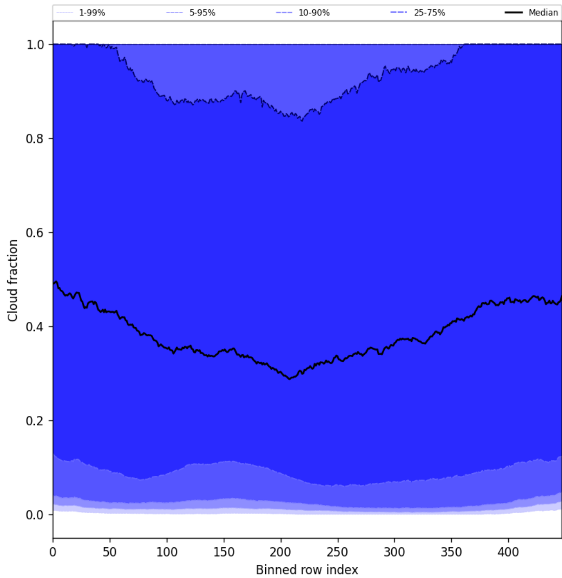
Figure 47: Along track statistics of “Cloud fraction” for 2025-05-01 to 2025-05-02
