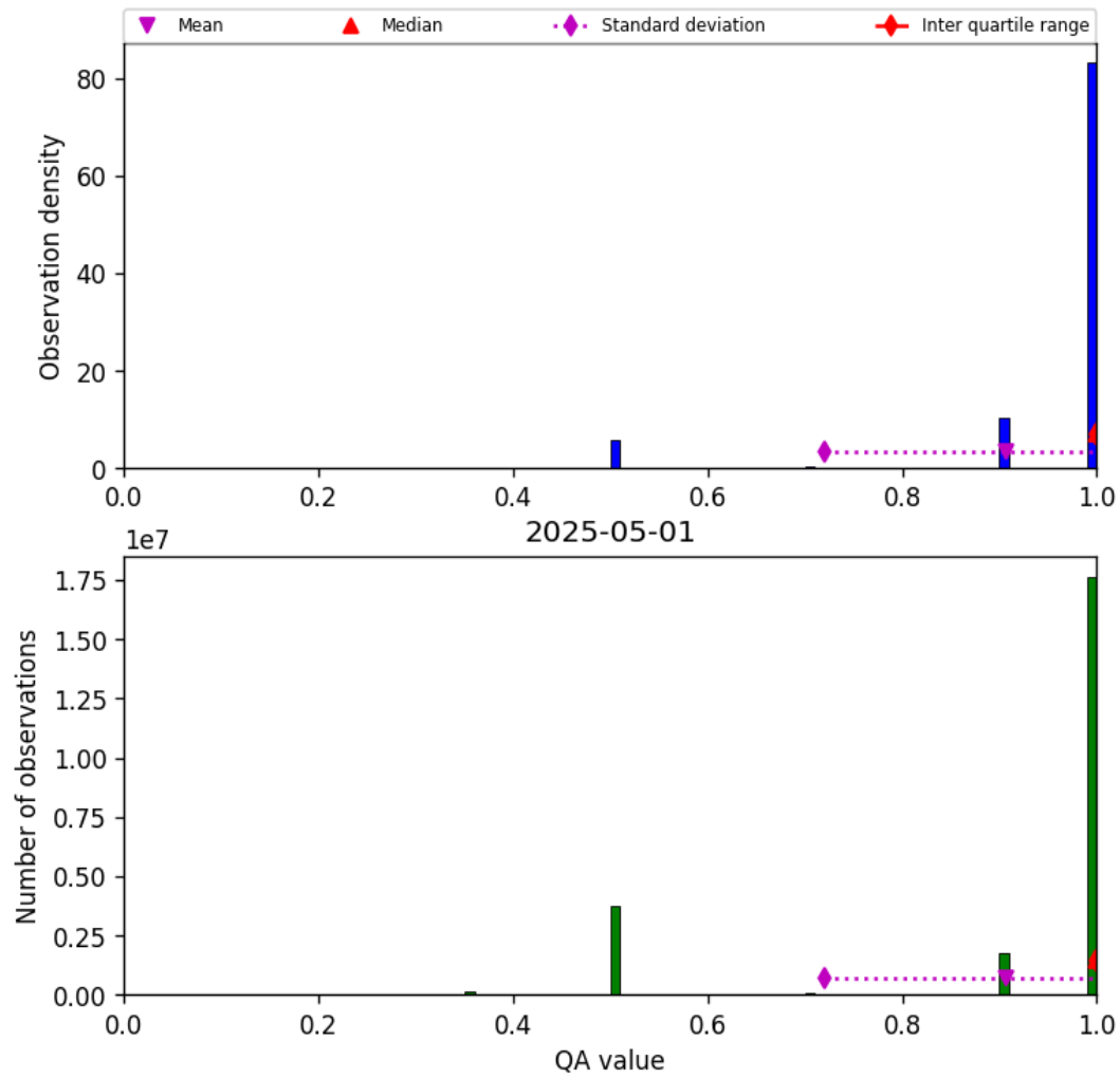
Figure 27: Histogram of “QA value” for 2025-05-01 to 2025-05-02
