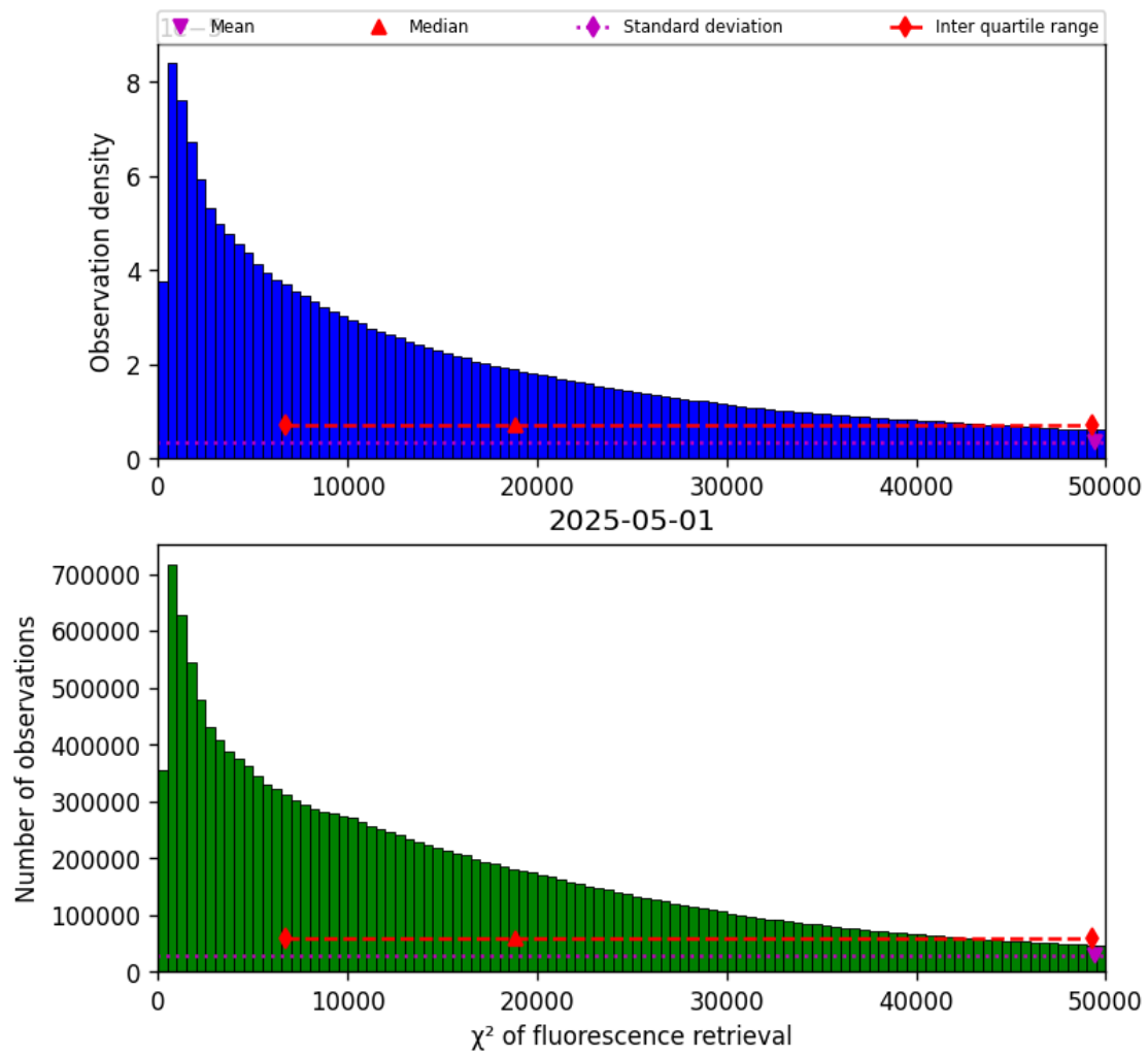
Figure 40: Histogram of “ \chi^2 of fluorescence retrieval” for 2025-05-01 to 2025-05-02
