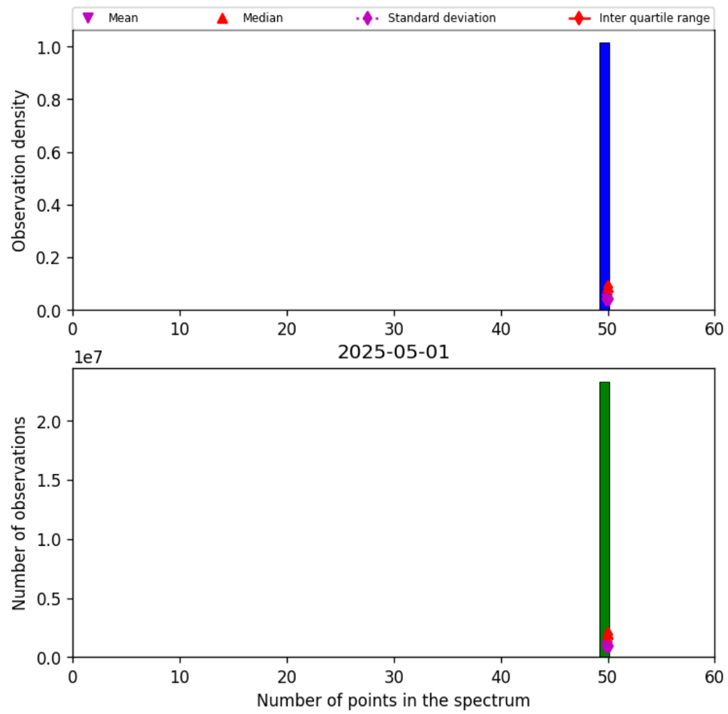
Figure 42: Histogram of “Number of points in the spectrum” for 2025-05-01 to 2025-05-02
