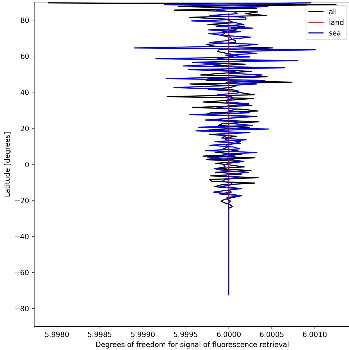
Figure 24: Zonal average of “Degrees of freedom for signal of fluorescence retrieval” for 2025-05-01 to 2025-05-02.
