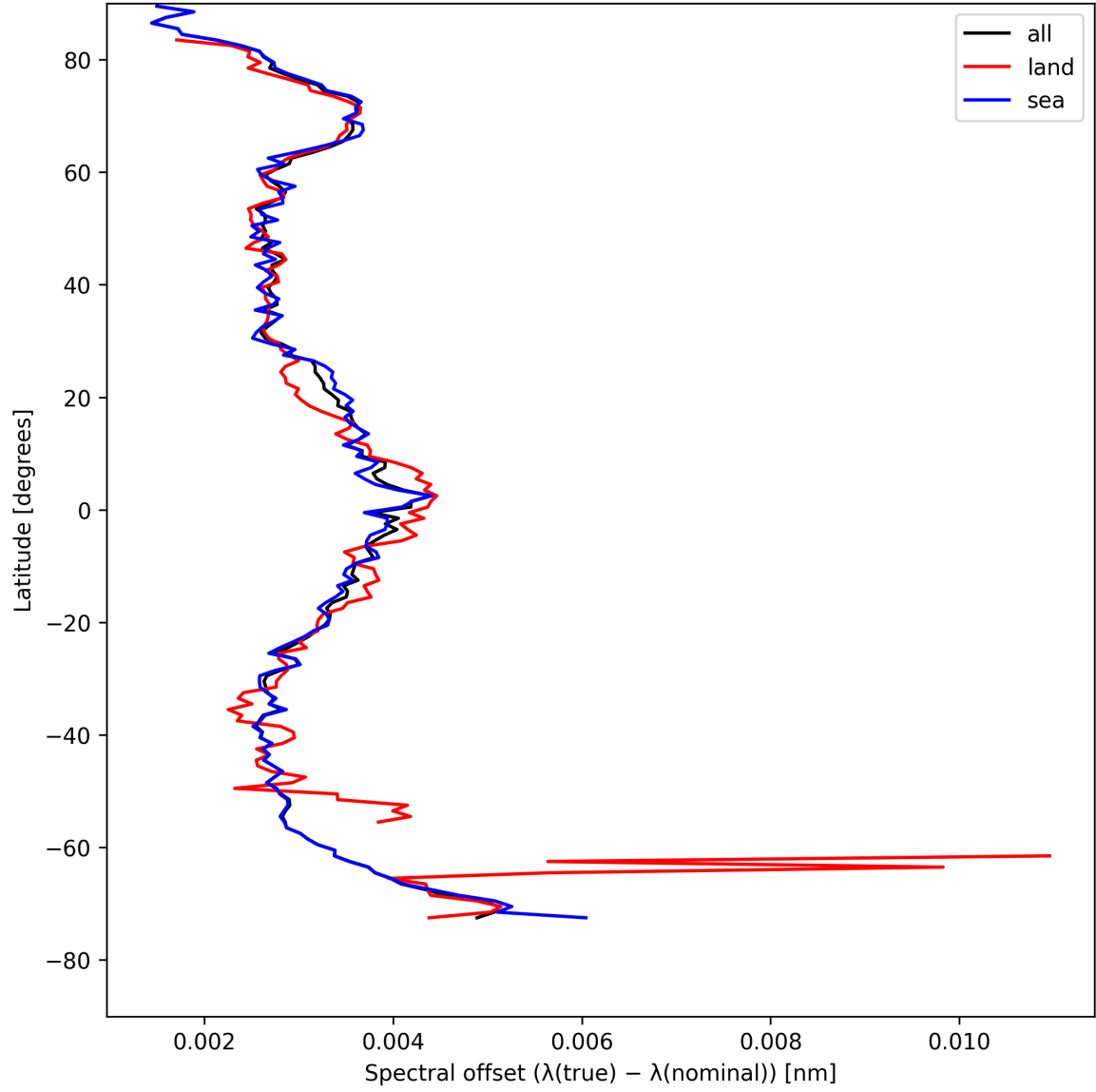
Figure 26: Zonal average of “Spectral offset ( \lambda_{\text{true}} - \lambda_{\text{nominal}} )” for 2025-05-01 to 2025-05-02.
