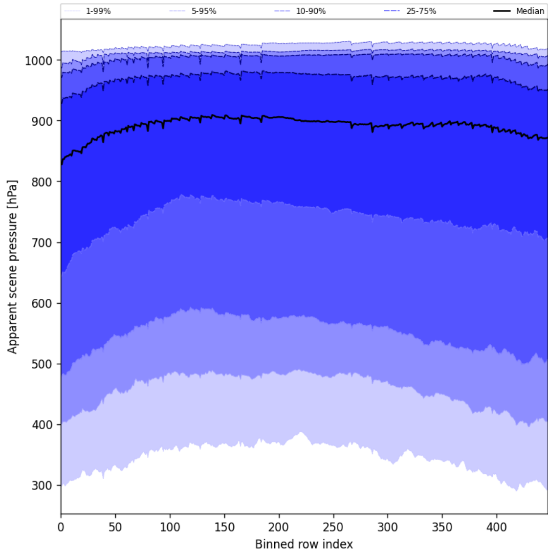
Figure 51: Along track statistics of “Apparent scene pressure” for 2025-05-01 to 2025-05-02
