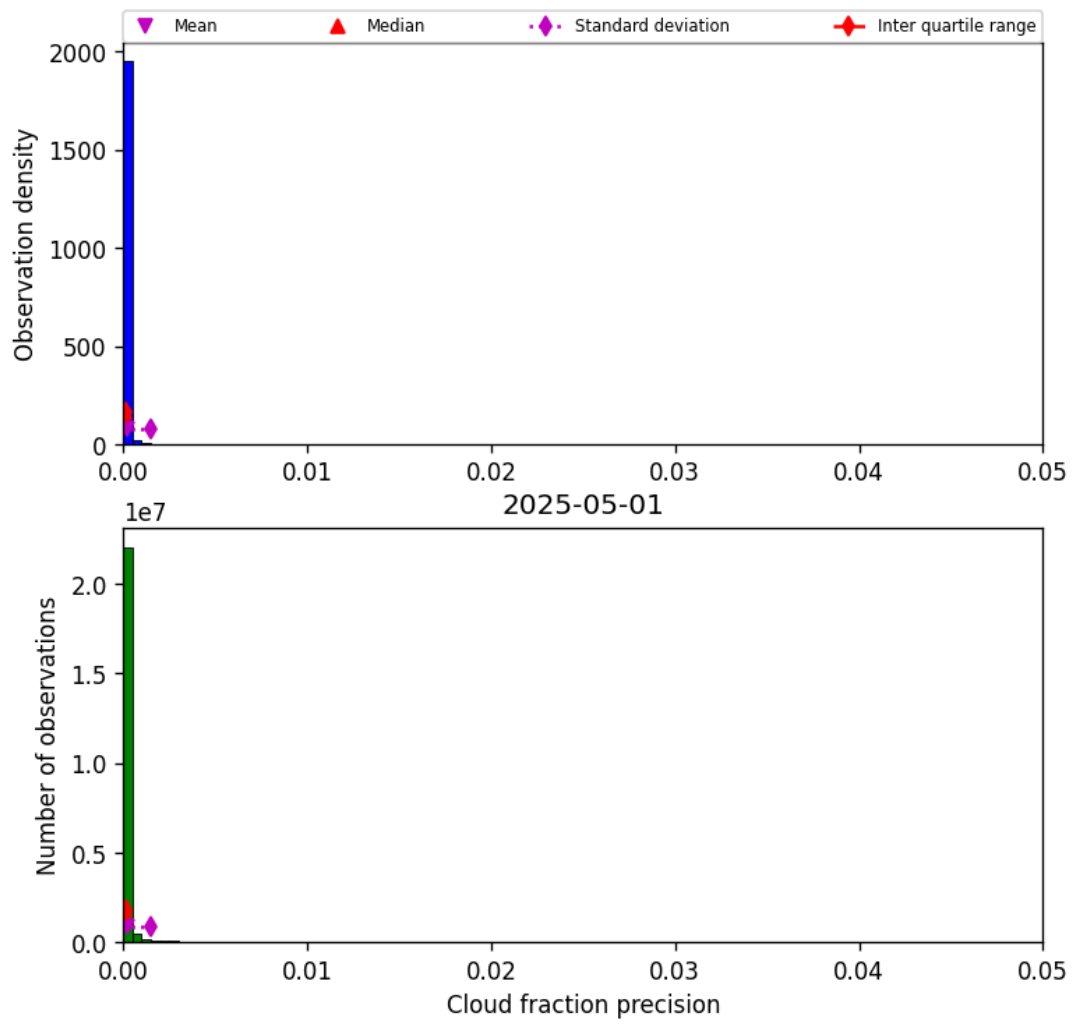
Figure 31: Histogram of “Cloud fraction precision” for 2025-05-01 to 2025-05-02
