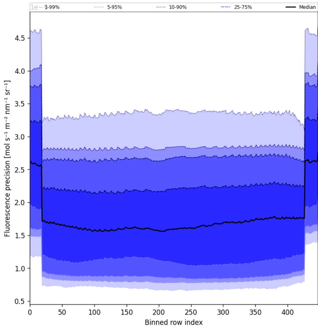
Figure 56: Along track statistics of “Fluorescence precision” for 2025-05-01 to 2025-05-02
