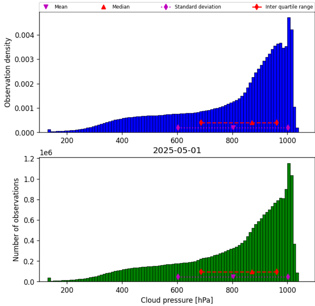
Figure 28: Histogram of “Cloud pressure” for 2025-05-01 to 2025-05-02
