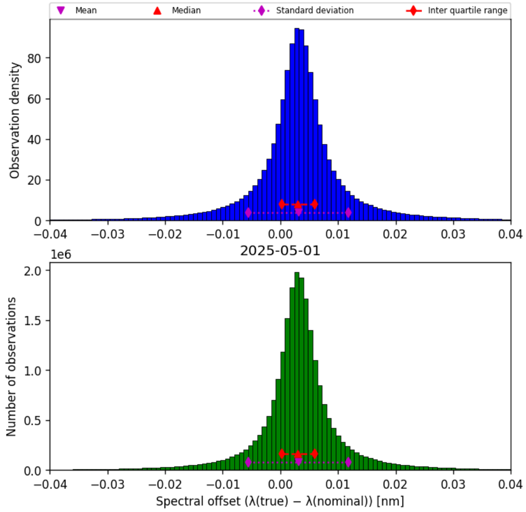
Figure 43: Histogram of “Spectral offset ( \lambda_{\text{true}} - \lambda_{\text{nominal}} )” for 2025-05-01 to 2025-05-02
