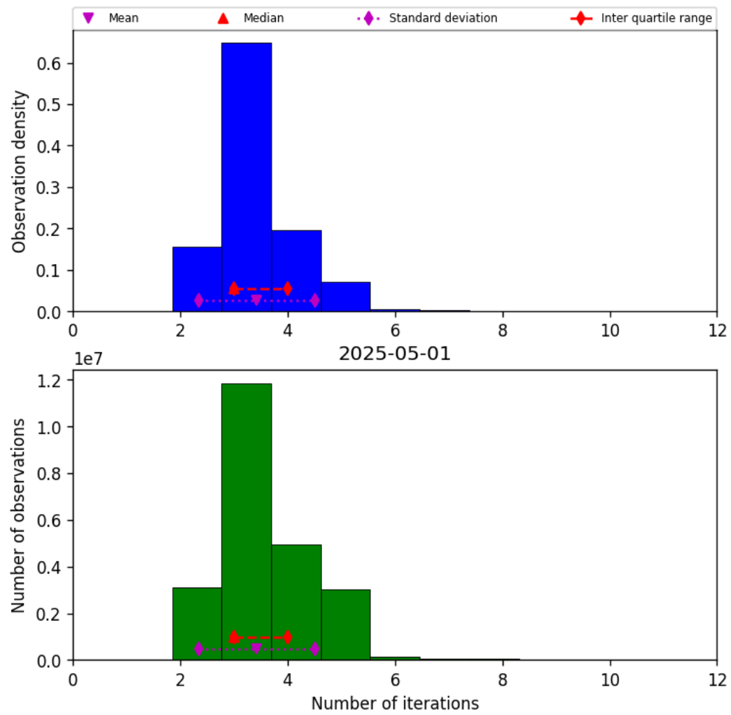
Figure 37: Histogram of “Number of iterations” for 2025-05-01 to 2025-05-02
