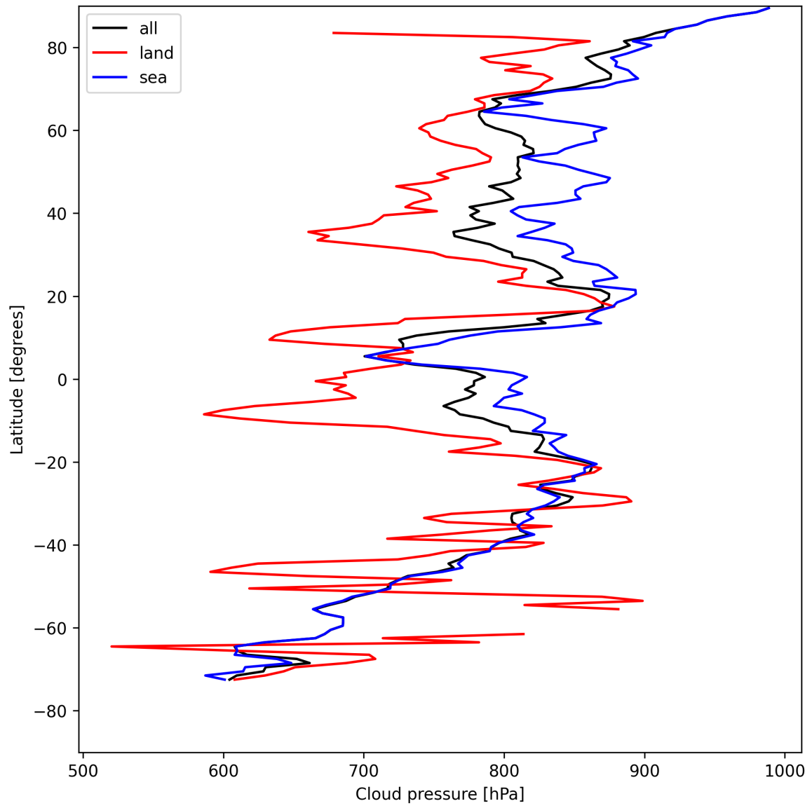
Figure 11: Zonal average of “Cloud pressure” for 2025-05-01 to 2025-05-02.
