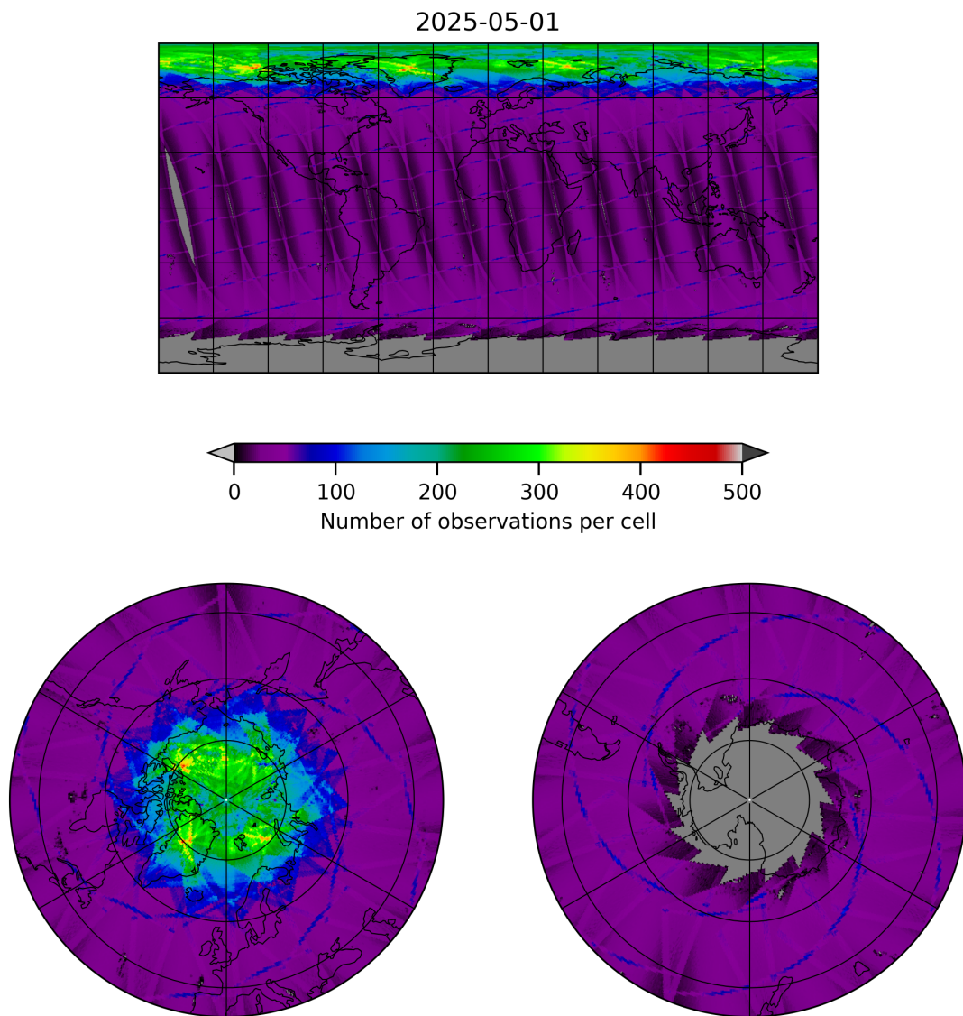
Figure 9: Map of the number of observations for 2025-05-01 to 2025-05-02
