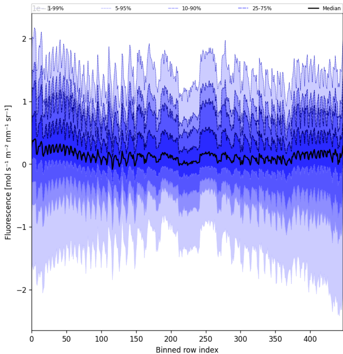
Figure 55: Along track statistics of “Fluorescence” for 2025-05-01 to 2025-05-02
