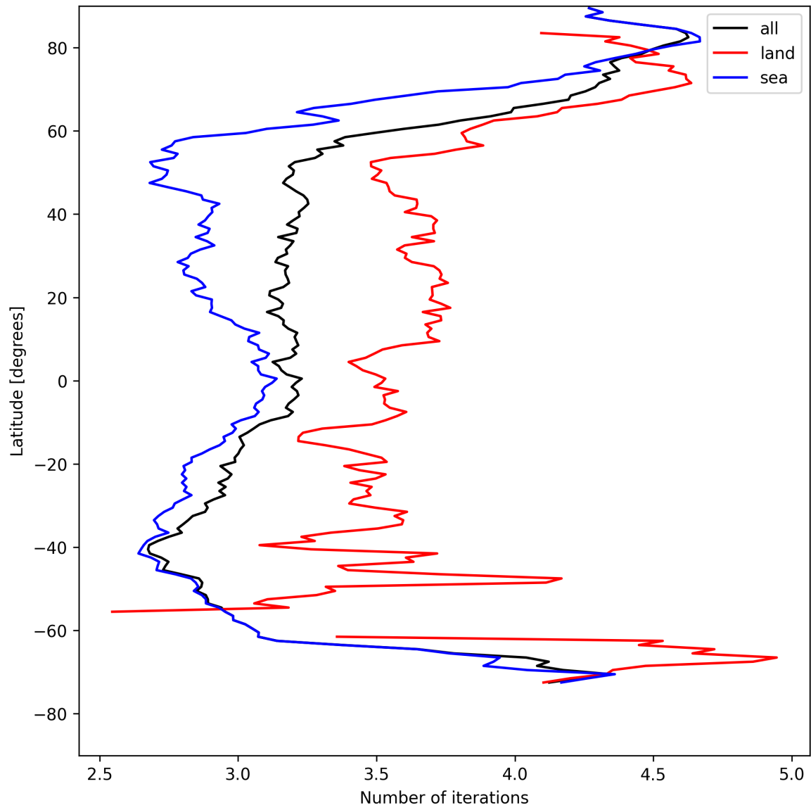
Figure 20: Zonal average of “Number of iterations” for 2025-05-01 to 2025-05-02.
