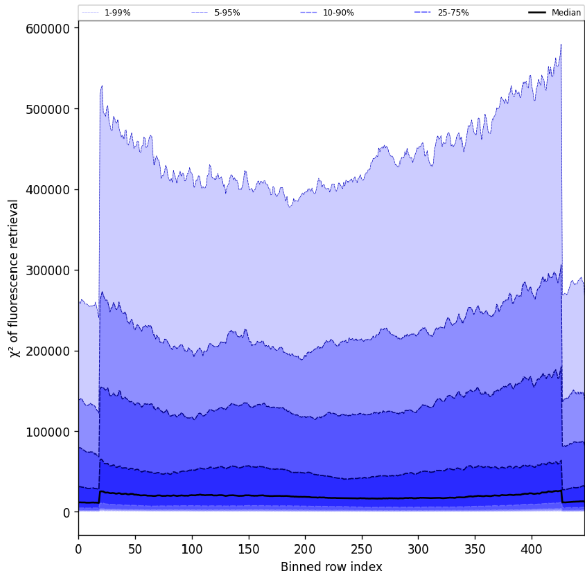
Figure 57: Along track statistics of “ \chi^2 of fluorescence retrieval” for 2025-05-01 to 2025-05-02
