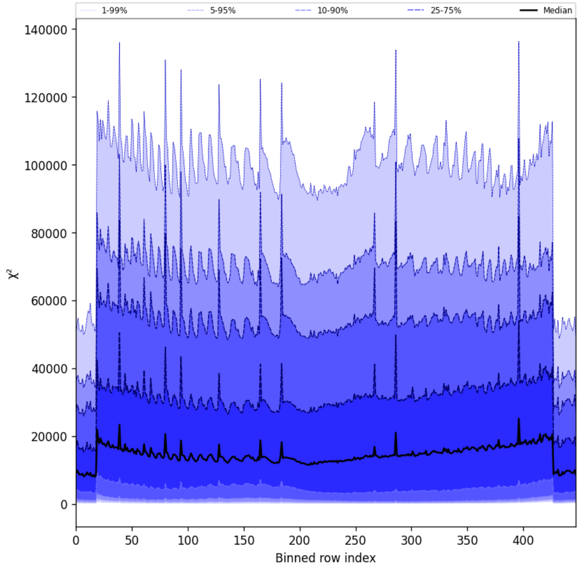
Figure 53: Along track statistics of “ \chi^2 ” for 2025-05-01 to 2025-05-02
