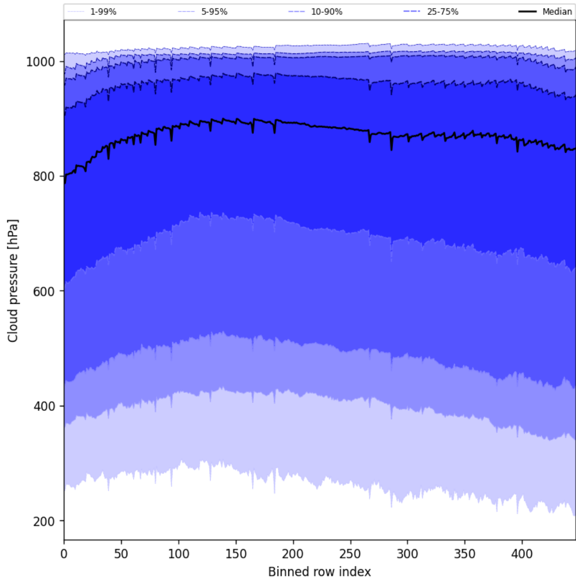
Figure 45: Along track statistics of “Cloud pressure” for 2025-05-01 to 2025-05-02
