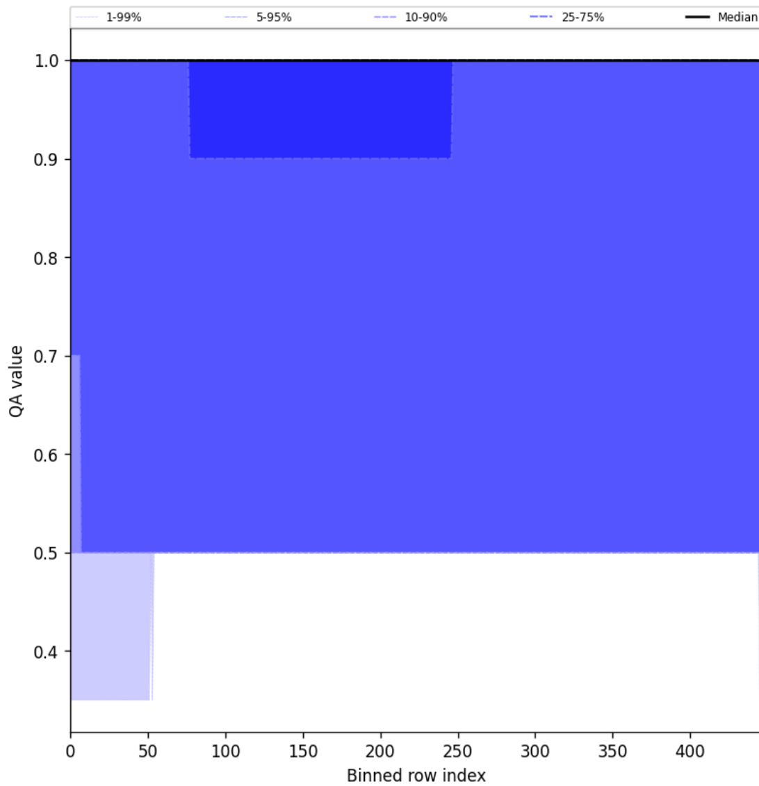
Figure 44: Along track statistics of “QA value” for 2025-05-01 to 2025-05-02
