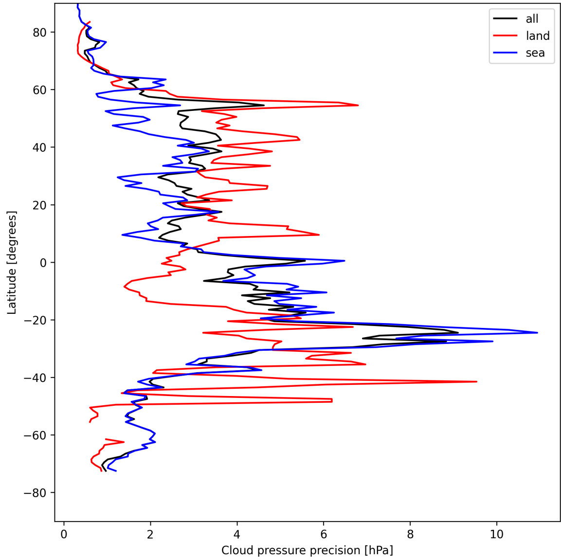
Figure 12: Zonal average of “Cloud pressure precision” for 2025-05-01 to 2025-05-02.
