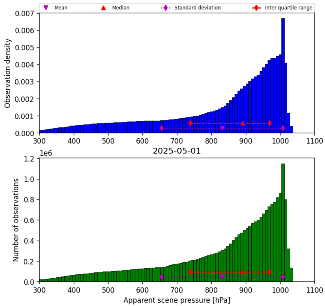
Figure 34: Histogram of “Apparent scene pressure” for 2025-05-01 to 2025-05-02
