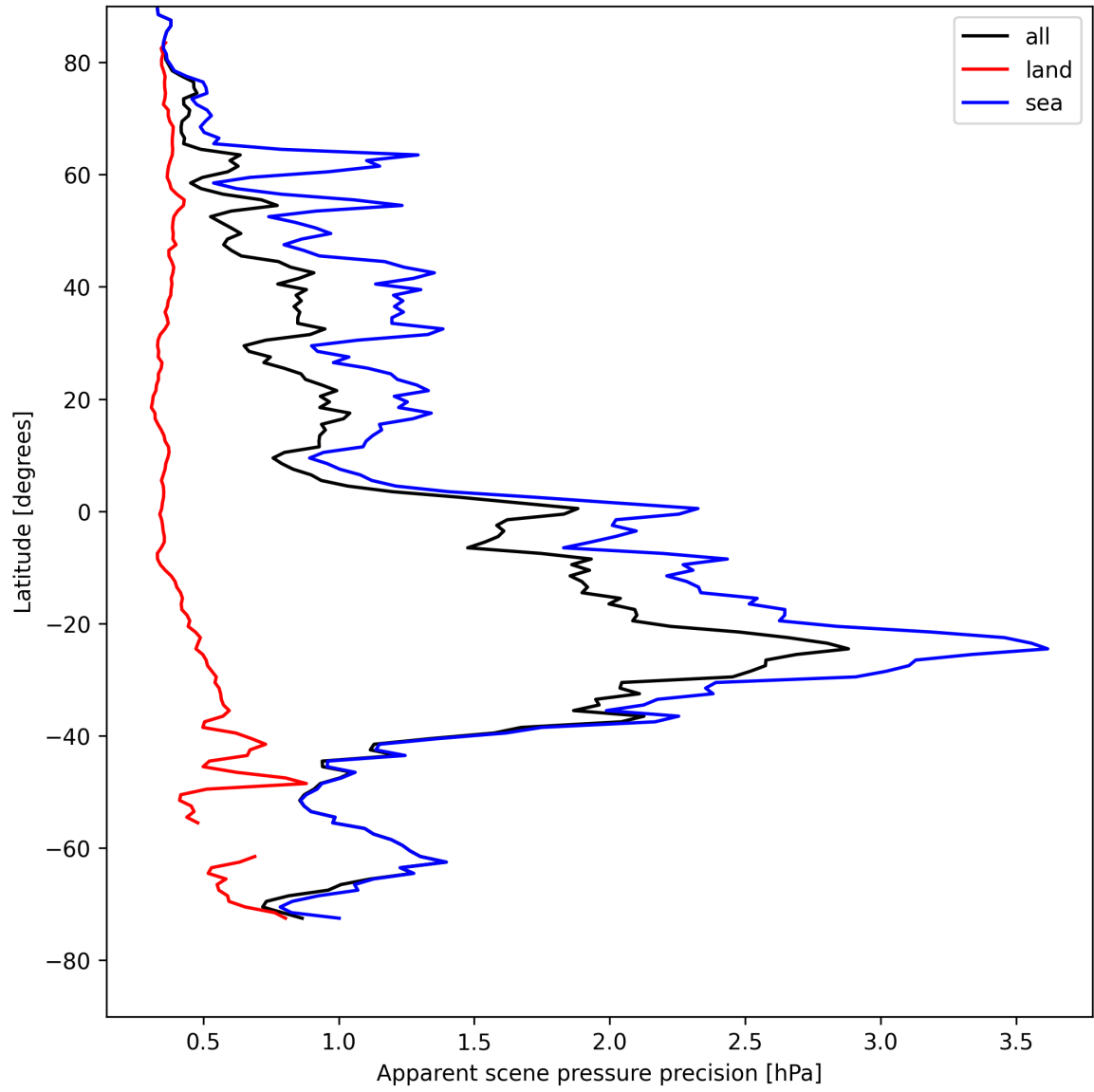
Figure 18: Zonal average of “Apparent scene pressure precision” for 2025-05-01 to 2025-05-02.
