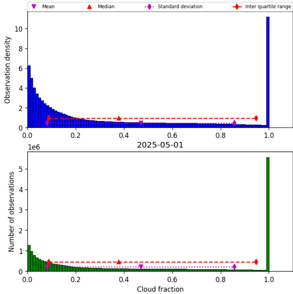
Figure 30: Histogram of “Cloud fraction” for 2025-05-01 to 2025-05-02
