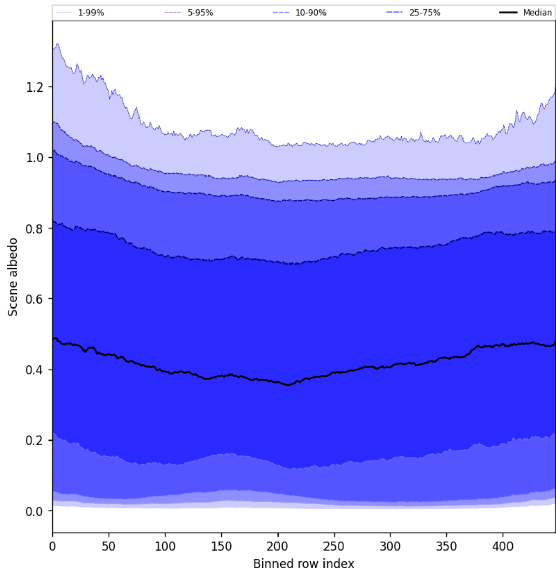
Figure 49: Along track statistics of “Scene albedo” for 2025-05-01 to 2025-05-02
