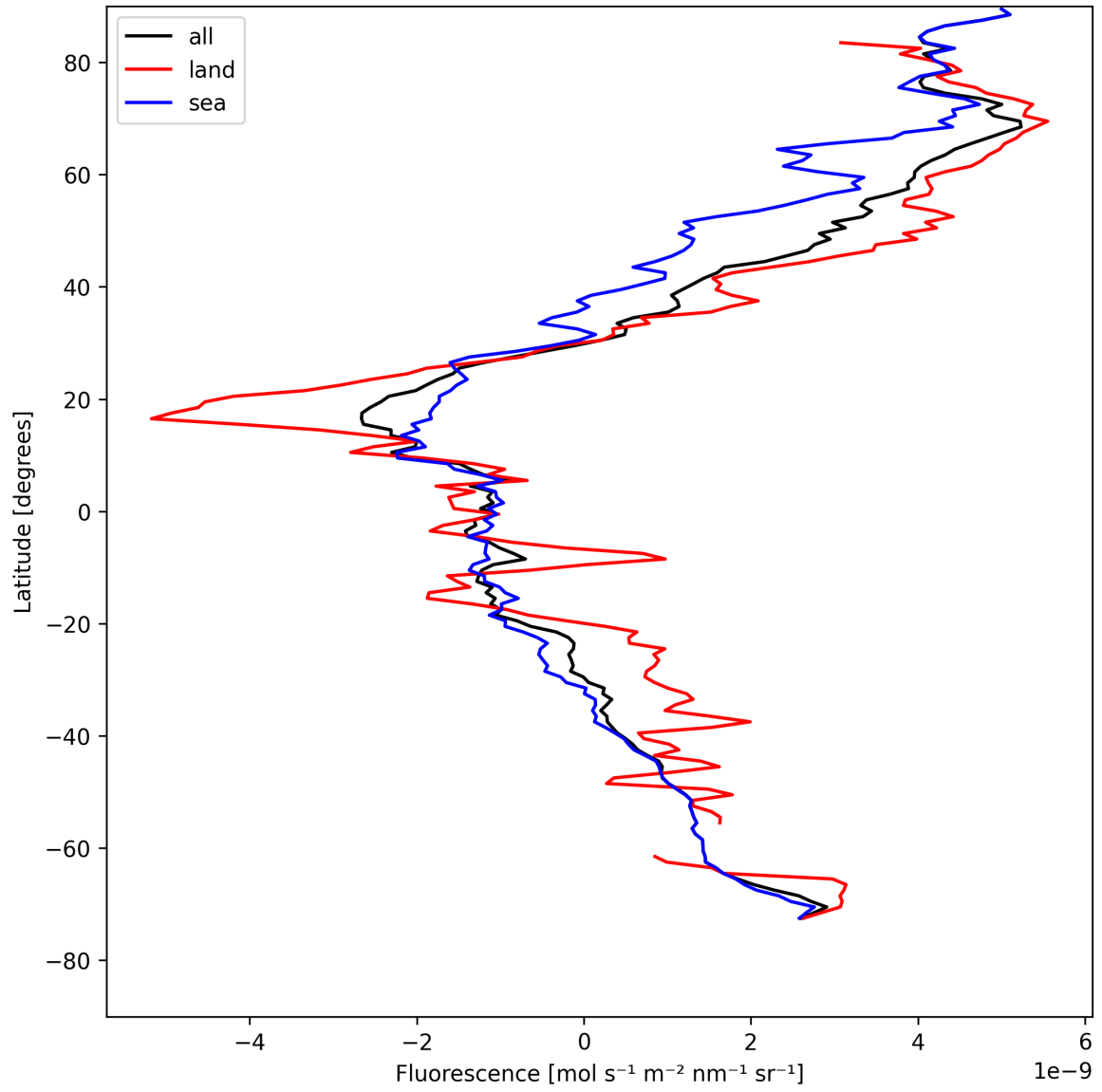
Figure 21: Zonal average of “Fluorescence” for 2025-05-01 to 2025-05-02.
