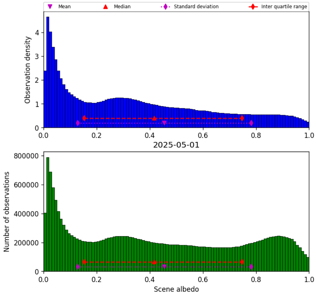
Figure 32: Histogram of “Scene albedo” for 2025-05-01 to 2025-05-02
