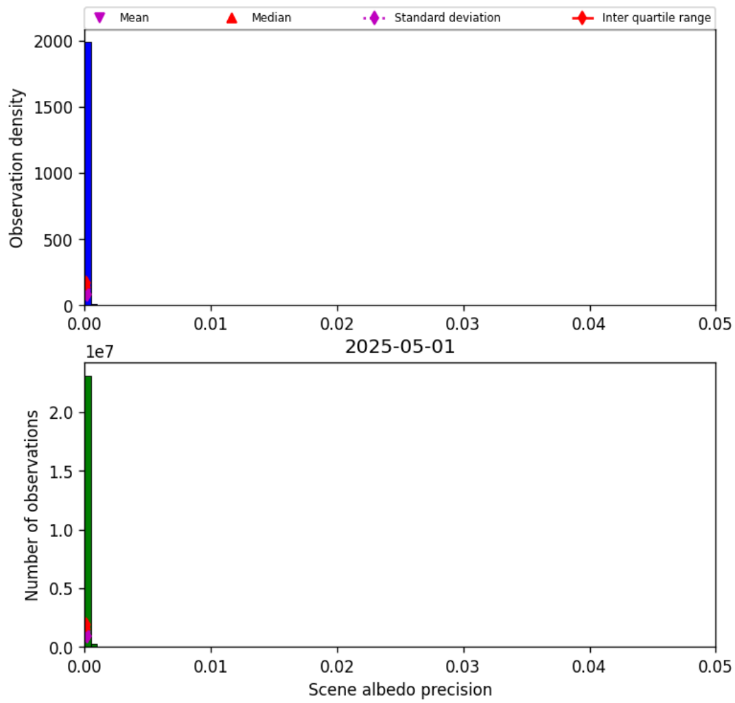
Figure 33: Histogram of “Scene albedo precision” for 2025-05-01 to 2025-05-02
