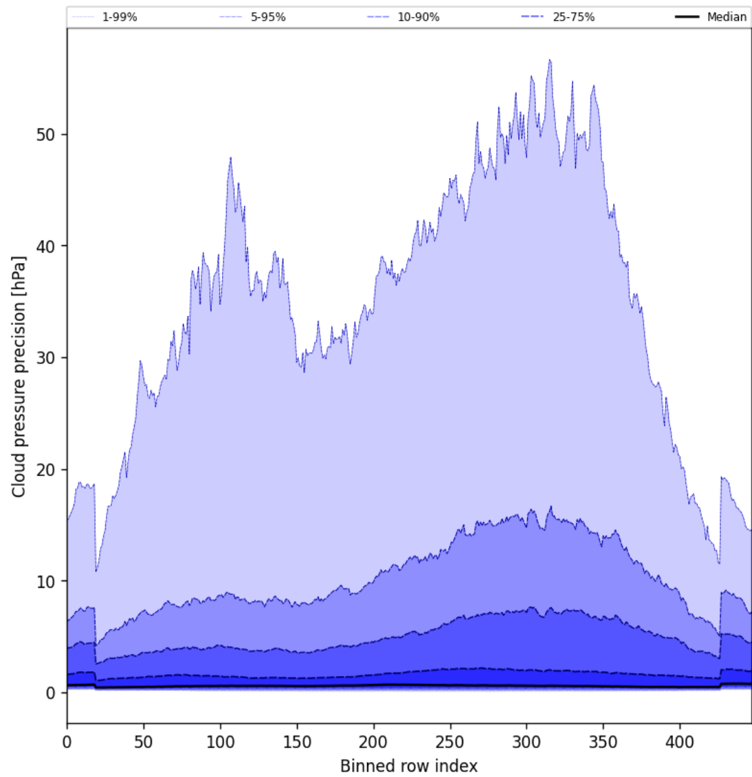
Figure 46: Along track statistics of “Cloud pressure precision” for 2025-05-01 to 2025-05-02
