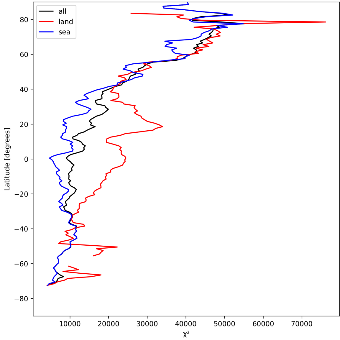
Figure 19: Zonal average of “ \chi^2 ” for 2025-05-01 to 2025-05-02.
