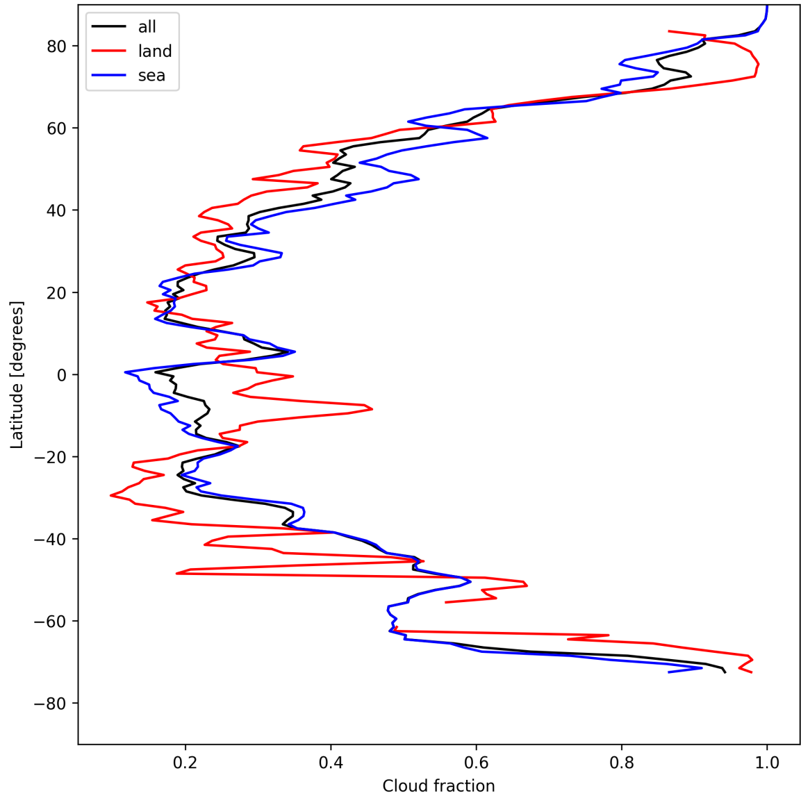
Figure 13: Zonal average of “Cloud fraction” for 2025-05-01 to 2025-05-02.
