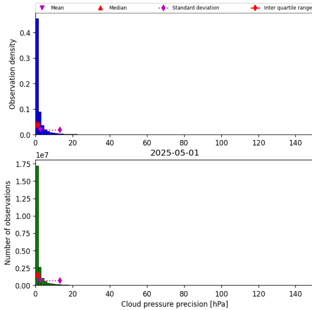
Figure 29: Histogram of “Cloud pressure precision” for 2025-05-01 to 2025-05-02
