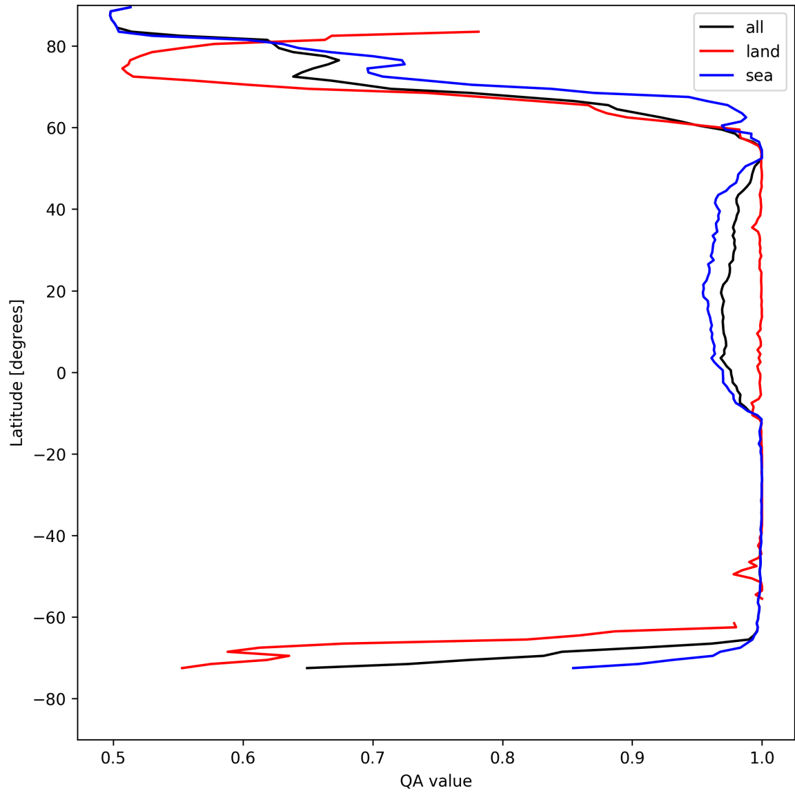
Figure 10: Zonal average of “QA value” for 2025-05-01 to 2025-05-02.
