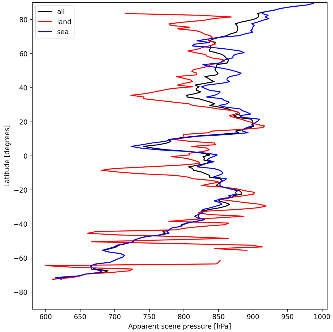
Figure 17: Zonal average of “Apparent scene pressure” for 2025-05-01 to 2025-05-02.
