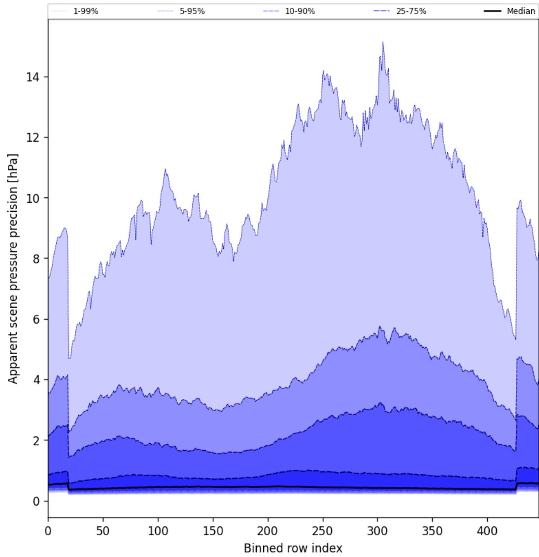
Figure 52: Along track statistics of “Apparent scene pressure precision” for 2025-05-01 to 2025-05-02
