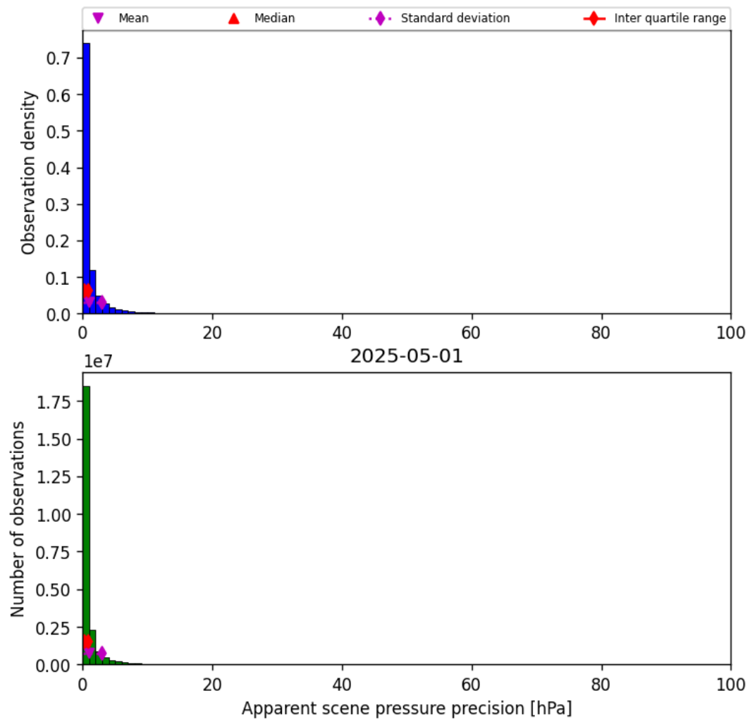
Figure 35: Histogram of “Apparent scene pressure precision” for 2025-05-01 to 2025-05-02
