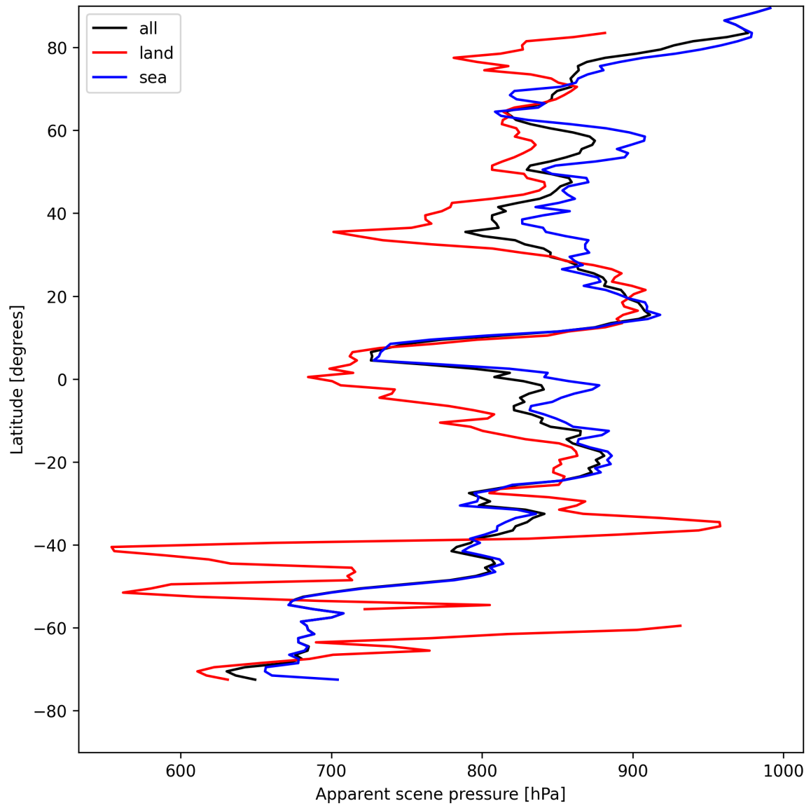
Figure 17: Zonal average of “Apparent scene pressure” for 2025-05-02 to 2025-05-02.
