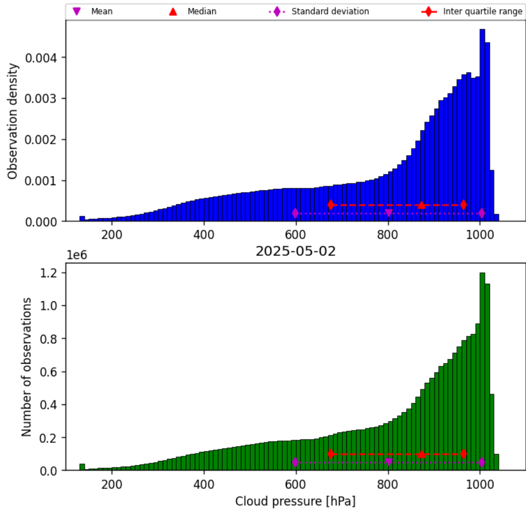
Figure 28: Histogram of “Cloud pressure” for 2025-05-02 to 2025-05-02
