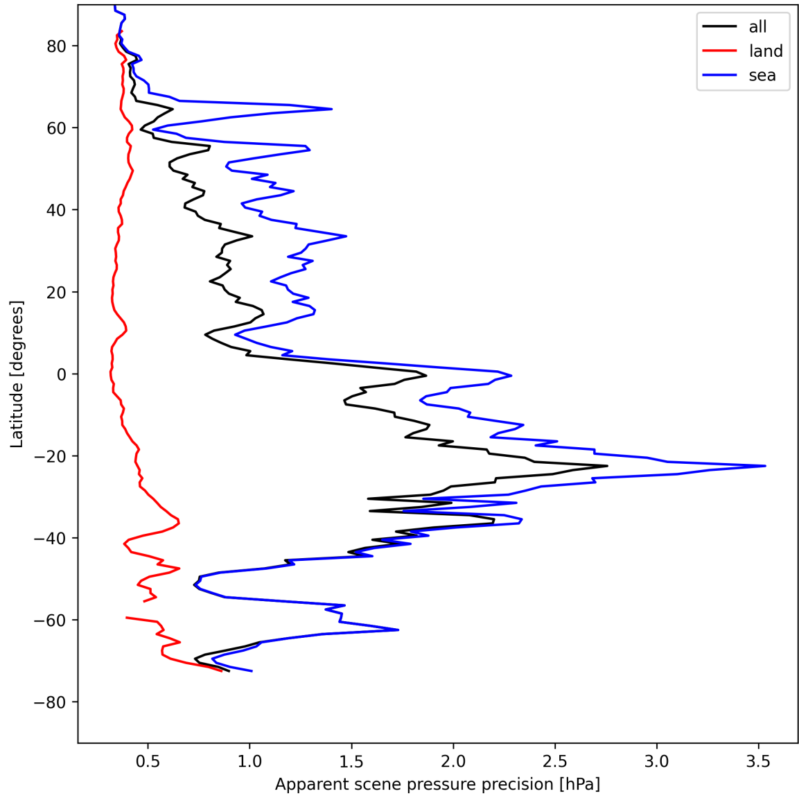
Figure 18: Zonal average of “Apparent scene pressure precision” for 2025-05-02 to 2025-05-02.
