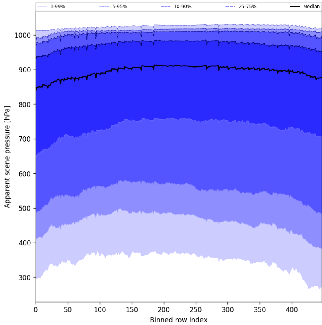
Figure 51: Along track statistics of “Apparent scene pressure” for 2025-05-02 to 2025-05-02
