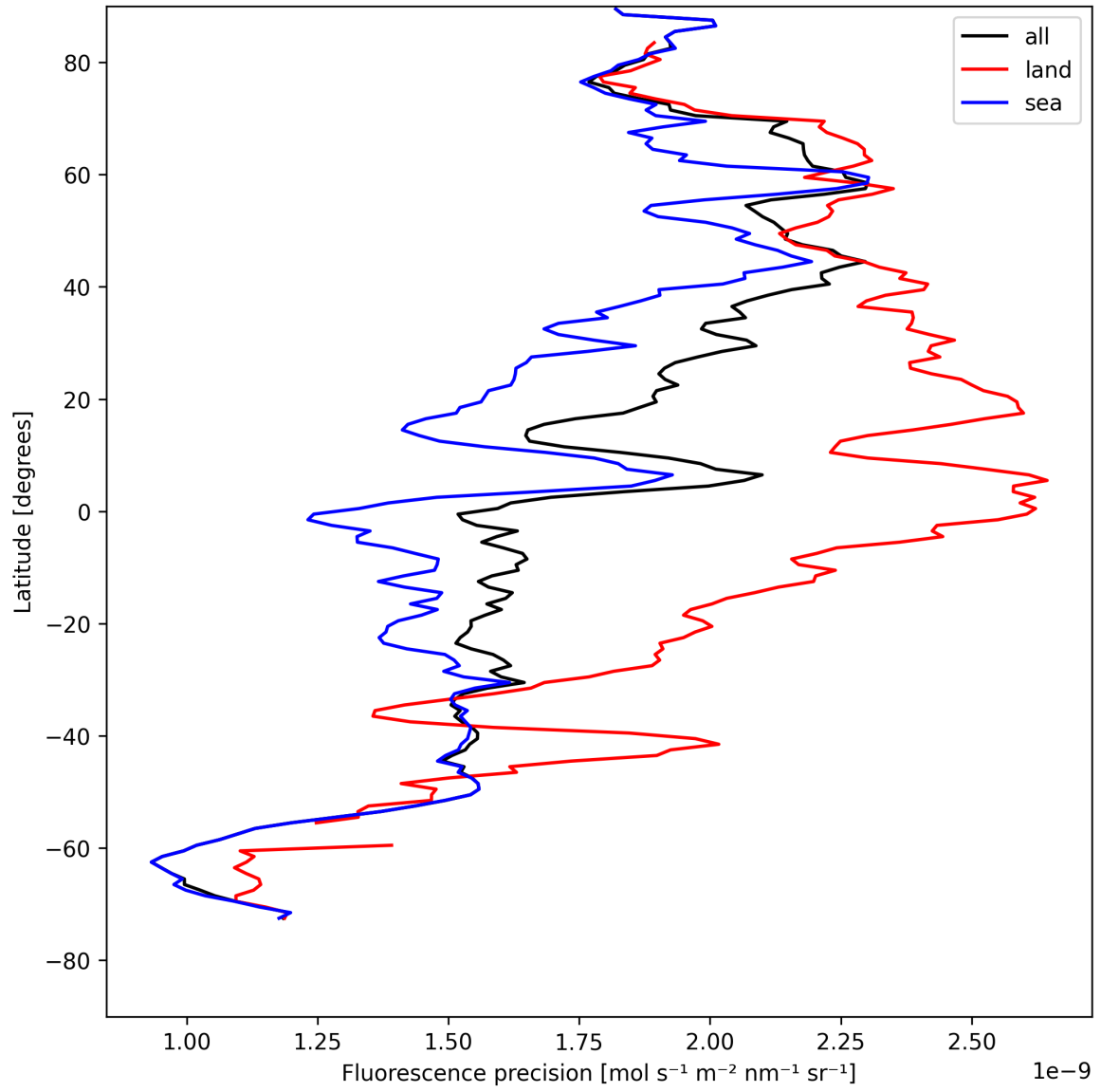
Figure 22: Zonal average of “Fluorescence precision” for 2025-05-02 to 2025-05-02.
