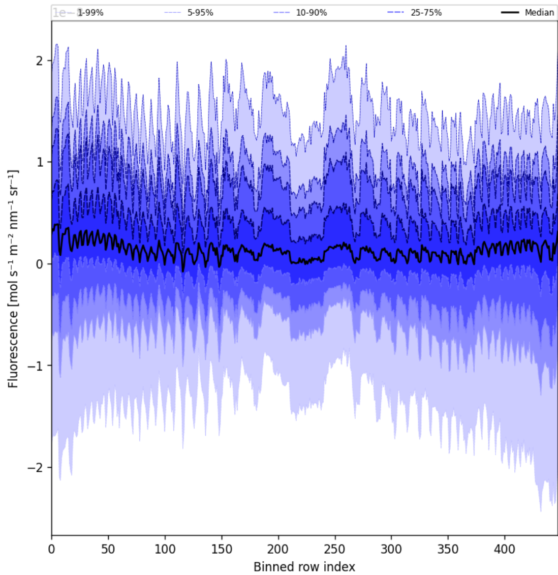
Figure 55: Along track statistics of “Fluorescence” for 2025-05-07 to 2025-05-08
