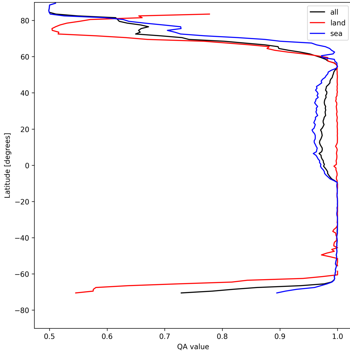
Figure 10: Zonal average of “QA value” for 2025-05-07 to 2025-05-08.
