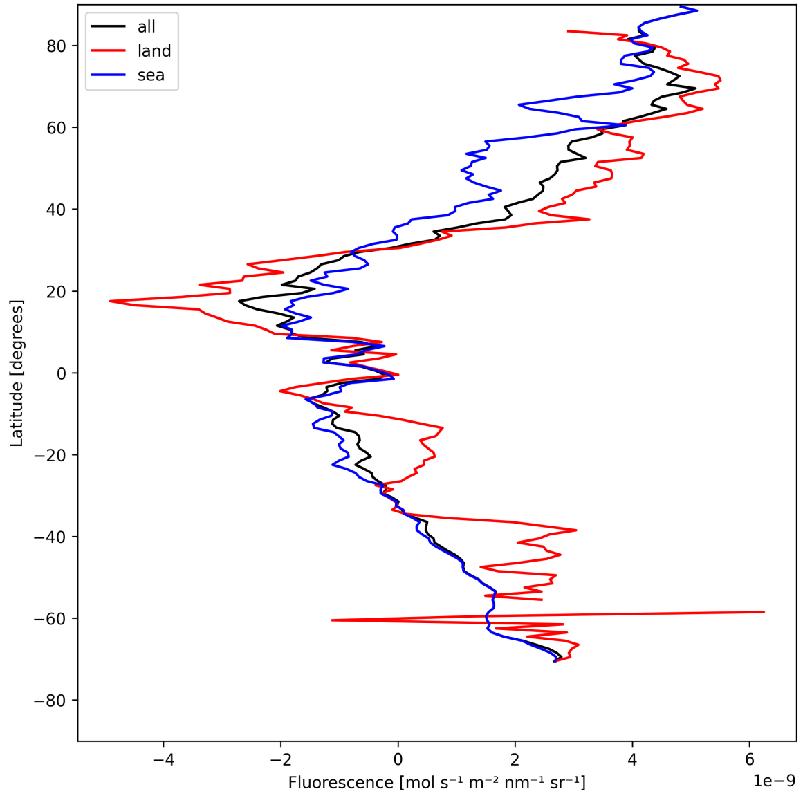
Figure 21: Zonal average of “Fluorescence” for 2025-05-07 to 2025-05-08.
