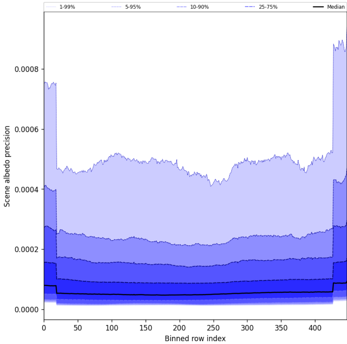
Figure 50: Along track statistics of “Scene albedo precision” for 2025-05-07 to 2025-05-08
