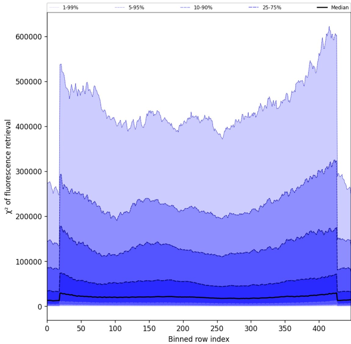
Figure 57: Along track statistics of “ \chi^2 of fluorescence retrieval” for 2025-05-07 to 2025-05-08
