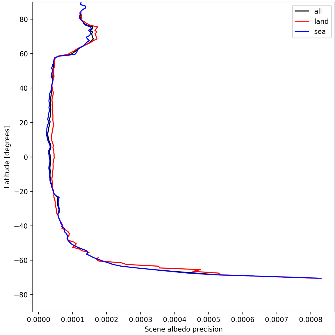
Figure 16: Zonal average of “Scene albedo precision” for 2025-05-07 to 2025-05-08.
