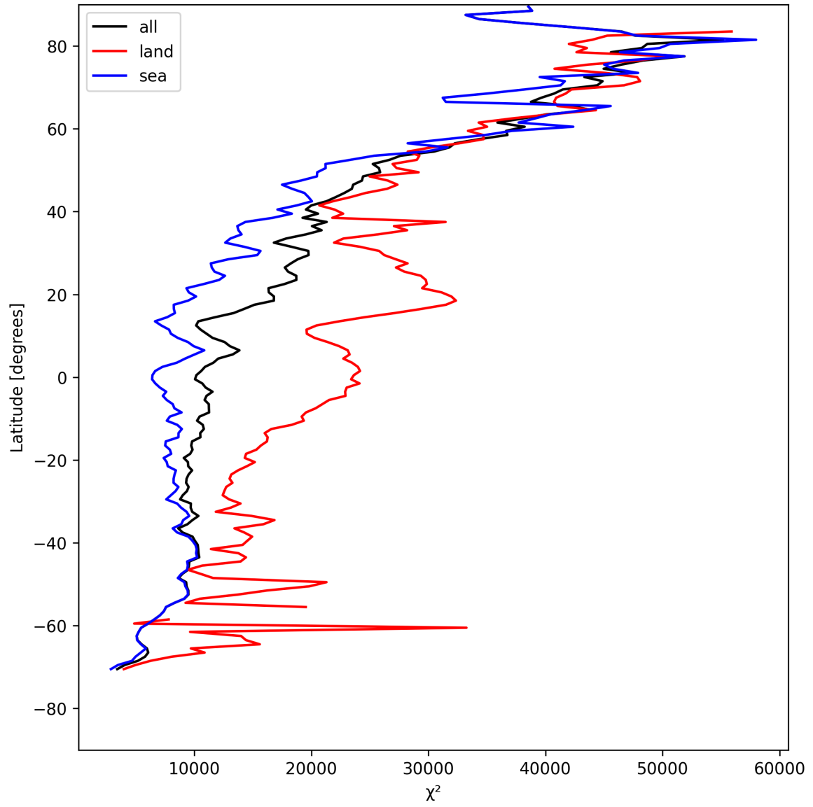
Figure 19: Zonal average of “ \chi^2 ” for 2025-05-07 to 2025-05-08.
