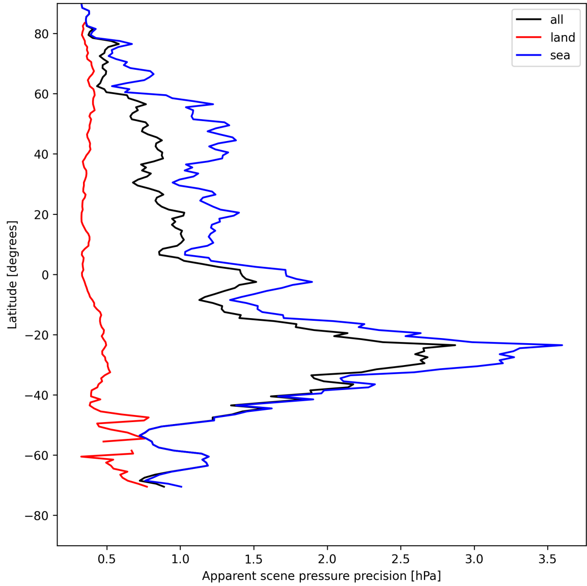
Figure 18: Zonal average of “Apparent scene pressure precision” for 2025-05-07 to 2025-05-08.
