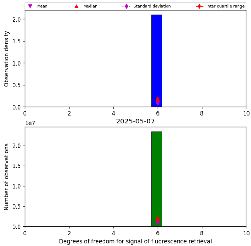
Figure 41: Histogram of “Degrees of freedom for signal of fluorescence retrieval” for 2025-05-07 to 2025-05-08
