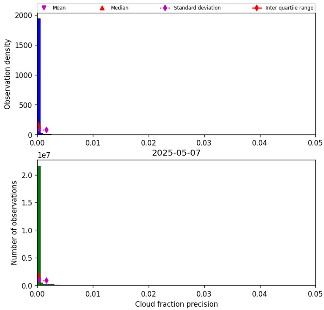
Figure 31: Histogram of “Cloud fraction precision” for 2025-05-07 to 2025-05-08
