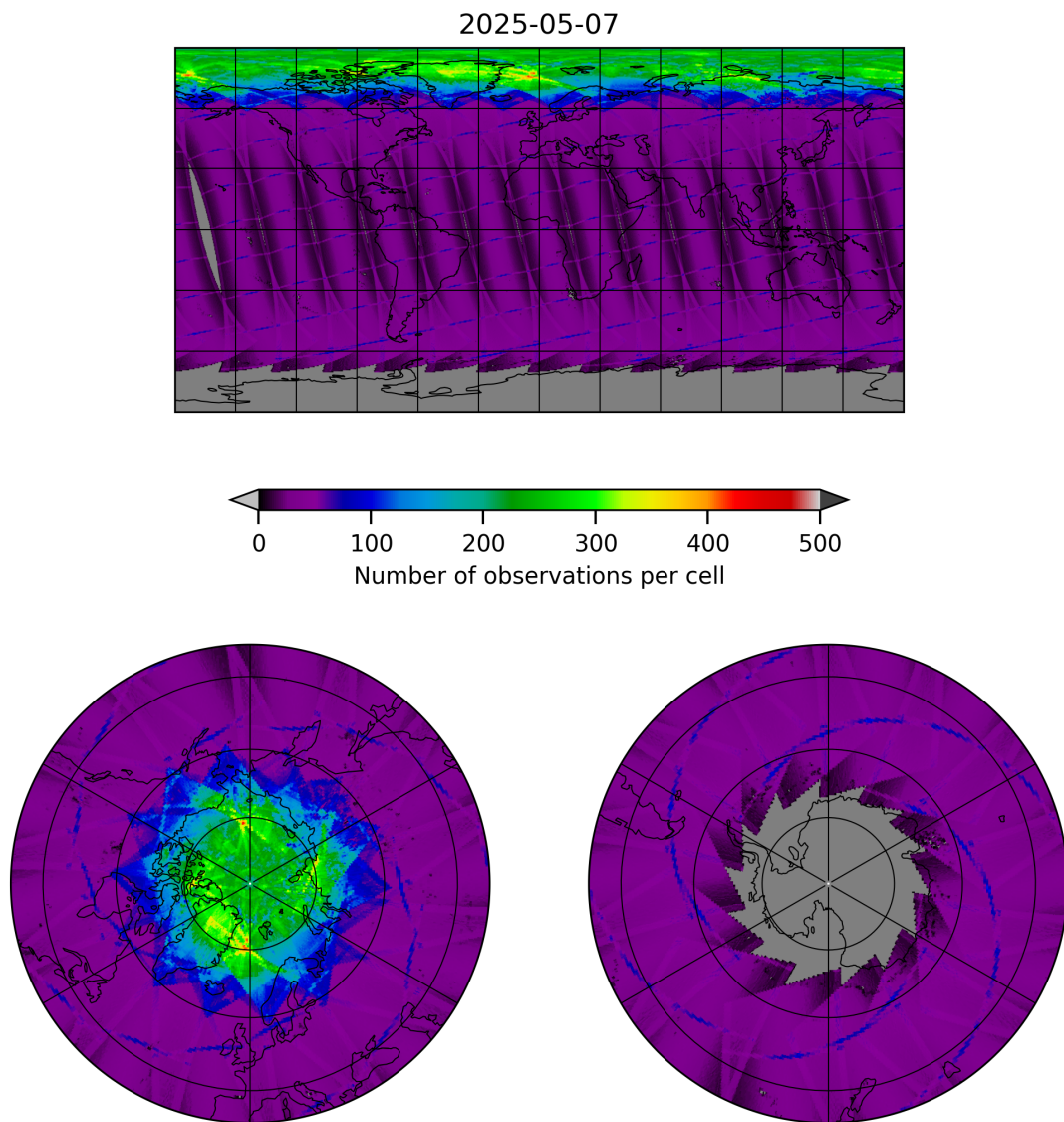
Figure 9: Map of the number of observations for 2025-05-07 to 2025-05-08
