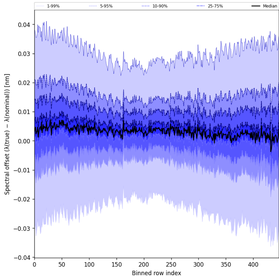
Figure 60: Along track statistics of “Spectral offset ( \lambda_{\text{true}} - \lambda_{\text{nominal}} )” for 2025-05-07 to 2025-05-08
