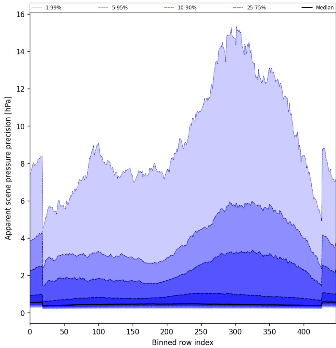
Figure 52: Along track statistics of “Apparent scene pressure precision” for 2025-05-07 to 2025-05-08
