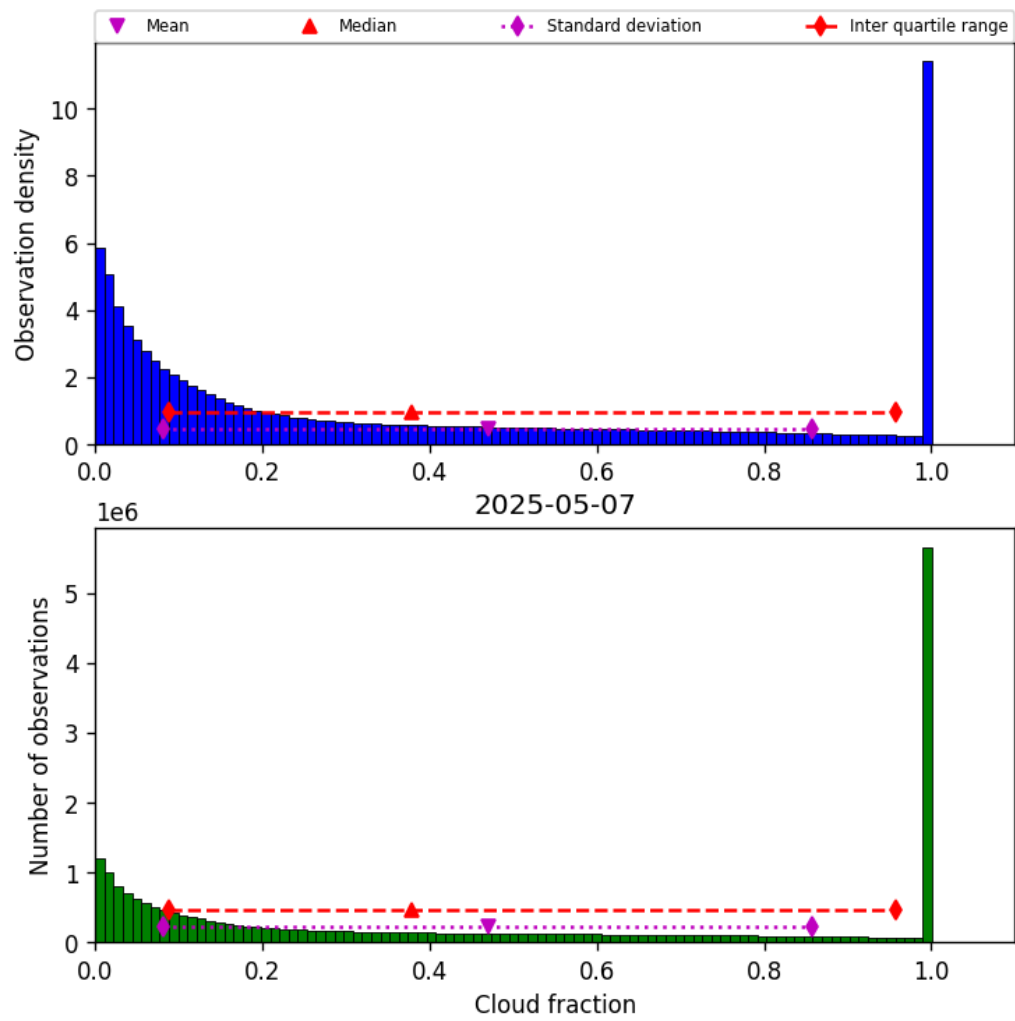
Figure 30: Histogram of “Cloud fraction” for 2025-05-07 to 2025-05-08
