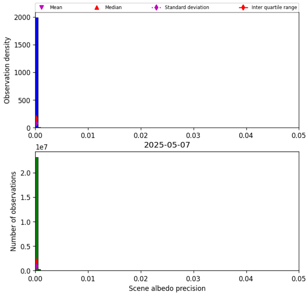
Figure 33: Histogram of “Scene albedo precision” for 2025-05-07 to 2025-05-08
