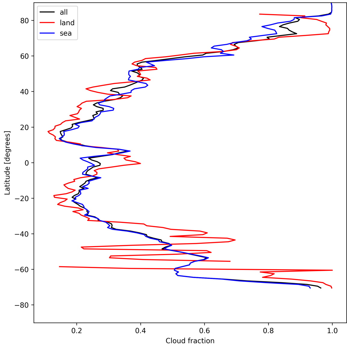
Figure 13: Zonal average of “Cloud fraction” for 2025-05-07 to 2025-05-08.
