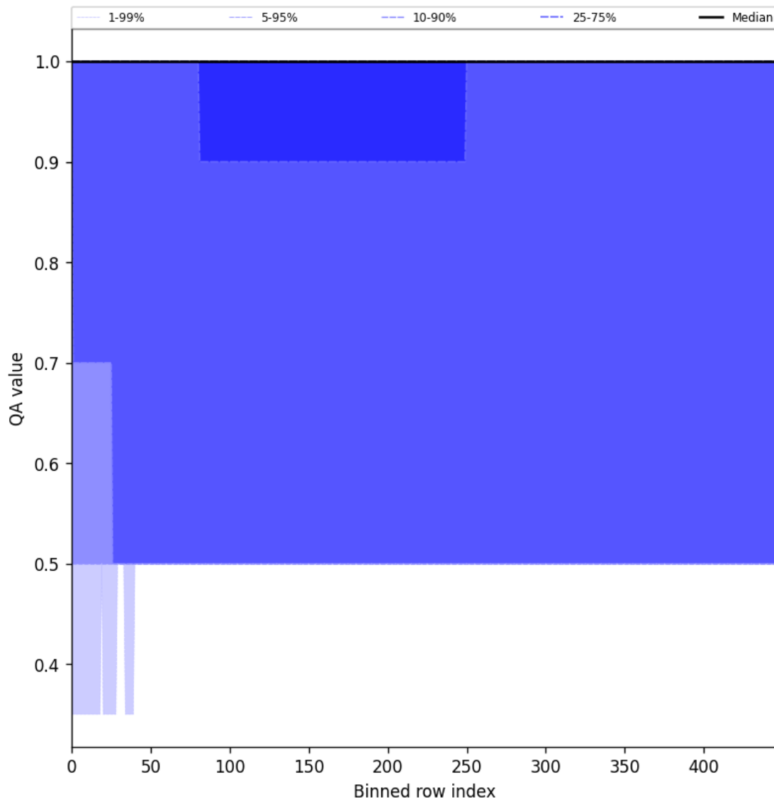
Figure 44: Along track statistics of “QA value” for 2025-05-07 to 2025-05-08
