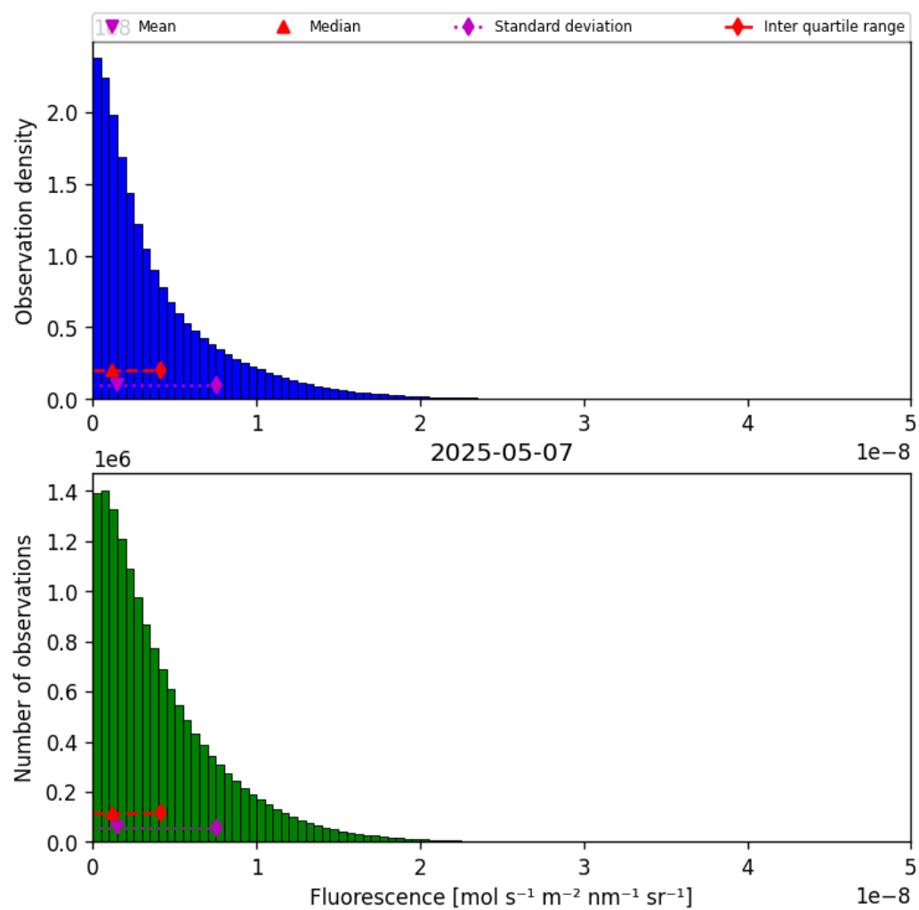
Figure 38: Histogram of “Fluorescence” for 2025-05-07 to 2025-05-08
