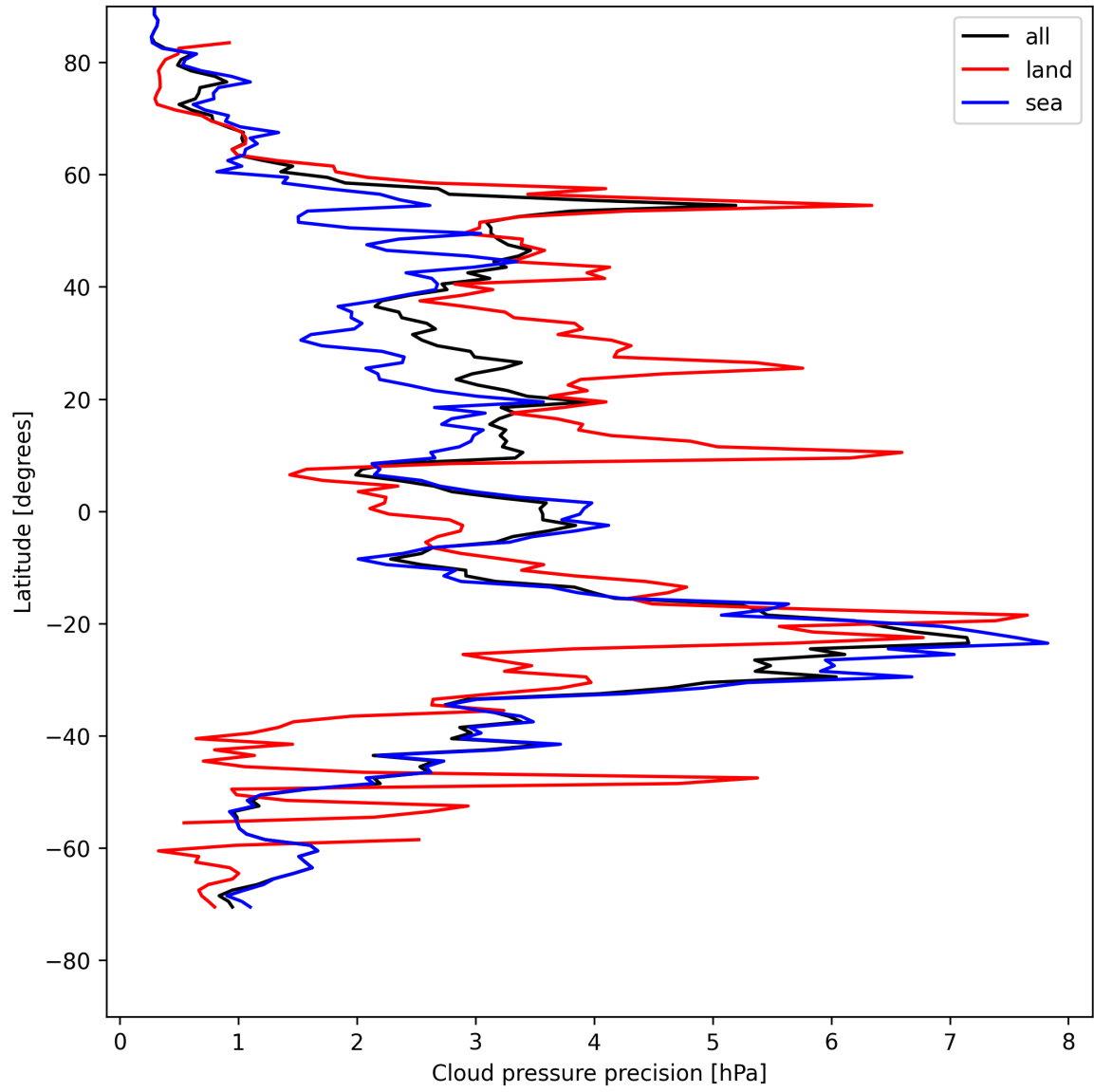
Figure 12: Zonal average of “Cloud pressure precision” for 2025-05-07 to 2025-05-08.
