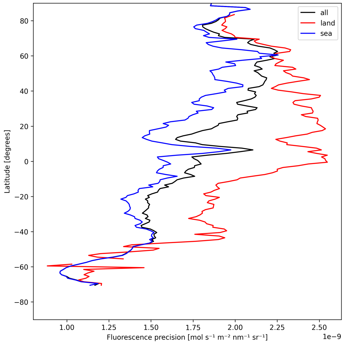
Figure 22: Zonal average of “Fluorescence precision” for 2025-05-07 to 2025-05-08.
