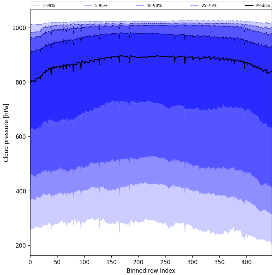
Figure 45: Along track statistics of “Cloud pressure” for 2025-05-07 to 2025-05-08
