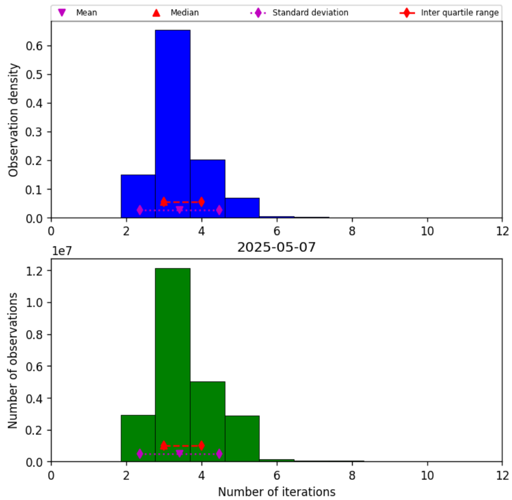
Figure 37: Histogram of “Number of iterations” for 2025-05-07 to 2025-05-08
