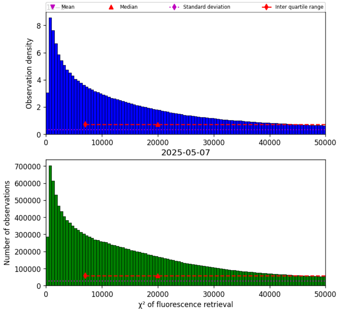
Figure 40: Histogram of “ \chi^2 of fluorescence retrieval” for 2025-05-07 to 2025-05-08
