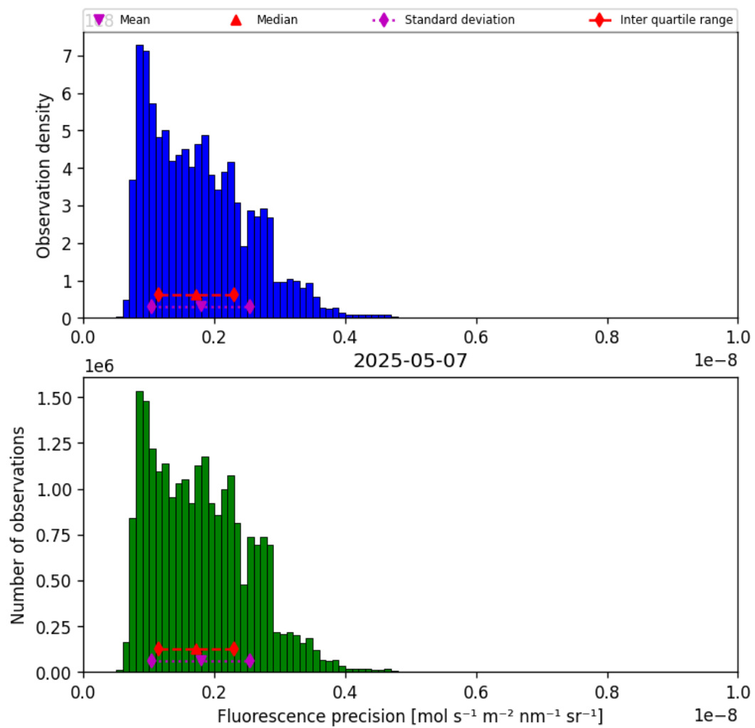
Figure 39: Histogram of “Fluorescence precision” for 2025-05-07 to 2025-05-08
