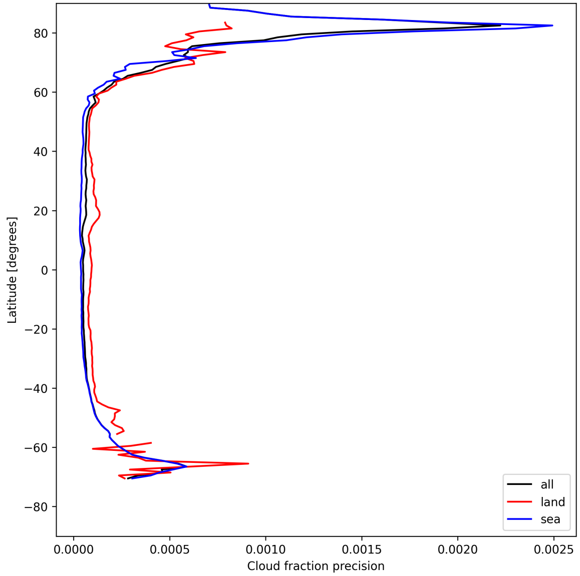
Figure 14: Zonal average of “Cloud fraction precision” for 2025-05-07 to 2025-05-08.
