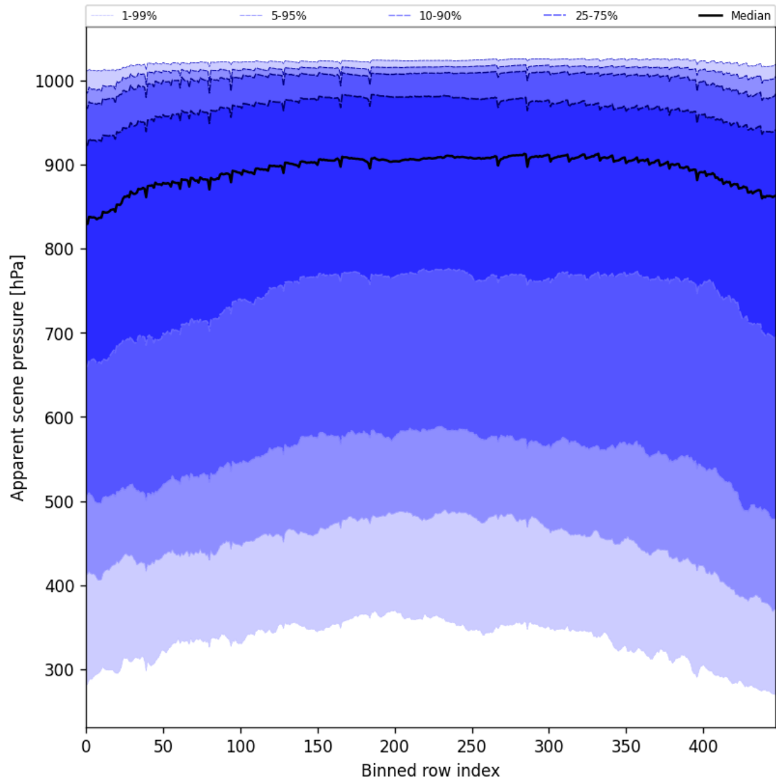
Figure 51: Along track statistics of “Apparent scene pressure” for 2025-05-07 to 2025-05-08
