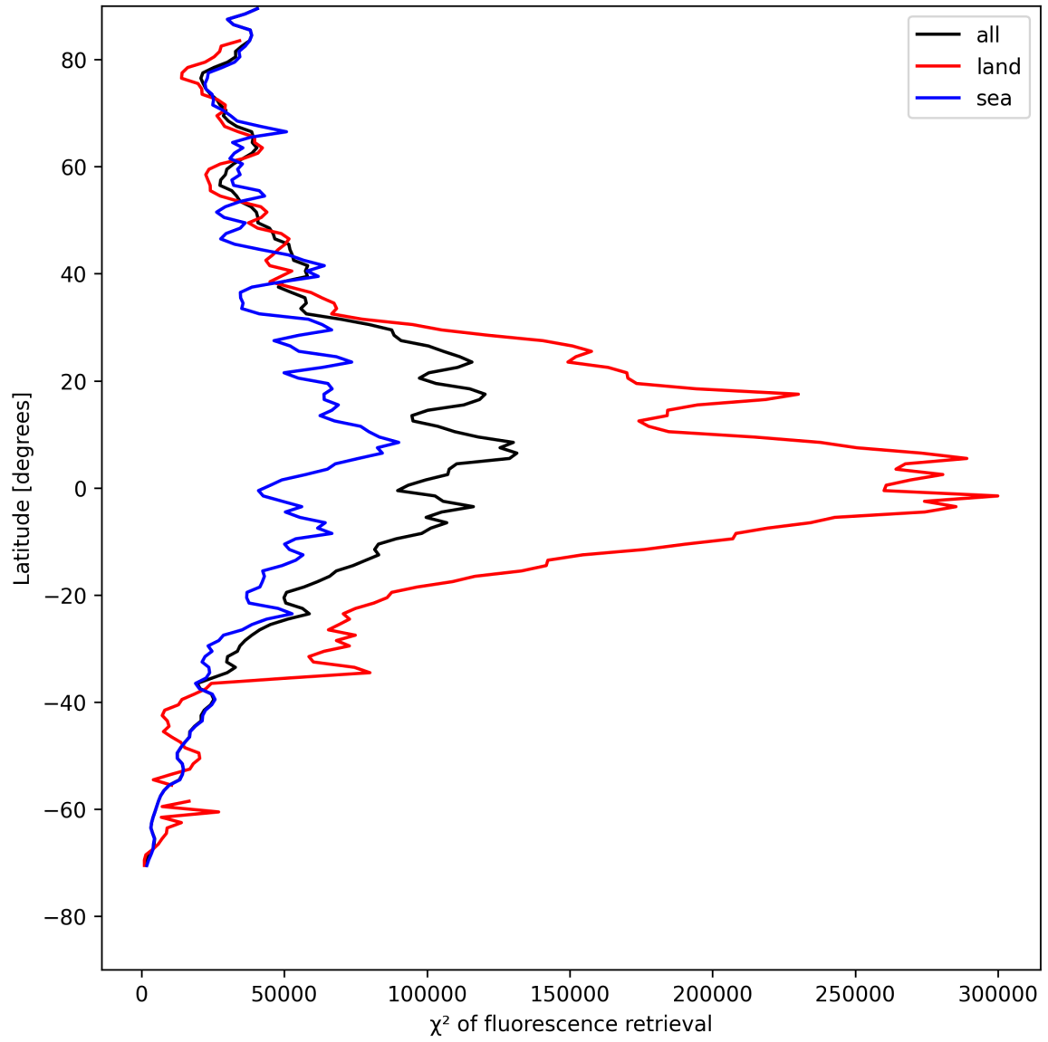
Figure 23: Zonal average of “ \chi^2 of fluorescence retrieval” for 2025-05-07 to 2025-05-08.
