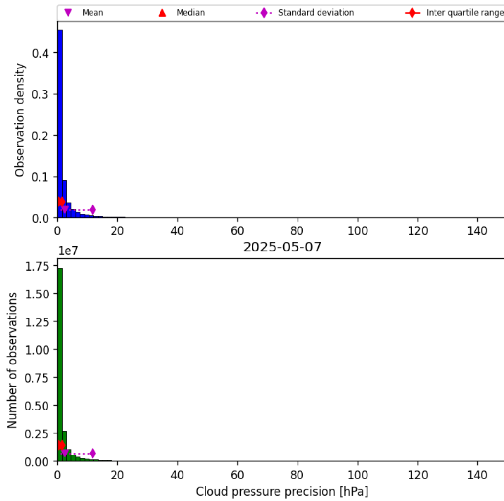
Figure 29: Histogram of “Cloud pressure precision” for 2025-05-07 to 2025-05-08
