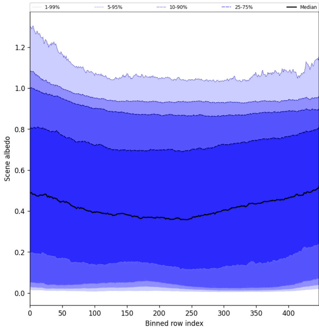
Figure 49: Along track statistics of “Scene albedo” for 2025-05-07 to 2025-05-08
