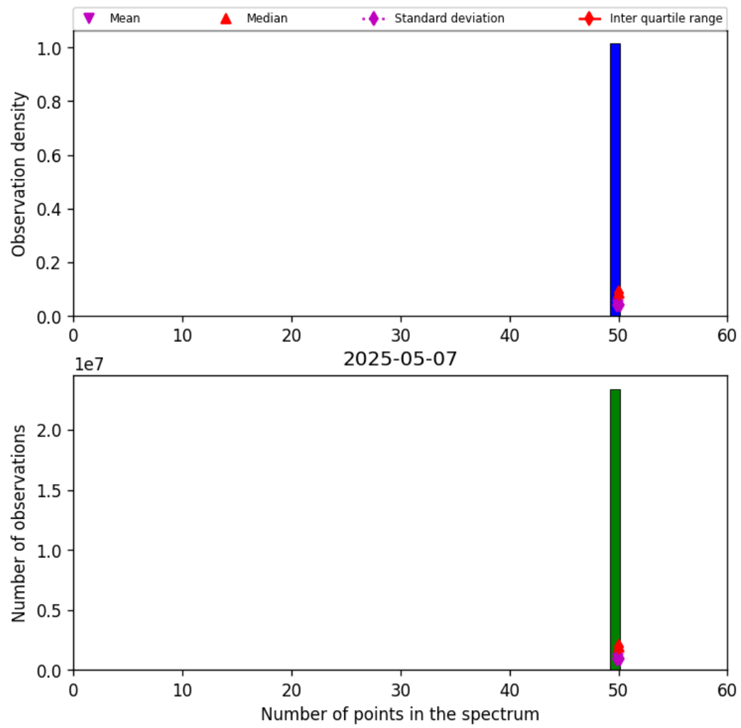
Figure 42: Histogram of “Number of points in the spectrum” for 2025-05-07 to 2025-05-08
