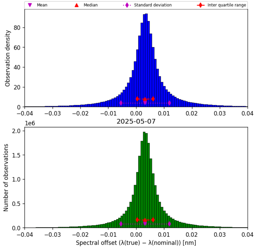
Figure 43: Histogram of “Spectral offset ( \lambda_{\text{true}} - \lambda_{\text{nominal}} )” for 2025-05-07 to 2025-05-08
