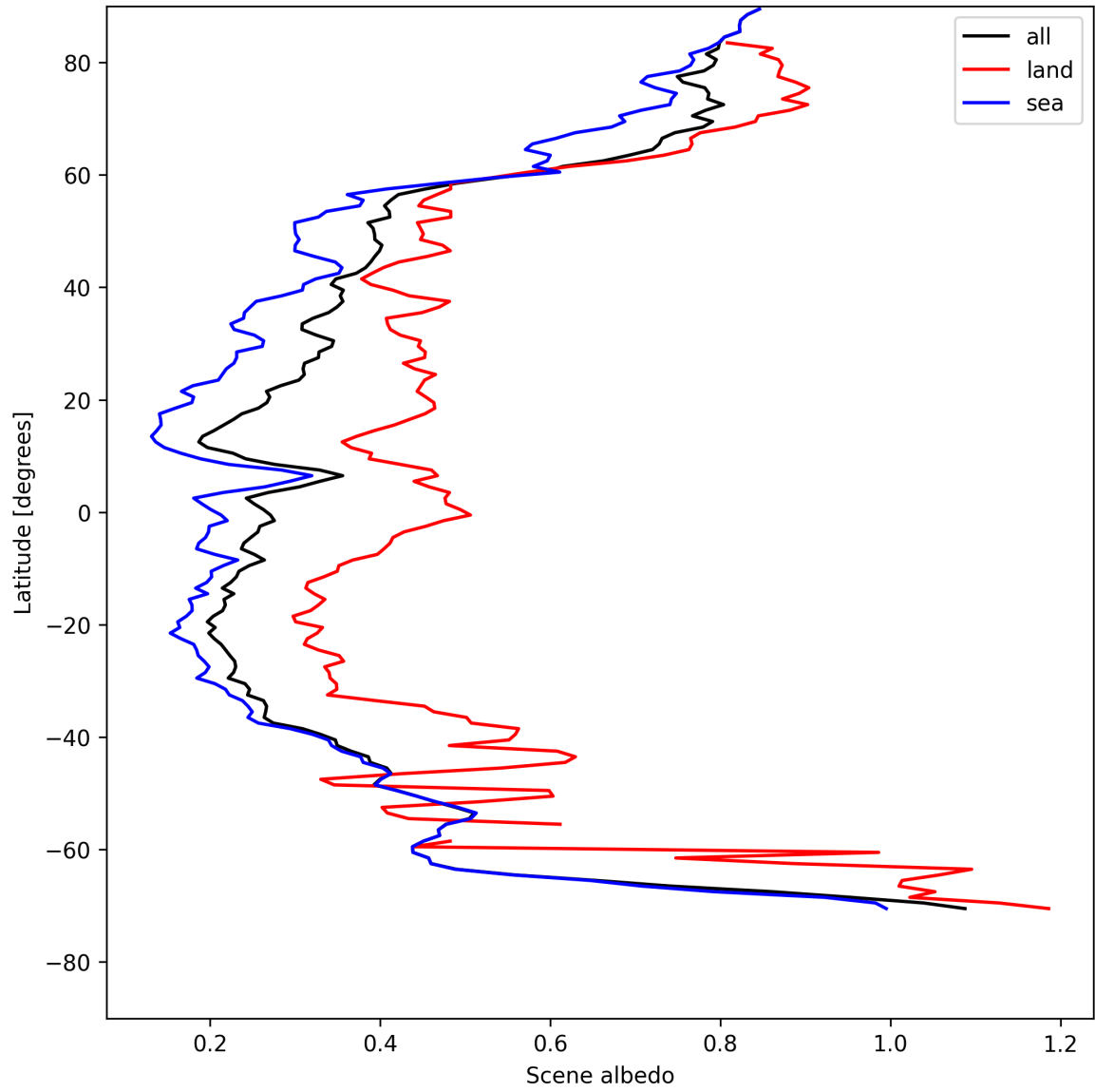
Figure 15: Zonal average of “Scene albedo” for 2025-05-07 to 2025-05-08.
