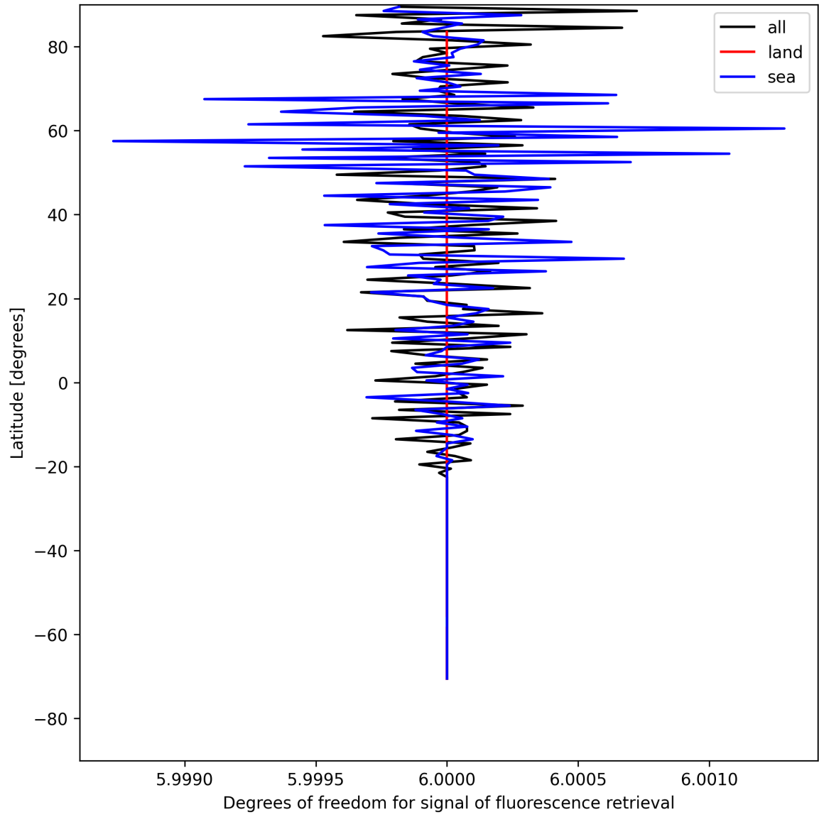
Figure 24: Zonal average of “Degrees of freedom for signal of fluorescence retrieval” for 2025-05-07 to 2025-05-08.
