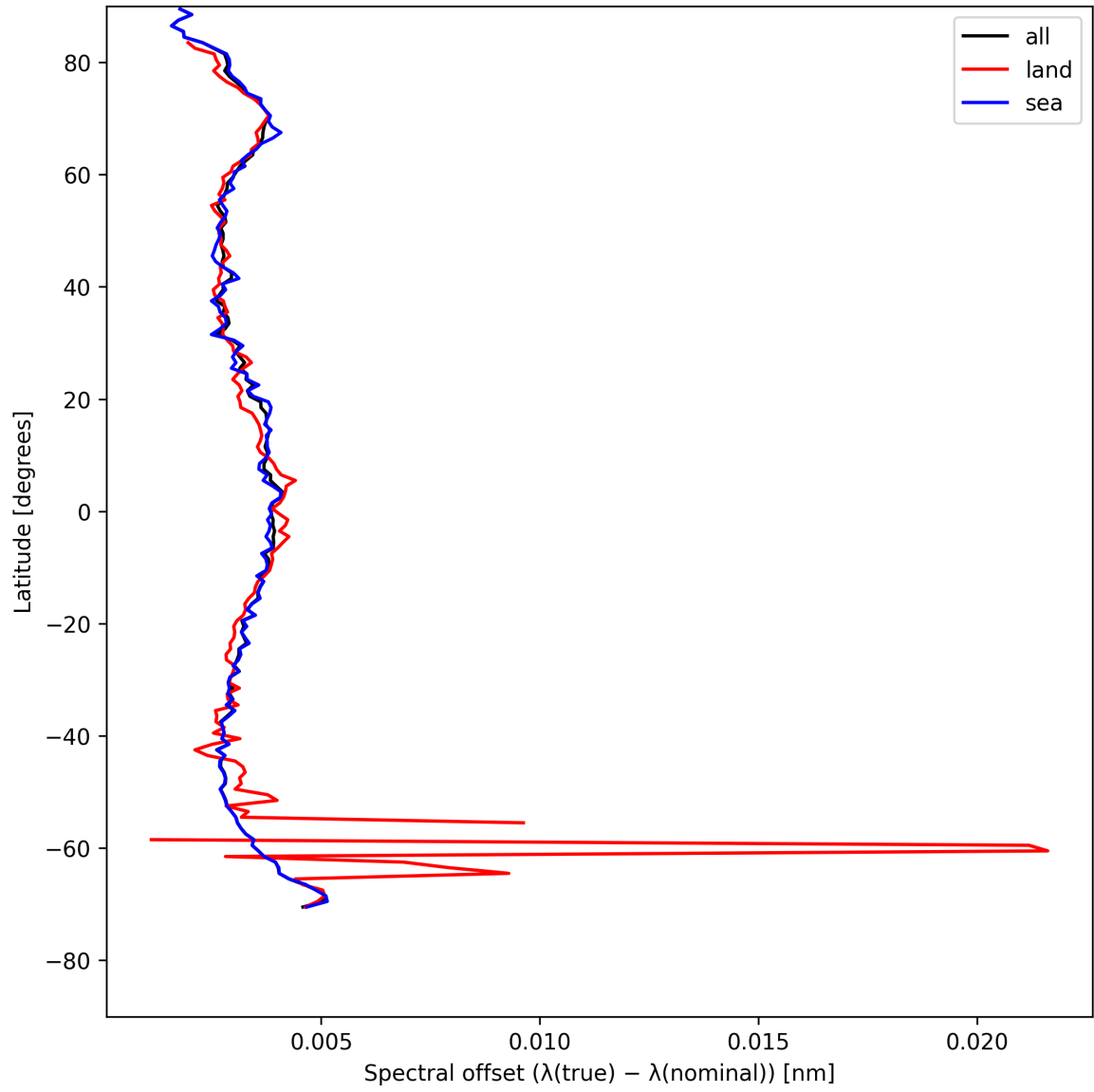
Figure 26: Zonal average of “Spectral offset ( \lambda_{\text{true}} - \lambda_{\text{nominal}} )” for 2025-05-07 to 2025-05-08.
