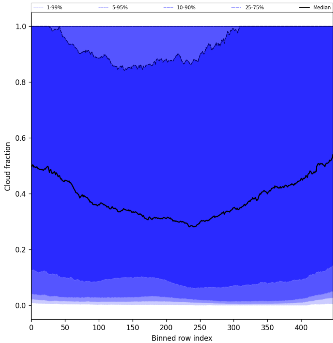
Figure 47: Along track statistics of “Cloud fraction” for 2025-05-07 to 2025-05-08
