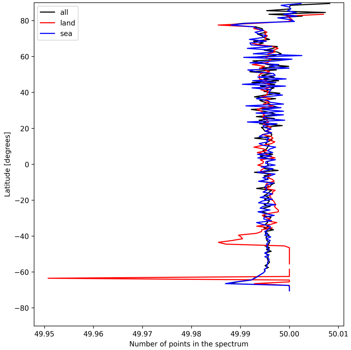
Figure 25: Zonal average of “Number of points in the spectrum” for 2025-05-07 to 2025-05-08.
