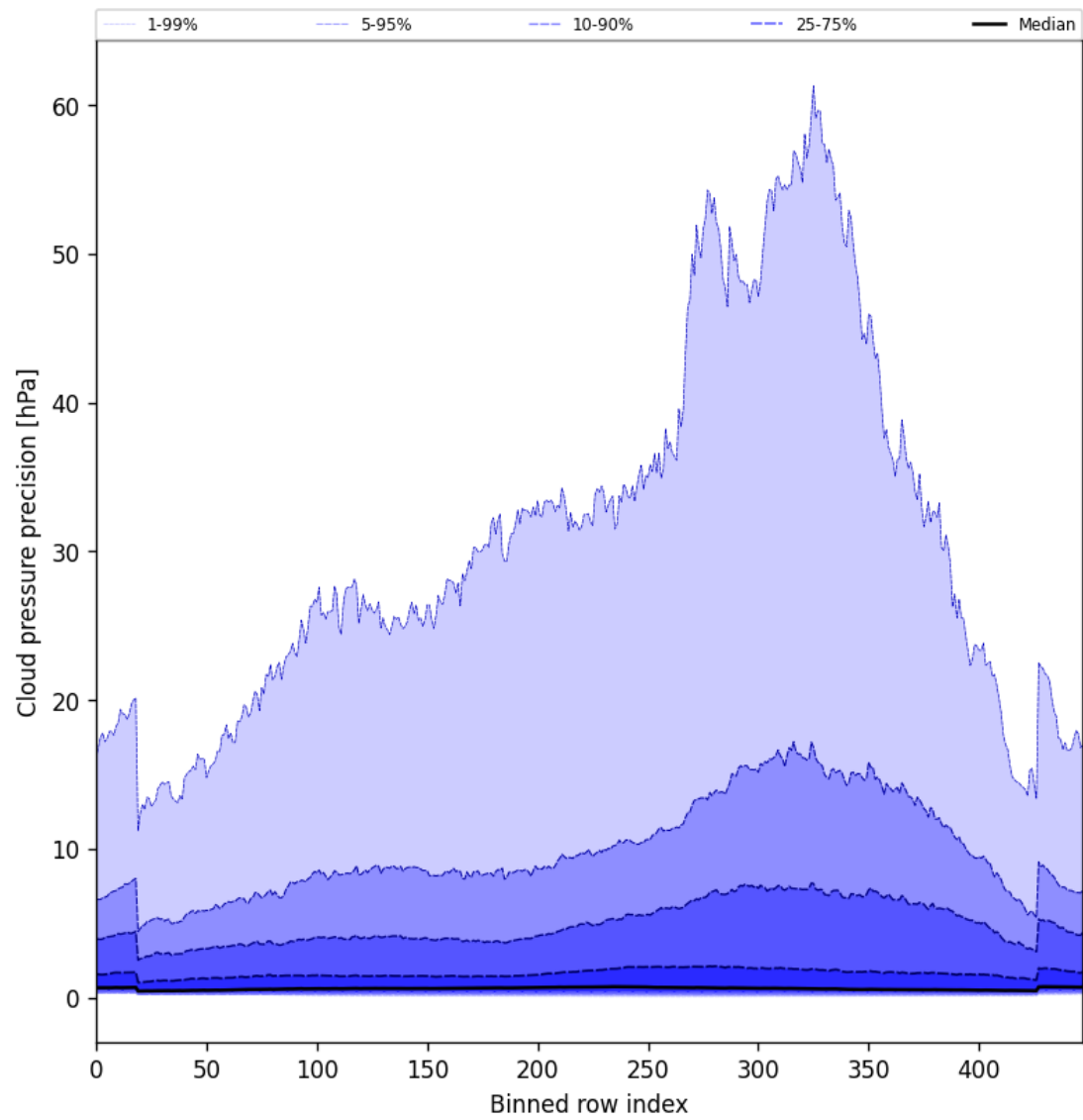
Figure 46: Along track statistics of “Cloud pressure precision” for 2025-05-07 to 2025-05-08
