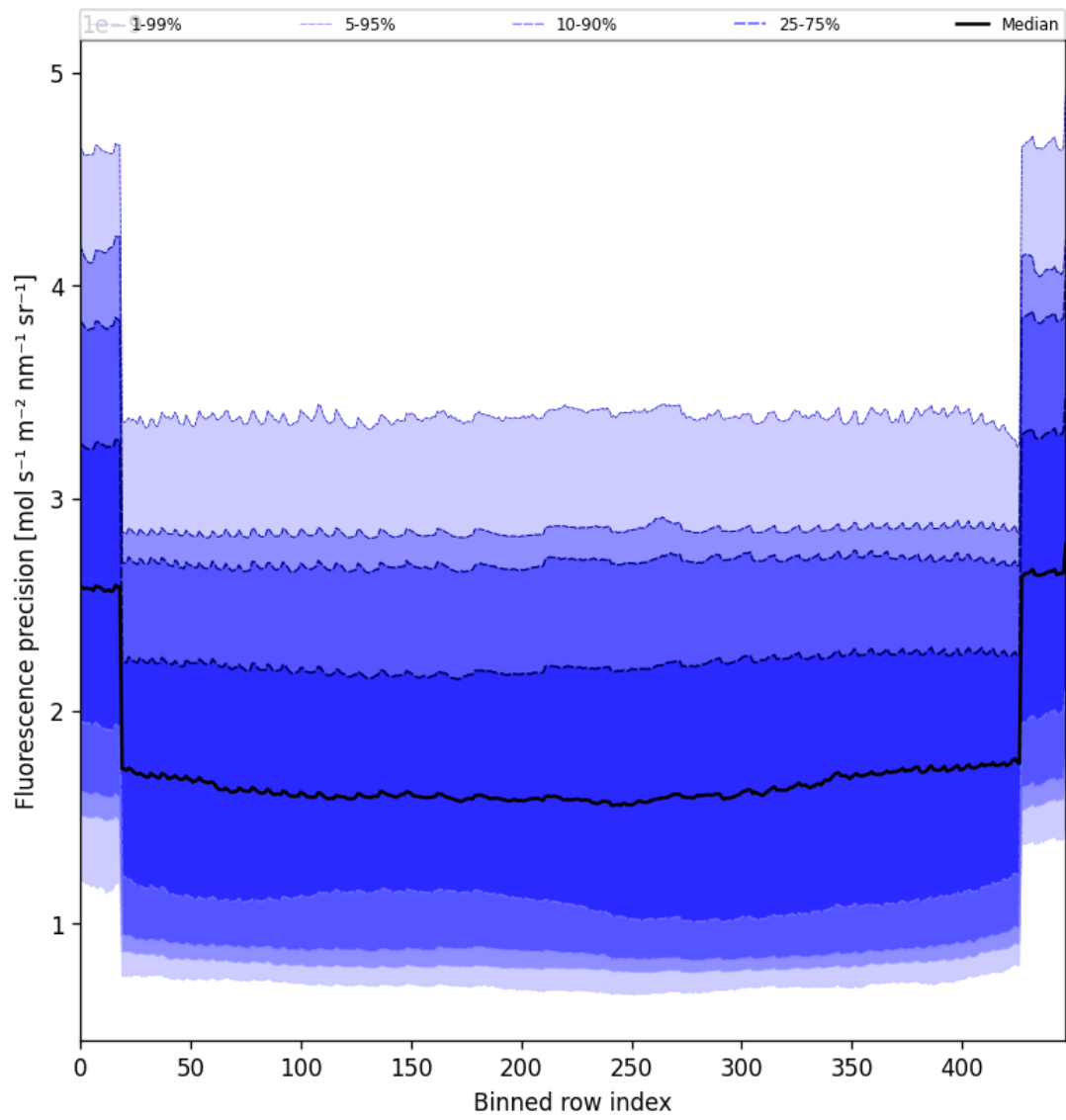
Figure 56: Along track statistics of “Fluorescence precision” for 2025-05-07 to 2025-05-08
