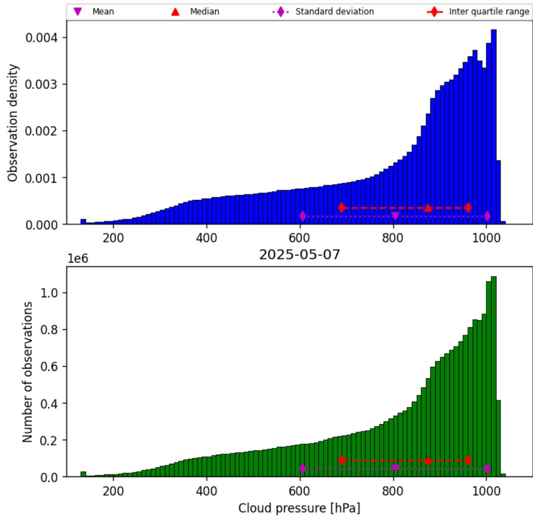
Figure 28: Histogram of “Cloud pressure” for 2025-05-07 to 2025-05-08
