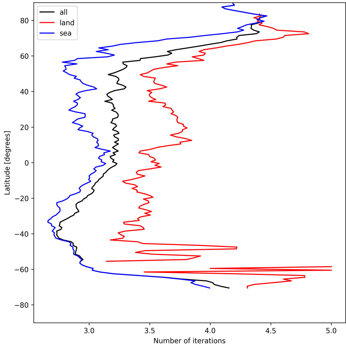
Figure 20: Zonal average of “Number of iterations” for 2025-05-07 to 2025-05-08.
