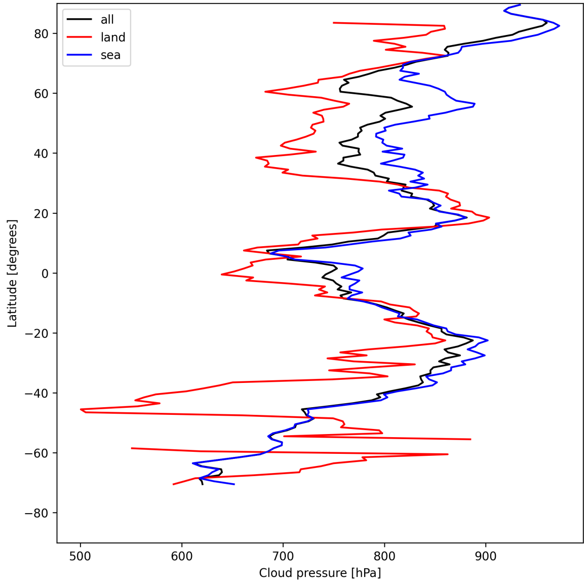
Figure 11: Zonal average of “Cloud pressure” for 2025-05-07 to 2025-05-08.
