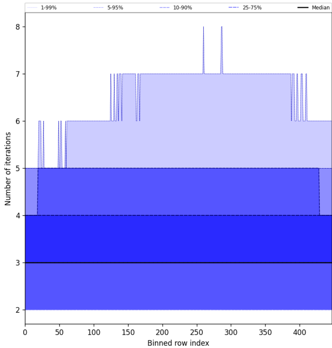
Figure 54: Along track statistics of “Number of iterations” for 2025-05-07 to 2025-05-08
