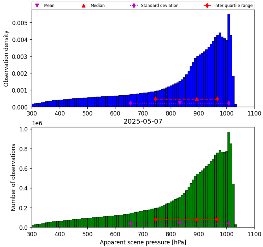
Figure 34: Histogram of “Apparent scene pressure” for 2025-05-07 to 2025-05-08
