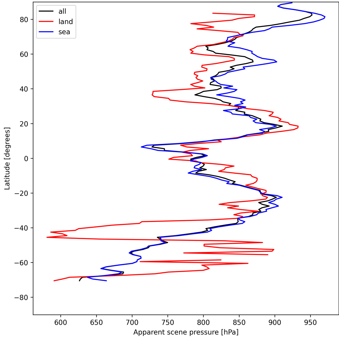
Figure 17: Zonal average of “Apparent scene pressure” for 2025-05-07 to 2025-05-08.
