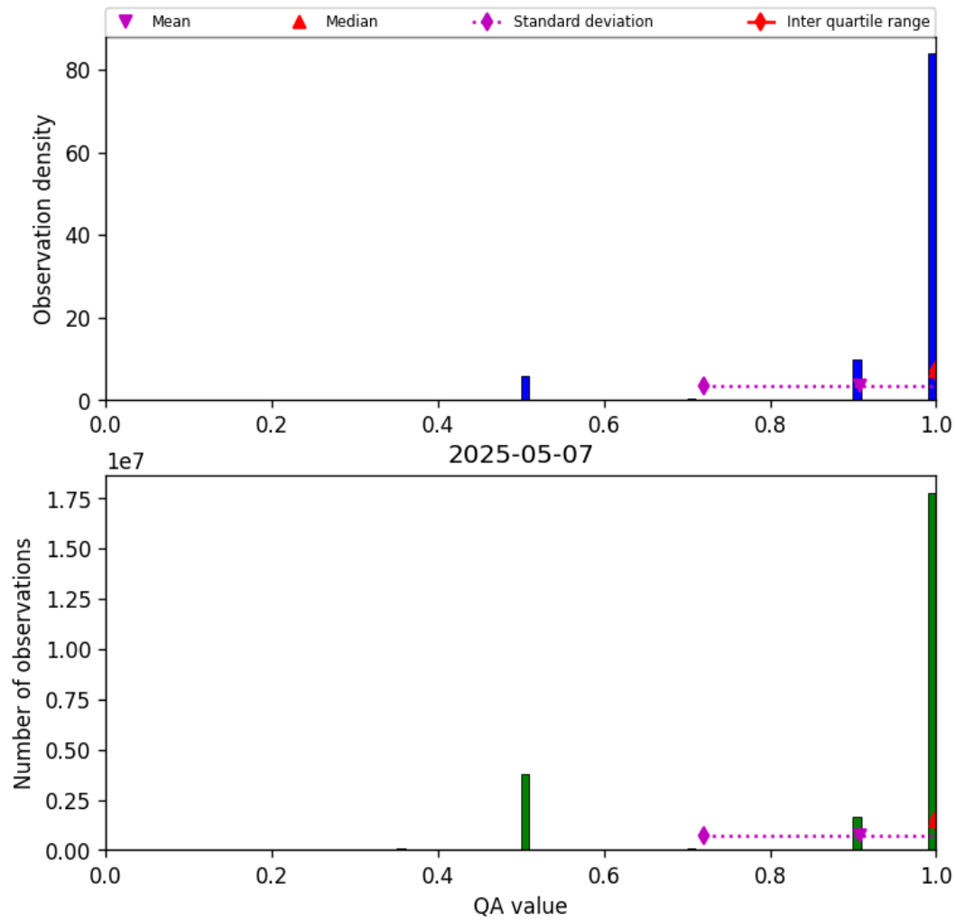
Figure 27: Histogram of “QA value” for 2025-05-07 to 2025-05-08
