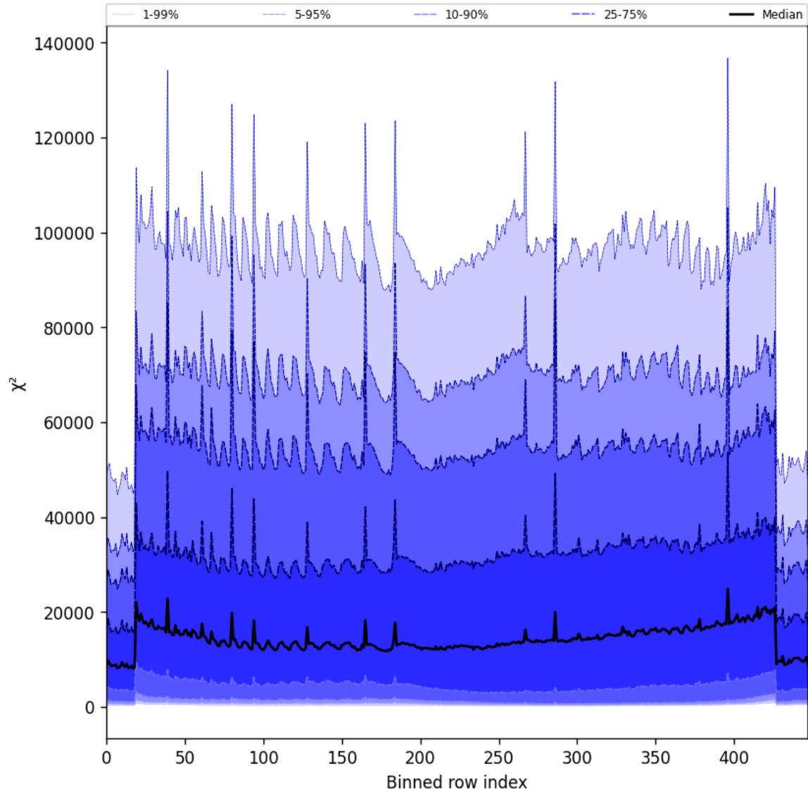
Figure 53: Along track statistics of “ \chi^2 ” for 2025-05-07 to 2025-05-08
