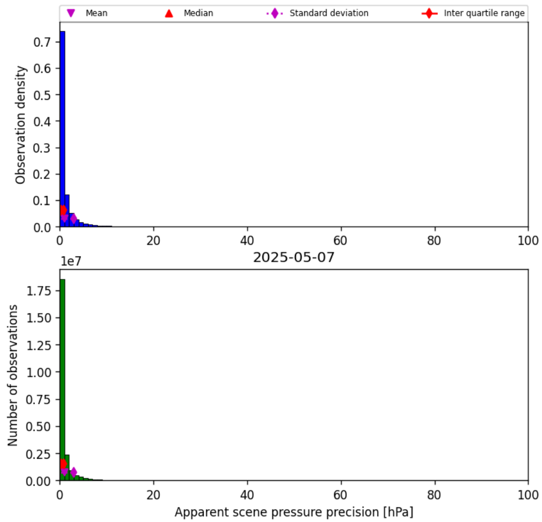
Figure 35: Histogram of “Apparent scene pressure precision” for 2025-05-07 to 2025-05-08
