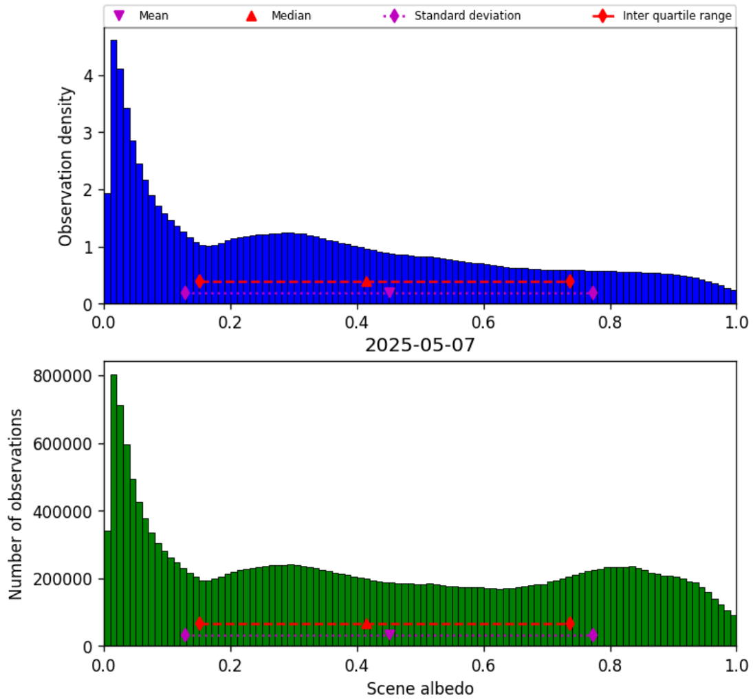
Figure 32: Histogram of “Scene albedo” for 2025-05-07 to 2025-05-08
