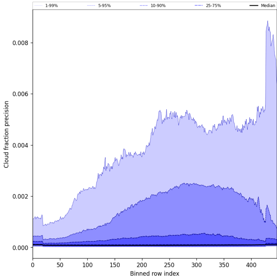
Figure 48: Along track statistics of “Cloud fraction precision” for 2025-05-07 to 2025-05-08
