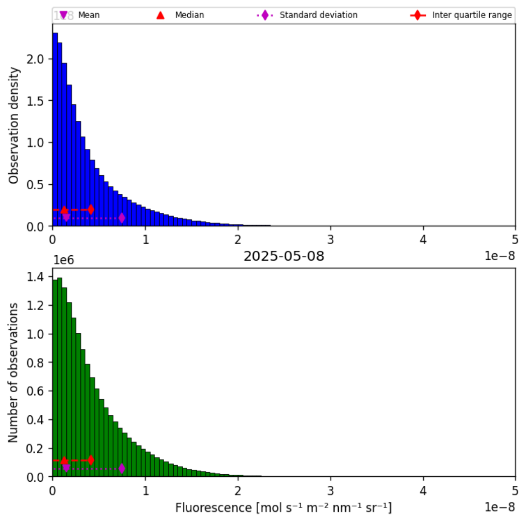
Figure 38: Histogram of “Fluorescence” for 2025-05-08 to 2025-05-08
