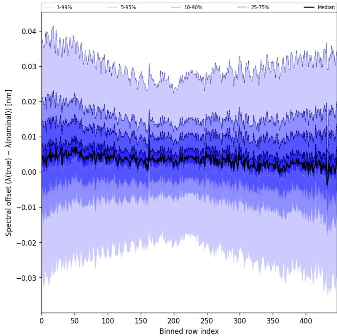
Figure 60: Along track statistics of “Spectral offset ( \lambda_{\text{true}} - \lambda_{\text{nominal}} )” for 2025-05-08 to 2025-05-08
