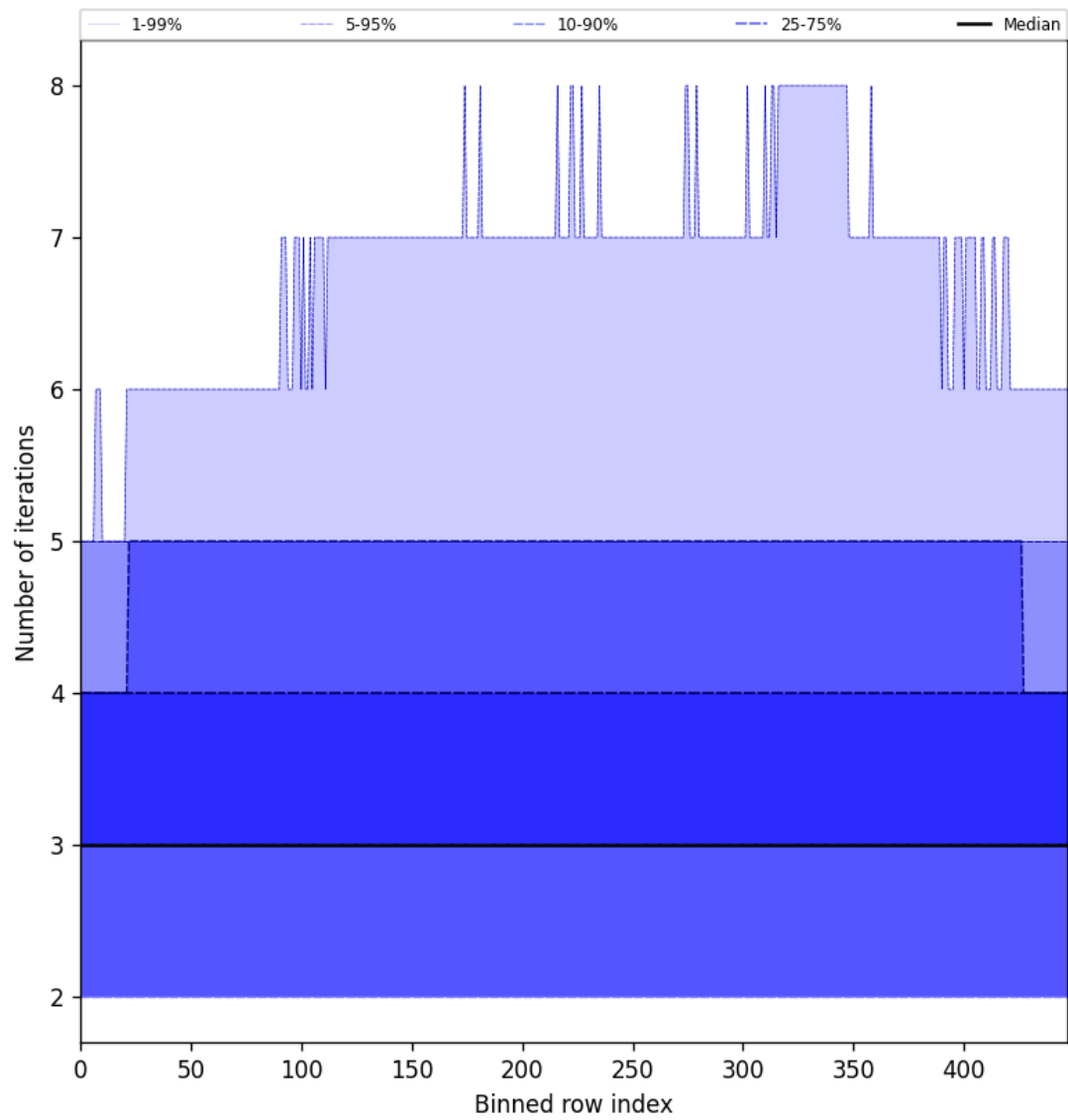
Figure 54: Along track statistics of “Number of iterations” for 2025-05-08 to 2025-05-08
