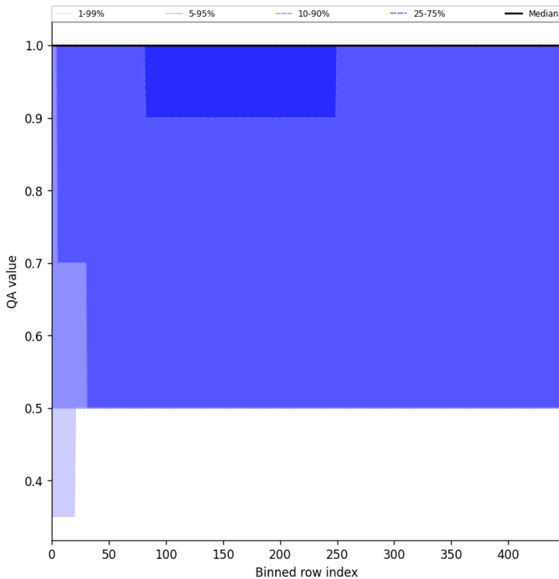
Figure 44: Along track statistics of “QA value” for 2025-05-08 to 2025-05-08
