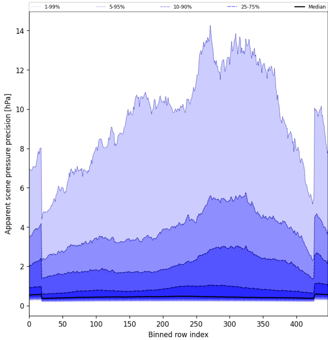
Figure 52: Along track statistics of “Apparent scene pressure precision” for 2025-05-08 to 2025-05-08
