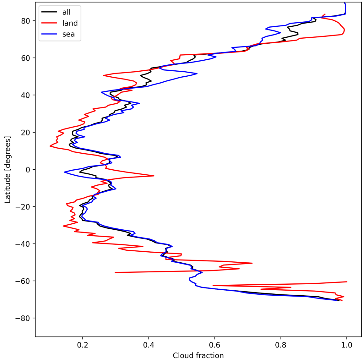
Figure 13: Zonal average of “Cloud fraction” for 2025-05-08 to 2025-05-08.
