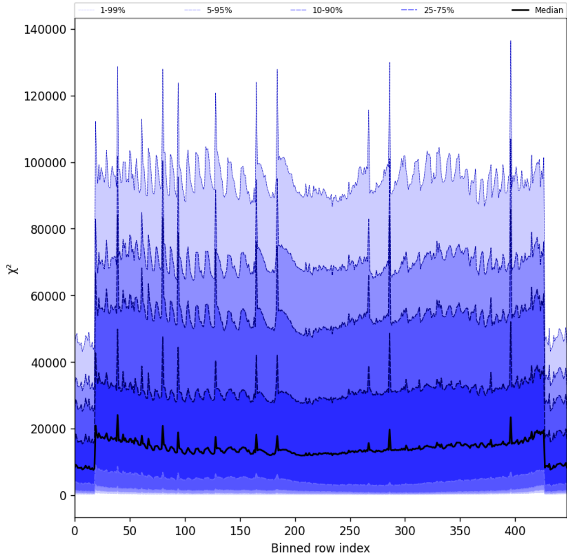
Figure 53: Along track statistics of “ \chi^2 ” for 2025-05-08 to 2025-05-08
