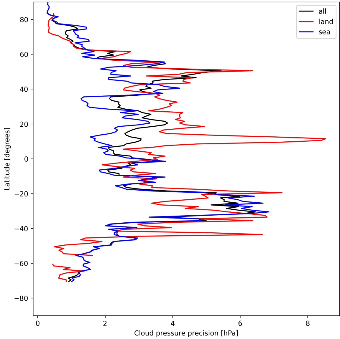
Figure 12: Zonal average of “Cloud pressure precision” for 2025-05-08 to 2025-05-08.
