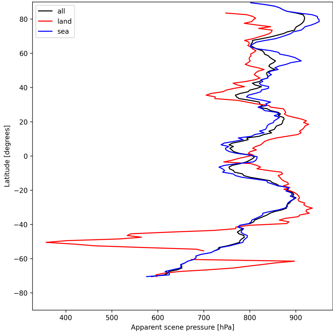
Figure 17: Zonal average of “Apparent scene pressure” for 2025-05-08 to 2025-05-08.
