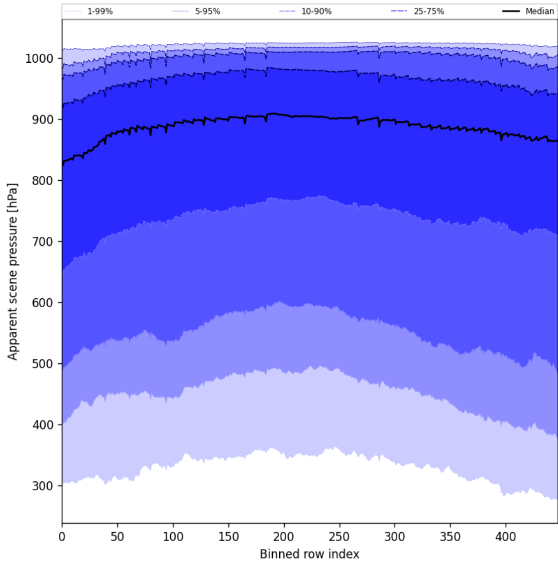
Figure 51: Along track statistics of “Apparent scene pressure” for 2025-05-08 to 2025-05-08
