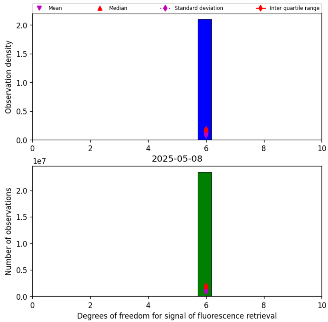
Figure 41: Histogram of “Degrees of freedom for signal of fluorescence retrieval” for 2025-05-08 to 2025-05-08
