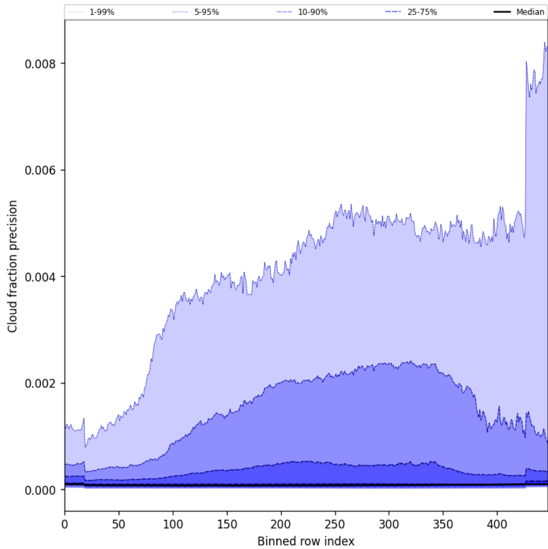
Figure 48: Along track statistics of “Cloud fraction precision” for 2025-05-08 to 2025-05-08
