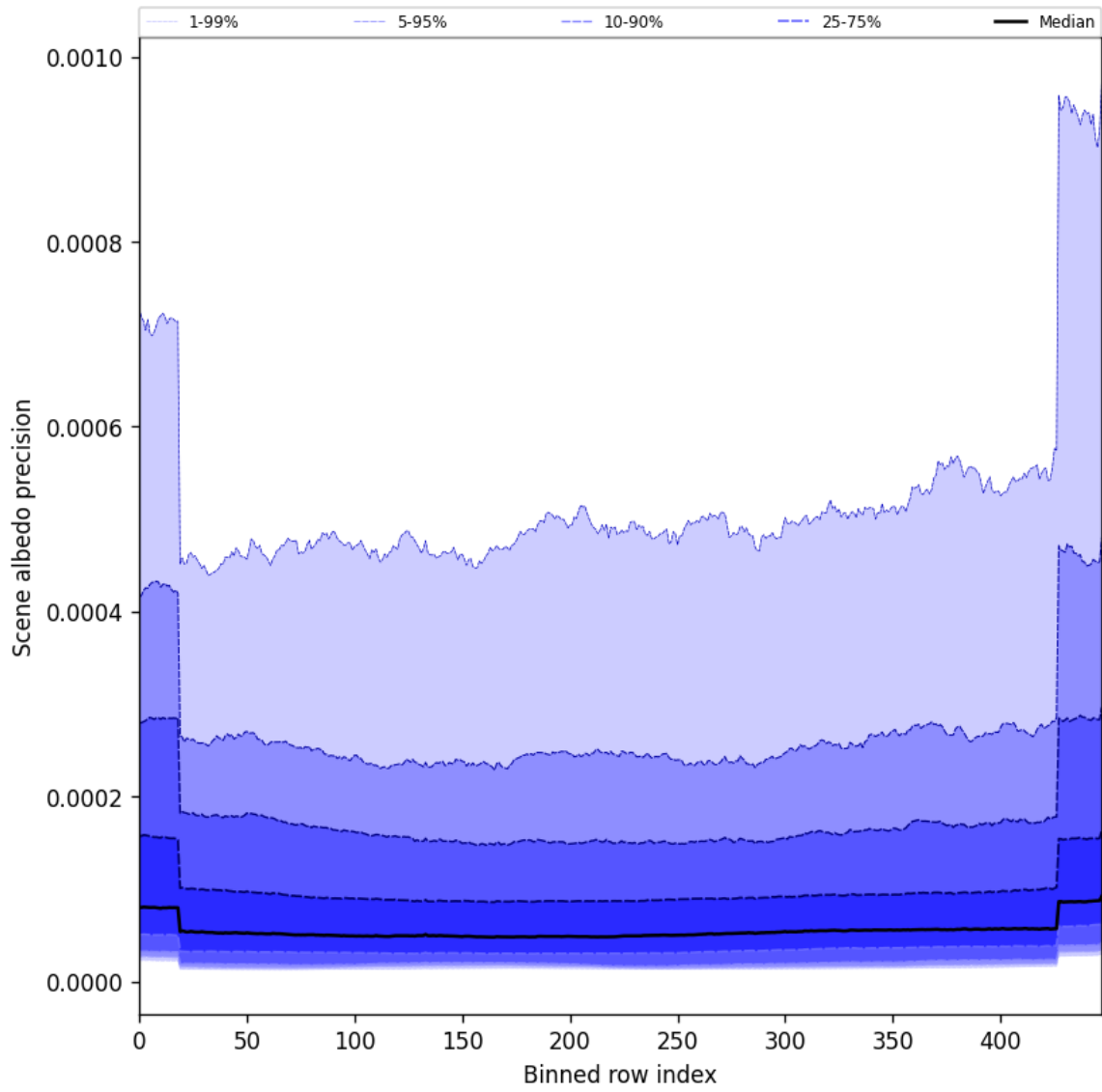
Figure 50: Along track statistics of “Scene albedo precision” for 2025-05-08 to 2025-05-08
