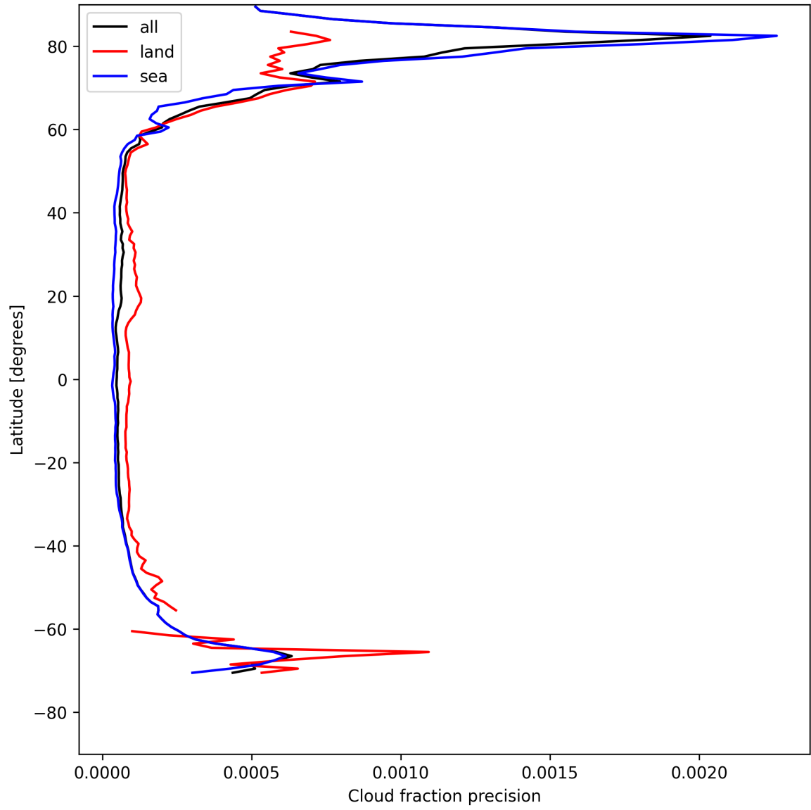
Figure 14: Zonal average of “Cloud fraction precision” for 2025-05-08 to 2025-05-08.
