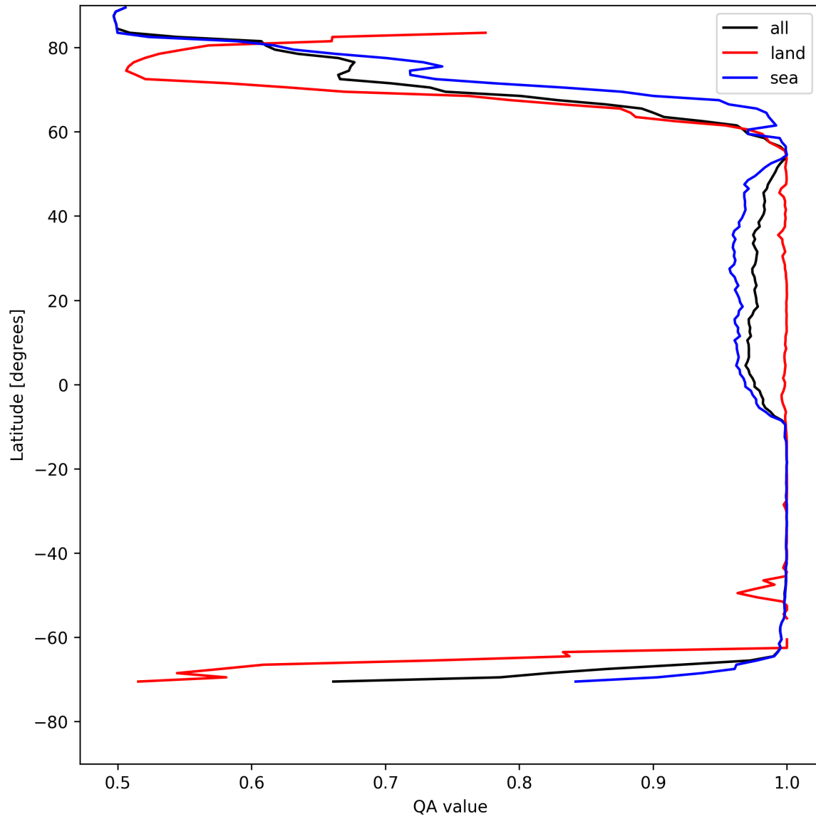
Figure 10: Zonal average of “QA value” for 2025-05-08 to 2025-05-08.
