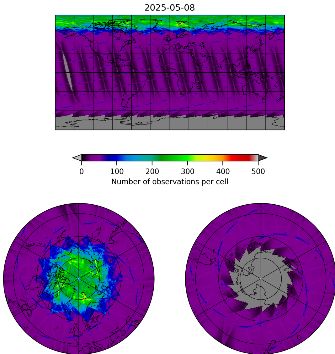
Figure 9: Map of the number of observations for 2025-05-08 to 2025-05-08
