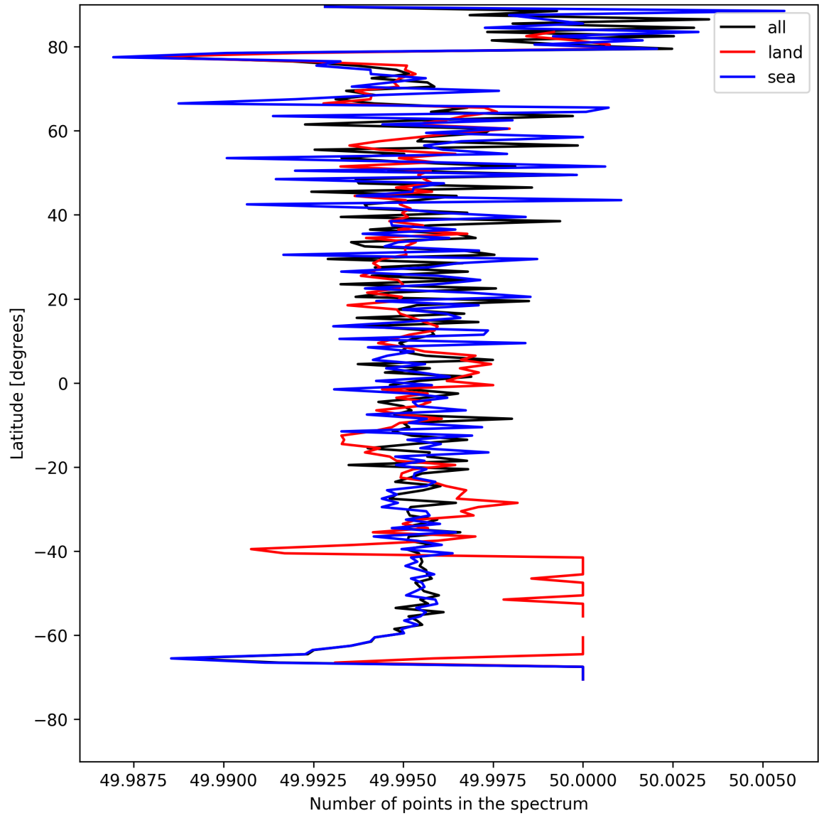
Figure 25: Zonal average of “Number of points in the spectrum” for 2025-05-08 to 2025-05-08.
