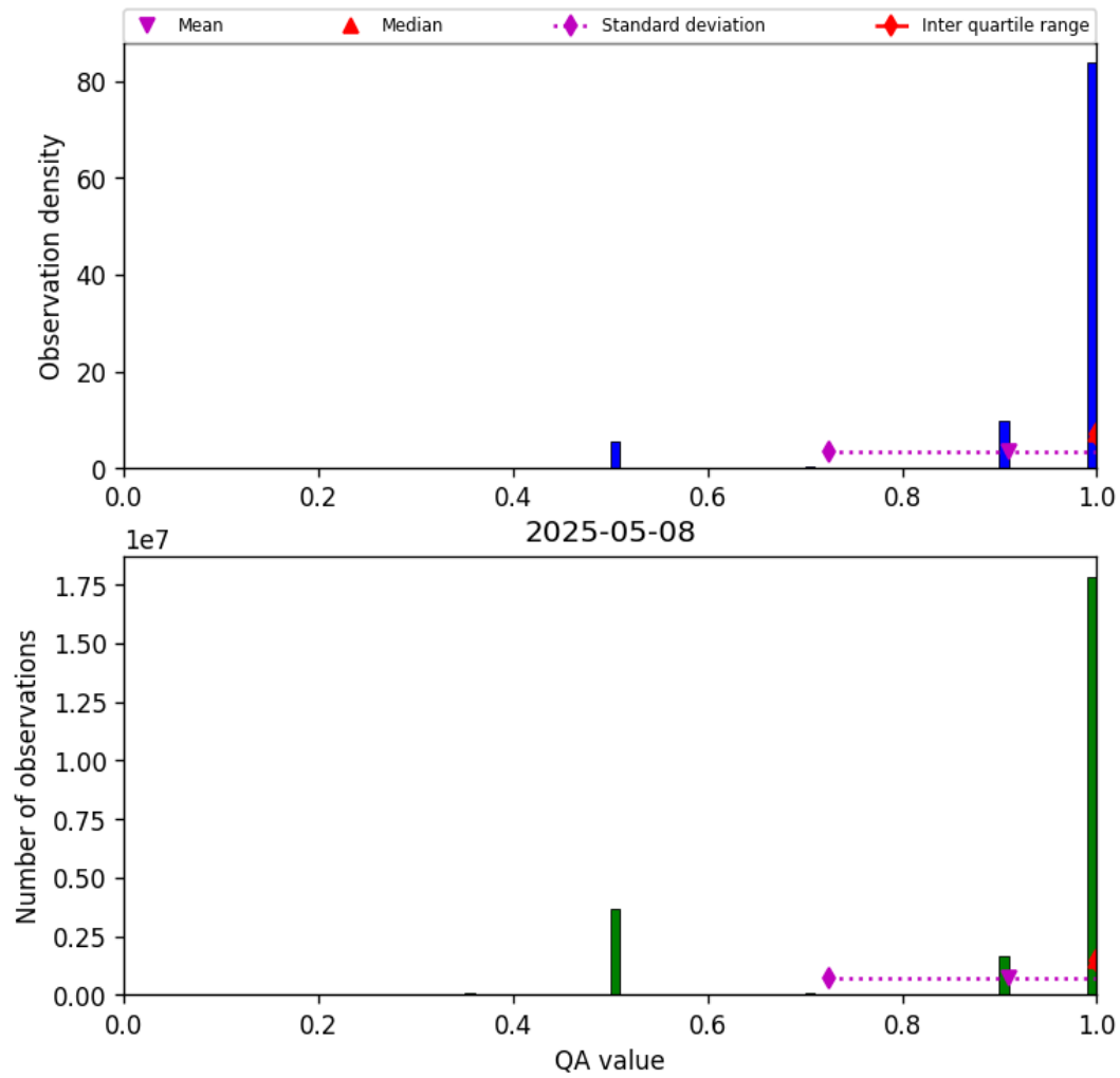
Figure 27: Histogram of “QA value” for 2025-05-08 to 2025-05-08
