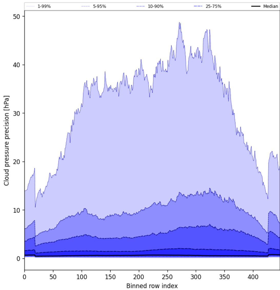
Figure 46: Along track statistics of “Cloud pressure precision” for 2025-05-08 to 2025-05-08
