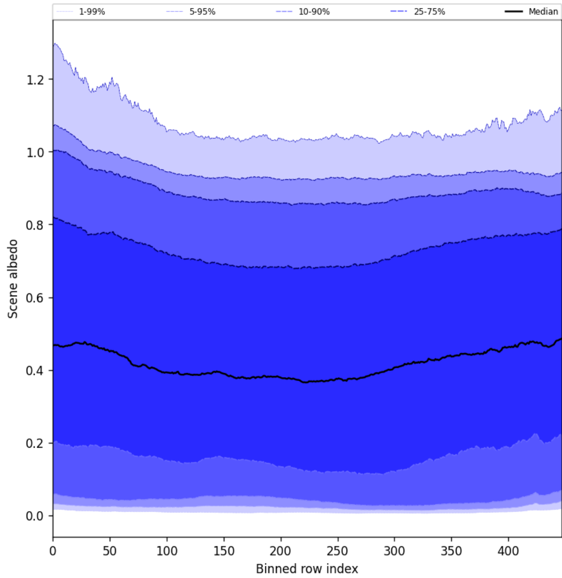
Figure 49: Along track statistics of “Scene albedo” for 2025-05-08 to 2025-05-08
