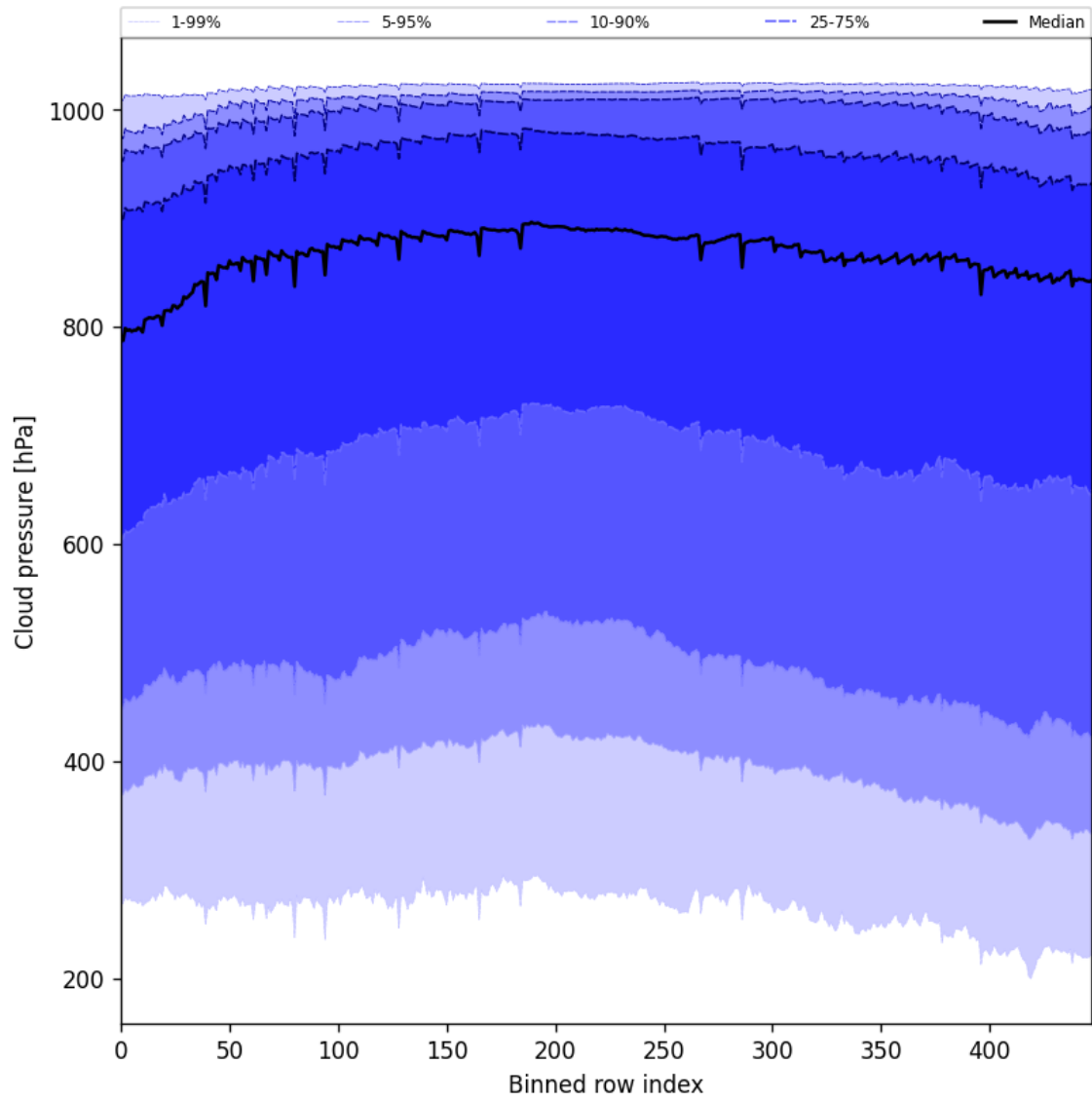
Figure 45: Along track statistics of “Cloud pressure” for 2025-05-08 to 2025-05-08
