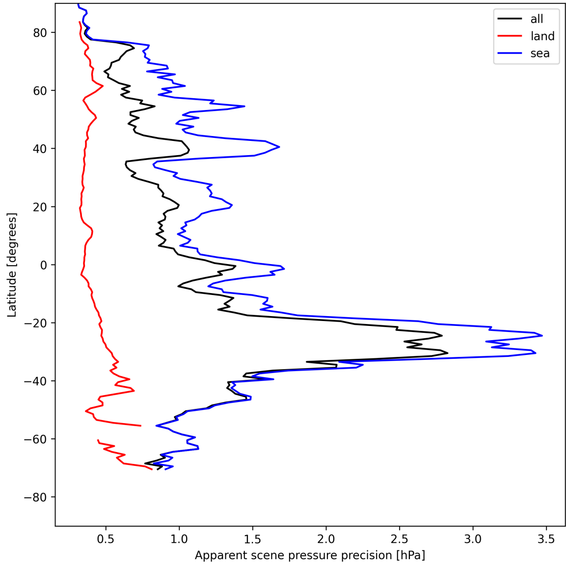
Figure 18: Zonal average of “Apparent scene pressure precision” for 2025-05-08 to 2025-05-08.
