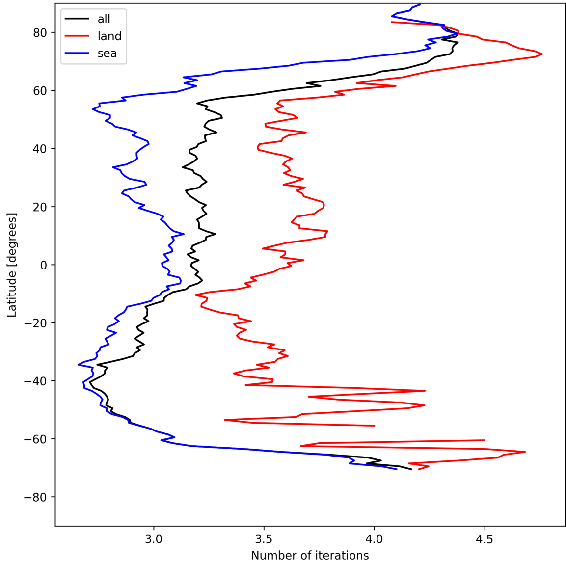
Figure 20: Zonal average of “Number of iterations” for 2025-05-08 to 2025-05-08.
