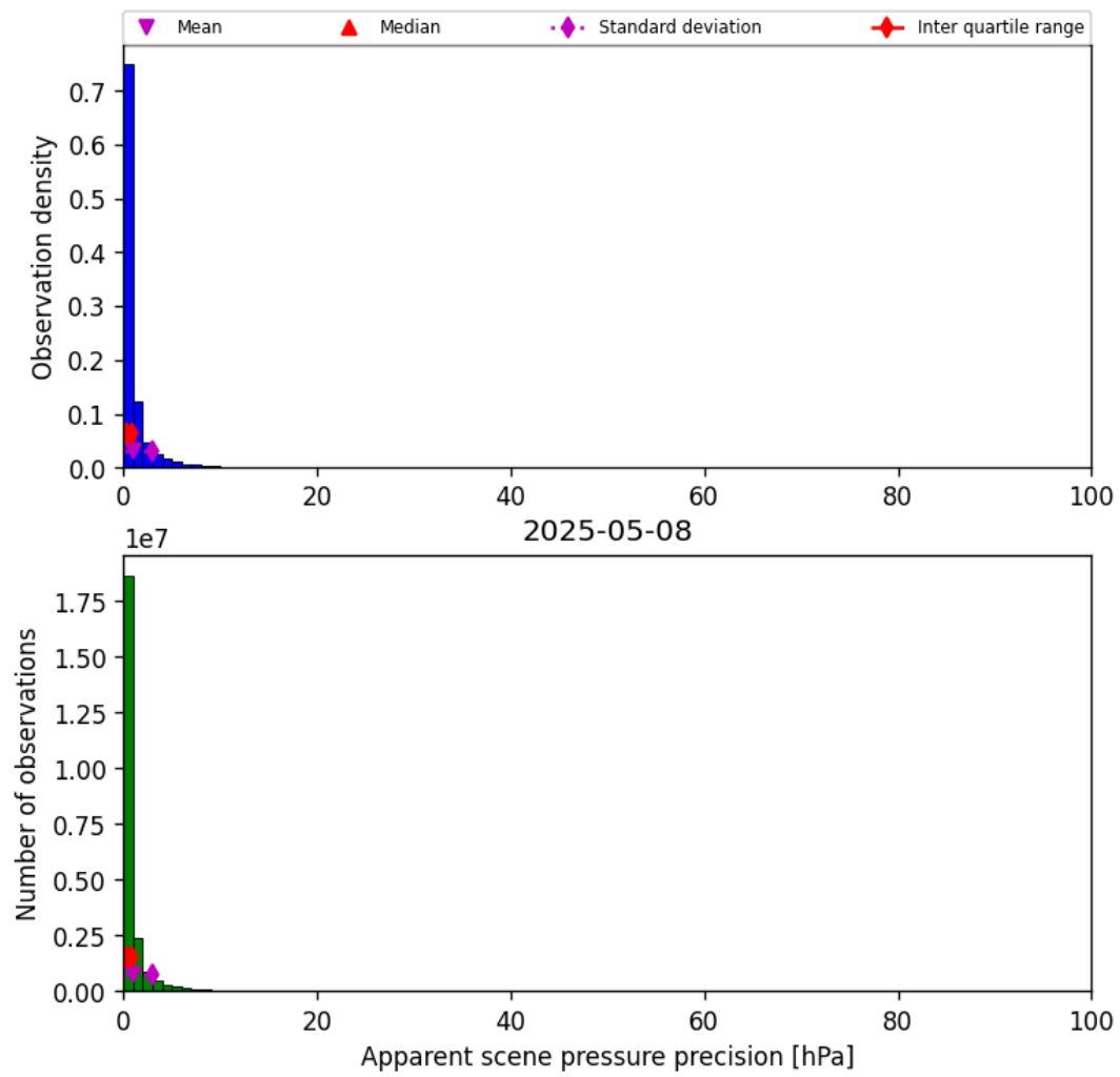
Figure 35: Histogram of “Apparent scene pressure precision” for 2025-05-08 to 2025-05-08
