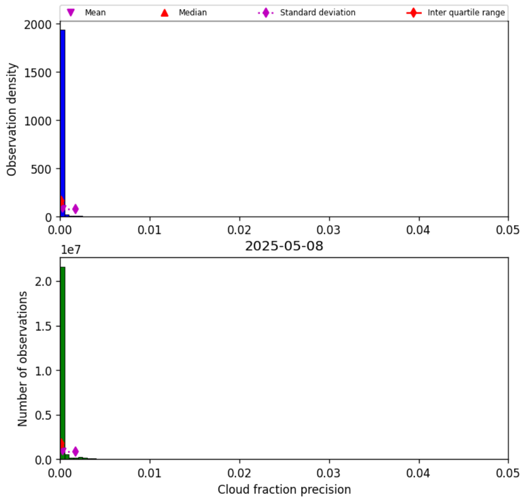
Figure 31: Histogram of “Cloud fraction precision” for 2025-05-08 to 2025-05-08
