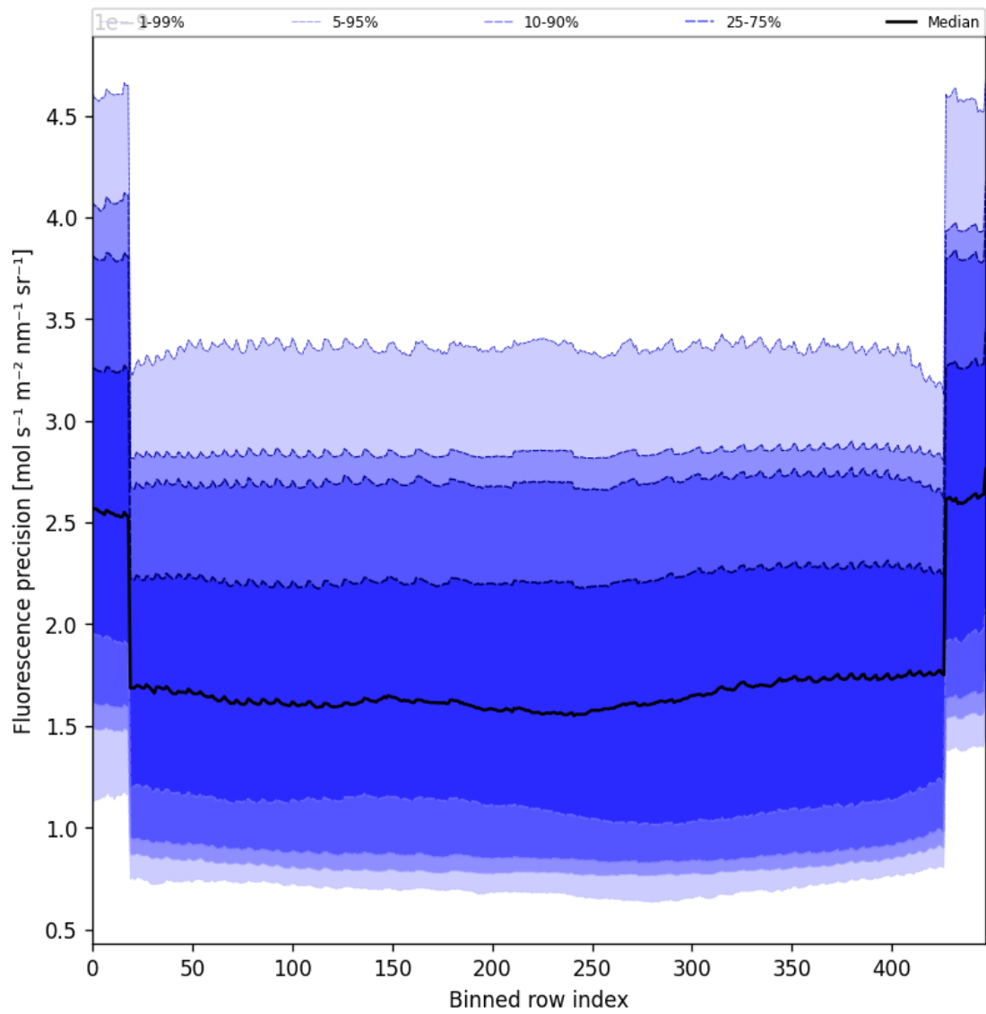
Figure 56: Along track statistics of “Fluorescence precision” for 2025-05-08 to 2025-05-08
