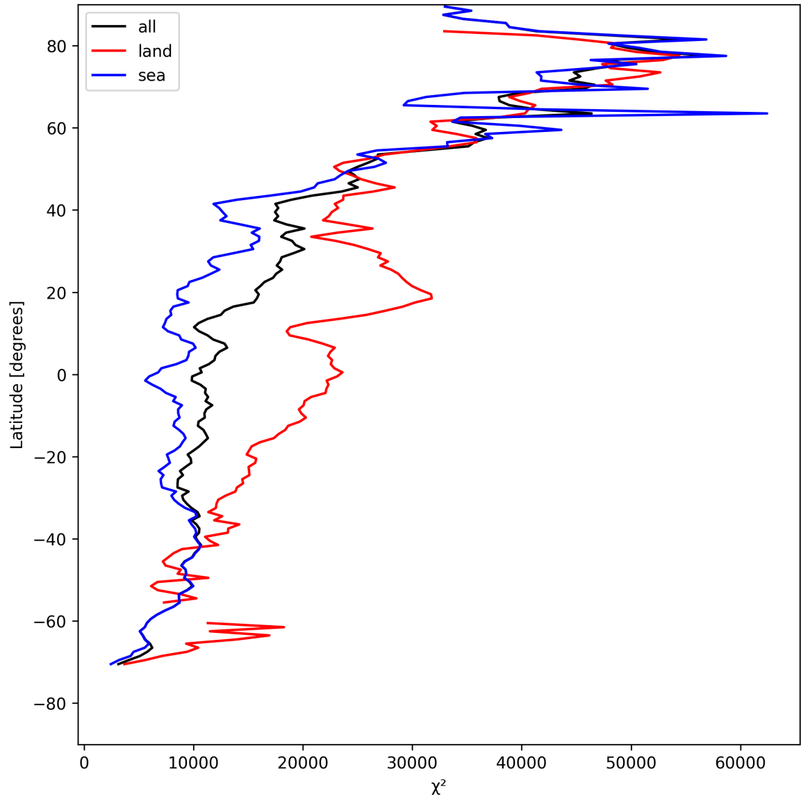
Figure 19: Zonal average of “ \chi^2 ” for 2025-05-08 to 2025-05-08.
