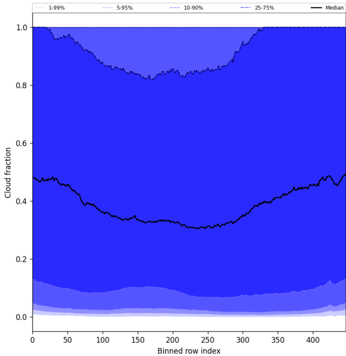
Figure 47: Along track statistics of “Cloud fraction” for 2025-05-08 to 2025-05-08
