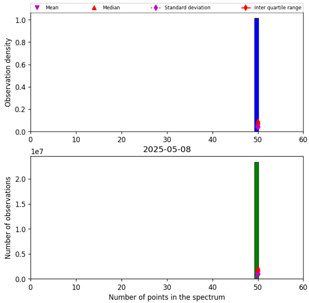
Figure 42: Histogram of "Number of points in the spectrum" for 2025-05-08 to 2025-05-08
