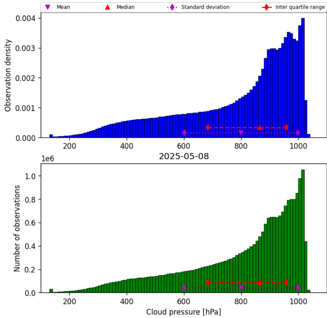
Figure 28: Histogram of “Cloud pressure” for 2025-05-08 to 2025-05-08
