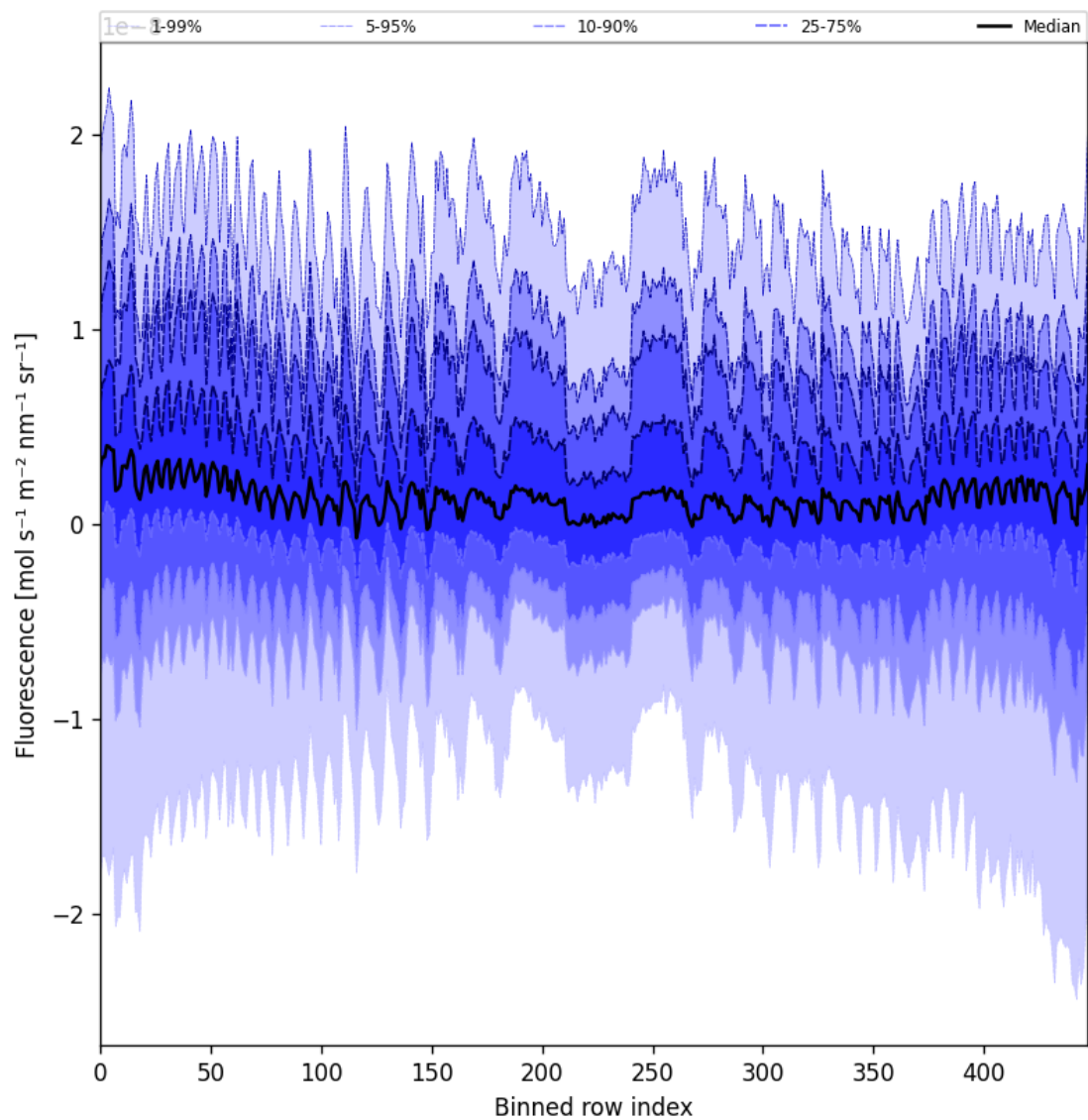
Figure 55: Along track statistics of “Fluorescence” for 2025-05-08 to 2025-05-08
