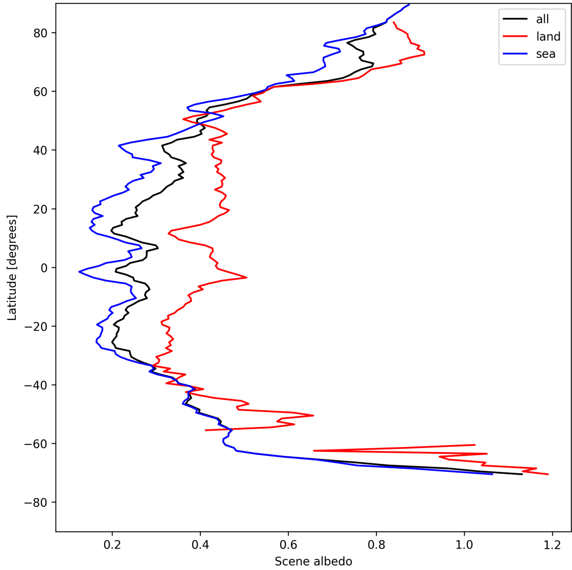
Figure 15: Zonal average of “Scene albedo” for 2025-05-08 to 2025-05-08.
