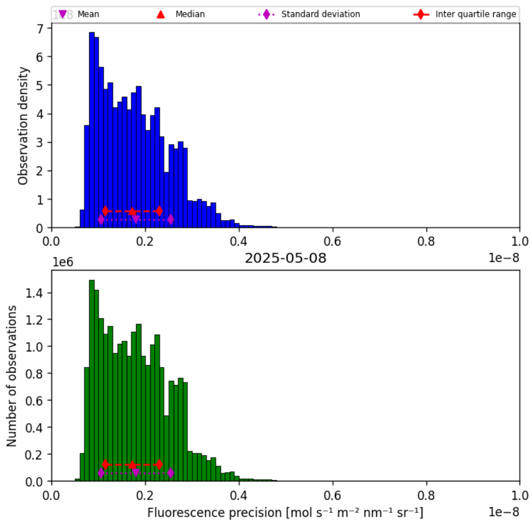
Figure 39: Histogram of “Fluorescence precision” for 2025-05-08 to 2025-05-08
