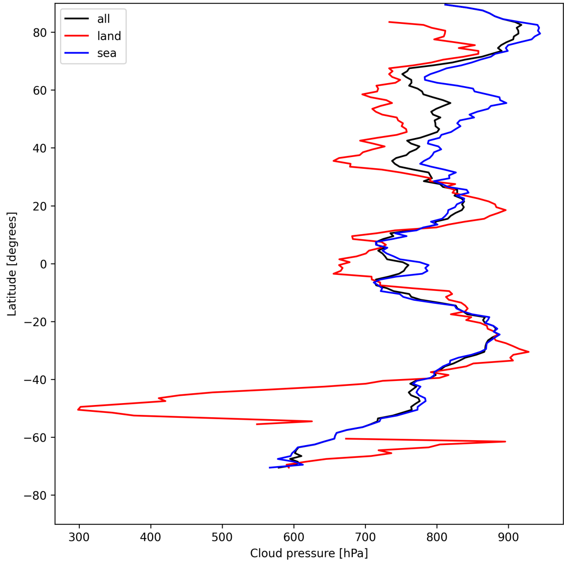
Figure 11: Zonal average of “Cloud pressure” for 2025-05-08 to 2025-05-08.
