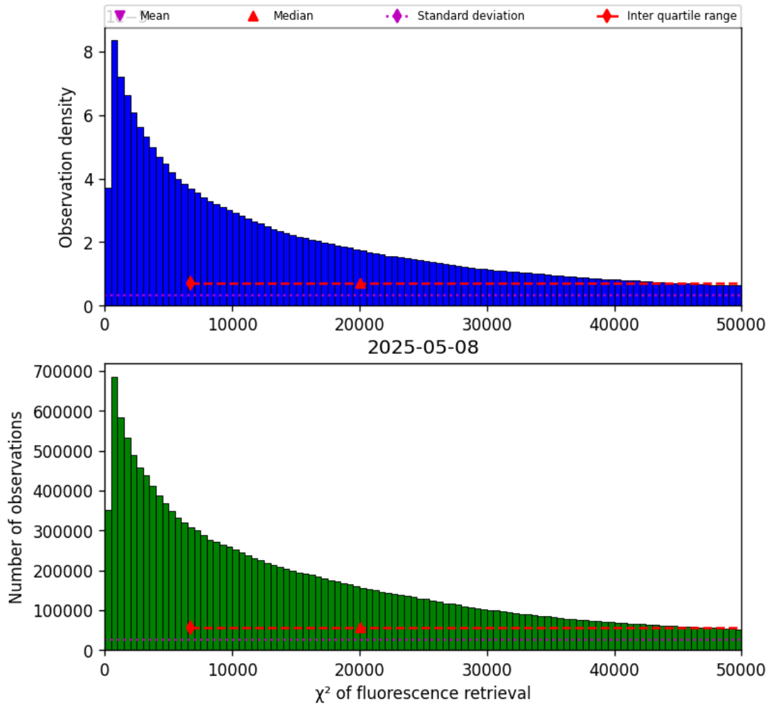
Figure 40: Histogram of “ \chi^2 of fluorescence retrieval” for 2025-05-08 to 2025-05-08
