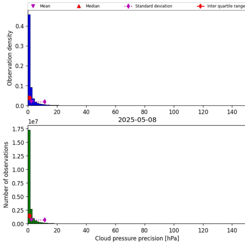
Figure 29: Histogram of “Cloud pressure precision” for 2025-05-08 to 2025-05-08
