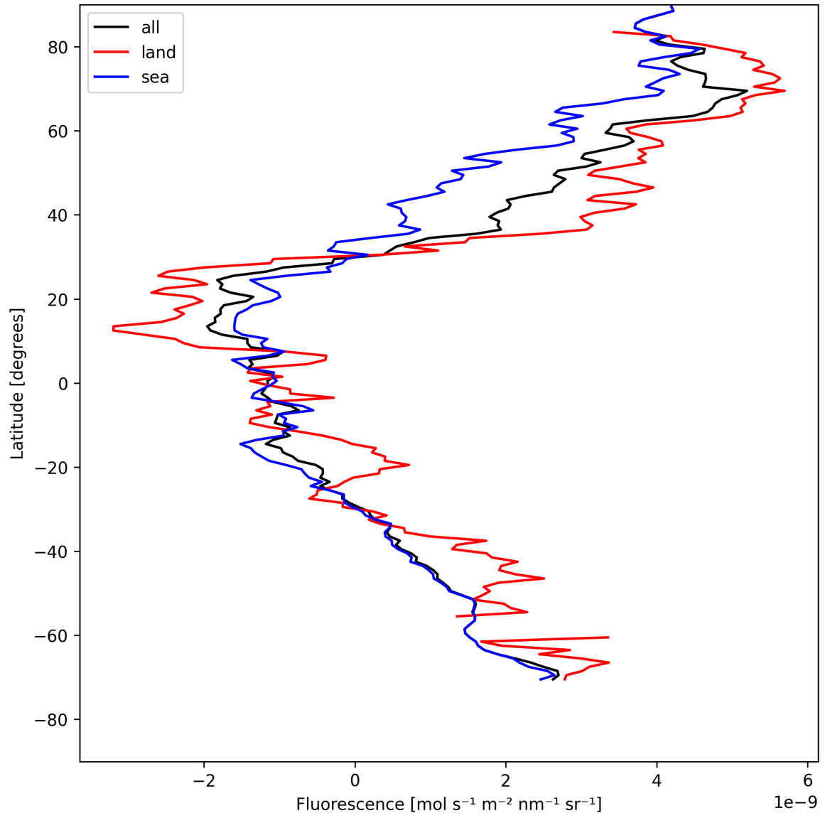
Figure 21: Zonal average of “Fluorescence” for 2025-05-08 to 2025-05-08.
