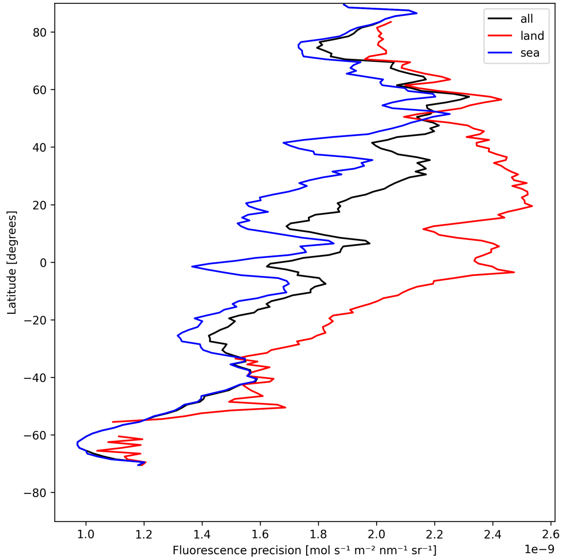
Figure 22: Zonal average of “Fluorescence precision” for 2025-05-08 to 2025-05-08.
