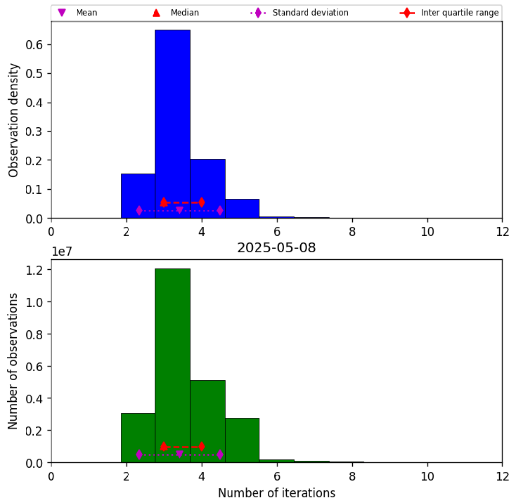
Figure 37: Histogram of “Number of iterations” for 2025-05-08 to 2025-05-08
