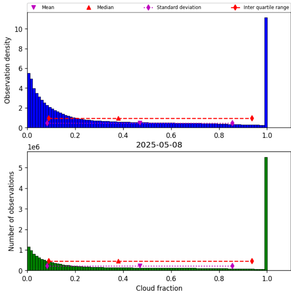
Figure 30: Histogram of “Cloud fraction” for 2025-05-08 to 2025-05-08
