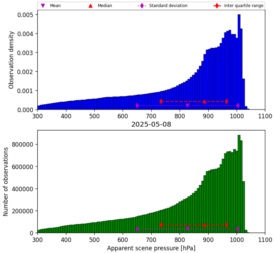
Figure 34: Histogram of “Apparent scene pressure” for 2025-05-08 to 2025-05-08
