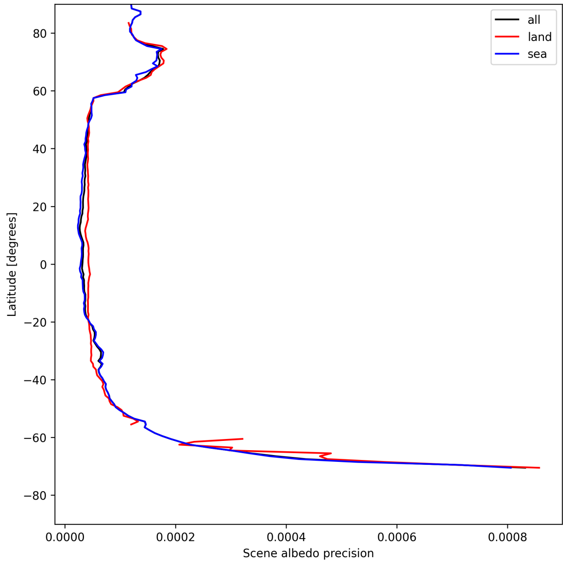
Figure 16: Zonal average of “Scene albedo precision” for 2025-05-08 to 2025-05-08.
