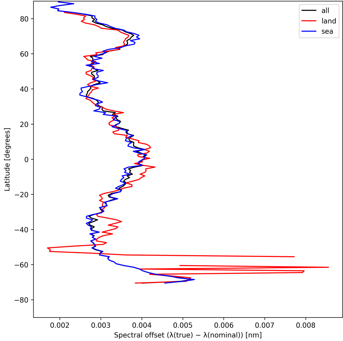
Figure 26: Zonal average of “Spectral offset ( \lambda_{\text{true}} - \lambda_{\text{nominal}} )” for 2025-05-08 to 2025-05-08.
