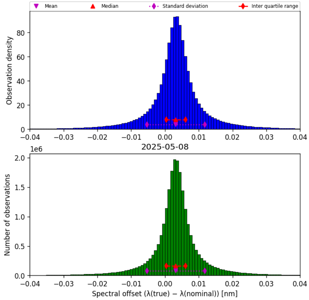
Figure 43: Histogram of “Spectral offset ( \lambda_{\text{true}} - \lambda_{\text{nominal}} )” for 2025-05-08 to 2025-05-08
