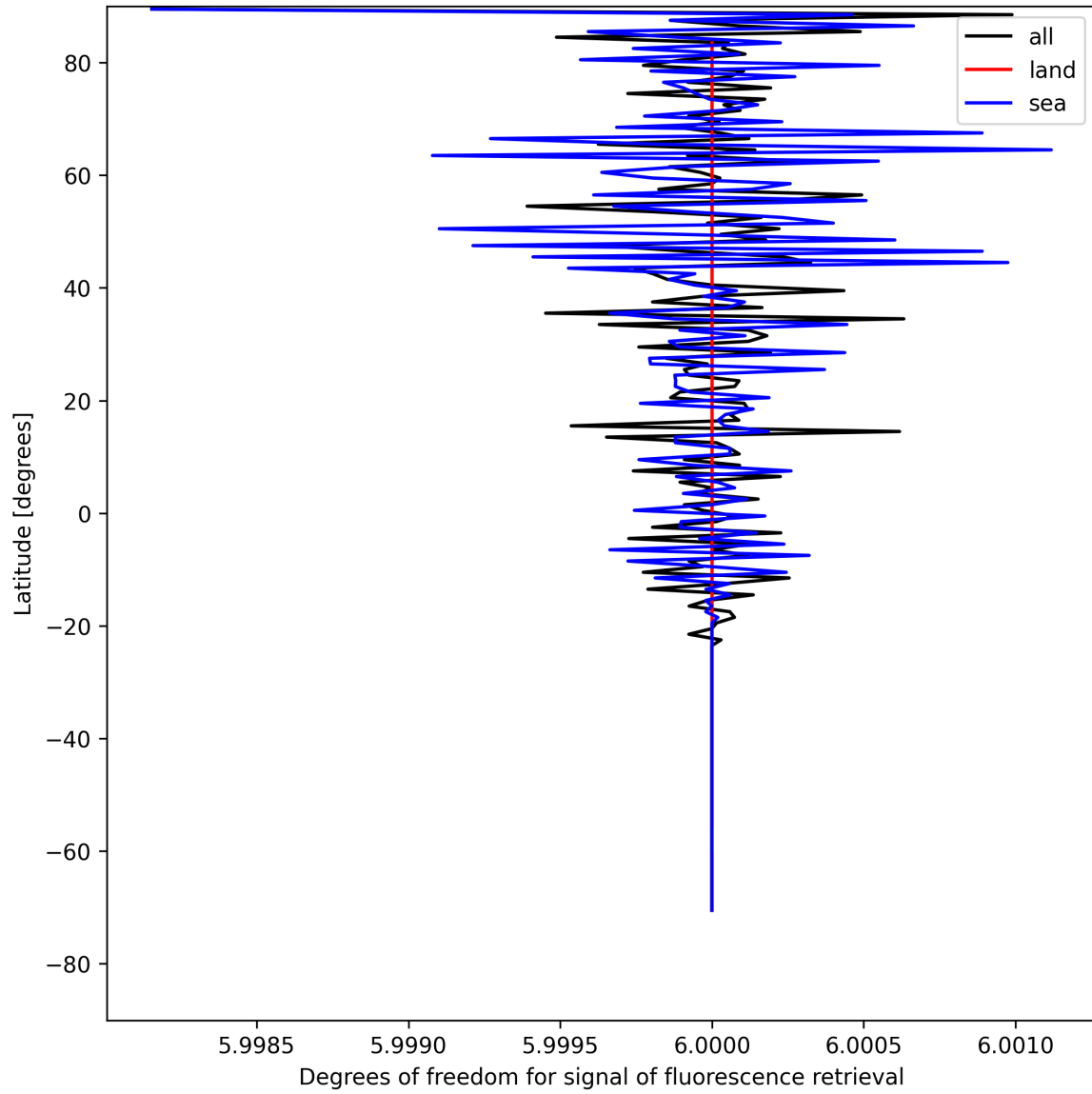
Figure 24: Zonal average of “Degrees of freedom for signal of fluorescence retrieval” for 2025-05-08 to 2025-05-08.
