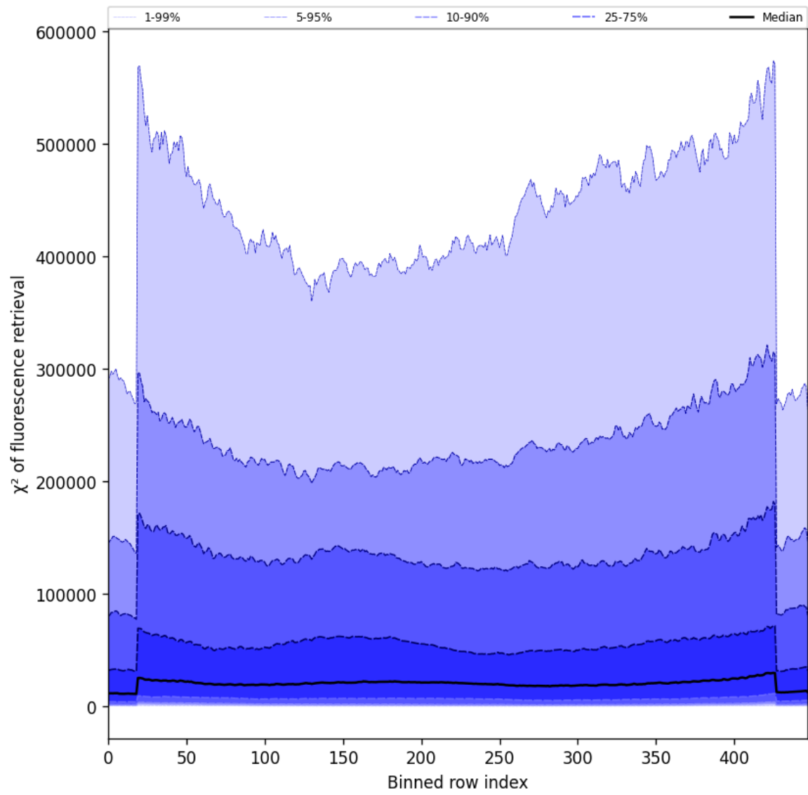
Figure 57: Along track statistics of “ \chi^2 of fluorescence retrieval” for 2025-05-08 to 2025-05-08
