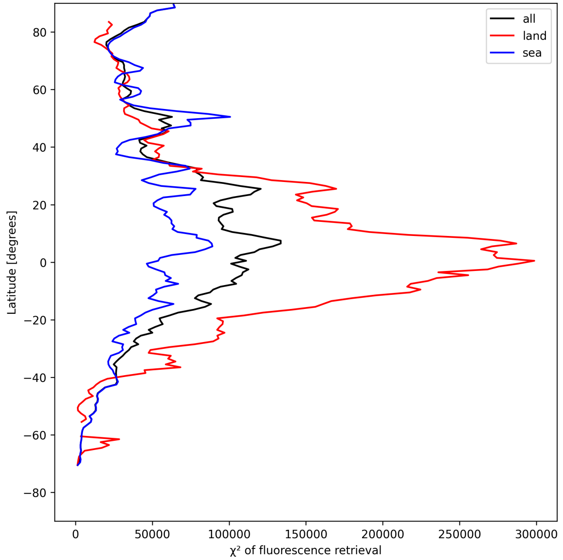
Figure 23: Zonal average of “ \chi^2 of fluorescence retrieval” for 2025-05-08 to 2025-05-08.
