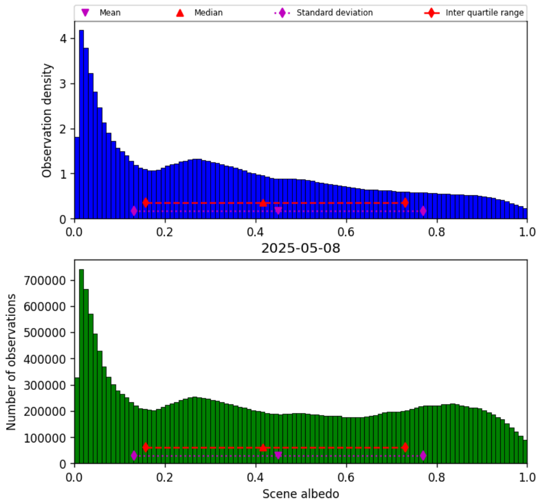
Figure 32: Histogram of “Scene albedo” for 2025-05-08 to 2025-05-08
