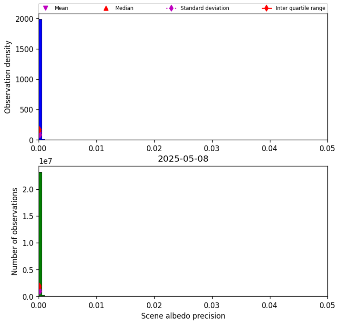
Figure 33: Histogram of “Scene albedo precision” for 2025-05-08 to 2025-05-08
