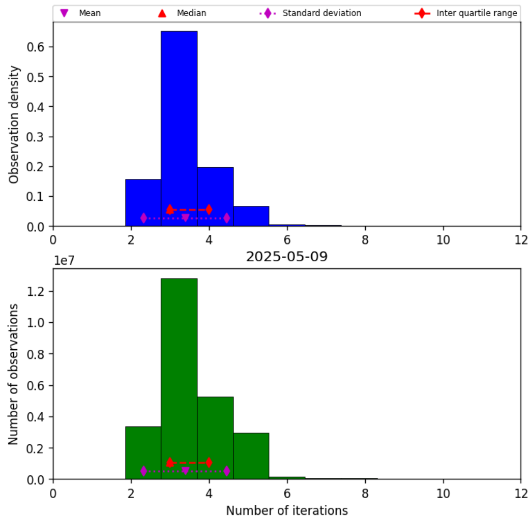
Figure 37: Histogram of “Number of iterations” for 2025-05-09 to 2025-05-10
