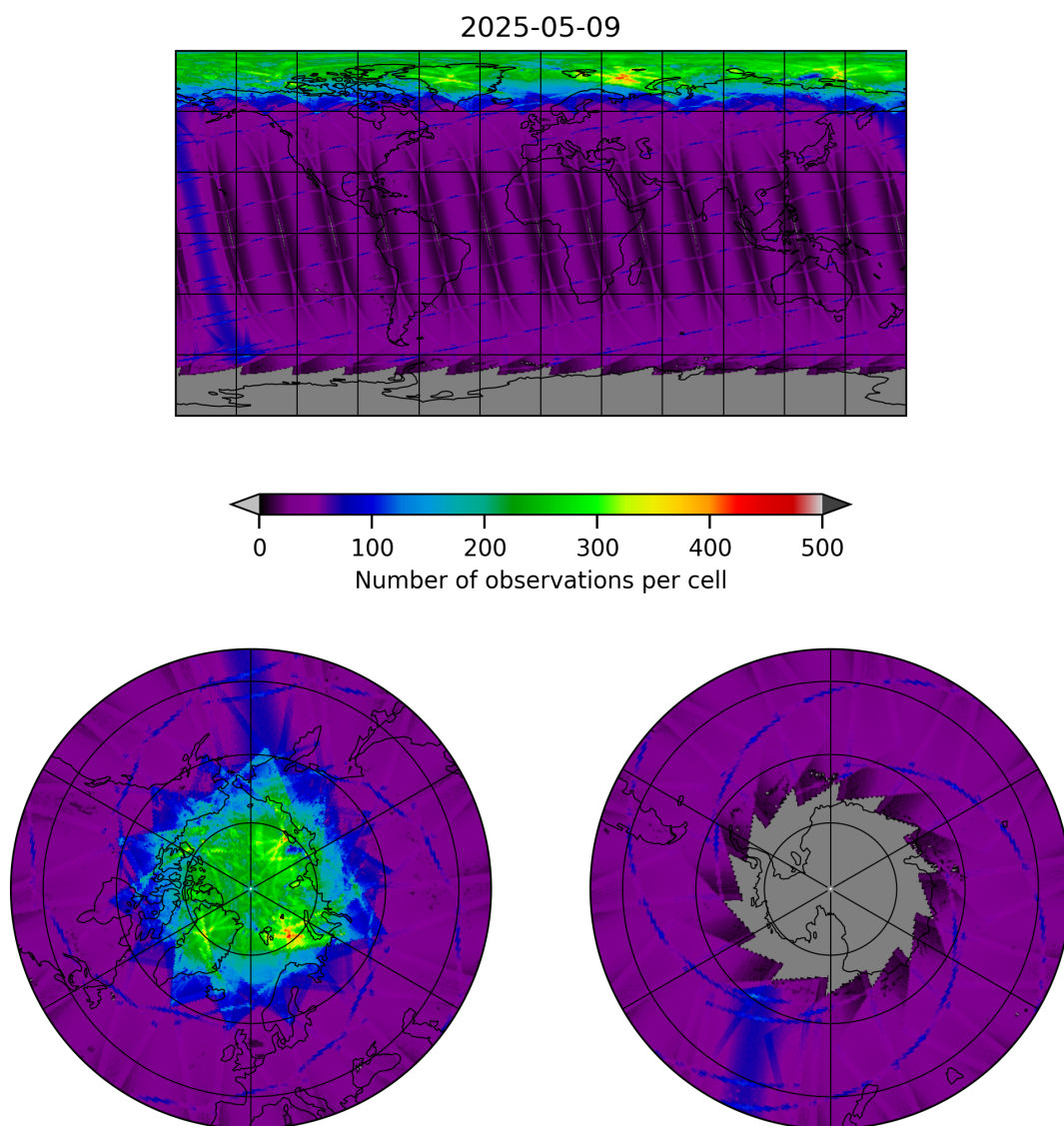
Figure 9: Map of the number of observations for 2025-05-09 to 2025-05-10
