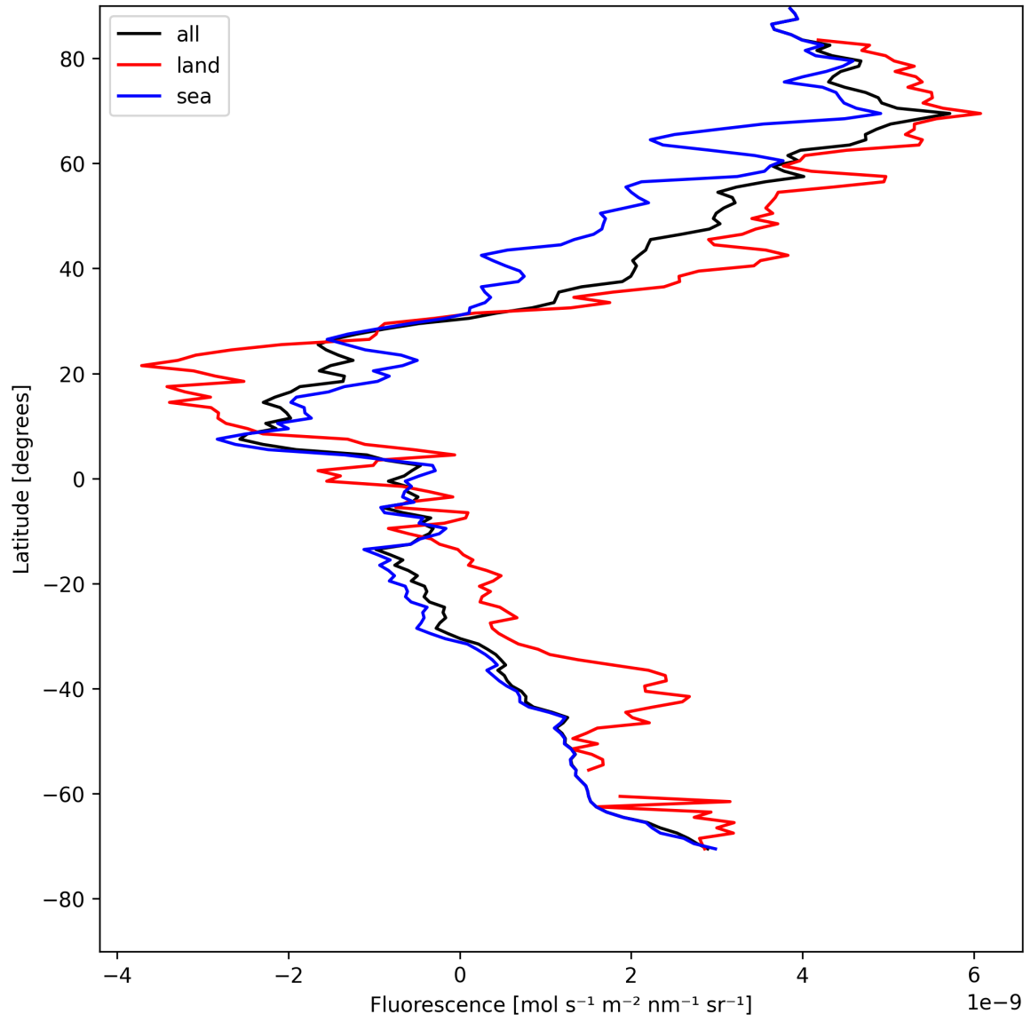
Figure 21: Zonal average of “Fluorescence” for 2025-05-09 to 2025-05-10.
