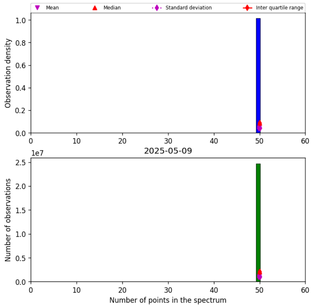
Figure 42: Histogram of “Number of points in the spectrum” for 2025-05-09 to 2025-05-10
