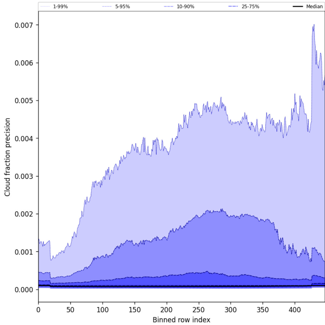
Figure 48: Along track statistics of “Cloud fraction precision” for 2025-05-09 to 2025-05-10
