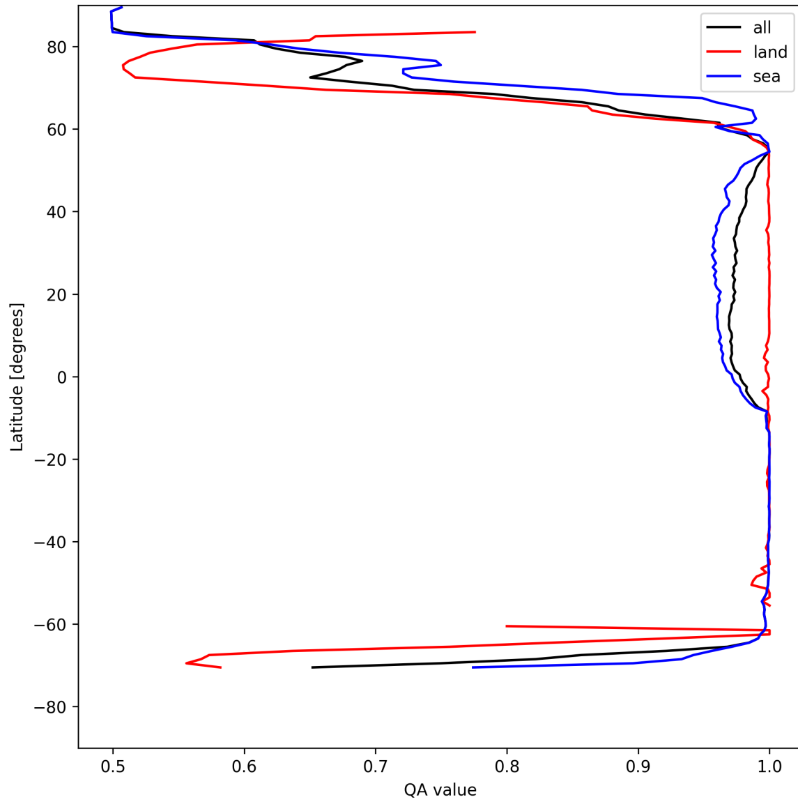
Figure 10: Zonal average of “QA value” for 2025-05-09 to 2025-05-10.
