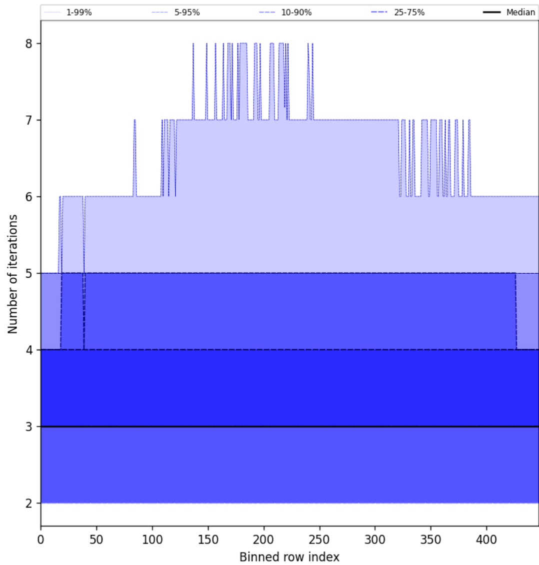
Figure 54: Along track statistics of “Number of iterations” for 2025-05-09 to 2025-05-10
