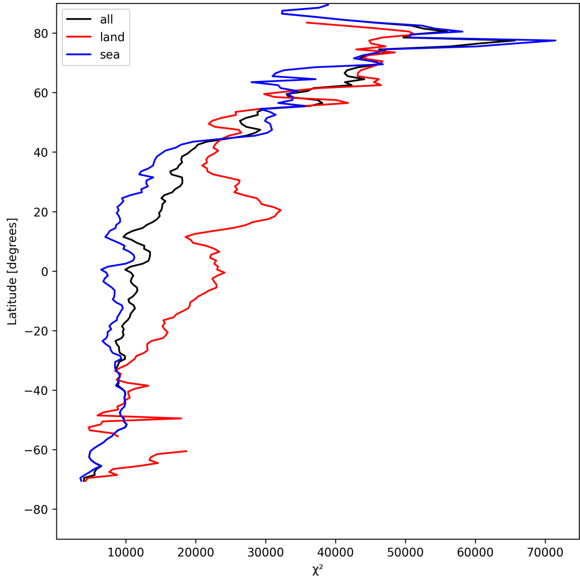
Figure 19: Zonal average of “ \chi^2 ” for 2025-05-09 to 2025-05-10.
