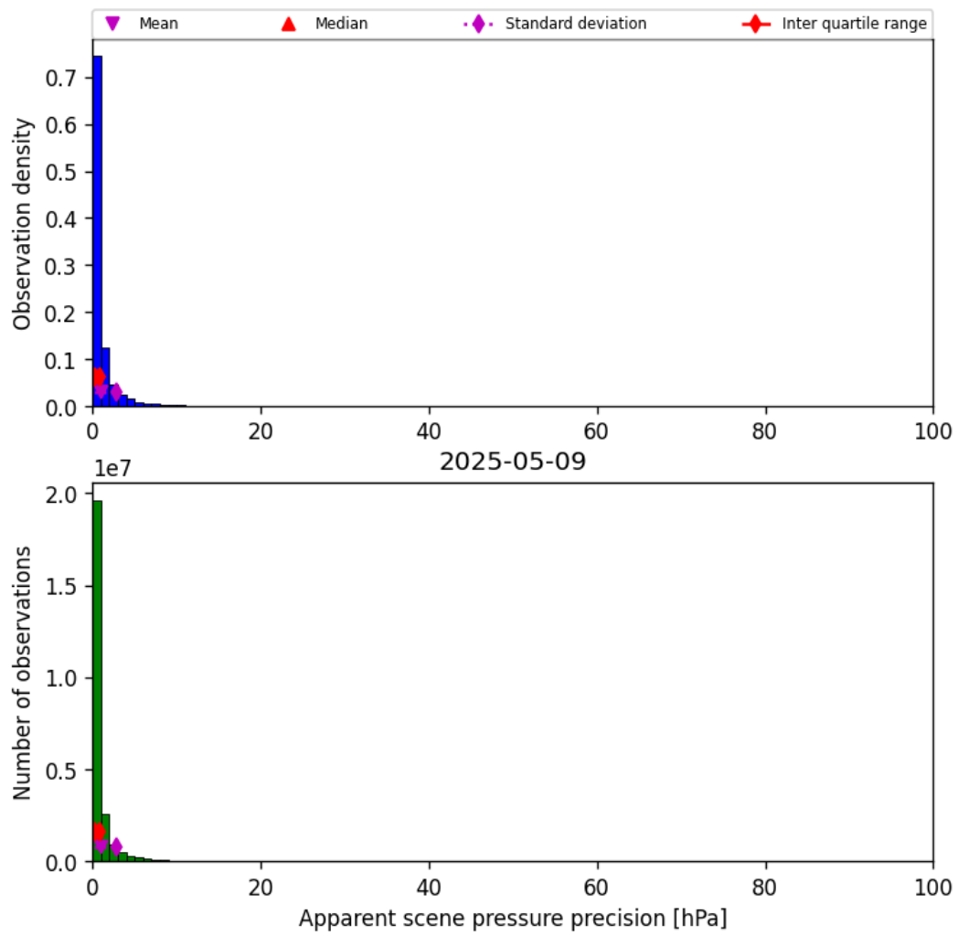
Figure 35: Histogram of “Apparent scene pressure precision” for 2025-05-09 to 2025-05-10
