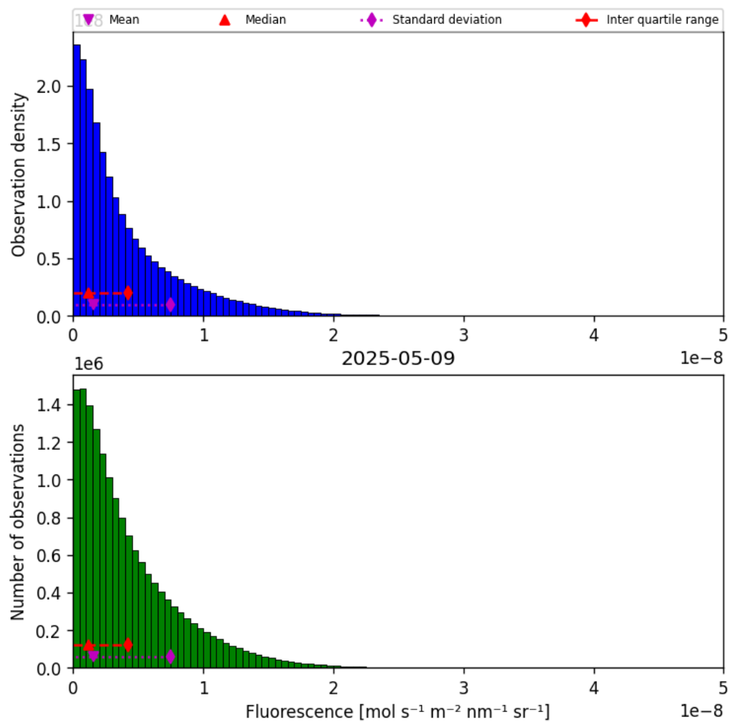
Figure 38: Histogram of “Fluorescence” for 2025-05-09 to 2025-05-10
