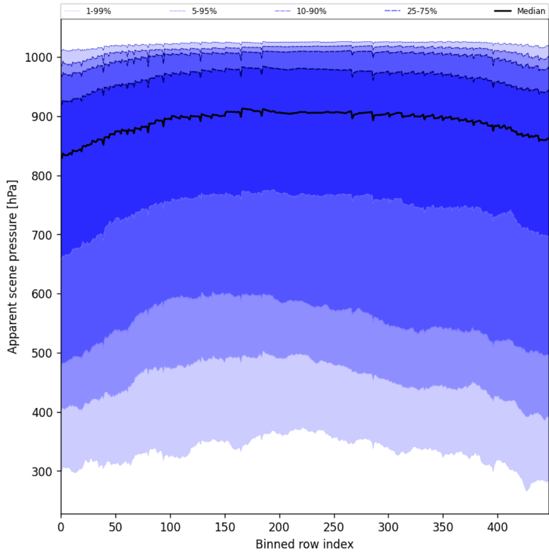
Figure 51: Along track statistics of “Apparent scene pressure” for 2025-05-09 to 2025-05-10
