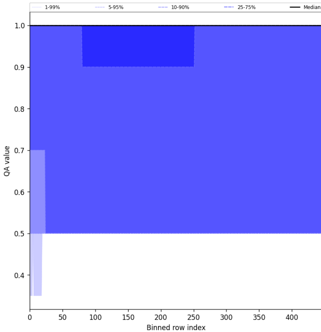
Figure 44: Along track statistics of “QA value” for 2025-05-09 to 2025-05-10
