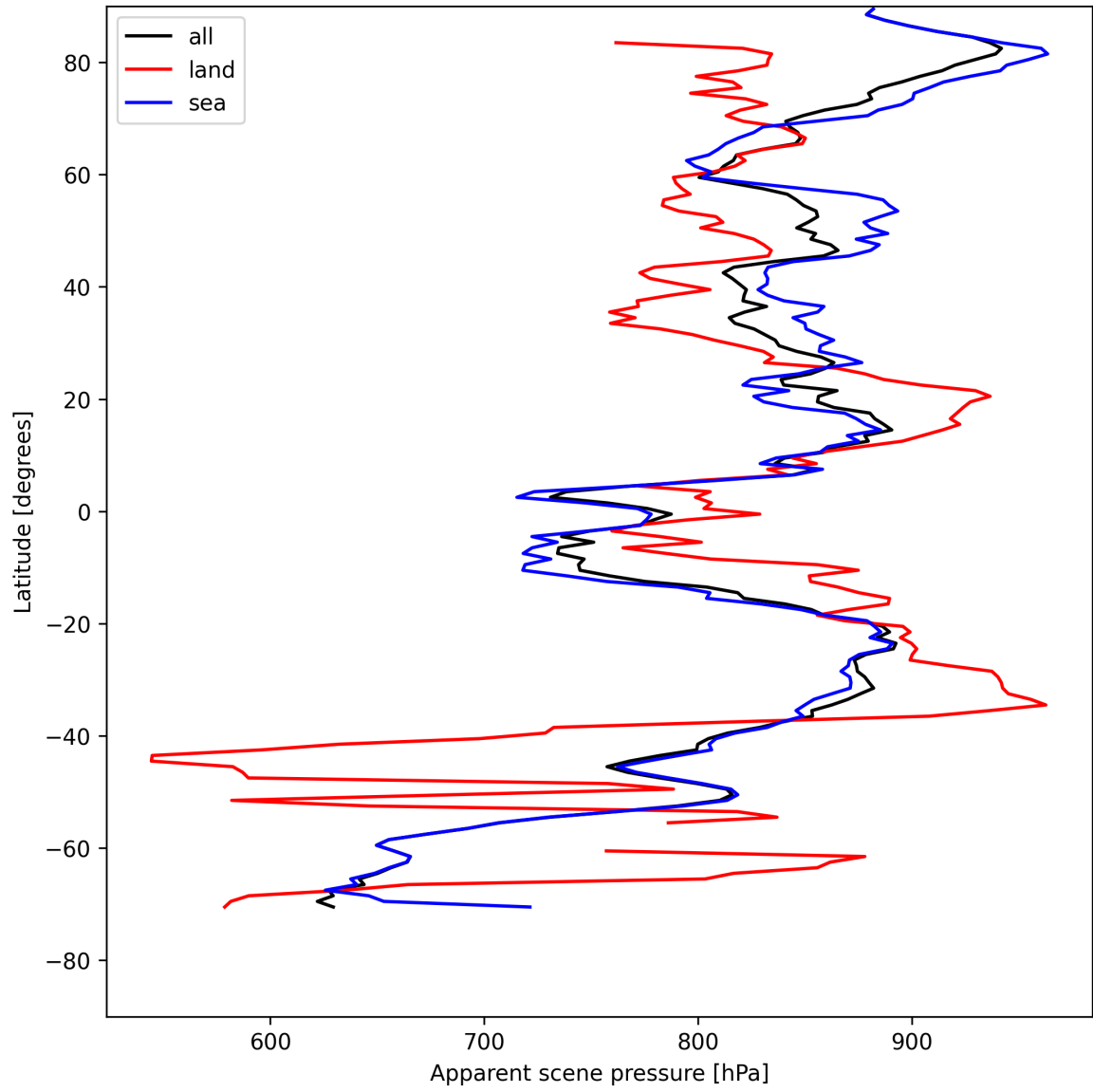
Figure 17: Zonal average of “Apparent scene pressure” for 2025-05-09 to 2025-05-10.
