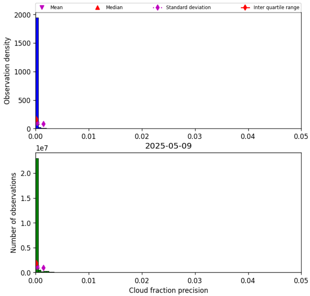
Figure 31: Histogram of “Cloud fraction precision” for 2025-05-09 to 2025-05-10
