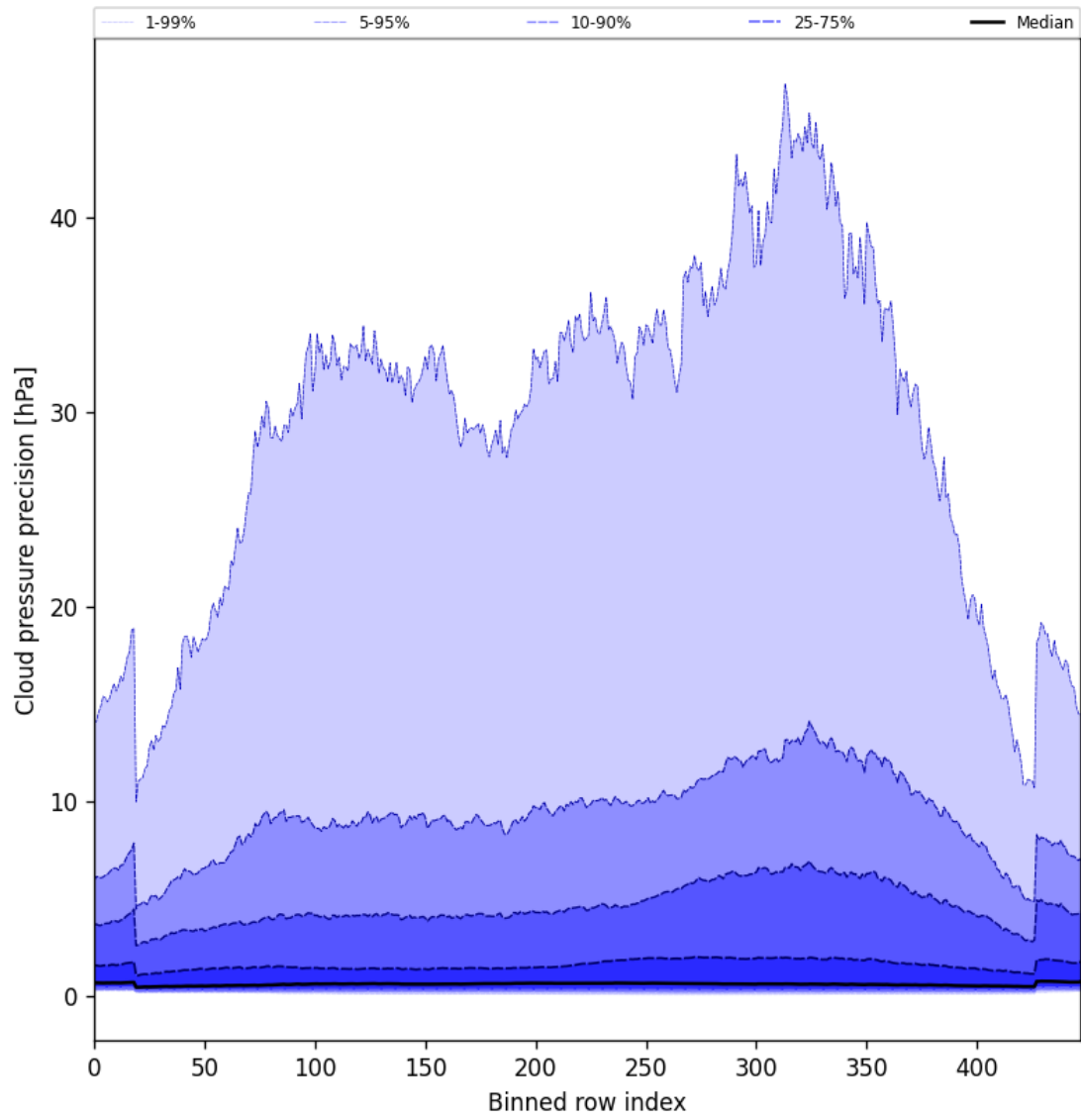
Figure 46: Along track statistics of “Cloud pressure precision” for 2025-05-09 to 2025-05-10
