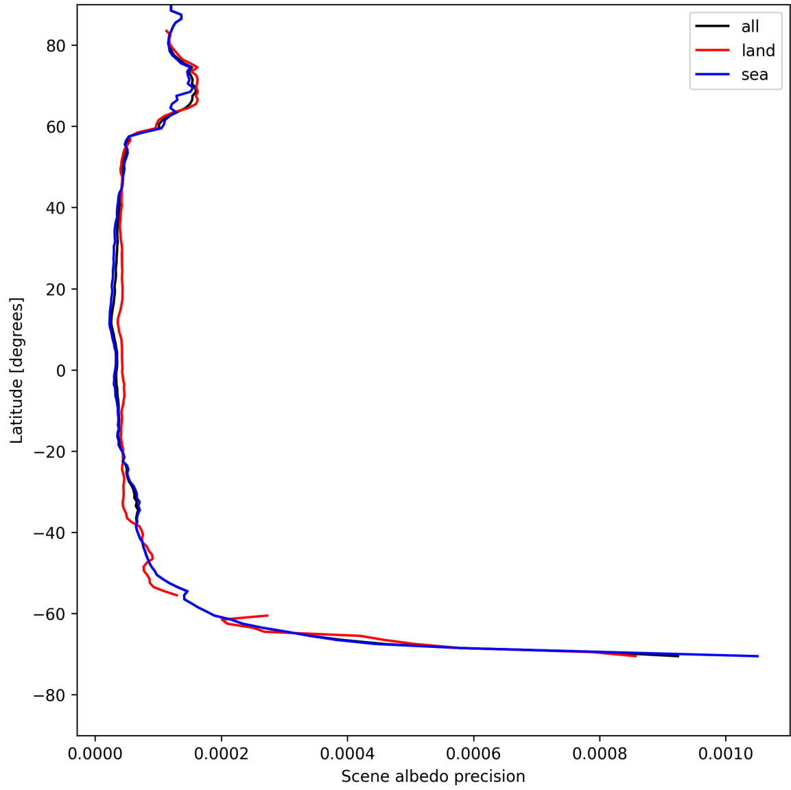
Figure 16: Zonal average of “Scene albedo precision” for 2025-05-09 to 2025-05-10.
