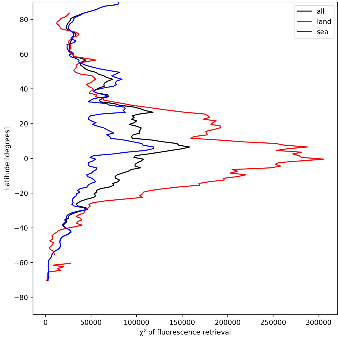
Figure 23: Zonal average of “ \chi^2 of fluorescence retrieval” for 2025-05-09 to 2025-05-10.
