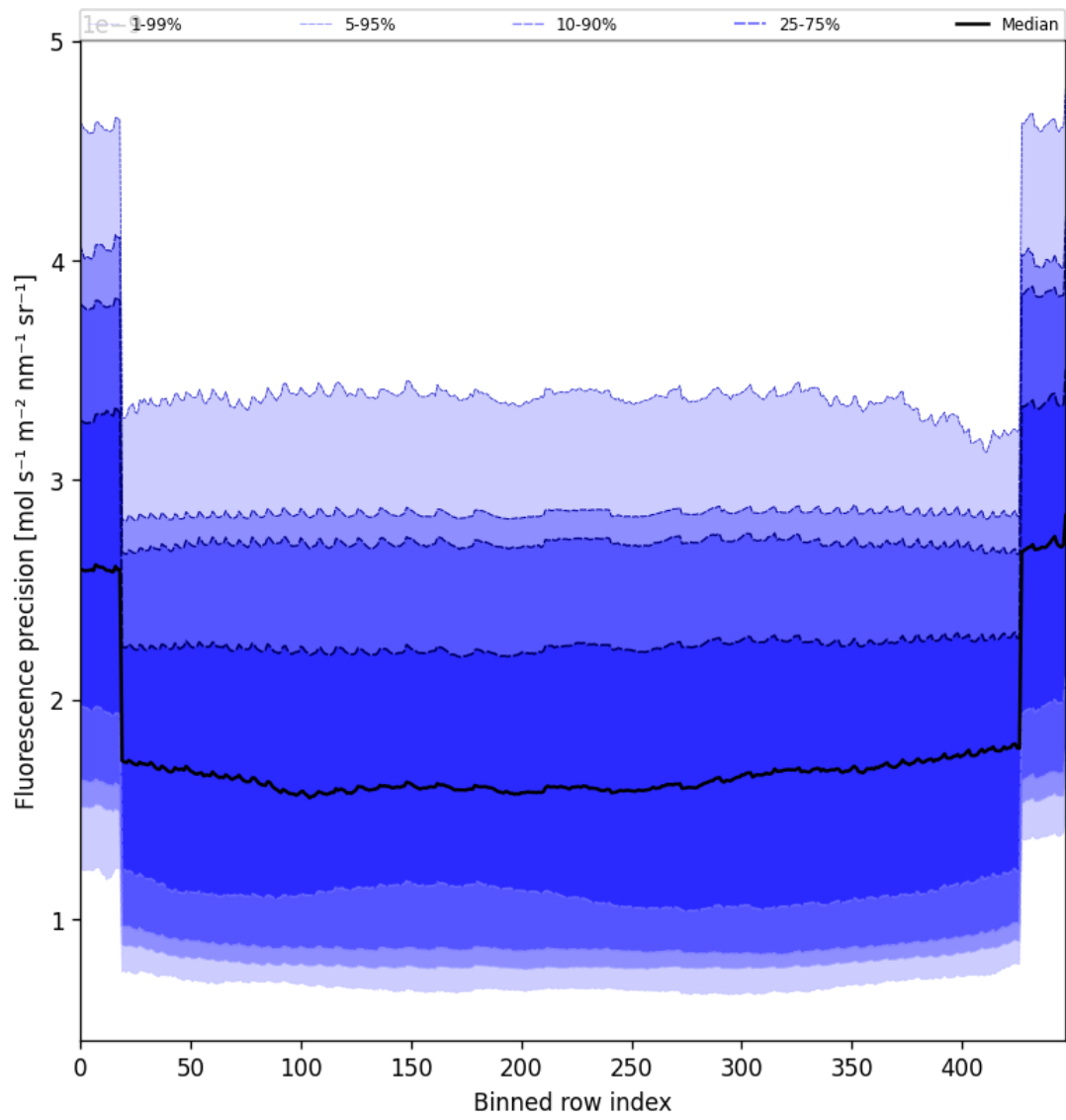
Figure 56: Along track statistics of “Fluorescence precision” for 2025-05-09 to 2025-05-10
