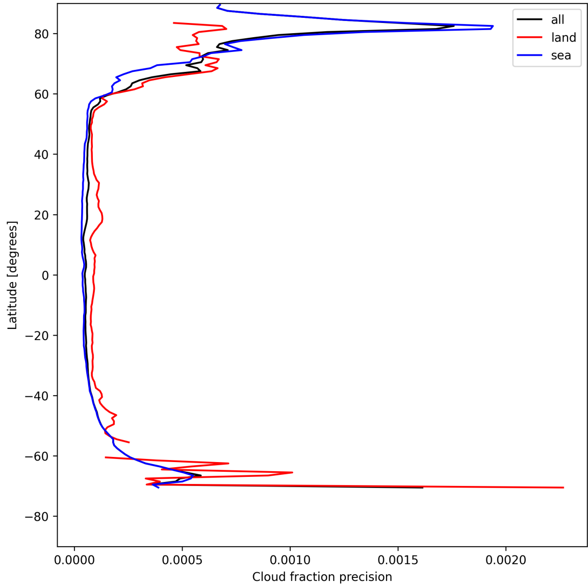
Figure 14: Zonal average of “Cloud fraction precision” for 2025-05-09 to 2025-05-10.
