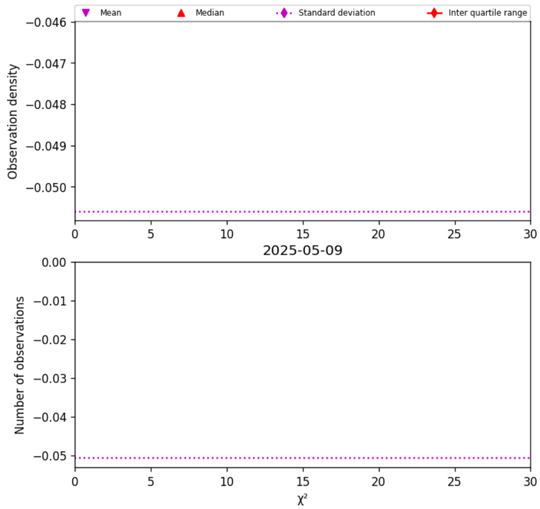
Figure 36: Histogram of “ \chi^2 ” for 2025-05-09 to 2025-05-10
