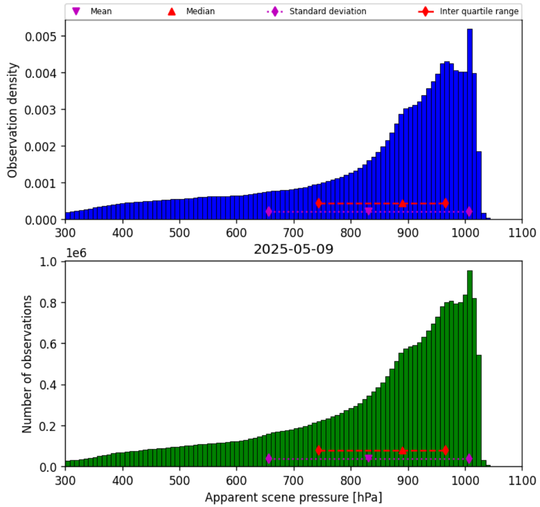
Figure 34: Histogram of “Apparent scene pressure” for 2025-05-09 to 2025-05-10
