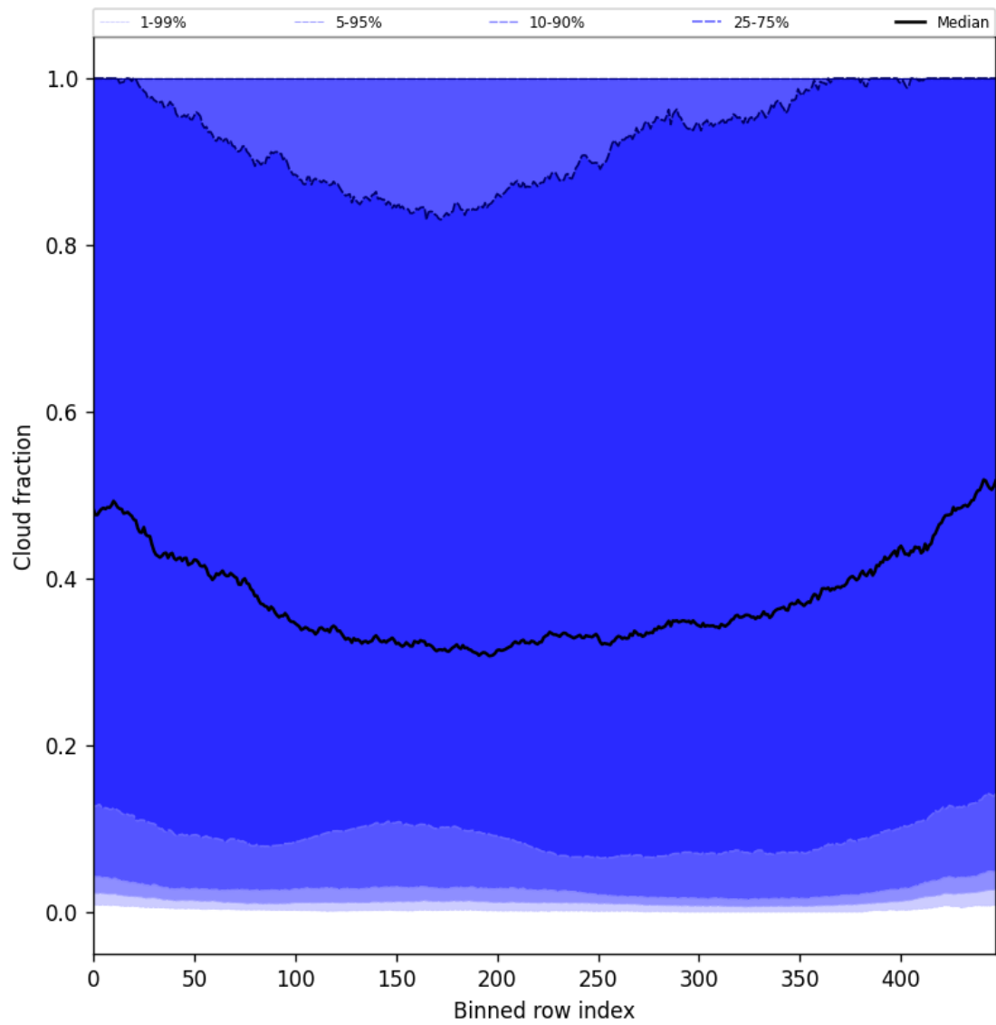
Figure 47: Along track statistics of “Cloud fraction” for 2025-05-09 to 2025-05-10
