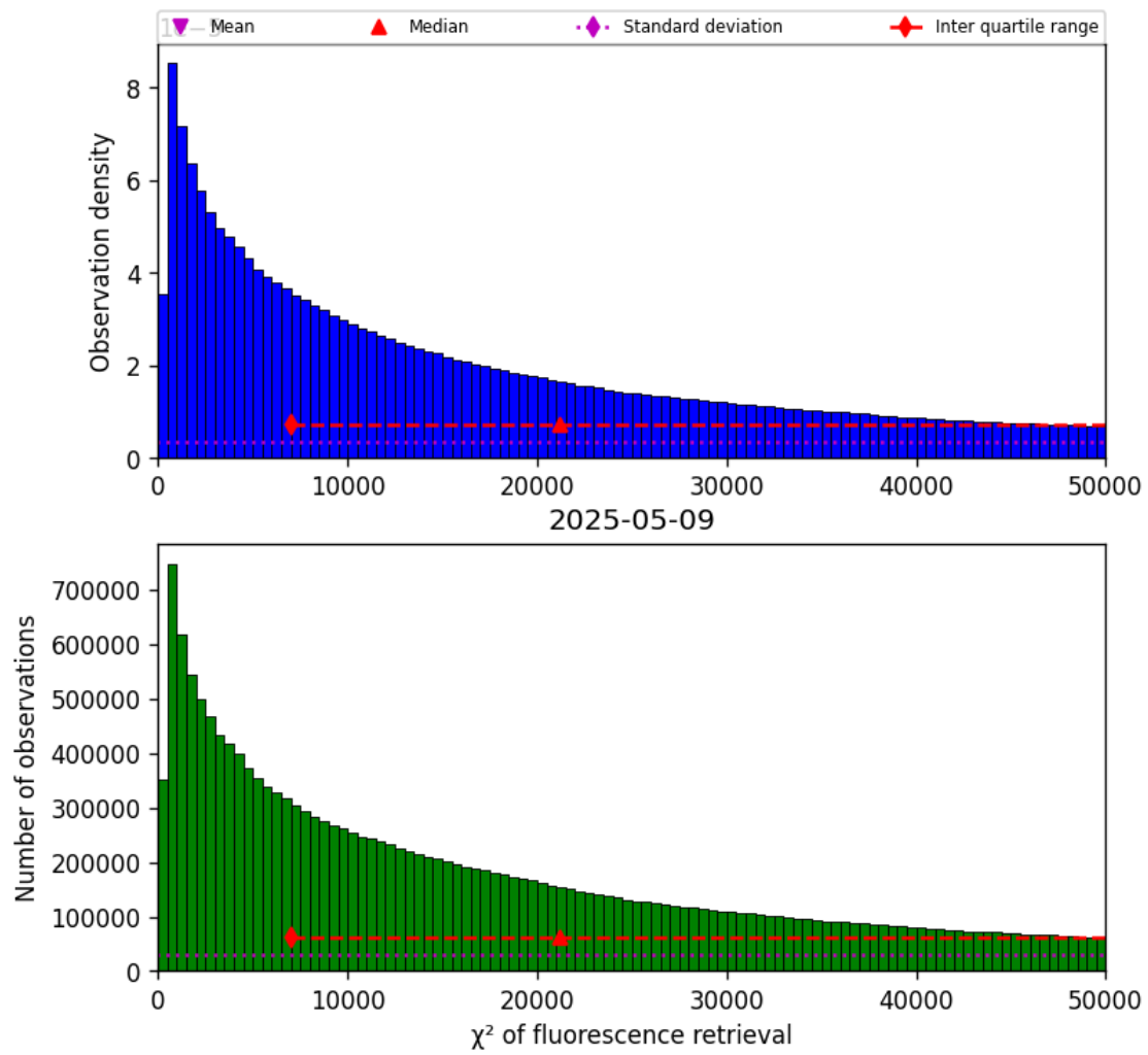
Figure 40: Histogram of “ \chi^2 of fluorescence retrieval” for 2025-05-09 to 2025-05-10
