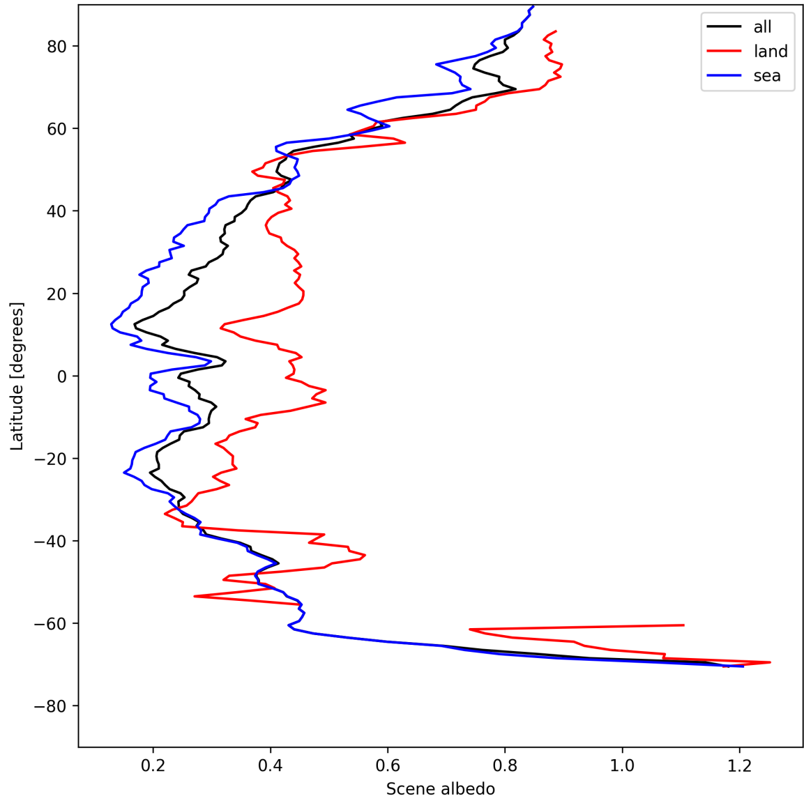
Figure 15: Zonal average of “Scene albedo” for 2025-05-09 to 2025-05-10.
