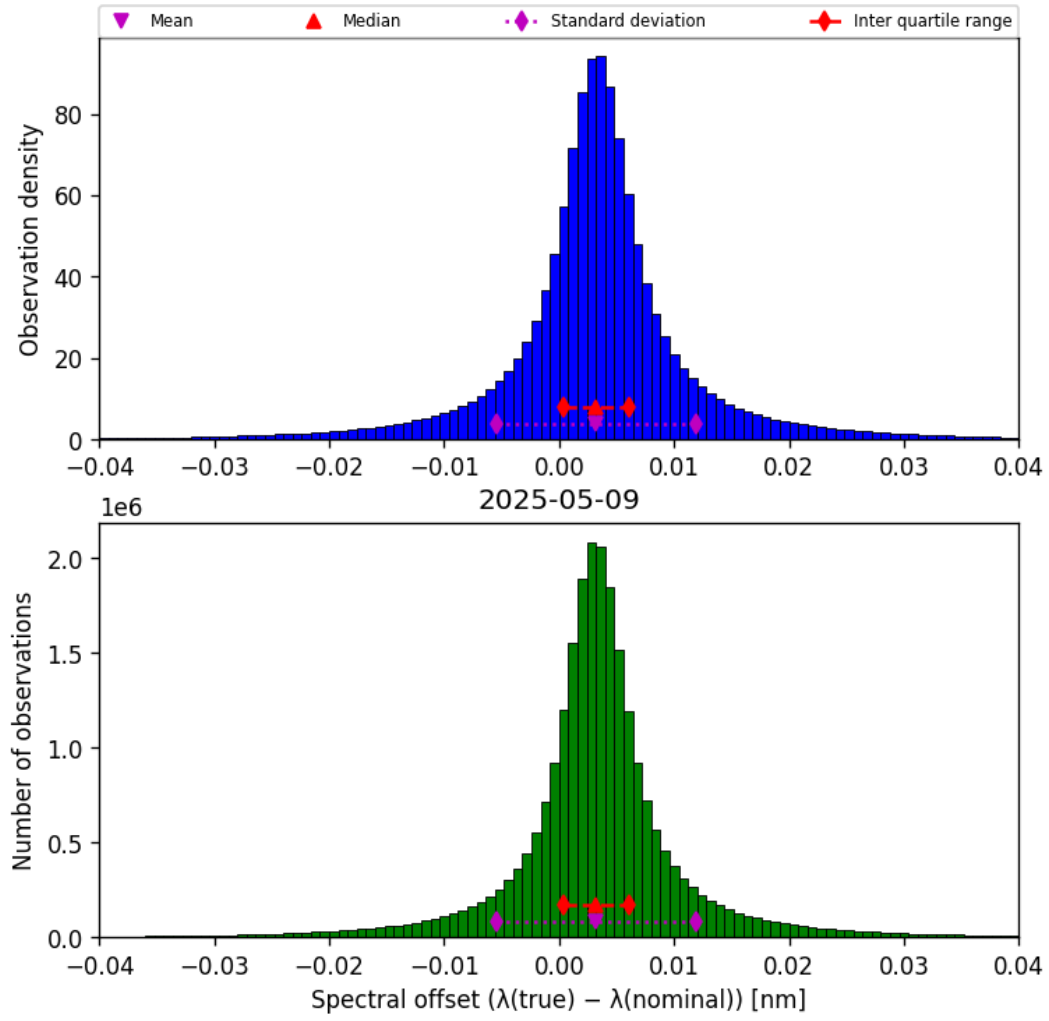
Figure 43: Histogram of “Spectral offset ( \lambda_{\text{true}} - \lambda_{\text{nominal}} )” for 2025-05-09 to 2025-05-10
