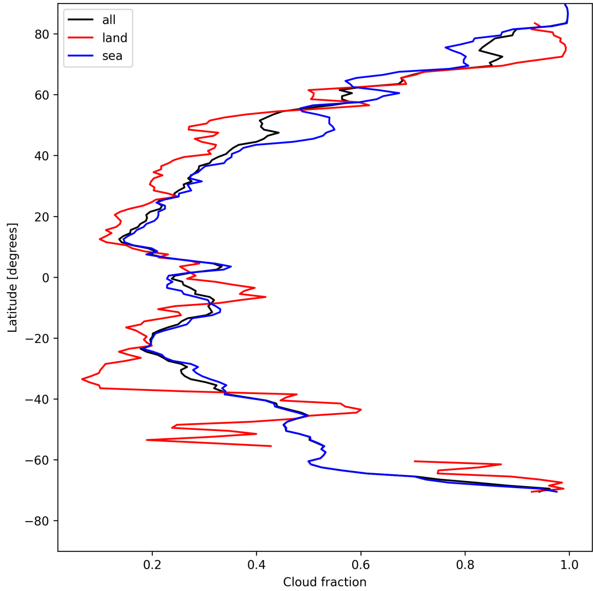
Figure 13: Zonal average of “Cloud fraction” for 2025-05-09 to 2025-05-10.
