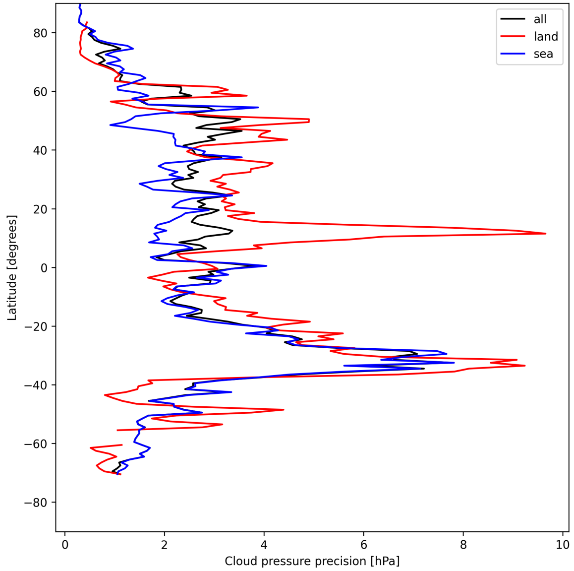
Figure 12: Zonal average of "Cloud pressure precision" for 2025-05-09 to 2025-05-10.
