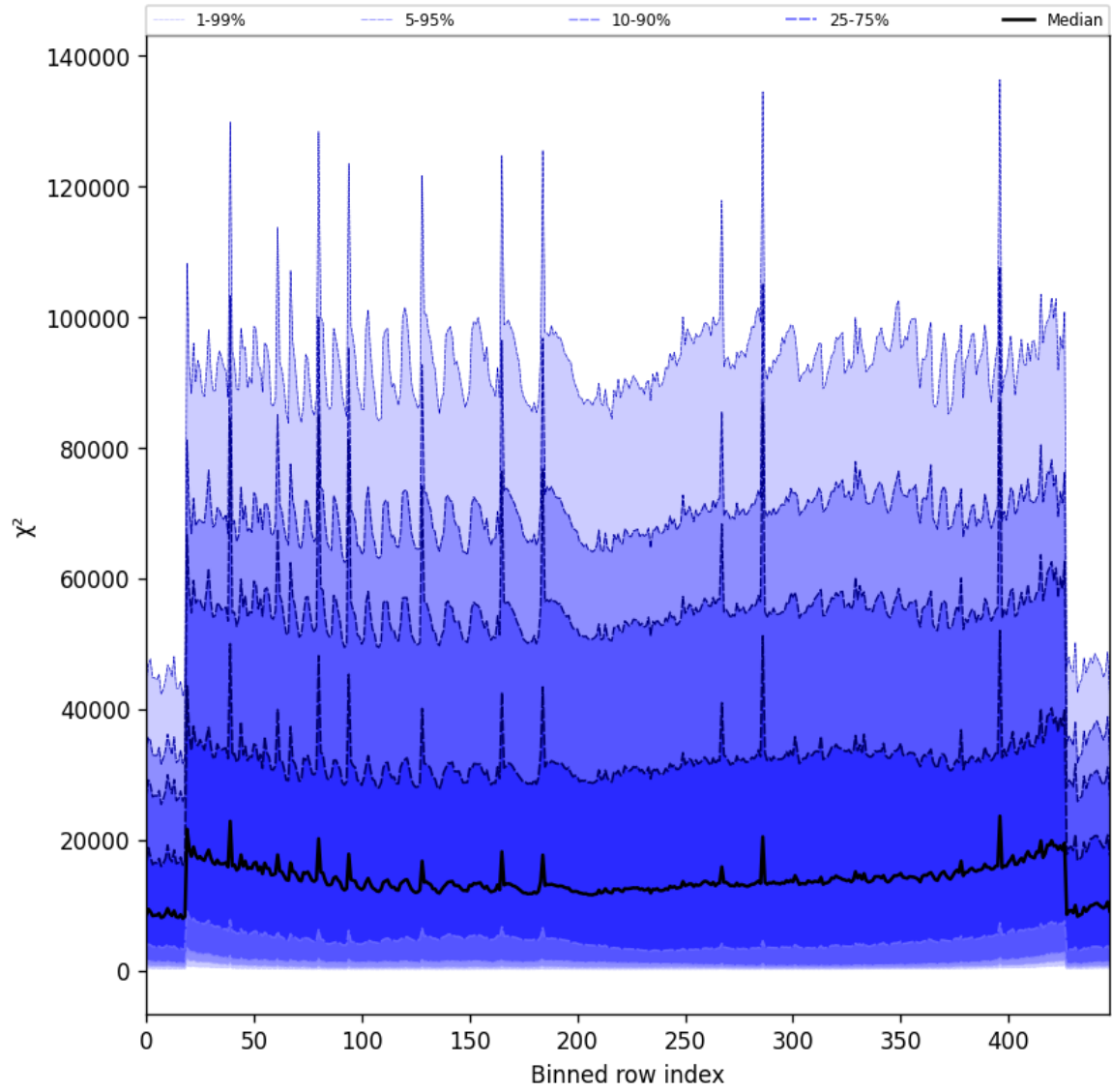
Figure 53: Along track statistics of “ \chi^2 ” for 2025-05-09 to 2025-05-10
