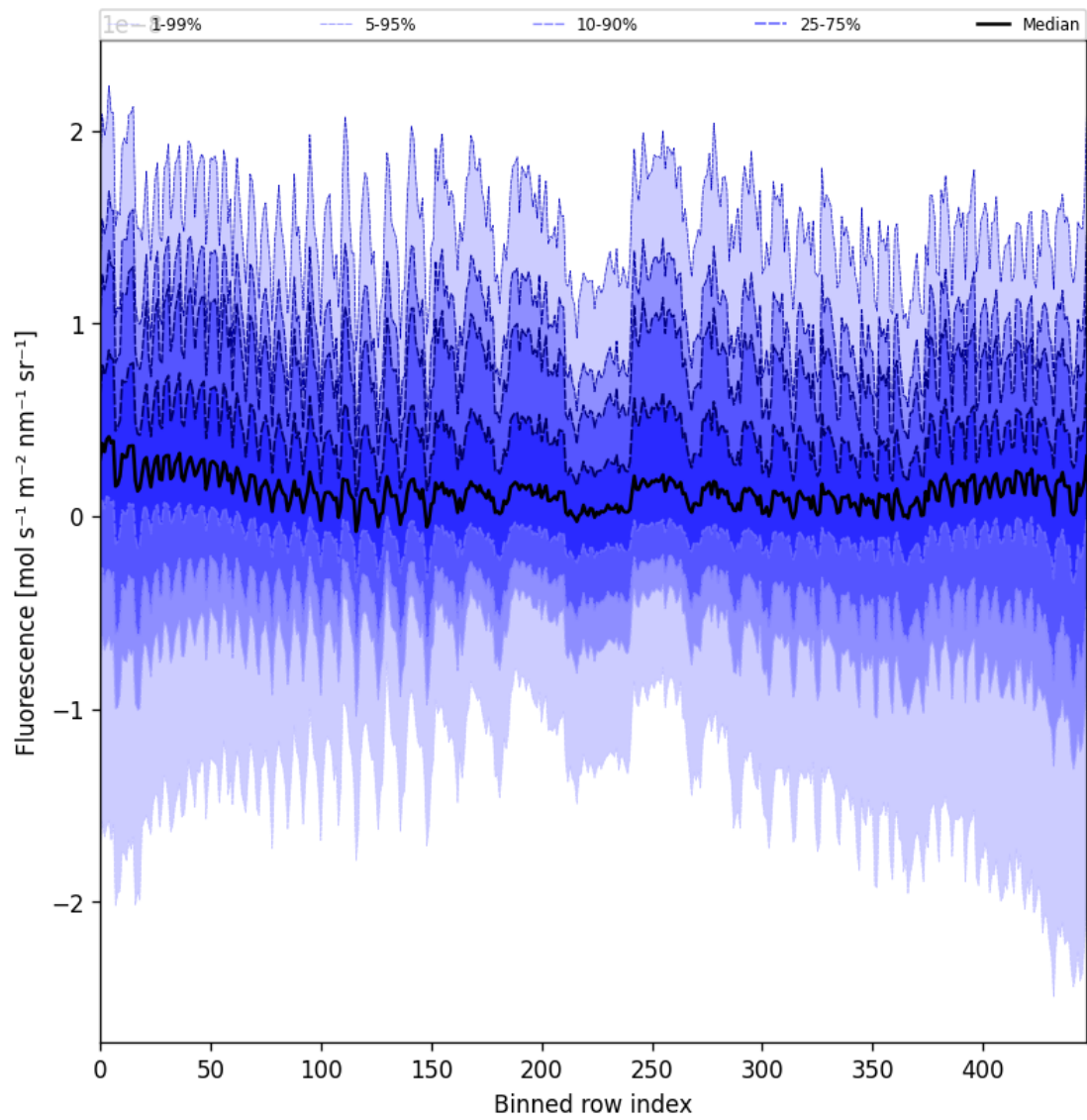
Figure 55: Along track statistics of “Fluorescence” for 2025-05-09 to 2025-05-10
