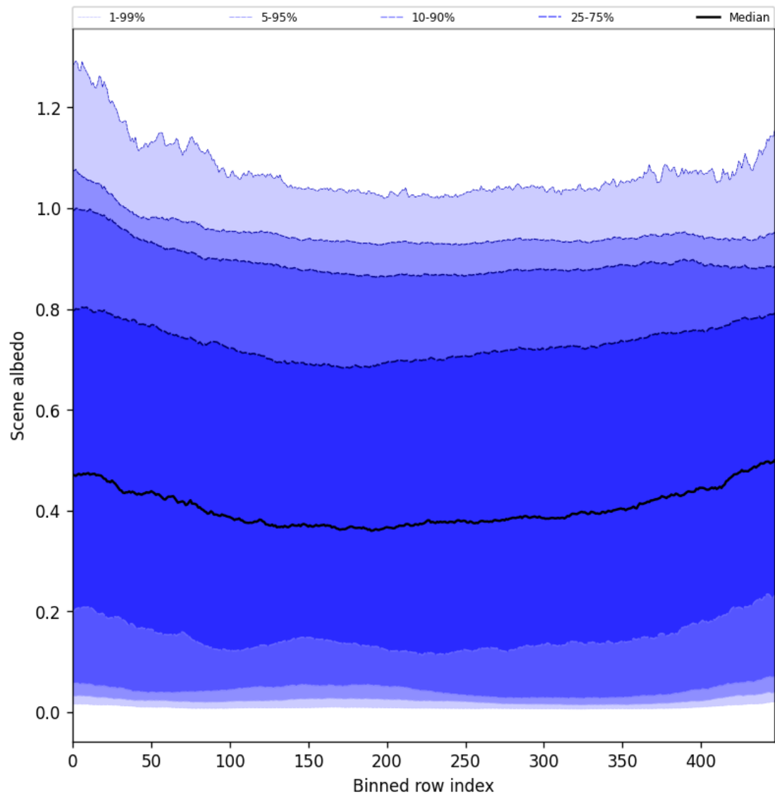
Figure 49: Along track statistics of “Scene albedo” for 2025-05-09 to 2025-05-10
