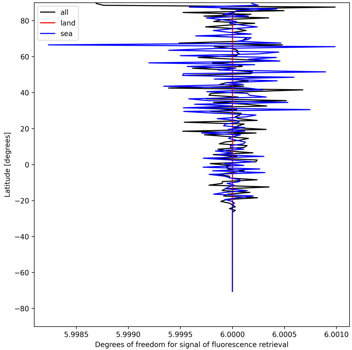
Figure 24: Zonal average of “Degrees of freedom for signal of fluorescence retrieval” for 2025-05-09 to 2025-05-10.
