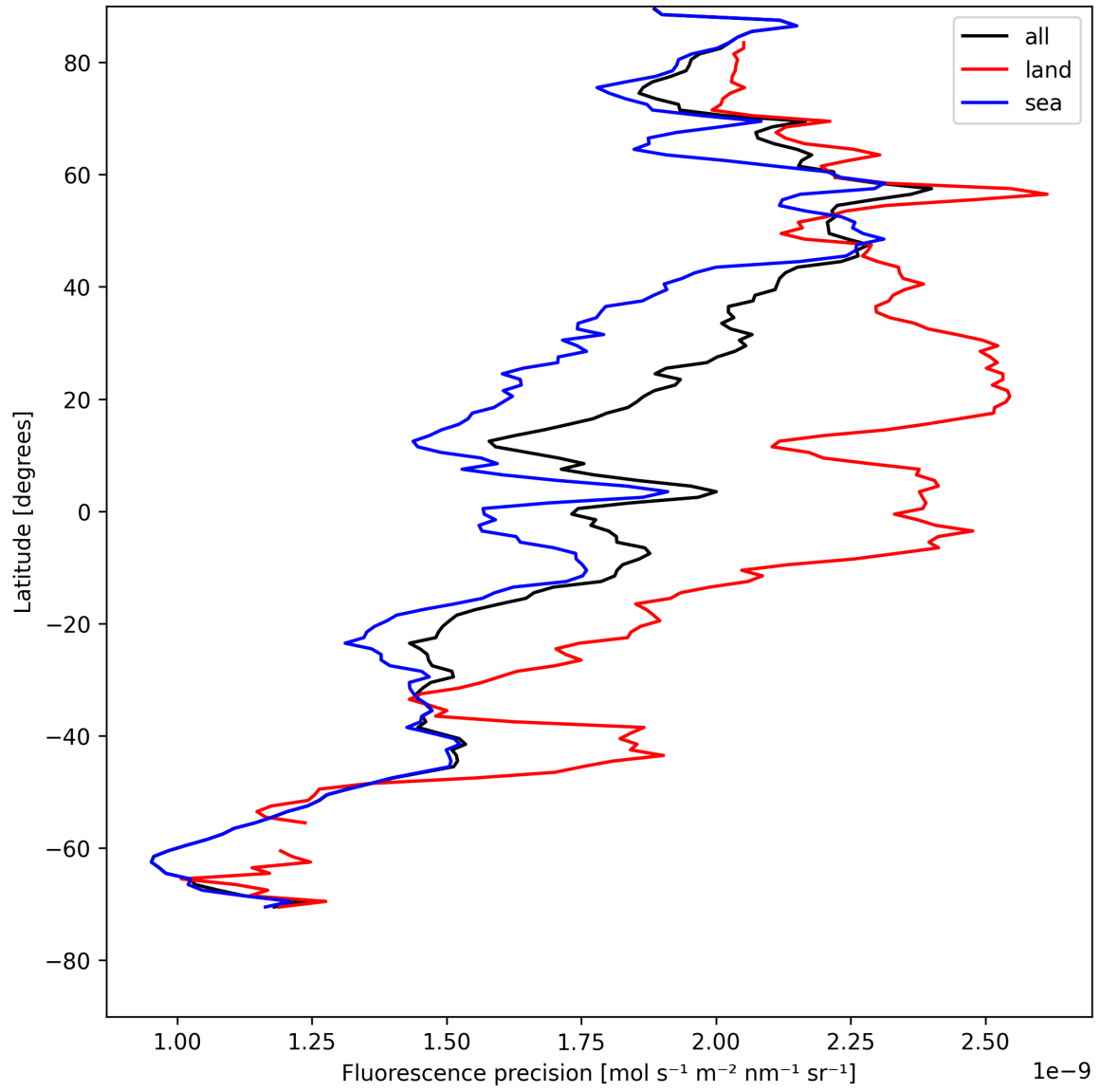
Figure 22: Zonal average of “Fluorescence precision” for 2025-05-09 to 2025-05-10.
