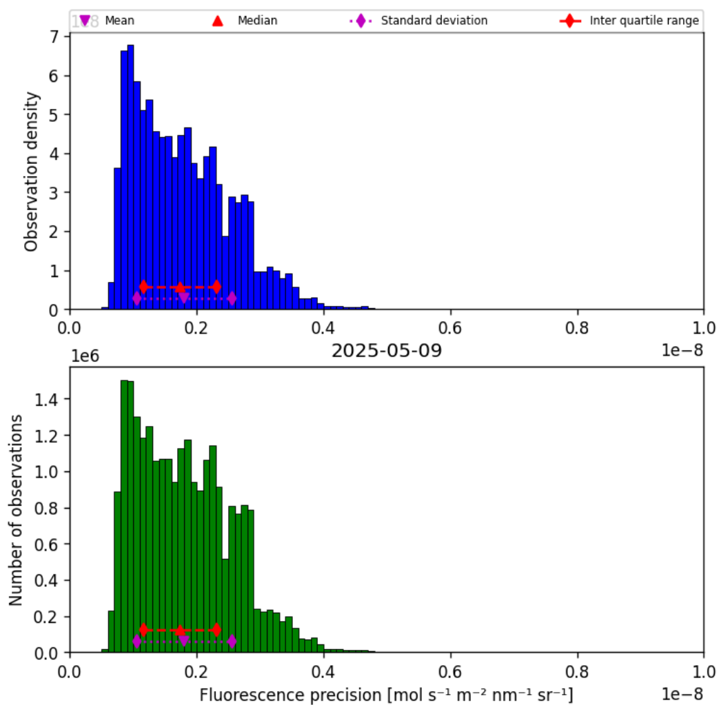
Figure 39: Histogram of “Fluorescence precision” for 2025-05-09 to 2025-05-10
