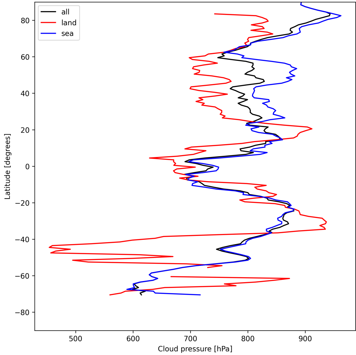
Figure 11: Zonal average of “Cloud pressure” for 2025-05-09 to 2025-05-10.
