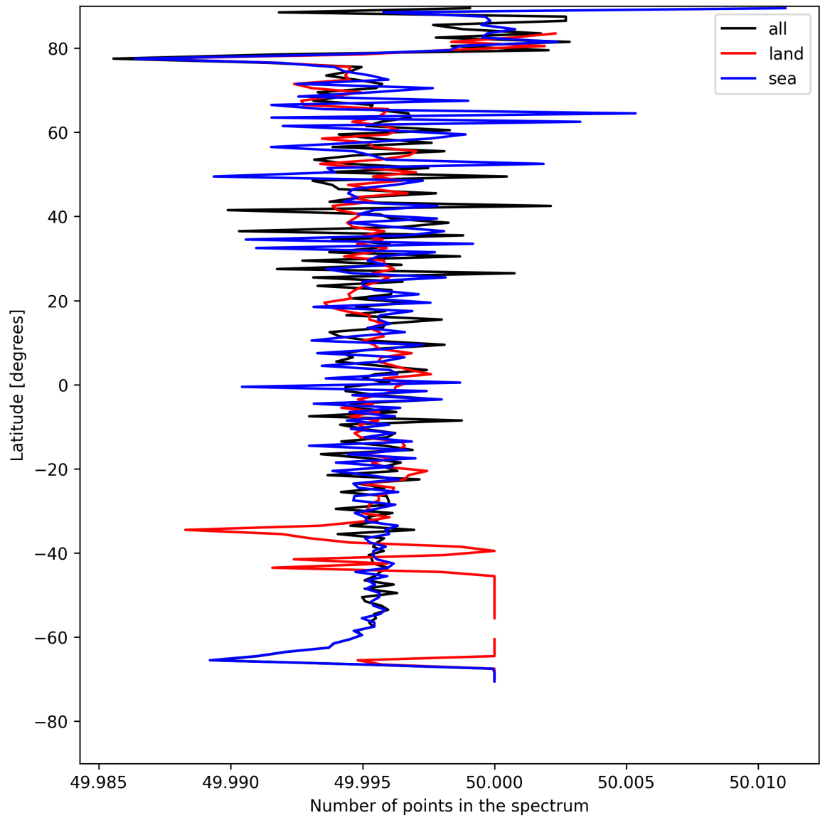
Figure 25: Zonal average of “Number of points in the spectrum” for 2025-05-09 to 2025-05-10.
