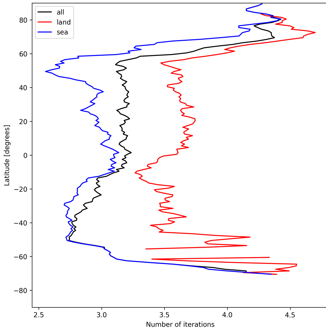
Figure 20: Zonal average of “Number of iterations” for 2025-05-09 to 2025-05-10.
