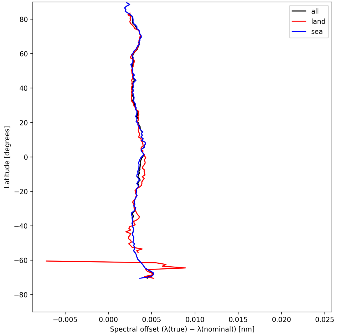
Figure 26: Zonal average of “Spectral offset ( \lambda_{\text{true}} - \lambda_{\text{nominal}} )” for 2025-05-09 to 2025-05-10.
