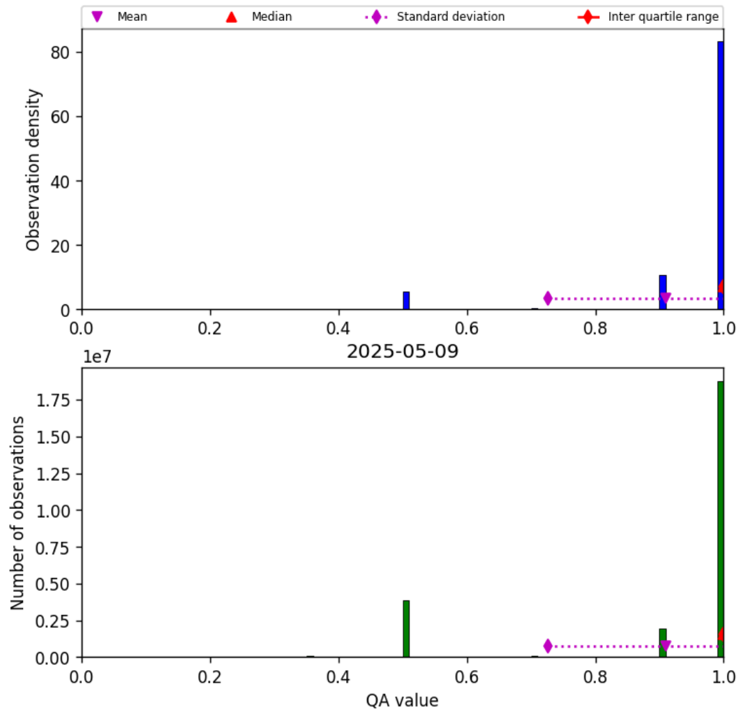
Figure 27: Histogram of “QA value” for 2025-05-09 to 2025-05-10
