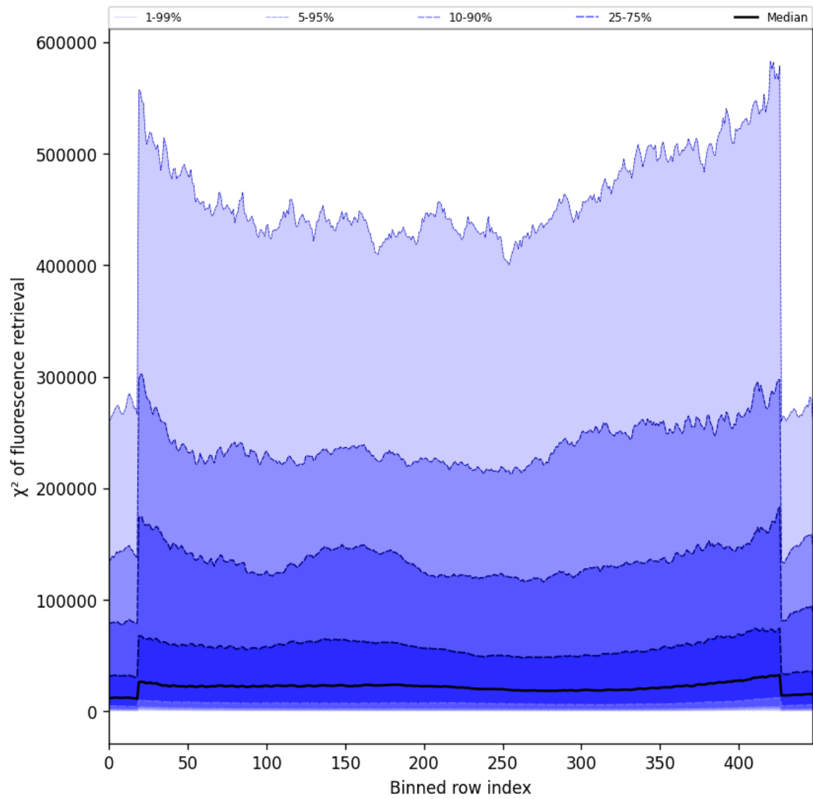
Figure 57: Along track statistics of “ \chi^2 of fluorescence retrieval” for 2025-05-09 to 2025-05-10
