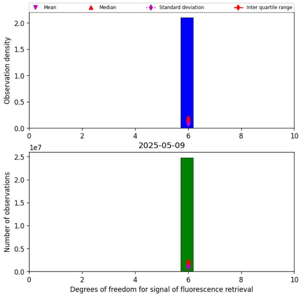
Figure 41: Histogram of “Degrees of freedom for signal of fluorescence retrieval” for 2025-05-09 to 2025-05-10
