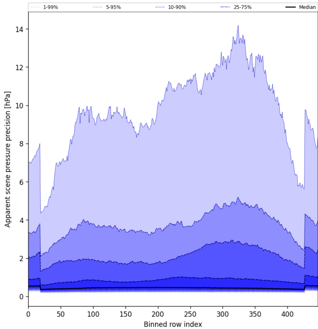
Figure 52: Along track statistics of “Apparent scene pressure precision” for 2025-05-09 to 2025-05-10
