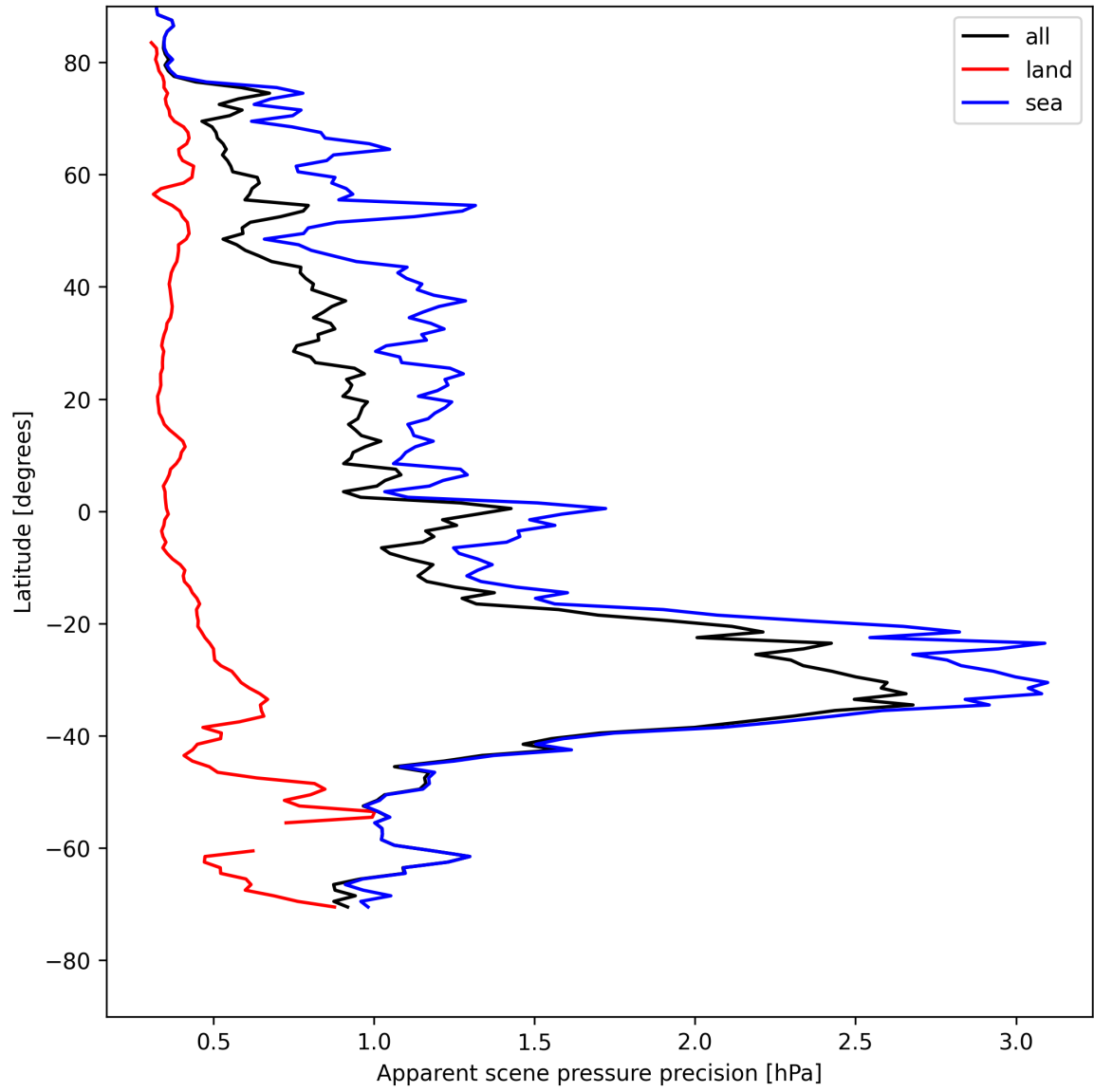
Figure 18: Zonal average of “Apparent scene pressure precision” for 2025-05-09 to 2025-05-10.
