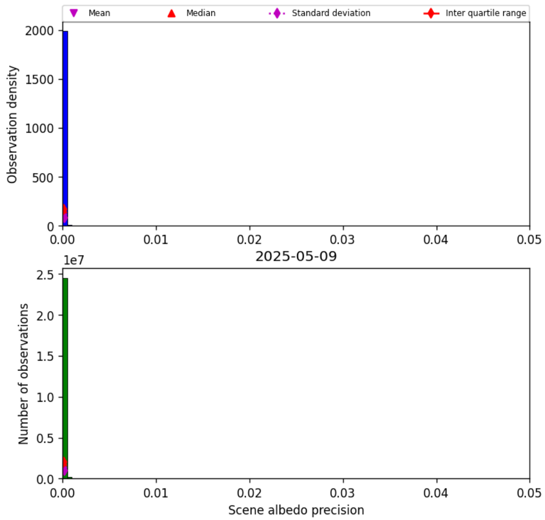
Figure 33: Histogram of “Scene albedo precision” for 2025-05-09 to 2025-05-10
