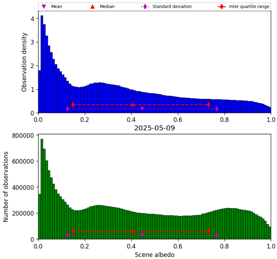
Figure 32: Histogram of “Scene albedo” for 2025-05-09 to 2025-05-10
