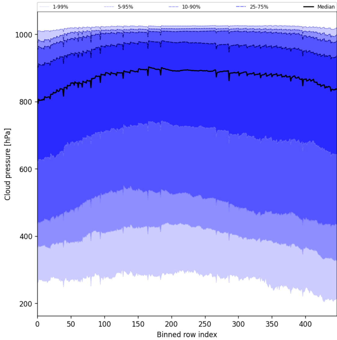
Figure 45: Along track statistics of “Cloud pressure” for 2025-05-09 to 2025-05-10
