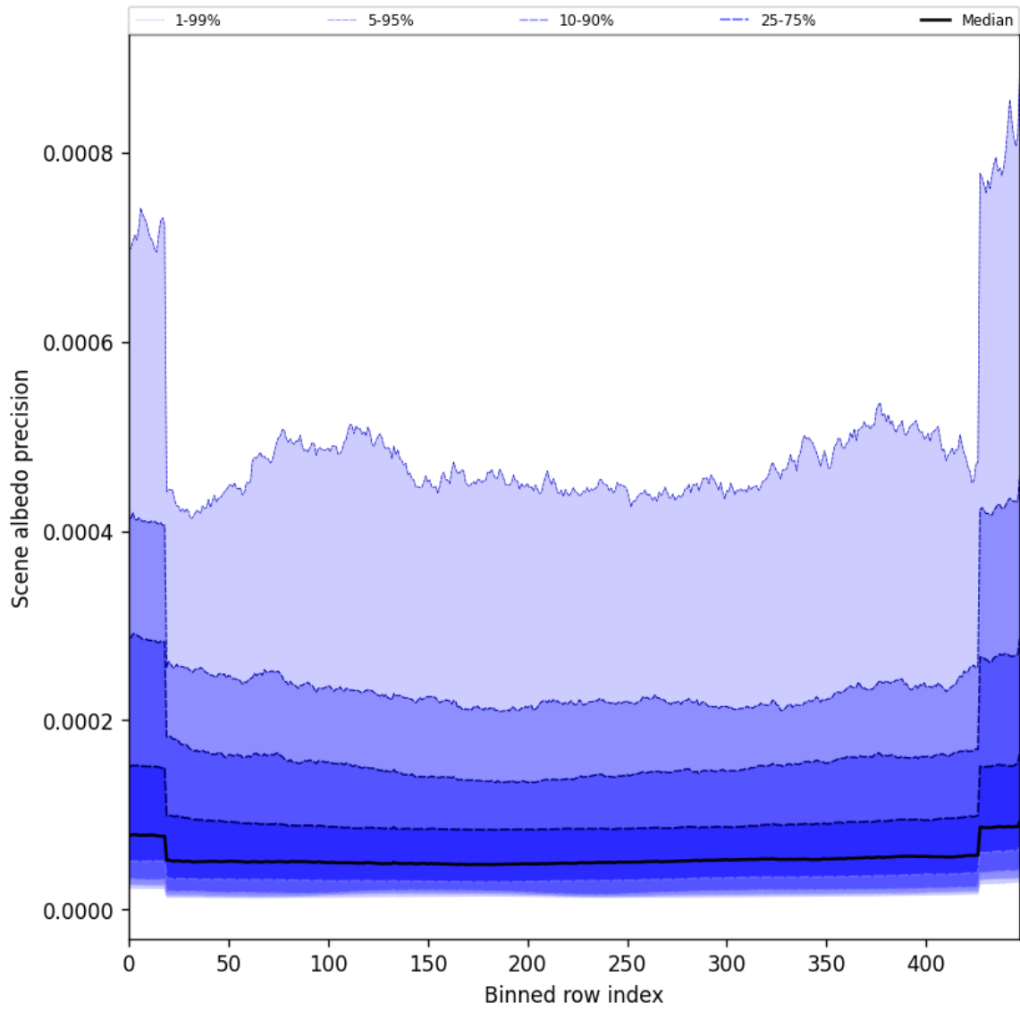
Figure 50: Along track statistics of “Scene albedo precision” for 2025-05-09 to 2025-05-10
