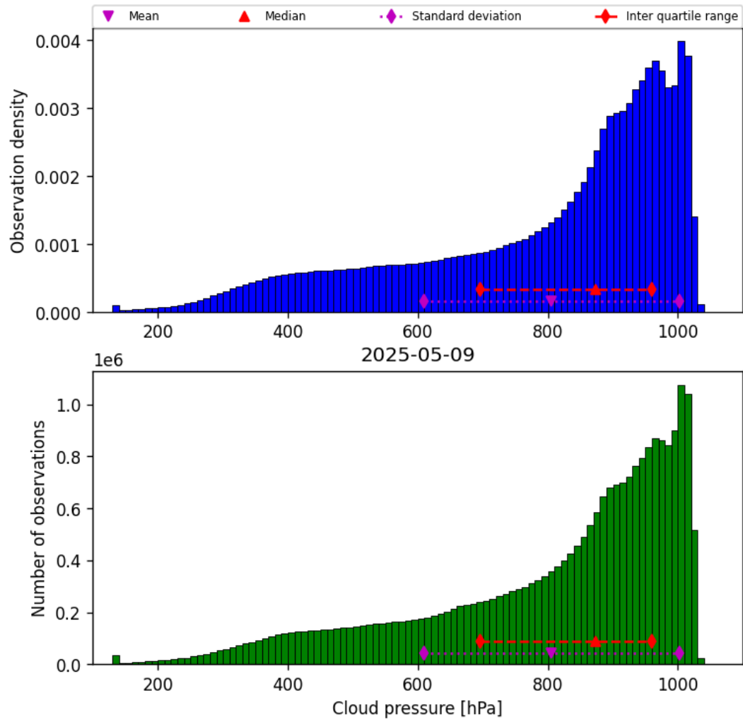
Figure 28: Histogram of “Cloud pressure” for 2025-05-09 to 2025-05-10
