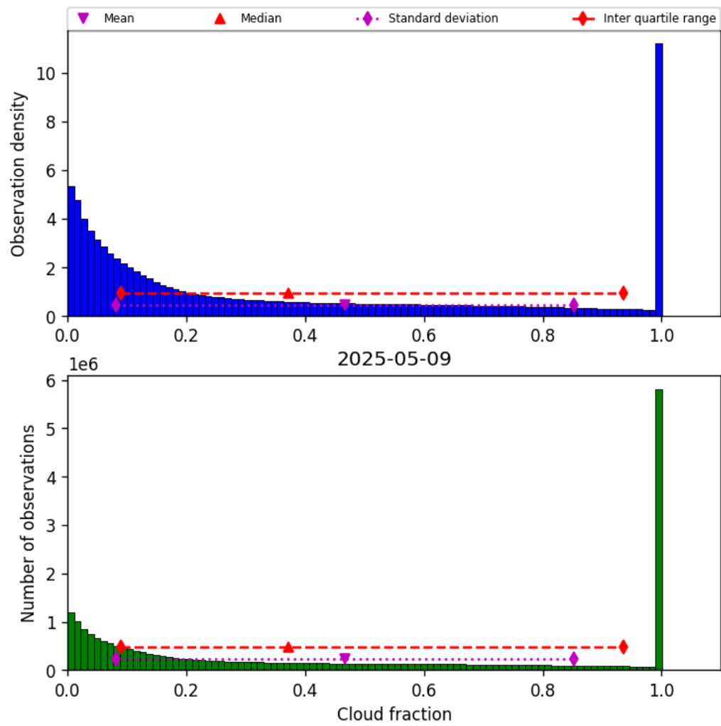
Figure 30: Histogram of “Cloud fraction” for 2025-05-09 to 2025-05-10
