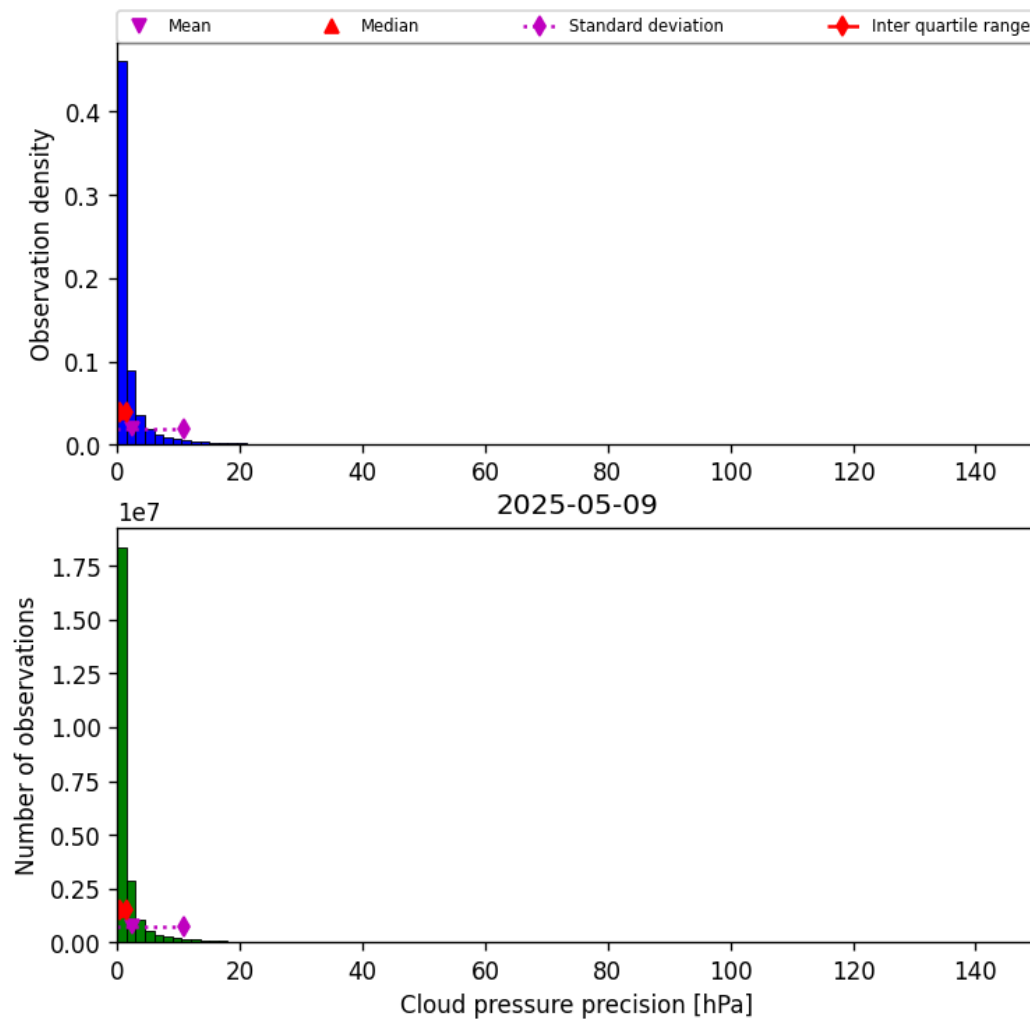
Figure 29: Histogram of “Cloud pressure precision” for 2025-05-09 to 2025-05-10
