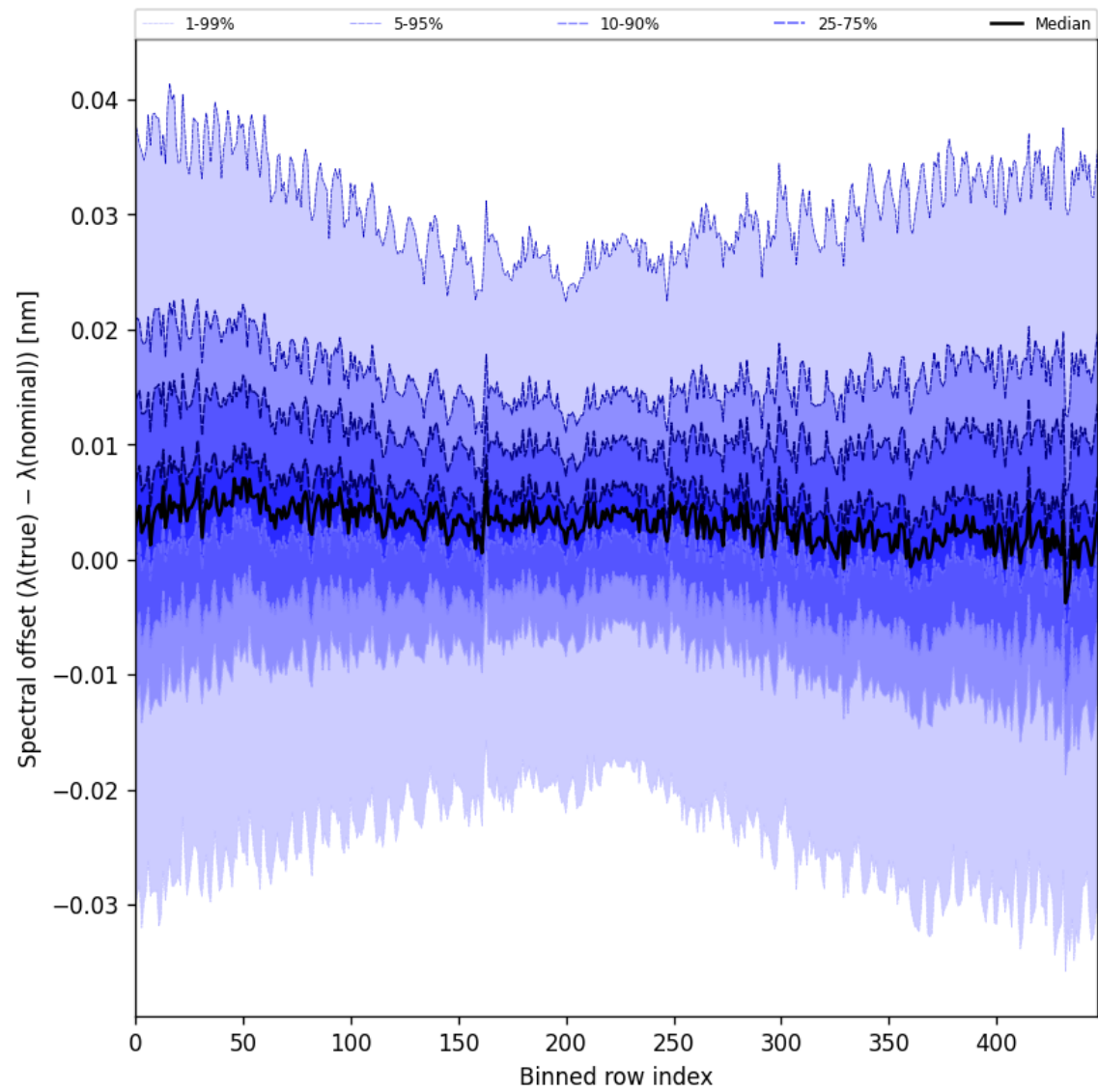
Figure 60: Along track statistics of “Spectral offset ( \lambda_{\text{true}} - \lambda_{\text{nominal}} )” for 2025-05-09 to 2025-05-10
