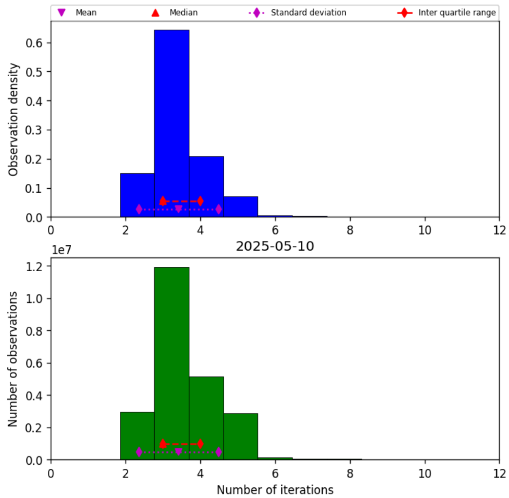
Figure 37: Histogram of “Number of iterations” for 2025-05-10 to 2025-05-11
