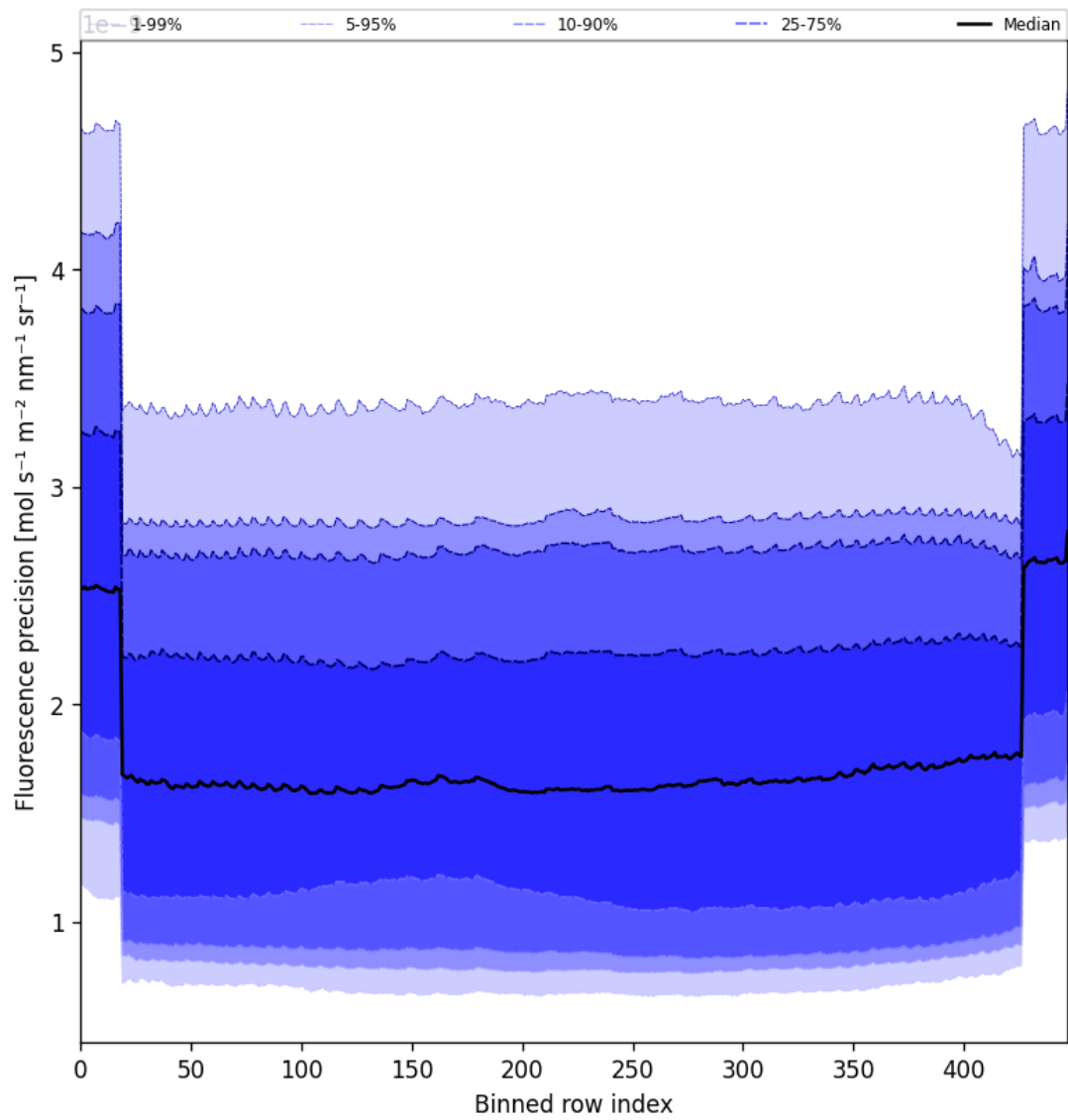
Figure 56: Along track statistics of “Fluorescence precision” for 2025-05-10 to 2025-05-11
