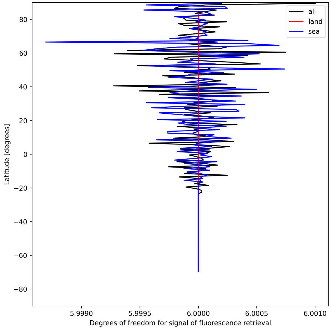
Figure 24: Zonal average of “Degrees of freedom for signal of fluorescence retrieval” for 2025-05-10 to 2025-05-11.
