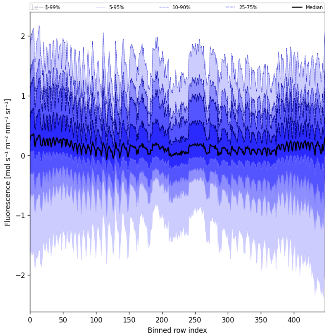
Figure 55: Along track statistics of “Fluorescence” for 2025-05-10 to 2025-05-11
