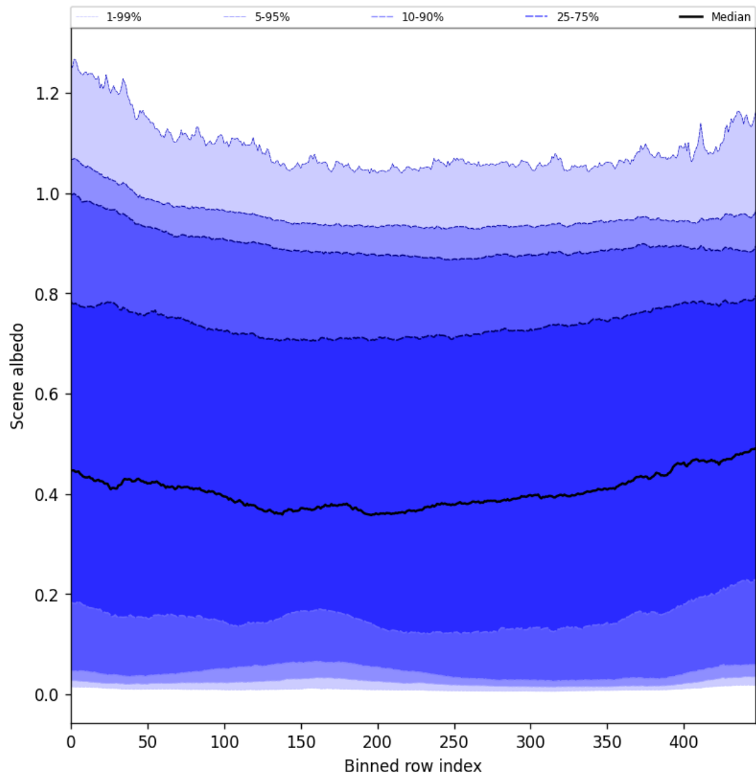
Figure 49: Along track statistics of “Scene albedo” for 2025-05-10 to 2025-05-11
