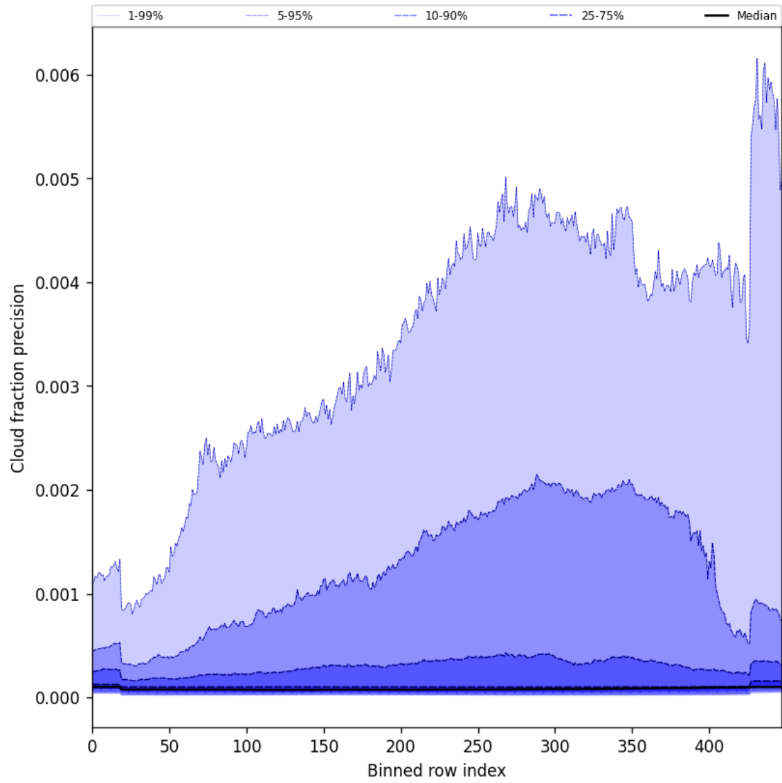
Figure 48: Along track statistics of “Cloud fraction precision” for 2025-05-10 to 2025-05-11
