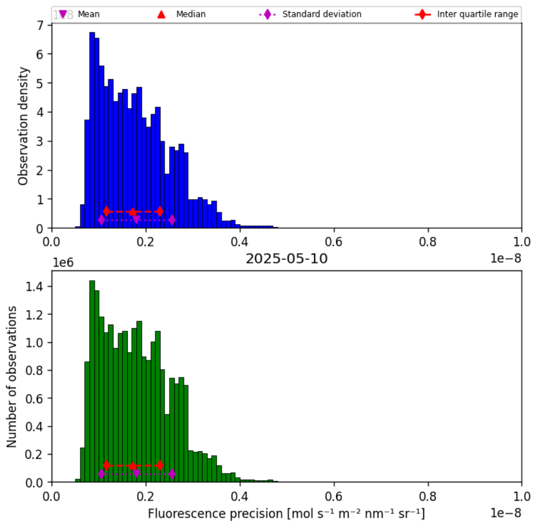
Figure 39: Histogram of “Fluorescence precision” for 2025-05-10 to 2025-05-11
