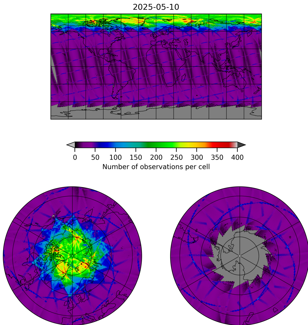
Figure 9: Map of the number of observations for 2025-05-10 to 2025-05-11
