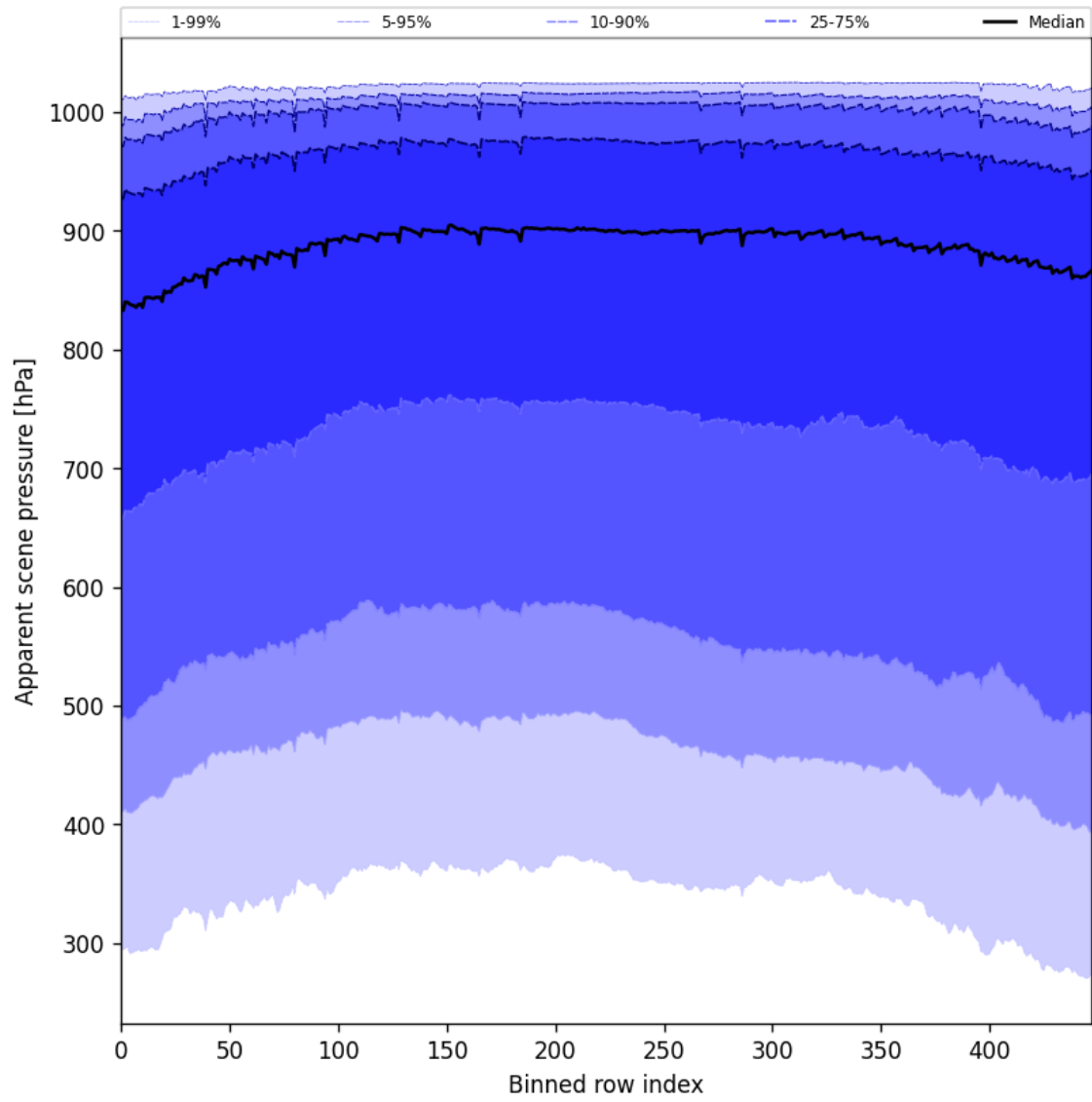
Figure 51: Along track statistics of “Apparent scene pressure” for 2025-05-10 to 2025-05-11
