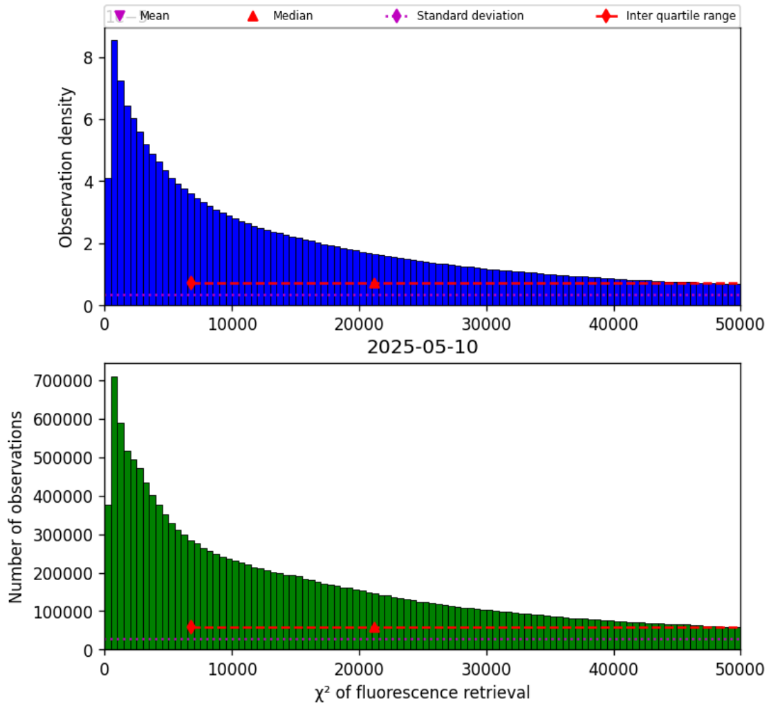
Figure 40: Histogram of “ \chi^2 of fluorescence retrieval” for 2025-05-10 to 2025-05-11
