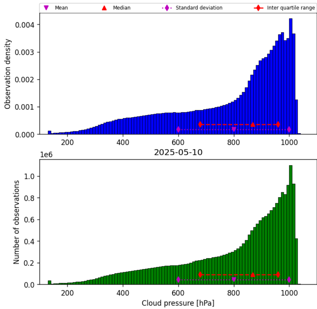
Figure 28: Histogram of “Cloud pressure” for 2025-05-10 to 2025-05-11
