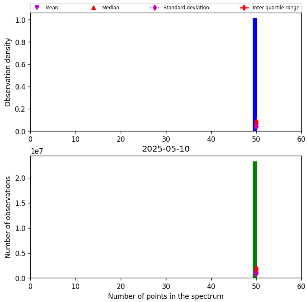
Figure 42: Histogram of “Number of points in the spectrum” for 2025-05-10 to 2025-05-11
