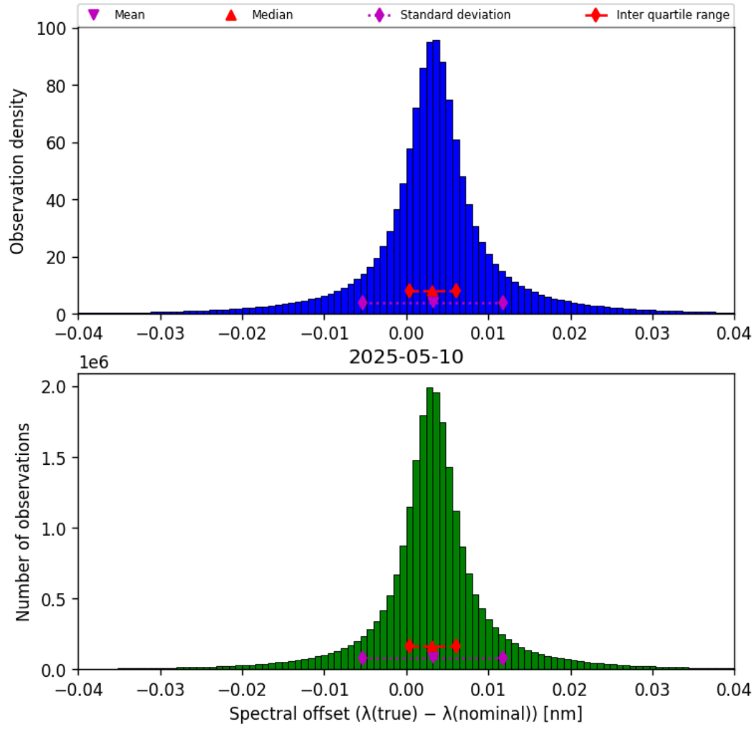
Figure 43: Histogram of “Spectral offset ( \lambda_{\text{true}} - \lambda_{\text{nominal}} )” for 2025-05-10 to 2025-05-11
