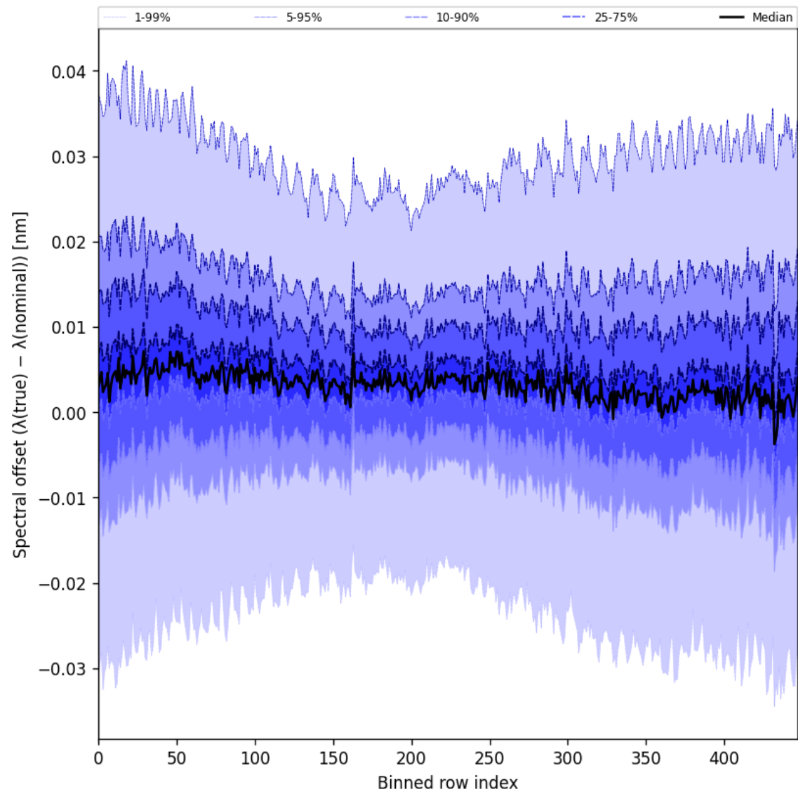
Figure 60: Along track statistics of “Spectral offset ( \lambda_{\text{true}} - \lambda_{\text{nominal}} )” for 2025-05-10 to 2025-05-11
