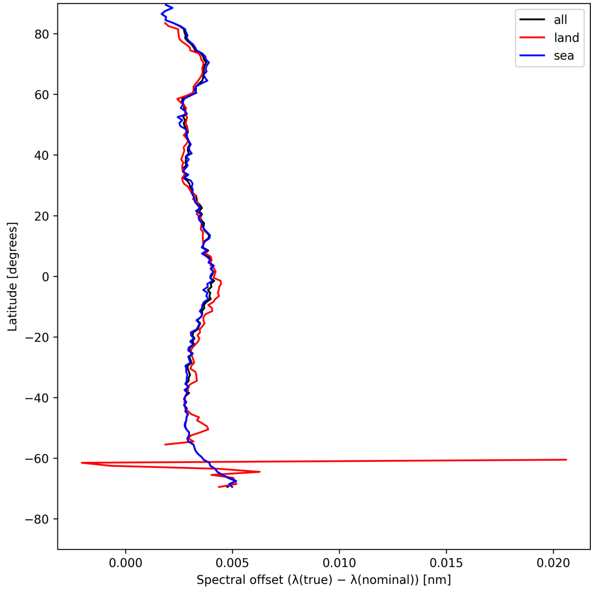
Figure 26: Zonal average of “Spectral offset ( \lambda_{\text{true}} - \lambda_{\text{nominal}} )” for 2025-05-10 to 2025-05-11.
