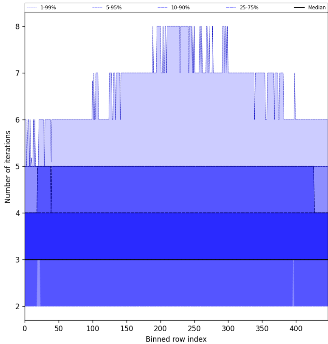
Figure 54: Along track statistics of “Number of iterations” for 2025-05-10 to 2025-05-11
