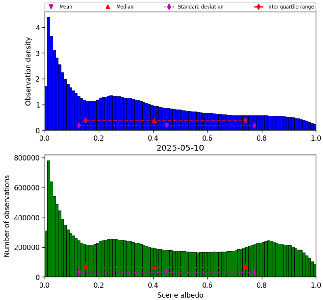
Figure 32: Histogram of “Scene albedo” for 2025-05-10 to 2025-05-11
