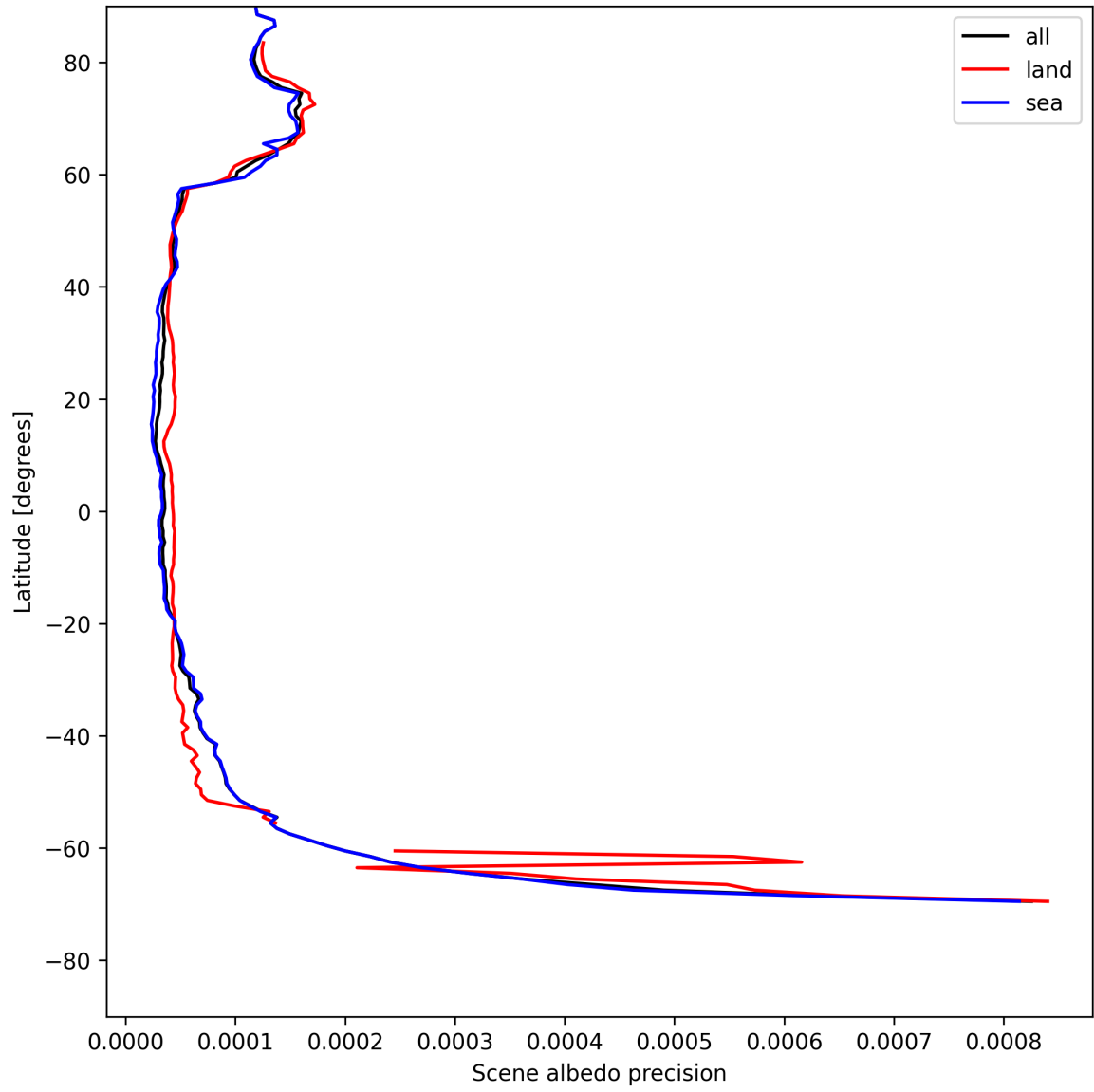
Figure 16: Zonal average of "Scene albedo precision" for 2025-05-10 to 2025-05-11.
