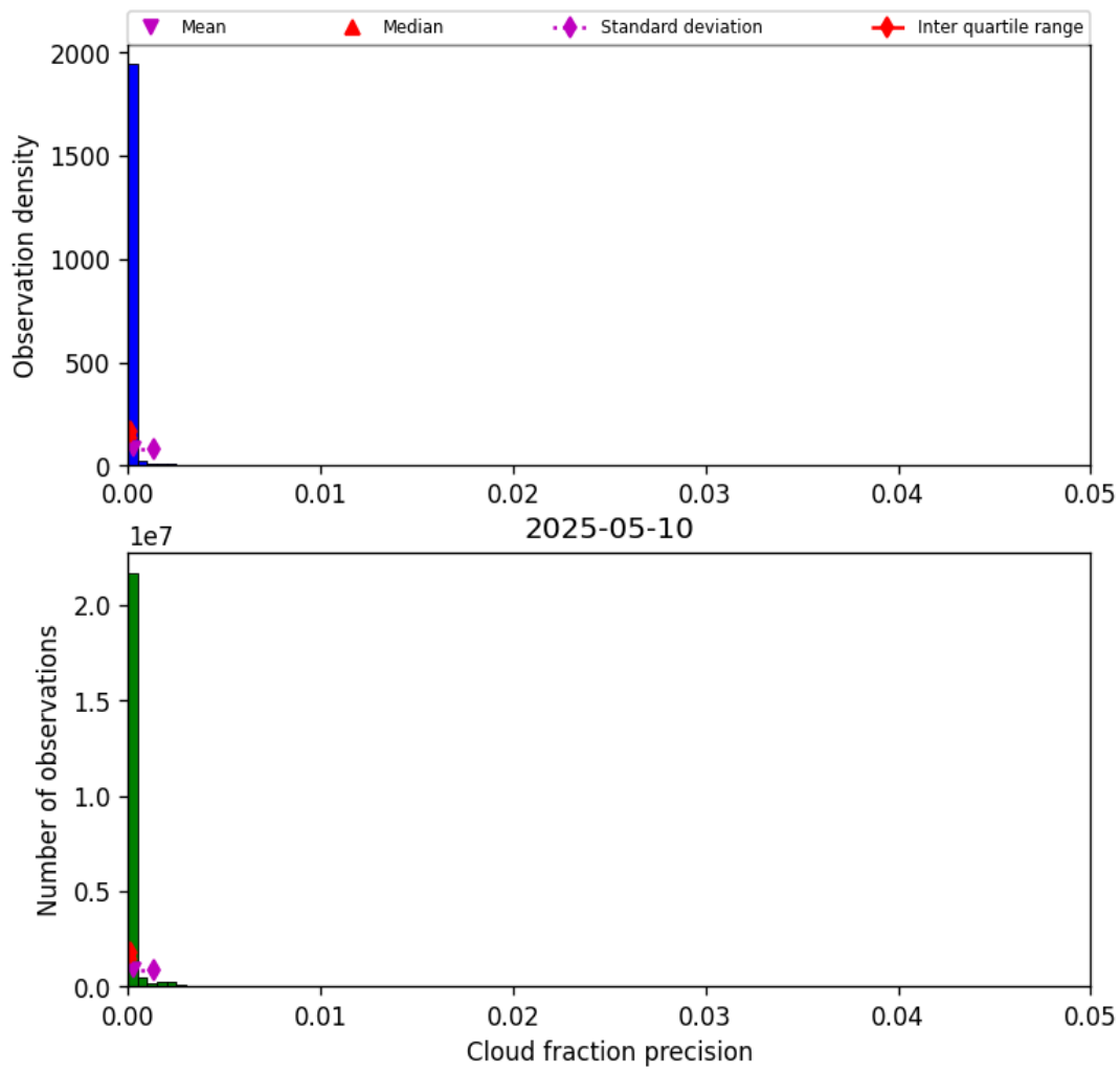
Figure 31: Histogram of “Cloud fraction precision” for 2025-05-10 to 2025-05-11
