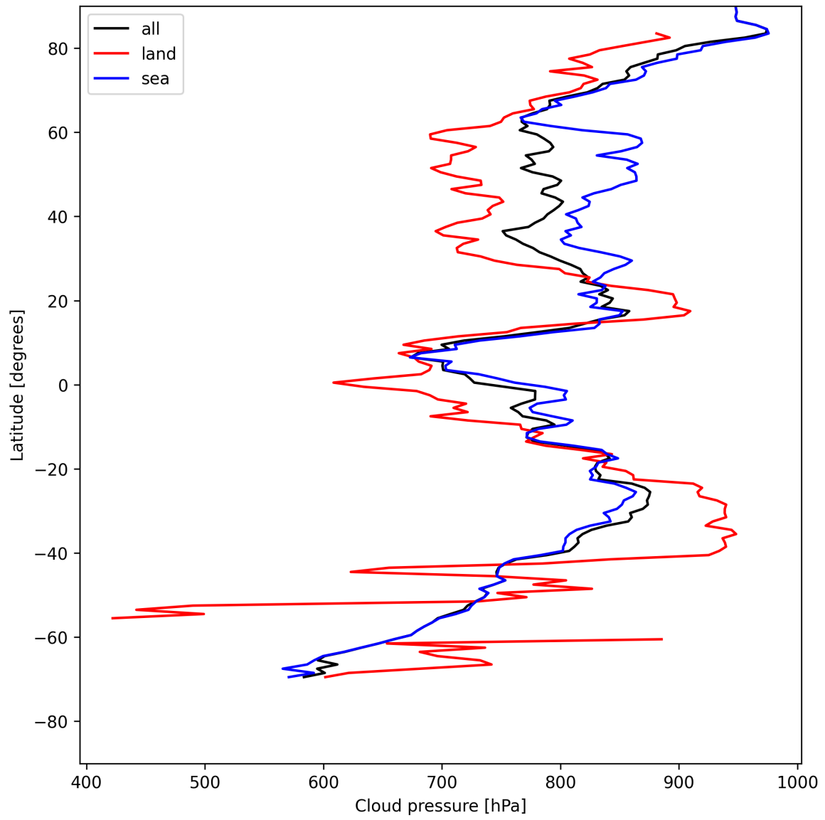
Figure 11: Zonal average of “Cloud pressure” for 2025-05-10 to 2025-05-11.
