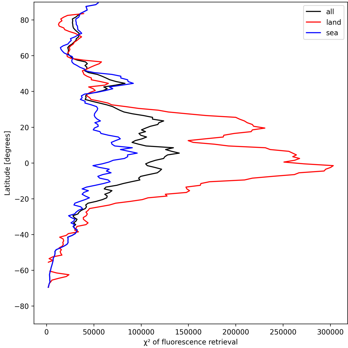
Figure 23: Zonal average of “ \chi^2 of fluorescence retrieval” for 2025-05-10 to 2025-05-11.
