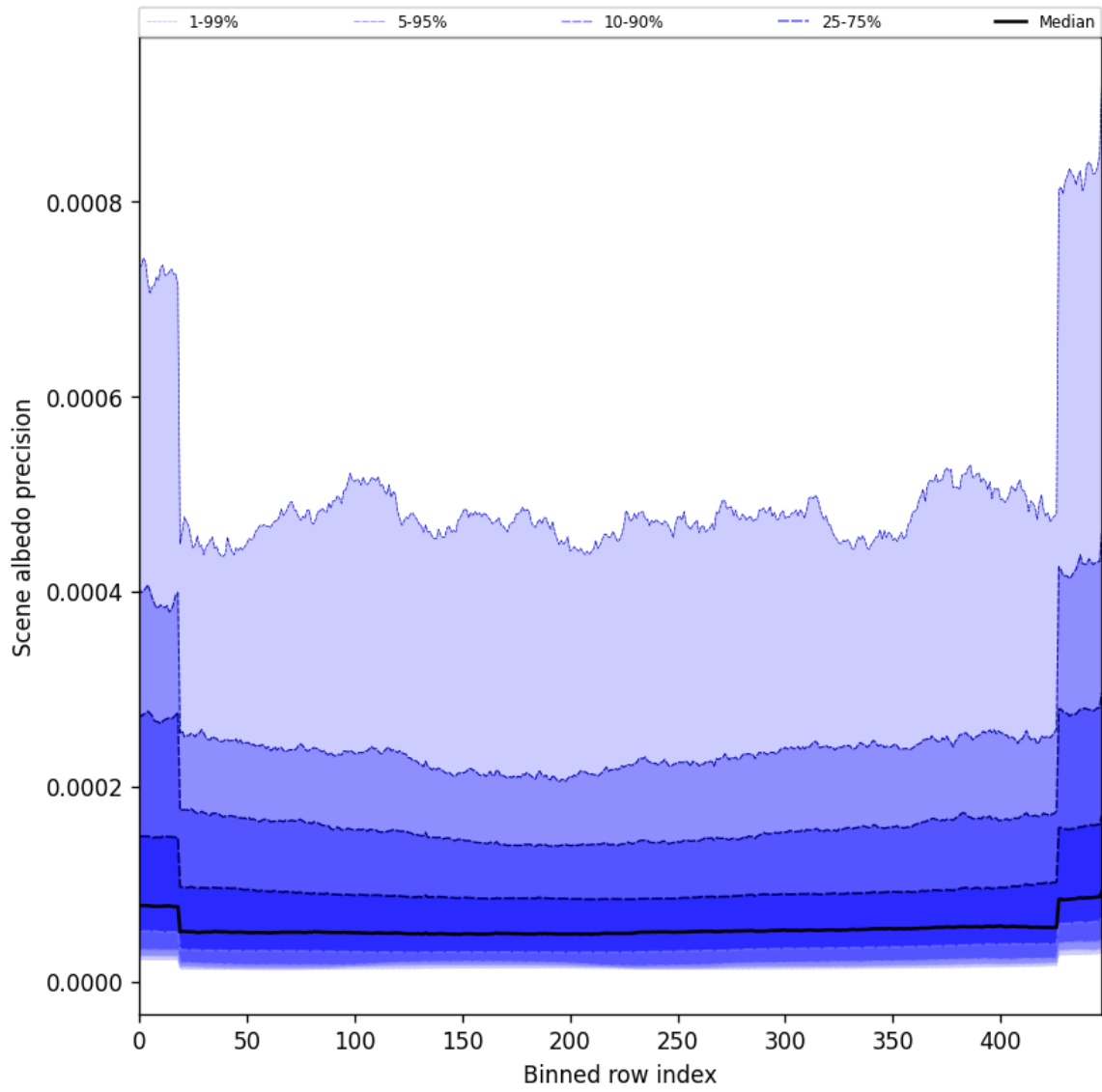
Figure 50: Along track statistics of “Scene albedo precision” for 2025-05-10 to 2025-05-11
