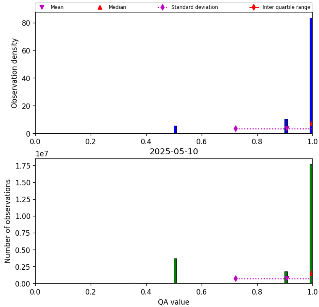
Figure 27: Histogram of “QA value” for 2025-05-10 to 2025-05-11
