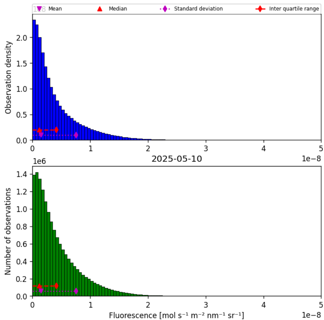
Figure 38: Histogram of “Fluorescence” for 2025-05-10 to 2025-05-11
