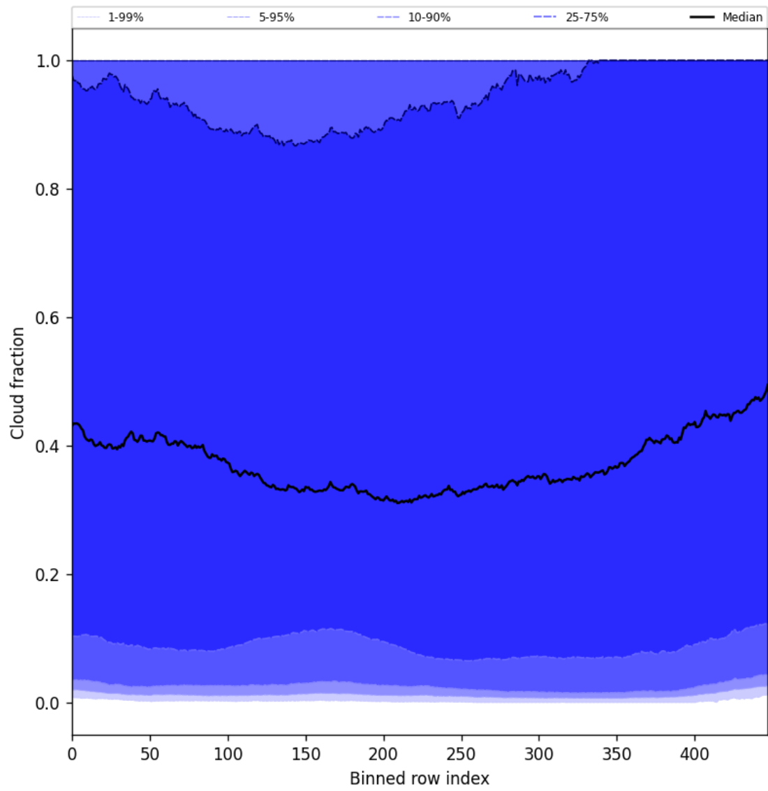
Figure 47: Along track statistics of “Cloud fraction” for 2025-05-10 to 2025-05-11
