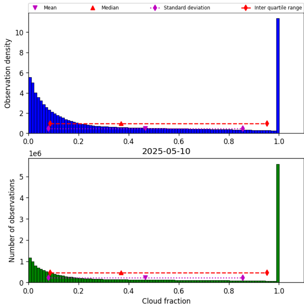
Figure 30: Histogram of “Cloud fraction” for 2025-05-10 to 2025-05-11
