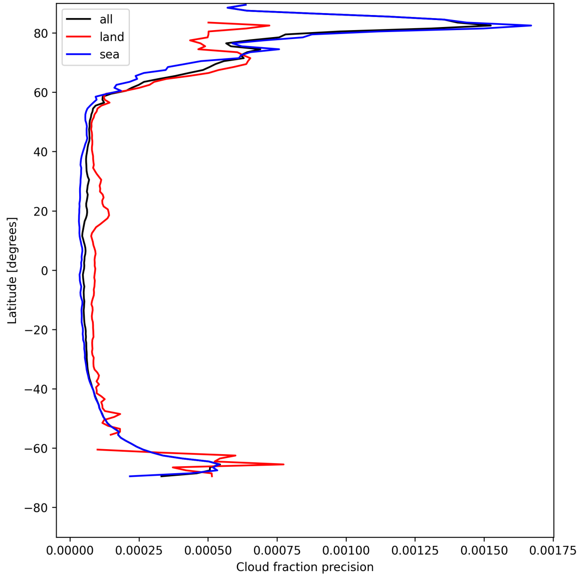
Figure 14: Zonal average of “Cloud fraction precision” for 2025-05-10 to 2025-05-11.
