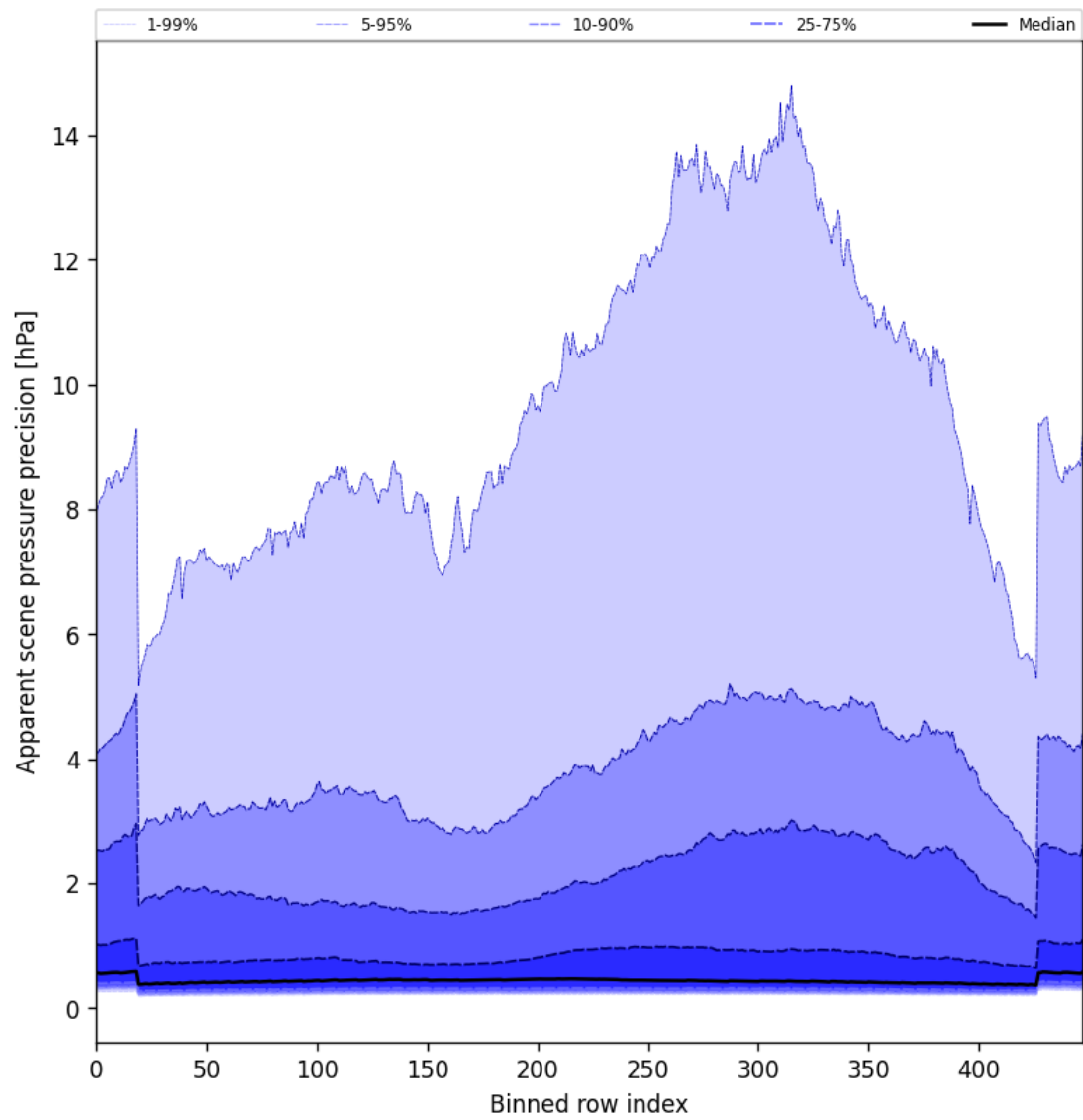
Figure 52: Along track statistics of “Apparent scene pressure precision” for 2025-05-10 to 2025-05-11
