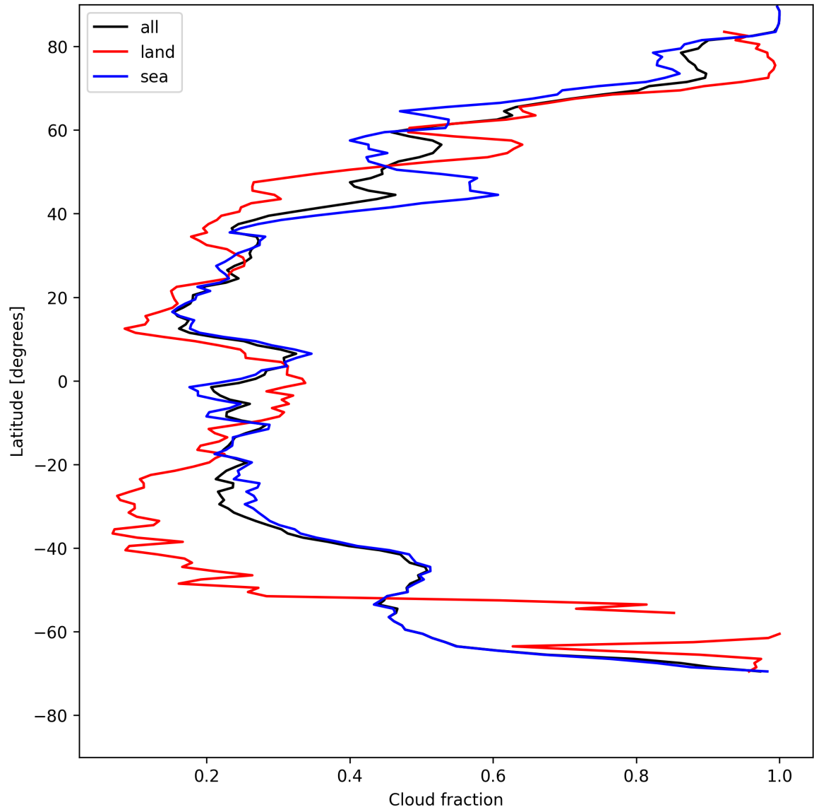
Figure 13: Zonal average of “Cloud fraction” for 2025-05-10 to 2025-05-11.
