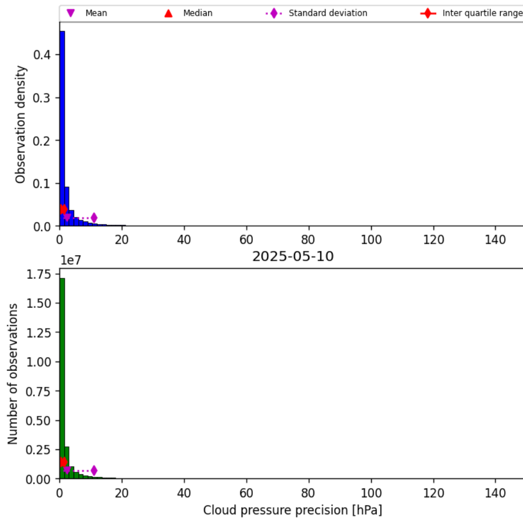
Figure 29: Histogram of "Cloud pressure precision" for 2025-05-10 to 2025-05-11
