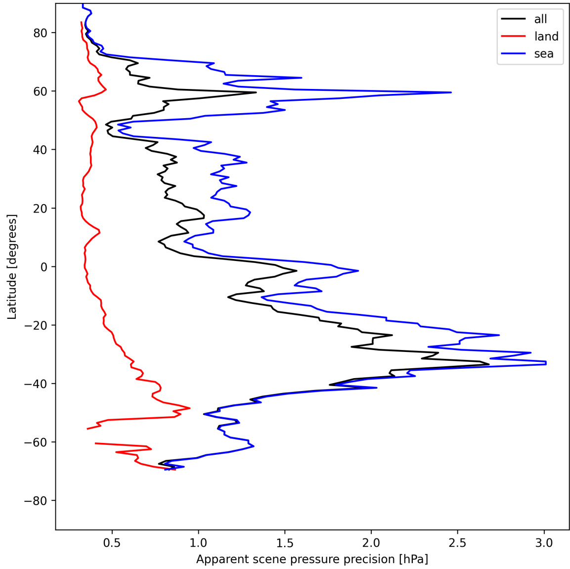
Figure 18: Zonal average of “Apparent scene pressure precision” for 2025-05-10 to 2025-05-11.
