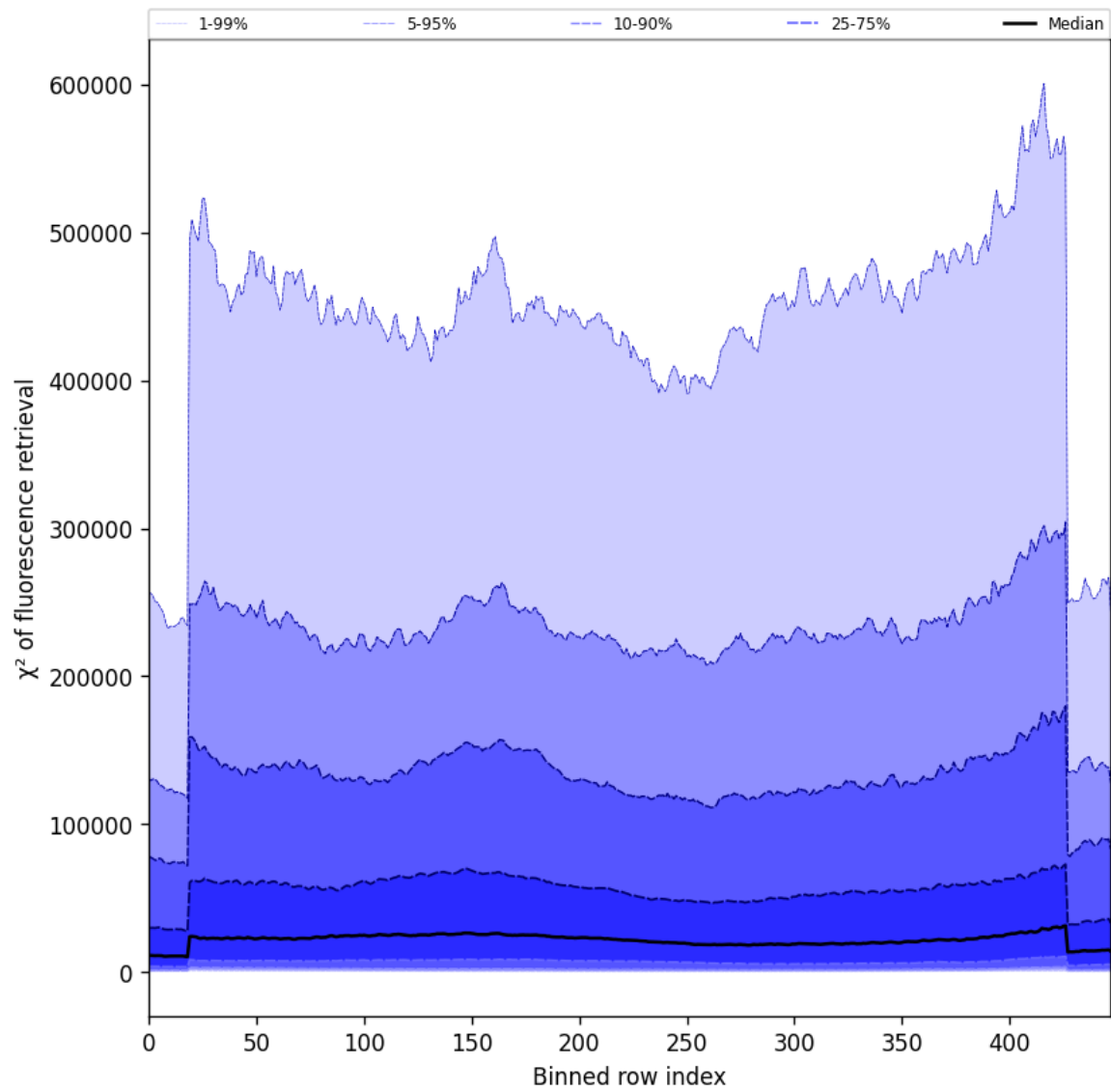
Figure 57: Along track statistics of “ \chi^2 of fluorescence retrieval” for 2025-05-10 to 2025-05-11
