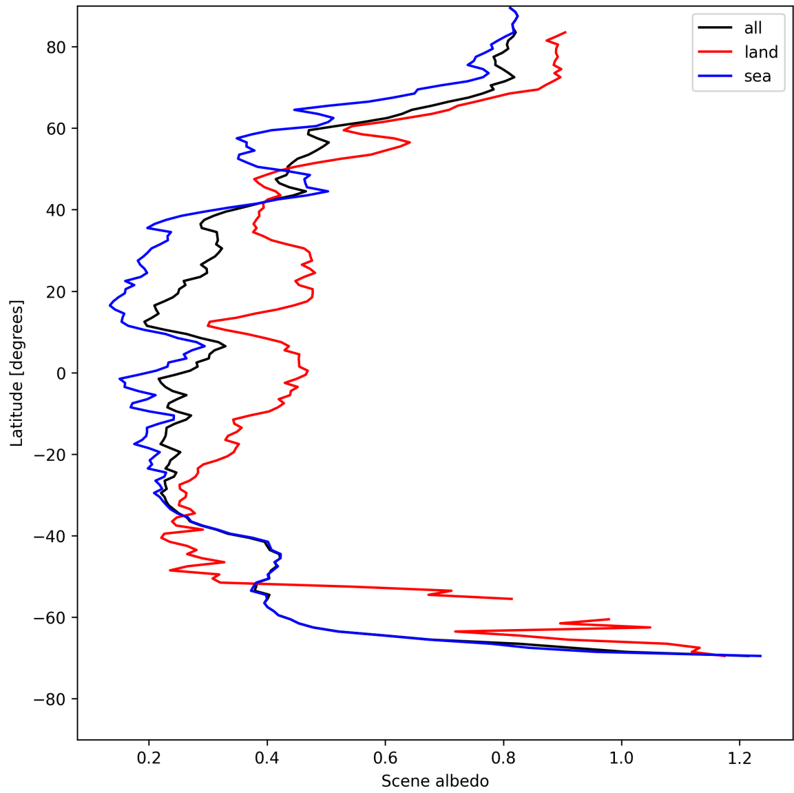
Figure 15: Zonal average of “Scene albedo” for 2025-05-10 to 2025-05-11.
