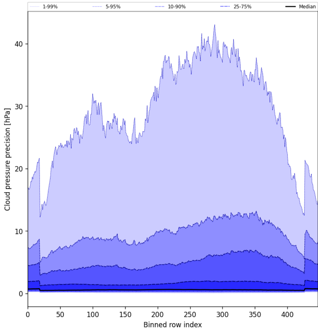
Figure 46: Along track statistics of “Cloud pressure precision” for 2025-05-10 to 2025-05-11
