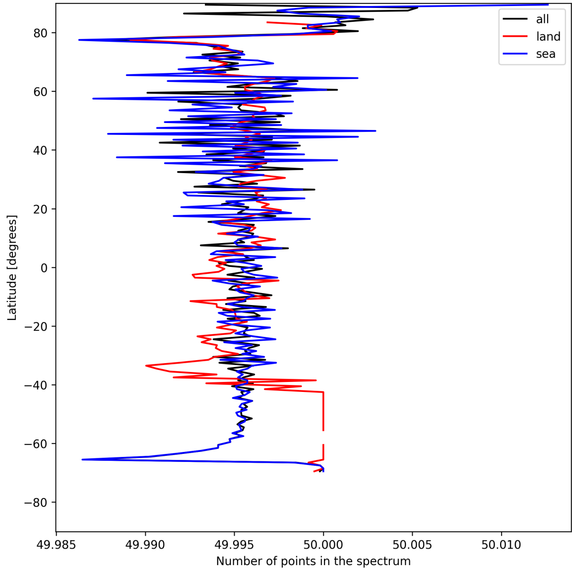
Figure 25: Zonal average of “Number of points in the spectrum” for 2025-05-10 to 2025-05-11.
