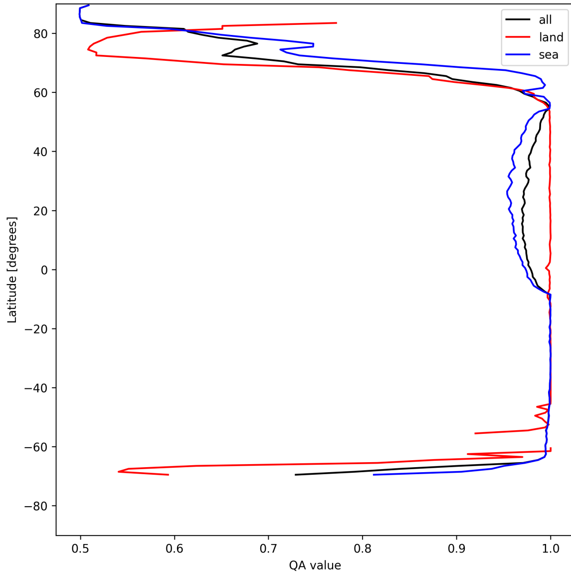
Figure 10: Zonal average of “QA value” for 2025-05-10 to 2025-05-11.
