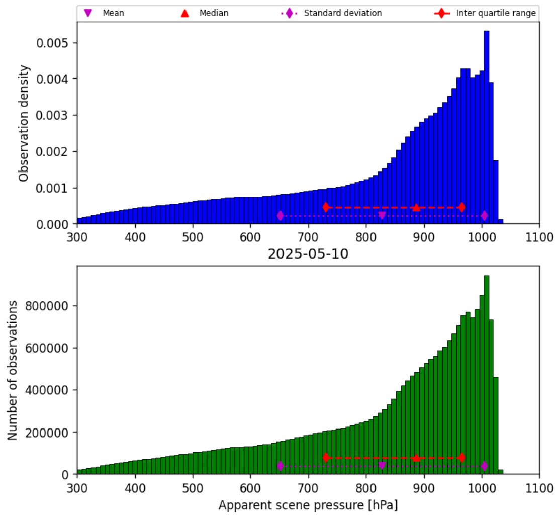
Figure 34: Histogram of “Apparent scene pressure” for 2025-05-10 to 2025-05-11
