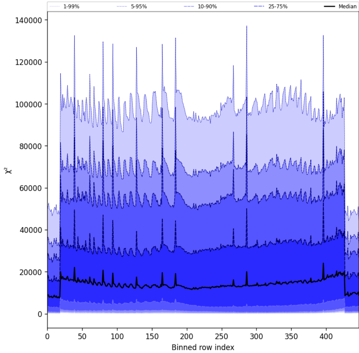
Figure 53: Along track statistics of “ \chi^2 ” for 2025-05-10 to 2025-05-11
