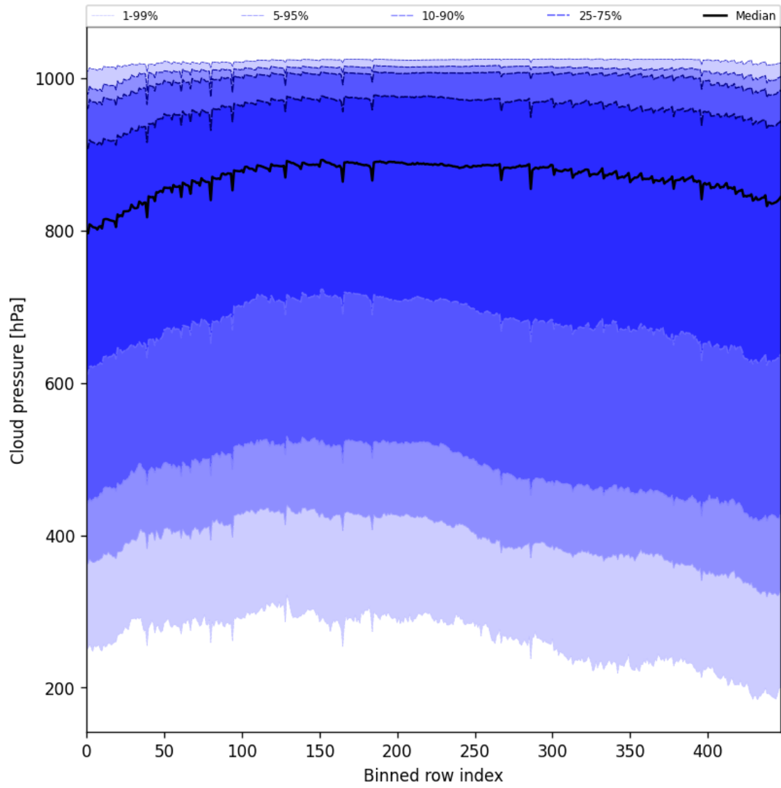
Figure 45: Along track statistics of “Cloud pressure” for 2025-05-10 to 2025-05-11
