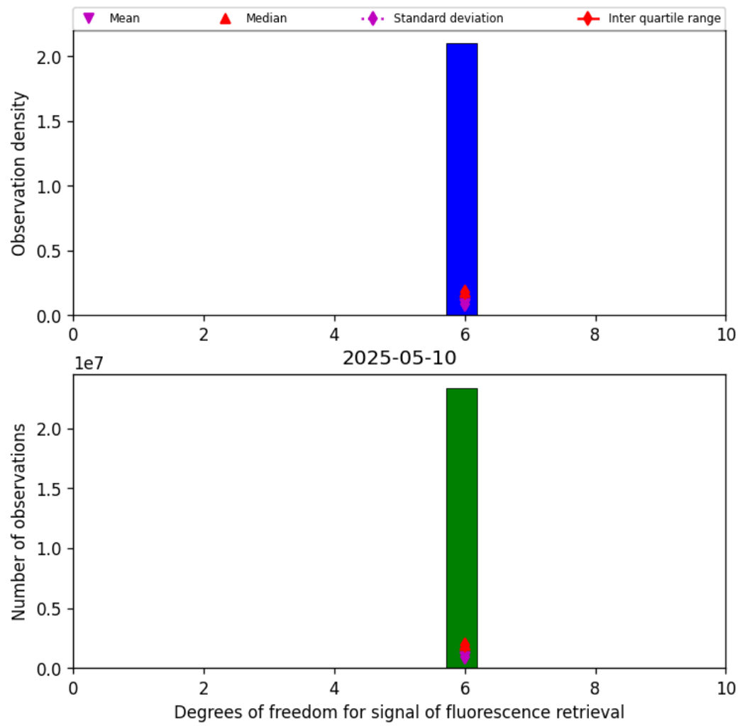
Figure 41: Histogram of “Degrees of freedom for signal of fluorescence retrieval” for 2025-05-10 to 2025-05-11
