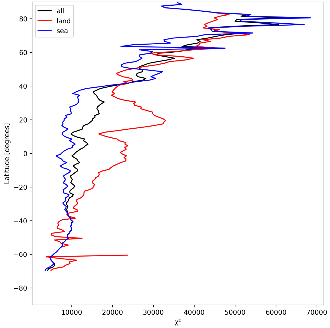
Figure 19: Zonal average of “ \chi^2 ” for 2025-05-10 to 2025-05-11.
