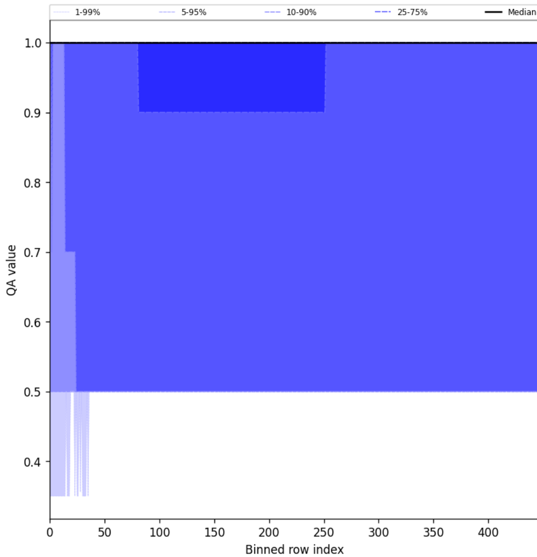
Figure 44: Along track statistics of “QA value” for 2025-05-10 to 2025-05-11
