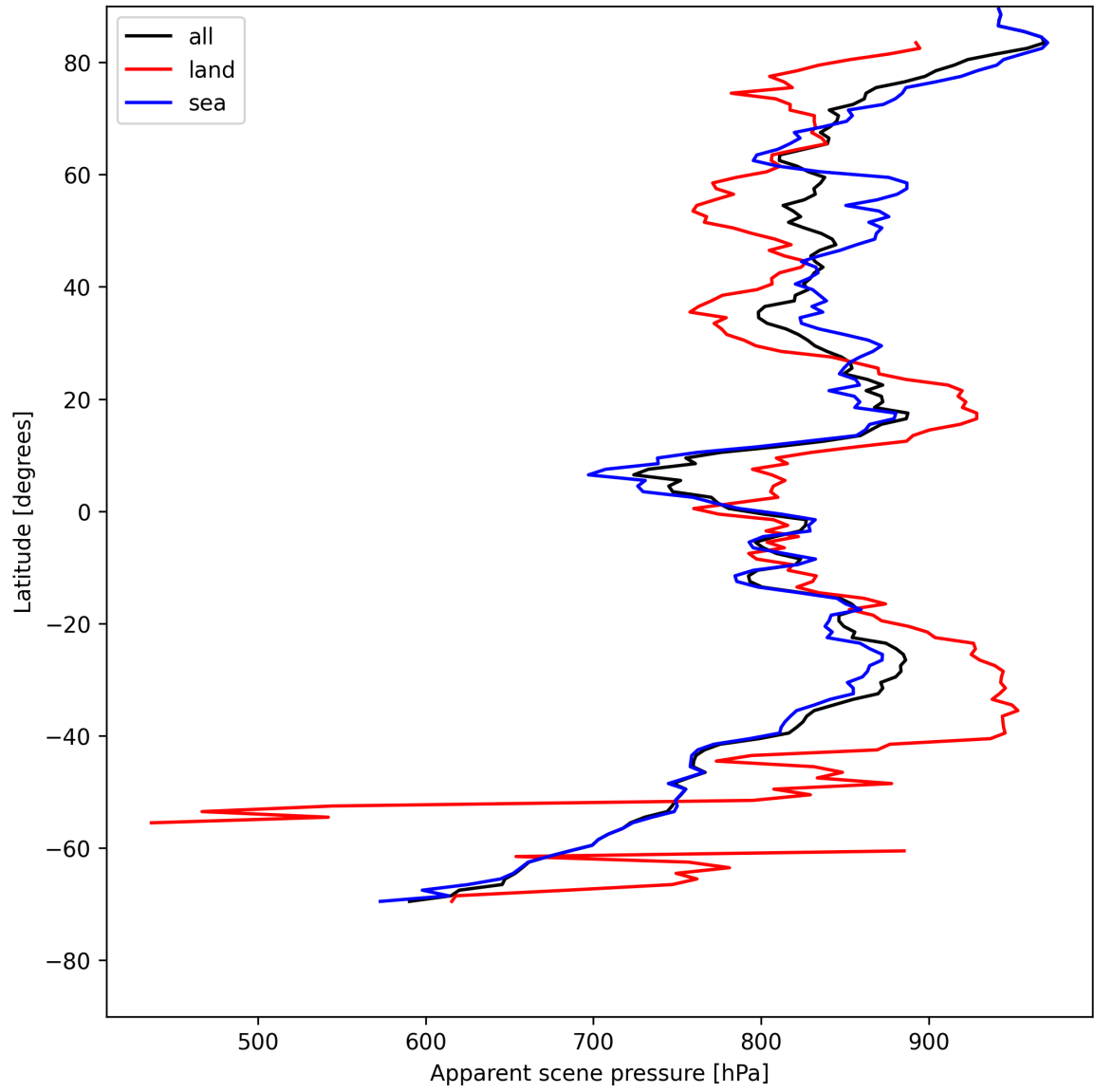
Figure 17: Zonal average of “Apparent scene pressure” for 2025-05-10 to 2025-05-11.
