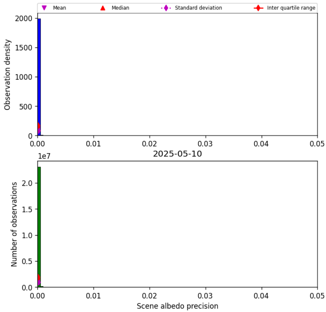
Figure 33: Histogram of “Scene albedo precision” for 2025-05-10 to 2025-05-11
