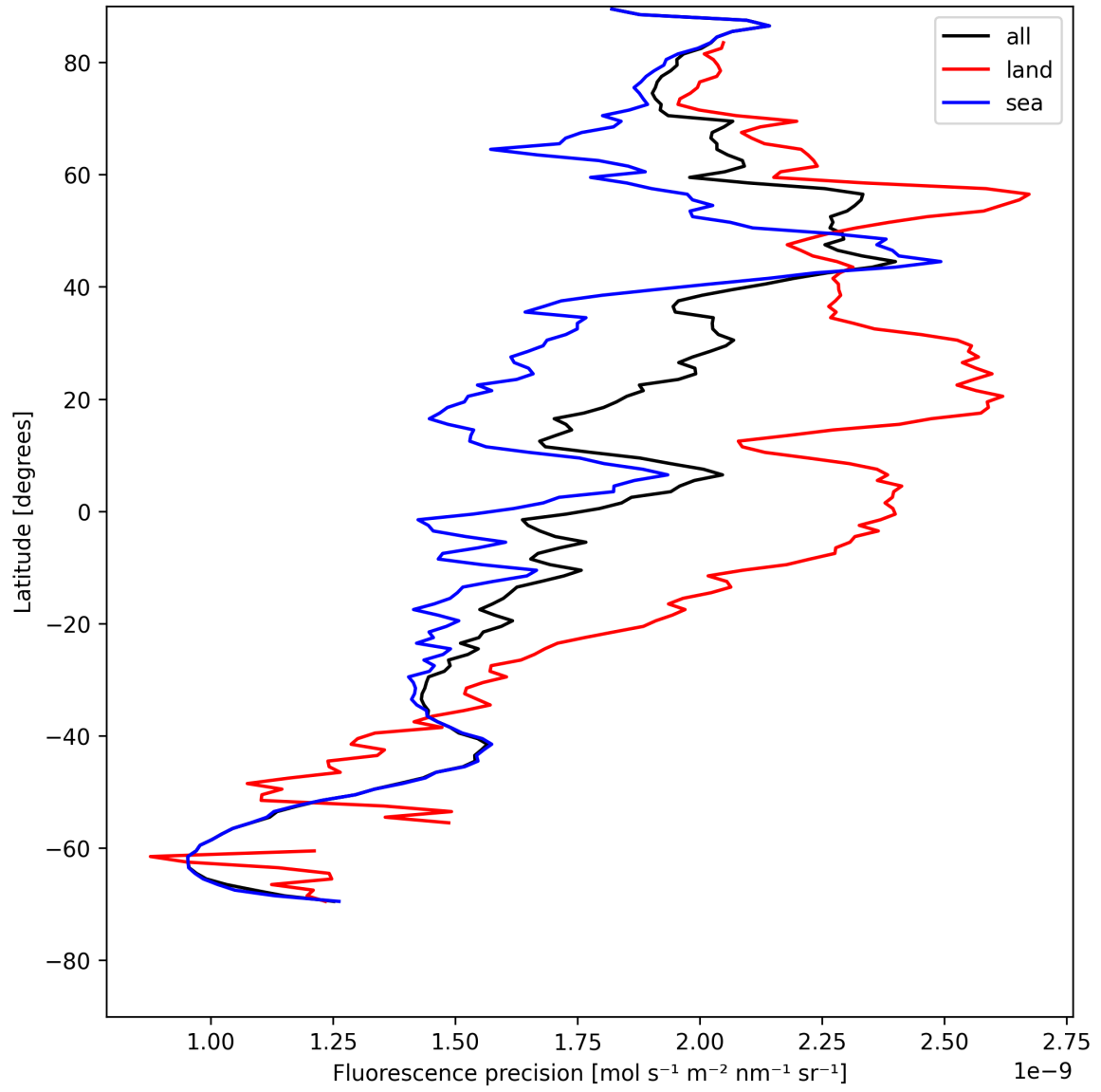
Figure 22: Zonal average of “Fluorescence precision” for 2025-05-10 to 2025-05-11.
