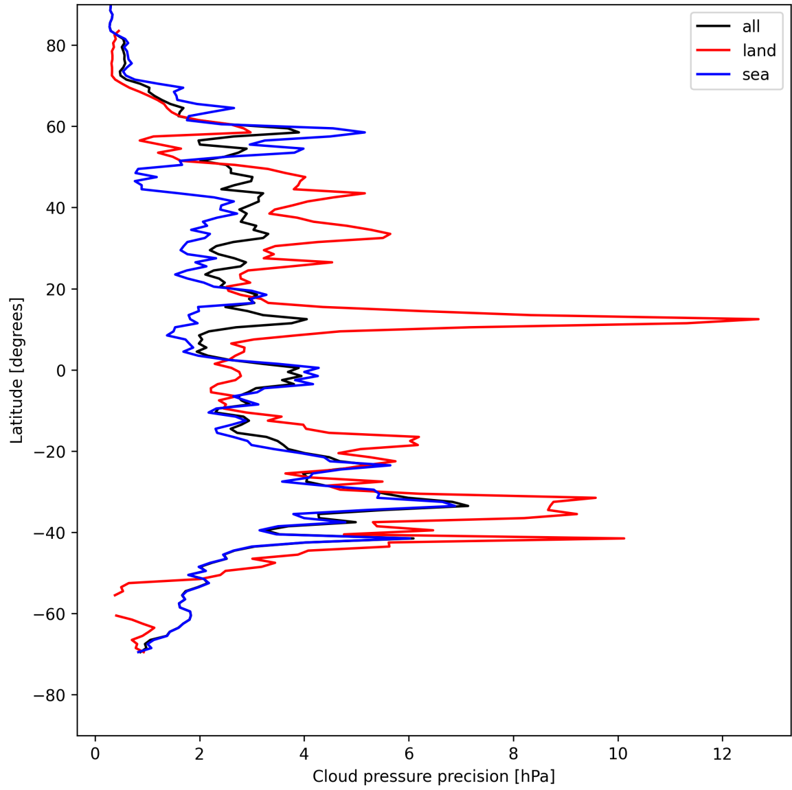
Figure 12: Zonal average of “Cloud pressure precision” for 2025-05-10 to 2025-05-11.
