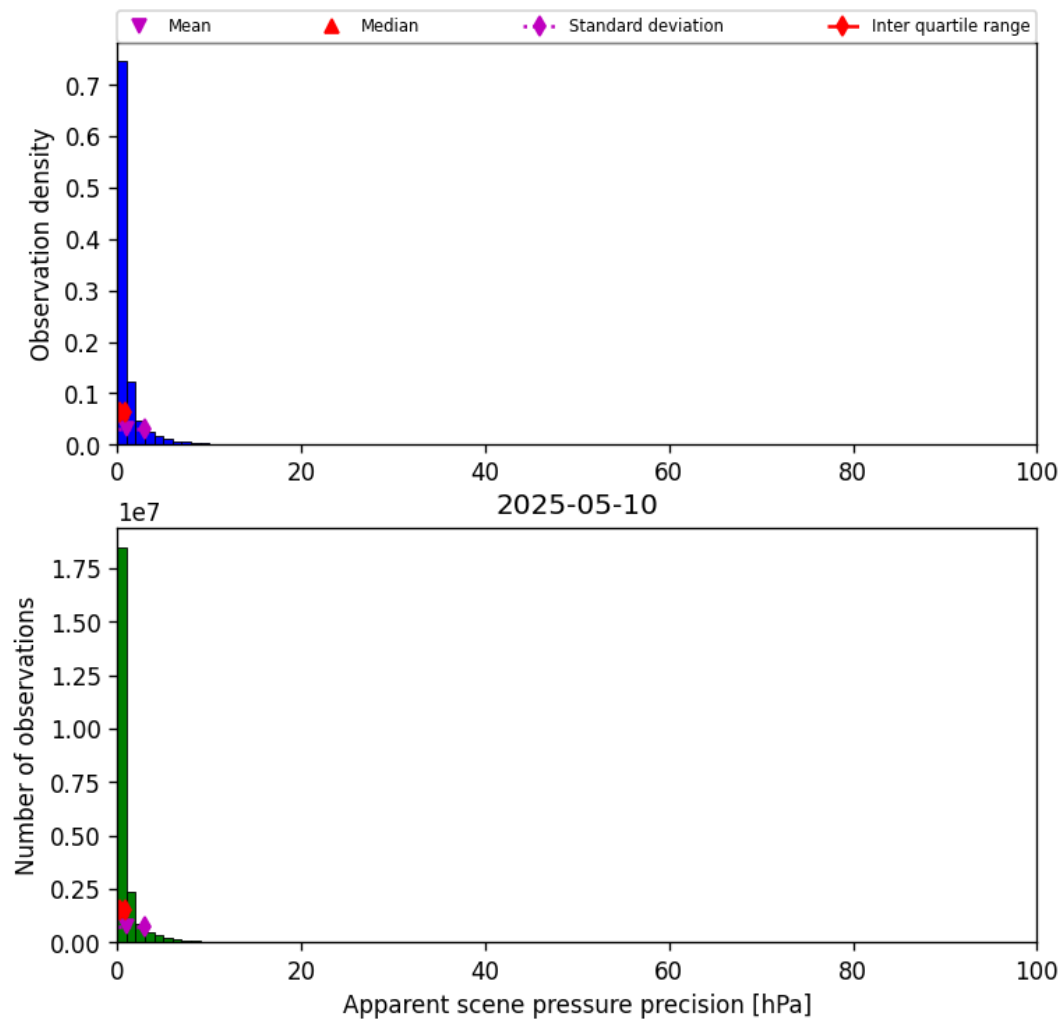
Figure 35: Histogram of “Apparent scene pressure precision” for 2025-05-10 to 2025-05-11
