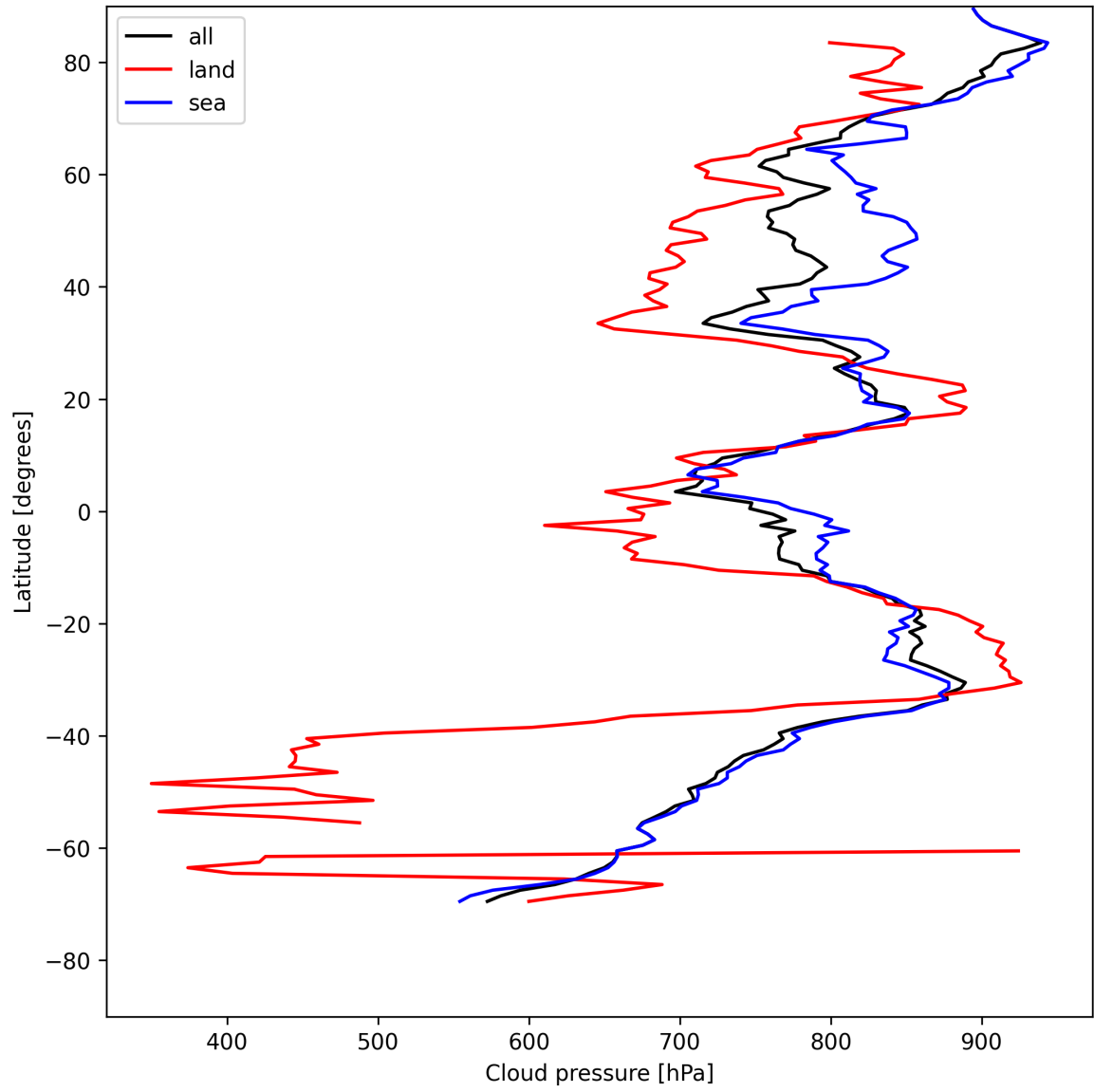
Figure 11: Zonal average of “Cloud pressure” for 2025-05-11 to 2025-05-12.
