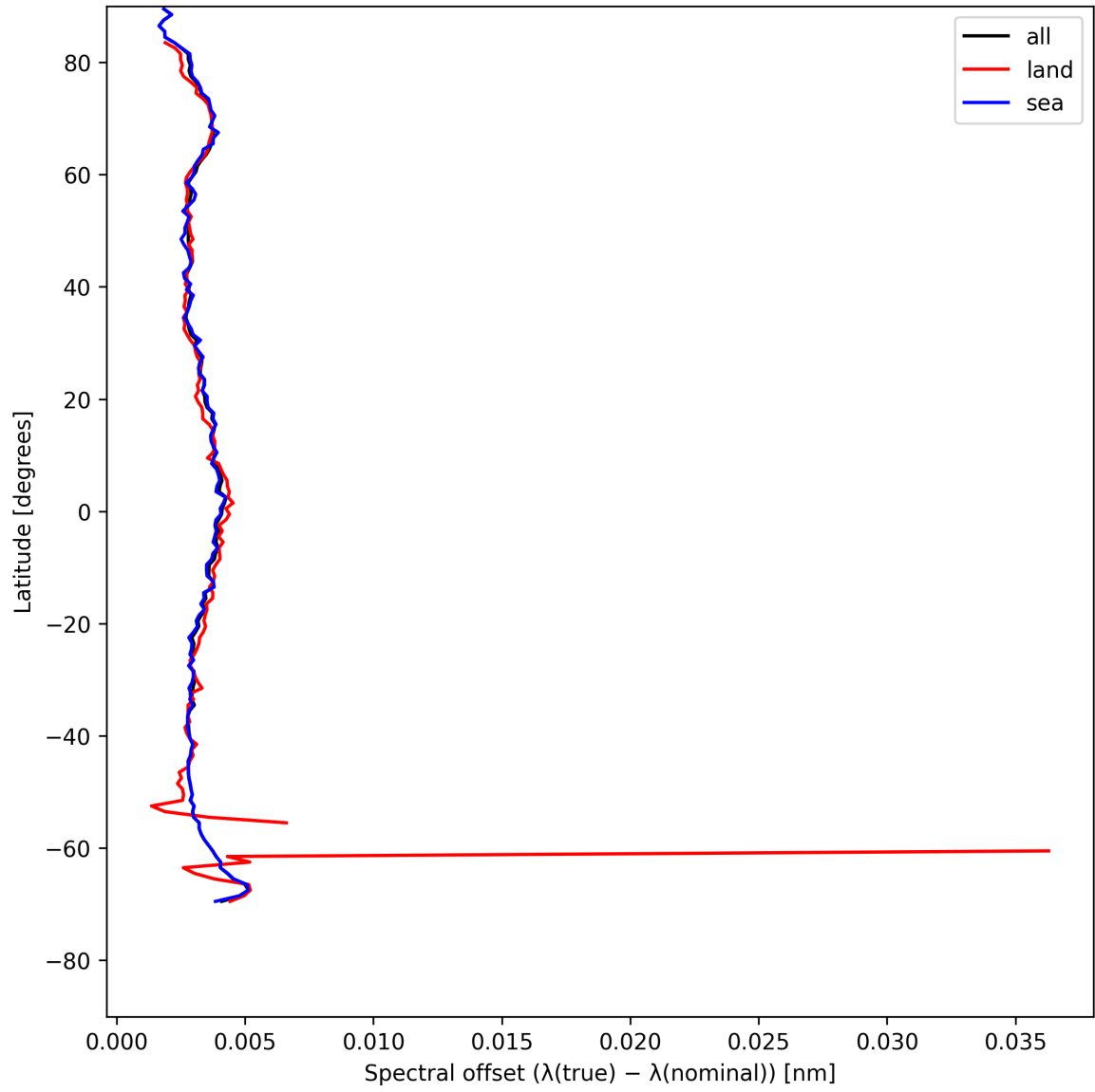
Figure 26: Zonal average of “Spectral offset ( \lambda_{\text{true}} - \lambda_{\text{nominal}} )” for 2025-05-11 to 2025-05-12.
