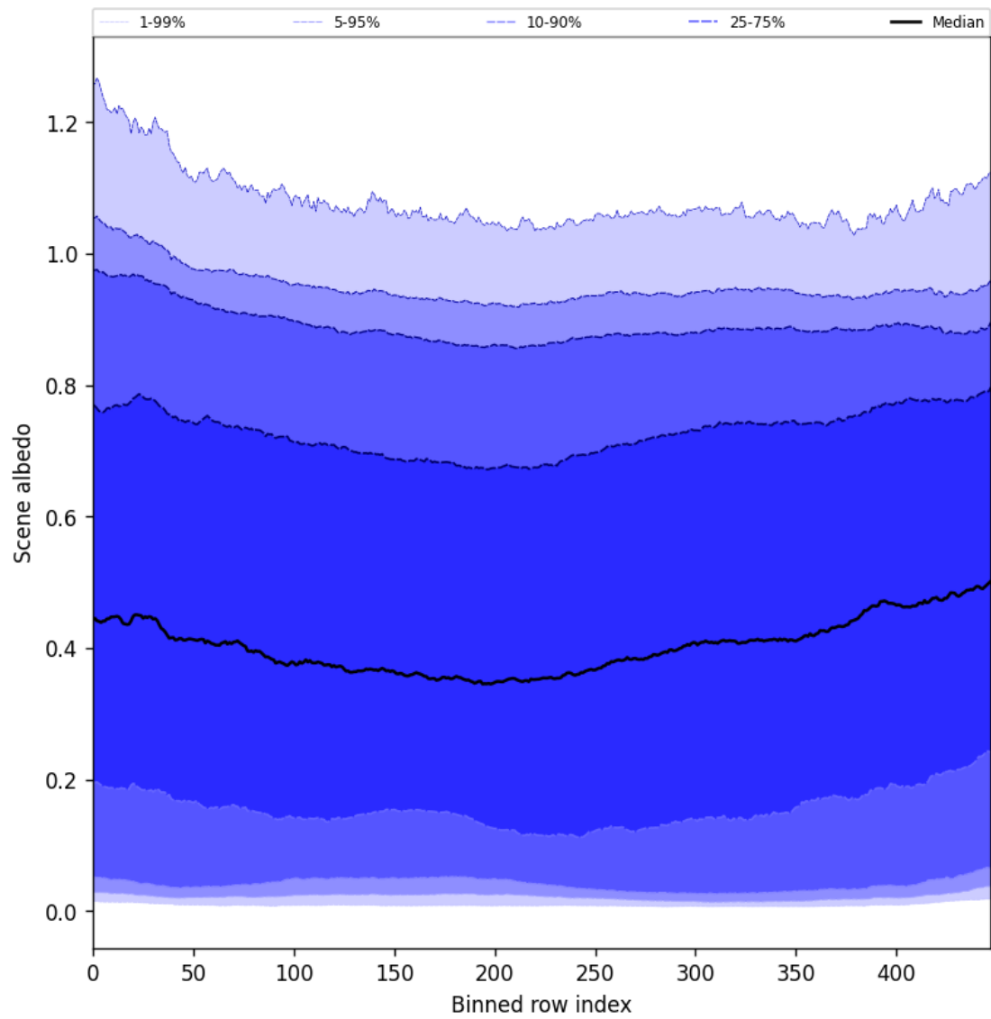
Figure 49: Along track statistics of “Scene albedo” for 2025-05-11 to 2025-05-12
