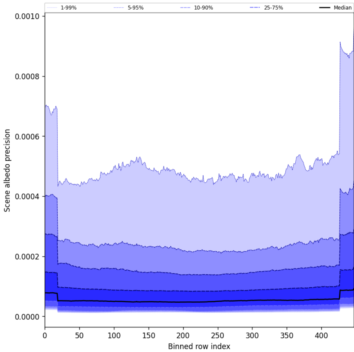
Figure 50: Along track statistics of “Scene albedo precision” for 2025-05-11 to 2025-05-12
