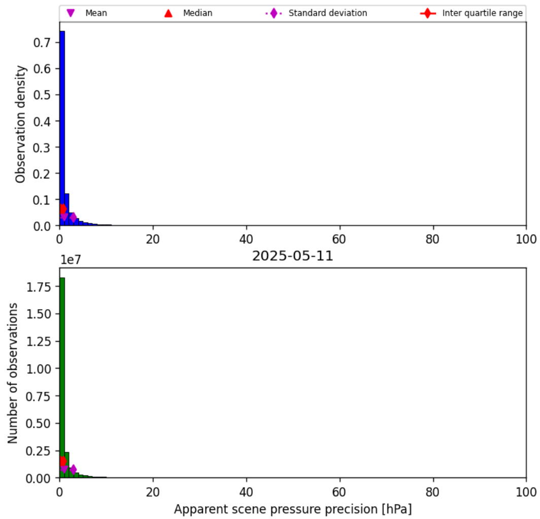
Figure 35: Histogram of “Apparent scene pressure precision” for 2025-05-11 to 2025-05-12
