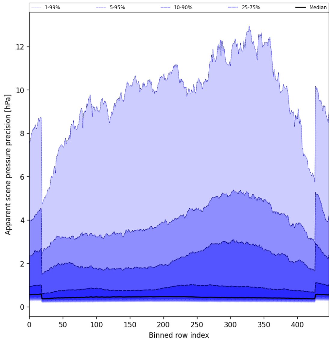
Figure 52: Along track statistics of “Apparent scene pressure precision” for 2025-05-11 to 2025-05-12
