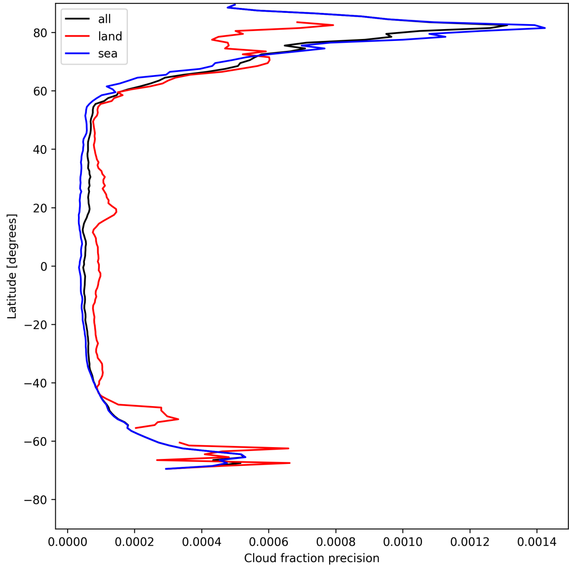
Figure 14: Zonal average of “Cloud fraction precision” for 2025-05-11 to 2025-05-12.
