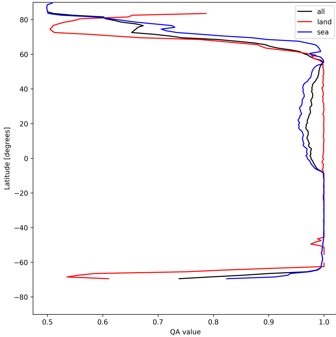
Figure 10: Zonal average of “QA value” for 2025-05-11 to 2025-05-12.
