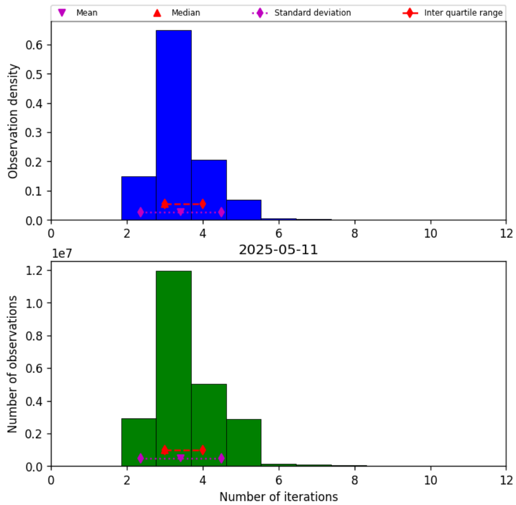
Figure 37: Histogram of “Number of iterations” for 2025-05-11 to 2025-05-12
