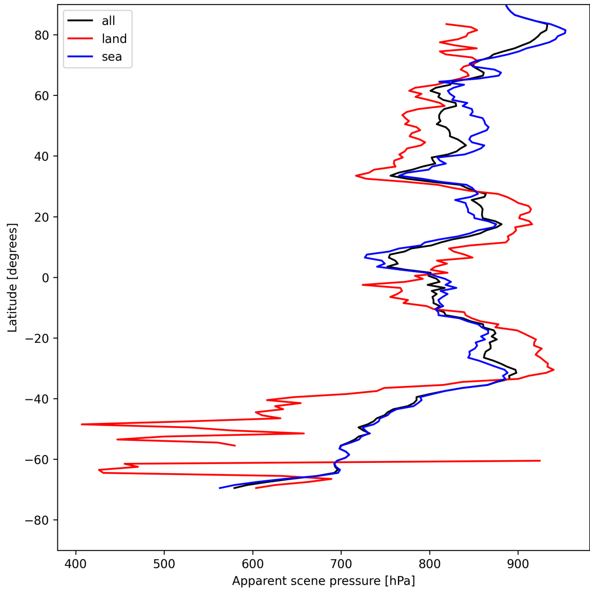
Figure 17: Zonal average of “Apparent scene pressure” for 2025-05-11 to 2025-05-12.
