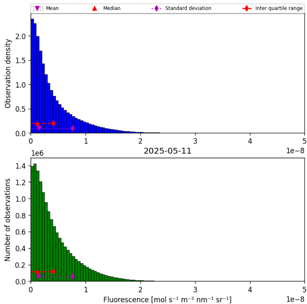
Figure 38: Histogram of “Fluorescence” for 2025-05-11 to 2025-05-12
