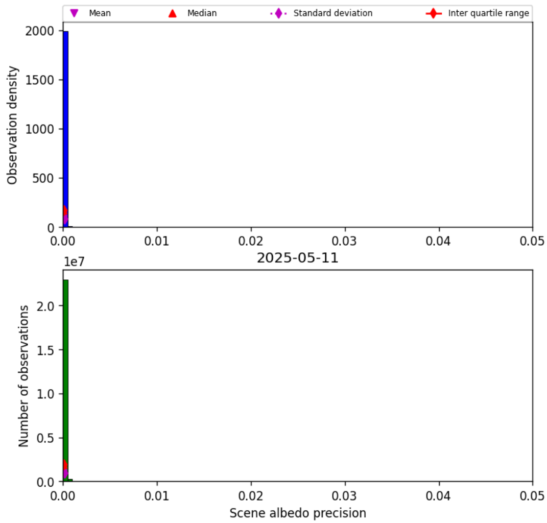
Figure 33: Histogram of “Scene albedo precision” for 2025-05-11 to 2025-05-12
