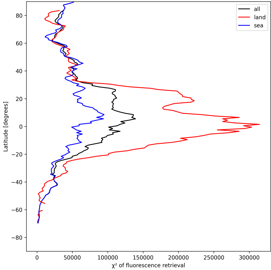
Figure 23: Zonal average of “ \chi^2 of fluorescence retrieval” for 2025-05-11 to 2025-05-12.
