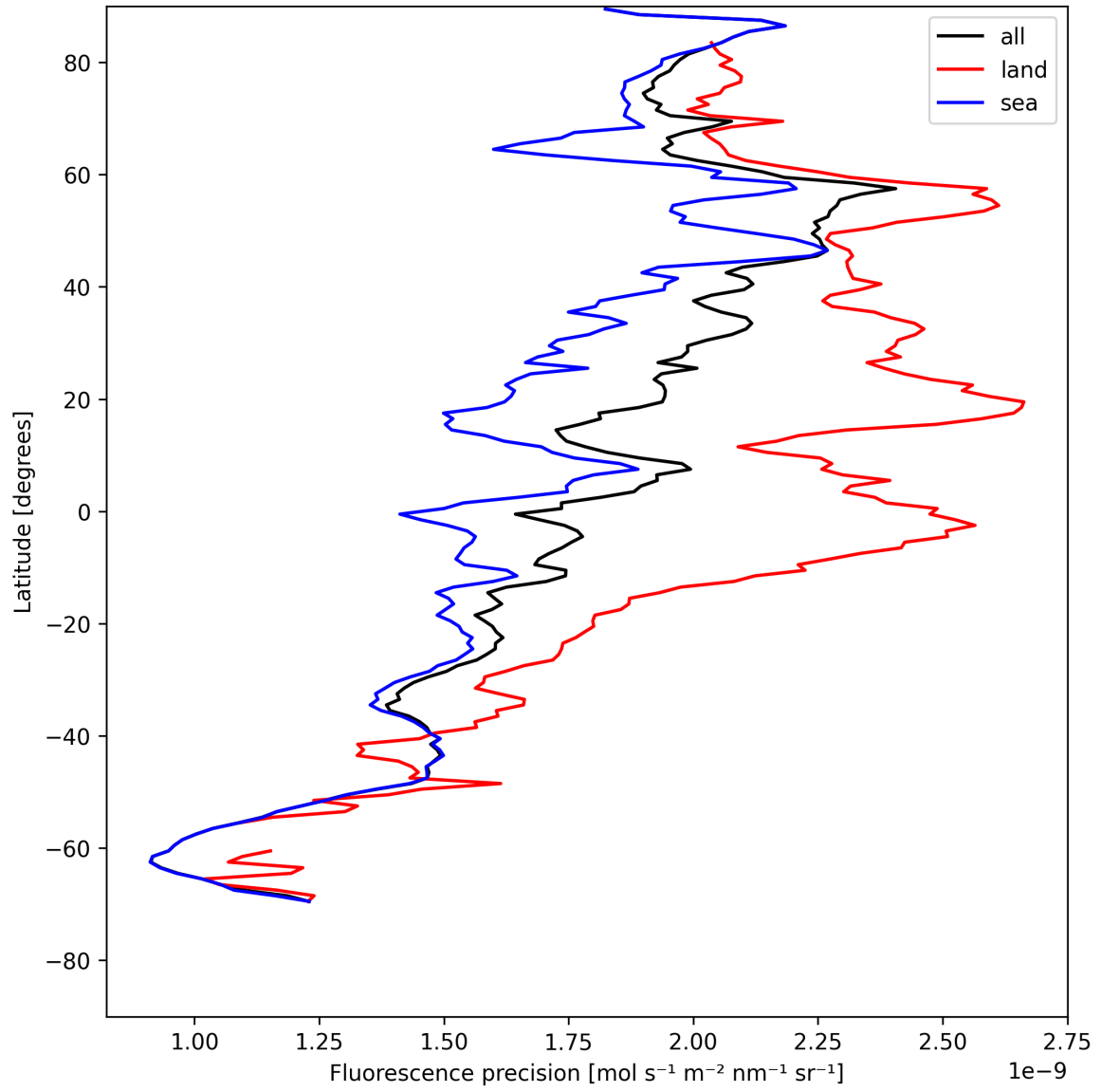
Figure 22: Zonal average of “Fluorescence precision” for 2025-05-11 to 2025-05-12.
