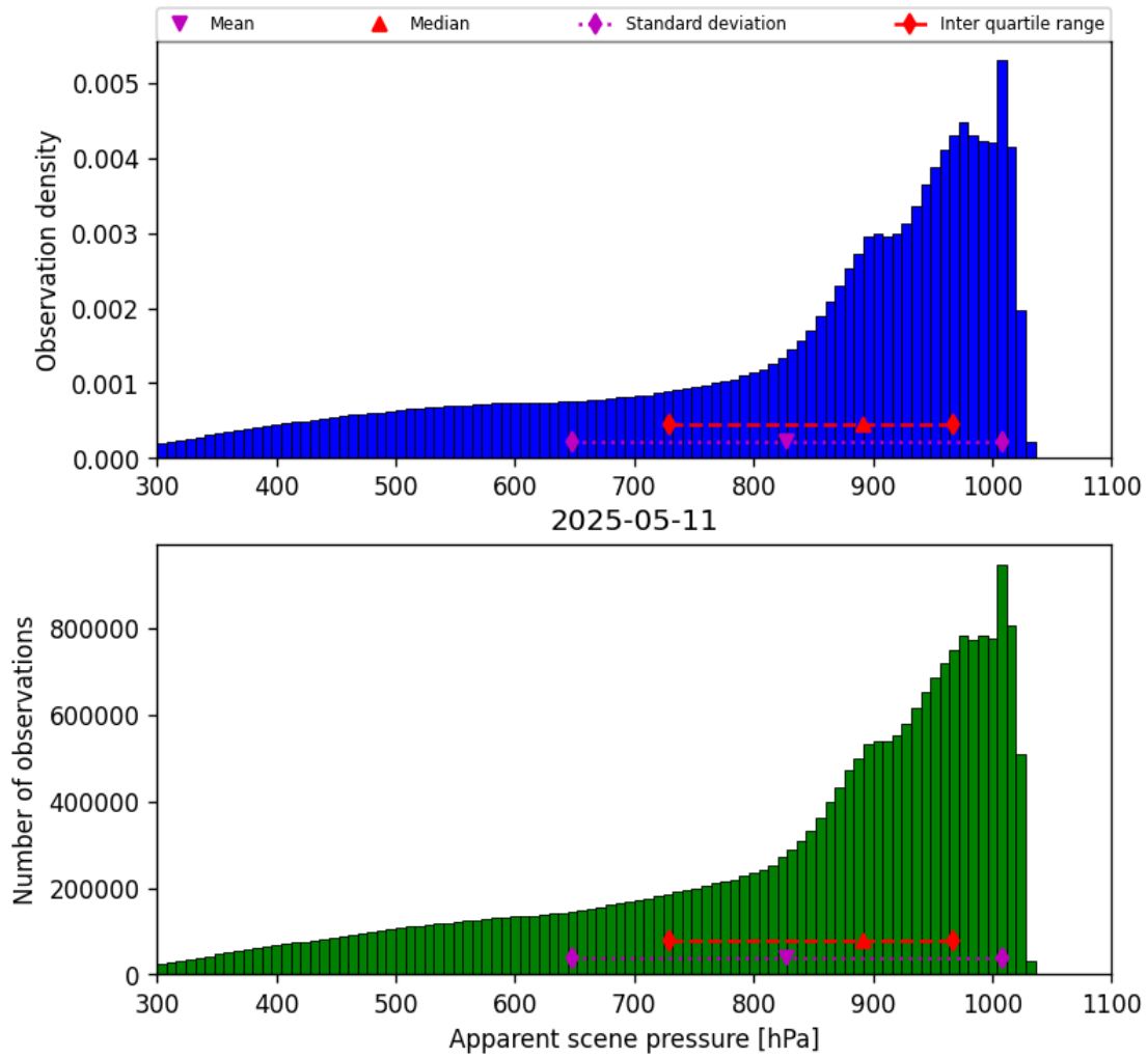
Figure 34: Histogram of “Apparent scene pressure” for 2025-05-11 to 2025-05-12
