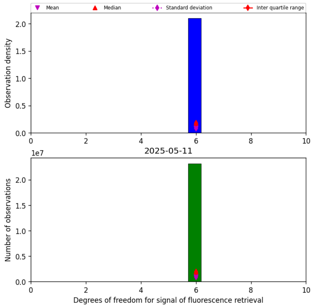
Figure 41: Histogram of “Degrees of freedom for signal of fluorescence retrieval” for 2025-05-11 to 2025-05-12
