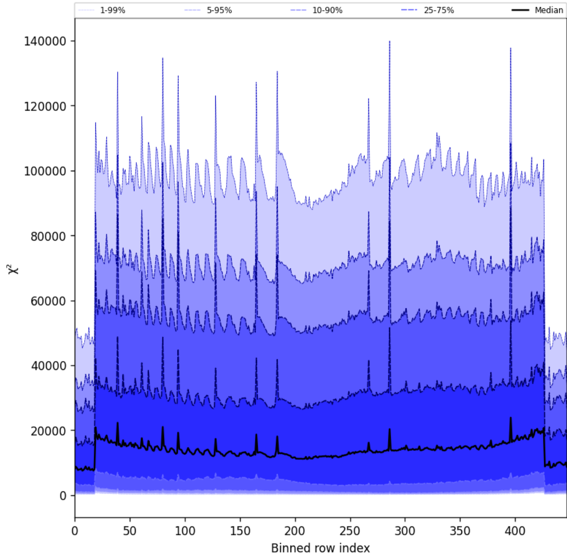
Figure 53: Along track statistics of “ \chi^2 ” for 2025-05-11 to 2025-05-12
