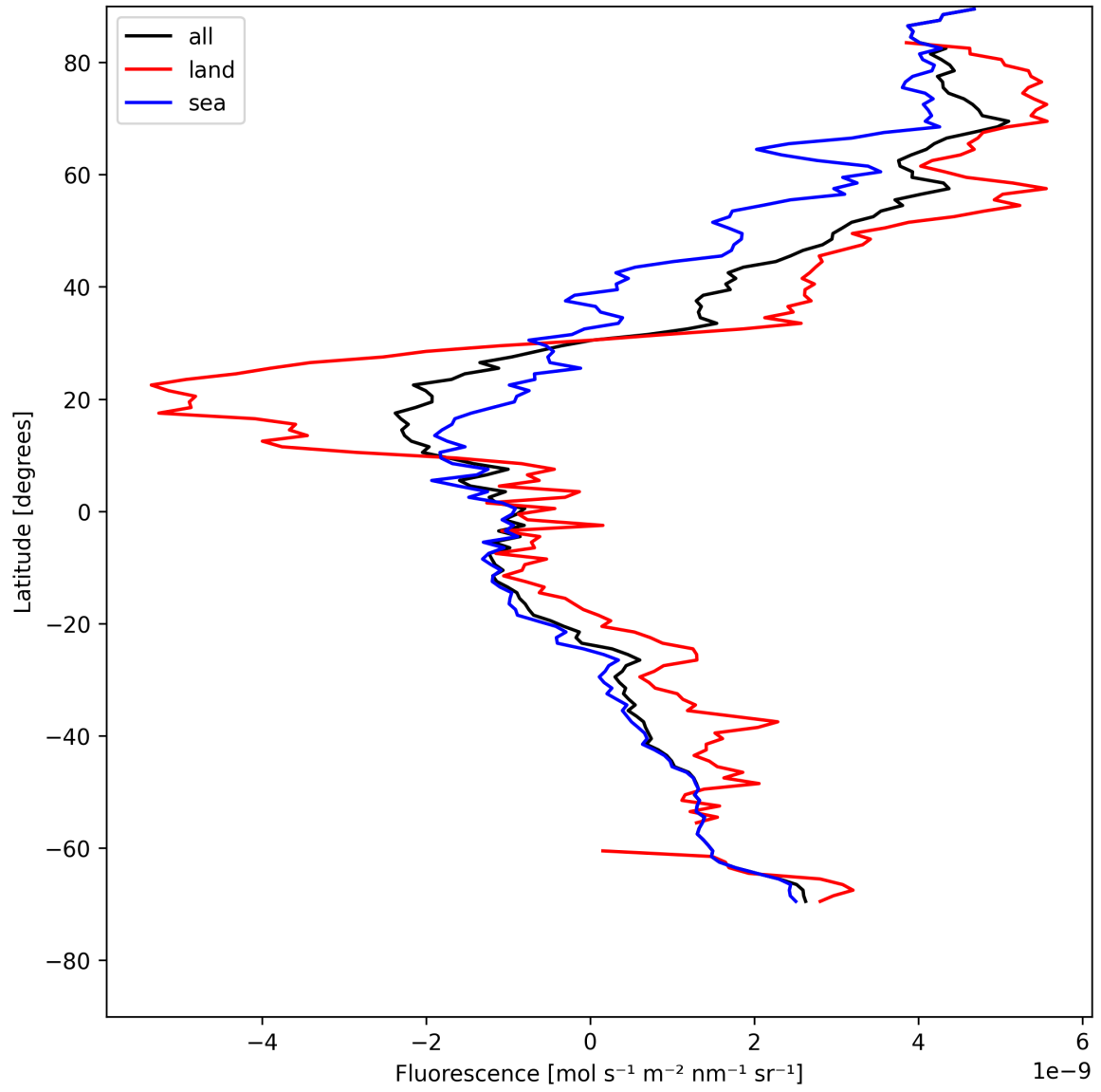
Figure 21: Zonal average of “Fluorescence” for 2025-05-11 to 2025-05-12.
