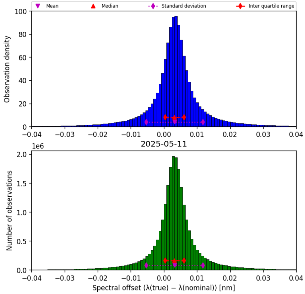
Figure 43: Histogram of “Spectral offset ( \lambda_{\text{true}} - \lambda_{\text{nominal}} )” for 2025-05-11 to 2025-05-12
