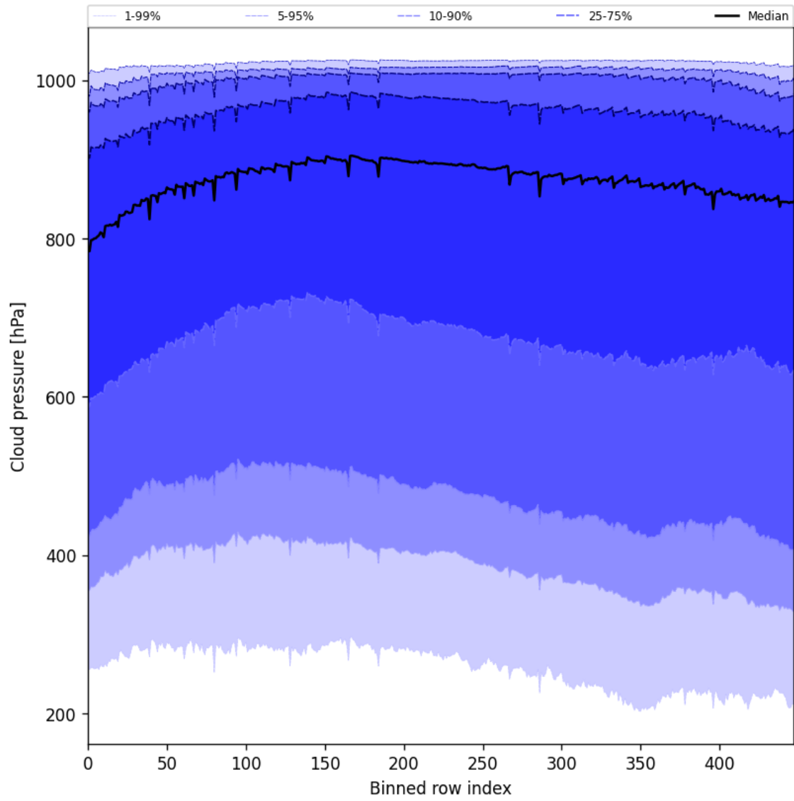
Figure 45: Along track statistics of “Cloud pressure” for 2025-05-11 to 2025-05-12
