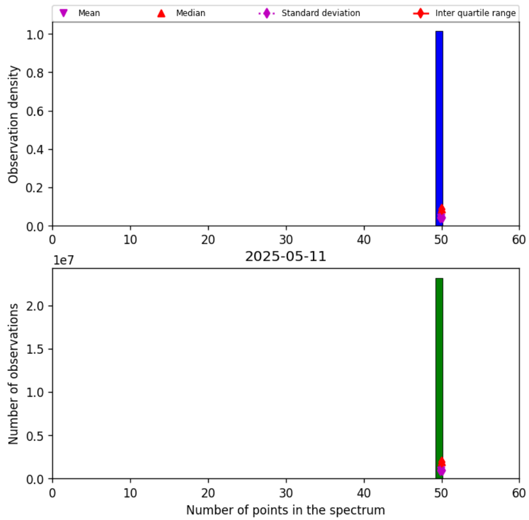
Figure 42: Histogram of “Number of points in the spectrum” for 2025-05-11 to 2025-05-12
