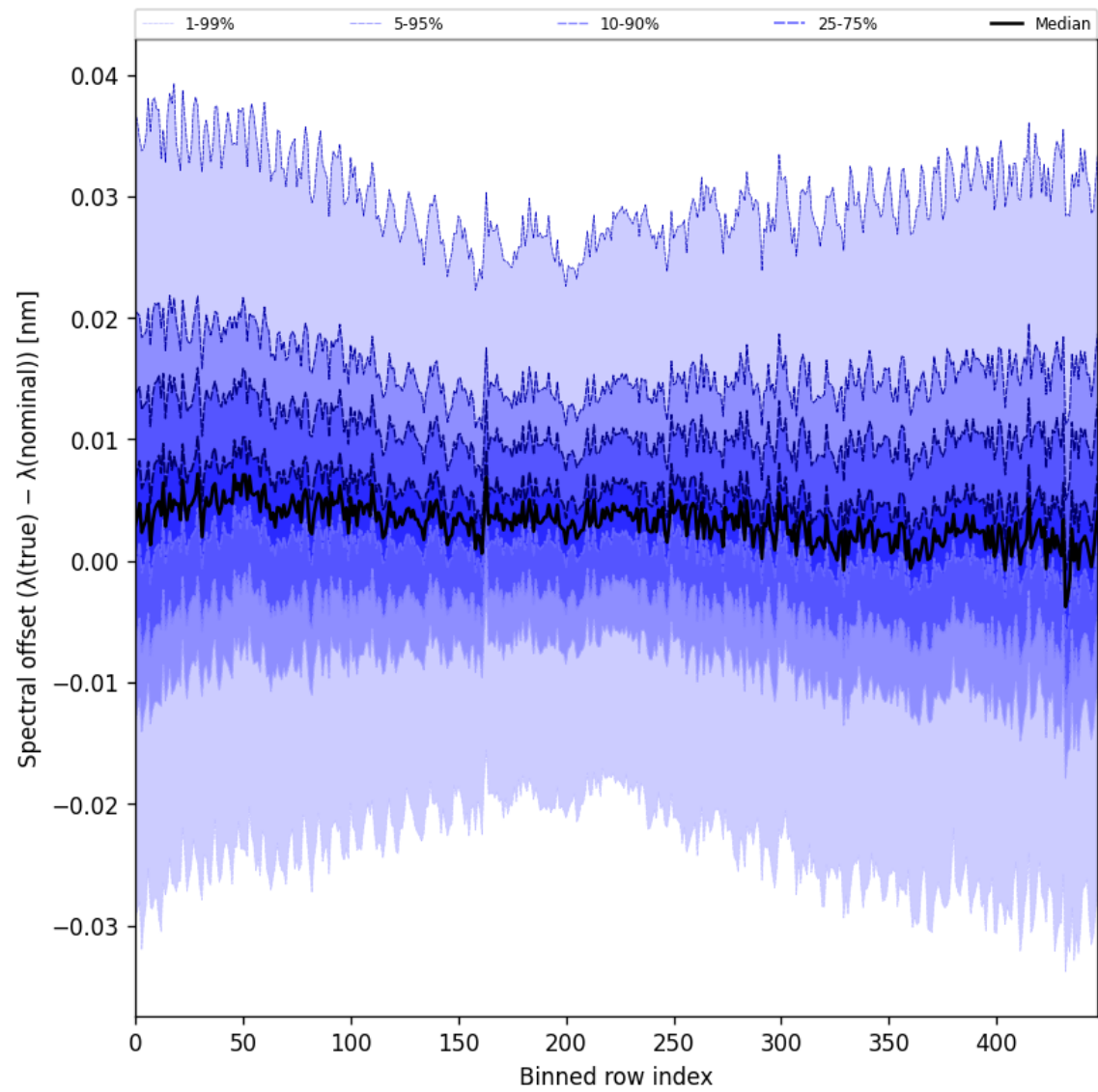
Figure 60: Along track statistics of “Spectral offset ( \lambda_{\text{true}} - \lambda_{\text{nominal}} )” for 2025-05-11 to 2025-05-12
