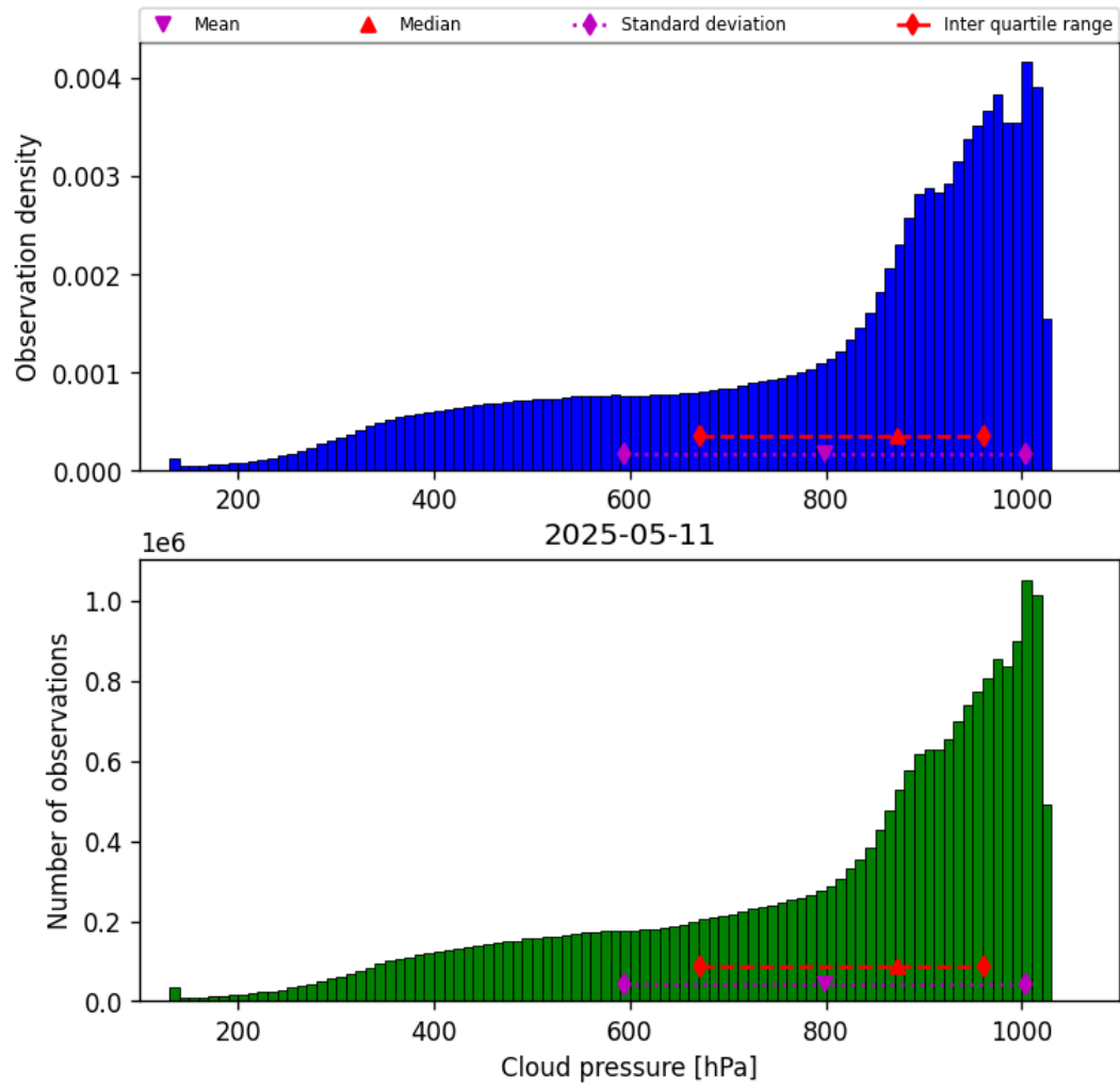
Figure 28: Histogram of “Cloud pressure” for 2025-05-11 to 2025-05-12
