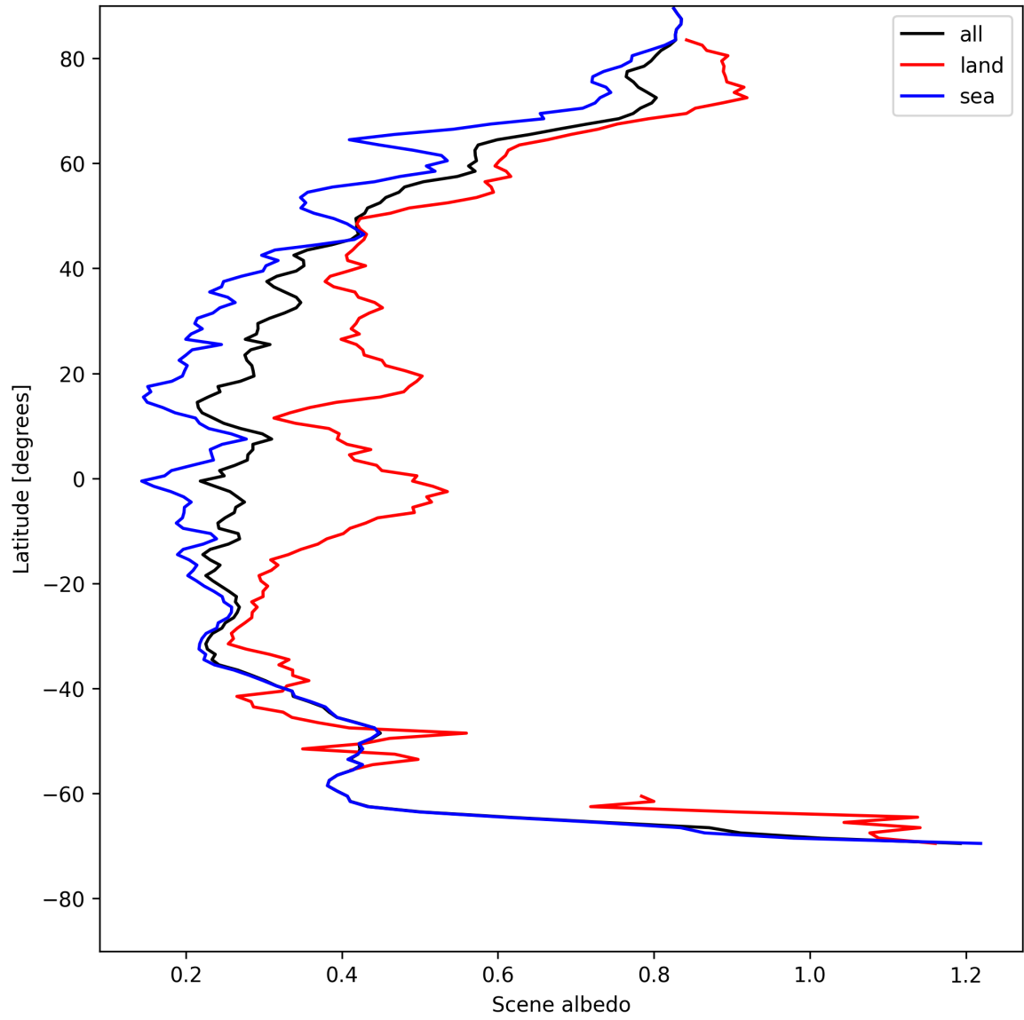
Figure 15: Zonal average of "Scene albedo" for 2025-05-11 to 2025-05-12.
