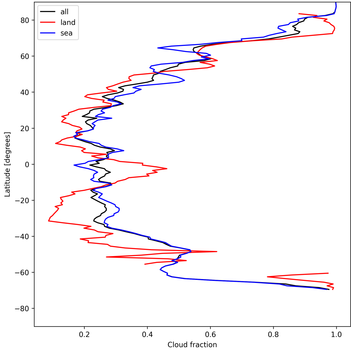
Figure 13: Zonal average of “Cloud fraction” for 2025-05-11 to 2025-05-12.
