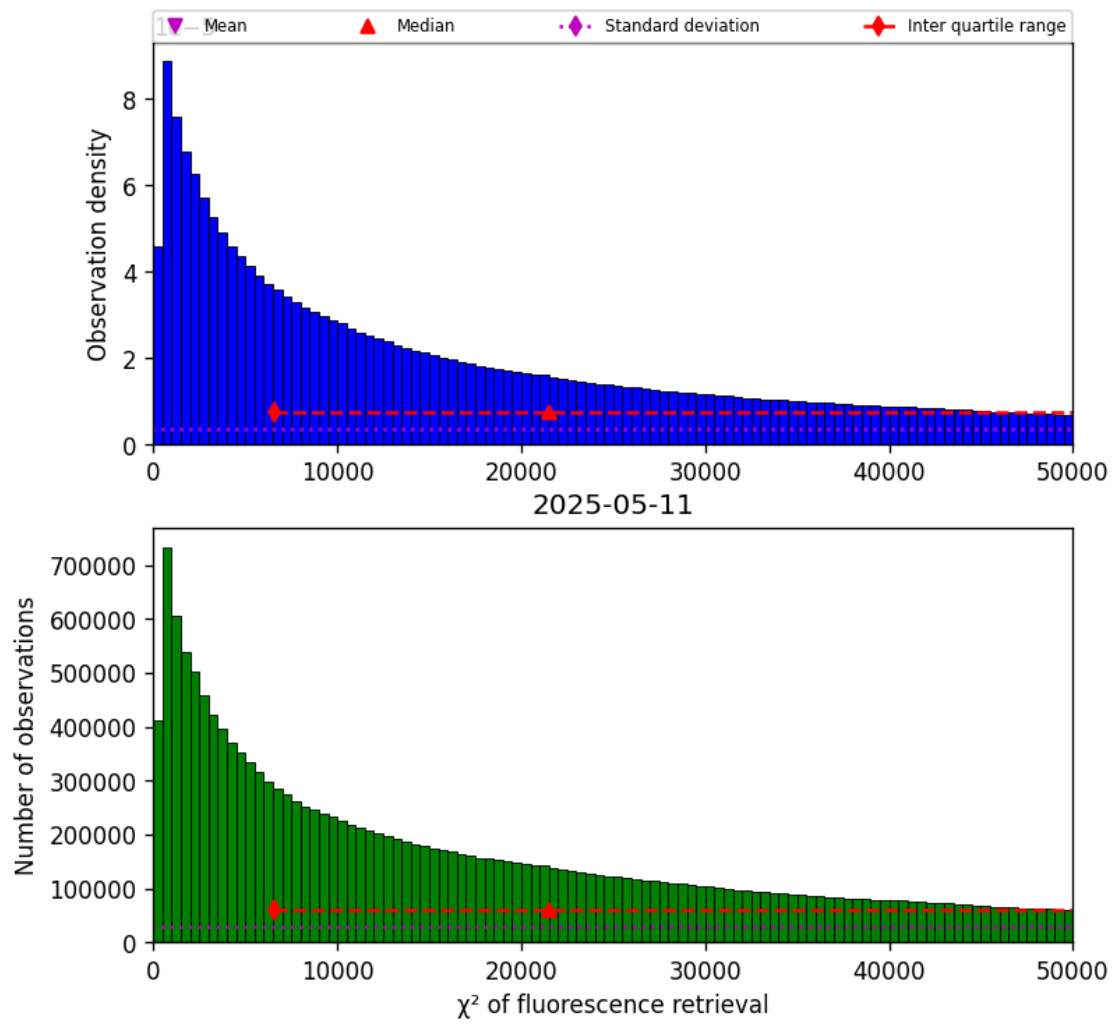
Figure 40: Histogram of “ \chi^2 of fluorescence retrieval” for 2025-05-11 to 2025-05-12
