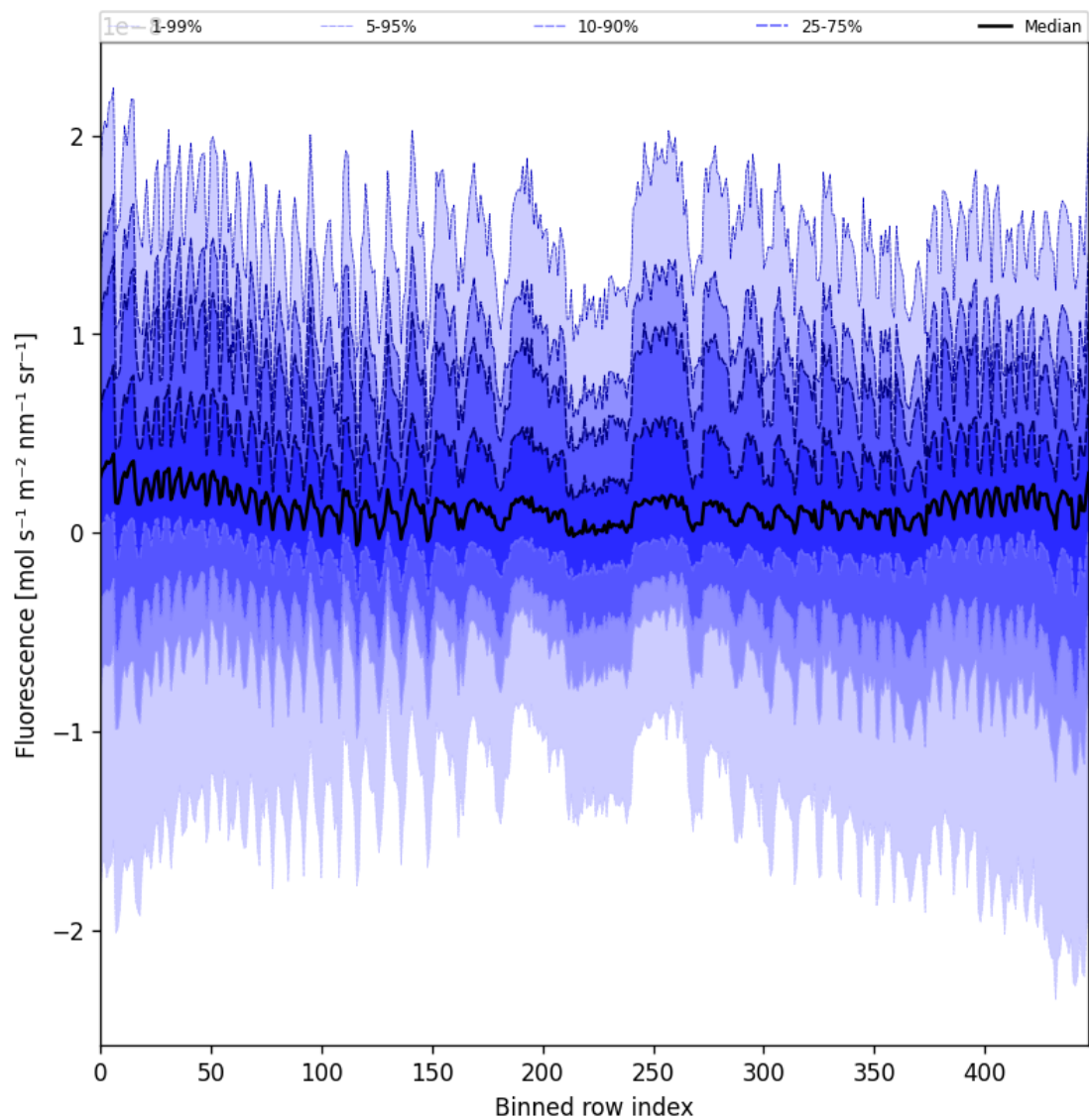
Figure 55: Along track statistics of “Fluorescence” for 2025-05-11 to 2025-05-12
