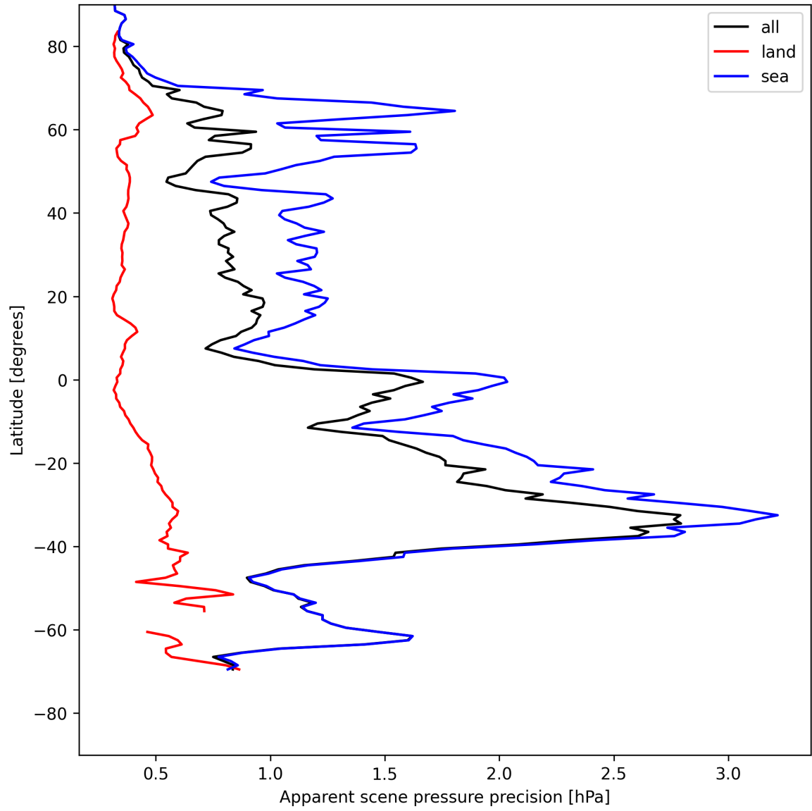
Figure 18: Zonal average of “Apparent scene pressure precision” for 2025-05-11 to 2025-05-12.
