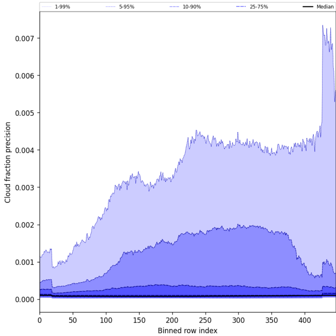
Figure 48: Along track statistics of “Cloud fraction precision” for 2025-05-11 to 2025-05-12
