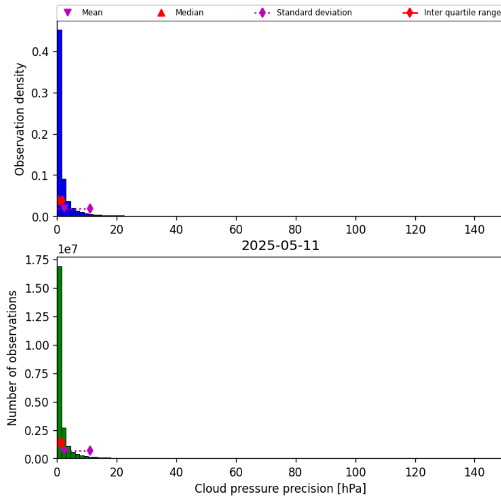
Figure 29: Histogram of “Cloud pressure precision” for 2025-05-11 to 2025-05-12
