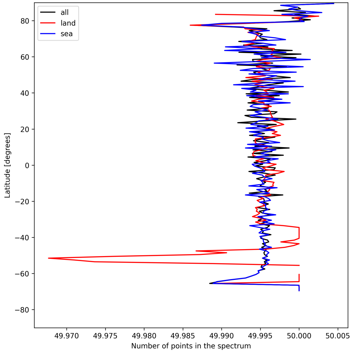
Figure 25: Zonal average of “Number of points in the spectrum” for 2025-05-11 to 2025-05-12.
