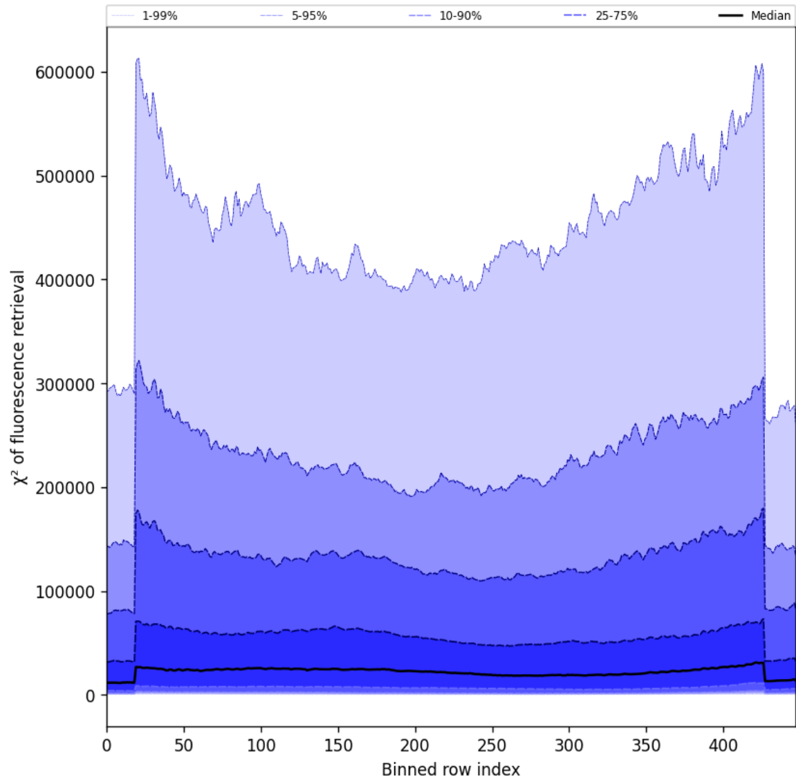
Figure 57: Along track statistics of “ \chi^2 of fluorescence retrieval” for 2025-05-11 to 2025-05-12
