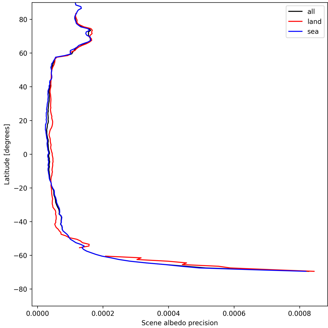
Figure 16: Zonal average of “Scene albedo precision” for 2025-05-11 to 2025-05-12.
