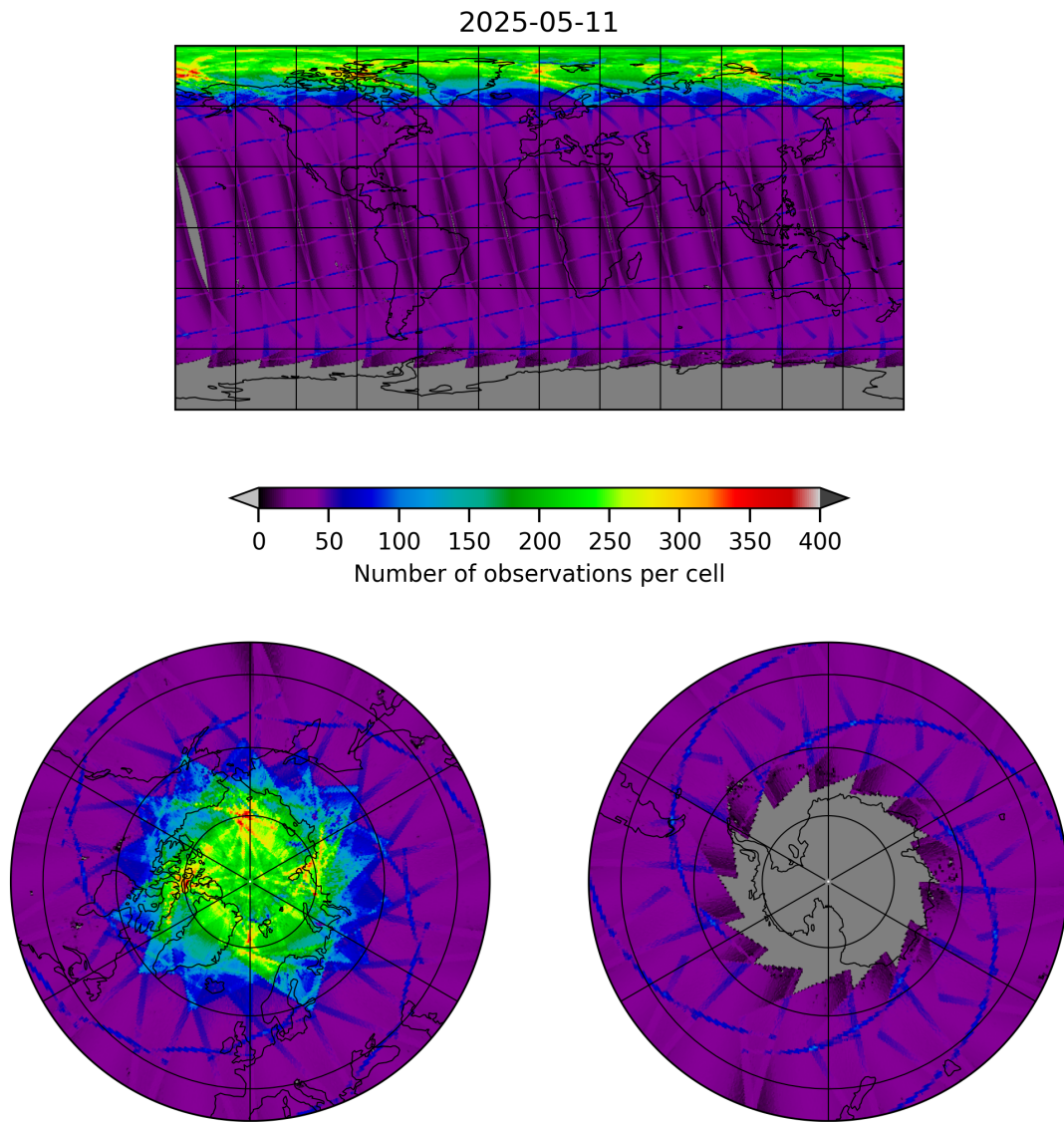
Figure 9: Map of the number of observations for 2025-05-11 to 2025-05-12
