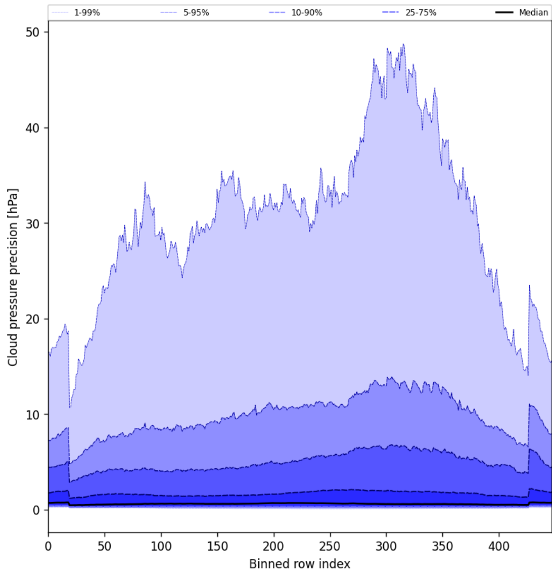
Figure 46: Along track statistics of “Cloud pressure precision” for 2025-05-11 to 2025-05-12
