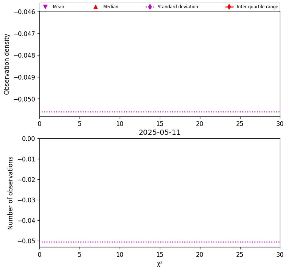
Figure 36: Histogram of " \chi^2 " for 2025-05-11 to 2025-05-12
