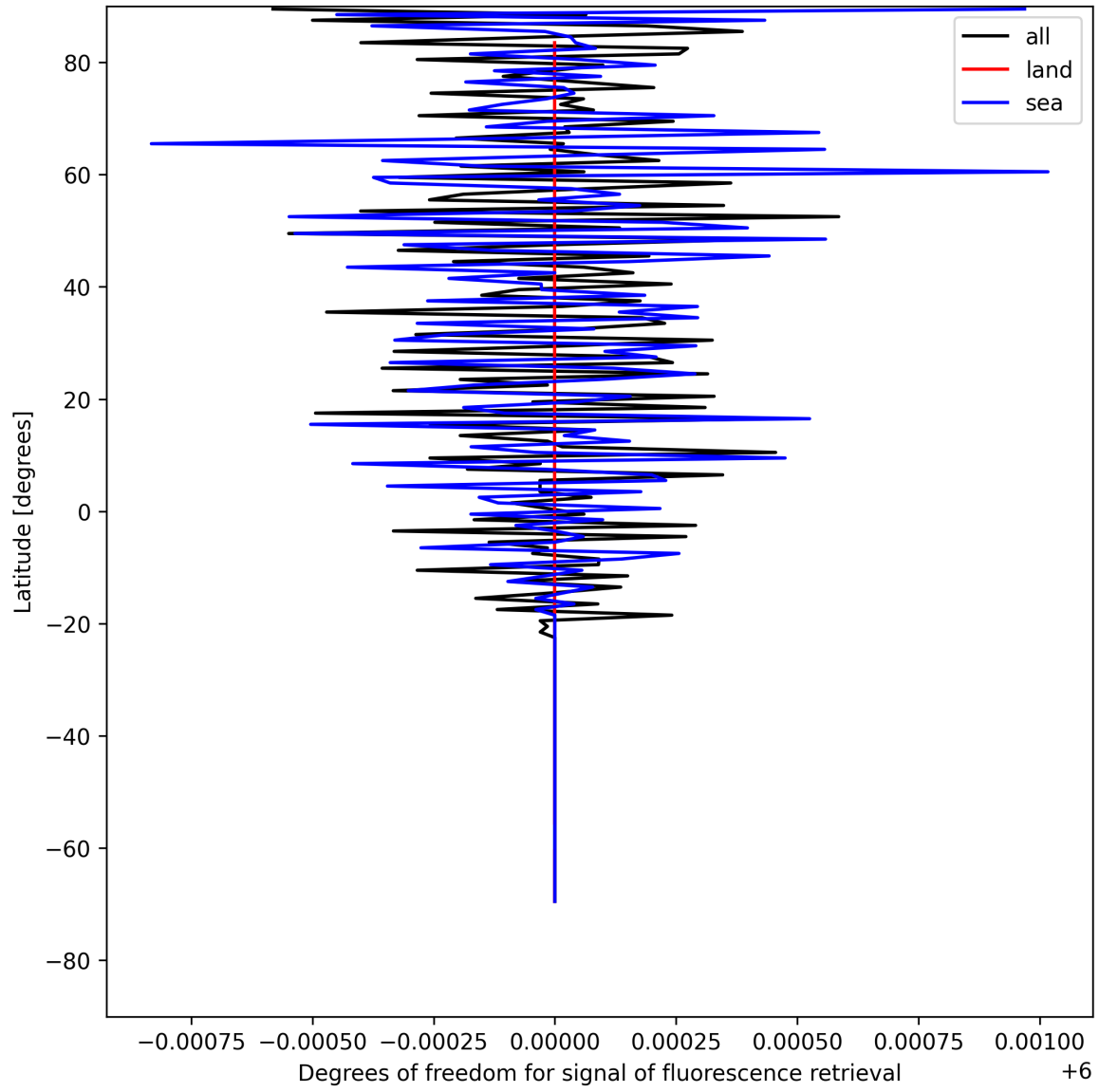
Figure 24: Zonal average of “Degrees of freedom for signal of fluorescence retrieval” for 2025-05-11 to 2025-05-12.
