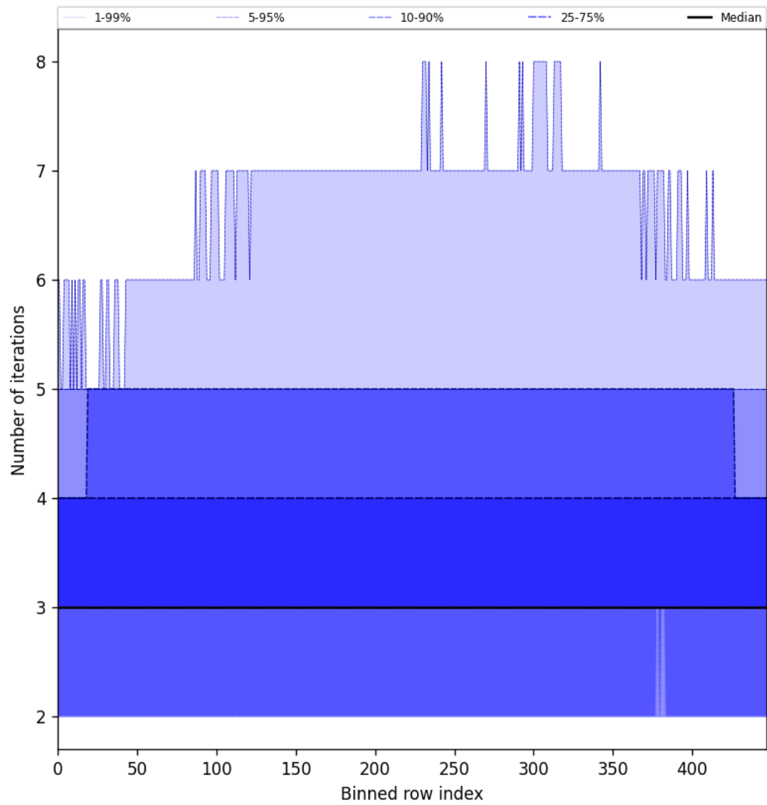
Figure 54: Along track statistics of “Number of iterations” for 2025-05-11 to 2025-05-12
