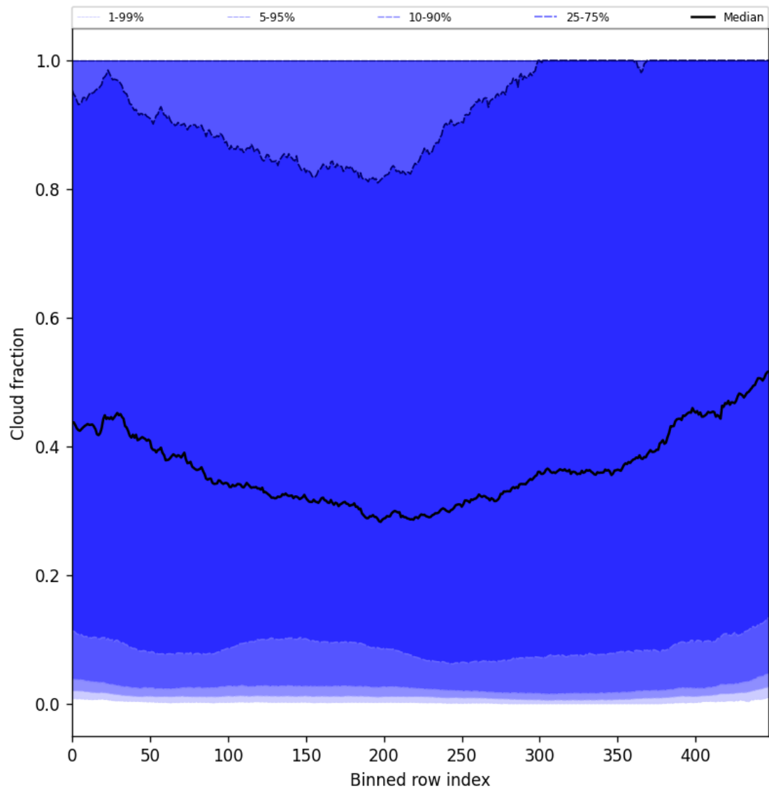
Figure 47: Along track statistics of “Cloud fraction” for 2025-05-11 to 2025-05-12
