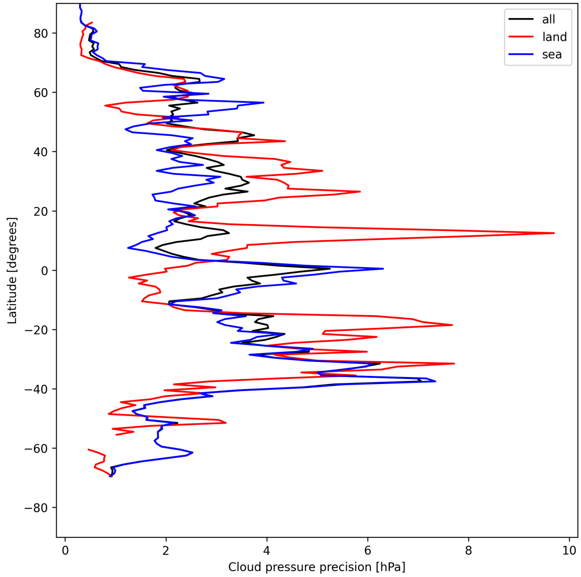
Figure 12: Zonal average of “Cloud pressure precision” for 2025-05-11 to 2025-05-12.
