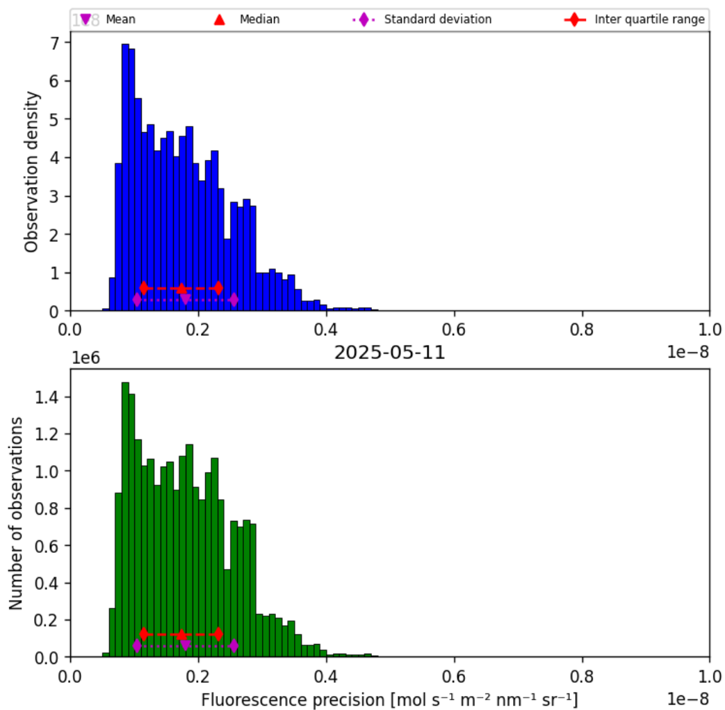
Figure 39: Histogram of “Fluorescence precision” for 2025-05-11 to 2025-05-12
