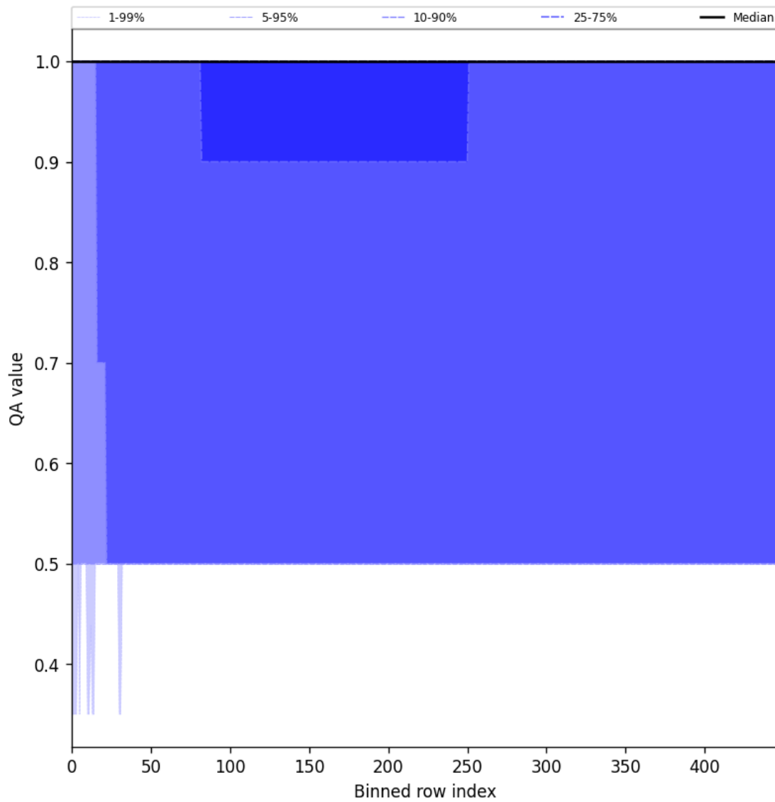
Figure 44: Along track statistics of “QA value” for 2025-05-11 to 2025-05-12
