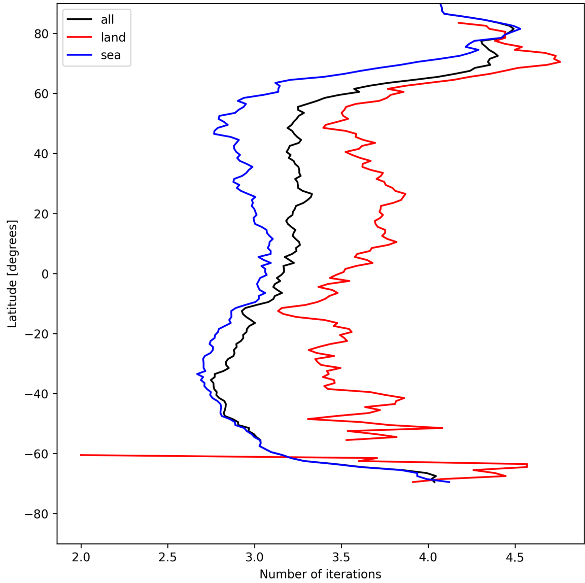
Figure 20: Zonal average of “Number of iterations” for 2025-05-11 to 2025-05-12.
