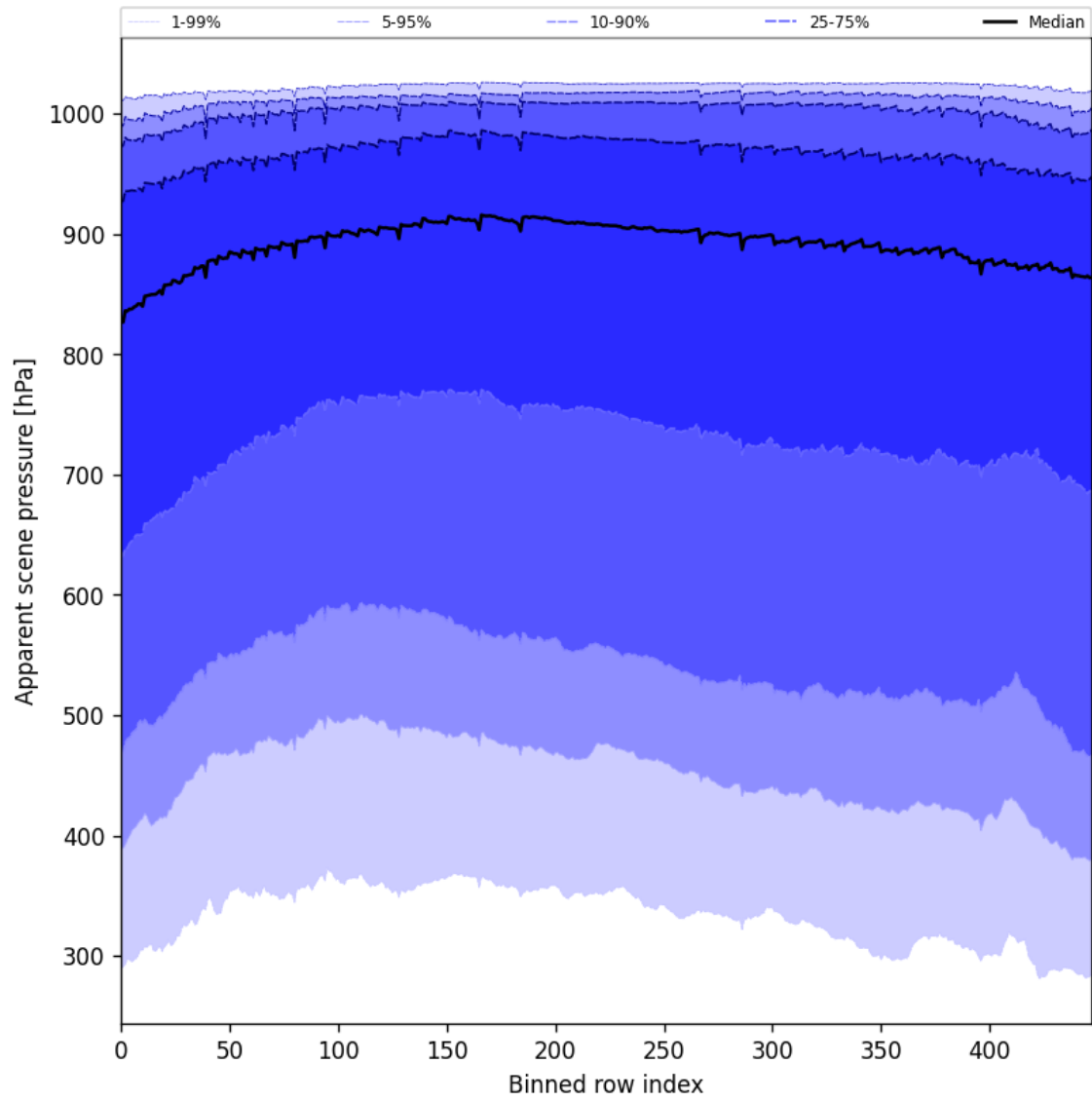
Figure 51: Along track statistics of “Apparent scene pressure” for 2025-05-11 to 2025-05-12
