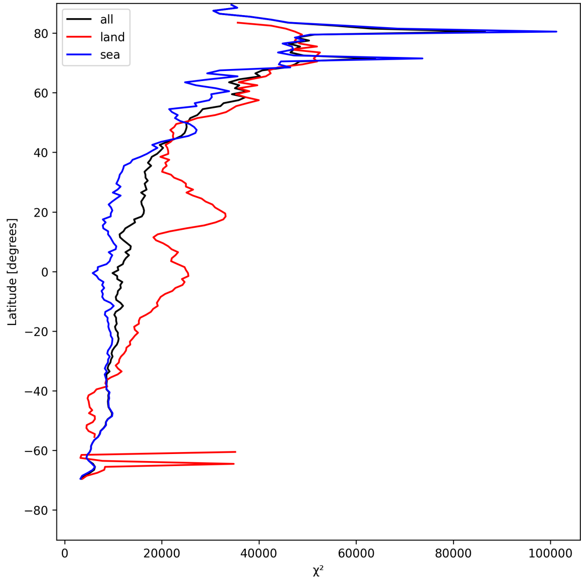
Figure 19: Zonal average of “ \chi^2 ” for 2025-05-11 to 2025-05-12.
