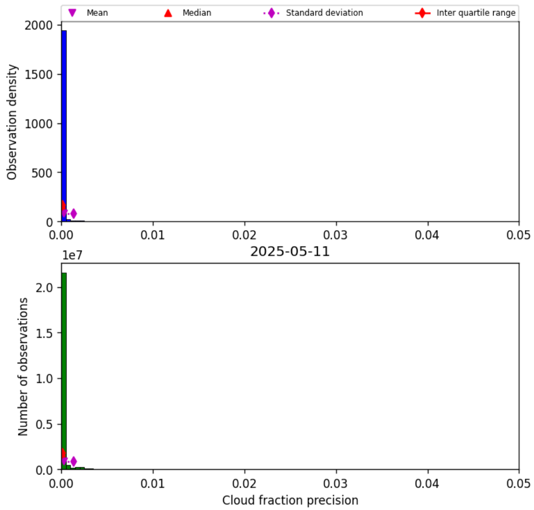
Figure 31: Histogram of “Cloud fraction precision” for 2025-05-11 to 2025-05-12
