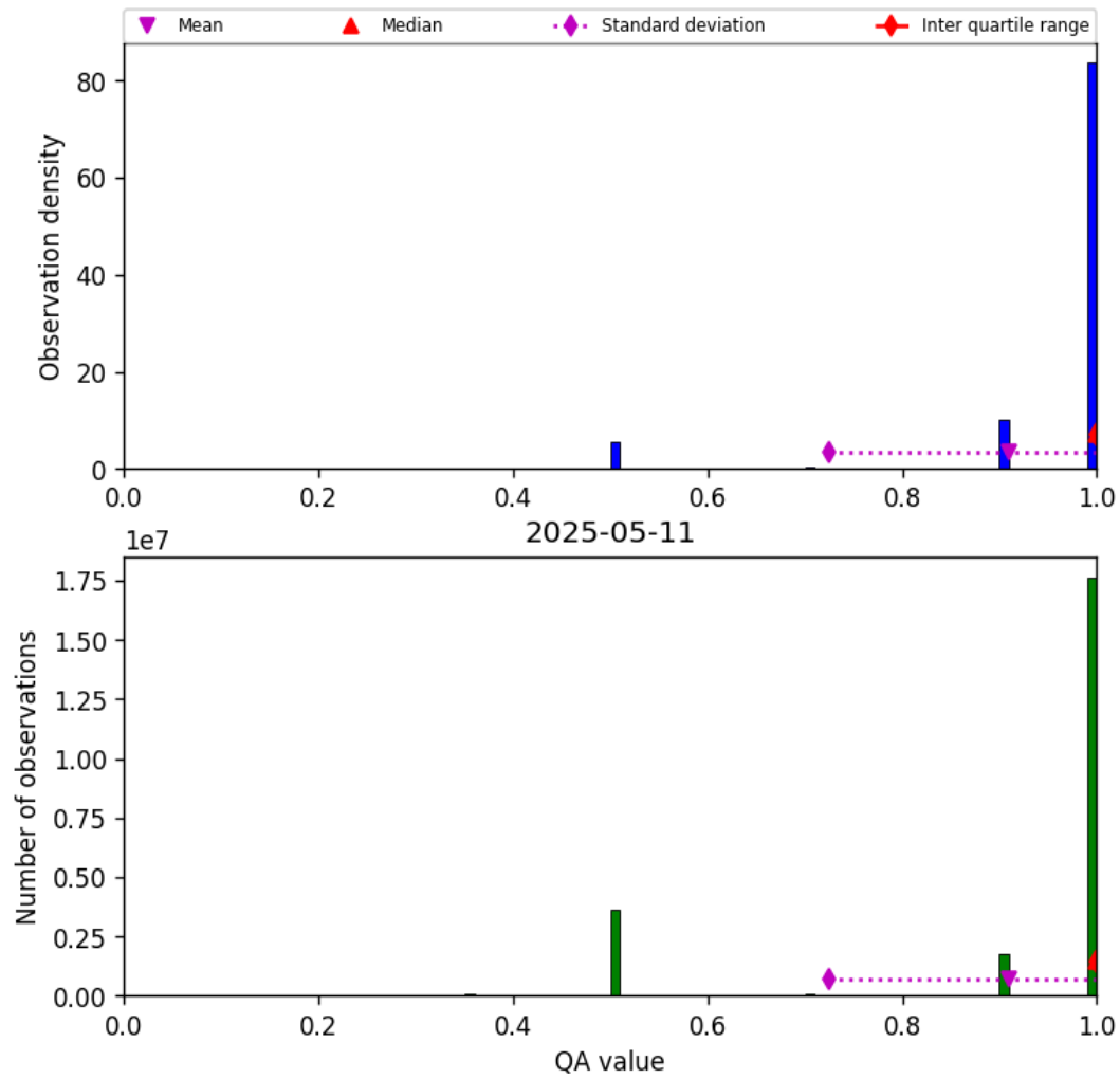
Figure 27: Histogram of “QA value” for 2025-05-11 to 2025-05-12
