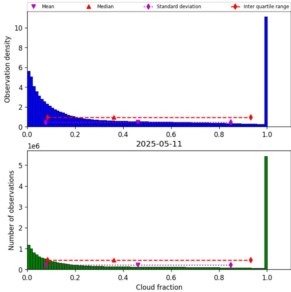
Figure 30: Histogram of “Cloud fraction” for 2025-05-11 to 2025-05-12
