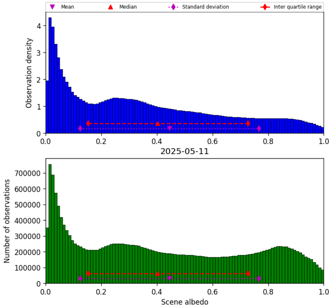
Figure 32: Histogram of “Scene albedo” for 2025-05-11 to 2025-05-12
