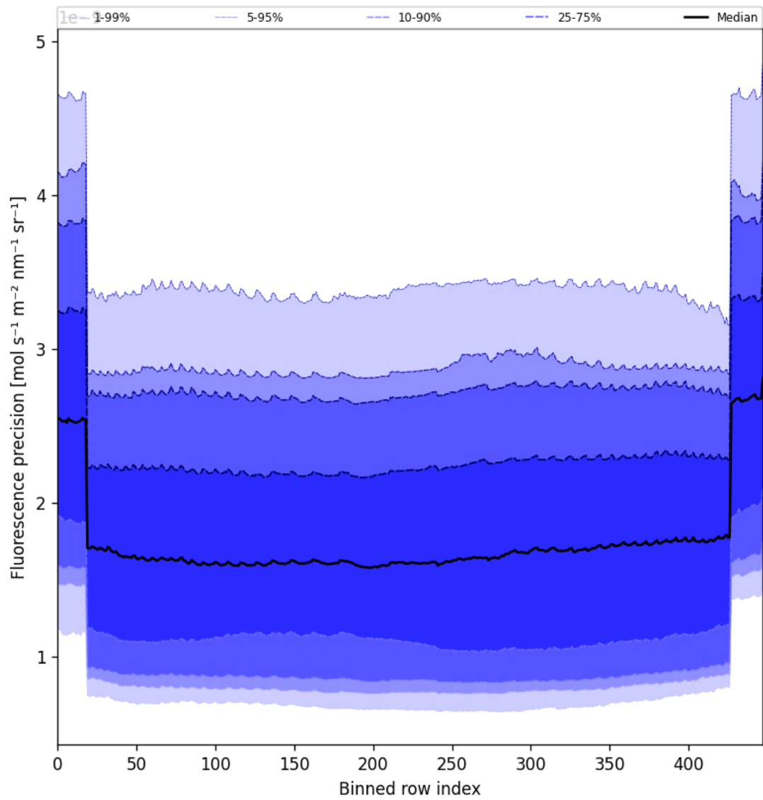
Figure 56: Along track statistics of “Fluorescence precision” for 2025-05-11 to 2025-05-12
