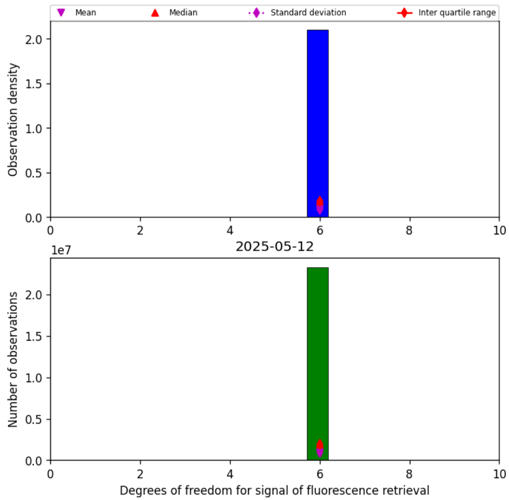
Figure 41: Histogram of “Degrees of freedom for signal of fluorescence retrieval” for 2025-05-12 to 2025-05-13
