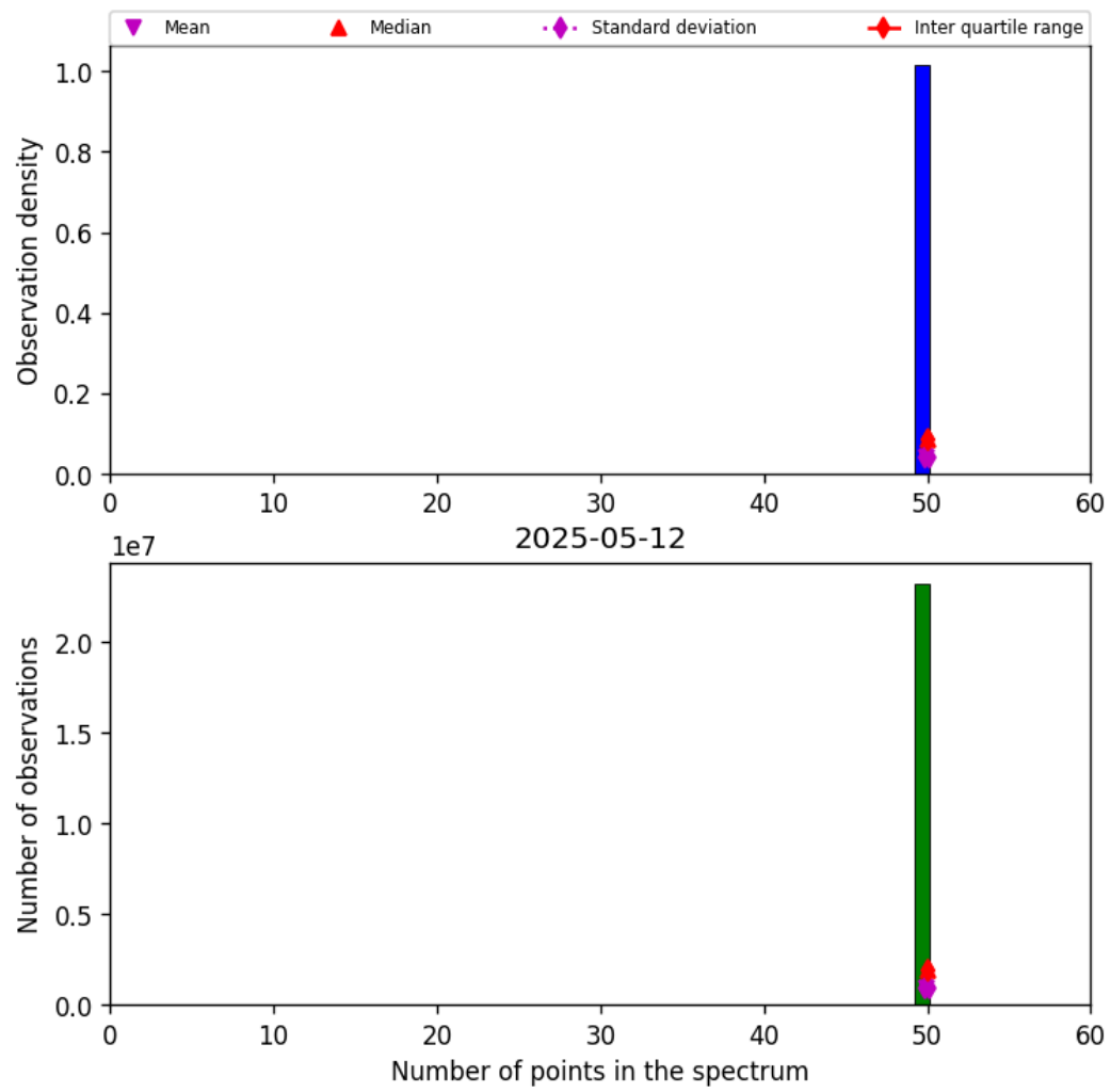
Figure 42: Histogram of “Number of points in the spectrum” for 2025-05-12 to 2025-05-13
