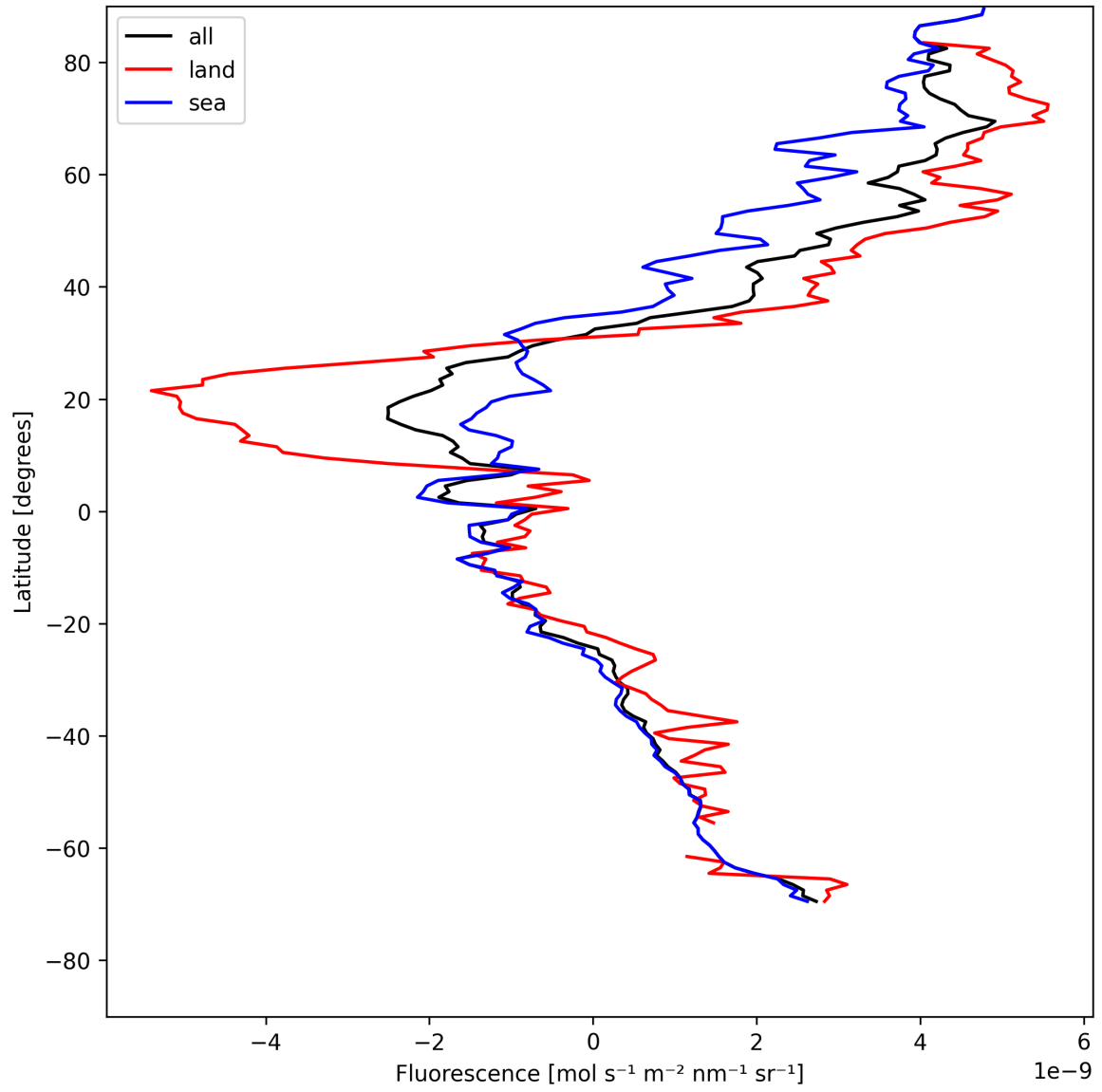
Figure 21: Zonal average of “Fluorescence” for 2025-05-12 to 2025-05-13.
