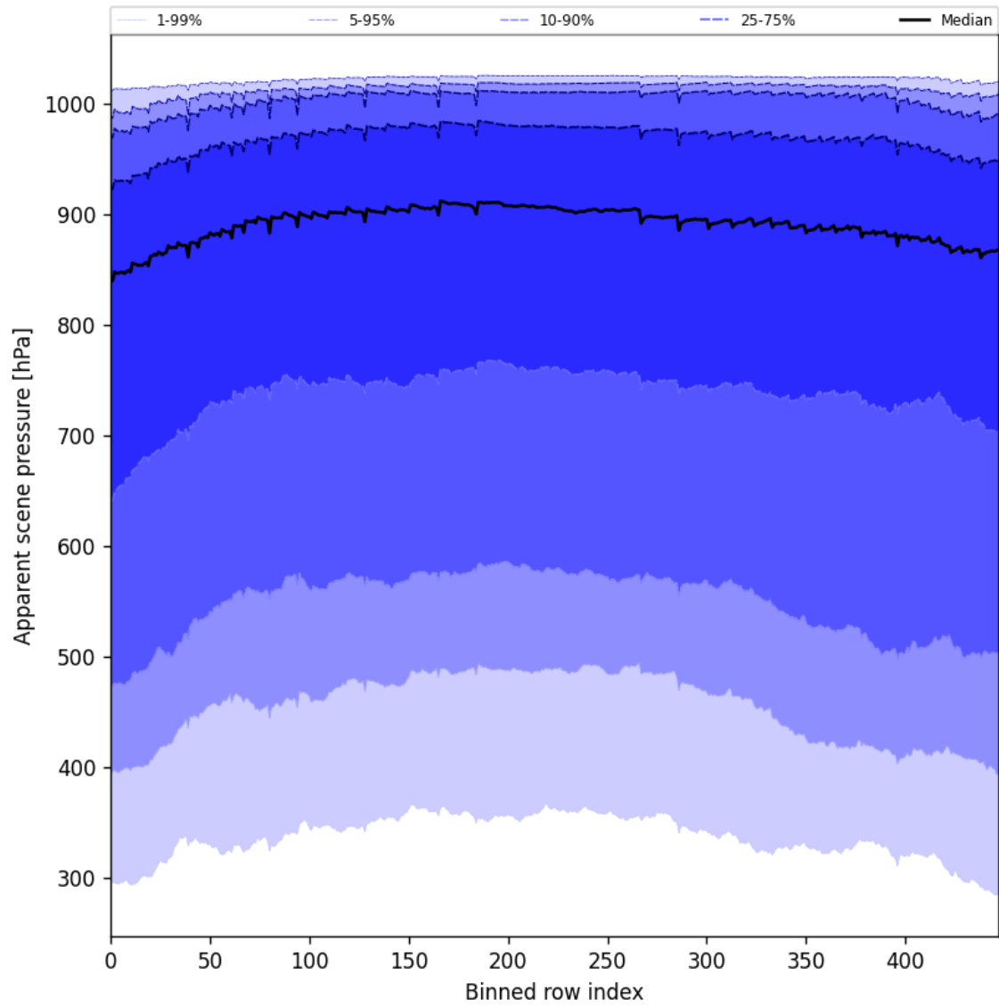
Figure 51: Along track statistics of “Apparent scene pressure” for 2025-05-12 to 2025-05-13
