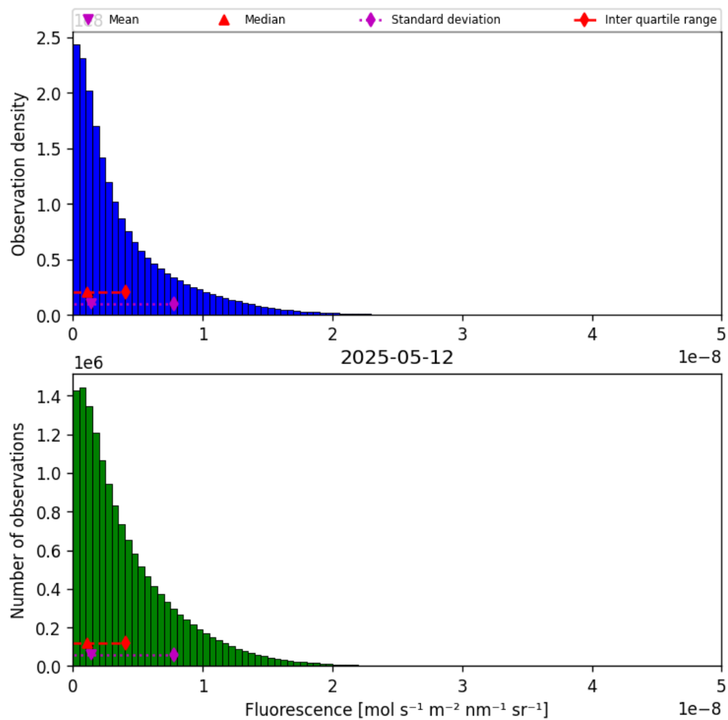
Figure 38: Histogram of “Fluorescence” for 2025-05-12 to 2025-05-13
