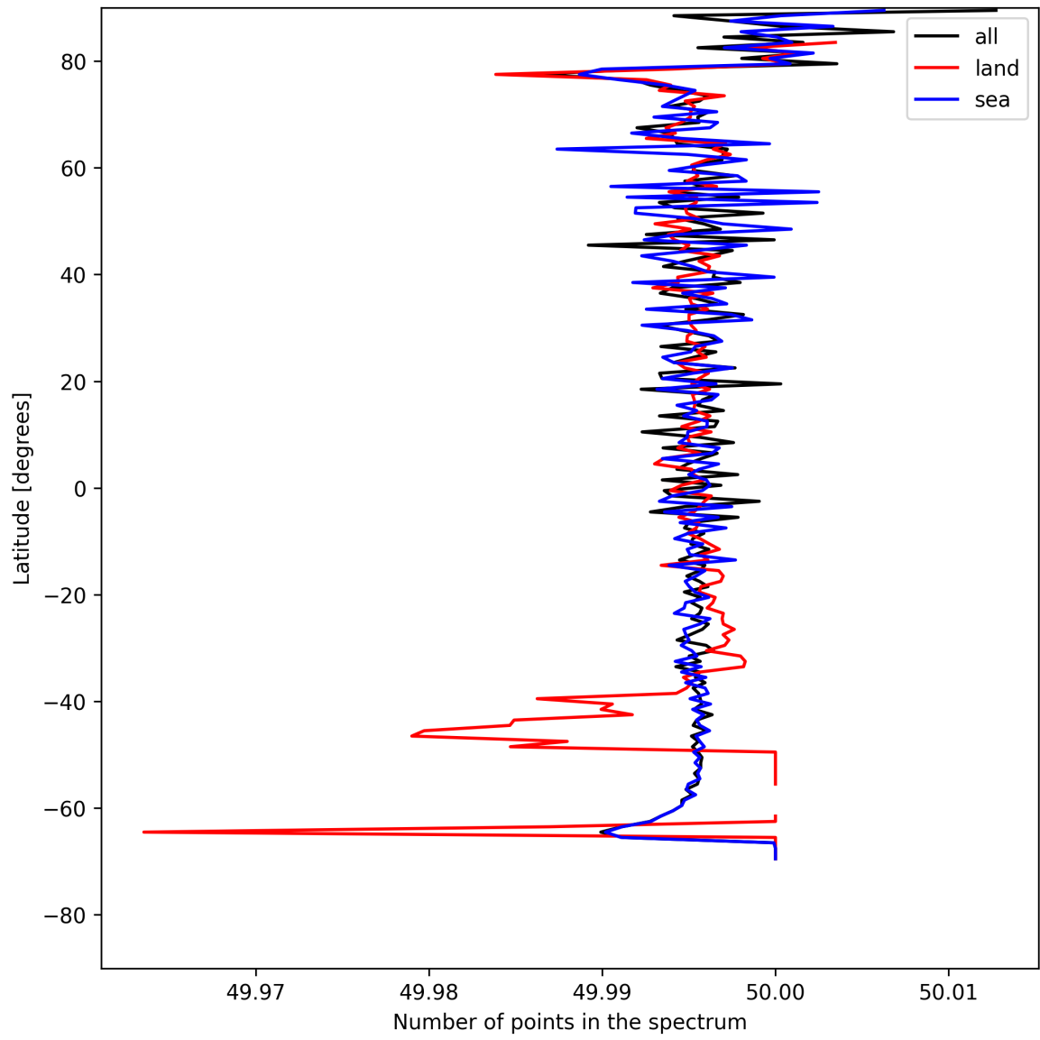
Figure 25: Zonal average of “Number of points in the spectrum” for 2025-05-12 to 2025-05-13.
