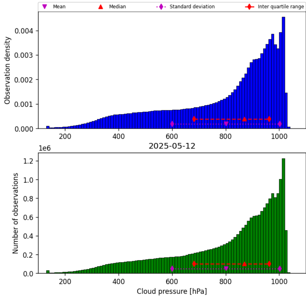
Figure 28: Histogram of “Cloud pressure” for 2025-05-12 to 2025-05-13
