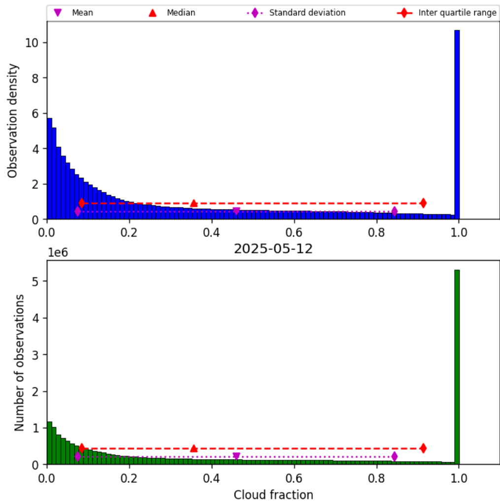
Figure 30: Histogram of “Cloud fraction” for 2025-05-12 to 2025-05-13
