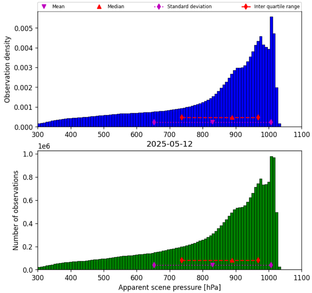
Figure 34: Histogram of “Apparent scene pressure” for 2025-05-12 to 2025-05-13
