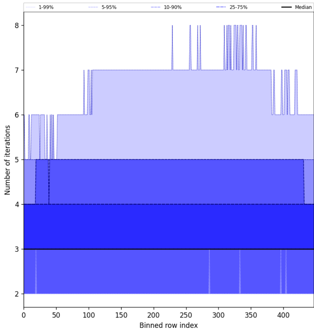
Figure 54: Along track statistics of “Number of iterations” for 2025-05-12 to 2025-05-13
