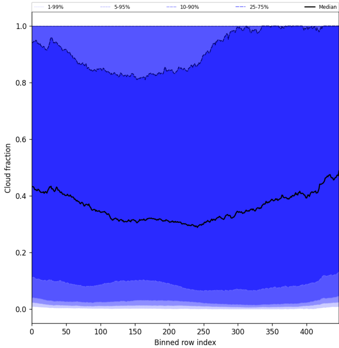
Figure 47: Along track statistics of “Cloud fraction” for 2025-05-12 to 2025-05-13
