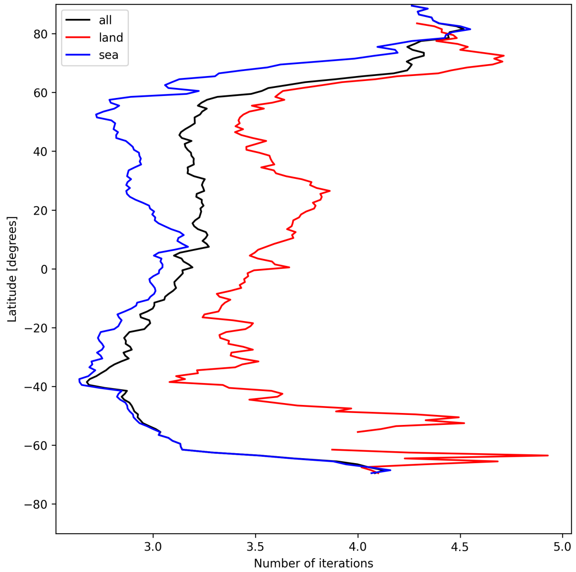
Figure 20: Zonal average of “Number of iterations” for 2025-05-12 to 2025-05-13.
