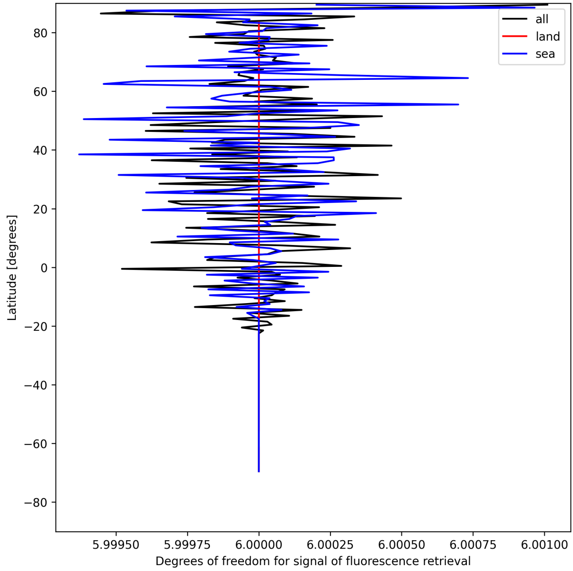
Figure 24: Zonal average of “Degrees of freedom for signal of fluorescence retrieval” for 2025-05-12 to 2025-05-13.
