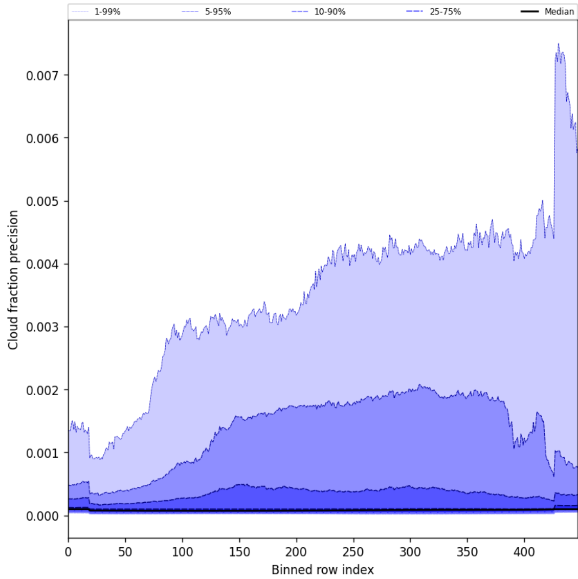
Figure 48: Along track statistics of “Cloud fraction precision” for 2025-05-12 to 2025-05-13
