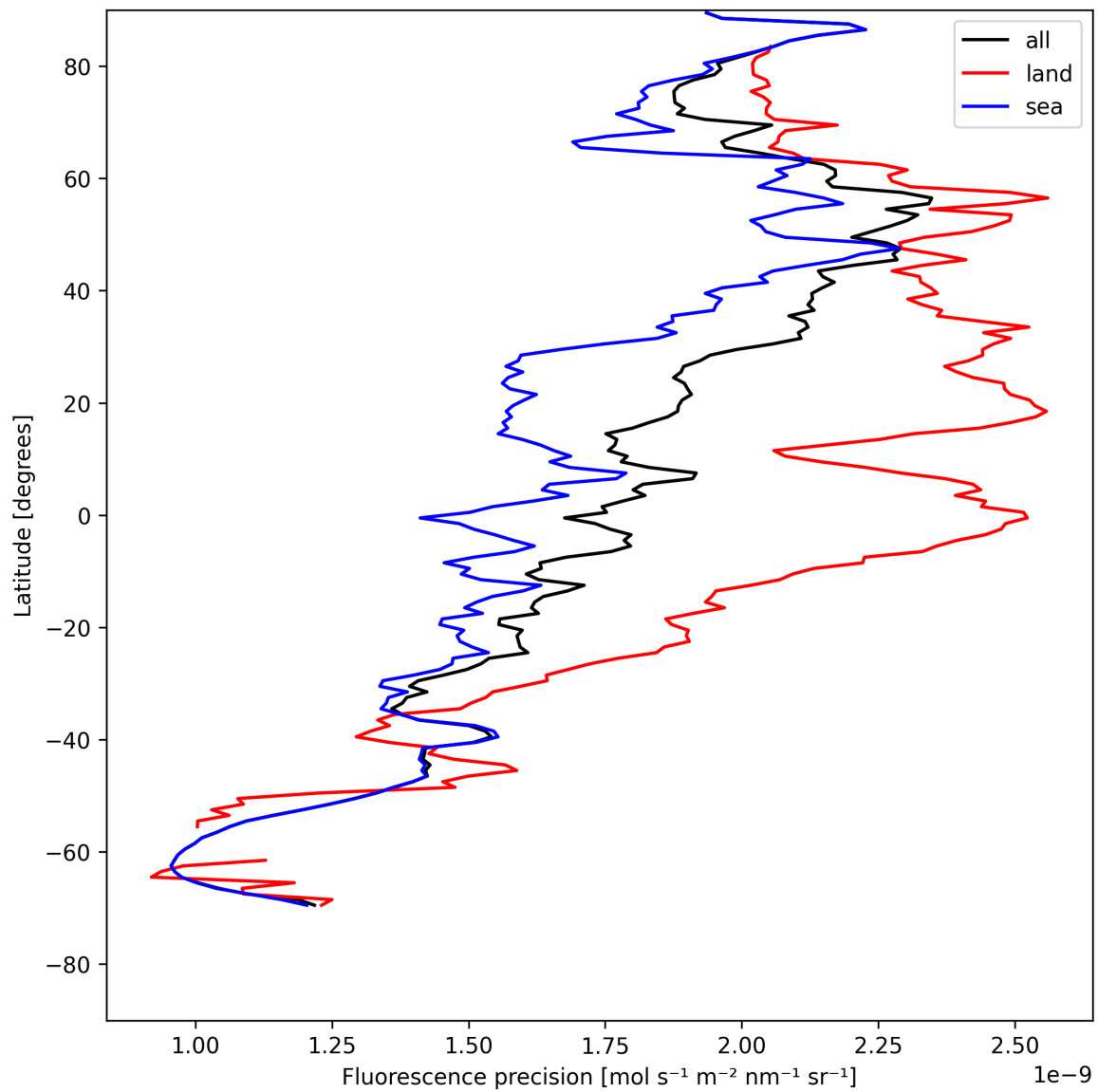
Figure 22: Zonal average of “Fluorescence precision” for 2025-05-12 to 2025-05-13.
