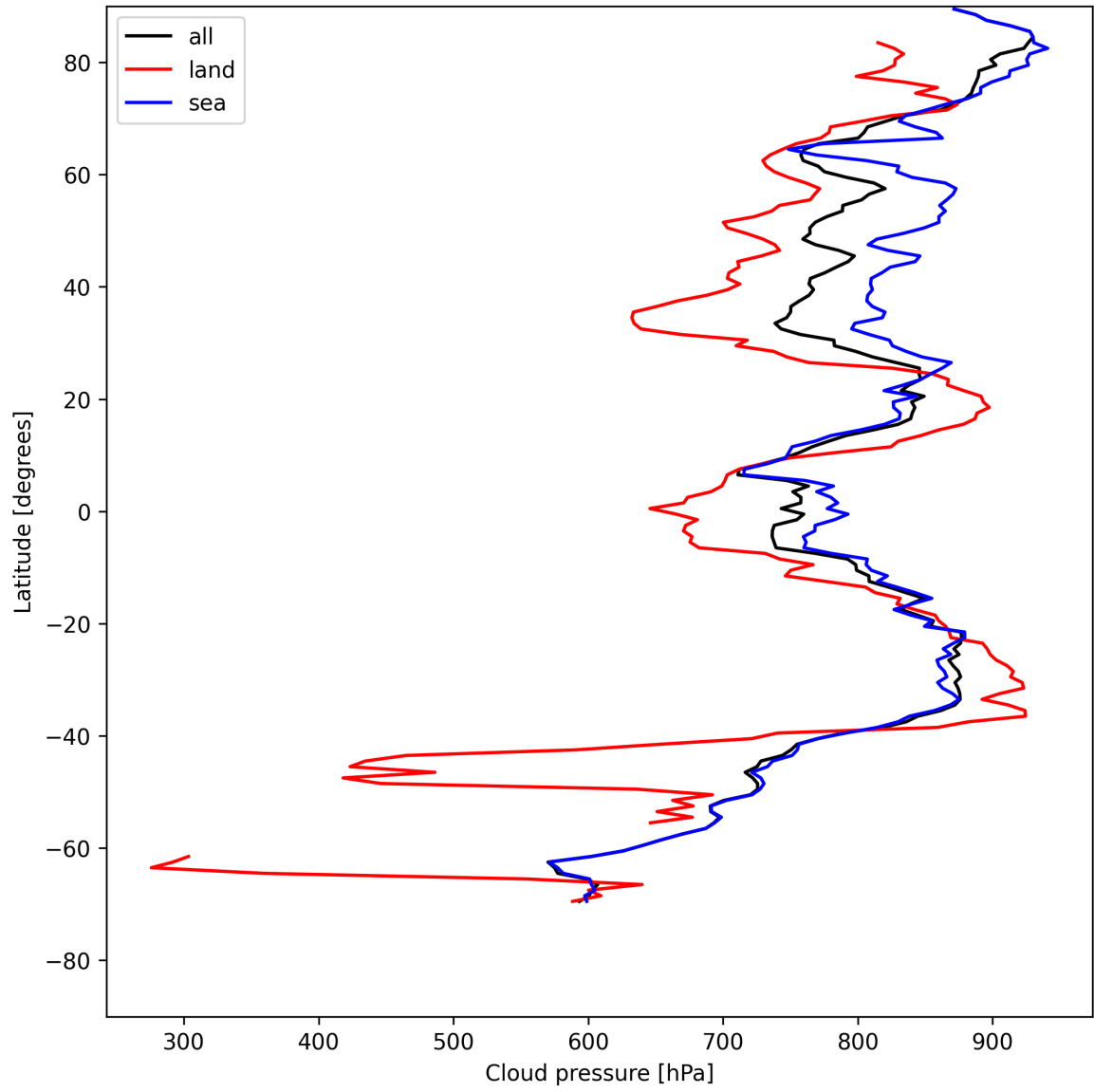
Figure 11: Zonal average of “Cloud pressure” for 2025-05-12 to 2025-05-13.
