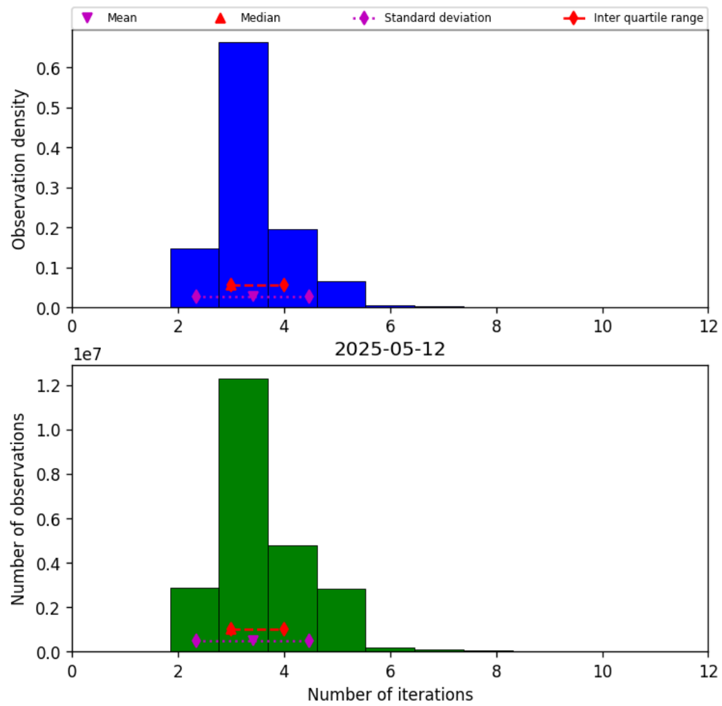
Figure 37: Histogram of “Number of iterations” for 2025-05-12 to 2025-05-13
