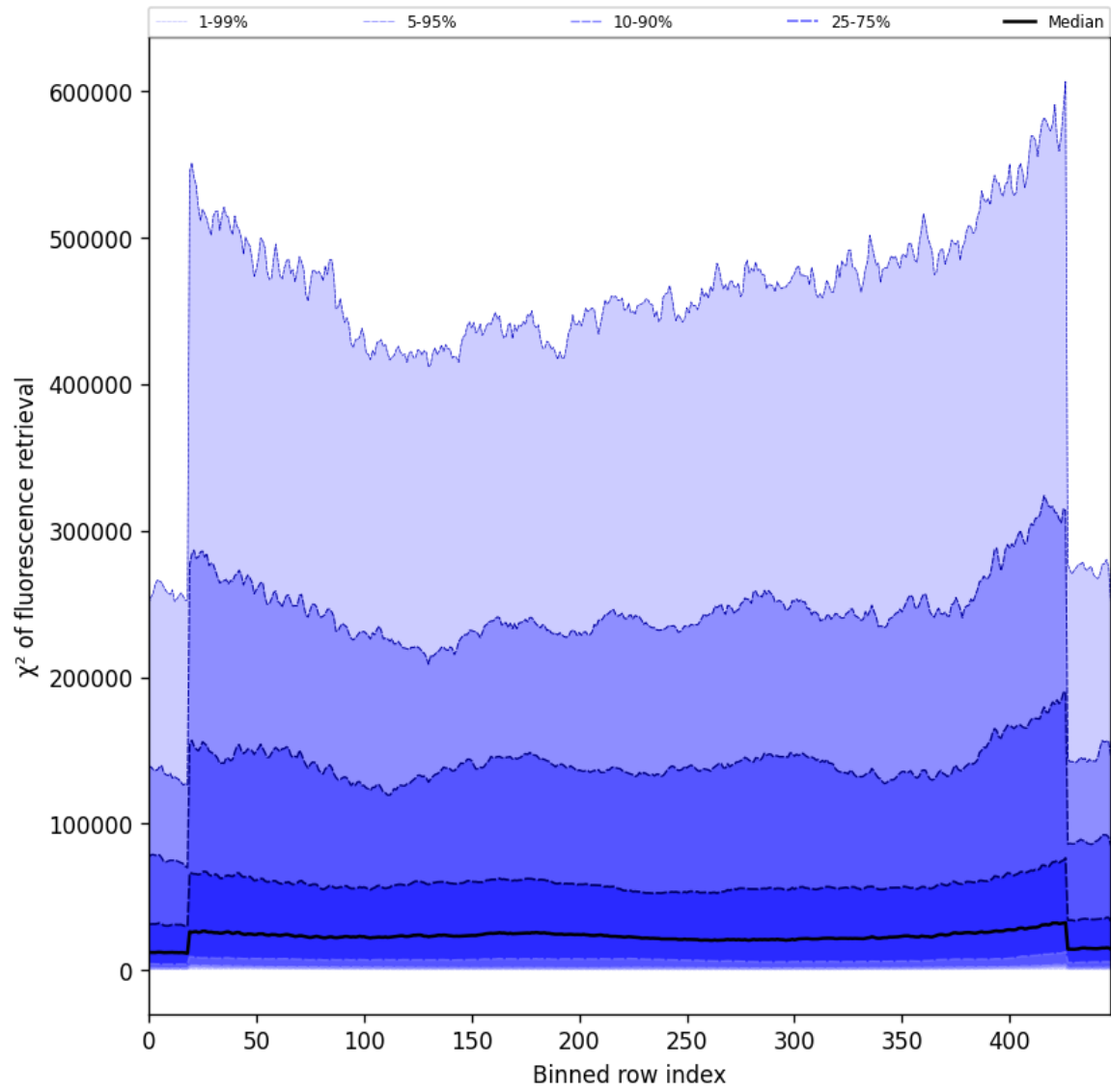
Figure 57: Along track statistics of “ \chi^2 of fluorescence retrieval” for 2025-05-12 to 2025-05-13
