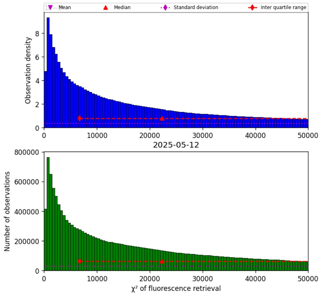
Figure 40: Histogram of “ \chi^2 of fluorescence retrieval” for 2025-05-12 to 2025-05-13
