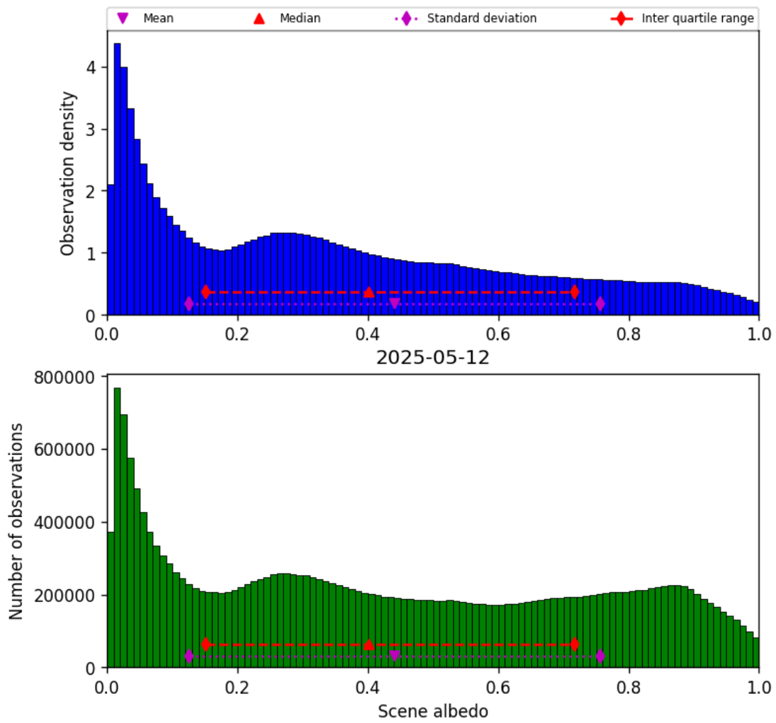
Figure 32: Histogram of “Scene albedo” for 2025-05-12 to 2025-05-13
