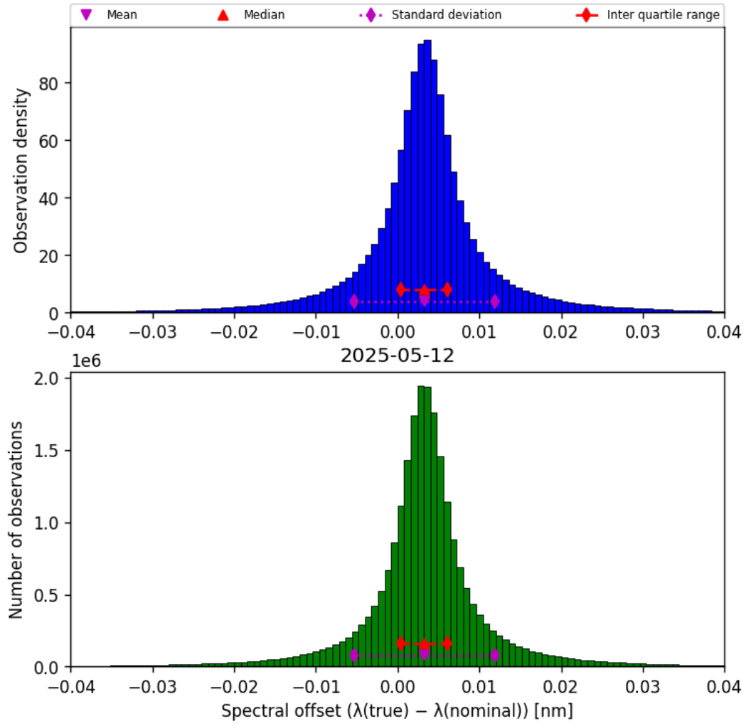
Figure 43: Histogram of “Spectral offset ( \lambda_{\text{true}} - \lambda_{\text{nominal}} )” for 2025-05-12 to 2025-05-13
