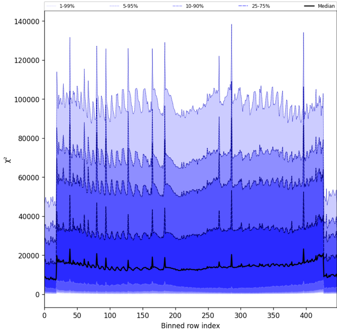
Figure 53: Along track statistics of “ \chi^2 ” for 2025-05-12 to 2025-05-13
