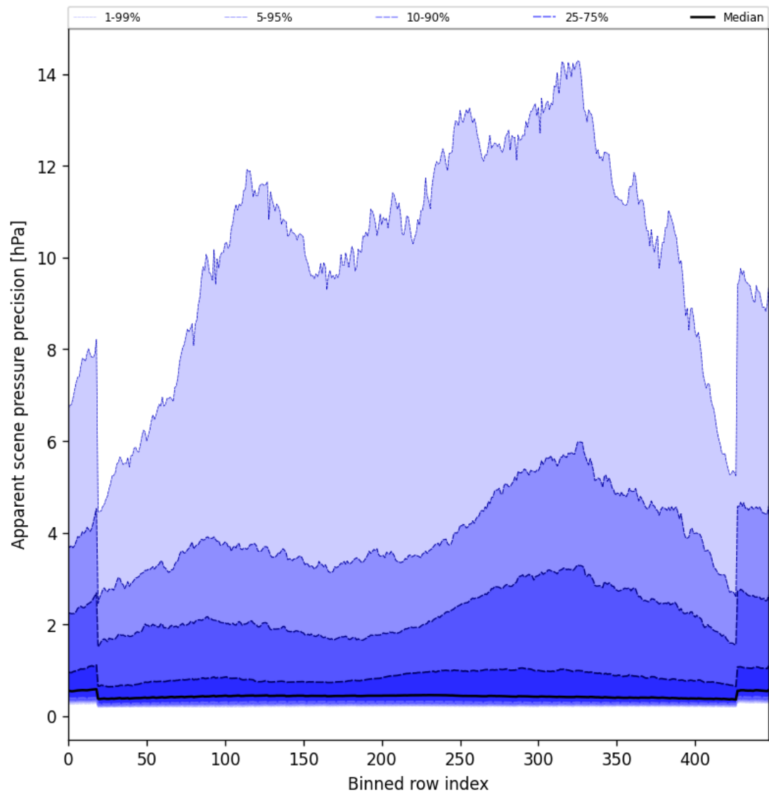
Figure 52: Along track statistics of “Apparent scene pressure precision” for 2025-05-12 to 2025-05-13
