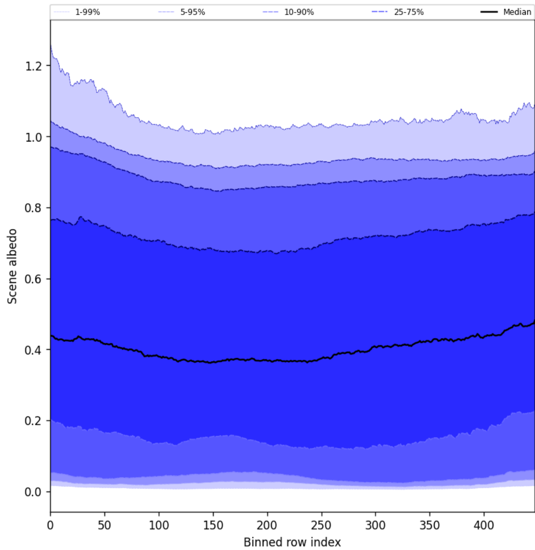
Figure 49: Along track statistics of “Scene albedo” for 2025-05-12 to 2025-05-13
