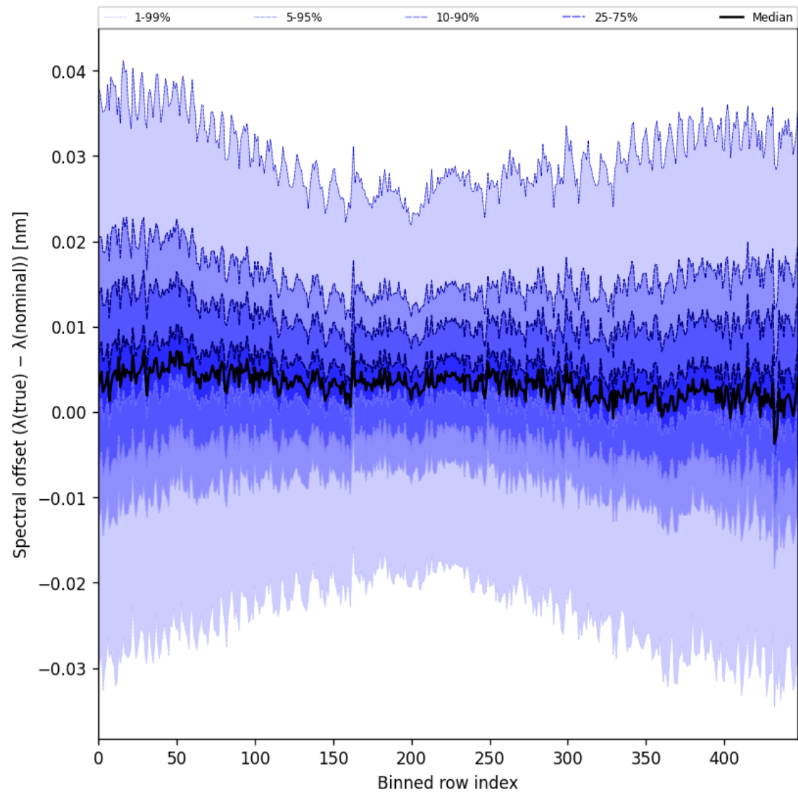
Figure 60: Along track statistics of “Spectral offset ( \lambda_{\text{true}} - \lambda_{\text{nominal}} )” for 2025-05-12 to 2025-05-13
