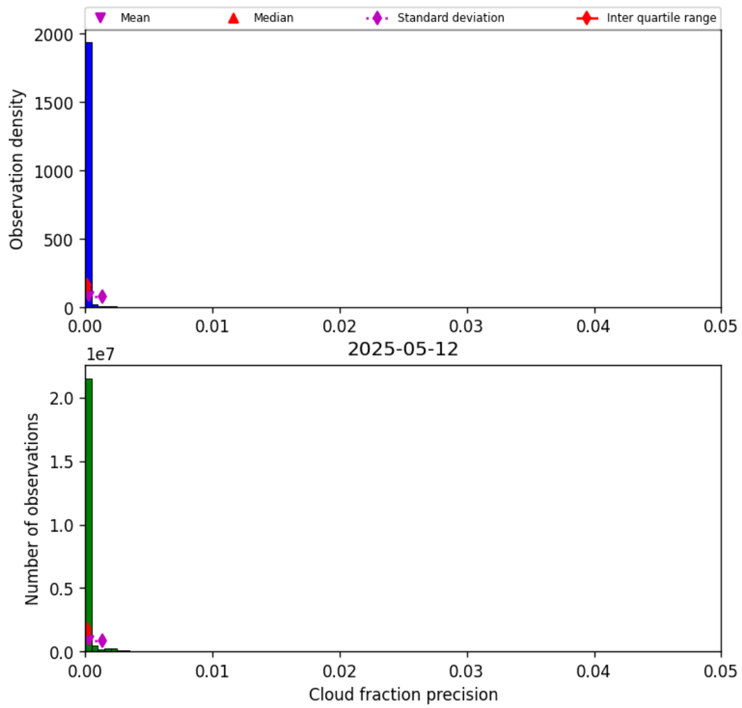
Figure 31: Histogram of “Cloud fraction precision” for 2025-05-12 to 2025-05-13
