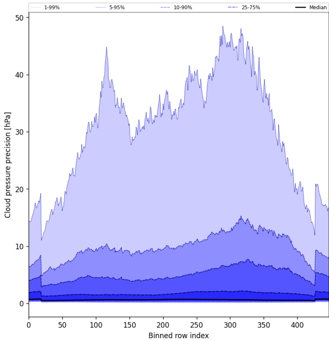
Figure 46: Along track statistics of “Cloud pressure precision” for 2025-05-12 to 2025-05-13
