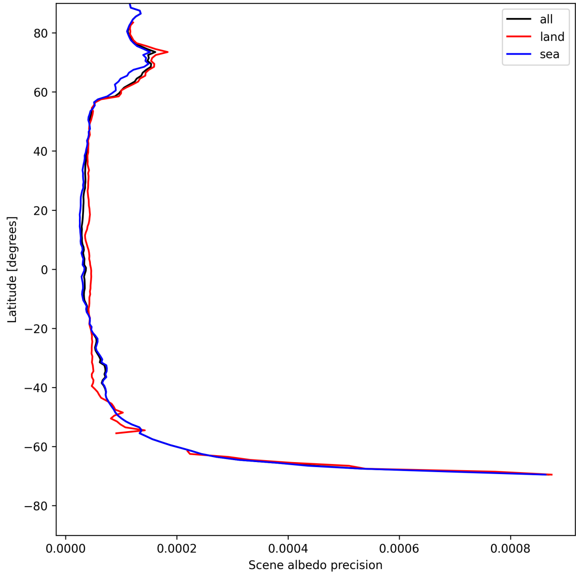
Figure 16: Zonal average of “Scene albedo precision” for 2025-05-12 to 2025-05-13.
