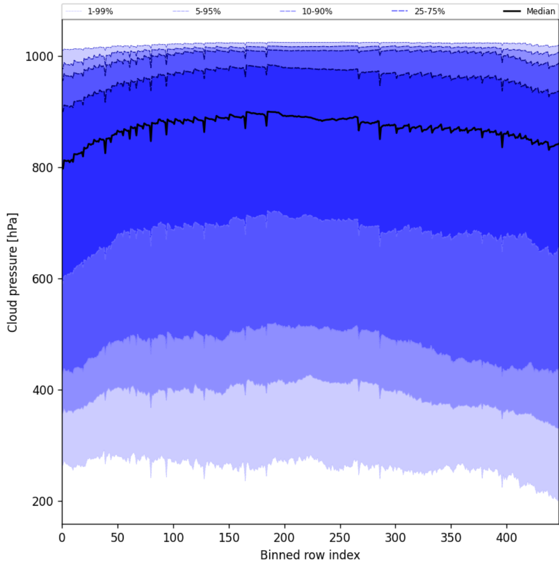
Figure 45: Along track statistics of “Cloud pressure” for 2025-05-12 to 2025-05-13
