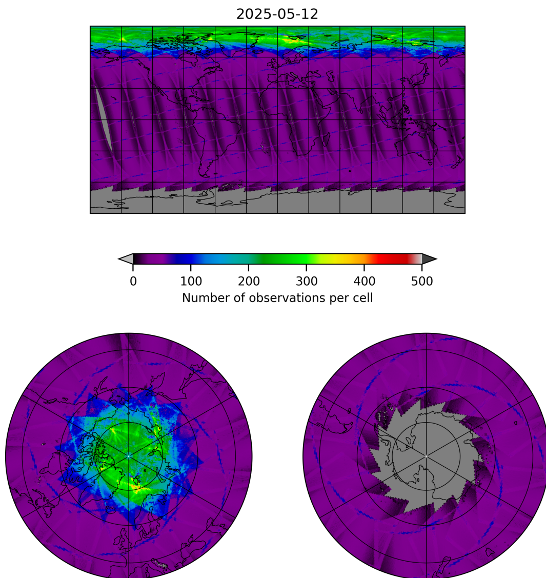
Figure 9: Map of the number of observations for 2025-05-12 to 2025-05-13
