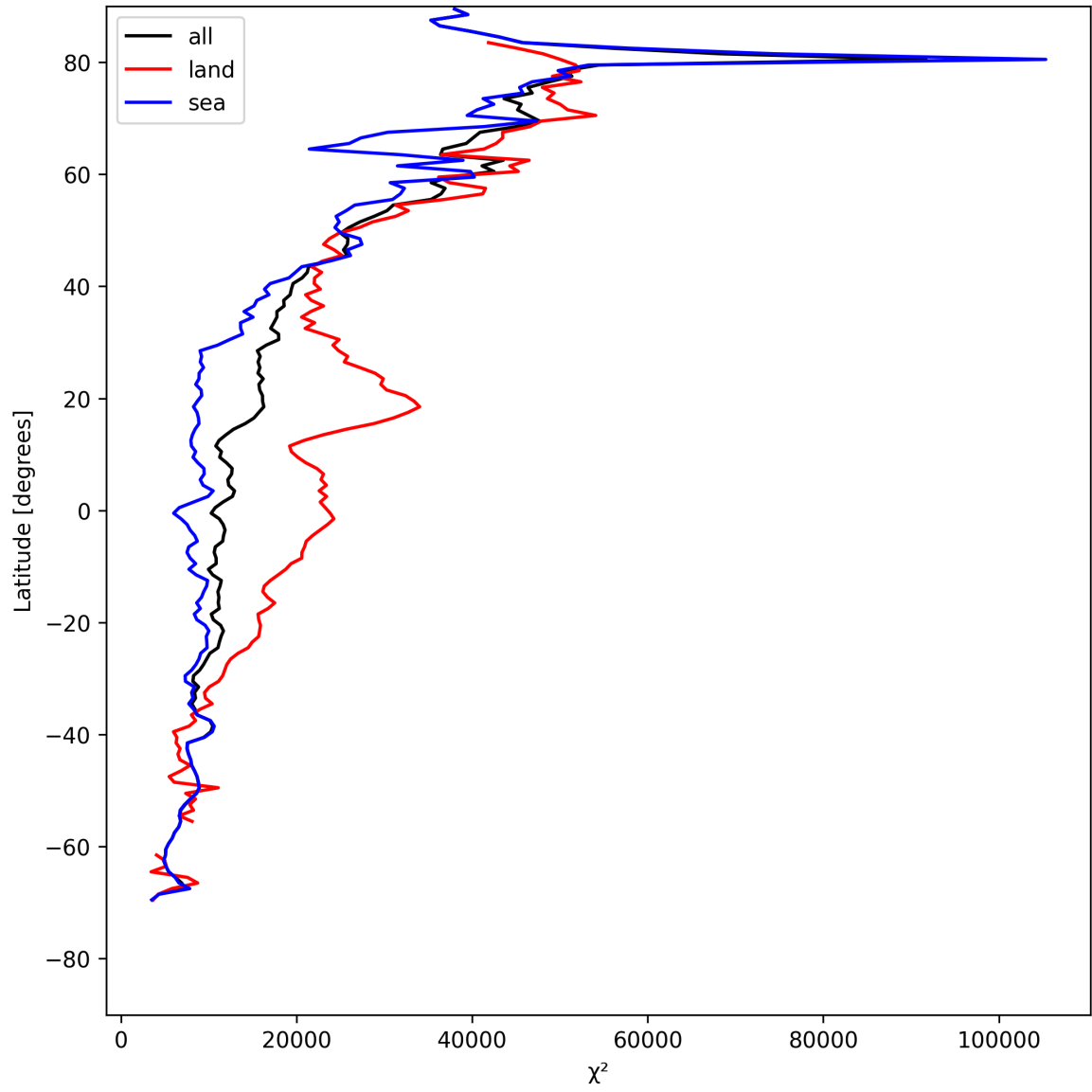
Figure 19: Zonal average of “ \chi^2 ” for 2025-05-12 to 2025-05-13.
