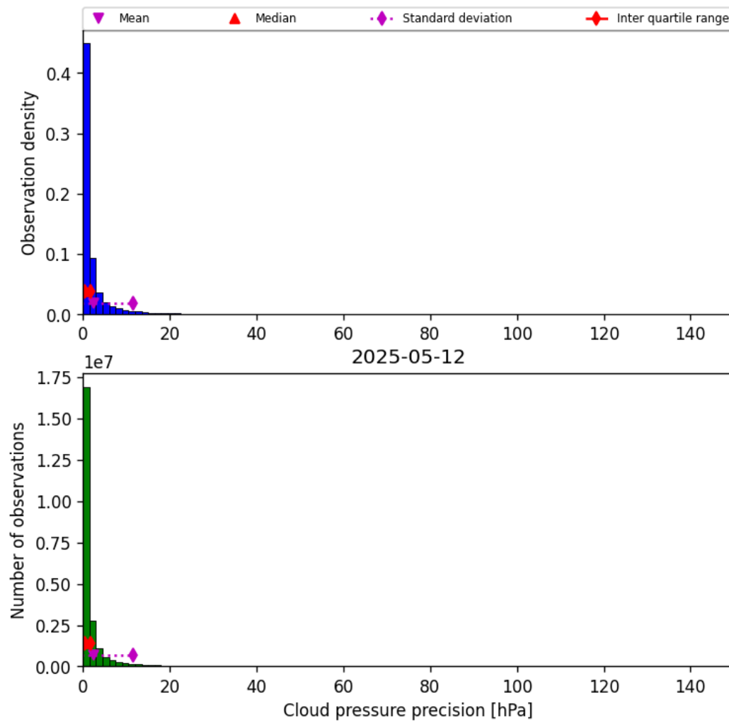
Figure 29: Histogram of “Cloud pressure precision” for 2025-05-12 to 2025-05-13
