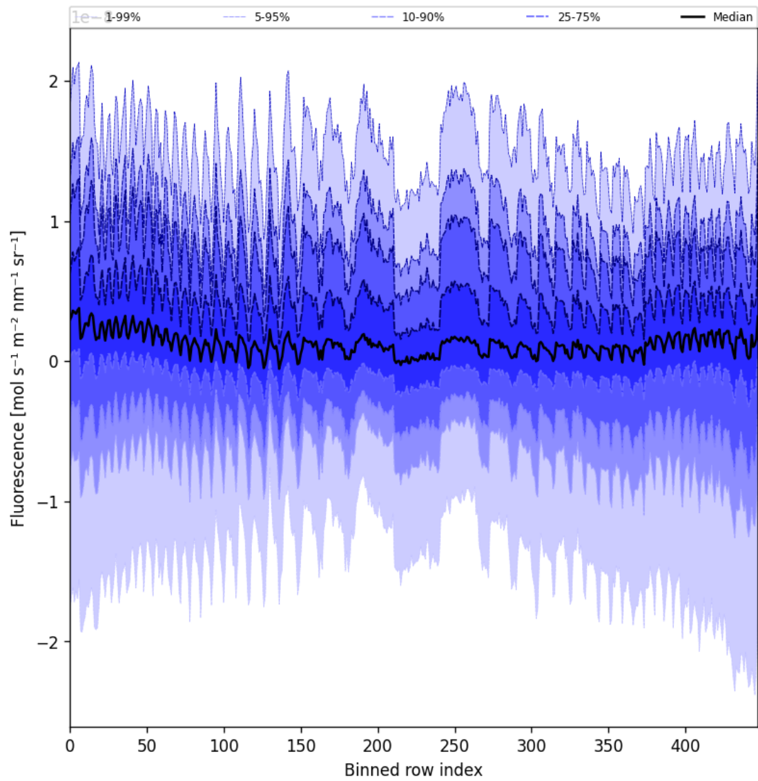
Figure 55: Along track statistics of "Fluorescence" for 2025-05-12 to 2025-05-13
