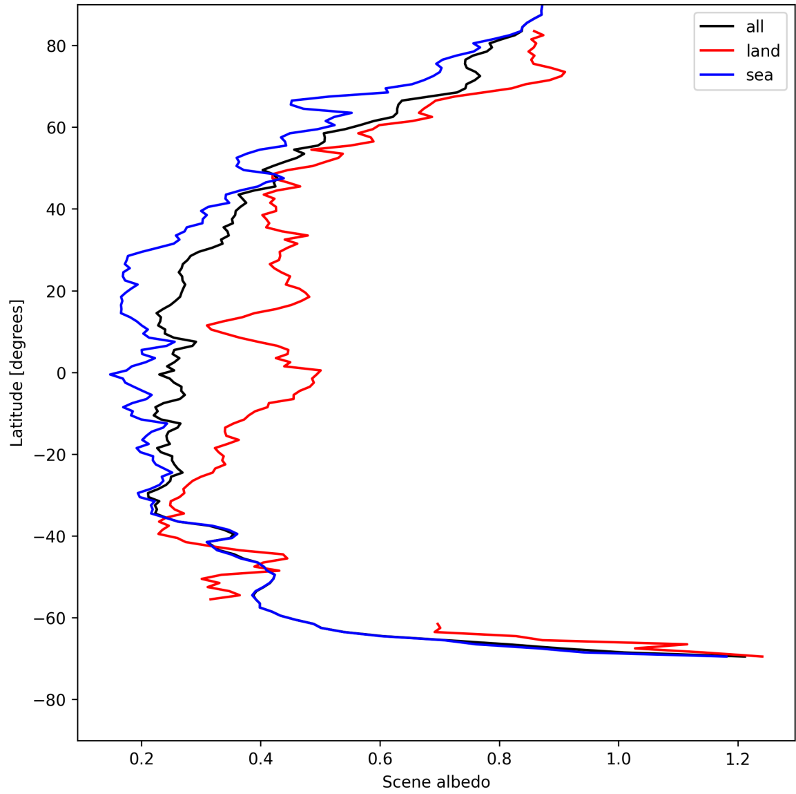
Figure 15: Zonal average of “Scene albedo” for 2025-05-12 to 2025-05-13.
