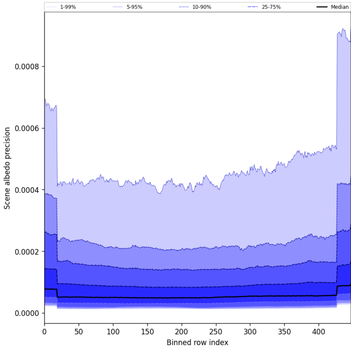
Figure 50: Along track statistics of “Scene albedo precision” for 2025-05-12 to 2025-05-13
