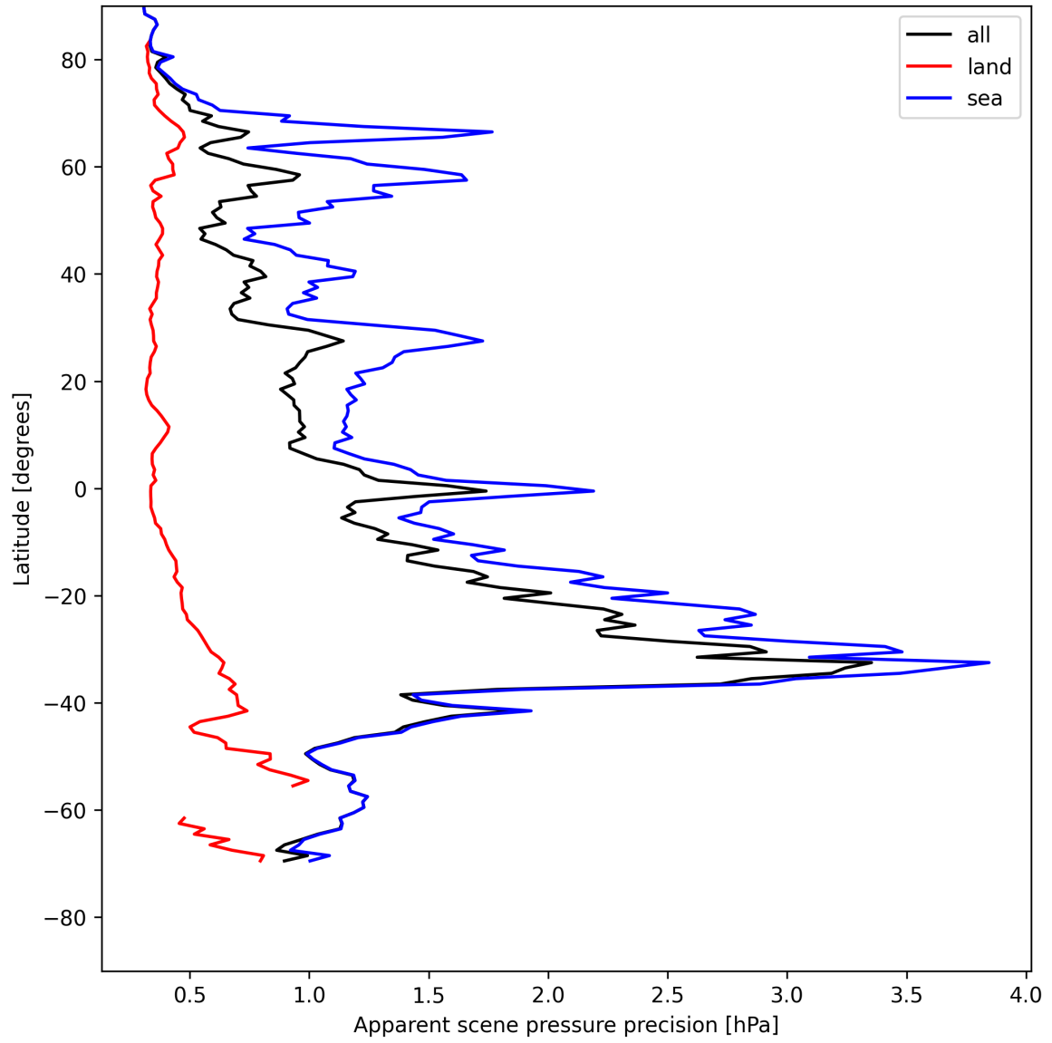
Figure 18: Zonal average of “Apparent scene pressure precision” for 2025-05-12 to 2025-05-13.
