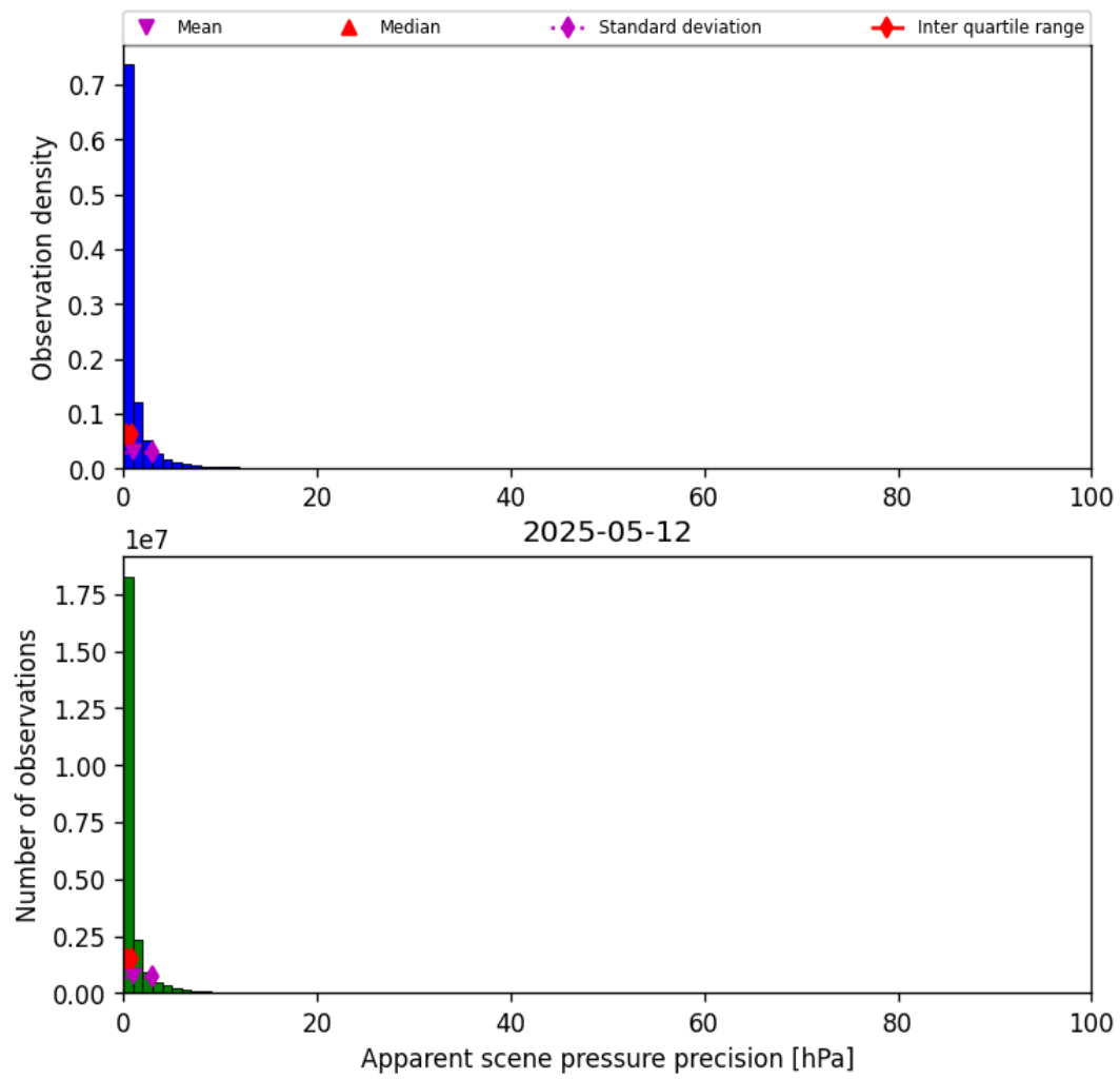
Figure 35: Histogram of “Apparent scene pressure precision” for 2025-05-12 to 2025-05-13
