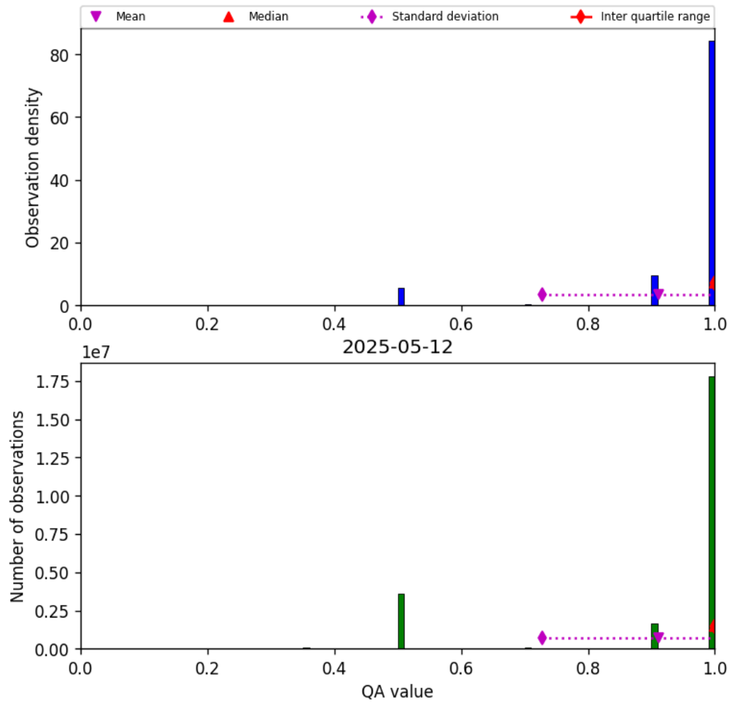
Figure 27: Histogram of “QA value” for 2025-05-12 to 2025-05-13
