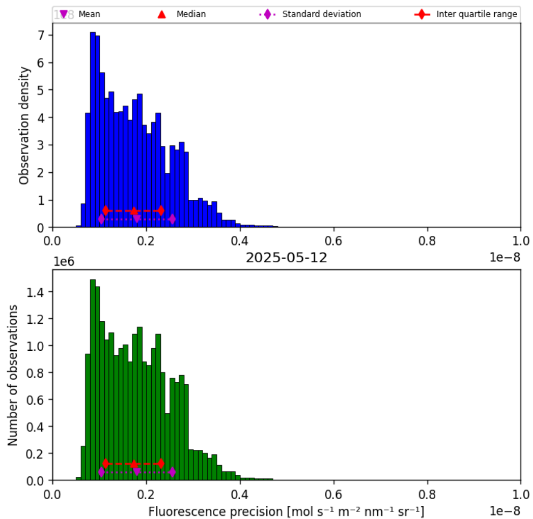
Figure 39: Histogram of “Fluorescence precision” for 2025-05-12 to 2025-05-13
