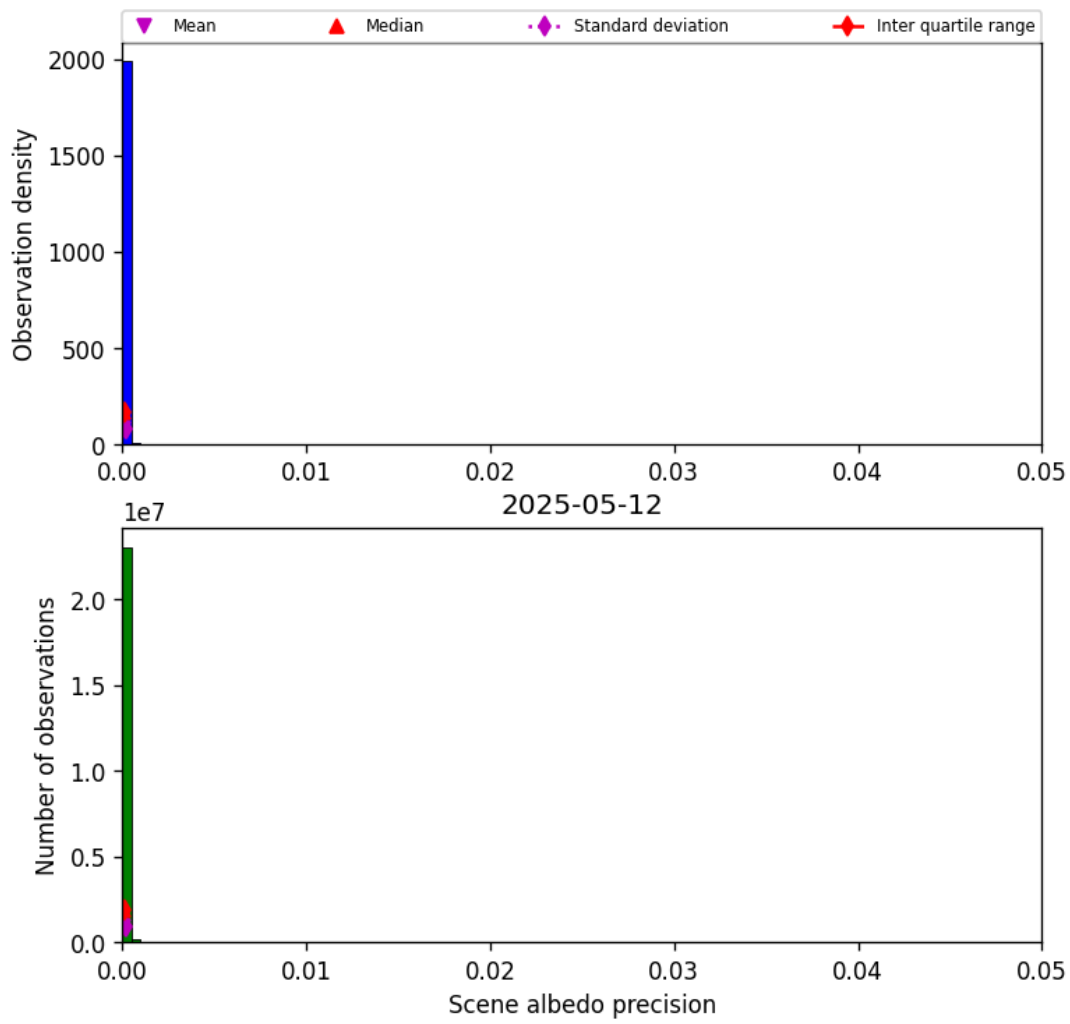
Figure 33: Histogram of “Scene albedo precision” for 2025-05-12 to 2025-05-13
