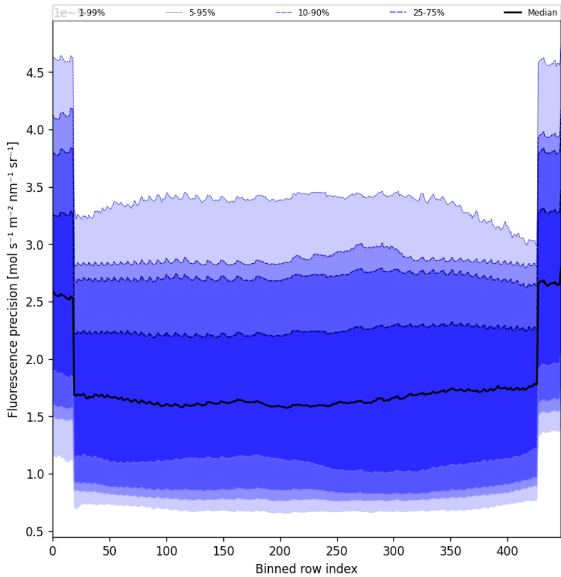
Figure 56: Along track statistics of “Fluorescence precision” for 2025-05-12 to 2025-05-13
