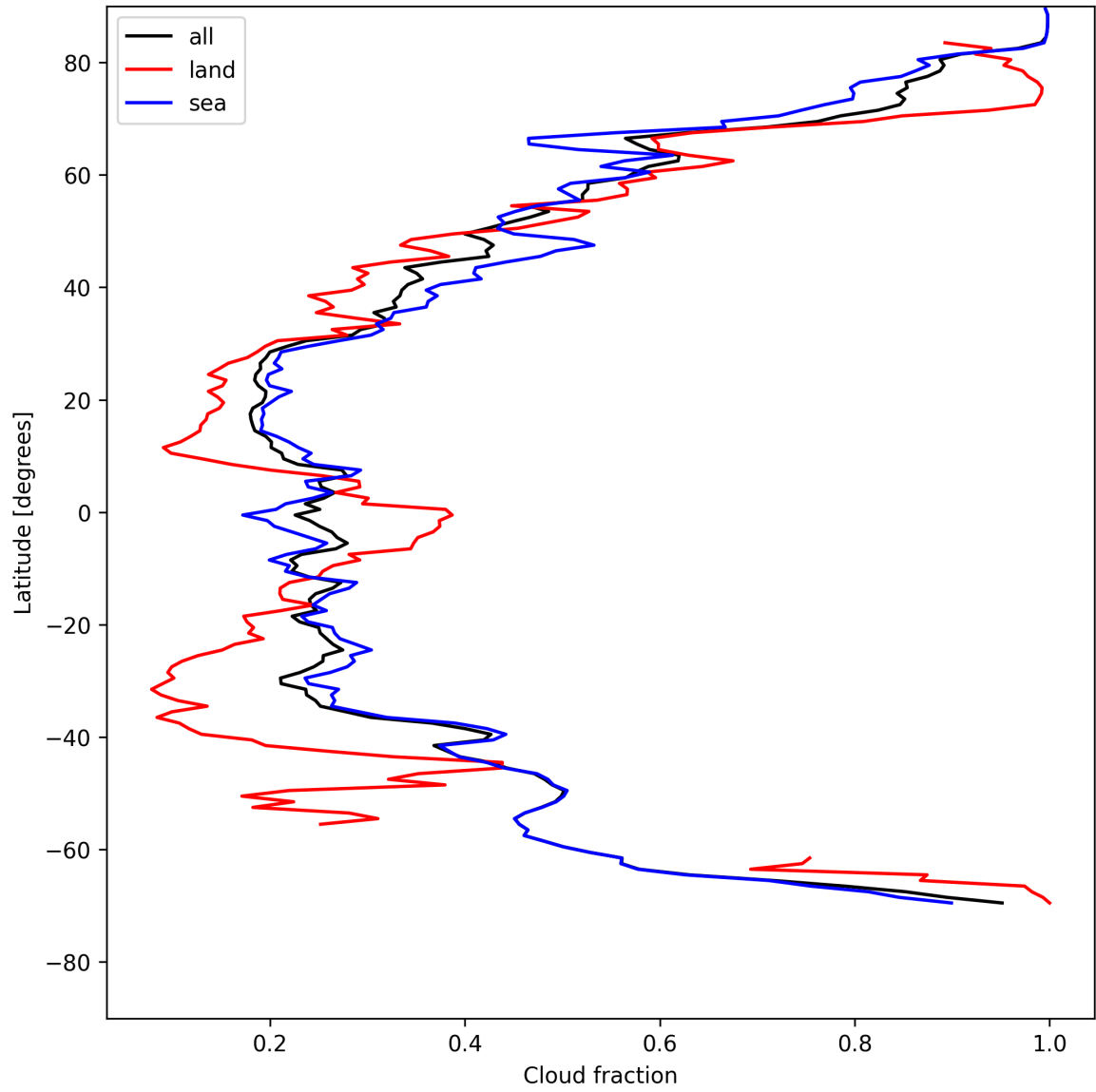
Figure 13: Zonal average of “Cloud fraction” for 2025-05-12 to 2025-05-13.
