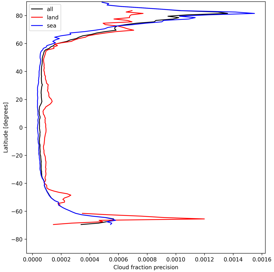
Figure 14: Zonal average of “Cloud fraction precision” for 2025-05-12 to 2025-05-13.
