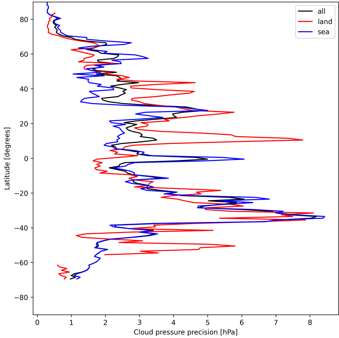
Figure 12: Zonal average of “Cloud pressure precision” for 2025-05-12 to 2025-05-13.
