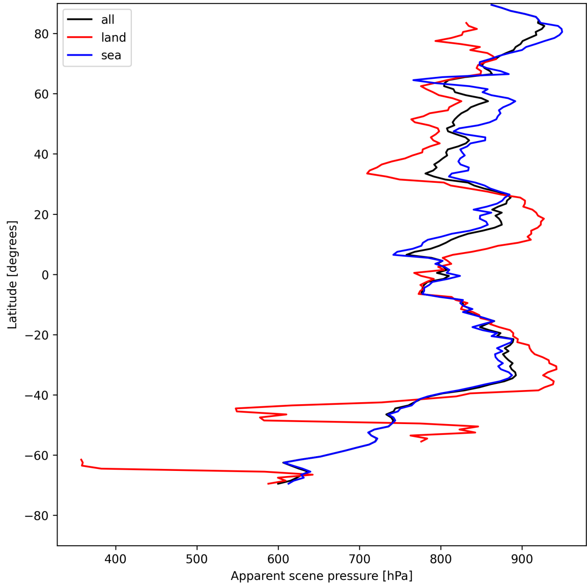
Figure 17: Zonal average of “Apparent scene pressure” for 2025-05-12 to 2025-05-13.
