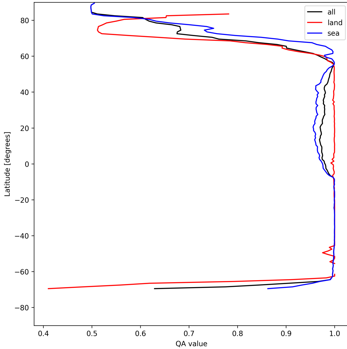
Figure 10: Zonal average of “QA value” for 2025-05-12 to 2025-05-13.
