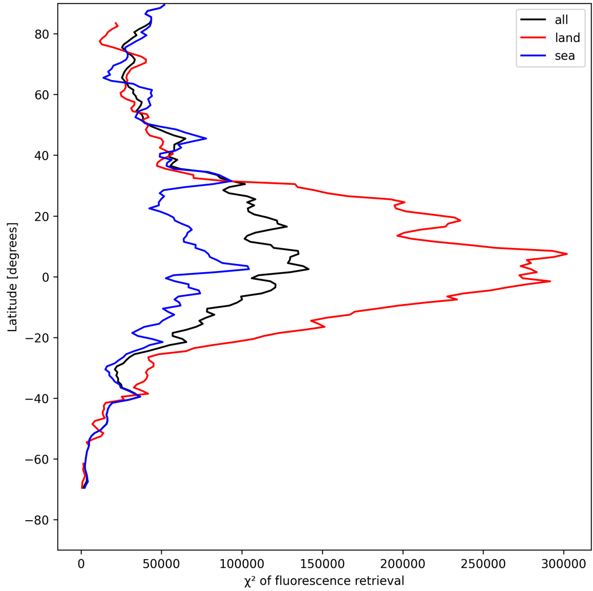
Figure 23: Zonal average of “ \chi^2 of fluorescence retrieval” for 2025-05-12 to 2025-05-13.
