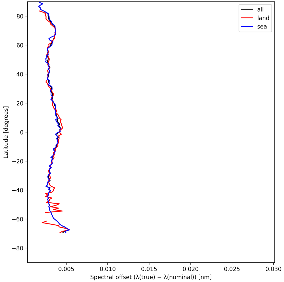
Figure 26: Zonal average of “Spectral offset ( \lambda_{\text{true}} - \lambda_{\text{nominal}} )” for 2025-05-12 to 2025-05-13.
