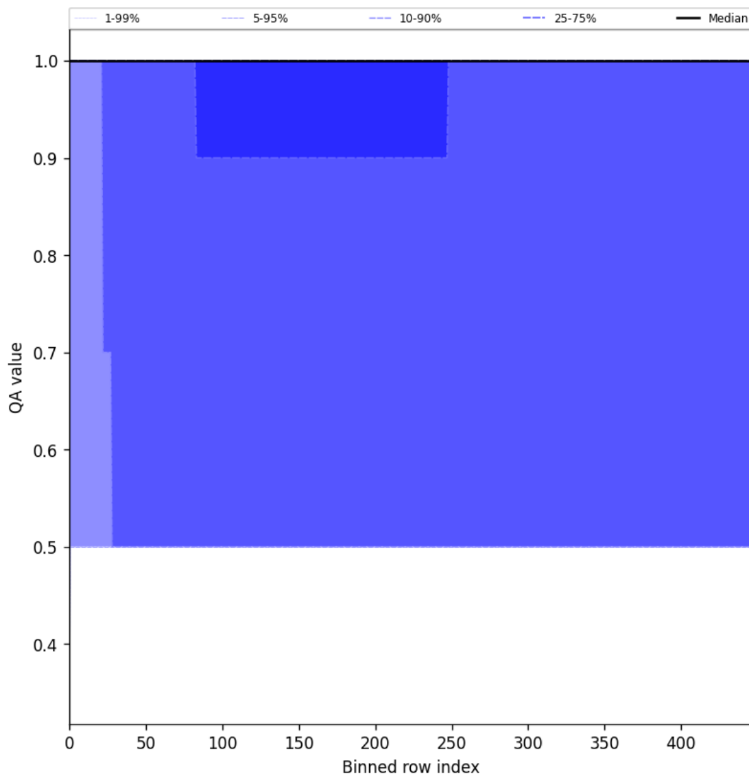
Figure 44: Along track statistics of “QA value” for 2025-05-12 to 2025-05-13
