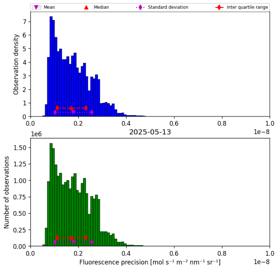
Figure 39: Histogram of “Fluorescence precision” for 2025-05-13 to 2025-05-13
