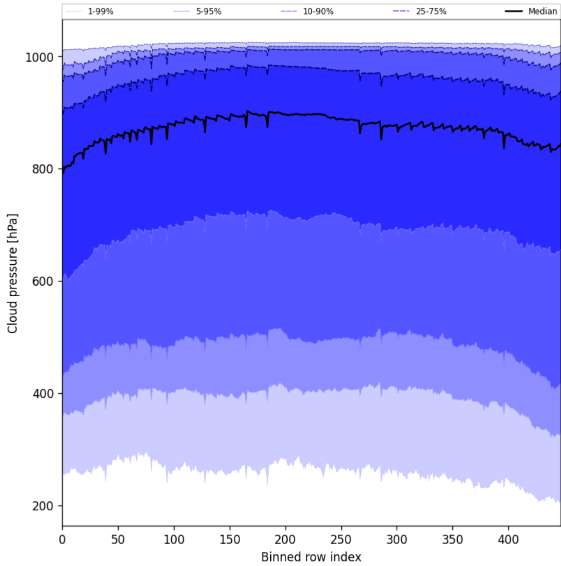
Figure 45: Along track statistics of “Cloud pressure” for 2025-05-13 to 2025-05-13
