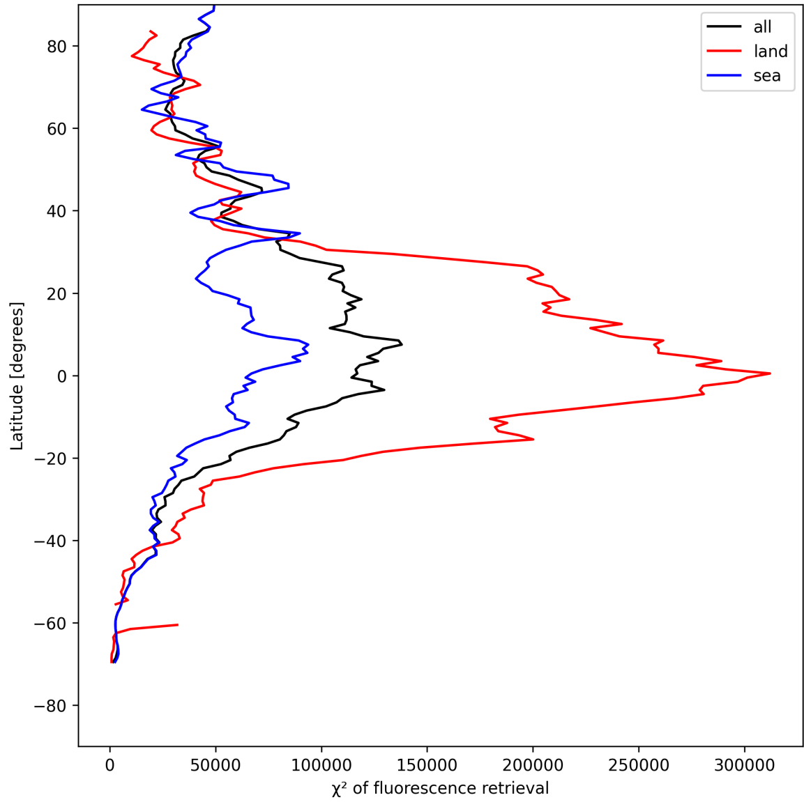
Figure 23: Zonal average of “ \chi^2 of fluorescence retrieval” for 2025-05-13 to 2025-05-13.
