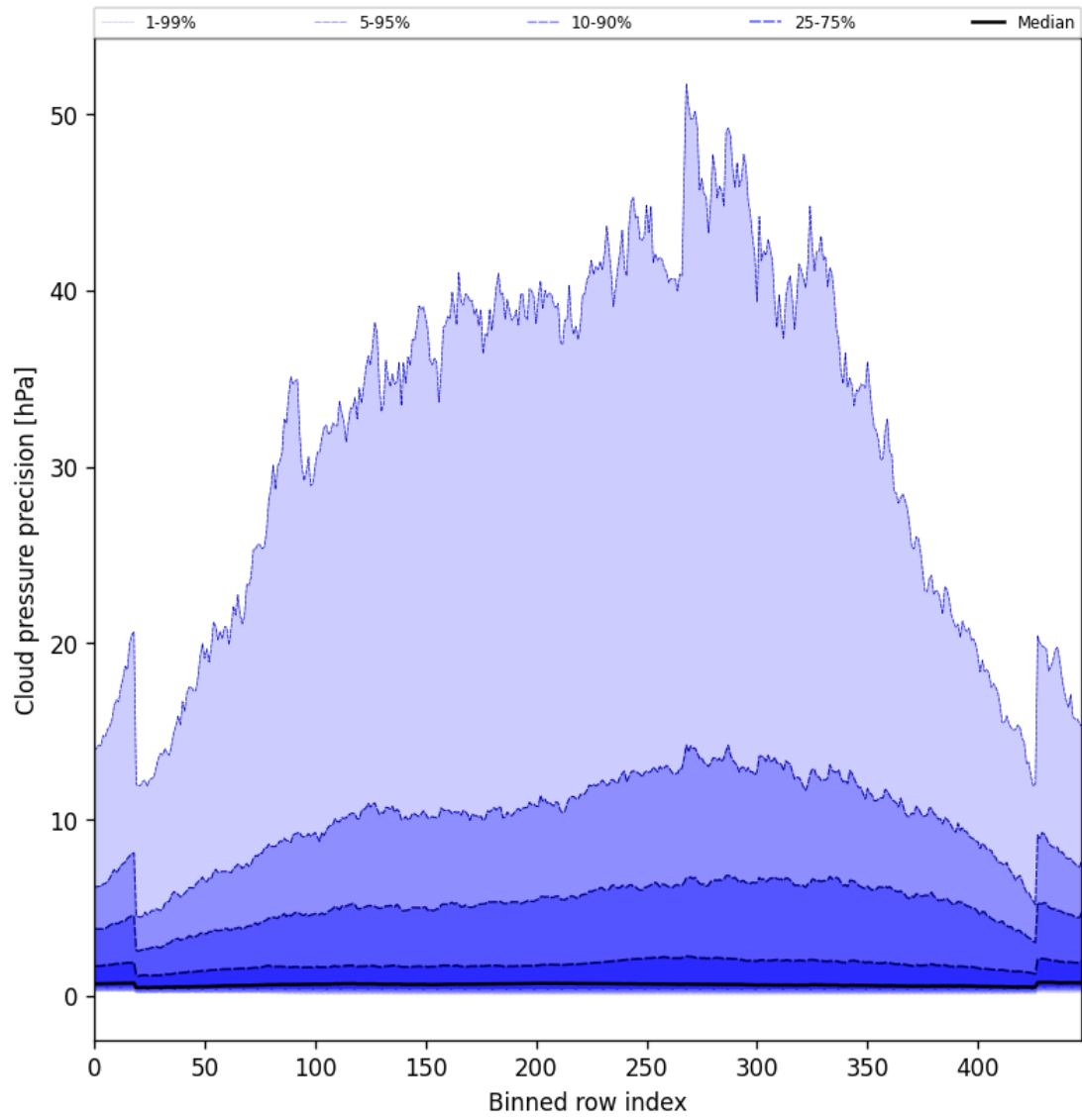
Figure 46: Along track statistics of “Cloud pressure precision” for 2025-05-13 to 2025-05-13
