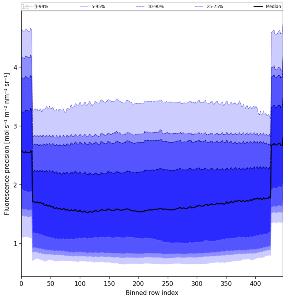
Figure 56: Along track statistics of “Fluorescence precision” for 2025-05-13 to 2025-05-13
