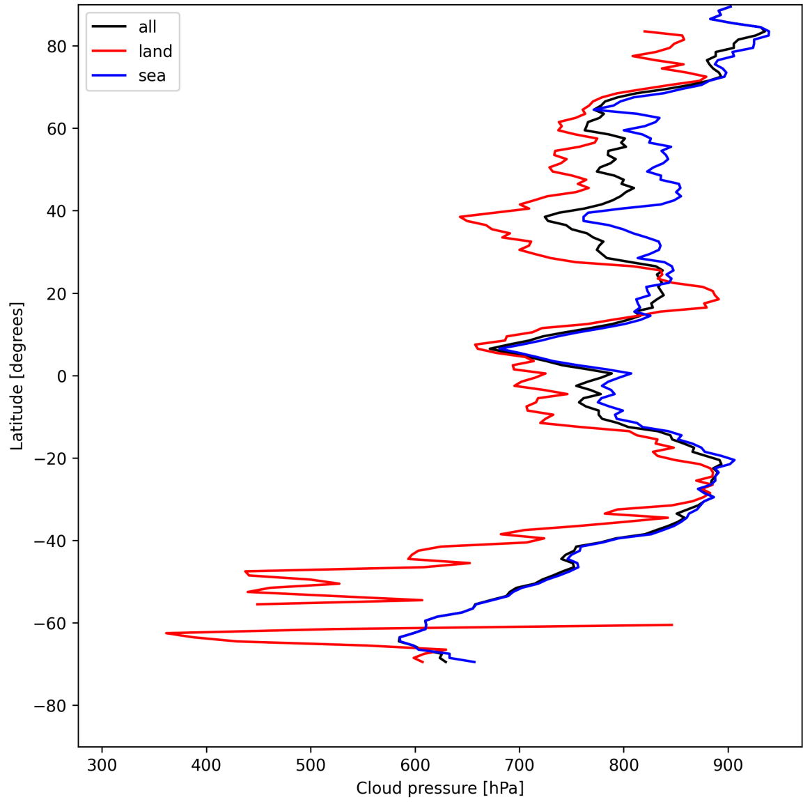
Figure 11: Zonal average of “Cloud pressure” for 2025-05-13 to 2025-05-13.
