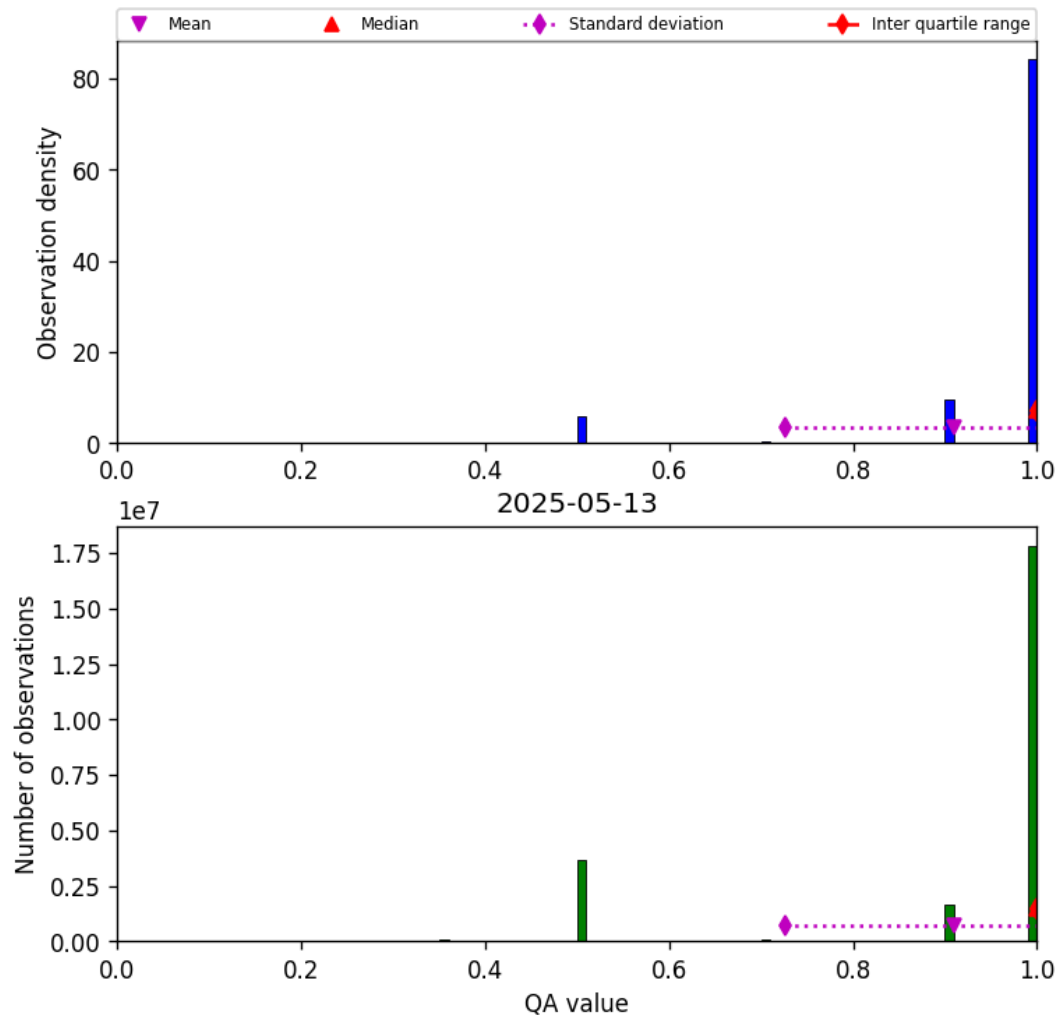
Figure 27: Histogram of “QA value” for 2025-05-13 to 2025-05-13
