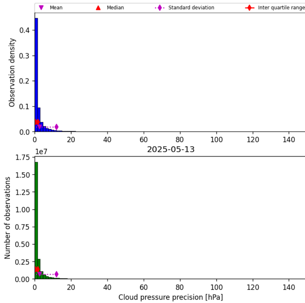
Figure 29: Histogram of “Cloud pressure precision” for 2025-05-13 to 2025-05-13
