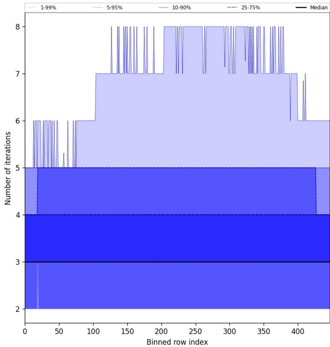
Figure 54: Along track statistics of “Number of iterations” for 2025-05-13 to 2025-05-13
