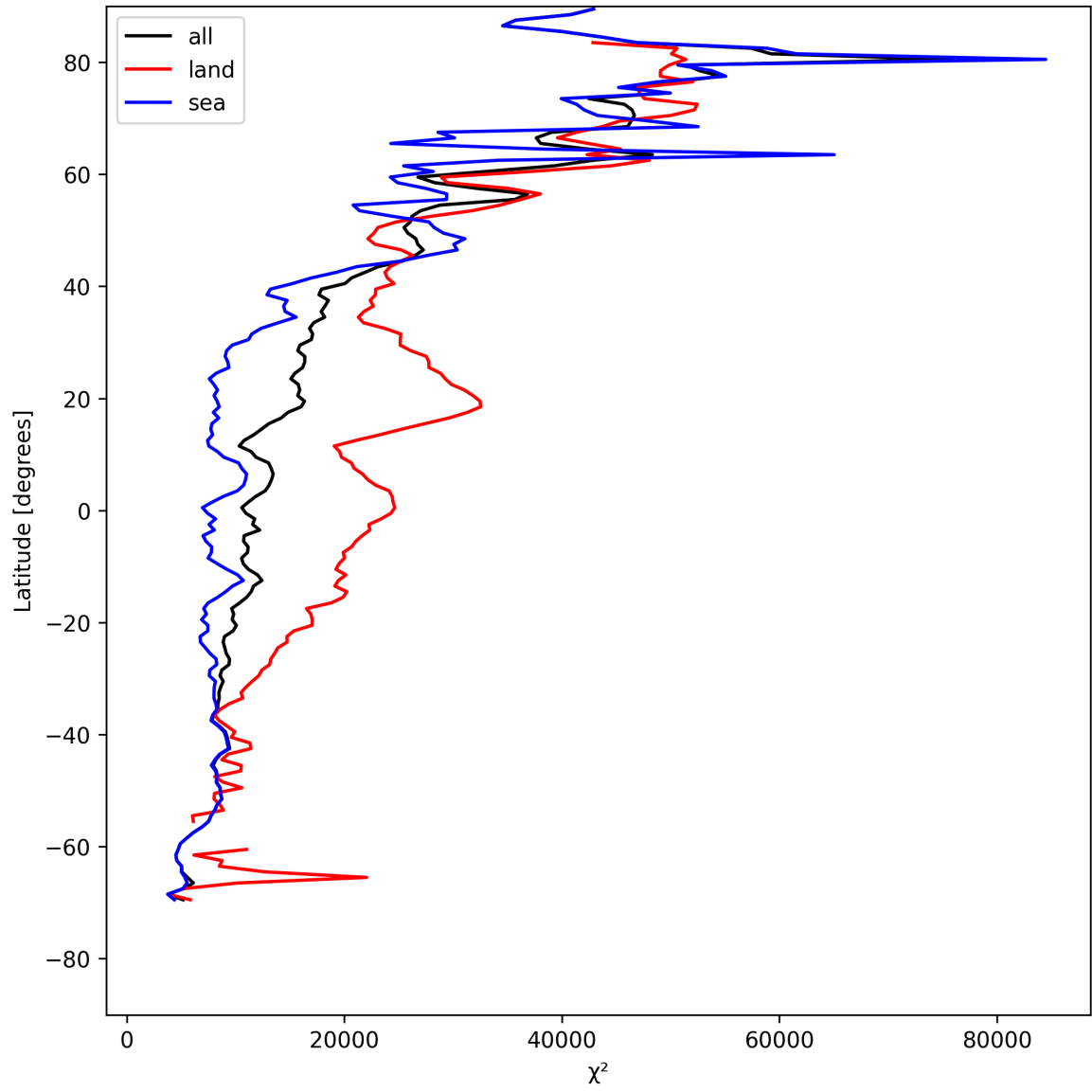
Figure 19: Zonal average of “ \chi^2 ” for 2025-05-13 to 2025-05-13.
