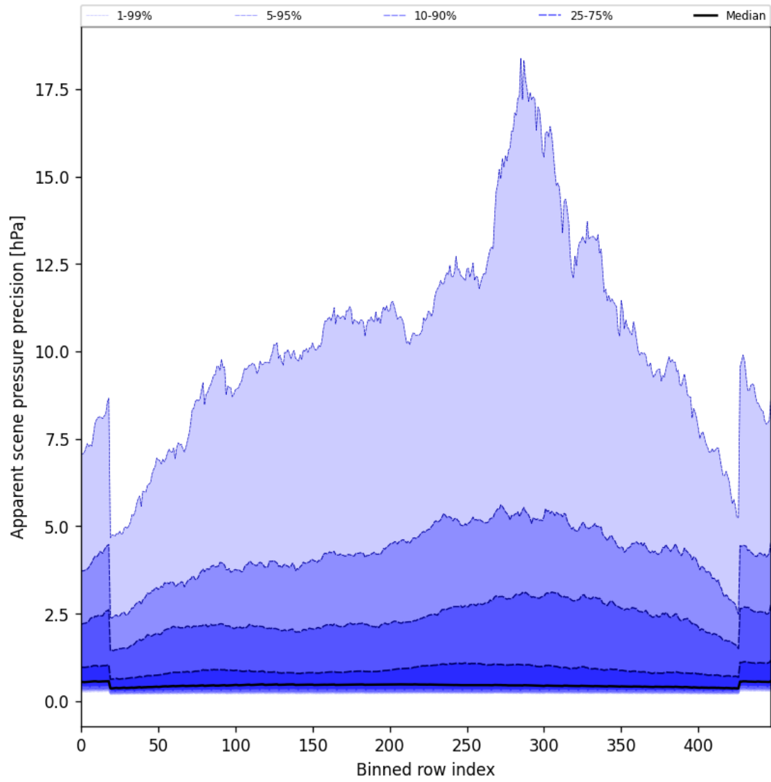
Figure 52: Along track statistics of “Apparent scene pressure precision” for 2025-05-13 to 2025-05-13
