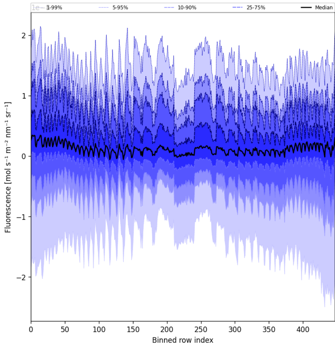
Figure 55: Along track statistics of “Fluorescence” for 2025-05-13 to 2025-05-13
