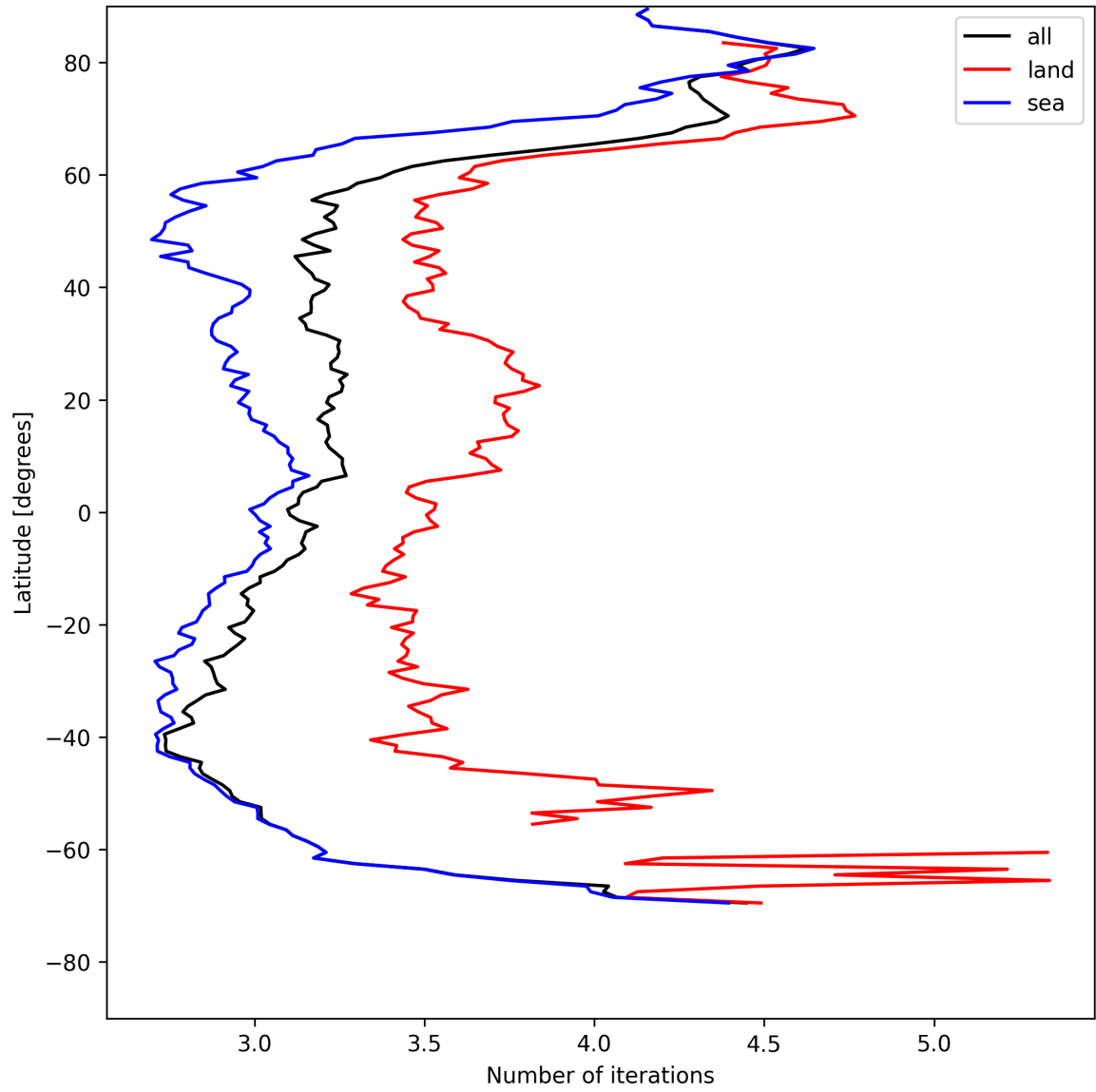
Figure 20: Zonal average of “Number of iterations” for 2025-05-13 to 2025-05-13.
