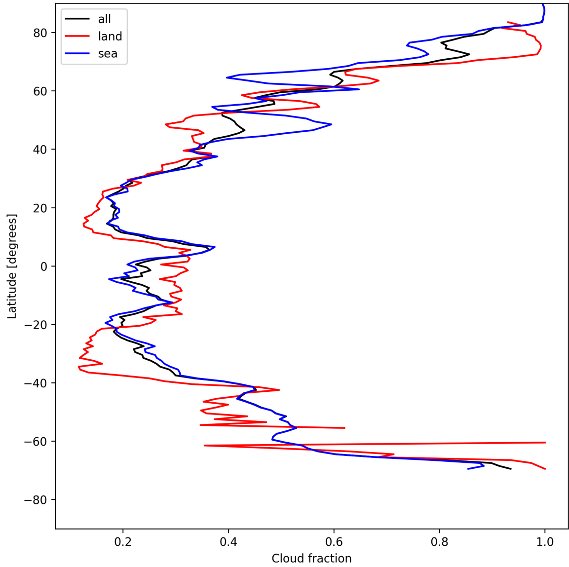
Figure 13: Zonal average of “Cloud fraction” for 2025-05-13 to 2025-05-13.
