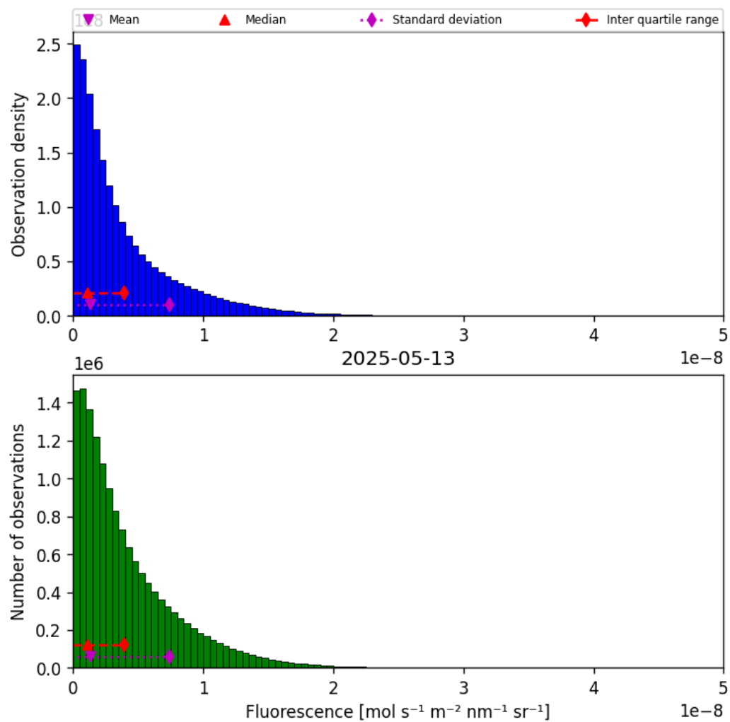
Figure 38: Histogram of “Fluorescence” for 2025-05-13 to 2025-05-13
