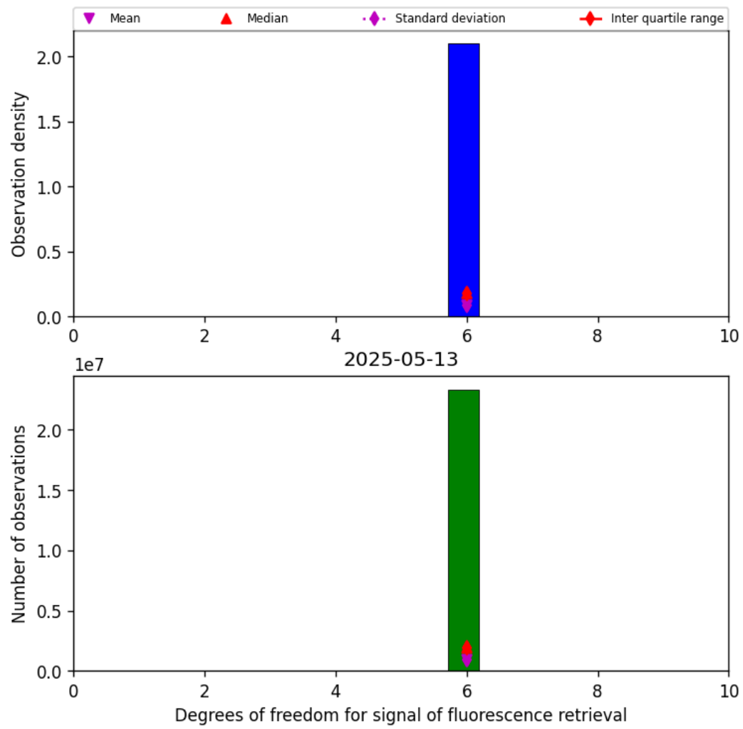
Figure 41: Histogram of “Degrees of freedom for signal of fluorescence retrieval” for 2025-05-13 to 2025-05-13
