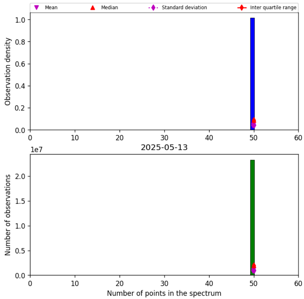
Figure 42: Histogram of "Number of points in the spectrum" for 2025-05-13 to 2025-05-13
