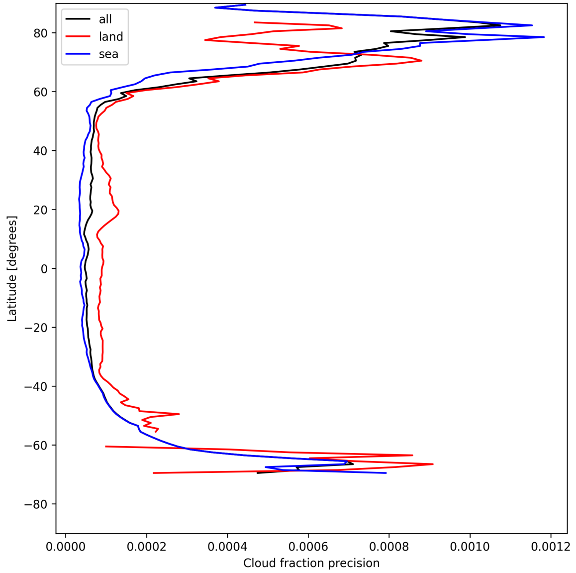
Figure 14: Zonal average of “Cloud fraction precision” for 2025-05-13 to 2025-05-13.
