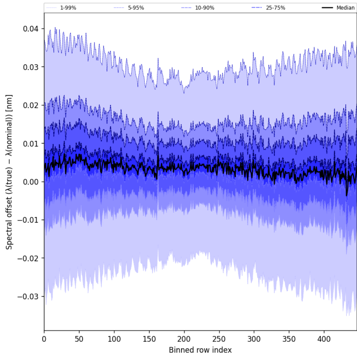
Figure 60: Along track statistics of “Spectral offset ( \lambda_{\text{true}} - \lambda_{\text{nominal}} )” for 2025-05-13 to 2025-05-13
