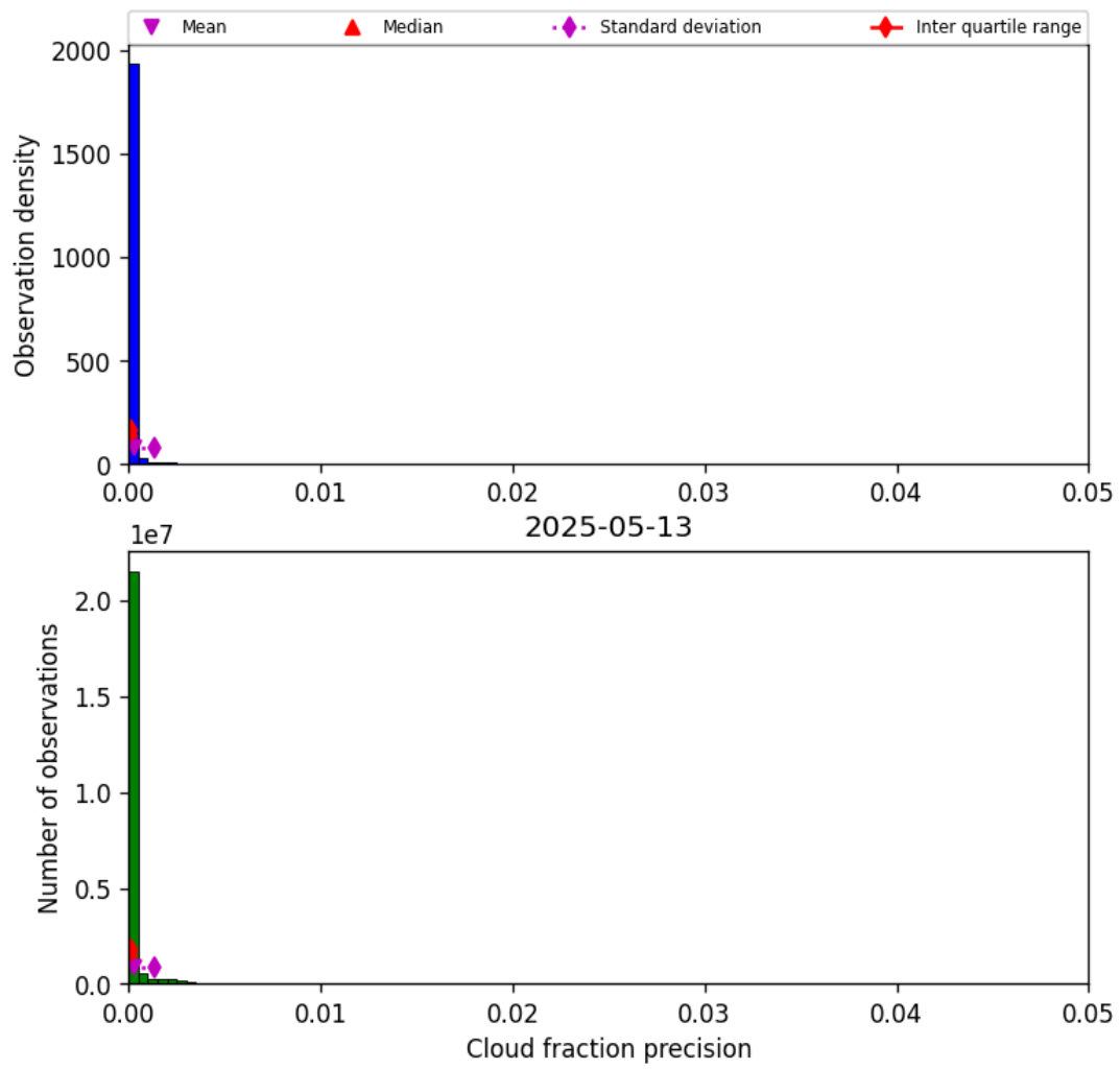
Figure 31: Histogram of “Cloud fraction precision” for 2025-05-13 to 2025-05-13
