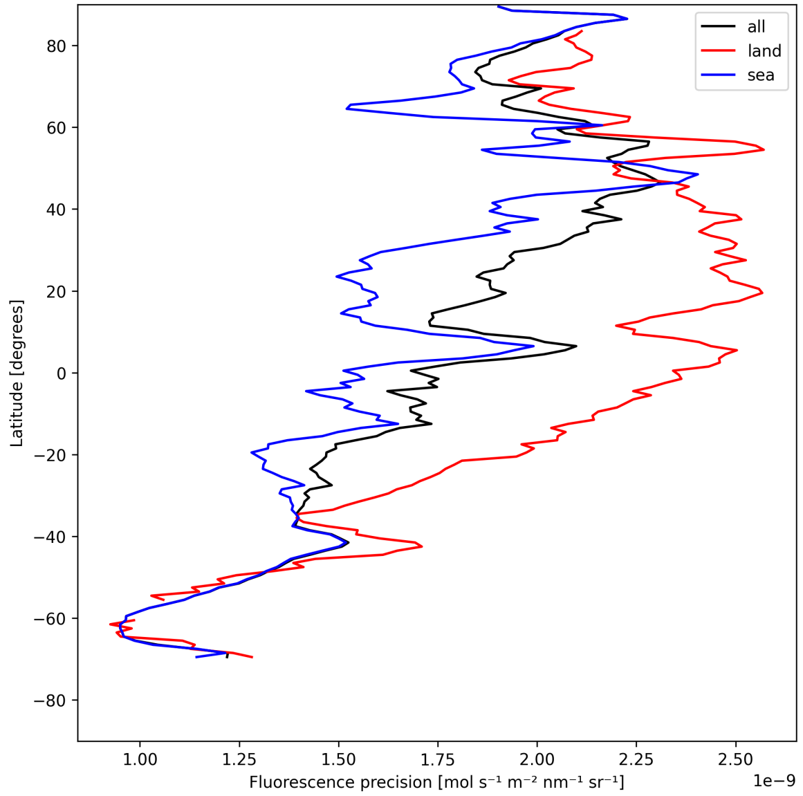
Figure 22: Zonal average of “Fluorescence precision” for 2025-05-13 to 2025-05-13.
