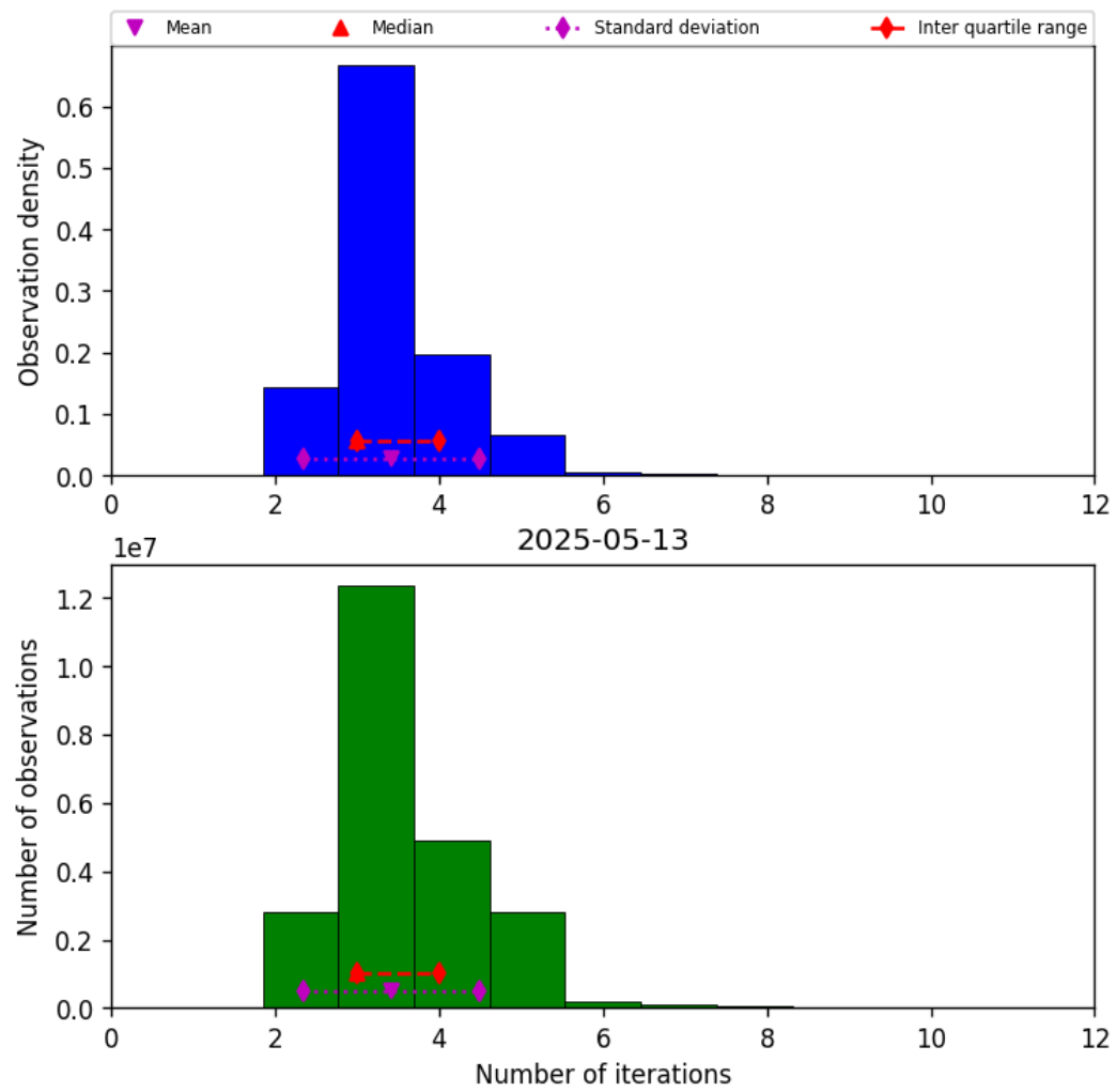
Figure 37: Histogram of “Number of iterations” for 2025-05-13 to 2025-05-13
