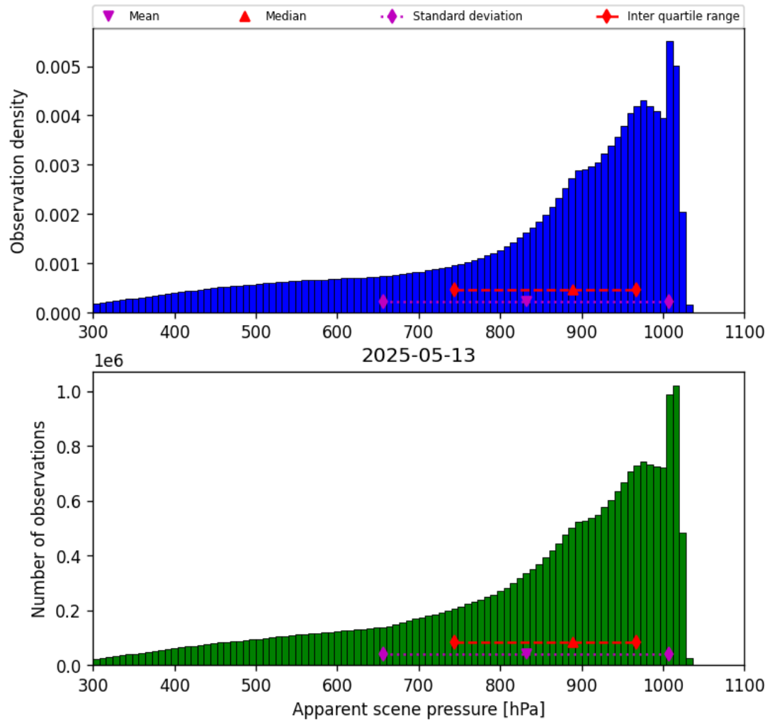
Figure 34: Histogram of “Apparent scene pressure” for 2025-05-13 to 2025-05-13
