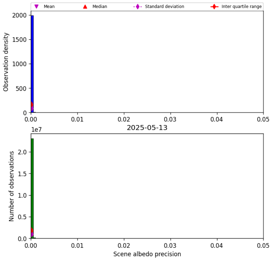
Figure 33: Histogram of "Scene albedo precision" for 2025-05-13 to 2025-05-13
