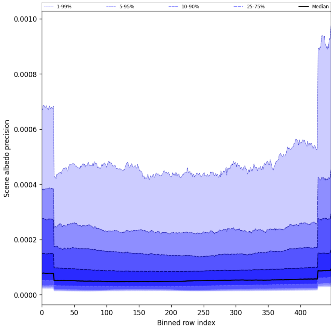
Figure 50: Along track statistics of “Scene albedo precision” for 2025-05-13 to 2025-05-13
