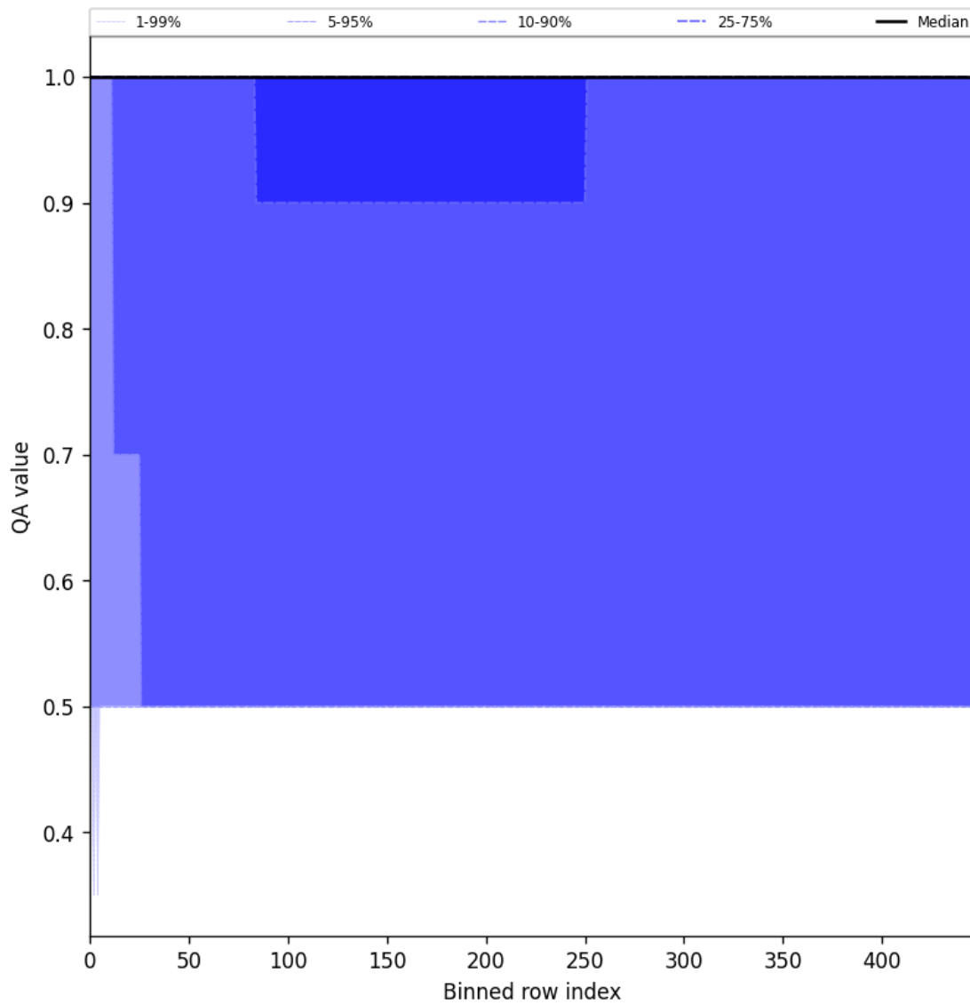
Figure 44: Along track statistics of “QA value” for 2025-05-13 to 2025-05-13
