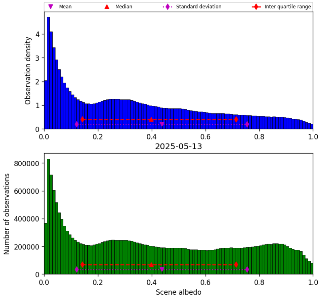
Figure 32: Histogram of “Scene albedo” for 2025-05-13 to 2025-05-13
