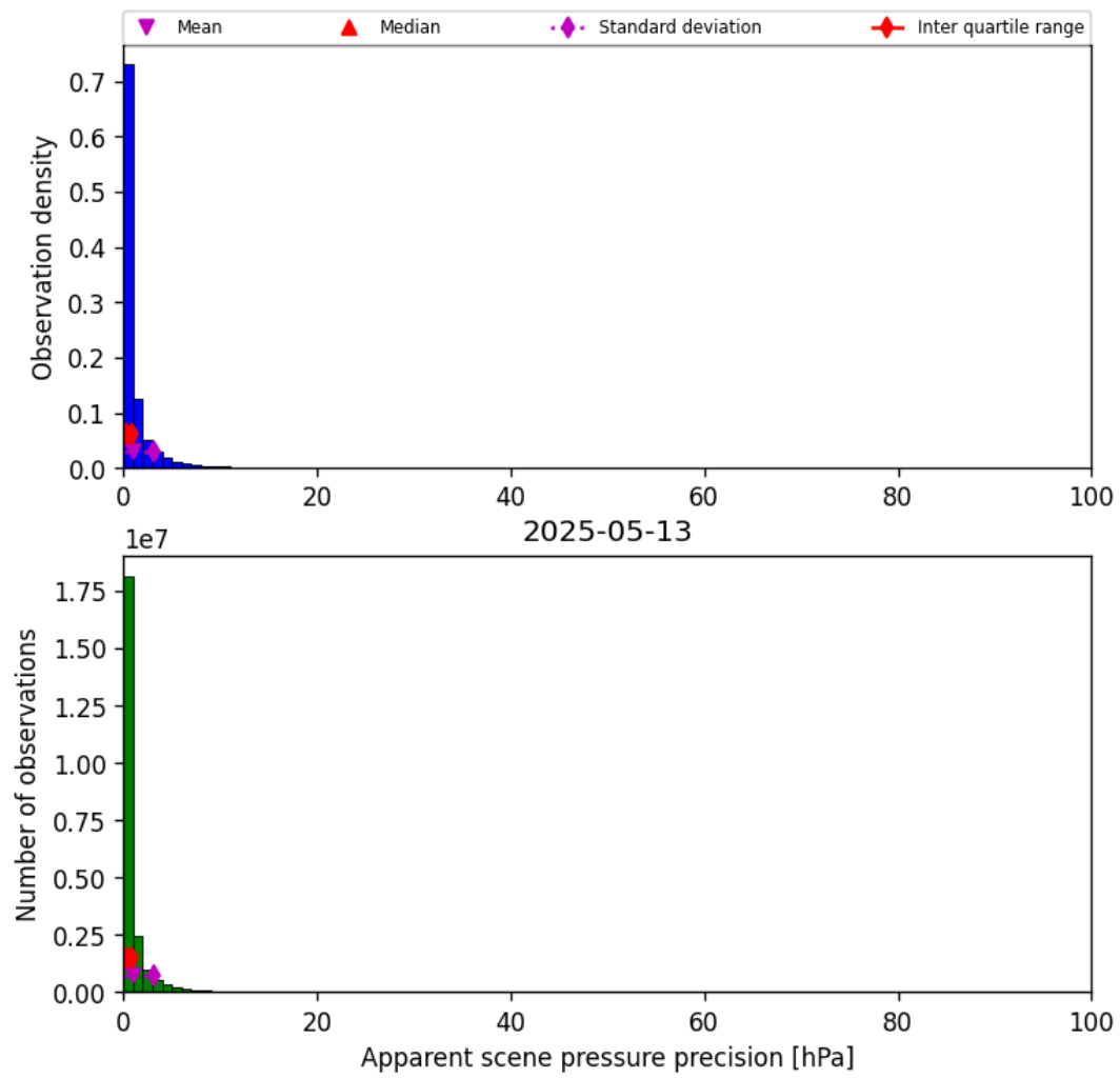
Figure 35: Histogram of “Apparent scene pressure precision” for 2025-05-13 to 2025-05-13
