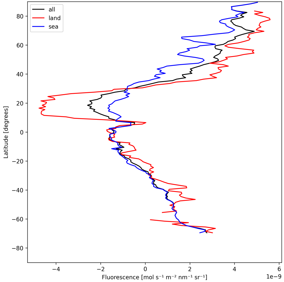
Figure 21: Zonal average of “Fluorescence” for 2025-05-13 to 2025-05-13.
