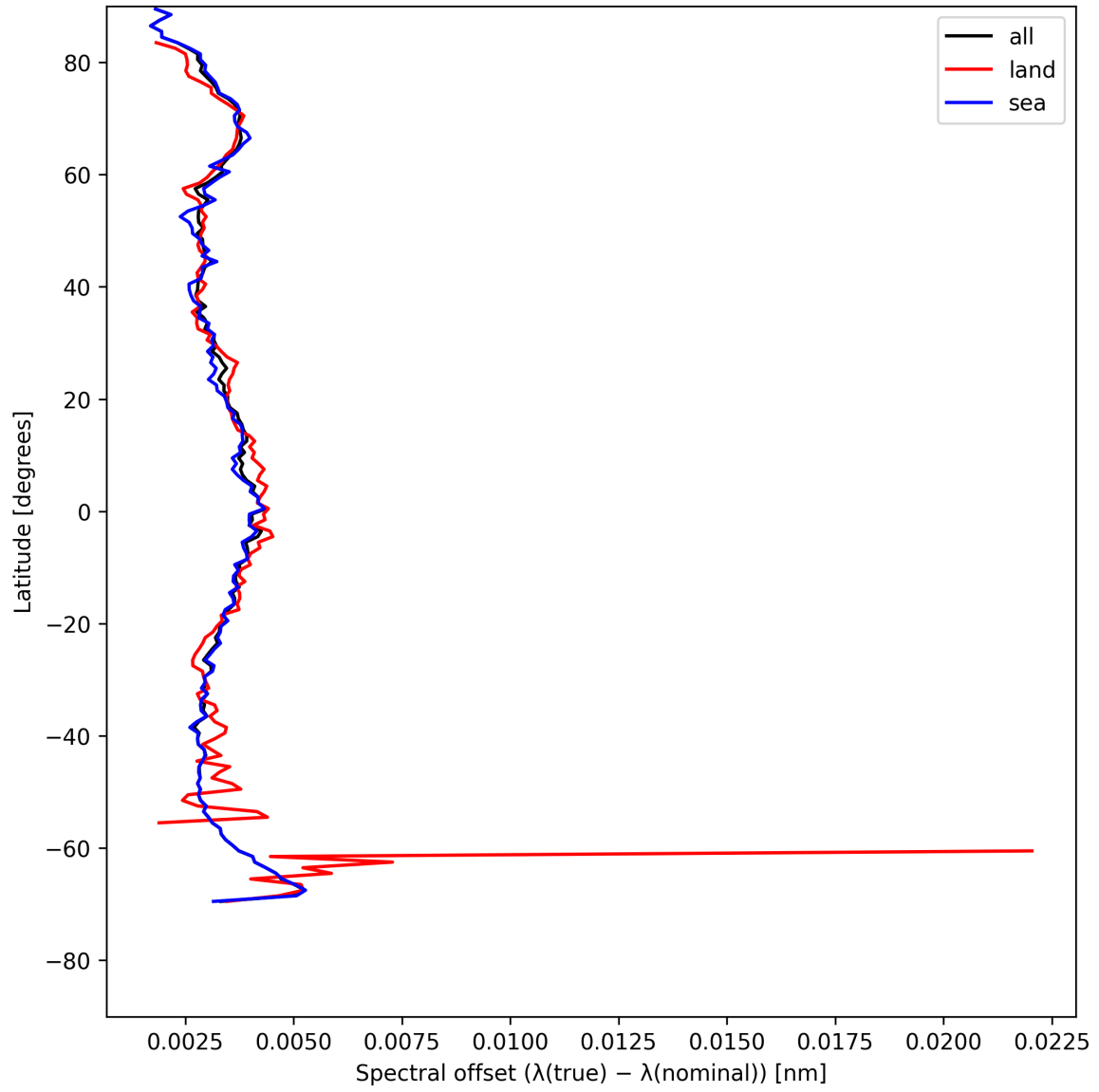
Figure 26: Zonal average of “Spectral offset ( \lambda_{\text{true}} - \lambda_{\text{nominal}} )” for 2025-05-13 to 2025-05-13.
