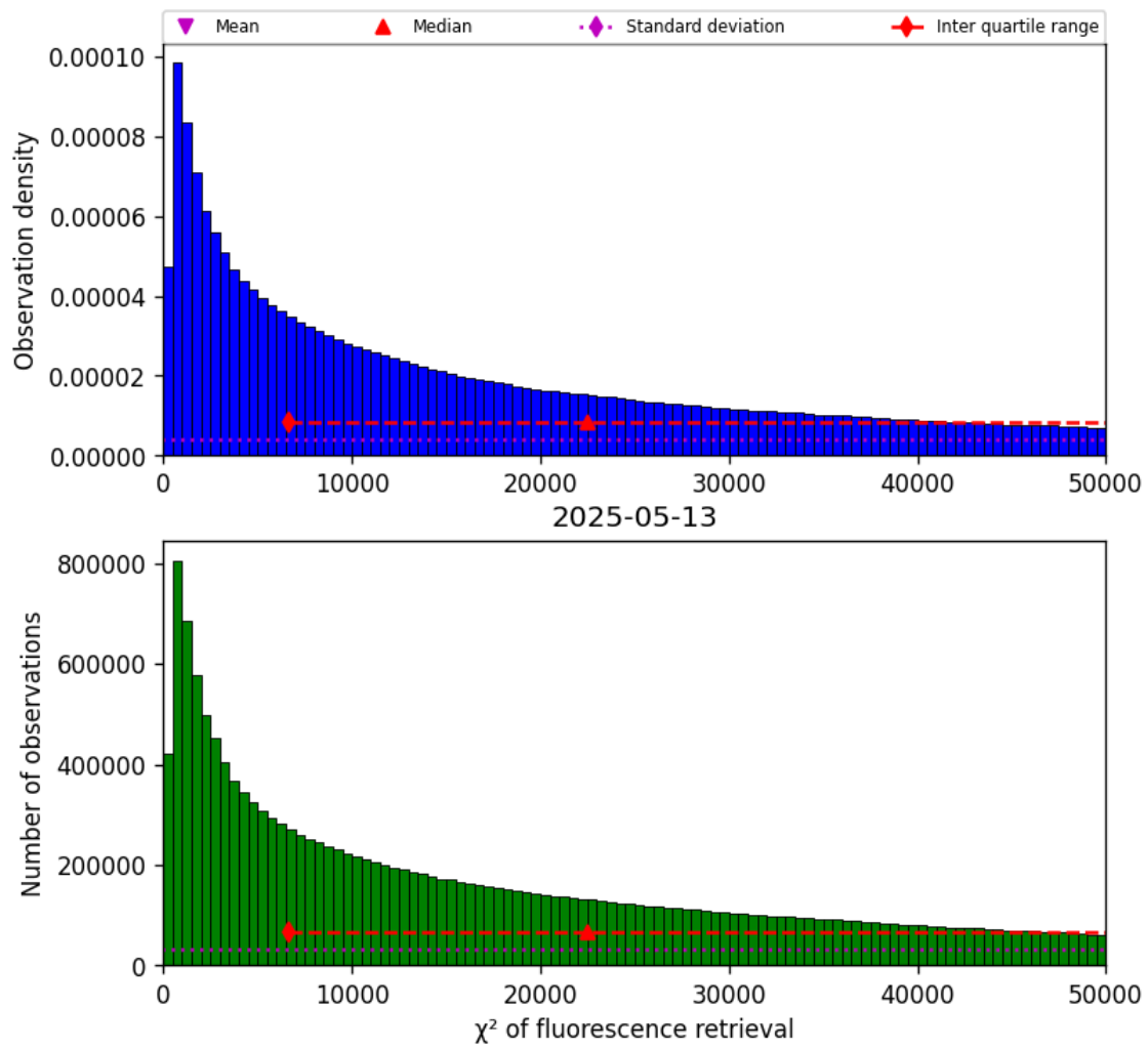
Figure 40: Histogram of “ \chi^2 of fluorescence retrieval” for 2025-05-13 to 2025-05-13
