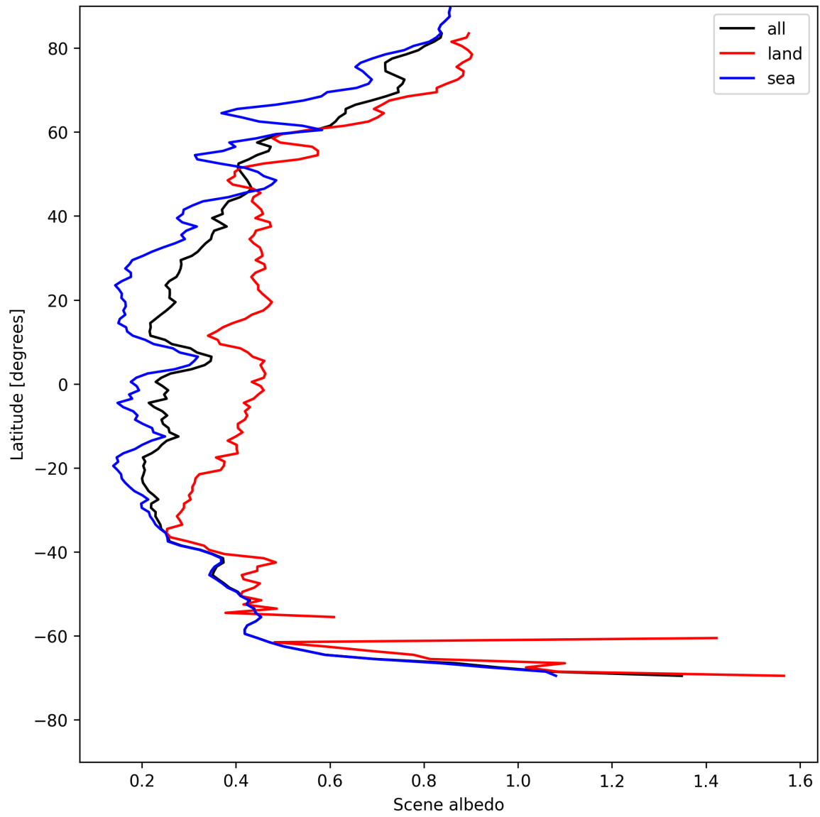
Figure 15: Zonal average of “Scene albedo” for 2025-05-13 to 2025-05-13.
