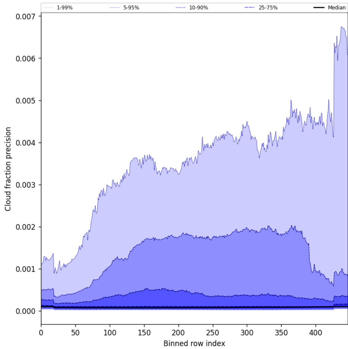
Figure 48: Along track statistics of “Cloud fraction precision” for 2025-05-13 to 2025-05-13
