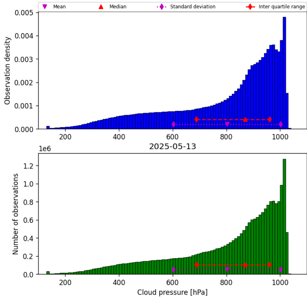
Figure 28: Histogram of “Cloud pressure” for 2025-05-13 to 2025-05-13
