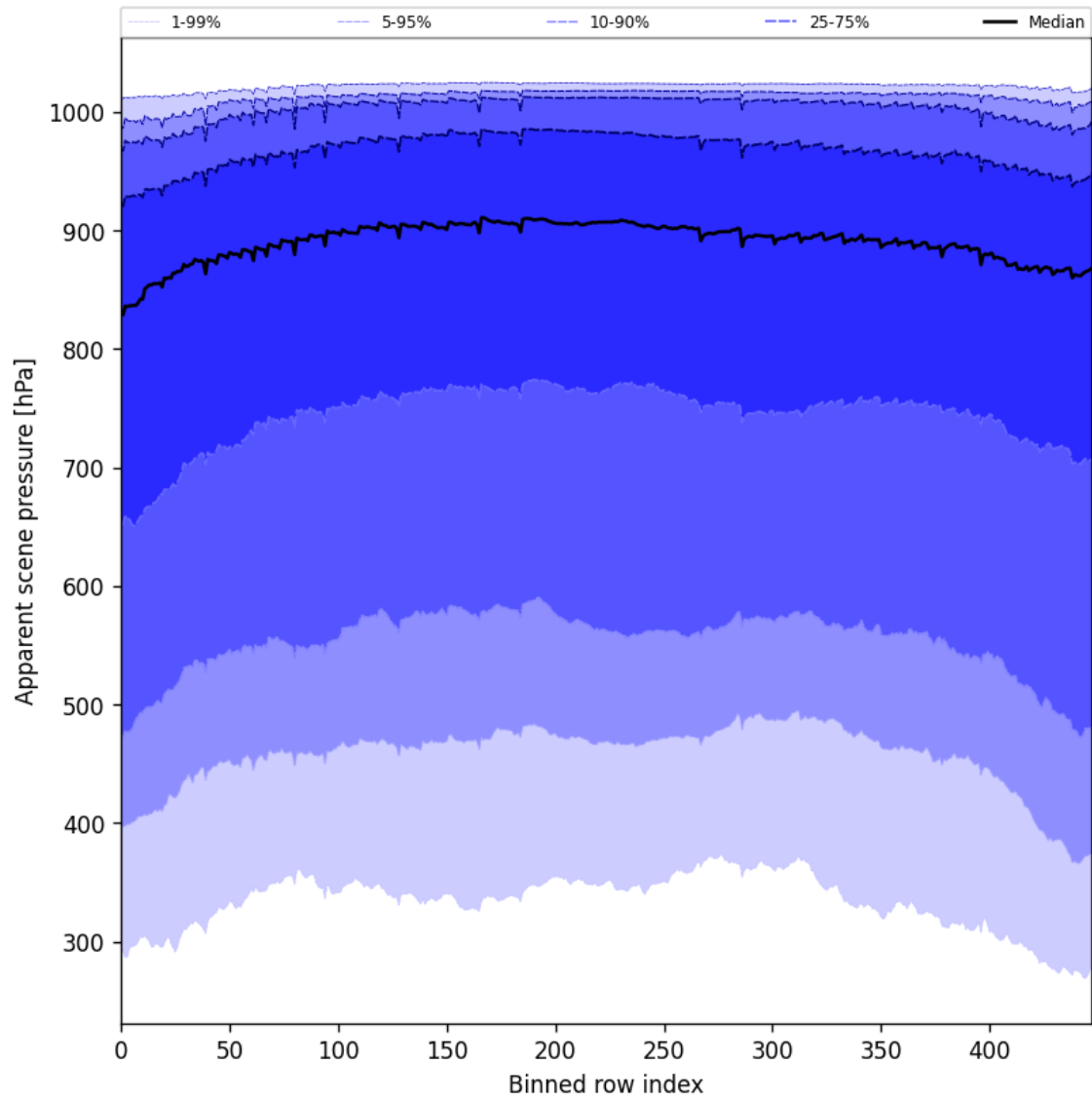
Figure 51: Along track statistics of “Apparent scene pressure” for 2025-05-13 to 2025-05-13
