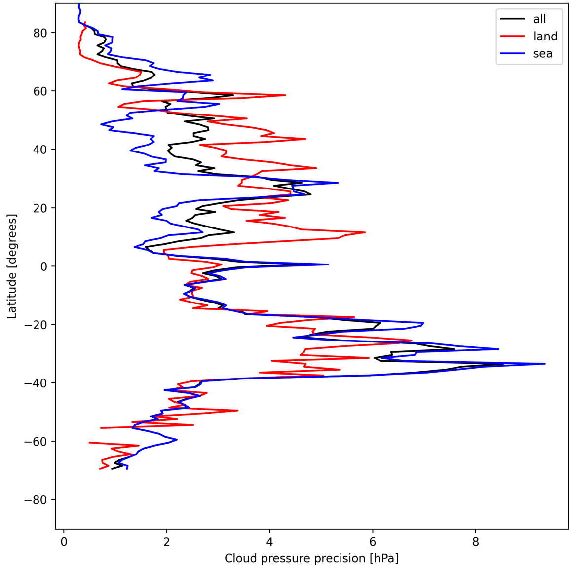
Figure 12: Zonal average of “Cloud pressure precision” for 2025-05-13 to 2025-05-13.
