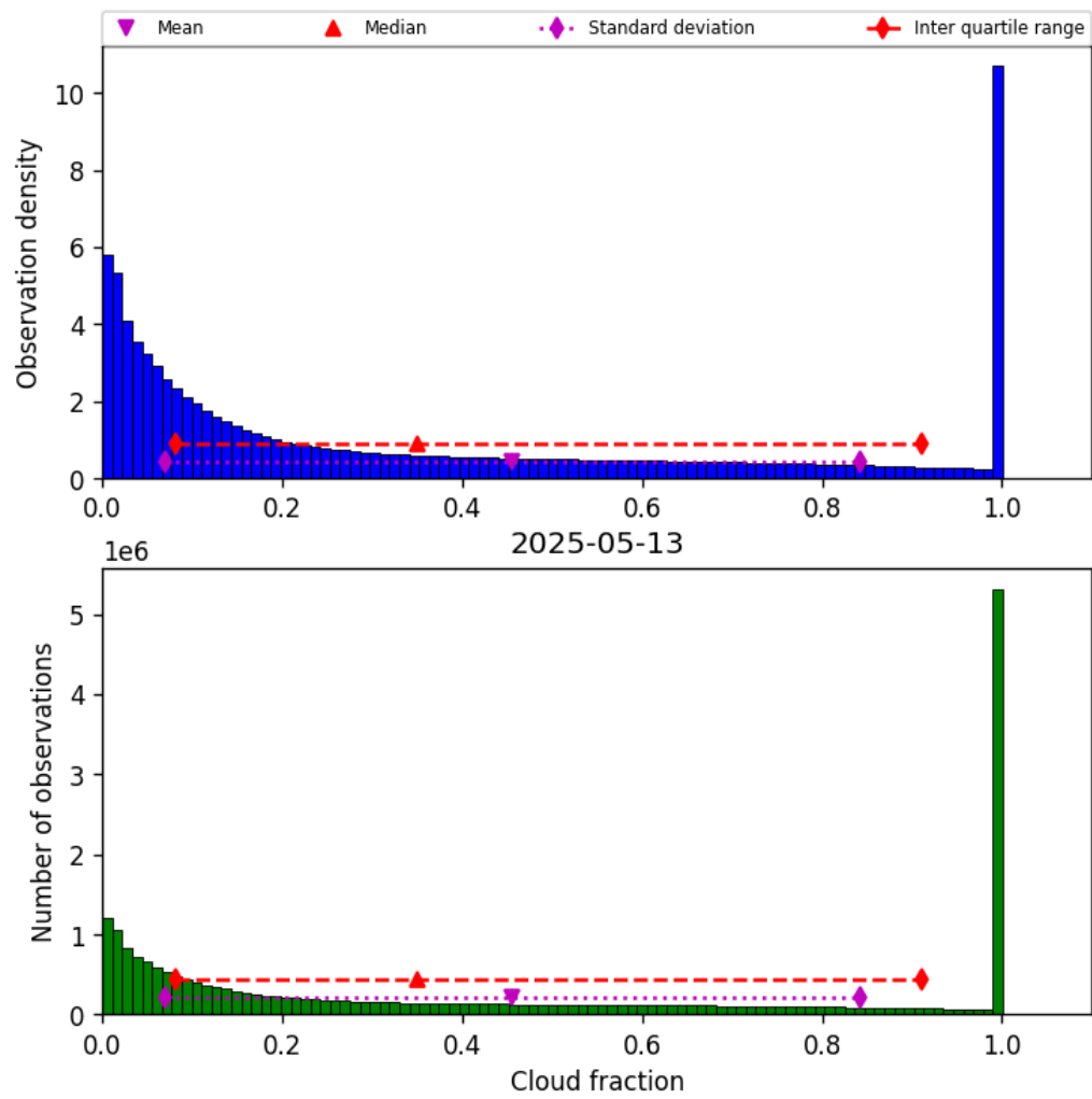
Figure 30: Histogram of "Cloud fraction" for 2025-05-13 to 2025-05-13
