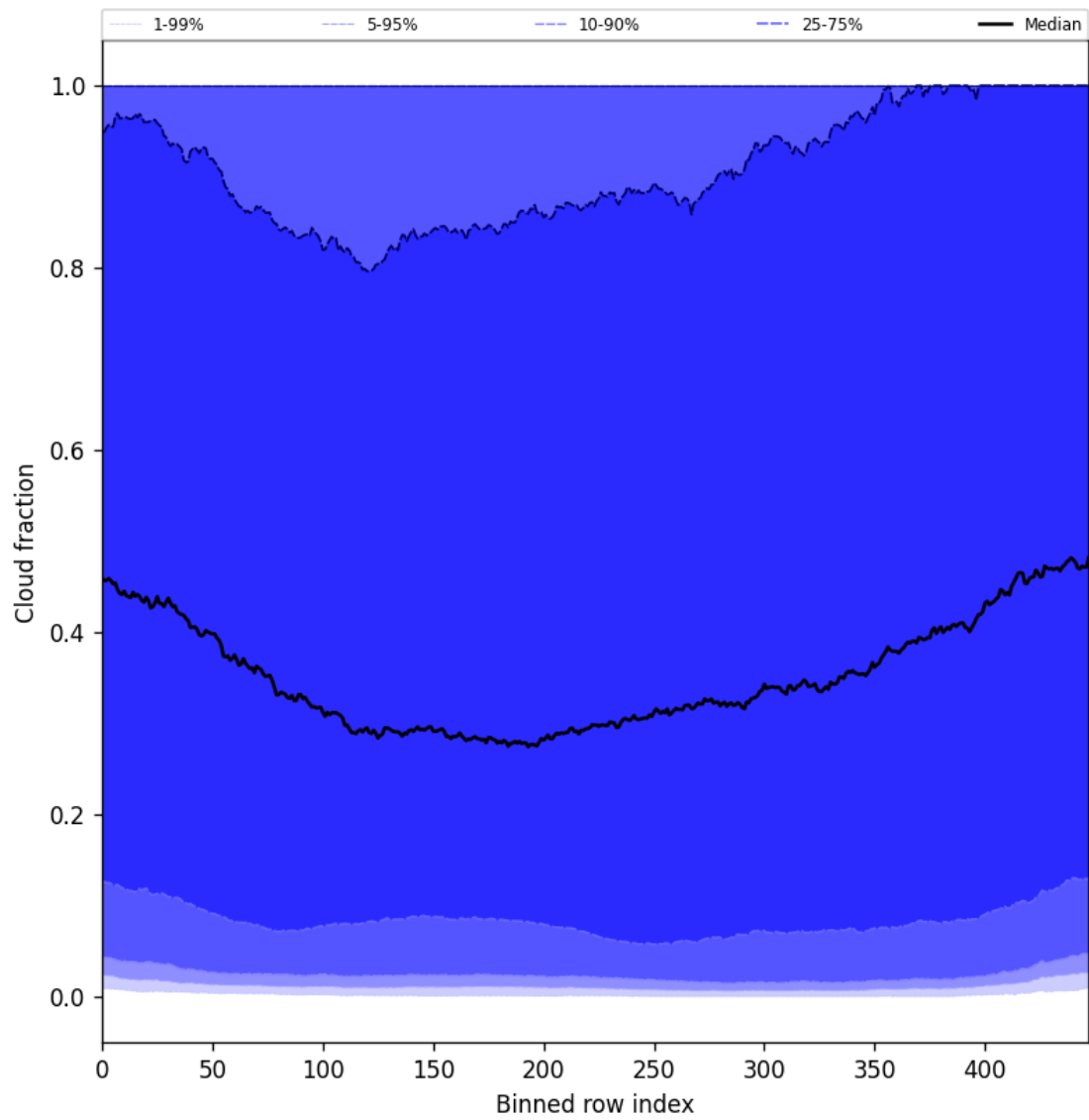
Figure 47: Along track statistics of “Cloud fraction” for 2025-05-13 to 2025-05-13
