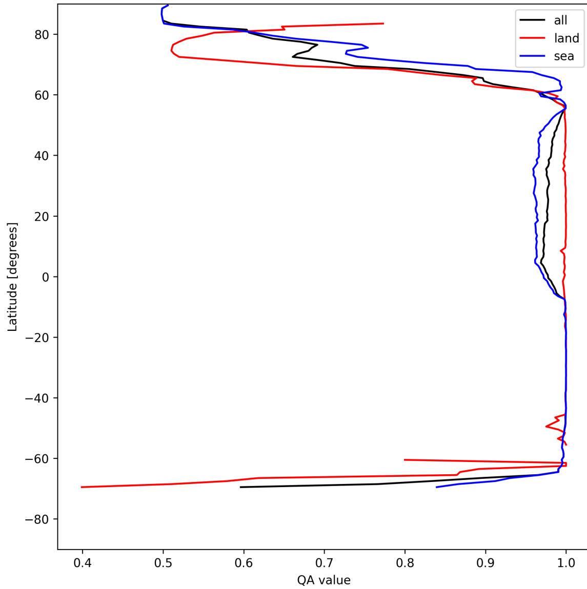
Figure 10: Zonal average of “QA value” for 2025-05-13 to 2025-05-13.
