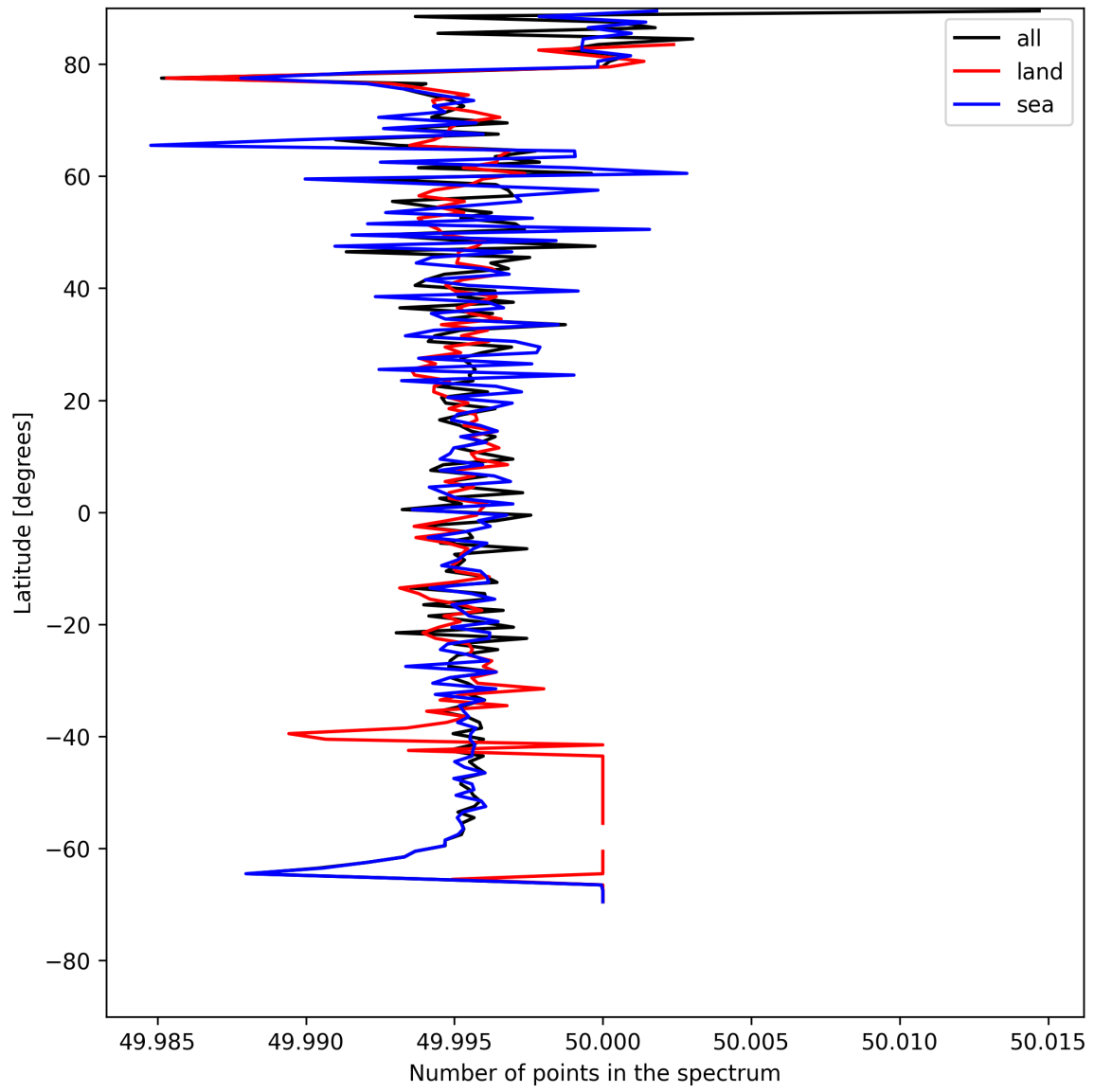
Figure 25: Zonal average of “Number of points in the spectrum” for 2025-05-13 to 2025-05-13.
