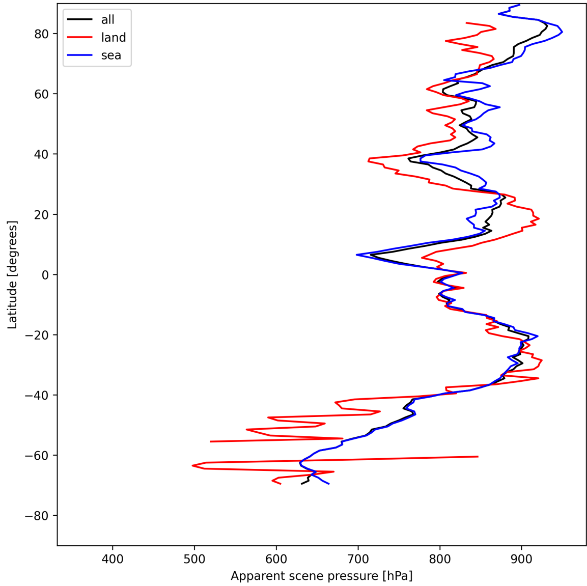
Figure 17: Zonal average of “Apparent scene pressure” for 2025-05-13 to 2025-05-13.
