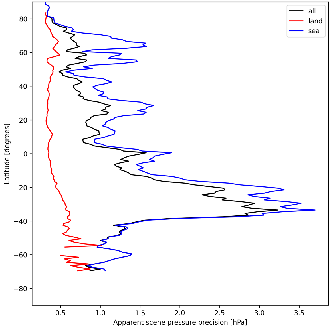
Figure 18: Zonal average of “Apparent scene pressure precision” for 2025-05-13 to 2025-05-13.
