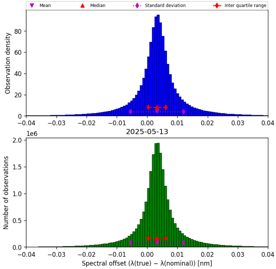
Figure 43: Histogram of “Spectral offset ( \lambda_{\text{true}} - \lambda_{\text{nominal}} )” for 2025-05-13 to 2025-05-13
