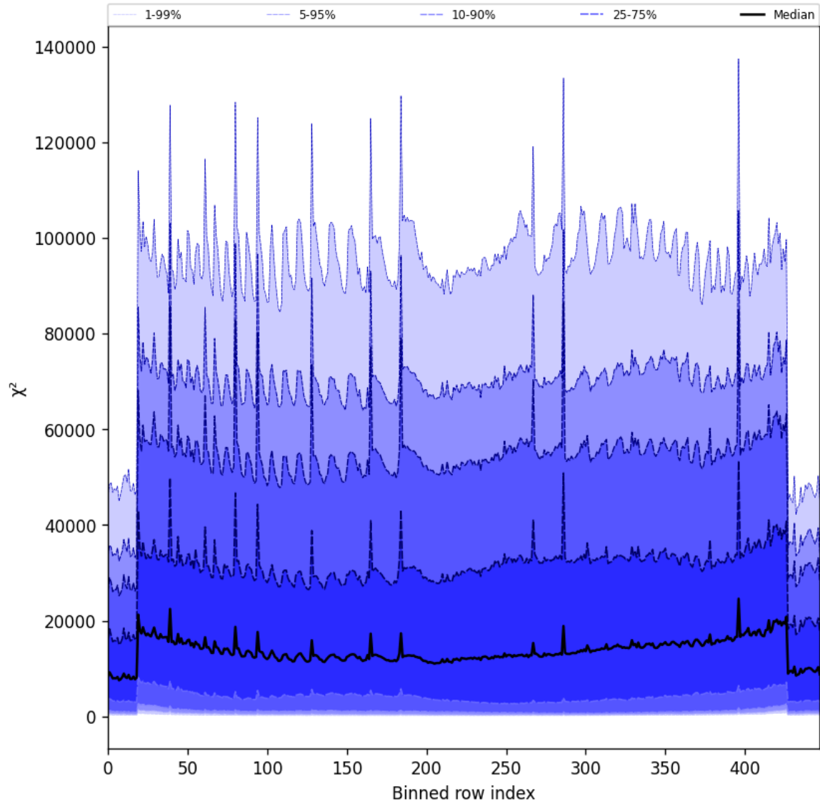
Figure 53: Along track statistics of “ \chi^2 ” for 2025-05-13 to 2025-05-13
