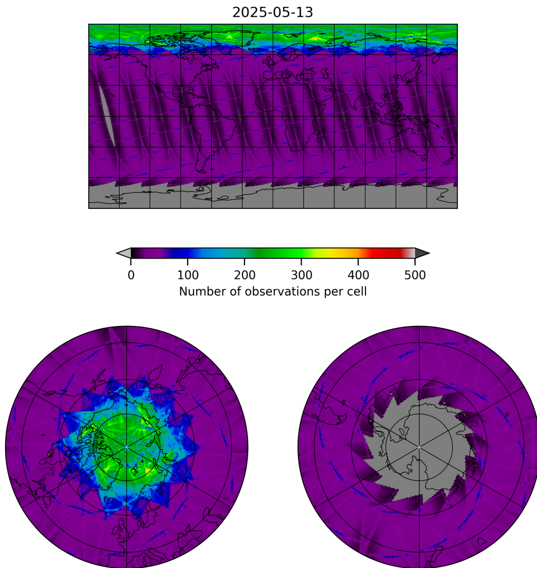
Figure 9: Map of the number of observations for 2025-05-13 to 2025-05-13
