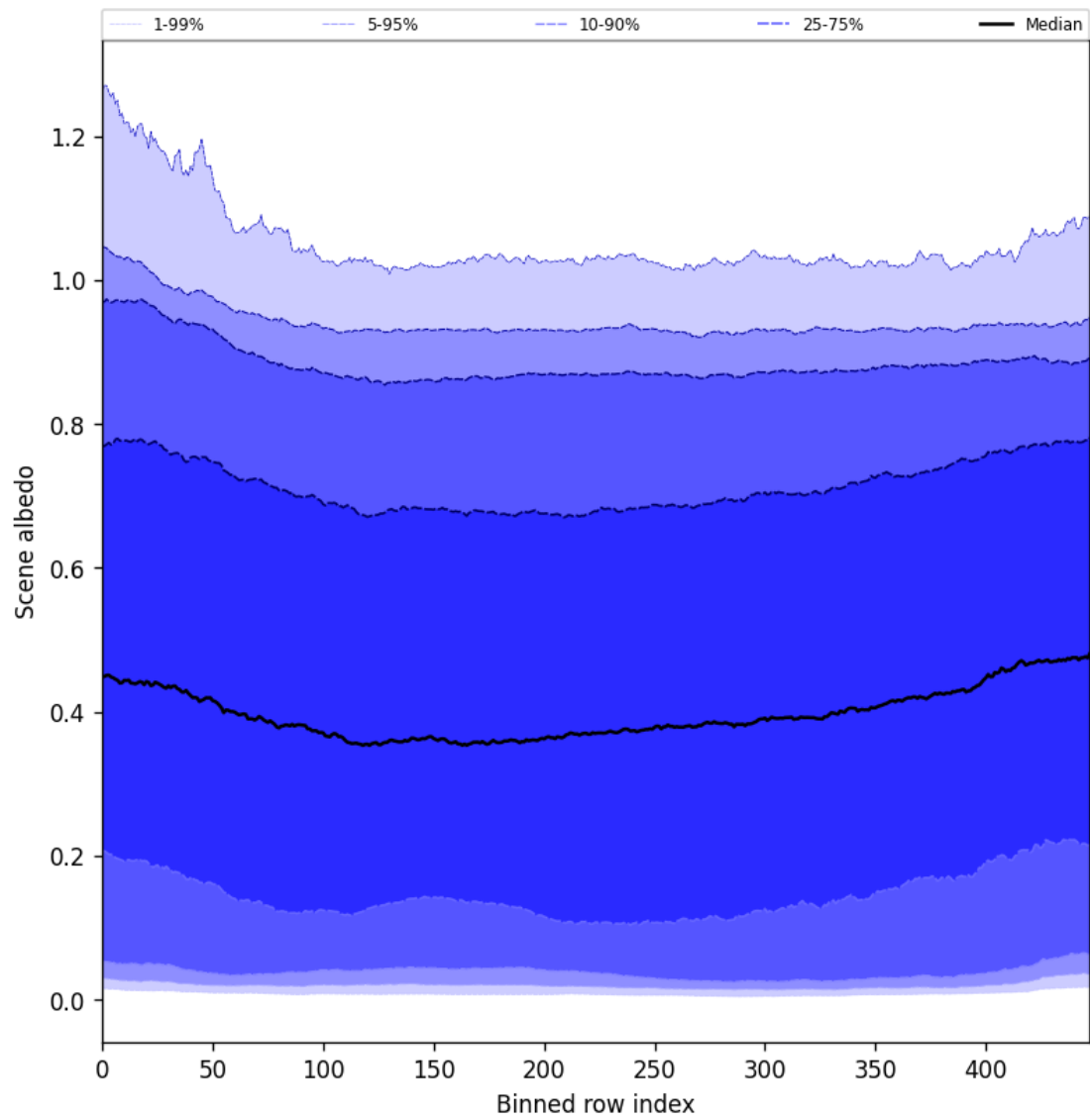
Figure 49: Along track statistics of “Scene albedo” for 2025-05-13 to 2025-05-13
