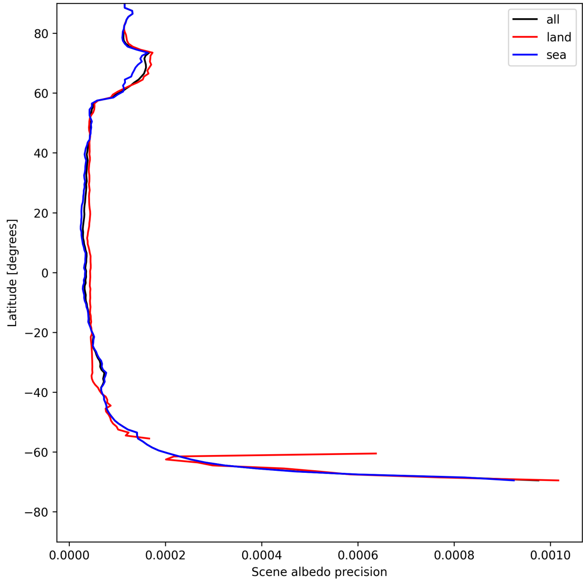
Figure 16: Zonal average of “Scene albedo precision” for 2025-05-13 to 2025-05-13.
