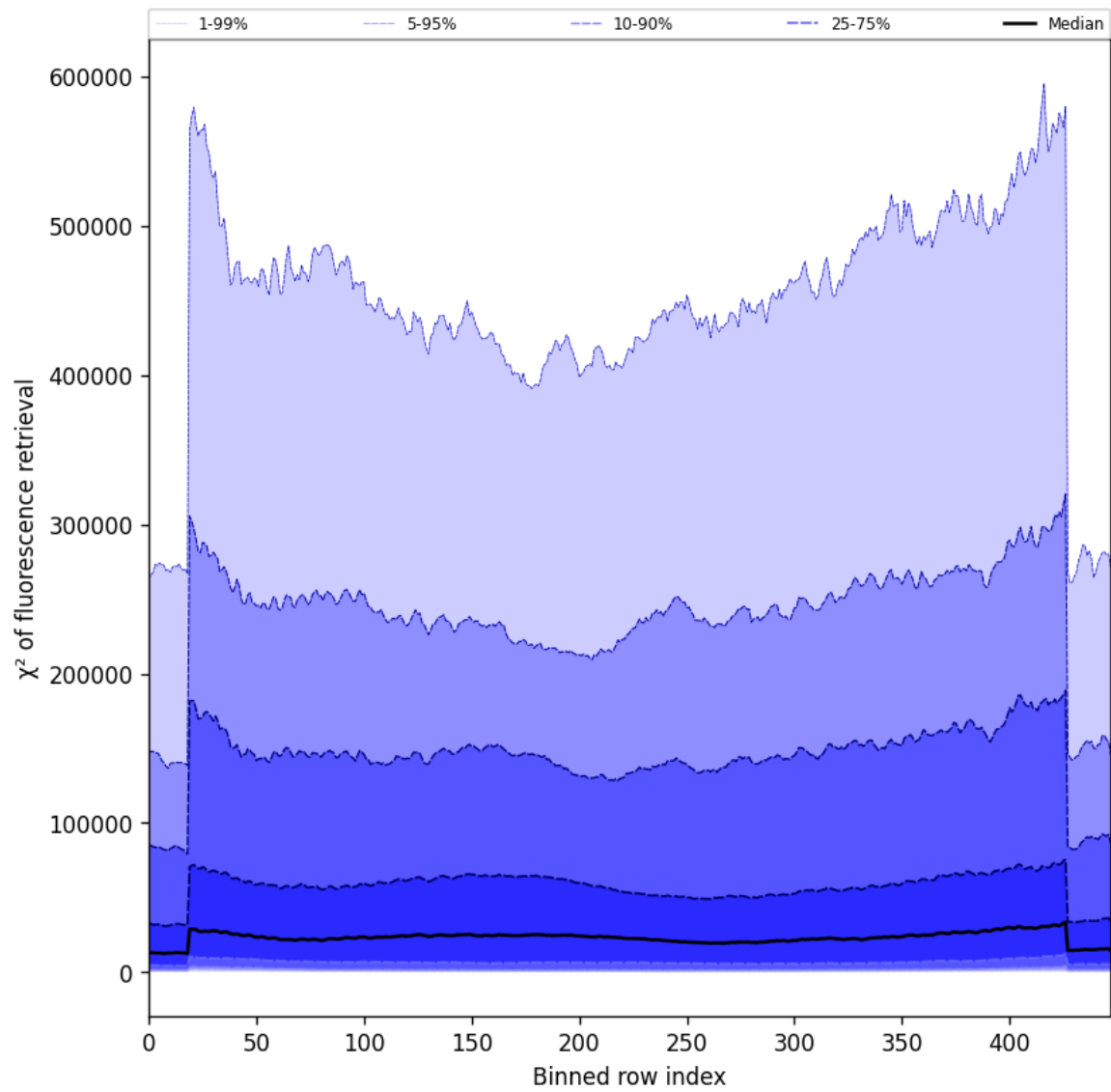
Figure 57: Along track statistics of “ \chi^2 of fluorescence retrieval” for 2025-05-13 to 2025-05-13
