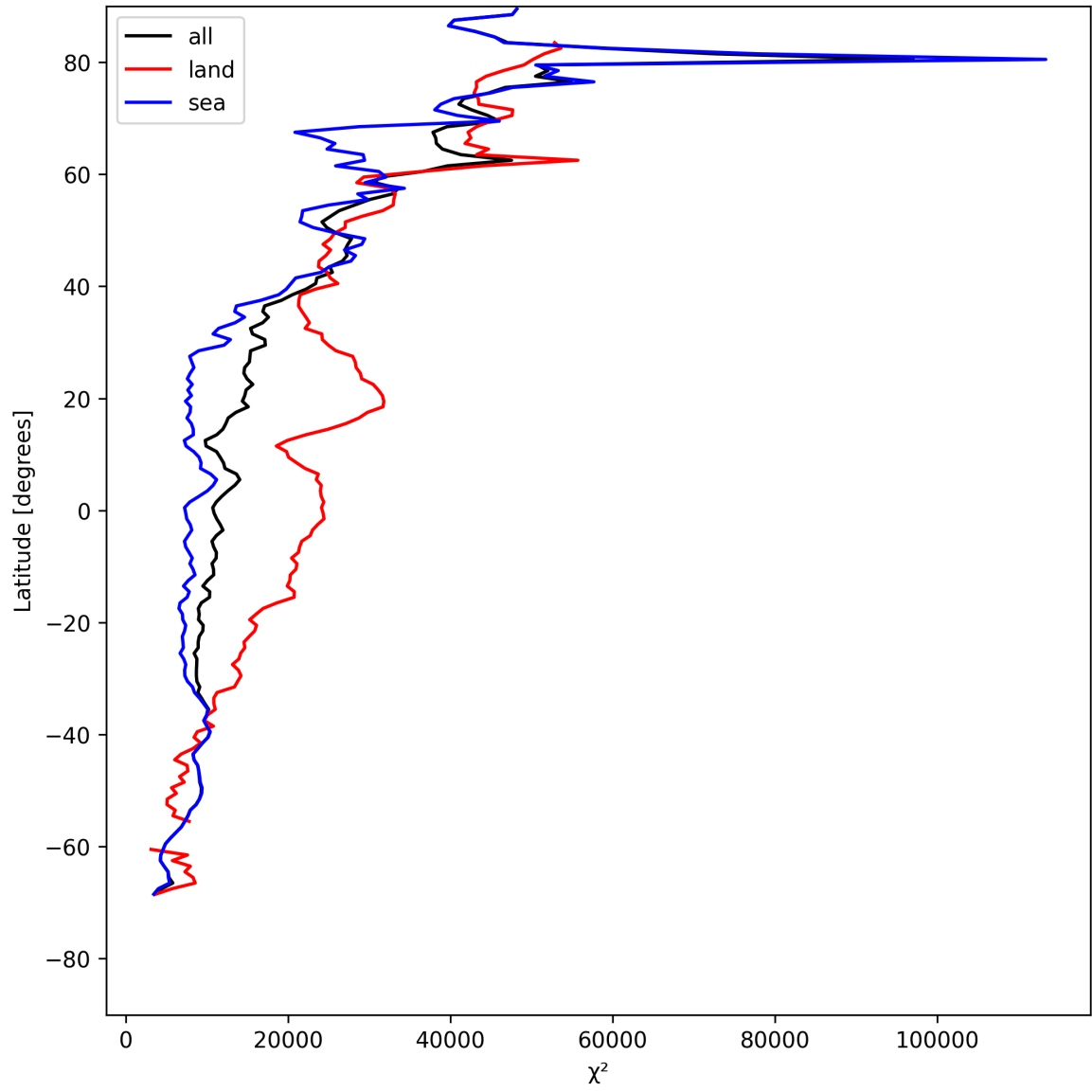
Figure 19: Zonal average of “ \chi^2 ” for 2025-05-14 to 2025-05-15.
