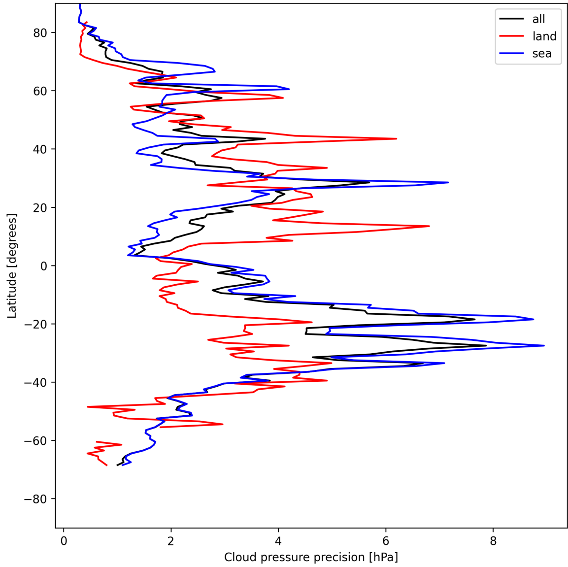
Figure 12: Zonal average of "Cloud pressure precision" for 2025-05-14 to 2025-05-15.
