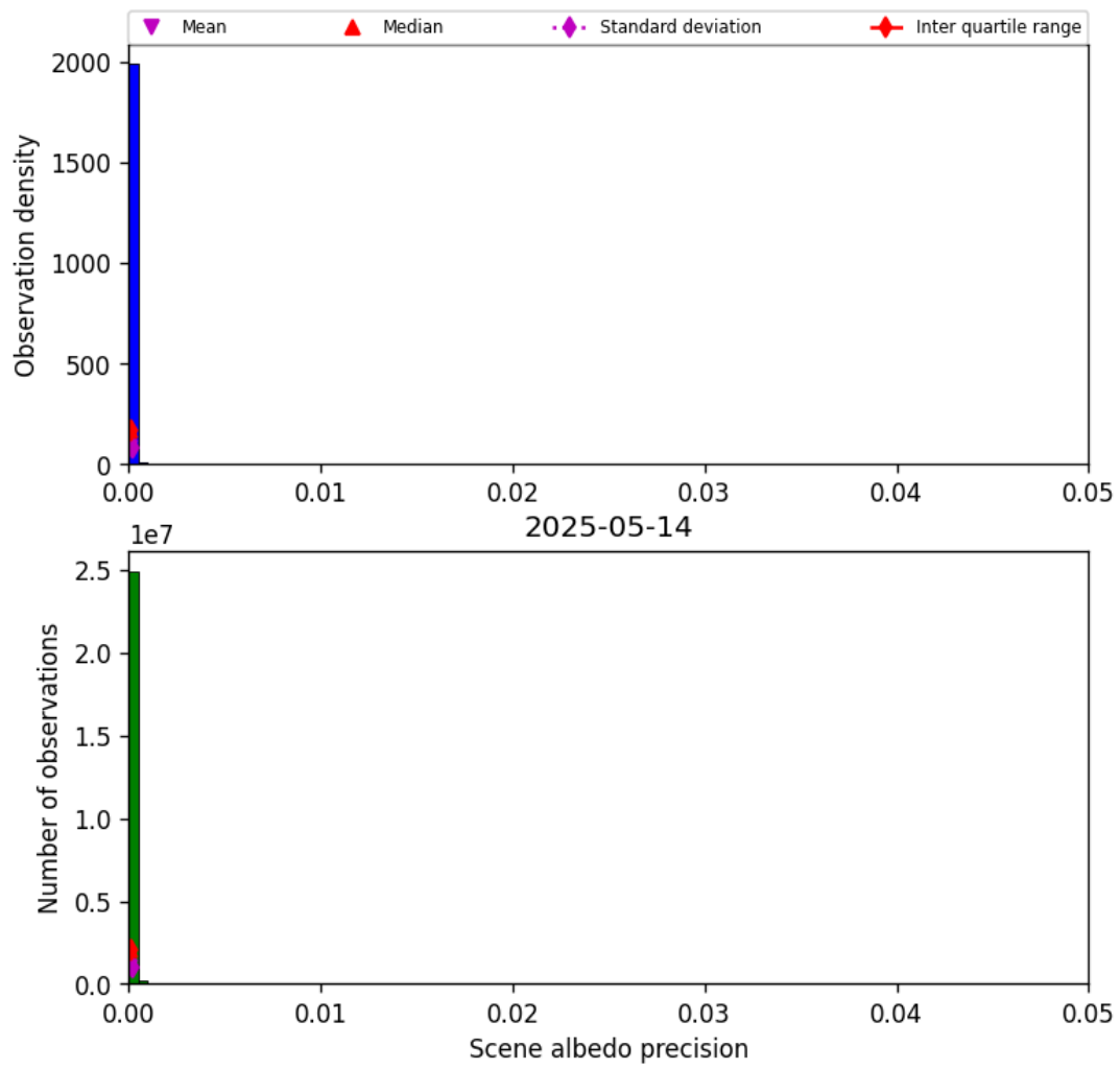
Figure 33: Histogram of “Scene albedo precision” for 2025-05-14 to 2025-05-15
