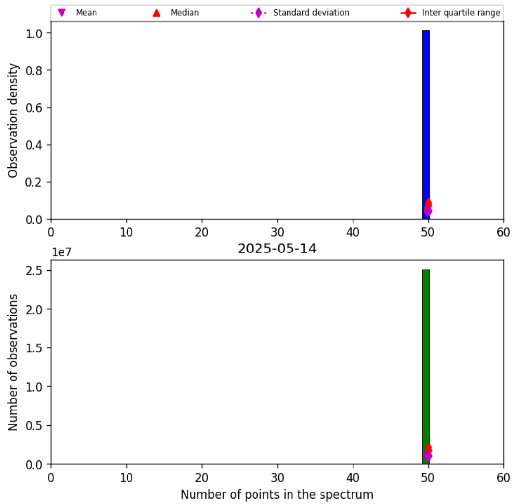
Figure 42: Histogram of “Number of points in the spectrum” for 2025-05-14 to 2025-05-15
