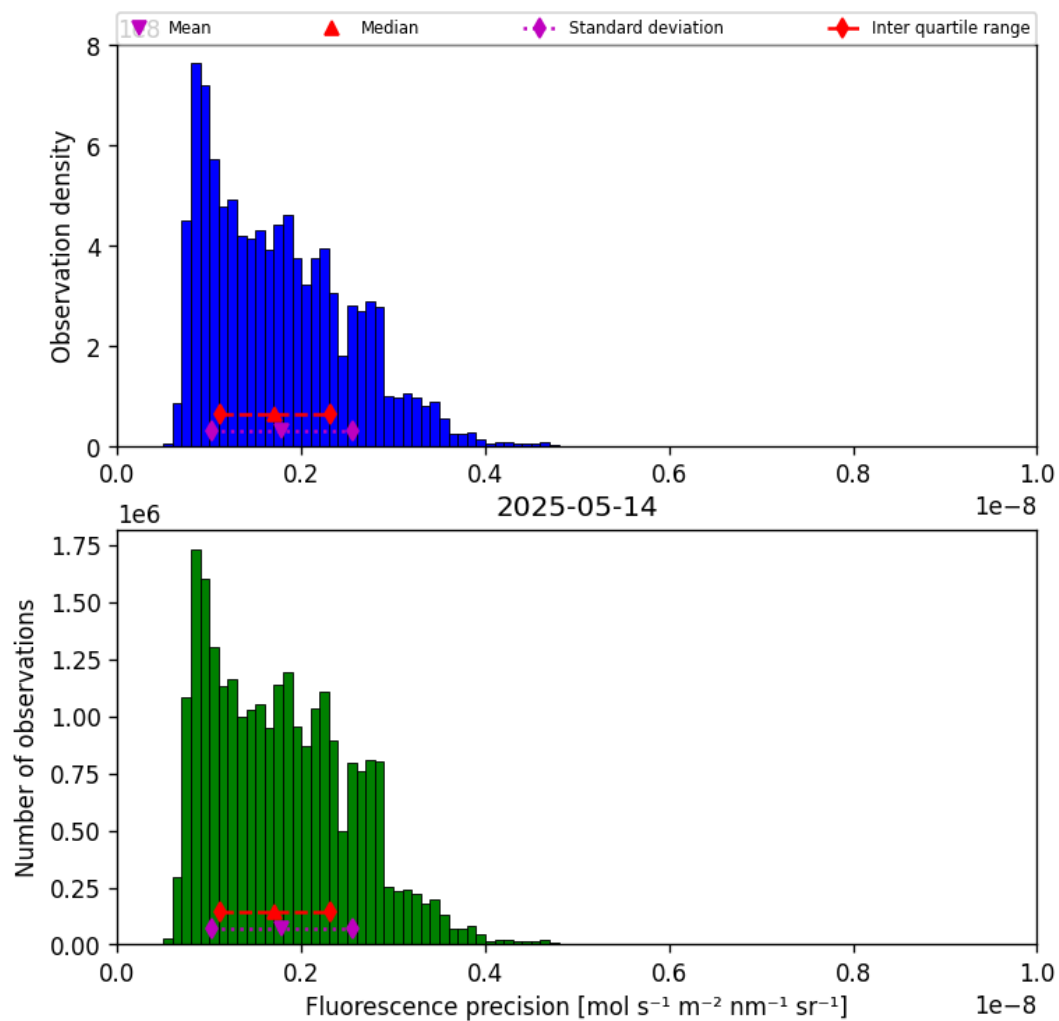
Figure 39: Histogram of “Fluorescence precision” for 2025-05-14 to 2025-05-15
