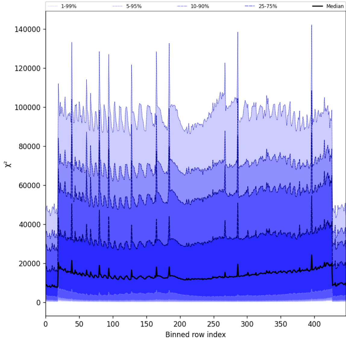
Figure 53: Along track statistics of “ \chi^2 ” for 2025-05-14 to 2025-05-15
