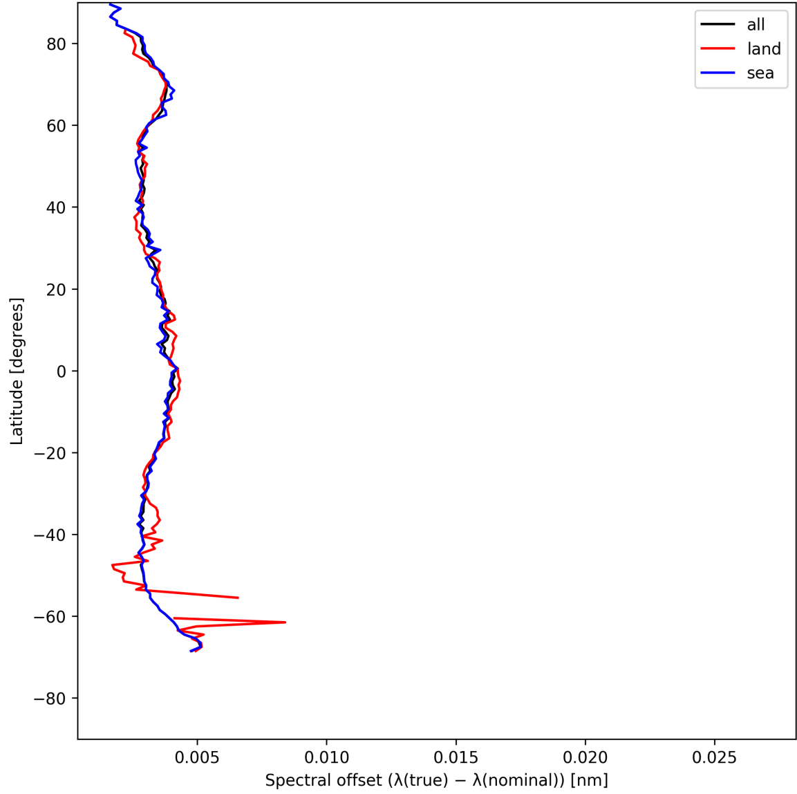
Figure 26: Zonal average of “Spectral offset ( \lambda_{\text{true}} - \lambda_{\text{nominal}} )” for 2025-05-14 to 2025-05-15.
