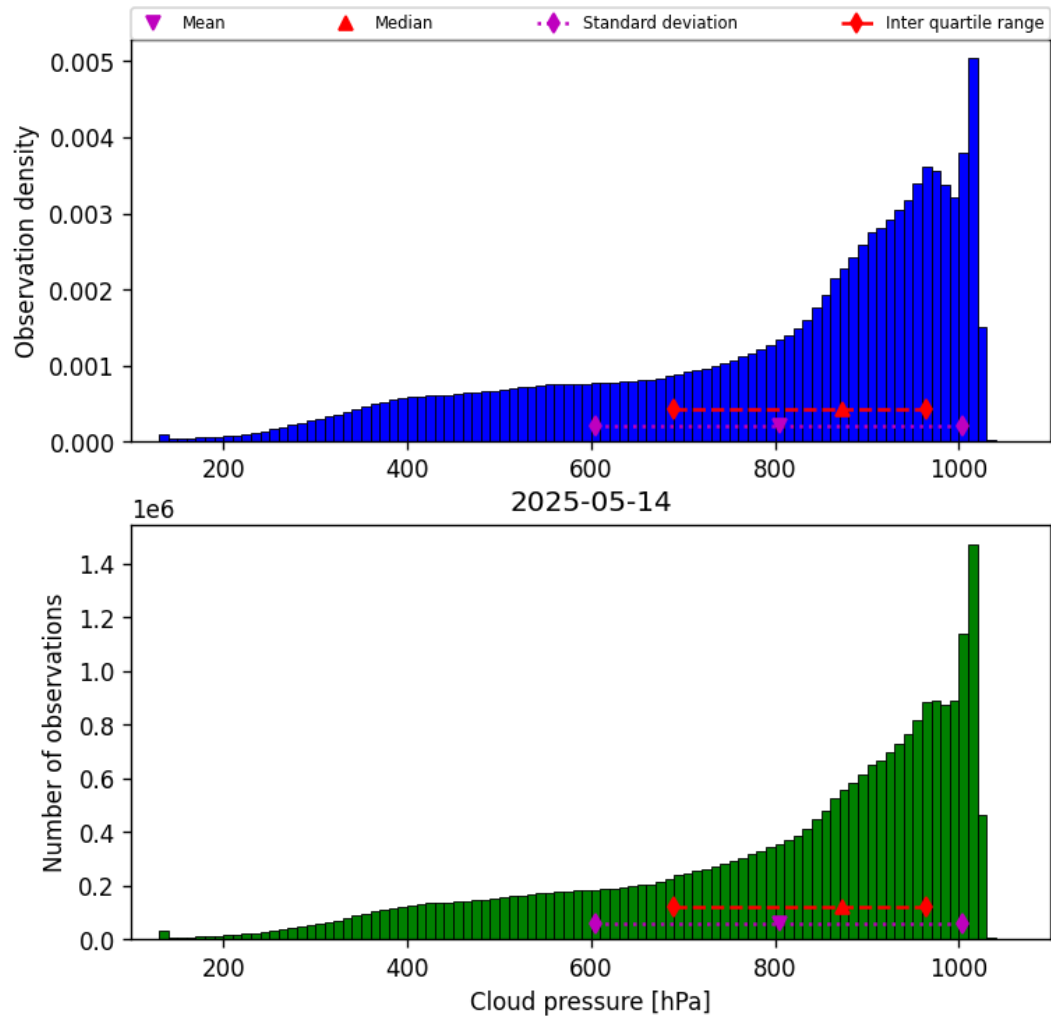
Figure 28: Histogram of “Cloud pressure” for 2025-05-14 to 2025-05-15
