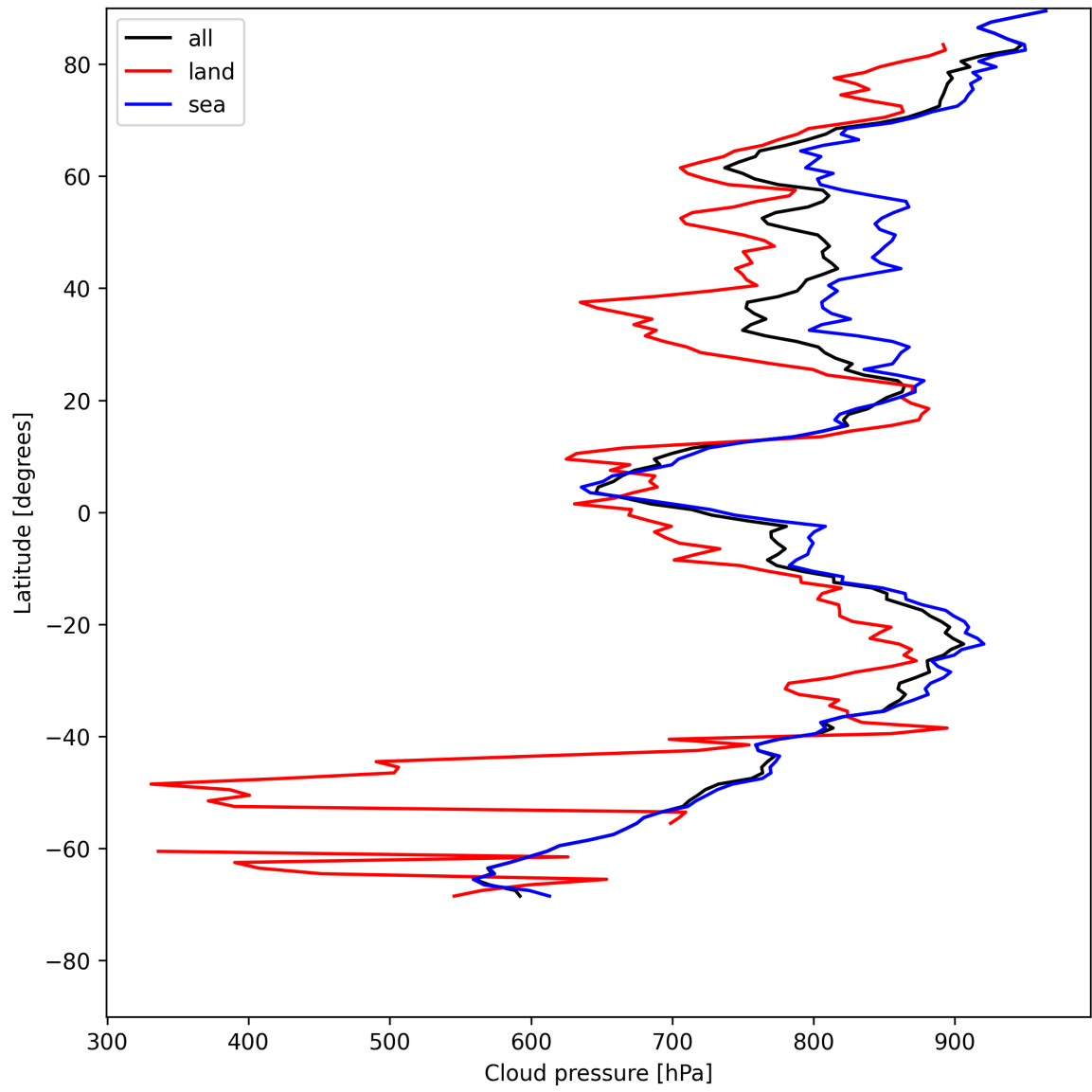
Figure 11: Zonal average of “Cloud pressure” for 2025-05-14 to 2025-05-15.
