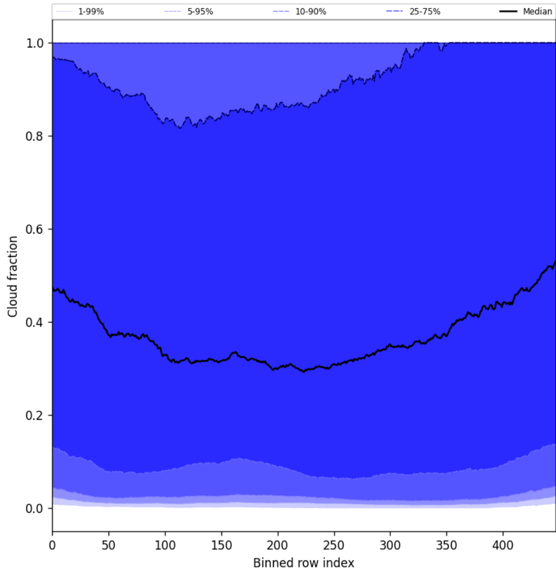
Figure 47: Along track statistics of “Cloud fraction” for 2025-05-14 to 2025-05-15
