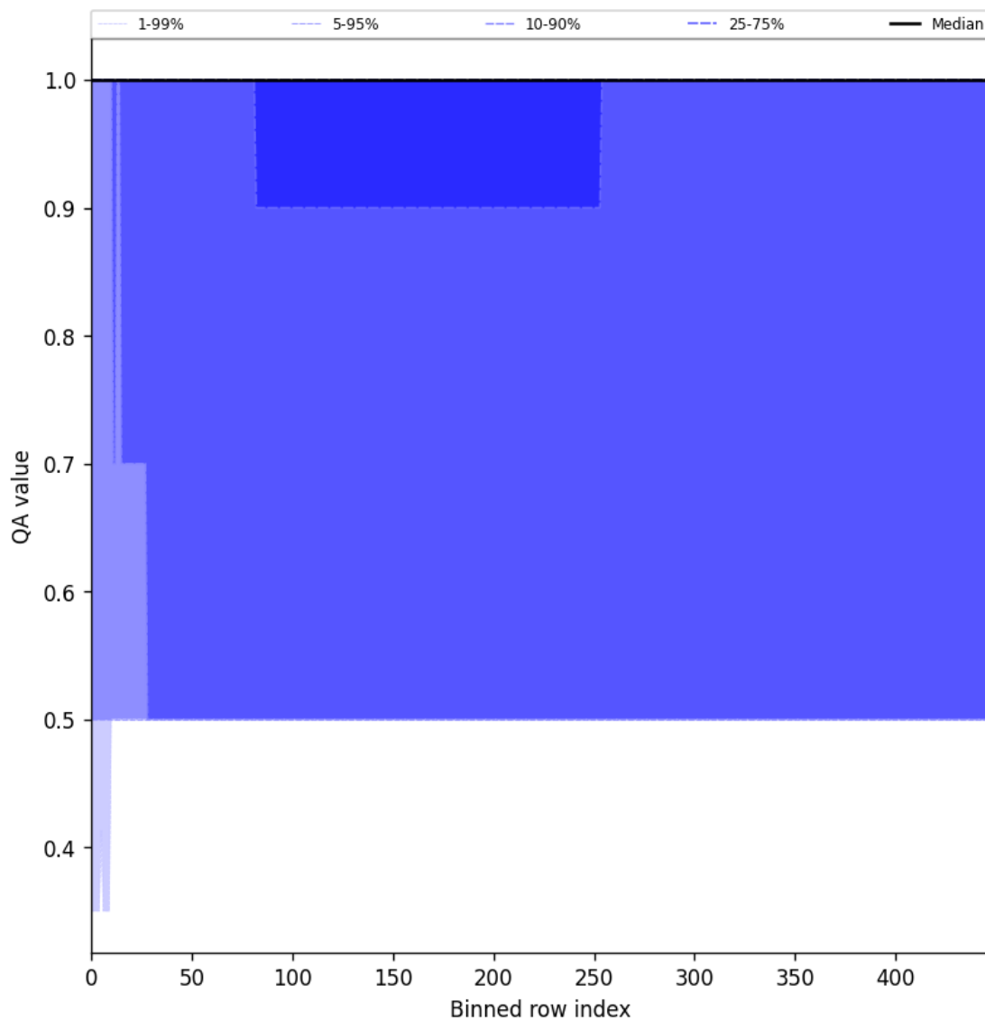
Figure 44: Along track statistics of “QA value” for 2025-05-14 to 2025-05-15
