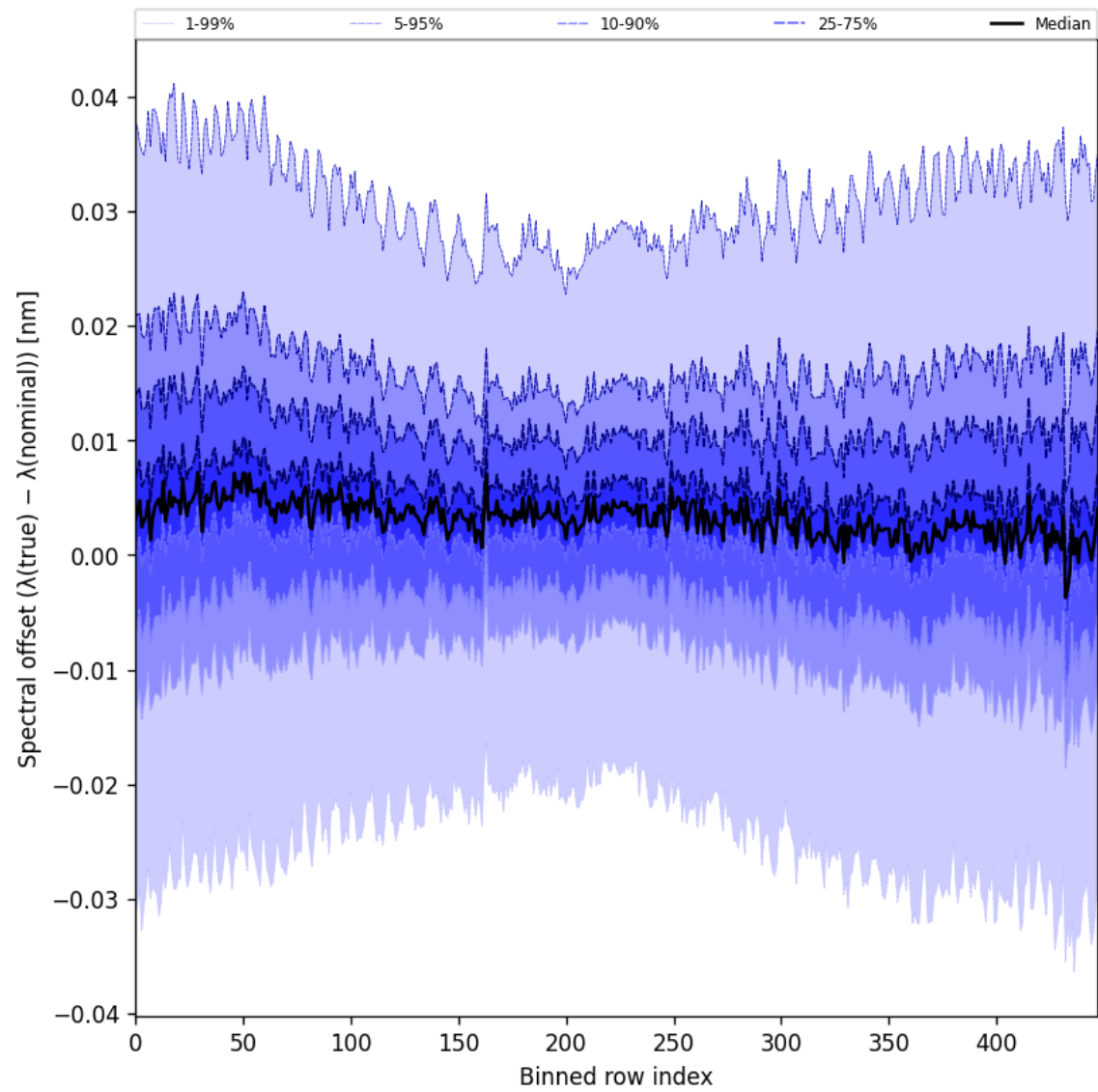
Figure 60: Along track statistics of “Spectral offset ( \lambda_{\text{true}} - \lambda_{\text{nominal}} )” for 2025-05-14 to 2025-05-15
