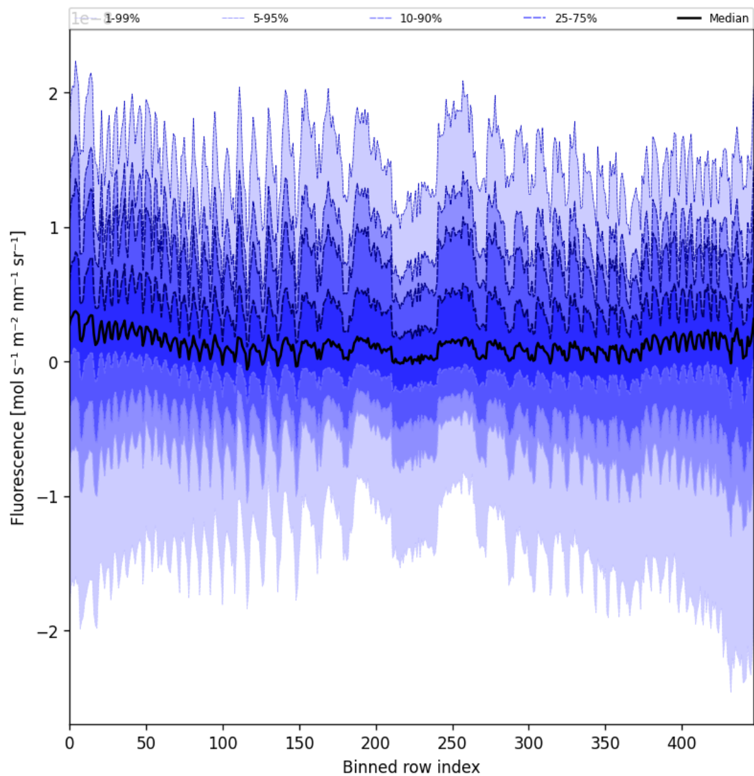
Figure 55: Along track statistics of “Fluorescence” for 2025-05-14 to 2025-05-15
