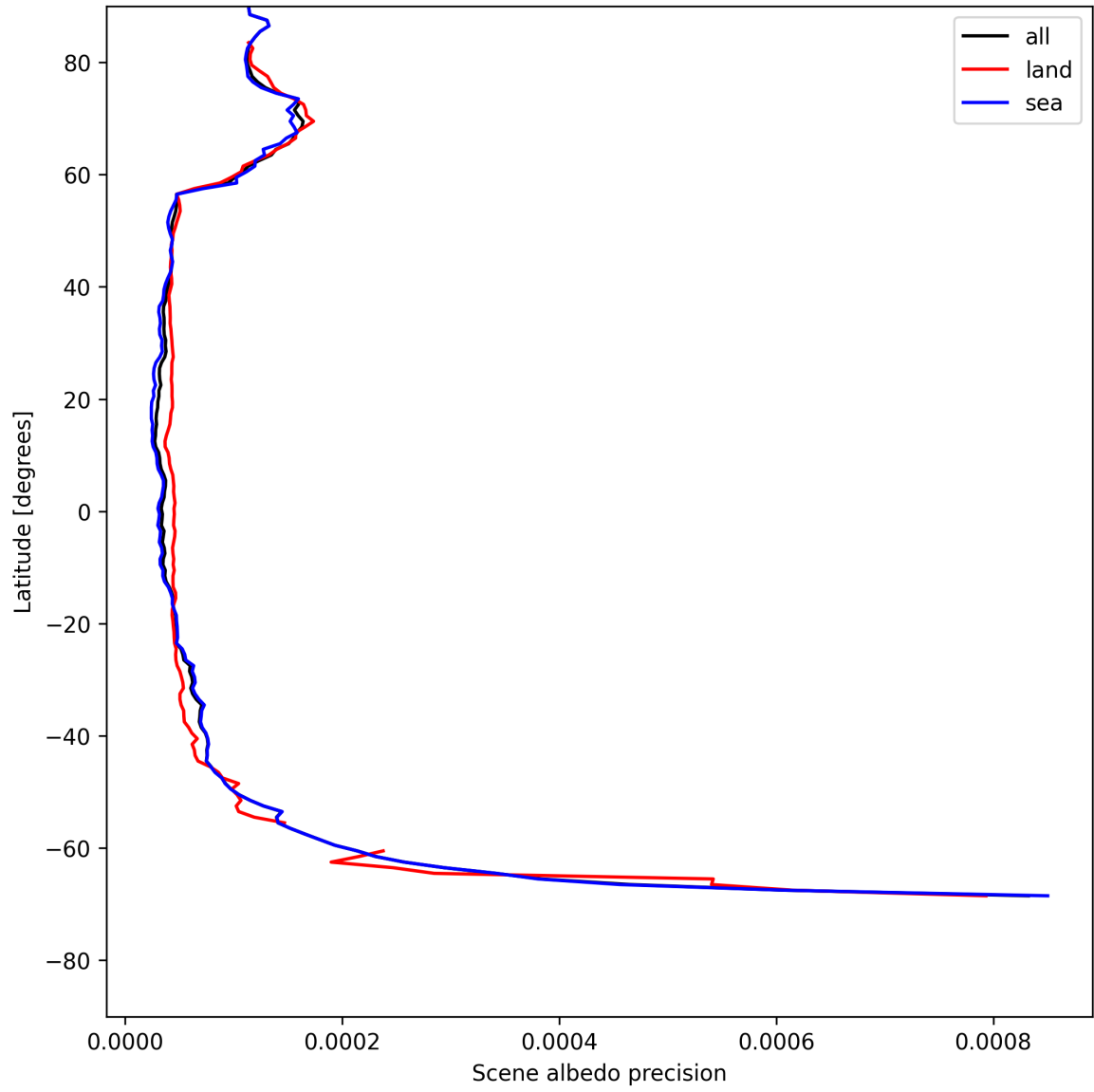
Figure 16: Zonal average of “Scene albedo precision” for 2025-05-14 to 2025-05-15.
