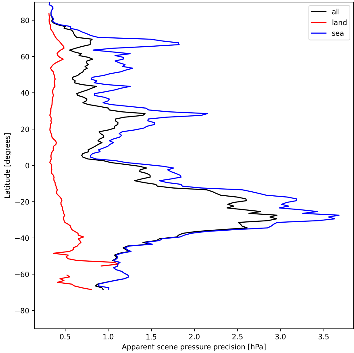
Figure 18: Zonal average of “Apparent scene pressure precision” for 2025-05-14 to 2025-05-15.
