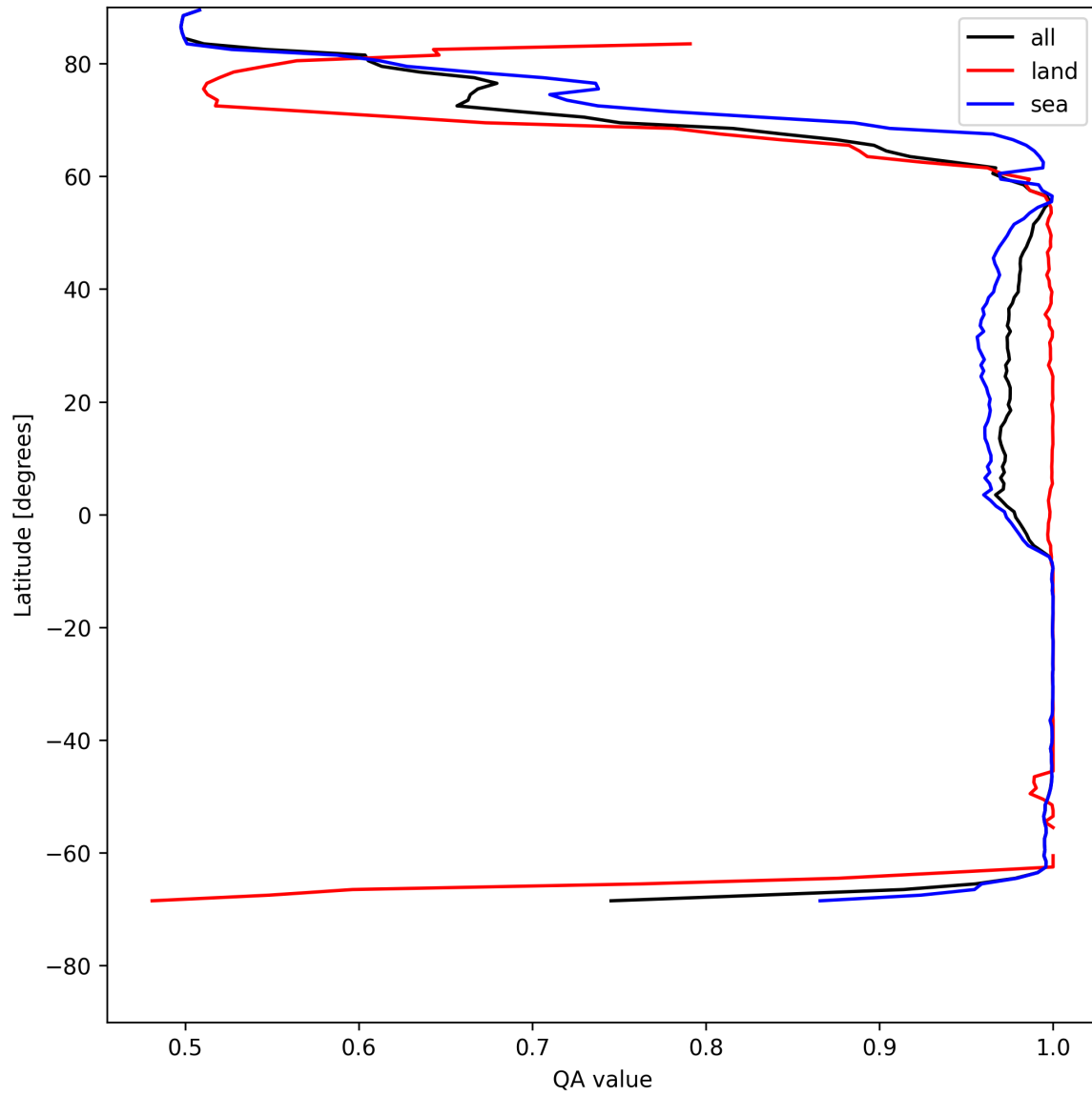
Figure 10: Zonal average of “QA value” for 2025-05-14 to 2025-05-15.
