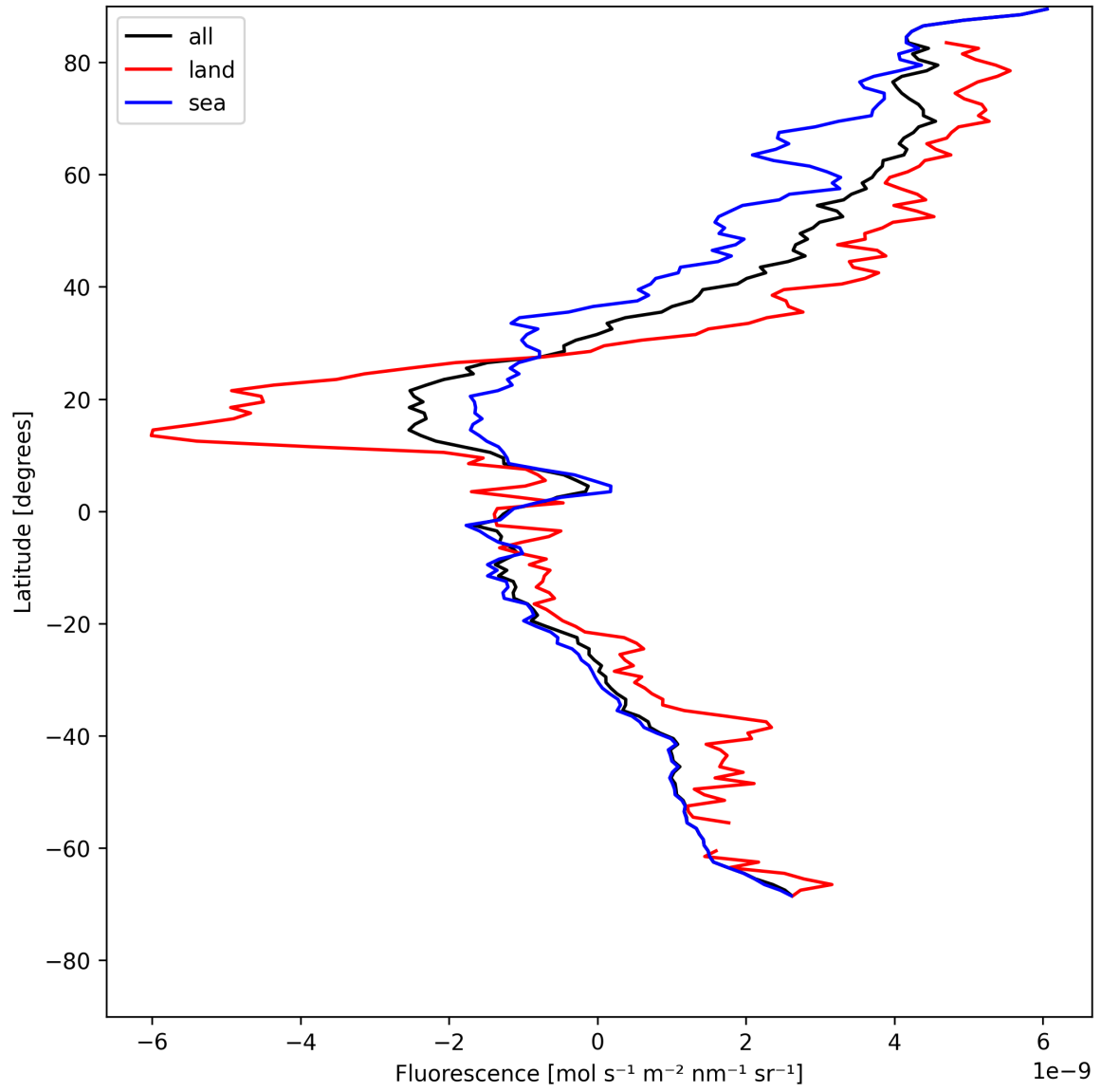
Figure 21: Zonal average of “Fluorescence” for 2025-05-14 to 2025-05-15.
