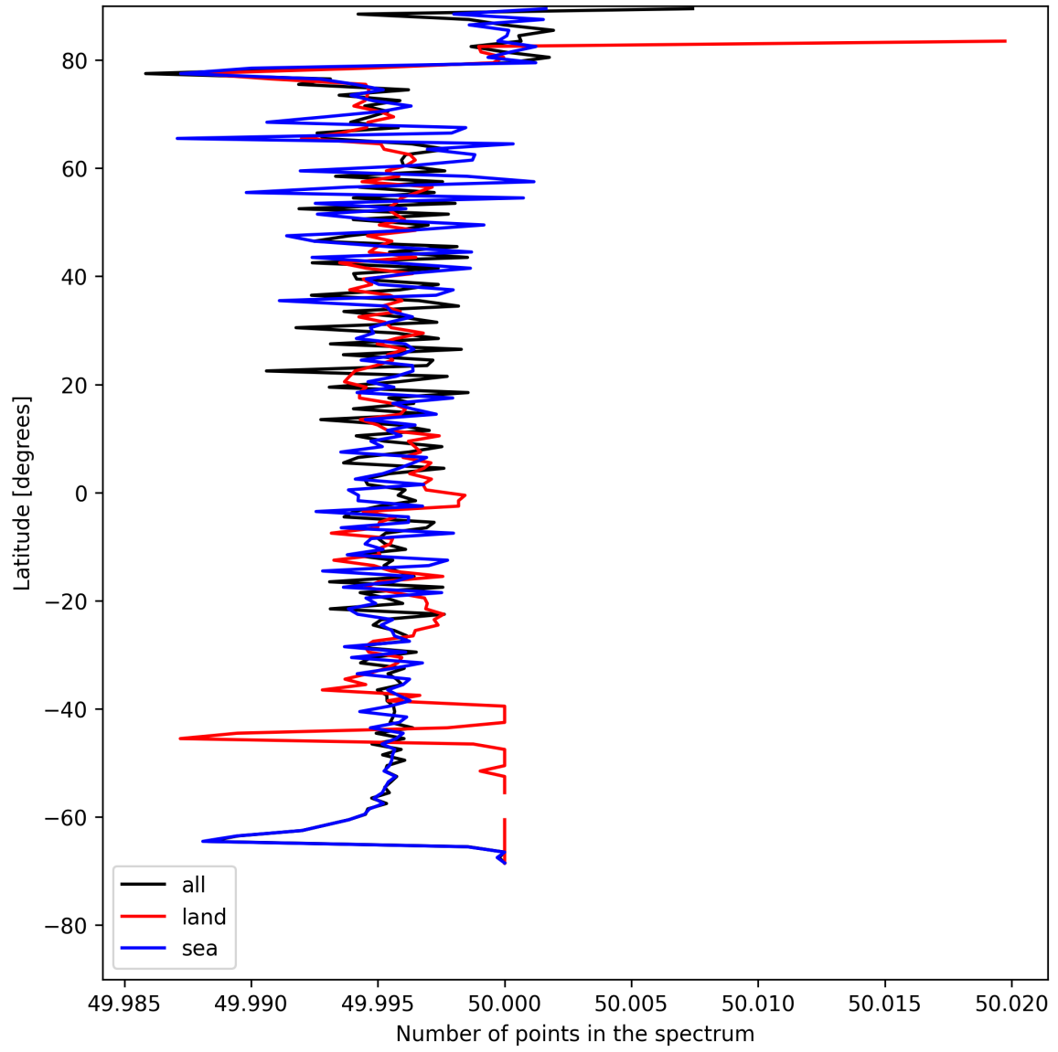
Figure 25: Zonal average of “Number of points in the spectrum” for 2025-05-14 to 2025-05-15.
