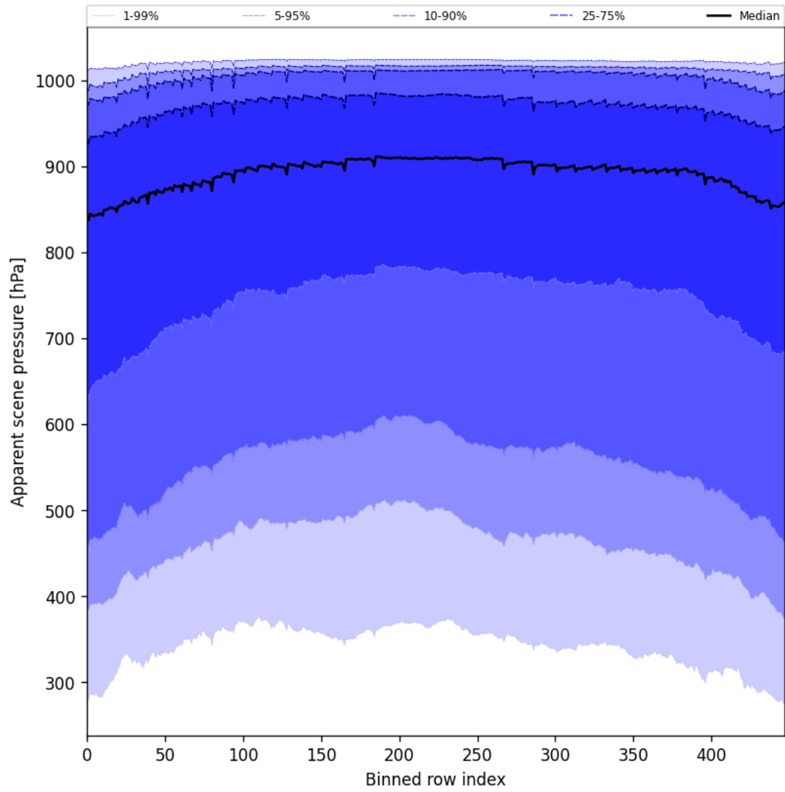
Figure 51: Along track statistics of “Apparent scene pressure” for 2025-05-14 to 2025-05-15
