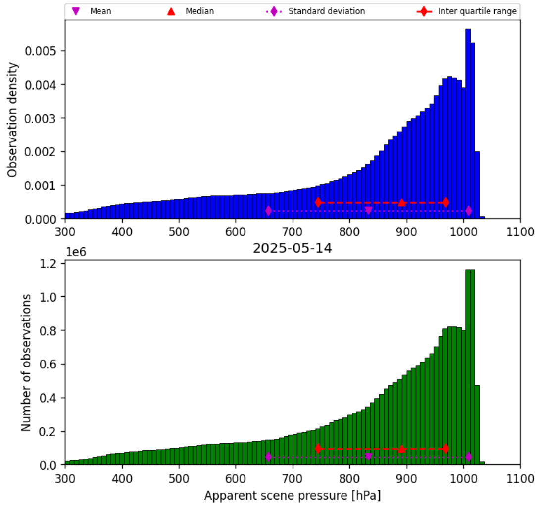
Figure 34: Histogram of “Apparent scene pressure” for 2025-05-14 to 2025-05-15
