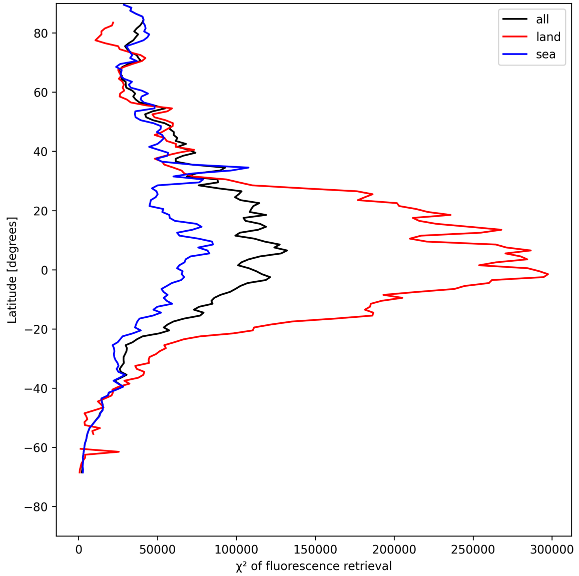
Figure 23: Zonal average of “ \chi^2 of fluorescence retrieval” for 2025-05-14 to 2025-05-15.
