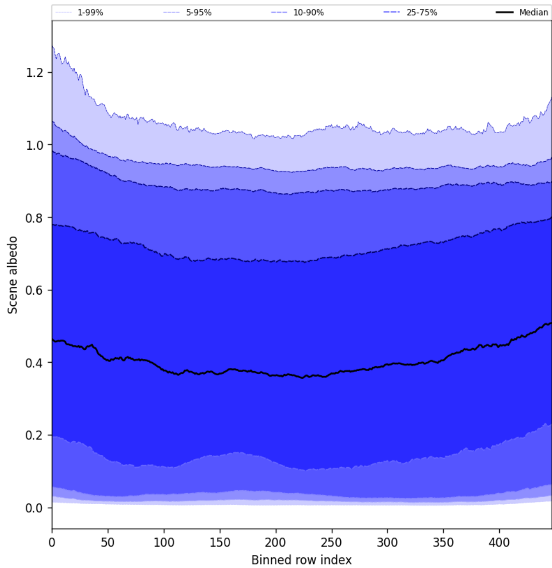
Figure 49: Along track statistics of “Scene albedo” for 2025-05-14 to 2025-05-15
