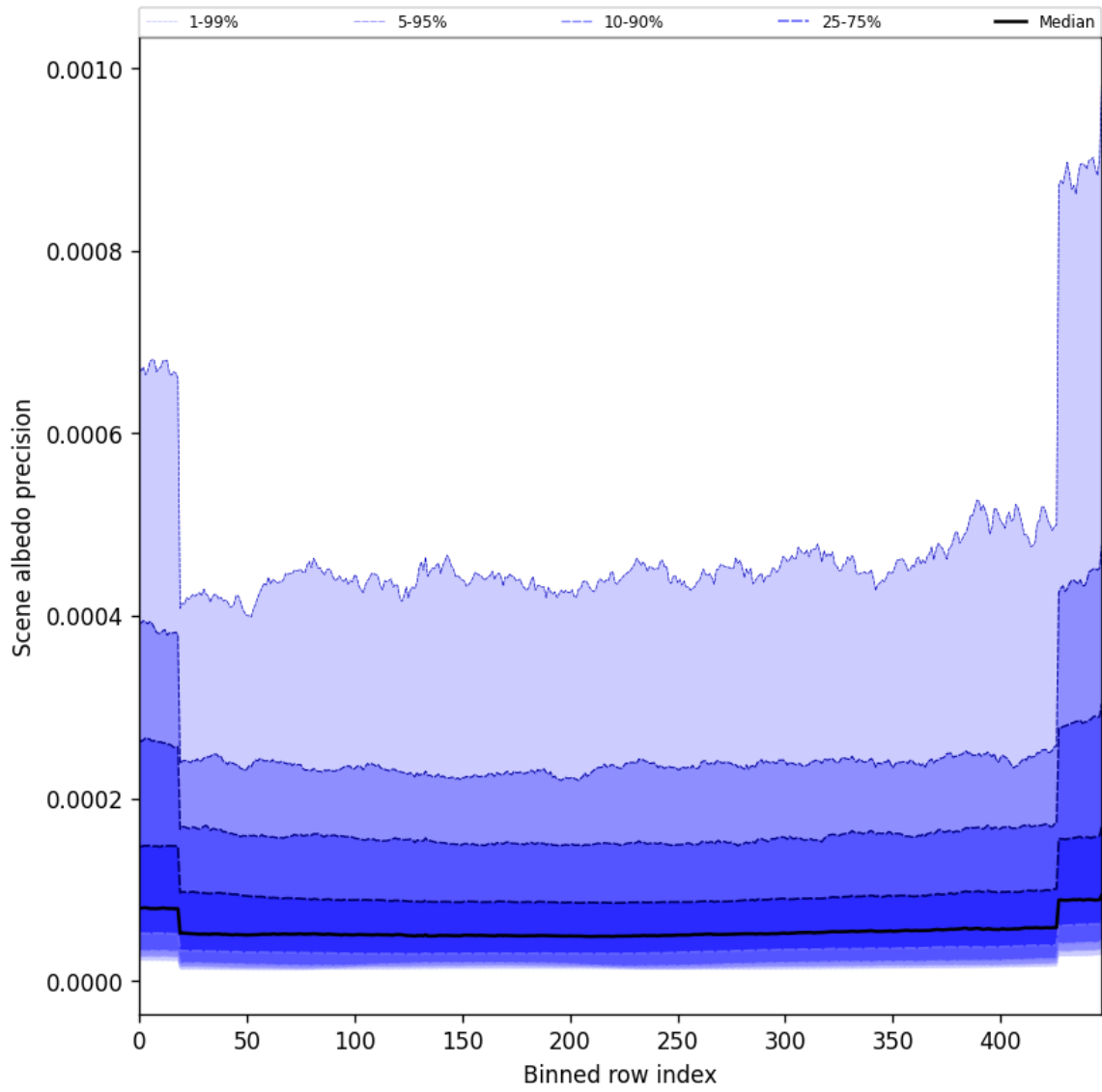
Figure 50: Along track statistics of “Scene albedo precision” for 2025-05-14 to 2025-05-15
