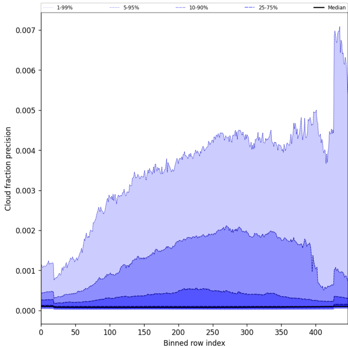
Figure 48: Along track statistics of “Cloud fraction precision” for 2025-05-14 to 2025-05-15
