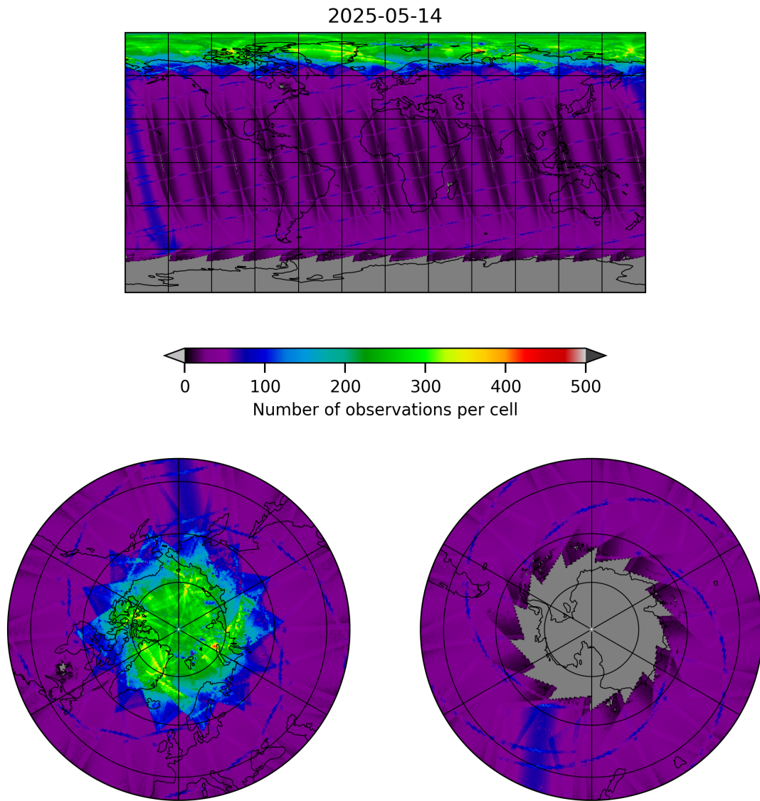
Figure 9: Map of the number of observations for 2025-05-14 to 2025-05-15
