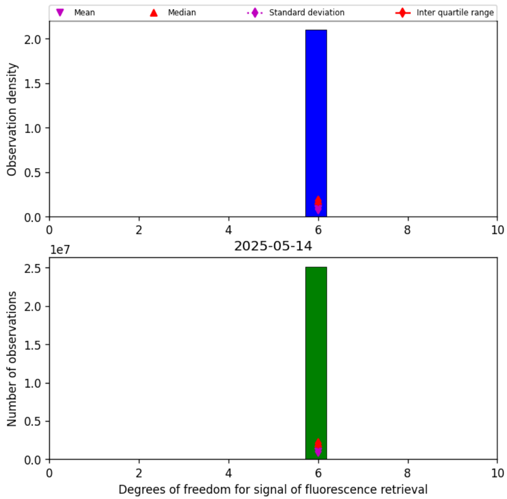
Figure 41: Histogram of “Degrees of freedom for signal of fluorescence retrieval” for 2025-05-14 to 2025-05-15
