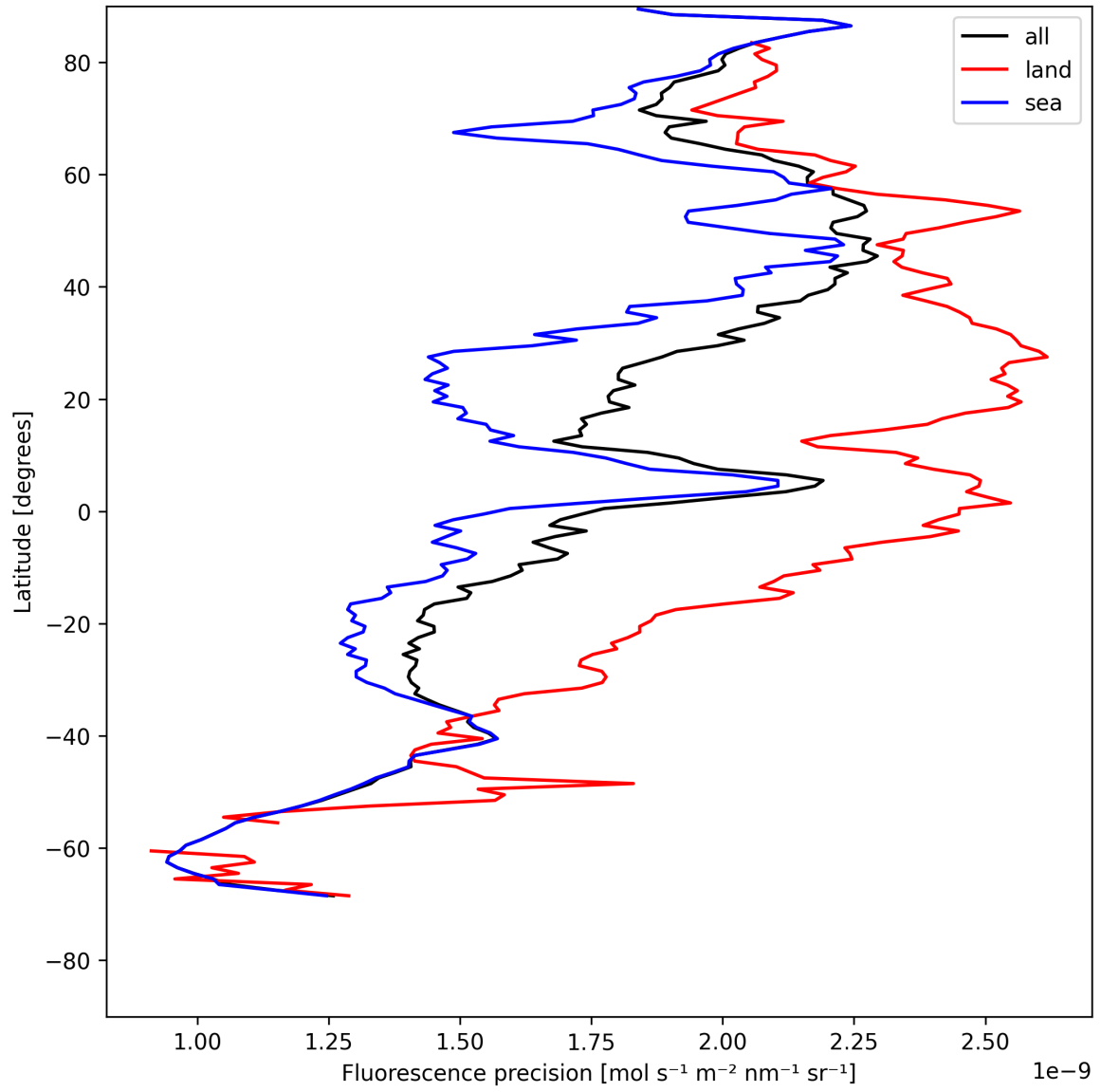
Figure 22: Zonal average of “Fluorescence precision” for 2025-05-14 to 2025-05-15.
