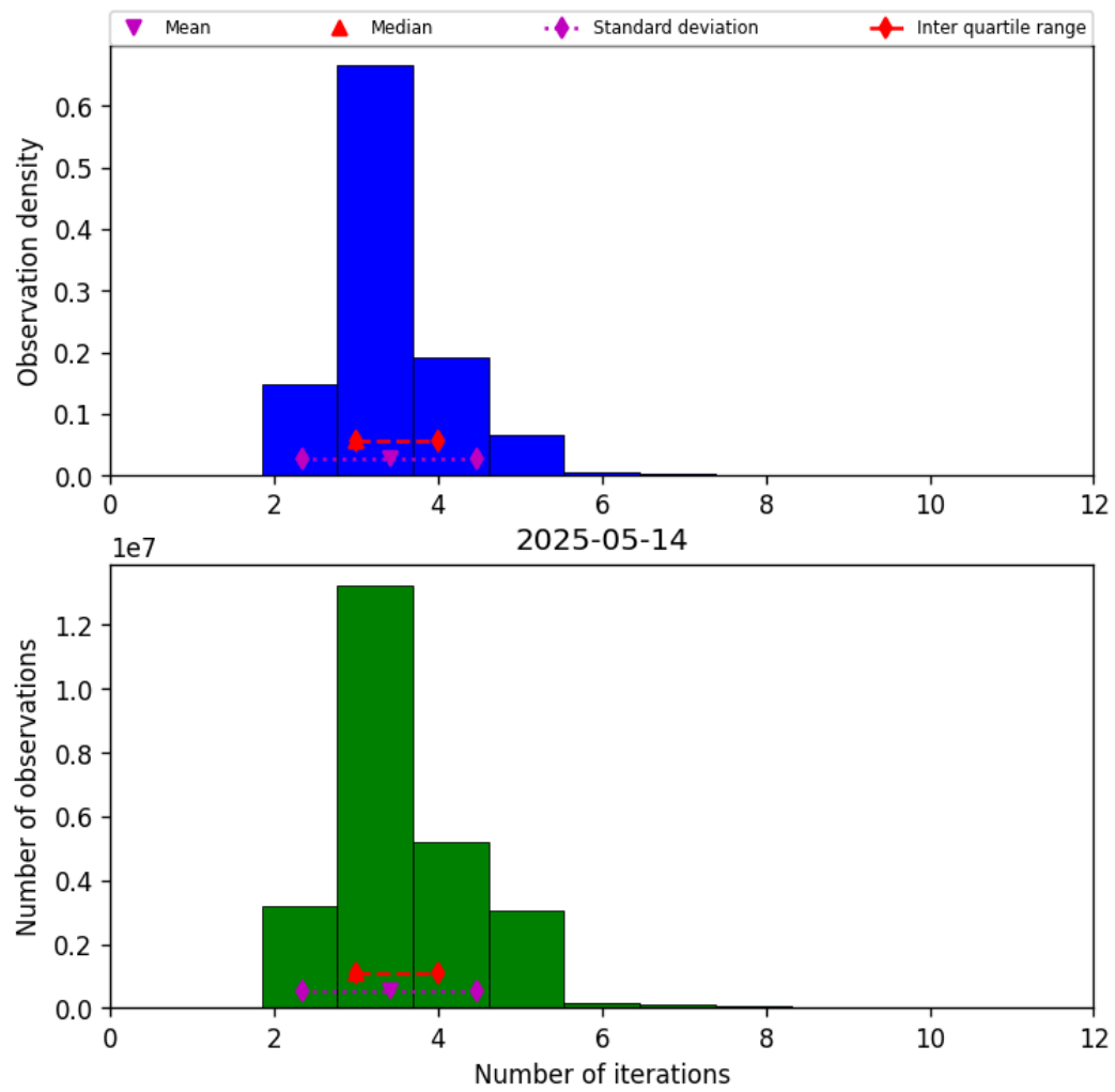
Figure 37: Histogram of “Number of iterations” for 2025-05-14 to 2025-05-15
