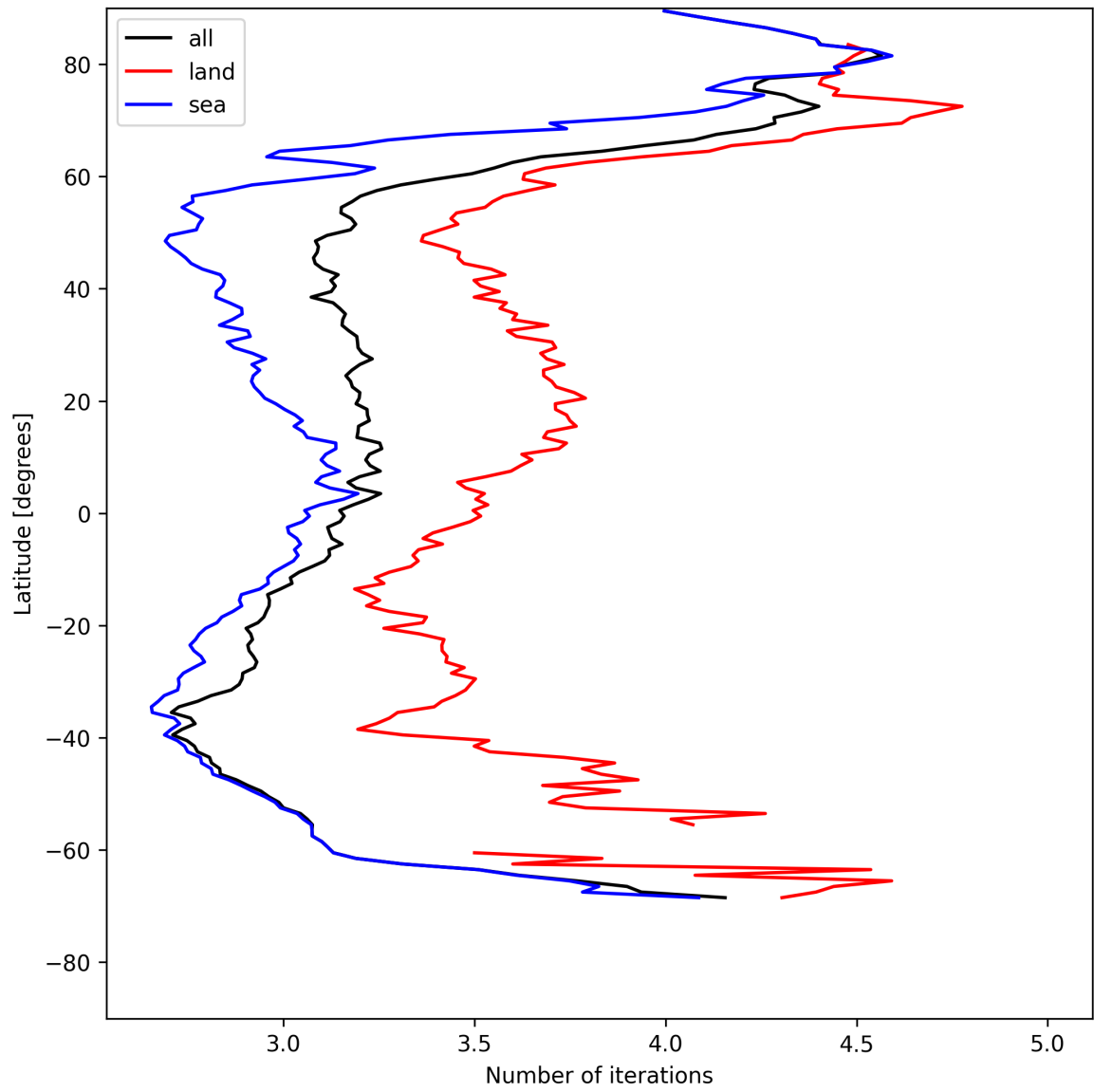
Figure 20: Zonal average of “Number of iterations” for 2025-05-14 to 2025-05-15.
