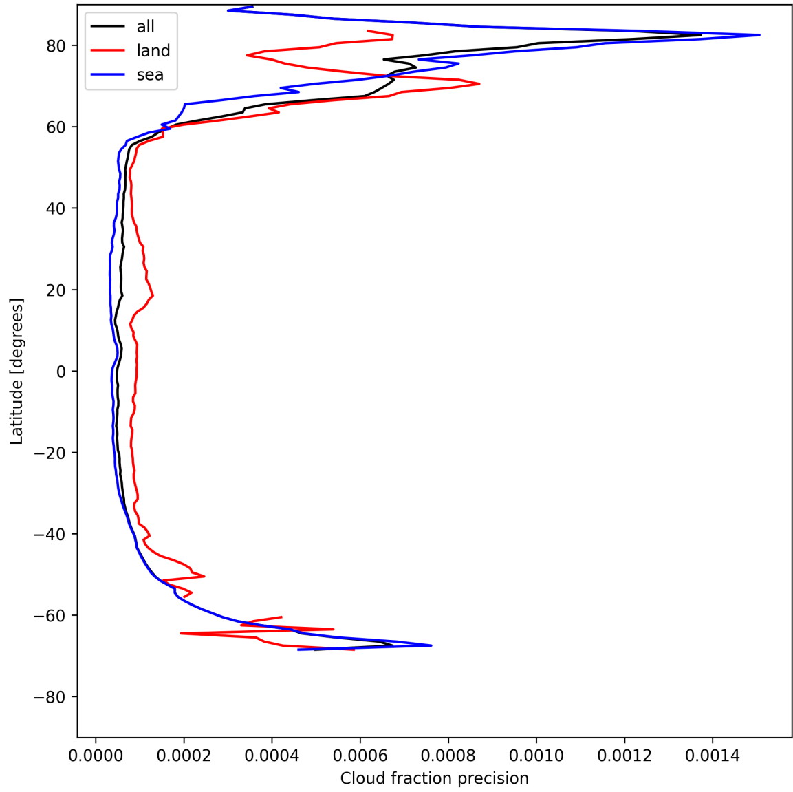
Figure 14: Zonal average of “Cloud fraction precision” for 2025-05-14 to 2025-05-15.
