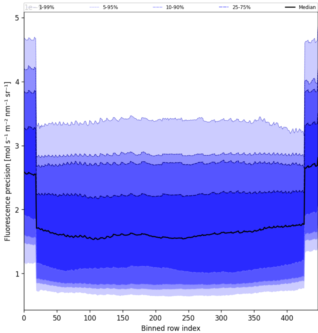
Figure 56: Along track statistics of “Fluorescence precision” for 2025-05-14 to 2025-05-15
