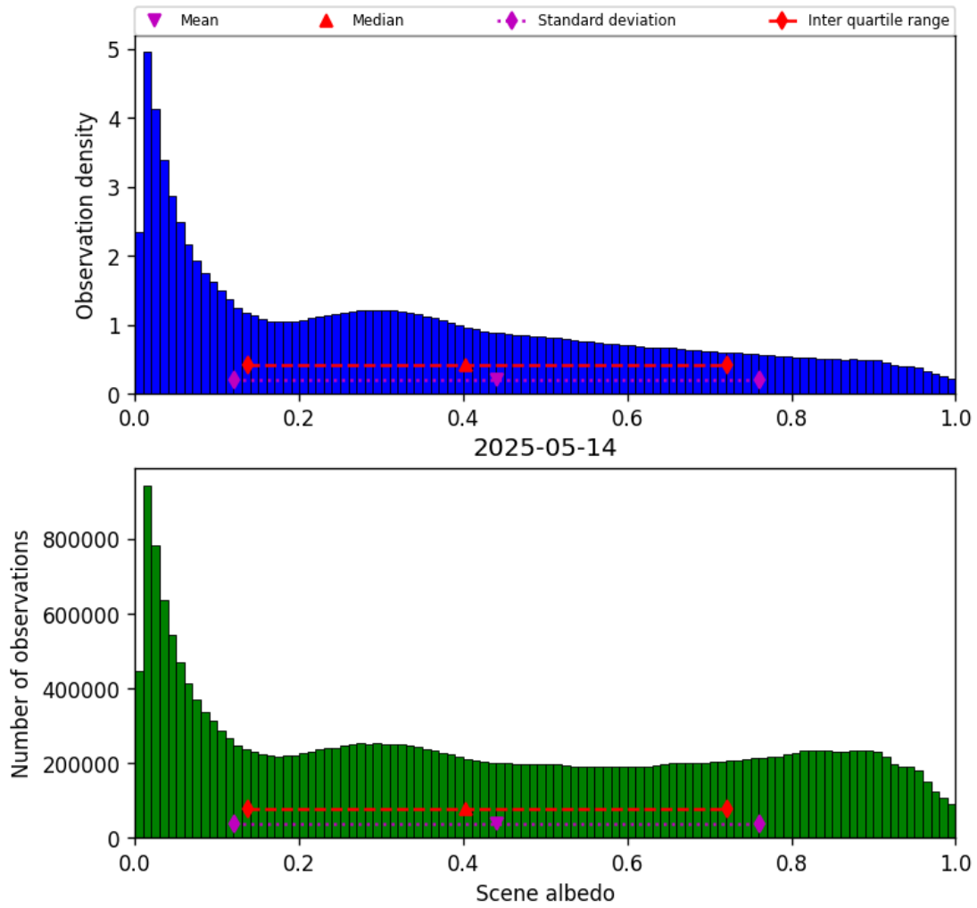
Figure 32: Histogram of “Scene albedo” for 2025-05-14 to 2025-05-15
