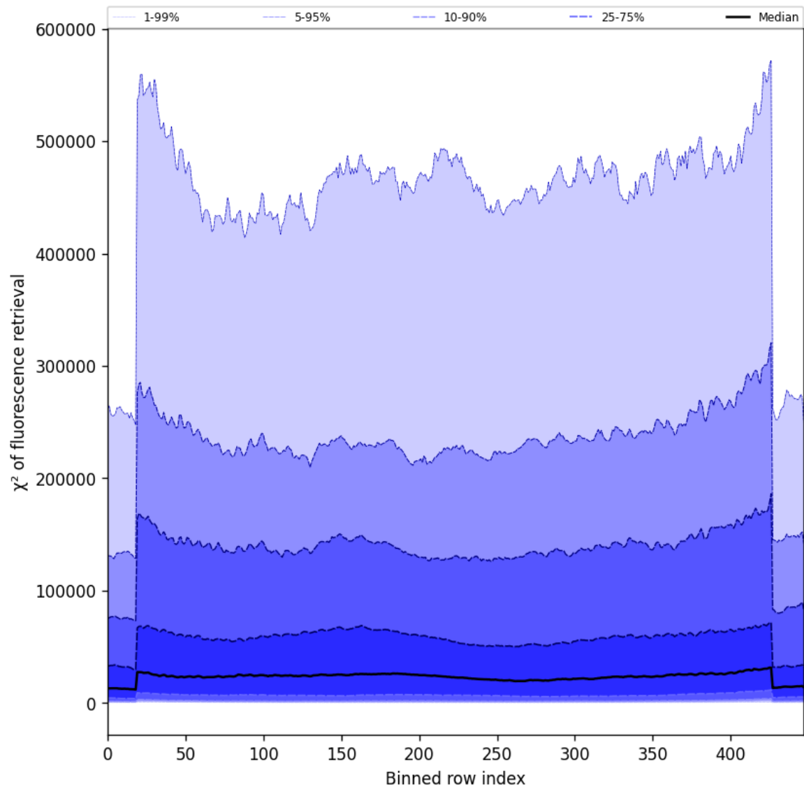
Figure 57: Along track statistics of “ \chi^2 of fluorescence retrieval” for 2025-05-14 to 2025-05-15
