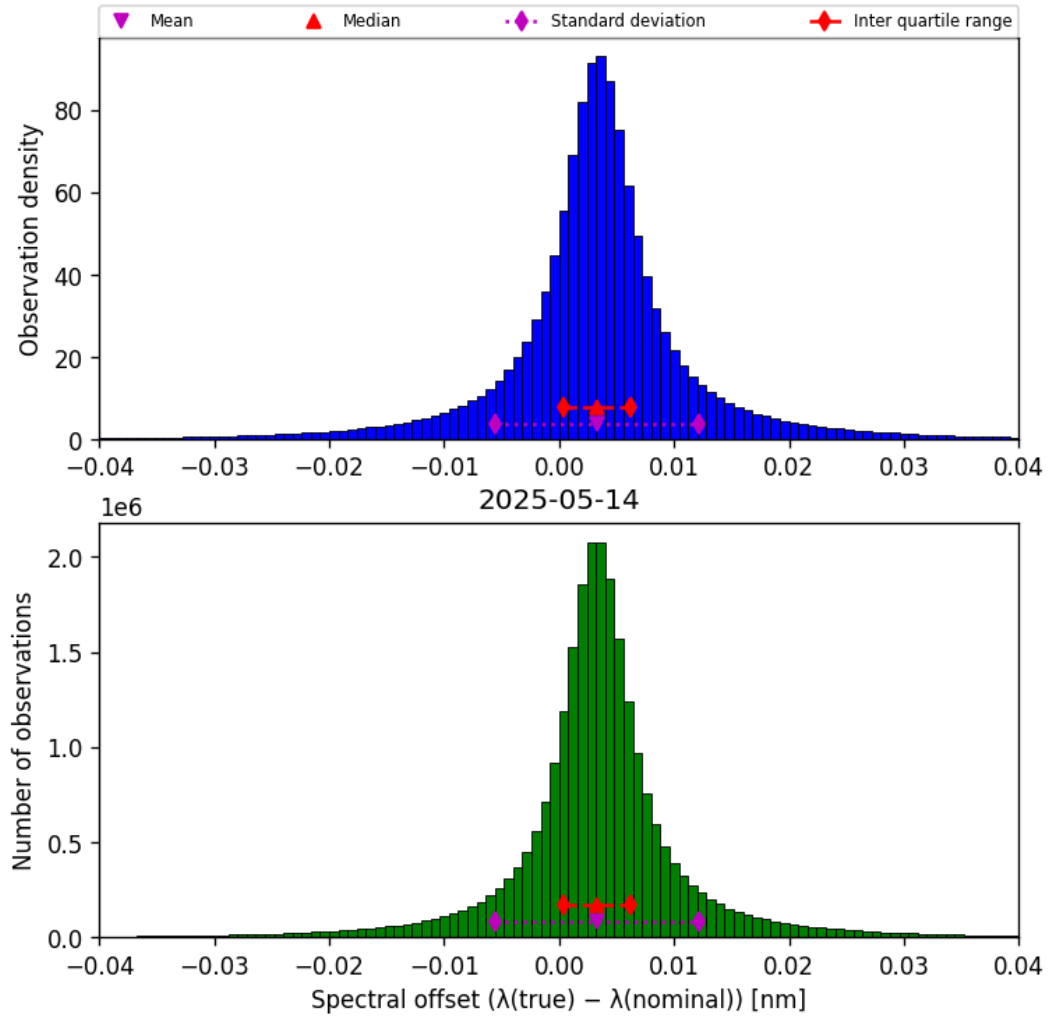
Figure 43: Histogram of “Spectral offset ( \lambda_{\text{true}} - \lambda_{\text{nominal}} )” for 2025-05-14 to 2025-05-15
