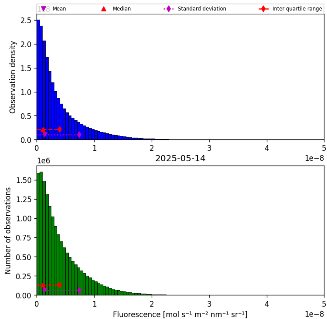
Figure 38: Histogram of “Fluorescence” for 2025-05-14 to 2025-05-15
