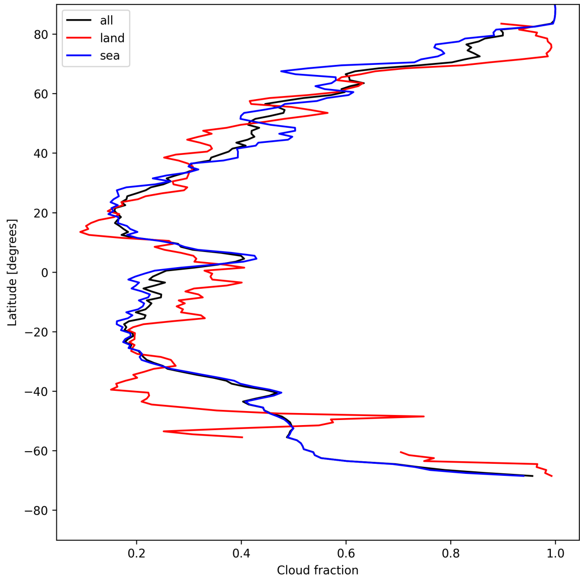
Figure 13: Zonal average of “Cloud fraction” for 2025-05-14 to 2025-05-15.
