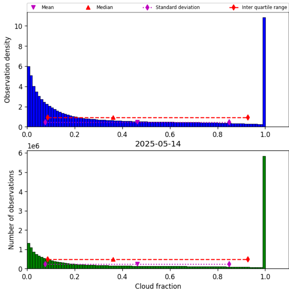
Figure 30: Histogram of “Cloud fraction” for 2025-05-14 to 2025-05-15
