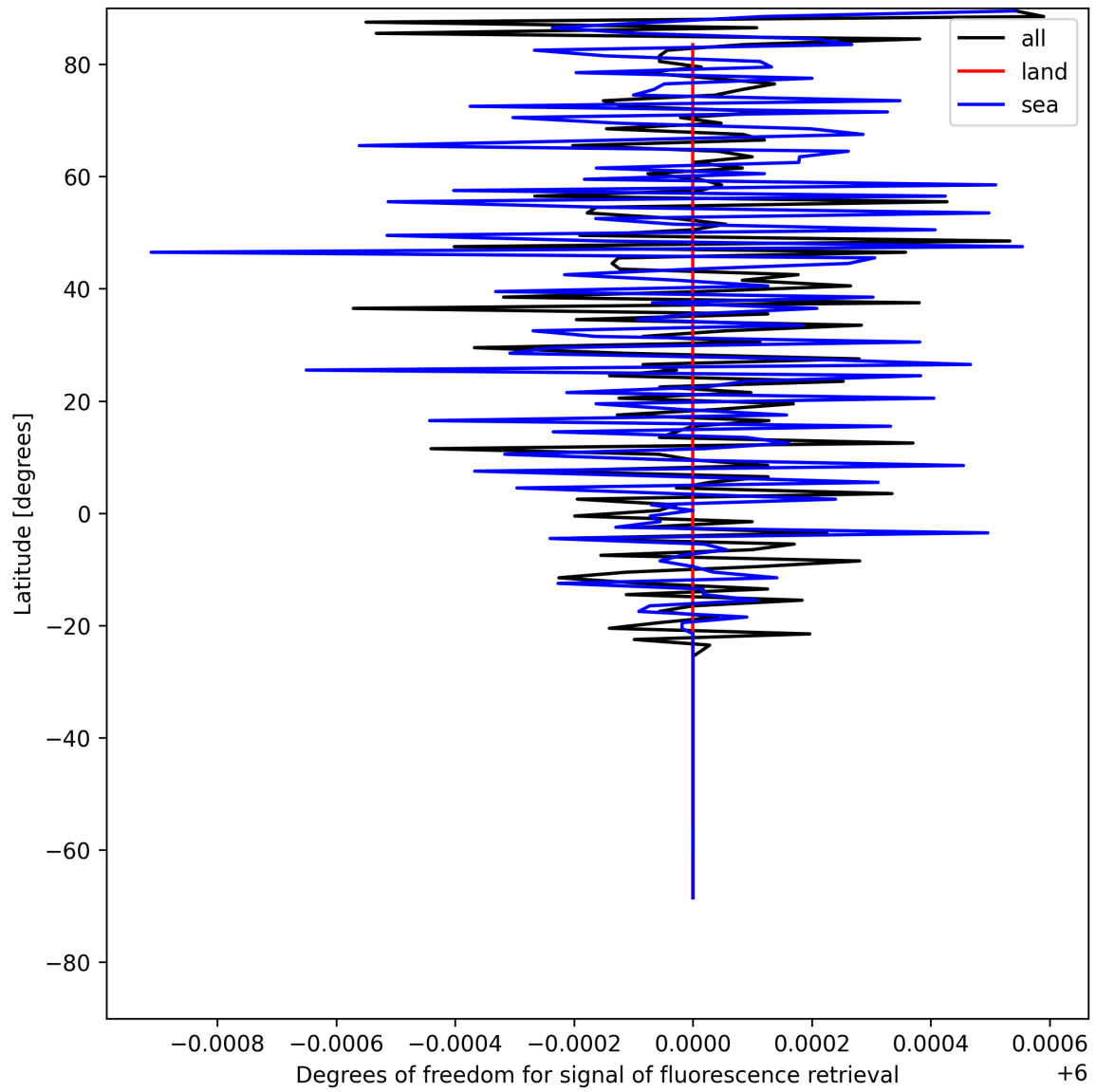
Figure 24: Zonal average of “Degrees of freedom for signal of fluorescence retrieval” for 2025-05-14 to 2025-05-15.
