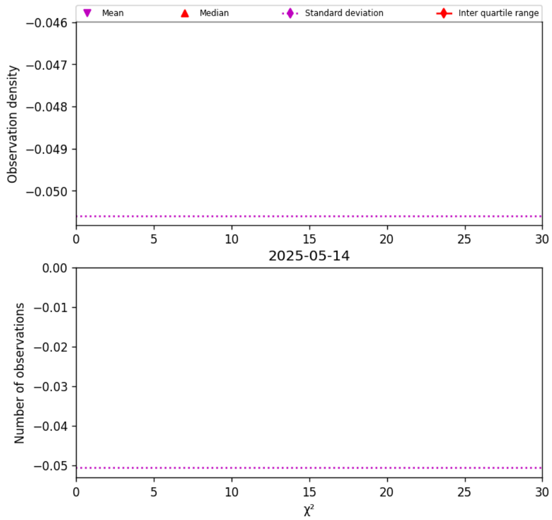
Figure 36: Histogram of " \chi^2 " for 2025-05-14 to 2025-05-15
