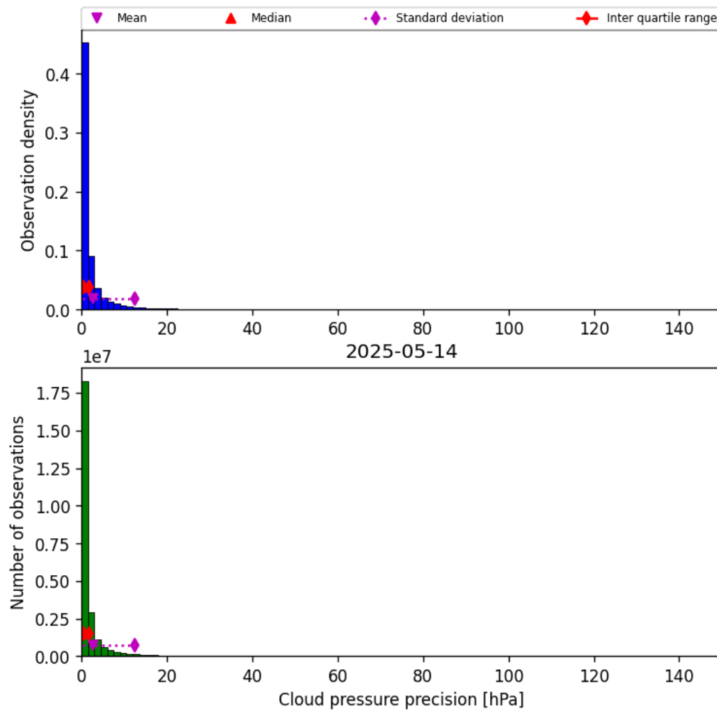
Figure 29: Histogram of “Cloud pressure precision” for 2025-05-14 to 2025-05-15
