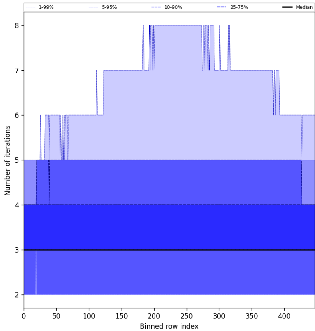
Figure 54: Along track statistics of “Number of iterations” for 2025-05-14 to 2025-05-15
