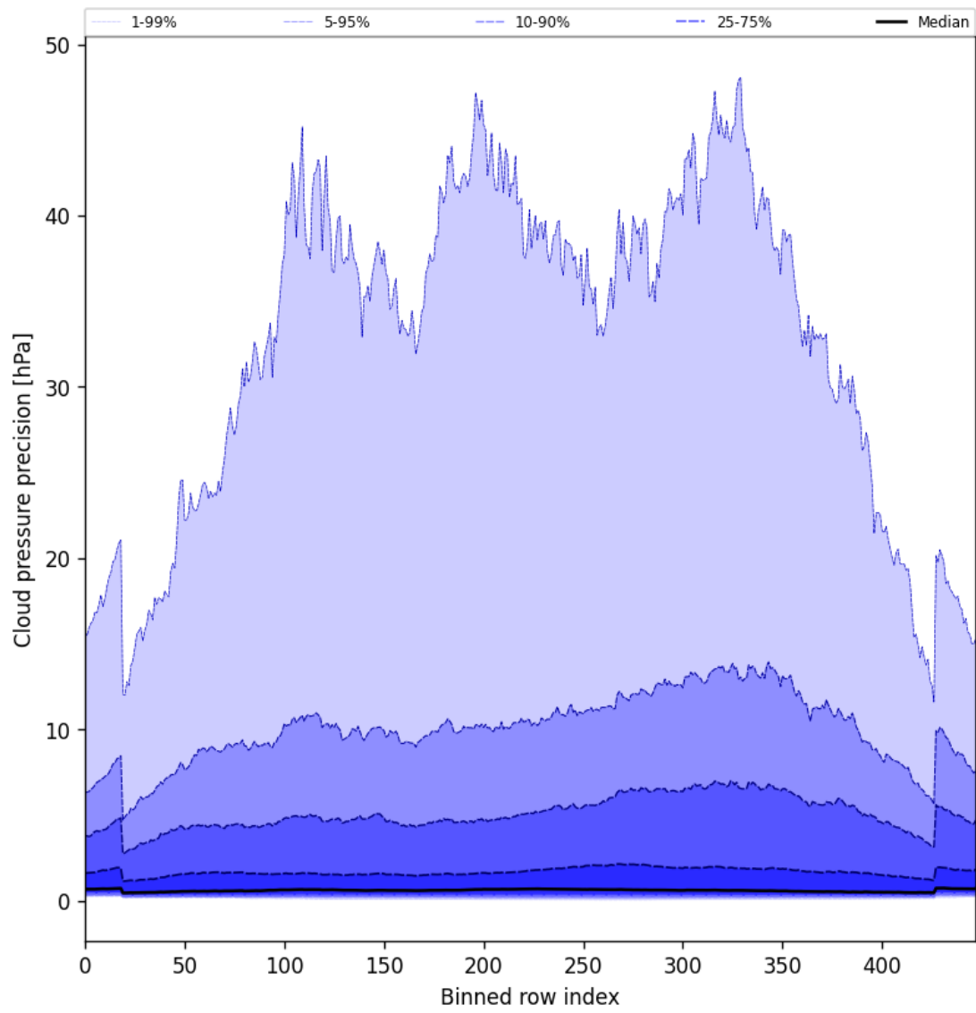
Figure 46: Along track statistics of “Cloud pressure precision” for 2025-05-14 to 2025-05-15
