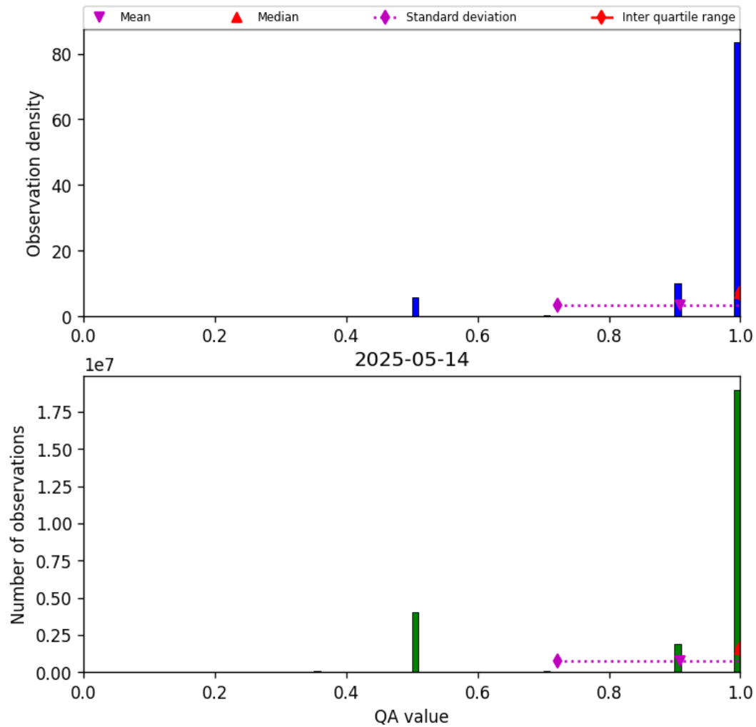
Figure 27: Histogram of “QA value” for 2025-05-14 to 2025-05-15
