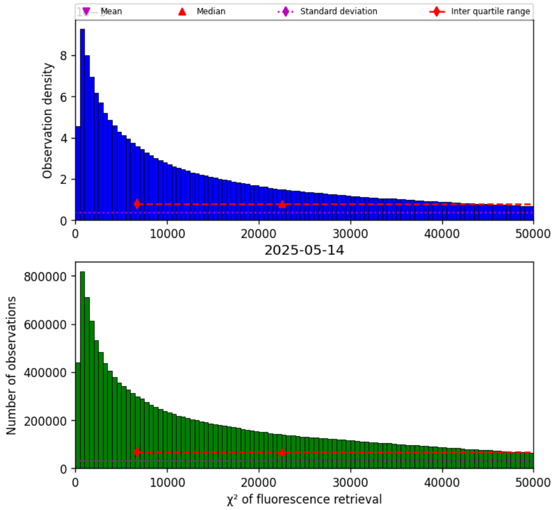
Figure 40: Histogram of “ \chi^2 of fluorescence retrieval” for 2025-05-14 to 2025-05-15
