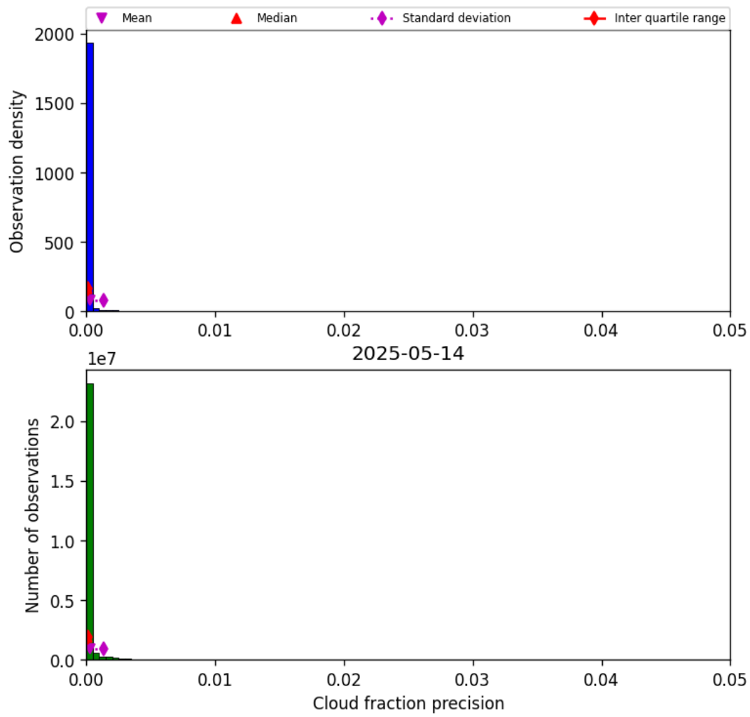
Figure 31: Histogram of “Cloud fraction precision” for 2025-05-14 to 2025-05-15
