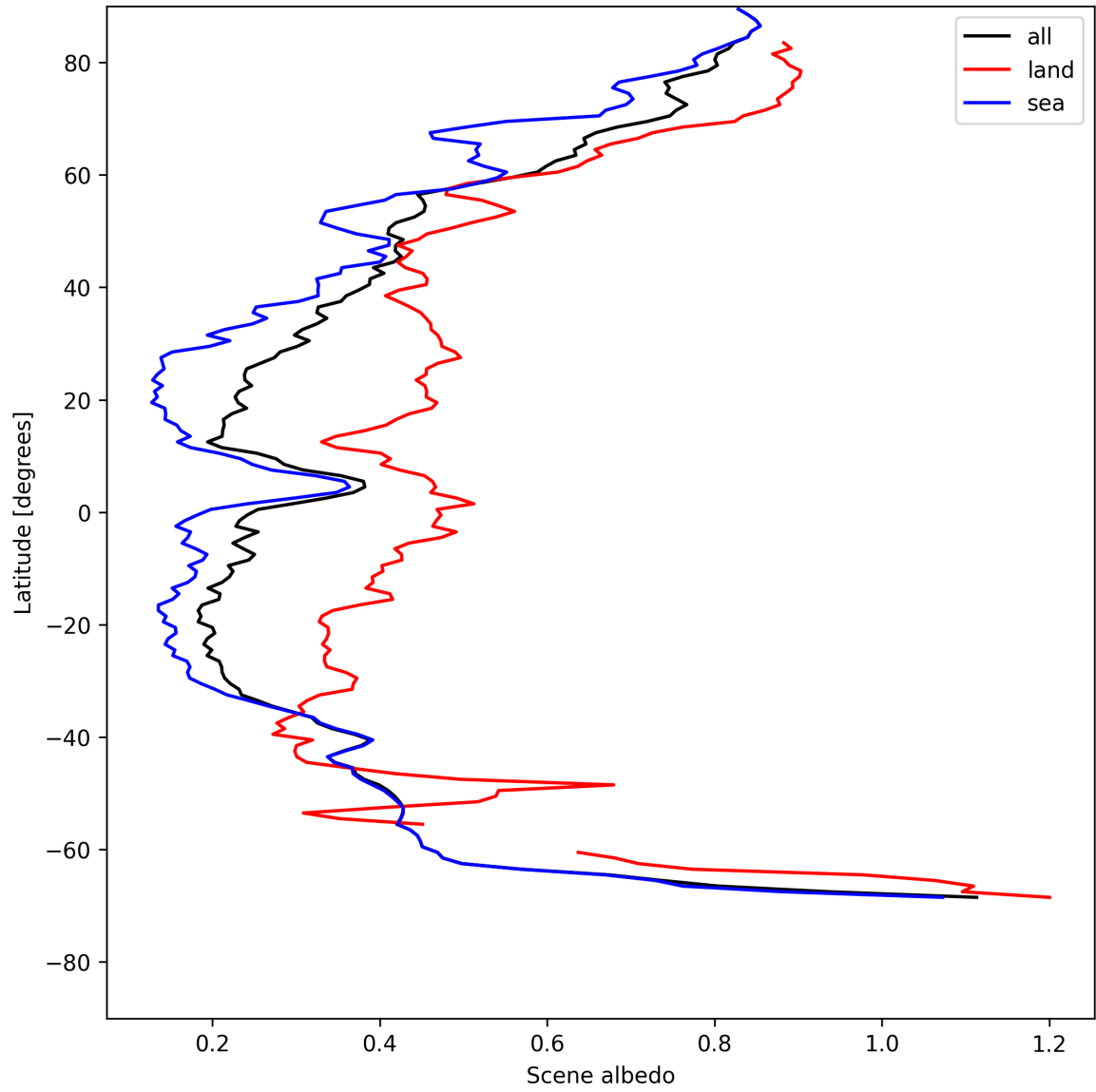
Figure 15: Zonal average of “Scene albedo” for 2025-05-14 to 2025-05-15.
