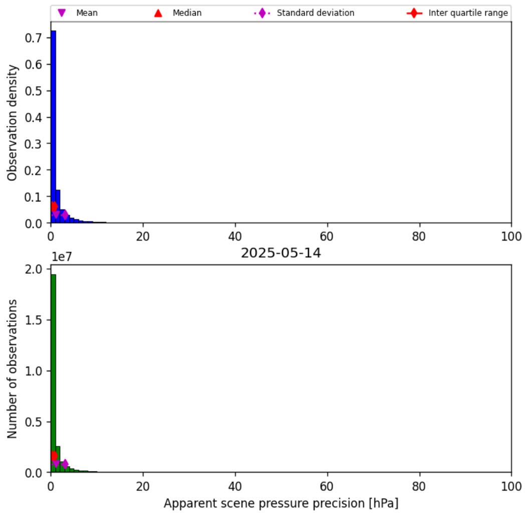
Figure 35: Histogram of “Apparent scene pressure precision” for 2025-05-14 to 2025-05-15
