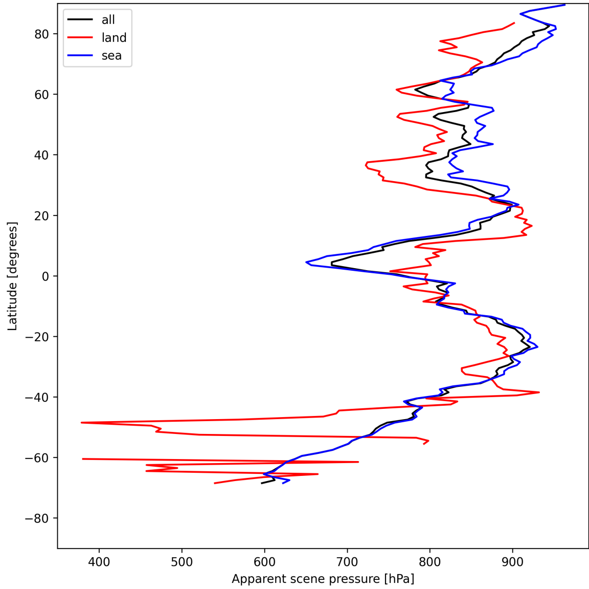
Figure 17: Zonal average of “Apparent scene pressure” for 2025-05-14 to 2025-05-15.
