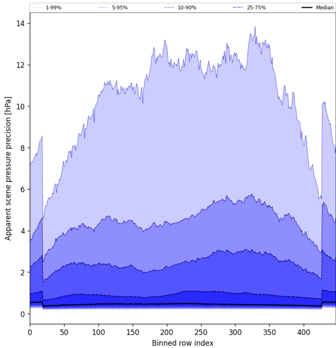
Figure 52: Along track statistics of “Apparent scene pressure precision” for 2025-05-14 to 2025-05-15
