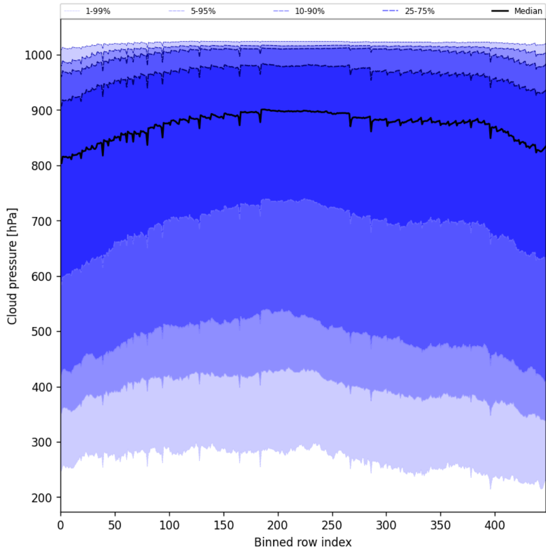
Figure 45: Along track statistics of “Cloud pressure” for 2025-05-14 to 2025-05-15
