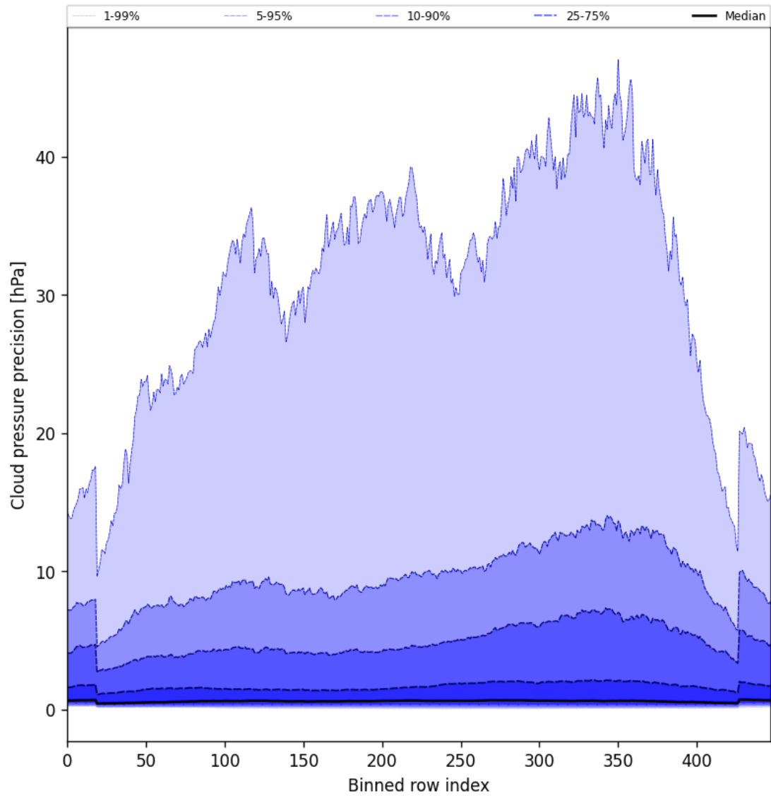
Figure 46: Along track statistics of “Cloud pressure precision” for 2025-05-16 to 2025-05-17
