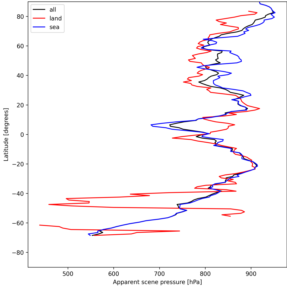
Figure 17: Zonal average of “Apparent scene pressure” for 2025-05-16 to 2025-05-17.
