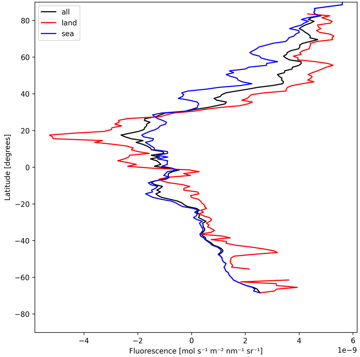
Figure 21: Zonal average of “Fluorescence” for 2025-05-16 to 2025-05-17.
