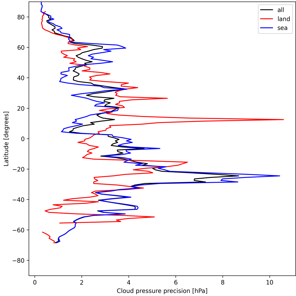
Figure 12: Zonal average of “Cloud pressure precision” for 2025-05-16 to 2025-05-17.
