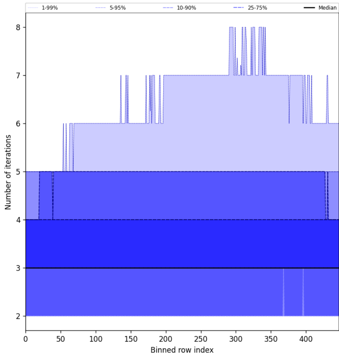
Figure 54: Along track statistics of “Number of iterations” for 2025-05-16 to 2025-05-17
