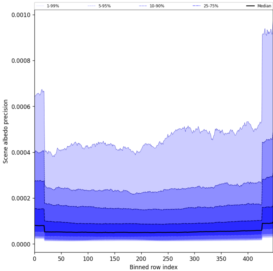
Figure 50: Along track statistics of “Scene albedo precision” for 2025-05-16 to 2025-05-17
