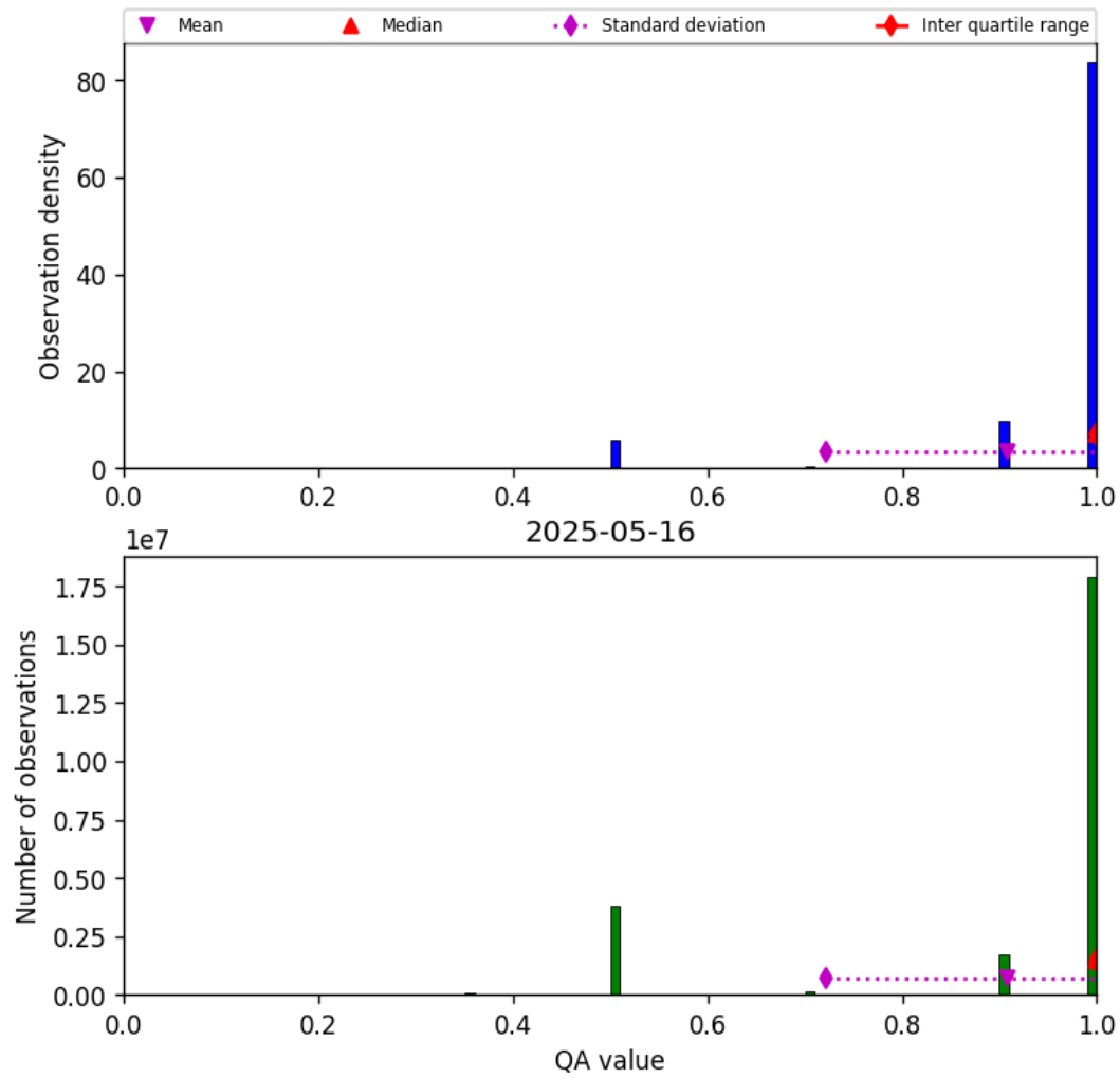
Figure 27: Histogram of “QA value” for 2025-05-16 to 2025-05-17
