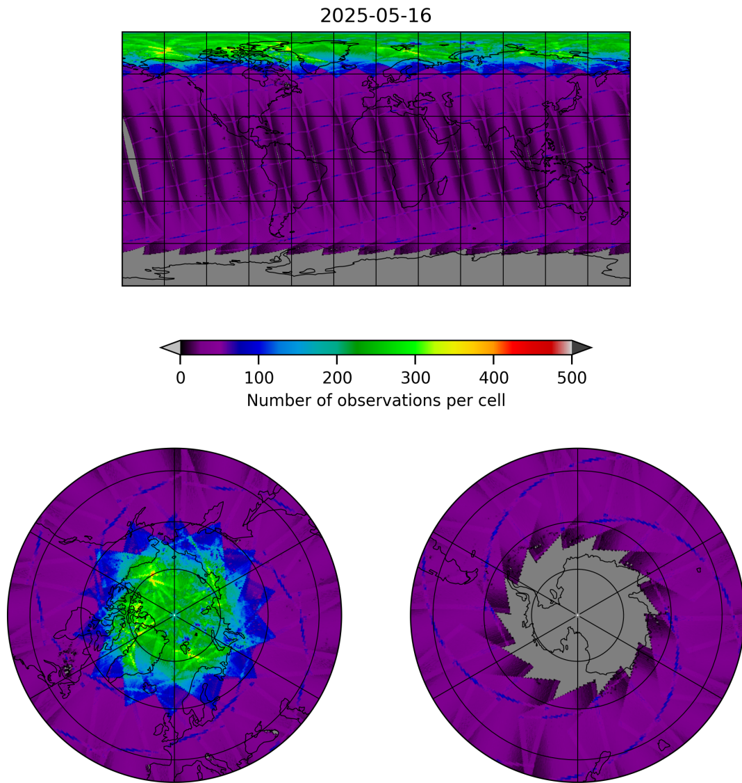
Figure 9: Map of the number of observations for 2025-05-16 to 2025-05-17
