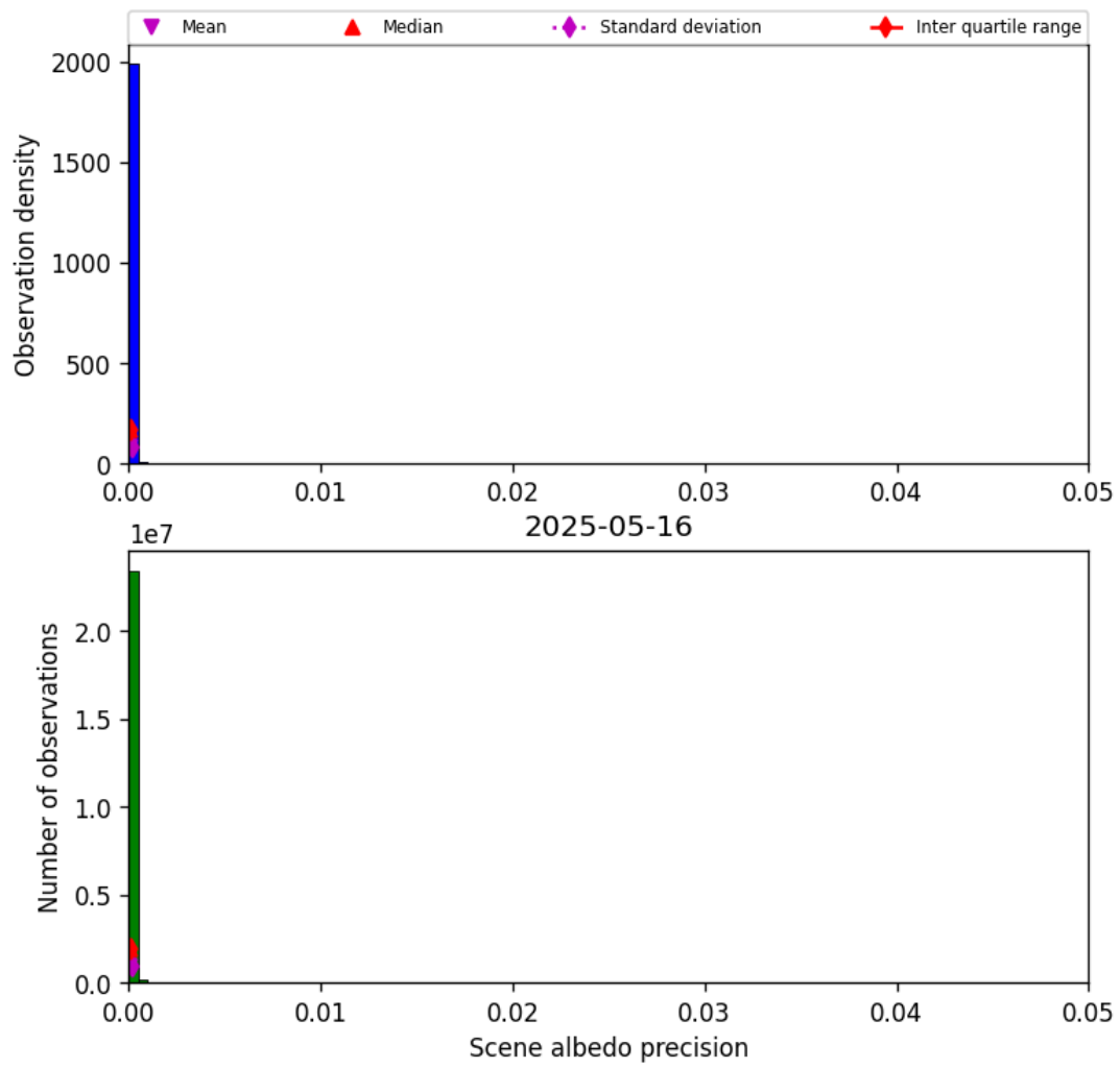
Figure 33: Histogram of “Scene albedo precision” for 2025-05-16 to 2025-05-17
