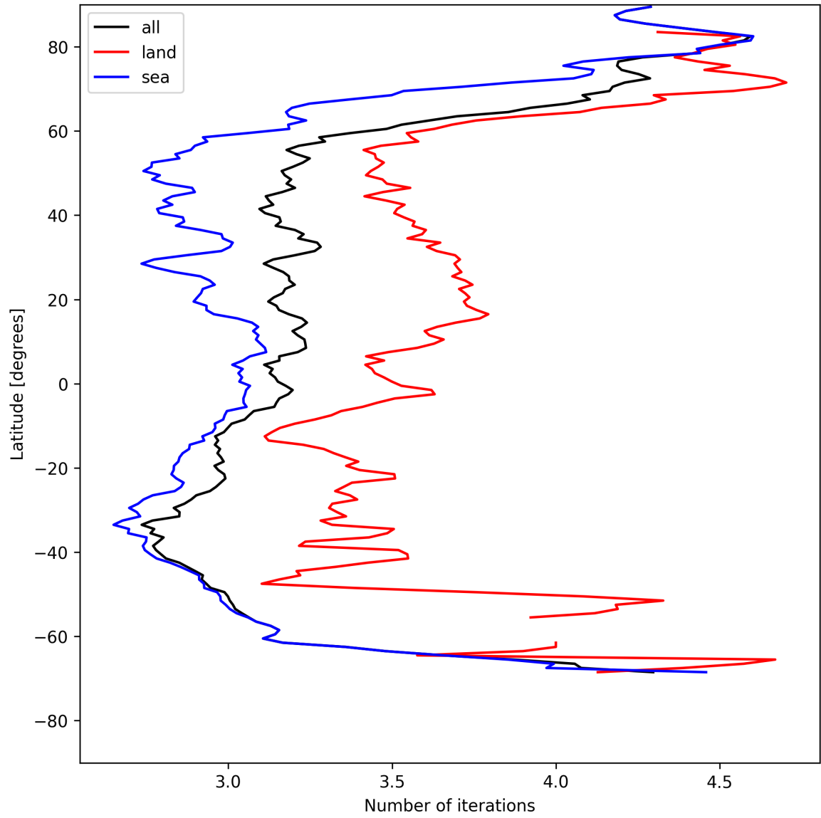
Figure 20: Zonal average of “Number of iterations” for 2025-05-16 to 2025-05-17.
