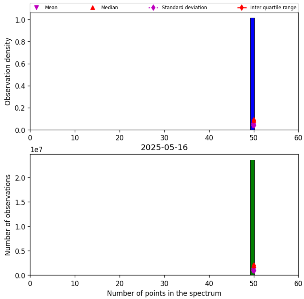
Figure 42: Histogram of “Number of points in the spectrum” for 2025-05-16 to 2025-05-17
