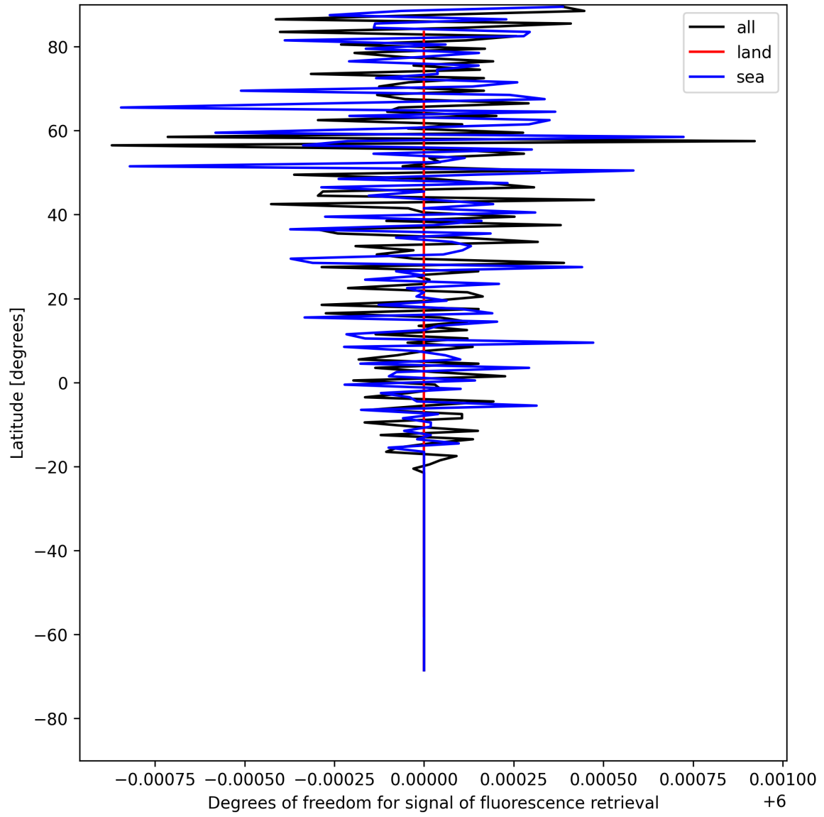
Figure 24: Zonal average of “Degrees of freedom for signal of fluorescence retrieval” for 2025-05-16 to 2025-05-17.
