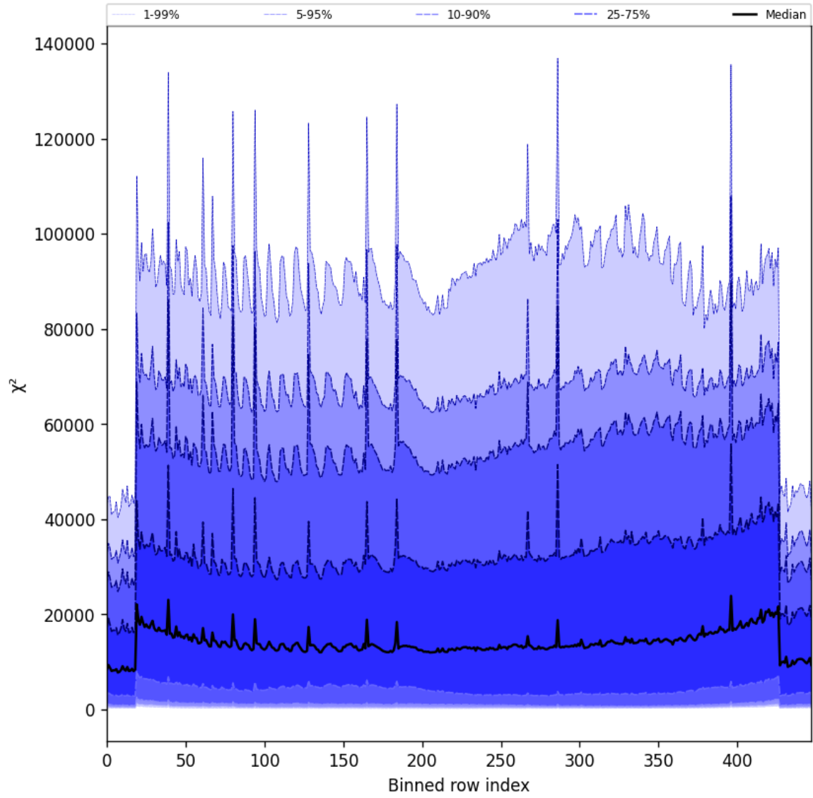
Figure 53: Along track statistics of “ \chi^2 ” for 2025-05-16 to 2025-05-17
