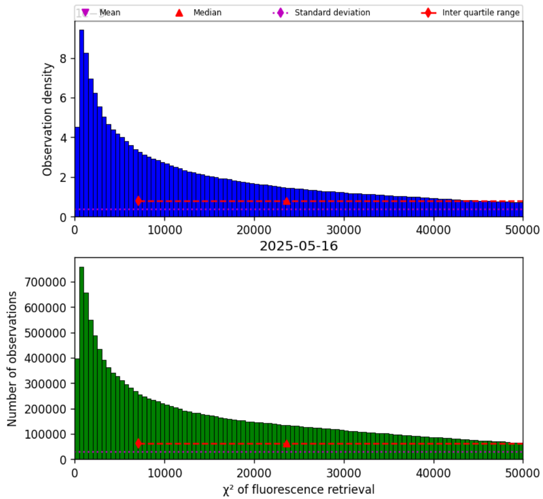
Figure 40: Histogram of “ \chi^2 of fluorescence retrieval” for 2025-05-16 to 2025-05-17
