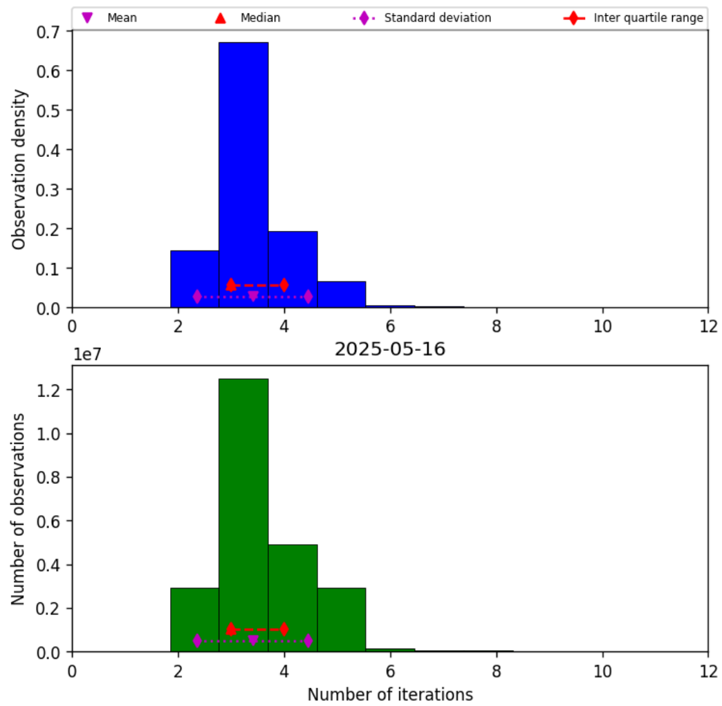
Figure 37: Histogram of “Number of iterations” for 2025-05-16 to 2025-05-17
