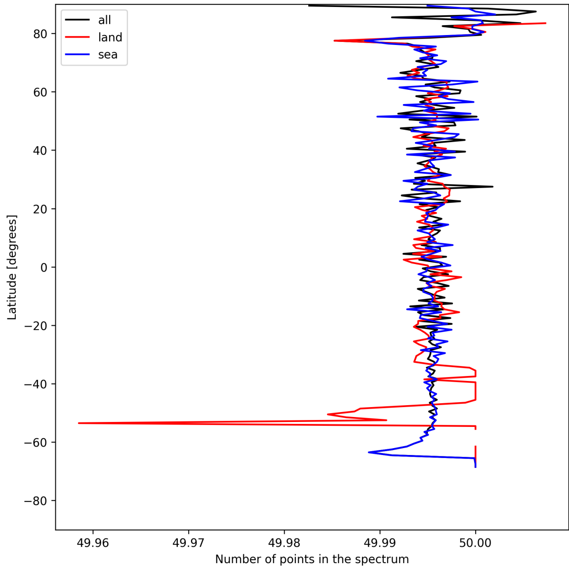
Figure 25: Zonal average of “Number of points in the spectrum” for 2025-05-16 to 2025-05-17.
