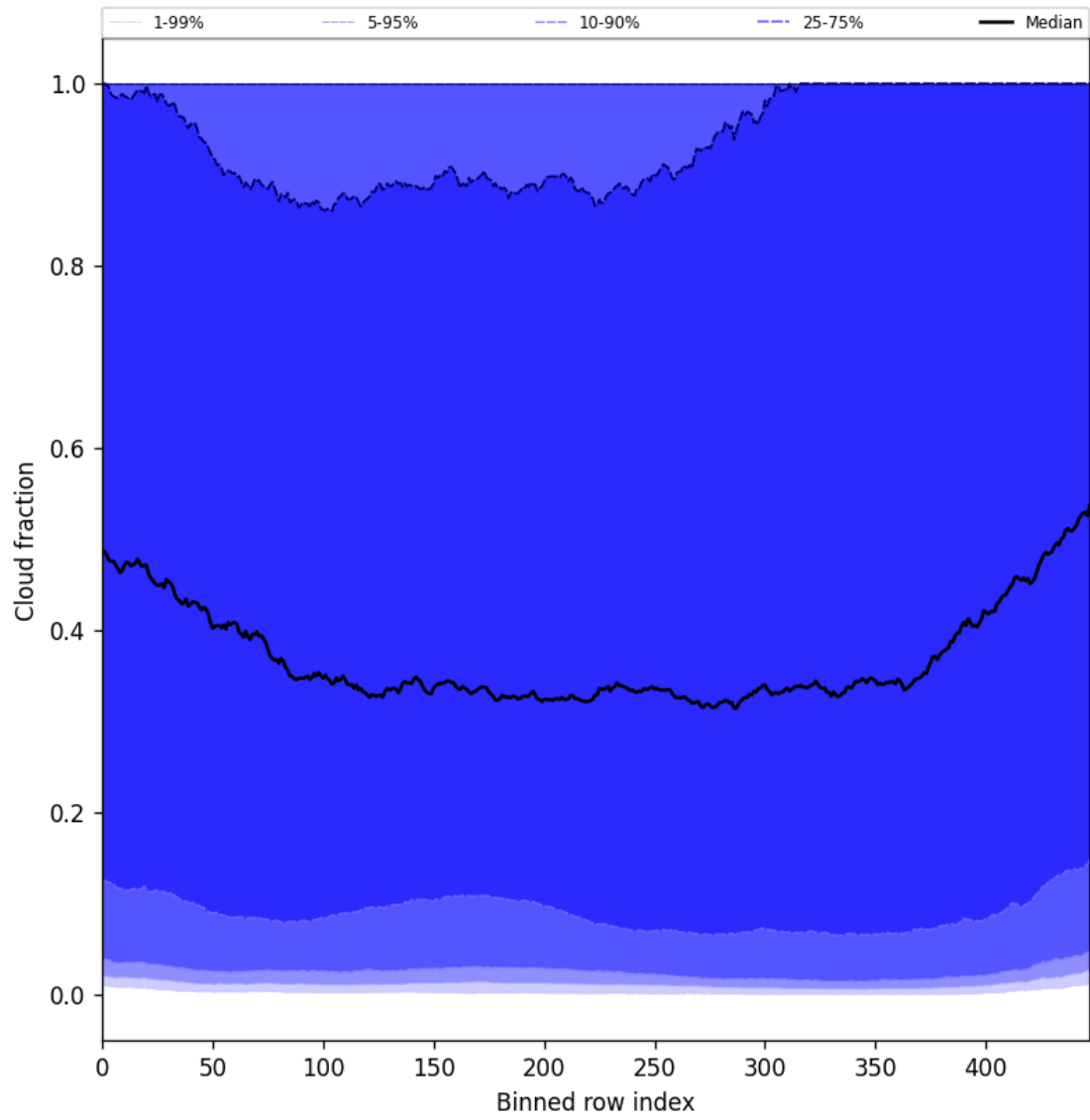
Figure 47: Along track statistics of “Cloud fraction” for 2025-05-16 to 2025-05-17
