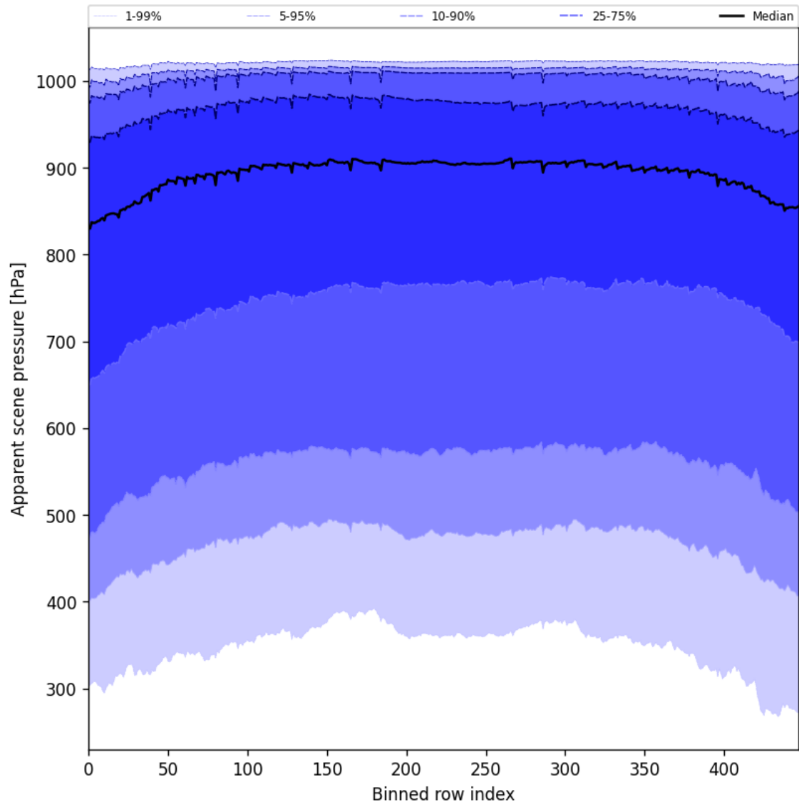
Figure 51: Along track statistics of “Apparent scene pressure” for 2025-05-16 to 2025-05-17
