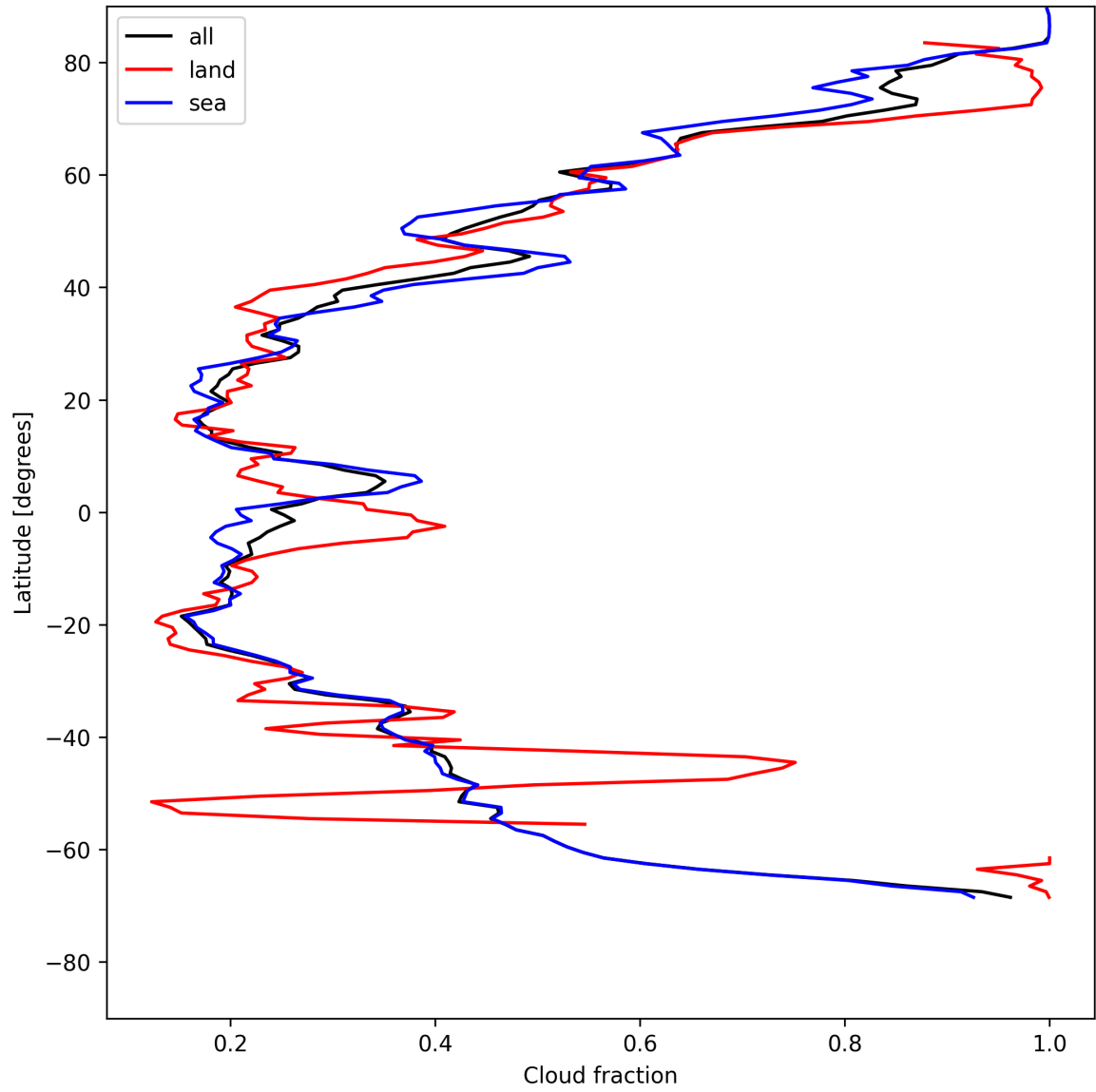
Figure 13: Zonal average of “Cloud fraction” for 2025-05-16 to 2025-05-17.
