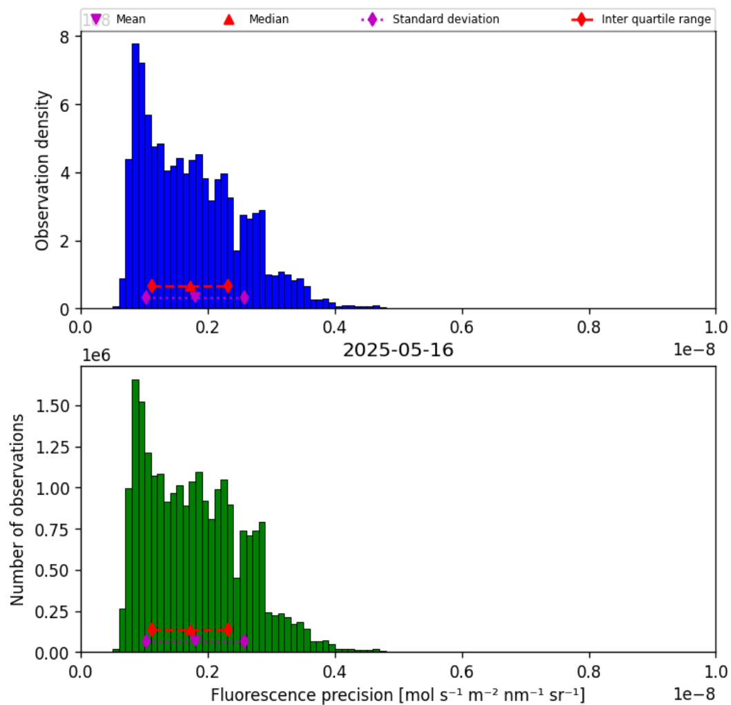
Figure 39: Histogram of “Fluorescence precision” for 2025-05-16 to 2025-05-17
