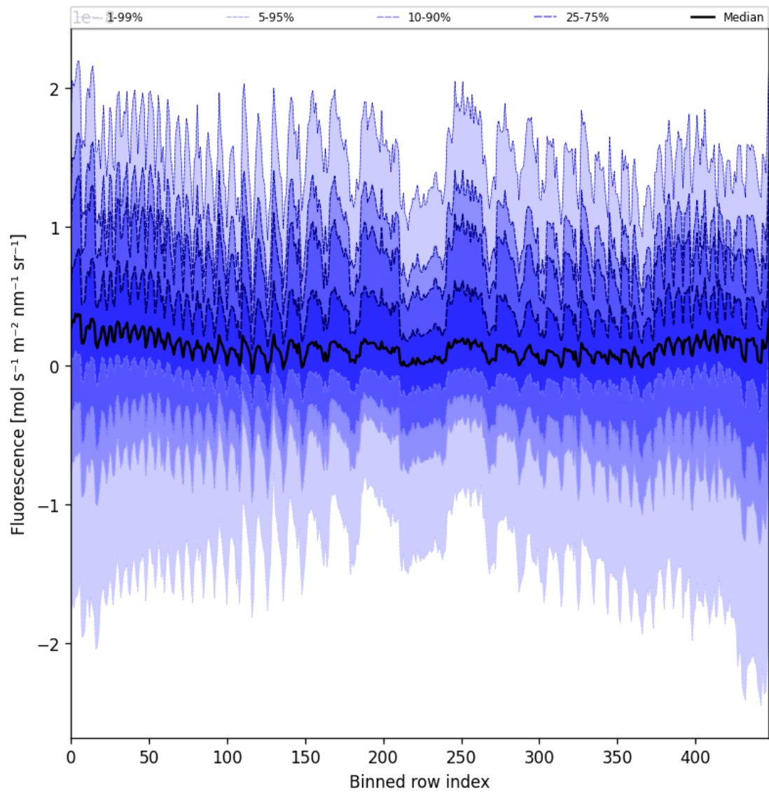
Figure 55: Along track statistics of “Fluorescence” for 2025-05-16 to 2025-05-17
