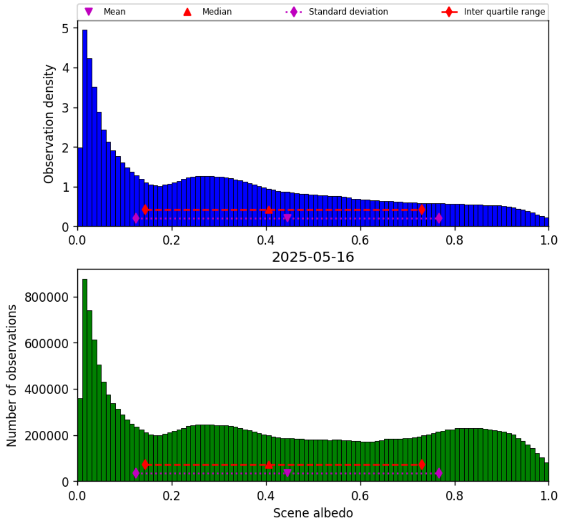
Figure 32: Histogram of “Scene albedo” for 2025-05-16 to 2025-05-17
