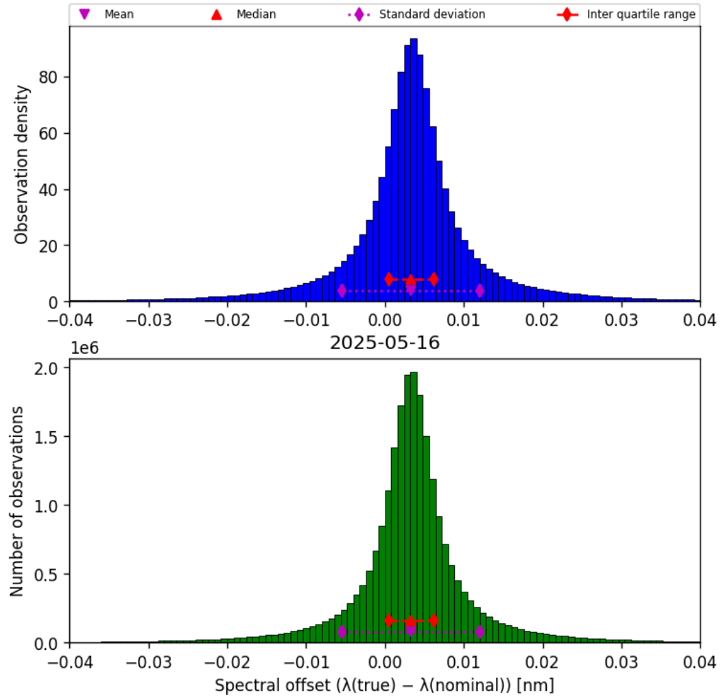
Figure 43: Histogram of “Spectral offset ( \lambda_{\text{true}} - \lambda_{\text{nominal}} )” for 2025-05-16 to 2025-05-17
