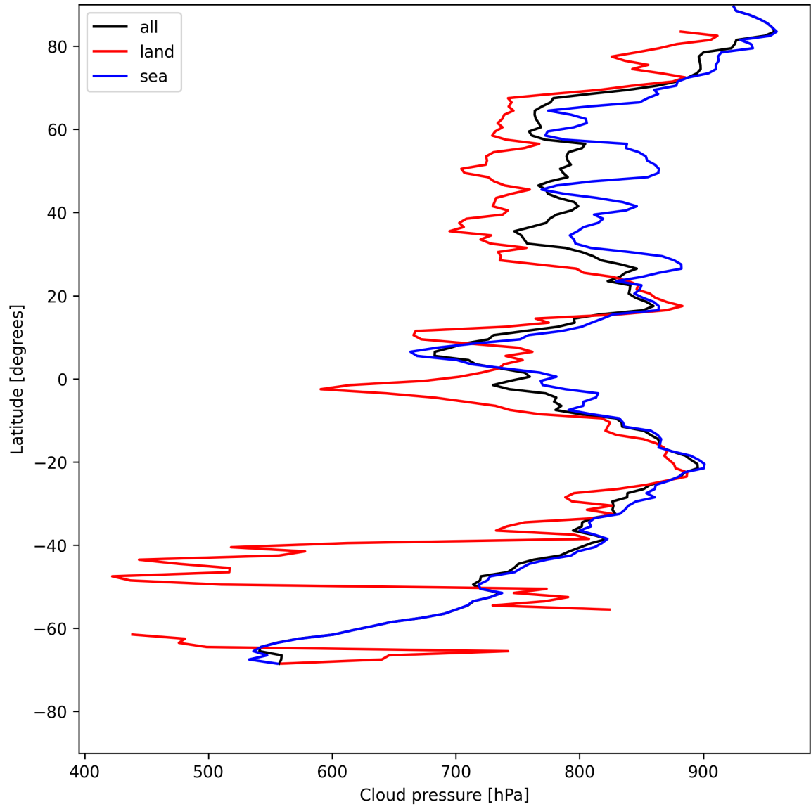
Figure 11: Zonal average of “Cloud pressure” for 2025-05-16 to 2025-05-17.
