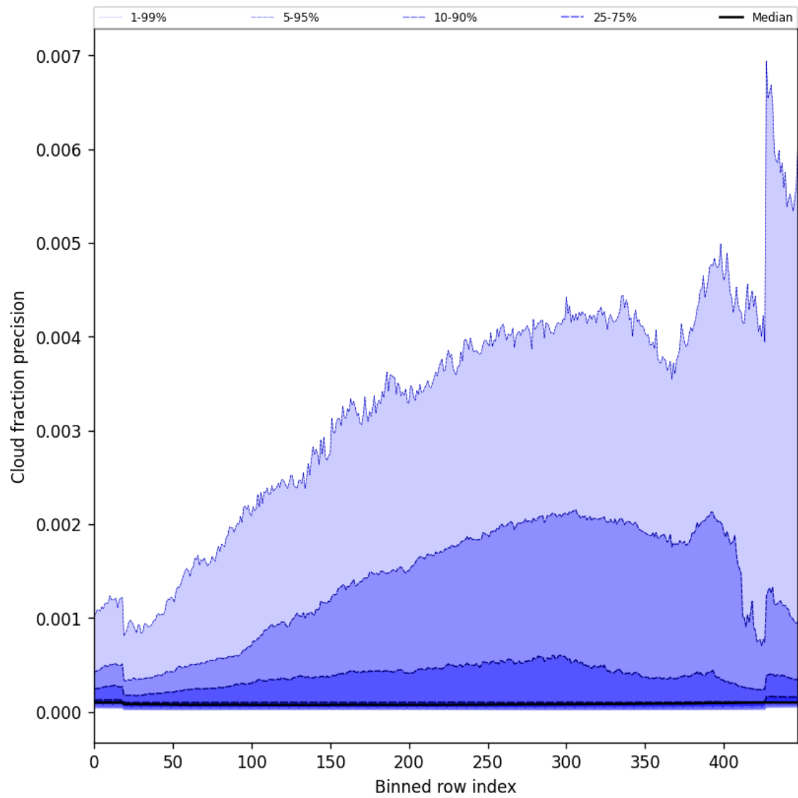
Figure 48: Along track statistics of “Cloud fraction precision” for 2025-05-16 to 2025-05-17
