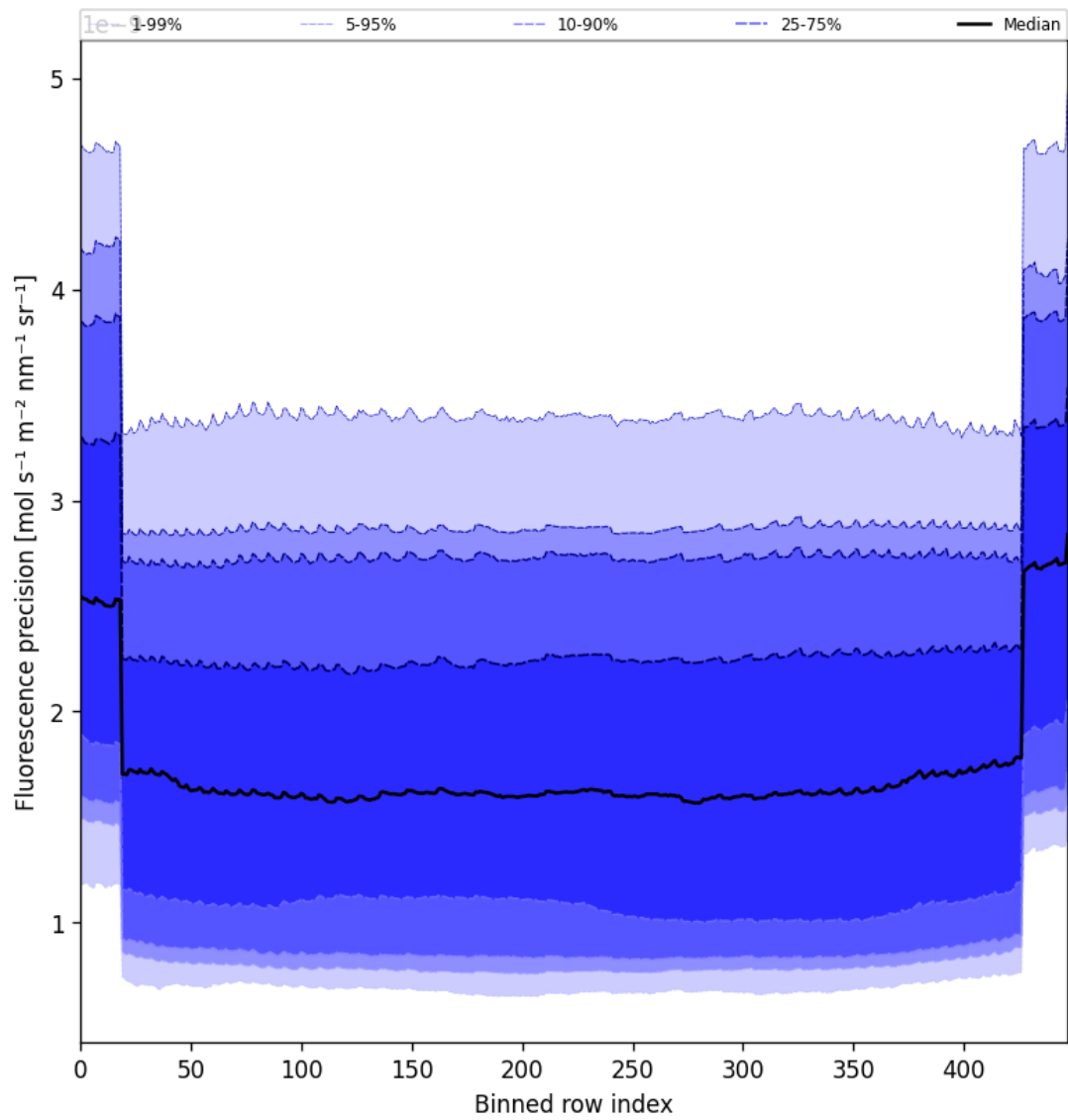
Figure 56: Along track statistics of “Fluorescence precision” for 2025-05-16 to 2025-05-17
