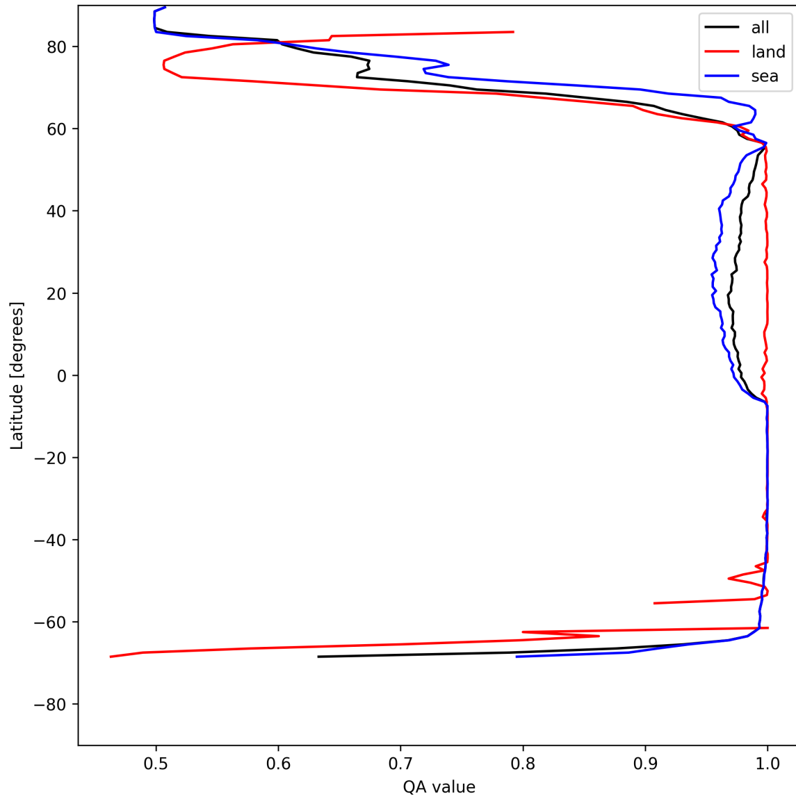
Figure 10: Zonal average of “QA value” for 2025-05-16 to 2025-05-17.
