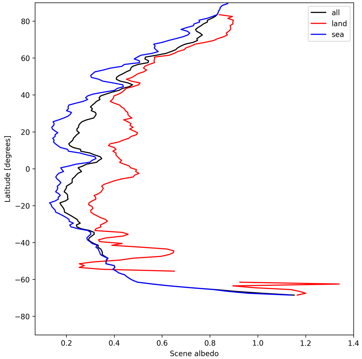
Figure 15: Zonal average of “Scene albedo” for 2025-05-16 to 2025-05-17.
