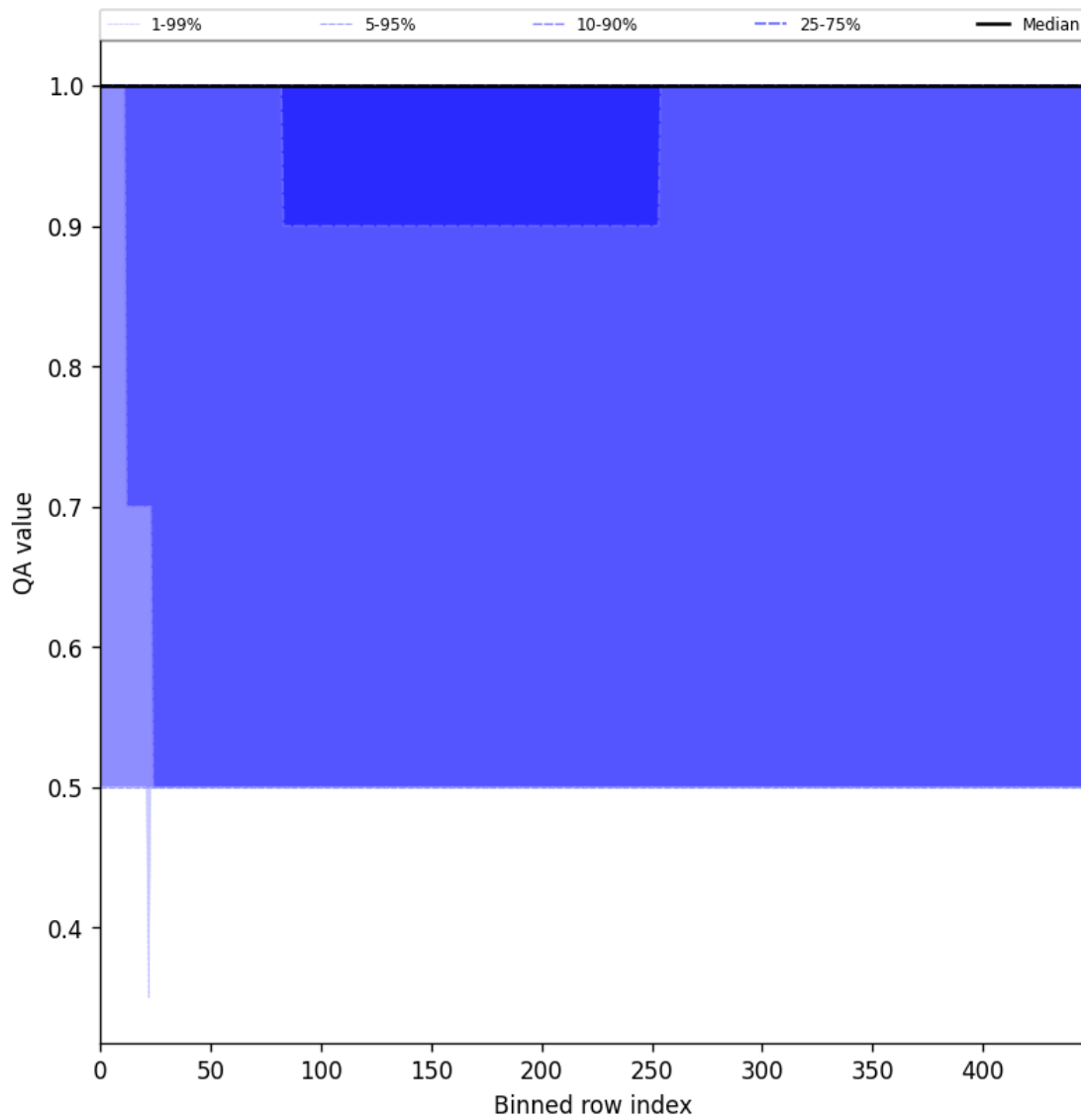
Figure 44: Along track statistics of “QA value” for 2025-05-16 to 2025-05-17
