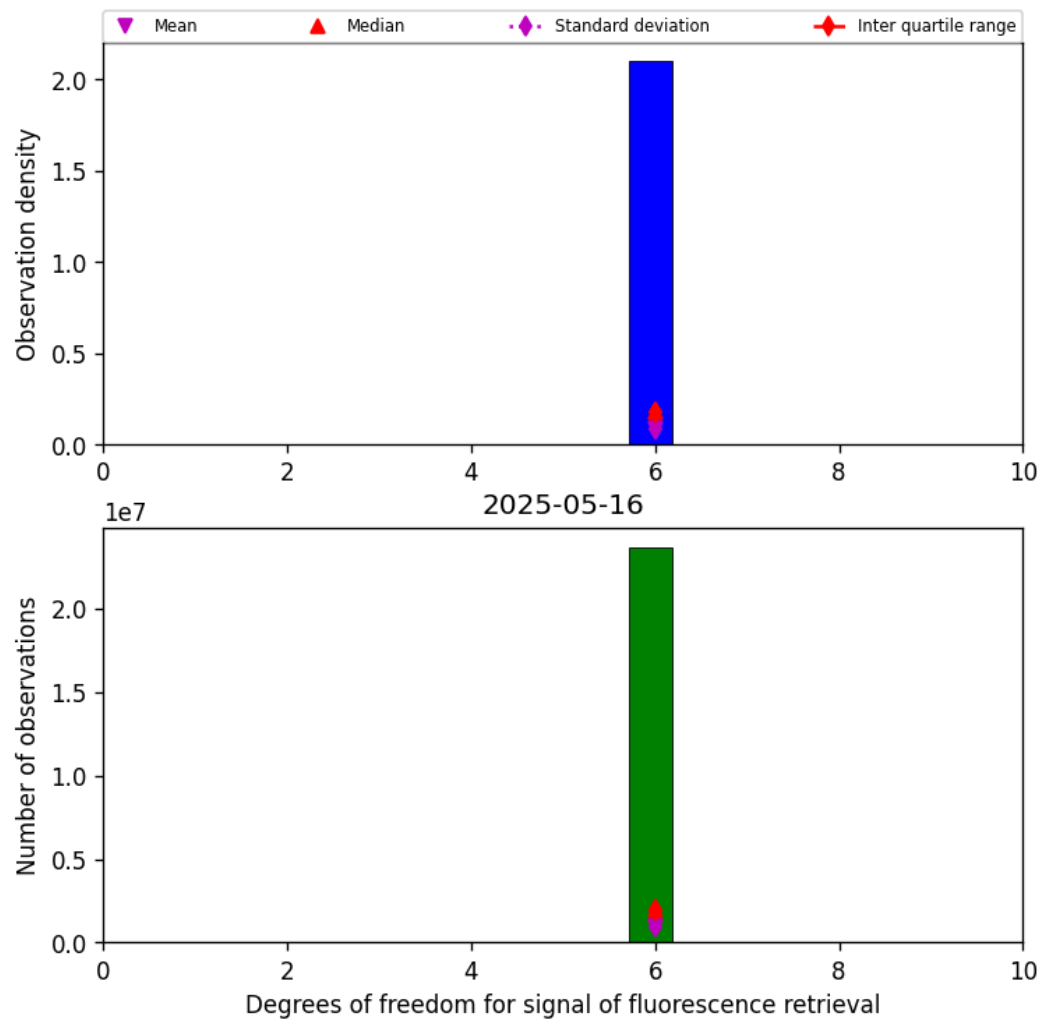
Figure 41: Histogram of “Degrees of freedom for signal of fluorescence retrieval” for 2025-05-16 to 2025-05-17
