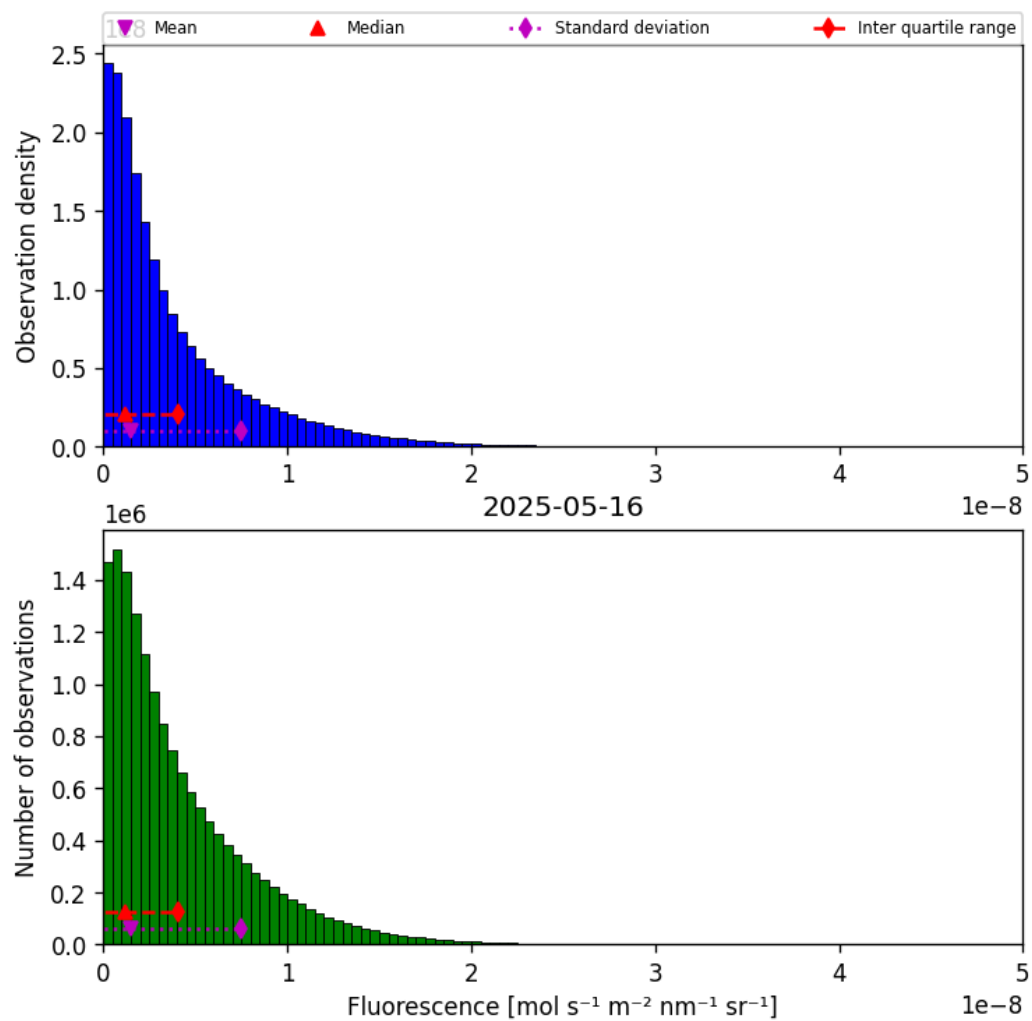
Figure 38: Histogram of “Fluorescence” for 2025-05-16 to 2025-05-17
