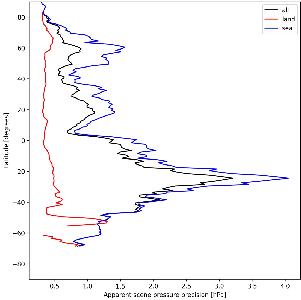
Figure 18: Zonal average of “Apparent scene pressure precision” for 2025-05-16 to 2025-05-17.
