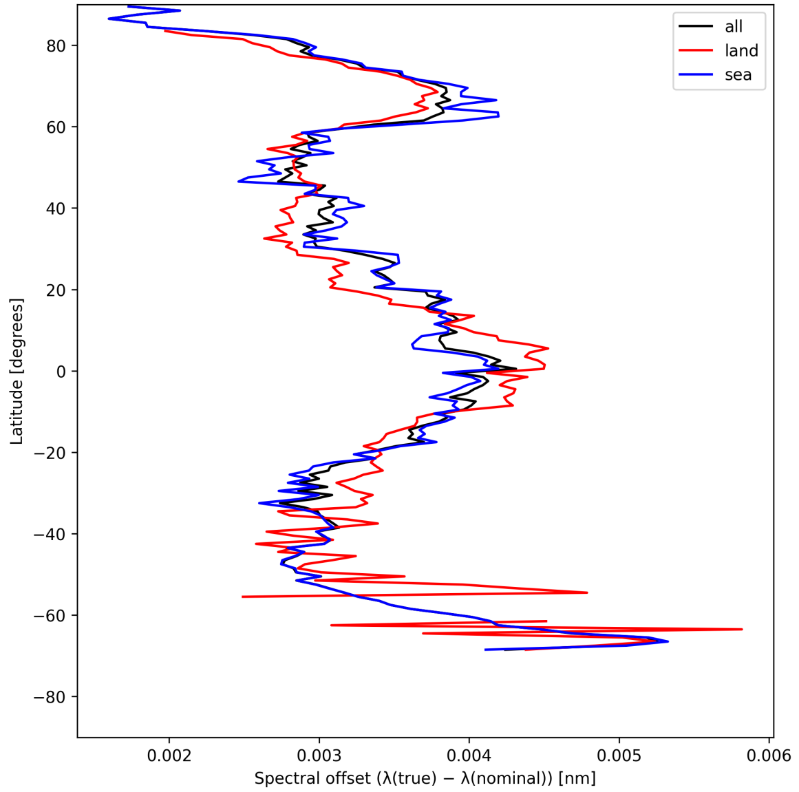
Figure 26: Zonal average of “Spectral offset ( \lambda_{\text{true}} - \lambda_{\text{nominal}} )” for 2025-05-16 to 2025-05-17.
