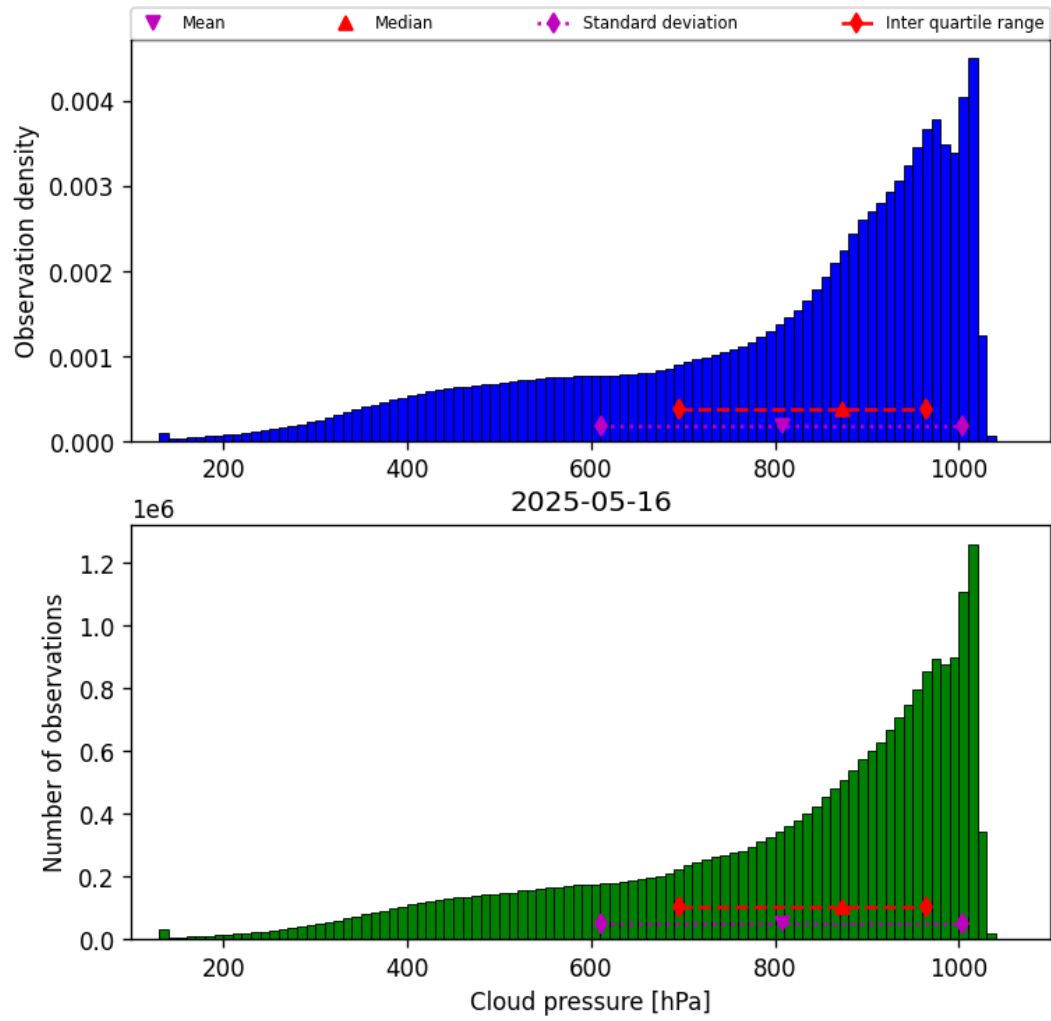
Figure 28: Histogram of “Cloud pressure” for 2025-05-16 to 2025-05-17
