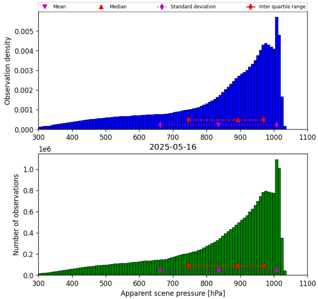
Figure 34: Histogram of “Apparent scene pressure” for 2025-05-16 to 2025-05-17
