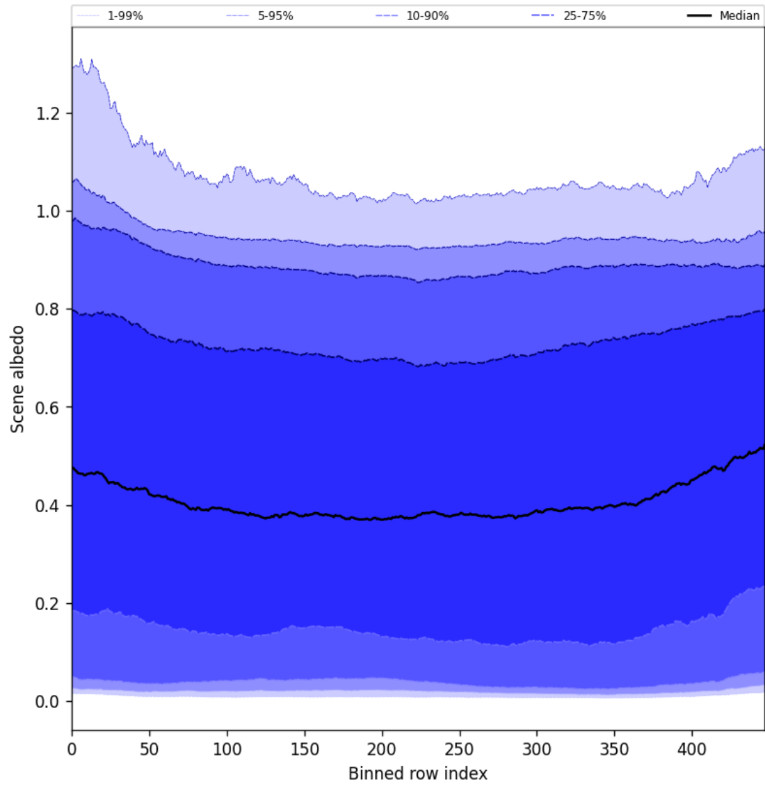
Figure 49: Along track statistics of “Scene albedo” for 2025-05-16 to 2025-05-17
