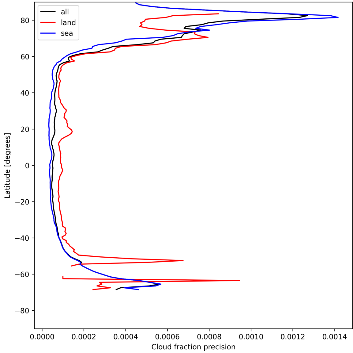
Figure 14: Zonal average of “Cloud fraction precision” for 2025-05-16 to 2025-05-17.
