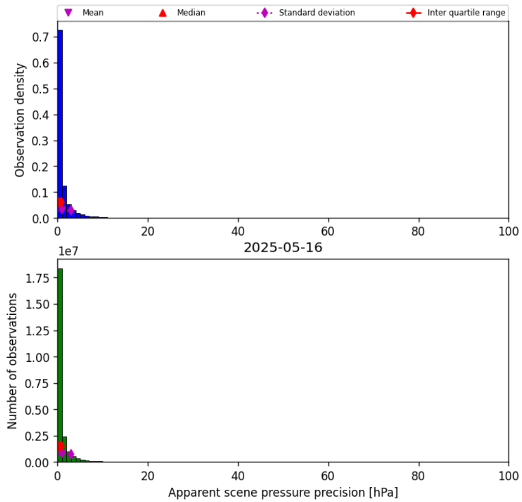
Figure 35: Histogram of “Apparent scene pressure precision” for 2025-05-16 to 2025-05-17
