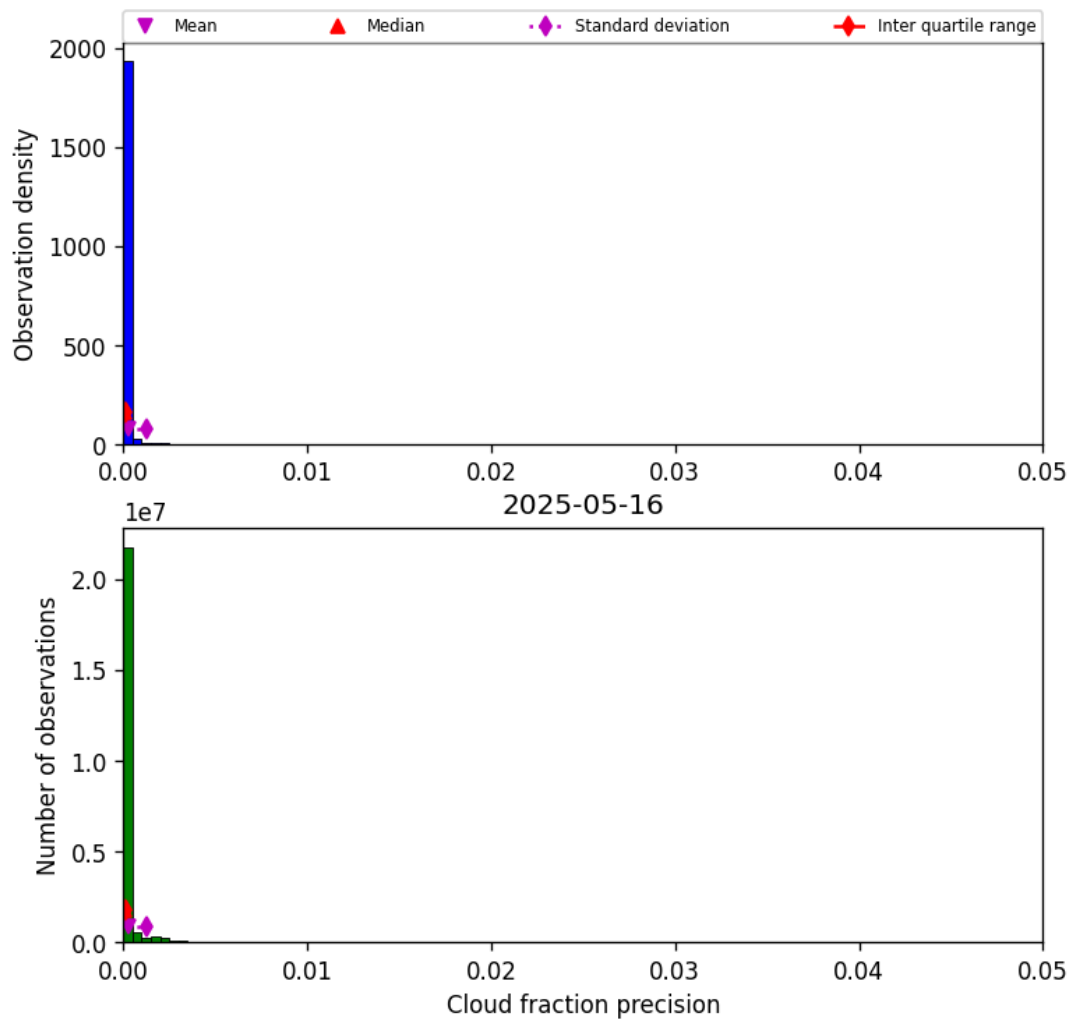
Figure 31: Histogram of “Cloud fraction precision” for 2025-05-16 to 2025-05-17
