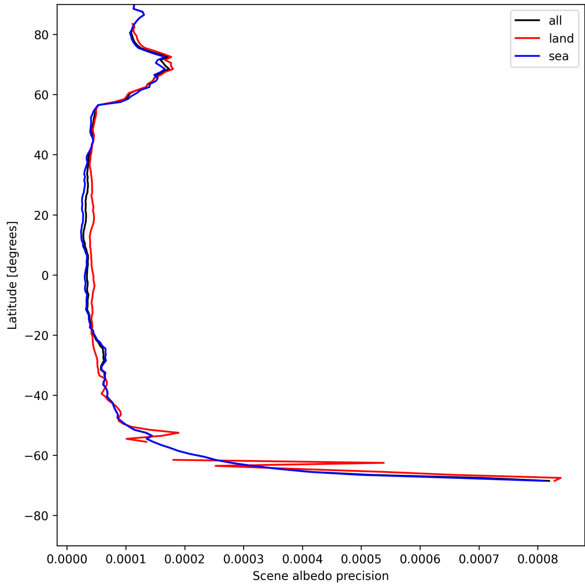
Figure 16: Zonal average of “Scene albedo precision” for 2025-05-16 to 2025-05-17.
