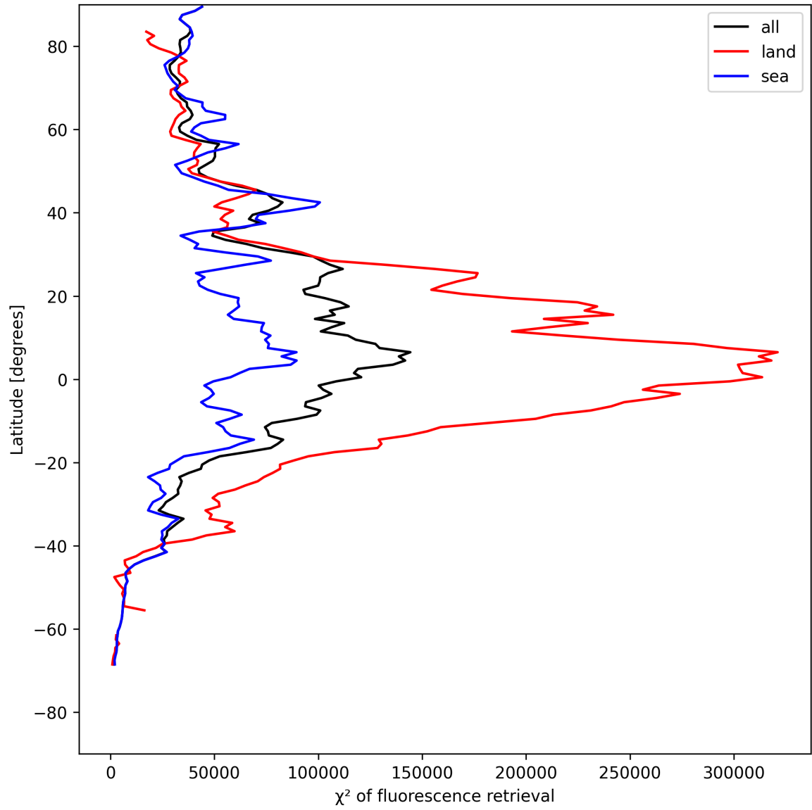
Figure 23: Zonal average of “ \chi^2 of fluorescence retrieval” for 2025-05-16 to 2025-05-17.
