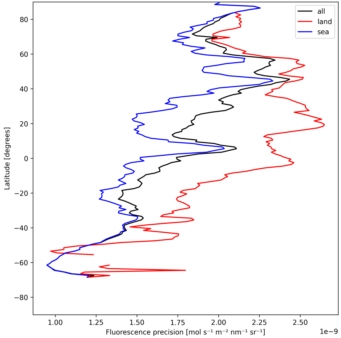
Figure 22: Zonal average of “Fluorescence precision” for 2025-05-16 to 2025-05-17.
