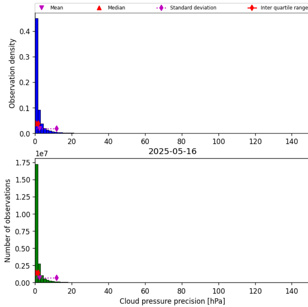
Figure 29: Histogram of “Cloud pressure precision” for 2025-05-16 to 2025-05-17
