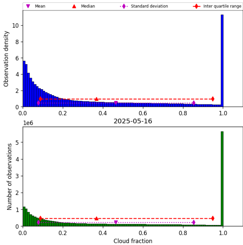
Figure 30: Histogram of “Cloud fraction” for 2025-05-16 to 2025-05-17
