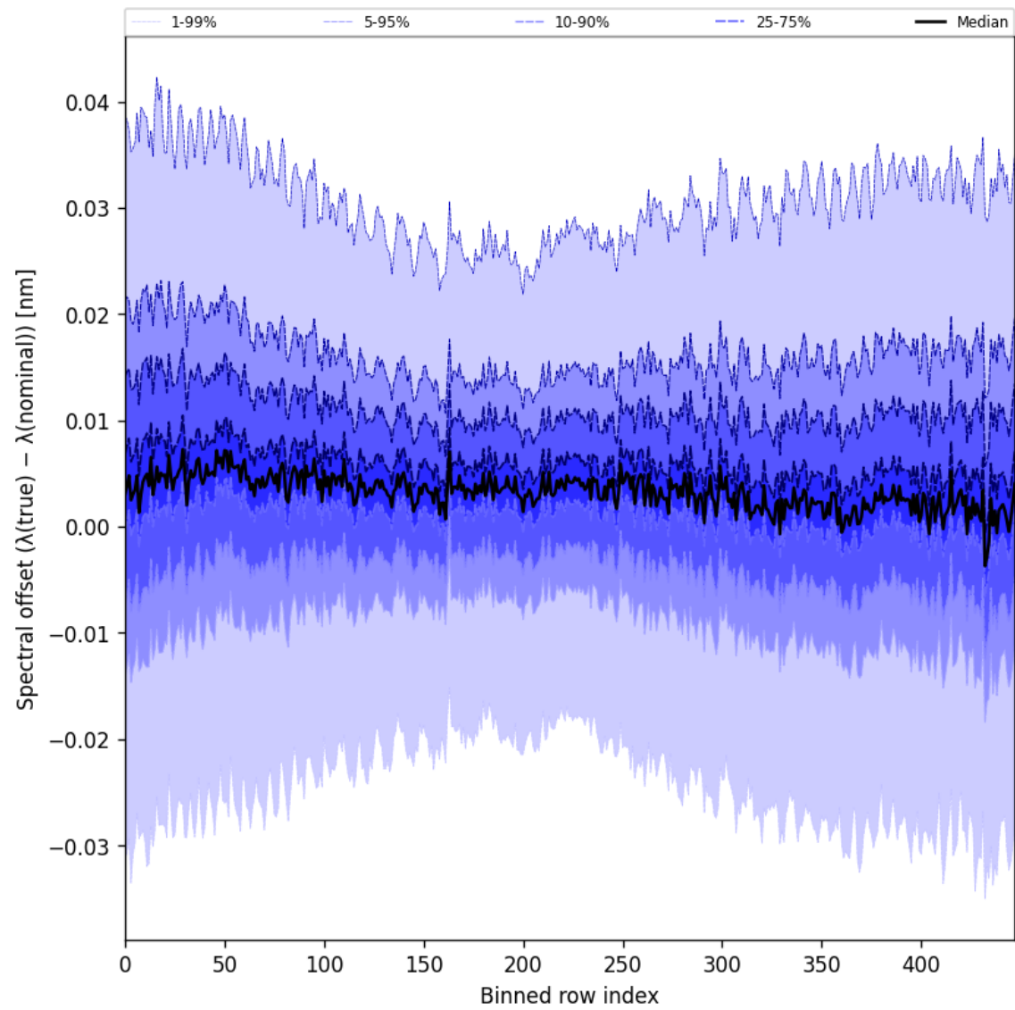
Figure 60: Along track statistics of “Spectral offset ( \lambda_{\text{true}} - \lambda_{\text{nominal}} )” for 2025-05-16 to 2025-05-17
