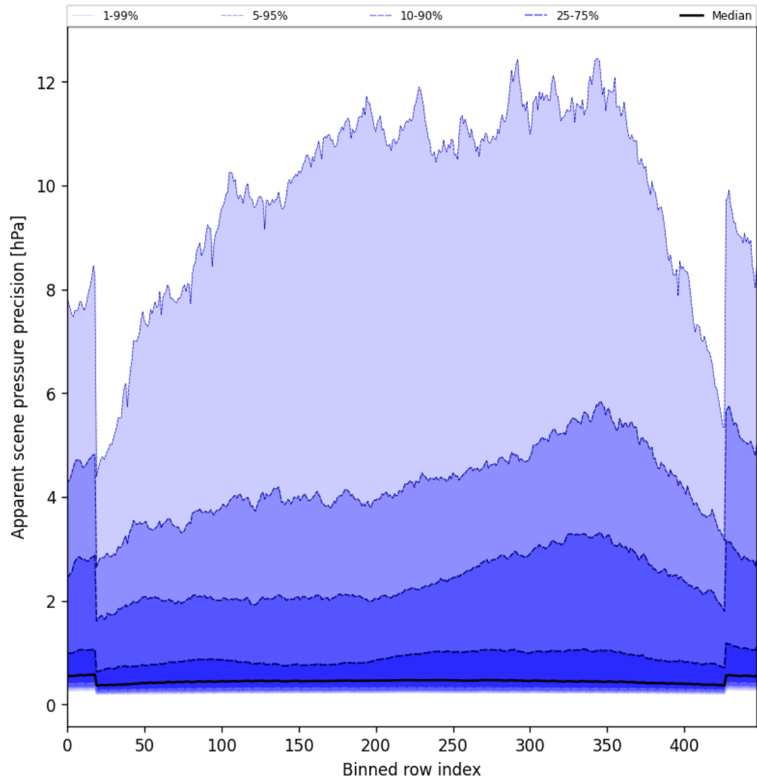
Figure 52: Along track statistics of “Apparent scene pressure precision” for 2025-05-16 to 2025-05-17
