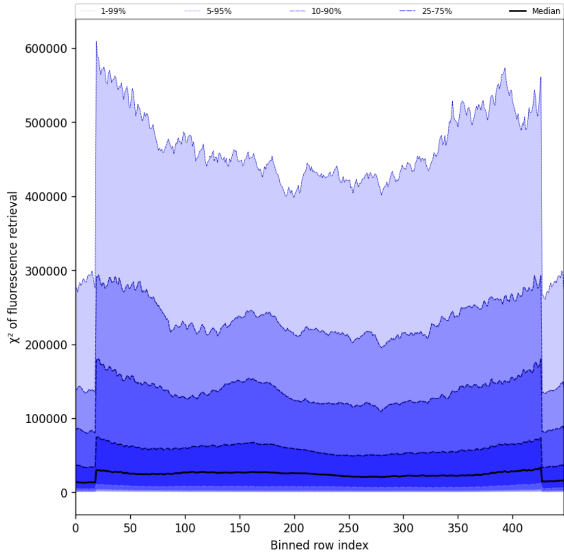
Figure 57: Along track statistics of “ \chi^2 of fluorescence retrieval” for 2025-05-16 to 2025-05-17
