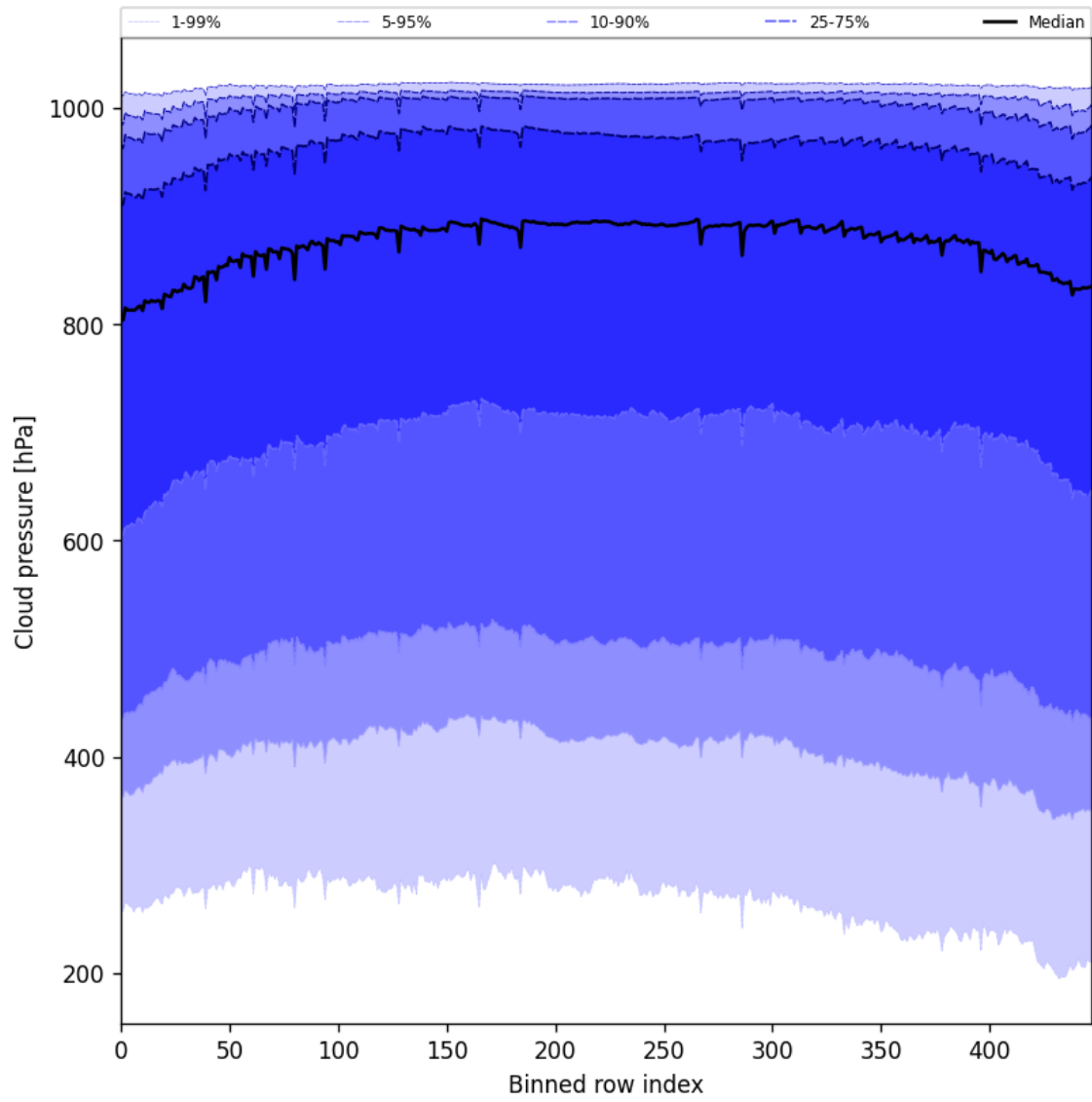
Figure 45: Along track statistics of “Cloud pressure” for 2025-05-16 to 2025-05-17
