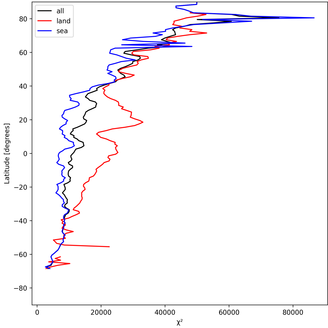
Figure 19: Zonal average of “ \chi^2 ” for 2025-05-16 to 2025-05-17.
