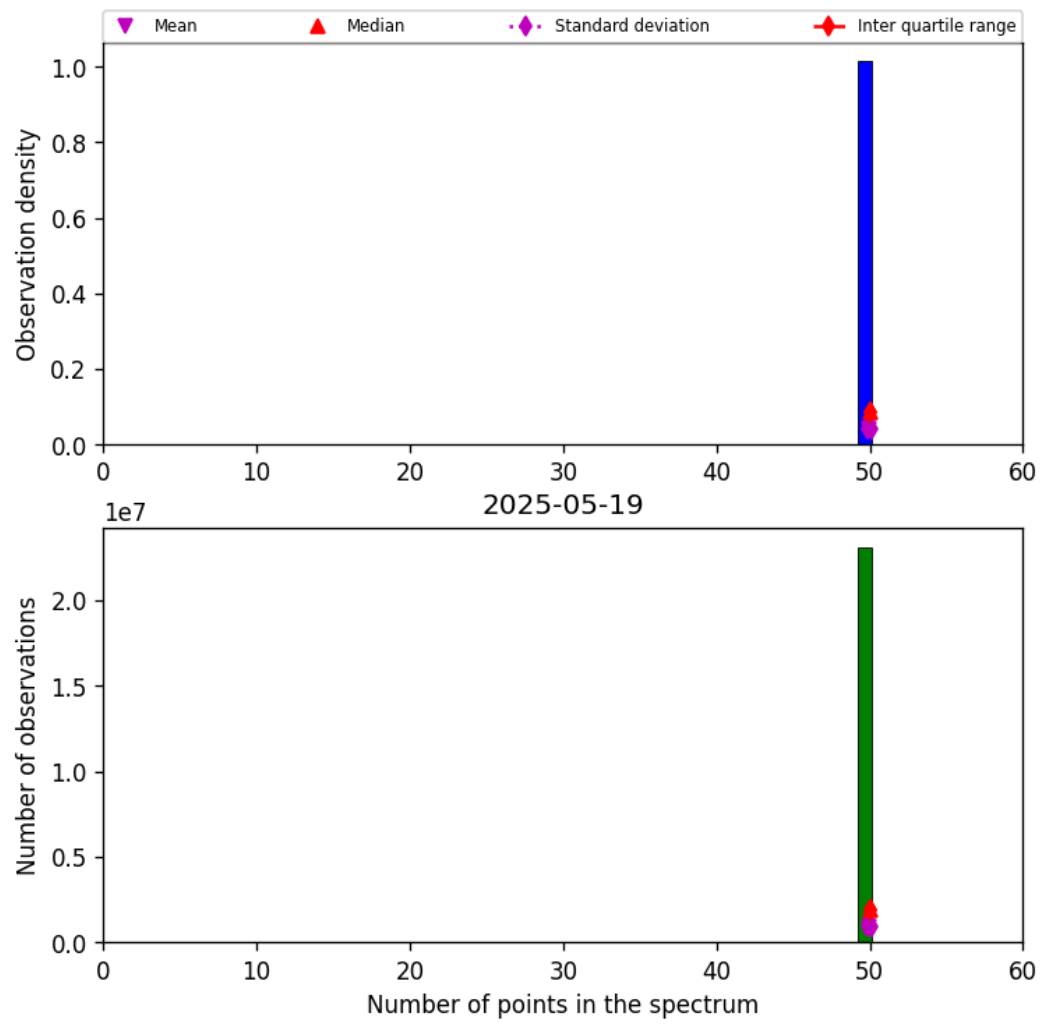
Figure 42: Histogram of "Number of points in the spectrum" for 2025-05-19 to 2025-05-19
