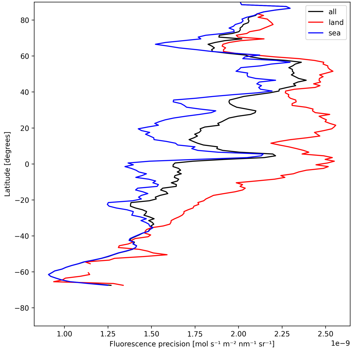
Figure 22: Zonal average of “Fluorescence precision” for 2025-05-19 to 2025-05-19.
