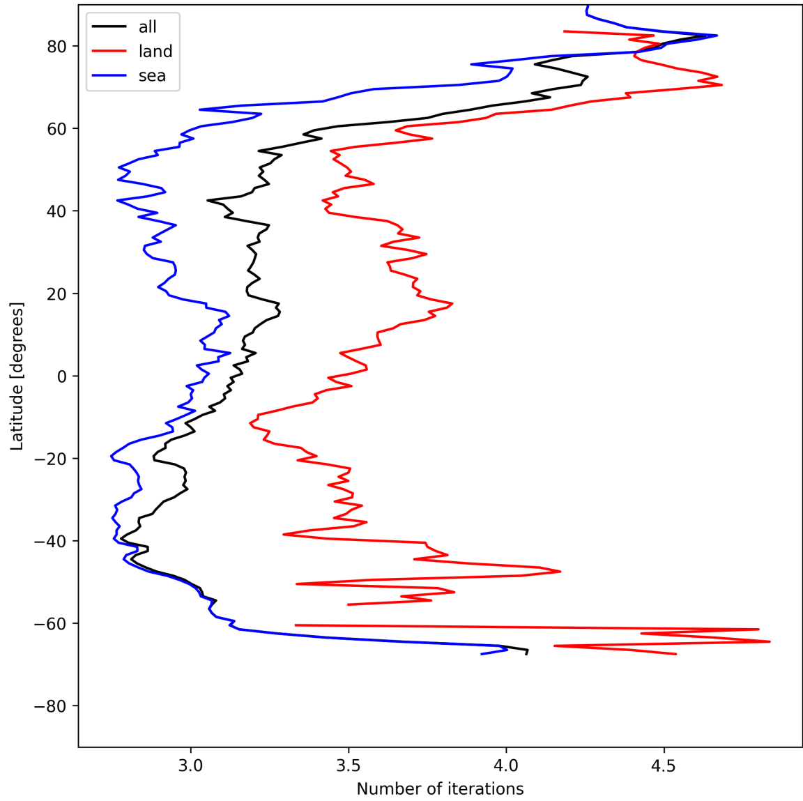
Figure 20: Zonal average of “Number of iterations” for 2025-05-19 to 2025-05-19.
