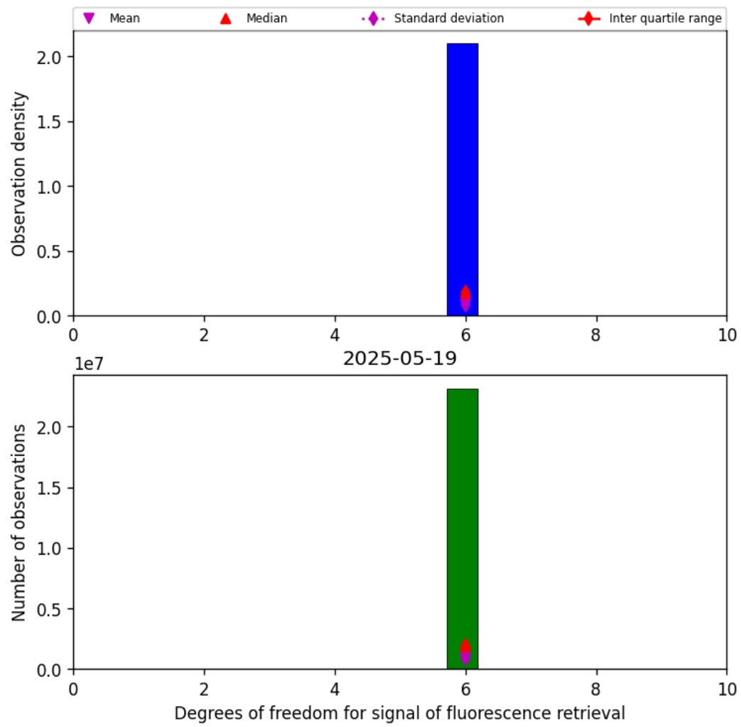
Figure 41: Histogram of “Degrees of freedom for signal of fluorescence retrieval” for 2025-05-19 to 2025-05-19
