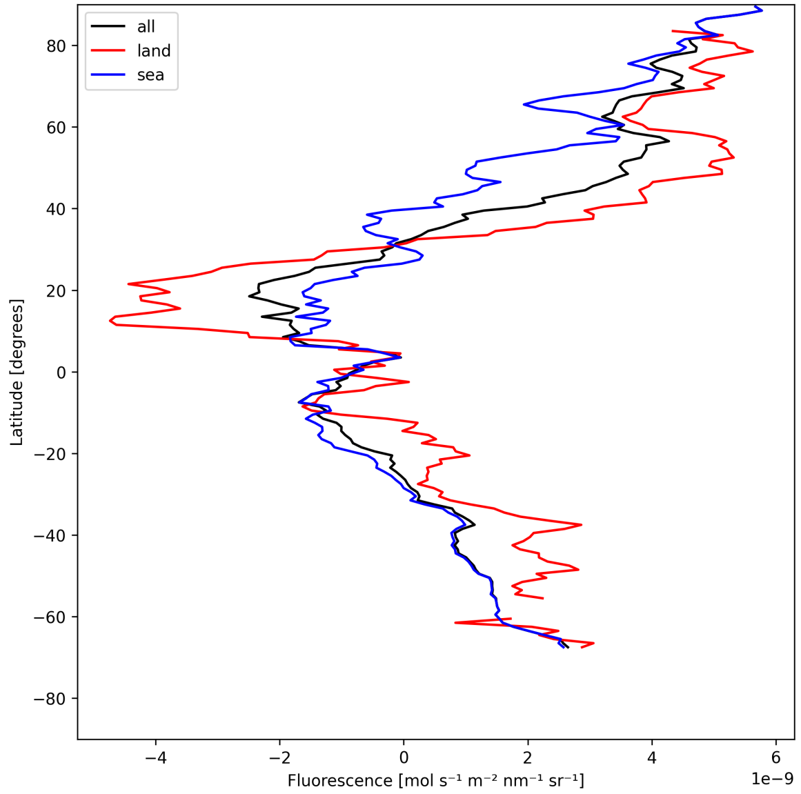
Figure 21: Zonal average of “Fluorescence” for 2025-05-19 to 2025-05-19.
