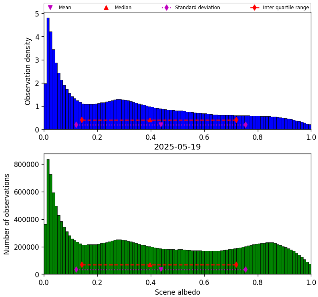
Figure 32: Histogram of “Scene albedo” for 2025-05-19 to 2025-05-19
