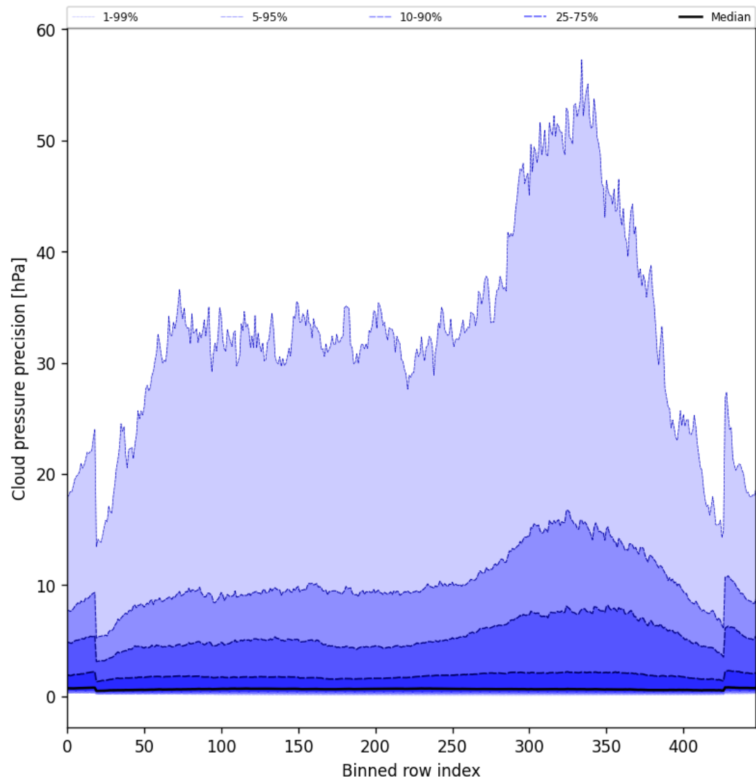
Figure 46: Along track statistics of “Cloud pressure precision” for 2025-05-19 to 2025-05-19
