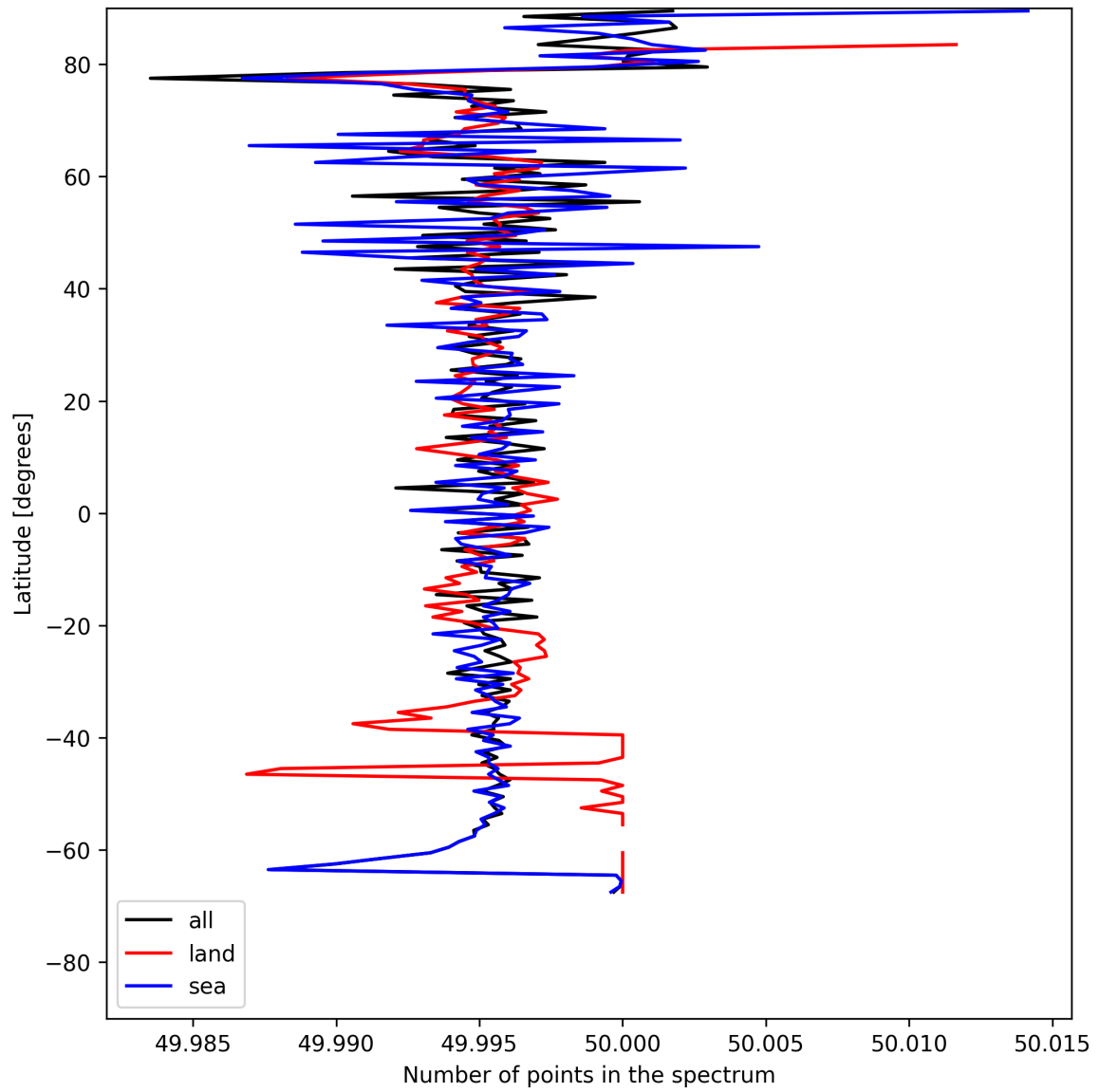
Figure 25: Zonal average of “Number of points in the spectrum” for 2025-05-19 to 2025-05-19.
