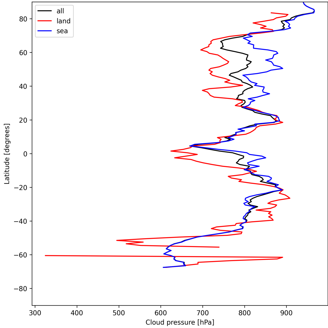
Figure 11: Zonal average of “Cloud pressure” for 2025-05-19 to 2025-05-19.
