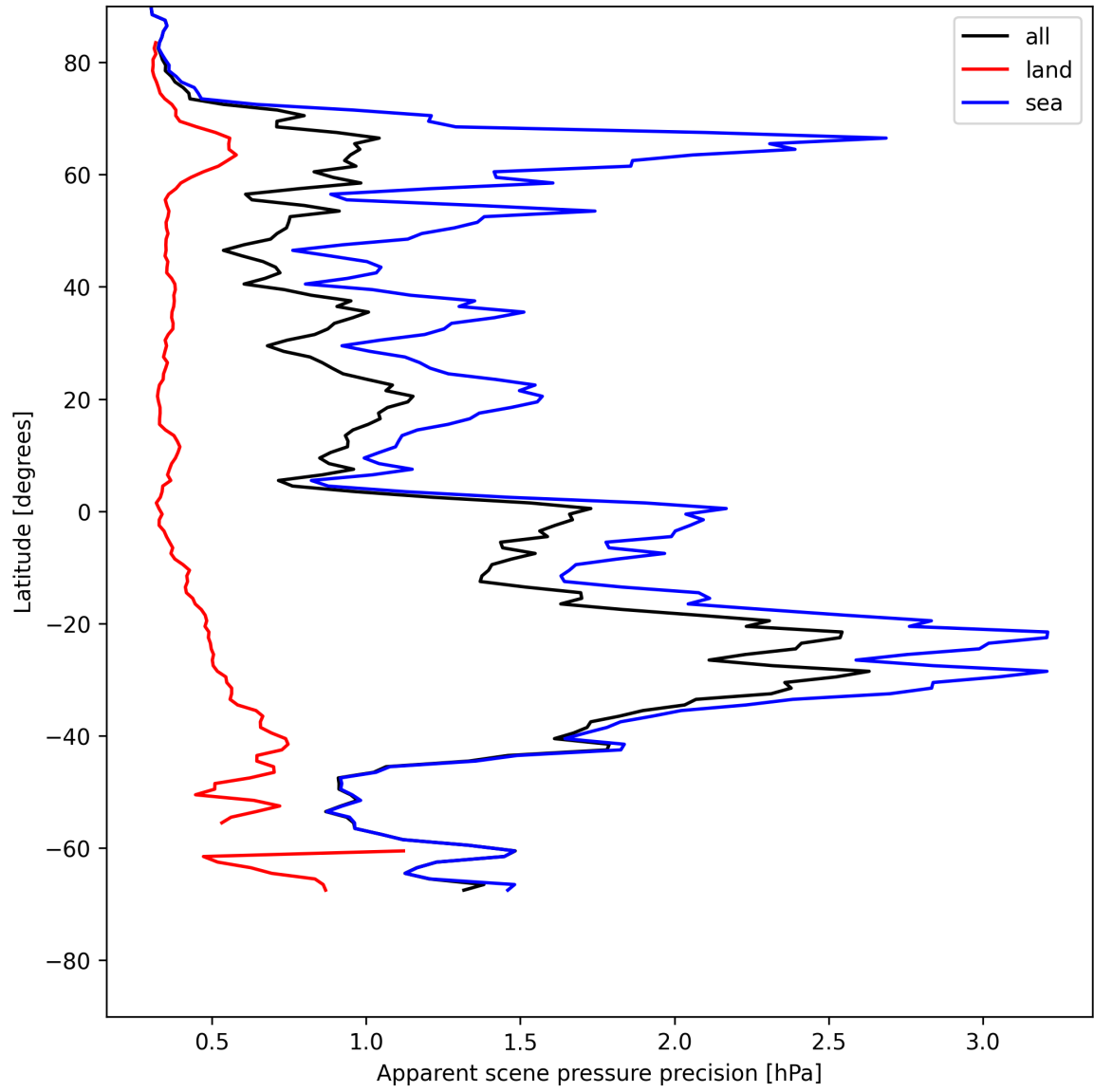
Figure 18: Zonal average of “Apparent scene pressure precision” for 2025-05-19 to 2025-05-19.
