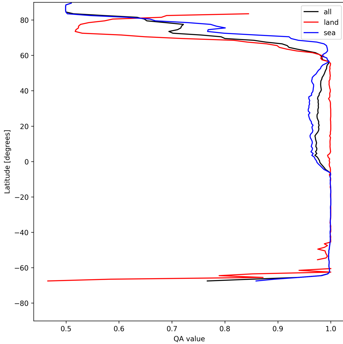
Figure 10: Zonal average of “QA value” for 2025-05-19 to 2025-05-19.
