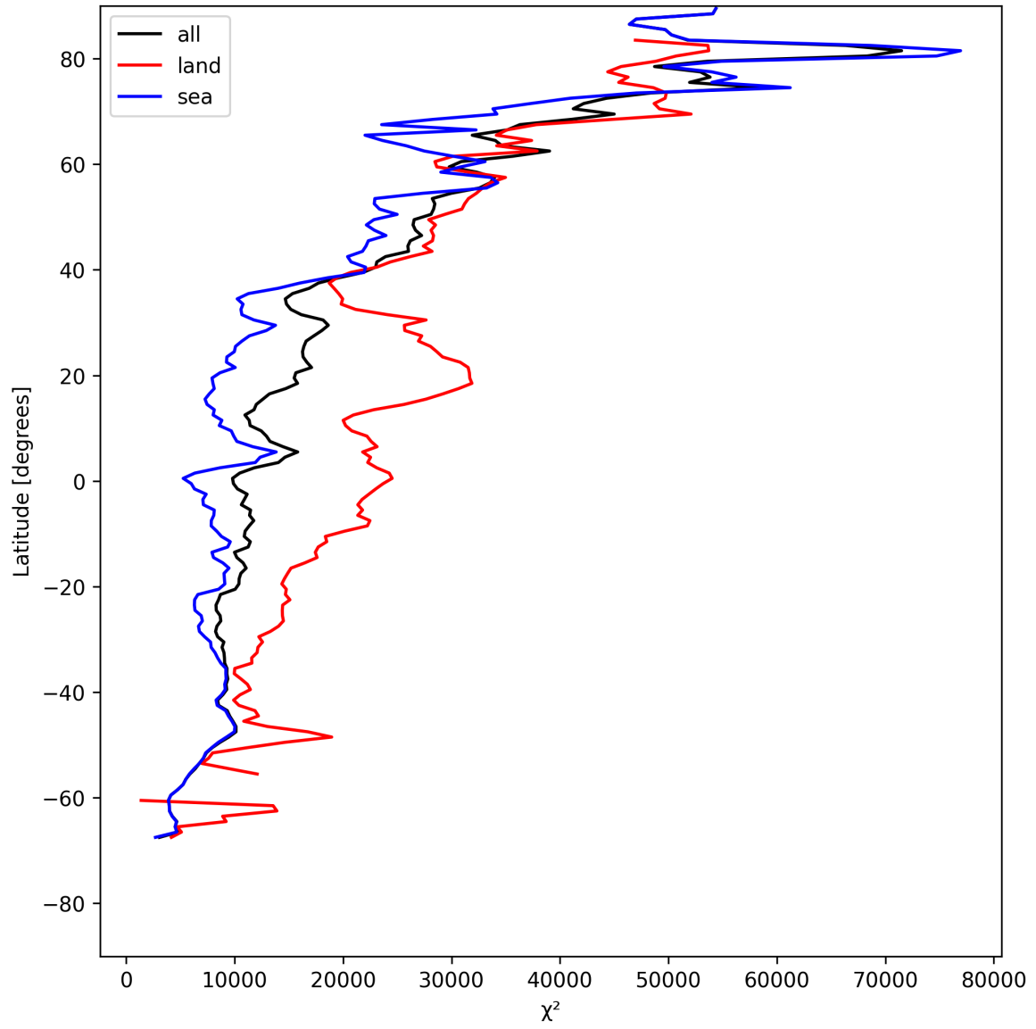
Figure 19: Zonal average of “ \chi^2 ” for 2025-05-19 to 2025-05-19.
