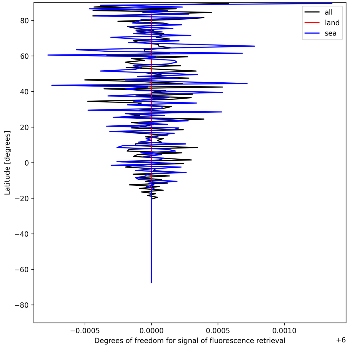
Figure 24: Zonal average of “Degrees of freedom for signal of fluorescence retrieval” for 2025-05-19 to 2025-05-19.
