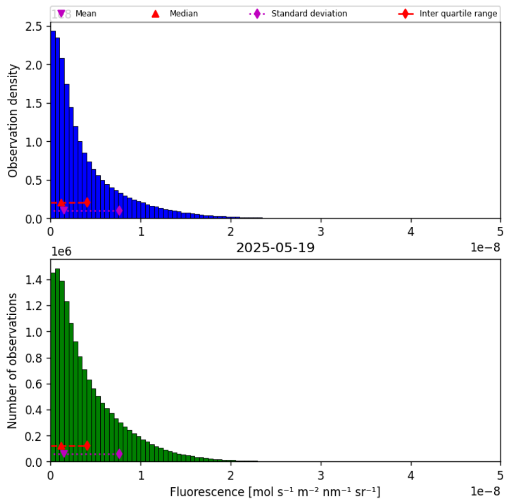
Figure 38: Histogram of “Fluorescence” for 2025-05-19 to 2025-05-19
