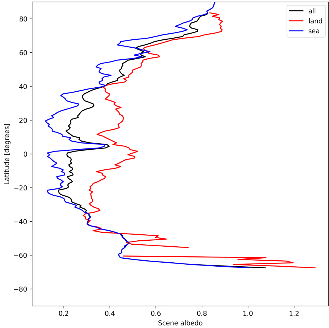
Figure 15: Zonal average of “Scene albedo” for 2025-05-19 to 2025-05-19.
