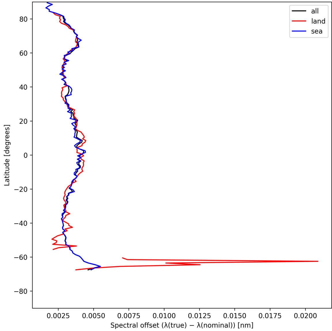
Figure 26: Zonal average of “Spectral offset ( \lambda_{\text{true}} - \lambda_{\text{nominal}} )” for 2025-05-19 to 2025-05-19.
