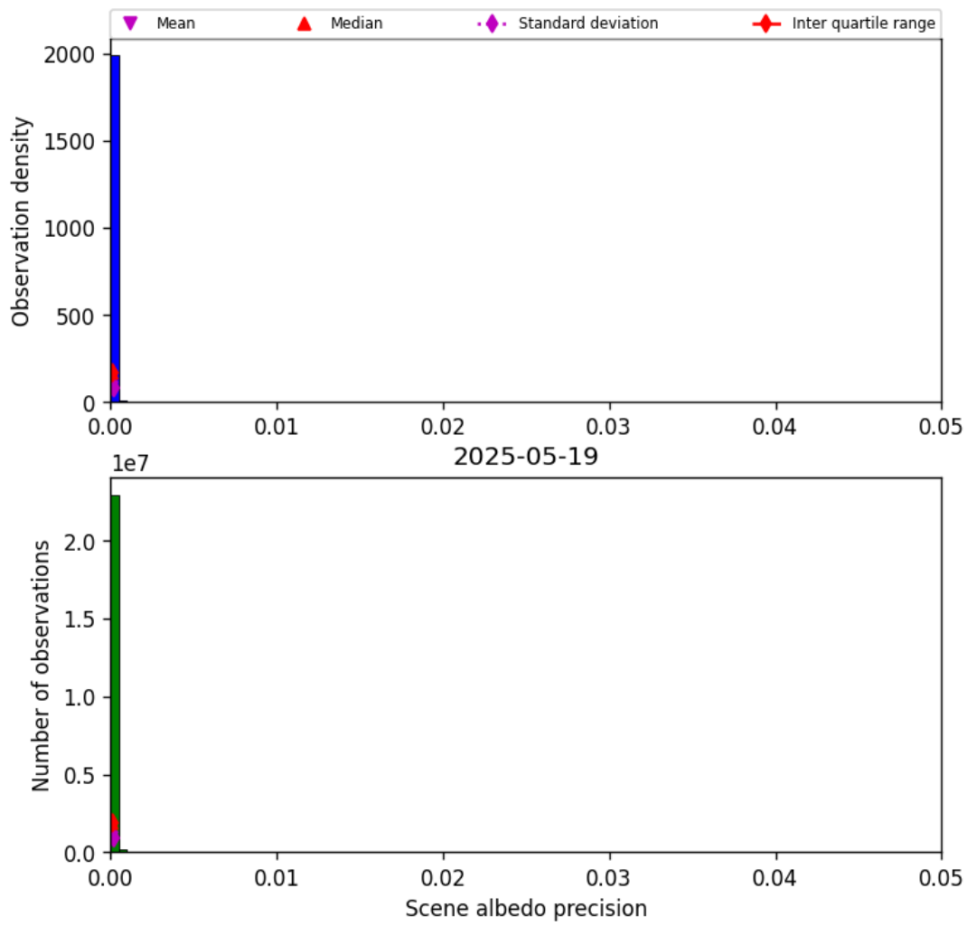
Figure 33: Histogram of “Scene albedo precision” for 2025-05-19 to 2025-05-19
