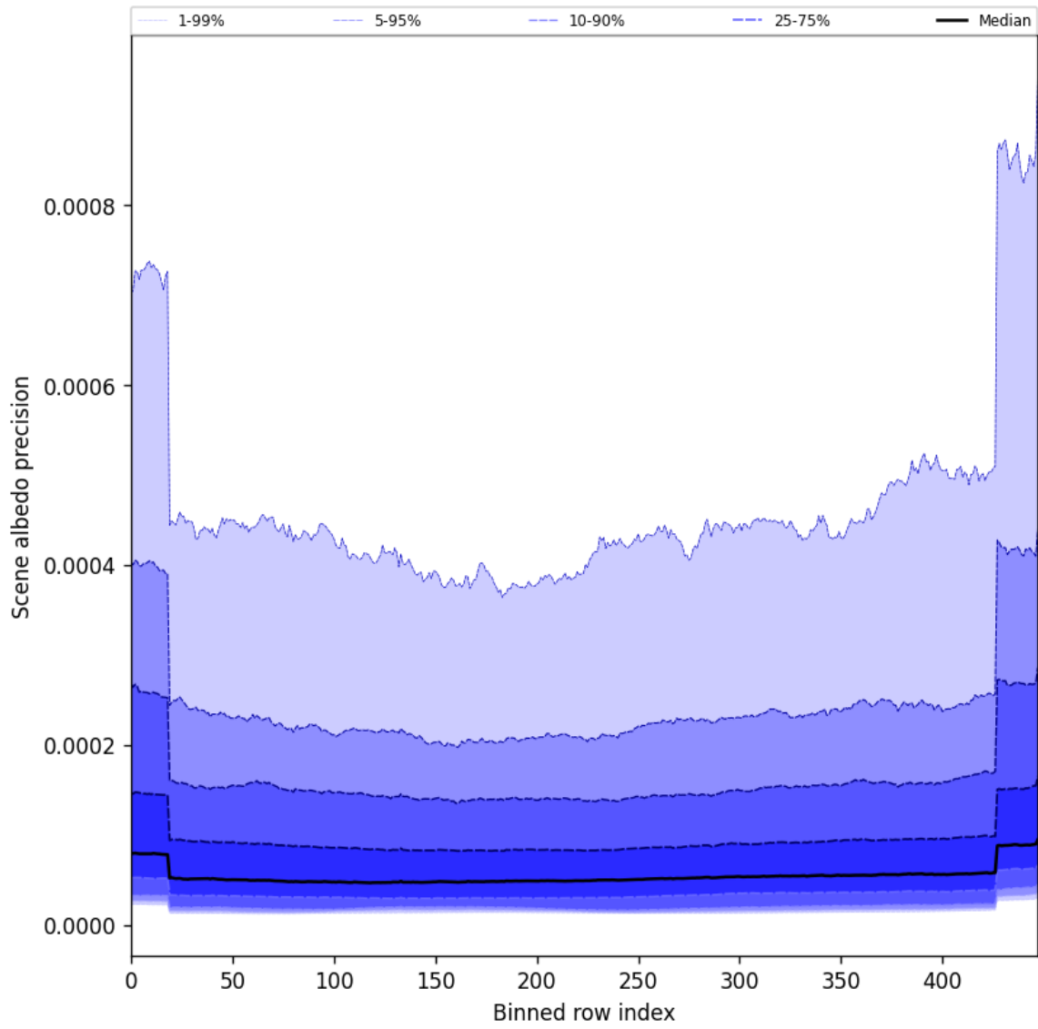
Figure 50: Along track statistics of “Scene albedo precision” for 2025-05-19 to 2025-05-19
