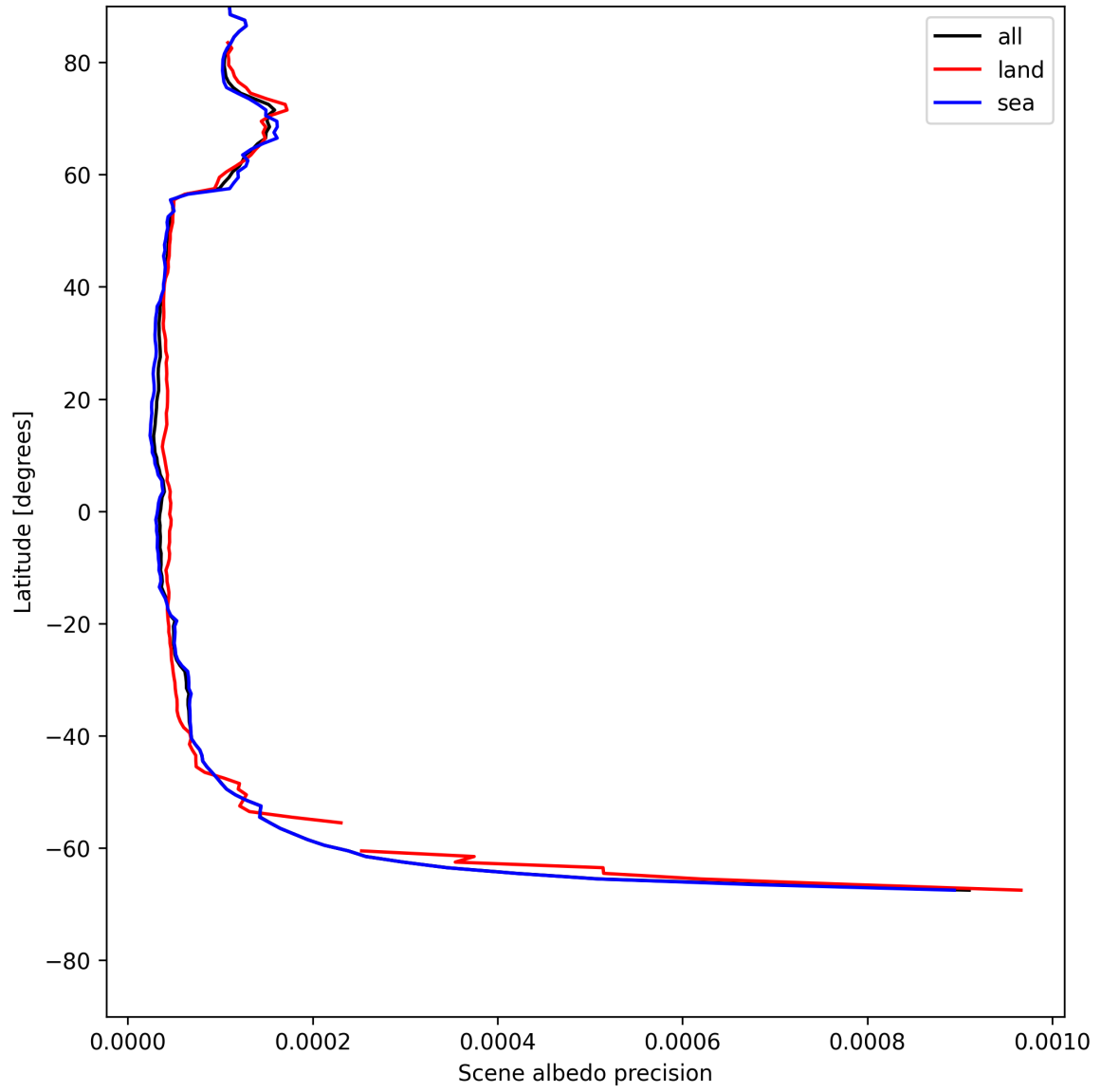
Figure 16: Zonal average of “Scene albedo precision” for 2025-05-19 to 2025-05-19.
