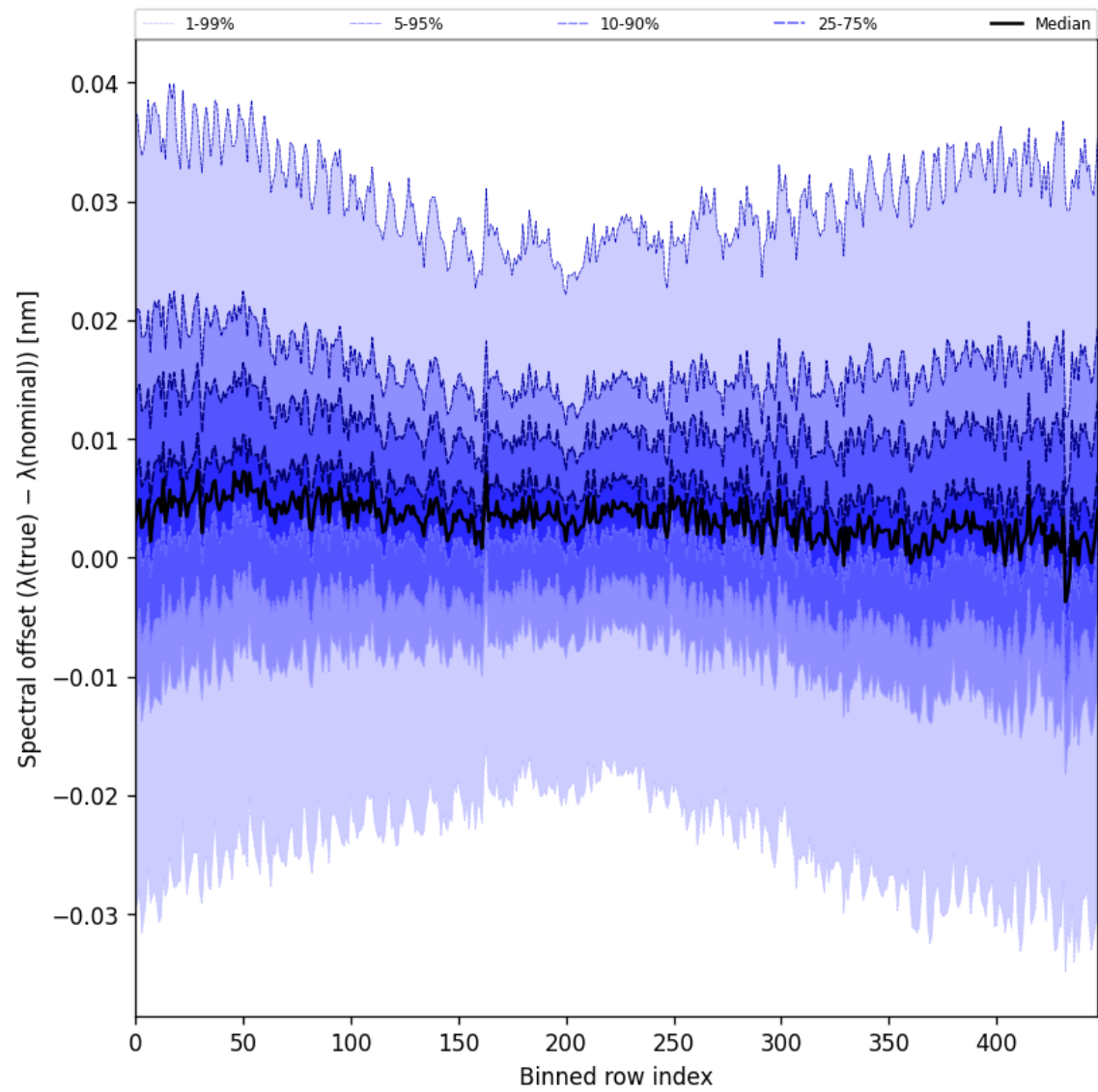
Figure 60: Along track statistics of “Spectral offset ( \lambda_{\text{true}} - \lambda_{\text{nominal}} )” for 2025-05-19 to 2025-05-19
