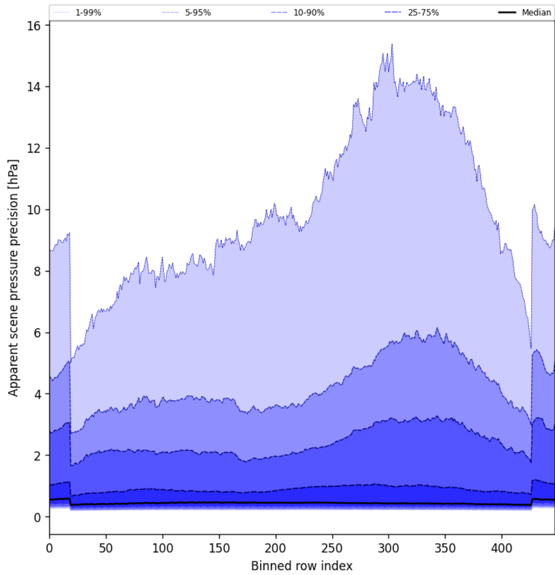
Figure 52: Along track statistics of “Apparent scene pressure precision” for 2025-05-19 to 2025-05-19
