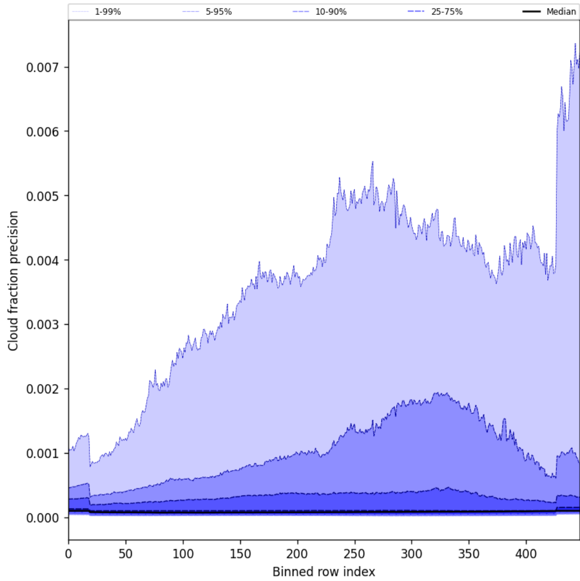
Figure 48: Along track statistics of “Cloud fraction precision” for 2025-05-19 to 2025-05-19
