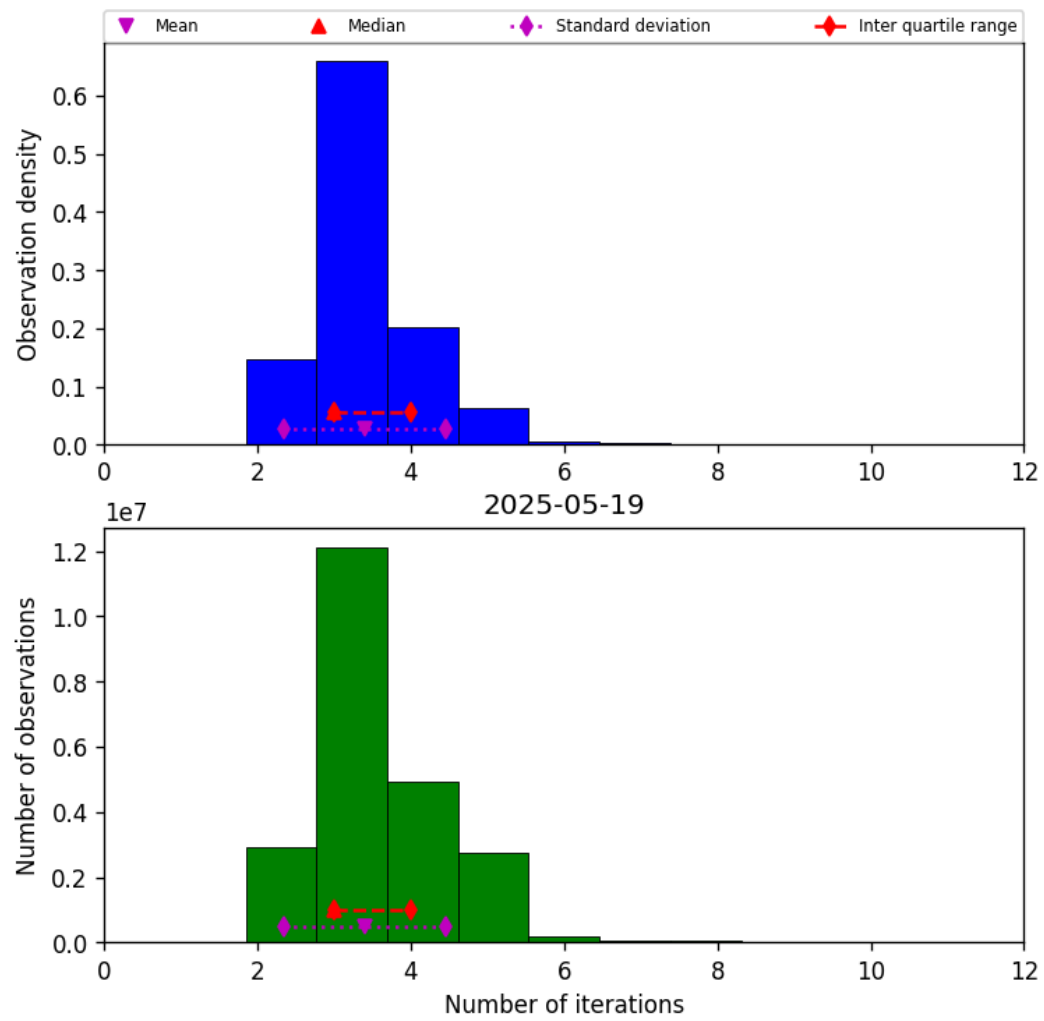
Figure 37: Histogram of “Number of iterations” for 2025-05-19 to 2025-05-19
