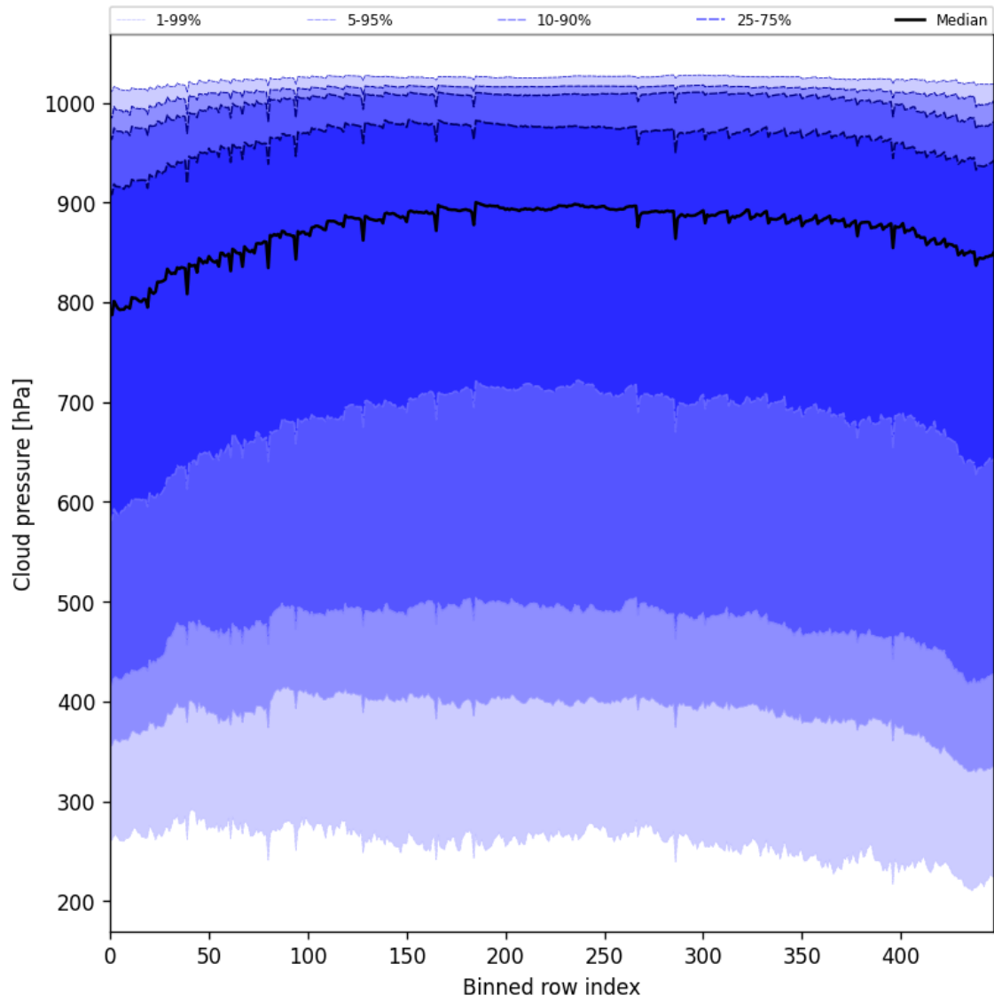
Figure 45: Along track statistics of “Cloud pressure” for 2025-05-19 to 2025-05-19
