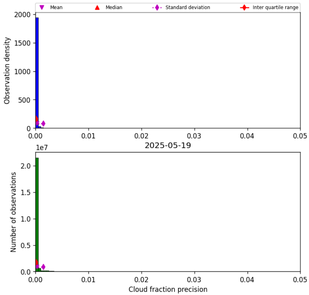
Figure 31: Histogram of “Cloud fraction precision” for 2025-05-19 to 2025-05-19
