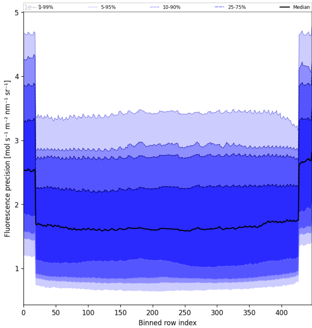
Figure 56: Along track statistics of “Fluorescence precision” for 2025-05-19 to 2025-05-19
