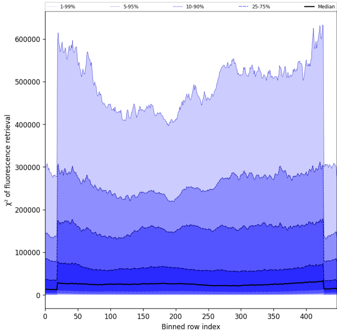
Figure 57: Along track statistics of “ \chi^2 of fluorescence retrieval” for 2025-05-19 to 2025-05-19
