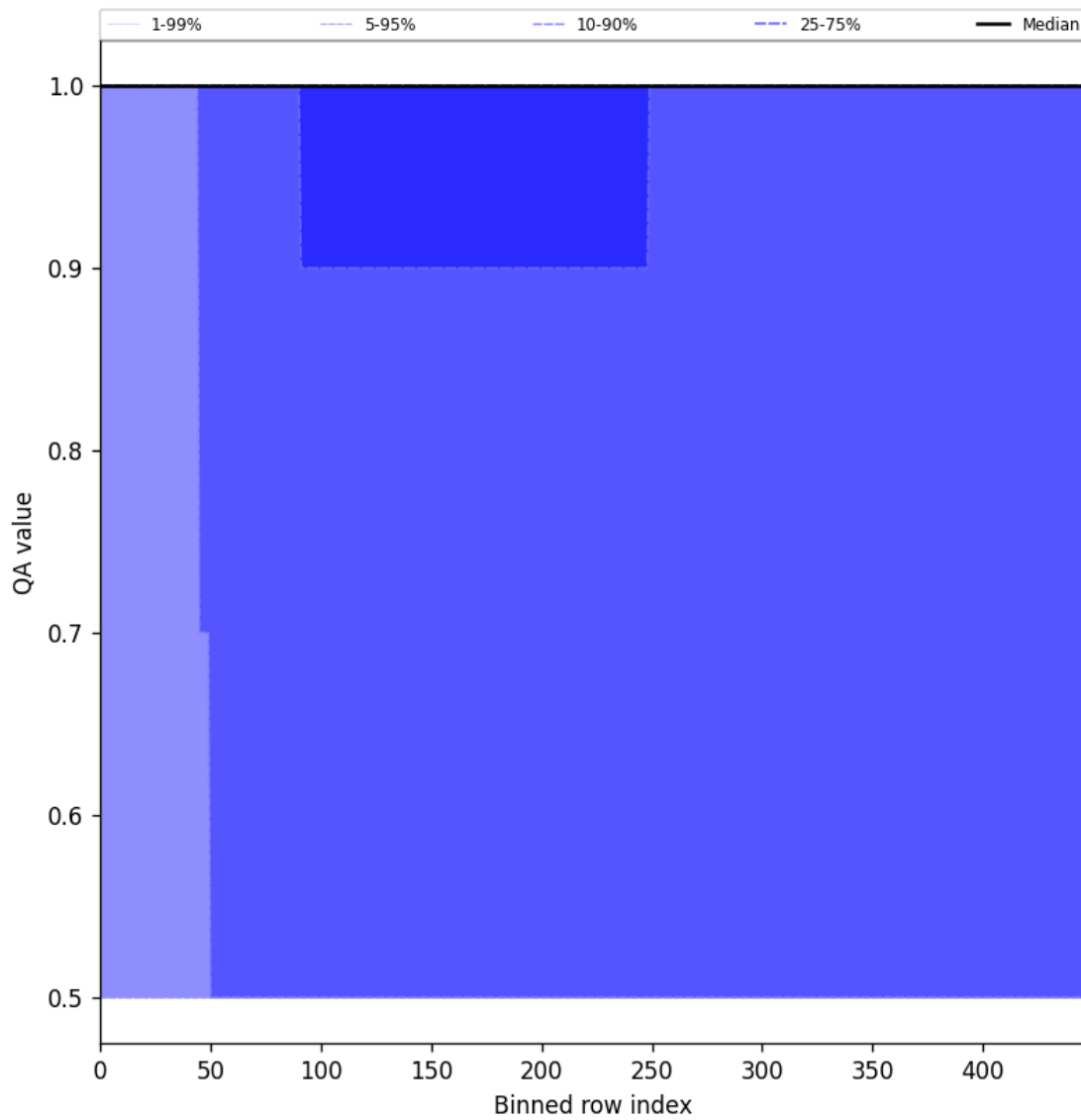
Figure 44: Along track statistics of “QA value” for 2025-05-19 to 2025-05-19
