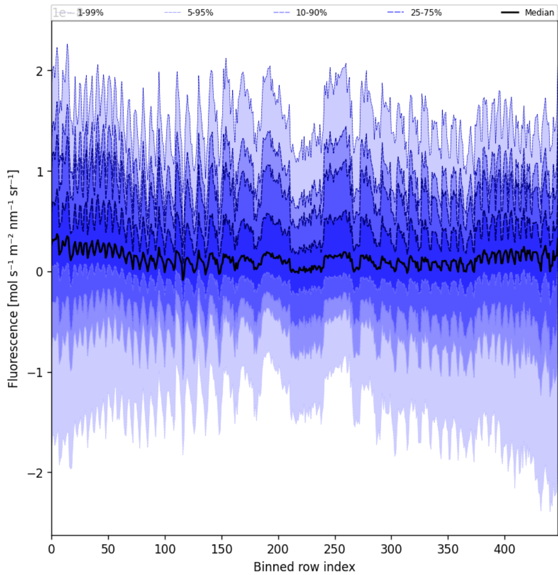
Figure 55: Along track statistics of “Fluorescence” for 2025-05-19 to 2025-05-19
