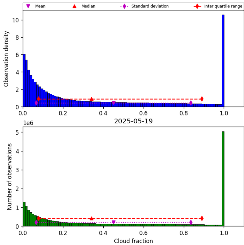
Figure 30: Histogram of “Cloud fraction” for 2025-05-19 to 2025-05-19
