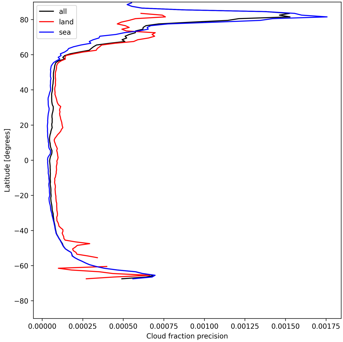
Figure 14: Zonal average of “Cloud fraction precision” for 2025-05-19 to 2025-05-19.
