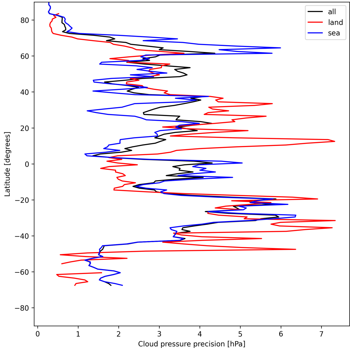
Figure 12: Zonal average of "Cloud pressure precision" for 2025-05-19 to 2025-05-19.
