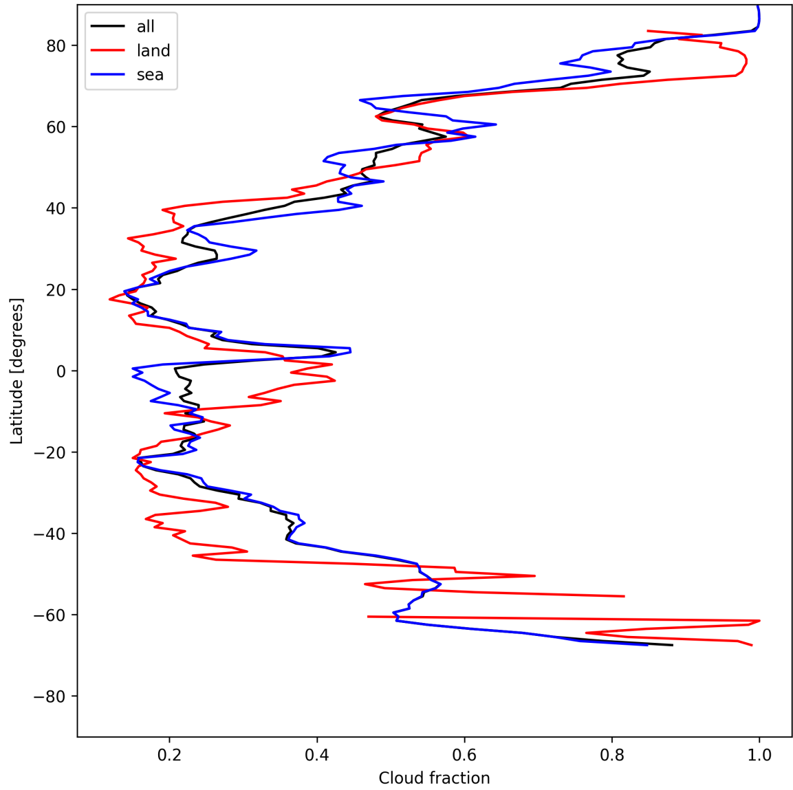
Figure 13: Zonal average of “Cloud fraction” for 2025-05-19 to 2025-05-19.
