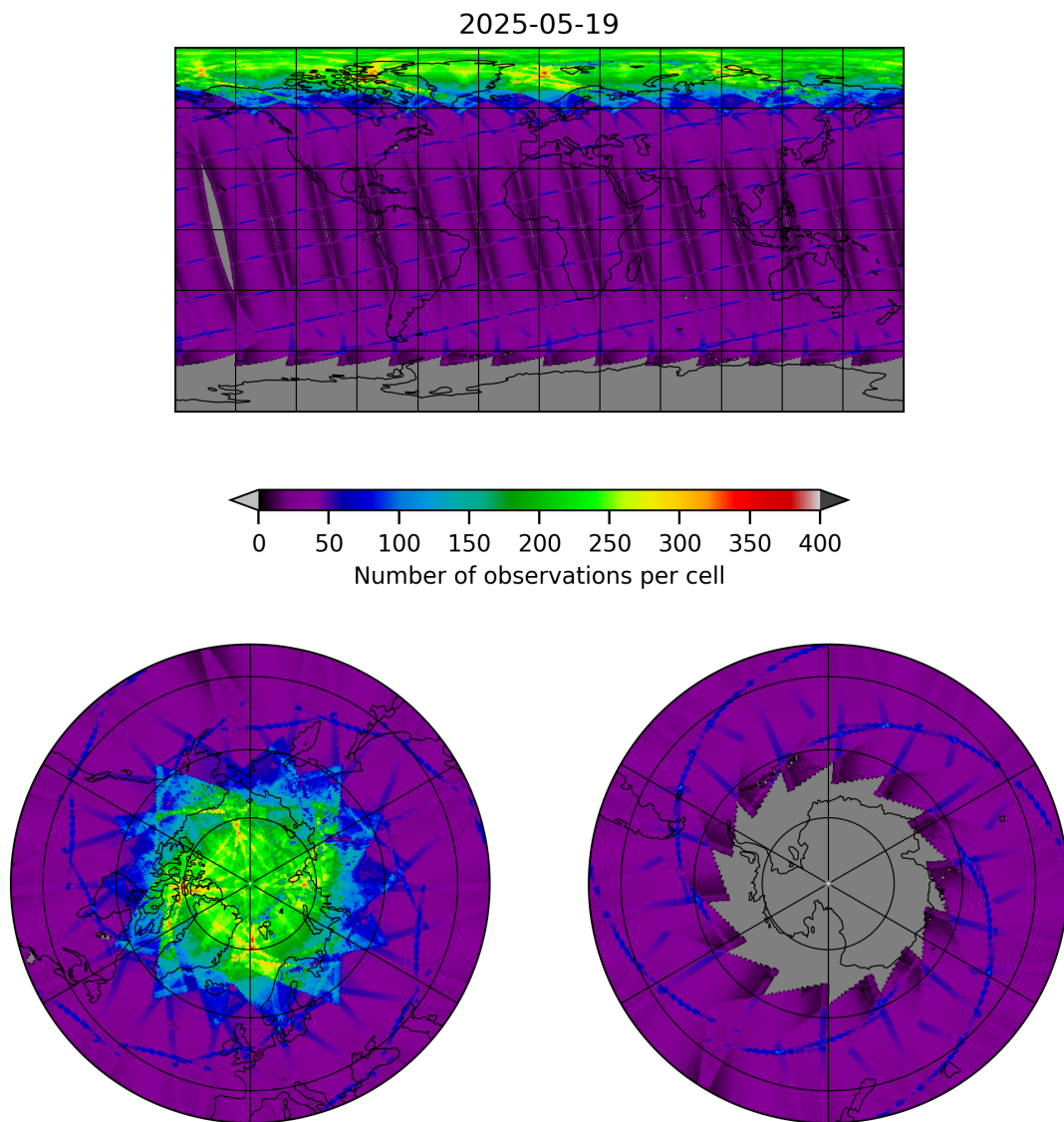
Figure 9: Map of the number of observations for 2025-05-19 to 2025-05-19
