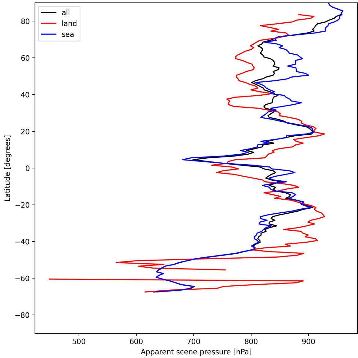
Figure 17: Zonal average of “Apparent scene pressure” for 2025-05-19 to 2025-05-19.
