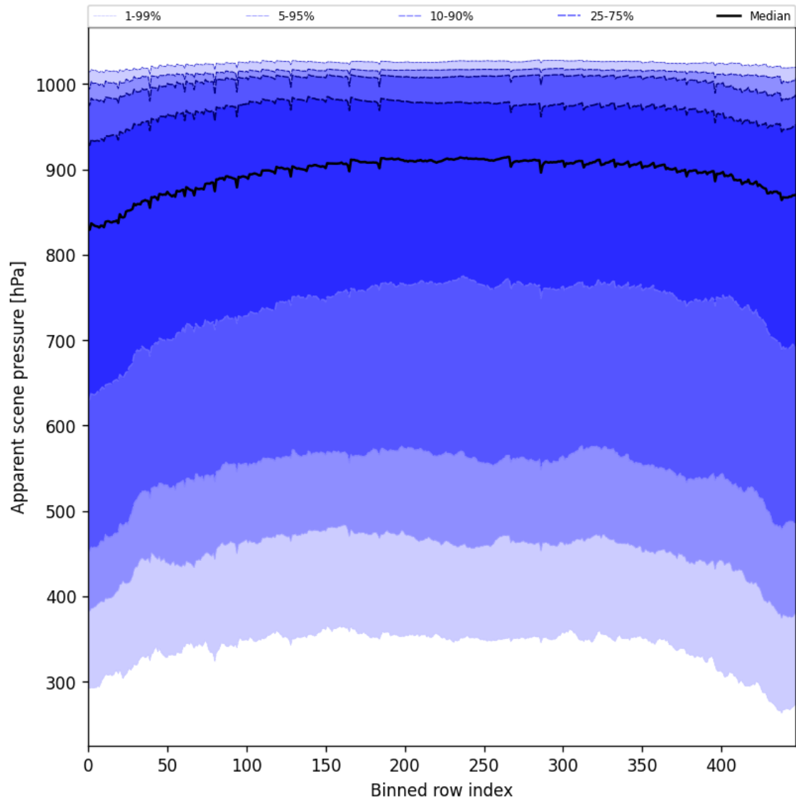
Figure 51: Along track statistics of “Apparent scene pressure” for 2025-05-19 to 2025-05-19
