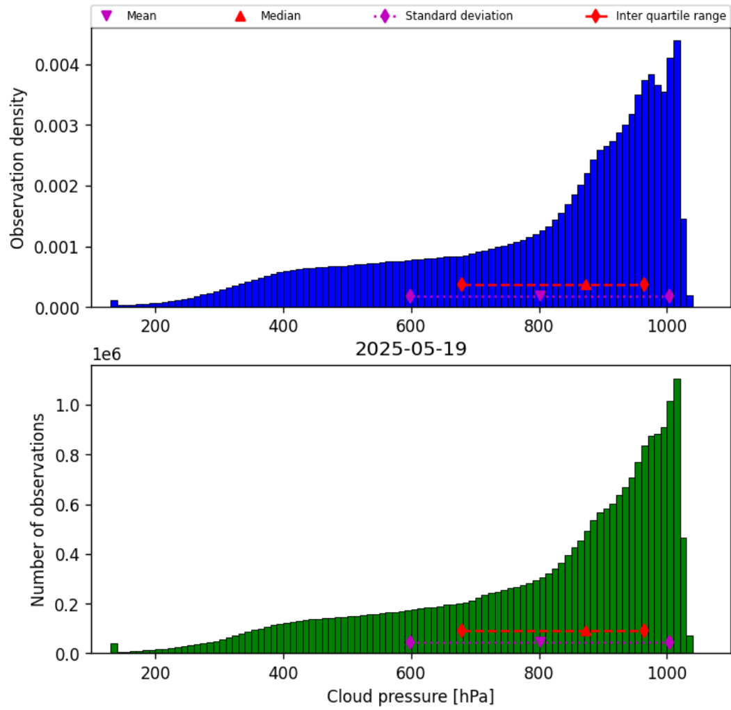
Figure 28: Histogram of “Cloud pressure” for 2025-05-19 to 2025-05-19
