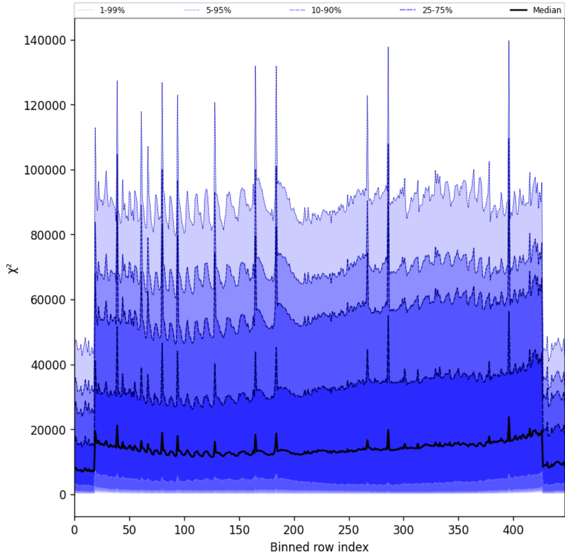
Figure 53: Along track statistics of “ \chi^2 ” for 2025-05-19 to 2025-05-19
