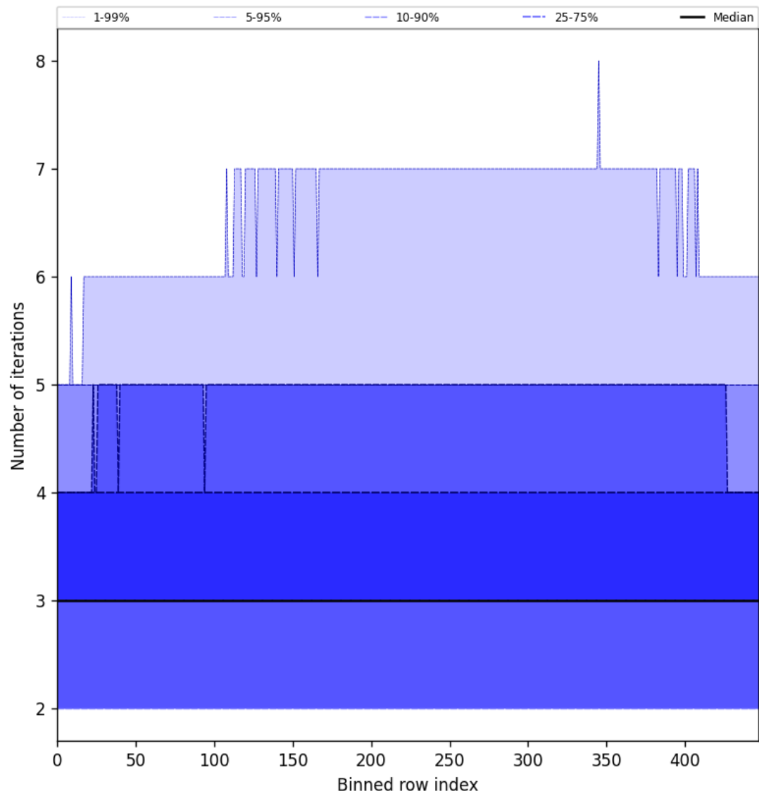
Figure 54: Along track statistics of “Number of iterations” for 2025-05-19 to 2025-05-19
