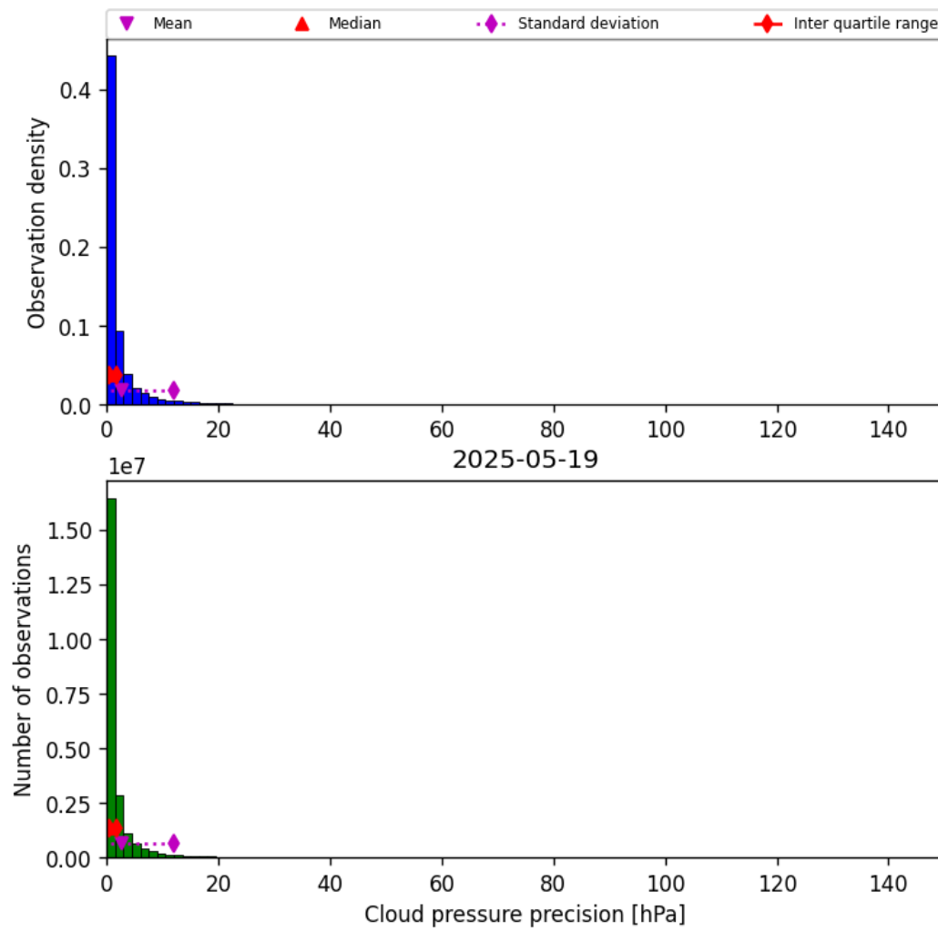
Figure 29: Histogram of “Cloud pressure precision” for 2025-05-19 to 2025-05-19
