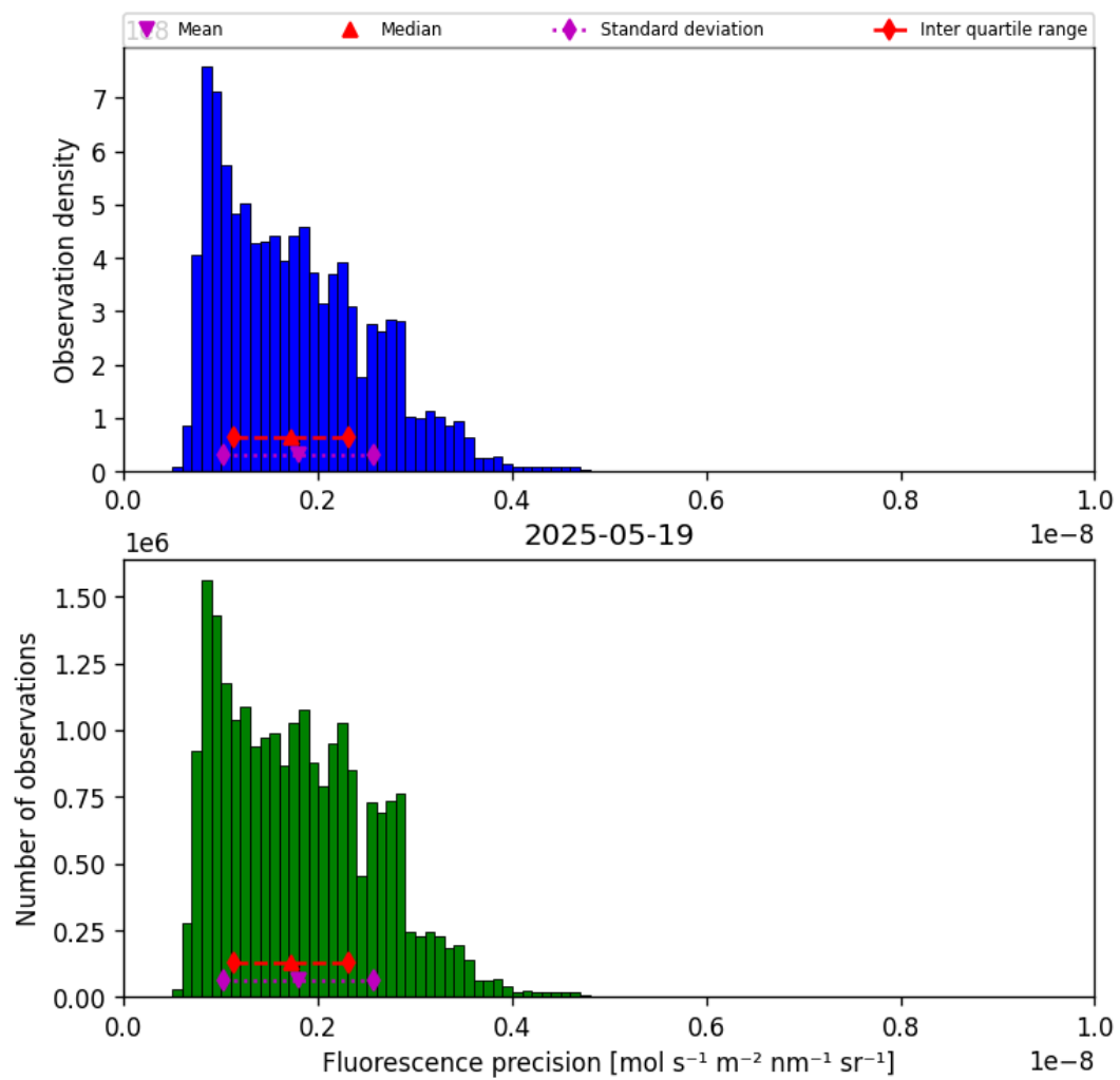
Figure 39: Histogram of “Fluorescence precision” for 2025-05-19 to 2025-05-19
