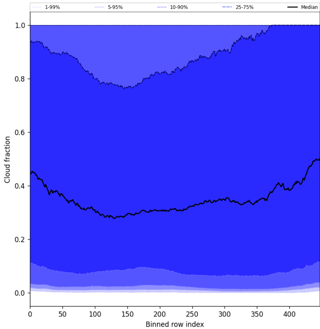
Figure 47: Along track statistics of “Cloud fraction” for 2025-05-19 to 2025-05-19
