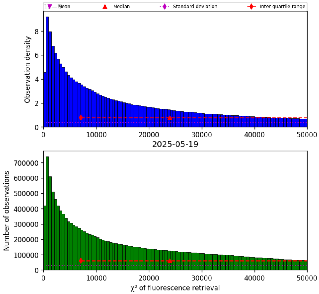
Figure 40: Histogram of “ \chi^2 of fluorescence retrieval” for 2025-05-19 to 2025-05-19
