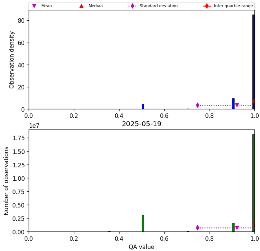
Figure 27: Histogram of “QA value” for 2025-05-19 to 2025-05-19
