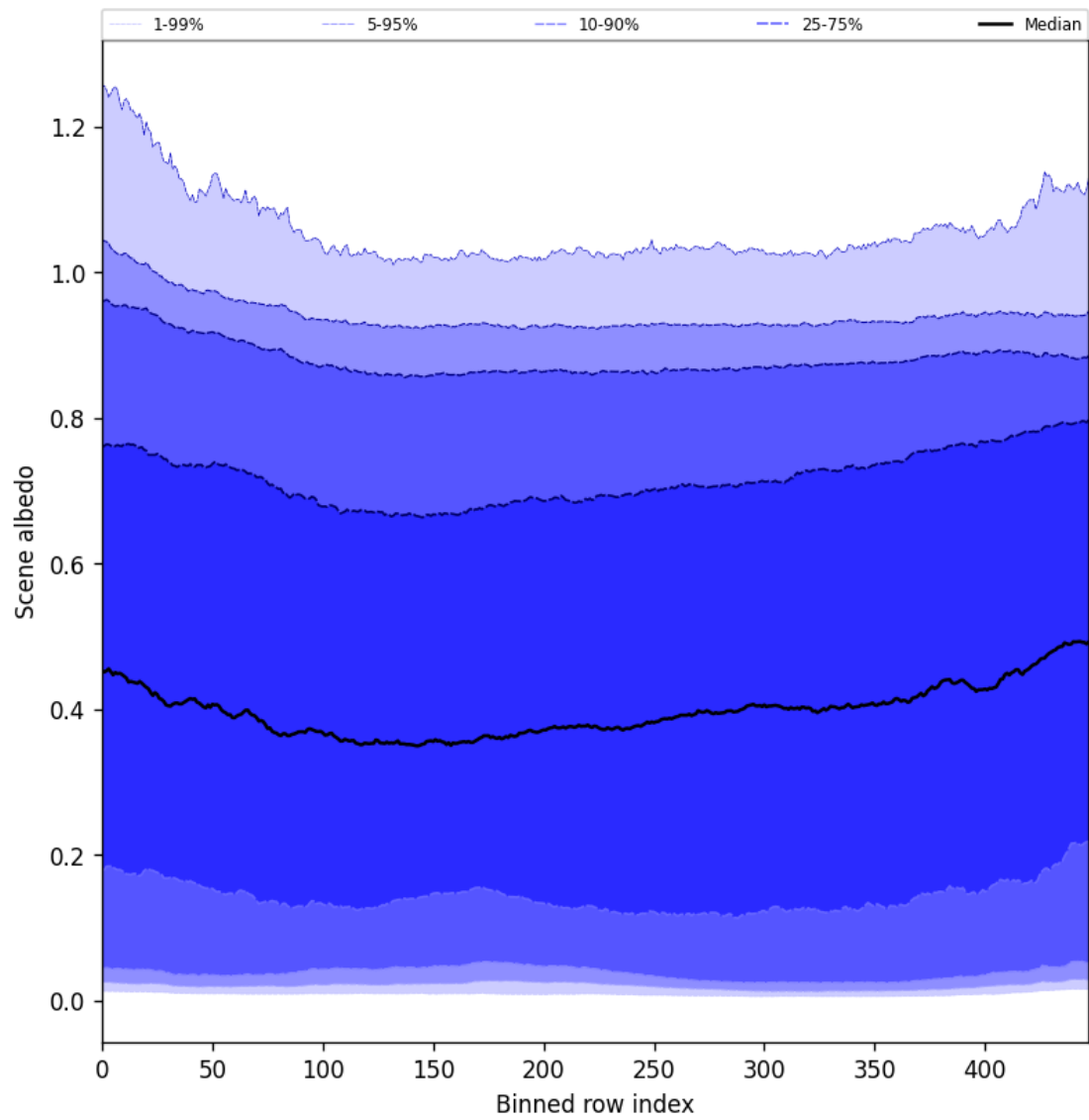
Figure 49: Along track statistics of “Scene albedo” for 2025-05-19 to 2025-05-19
