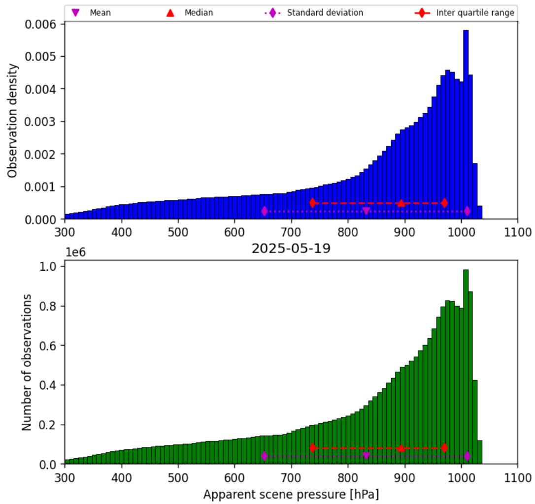
Figure 34: Histogram of “Apparent scene pressure” for 2025-05-19 to 2025-05-19
