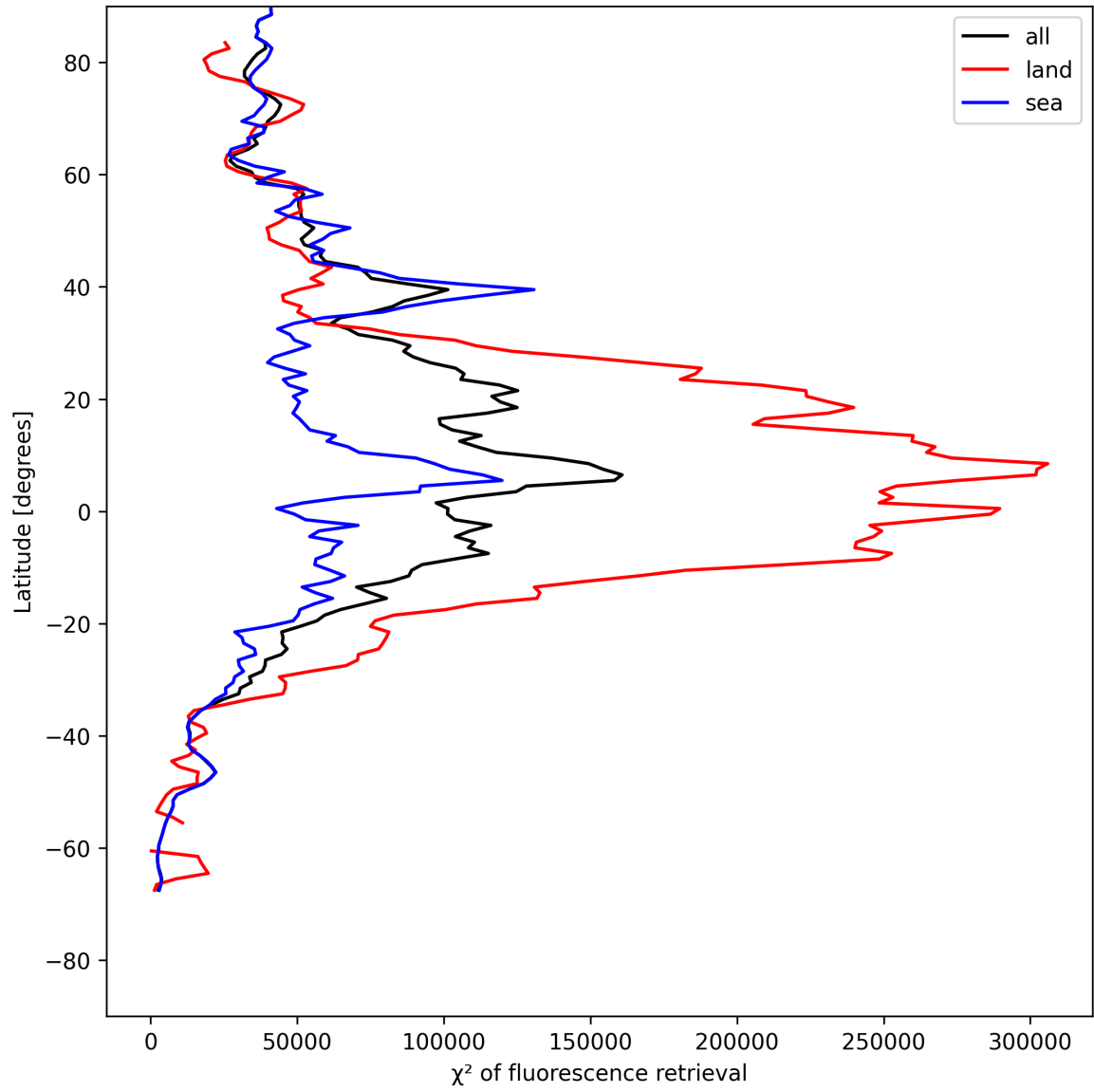
Figure 23: Zonal average of “ \chi^2 of fluorescence retrieval” for 2025-05-19 to 2025-05-19.
