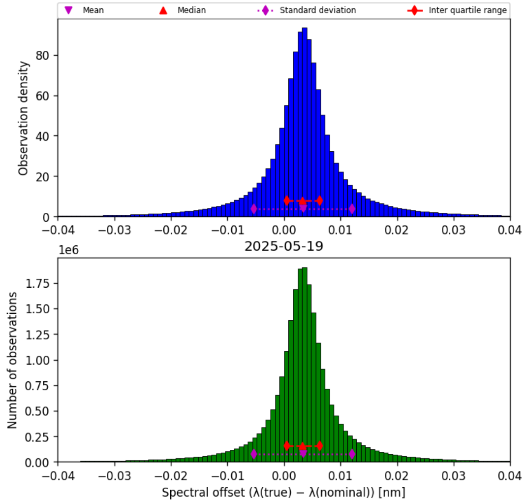
Figure 43: Histogram of “Spectral offset ( \lambda_{\text{true}} - \lambda_{\text{nominal}} )” for 2025-05-19 to 2025-05-19
