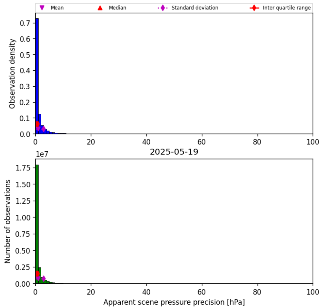
Figure 35: Histogram of “Apparent scene pressure precision” for 2025-05-19 to 2025-05-19
