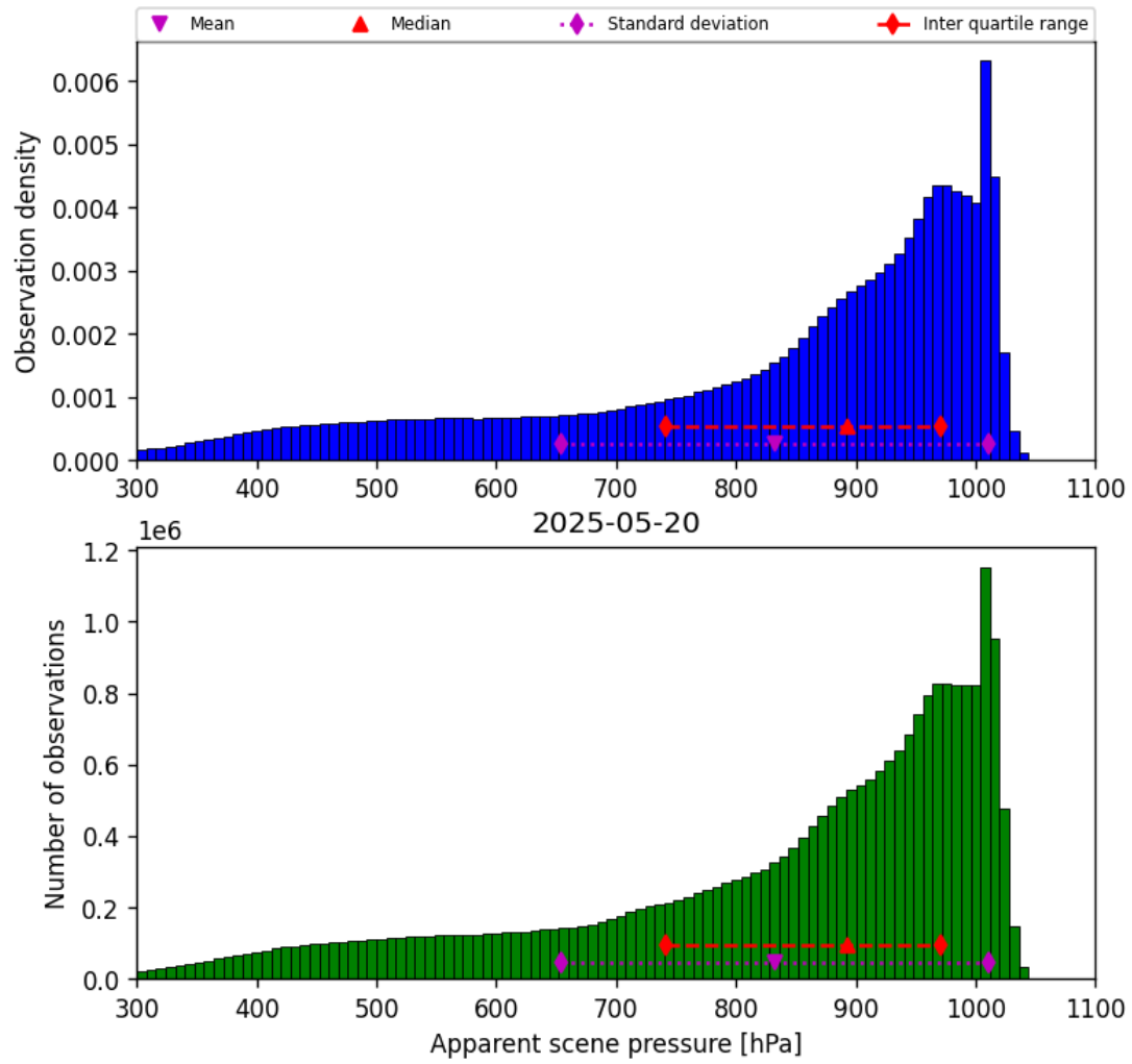
Figure 34: Histogram of “Apparent scene pressure” for 2025-05-20 to 2025-05-21
