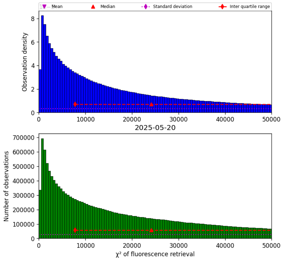
Figure 40: Histogram of “ \chi^2 of fluorescence retrieval” for 2025-05-20 to 2025-05-21
