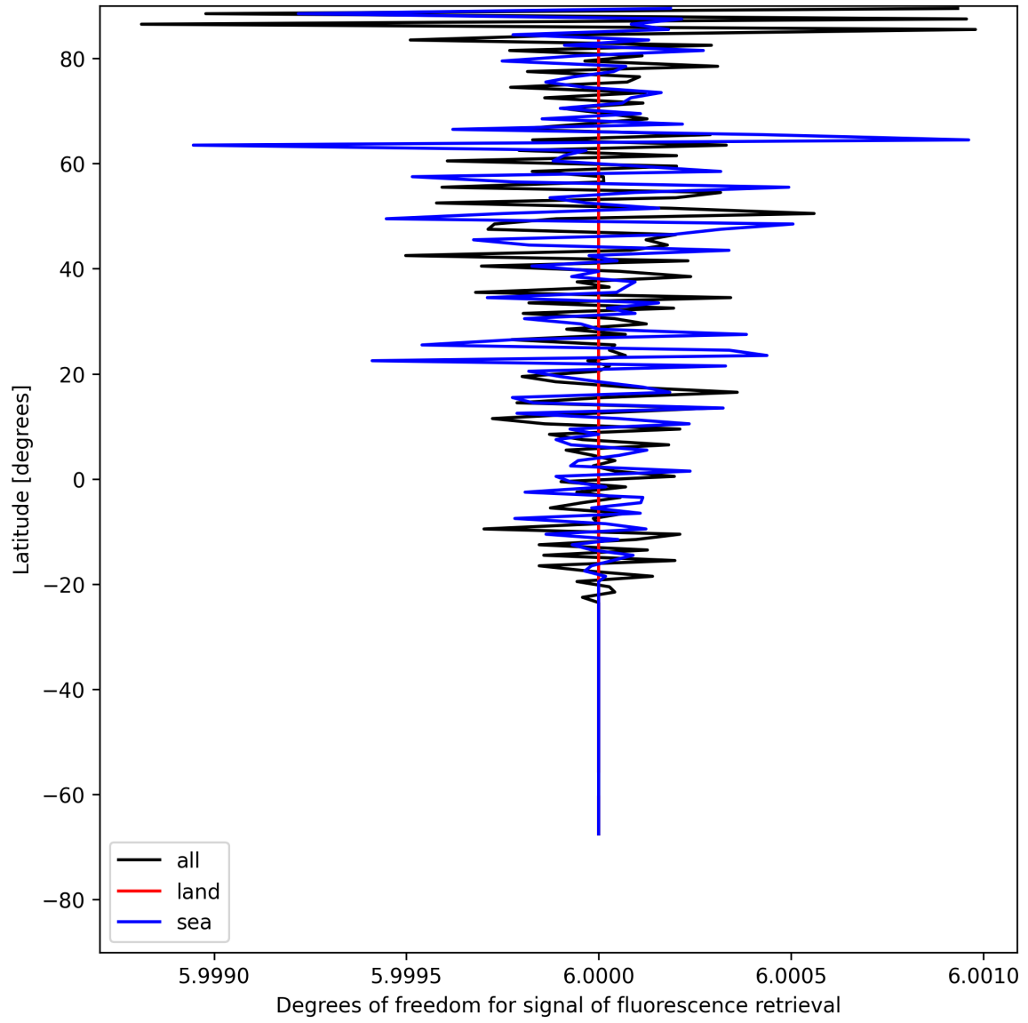
Figure 24: Zonal average of “Degrees of freedom for signal of fluorescence retrieval” for 2025-05-20 to 2025-05-21.
