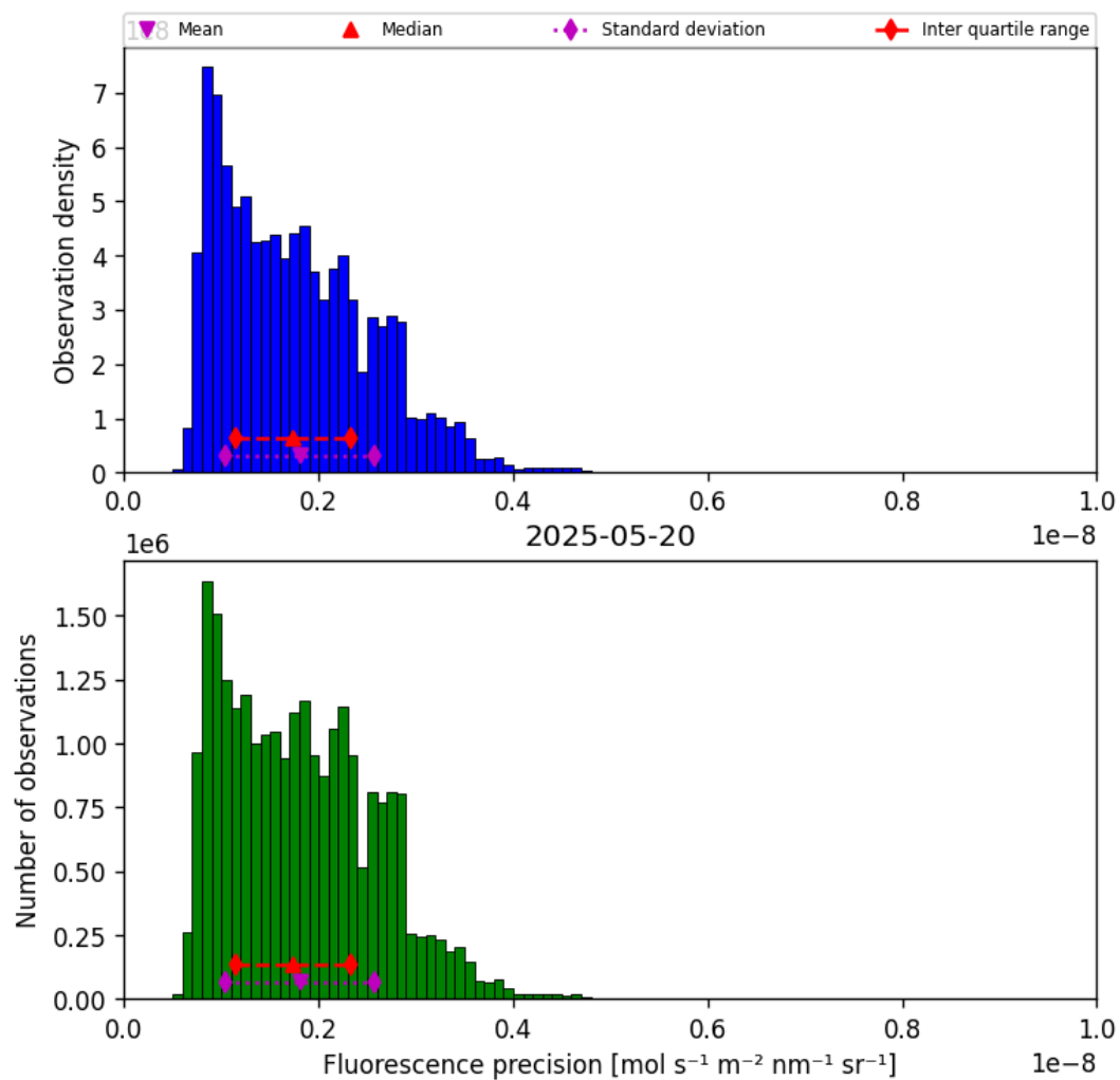
Figure 39: Histogram of “Fluorescence precision” for 2025-05-20 to 2025-05-21
