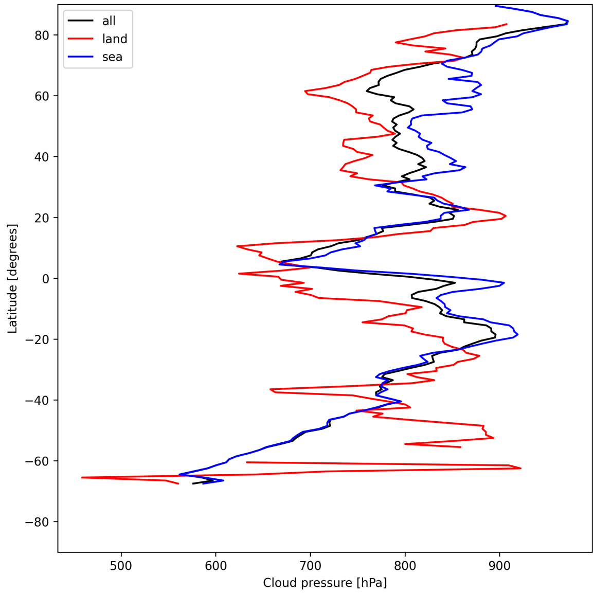
Figure 11: Zonal average of “Cloud pressure” for 2025-05-20 to 2025-05-21.
