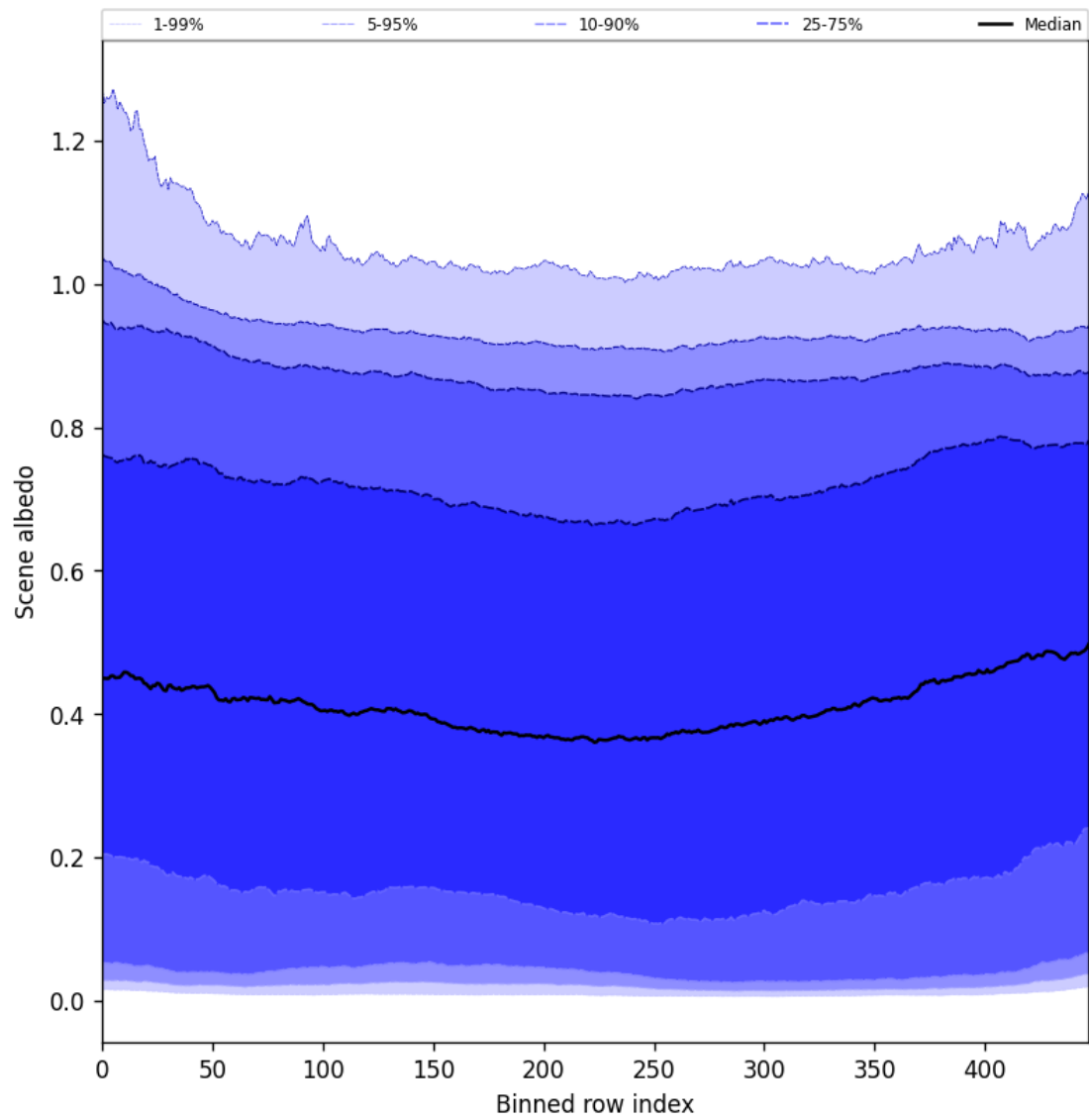
Figure 49: Along track statistics of “Scene albedo” for 2025-05-20 to 2025-05-21
