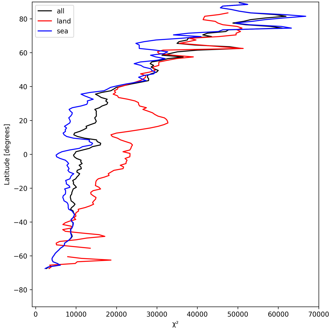
Figure 19: Zonal average of “ \chi^2 ” for 2025-05-20 to 2025-05-21.
