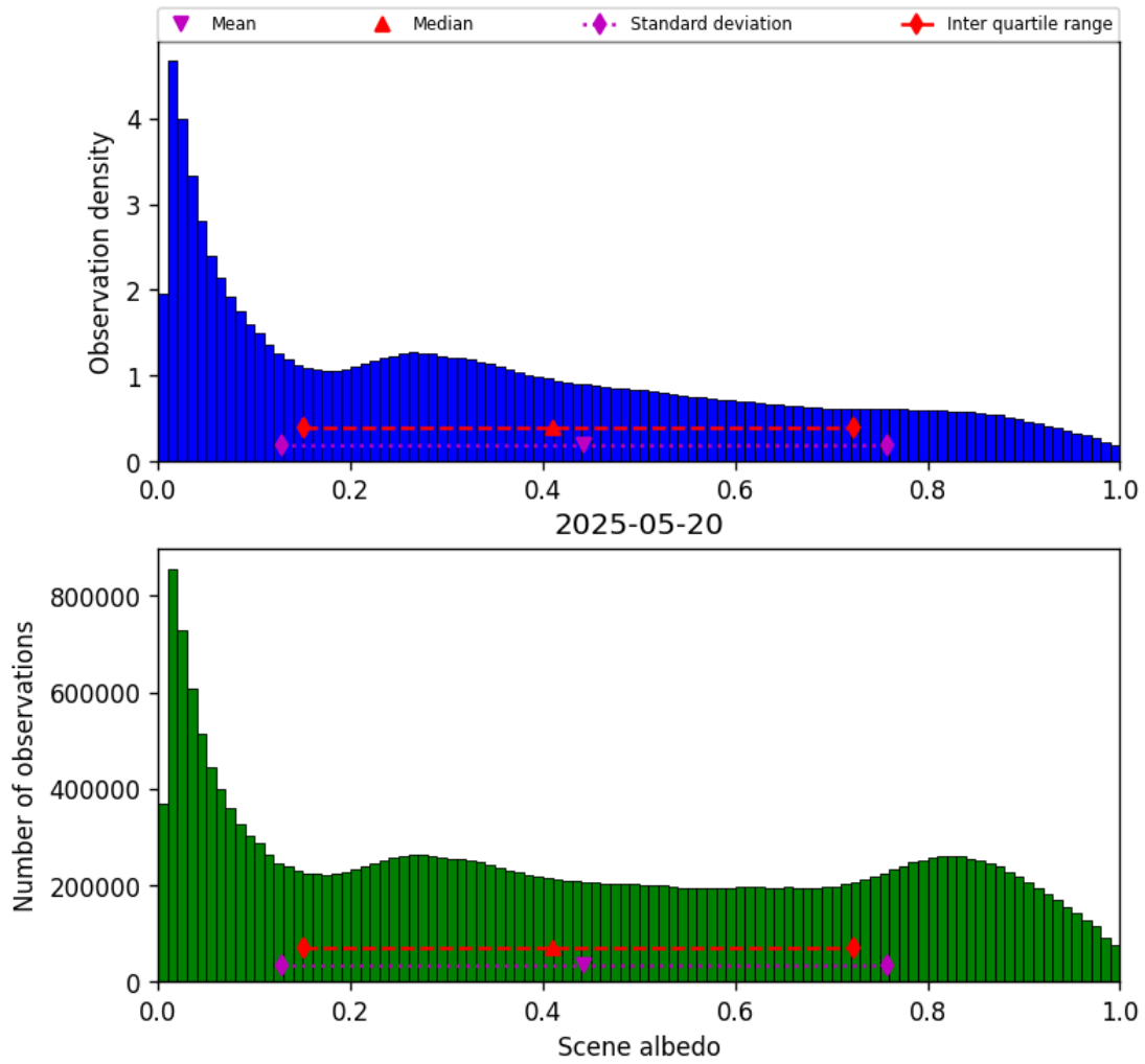
Figure 32: Histogram of “Scene albedo” for 2025-05-20 to 2025-05-21
