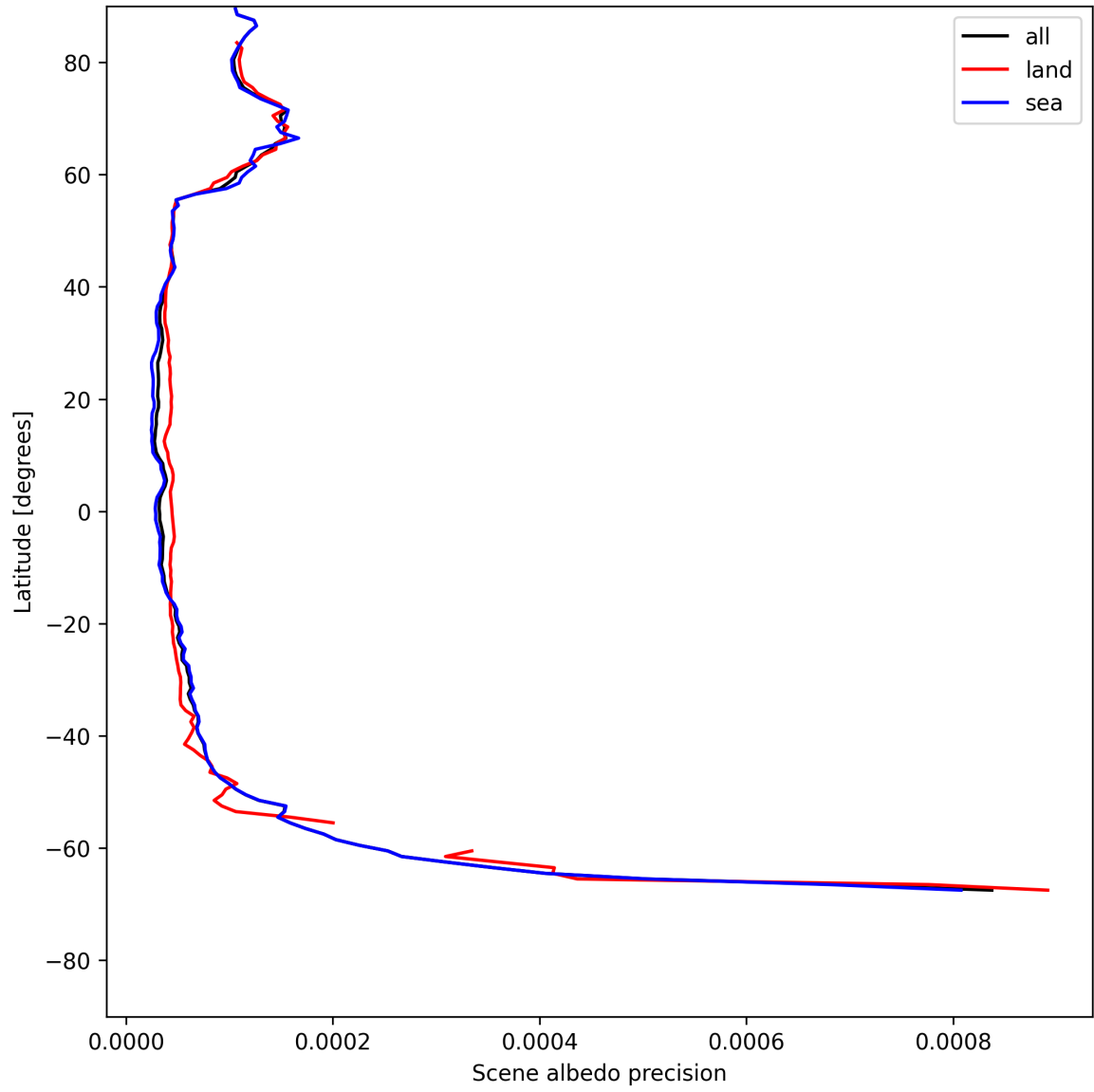
Figure 16: Zonal average of “Scene albedo precision” for 2025-05-20 to 2025-05-21.
