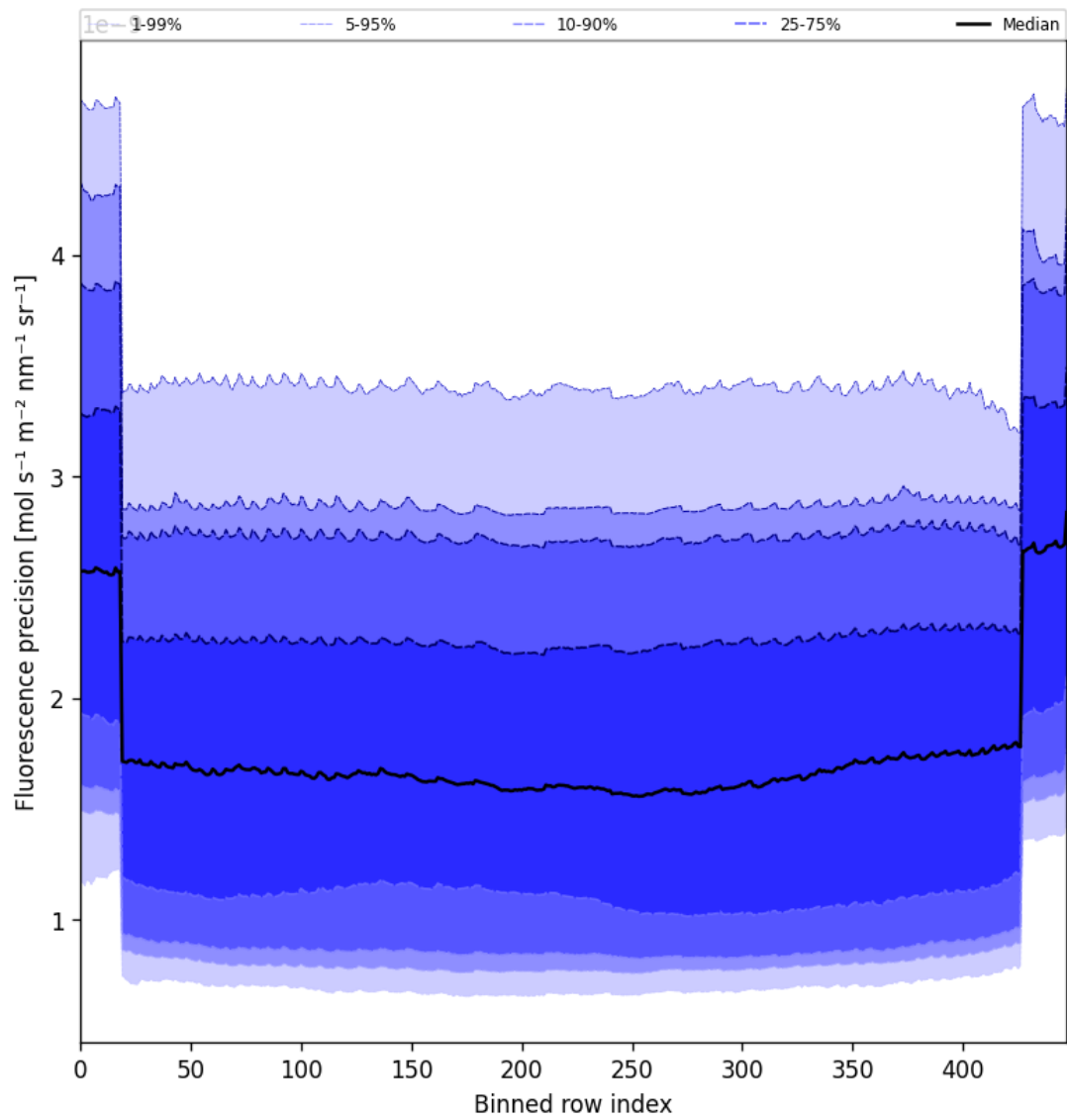
Figure 56: Along track statistics of “Fluorescence precision” for 2025-05-20 to 2025-05-21
