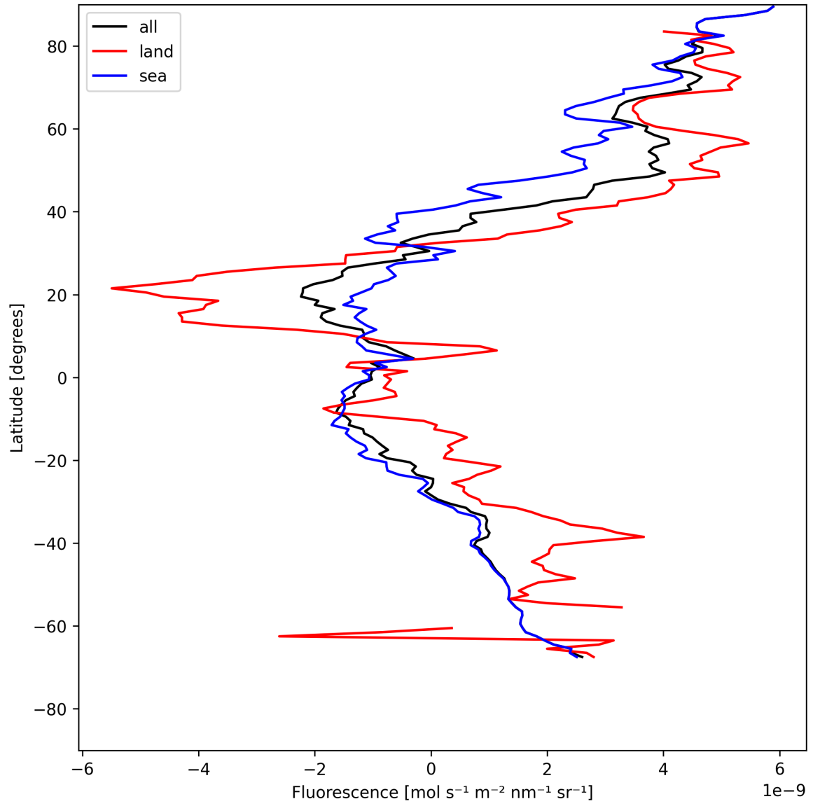
Figure 21: Zonal average of “Fluorescence” for 2025-05-20 to 2025-05-21.
