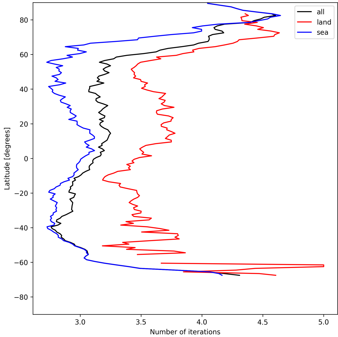
Figure 20: Zonal average of “Number of iterations” for 2025-05-20 to 2025-05-21.
