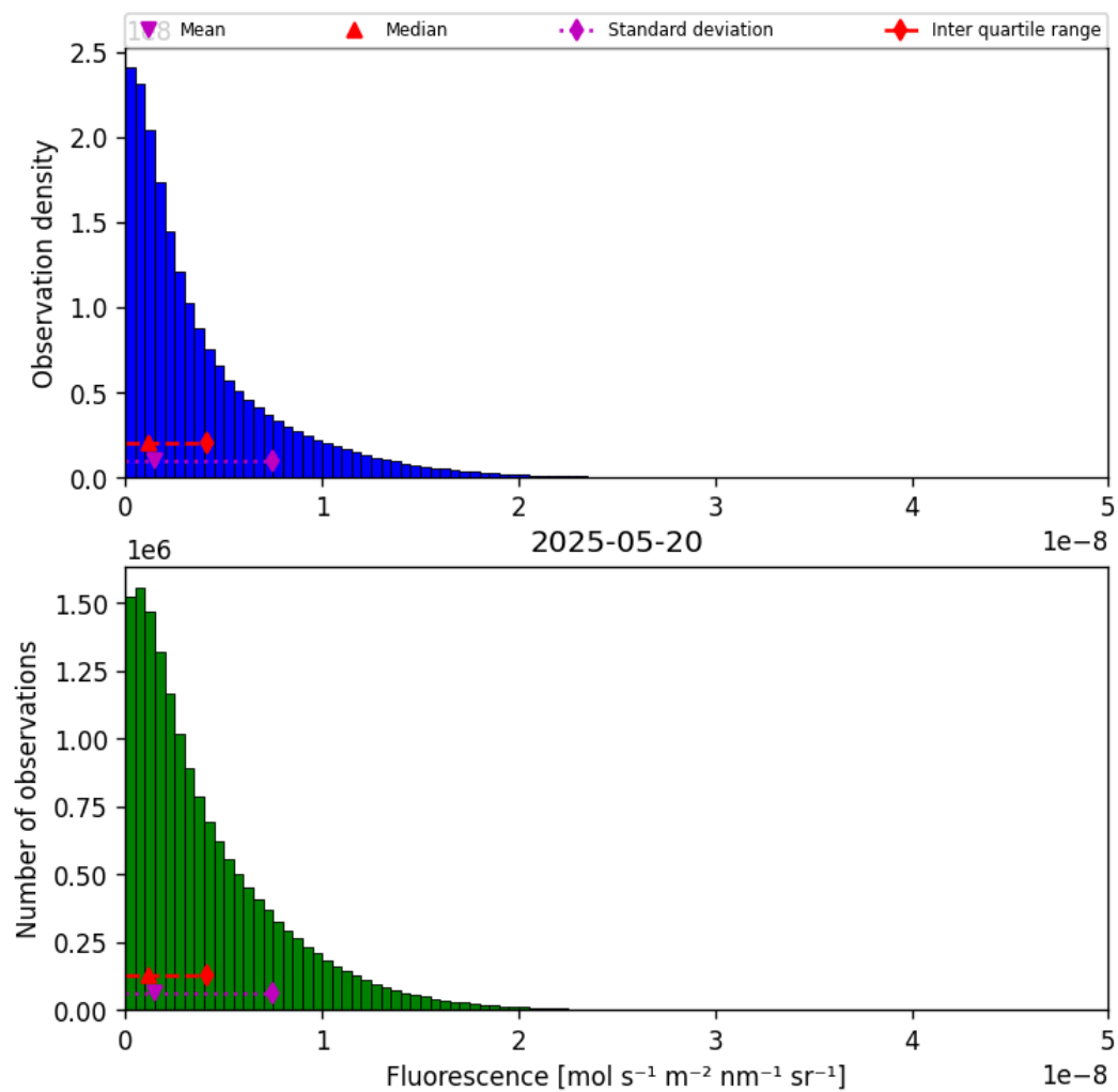
Figure 38: Histogram of “Fluorescence” for 2025-05-20 to 2025-05-21
