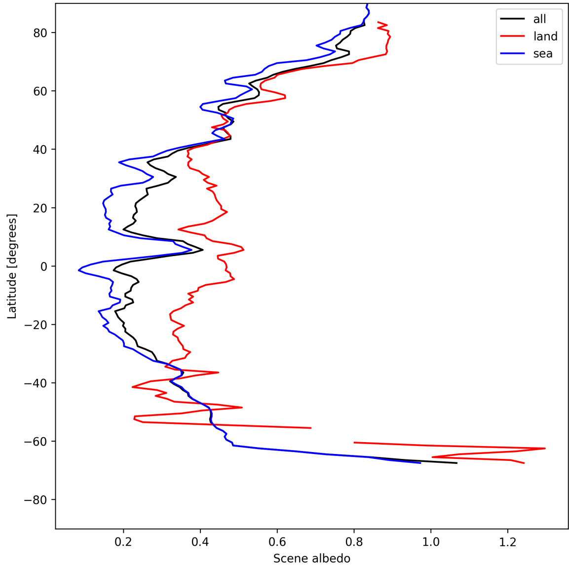
Figure 15: Zonal average of “Scene albedo” for 2025-05-20 to 2025-05-21.
