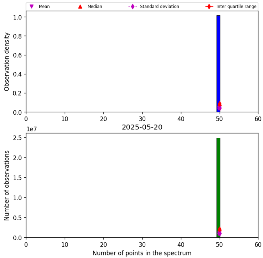
Figure 42: Histogram of “Number of points in the spectrum” for 2025-05-20 to 2025-05-21
