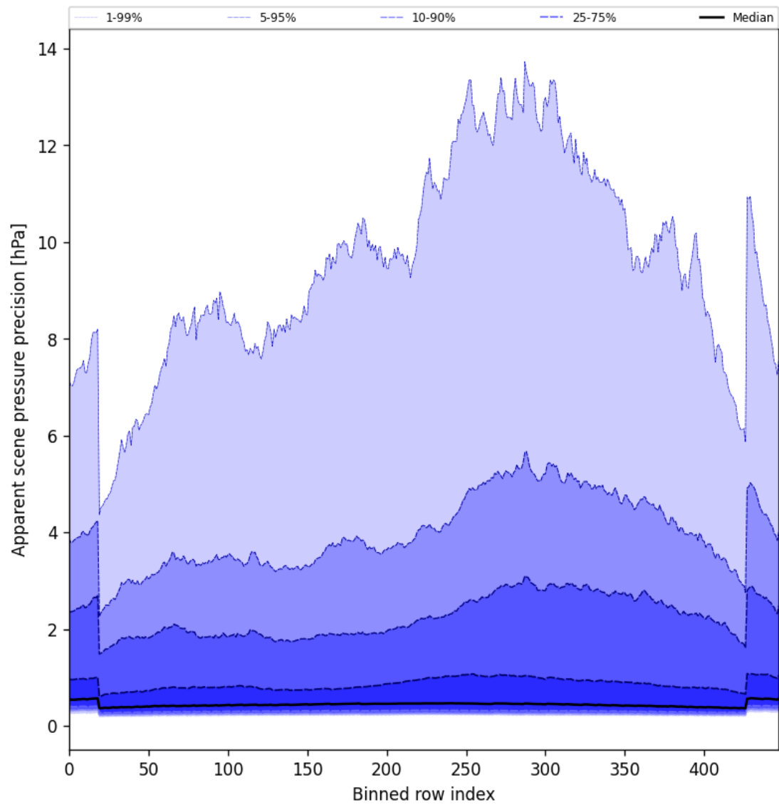
Figure 52: Along track statistics of “Apparent scene pressure precision” for 2025-05-20 to 2025-05-21
