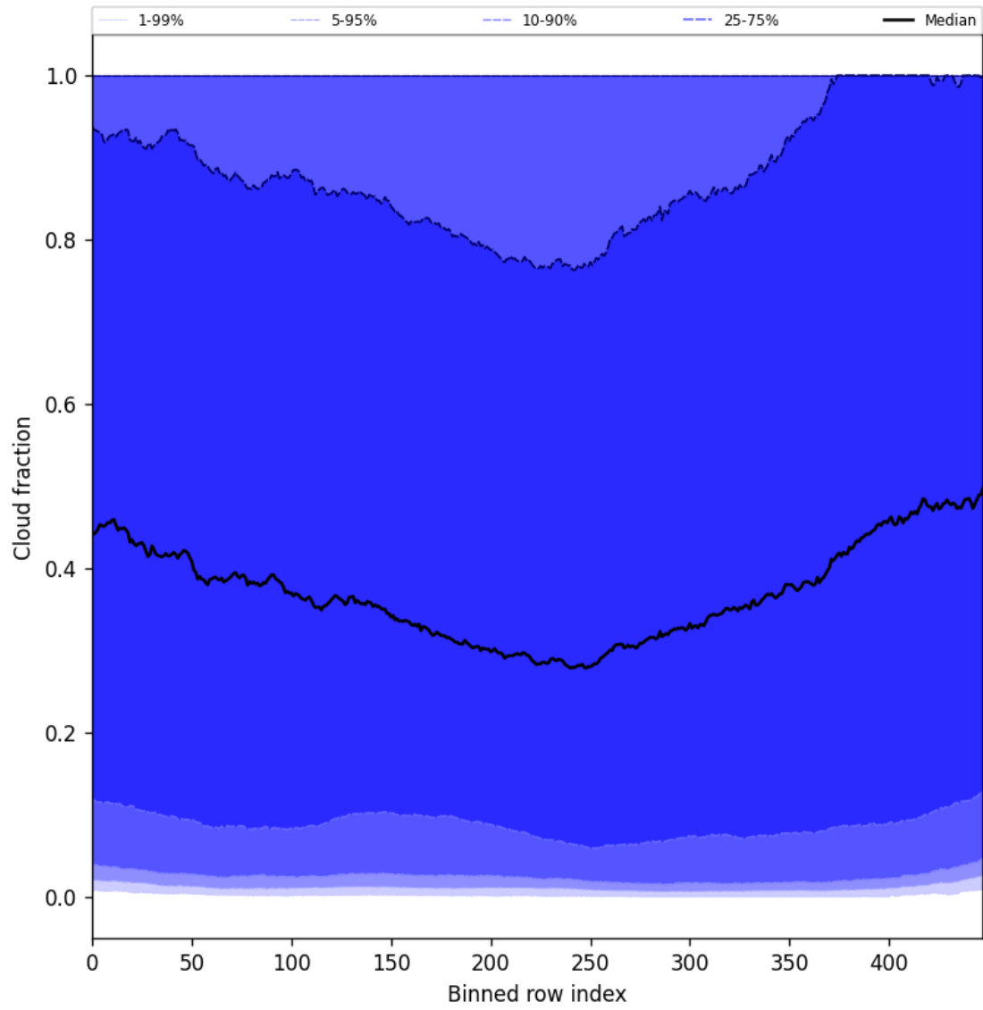
Figure 47: Along track statistics of “Cloud fraction” for 2025-05-20 to 2025-05-21
