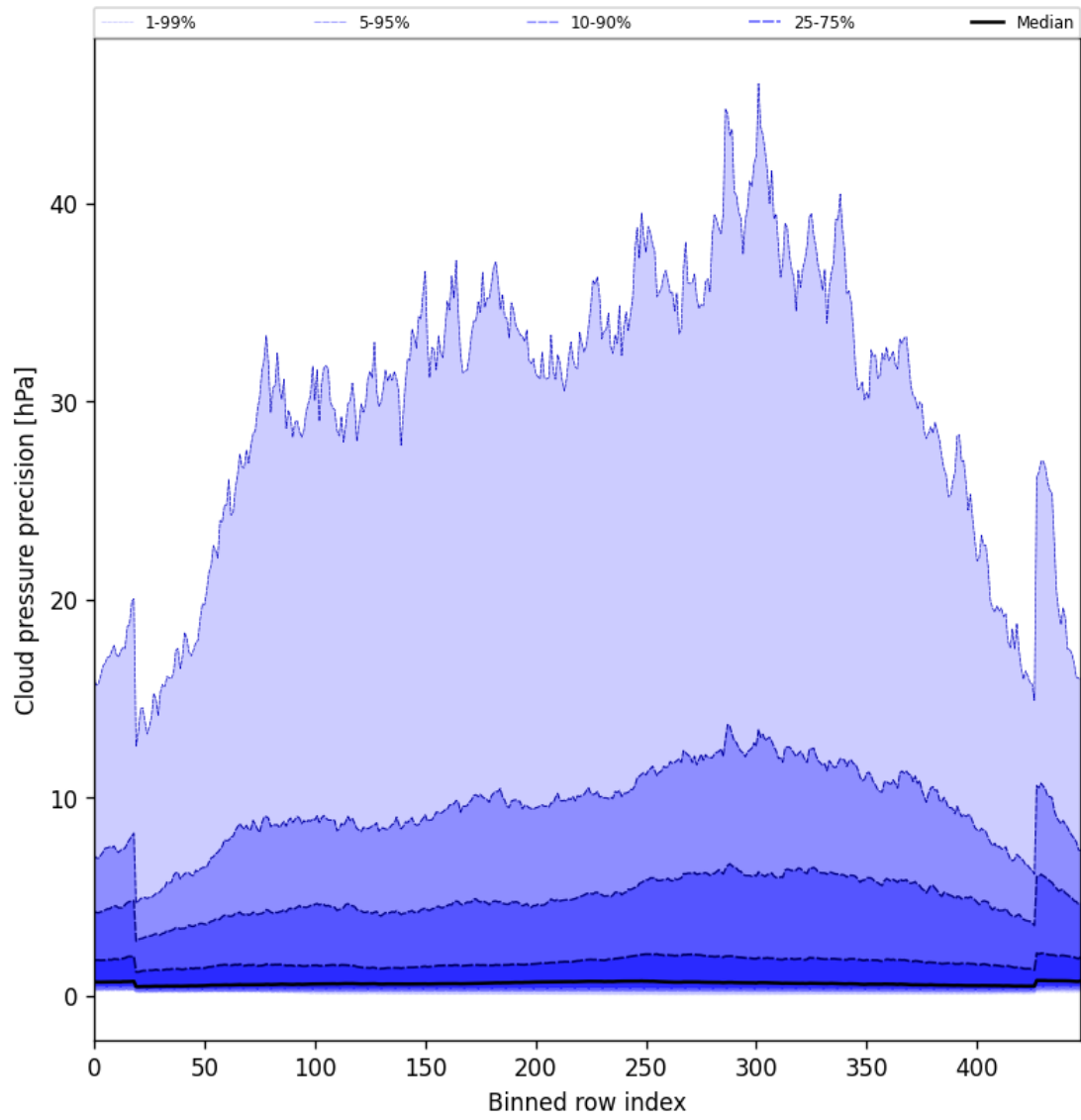
Figure 46: Along track statistics of “Cloud pressure precision” for 2025-05-20 to 2025-05-21
