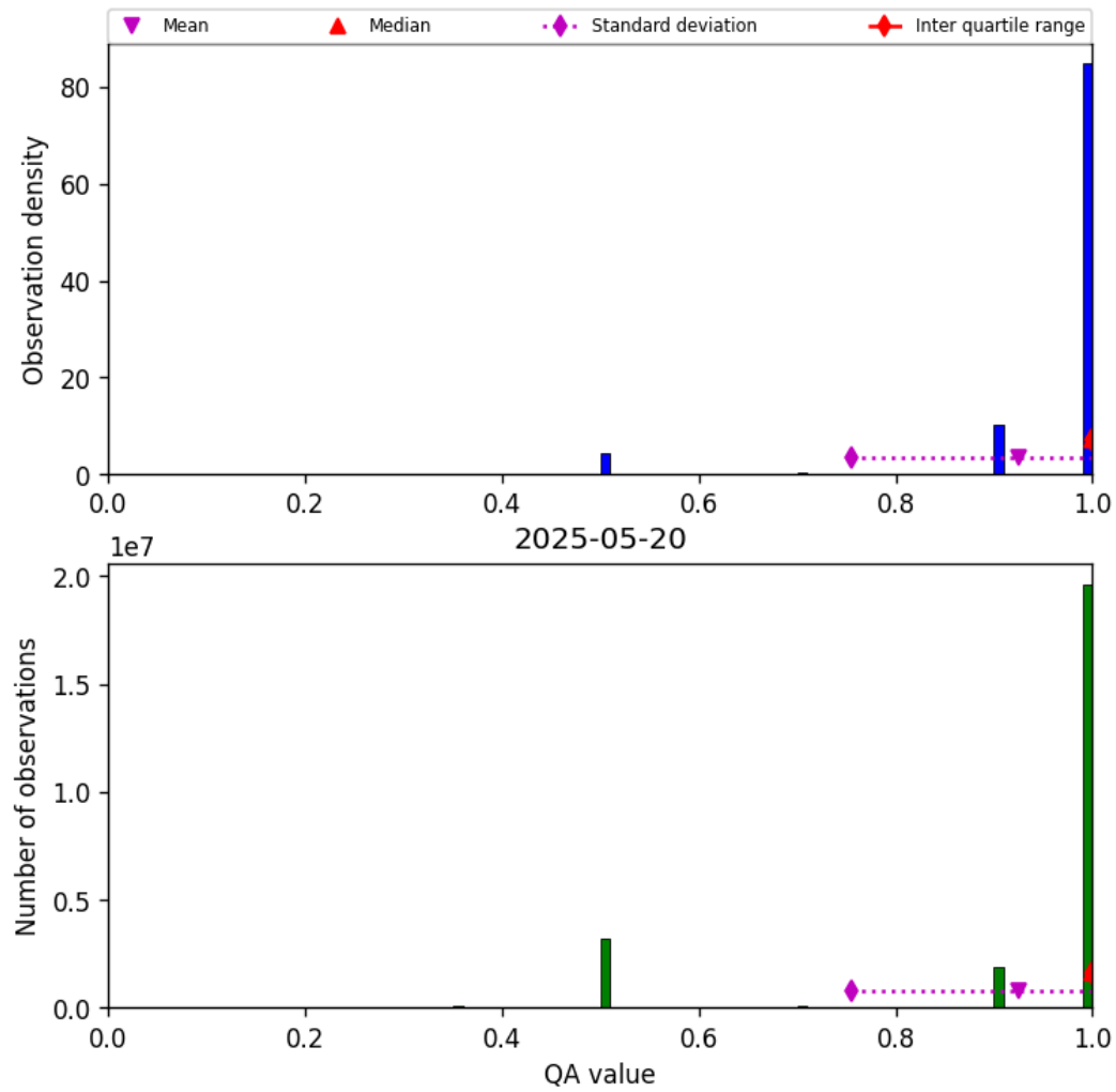
Figure 27: Histogram of “QA value” for 2025-05-20 to 2025-05-21
