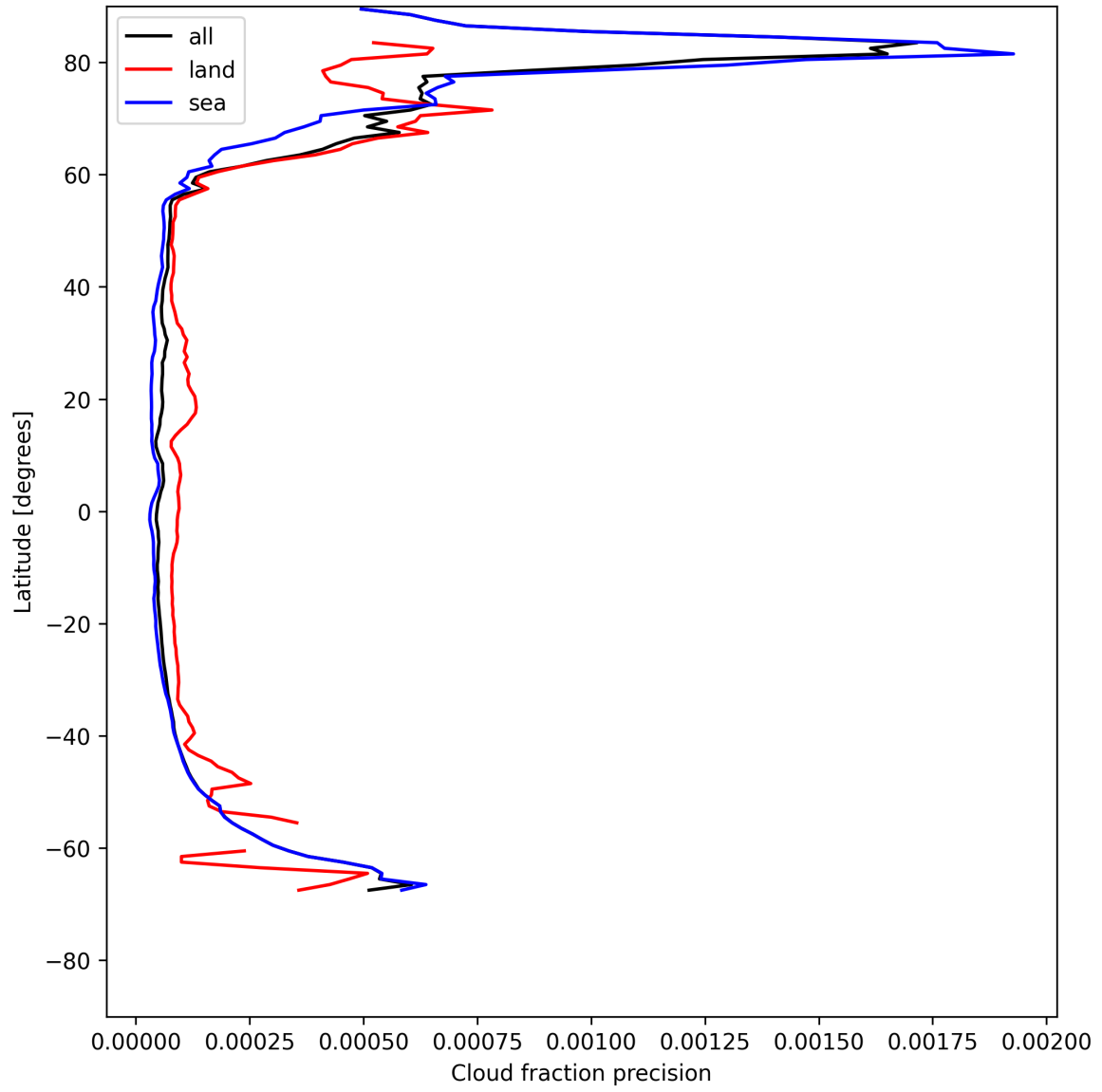
Figure 14: Zonal average of “Cloud fraction precision” for 2025-05-20 to 2025-05-21.
