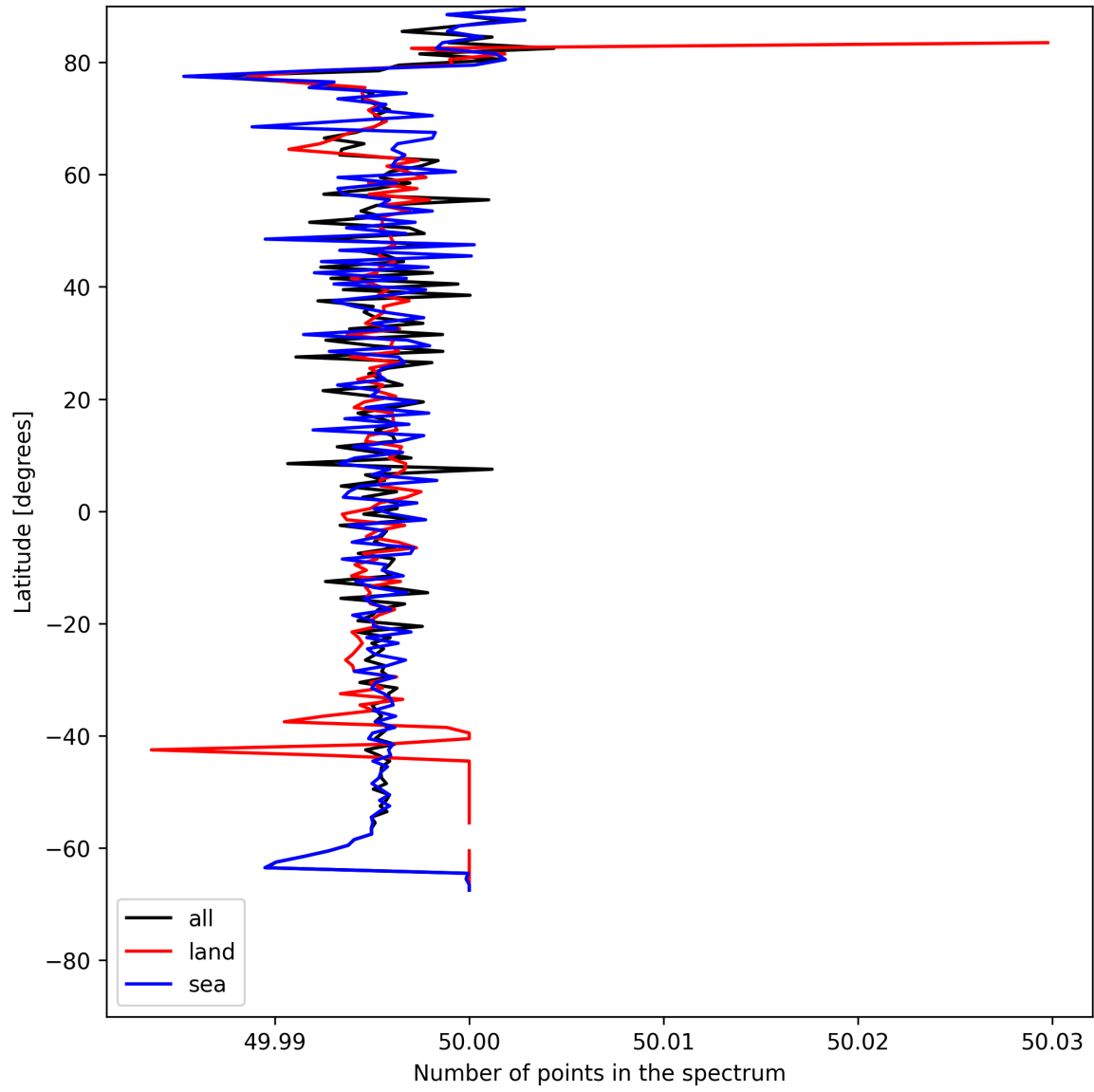
Figure 25: Zonal average of “Number of points in the spectrum” for 2025-05-20 to 2025-05-21.
