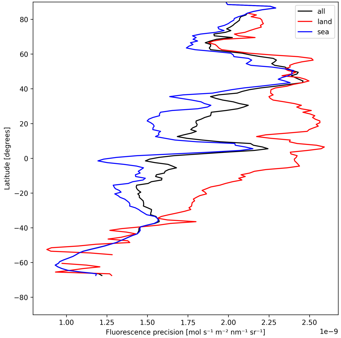
Figure 22: Zonal average of "Fluorescence precision" for 2025-05-20 to 2025-05-21.
