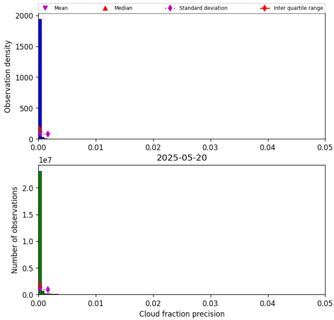
Figure 31: Histogram of “Cloud fraction precision” for 2025-05-20 to 2025-05-21
