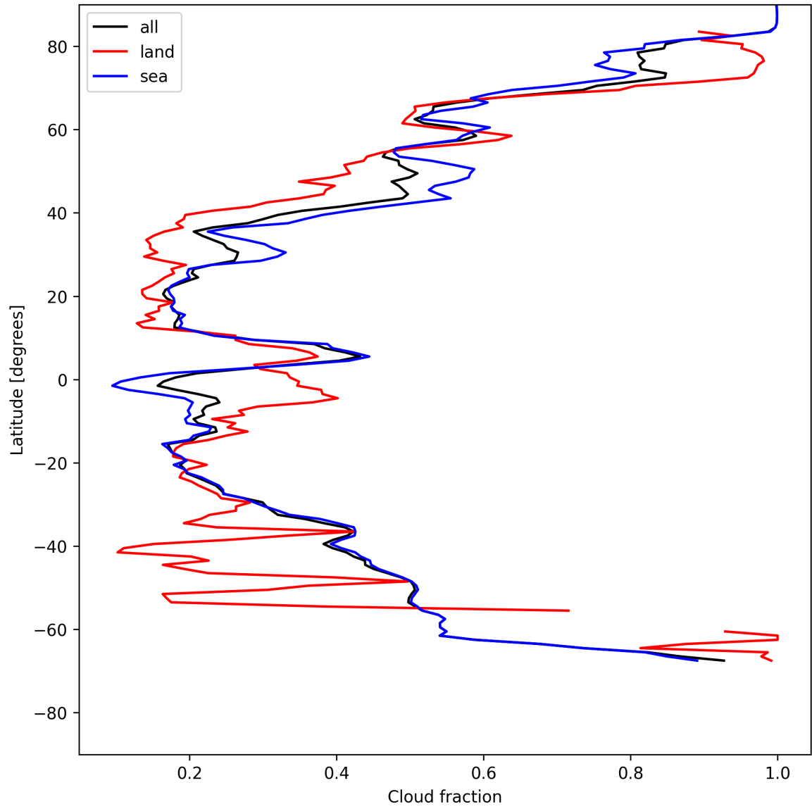
Figure 13: Zonal average of “Cloud fraction” for 2025-05-20 to 2025-05-21.
