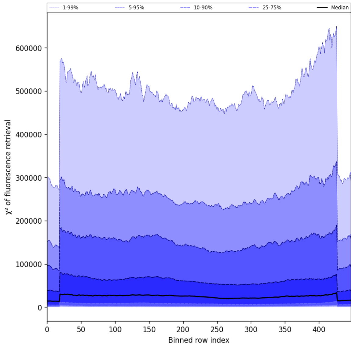
Figure 57: Along track statistics of “ \chi^2 of fluorescence retrieval” for 2025-05-20 to 2025-05-21
