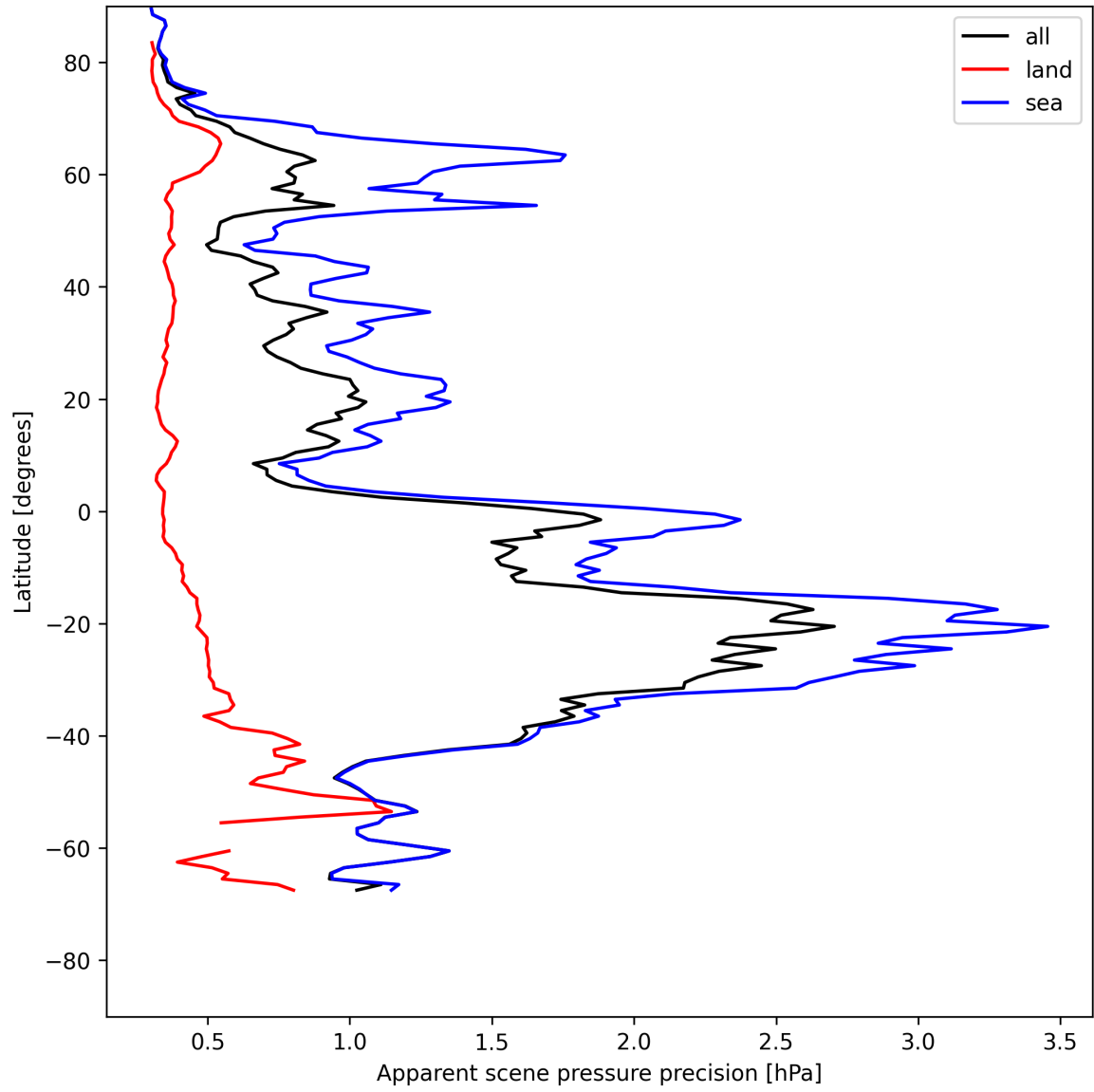
Figure 18: Zonal average of “Apparent scene pressure precision” for 2025-05-20 to 2025-05-21.
