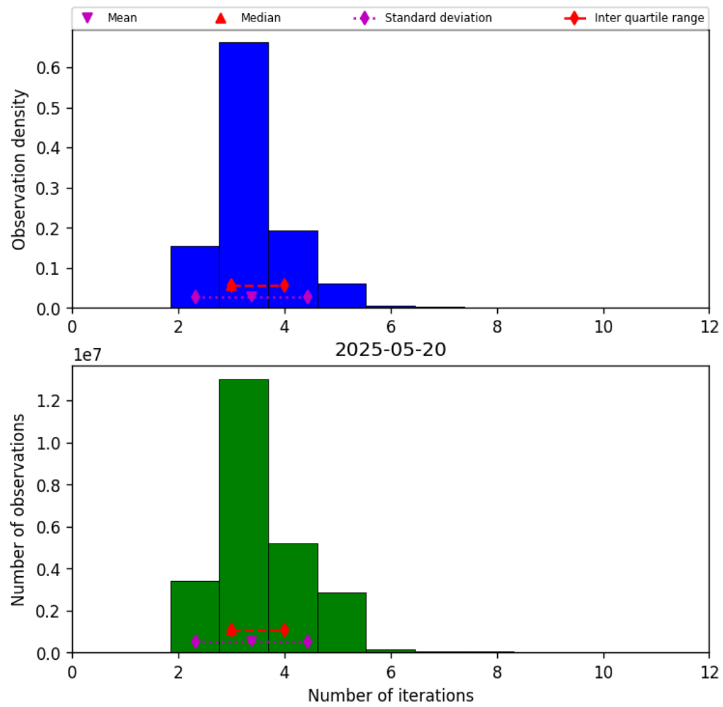
Figure 37: Histogram of “Number of iterations” for 2025-05-20 to 2025-05-21
