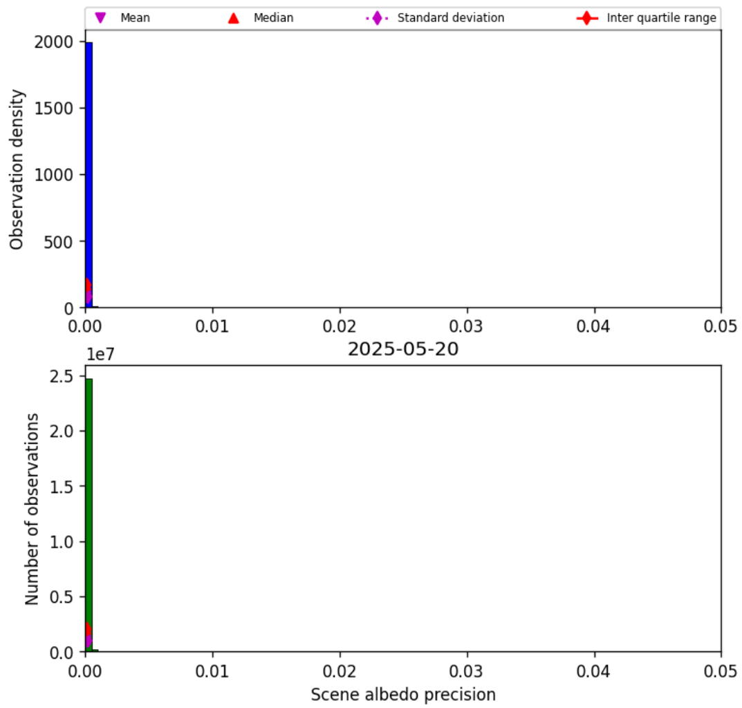
Figure 33: Histogram of “Scene albedo precision” for 2025-05-20 to 2025-05-21
