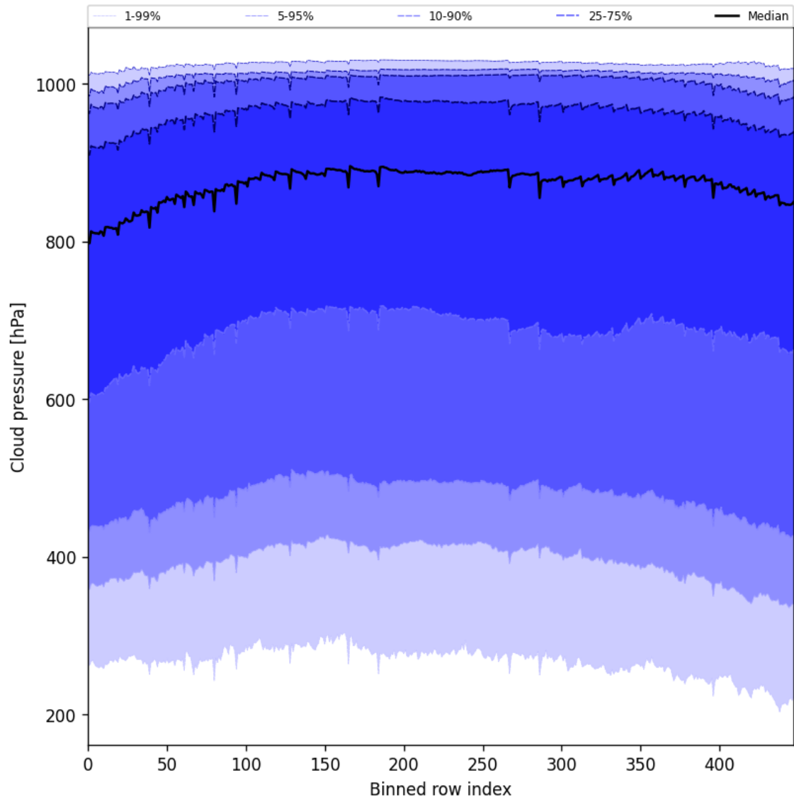
Figure 45: Along track statistics of “Cloud pressure” for 2025-05-20 to 2025-05-21
