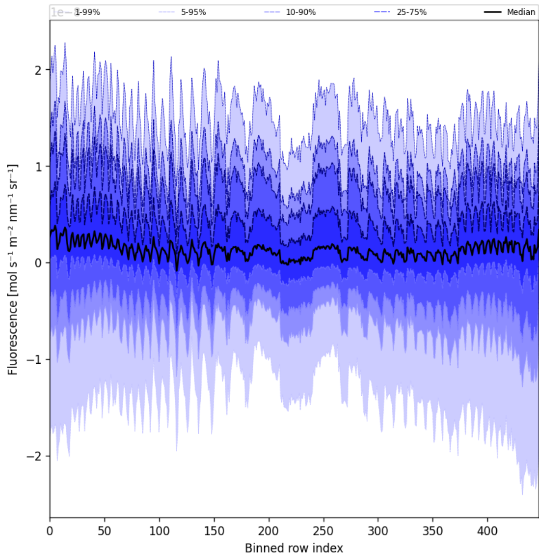
Figure 55: Along track statistics of “Fluorescence” for 2025-05-20 to 2025-05-21
