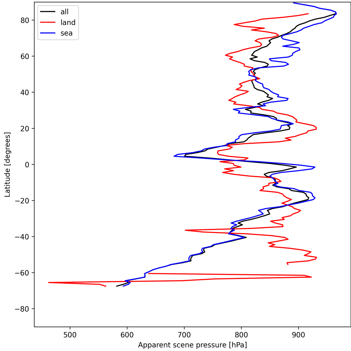
Figure 17: Zonal average of “Apparent scene pressure” for 2025-05-20 to 2025-05-21.
