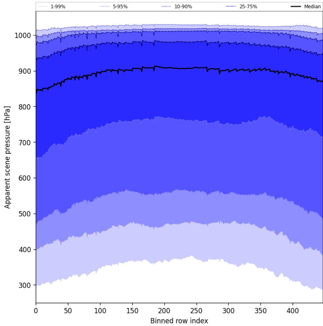
Figure 51: Along track statistics of “Apparent scene pressure” for 2025-05-20 to 2025-05-21
