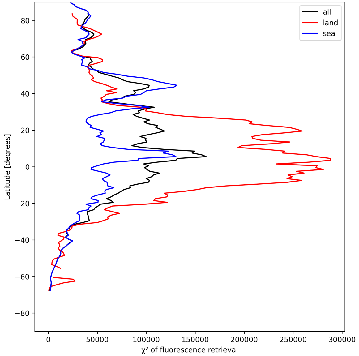
Figure 23: Zonal average of “ \chi^2 of fluorescence retrieval” for 2025-05-20 to 2025-05-21.
