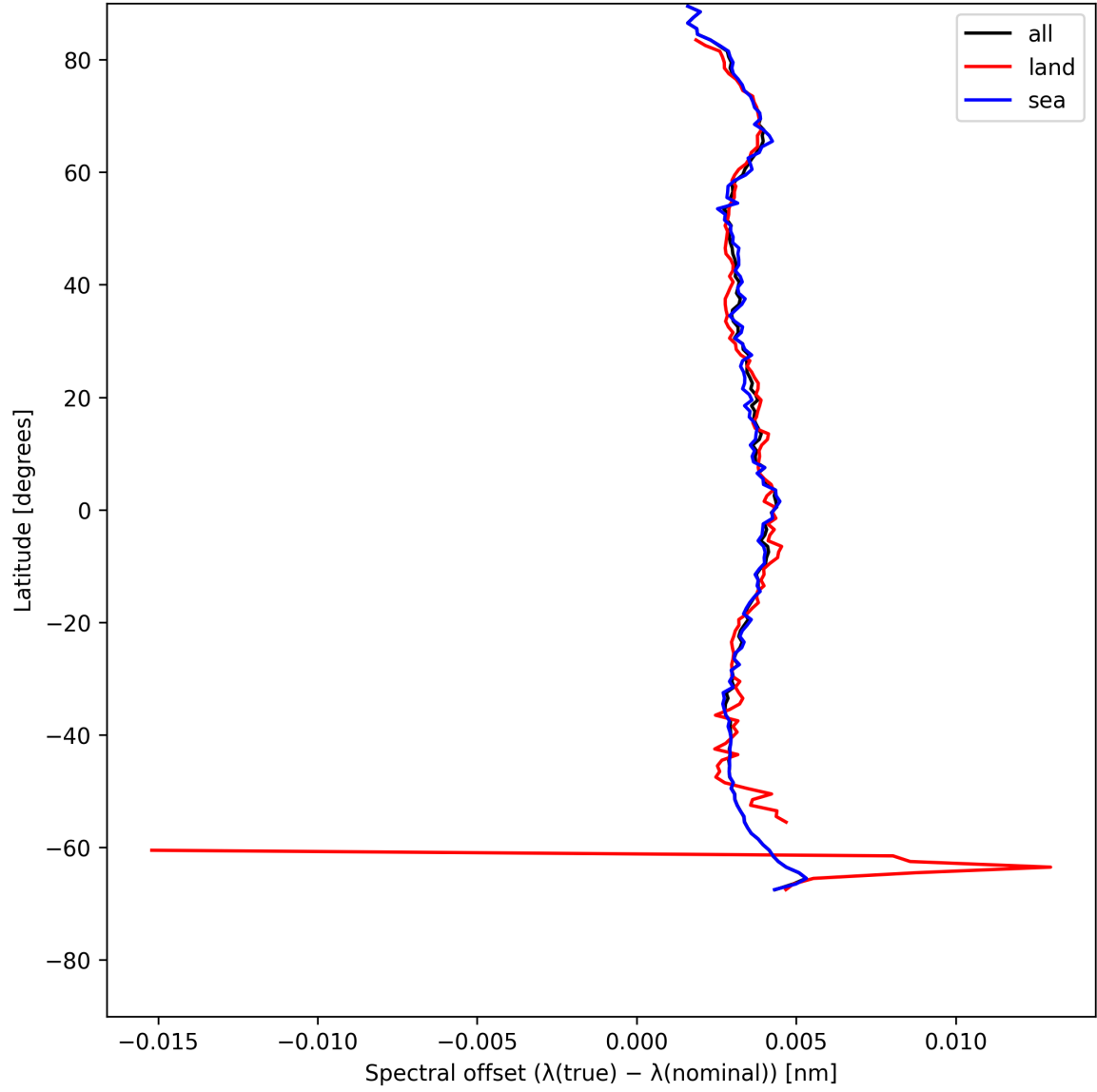
Figure 26: Zonal average of “Spectral offset ( \lambda_{\text{true}} - \lambda_{\text{nominal}} )” for 2025-05-20 to 2025-05-21.
