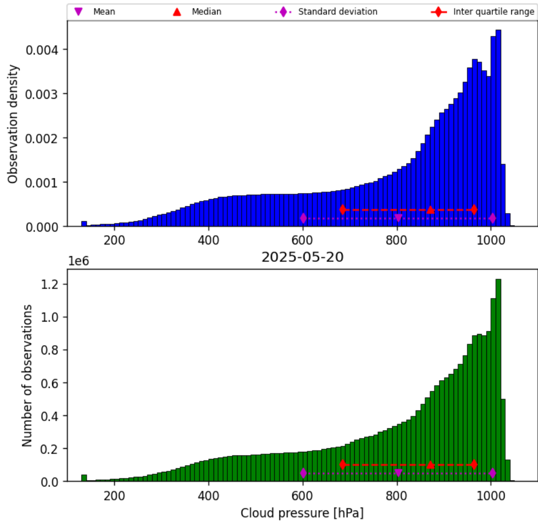
Figure 28: Histogram of “Cloud pressure” for 2025-05-20 to 2025-05-21
