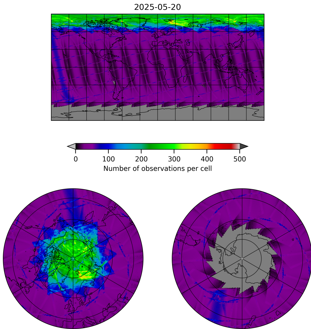
Figure 9: Map of the number of observations for 2025-05-20 to 2025-05-21
