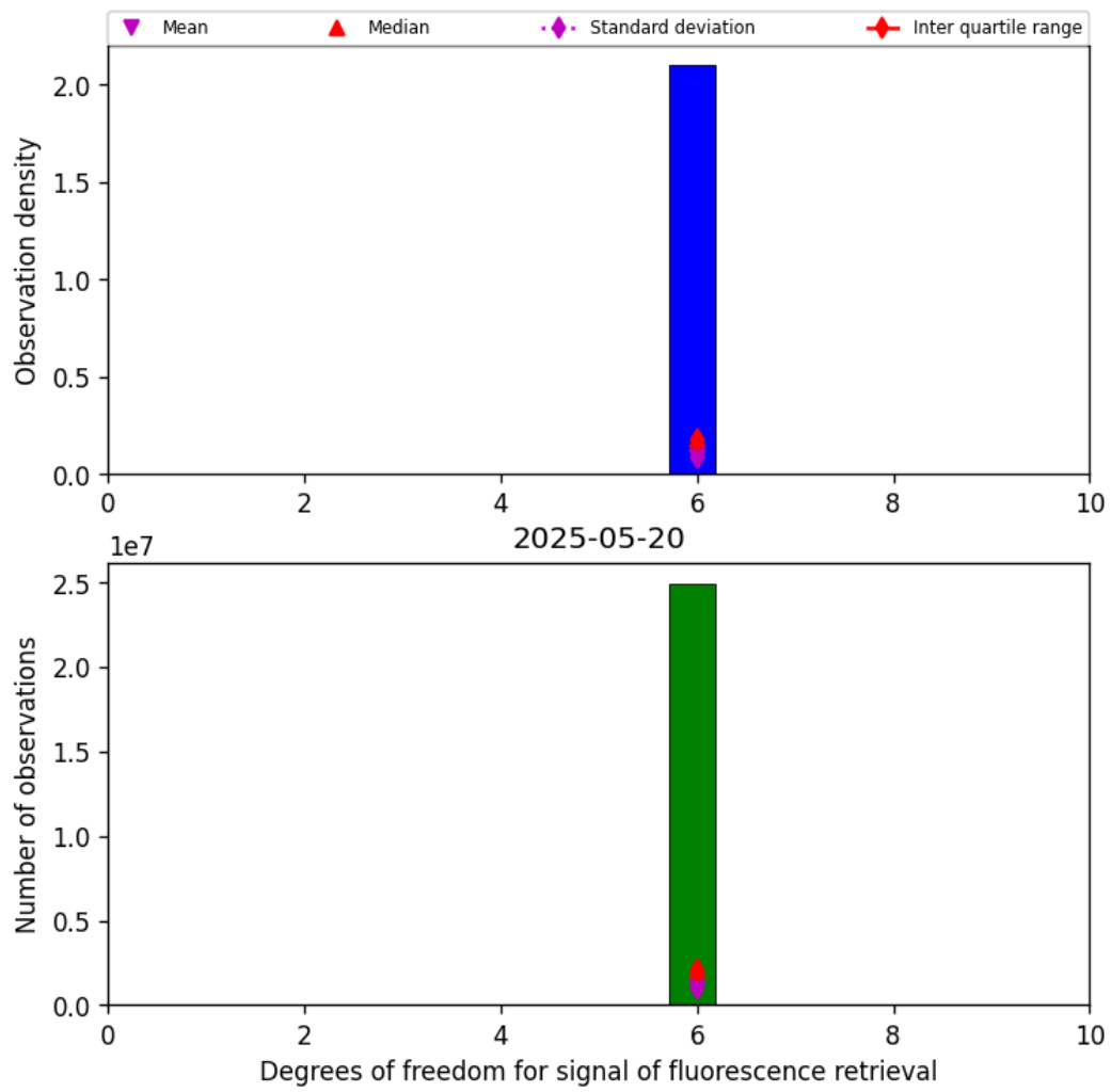
Figure 41: Histogram of “Degrees of freedom for signal of fluorescence retrieval” for 2025-05-20 to 2025-05-21
