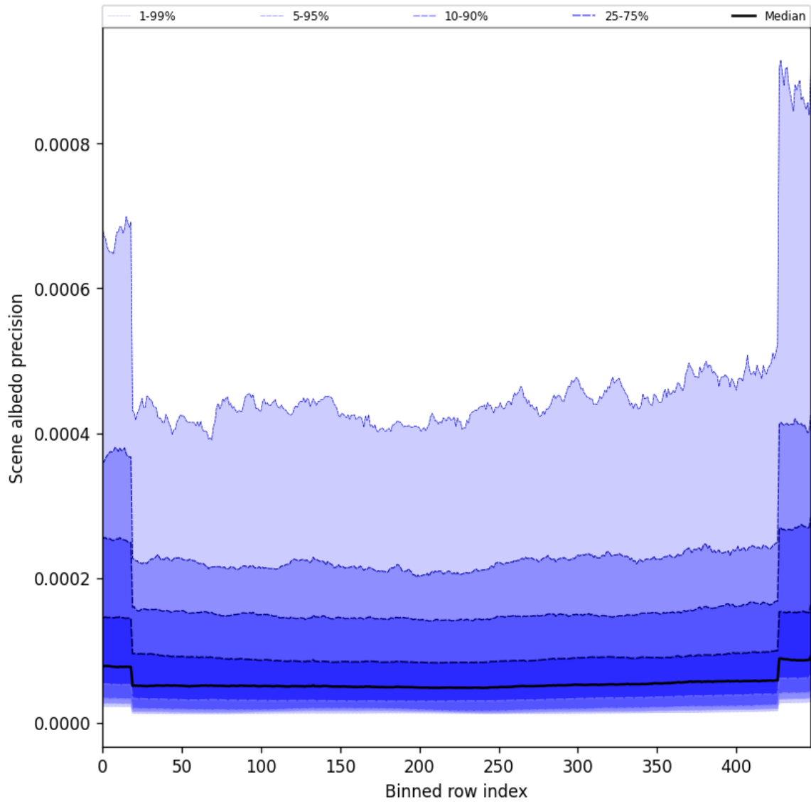
Figure 50: Along track statistics of “Scene albedo precision” for 2025-05-20 to 2025-05-21
