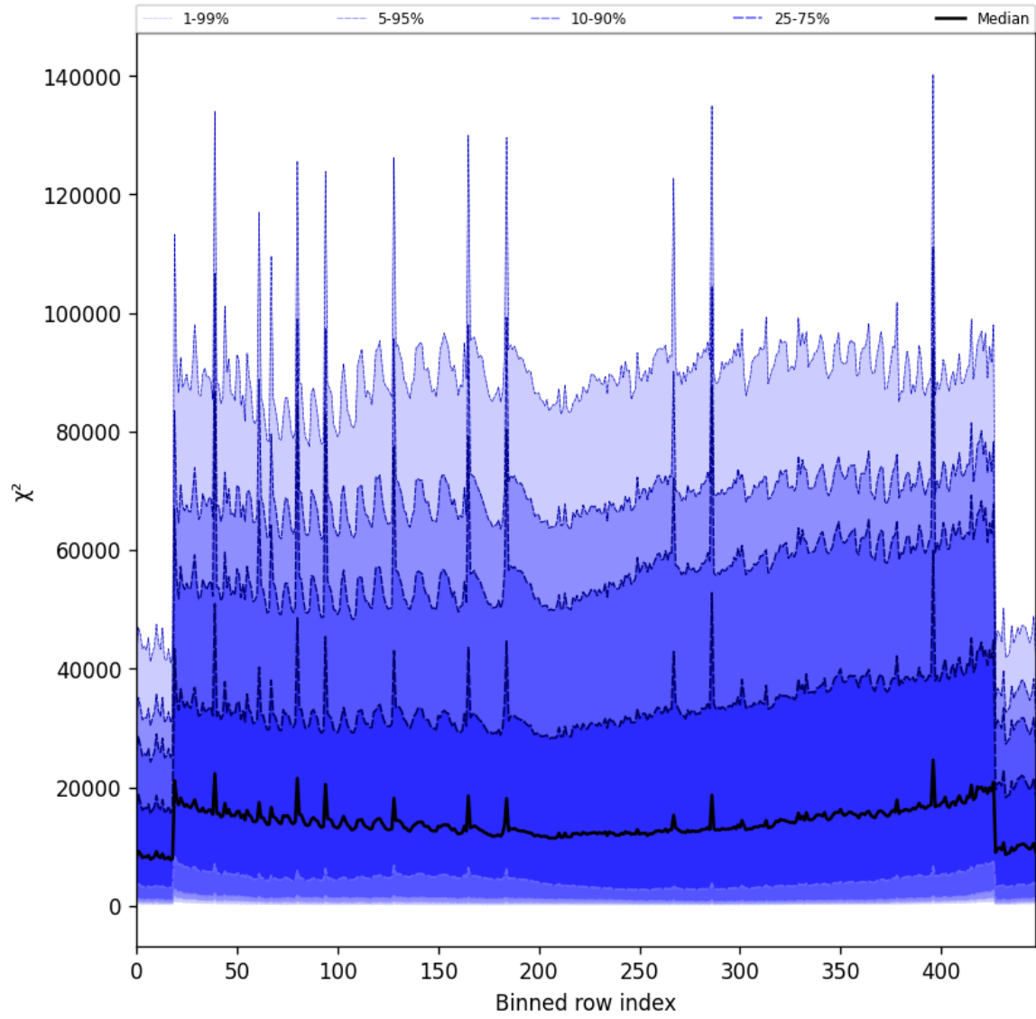
Figure 53: Along track statistics of “ \chi^2 ” for 2025-05-20 to 2025-05-21
