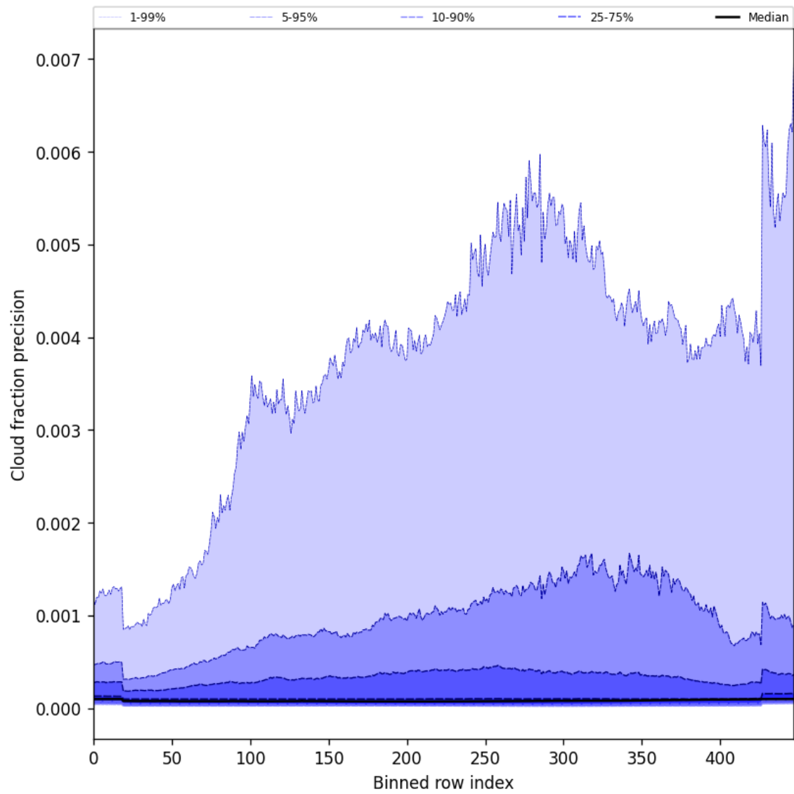
Figure 48: Along track statistics of “Cloud fraction precision” for 2025-05-20 to 2025-05-21
