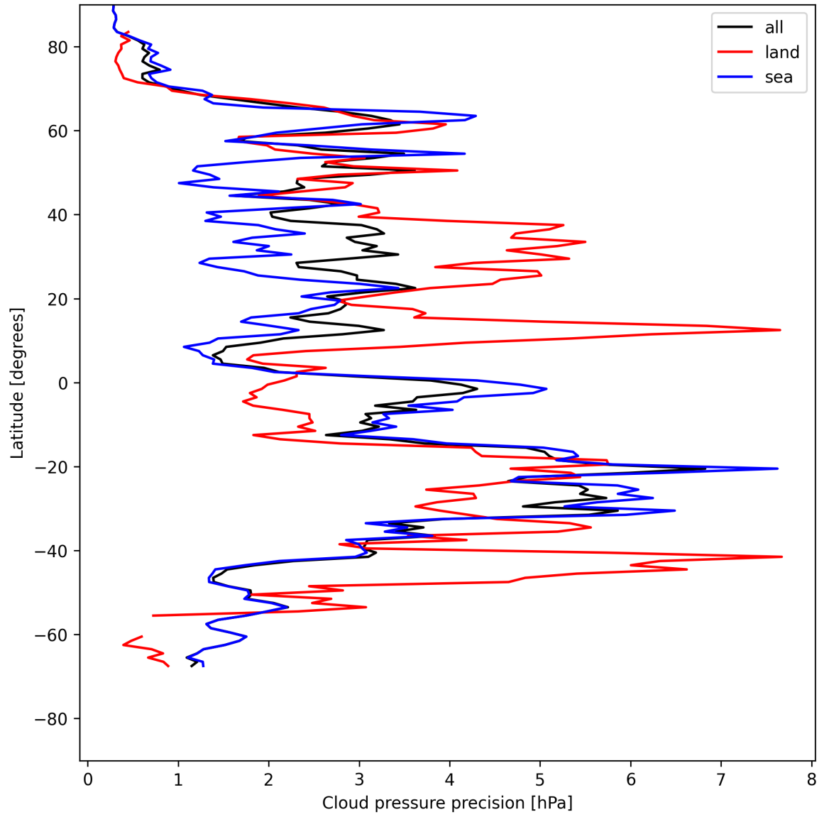
Figure 12: Zonal average of “Cloud pressure precision” for 2025-05-20 to 2025-05-21.
