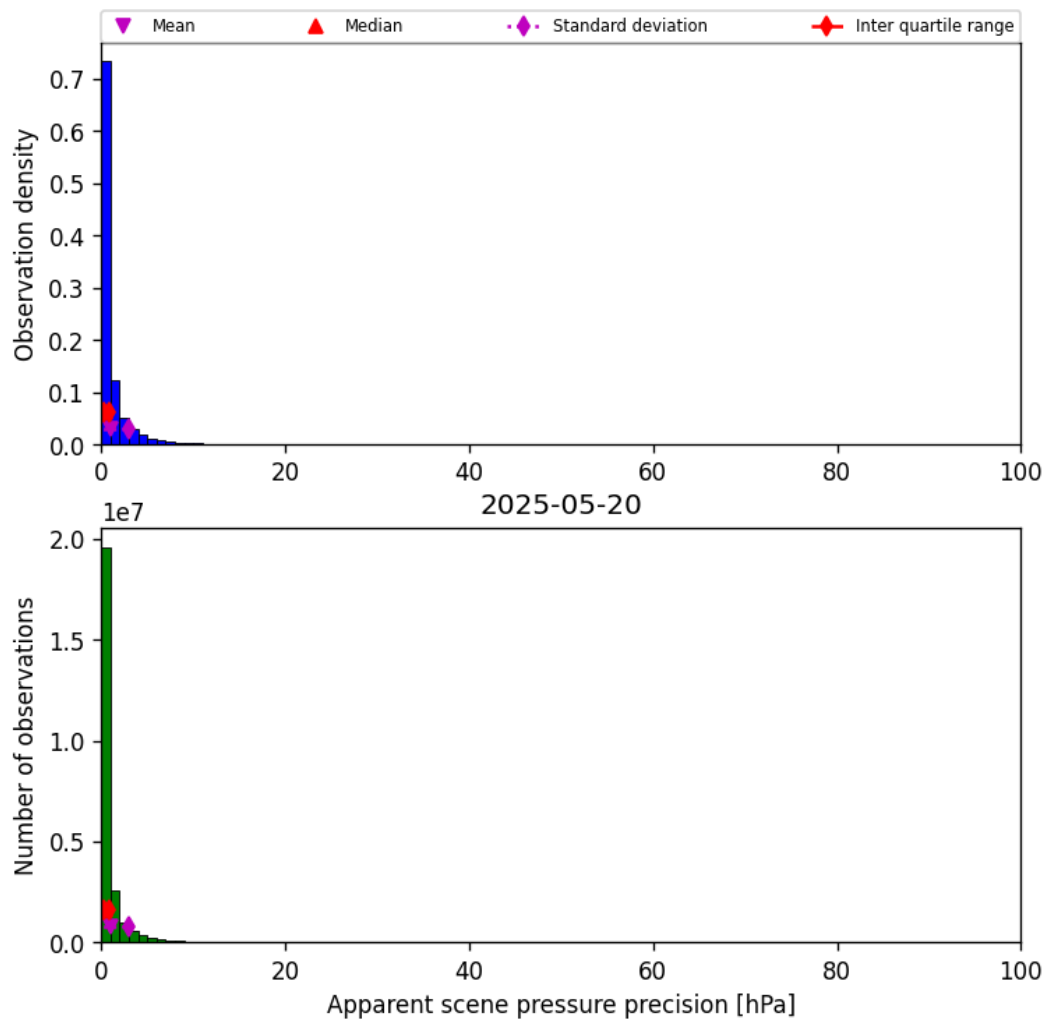
Figure 35: Histogram of “Apparent scene pressure precision” for 2025-05-20 to 2025-05-21
