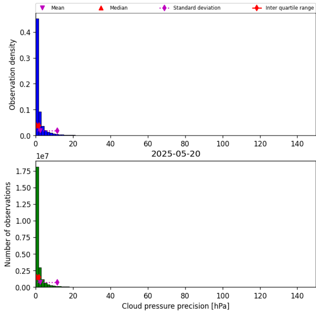
Figure 29: Histogram of “Cloud pressure precision” for 2025-05-20 to 2025-05-21
