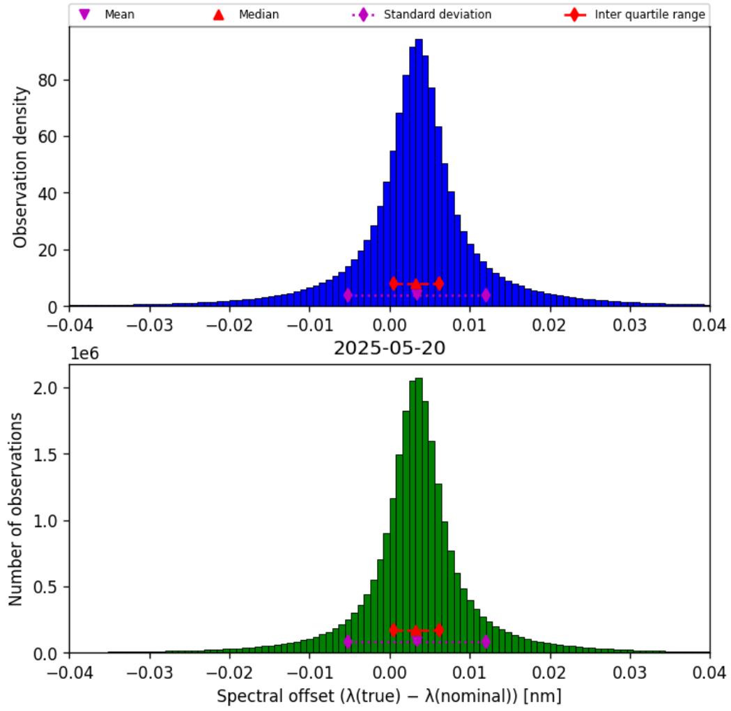
Figure 43: Histogram of “Spectral offset ( \lambda_{\text{true}} - \lambda_{\text{nominal}} )” for 2025-05-20 to 2025-05-21
