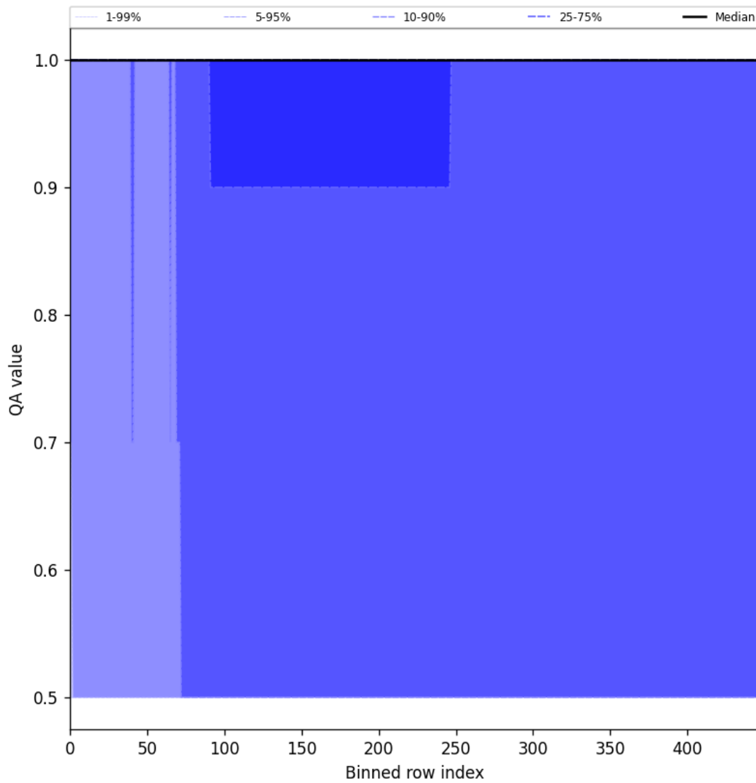
Figure 44: Along track statistics of “QA value” for 2025-05-20 to 2025-05-21
