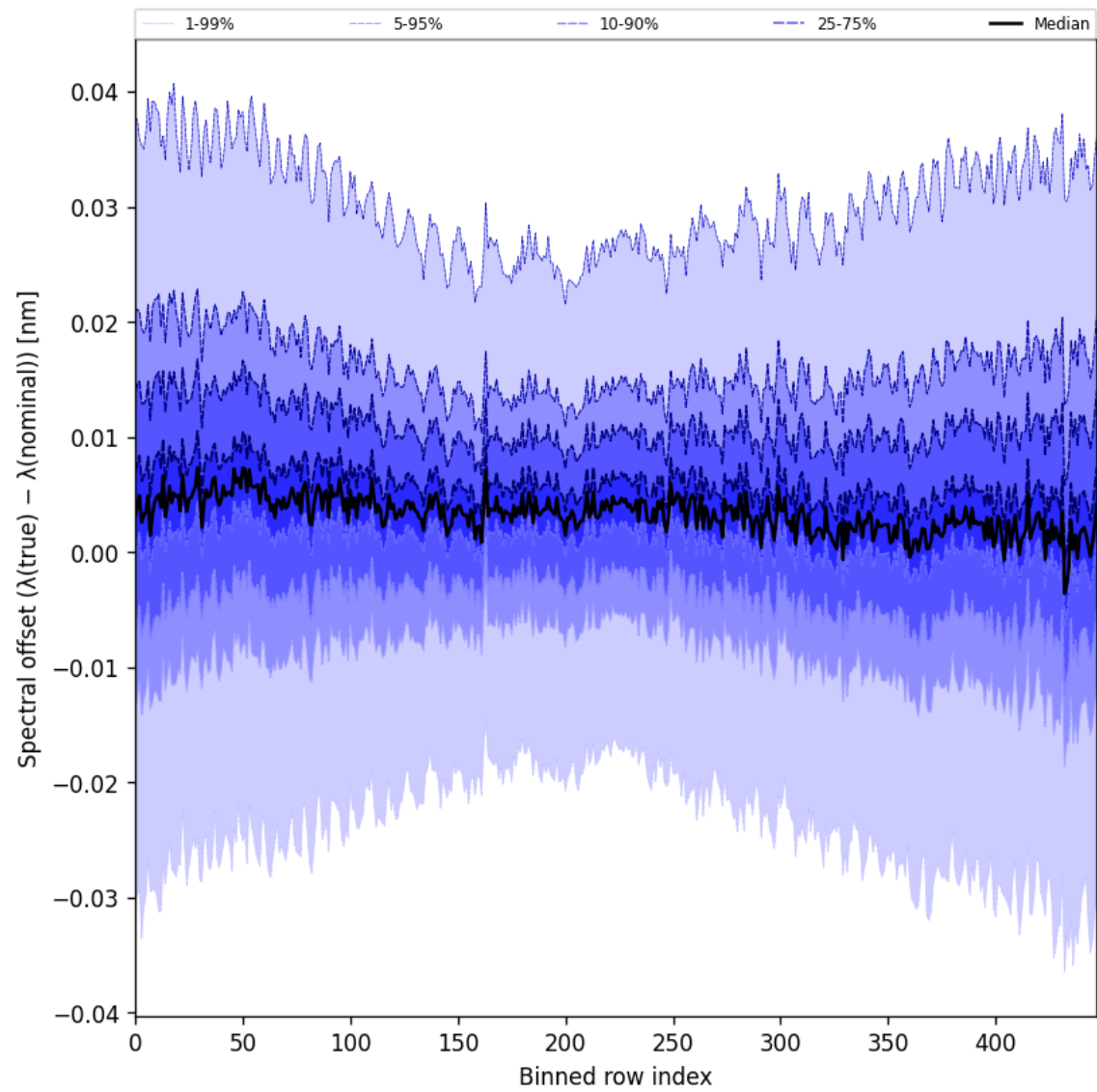
Figure 60: Along track statistics of “Spectral offset ( \lambda_{\text{true}} - \lambda_{\text{nominal}} )” for 2025-05-20 to 2025-05-21
