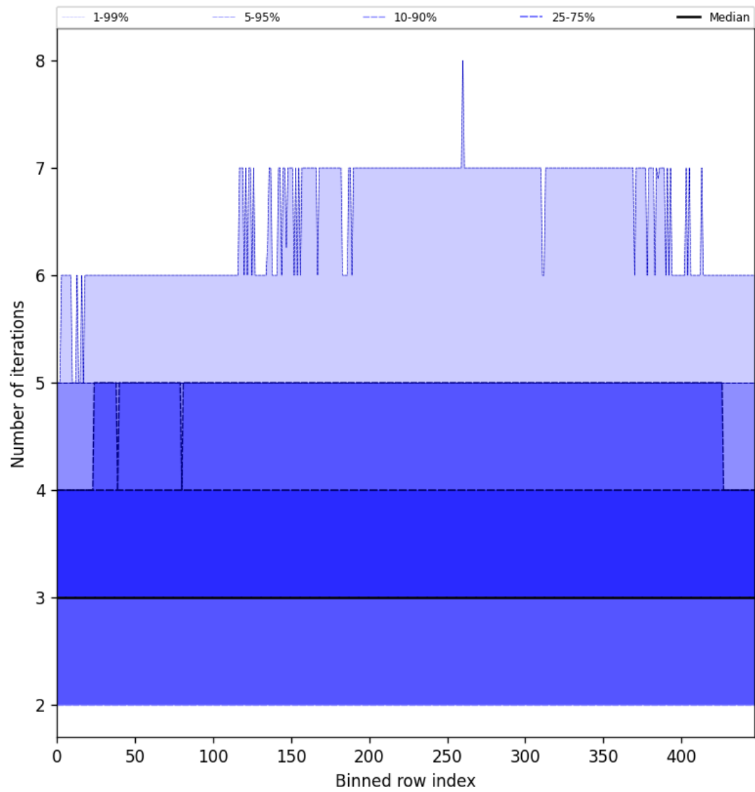
Figure 54: Along track statistics of “Number of iterations” for 2025-05-20 to 2025-05-21
