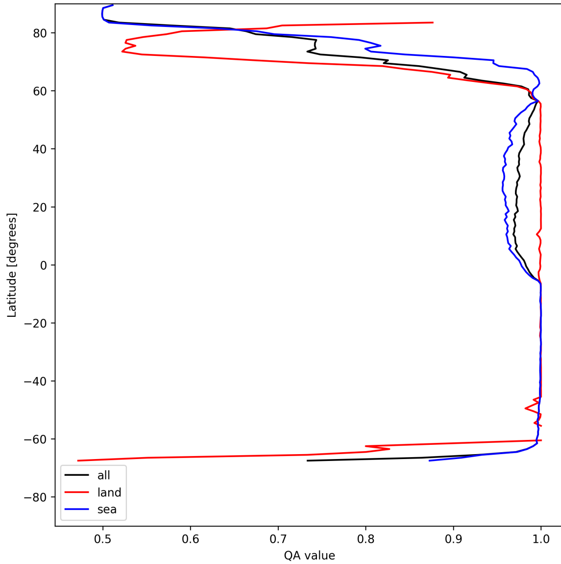
Figure 10: Zonal average of “QA value” for 2025-05-20 to 2025-05-21.
