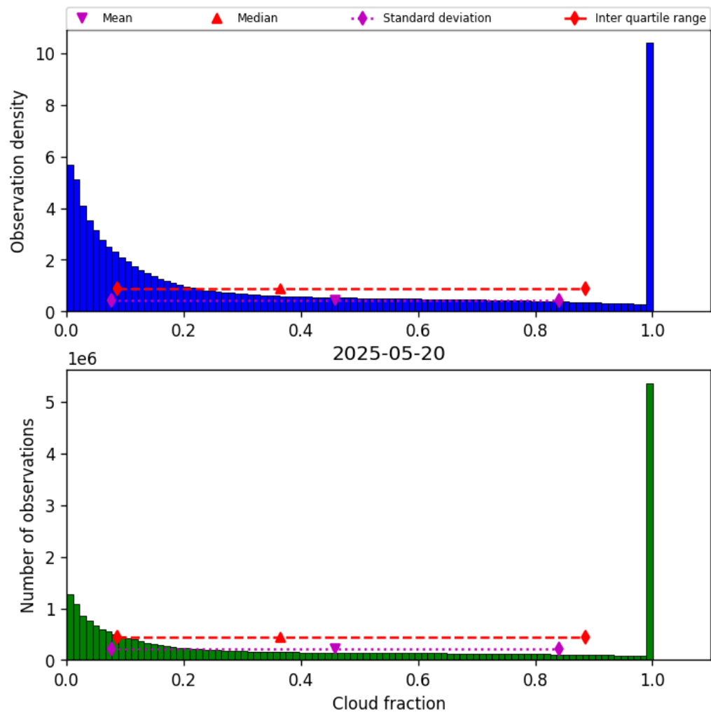
Figure 30: Histogram of “Cloud fraction” for 2025-05-20 to 2025-05-21
