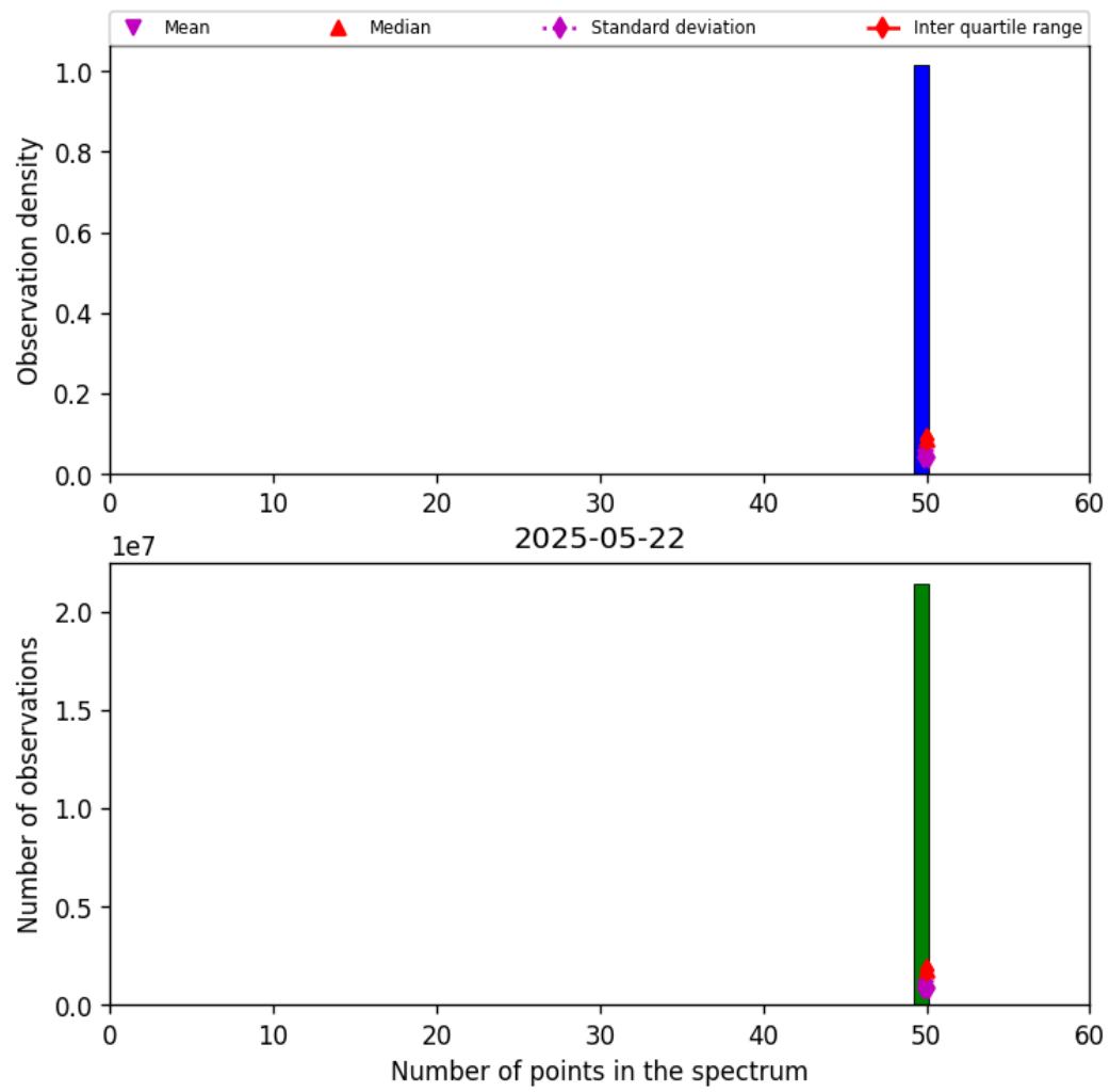
Figure 42: Histogram of “Number of points in the spectrum” for 2025-05-22 to 2025-05-23
