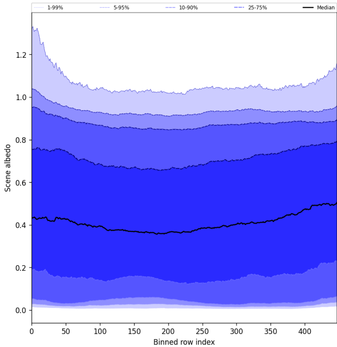
Figure 49: Along track statistics of “Scene albedo” for 2025-05-22 to 2025-05-23
