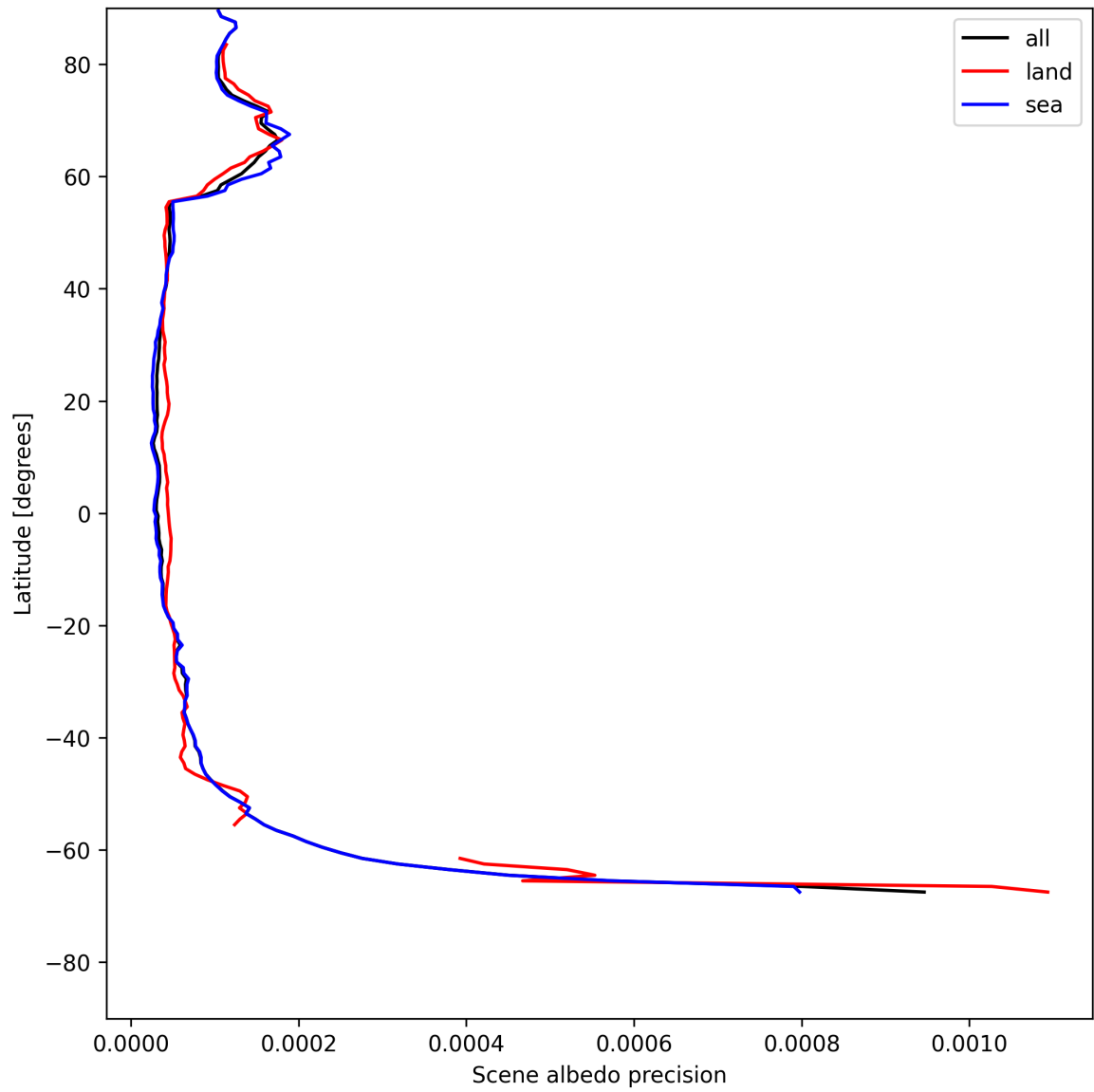
Figure 16: Zonal average of “Scene albedo precision” for 2025-05-22 to 2025-05-23.
