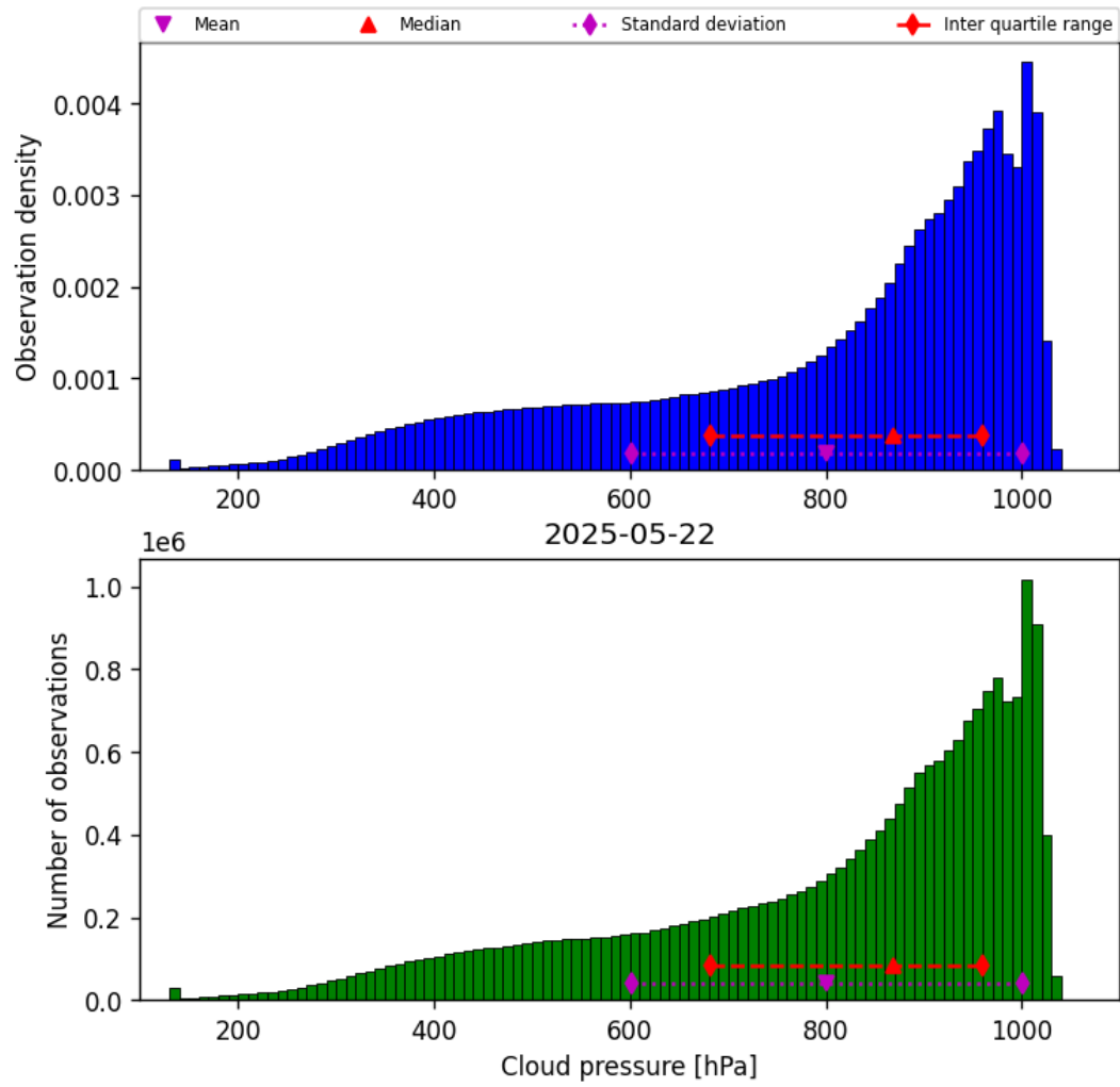
Figure 28: Histogram of “Cloud pressure” for 2025-05-22 to 2025-05-23
