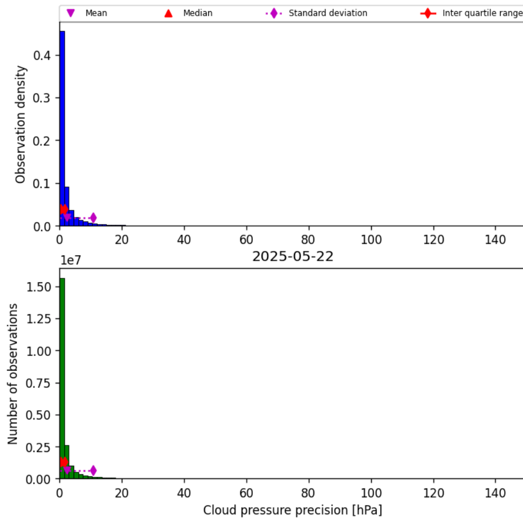
Figure 29: Histogram of “Cloud pressure precision” for 2025-05-22 to 2025-05-23
