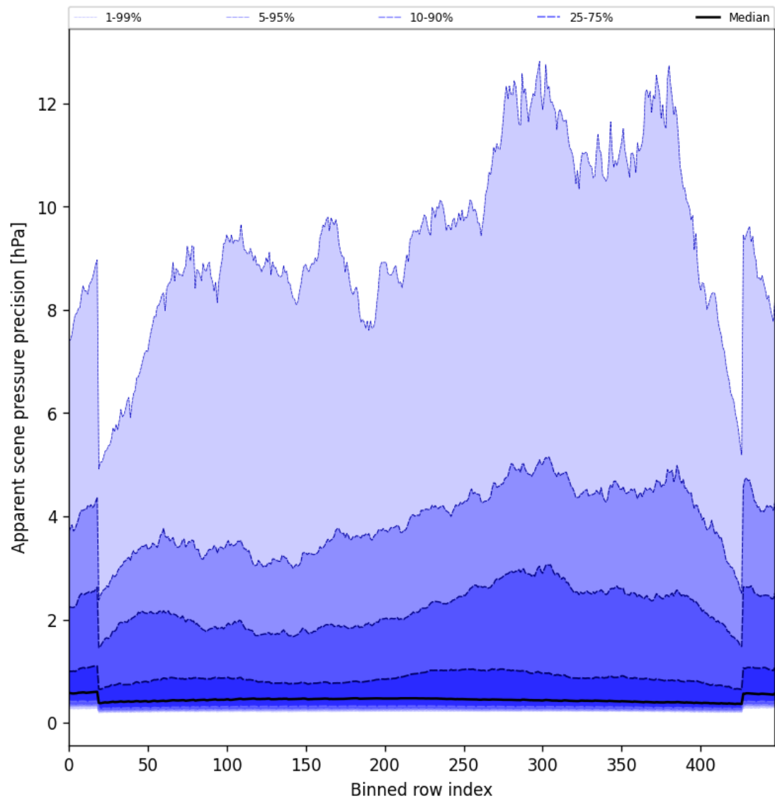
Figure 52: Along track statistics of “Apparent scene pressure precision” for 2025-05-22 to 2025-05-23
