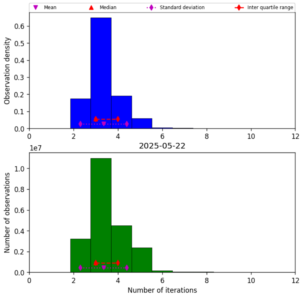
Figure 37: Histogram of “Number of iterations” for 2025-05-22 to 2025-05-23
