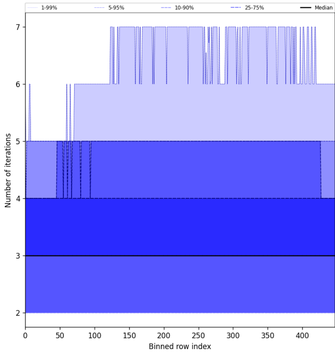
Figure 54: Along track statistics of “Number of iterations” for 2025-05-22 to 2025-05-23
