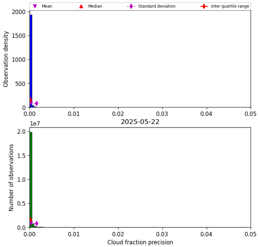
Figure 31: Histogram of “Cloud fraction precision” for 2025-05-22 to 2025-05-23
