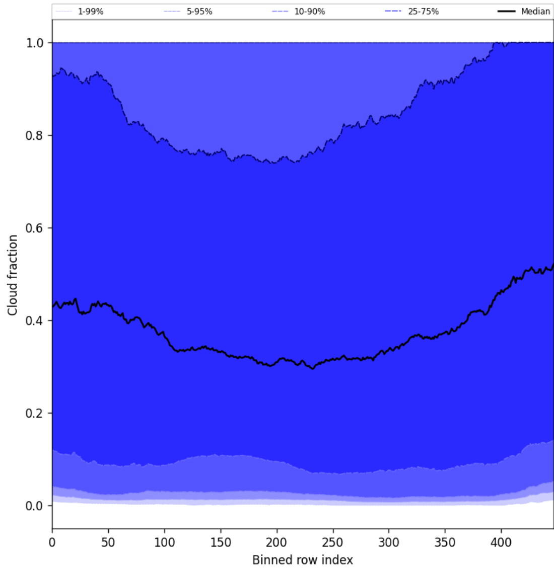
Figure 47: Along track statistics of “Cloud fraction” for 2025-05-22 to 2025-05-23
