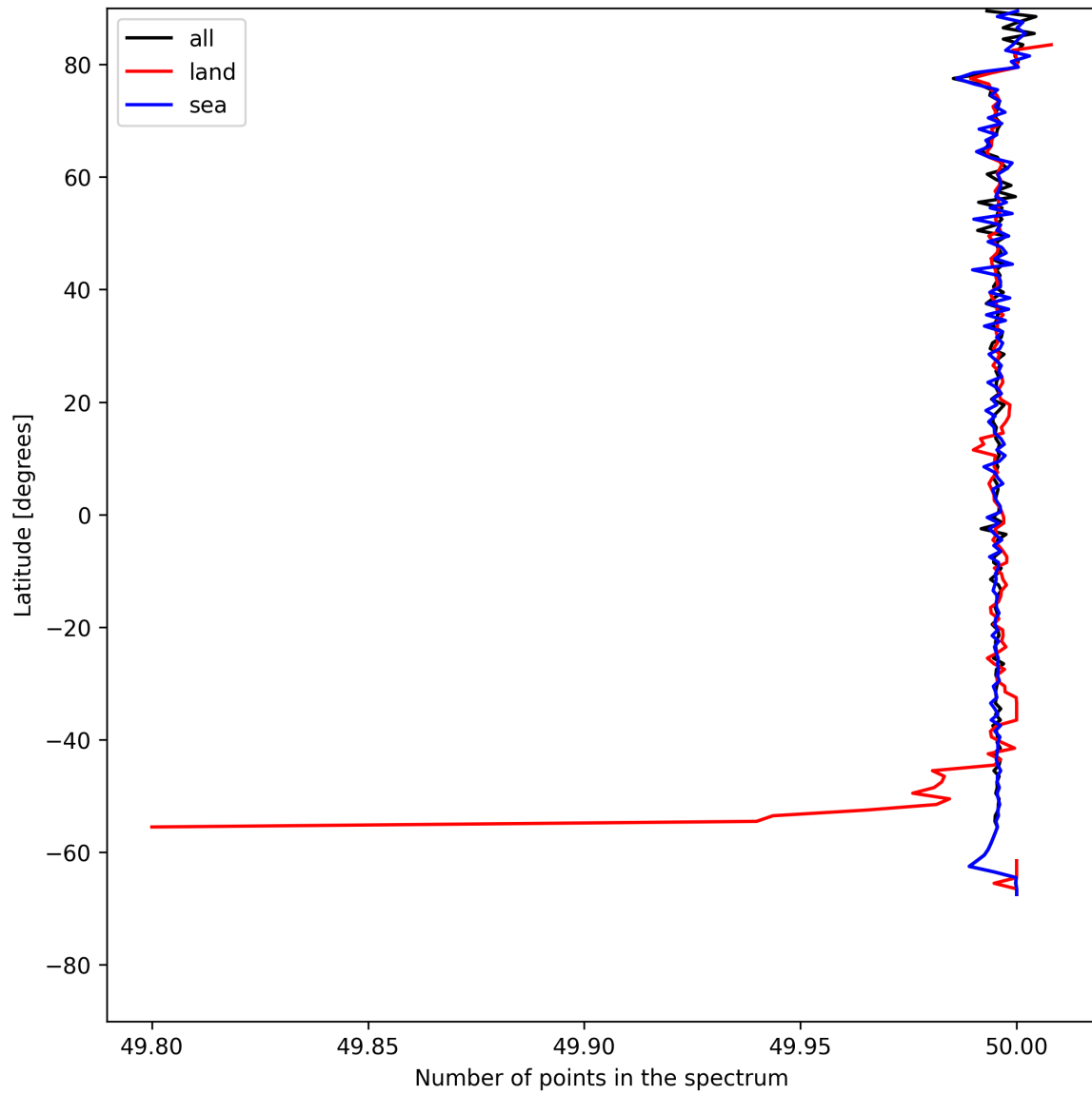
Figure 25: Zonal average of “Number of points in the spectrum” for 2025-05-22 to 2025-05-23.
