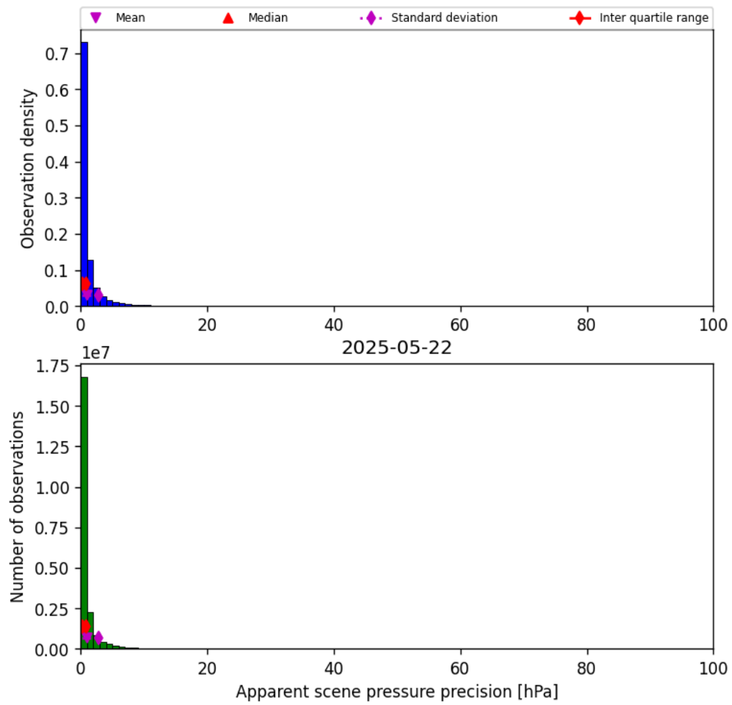
Figure 35: Histogram of “Apparent scene pressure precision” for 2025-05-22 to 2025-05-23
