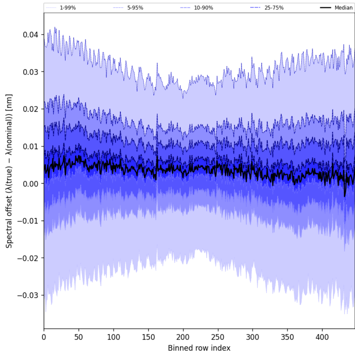
Figure 60: Along track statistics of “Spectral offset ( \lambda_{\text{true}} - \lambda_{\text{nominal}} )” for 2025-05-22 to 2025-05-23
