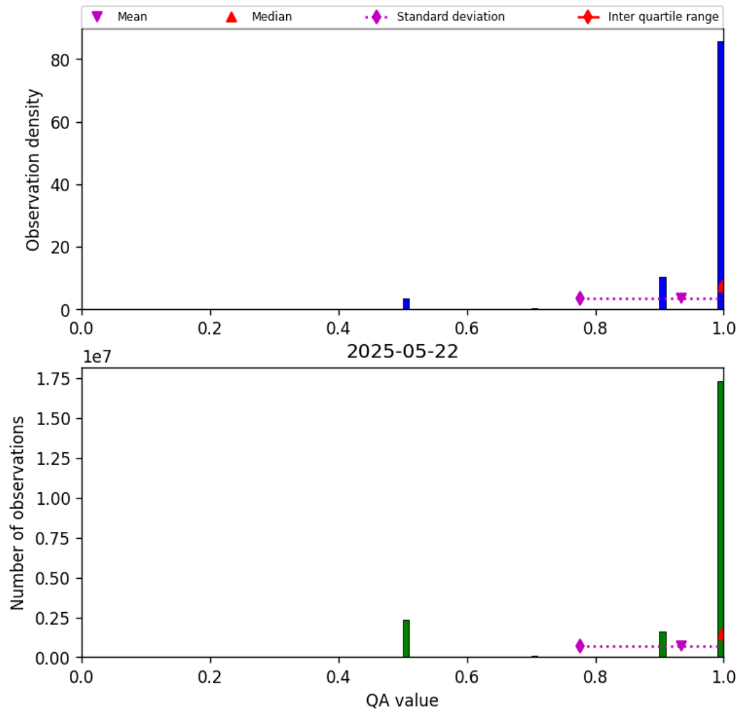
Figure 27: Histogram of “QA value” for 2025-05-22 to 2025-05-23
