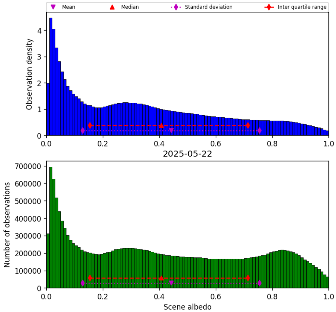
Figure 32: Histogram of “Scene albedo” for 2025-05-22 to 2025-05-23
