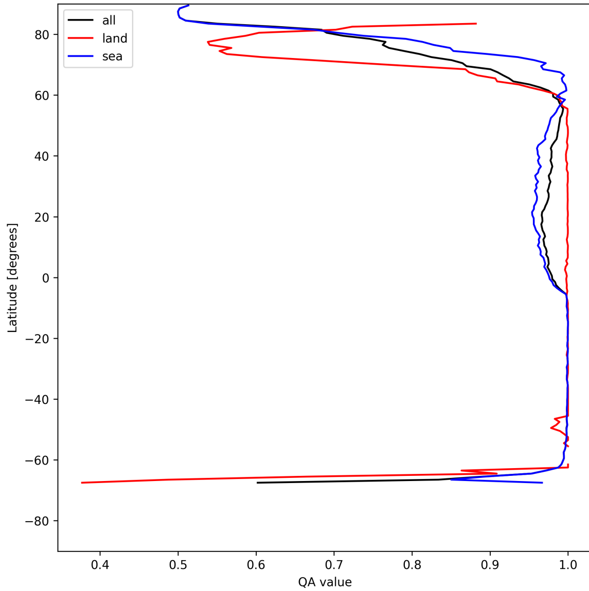
Figure 10: Zonal average of “QA value” for 2025-05-22 to 2025-05-23.
