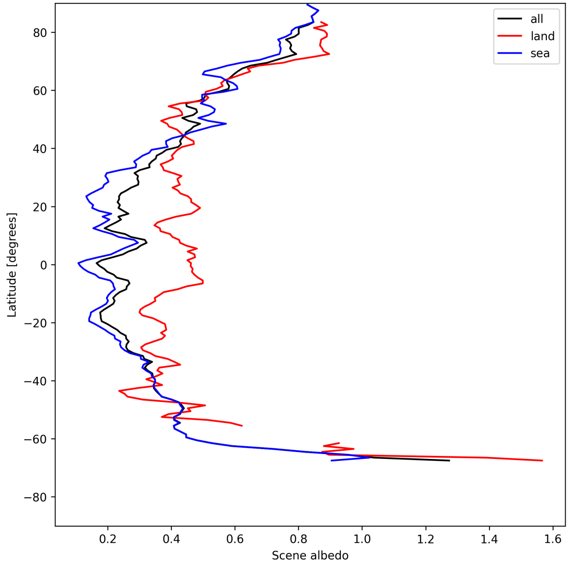
Figure 15: Zonal average of “Scene albedo” for 2025-05-22 to 2025-05-23.
