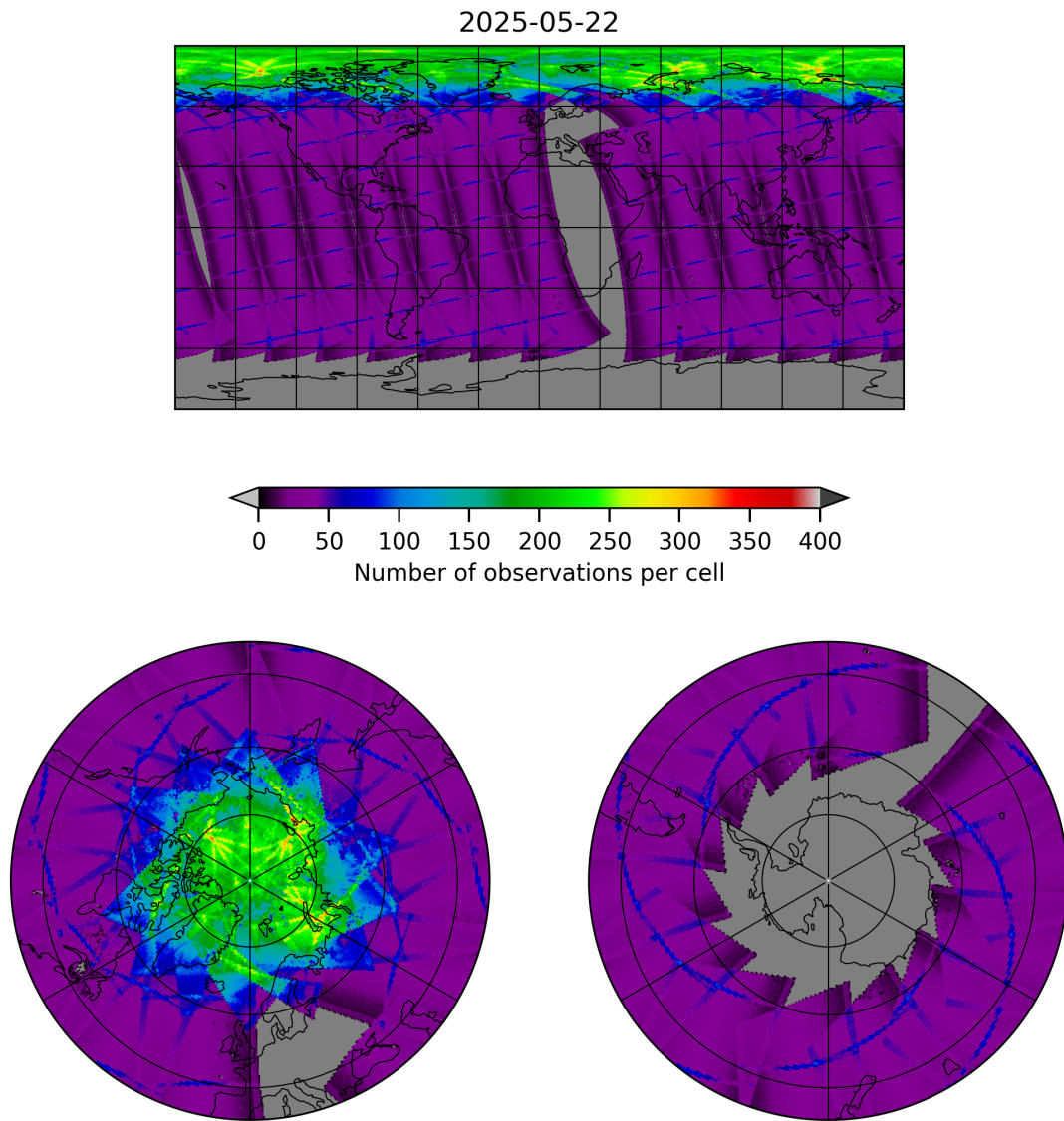
Figure 9: Map of the number of observations for 2025-05-22 to 2025-05-23
