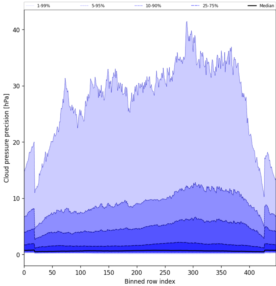
Figure 46: Along track statistics of “Cloud pressure precision” for 2025-05-22 to 2025-05-23
