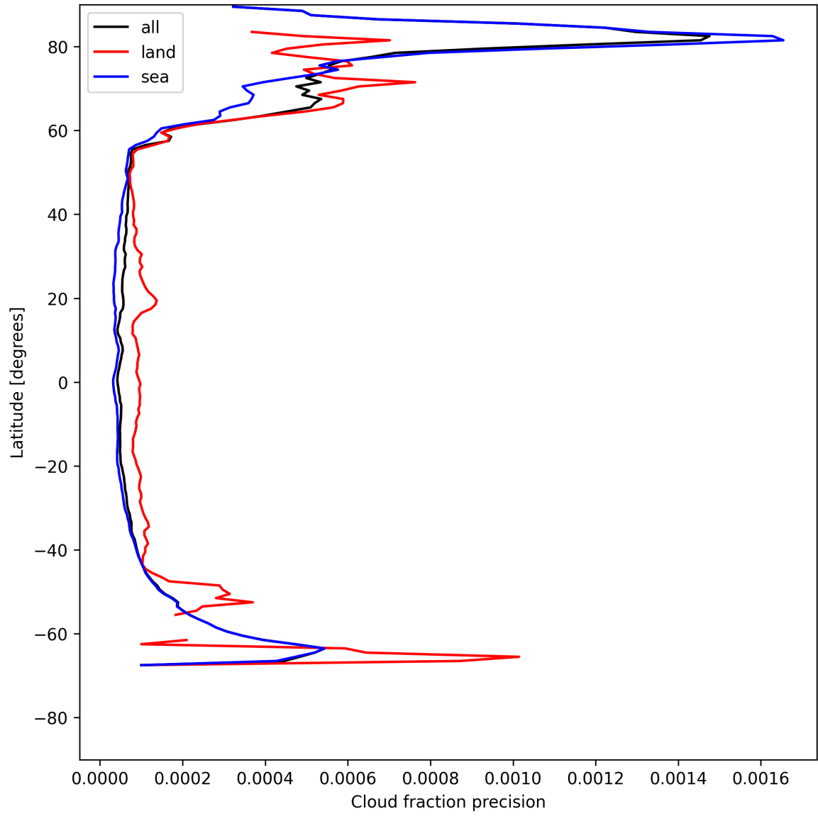
Figure 14: Zonal average of “Cloud fraction precision” for 2025-05-22 to 2025-05-23.
