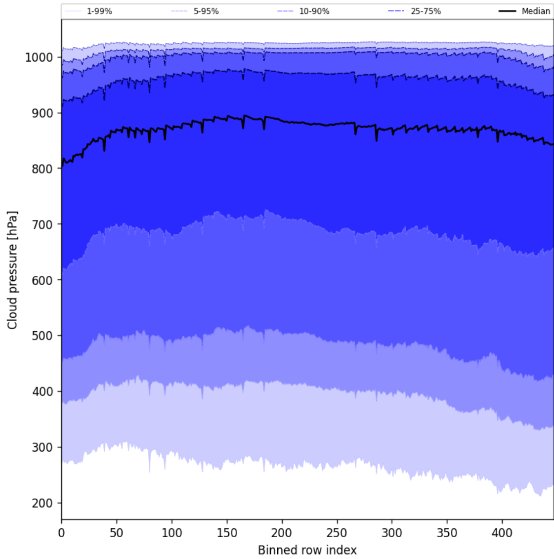
Figure 45: Along track statistics of “Cloud pressure” for 2025-05-22 to 2025-05-23
