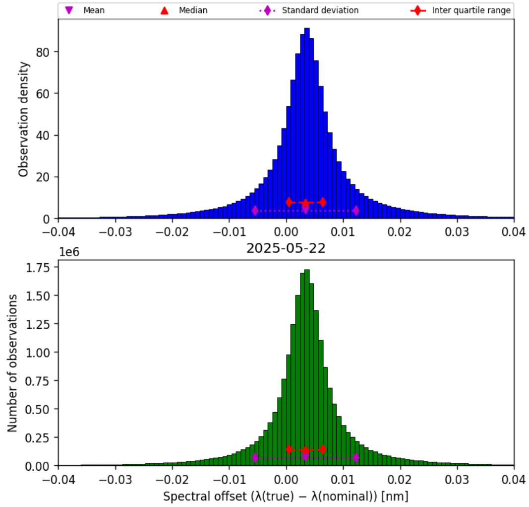
Figure 43: Histogram of “Spectral offset ( \lambda_{\text{true}} - \lambda_{\text{nominal}} )” for 2025-05-22 to 2025-05-23
