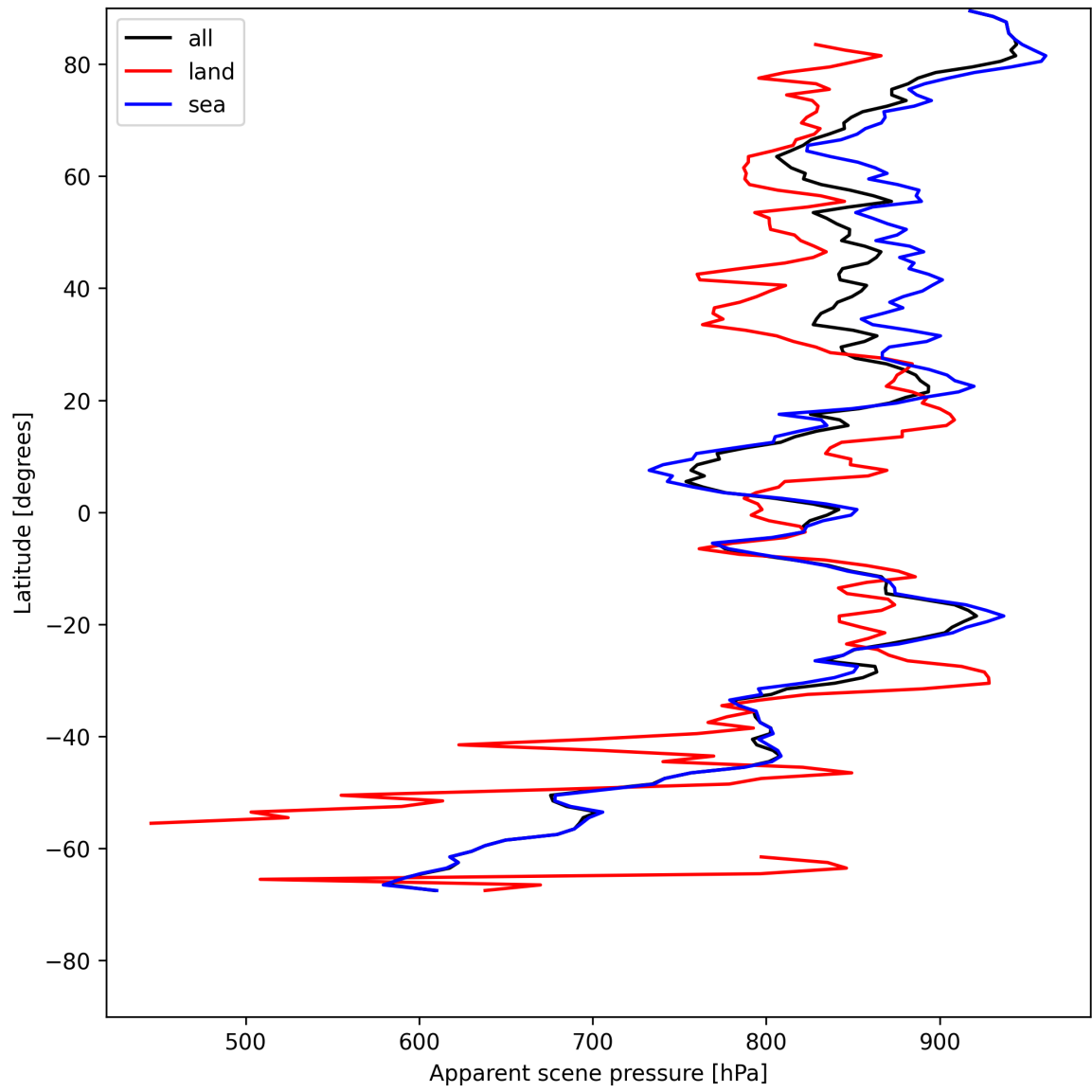
Figure 17: Zonal average of “Apparent scene pressure” for 2025-05-22 to 2025-05-23.
