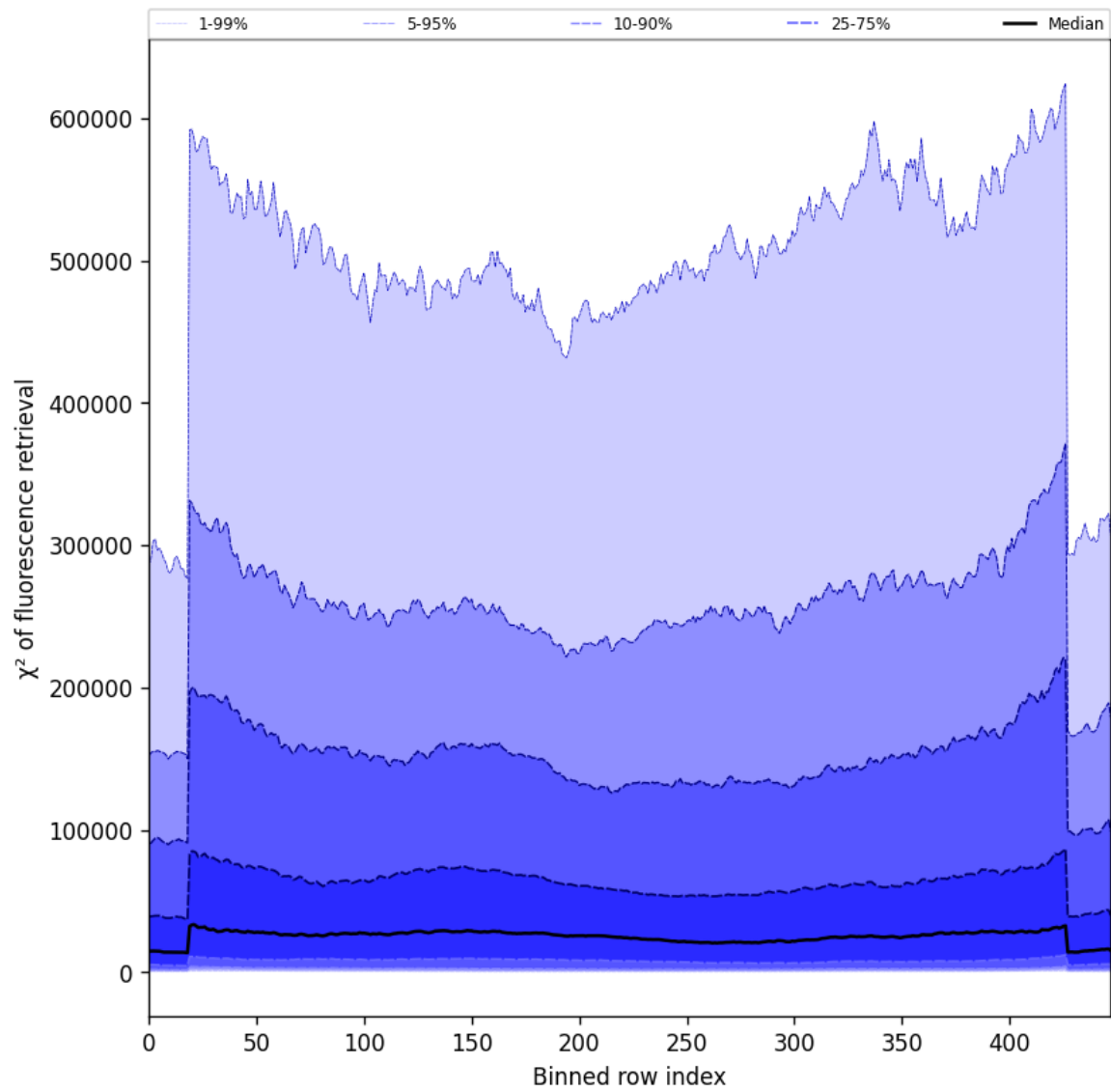
Figure 57: Along track statistics of “ \chi^2 of fluorescence retrieval” for 2025-05-22 to 2025-05-23
