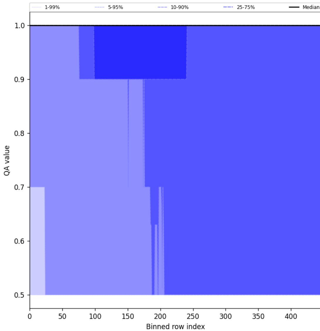
Figure 44: Along track statistics of “QA value” for 2025-05-22 to 2025-05-23
