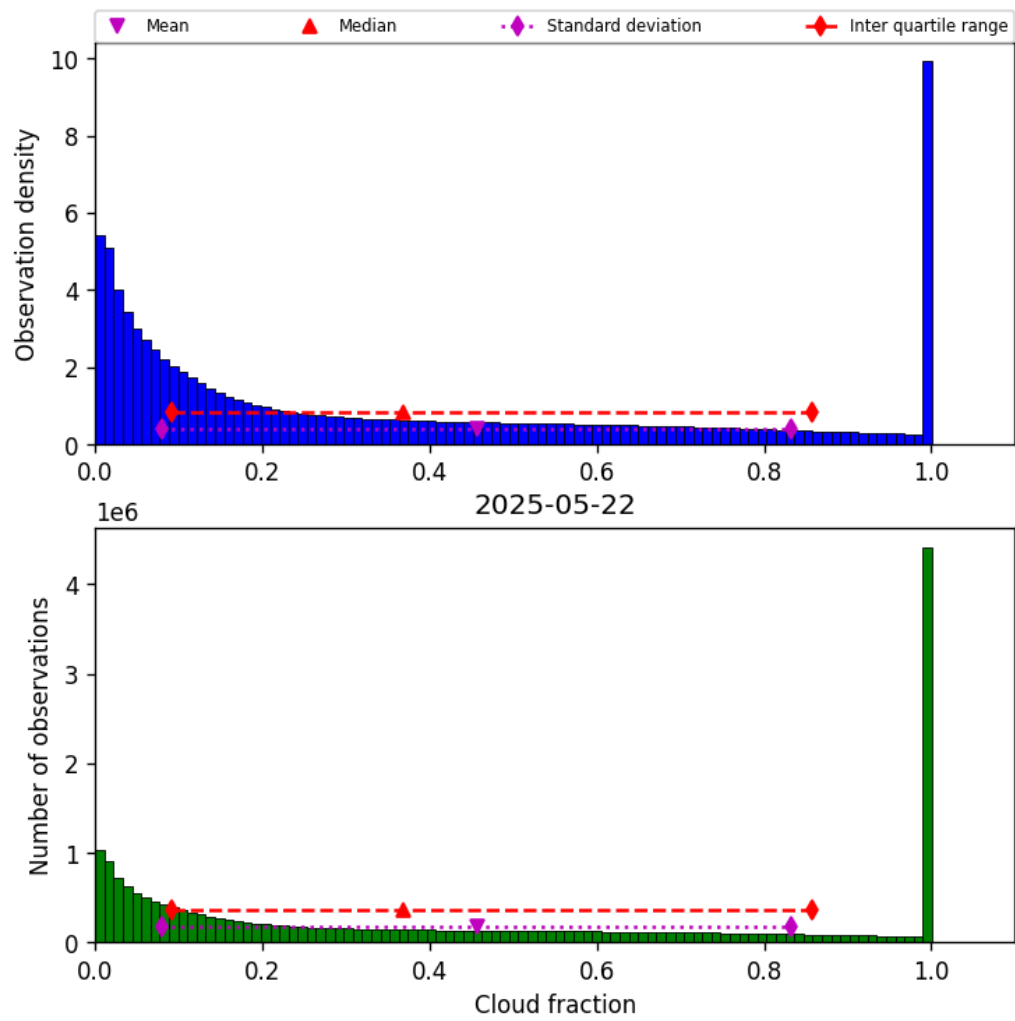
Figure 30: Histogram of “Cloud fraction” for 2025-05-22 to 2025-05-23
