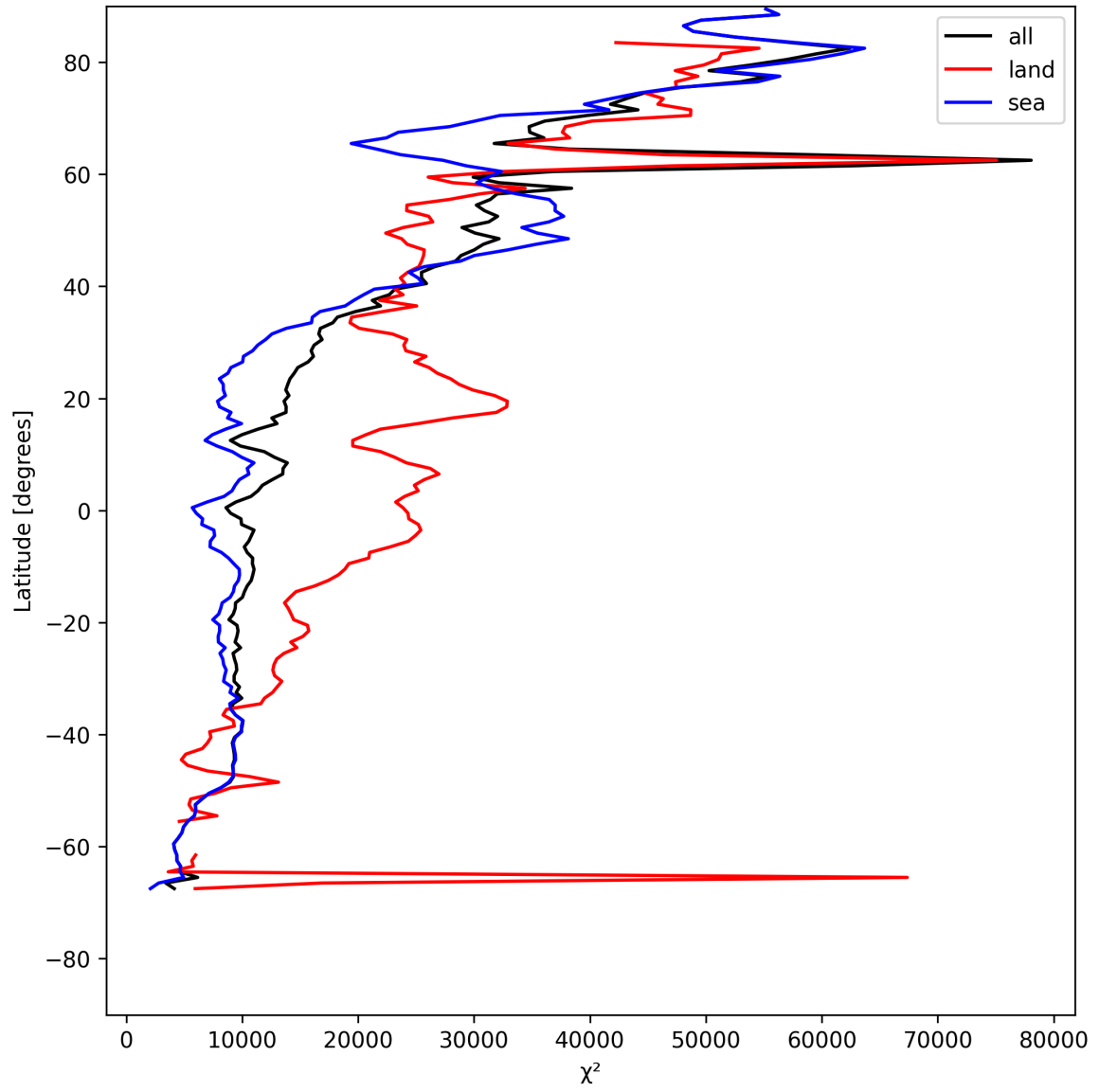
Figure 19: Zonal average of “ \chi^2 ” for 2025-05-22 to 2025-05-23.
