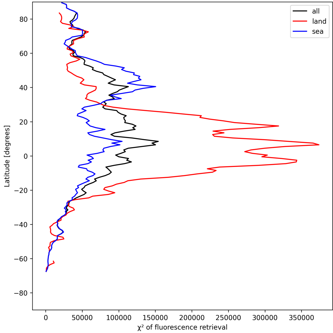
Figure 23: Zonal average of “ \chi^2 of fluorescence retrieval” for 2025-05-22 to 2025-05-23.
