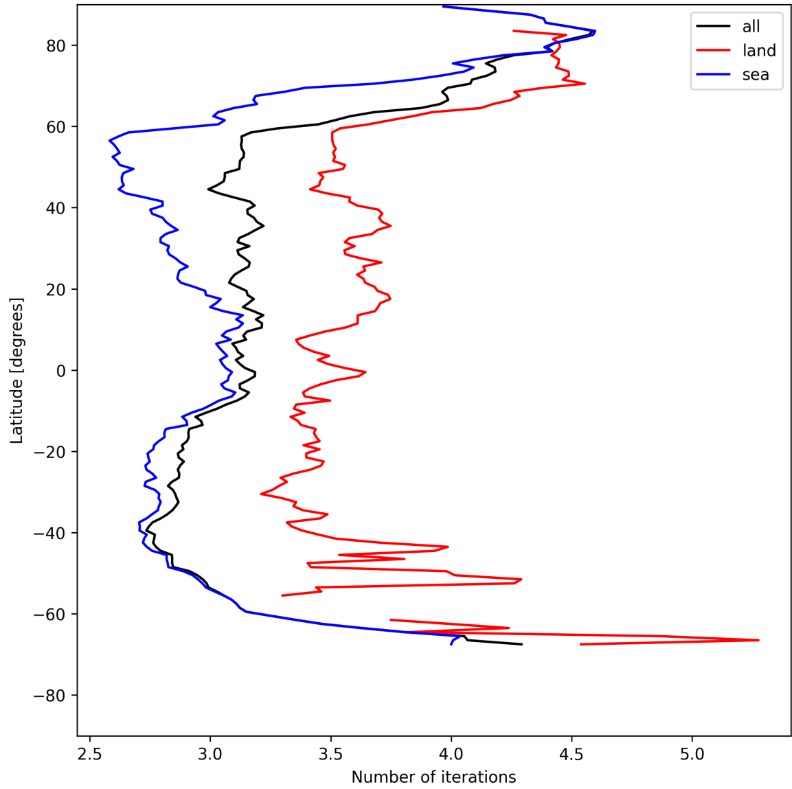
Figure 20: Zonal average of “Number of iterations” for 2025-05-22 to 2025-05-23.
