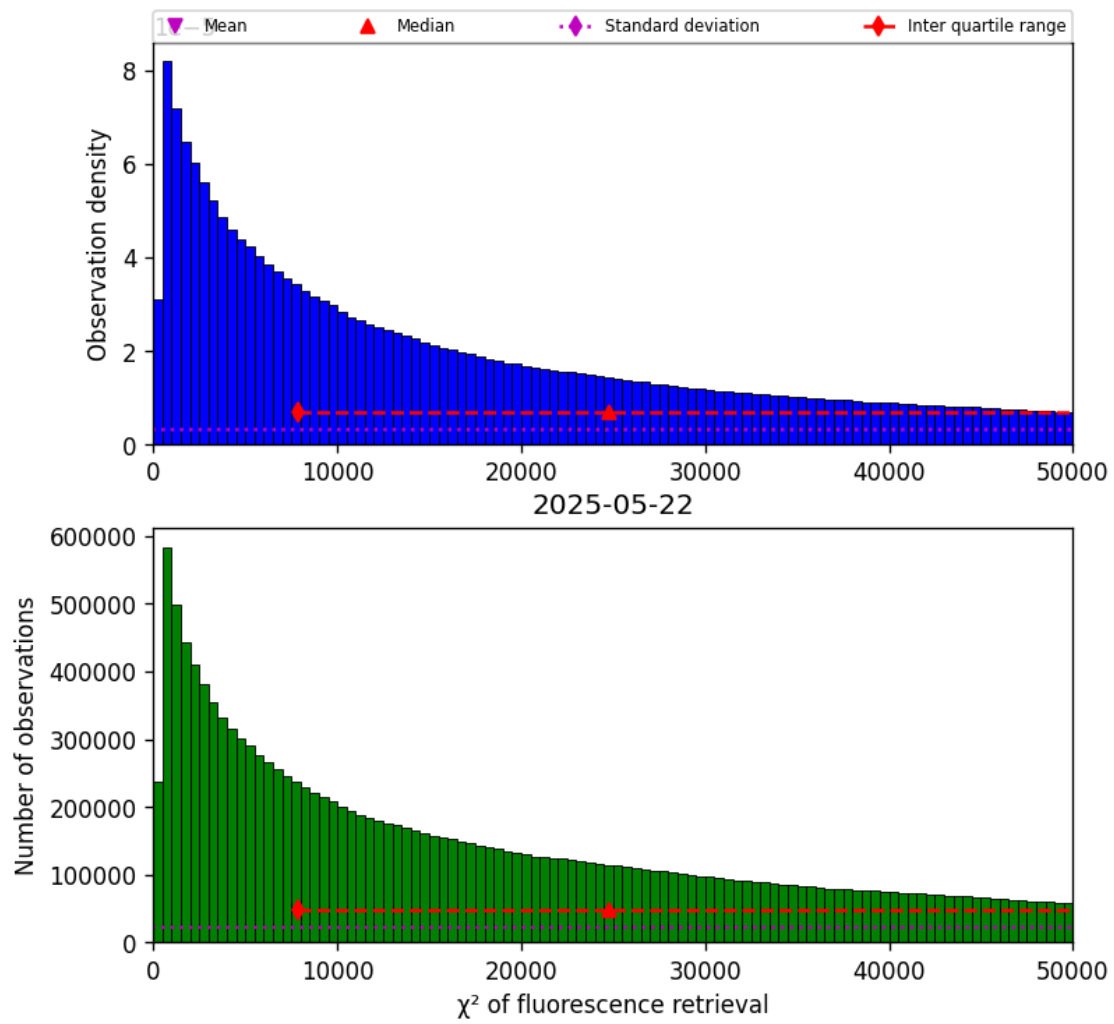
Figure 40: Histogram of “ \chi^2 of fluorescence retrieval” for 2025-05-22 to 2025-05-23
