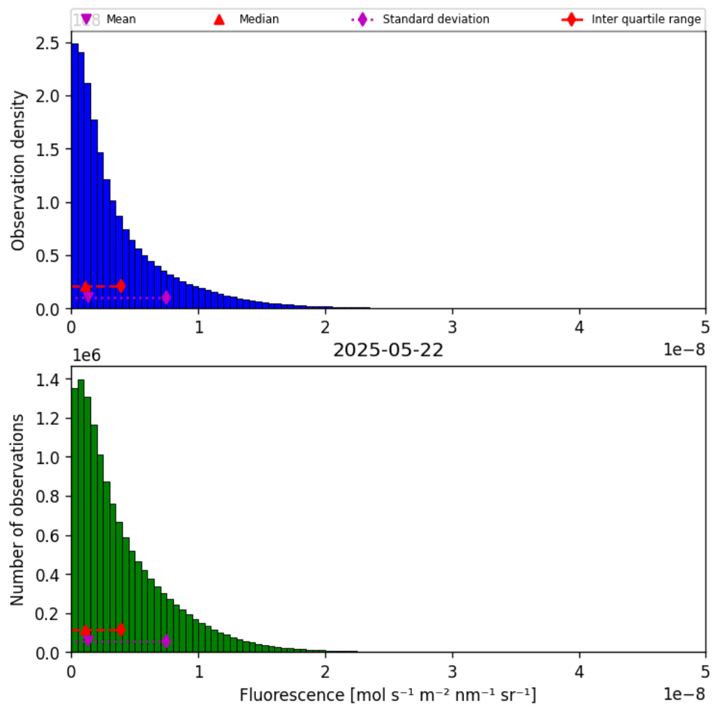
Figure 38: Histogram of “Fluorescence” for 2025-05-22 to 2025-05-23
