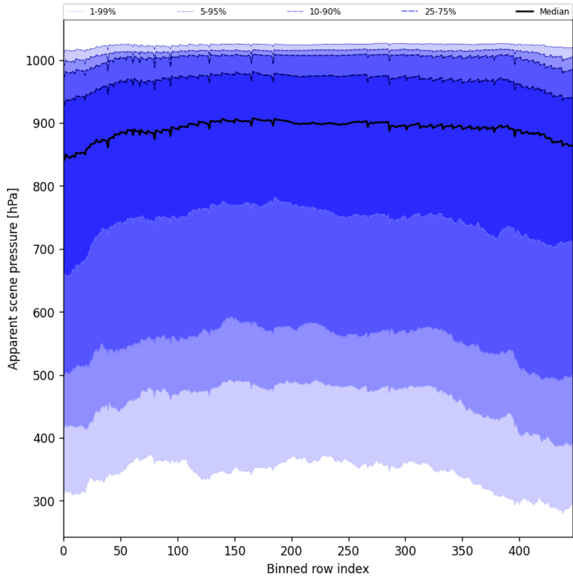
Figure 51: Along track statistics of “Apparent scene pressure” for 2025-05-22 to 2025-05-23
