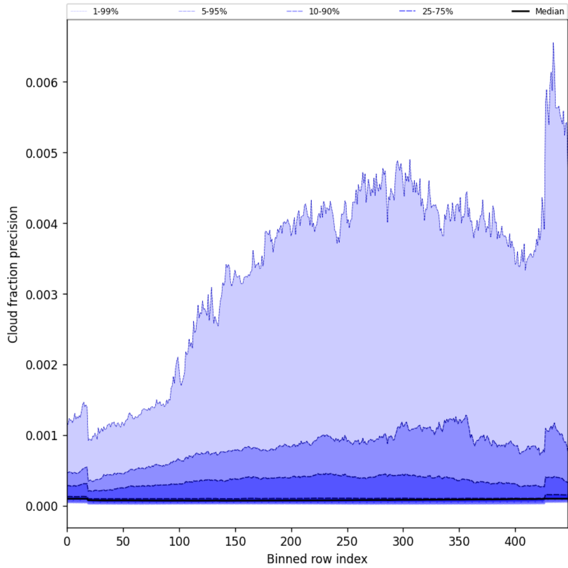
Figure 48: Along track statistics of “Cloud fraction precision” for 2025-05-22 to 2025-05-23
