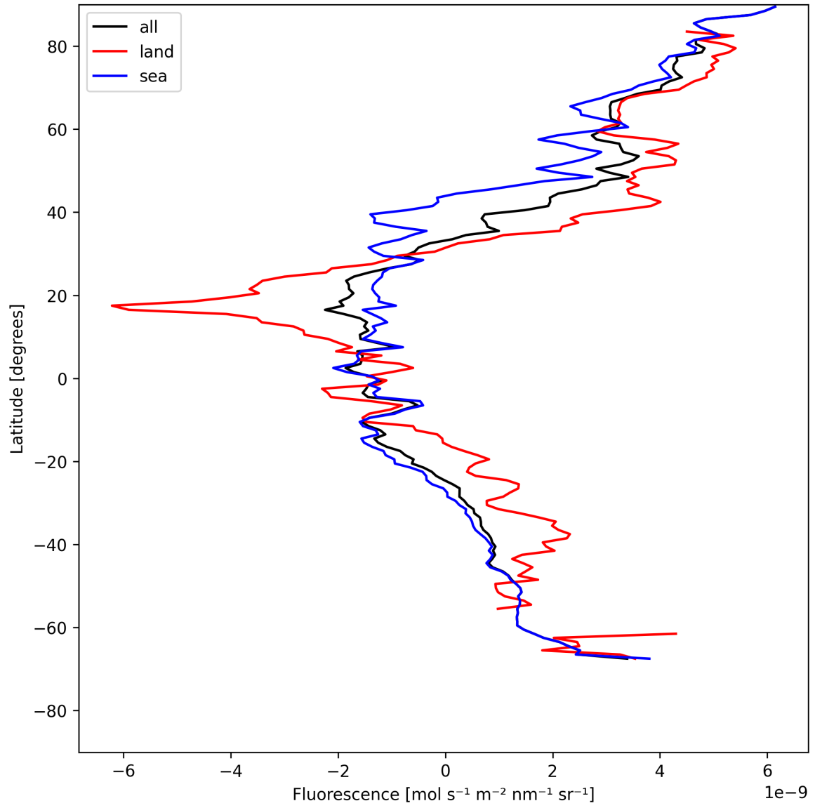
Figure 21: Zonal average of “Fluorescence” for 2025-05-22 to 2025-05-23.
