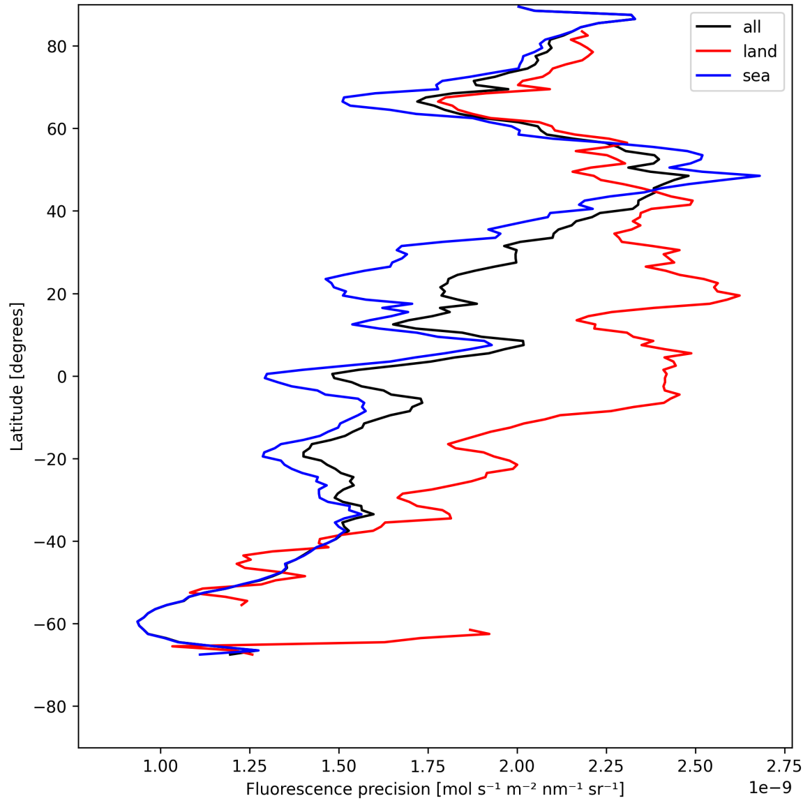
Figure 22: Zonal average of “Fluorescence precision” for 2025-05-22 to 2025-05-23.
