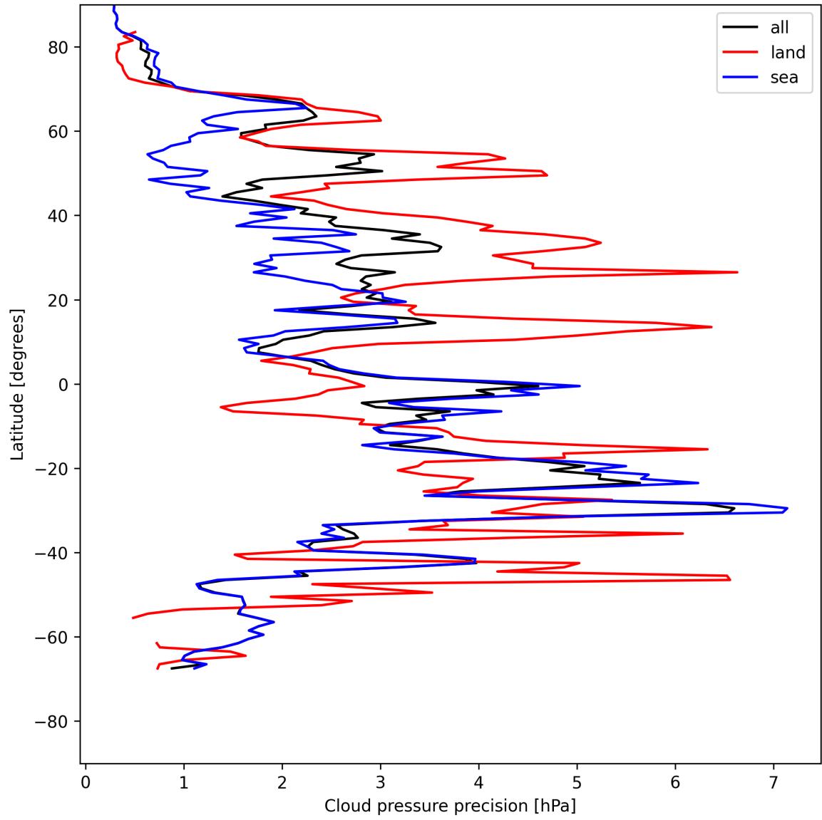
Figure 12: Zonal average of “Cloud pressure precision” for 2025-05-22 to 2025-05-23.
