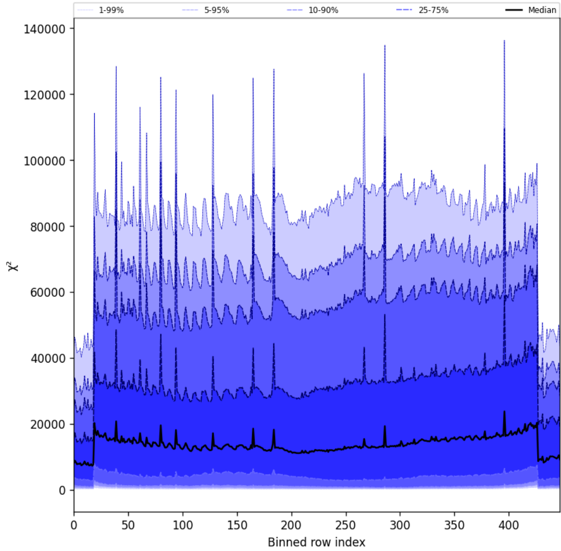
Figure 53: Along track statistics of “ \chi^2 ” for 2025-05-22 to 2025-05-23
