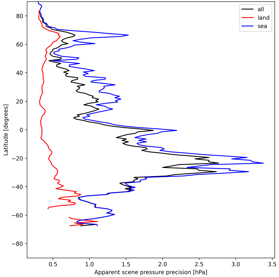
Figure 18: Zonal average of “Apparent scene pressure precision” for 2025-05-22 to 2025-05-23.
