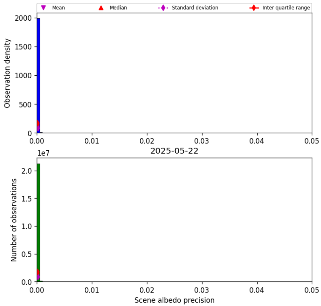
Figure 33: Histogram of “Scene albedo precision” for 2025-05-22 to 2025-05-23
