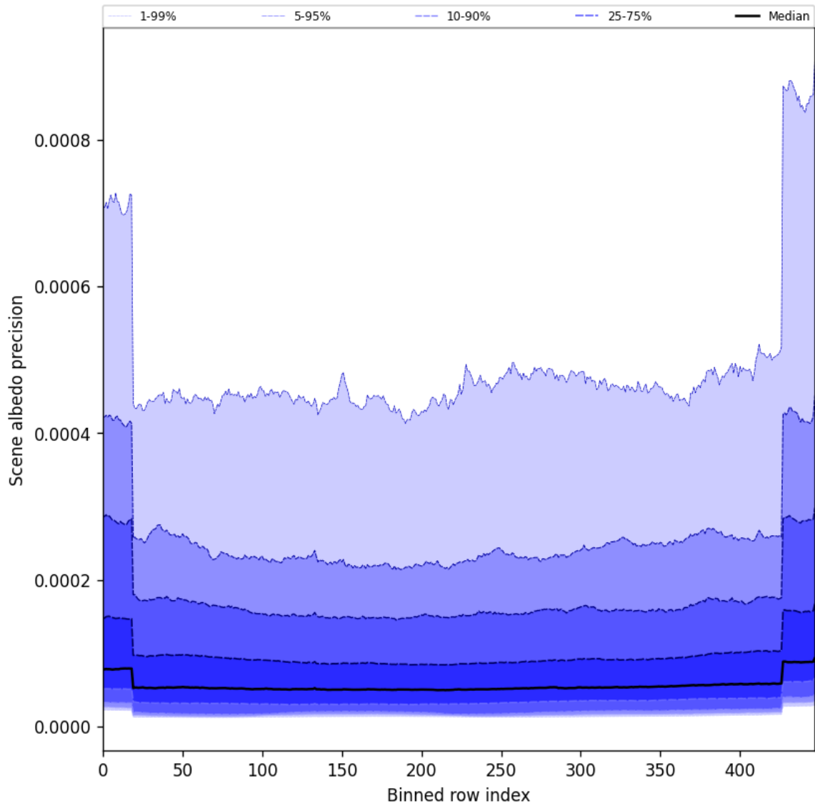
Figure 50: Along track statistics of “Scene albedo precision” for 2025-05-22 to 2025-05-23
