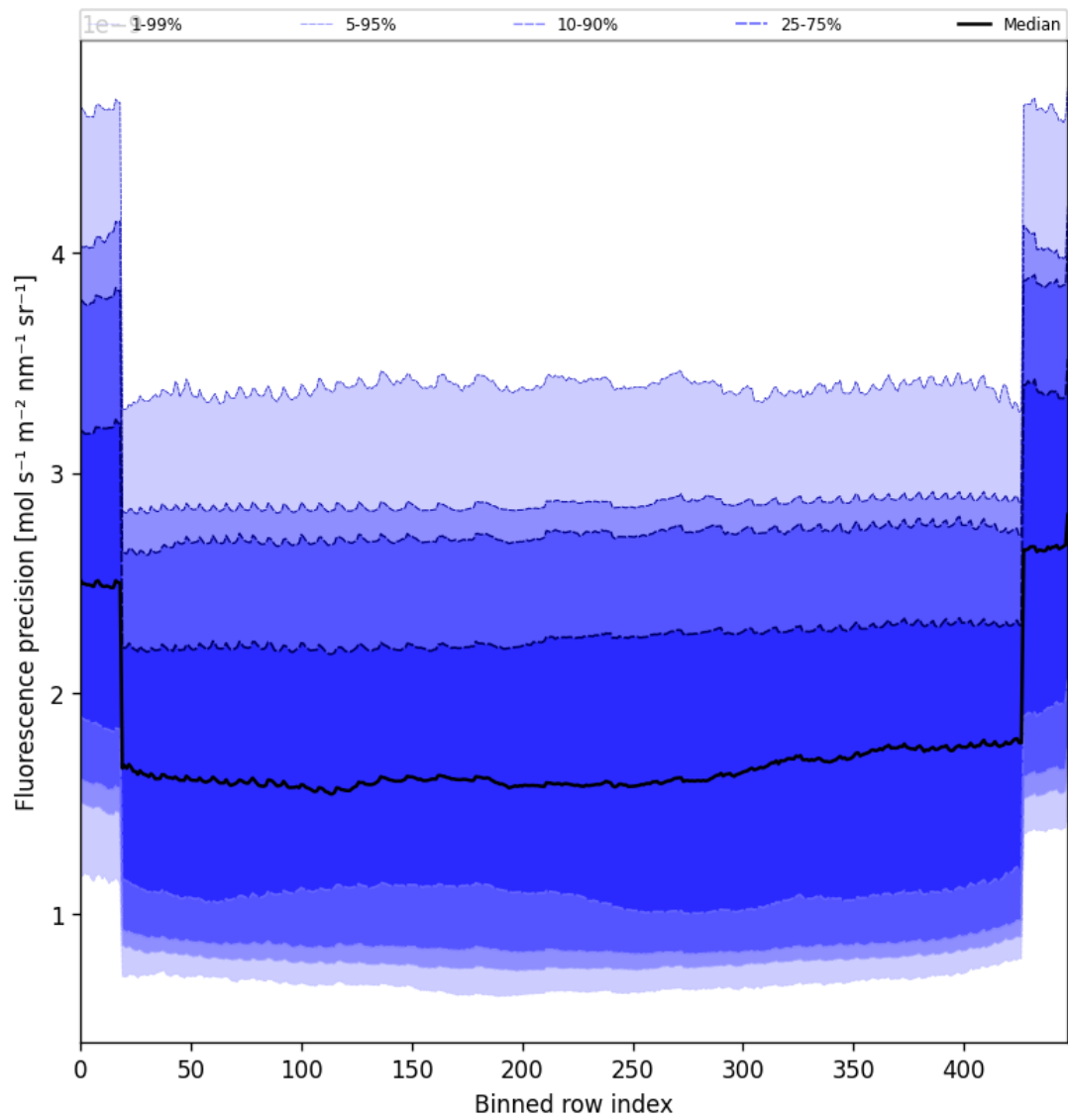
Figure 56: Along track statistics of “Fluorescence precision” for 2025-05-22 to 2025-05-23
