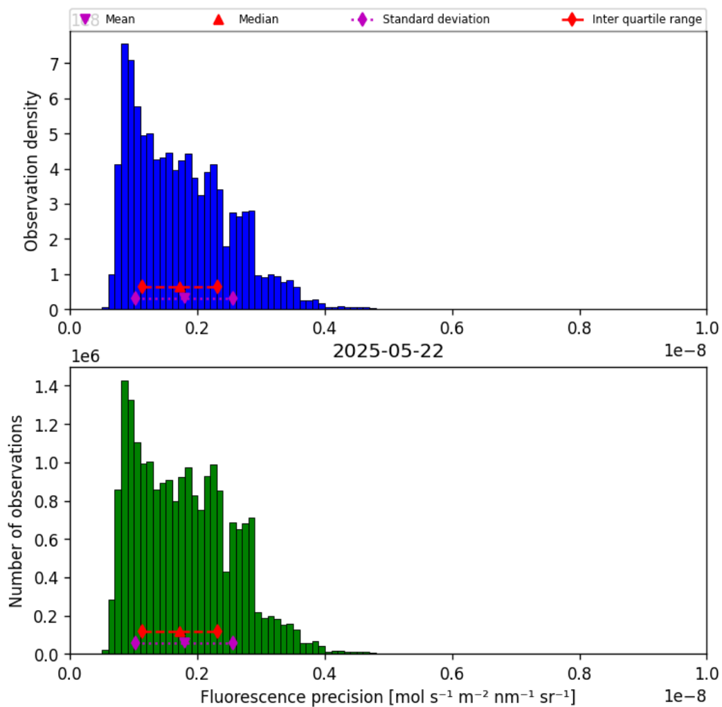
Figure 39: Histogram of “Fluorescence precision” for 2025-05-22 to 2025-05-23
