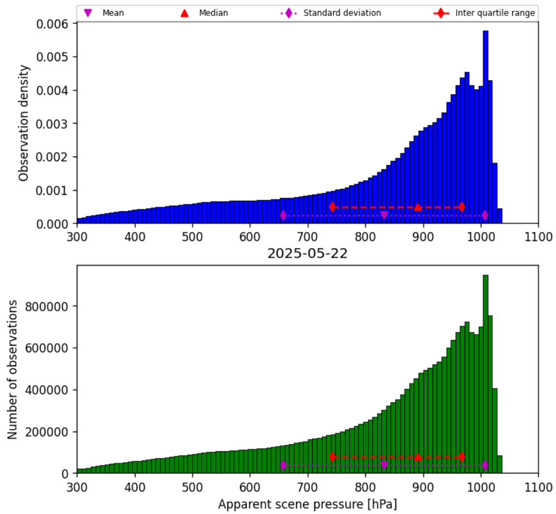
Figure 34: Histogram of “Apparent scene pressure” for 2025-05-22 to 2025-05-23
