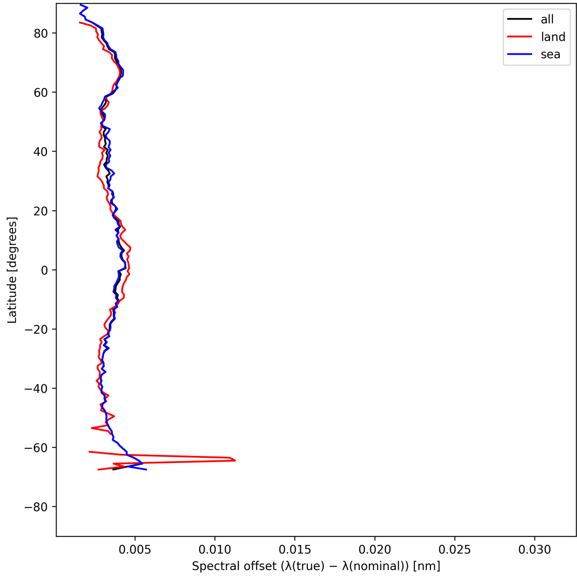
Figure 26: Zonal average of “Spectral offset ( \lambda_{\text{true}} - \lambda_{\text{nominal}} )” for 2025-05-22 to 2025-05-23.
