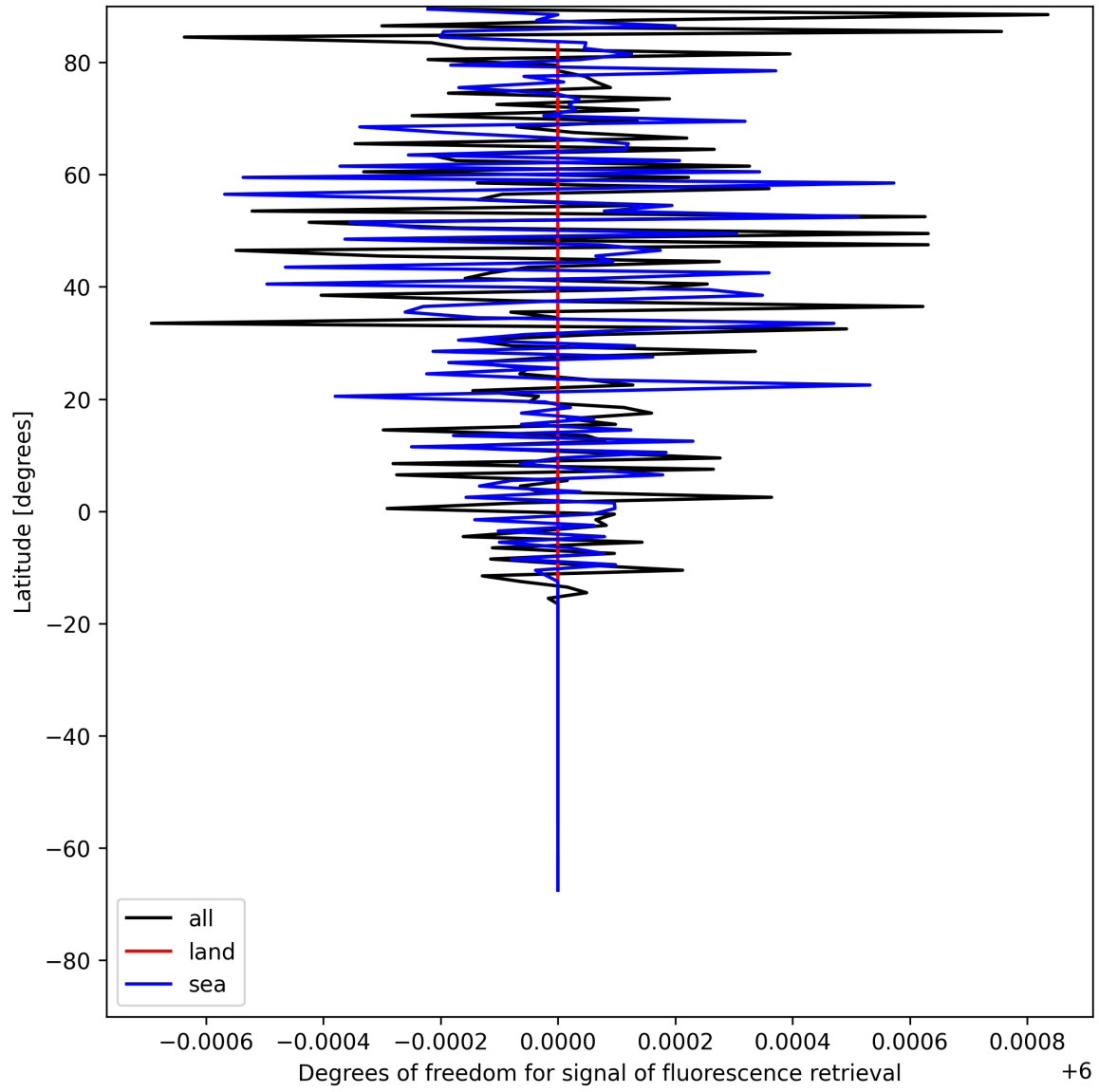
Figure 24: Zonal average of “Degrees of freedom for signal of fluorescence retrieval” for 2025-05-22 to 2025-05-23.
