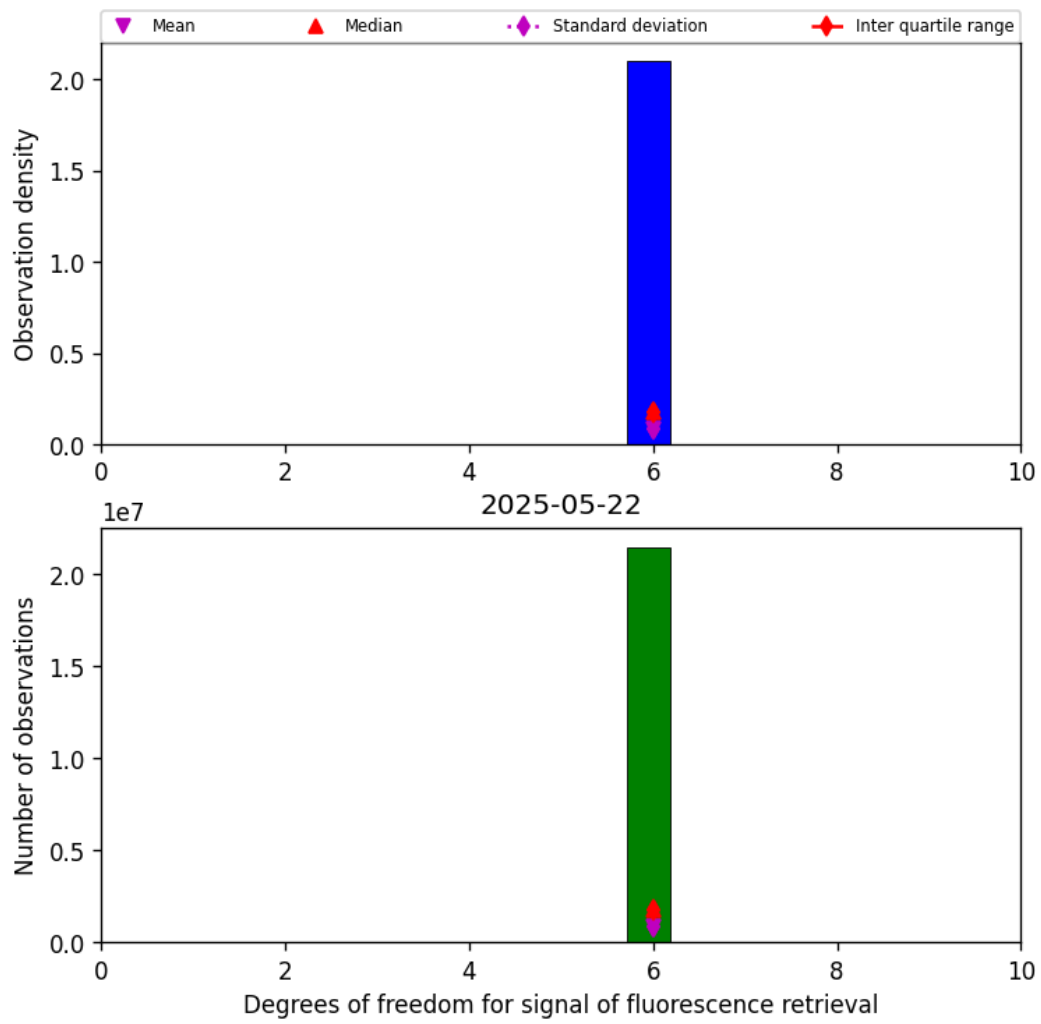
Figure 41: Histogram of “Degrees of freedom for signal of fluorescence retrieval” for 2025-05-22 to 2025-05-23
