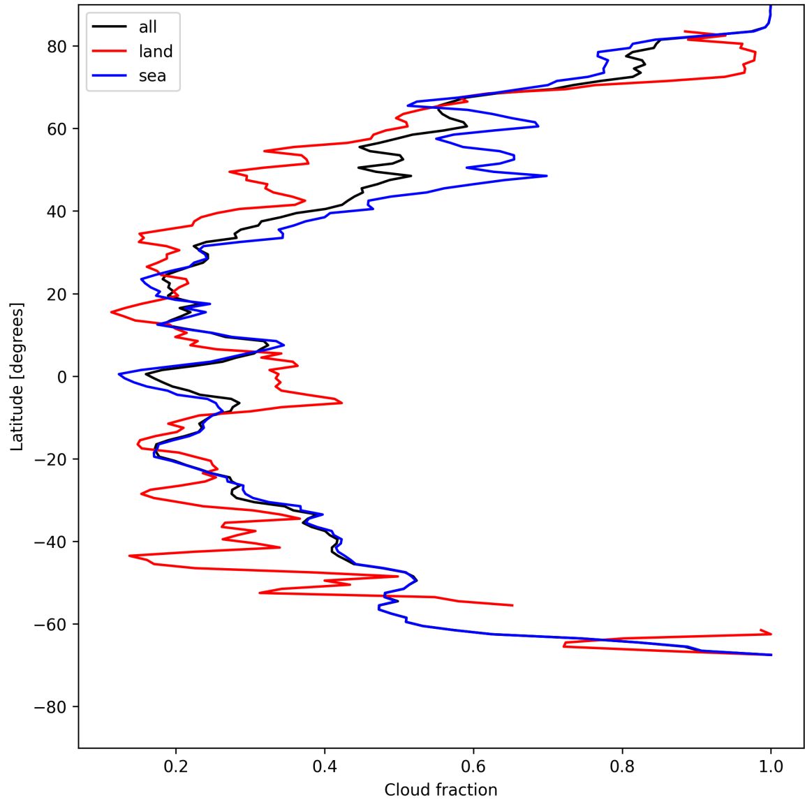
Figure 13: Zonal average of “Cloud fraction” for 2025-05-22 to 2025-05-23.
