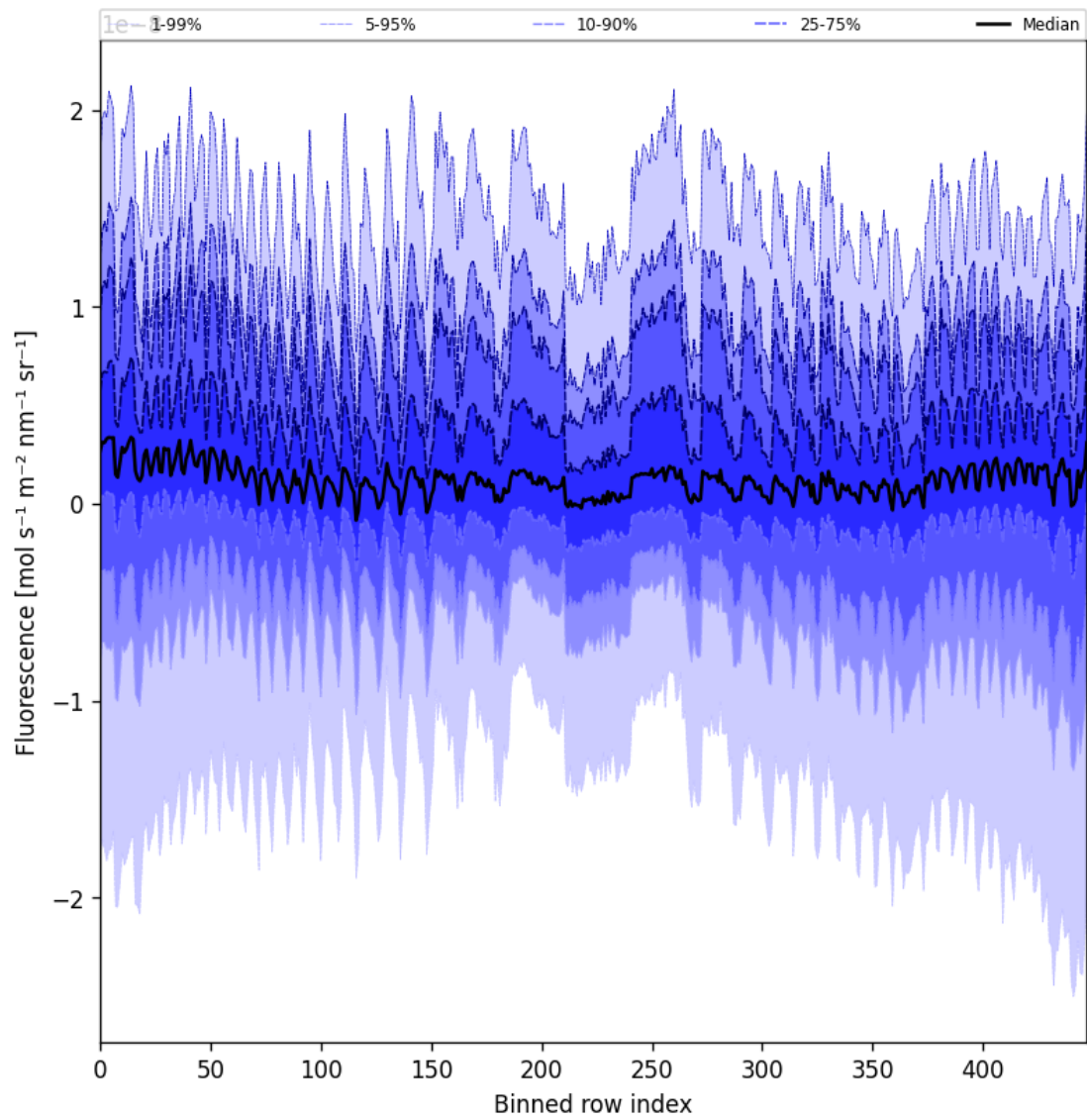
Figure 55: Along track statistics of “Fluorescence” for 2025-05-22 to 2025-05-23
