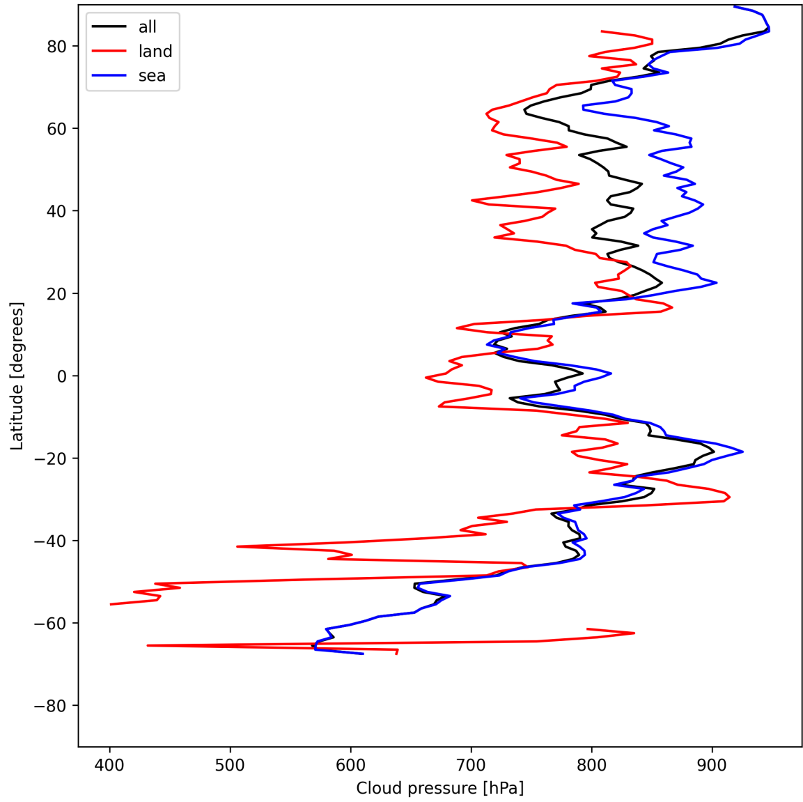
Figure 11: Zonal average of “Cloud pressure” for 2025-05-22 to 2025-05-23.
