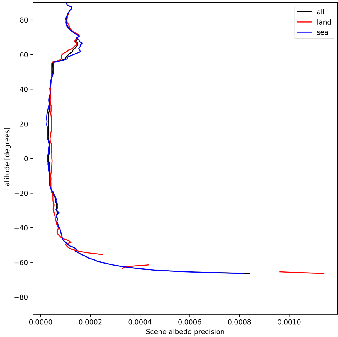
Figure 16: Zonal average of “Scene albedo precision” for 2025-05-23 to 2025-05-24.
