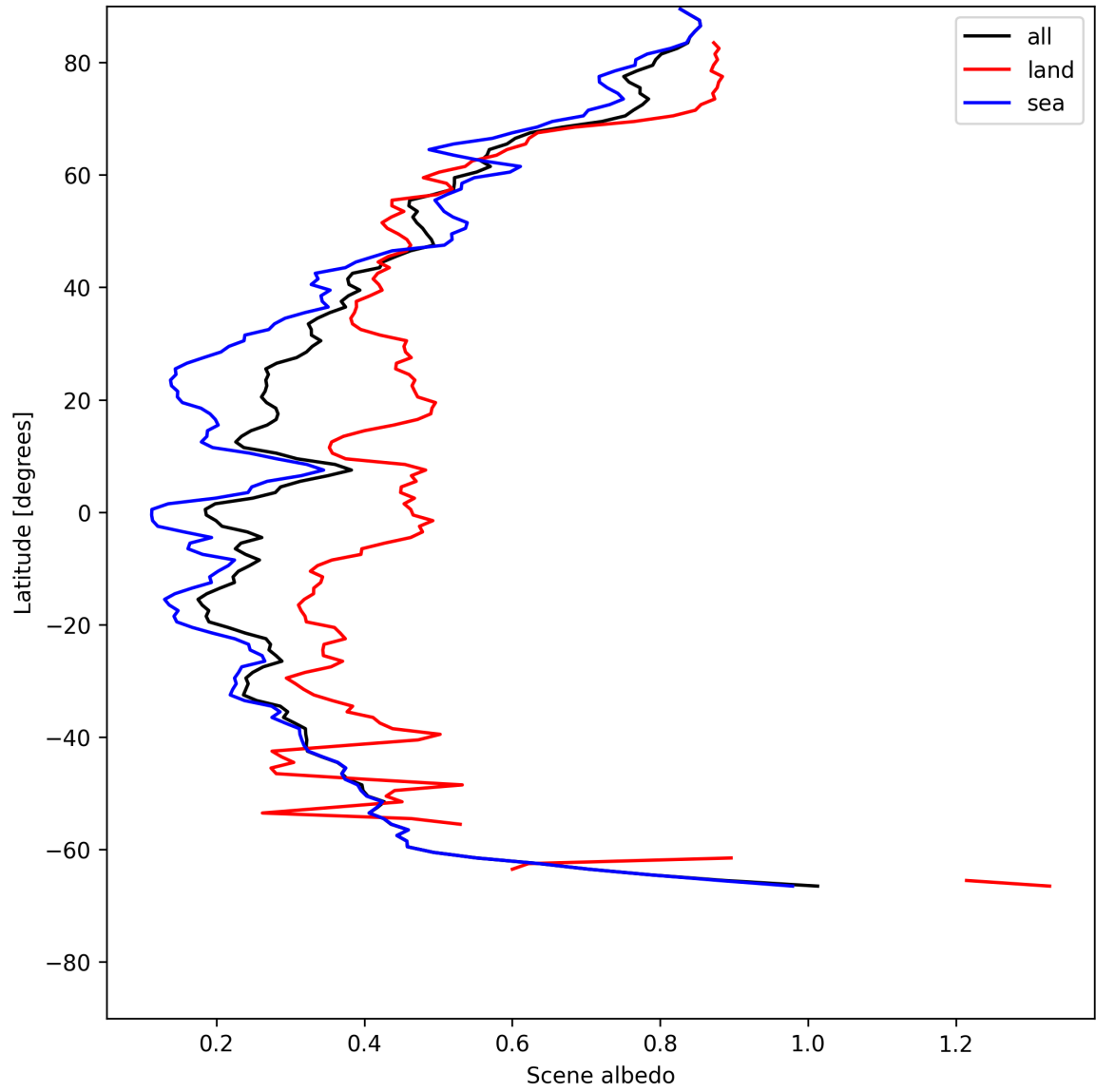
Figure 15: Zonal average of “Scene albedo” for 2025-05-23 to 2025-05-24.
