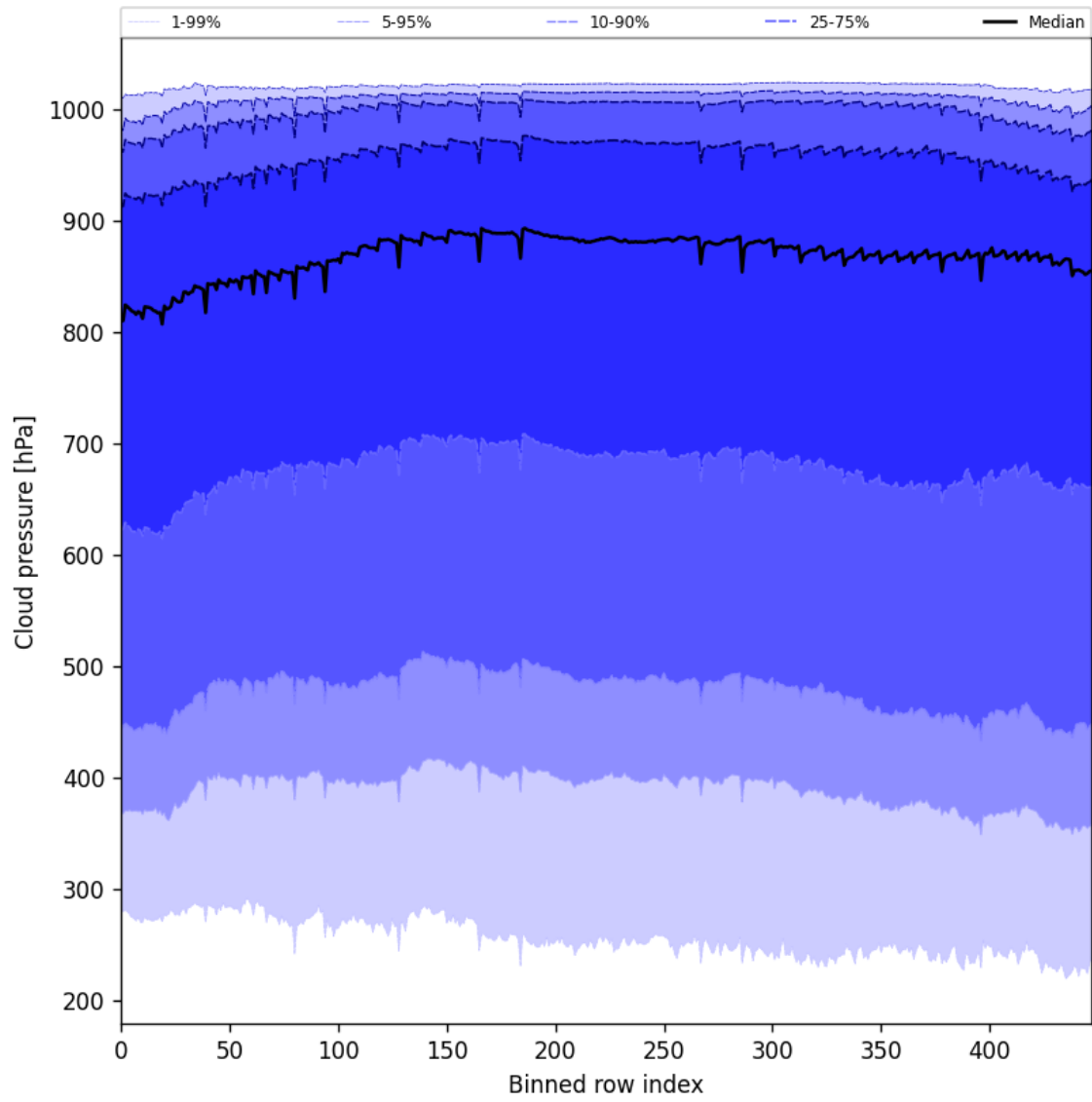
Figure 45: Along track statistics of “Cloud pressure” for 2025-05-23 to 2025-05-24
