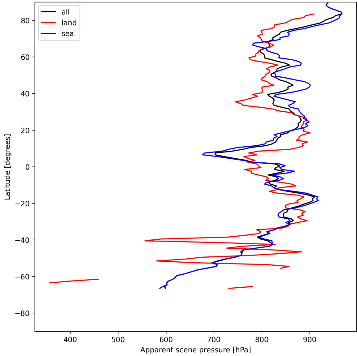
Figure 17: Zonal average of “Apparent scene pressure” for 2025-05-23 to 2025-05-24.
