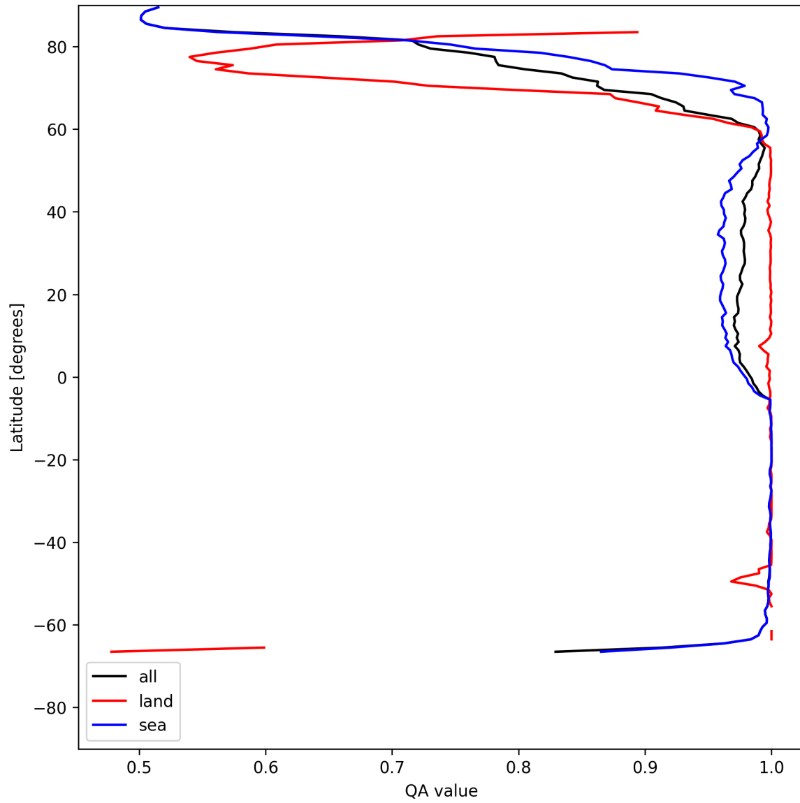
Figure 10: Zonal average of “QA value” for 2025-05-23 to 2025-05-24.
