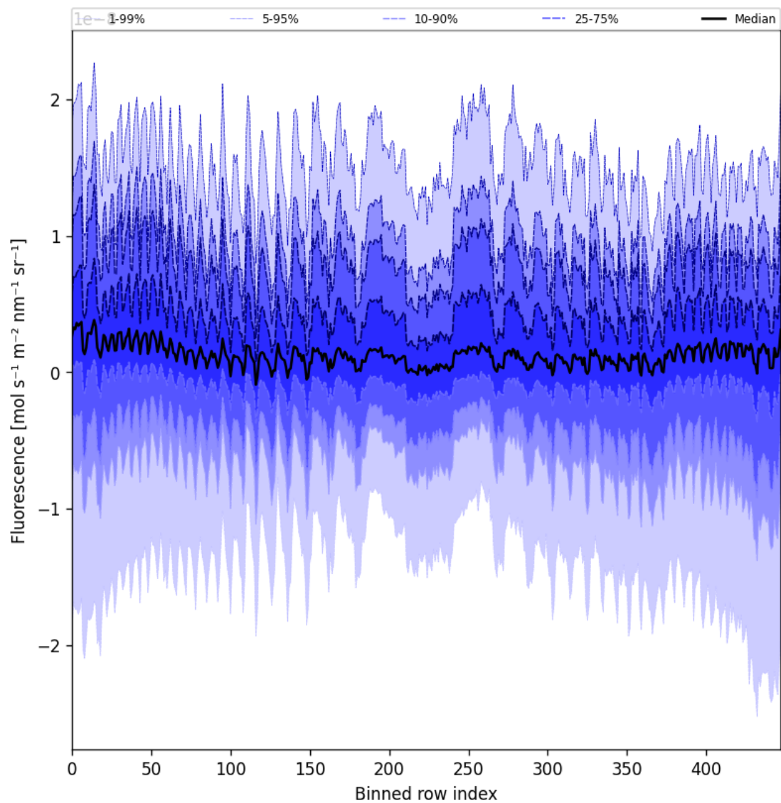
Figure 55: Along track statistics of “Fluorescence” for 2025-05-23 to 2025-05-24
