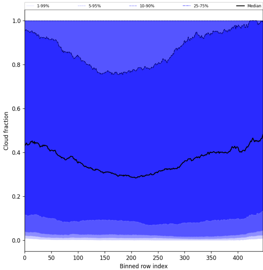
Figure 47: Along track statistics of “Cloud fraction” for 2025-05-23 to 2025-05-24
