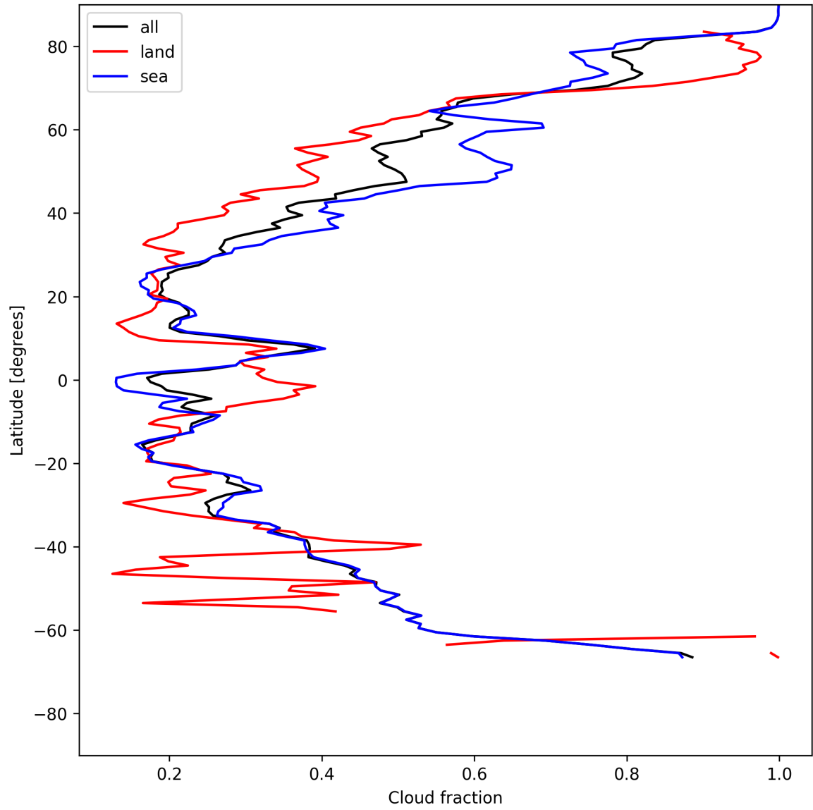
Figure 13: Zonal average of “Cloud fraction” for 2025-05-23 to 2025-05-24.
