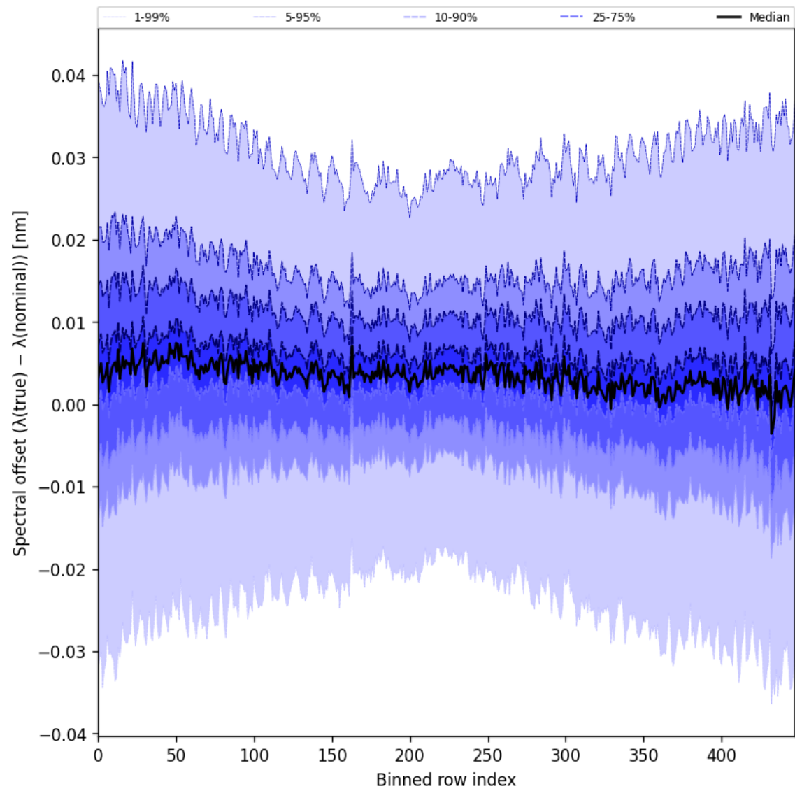
Figure 60: Along track statistics of “Spectral offset ( \lambda_{\text{true}} - \lambda_{\text{nominal}} )” for 2025-05-23 to 2025-05-24
