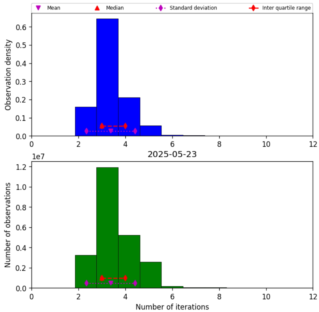
Figure 37: Histogram of “Number of iterations” for 2025-05-23 to 2025-05-24
