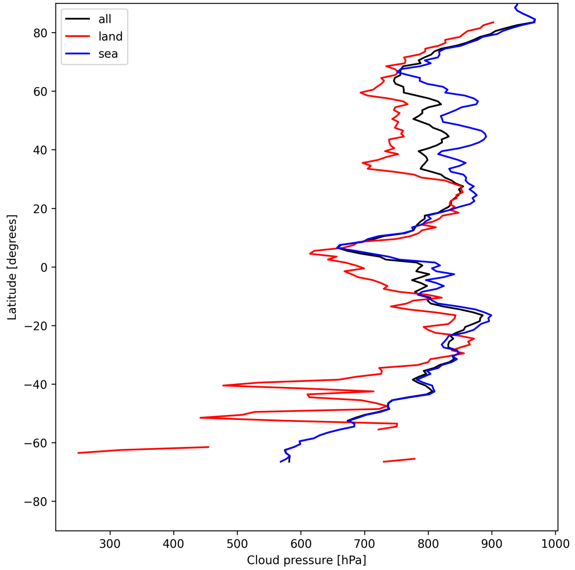
Figure 11: Zonal average of “Cloud pressure” for 2025-05-23 to 2025-05-24.
