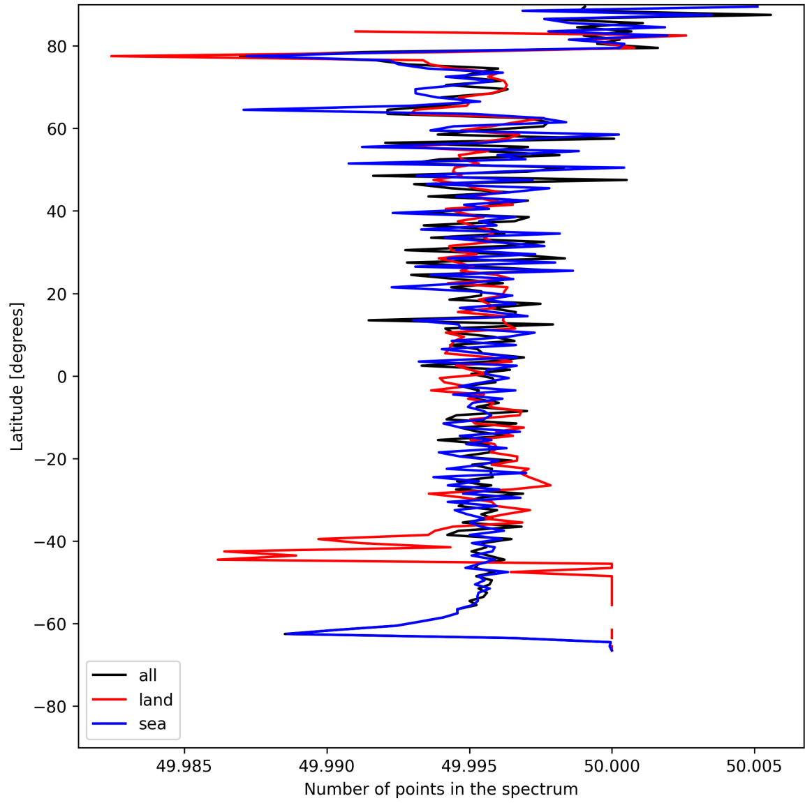
Figure 25: Zonal average of “Number of points in the spectrum” for 2025-05-23 to 2025-05-24.
