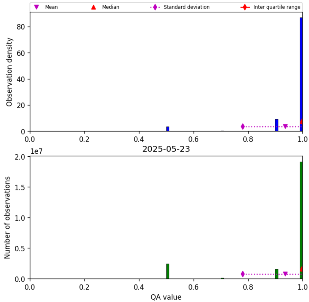
Figure 27: Histogram of “QA value” for 2025-05-23 to 2025-05-24
