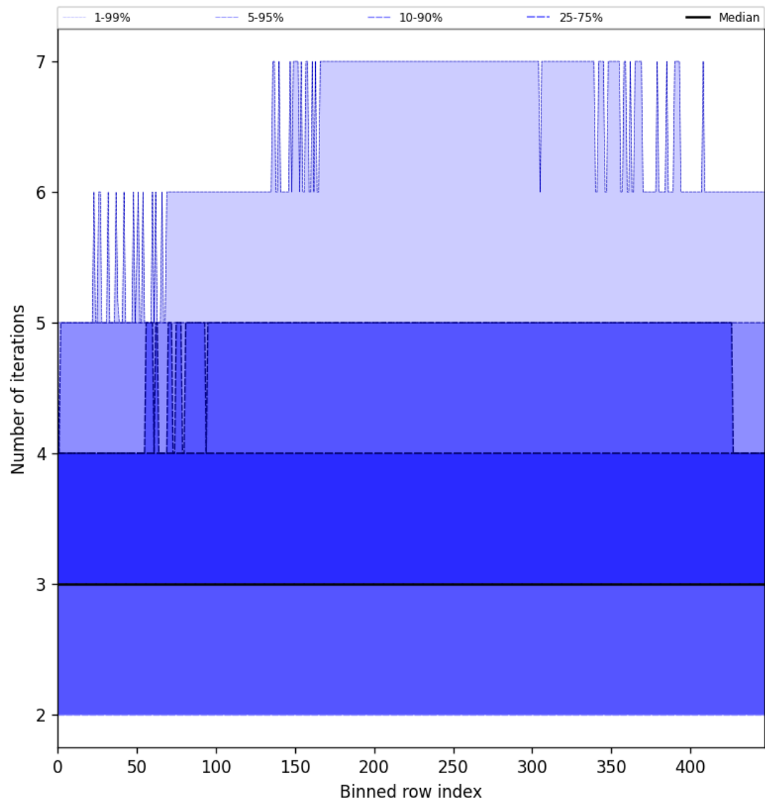
Figure 54: Along track statistics of “Number of iterations” for 2025-05-23 to 2025-05-24
