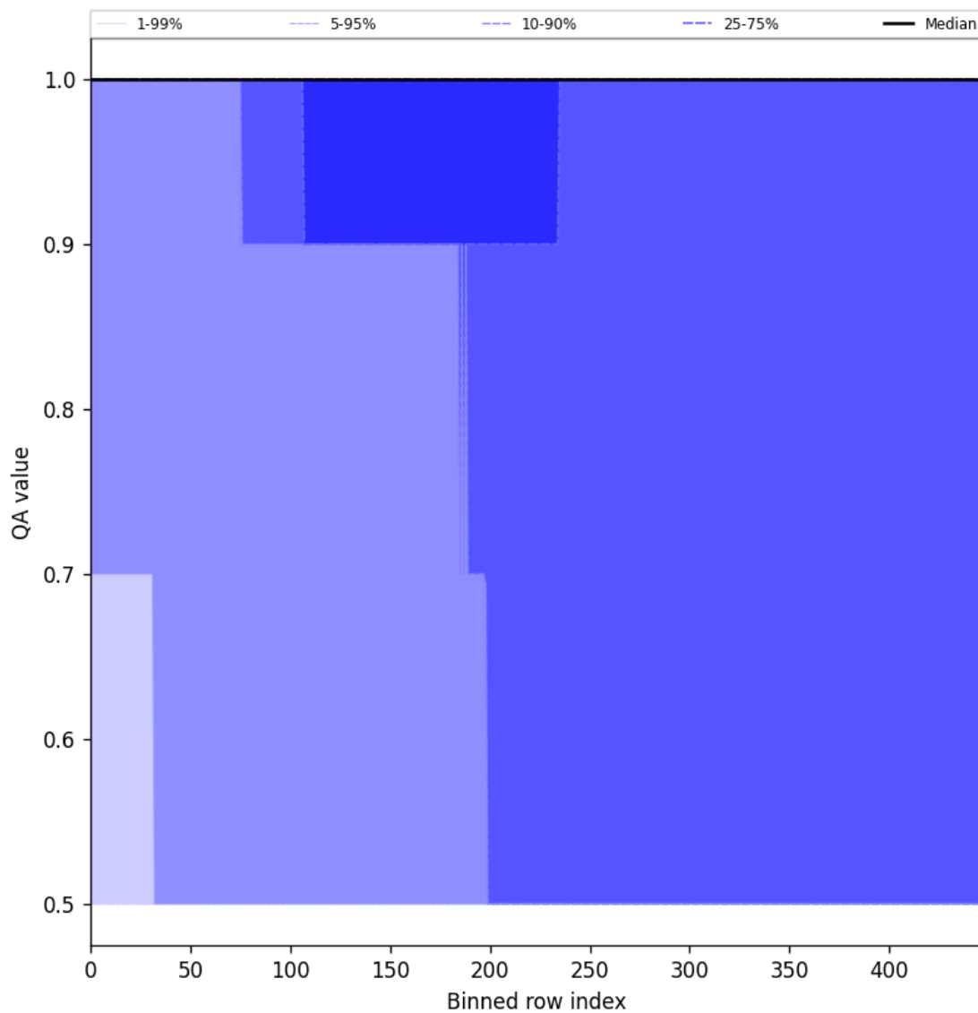
Figure 44: Along track statistics of “QA value” for 2025-05-23 to 2025-05-24
