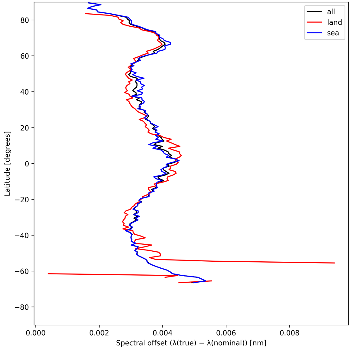
Figure 26: Zonal average of “Spectral offset ( \lambda_{\text{true}} - \lambda_{\text{nominal}} )” for 2025-05-23 to 2025-05-24.
