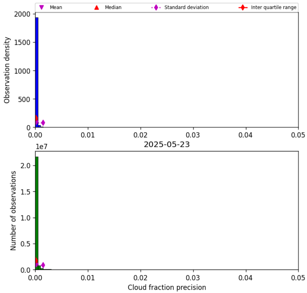
Figure 31: Histogram of “Cloud fraction precision” for 2025-05-23 to 2025-05-24
