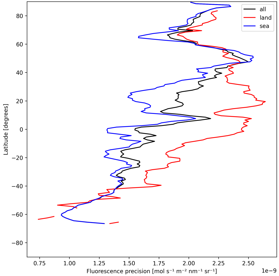
Figure 22: Zonal average of “Fluorescence precision” for 2025-05-23 to 2025-05-24.
