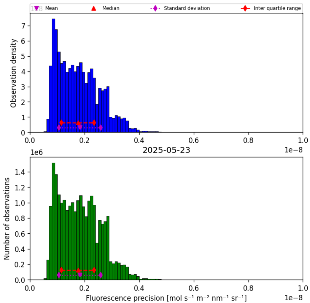
Figure 39: Histogram of “Fluorescence precision” for 2025-05-23 to 2025-05-24
