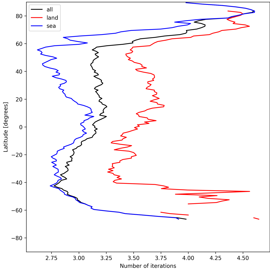
Figure 20: Zonal average of “Number of iterations” for 2025-05-23 to 2025-05-24.
