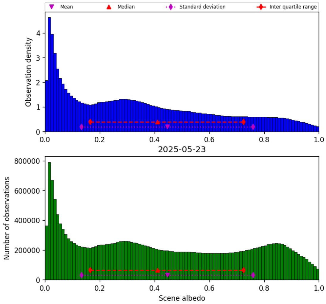
Figure 32: Histogram of “Scene albedo” for 2025-05-23 to 2025-05-24
