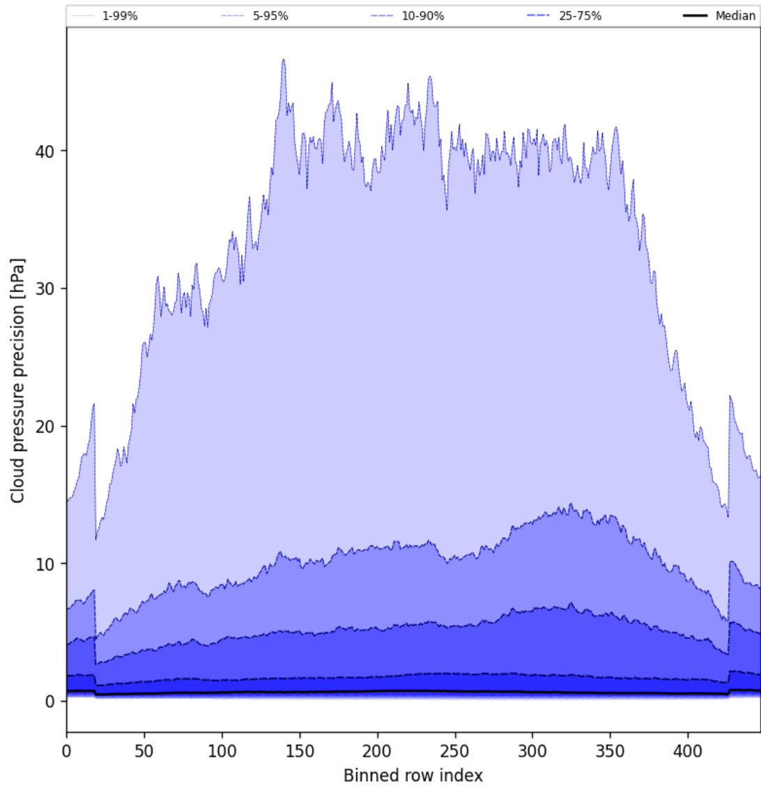
Figure 46: Along track statistics of “Cloud pressure precision” for 2025-05-23 to 2025-05-24
