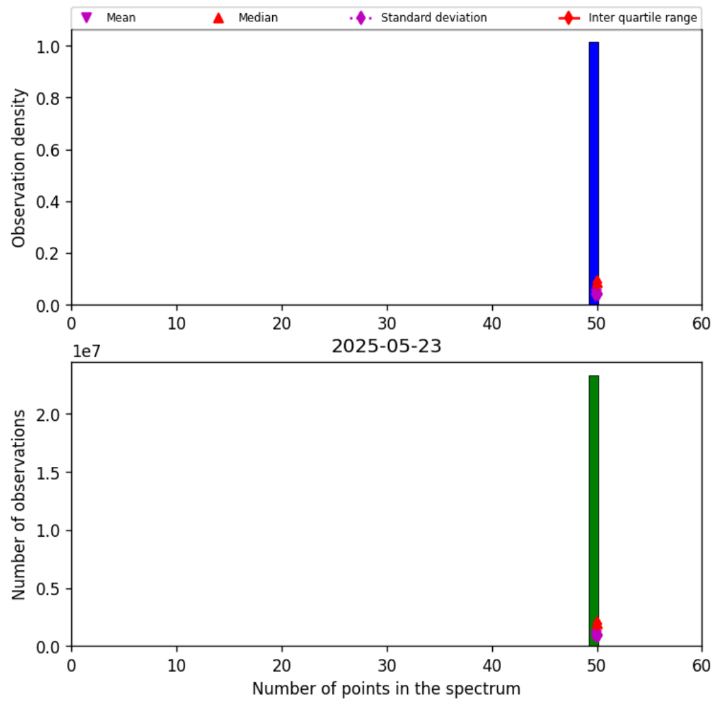
Figure 42: Histogram of “Number of points in the spectrum” for 2025-05-23 to 2025-05-24
