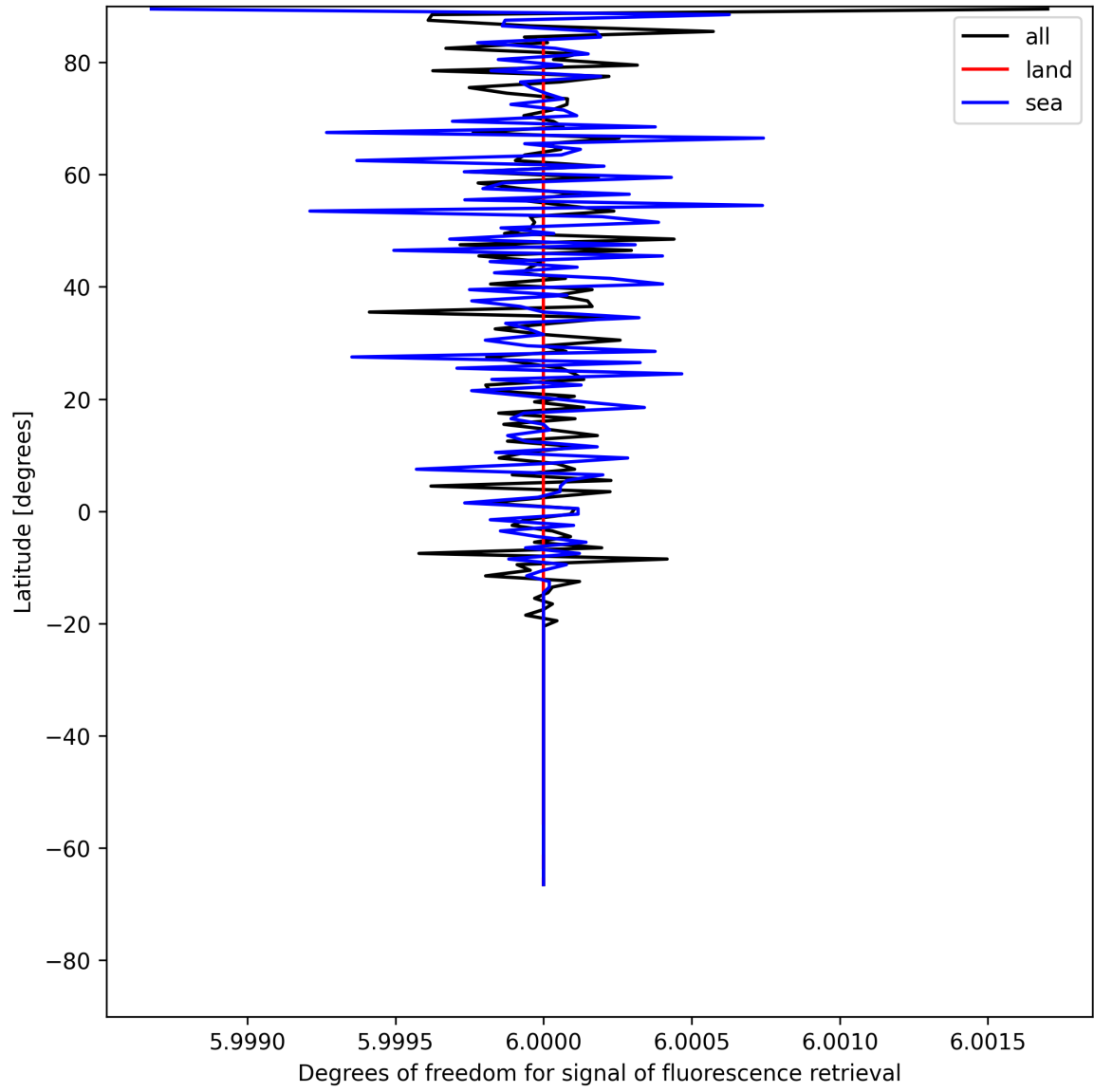
Figure 24: Zonal average of “Degrees of freedom for signal of fluorescence retrieval” for 2025-05-23 to 2025-05-24.
