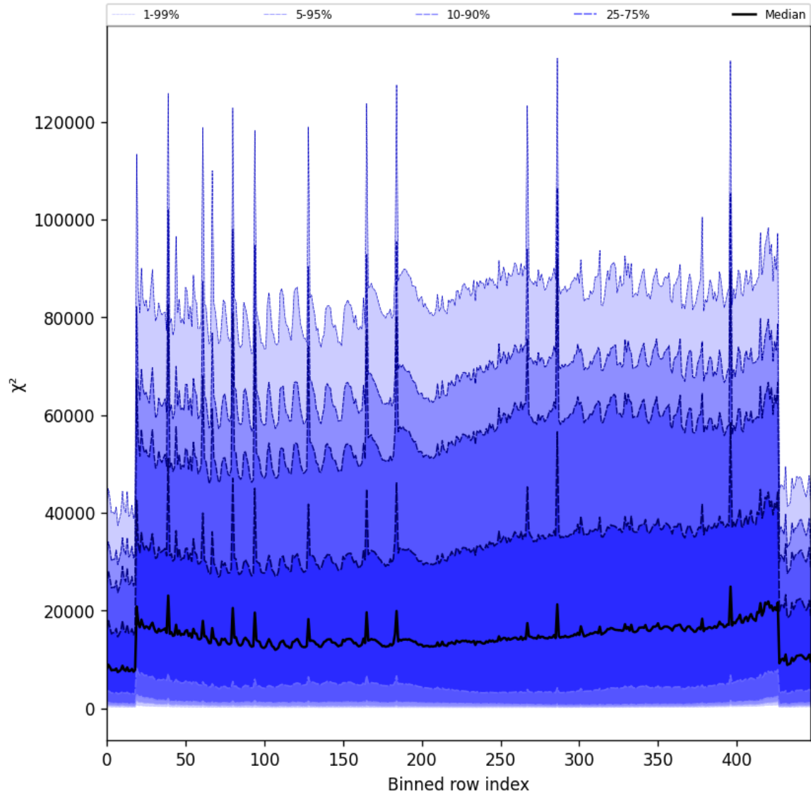
Figure 53: Along track statistics of “ \chi^2 ” for 2025-05-23 to 2025-05-24
