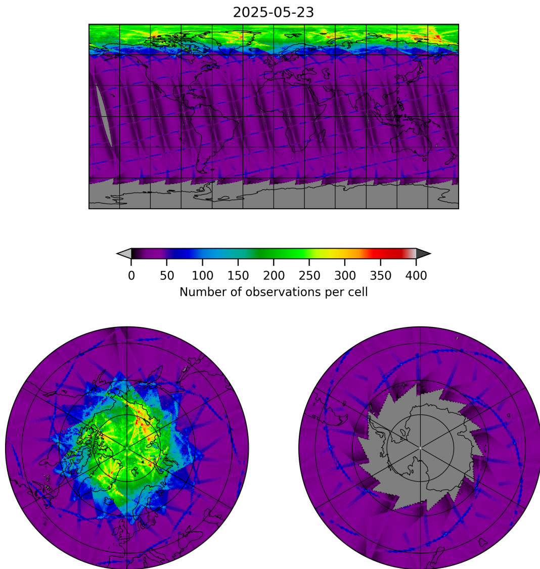
Figure 9: Map of the number of observations for 2025-05-23 to 2025-05-24
