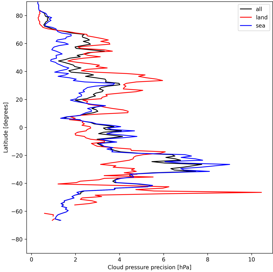
Figure 12: Zonal average of "Cloud pressure precision" for 2025-05-23 to 2025-05-24.
