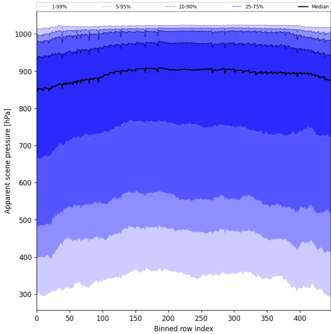
Figure 51: Along track statistics of “Apparent scene pressure” for 2025-05-23 to 2025-05-24
