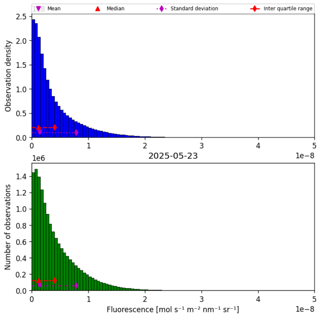
Figure 38: Histogram of “Fluorescence” for 2025-05-23 to 2025-05-24
