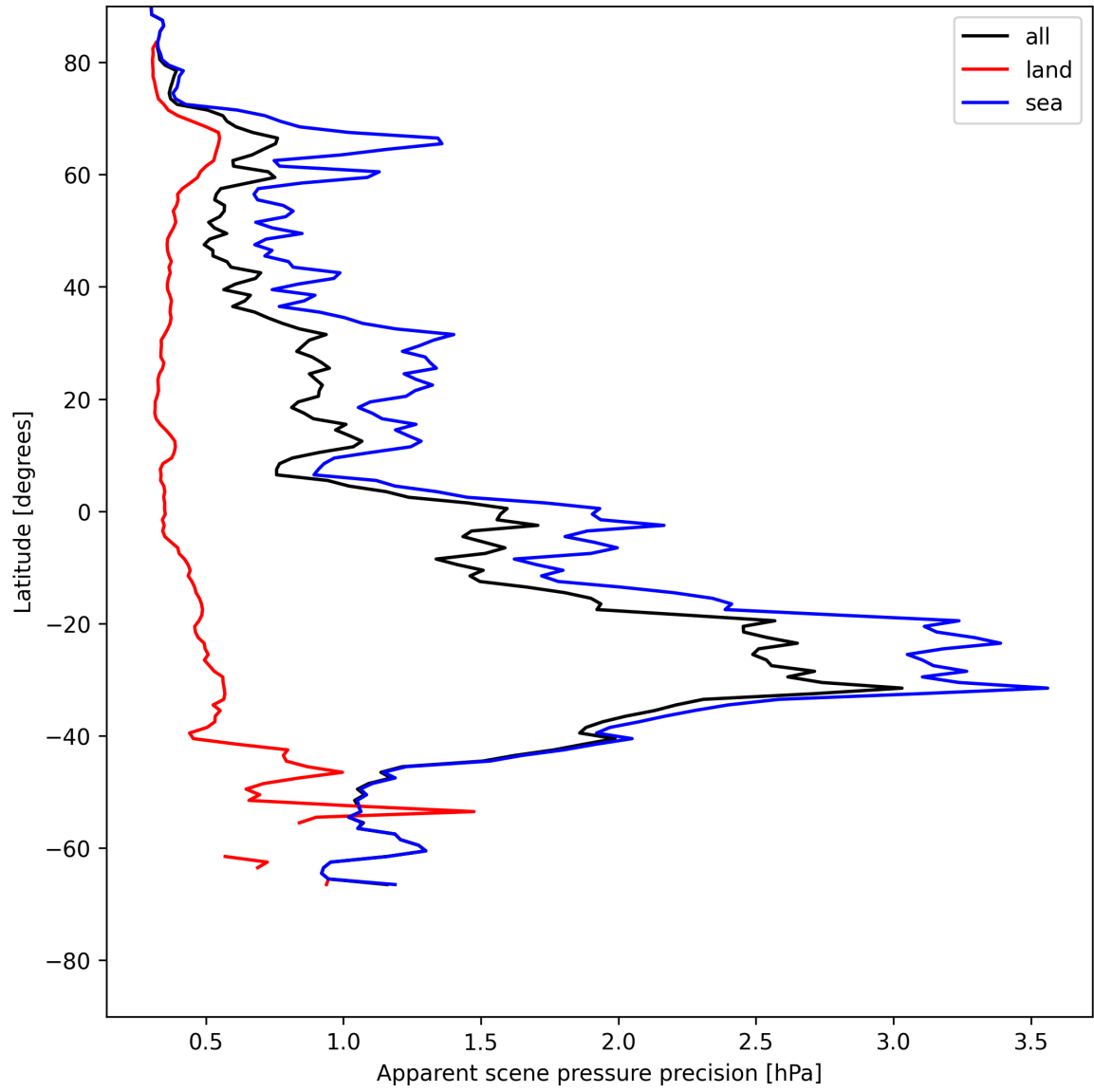
Figure 18: Zonal average of “Apparent scene pressure precision” for 2025-05-23 to 2025-05-24.
