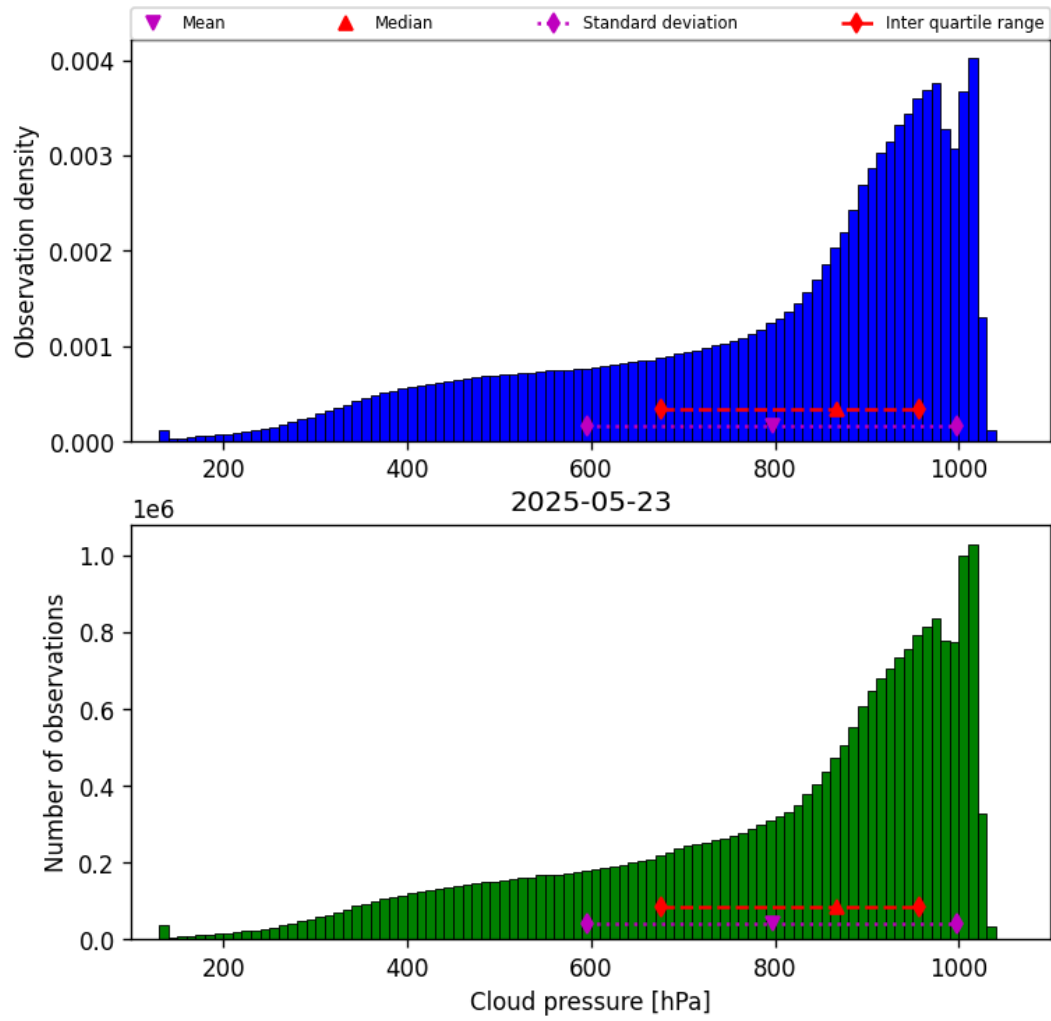
Figure 28: Histogram of “Cloud pressure” for 2025-05-23 to 2025-05-24
