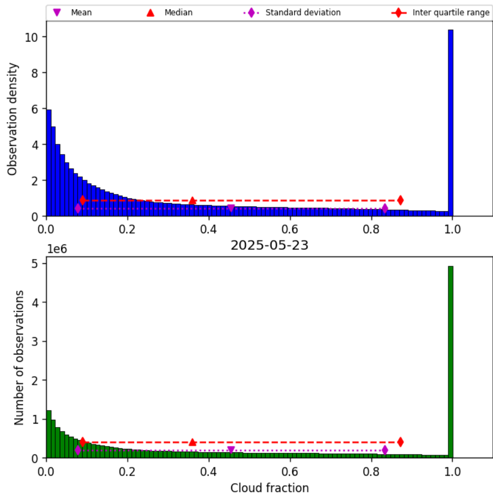
Figure 30: Histogram of “Cloud fraction” for 2025-05-23 to 2025-05-24
