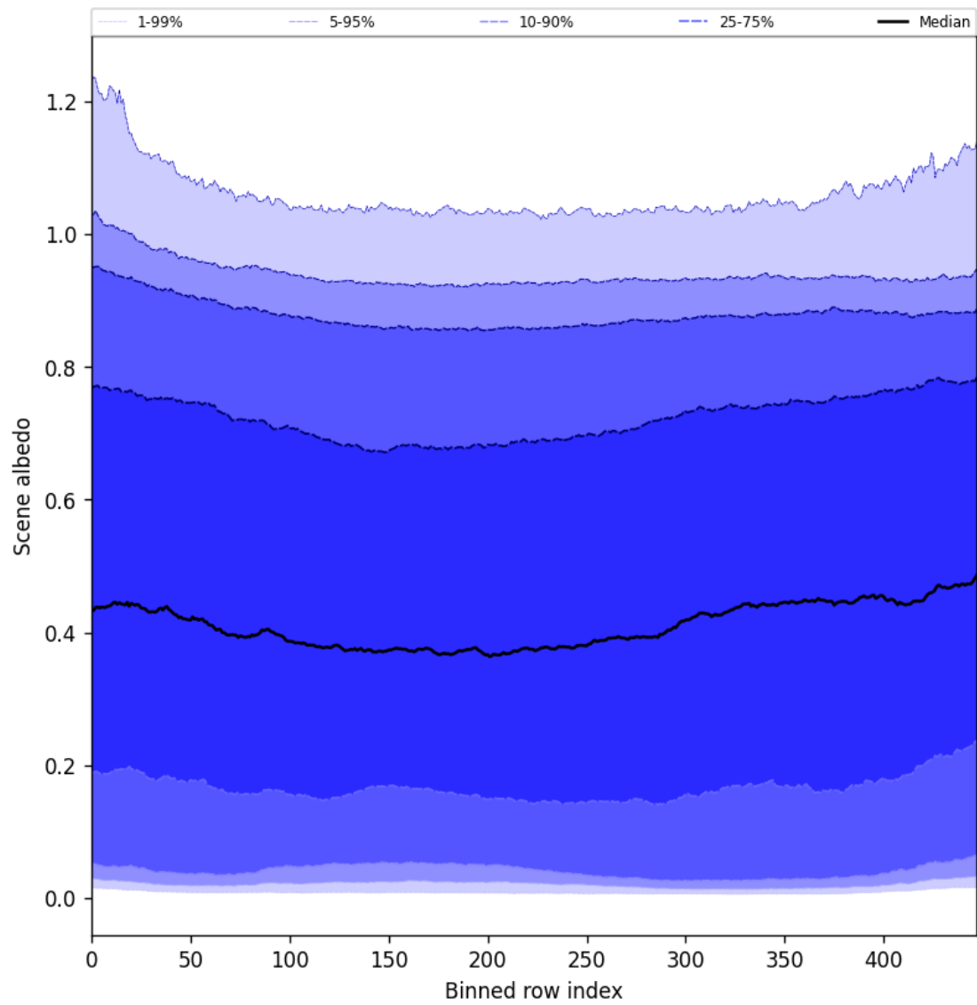
Figure 49: Along track statistics of “Scene albedo” for 2025-05-23 to 2025-05-24
