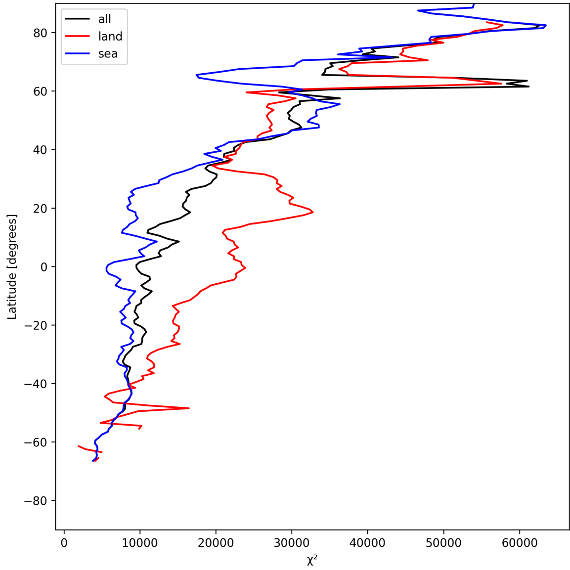
Figure 19: Zonal average of “ \chi^2 ” for 2025-05-23 to 2025-05-24.
