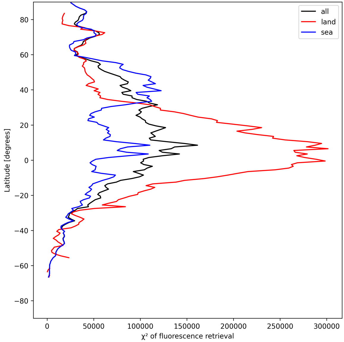
Figure 23: Zonal average of “ \chi^2 of fluorescence retrieval” for 2025-05-23 to 2025-05-24.
