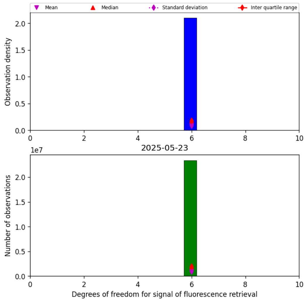
Figure 41: Histogram of “Degrees of freedom for signal of fluorescence retrieval” for 2025-05-23 to 2025-05-24
