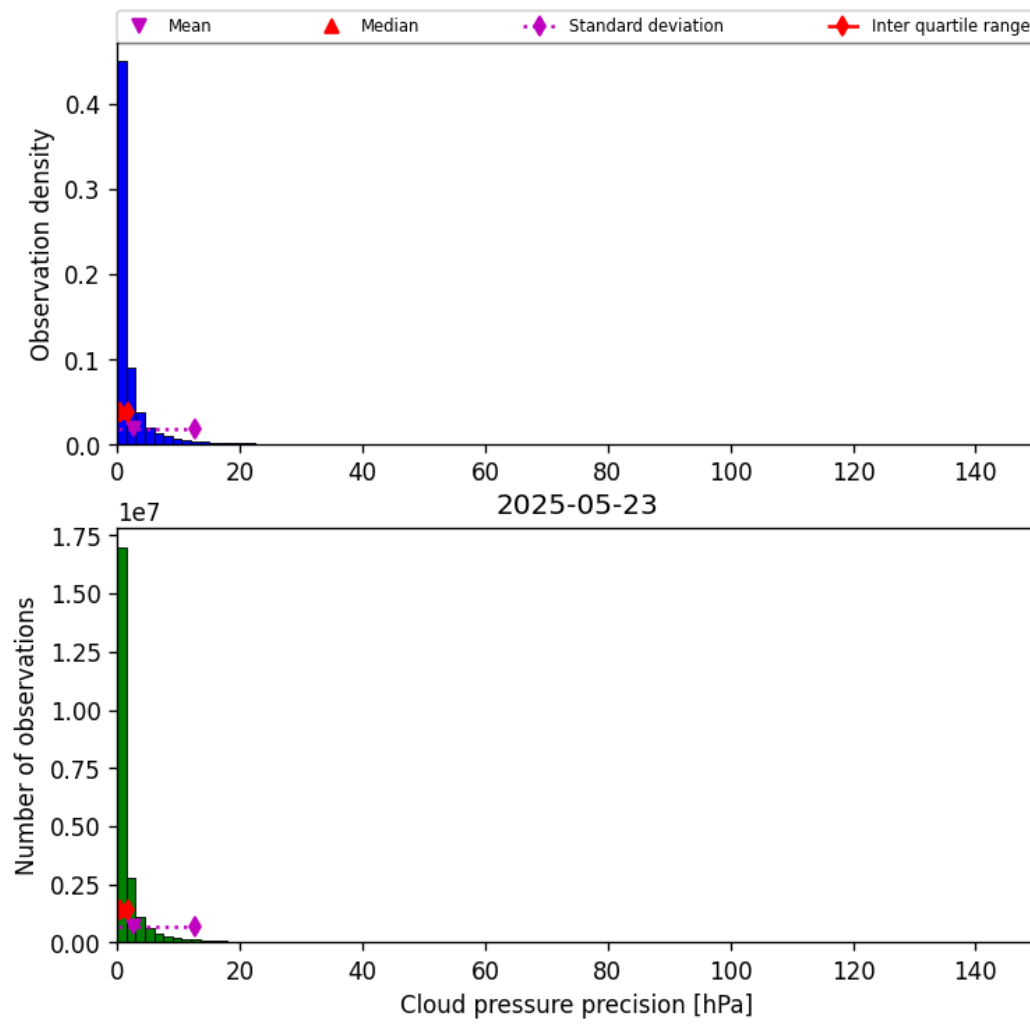
Figure 29: Histogram of “Cloud pressure precision” for 2025-05-23 to 2025-05-24
