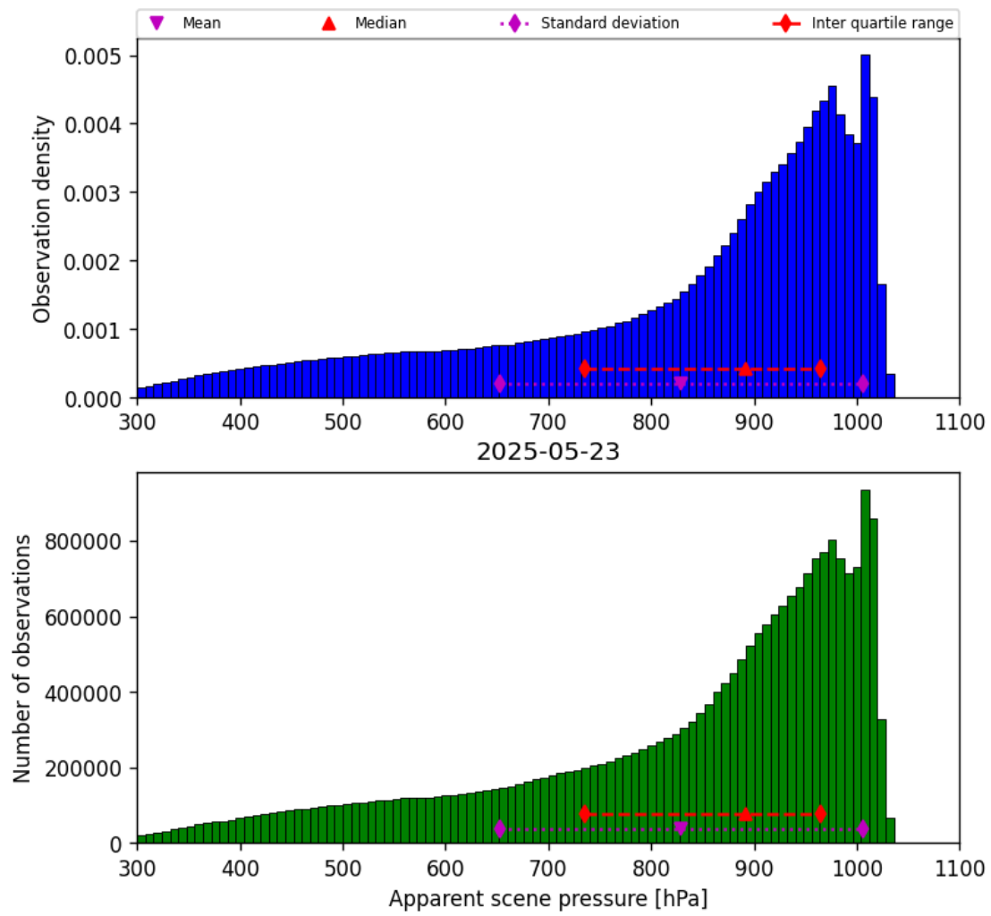
Figure 34: Histogram of “Apparent scene pressure” for 2025-05-23 to 2025-05-24
