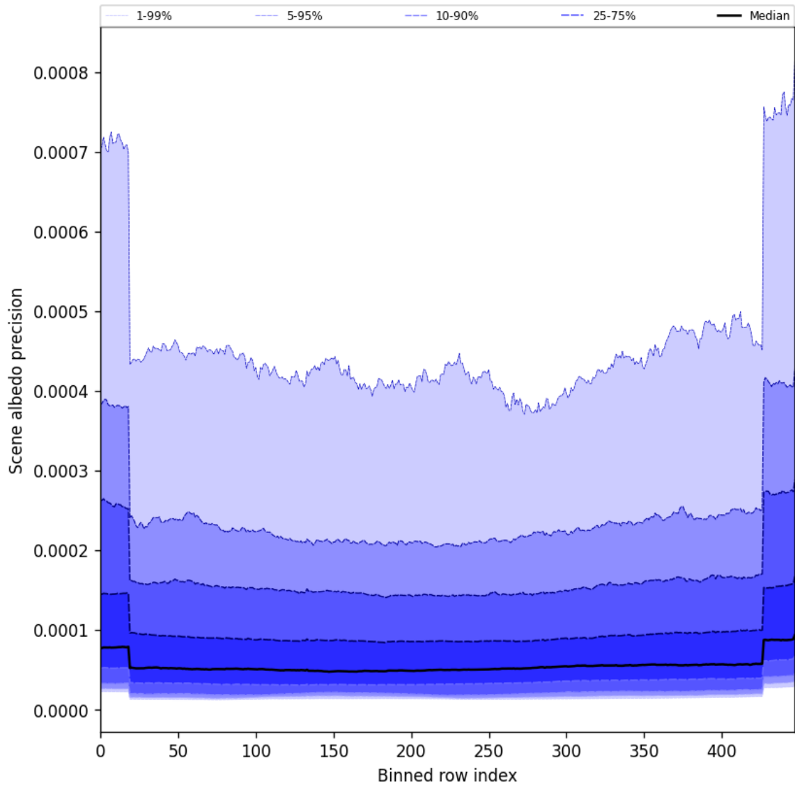
Figure 50: Along track statistics of “Scene albedo precision” for 2025-05-23 to 2025-05-24
