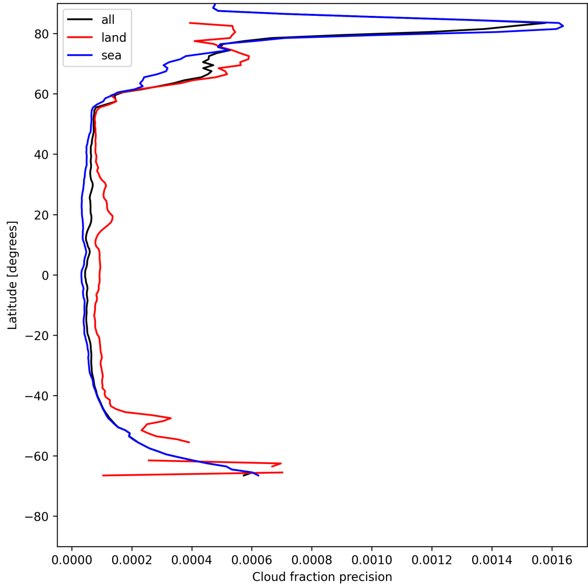
Figure 14: Zonal average of “Cloud fraction precision” for 2025-05-23 to 2025-05-24.
