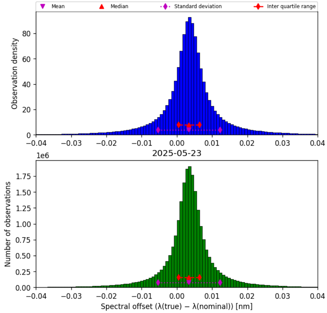
Figure 43: Histogram of “Spectral offset ( \lambda_{\text{true}} - \lambda_{\text{nominal}} )” for 2025-05-23 to 2025-05-24
