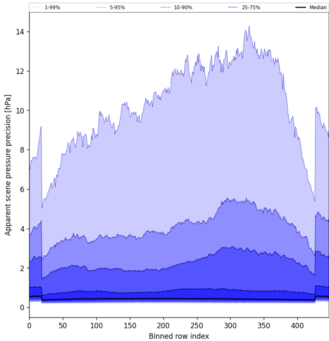
Figure 52: Along track statistics of “Apparent scene pressure precision” for 2025-05-23 to 2025-05-24
