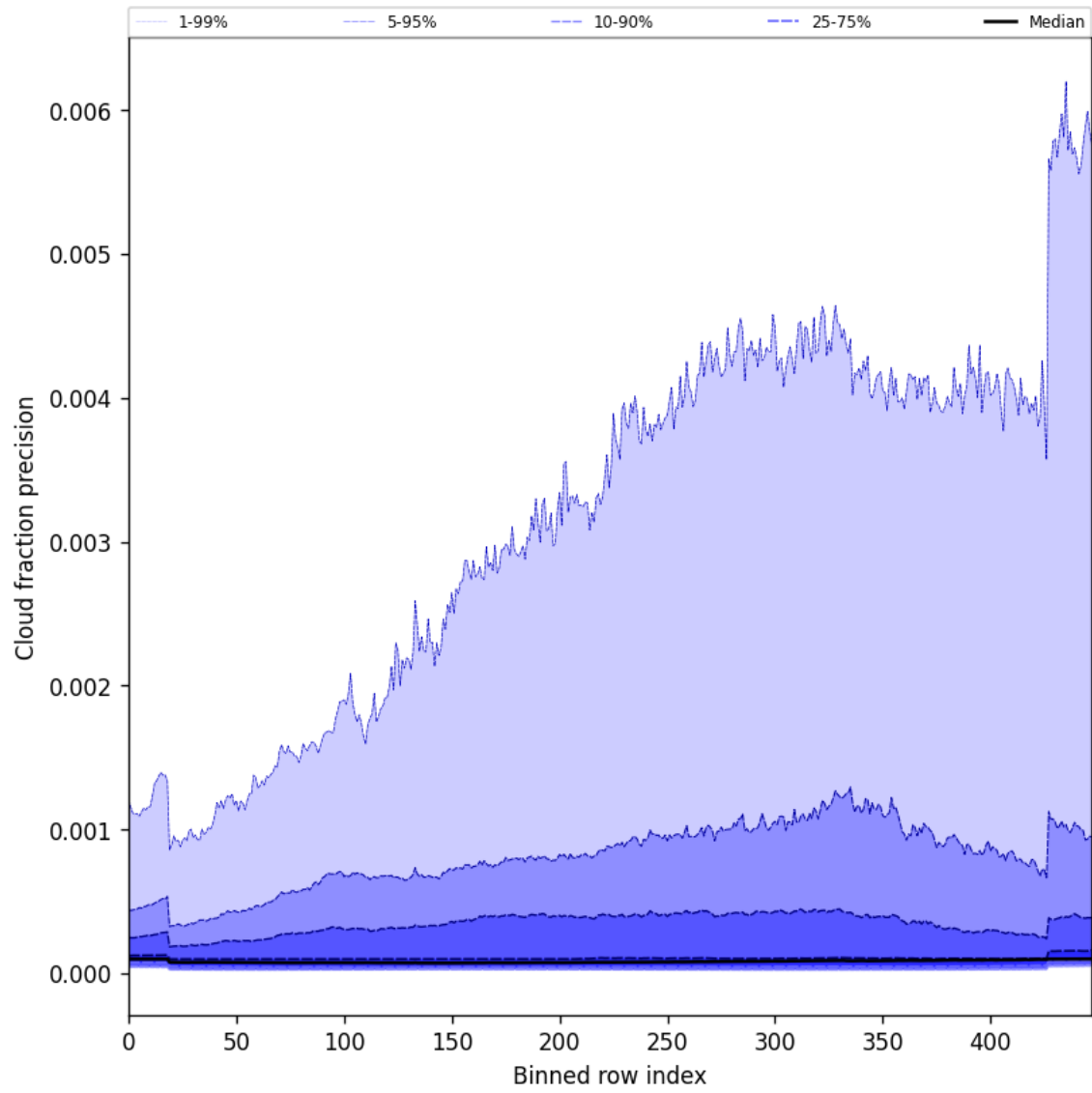
Figure 48: Along track statistics of “Cloud fraction precision” for 2025-05-23 to 2025-05-24
