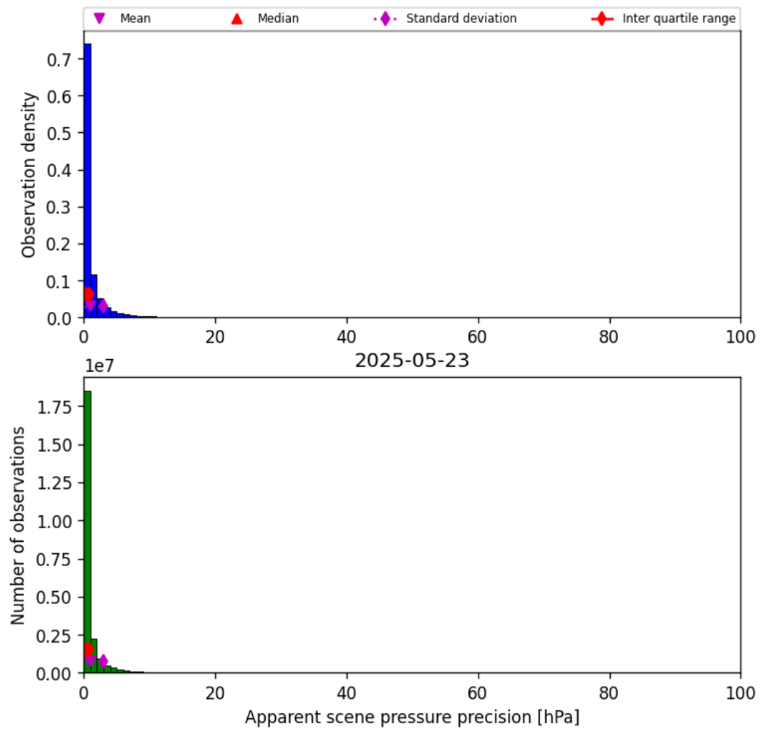
Figure 35: Histogram of “Apparent scene pressure precision” for 2025-05-23 to 2025-05-24
