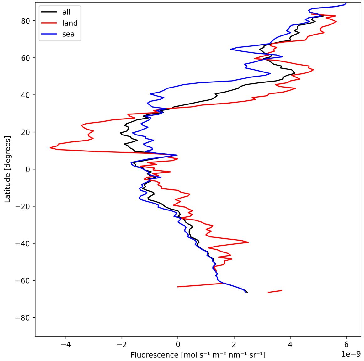
Figure 21: Zonal average of “Fluorescence” for 2025-05-23 to 2025-05-24.
