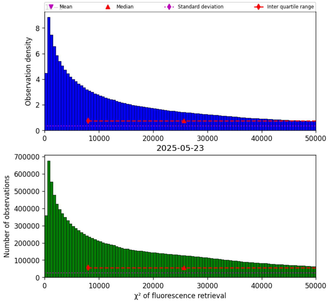
Figure 40: Histogram of “ \chi^2 of fluorescence retrieval” for 2025-05-23 to 2025-05-24
