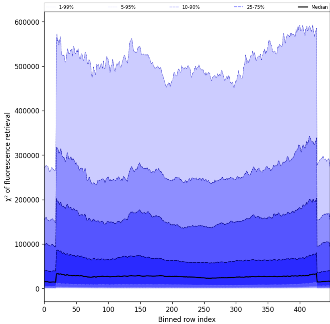
Figure 57: Along track statistics of “ \chi^2 of fluorescence retrieval” for 2025-05-23 to 2025-05-24
