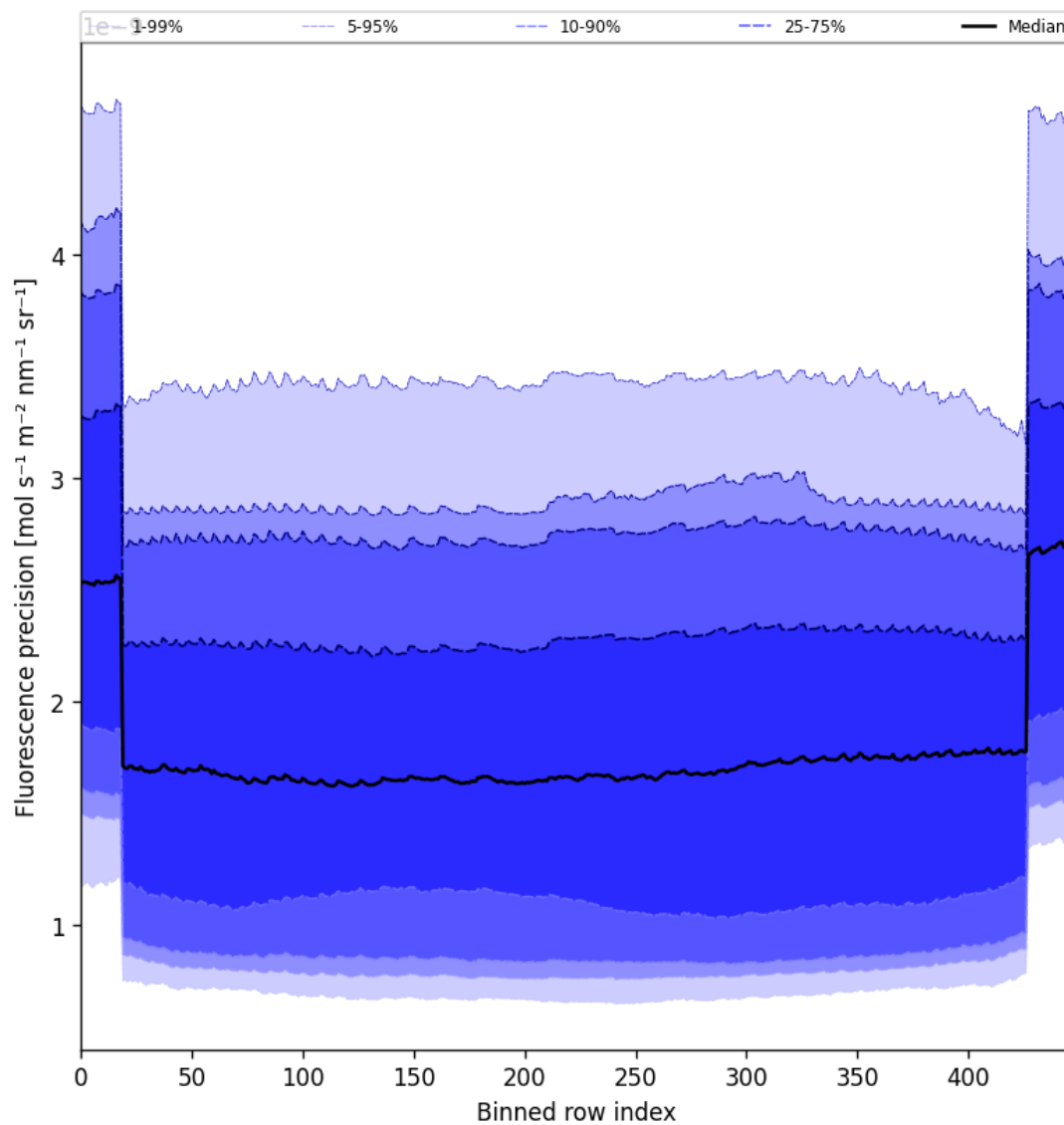
Figure 56: Along track statistics of “Fluorescence precision” for 2025-05-23 to 2025-05-24
