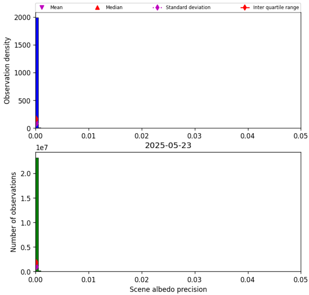
Figure 33: Histogram of “Scene albedo precision” for 2025-05-23 to 2025-05-24
