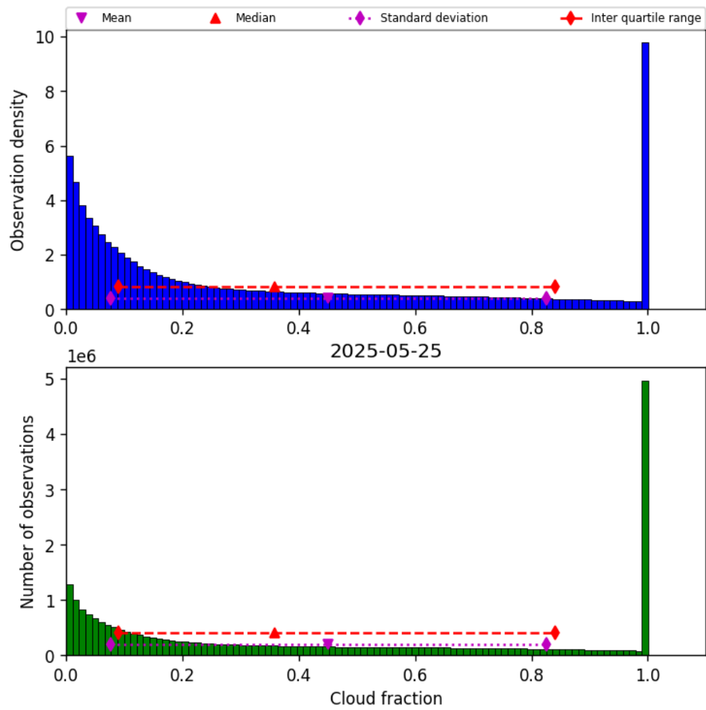
Figure 30: Histogram of “Cloud fraction” for 2025-05-25 to 2025-05-26
