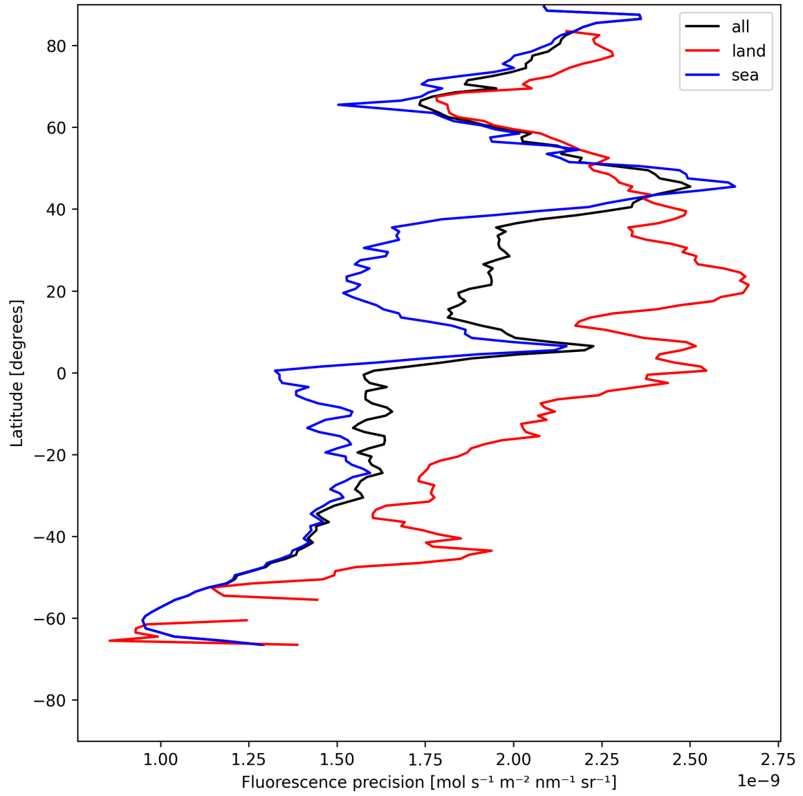
Figure 22: Zonal average of “Fluorescence precision” for 2025-05-25 to 2025-05-26.
