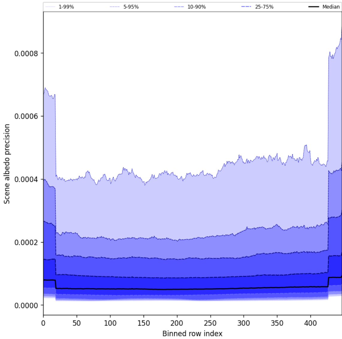
Figure 50: Along track statistics of “Scene albedo precision” for 2025-05-25 to 2025-05-26
