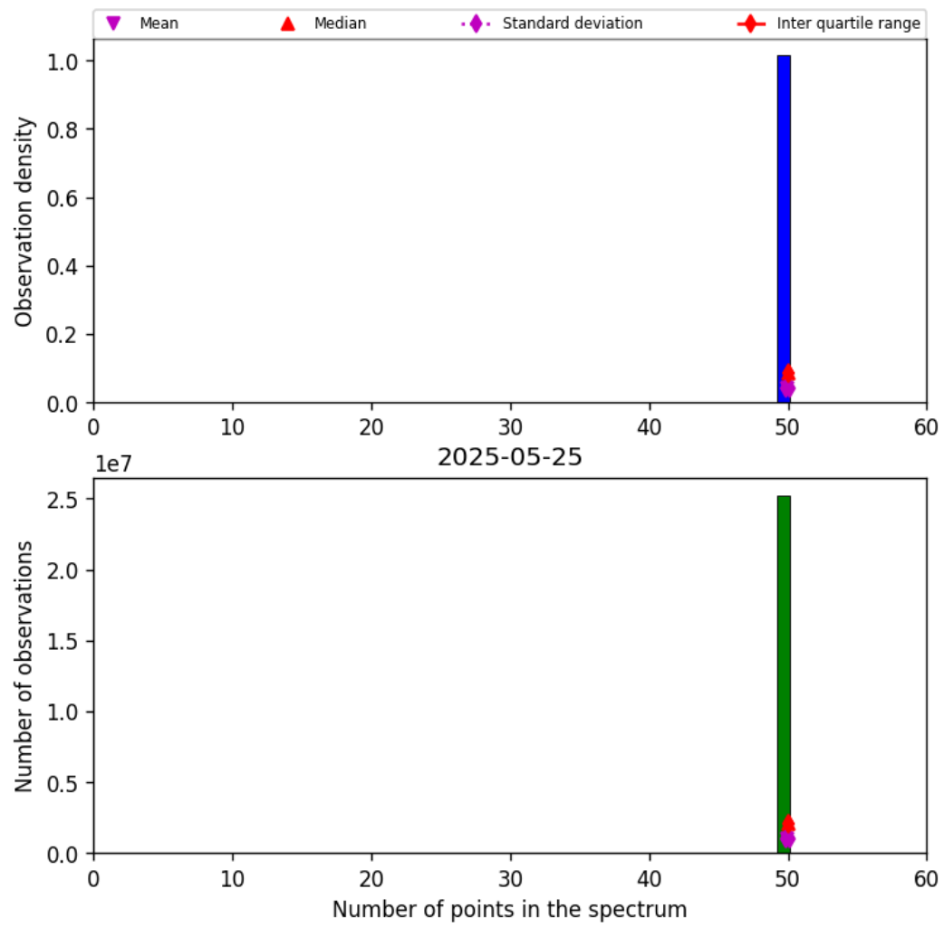
Figure 42: Histogram of “Number of points in the spectrum” for 2025-05-25 to 2025-05-26
