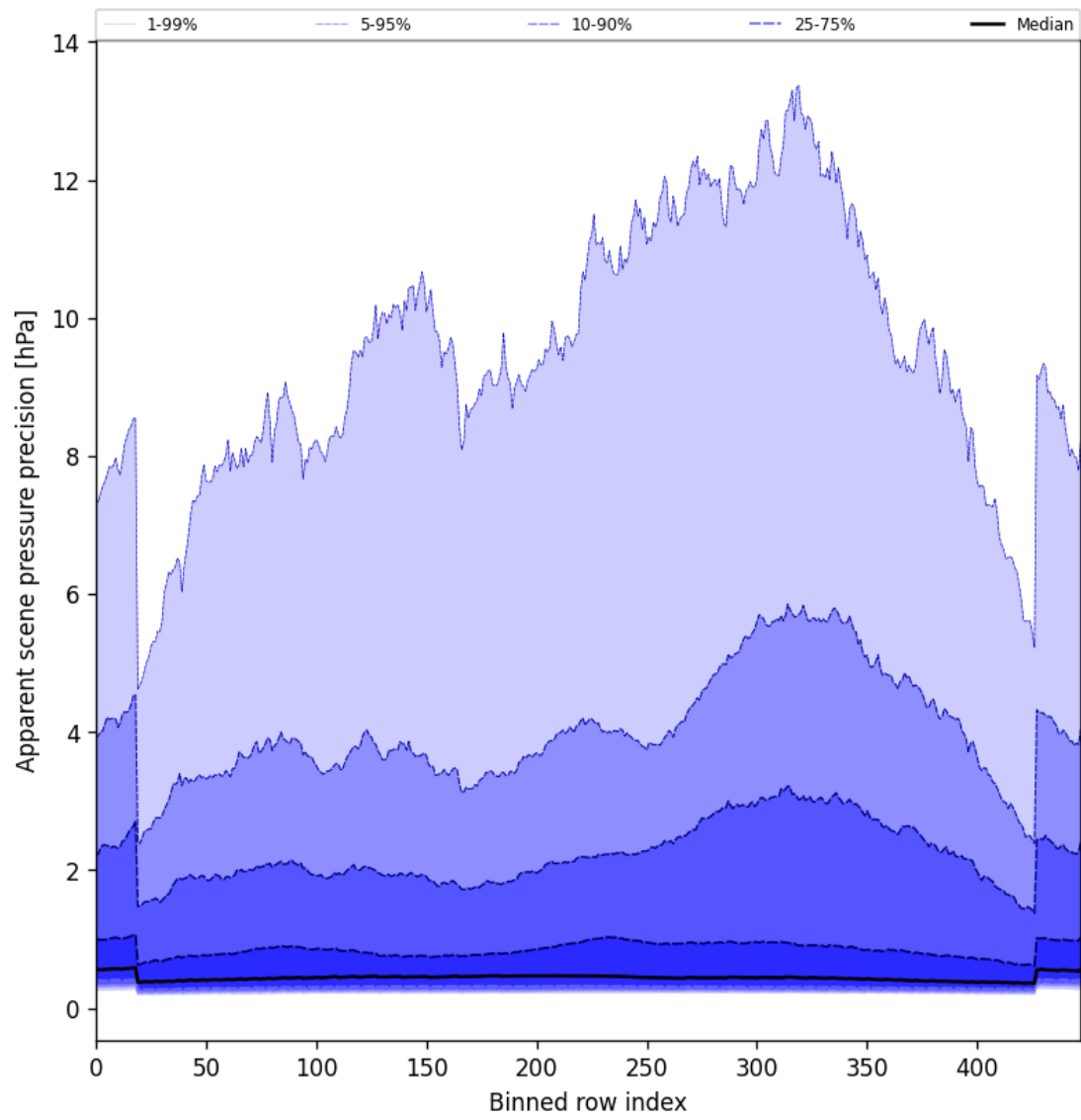
Figure 52: Along track statistics of “Apparent scene pressure precision” for 2025-05-25 to 2025-05-26
