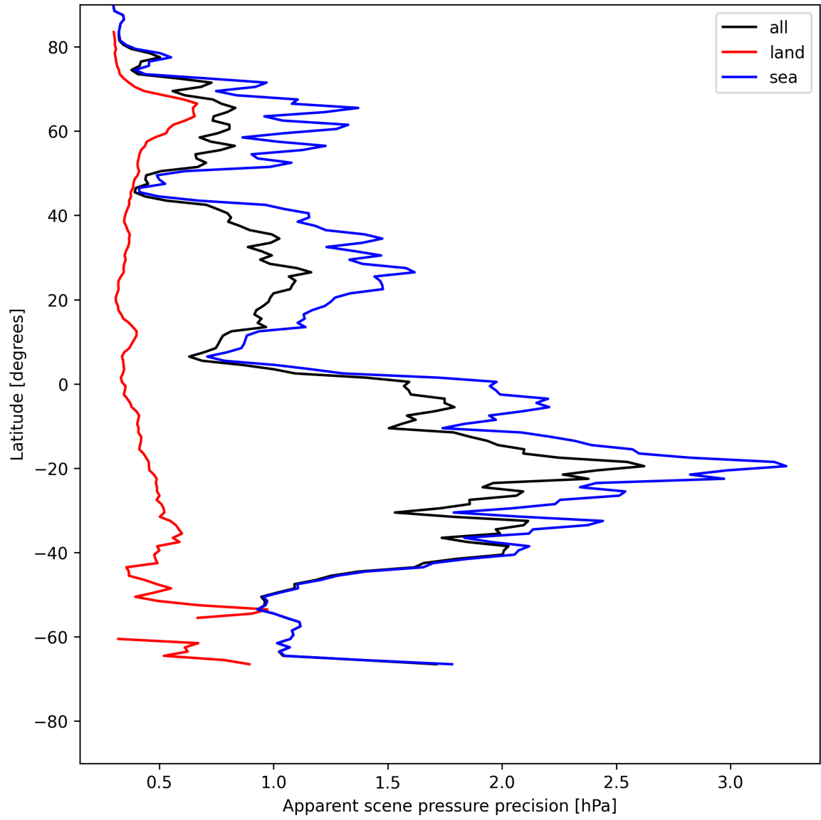
Figure 18: Zonal average of “Apparent scene pressure precision” for 2025-05-25 to 2025-05-26.
