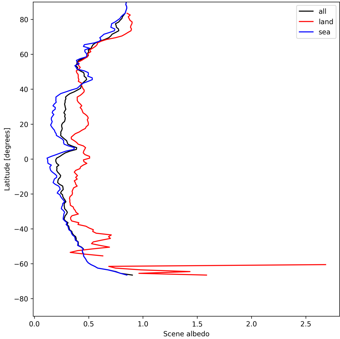
Figure 15: Zonal average of “Scene albedo” for 2025-05-25 to 2025-05-26.
