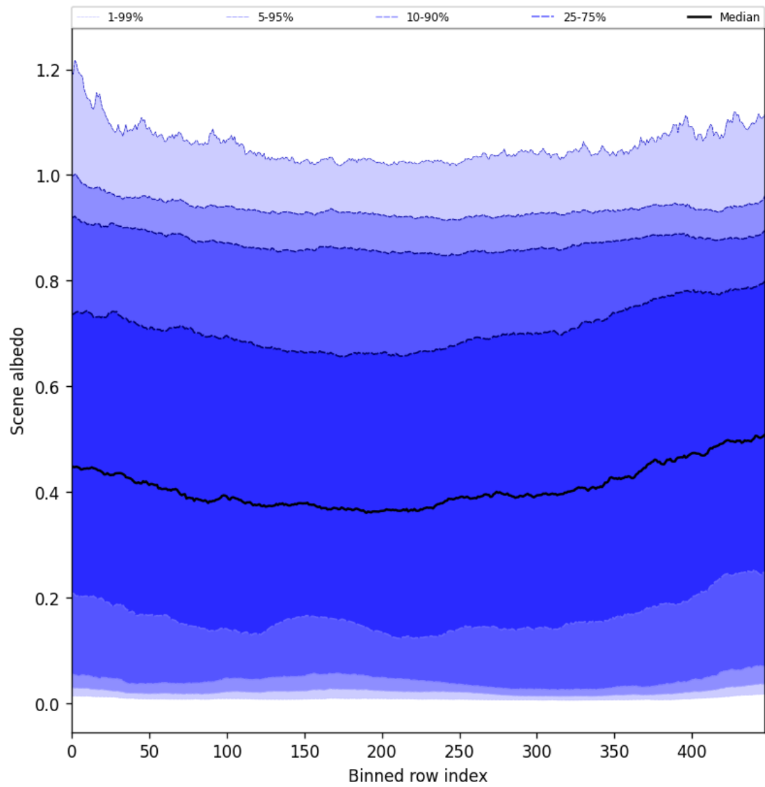
Figure 49: Along track statistics of “Scene albedo” for 2025-05-25 to 2025-05-26
