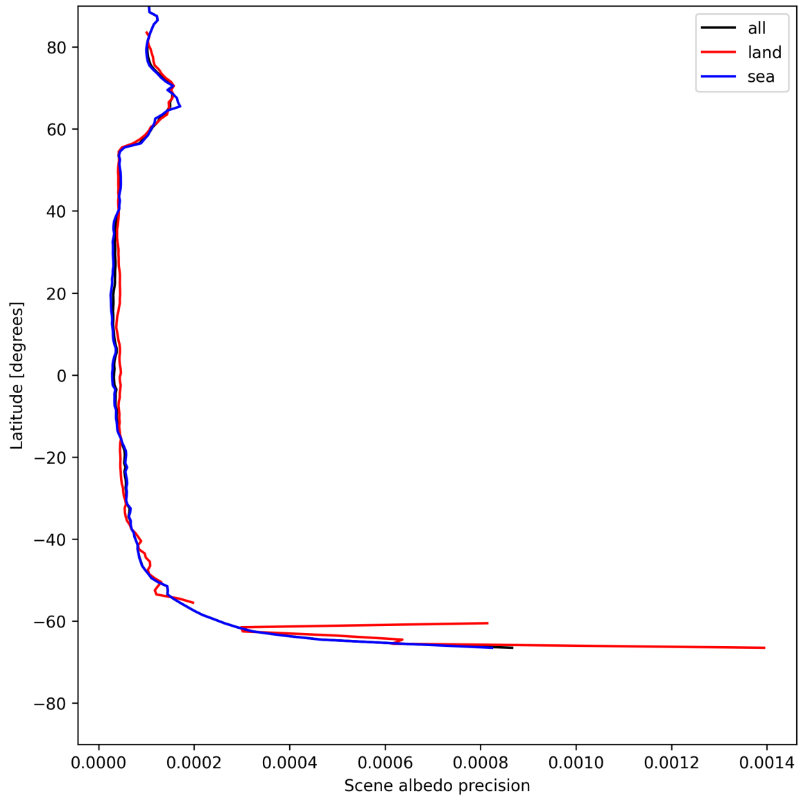
Figure 16: Zonal average of “Scene albedo precision” for 2025-05-25 to 2025-05-26.
