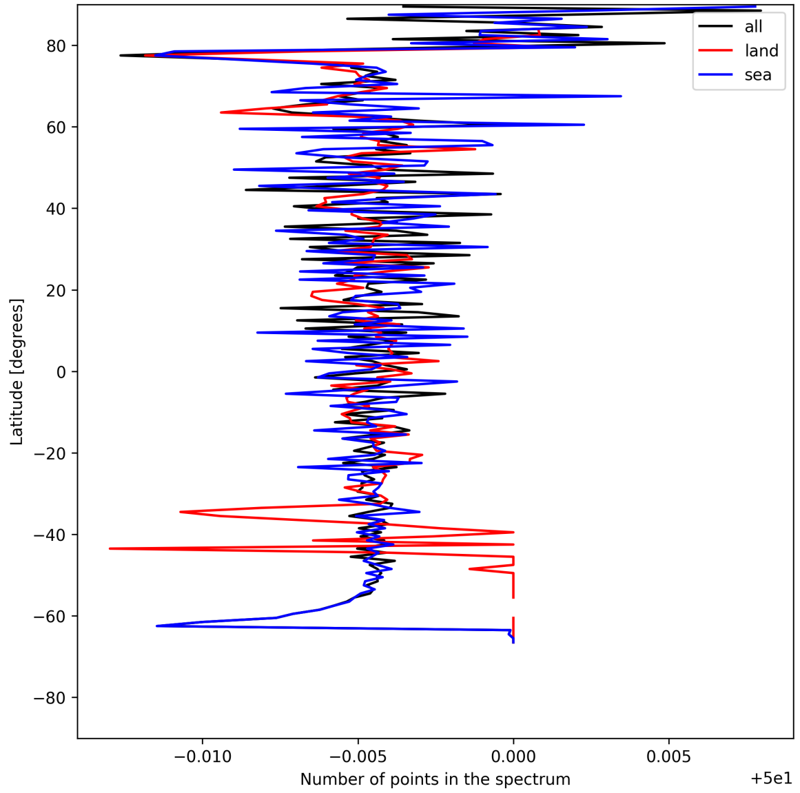
Figure 25: Zonal average of “Number of points in the spectrum” for 2025-05-25 to 2025-05-26.
