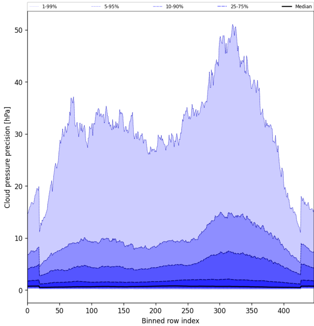
Figure 46: Along track statistics of “Cloud pressure precision” for 2025-05-25 to 2025-05-26
