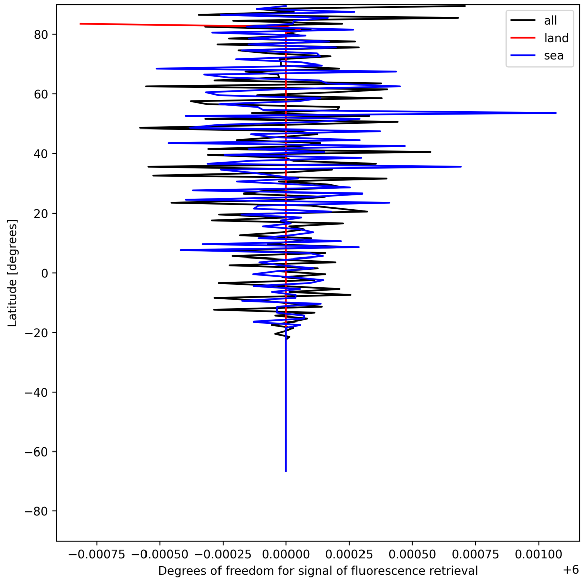
Figure 24: Zonal average of “Degrees of freedom for signal of fluorescence retrieval” for 2025-05-25 to 2025-05-26.
