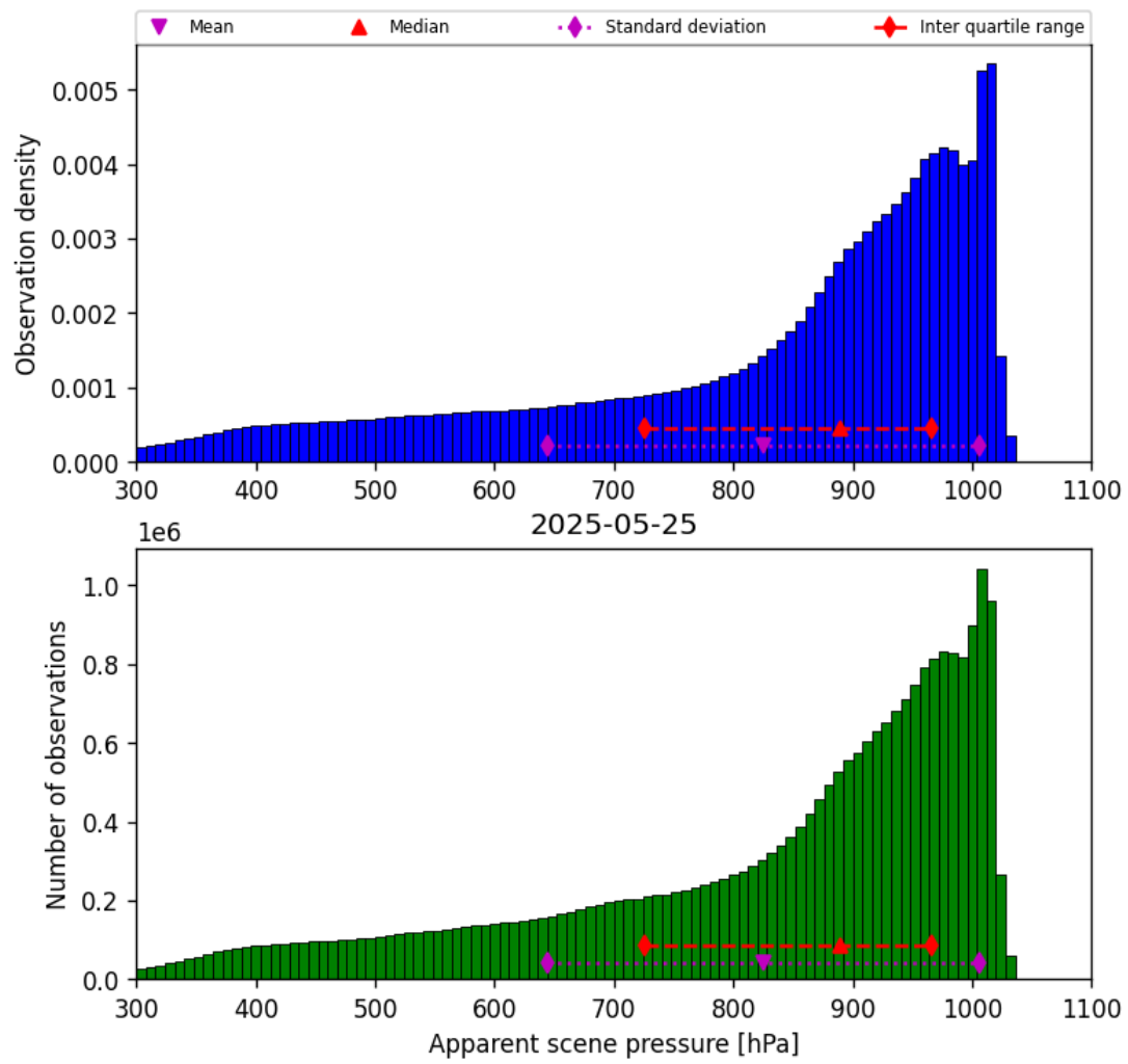
Figure 34: Histogram of “Apparent scene pressure” for 2025-05-25 to 2025-05-26
