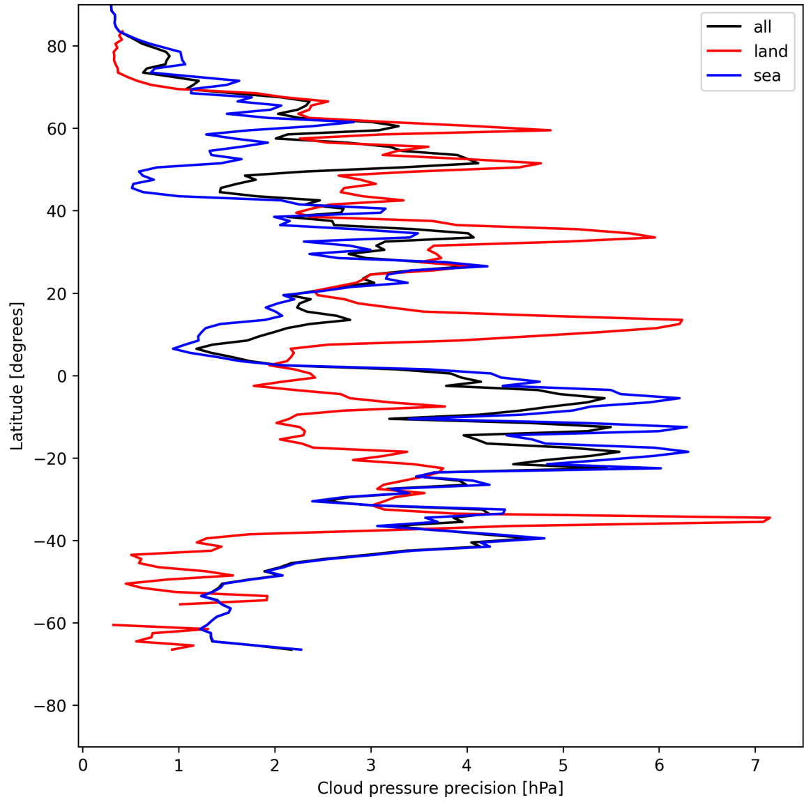
Figure 12: Zonal average of “Cloud pressure precision” for 2025-05-25 to 2025-05-26.
