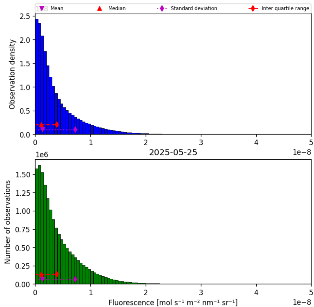
Figure 38: Histogram of “Fluorescence” for 2025-05-25 to 2025-05-26
