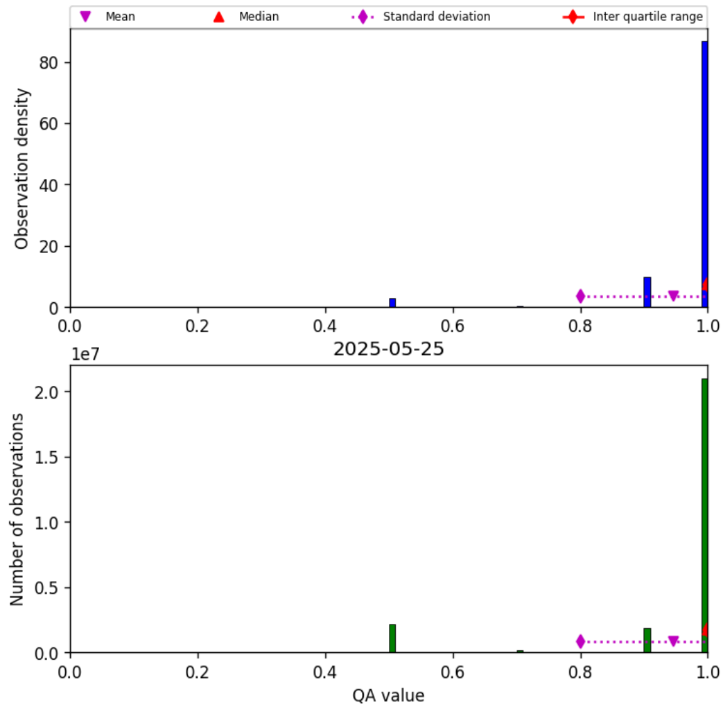
Figure 27: Histogram of “QA value” for 2025-05-25 to 2025-05-26
