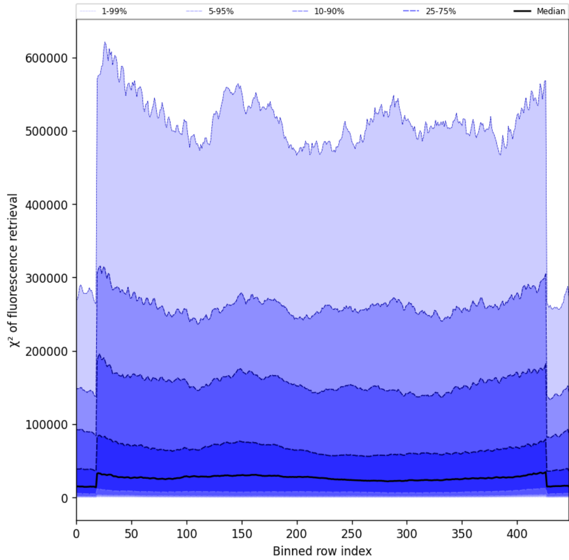
Figure 57: Along track statistics of “ \chi^2 of fluorescence retrieval” for 2025-05-25 to 2025-05-26
