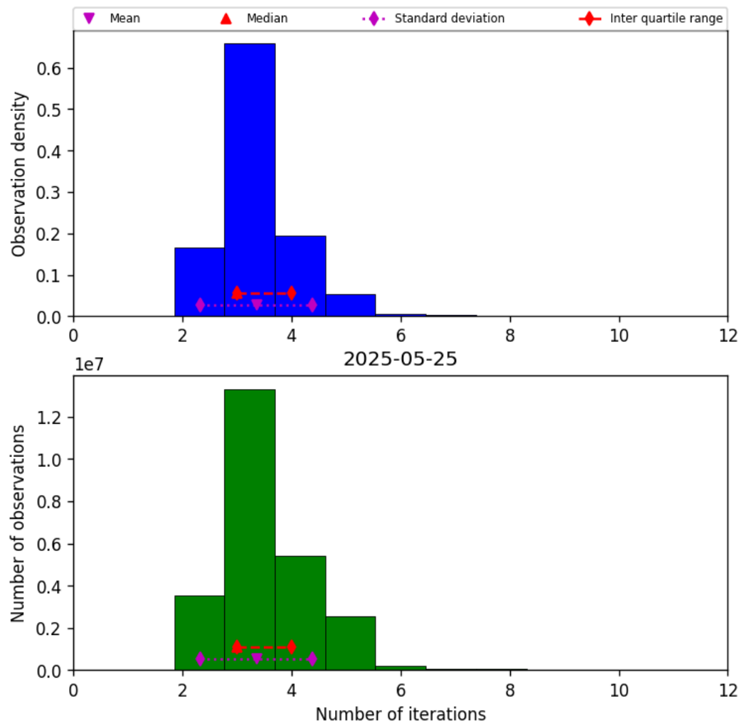
Figure 37: Histogram of “Number of iterations” for 2025-05-25 to 2025-05-26
