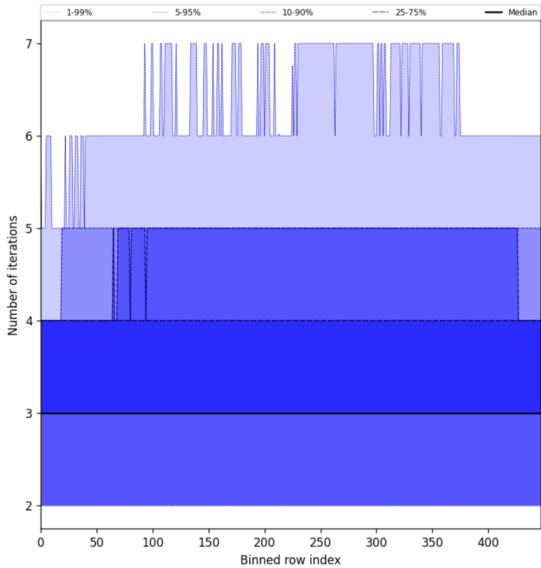
Figure 54: Along track statistics of “Number of iterations” for 2025-05-25 to 2025-05-26
