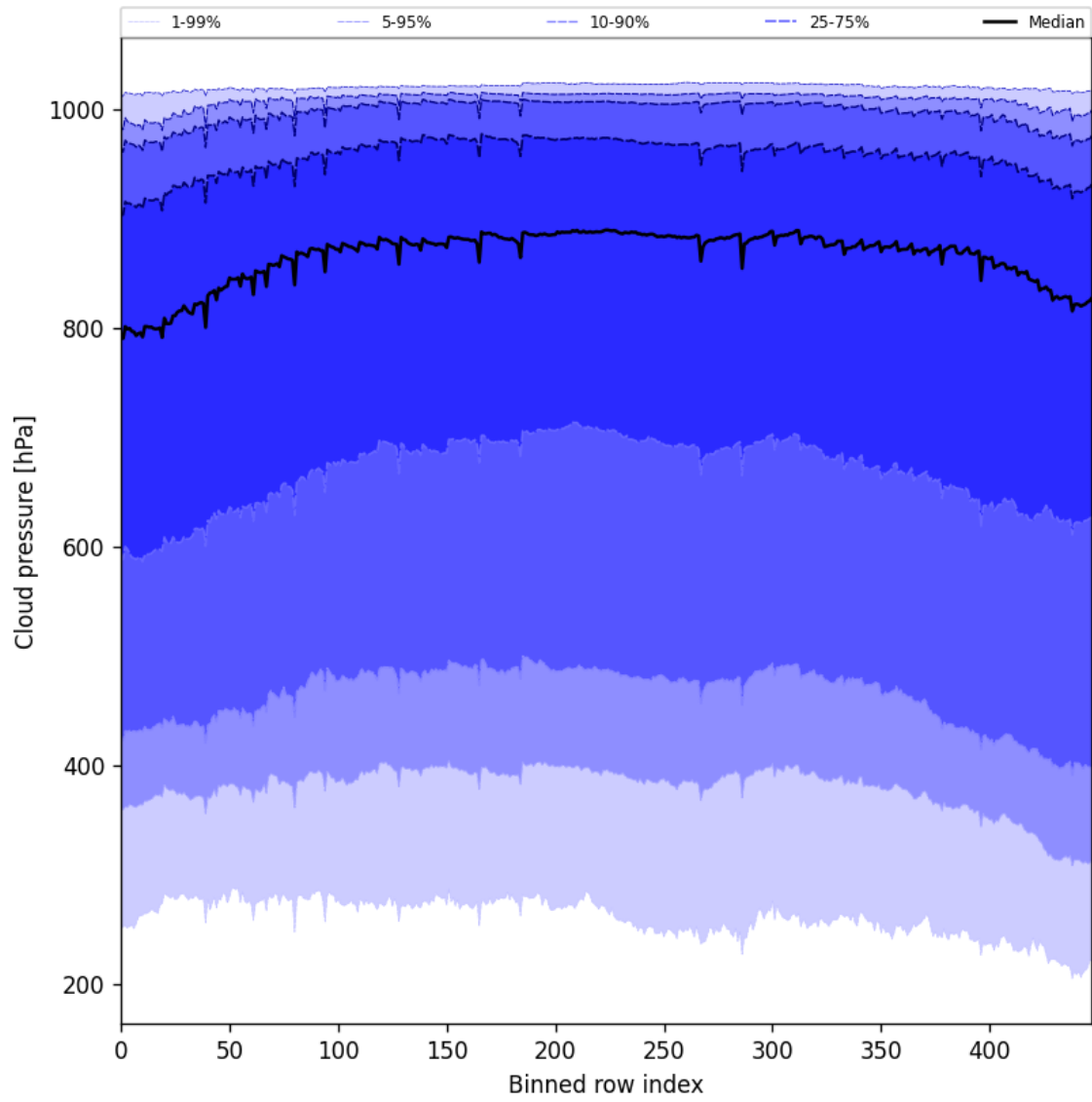
Figure 45: Along track statistics of “Cloud pressure” for 2025-05-25 to 2025-05-26
