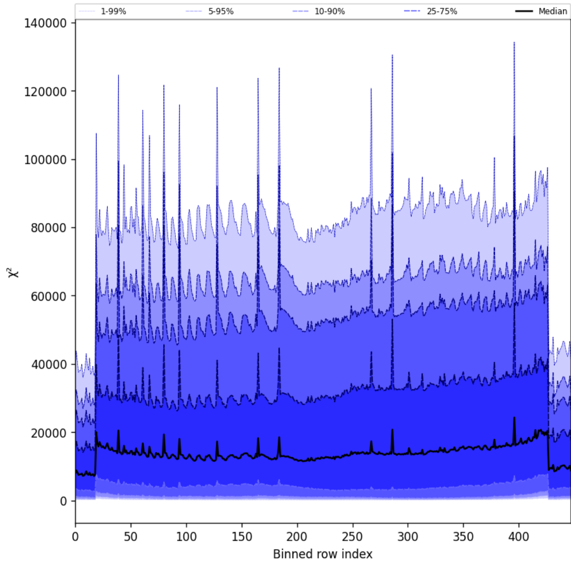
Figure 53: Along track statistics of “ \chi^2 ” for 2025-05-25 to 2025-05-26
