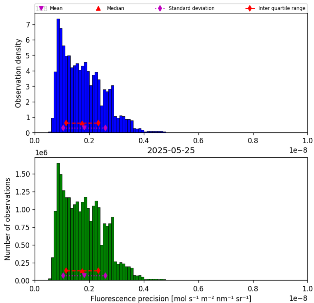
Figure 39: Histogram of “Fluorescence precision” for 2025-05-25 to 2025-05-26
