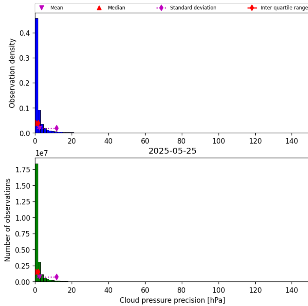
Figure 29: Histogram of “Cloud pressure precision” for 2025-05-25 to 2025-05-26
