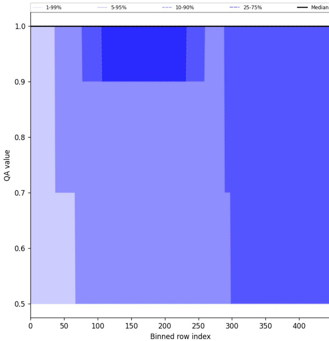
Figure 44: Along track statistics of “QA value” for 2025-05-25 to 2025-05-26
