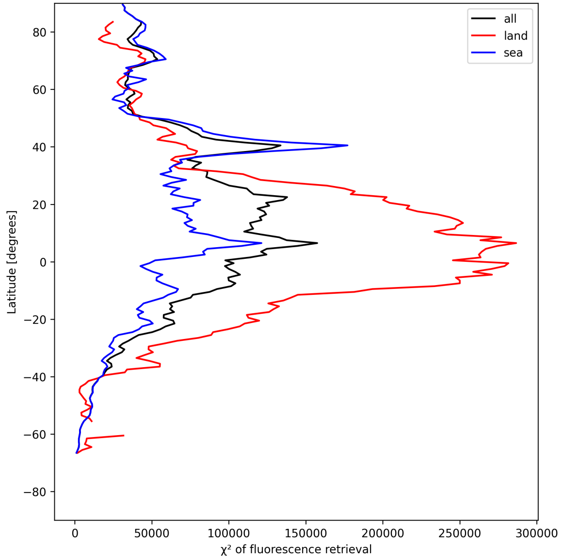
Figure 23: Zonal average of “ \chi^2 of fluorescence retrieval” for 2025-05-25 to 2025-05-26.
