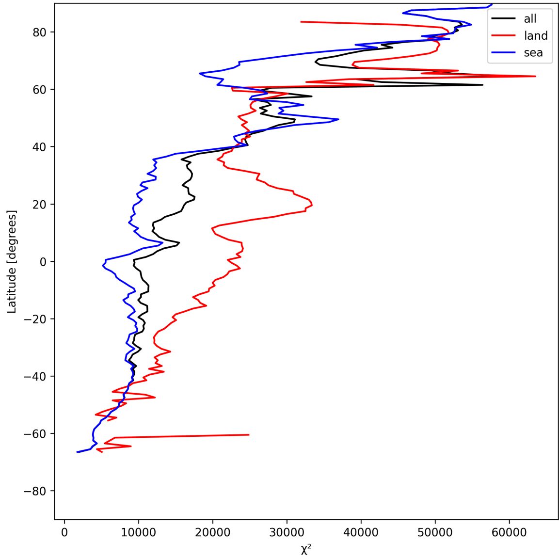
Figure 19: Zonal average of “ \chi^2 ” for 2025-05-25 to 2025-05-26.
