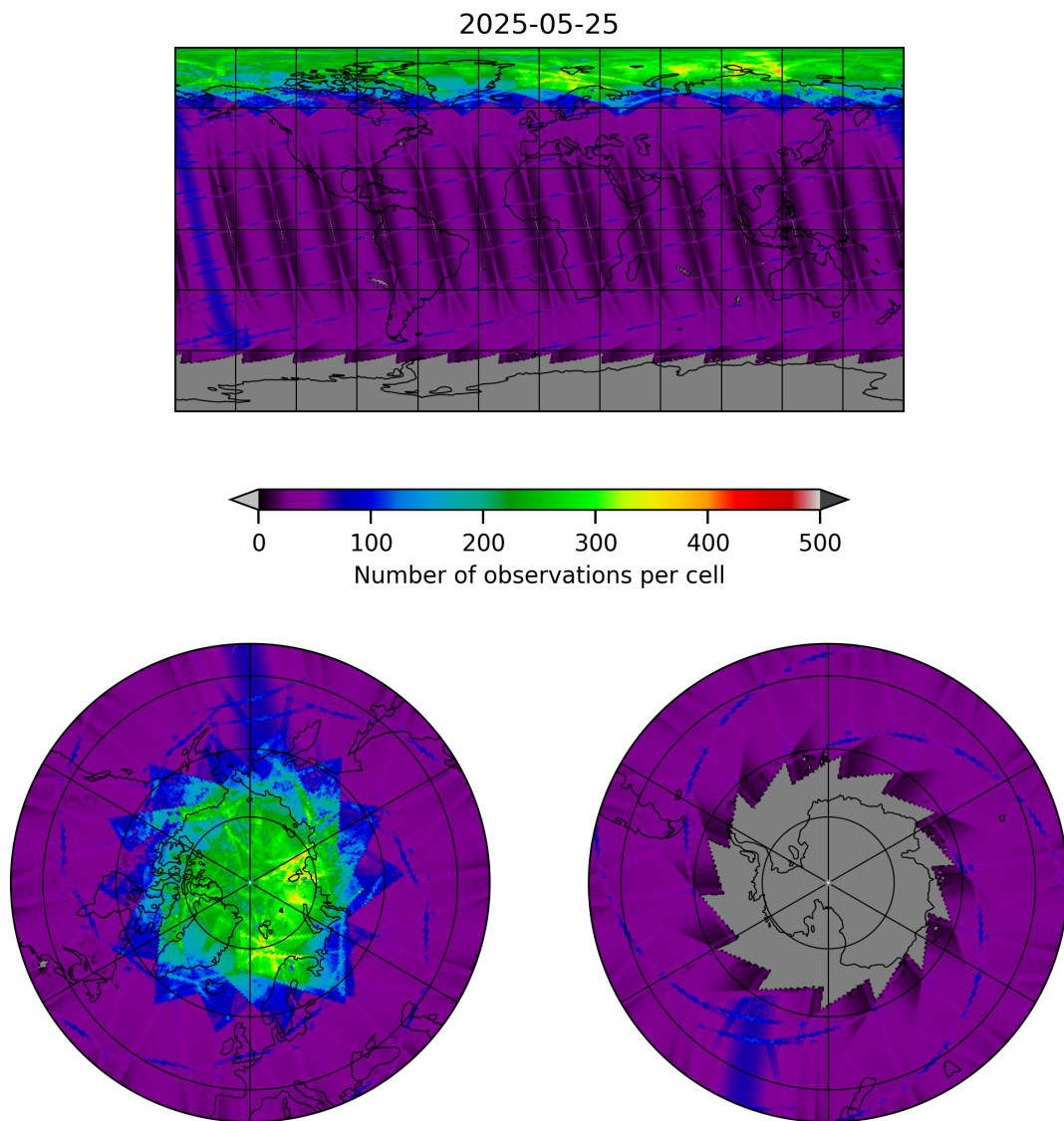
Figure 9: Map of the number of observations for 2025-05-25 to 2025-05-26
