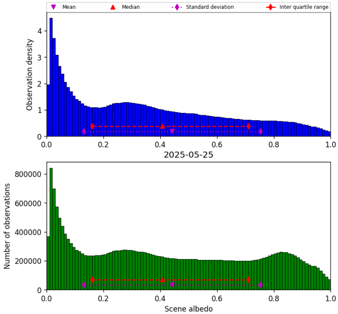
Figure 32: Histogram of “Scene albedo” for 2025-05-25 to 2025-05-26
