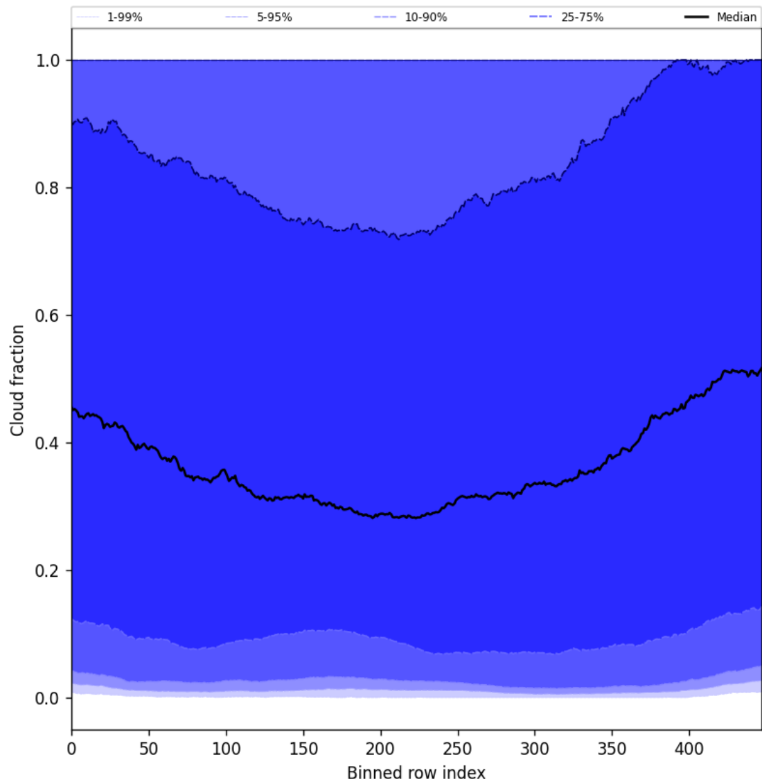
Figure 47: Along track statistics of “Cloud fraction” for 2025-05-25 to 2025-05-26
