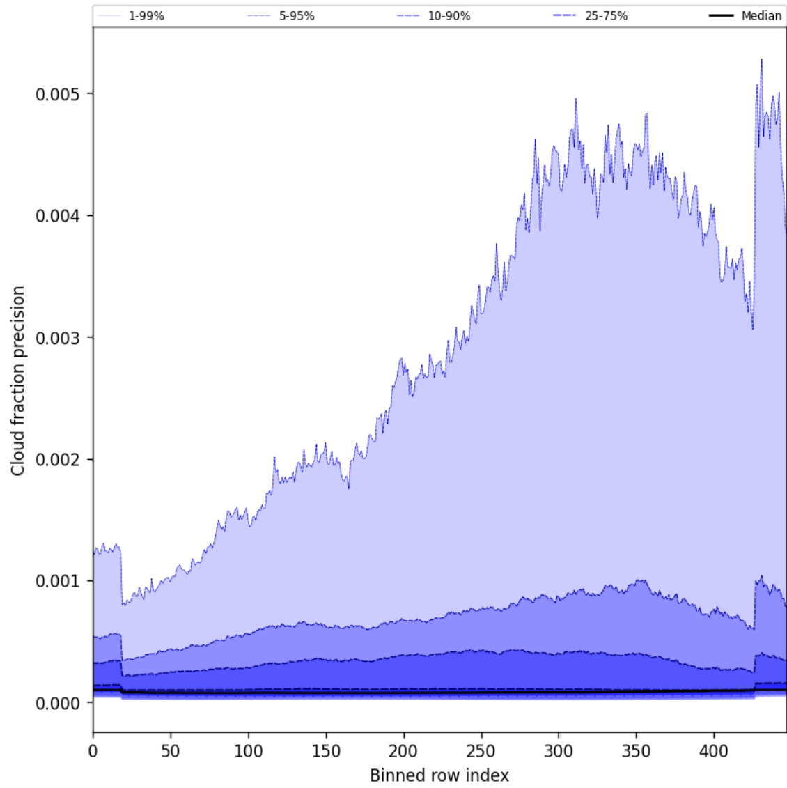
Figure 48: Along track statistics of “Cloud fraction precision” for 2025-05-25 to 2025-05-26
