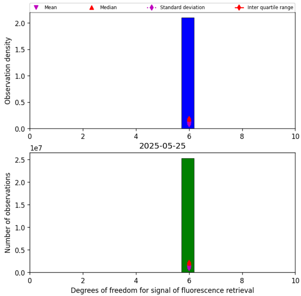
Figure 41: Histogram of “Degrees of freedom for signal of fluorescence retrieval” for 2025-05-25 to 2025-05-26
