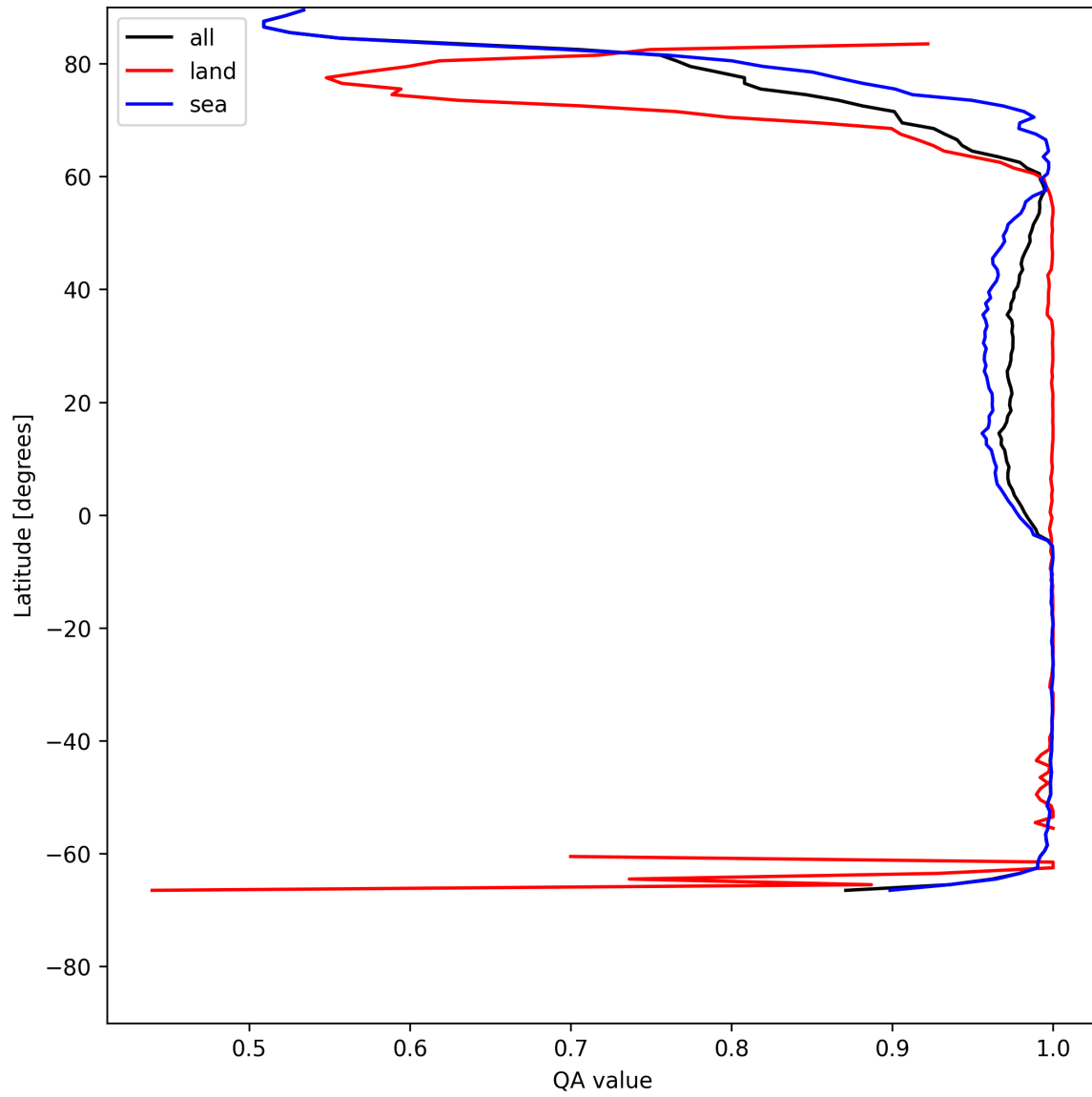
Figure 10: Zonal average of “QA value” for 2025-05-25 to 2025-05-26.
