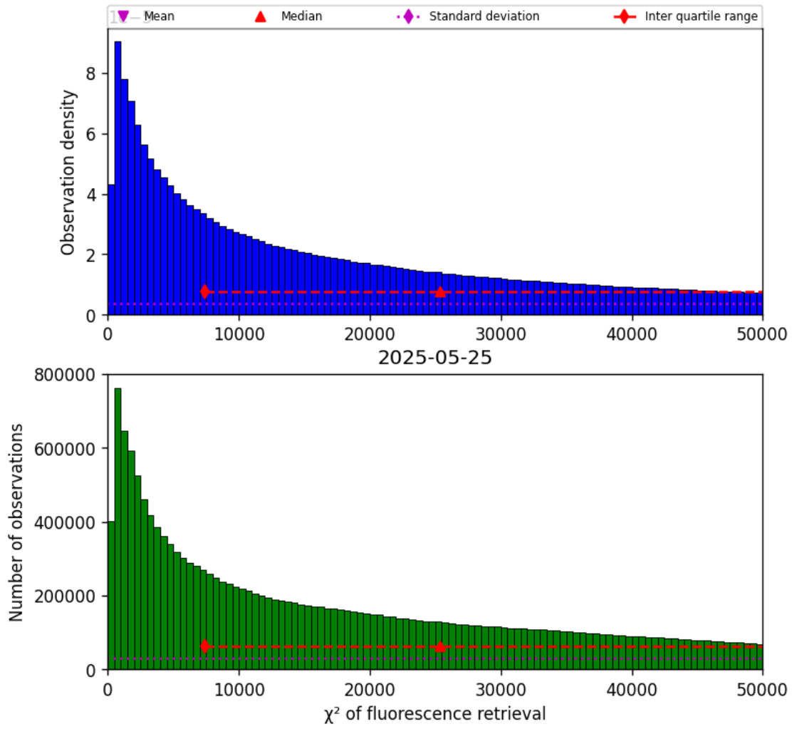
Figure 40: Histogram of “ \chi^2 of fluorescence retrieval” for 2025-05-25 to 2025-05-26
