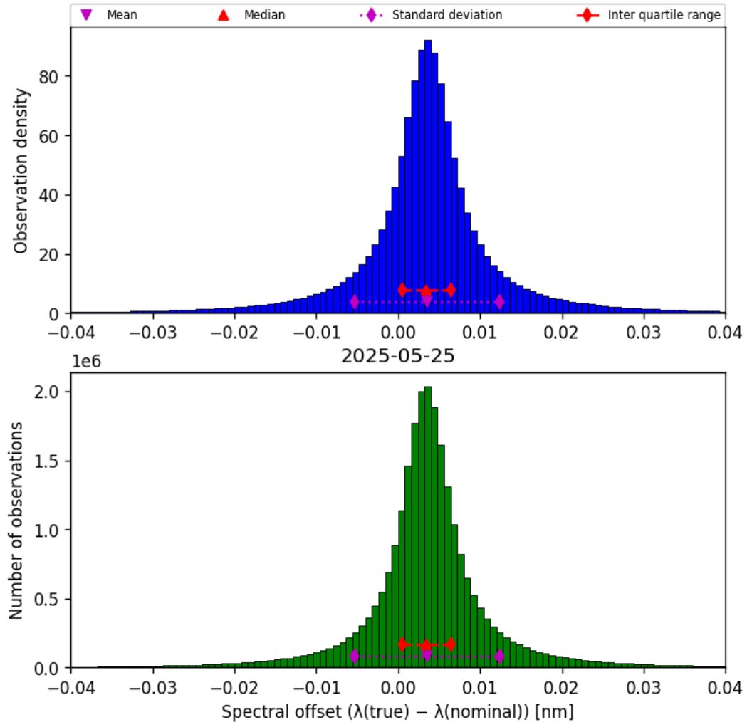
Figure 43: Histogram of “Spectral offset ( \lambda_{\text{true}} - \lambda_{\text{nominal}} )” for 2025-05-25 to 2025-05-26
