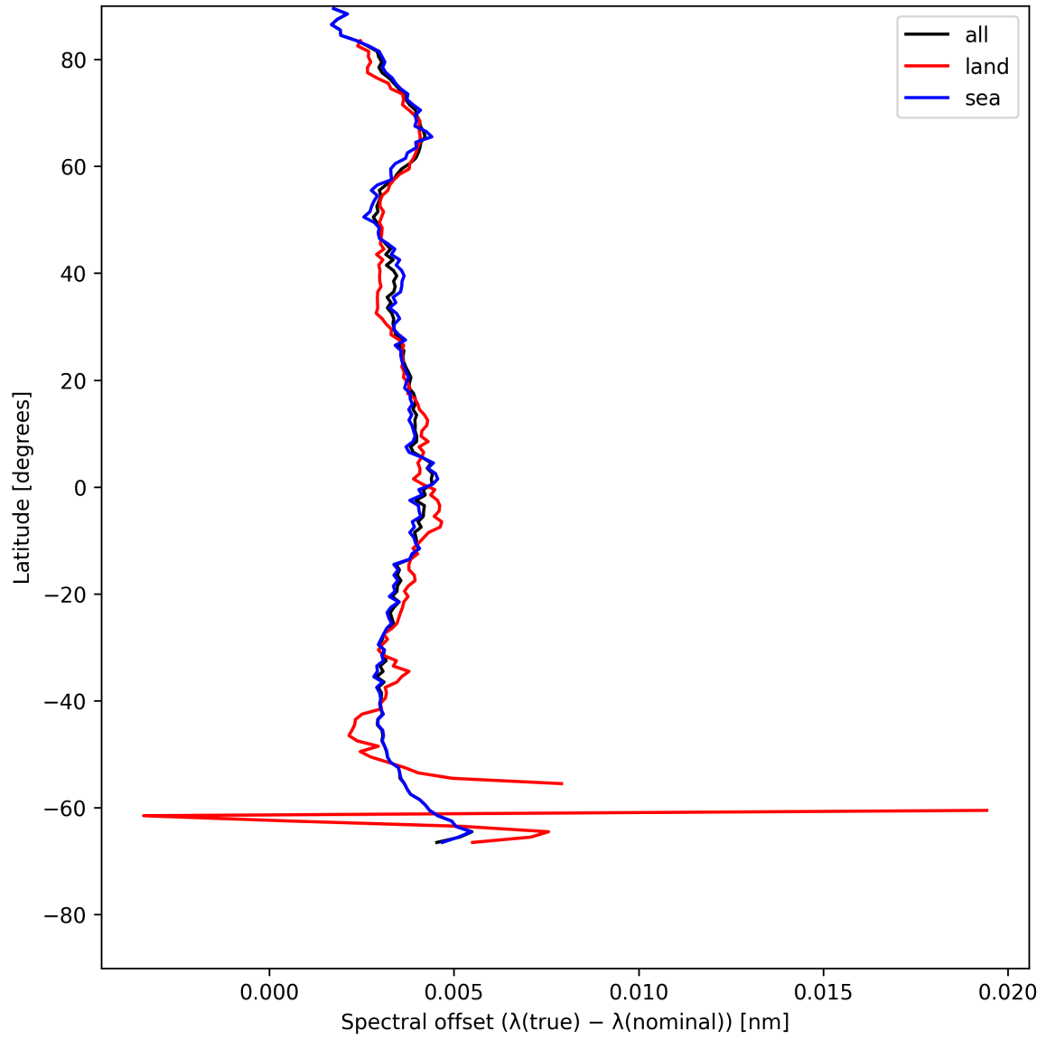
Figure 26: Zonal average of “Spectral offset ( \lambda_{\text{true}} - \lambda_{\text{nominal}} )” for 2025-05-25 to 2025-05-26.
