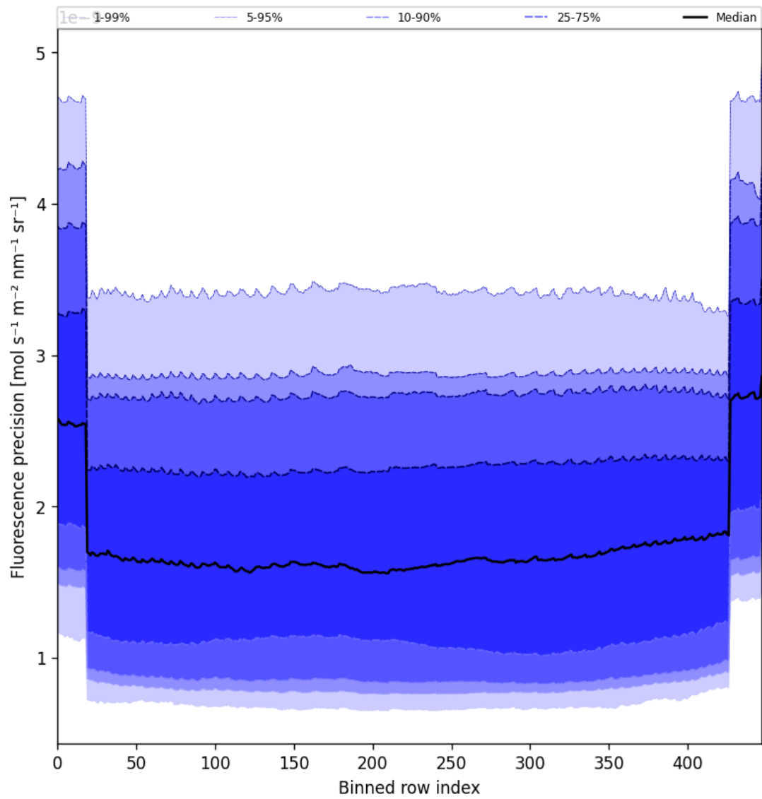
Figure 56: Along track statistics of “Fluorescence precision” for 2025-05-25 to 2025-05-26
