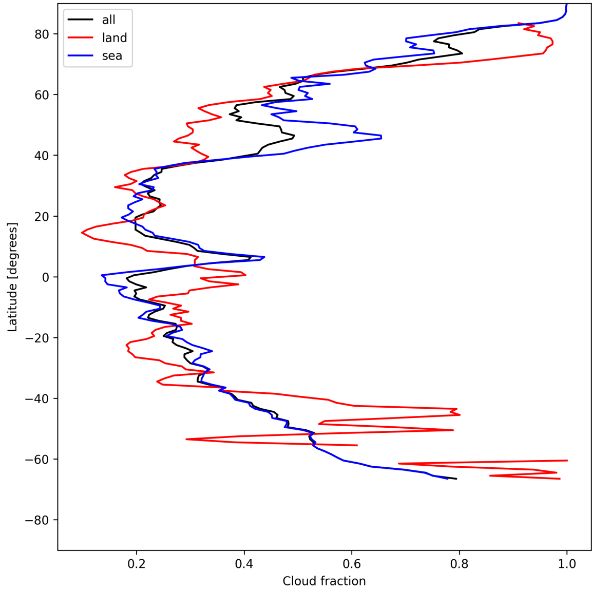
Figure 13: Zonal average of “Cloud fraction” for 2025-05-25 to 2025-05-26.
