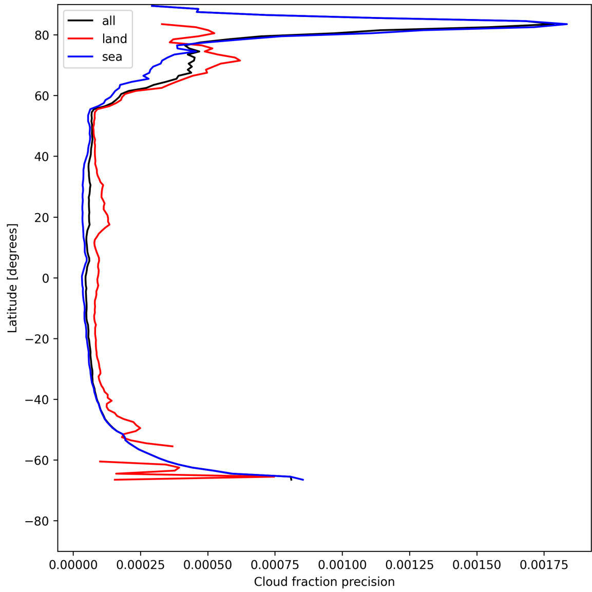
Figure 14: Zonal average of “Cloud fraction precision” for 2025-05-25 to 2025-05-26.
