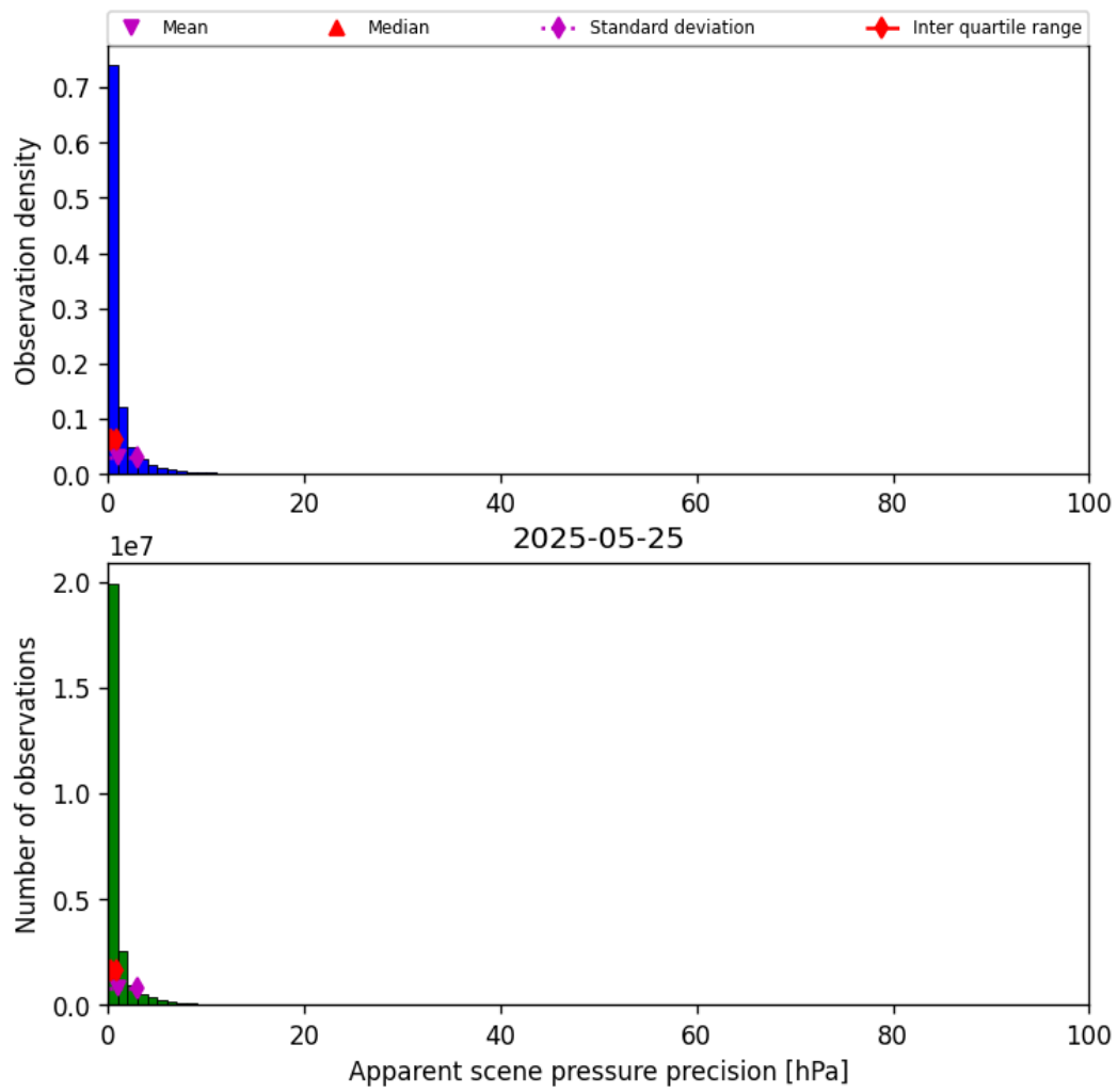
Figure 35: Histogram of “Apparent scene pressure precision” for 2025-05-25 to 2025-05-26
