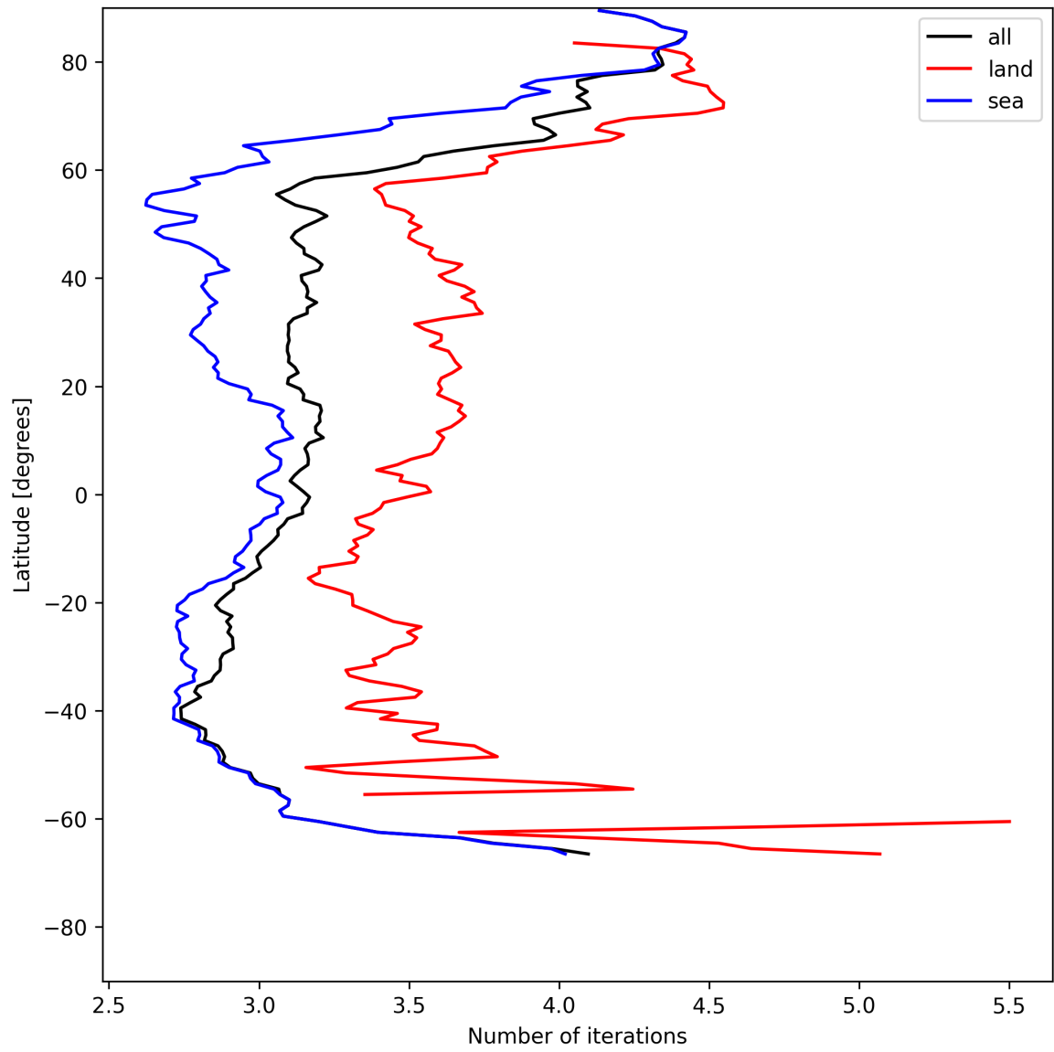
Figure 20: Zonal average of “Number of iterations” for 2025-05-25 to 2025-05-26.
