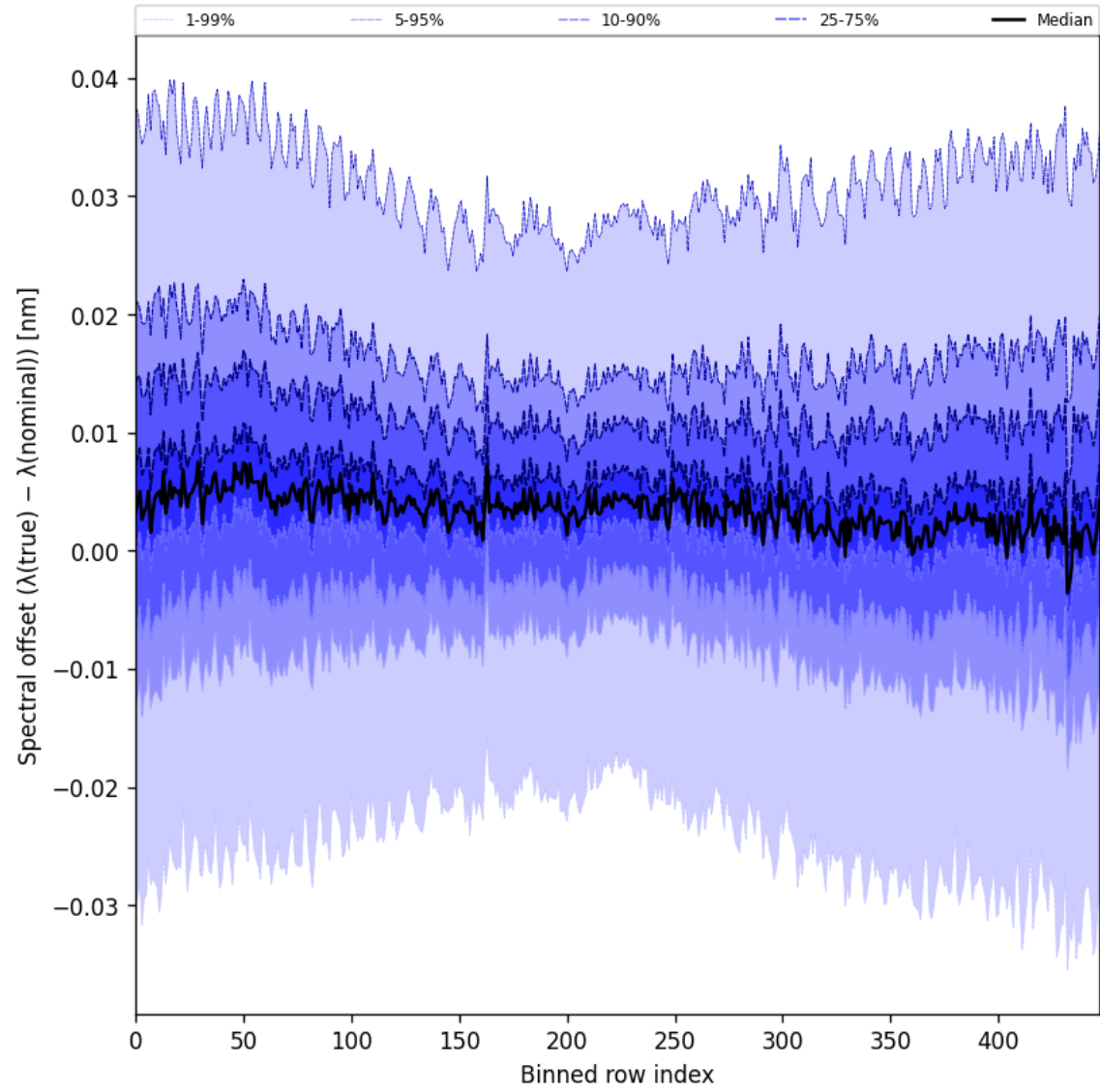
Figure 60: Along track statistics of “Spectral offset ( \lambda_{\text{true}} - \lambda_{\text{nominal}} )” for 2025-05-25 to 2025-05-26
