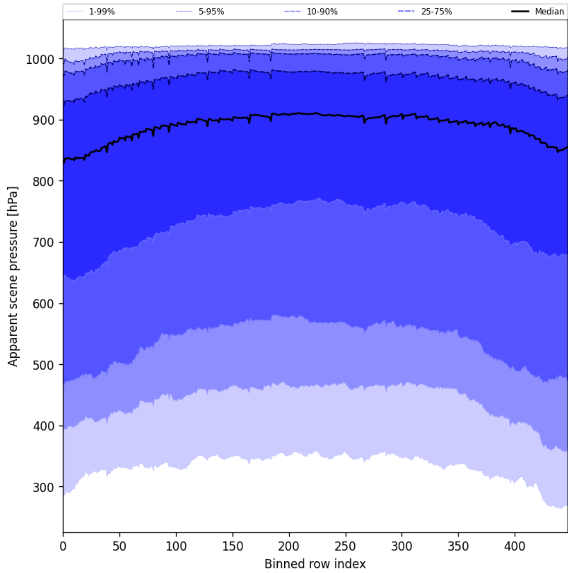
Figure 51: Along track statistics of “Apparent scene pressure” for 2025-05-25 to 2025-05-26
