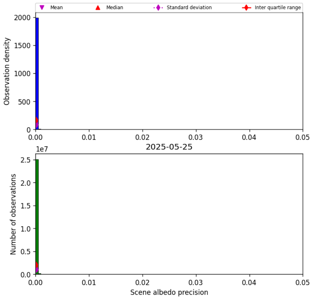
Figure 33: Histogram of “Scene albedo precision” for 2025-05-25 to 2025-05-26
