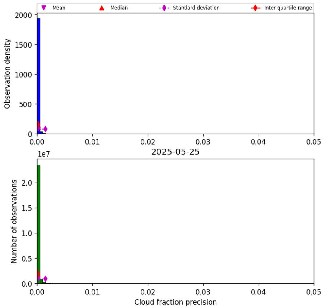
Figure 31: Histogram of “Cloud fraction precision” for 2025-05-25 to 2025-05-26
