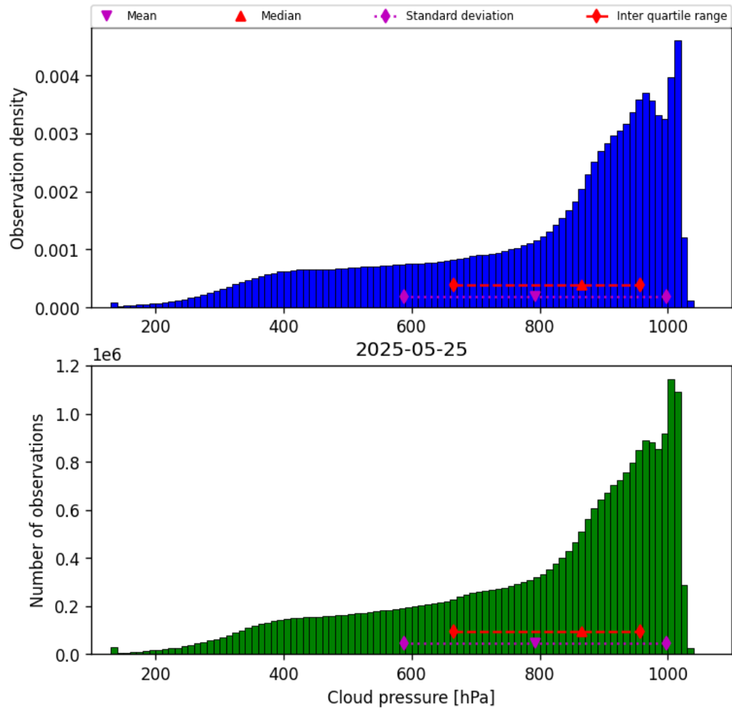
Figure 28: Histogram of “Cloud pressure” for 2025-05-25 to 2025-05-26
