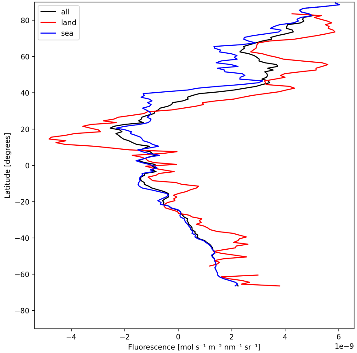
Figure 21: Zonal average of “Fluorescence” for 2025-05-25 to 2025-05-26.
