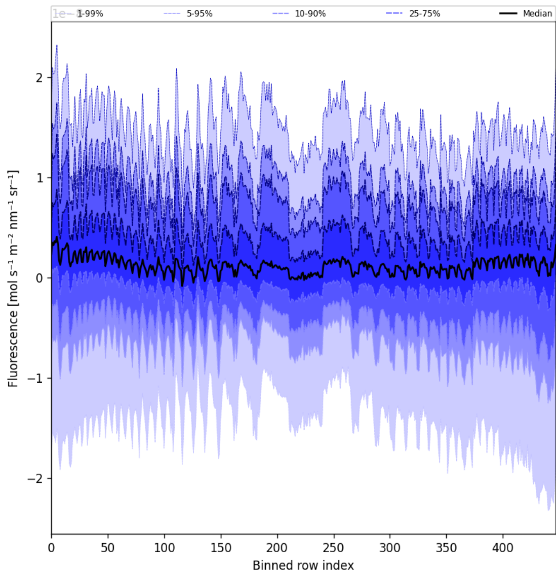
Figure 55: Along track statistics of “Fluorescence” for 2025-05-25 to 2025-05-26
