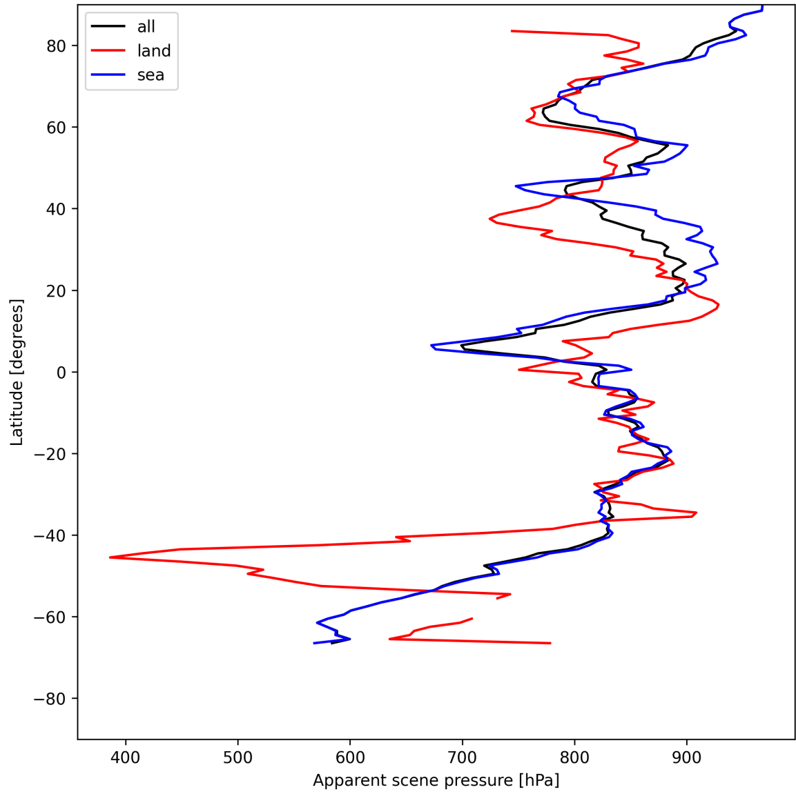
Figure 17: Zonal average of “Apparent scene pressure” for 2025-05-25 to 2025-05-26.
