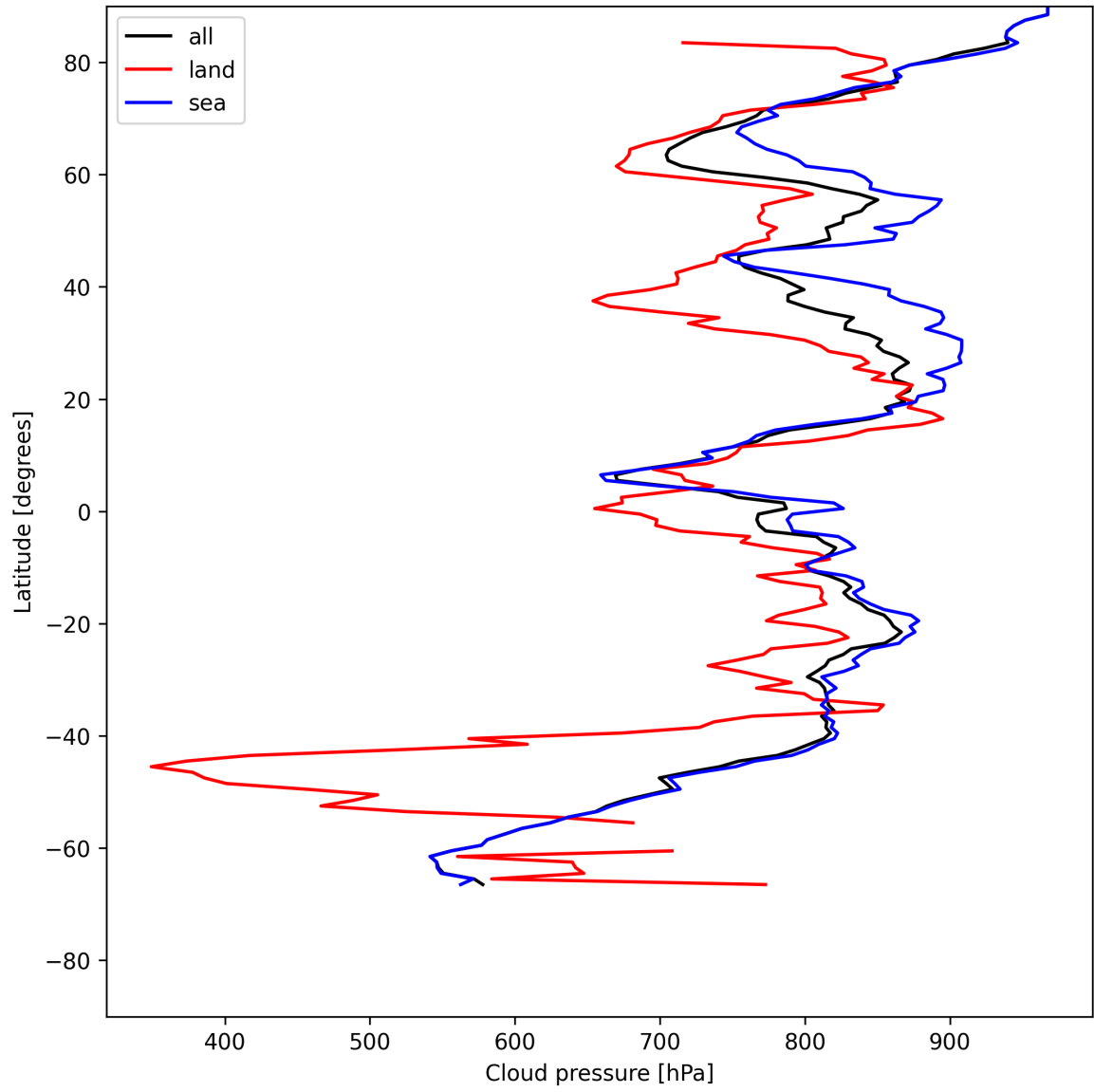
Figure 11: Zonal average of “Cloud pressure” for 2025-05-25 to 2025-05-26.
