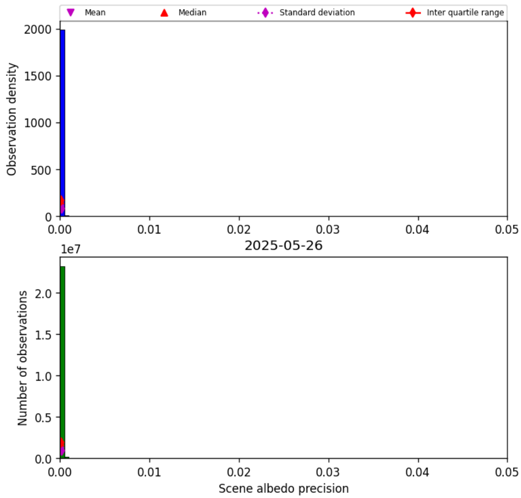
Figure 33: Histogram of “Scene albedo precision” for 2025-05-26 to 2025-05-27
