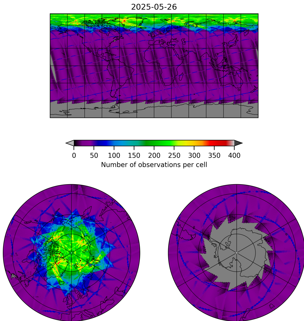
Figure 9: Map of the number of observations for 2025-05-26 to 2025-05-27
