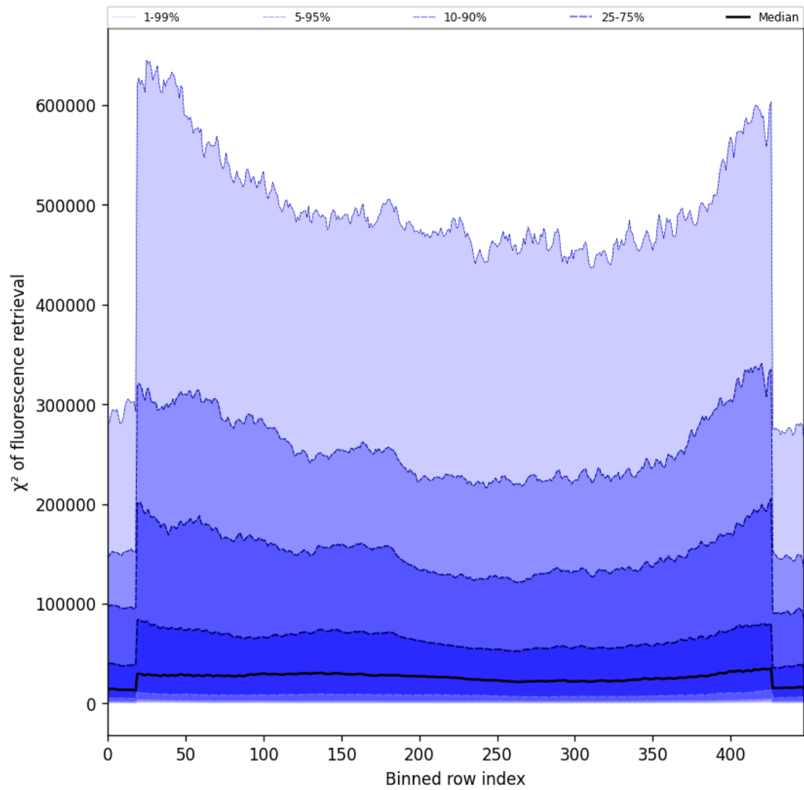
Figure 57: Along track statistics of “ \chi^2 of fluorescence retrieval” for 2025-05-26 to 2025-05-27
