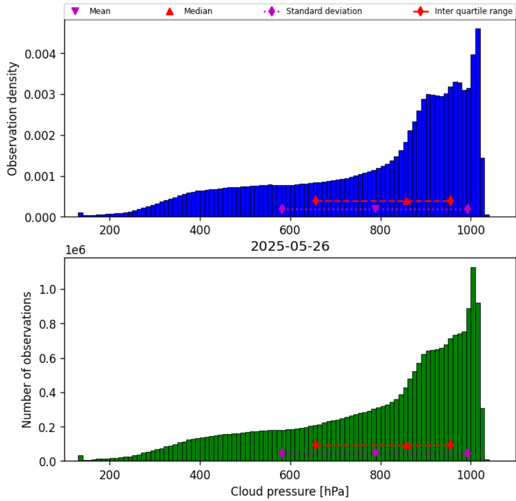
Figure 28: Histogram of “Cloud pressure” for 2025-05-26 to 2025-05-27
