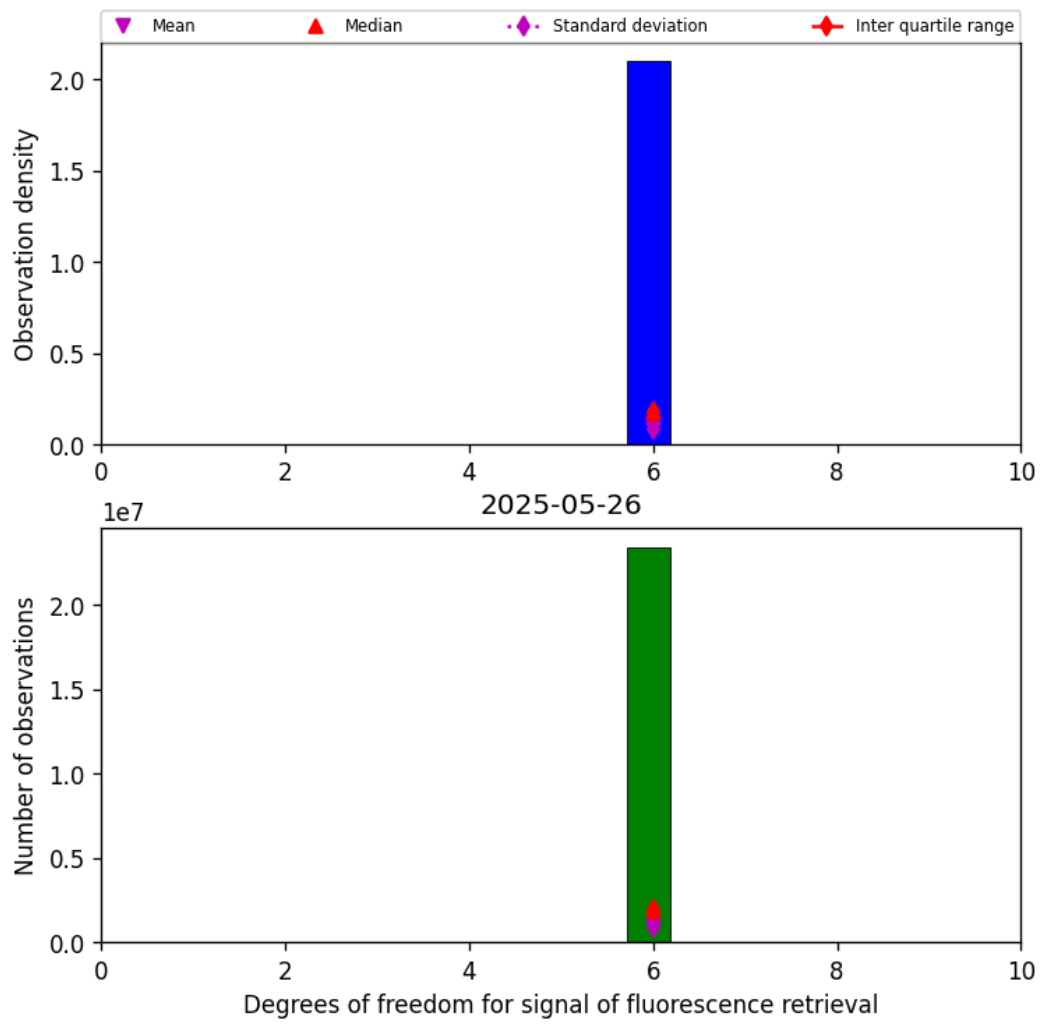
Figure 41: Histogram of “Degrees of freedom for signal of fluorescence retrieval” for 2025-05-26 to 2025-05-27
