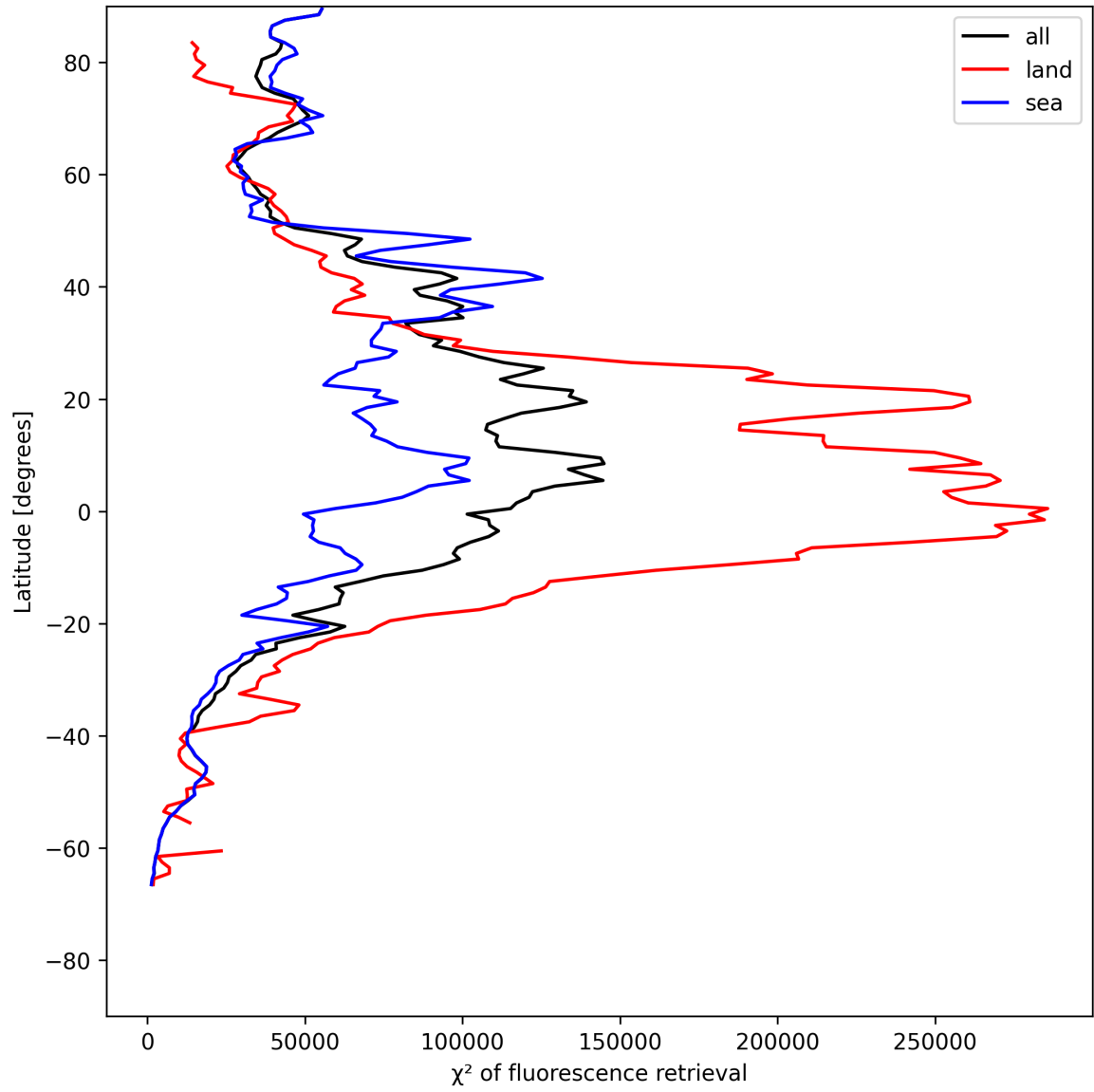
Figure 23: Zonal average of “ \chi^2 of fluorescence retrieval” for 2025-05-26 to 2025-05-27.
