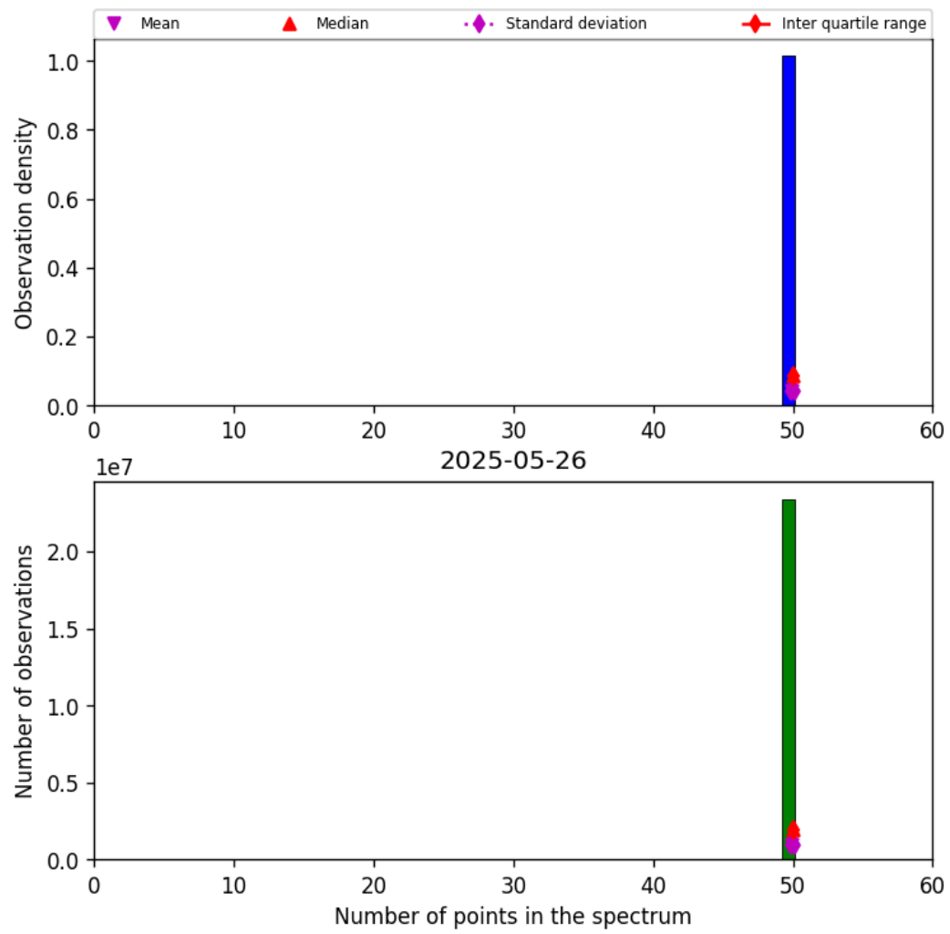
Figure 42: Histogram of “Number of points in the spectrum” for 2025-05-26 to 2025-05-27
