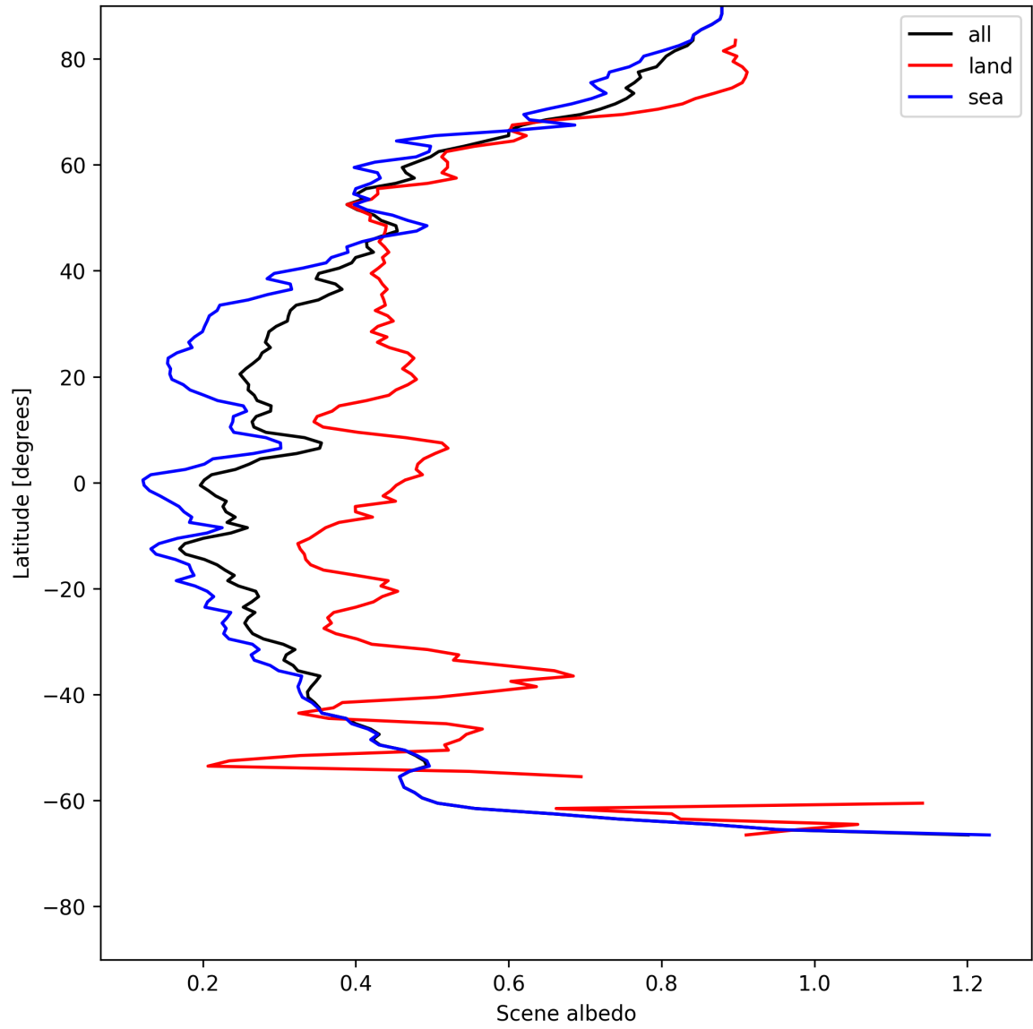
Figure 15: Zonal average of “Scene albedo” for 2025-05-26 to 2025-05-27.
