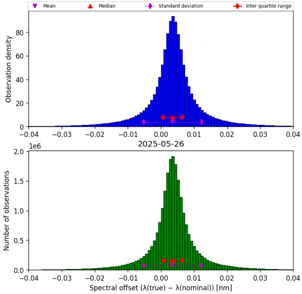
Figure 43: Histogram of “Spectral offset ( \lambda_{\text{true}} - \lambda_{\text{nominal}} )” for 2025-05-26 to 2025-05-27
