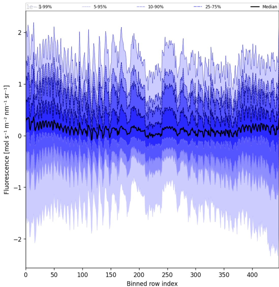
Figure 55: Along track statistics of “Fluorescence” for 2025-05-26 to 2025-05-27
