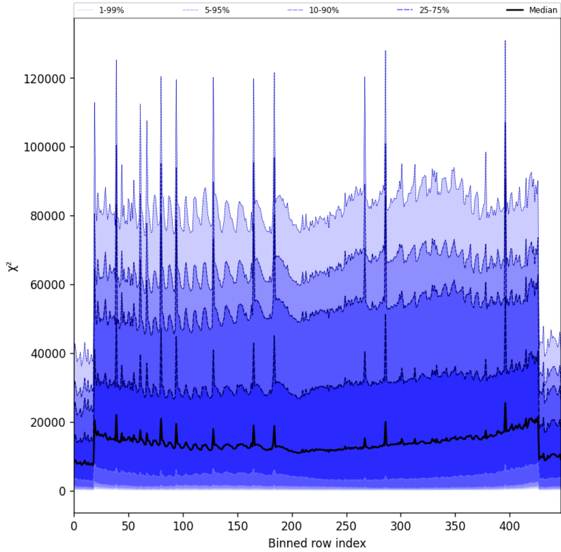
Figure 53: Along track statistics of “ \chi^2 ” for 2025-05-26 to 2025-05-27
