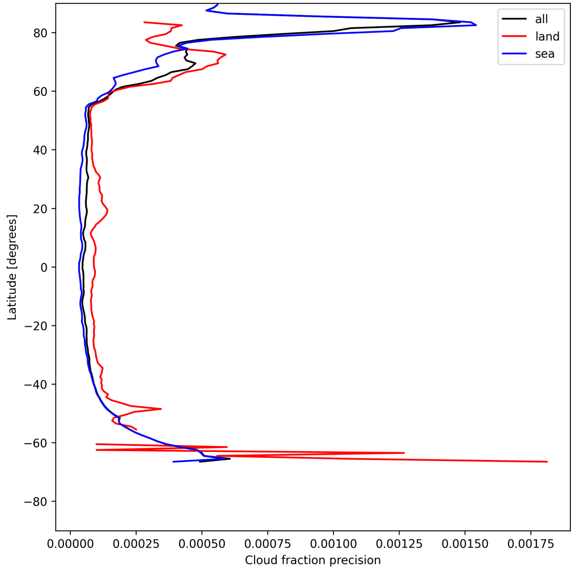
Figure 14: Zonal average of “Cloud fraction precision” for 2025-05-26 to 2025-05-27.
