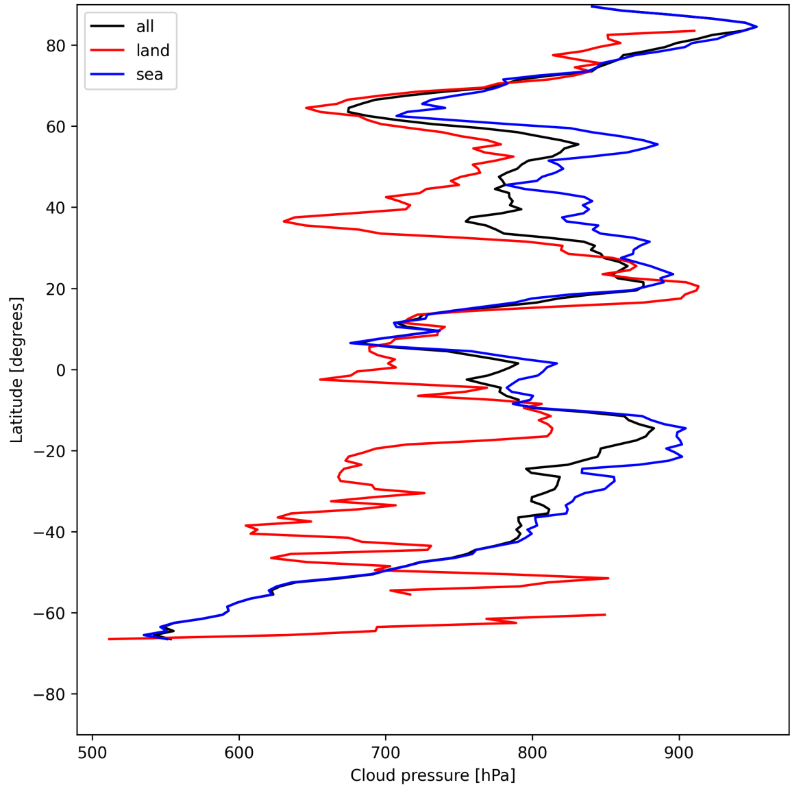
Figure 11: Zonal average of “Cloud pressure” for 2025-05-26 to 2025-05-27.
