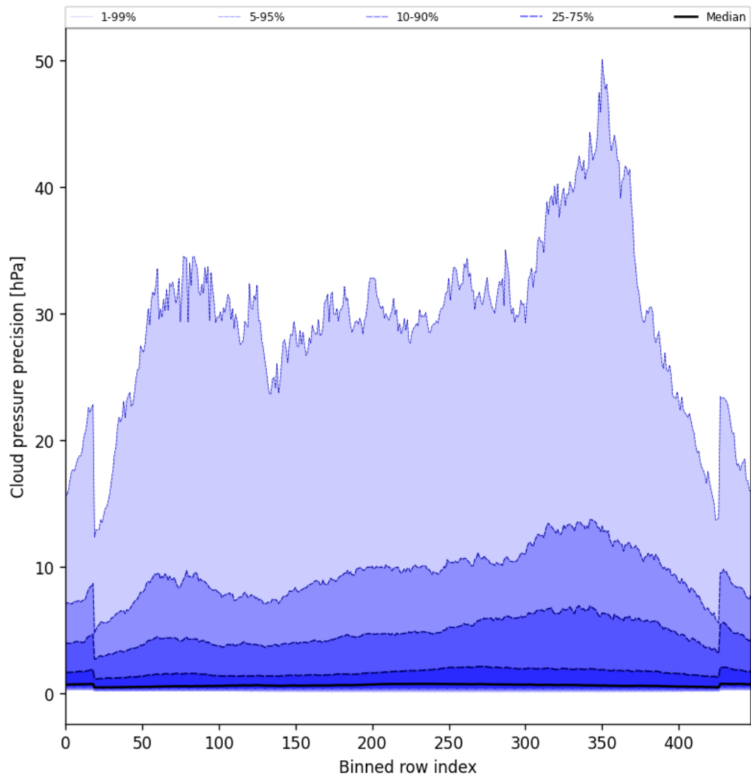
Figure 46: Along track statistics of “Cloud pressure precision” for 2025-05-26 to 2025-05-27
