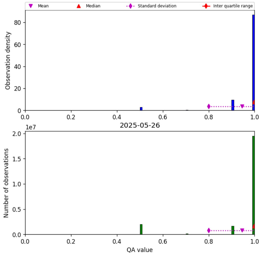
Figure 27: Histogram of “QA value” for 2025-05-26 to 2025-05-27
