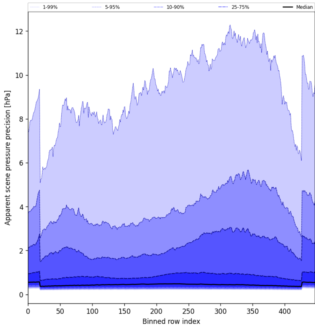
Figure 52: Along track statistics of “Apparent scene pressure precision” for 2025-05-26 to 2025-05-27
