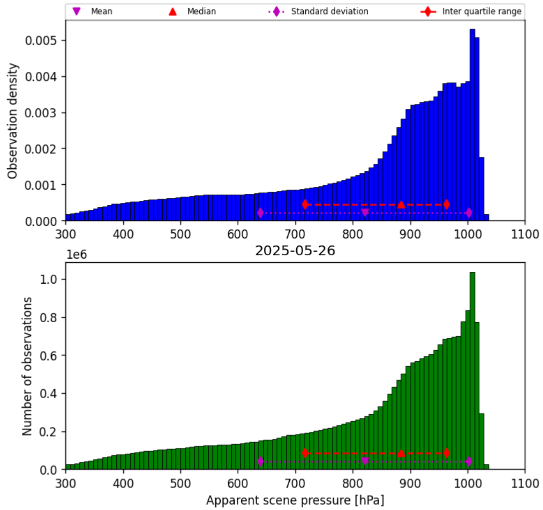
Figure 34: Histogram of “Apparent scene pressure” for 2025-05-26 to 2025-05-27
