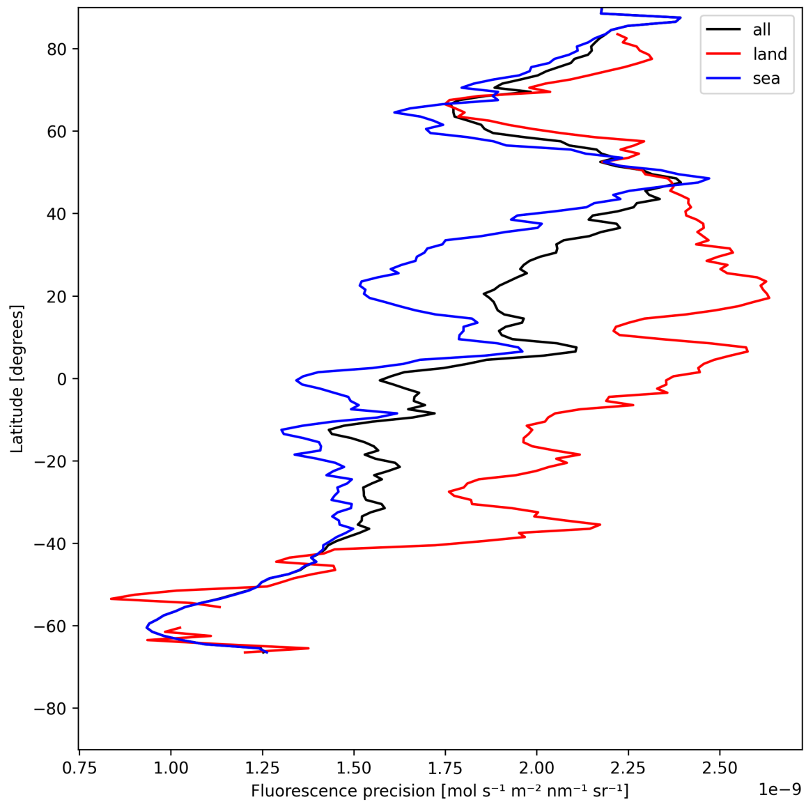
Figure 22: Zonal average of “Fluorescence precision” for 2025-05-26 to 2025-05-27.
