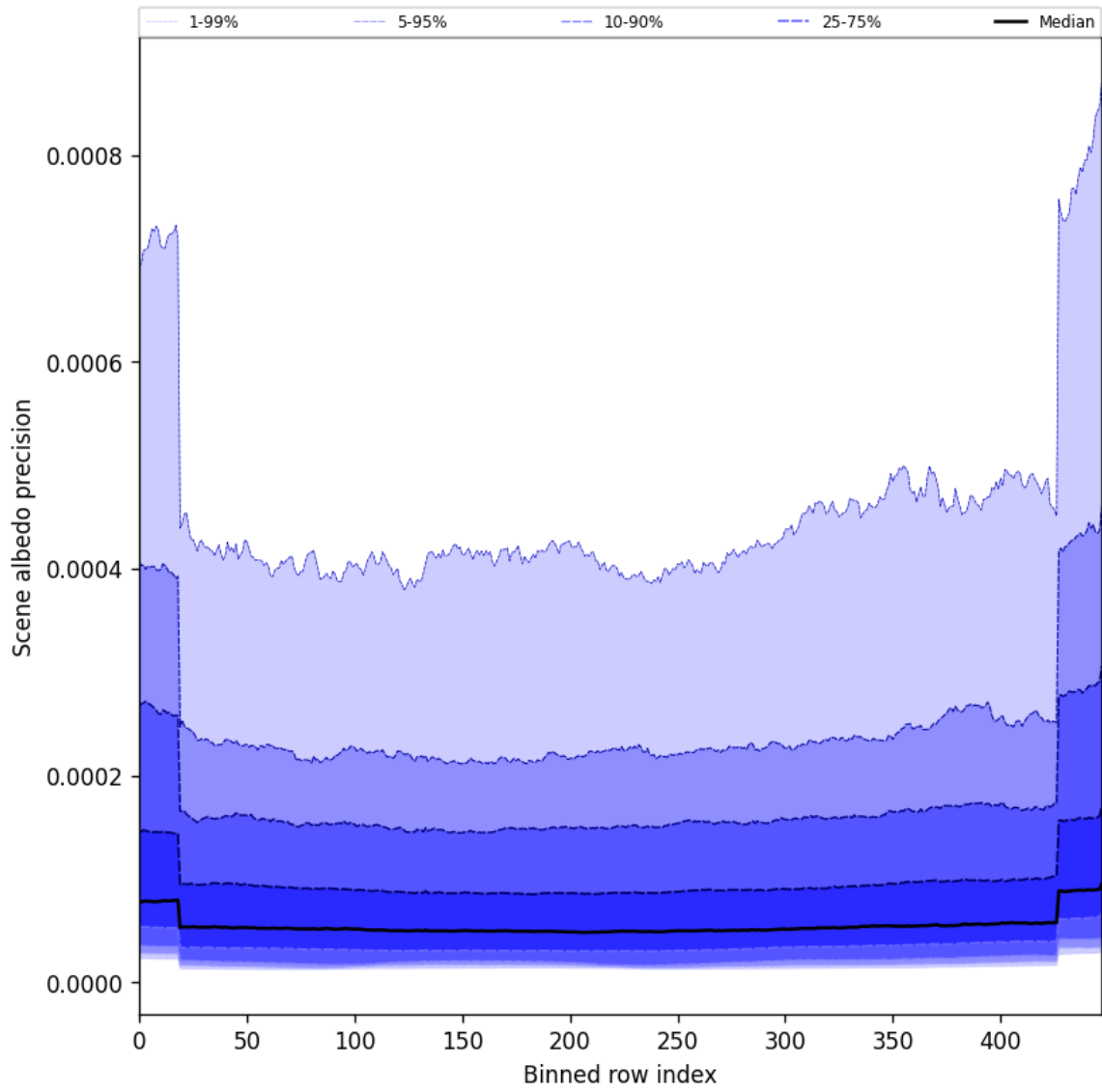
Figure 50: Along track statistics of “Scene albedo precision” for 2025-05-26 to 2025-05-27
