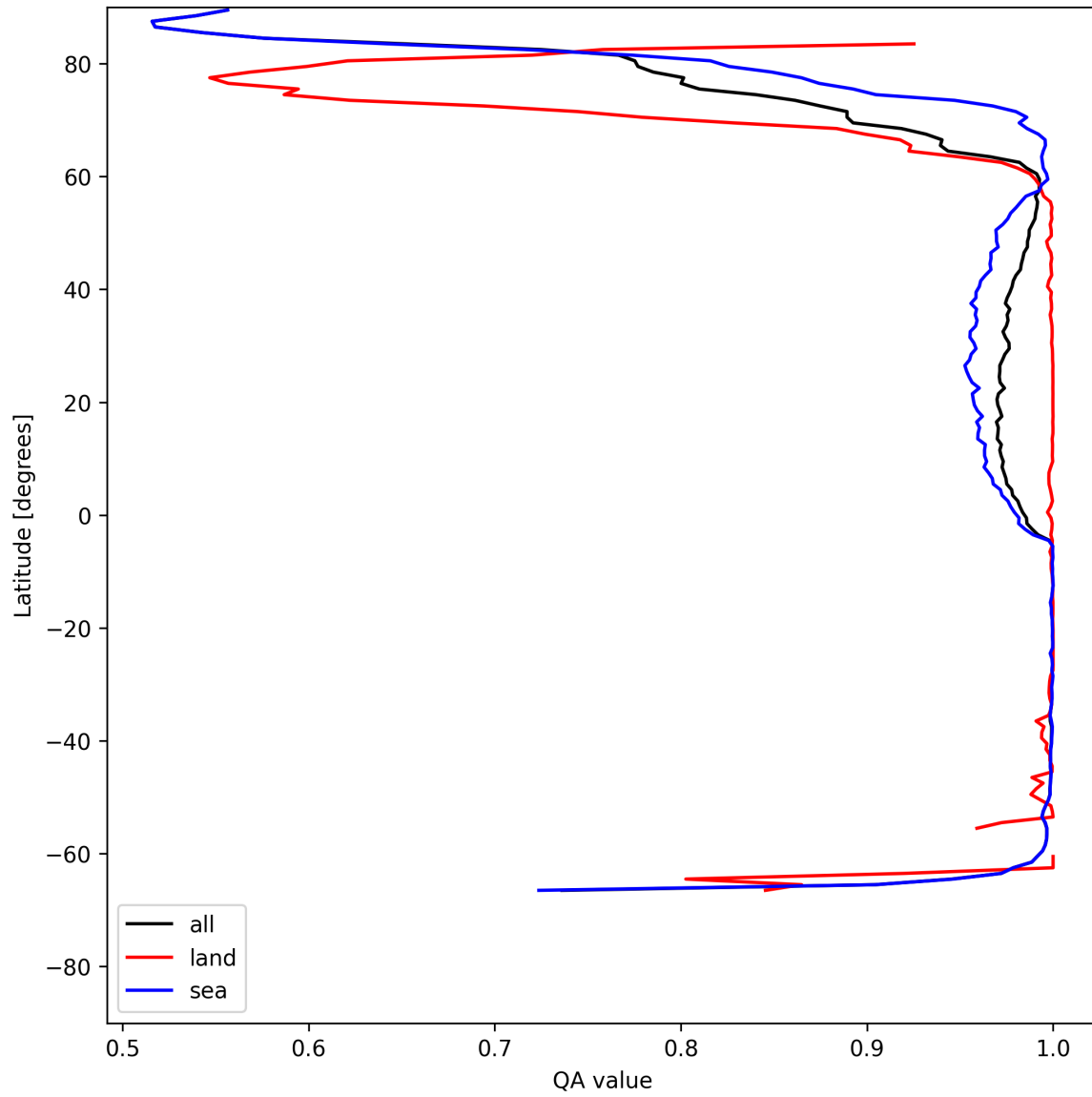
Figure 10: Zonal average of “QA value” for 2025-05-26 to 2025-05-27.
