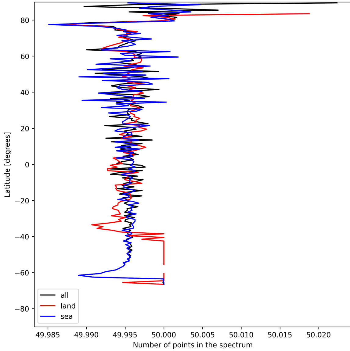
Figure 25: Zonal average of “Number of points in the spectrum” for 2025-05-26 to 2025-05-27.
