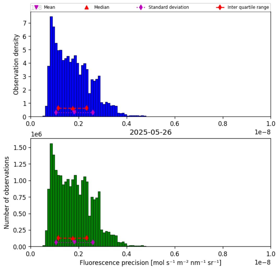
Figure 39: Histogram of “Fluorescence precision” for 2025-05-26 to 2025-05-27
