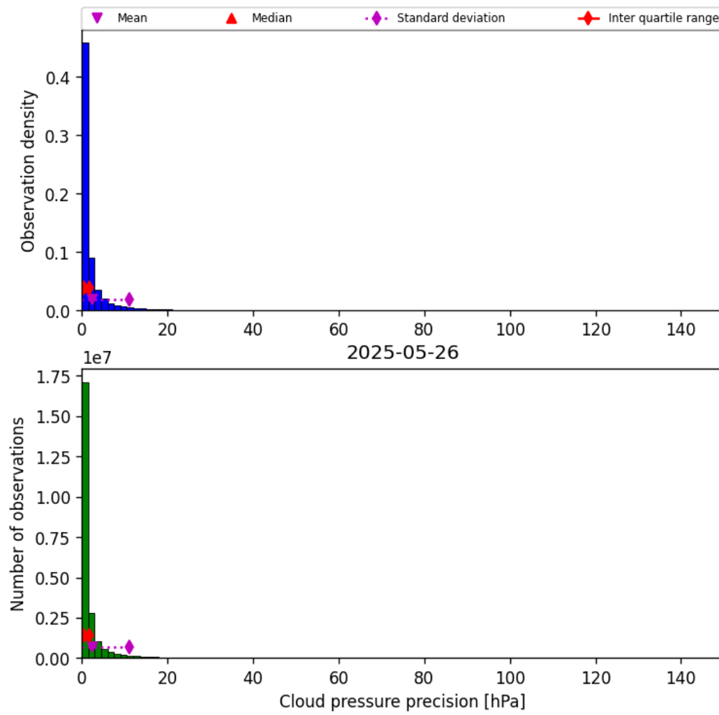
Figure 29: Histogram of “Cloud pressure precision” for 2025-05-26 to 2025-05-27
