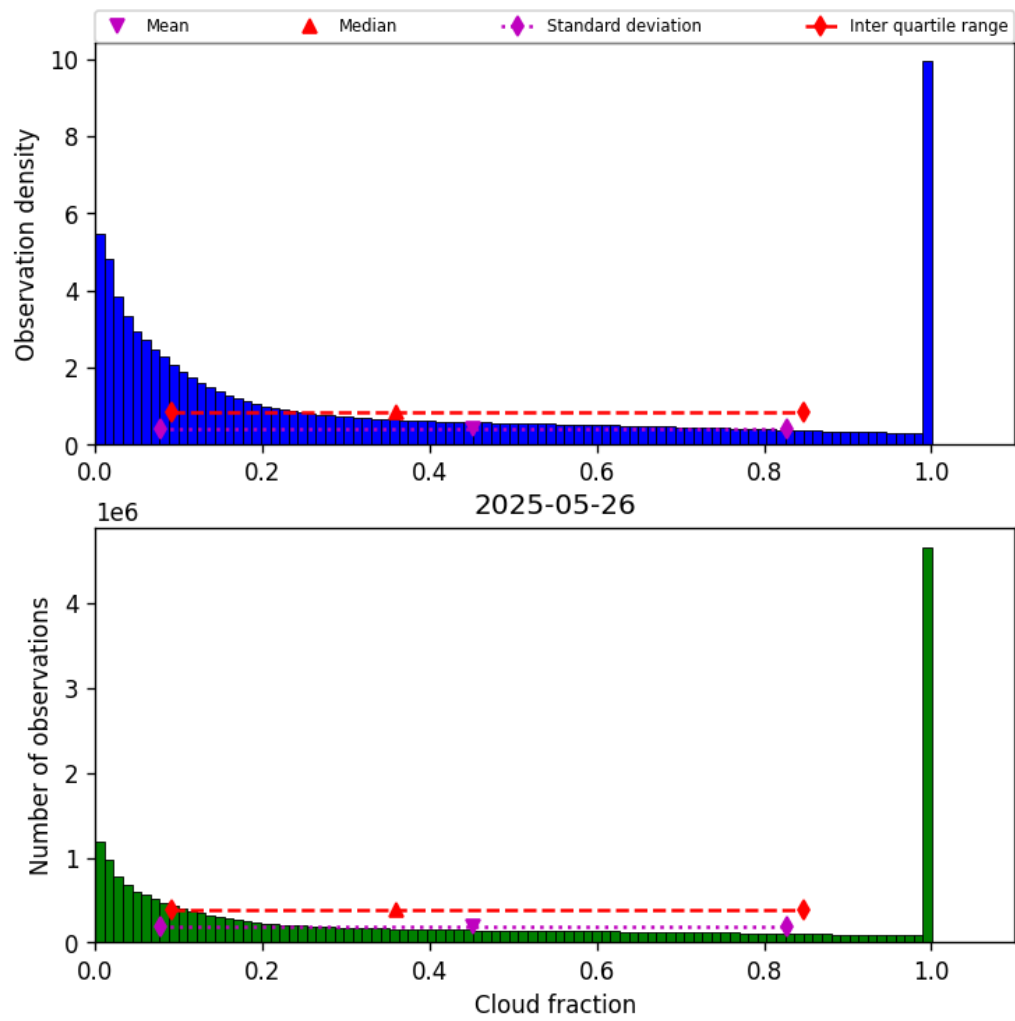
Figure 30: Histogram of “Cloud fraction” for 2025-05-26 to 2025-05-27
