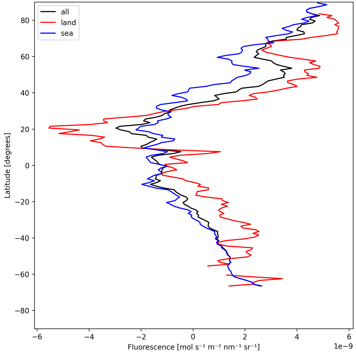
Figure 21: Zonal average of “Fluorescence” for 2025-05-26 to 2025-05-27.
