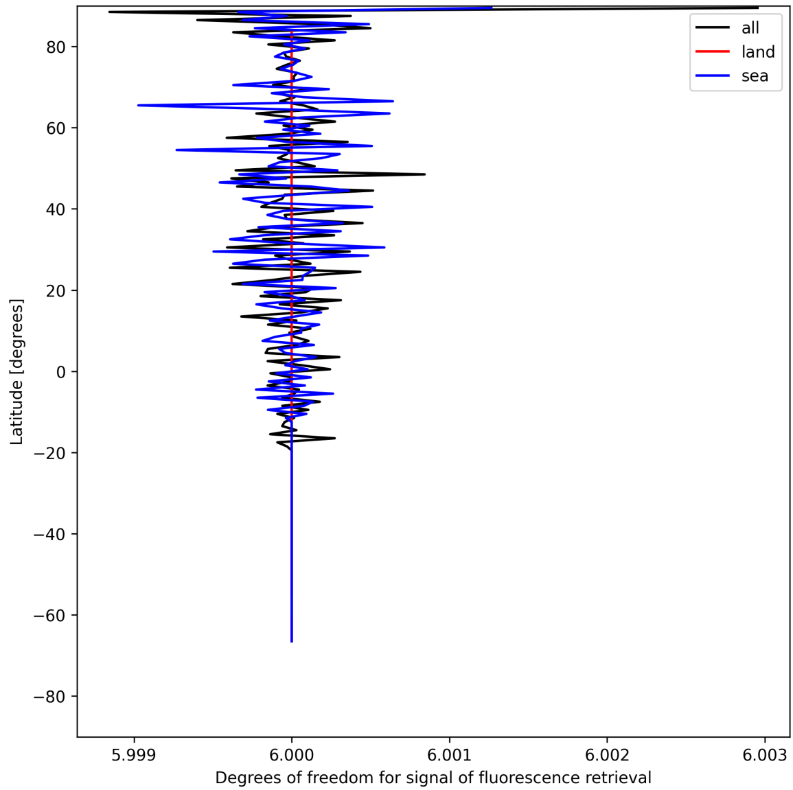
Figure 24: Zonal average of “Degrees of freedom for signal of fluorescence retrieval” for 2025-05-26 to 2025-05-27.
