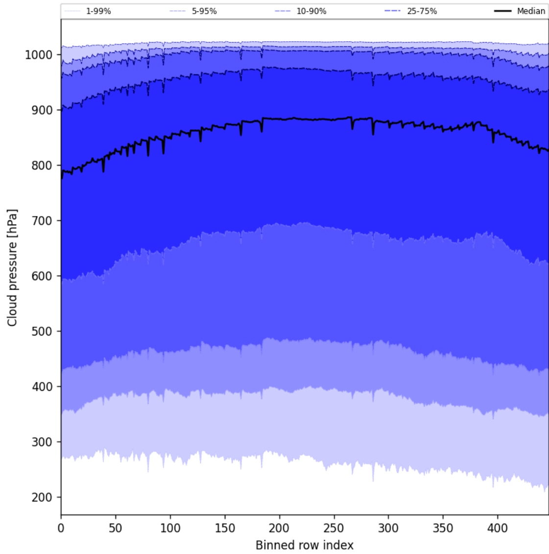
Figure 45: Along track statistics of “Cloud pressure” for 2025-05-26 to 2025-05-27
