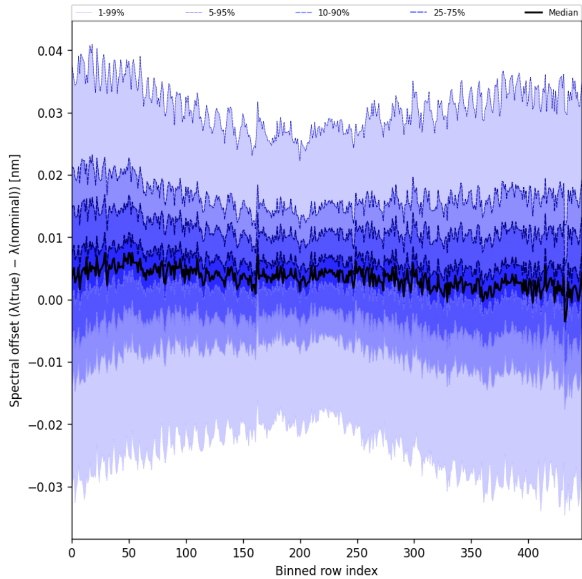
Figure 60: Along track statistics of “Spectral offset ( \lambda_{\text{true}} - \lambda_{\text{nominal}} )” for 2025-05-26 to 2025-05-27
