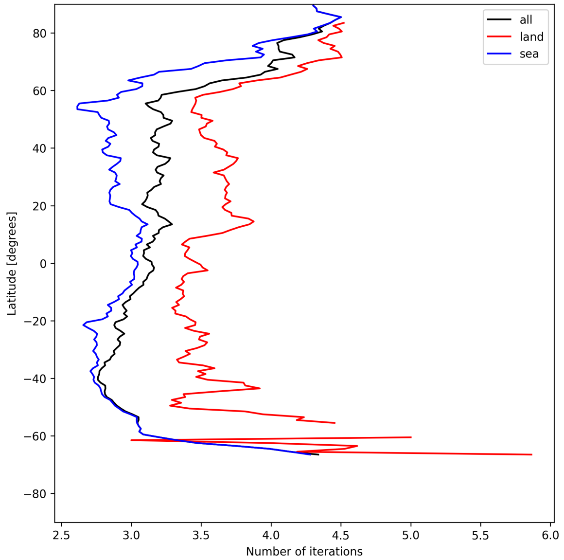
Figure 20: Zonal average of “Number of iterations” for 2025-05-26 to 2025-05-27.
