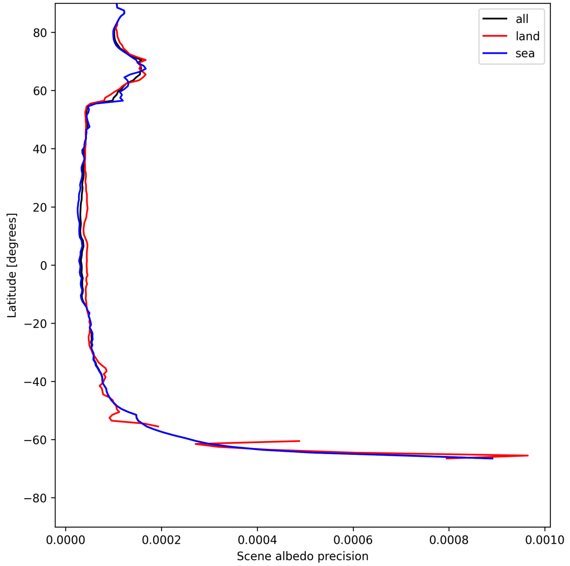
Figure 16: Zonal average of “Scene albedo precision” for 2025-05-26 to 2025-05-27.
