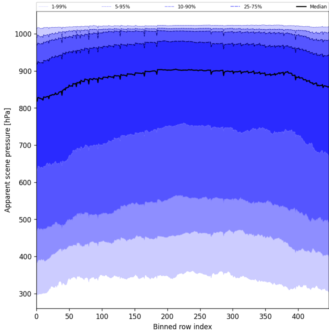
Figure 51: Along track statistics of “Apparent scene pressure” for 2025-05-26 to 2025-05-27
