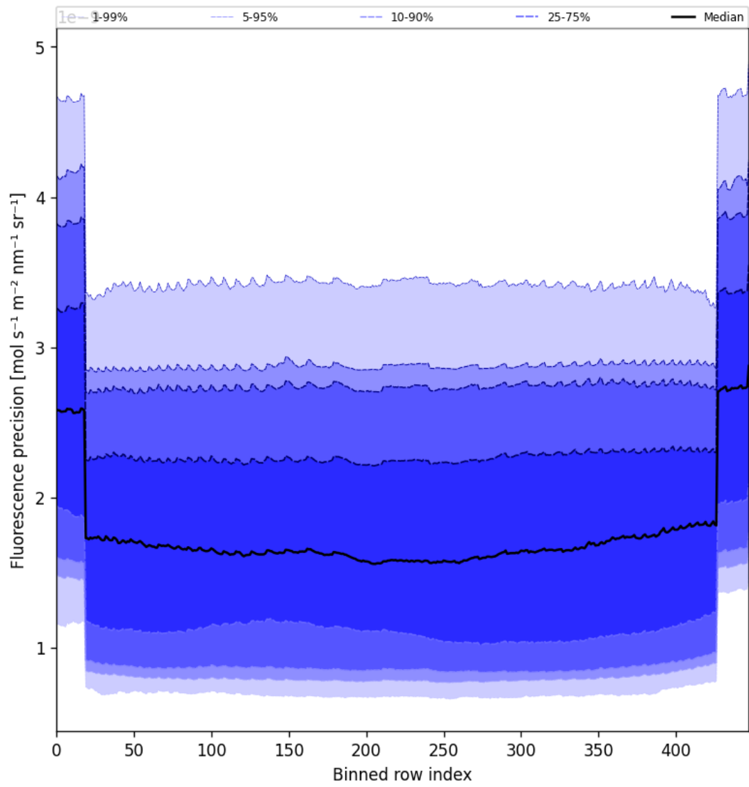
Figure 56: Along track statistics of “Fluorescence precision” for 2025-05-26 to 2025-05-27
