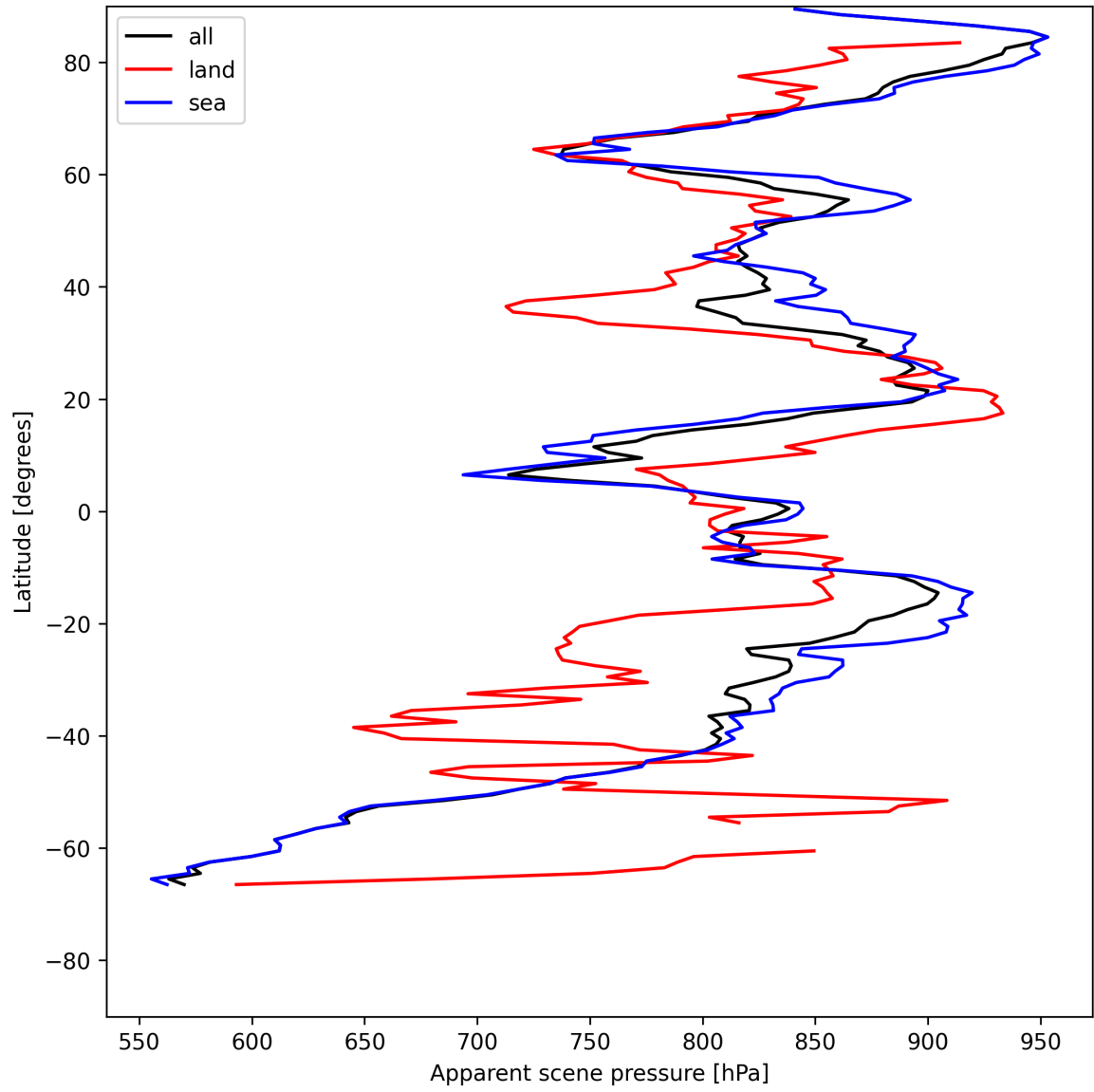
Figure 17: Zonal average of “Apparent scene pressure” for 2025-05-26 to 2025-05-27.
