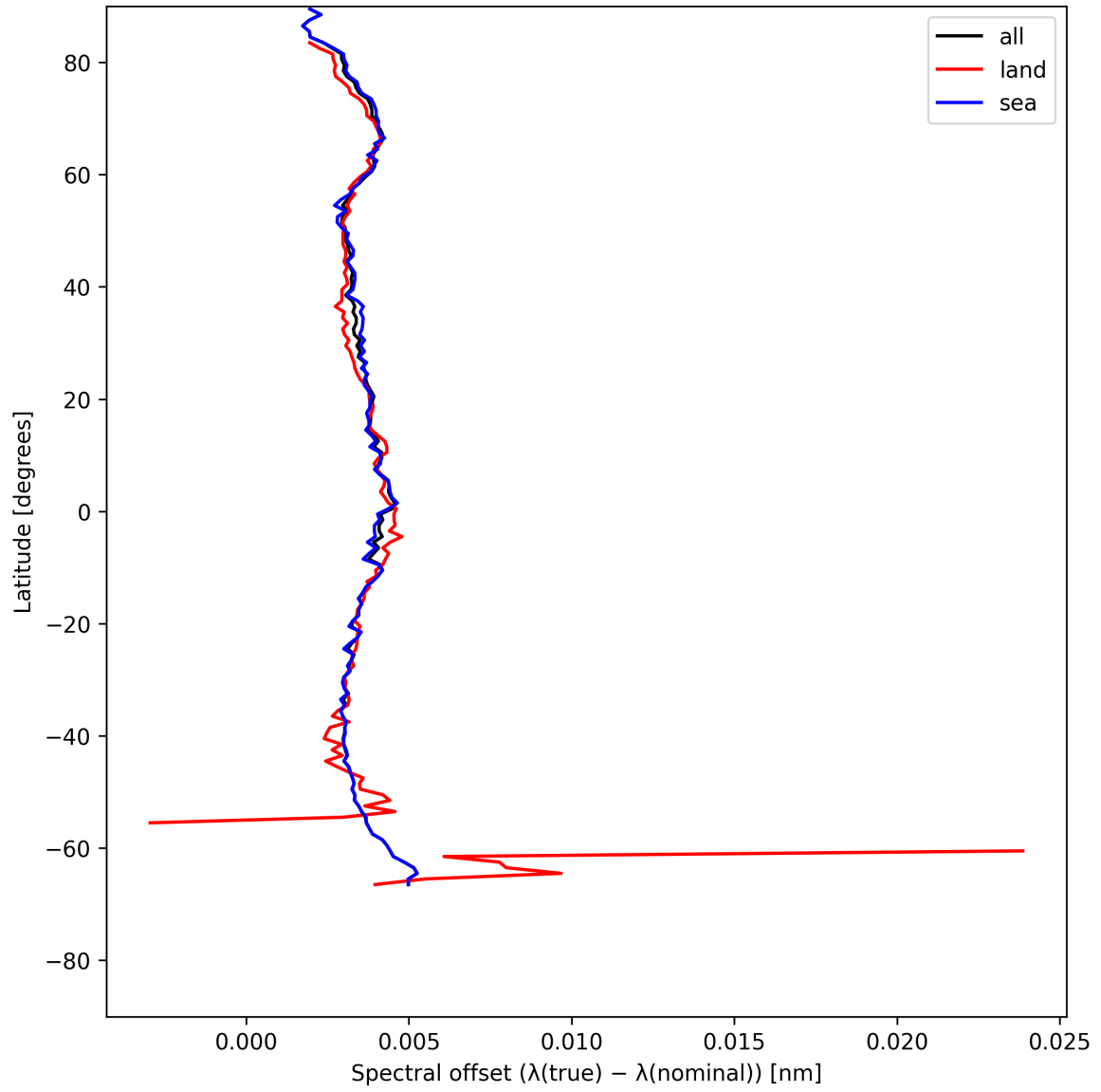
Figure 26: Zonal average of “Spectral offset ( \lambda_{\text{true}} - \lambda_{\text{nominal}} )” for 2025-05-26 to 2025-05-27.
