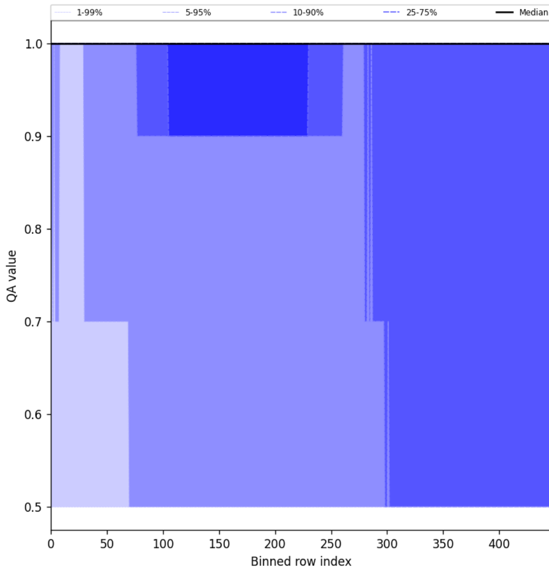
Figure 44: Along track statistics of “QA value” for 2025-05-26 to 2025-05-27
