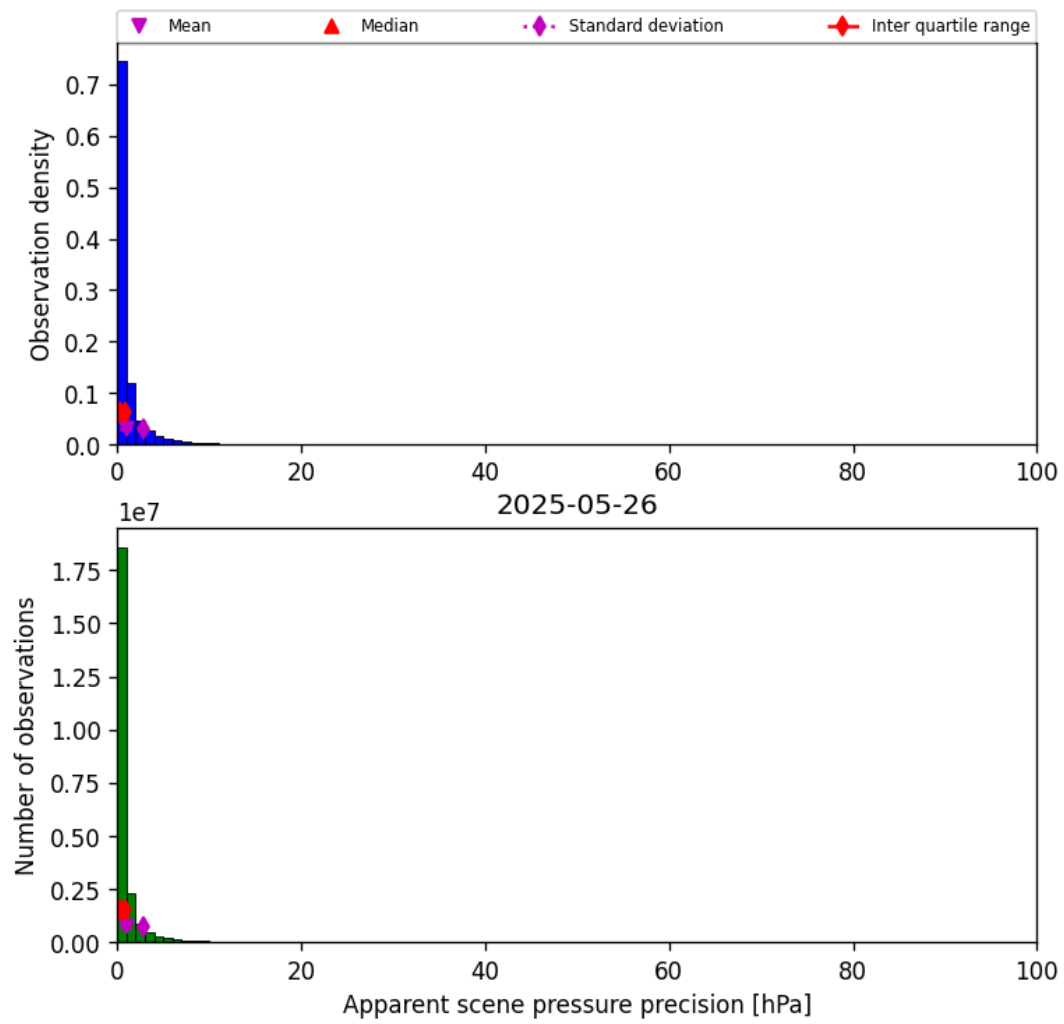
Figure 35: Histogram of “Apparent scene pressure precision” for 2025-05-26 to 2025-05-27
