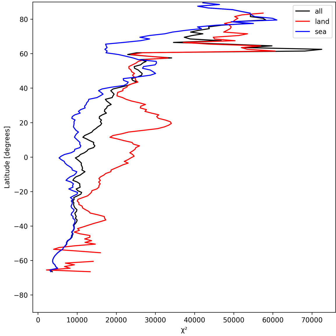
Figure 19: Zonal average of “ \chi^2 ” for 2025-05-26 to 2025-05-27.
