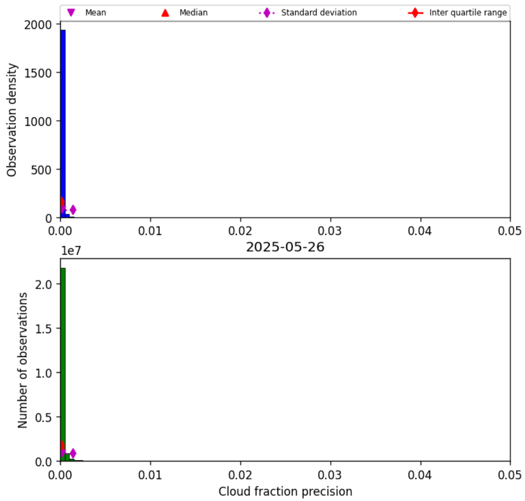
Figure 31: Histogram of “Cloud fraction precision” for 2025-05-26 to 2025-05-27
