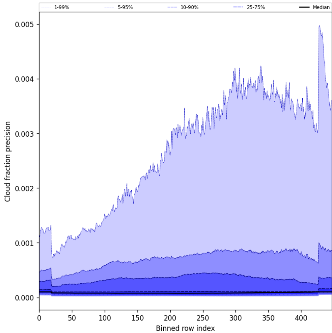
Figure 48: Along track statistics of “Cloud fraction precision” for 2025-05-26 to 2025-05-27
