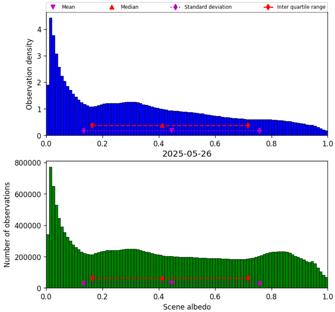
Figure 32: Histogram of “Scene albedo” for 2025-05-26 to 2025-05-27
