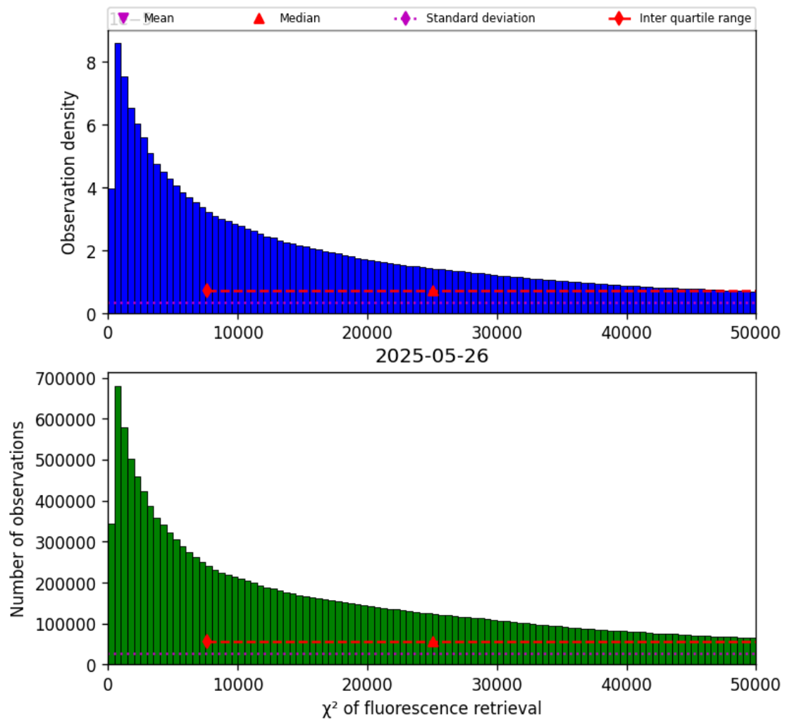
Figure 40: Histogram of “ \chi^2 of fluorescence retrieval” for 2025-05-26 to 2025-05-27
