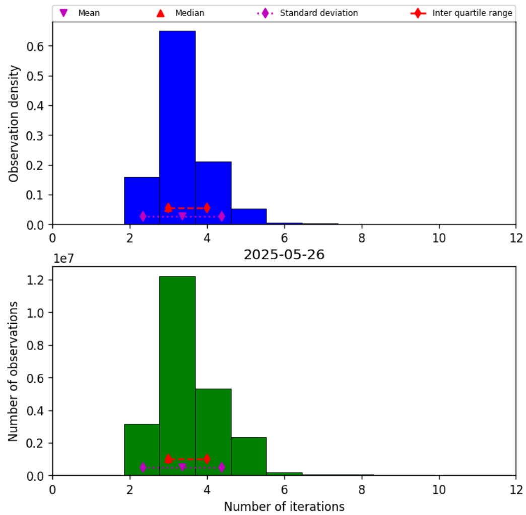
Figure 37: Histogram of “Number of iterations” for 2025-05-26 to 2025-05-27
