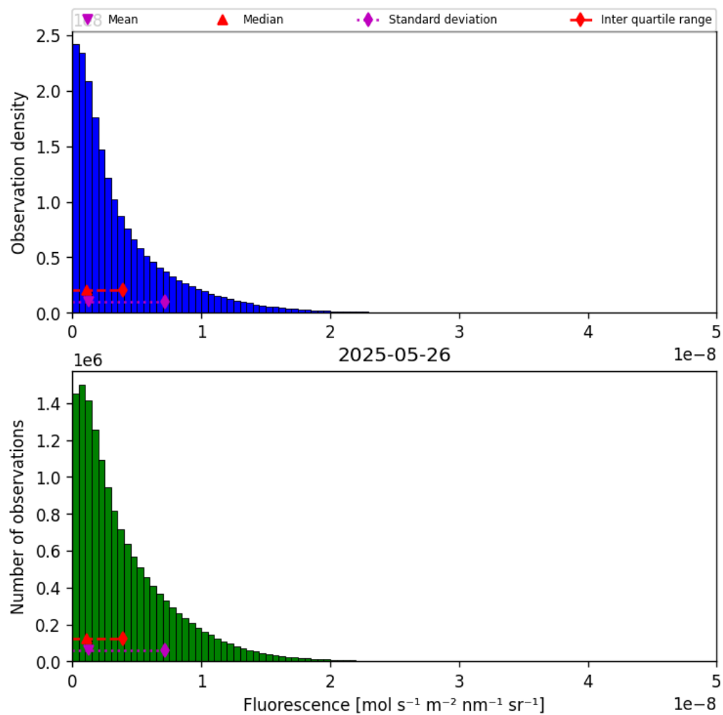
Figure 38: Histogram of “Fluorescence” for 2025-05-26 to 2025-05-27
