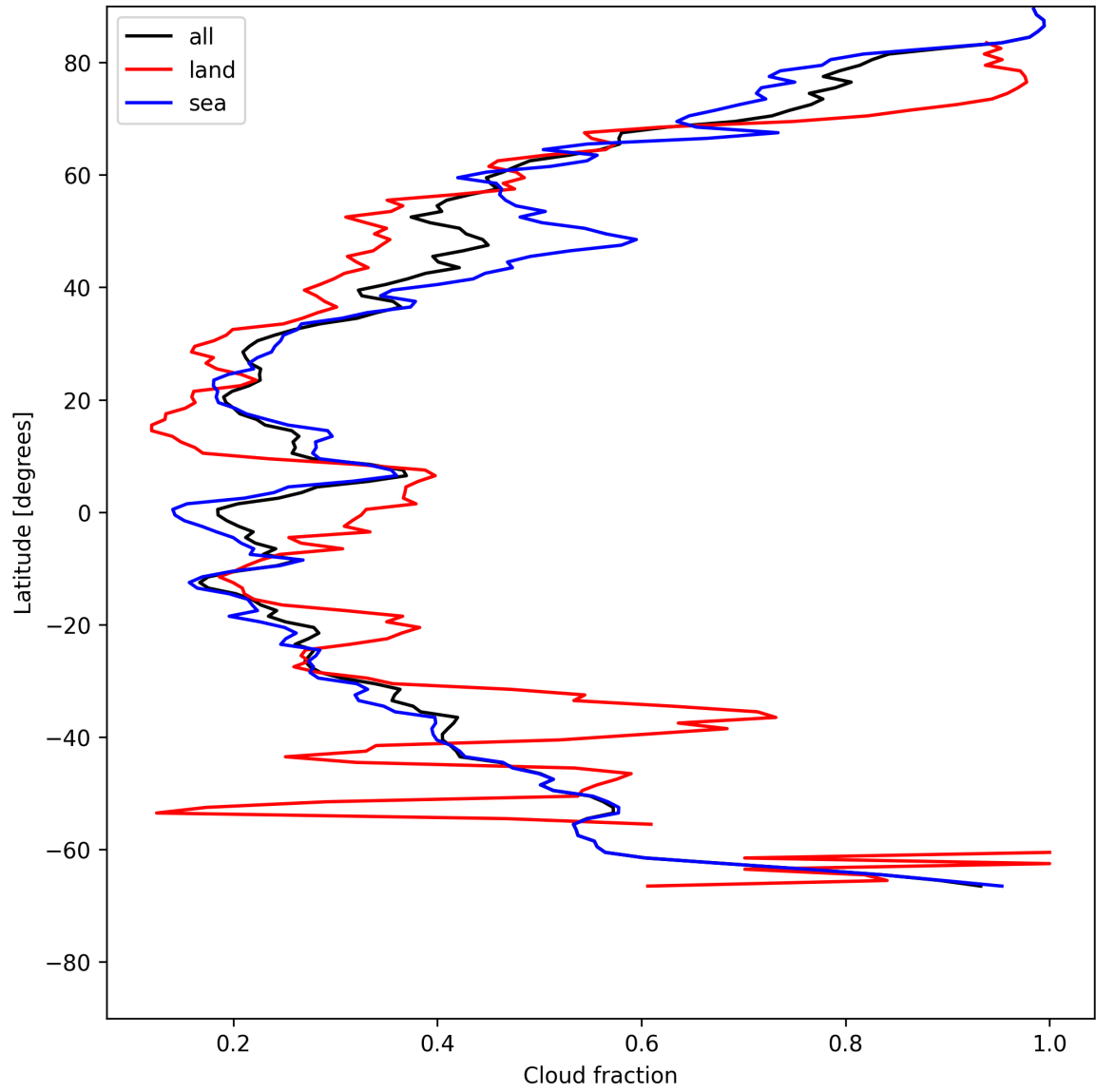
Figure 13: Zonal average of “Cloud fraction” for 2025-05-26 to 2025-05-27.
