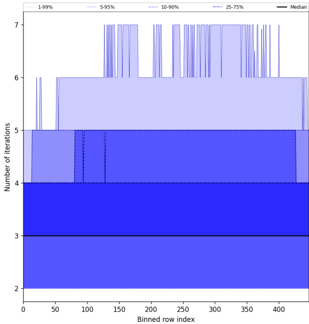
Figure 54: Along track statistics of “Number of iterations” for 2025-05-26 to 2025-05-27
