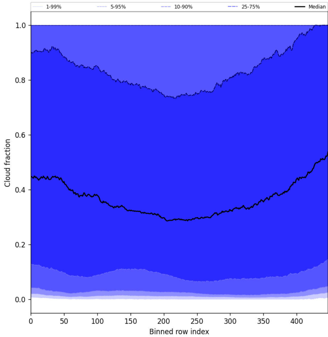
Figure 47: Along track statistics of “Cloud fraction” for 2025-05-26 to 2025-05-27
