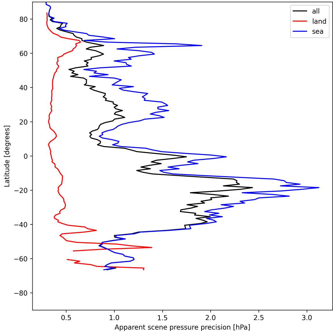
Figure 18: Zonal average of “Apparent scene pressure precision” for 2025-05-26 to 2025-05-27.
