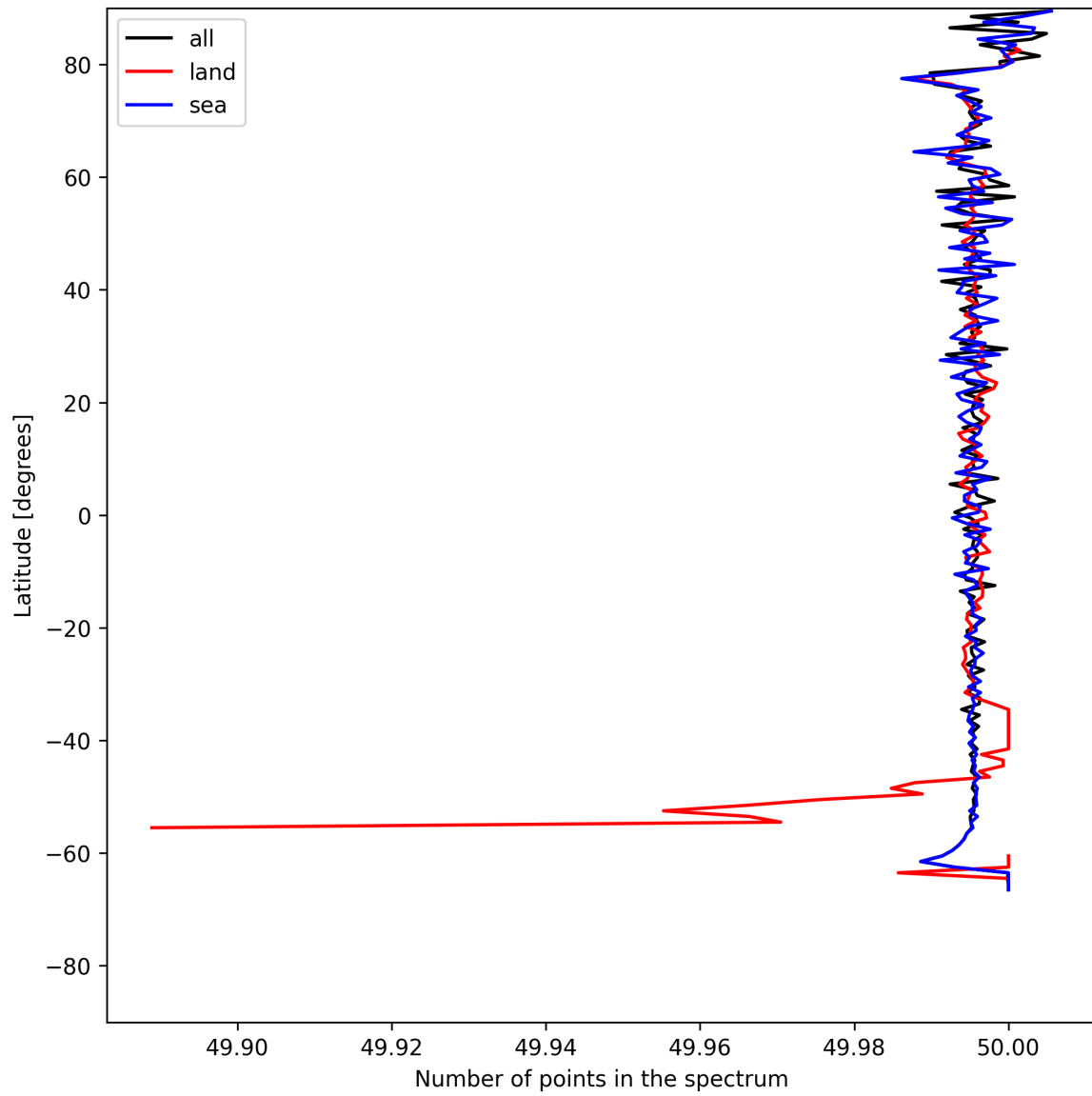
Figure 25: Zonal average of “Number of points in the spectrum” for 2025-05-27 to 2025-05-28.
