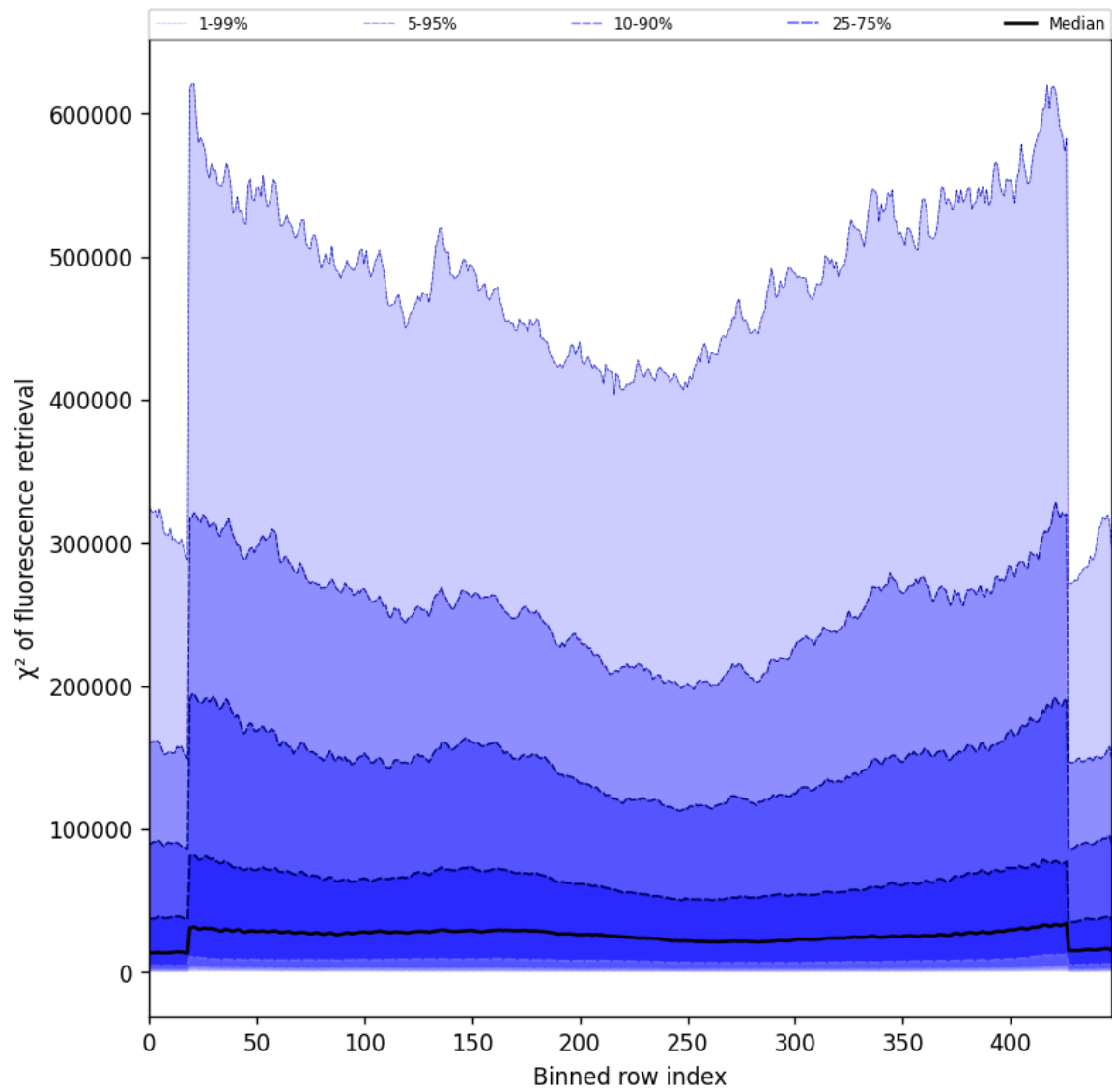
Figure 57: Along track statistics of “ \chi^2 of fluorescence retrieval” for 2025-05-27 to 2025-05-28
