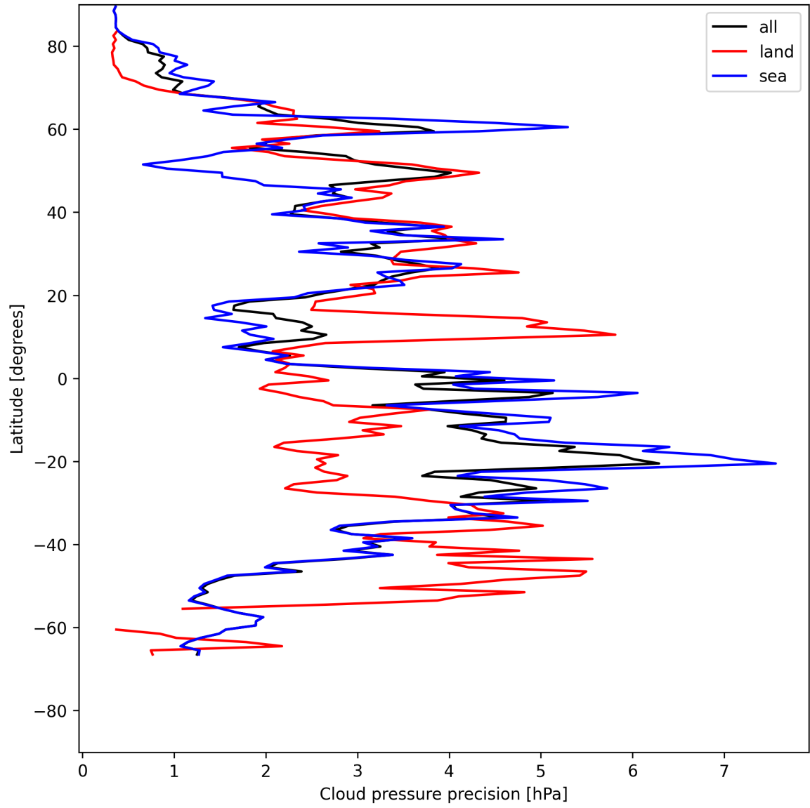
Figure 12: Zonal average of “Cloud pressure precision” for 2025-05-27 to 2025-05-28.
