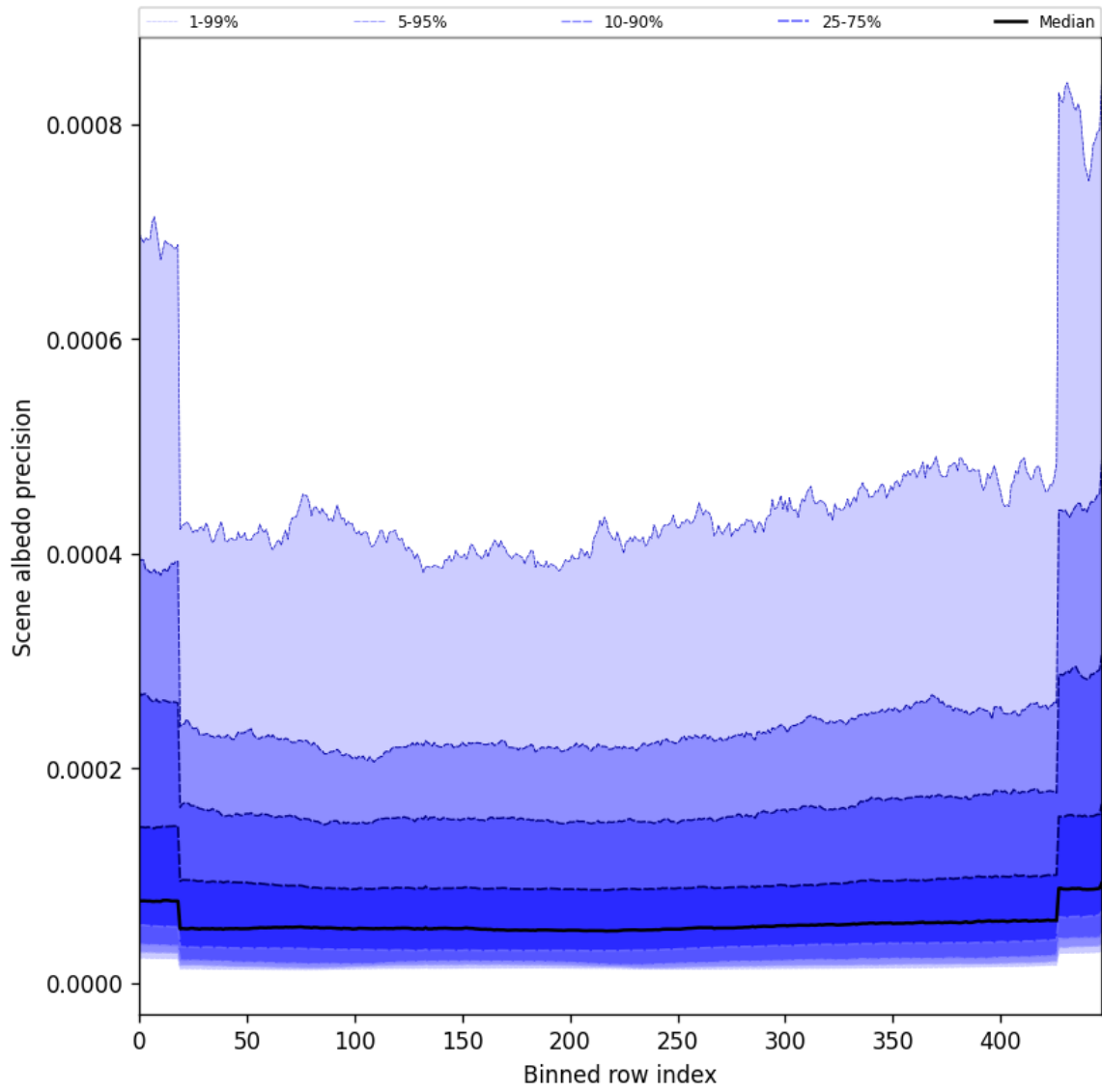
Figure 50: Along track statistics of “Scene albedo precision” for 2025-05-27 to 2025-05-28
