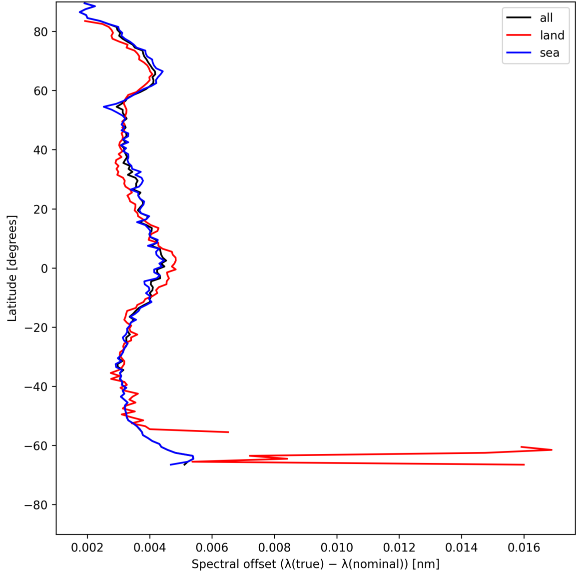
Figure 26: Zonal average of “Spectral offset ( \lambda_{\text{true}} - \lambda_{\text{nominal}} )” for 2025-05-27 to 2025-05-28.
