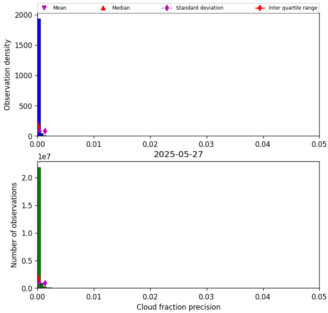
Figure 31: Histogram of “Cloud fraction precision” for 2025-05-27 to 2025-05-28
