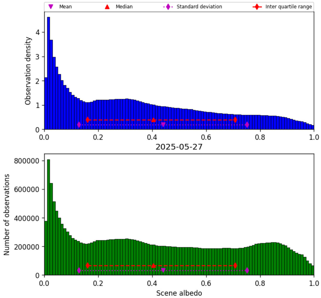
Figure 32: Histogram of “Scene albedo” for 2025-05-27 to 2025-05-28
