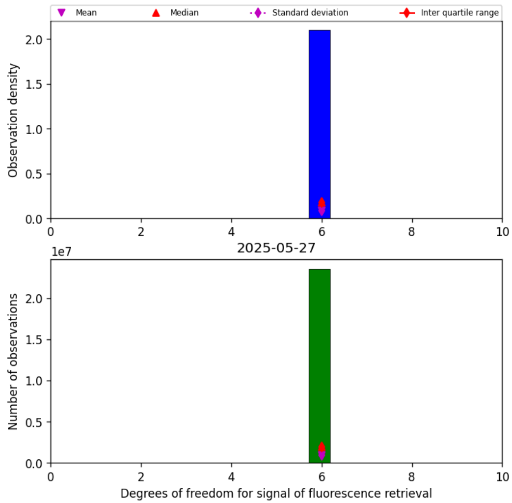
Figure 41: Histogram of “Degrees of freedom for signal of fluorescence retrieval” for 2025-05-27 to 2025-05-28
