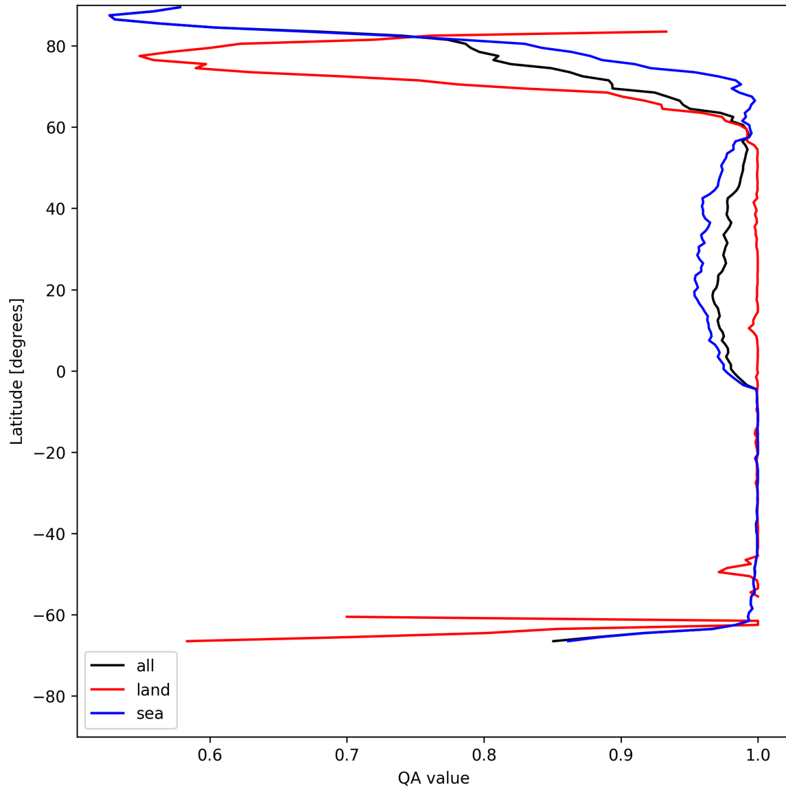
Figure 10: Zonal average of “QA value” for 2025-05-27 to 2025-05-28.
