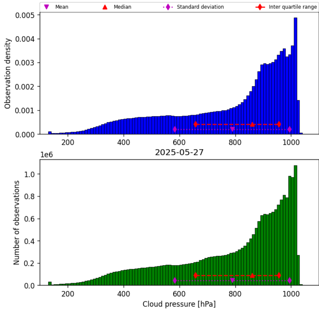
Figure 28: Histogram of “Cloud pressure” for 2025-05-27 to 2025-05-28
