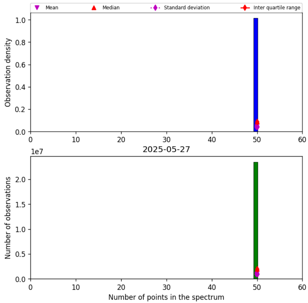
Figure 42: Histogram of “Number of points in the spectrum” for 2025-05-27 to 2025-05-28
