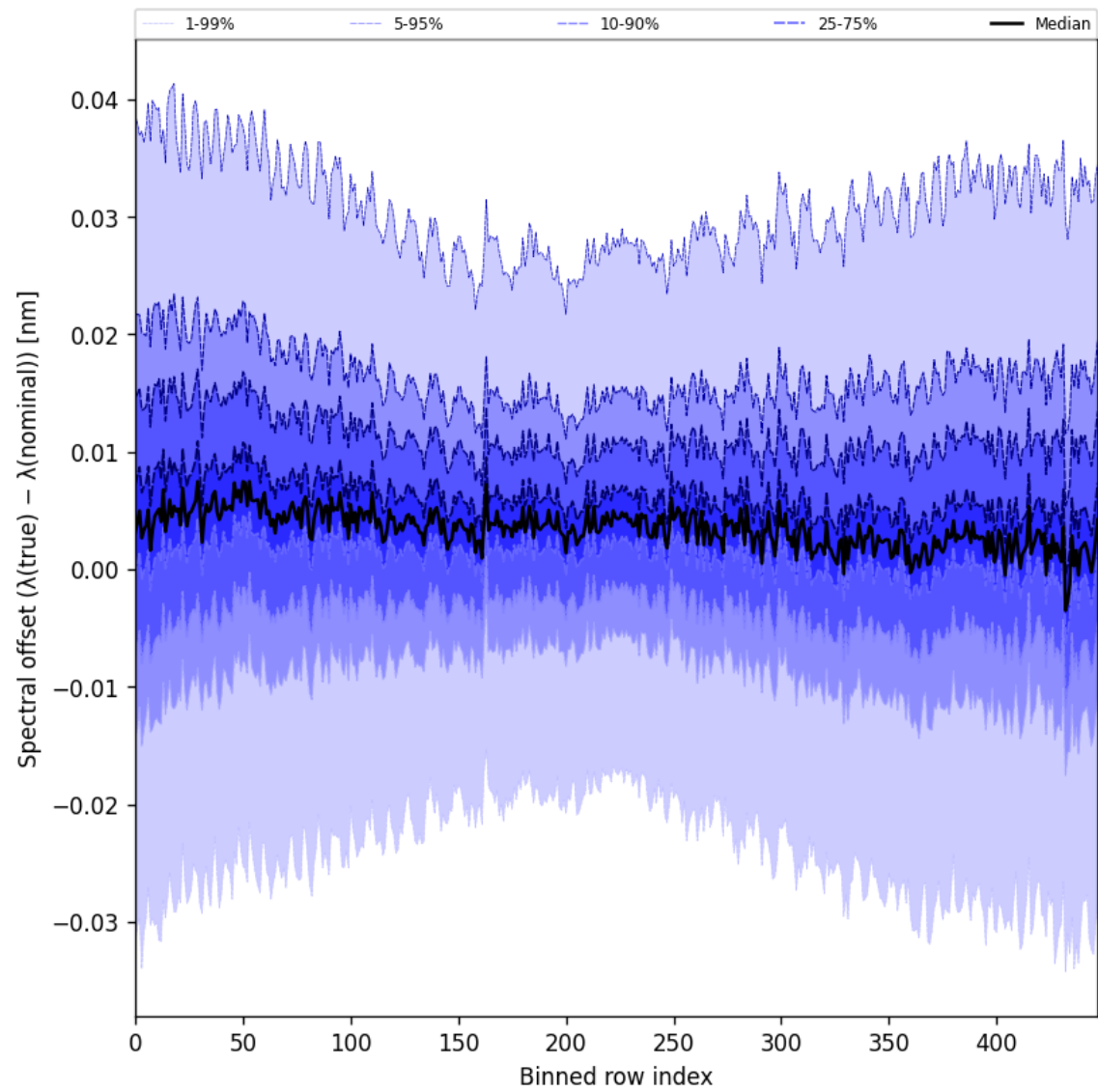
Figure 60: Along track statistics of “Spectral offset ( \lambda_{\text{true}} - \lambda_{\text{nominal}} )” for 2025-05-27 to 2025-05-28
