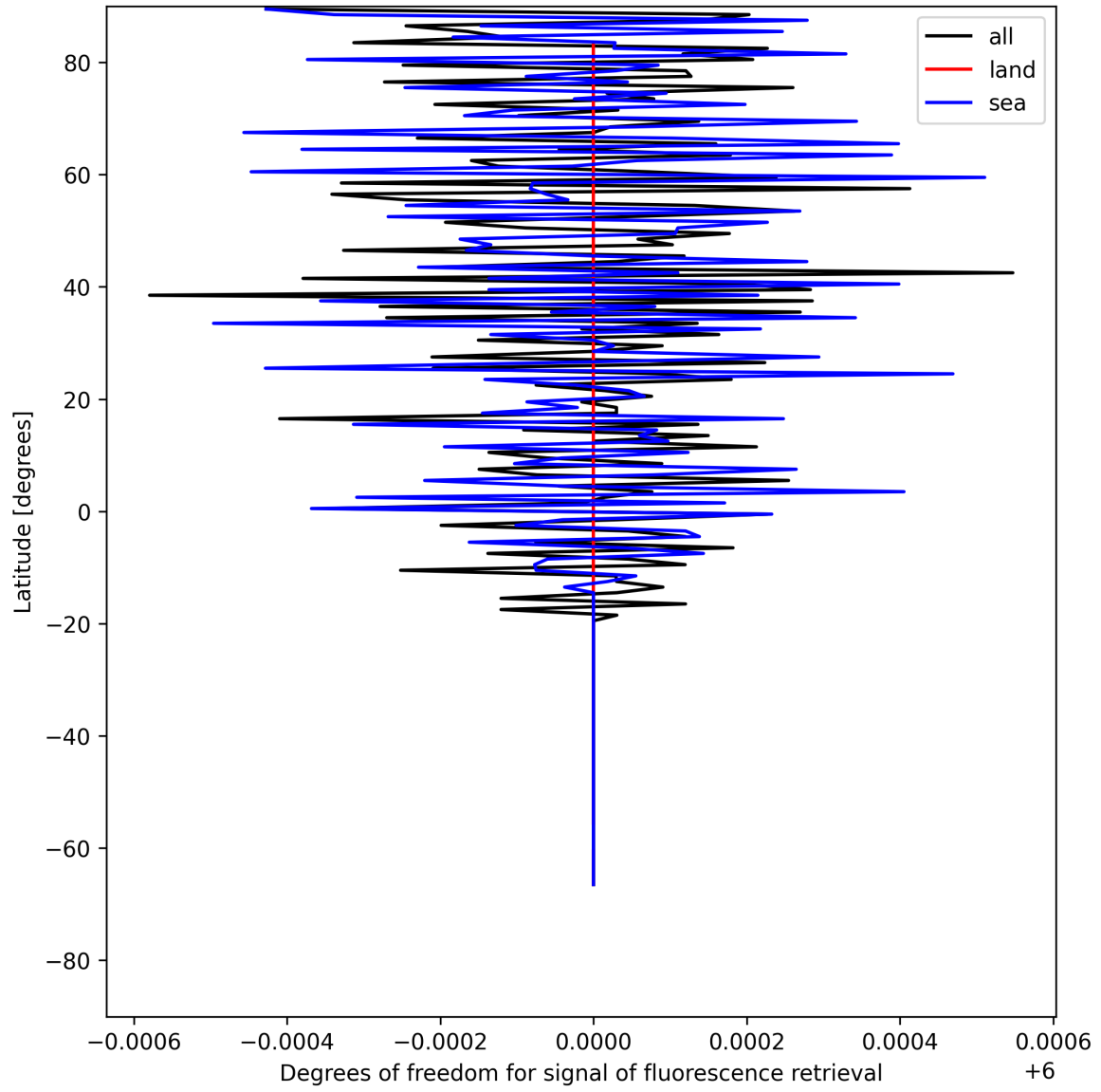
Figure 24: Zonal average of “Degrees of freedom for signal of fluorescence retrieval” for 2025-05-27 to 2025-05-28.
