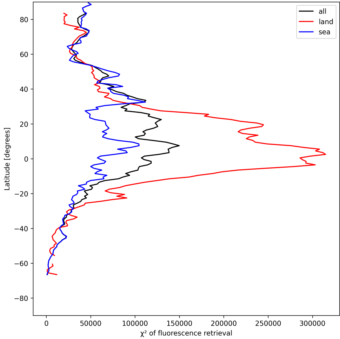
Figure 23: Zonal average of “ \chi^2 of fluorescence retrieval” for 2025-05-27 to 2025-05-28.
