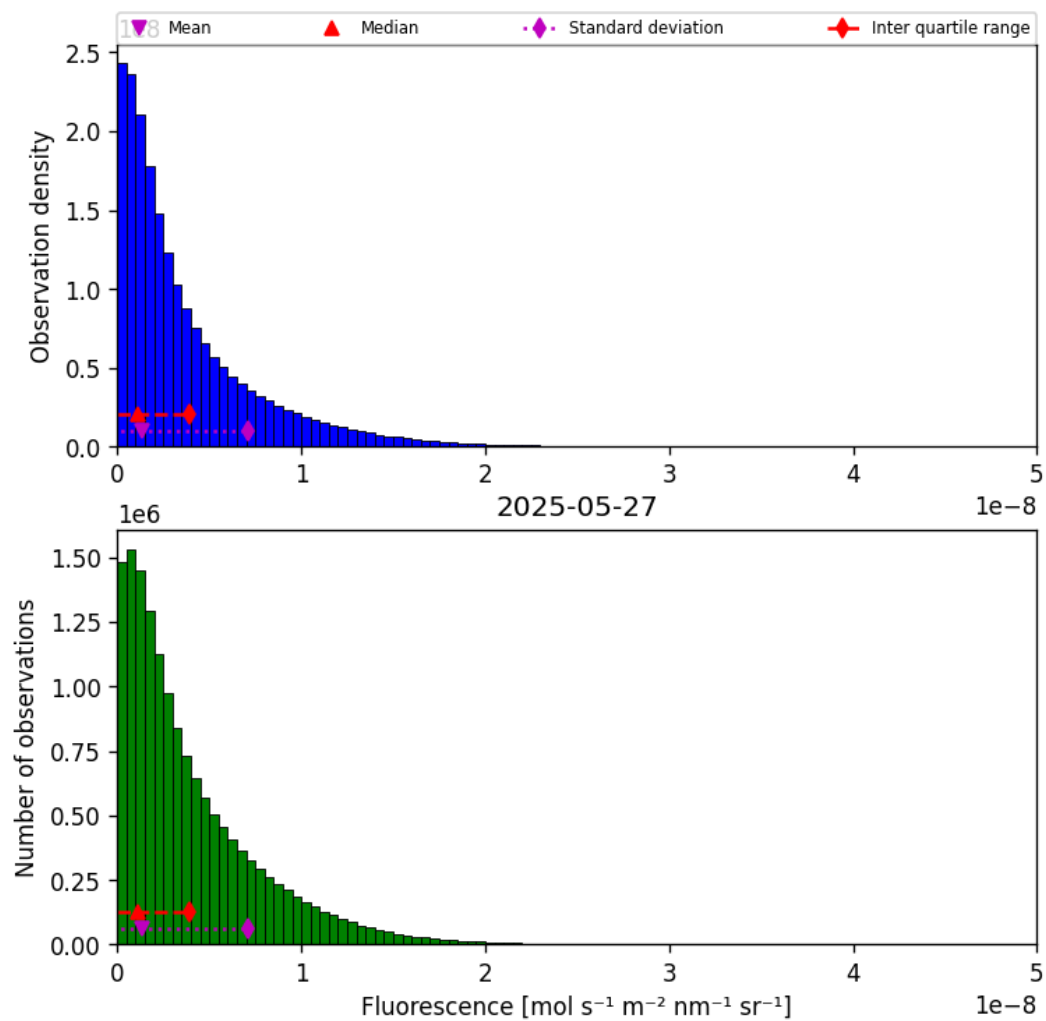
Figure 38: Histogram of “Fluorescence” for 2025-05-27 to 2025-05-28
