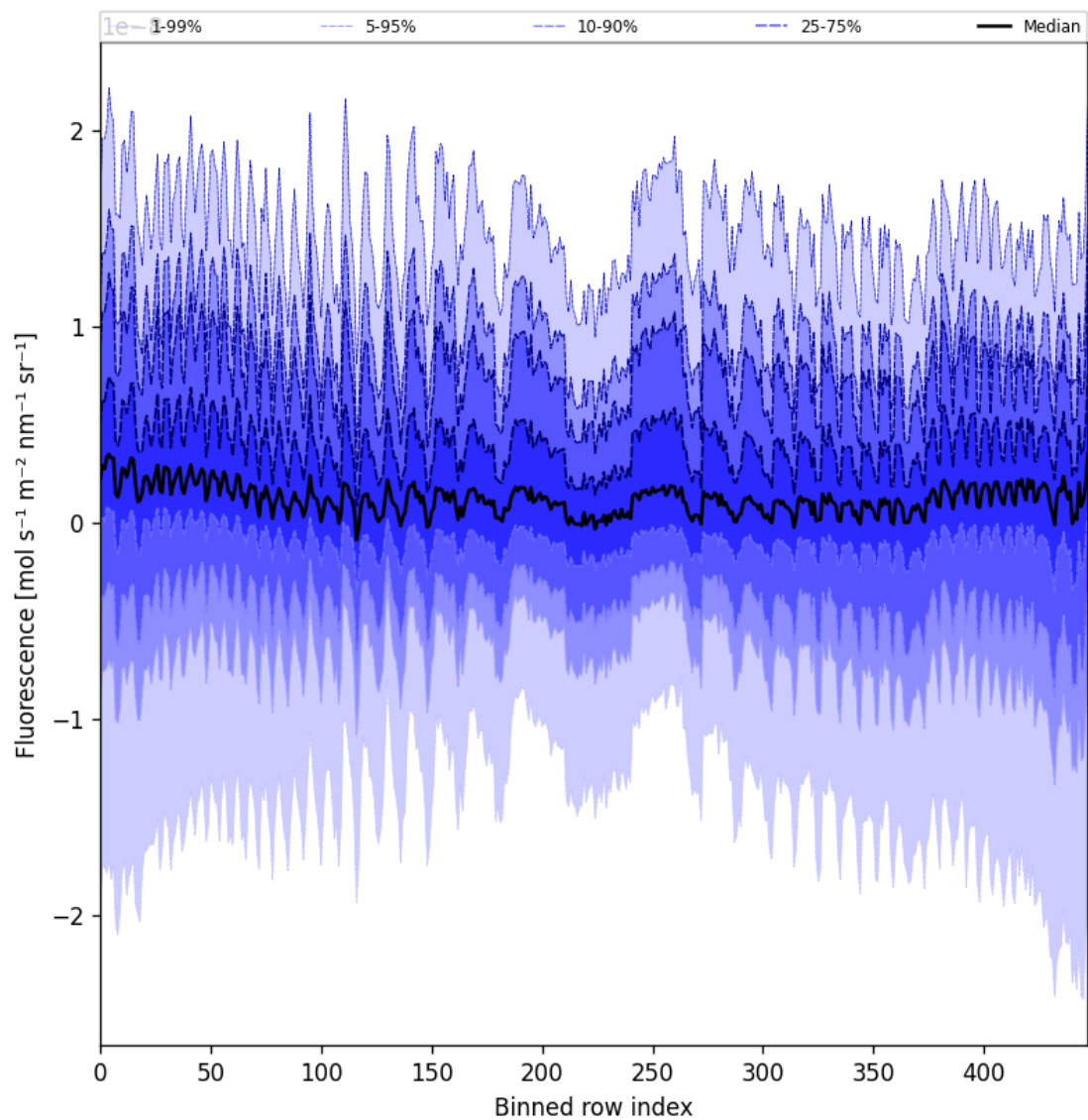
Figure 55: Along track statistics of “Fluorescence” for 2025-05-27 to 2025-05-28
