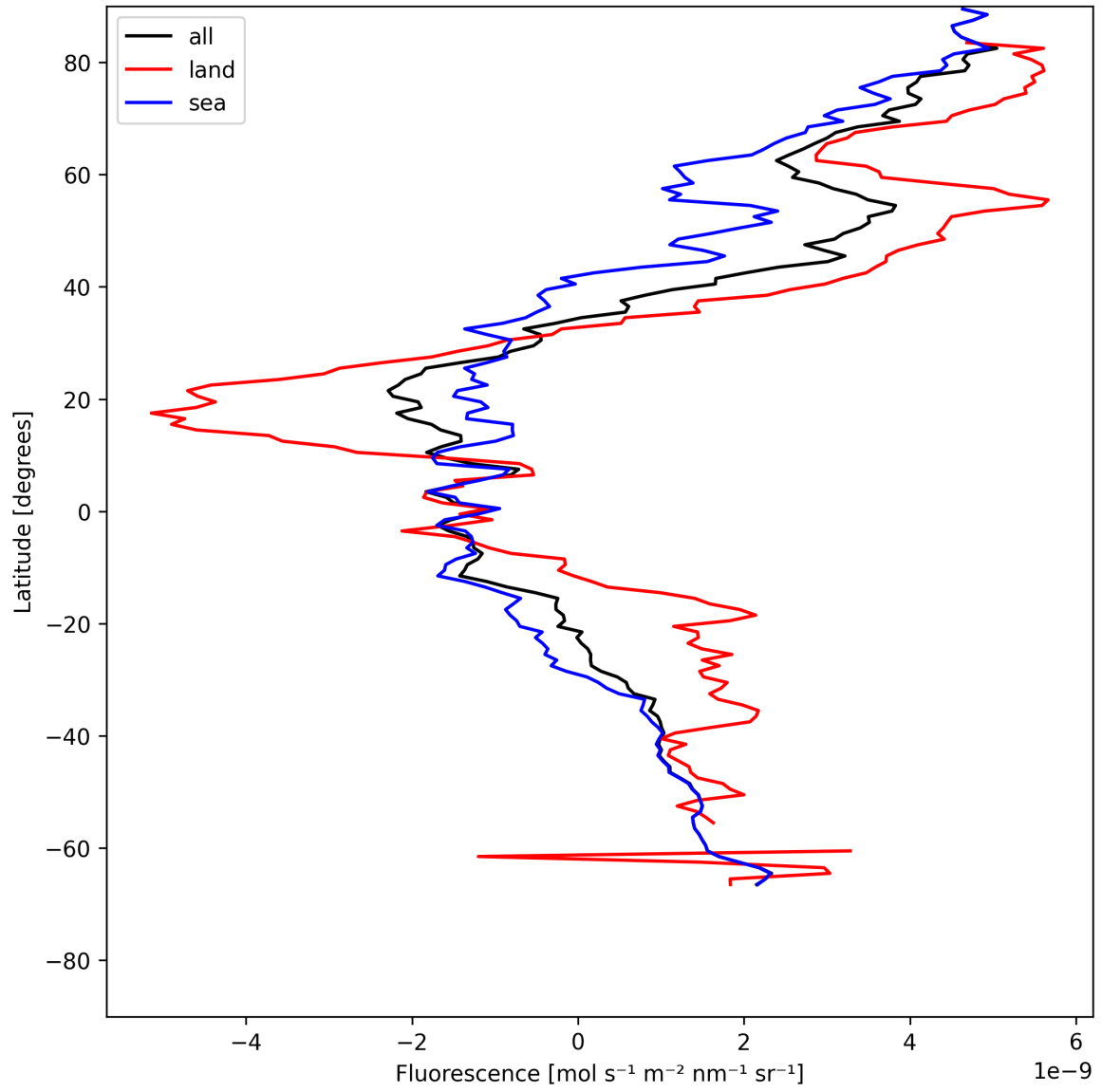
Figure 21: Zonal average of “Fluorescence” for 2025-05-27 to 2025-05-28.
