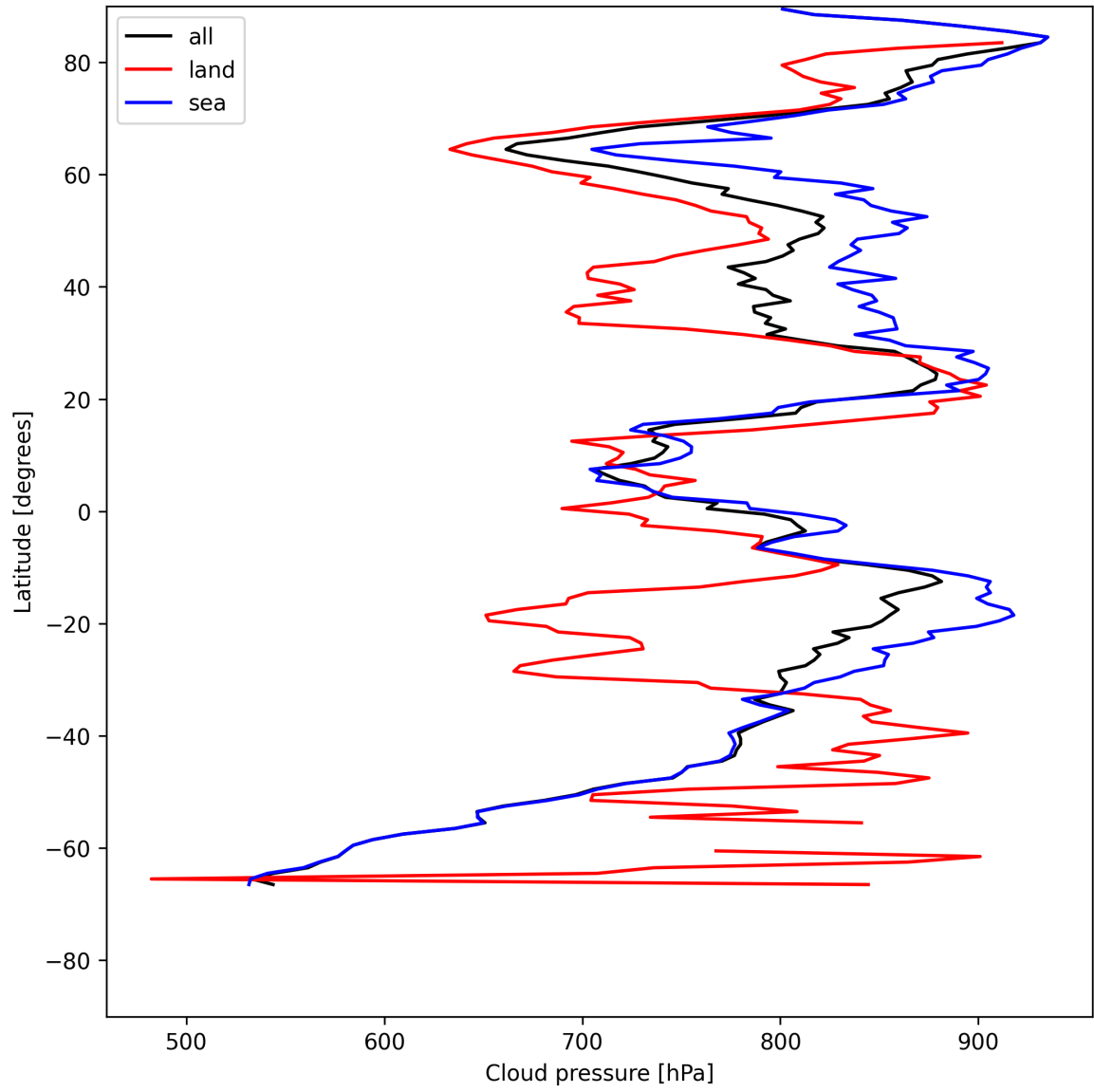
Figure 11: Zonal average of “Cloud pressure” for 2025-05-27 to 2025-05-28.
