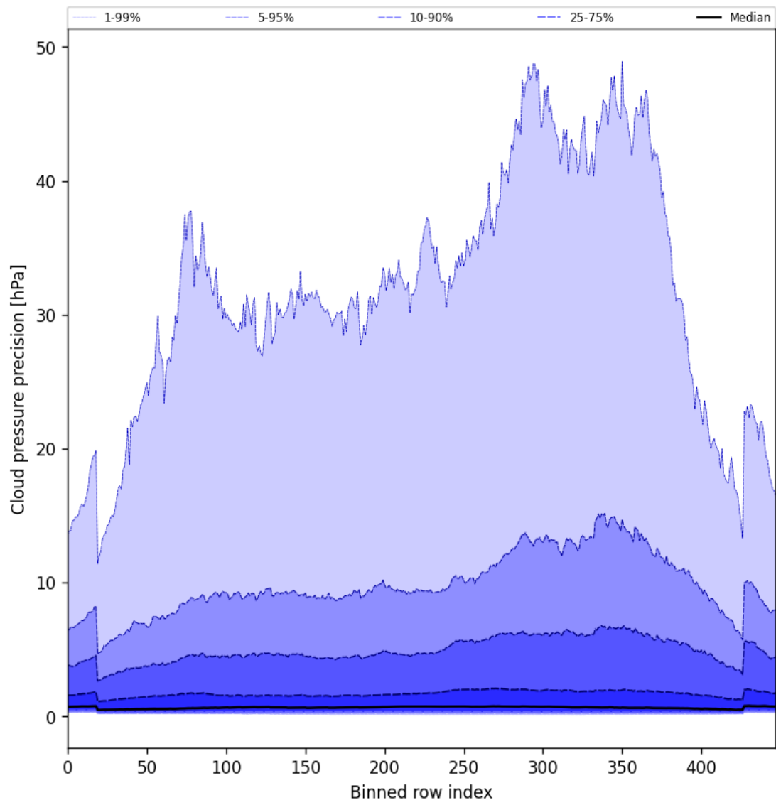
Figure 46: Along track statistics of “Cloud pressure precision” for 2025-05-27 to 2025-05-28
