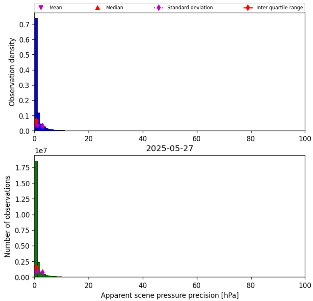
Figure 35: Histogram of “Apparent scene pressure precision” for 2025-05-27 to 2025-05-28
