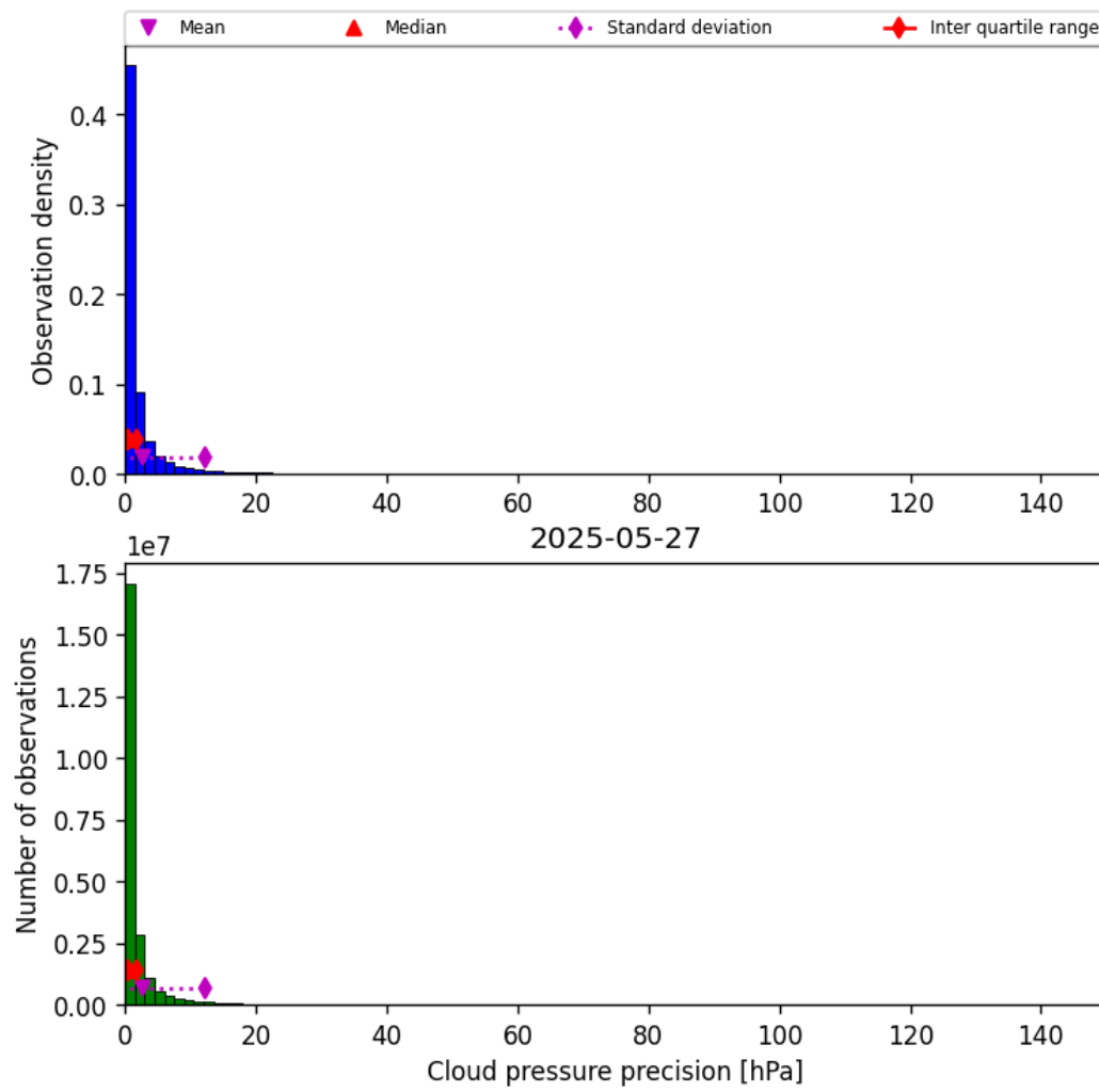
Figure 29: Histogram of “Cloud pressure precision” for 2025-05-27 to 2025-05-28
