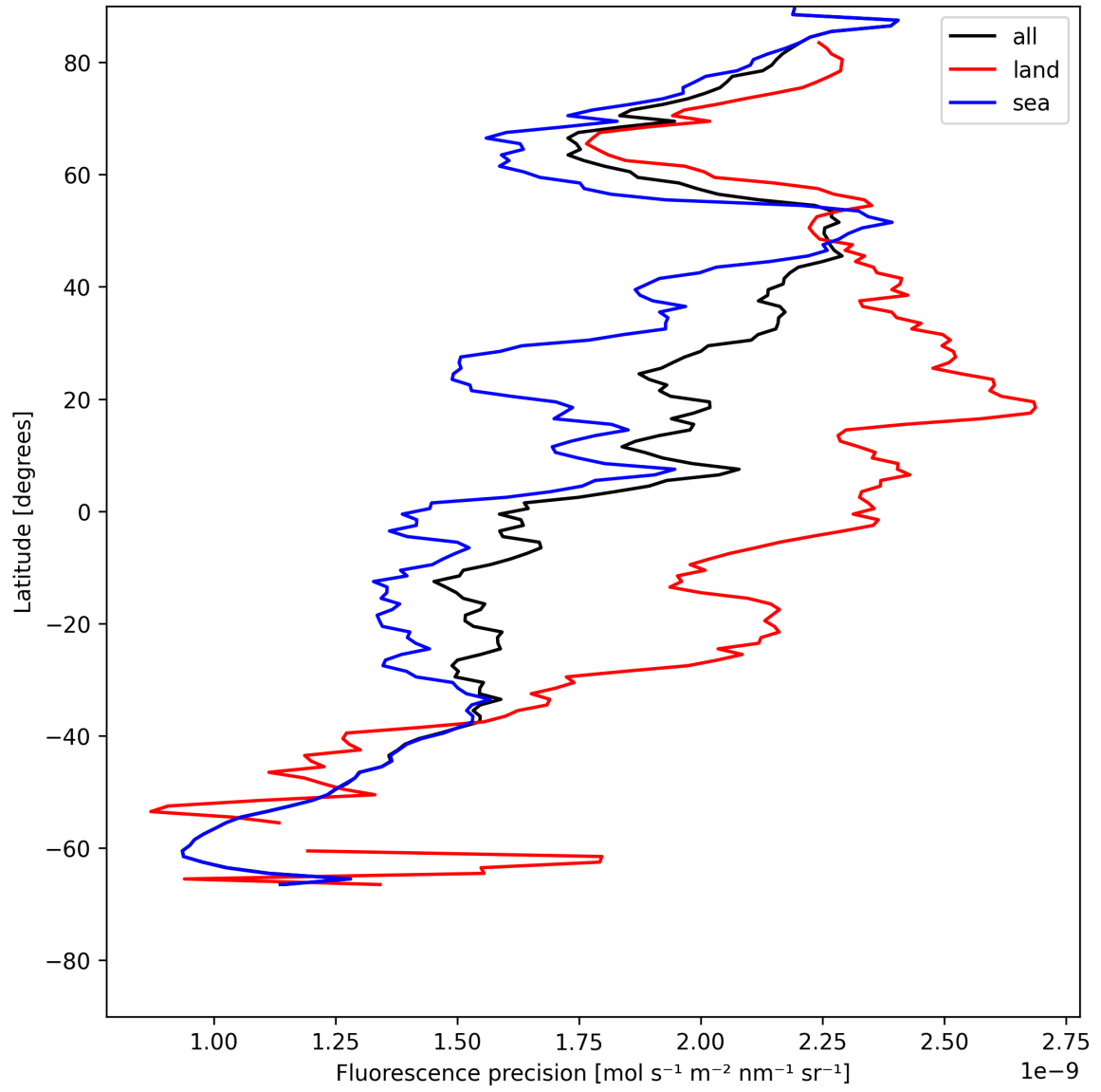
Figure 22: Zonal average of “Fluorescence precision” for 2025-05-27 to 2025-05-28.
