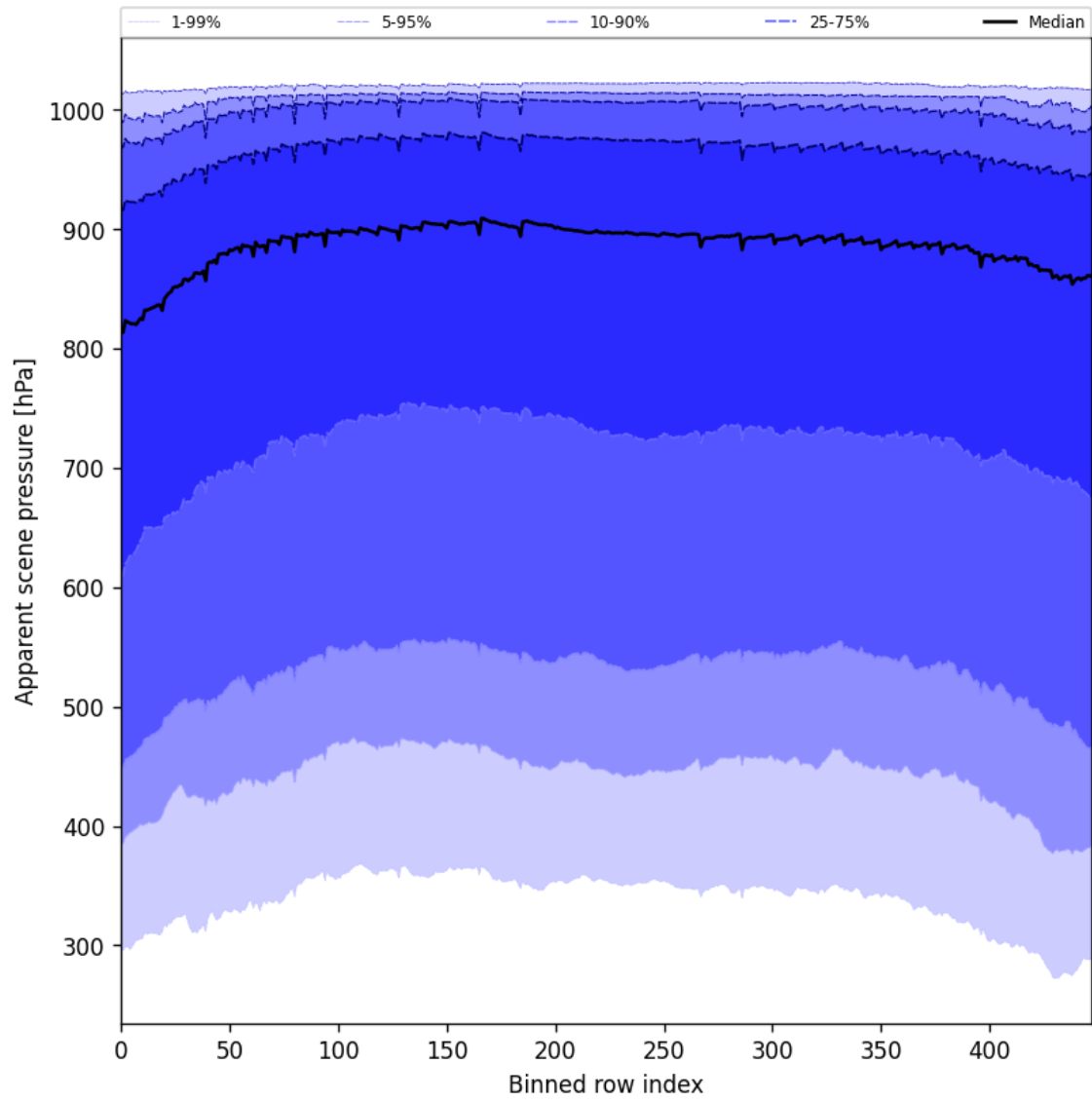
Figure 51: Along track statistics of “Apparent scene pressure” for 2025-05-27 to 2025-05-28
