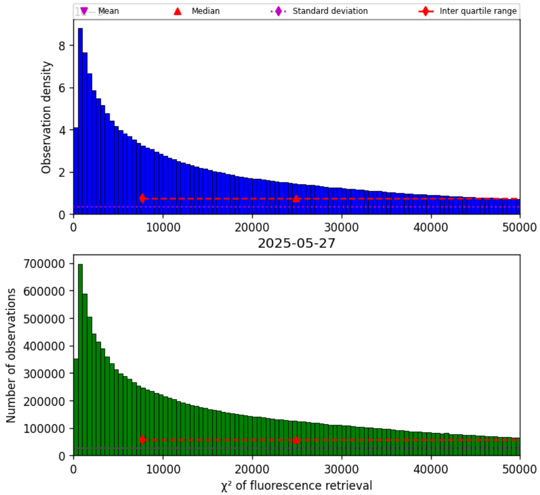
Figure 40: Histogram of “ \chi^2 of fluorescence retrieval” for 2025-05-27 to 2025-05-28
