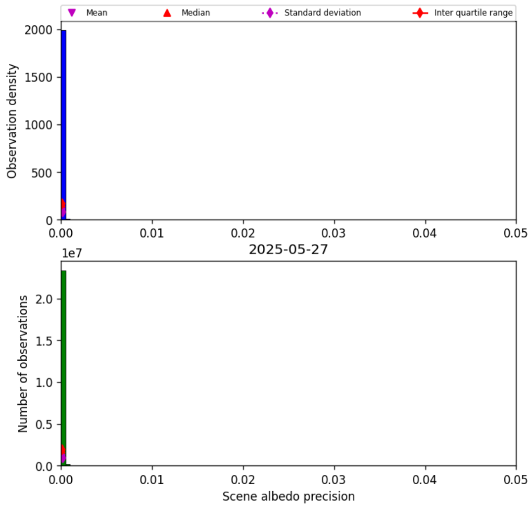
Figure 33: Histogram of “Scene albedo precision” for 2025-05-27 to 2025-05-28
