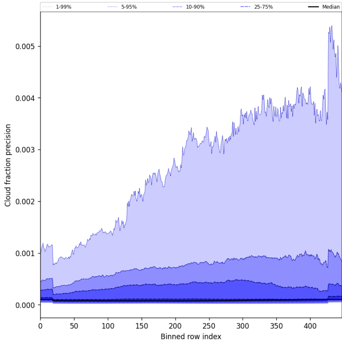
Figure 48: Along track statistics of “Cloud fraction precision” for 2025-05-27 to 2025-05-28
