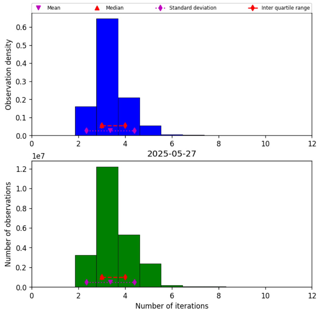
Figure 37: Histogram of “Number of iterations” for 2025-05-27 to 2025-05-28
