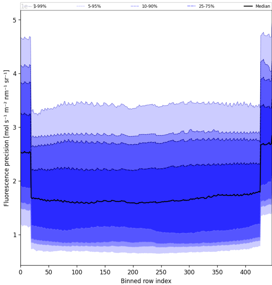
Figure 56: Along track statistics of “Fluorescence precision” for 2025-05-27 to 2025-05-28
