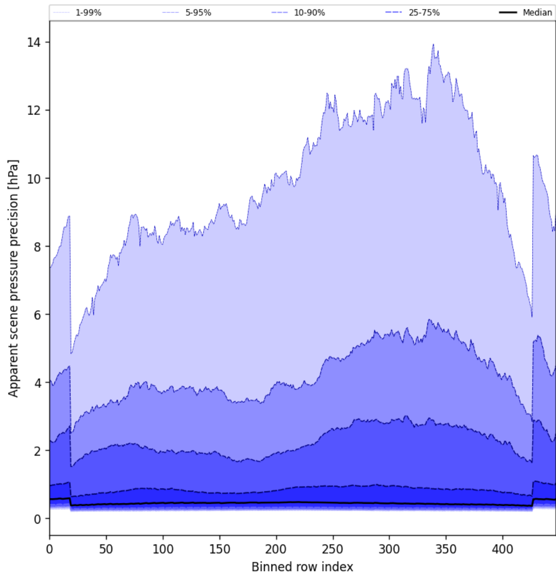
Figure 52: Along track statistics of “Apparent scene pressure precision” for 2025-05-27 to 2025-05-28
