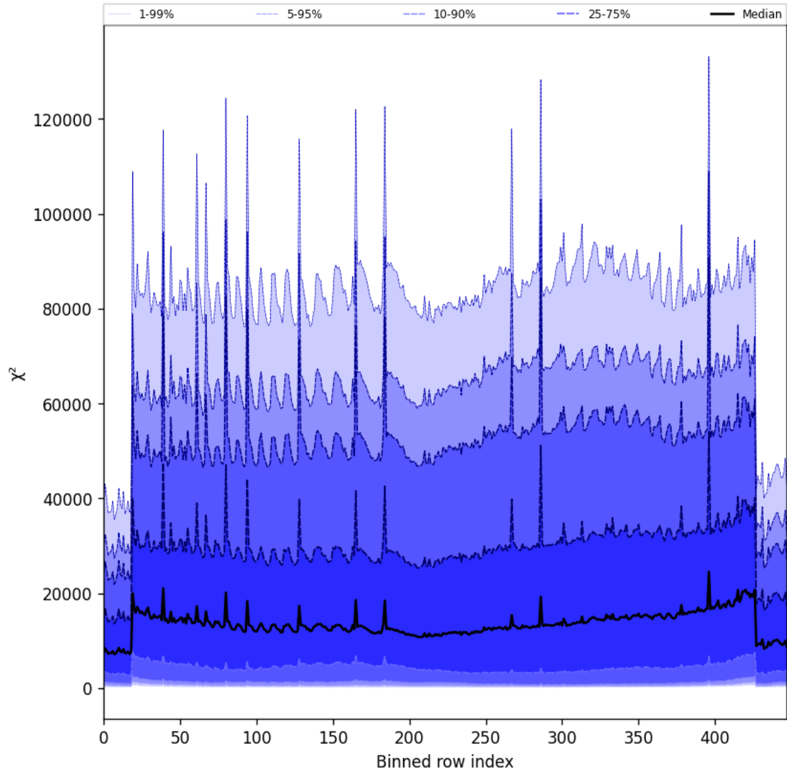
Figure 53: Along track statistics of “ \chi^2 ” for 2025-05-27 to 2025-05-28
