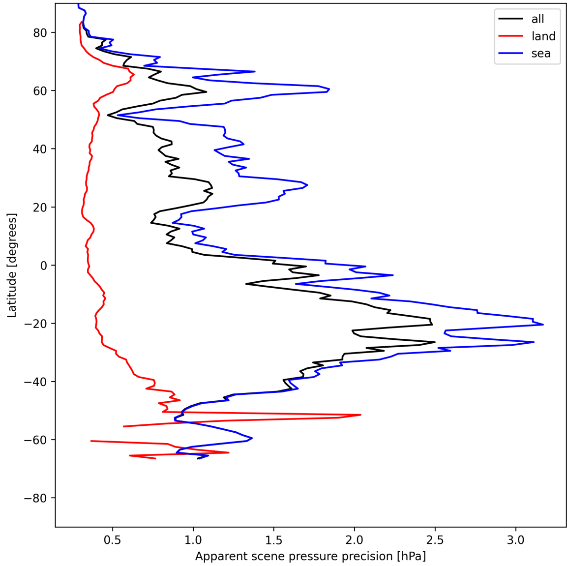
Figure 18: Zonal average of “Apparent scene pressure precision” for 2025-05-27 to 2025-05-28.
