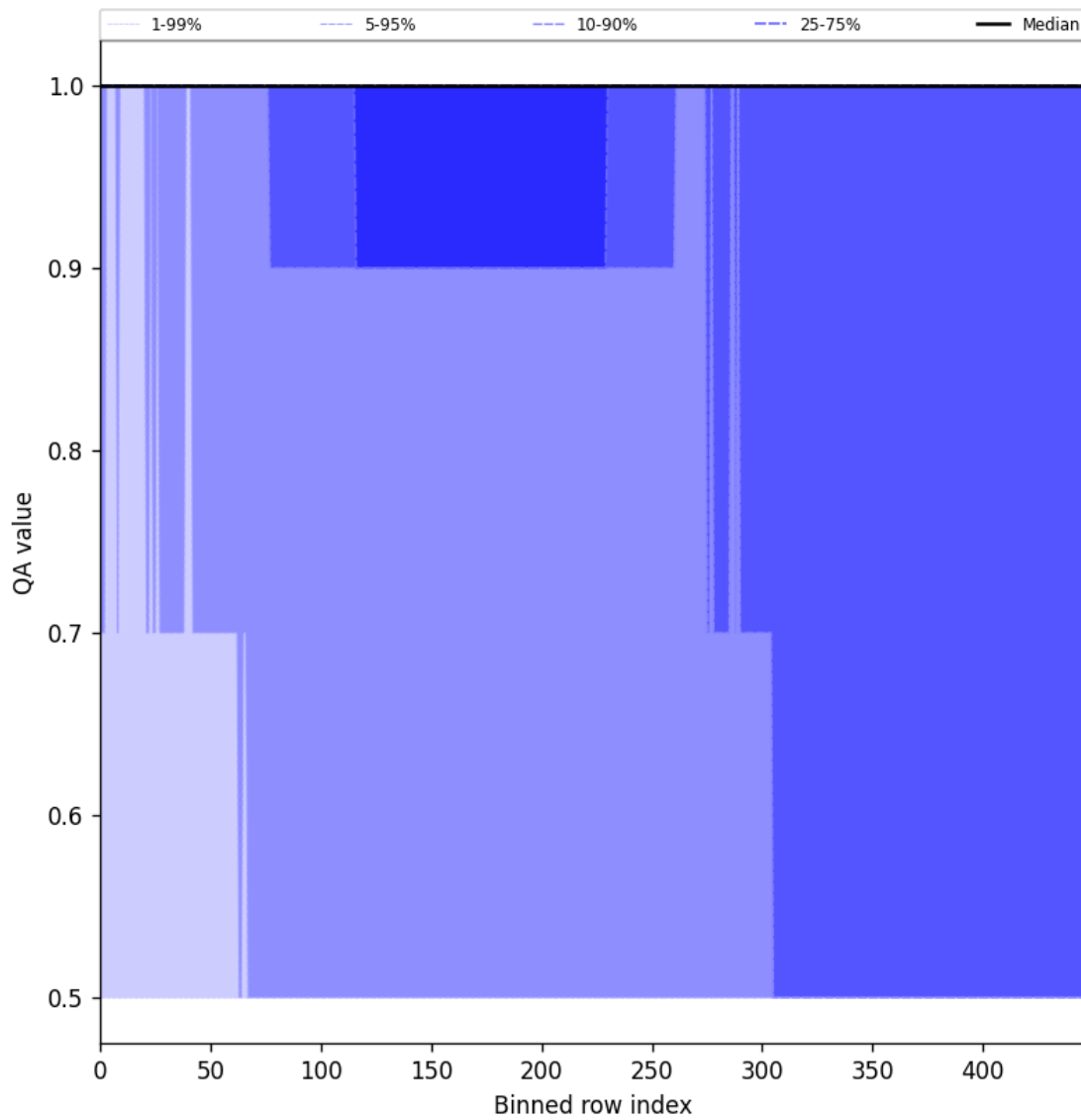
Figure 44: Along track statistics of “QA value” for 2025-05-27 to 2025-05-28
