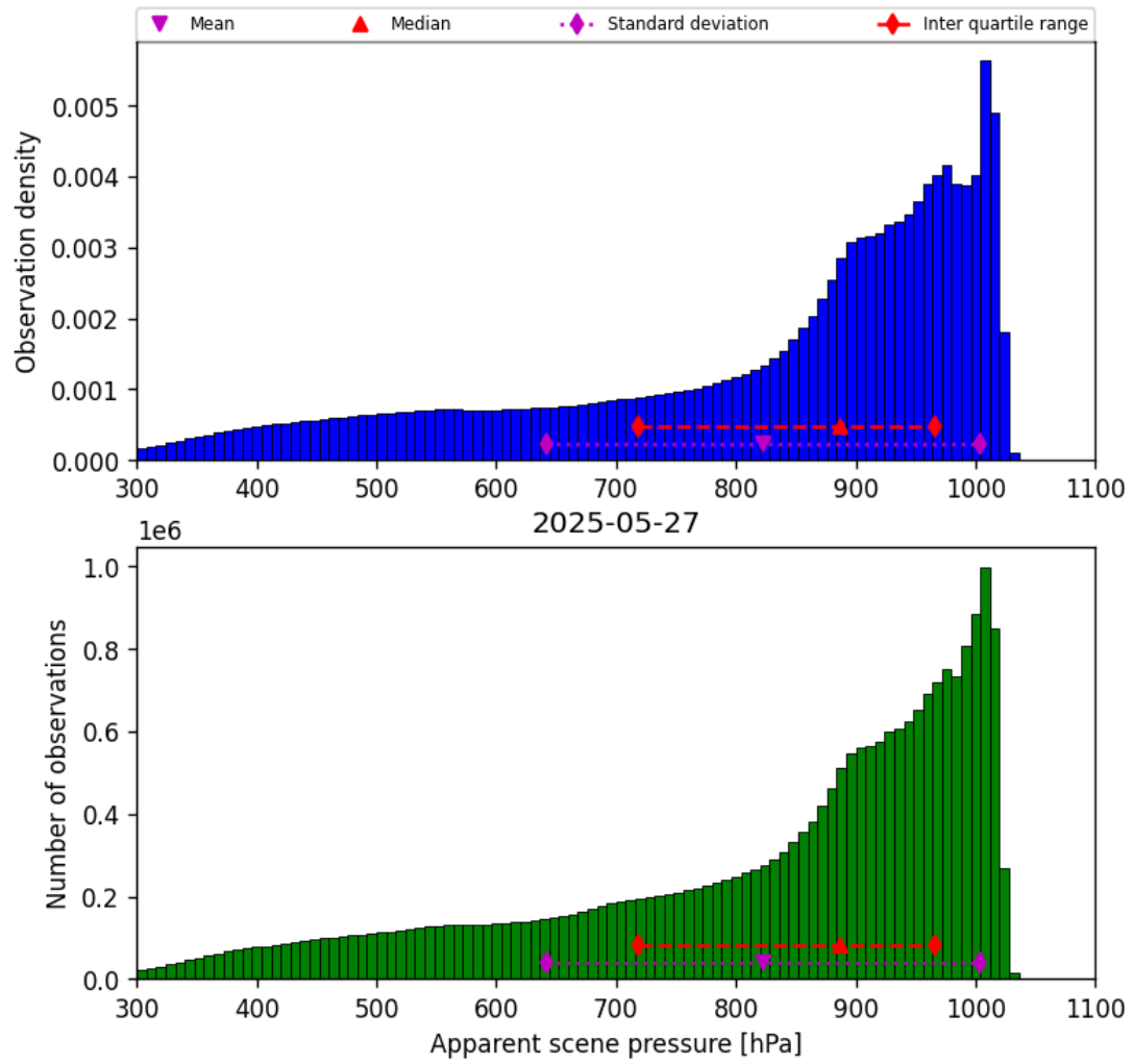
Figure 34: Histogram of “Apparent scene pressure” for 2025-05-27 to 2025-05-28
