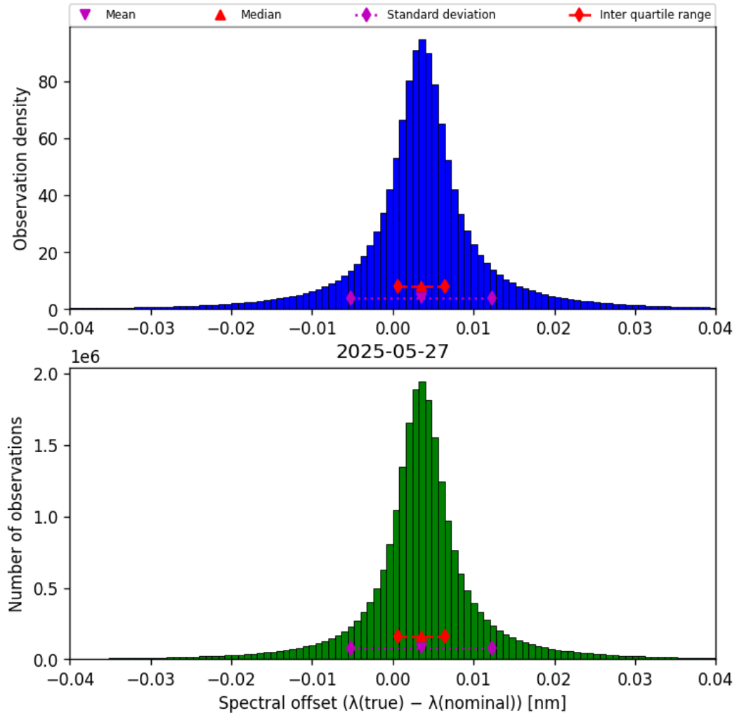
Figure 43: Histogram of “Spectral offset ( \lambda_{\text{true}} - \lambda_{\text{nominal}} )” for 2025-05-27 to 2025-05-28
