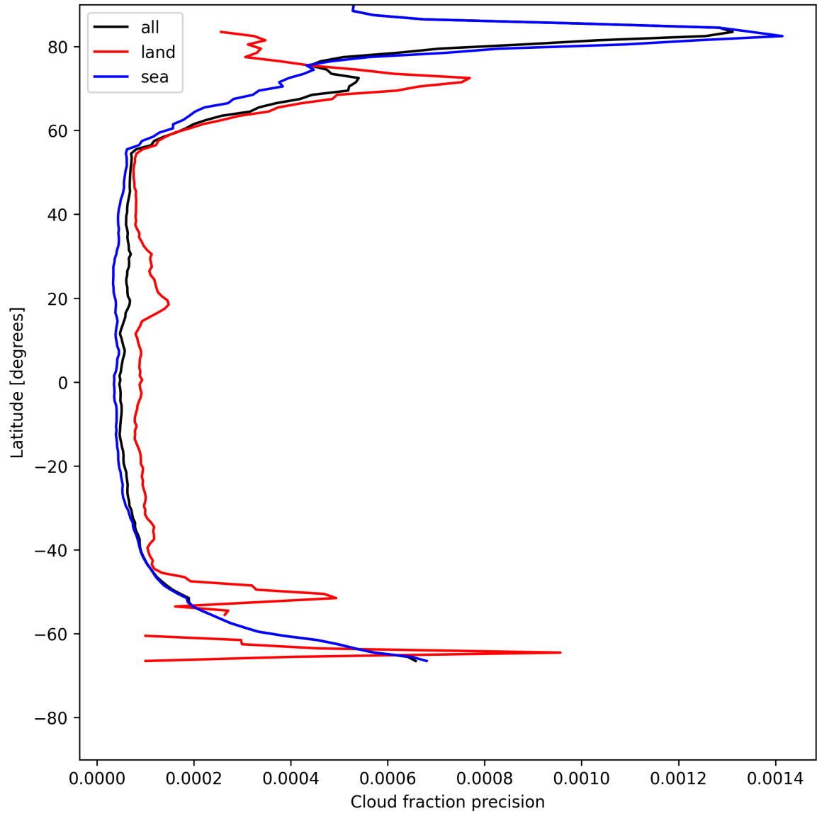
Figure 14: Zonal average of “Cloud fraction precision” for 2025-05-27 to 2025-05-28.
