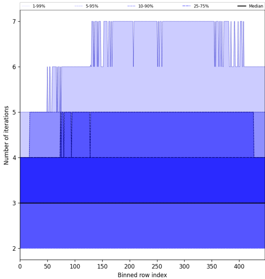
Figure 54: Along track statistics of “Number of iterations” for 2025-05-27 to 2025-05-28
