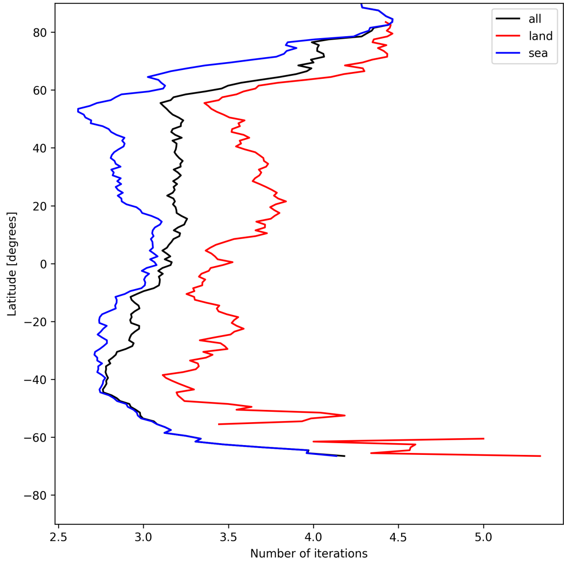
Figure 20: Zonal average of “Number of iterations” for 2025-05-27 to 2025-05-28.
