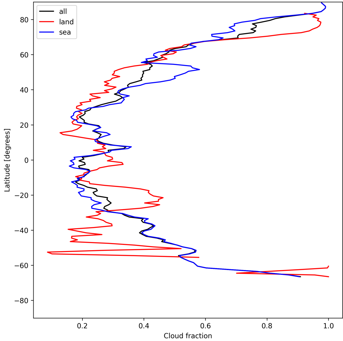
Figure 13: Zonal average of “Cloud fraction” for 2025-05-27 to 2025-05-28.
