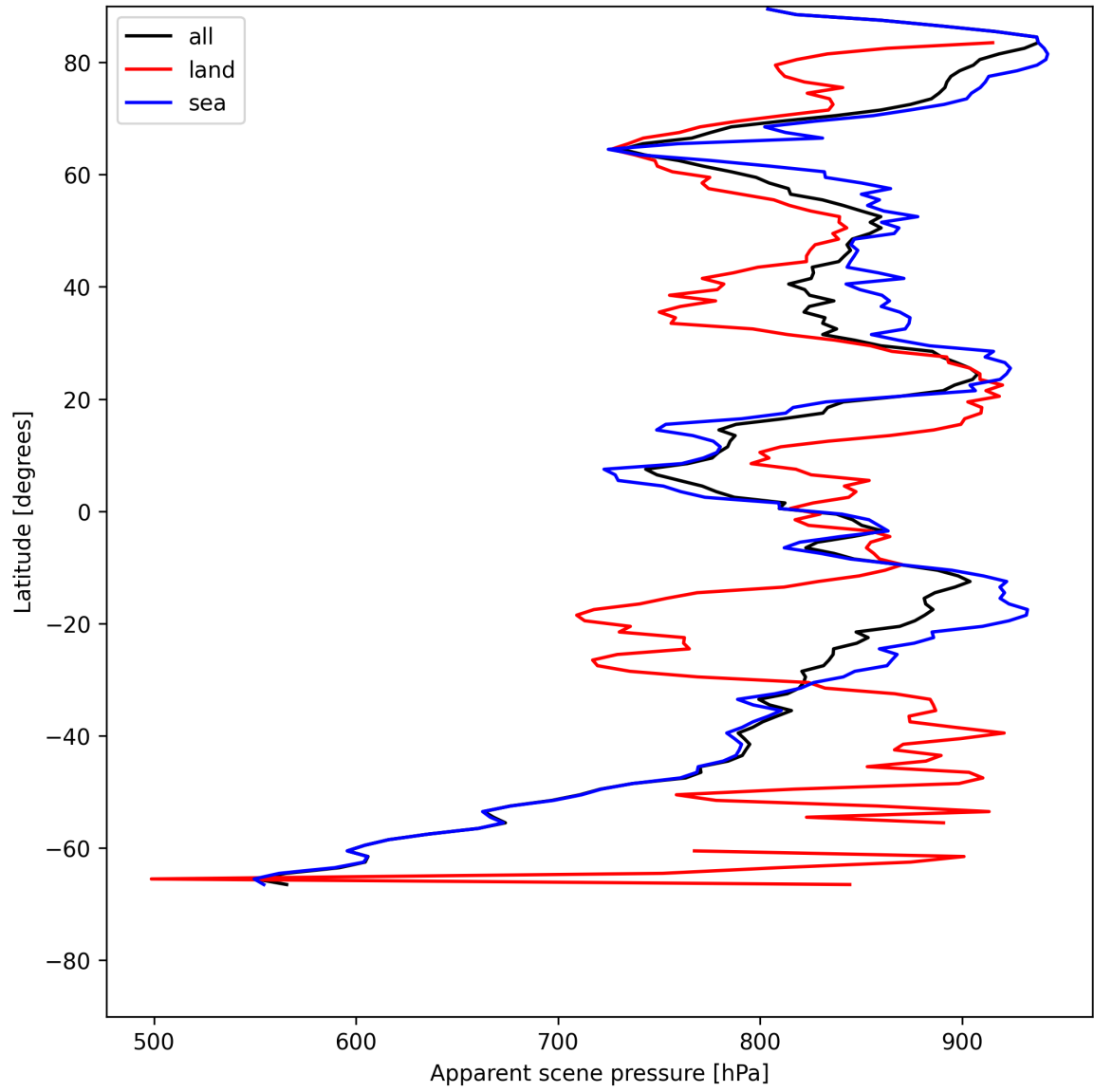
Figure 17: Zonal average of “Apparent scene pressure” for 2025-05-27 to 2025-05-28.
