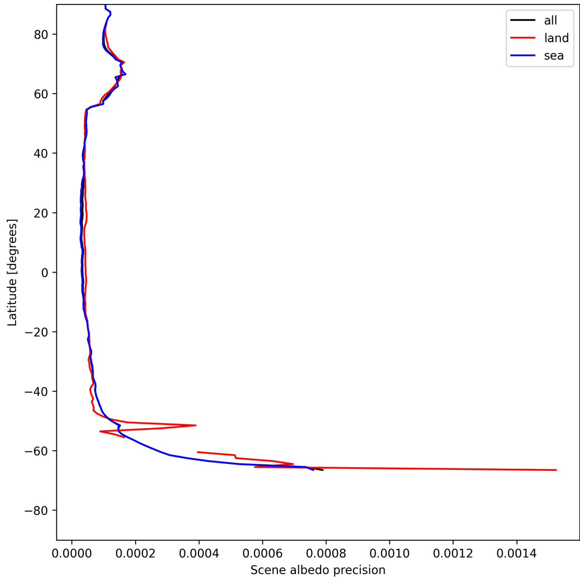
Figure 16: Zonal average of “Scene albedo precision” for 2025-05-27 to 2025-05-28.
