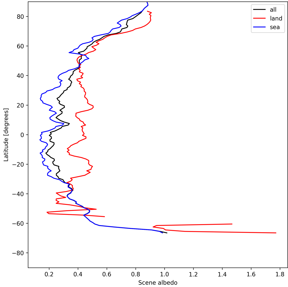
Figure 15: Zonal average of “Scene albedo” for 2025-05-27 to 2025-05-28.
