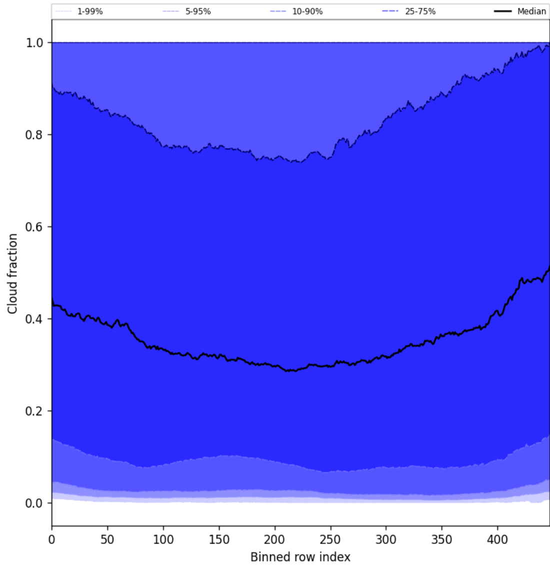
Figure 47: Along track statistics of “Cloud fraction” for 2025-05-27 to 2025-05-28
