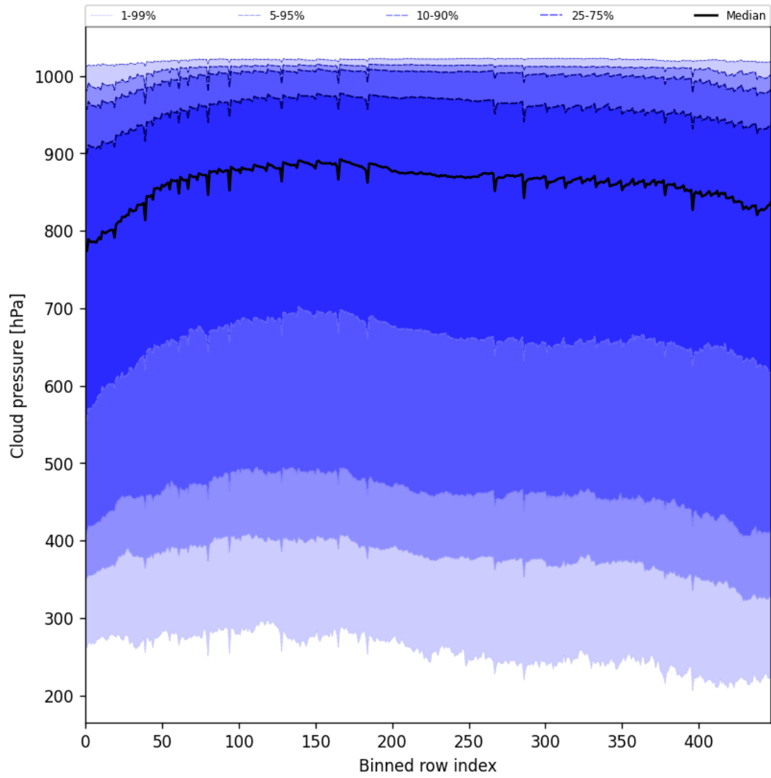
Figure 45: Along track statistics of “Cloud pressure” for 2025-05-27 to 2025-05-28
