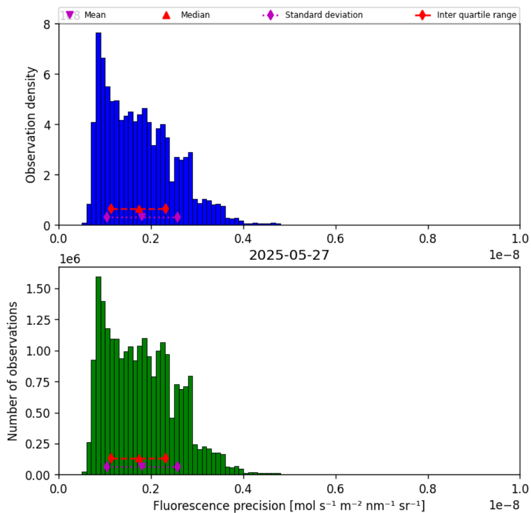
Figure 39: Histogram of “Fluorescence precision” for 2025-05-27 to 2025-05-28
