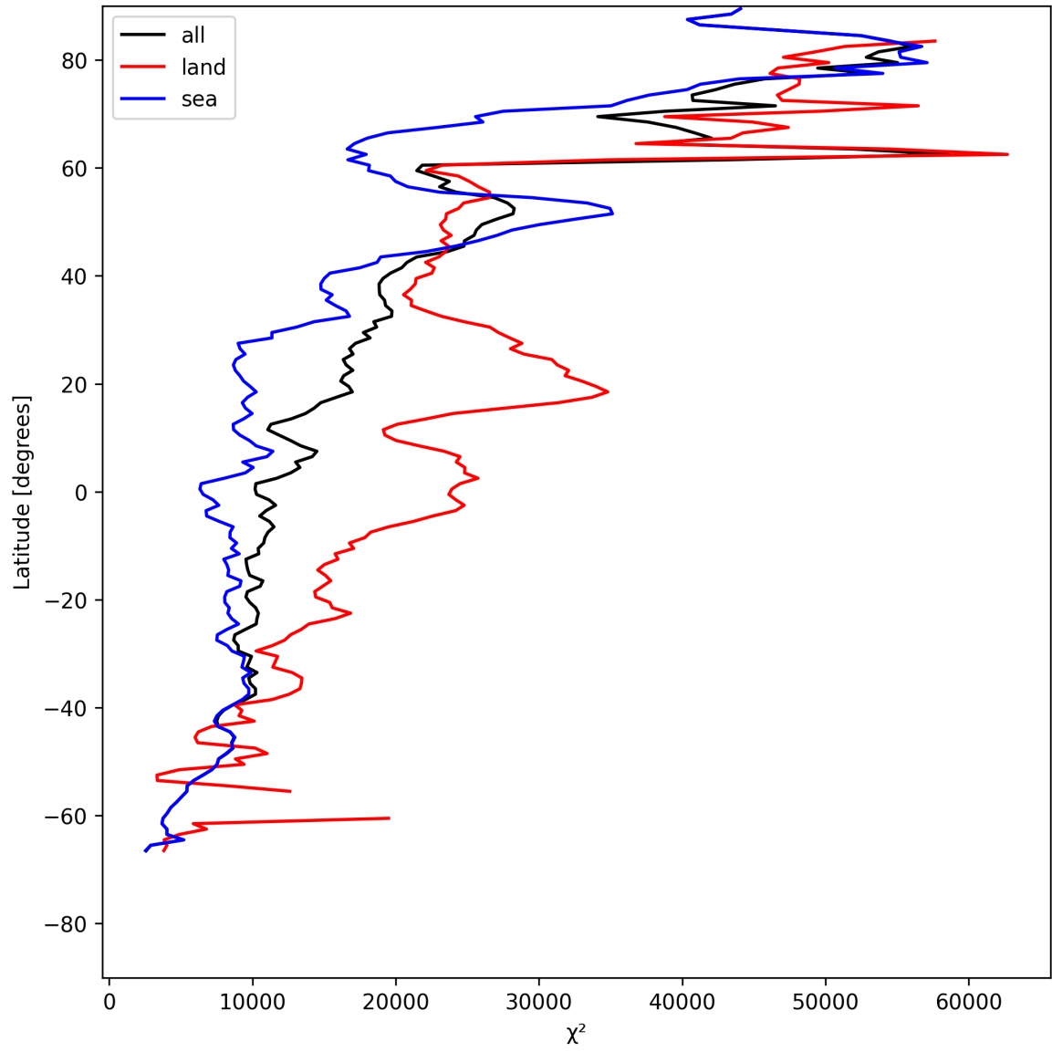
Figure 19: Zonal average of “ \chi^2 ” for 2025-05-27 to 2025-05-28.
