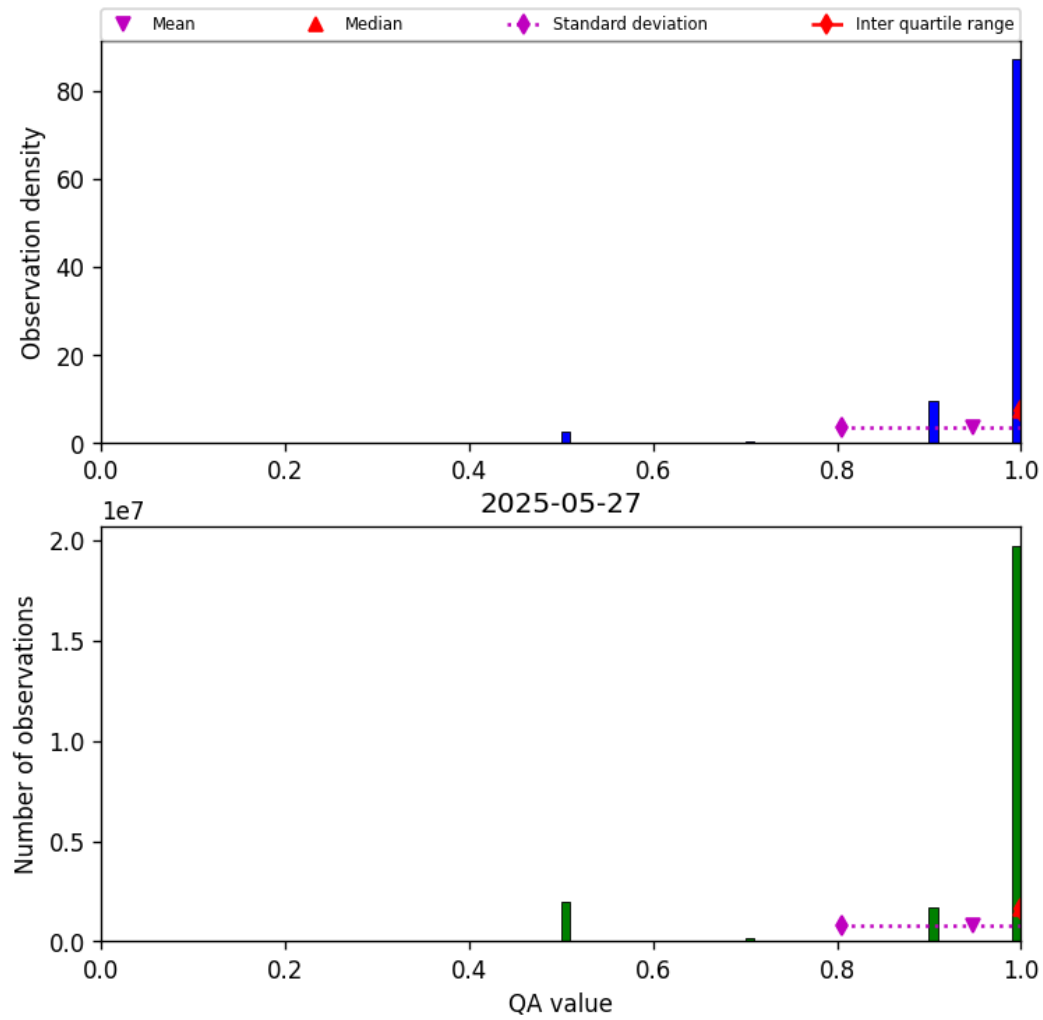
Figure 27: Histogram of “QA value” for 2025-05-27 to 2025-05-28
