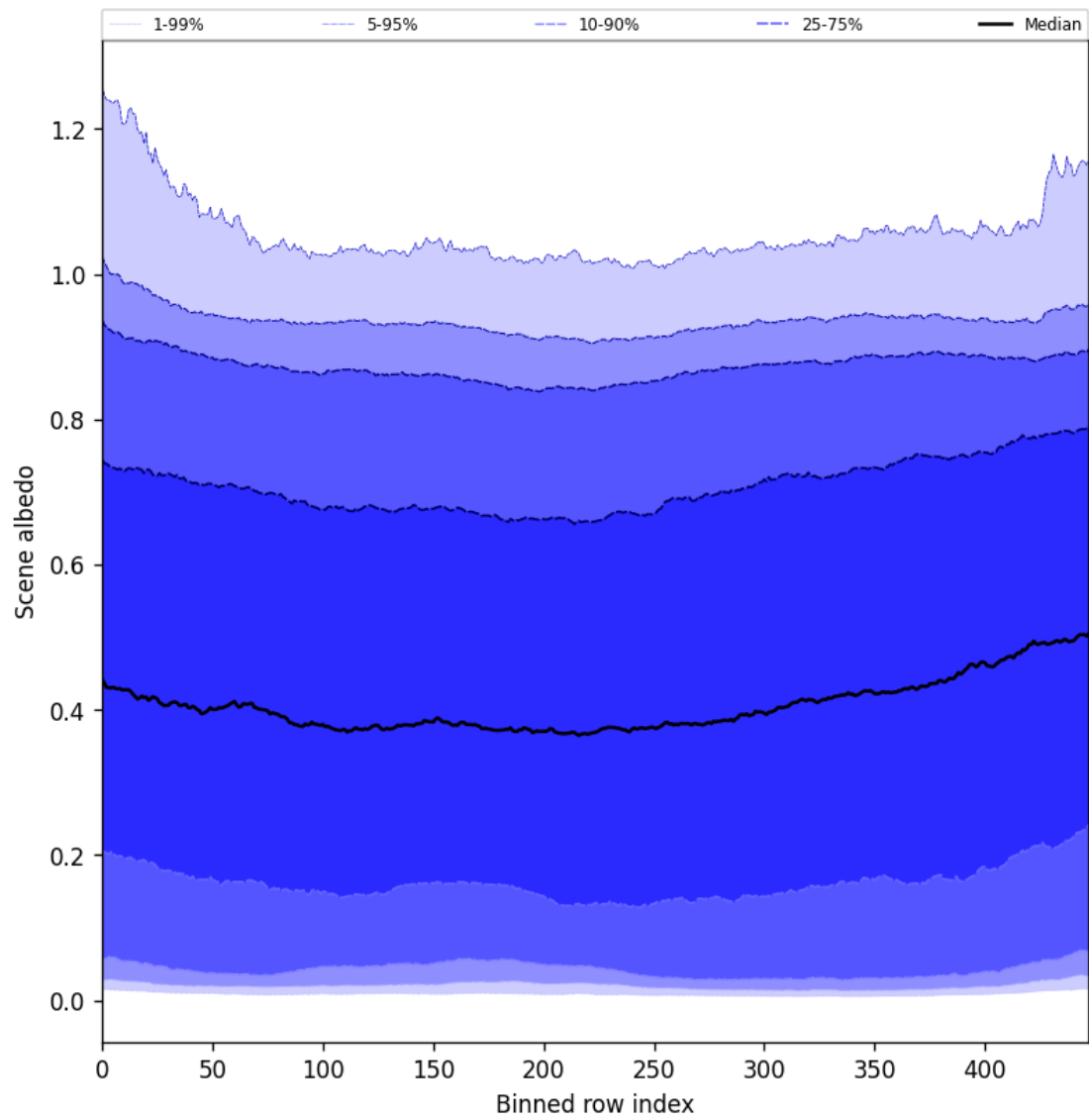
Figure 49: Along track statistics of “Scene albedo” for 2025-05-27 to 2025-05-28
