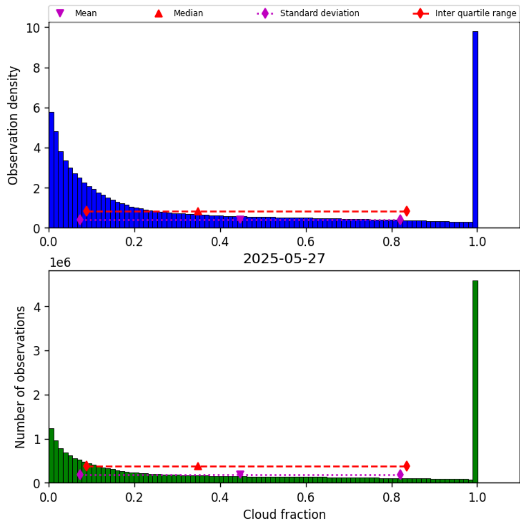
Figure 30: Histogram of “Cloud fraction” for 2025-05-27 to 2025-05-28
