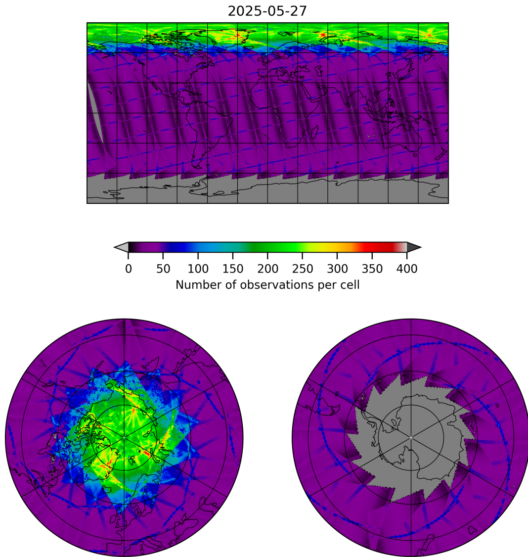
Figure 9: Map of the number of observations for 2025-05-27 to 2025-05-28
