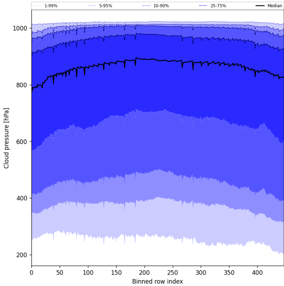
Figure 45: Along track statistics of “Cloud pressure” for 2025-05-28 to 2025-05-29
