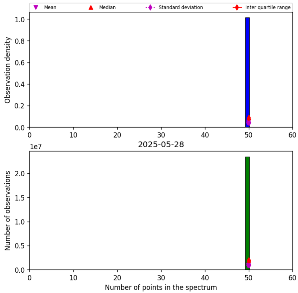
Figure 42: Histogram of “Number of points in the spectrum” for 2025-05-28 to 2025-05-29
