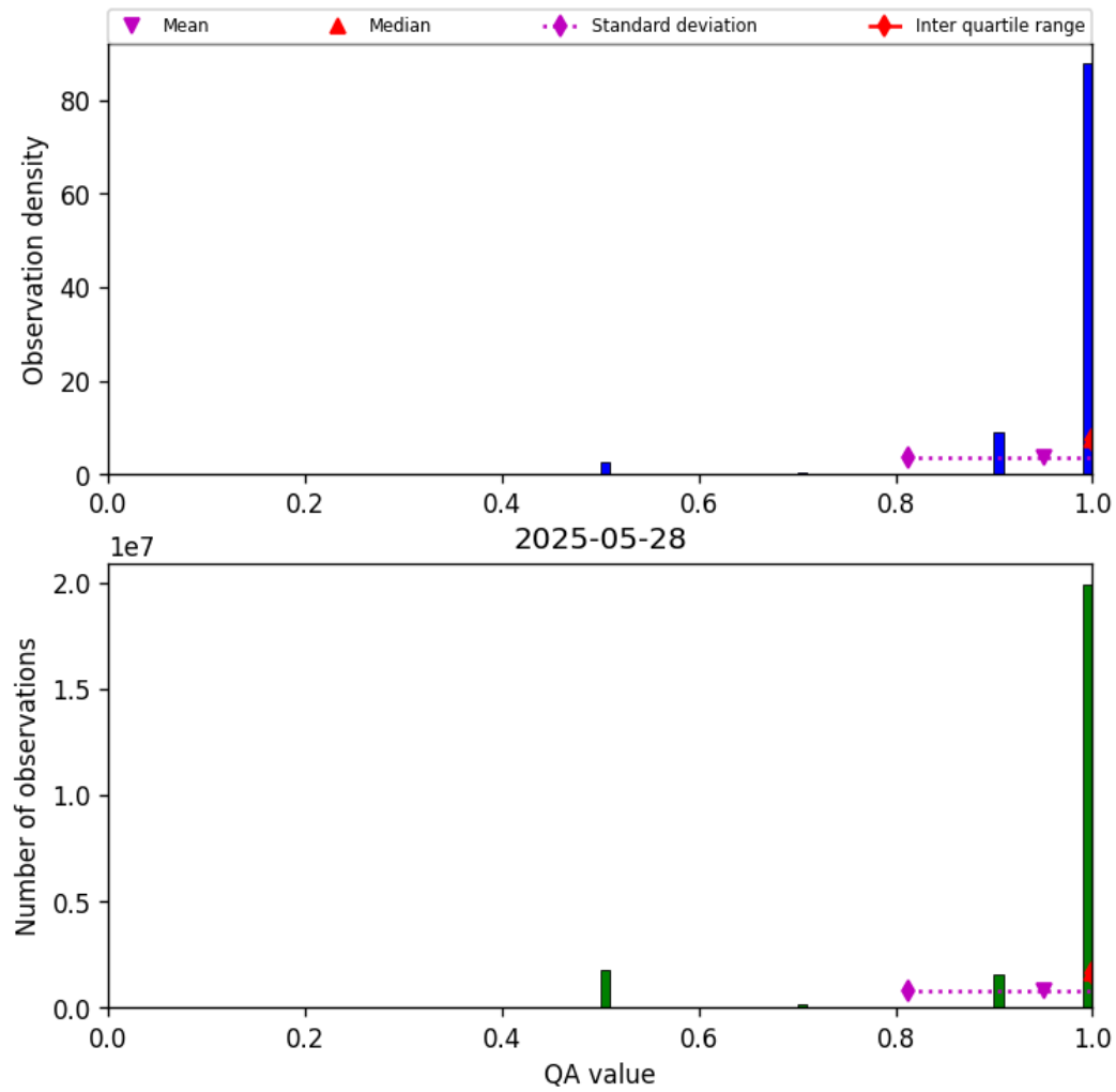
Figure 27: Histogram of “QA value” for 2025-05-28 to 2025-05-29
