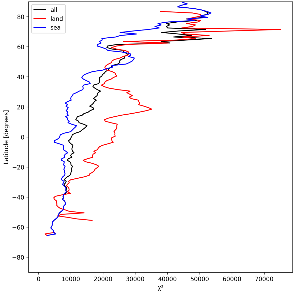
Figure 19: Zonal average of “ \chi^2 ” for 2025-05-28 to 2025-05-29.
