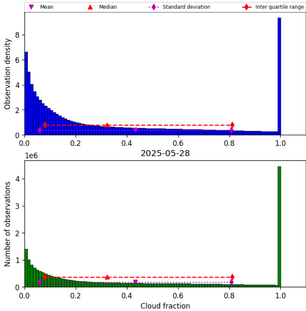
Figure 30: Histogram of “Cloud fraction” for 2025-05-28 to 2025-05-29
