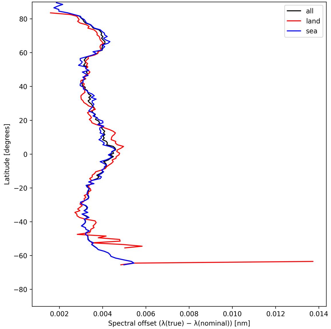
Figure 26: Zonal average of “Spectral offset ( \lambda_{\text{true}} - \lambda_{\text{nominal}} )” for 2025-05-28 to 2025-05-29.
