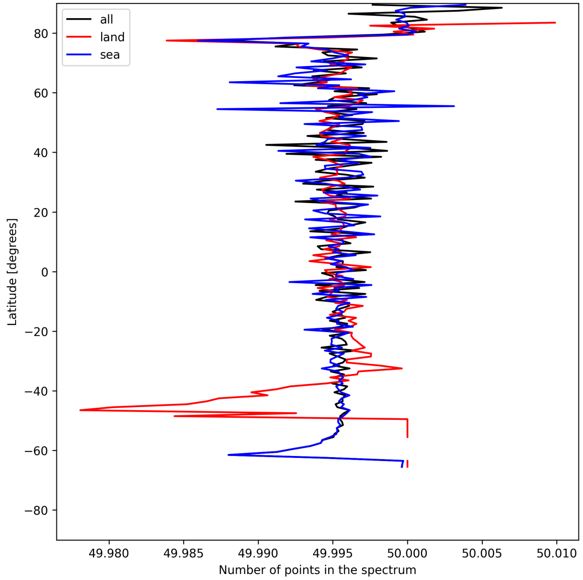
Figure 25: Zonal average of “Number of points in the spectrum” for 2025-05-28 to 2025-05-29.
