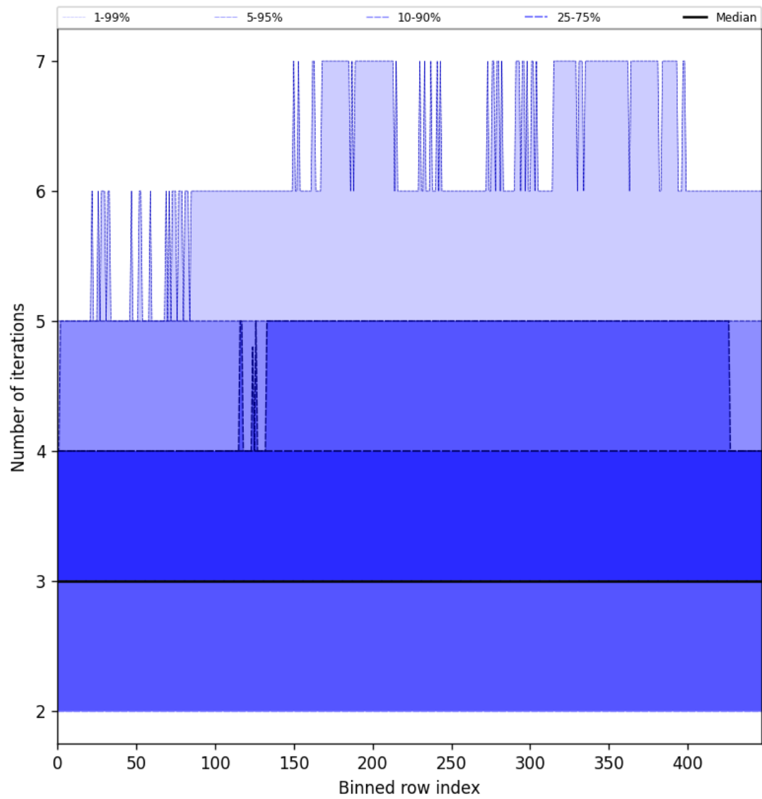
Figure 54: Along track statistics of “Number of iterations” for 2025-05-28 to 2025-05-29
