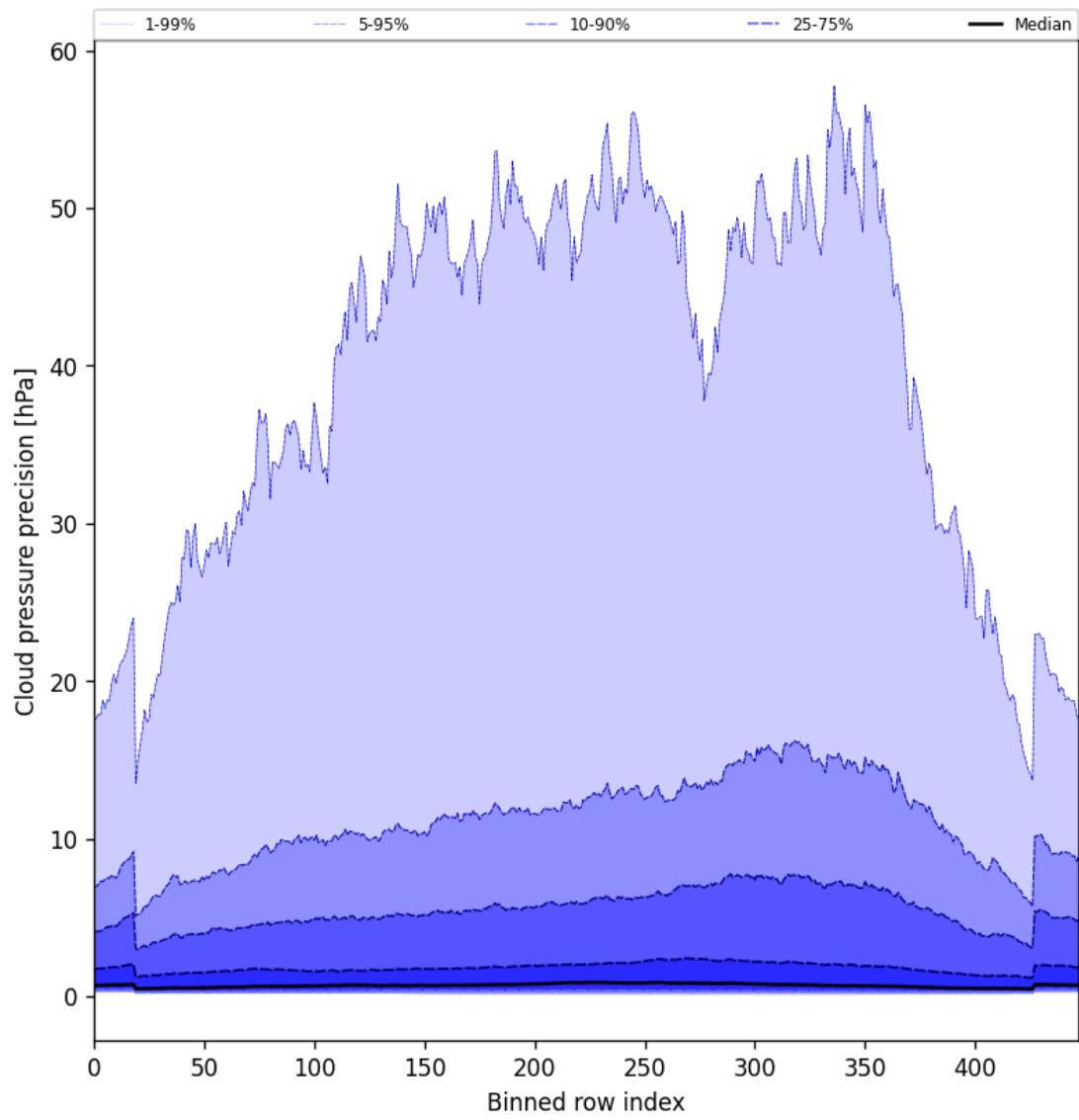
Figure 46: Along track statistics of “Cloud pressure precision” for 2025-05-28 to 2025-05-29
