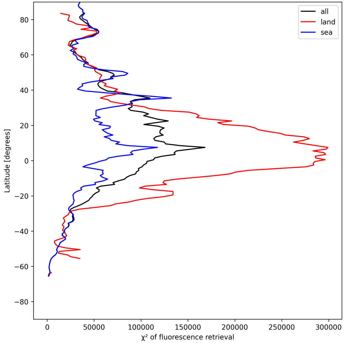
Figure 23: Zonal average of “ \chi^2 of fluorescence retrieval” for 2025-05-28 to 2025-05-29.
