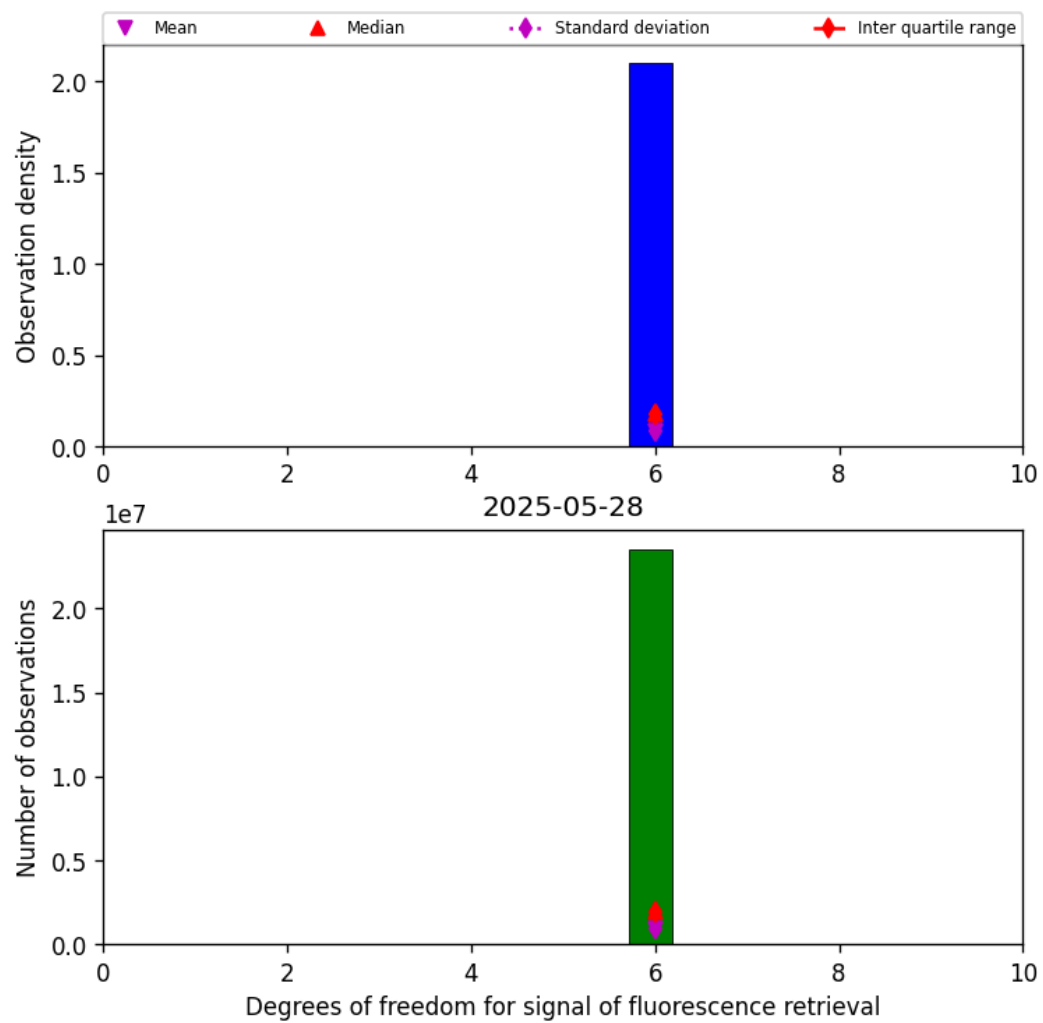
Figure 41: Histogram of “Degrees of freedom for signal of fluorescence retrieval” for 2025-05-28 to 2025-05-29
