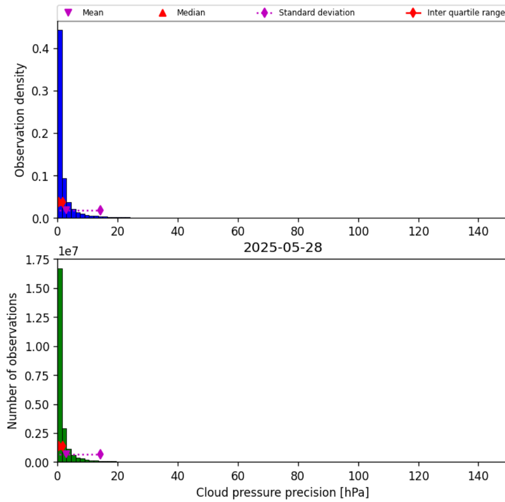
Figure 29: Histogram of “Cloud pressure precision” for 2025-05-28 to 2025-05-29
