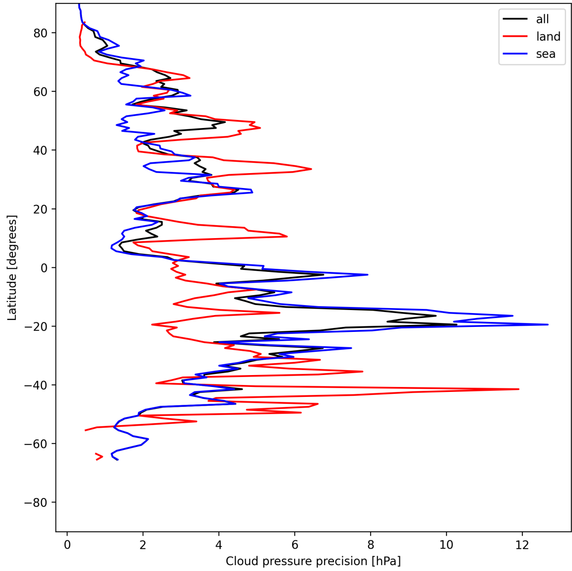
Figure 12: Zonal average of “Cloud pressure precision” for 2025-05-28 to 2025-05-29.
