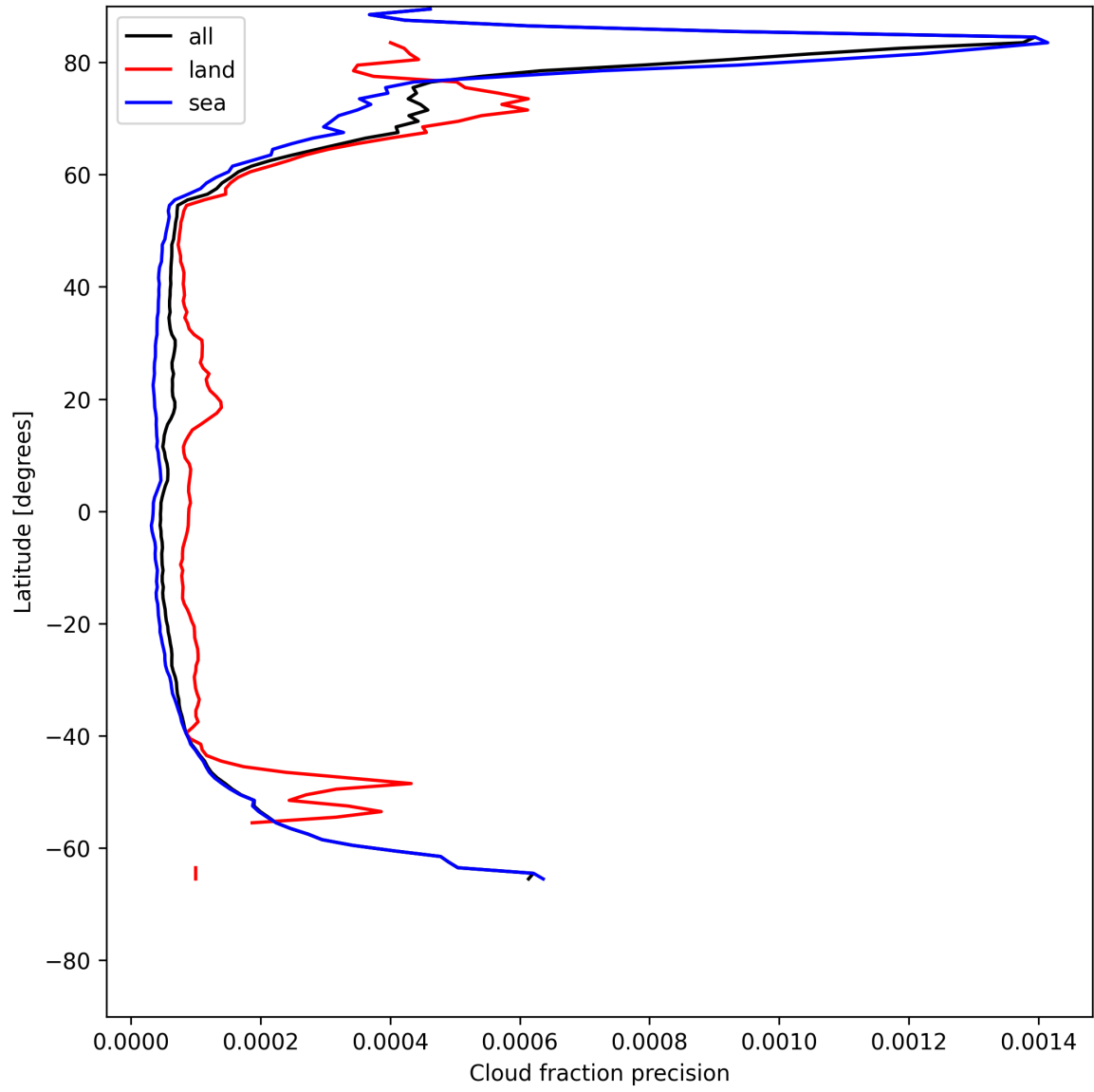
Figure 14: Zonal average of “Cloud fraction precision” for 2025-05-28 to 2025-05-29.
