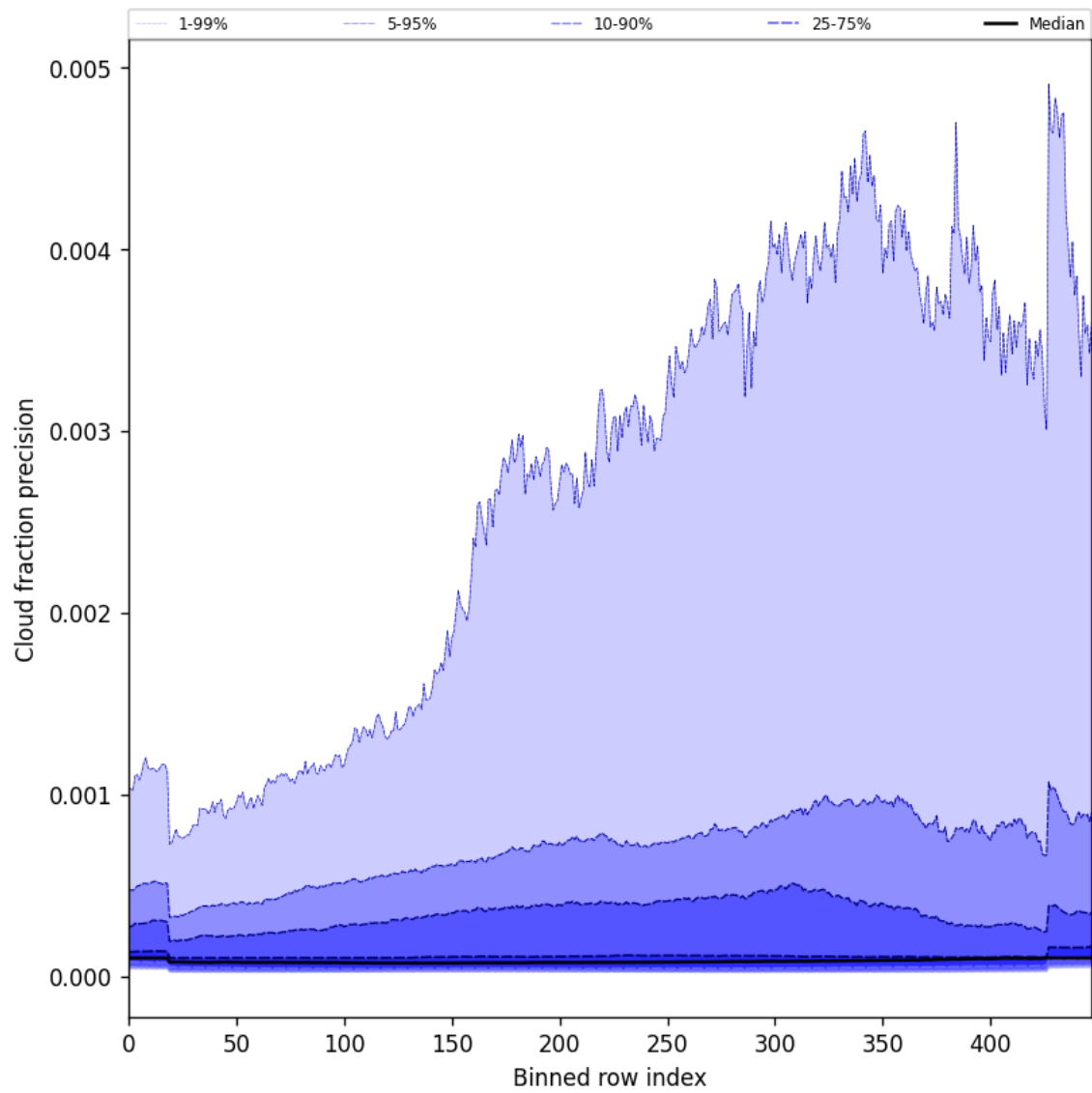
Figure 48: Along track statistics of “Cloud fraction precision” for 2025-05-28 to 2025-05-29
