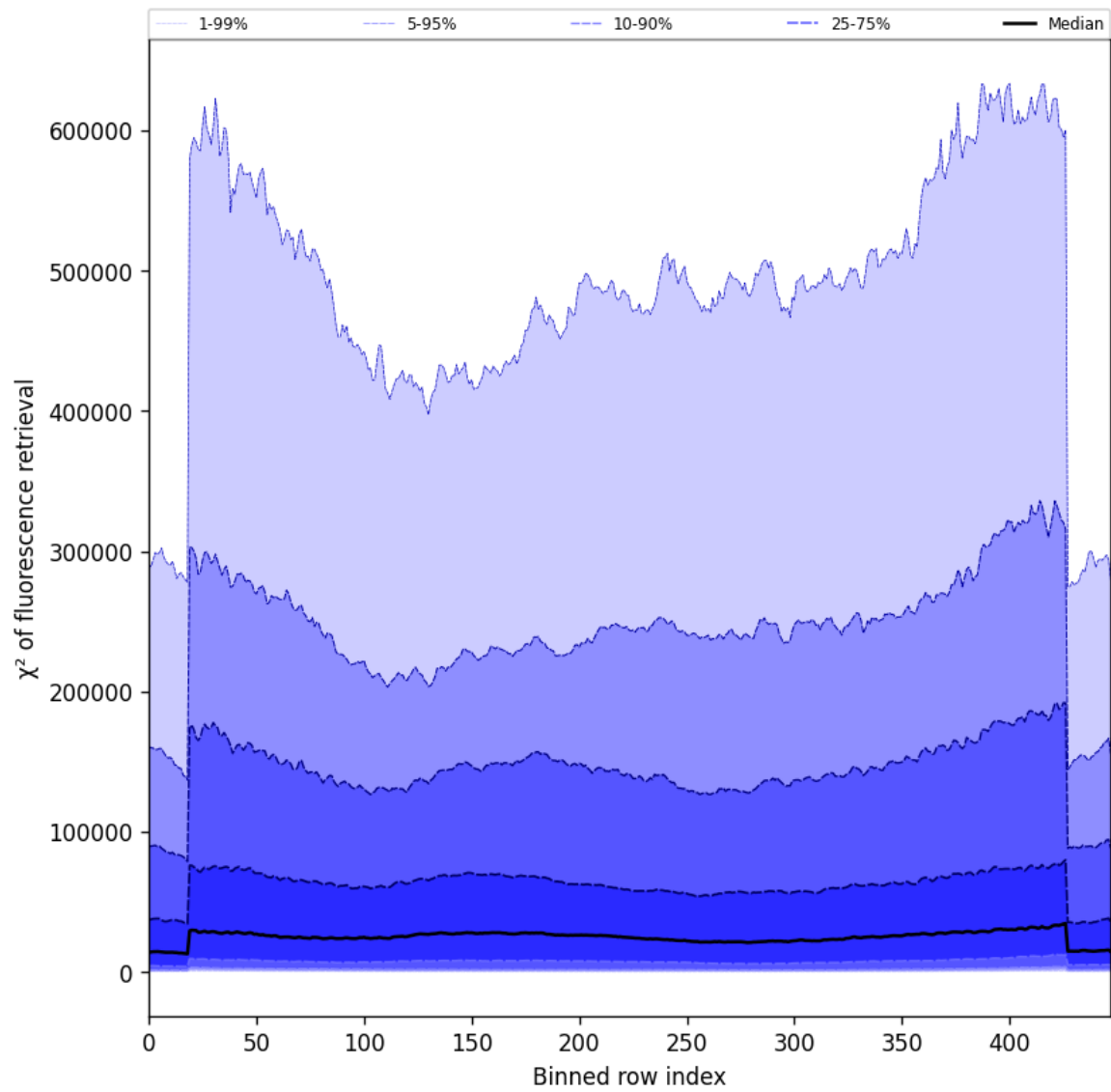
Figure 57: Along track statistics of “ \chi^2 of fluorescence retrieval” for 2025-05-28 to 2025-05-29
