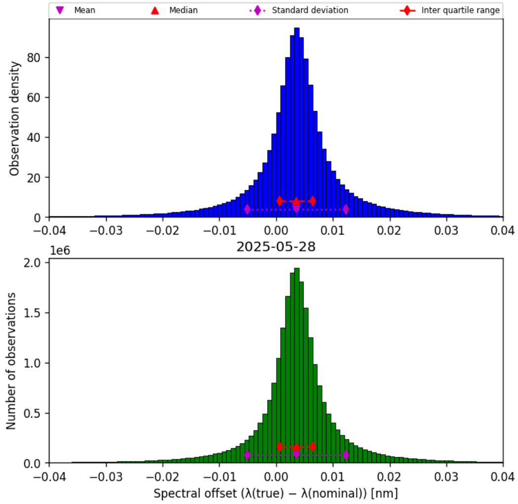
Figure 43: Histogram of “Spectral offset ( \lambda_{\text{true}} - \lambda_{\text{nominal}} )” for 2025-05-28 to 2025-05-29
