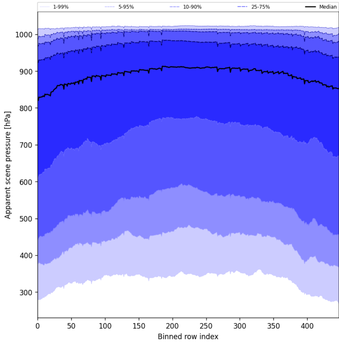
Figure 51: Along track statistics of “Apparent scene pressure” for 2025-05-28 to 2025-05-29
