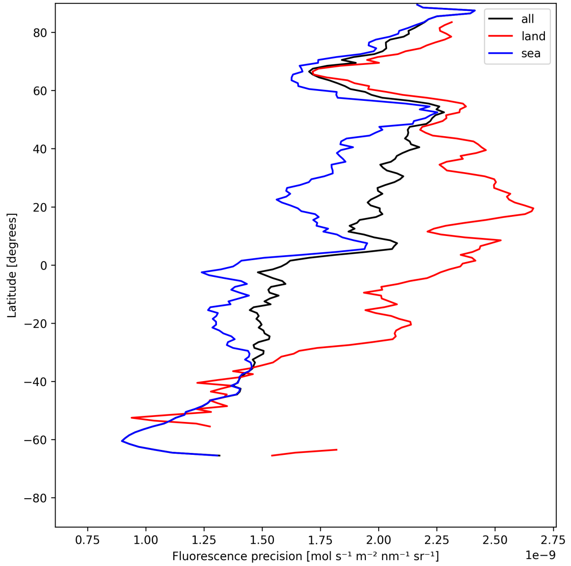
Figure 22: Zonal average of “Fluorescence precision” for 2025-05-28 to 2025-05-29.
