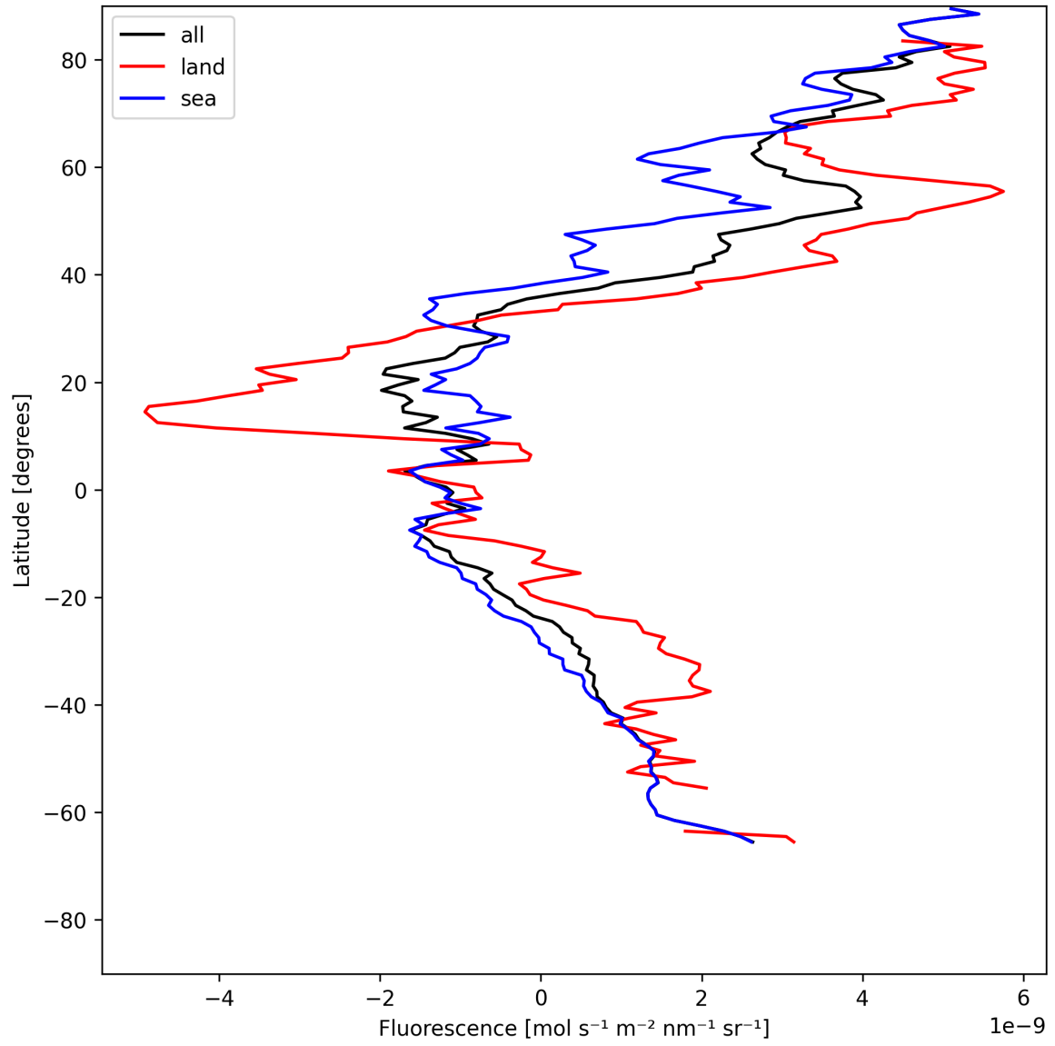
Figure 21: Zonal average of “Fluorescence” for 2025-05-28 to 2025-05-29.
