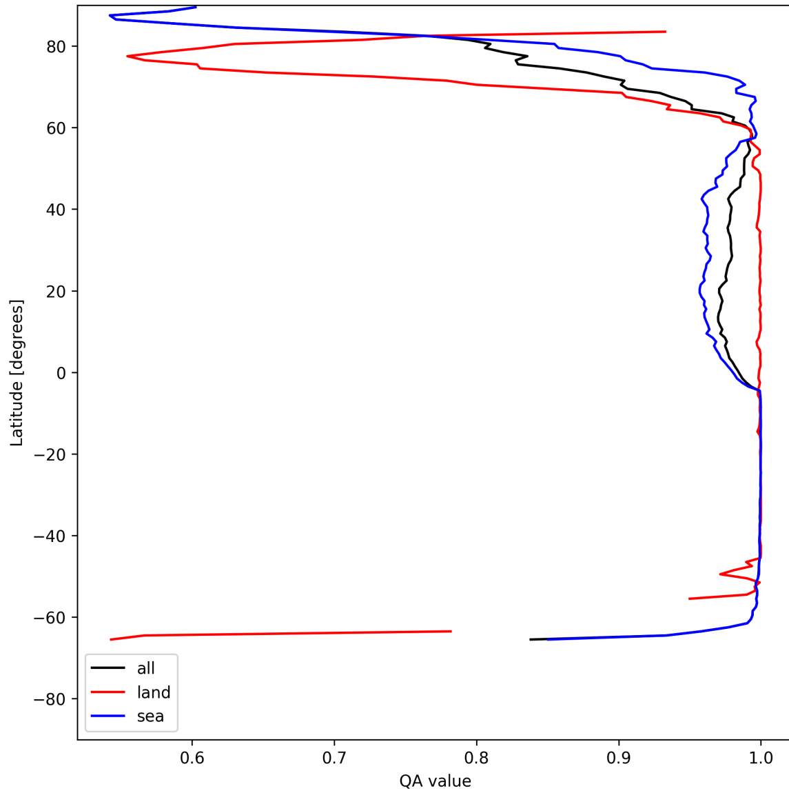
Figure 10: Zonal average of “QA value” for 2025-05-28 to 2025-05-29.
