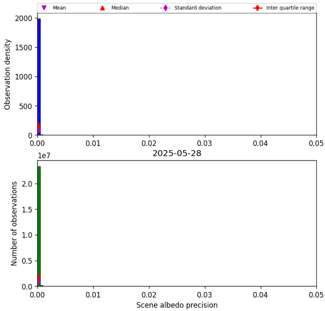
Figure 33: Histogram of “Scene albedo precision” for 2025-05-28 to 2025-05-29
