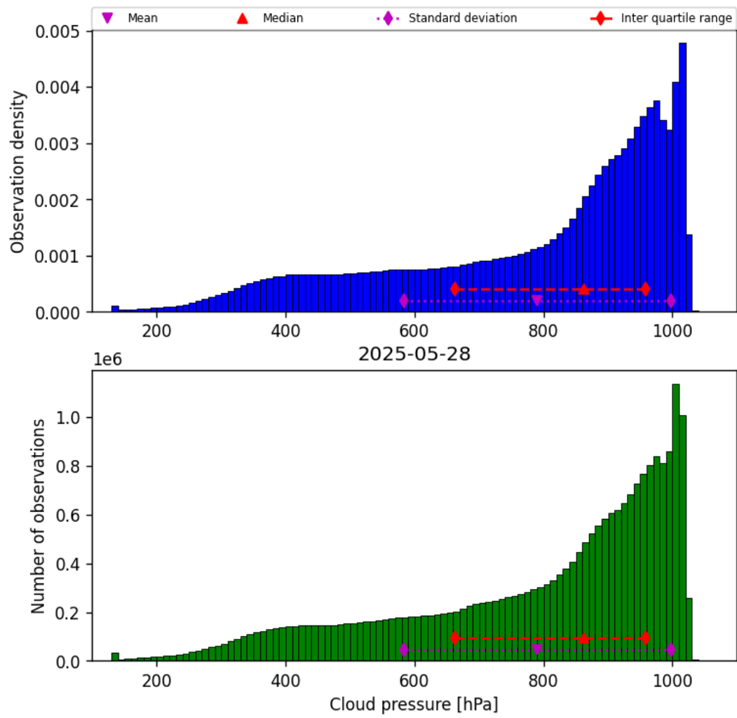
Figure 28: Histogram of “Cloud pressure” for 2025-05-28 to 2025-05-29
