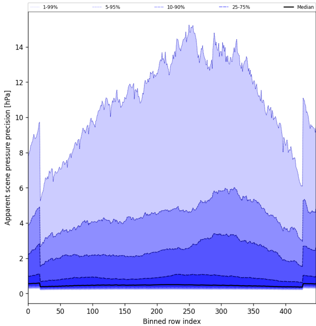
Figure 52: Along track statistics of “Apparent scene pressure precision” for 2025-05-28 to 2025-05-29
