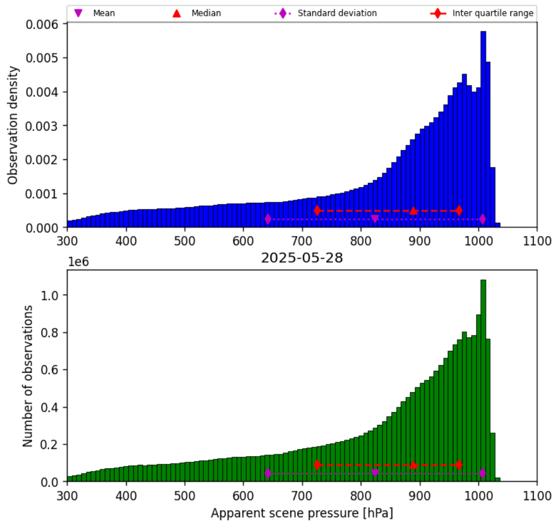
Figure 34: Histogram of “Apparent scene pressure” for 2025-05-28 to 2025-05-29
