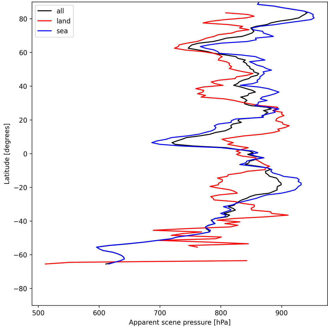
Figure 17: Zonal average of “Apparent scene pressure” for 2025-05-28 to 2025-05-29.
