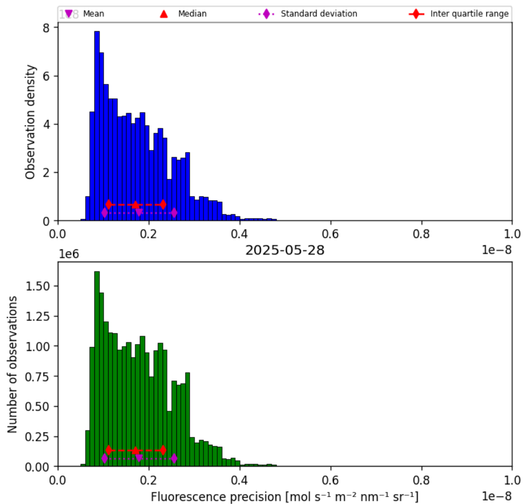
Figure 39: Histogram of “Fluorescence precision” for 2025-05-28 to 2025-05-29
