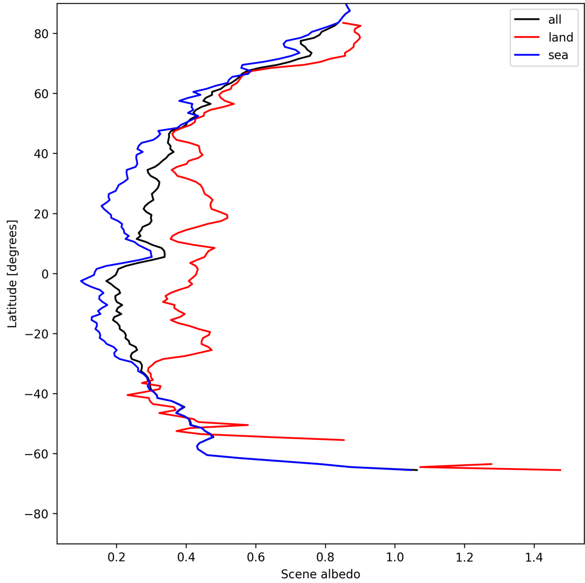
Figure 15: Zonal average of “Scene albedo” for 2025-05-28 to 2025-05-29.
