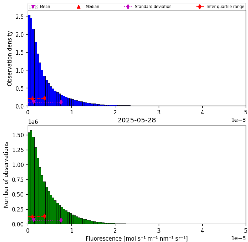
Figure 38: Histogram of “Fluorescence” for 2025-05-28 to 2025-05-29
