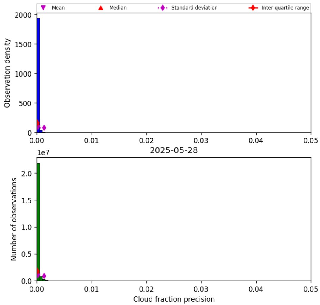
Figure 31: Histogram of “Cloud fraction precision” for 2025-05-28 to 2025-05-29
