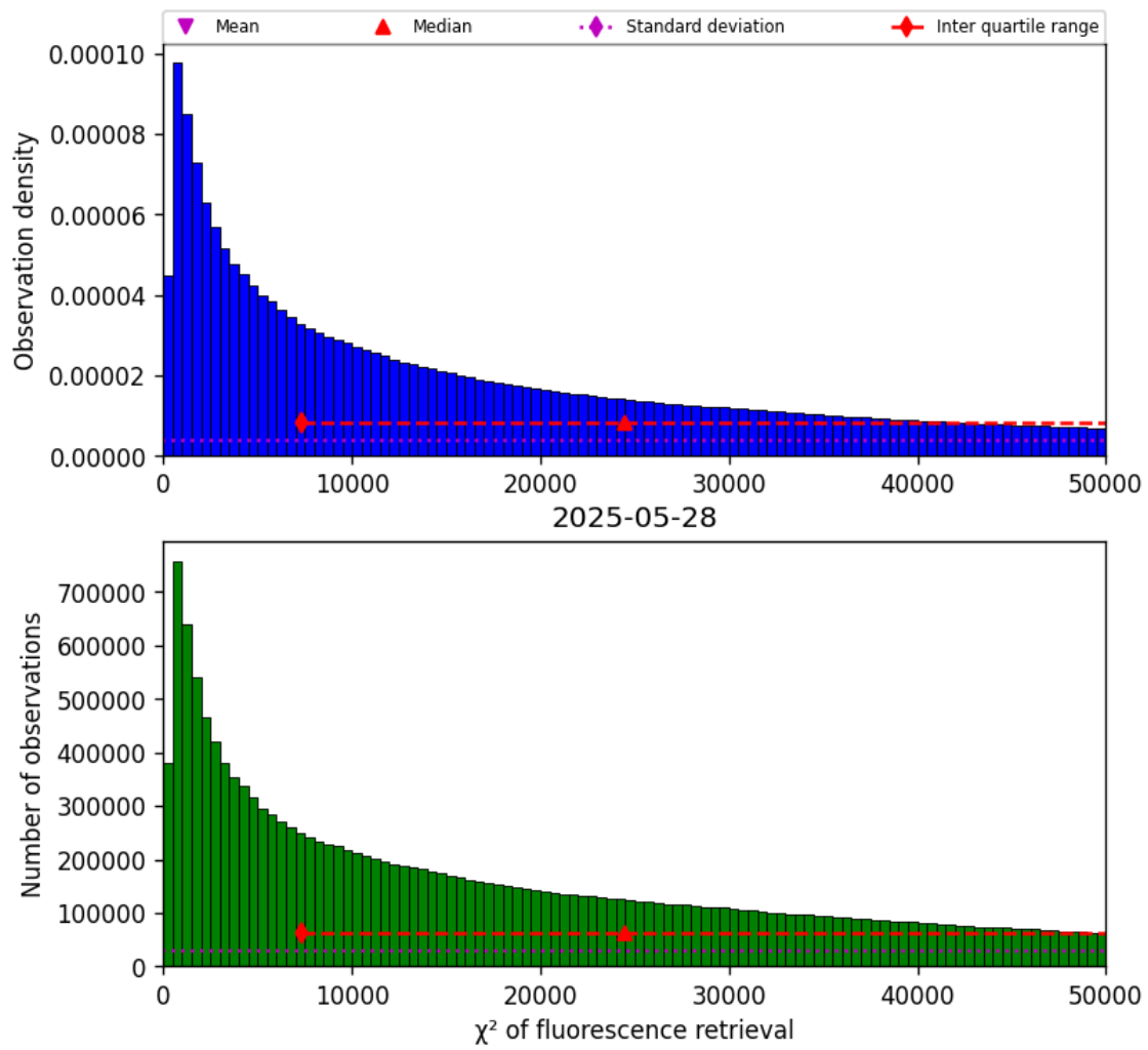
Figure 40: Histogram of “ \chi^2 of fluorescence retrieval” for 2025-05-28 to 2025-05-29
