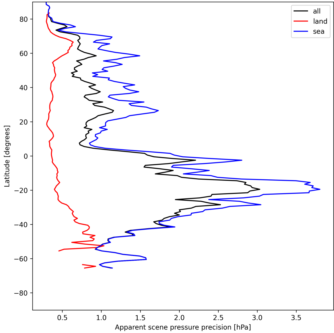
Figure 18: Zonal average of “Apparent scene pressure precision” for 2025-05-28 to 2025-05-29.
