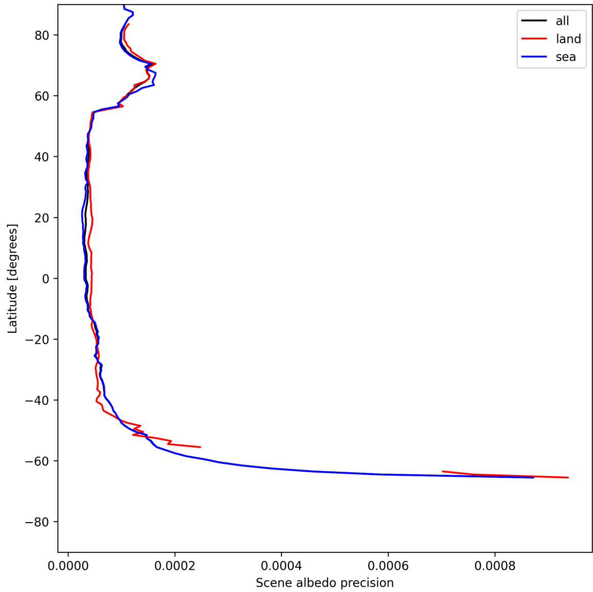
Figure 16: Zonal average of “Scene albedo precision” for 2025-05-28 to 2025-05-29.
