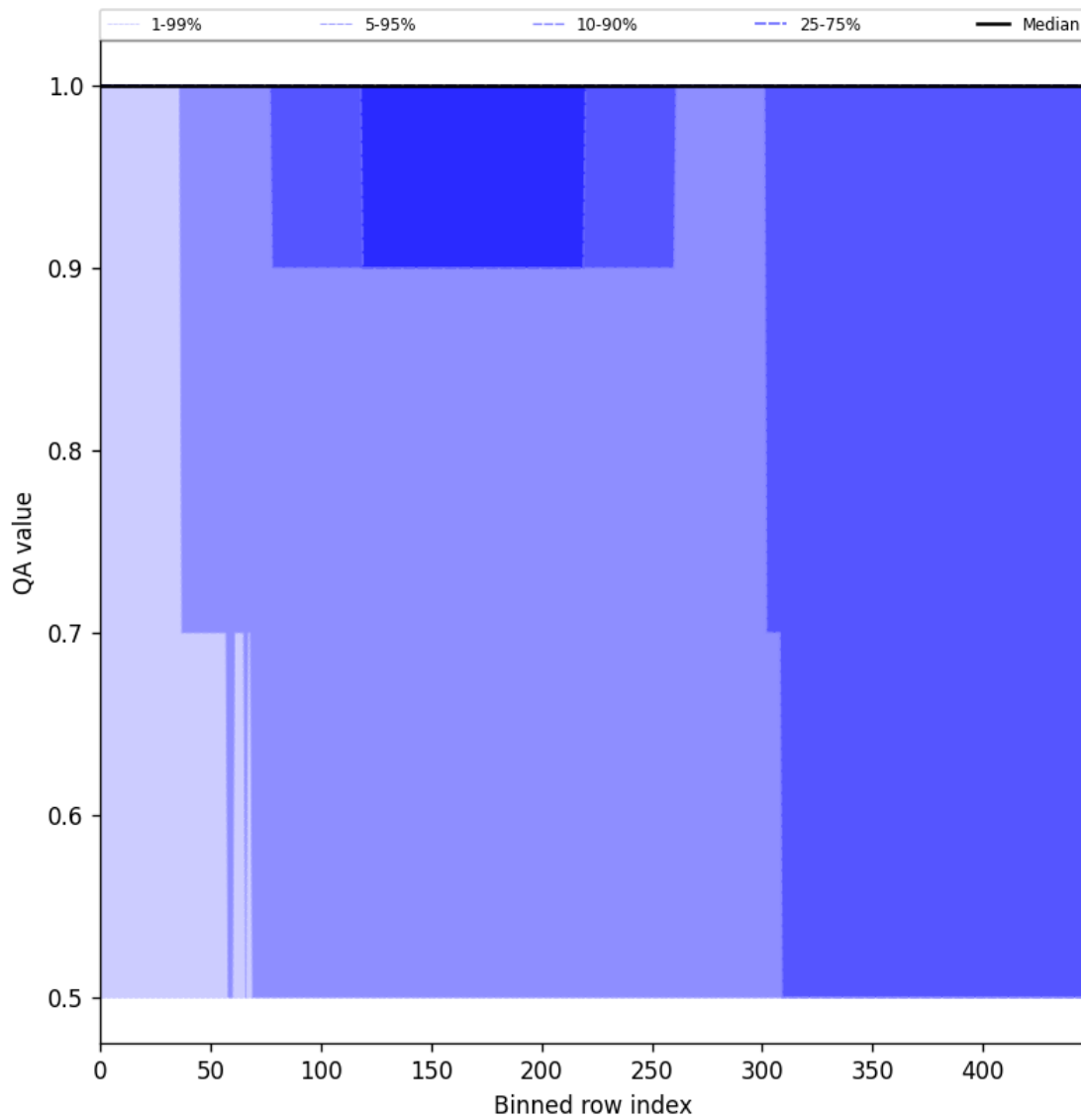
Figure 44: Along track statistics of “QA value” for 2025-05-28 to 2025-05-29
