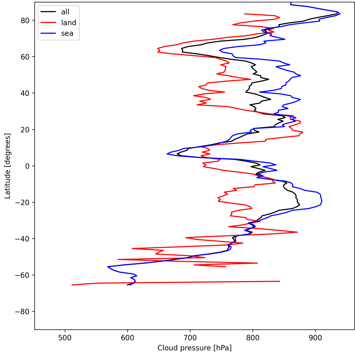
Figure 11: Zonal average of “Cloud pressure” for 2025-05-28 to 2025-05-29.
