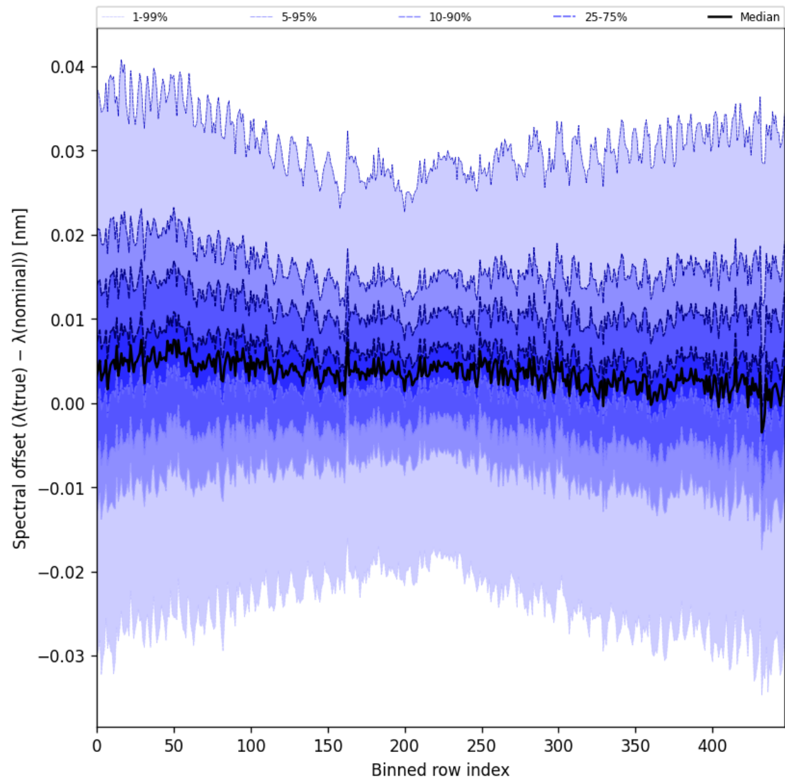
Figure 60: Along track statistics of “Spectral offset ( \lambda_{\text{true}} - \lambda_{\text{nominal}} )” for 2025-05-28 to 2025-05-29
