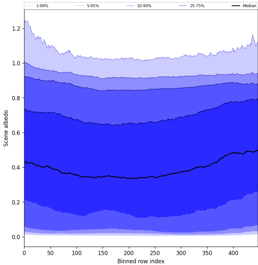
Figure 49: Along track statistics of “Scene albedo” for 2025-05-28 to 2025-05-29
