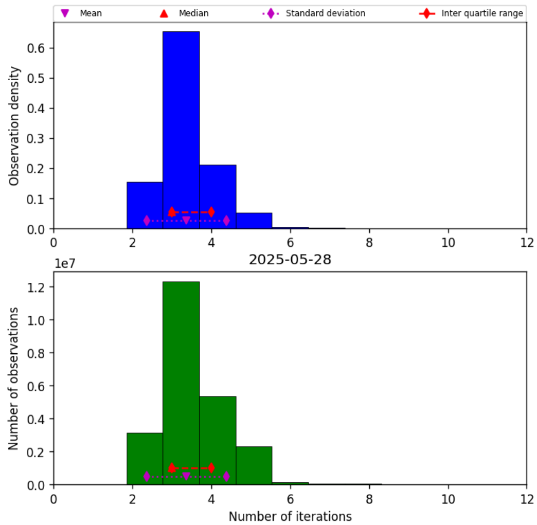
Figure 37: Histogram of “Number of iterations” for 2025-05-28 to 2025-05-29
