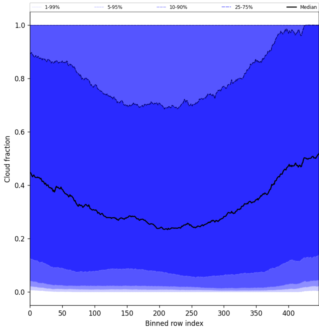
Figure 47: Along track statistics of “Cloud fraction” for 2025-05-28 to 2025-05-29
