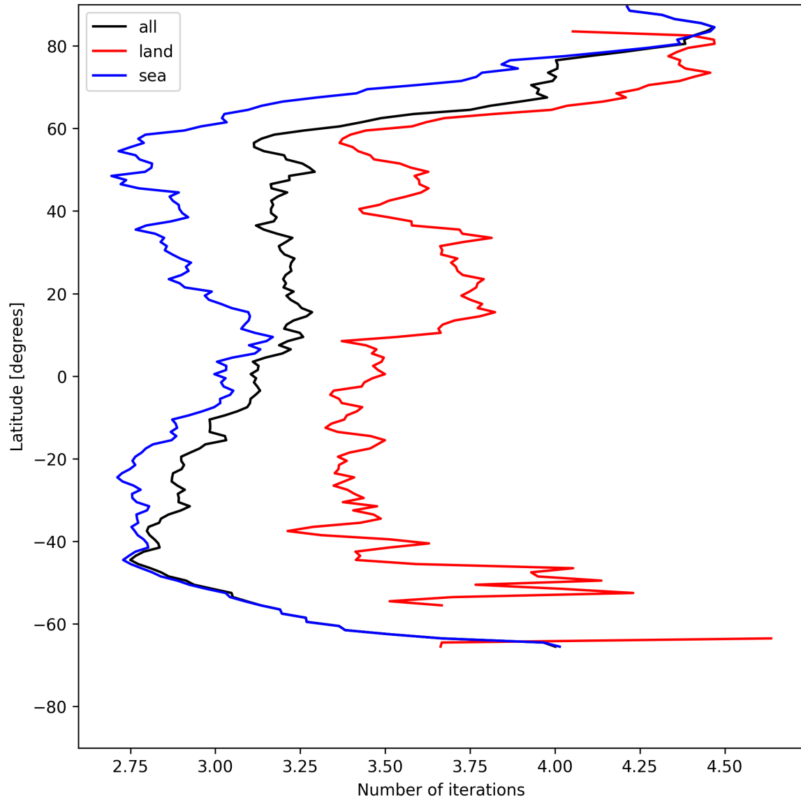
Figure 20: Zonal average of “Number of iterations” for 2025-05-28 to 2025-05-29.
