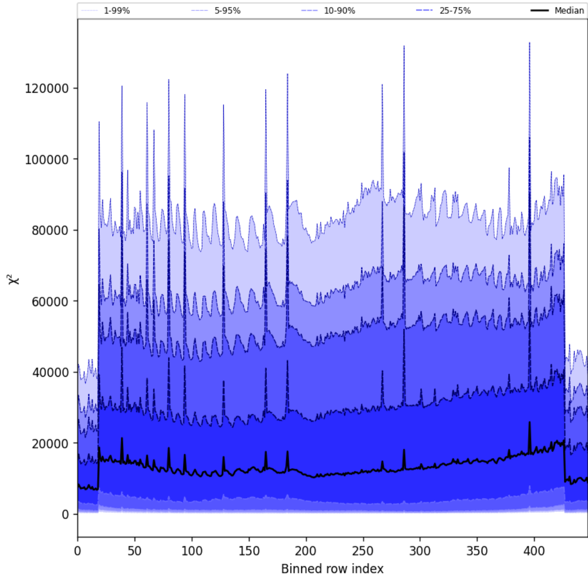
Figure 53: Along track statistics of “ \chi^2 ” for 2025-05-28 to 2025-05-29
