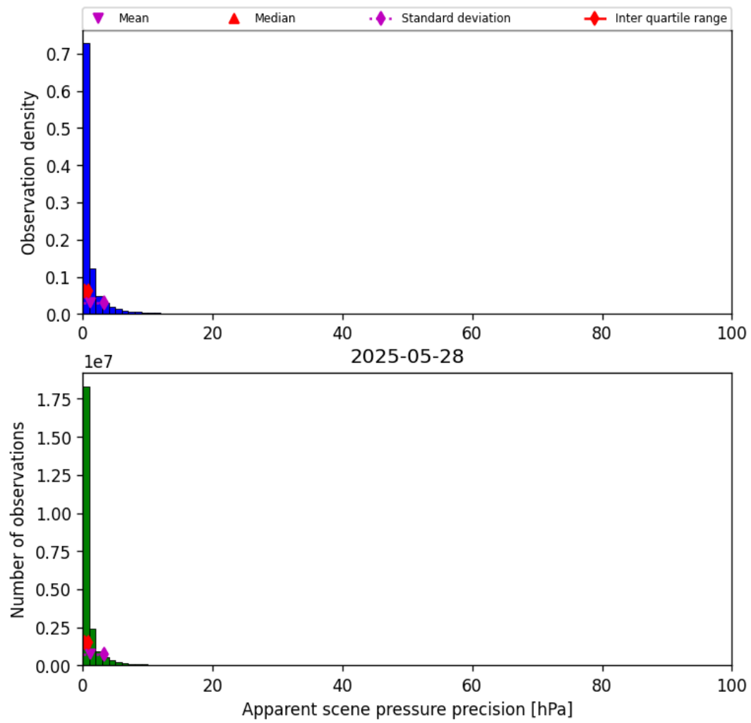
Figure 35: Histogram of “Apparent scene pressure precision” for 2025-05-28 to 2025-05-29
