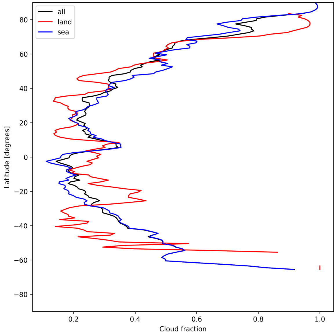
Figure 13: Zonal average of “Cloud fraction” for 2025-05-28 to 2025-05-29.
