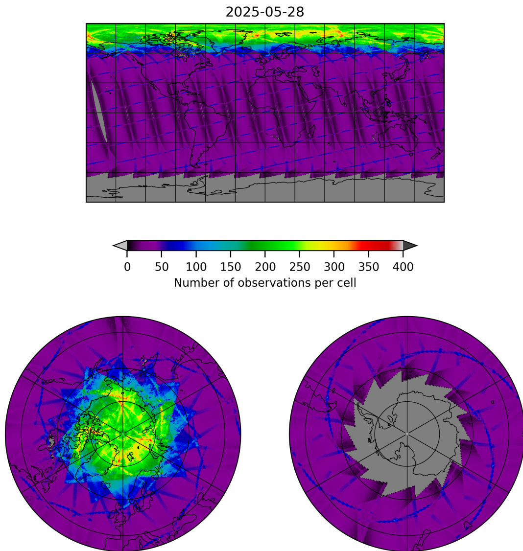
Figure 9: Map of the number of observations for 2025-05-28 to 2025-05-29
