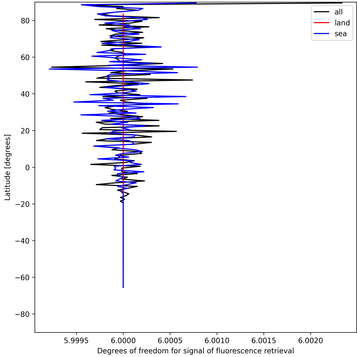
Figure 24: Zonal average of “Degrees of freedom for signal of fluorescence retrieval” for 2025-05-28 to 2025-05-29.
