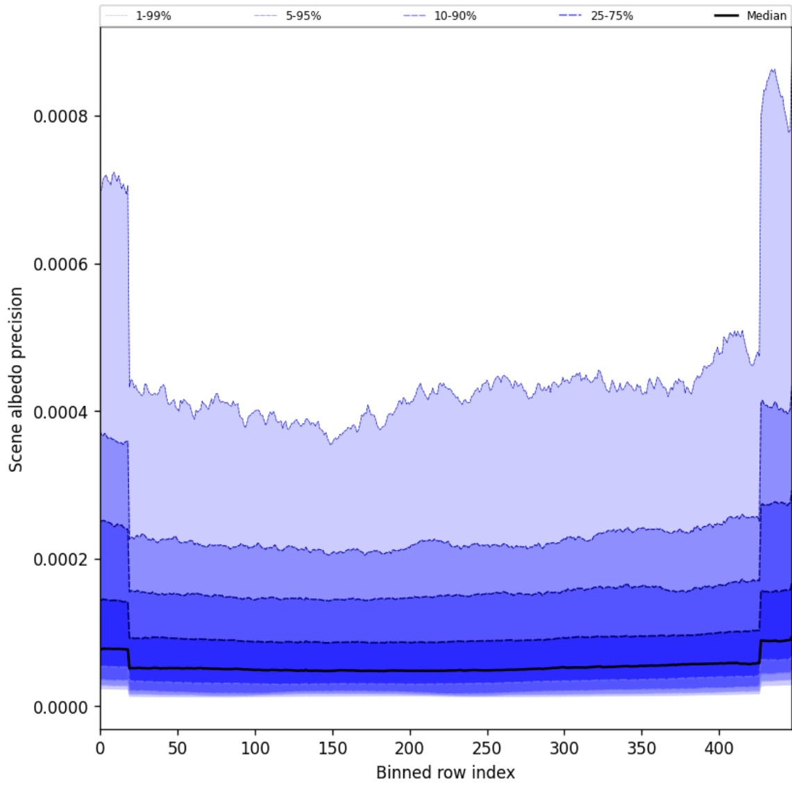
Figure 50: Along track statistics of “Scene albedo precision” for 2025-05-28 to 2025-05-29
