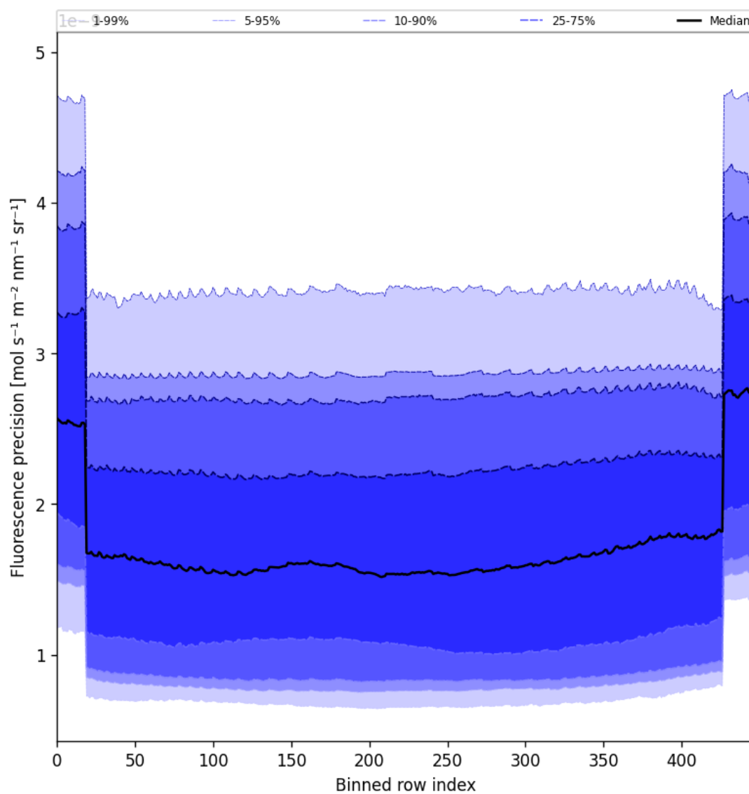
Figure 56: Along track statistics of “Fluorescence precision” for 2025-05-28 to 2025-05-29
