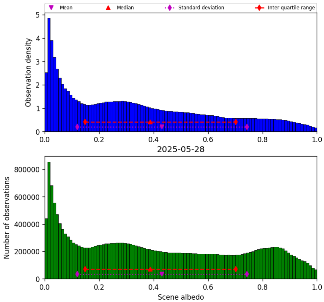
Figure 32: Histogram of “Scene albedo” for 2025-05-28 to 2025-05-29
