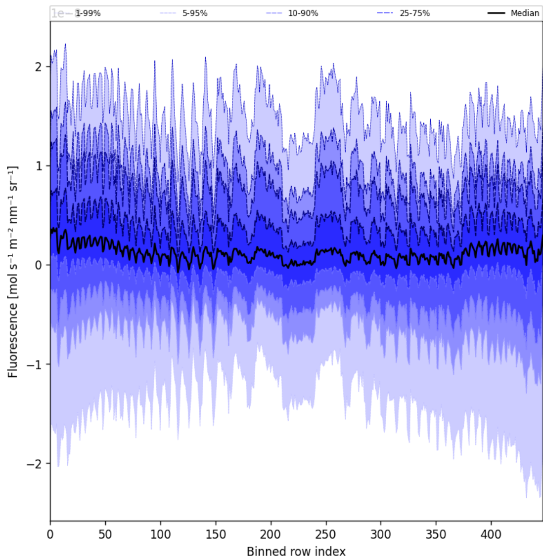
Figure 55: Along track statistics of “Fluorescence” for 2025-05-28 to 2025-05-29
