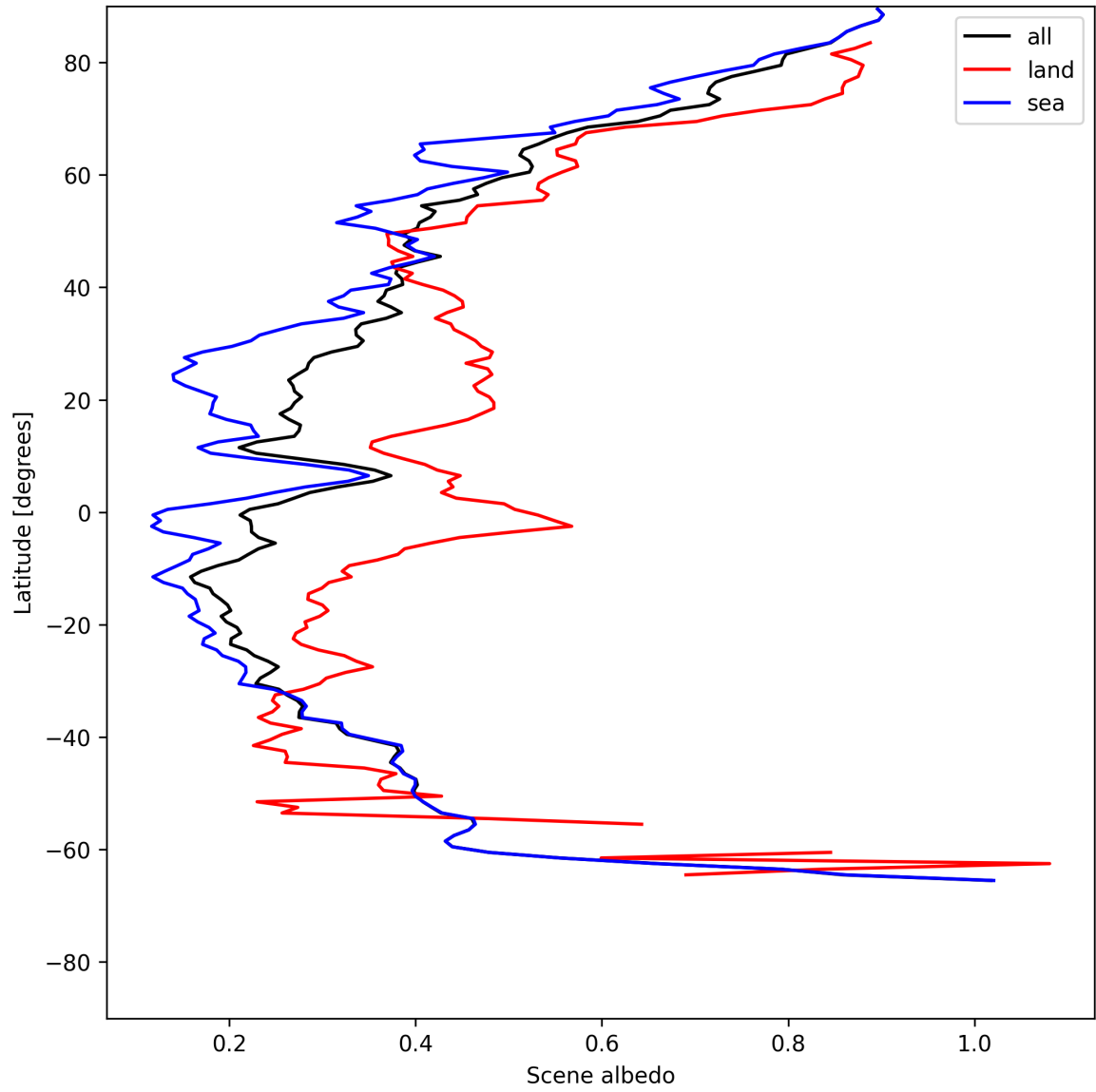
Figure 15: Zonal average of "Scene albedo" for 2025-05-31 to 2025-06-01.
