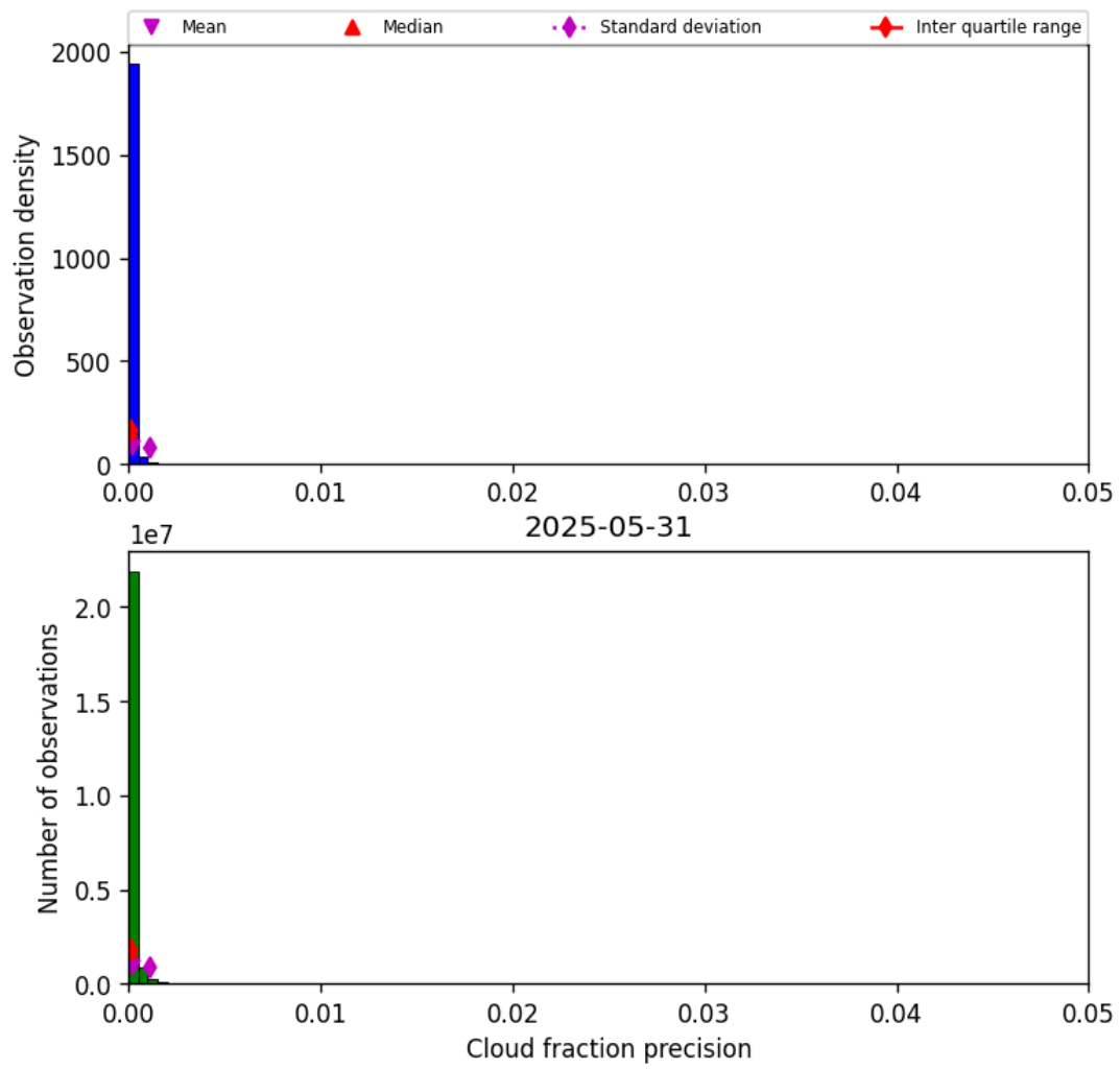
Figure 31: Histogram of “Cloud fraction precision” for 2025-05-31 to 2025-06-01
