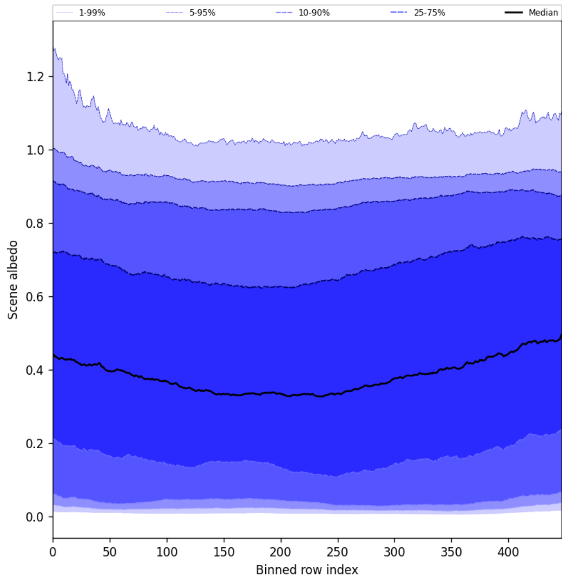
Figure 49: Along track statistics of “Scene albedo” for 2025-05-31 to 2025-06-01
