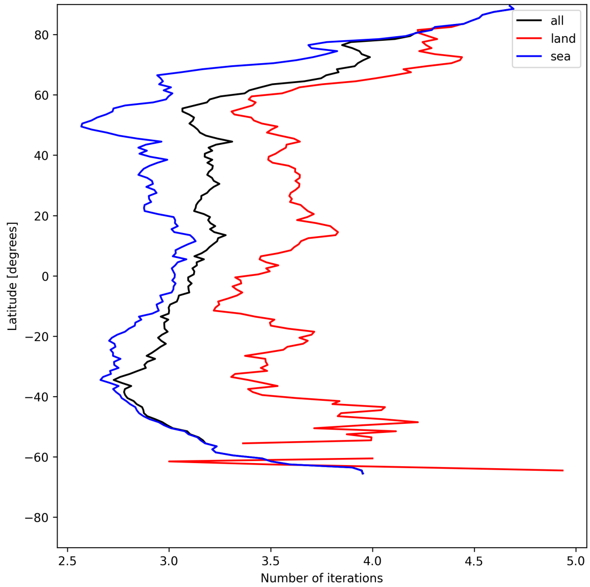
Figure 20: Zonal average of “Number of iterations” for 2025-05-31 to 2025-06-01.
