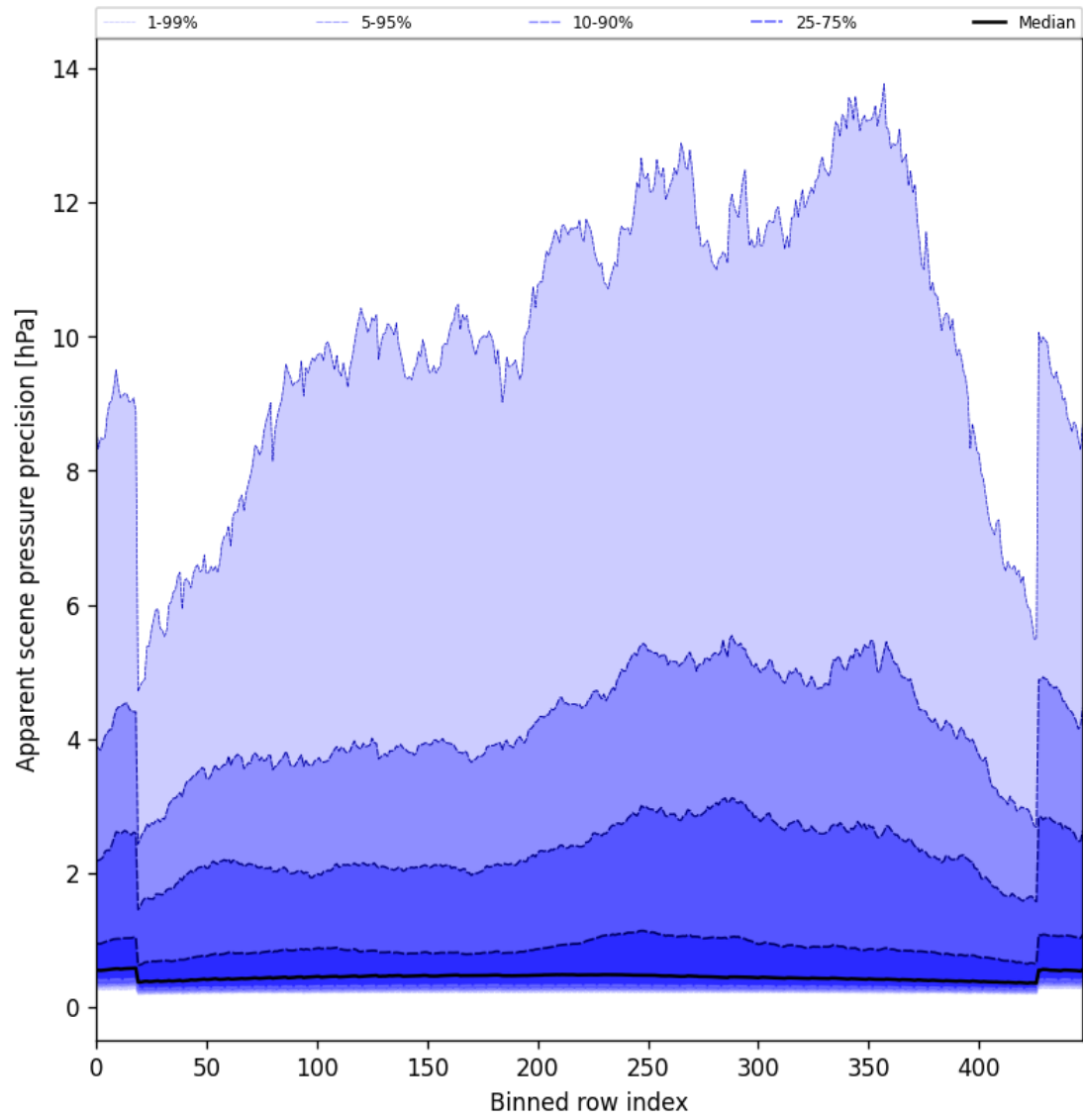
Figure 52: Along track statistics of “Apparent scene pressure precision” for 2025-05-31 to 2025-06-01
