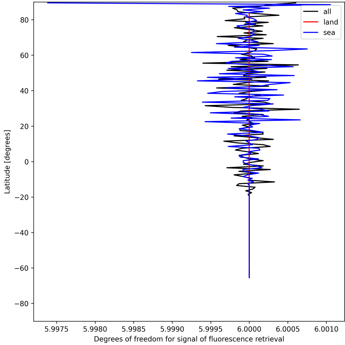
Figure 24: Zonal average of “Degrees of freedom for signal of fluorescence retrieval” for 2025-05-31 to 2025-06-01.
