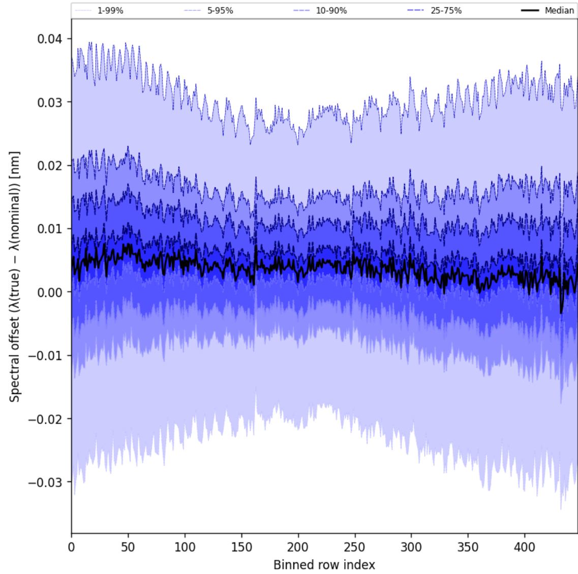
Figure 60: Along track statistics of “Spectral offset ( \lambda_{\text{true}} - \lambda_{\text{nominal}} )” for 2025-05-31 to 2025-06-01
