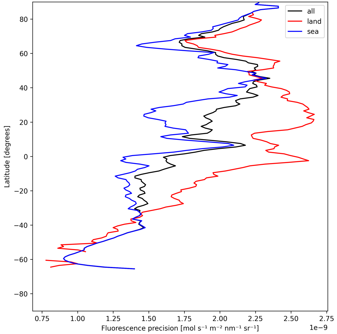
Figure 22: Zonal average of “Fluorescence precision” for 2025-05-31 to 2025-06-01.
