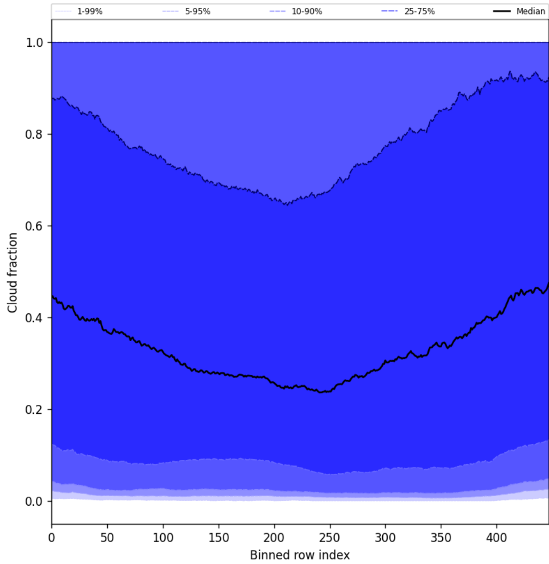
Figure 47: Along track statistics of “Cloud fraction” for 2025-05-31 to 2025-06-01
