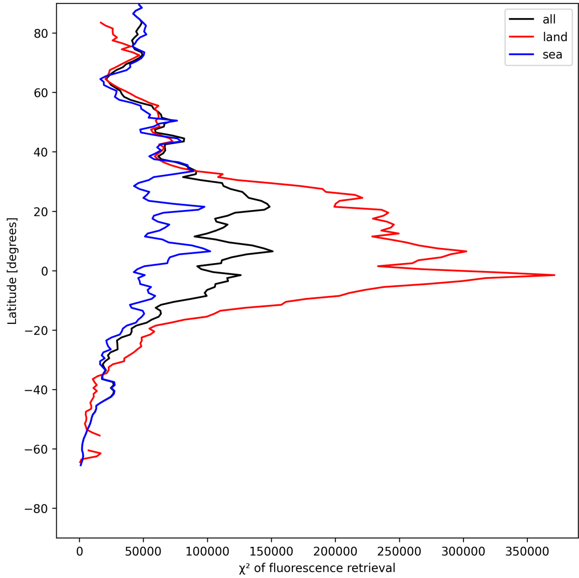
Figure 23: Zonal average of “ \chi^2 of fluorescence retrieval” for 2025-05-31 to 2025-06-01.
