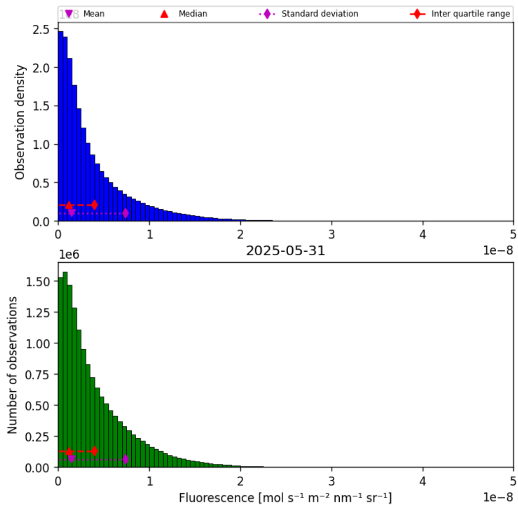
Figure 38: Histogram of “Fluorescence” for 2025-05-31 to 2025-06-01
