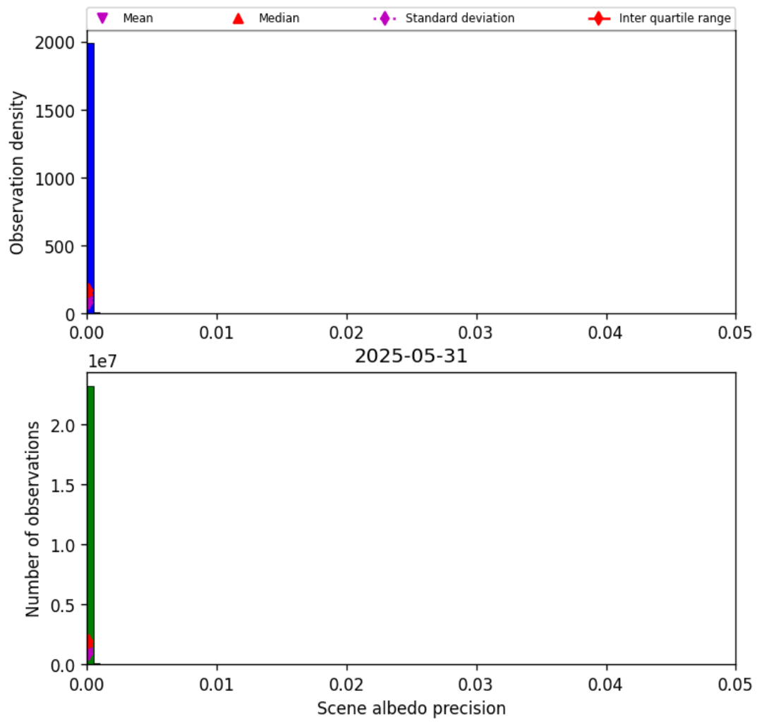
Figure 33: Histogram of “Scene albedo precision” for 2025-05-31 to 2025-06-01
