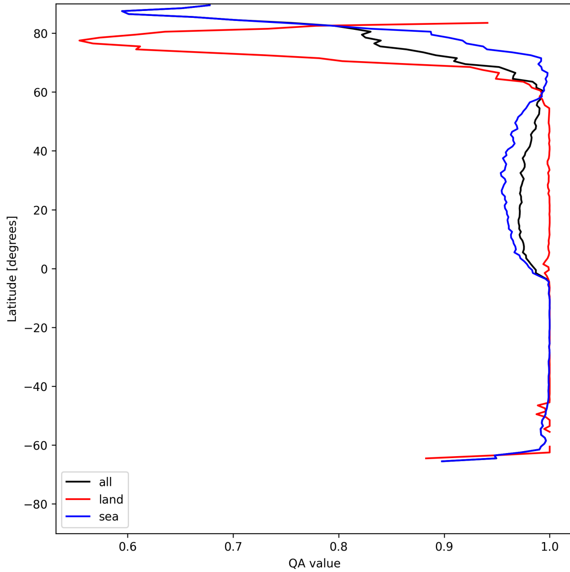
Figure 10: Zonal average of “QA value” for 2025-05-31 to 2025-06-01.
