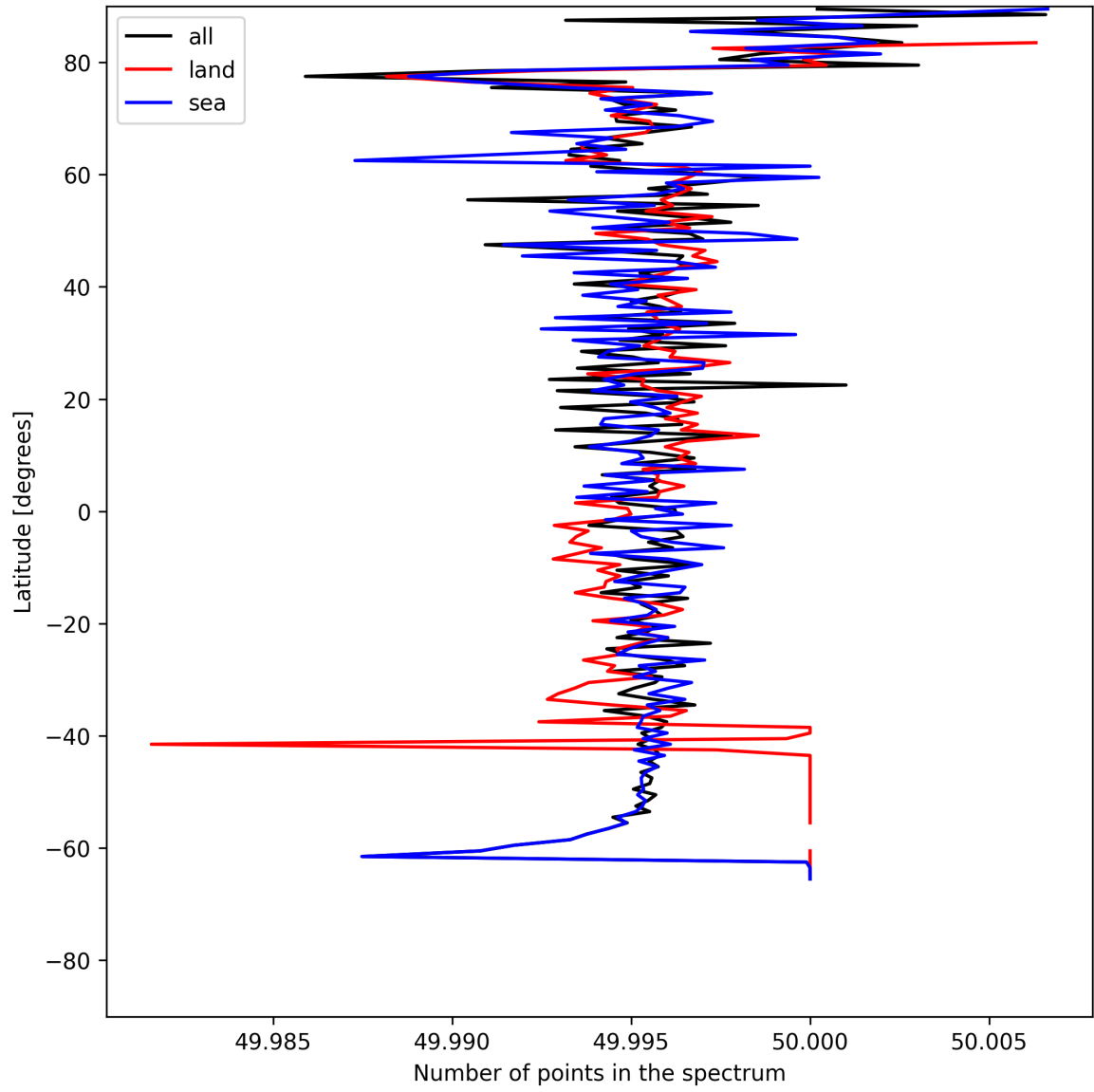
Figure 25: Zonal average of “Number of points in the spectrum” for 2025-05-31 to 2025-06-01.
