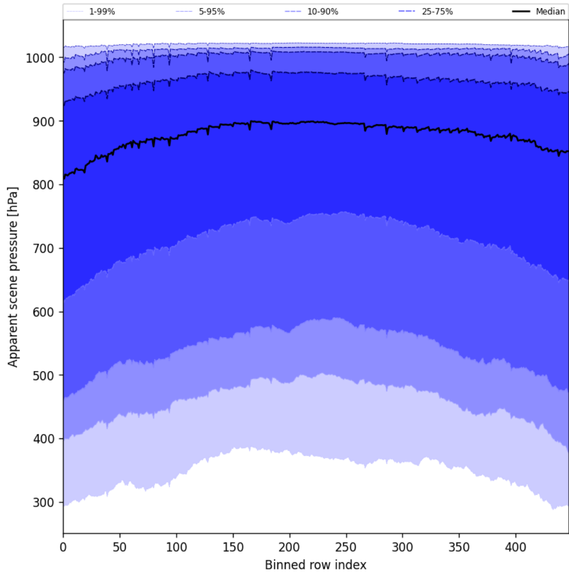
Figure 51: Along track statistics of “Apparent scene pressure” for 2025-05-31 to 2025-06-01
