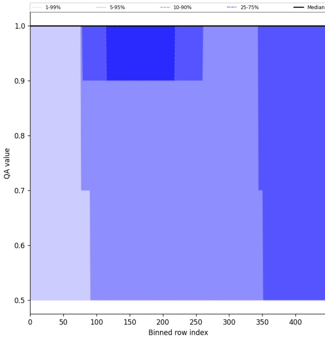
Figure 44: Along track statistics of “QA value” for 2025-05-31 to 2025-06-01
