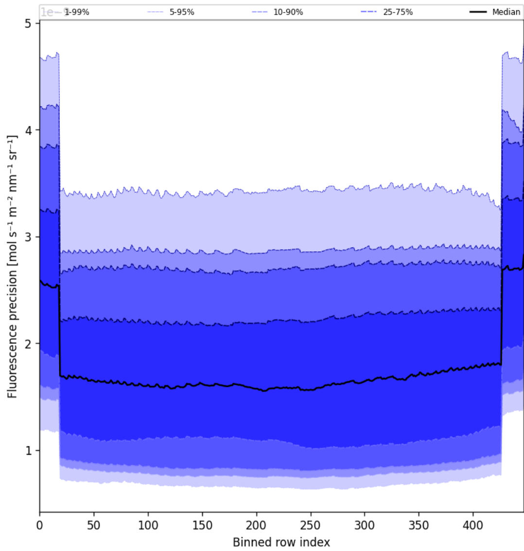
Figure 56: Along track statistics of “Fluorescence precision” for 2025-05-31 to 2025-06-01
