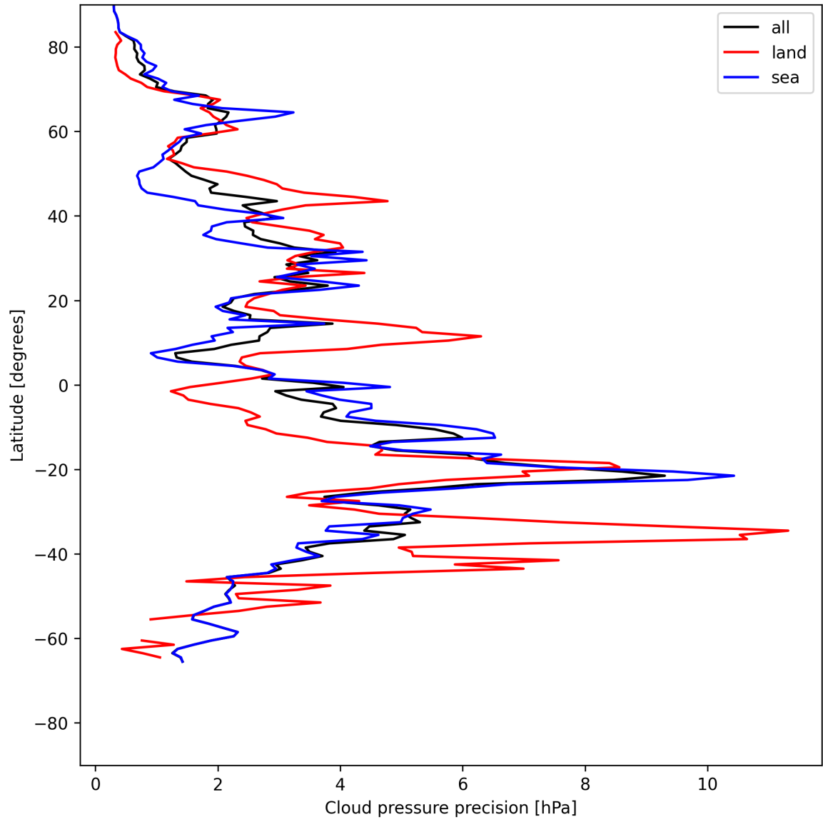
Figure 12: Zonal average of “Cloud pressure precision” for 2025-05-31 to 2025-06-01.
