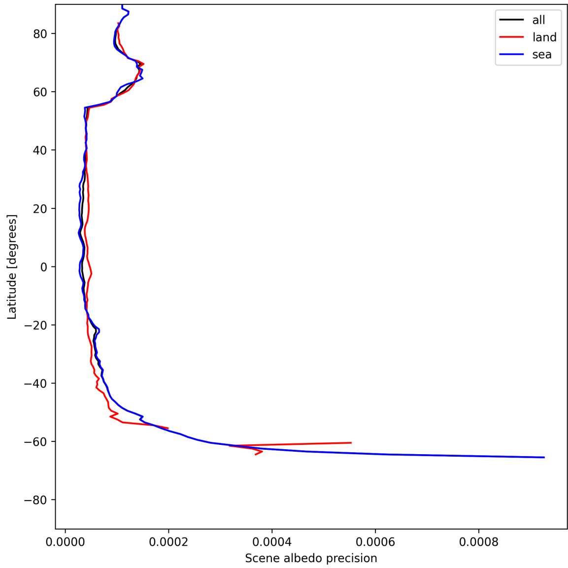
Figure 16: Zonal average of “Scene albedo precision” for 2025-05-31 to 2025-06-01.
