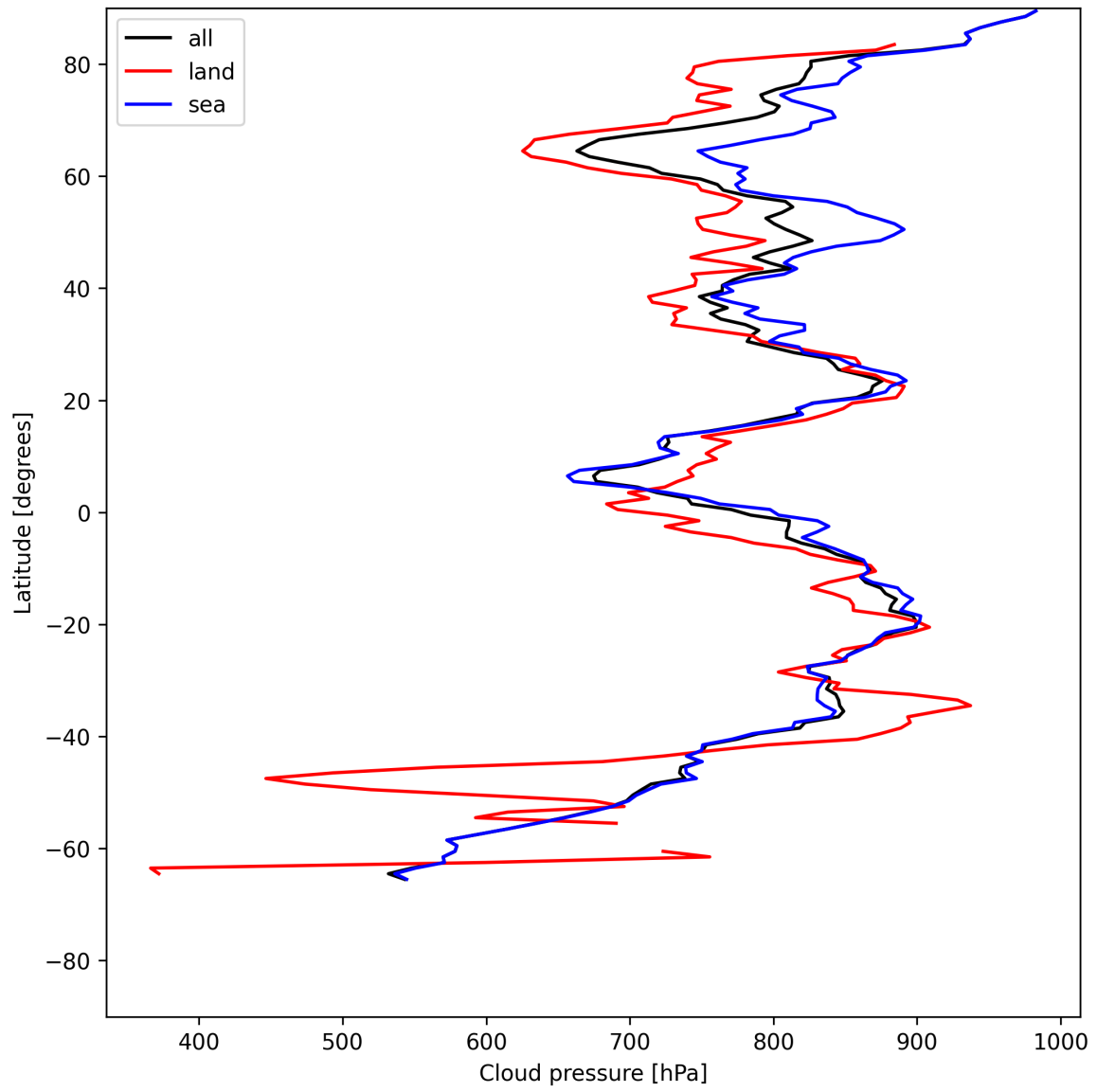
Figure 11: Zonal average of “Cloud pressure” for 2025-05-31 to 2025-06-01.
