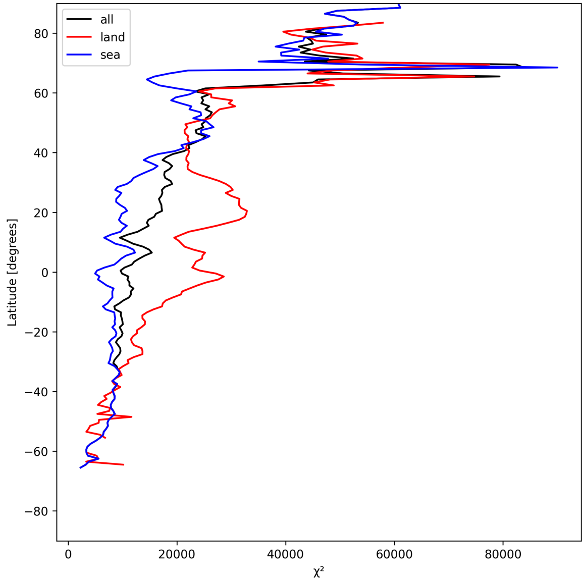
Figure 19: Zonal average of “ \chi^2 ” for 2025-05-31 to 2025-06-01.
