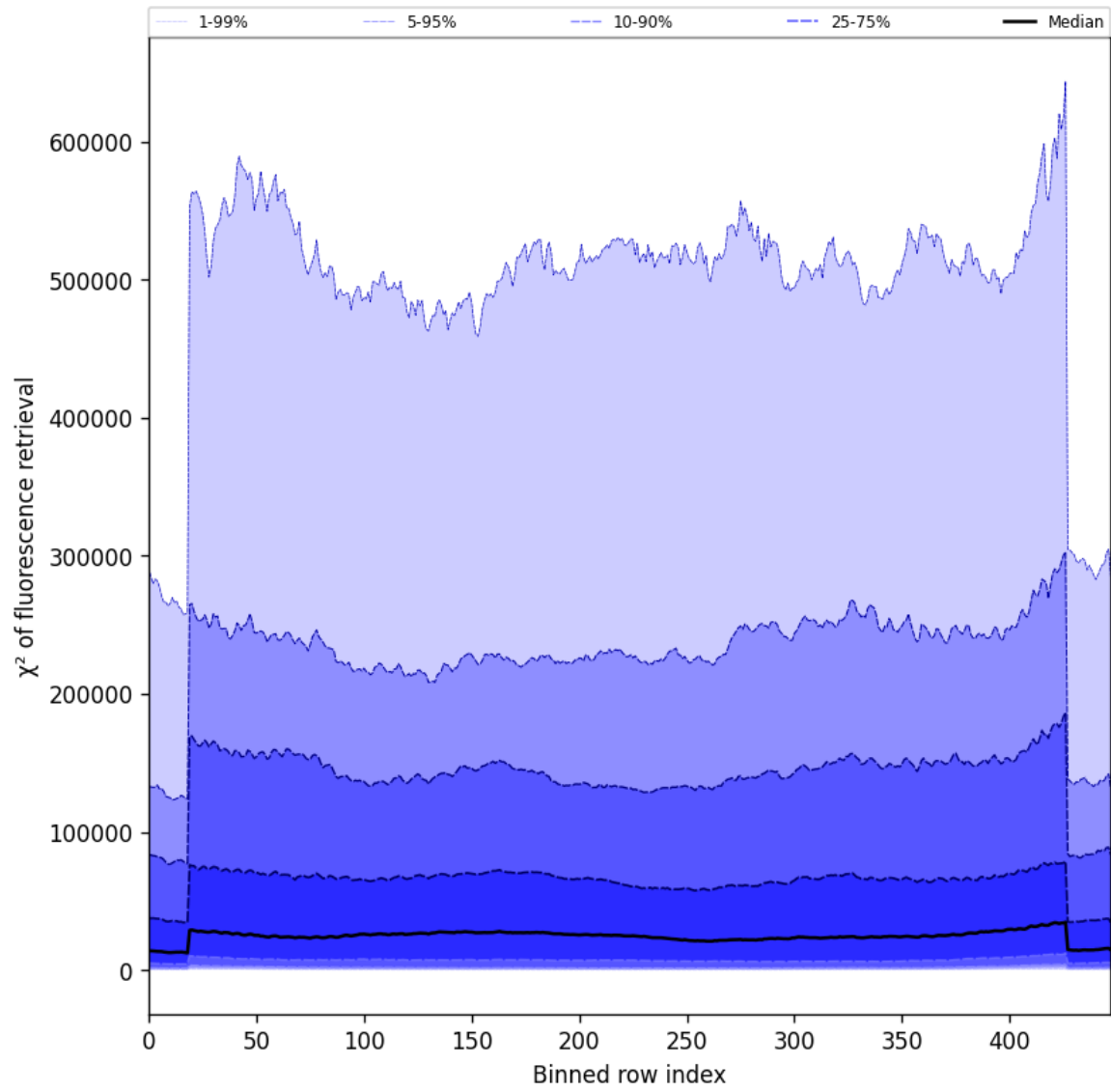
Figure 57: Along track statistics of “ \chi^2 of fluorescence retrieval” for 2025-05-31 to 2025-06-01
