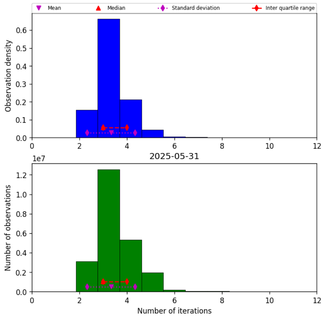
Figure 37: Histogram of “Number of iterations” for 2025-05-31 to 2025-06-01
