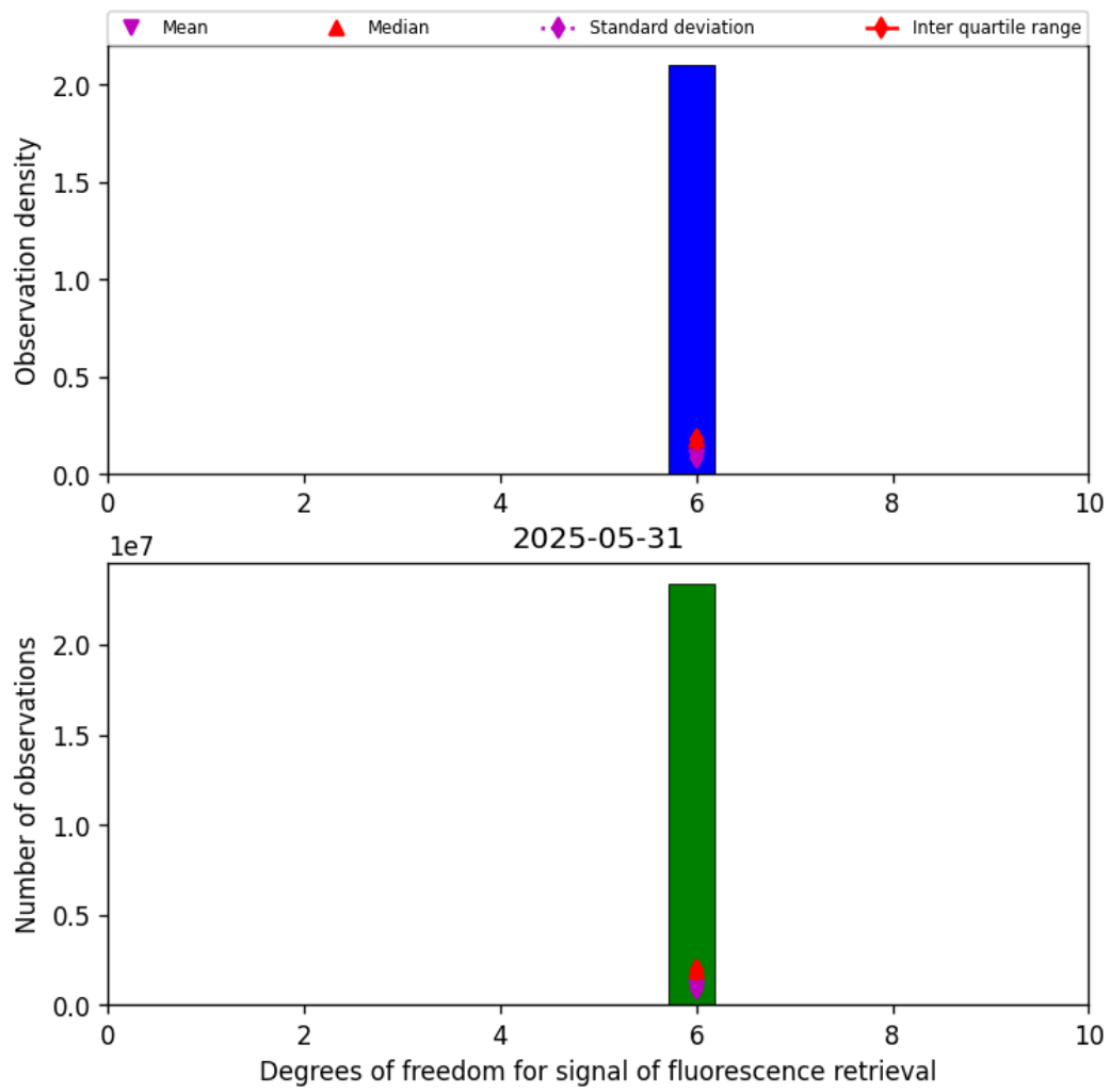
Figure 41: Histogram of “Degrees of freedom for signal of fluorescence retrieval” for 2025-05-31 to 2025-06-01
