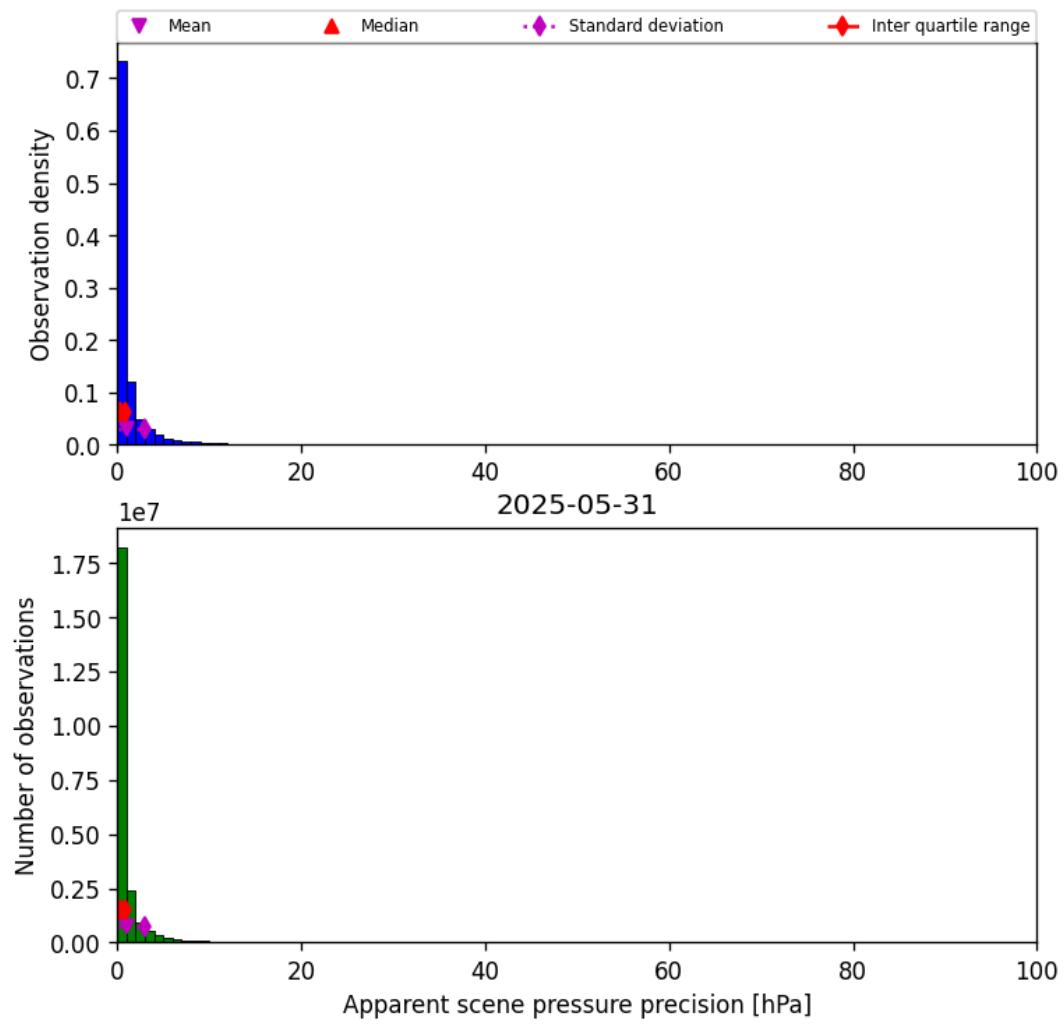
Figure 35: Histogram of “Apparent scene pressure precision” for 2025-05-31 to 2025-06-01
