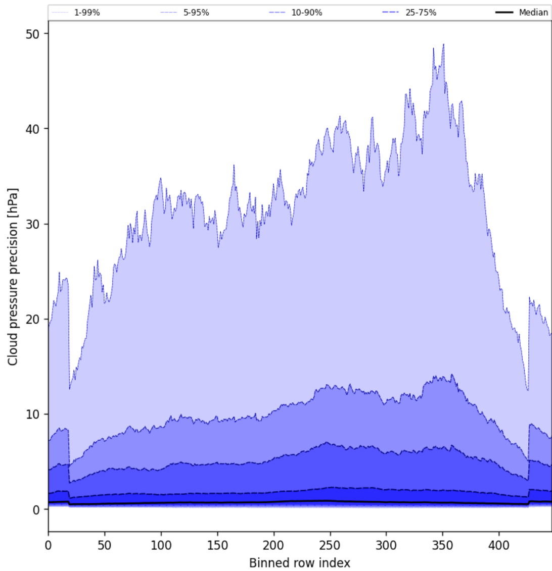
Figure 46: Along track statistics of “Cloud pressure precision” for 2025-05-31 to 2025-06-01
