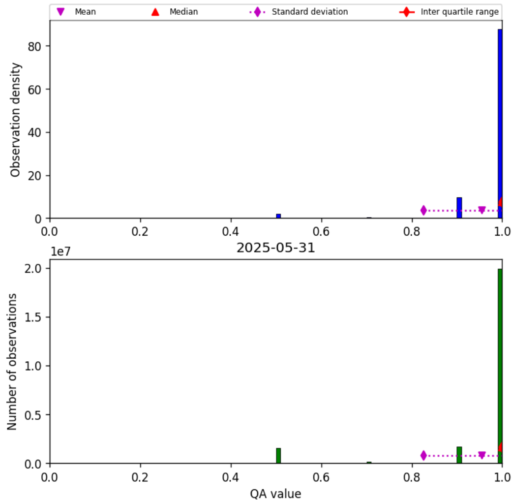
Figure 27: Histogram of “QA value” for 2025-05-31 to 2025-06-01
