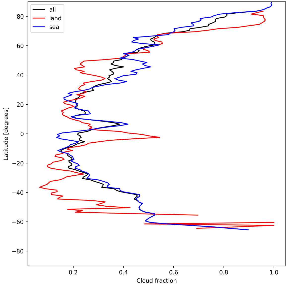
Figure 13: Zonal average of “Cloud fraction” for 2025-05-31 to 2025-06-01.
