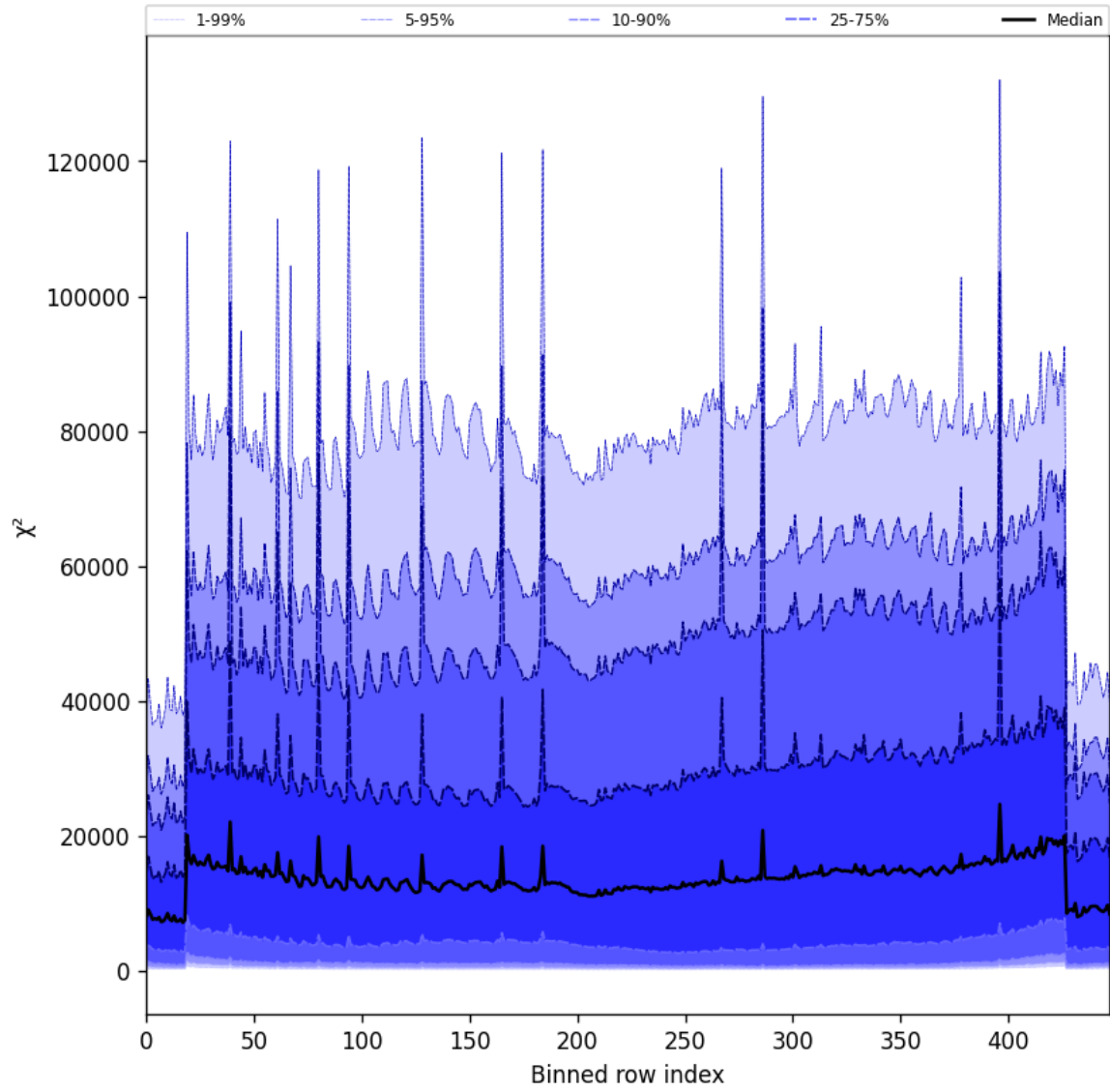
Figure 53: Along track statistics of “ \chi^2 ” for 2025-05-31 to 2025-06-01
