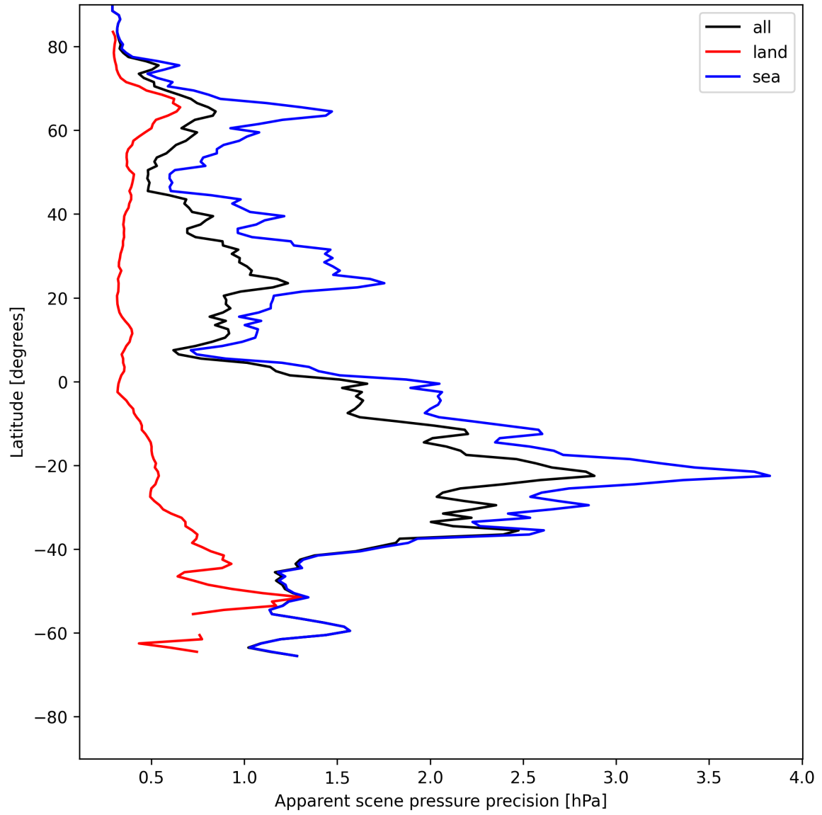
Figure 18: Zonal average of “Apparent scene pressure precision” for 2025-05-31 to 2025-06-01.
