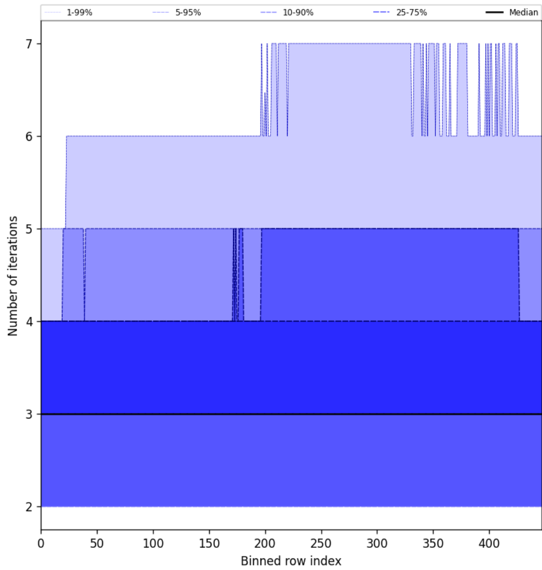
Figure 54: Along track statistics of “Number of iterations” for 2025-05-31 to 2025-06-01
