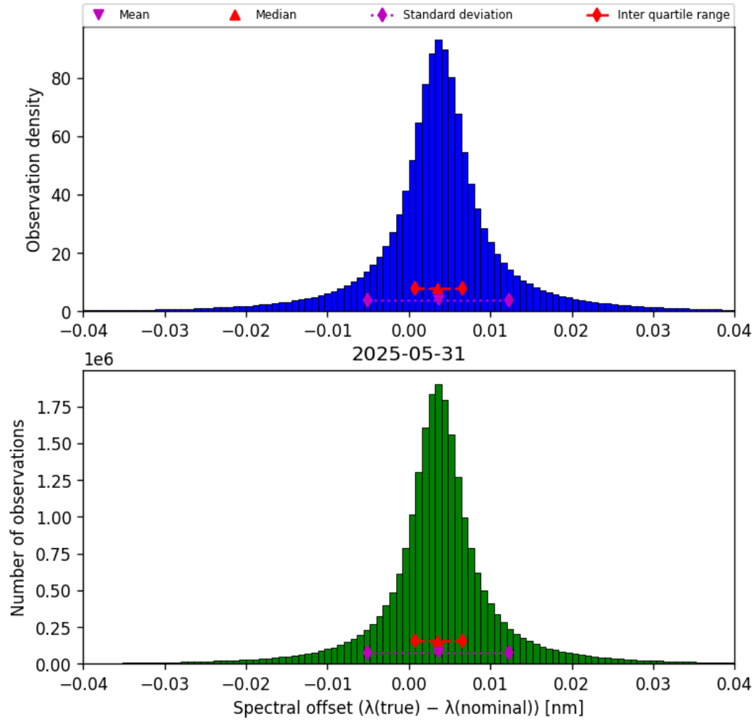
Figure 43: Histogram of “Spectral offset ( \lambda_{\text{true}} - \lambda_{\text{nominal}} )” for 2025-05-31 to 2025-06-01
