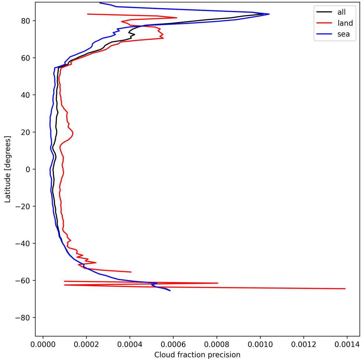
Figure 14: Zonal average of “Cloud fraction precision” for 2025-05-31 to 2025-06-01.
