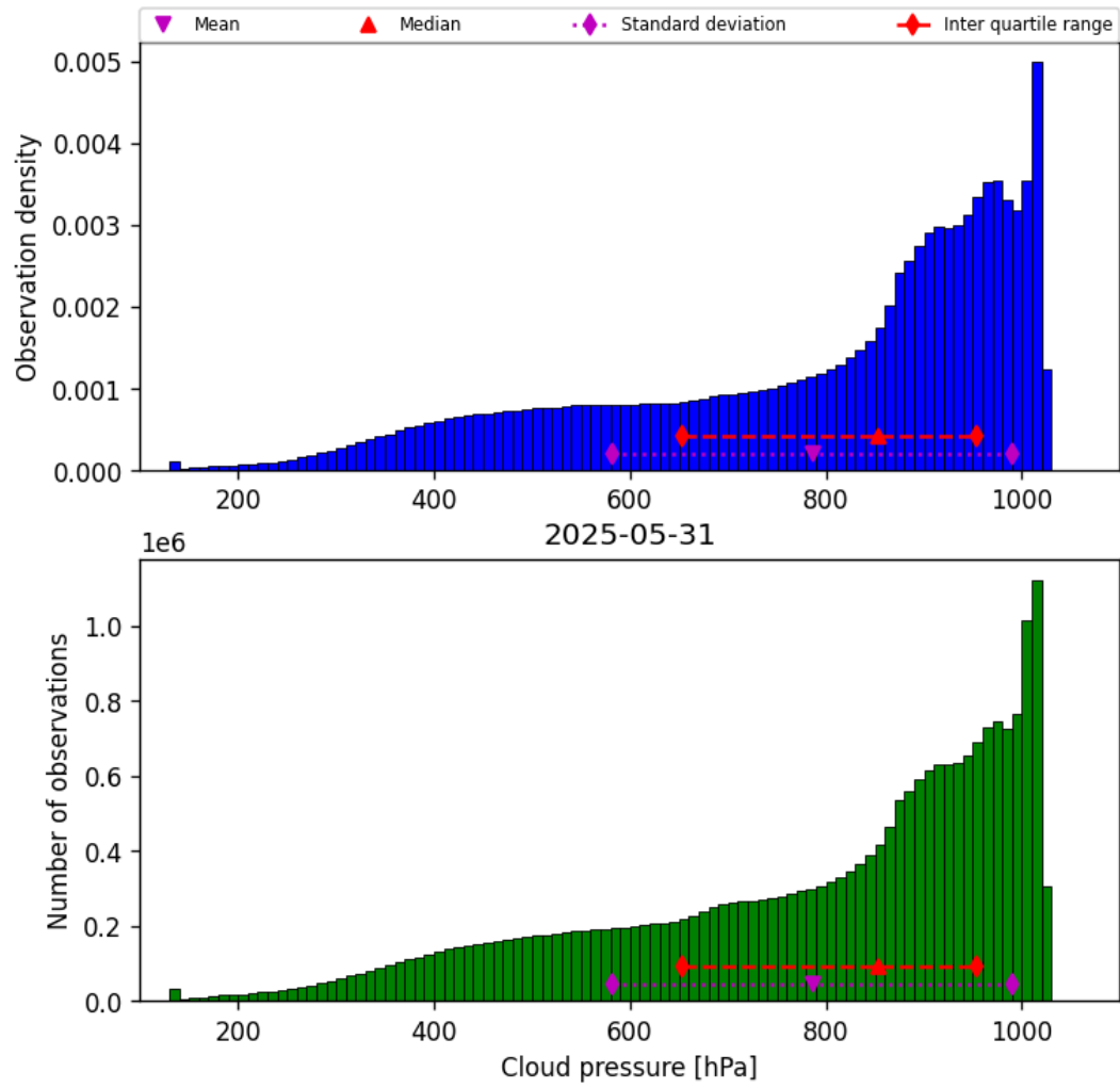
Figure 28: Histogram of “Cloud pressure” for 2025-05-31 to 2025-06-01
