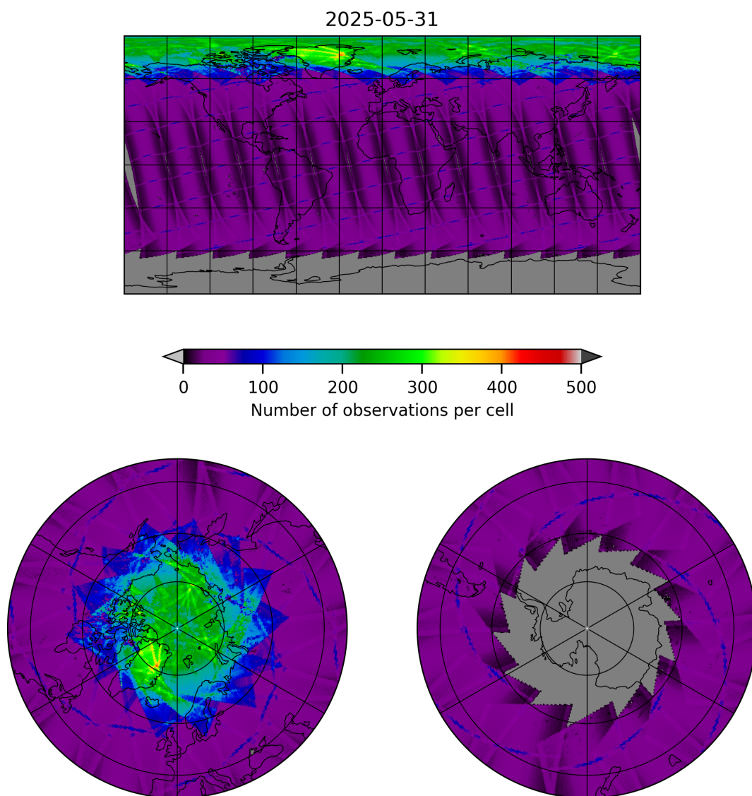
Figure 9: Map of the number of observations for 2025-05-31 to 2025-06-01
