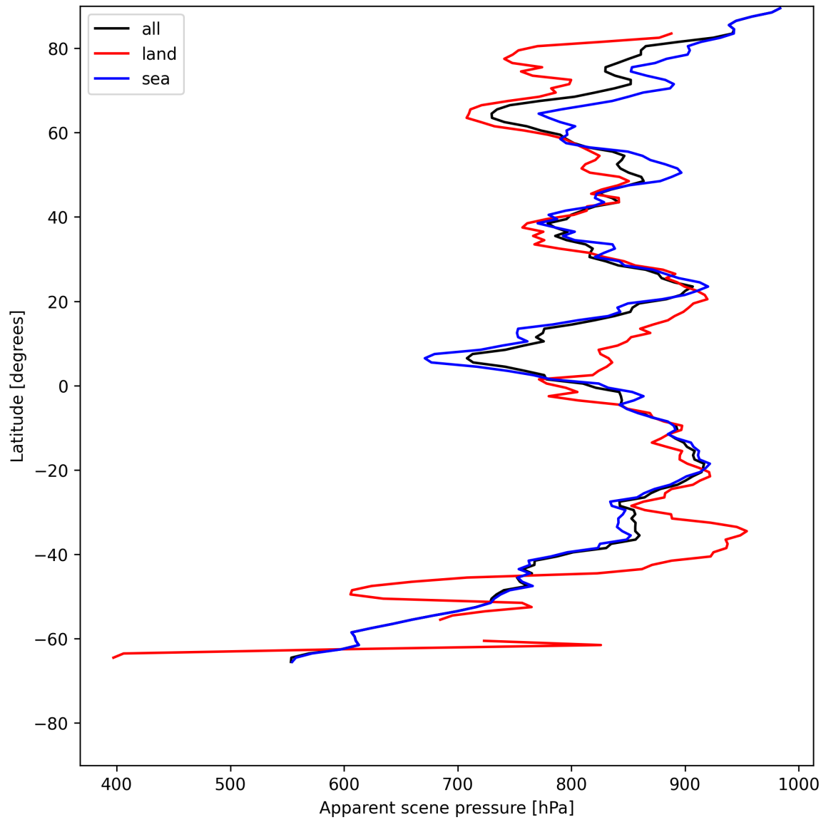
Figure 17: Zonal average of “Apparent scene pressure” for 2025-05-31 to 2025-06-01.
