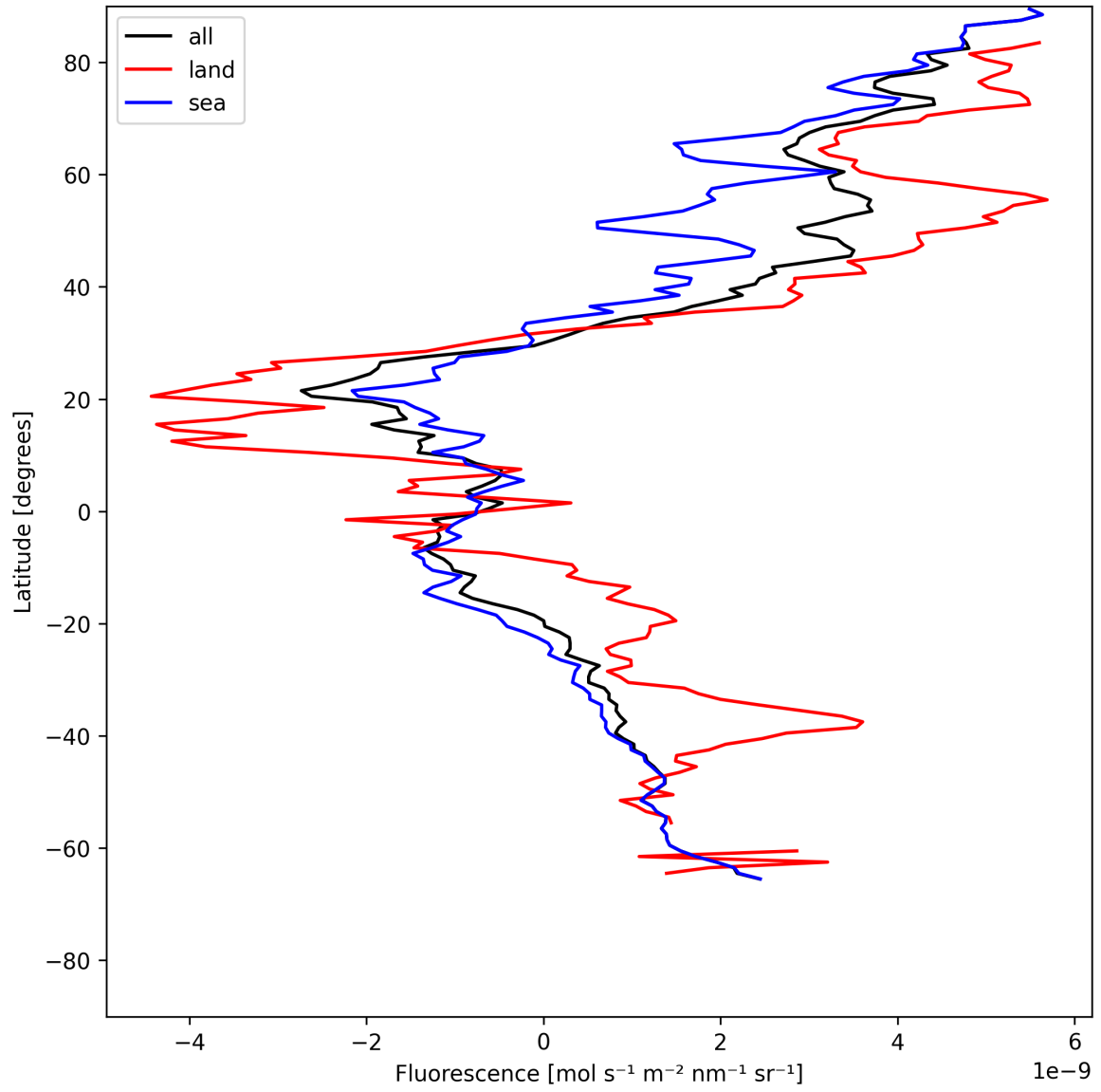
Figure 21: Zonal average of “Fluorescence” for 2025-05-31 to 2025-06-01.
