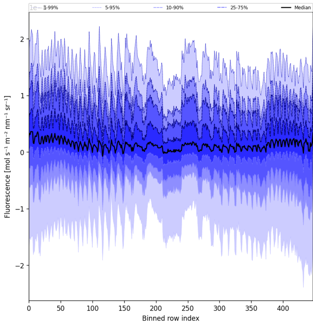
Figure 55: Along track statistics of “Fluorescence” for 2025-05-31 to 2025-06-01
