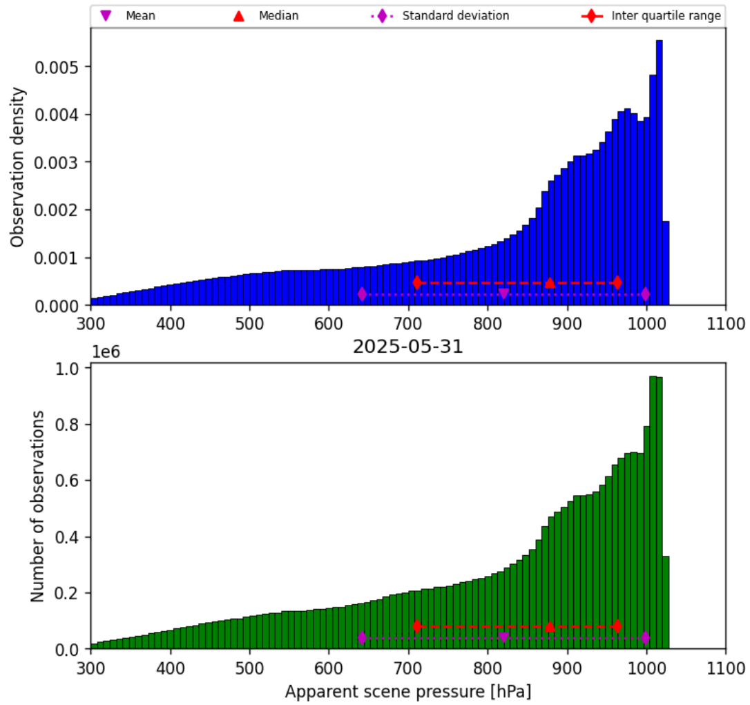
Figure 34: Histogram of “Apparent scene pressure” for 2025-05-31 to 2025-06-01
