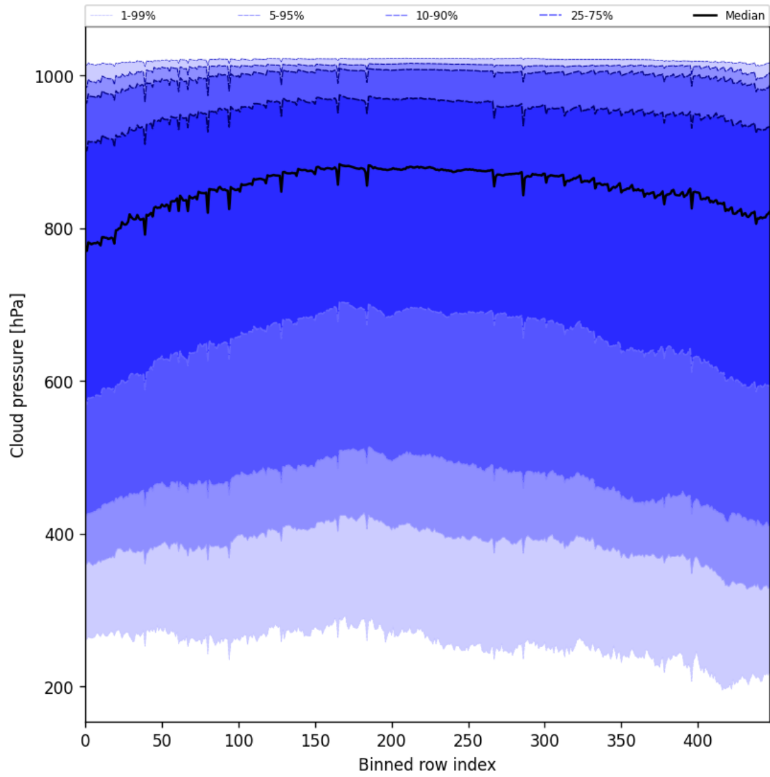
Figure 45: Along track statistics of “Cloud pressure” for 2025-05-31 to 2025-06-01
