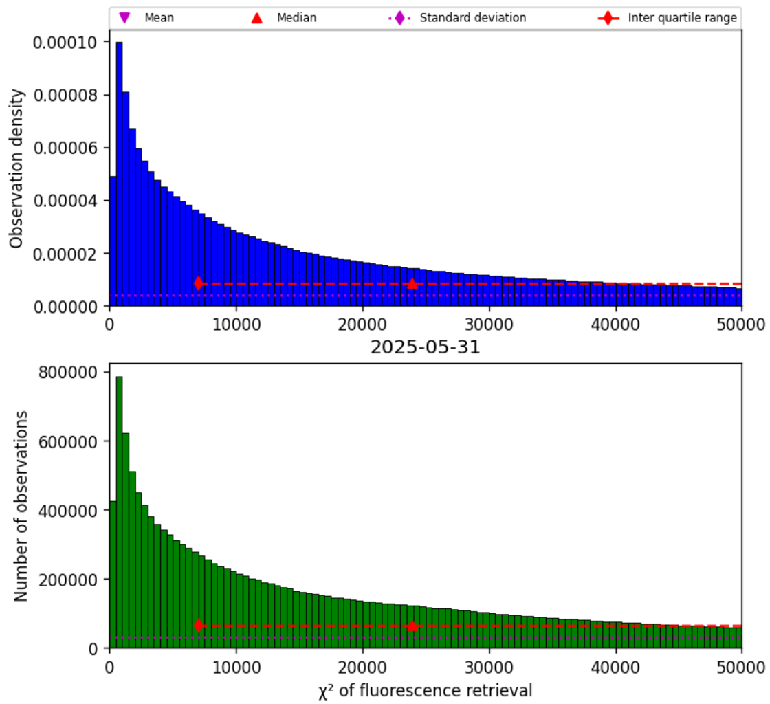
Figure 40: Histogram of “ \chi^2 of fluorescence retrieval” for 2025-05-31 to 2025-06-01
