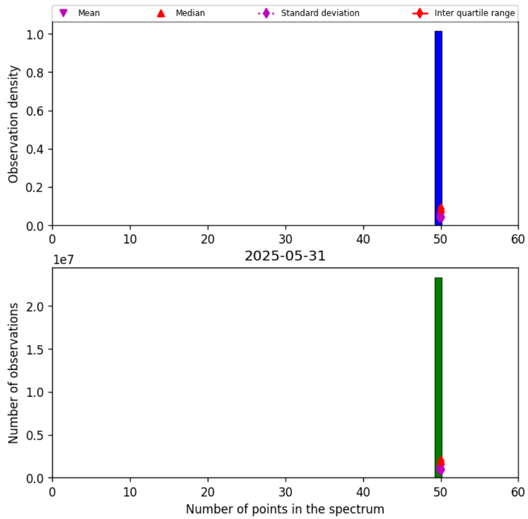
Figure 42: Histogram of "Number of points in the spectrum" for 2025-05-31 to 2025-06-01
