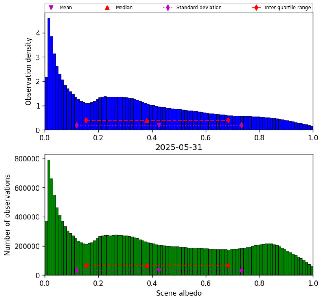
Figure 32: Histogram of “Scene albedo” for 2025-05-31 to 2025-06-01
