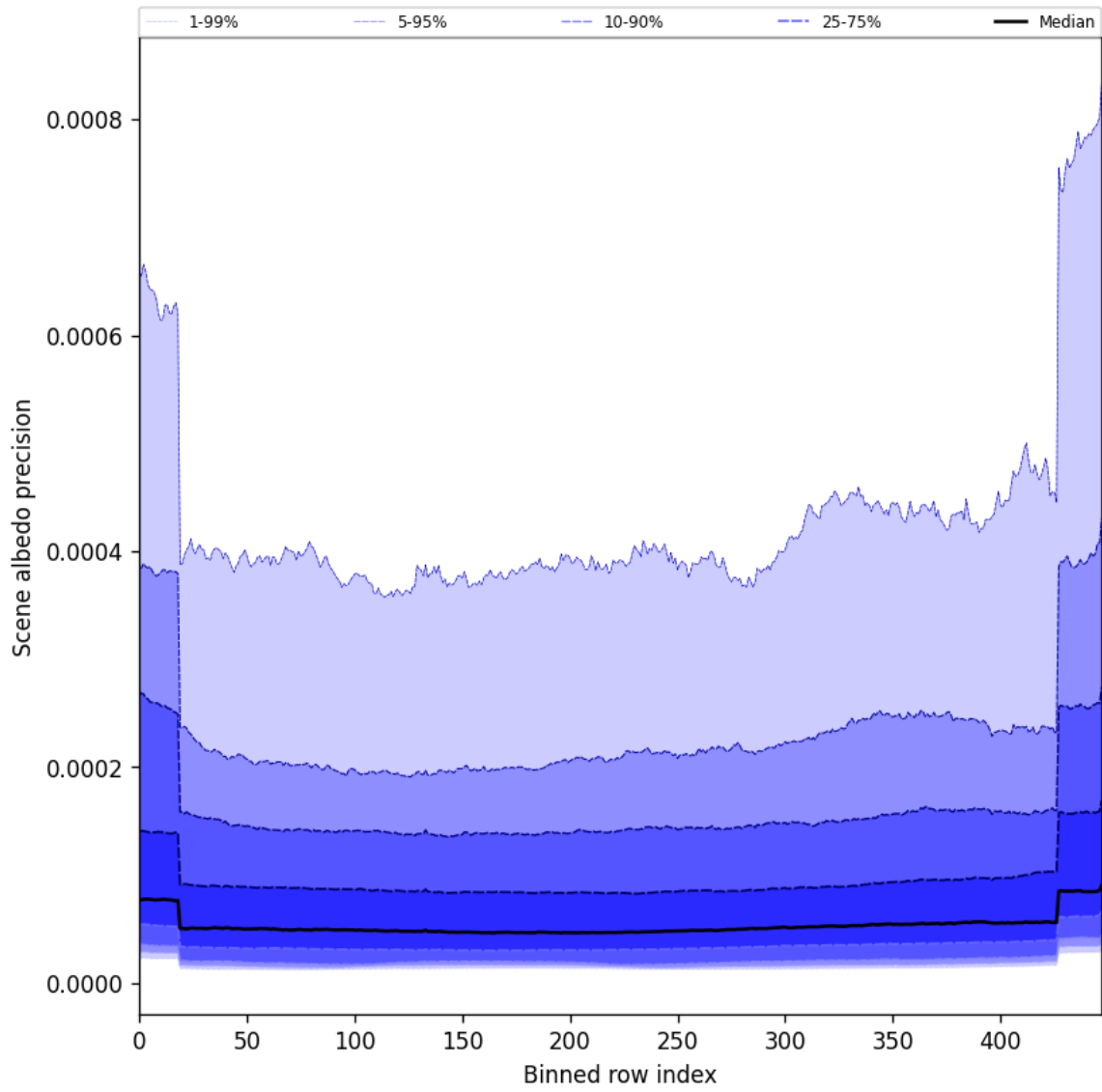
Figure 50: Along track statistics of “Scene albedo precision” for 2025-05-31 to 2025-06-01
