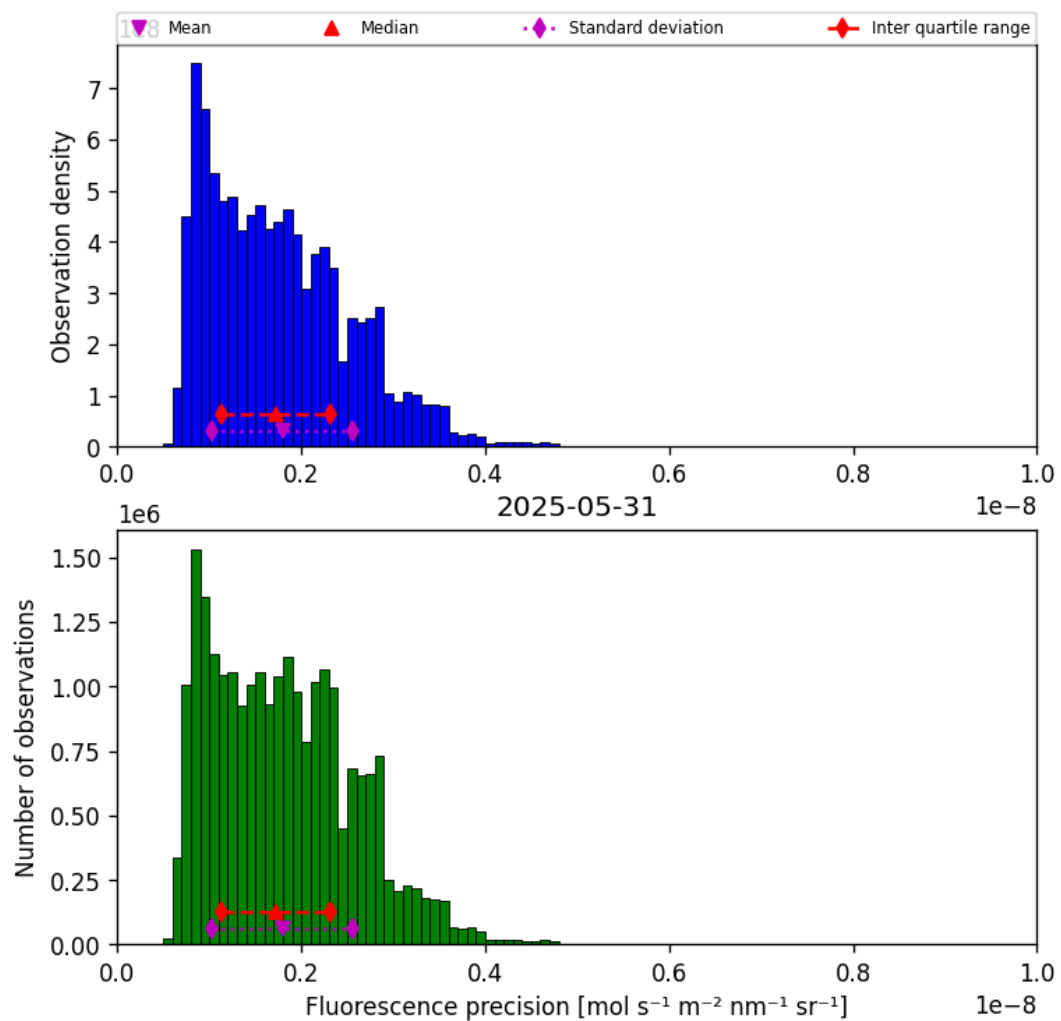
Figure 39: Histogram of “Fluorescence precision” for 2025-05-31 to 2025-06-01
