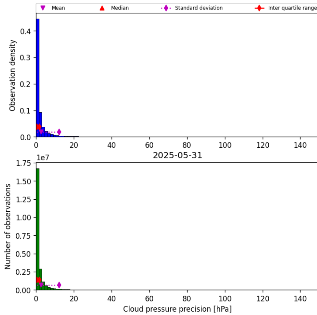
Figure 29: Histogram of “Cloud pressure precision” for 2025-05-31 to 2025-06-01
