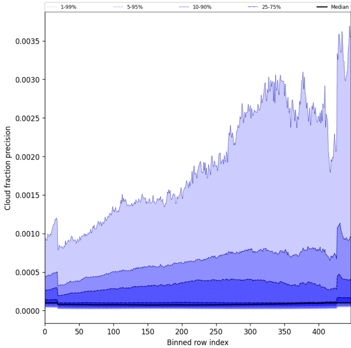
Figure 48: Along track statistics of “Cloud fraction precision” for 2025-05-31 to 2025-06-01
