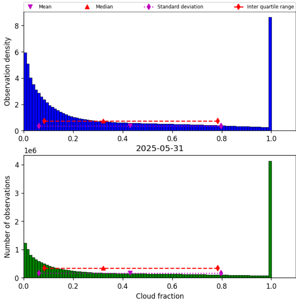
Figure 30: Histogram of “Cloud fraction” for 2025-05-31 to 2025-06-01
