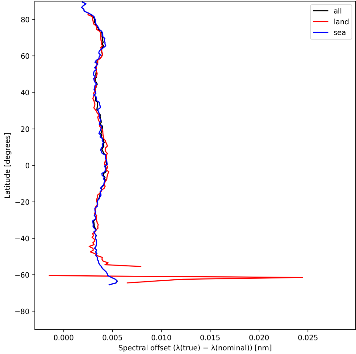
Figure 26: Zonal average of “Spectral offset ( \lambda_{\text{true}} - \lambda_{\text{nominal}} )” for 2025-05-31 to 2025-06-01.
