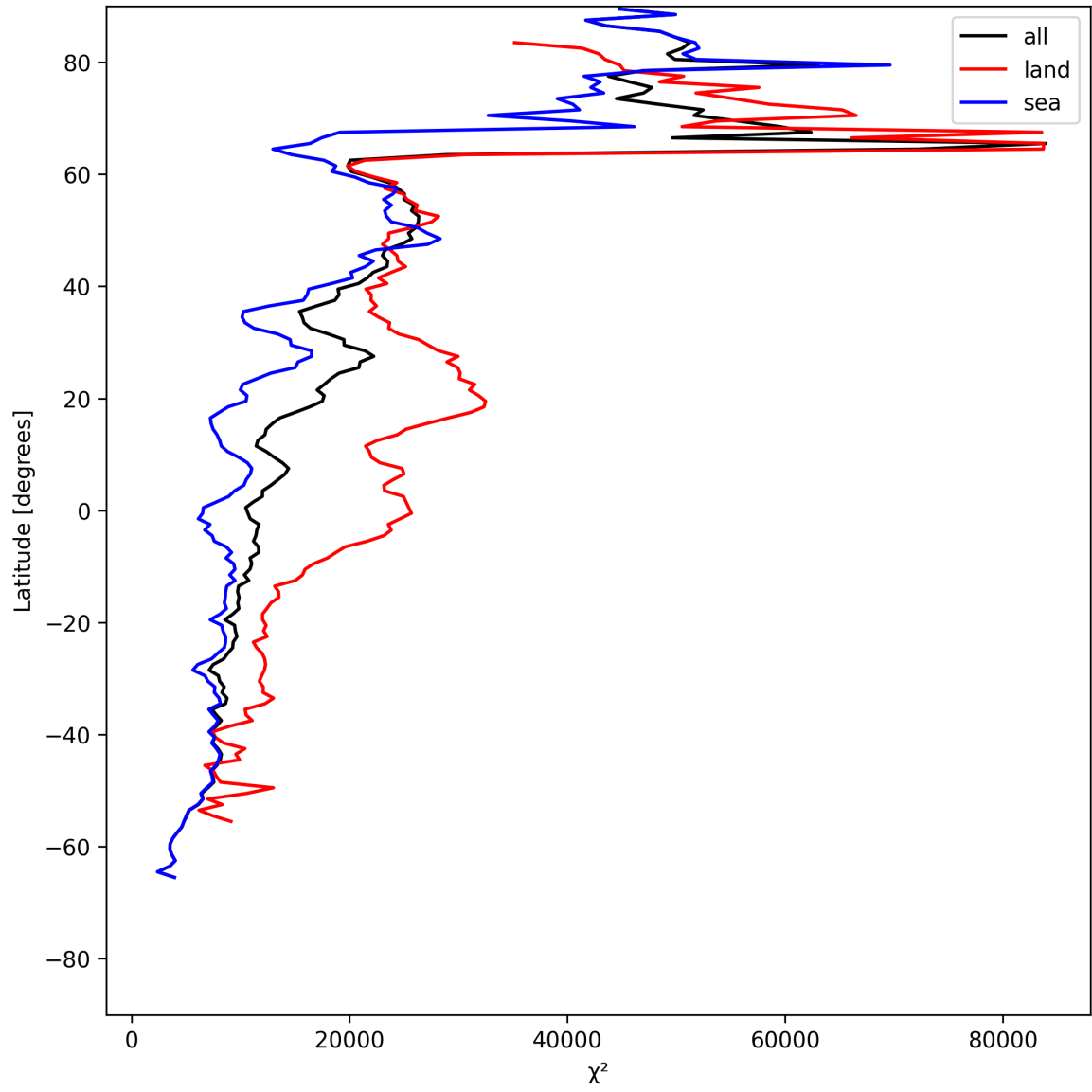
Figure 19: Zonal average of “ \chi^2 ” for 2025-06-03 to 2025-06-04.
