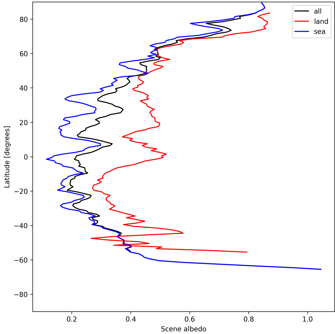
Figure 15: Zonal average of “Scene albedo” for 2025-06-03 to 2025-06-04.
