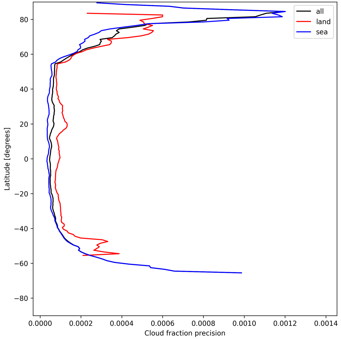
Figure 14: Zonal average of “Cloud fraction precision” for 2025-06-03 to 2025-06-04.
