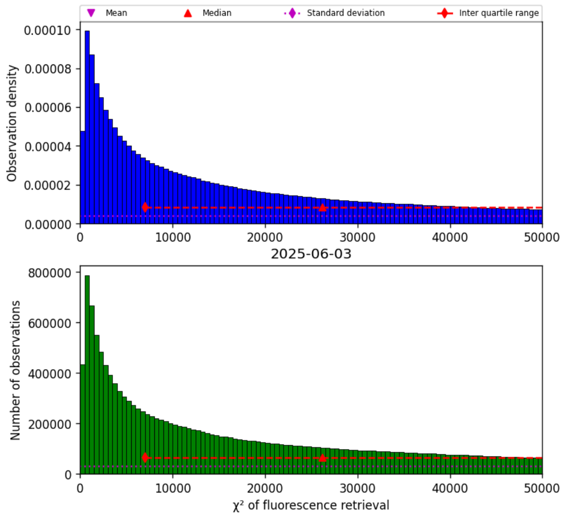
Figure 40: Histogram of “ \chi^2 of fluorescence retrieval” for 2025-06-03 to 2025-06-04
