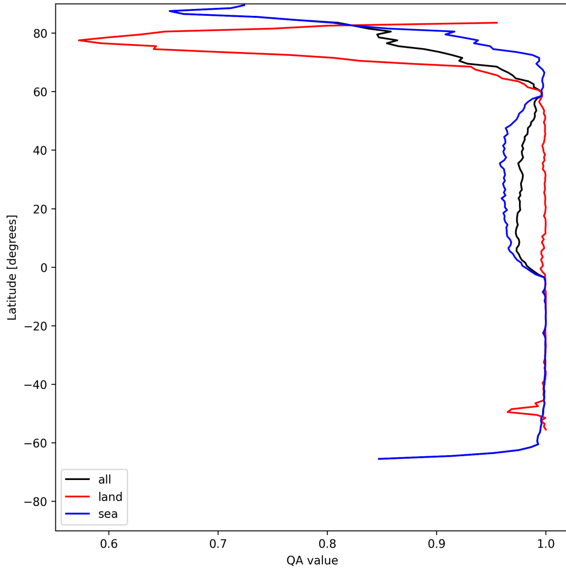
Figure 10: Zonal average of “QA value” for 2025-06-03 to 2025-06-04.
