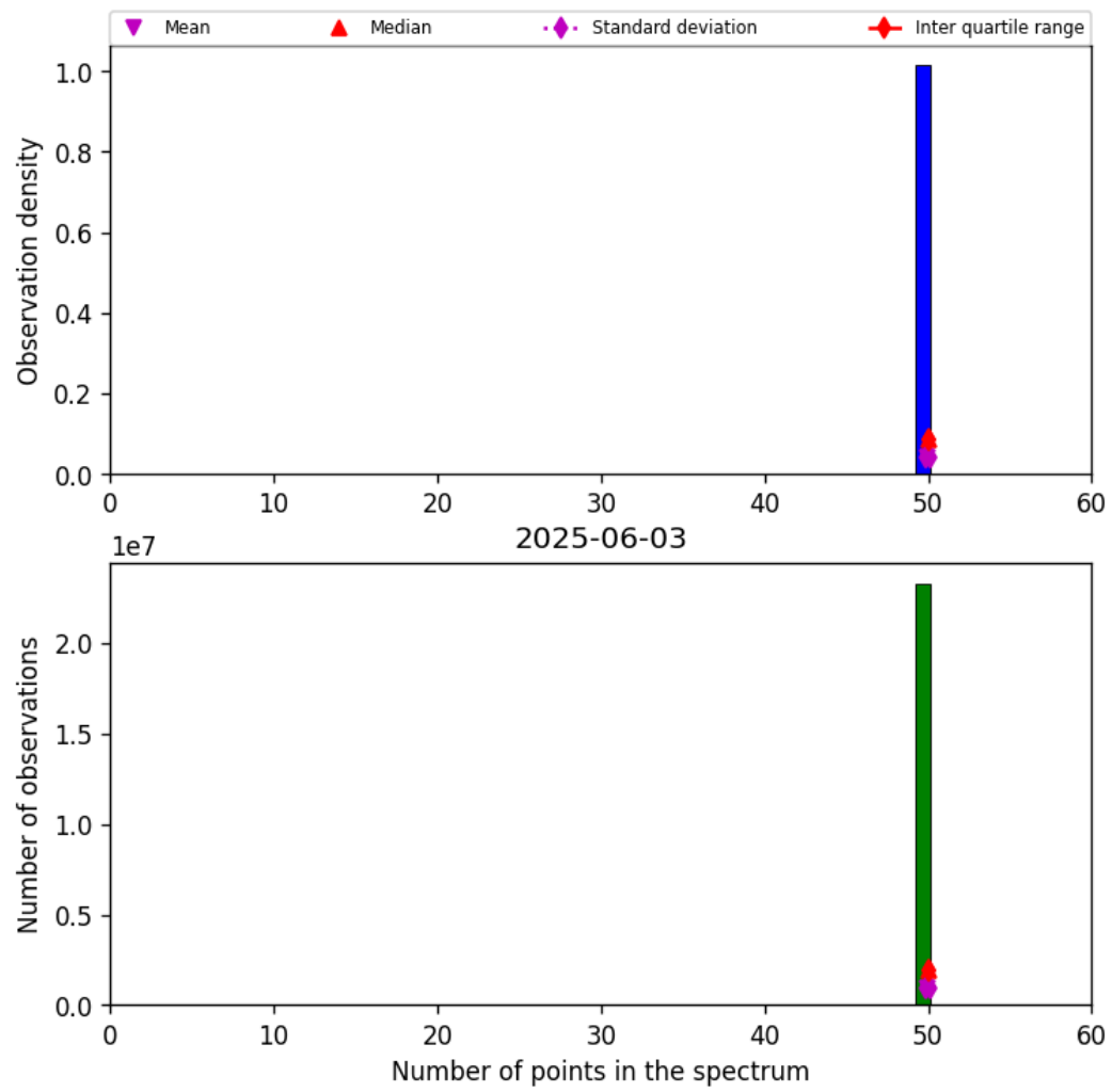
Figure 42: Histogram of “Number of points in the spectrum” for 2025-06-03 to 2025-06-04
