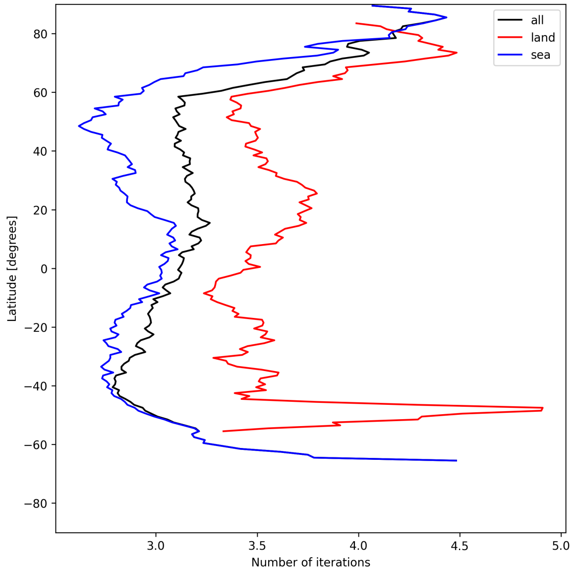
Figure 20: Zonal average of “Number of iterations” for 2025-06-03 to 2025-06-04.
