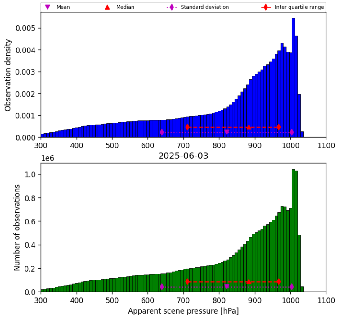
Figure 34: Histogram of “Apparent scene pressure” for 2025-06-03 to 2025-06-04
