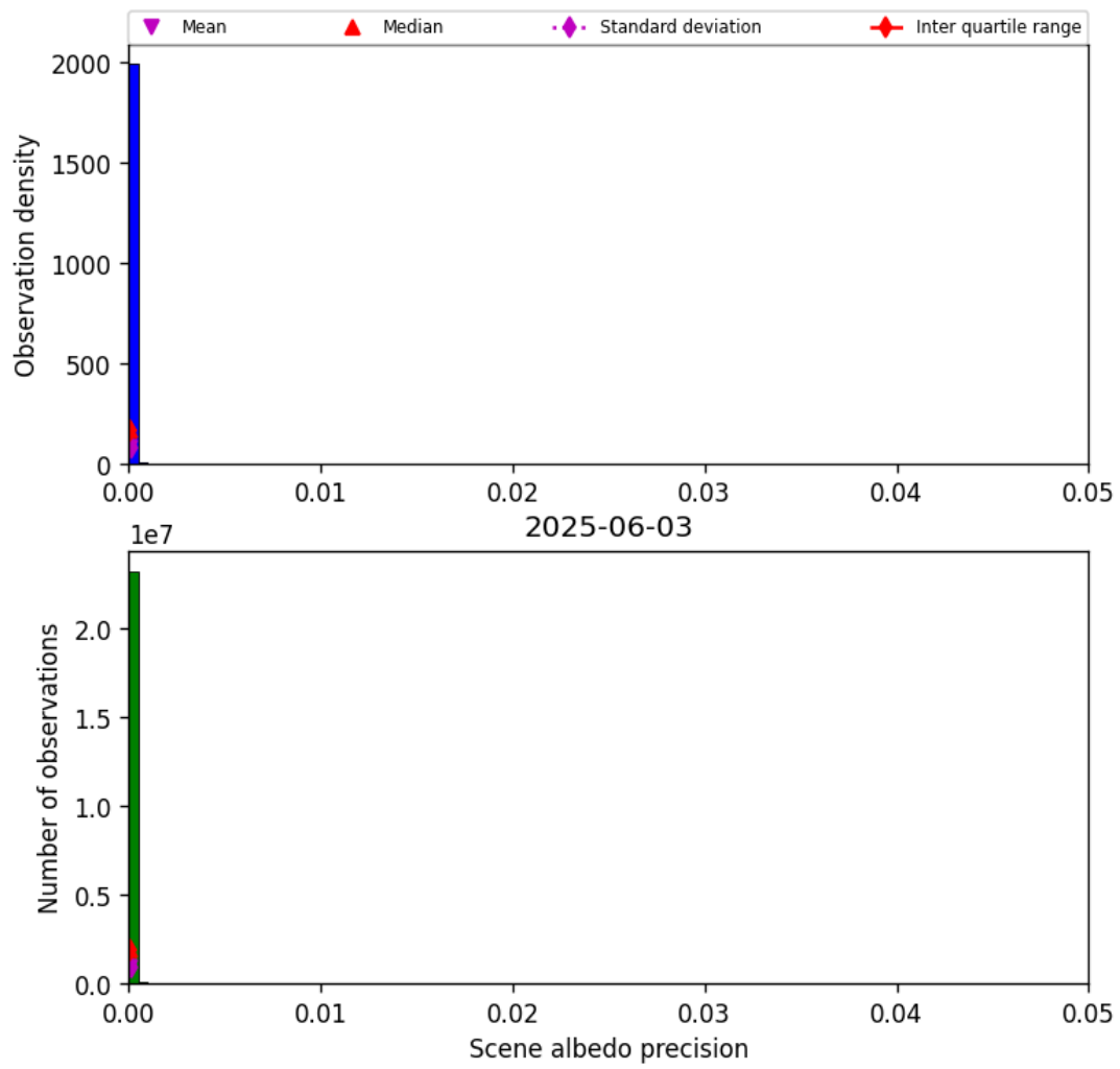
Figure 33: Histogram of “Scene albedo precision” for 2025-06-03 to 2025-06-04
