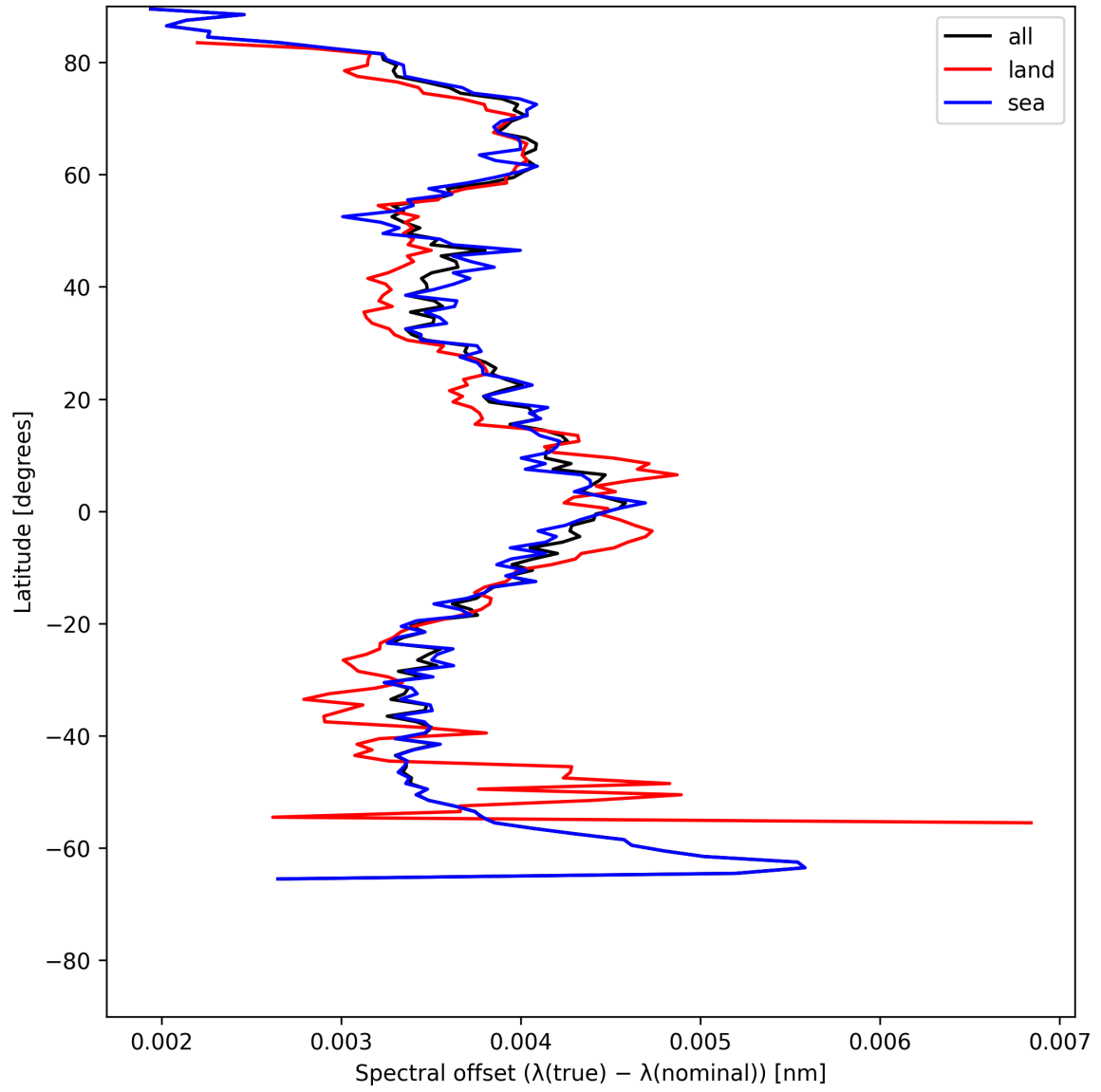
Figure 26: Zonal average of “Spectral offset ( \lambda_{\text{true}} - \lambda_{\text{nominal}} )” for 2025-06-03 to 2025-06-04.
