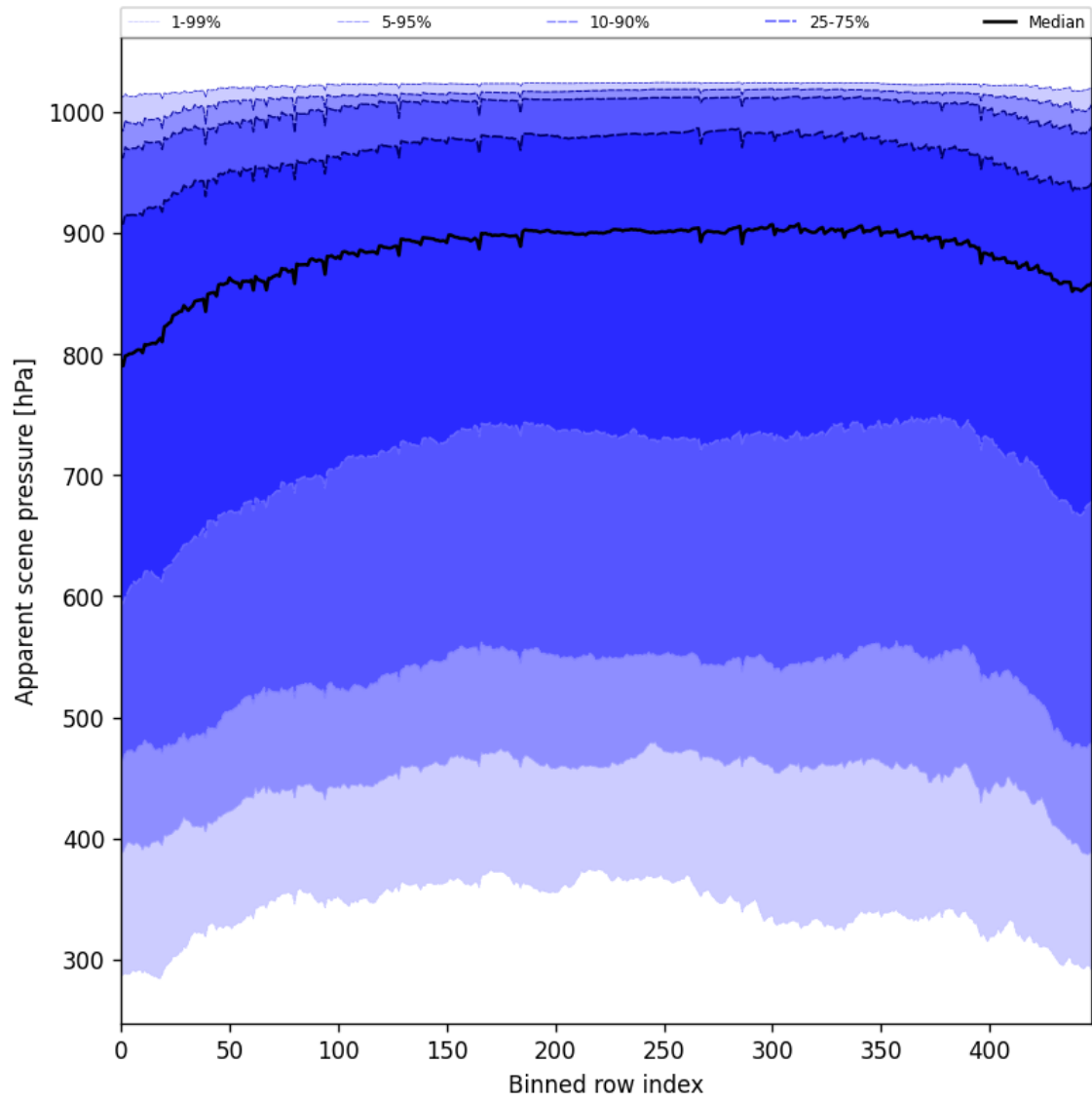
Figure 51: Along track statistics of “Apparent scene pressure” for 2025-06-03 to 2025-06-04
