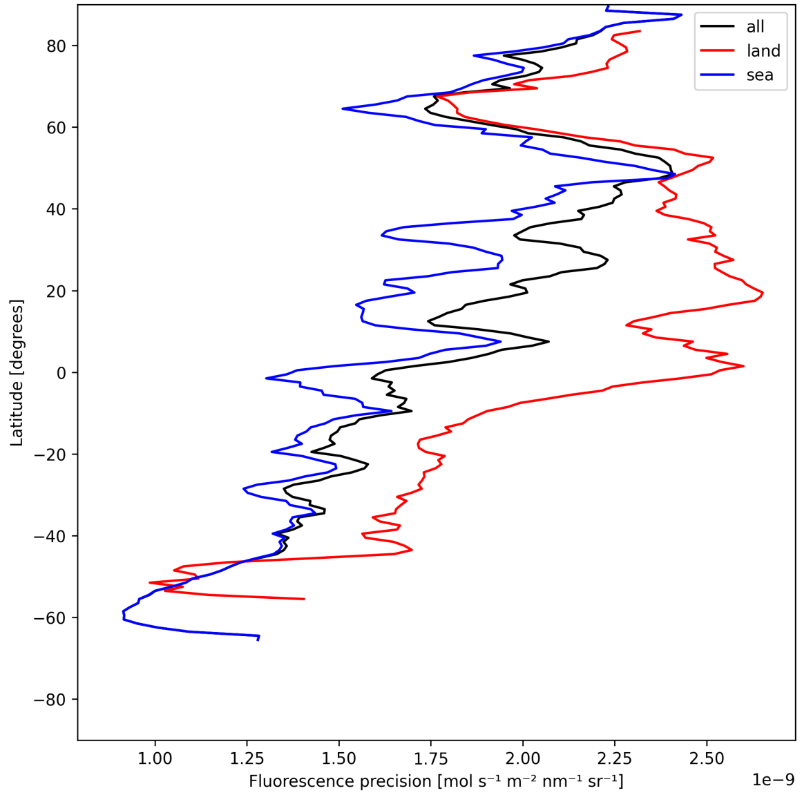
Figure 22: Zonal average of “Fluorescence precision” for 2025-06-03 to 2025-06-04.
