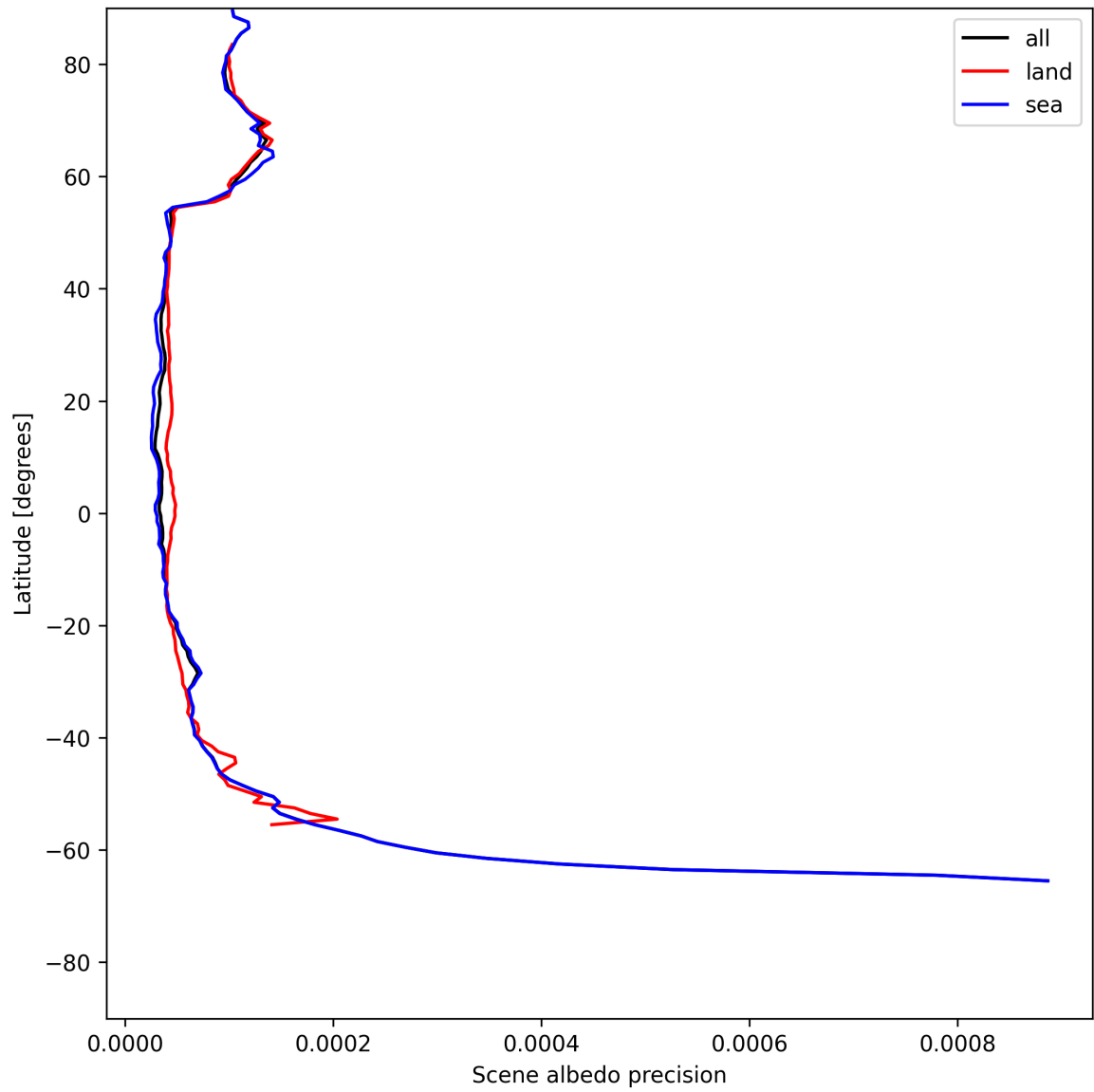
Figure 16: Zonal average of “Scene albedo precision” for 2025-06-03 to 2025-06-04.
