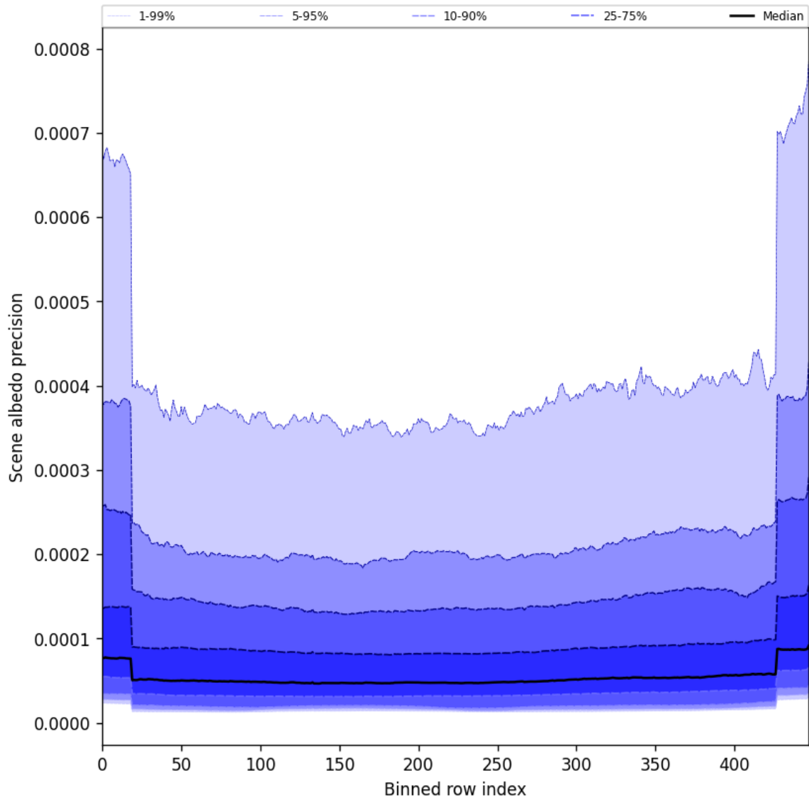
Figure 50: Along track statistics of “Scene albedo precision” for 2025-06-03 to 2025-06-04
