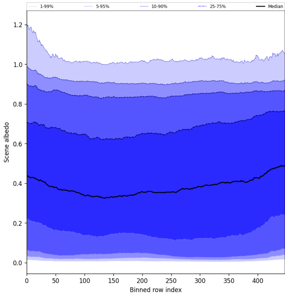
Figure 49: Along track statistics of “Scene albedo” for 2025-06-03 to 2025-06-04
