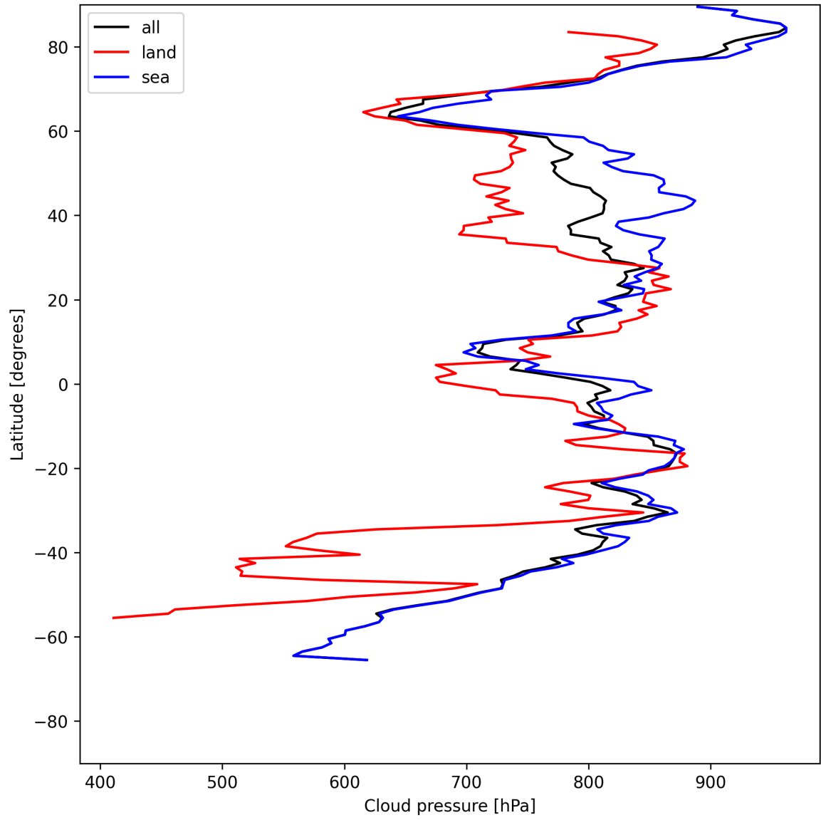
Figure 11: Zonal average of “Cloud pressure” for 2025-06-03 to 2025-06-04.
