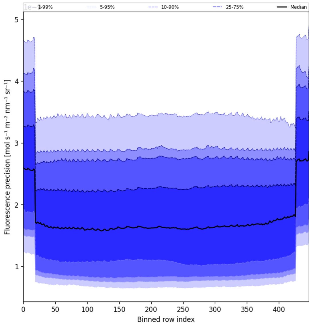
Figure 56: Along track statistics of “Fluorescence precision” for 2025-06-03 to 2025-06-04
