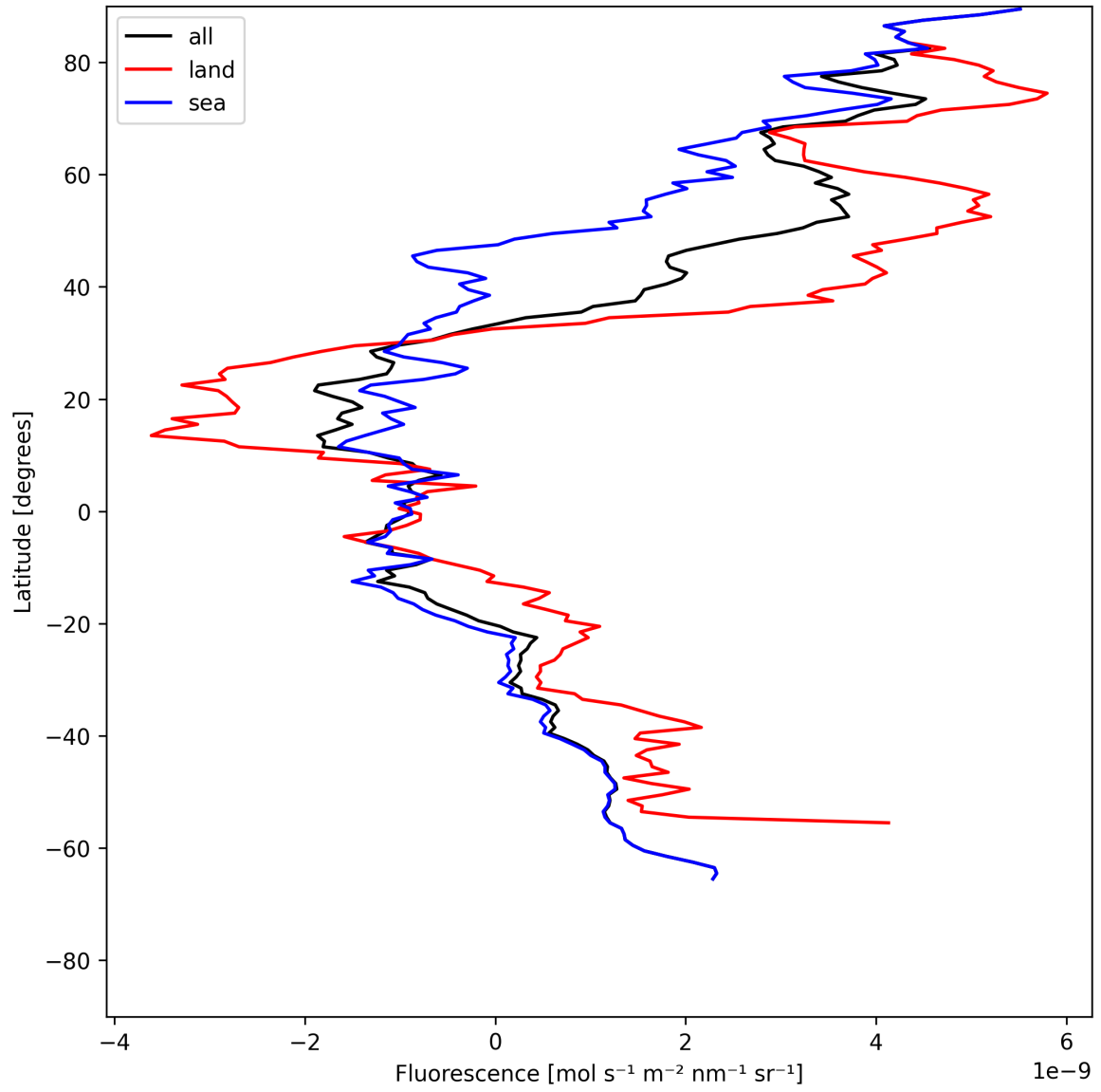
Figure 21: Zonal average of “Fluorescence” for 2025-06-03 to 2025-06-04.
