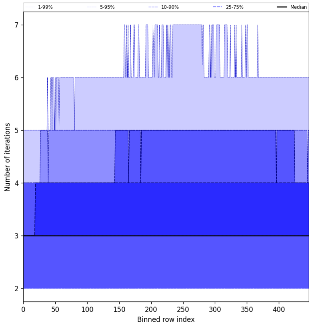
Figure 54: Along track statistics of “Number of iterations” for 2025-06-03 to 2025-06-04
