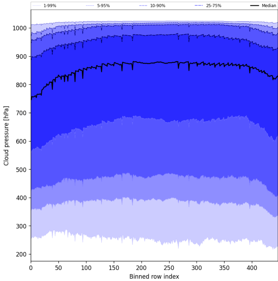
Figure 45: Along track statistics of “Cloud pressure” for 2025-06-03 to 2025-06-04
