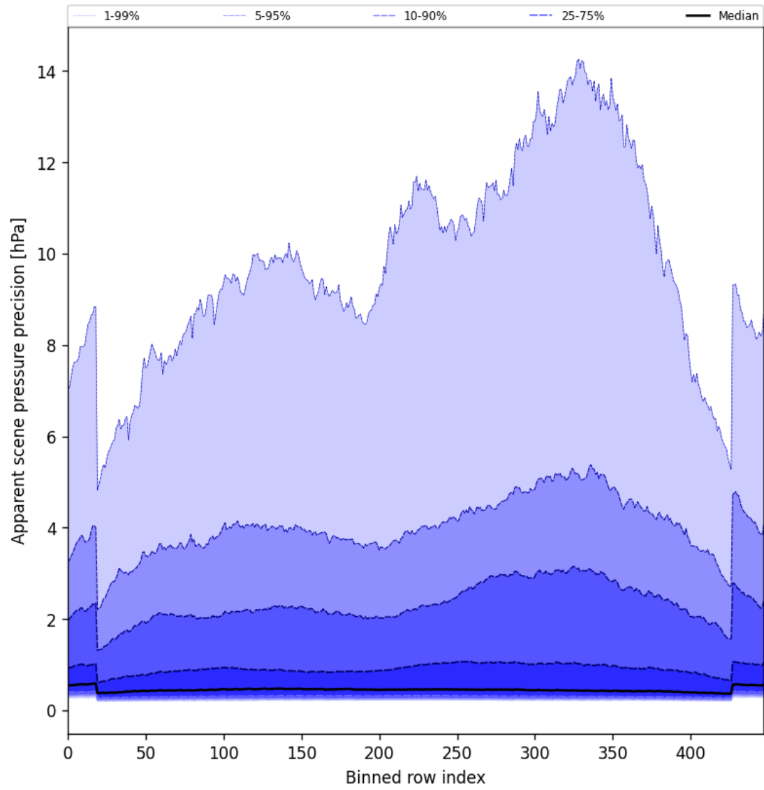
Figure 52: Along track statistics of “Apparent scene pressure precision” for 2025-06-03 to 2025-06-04
