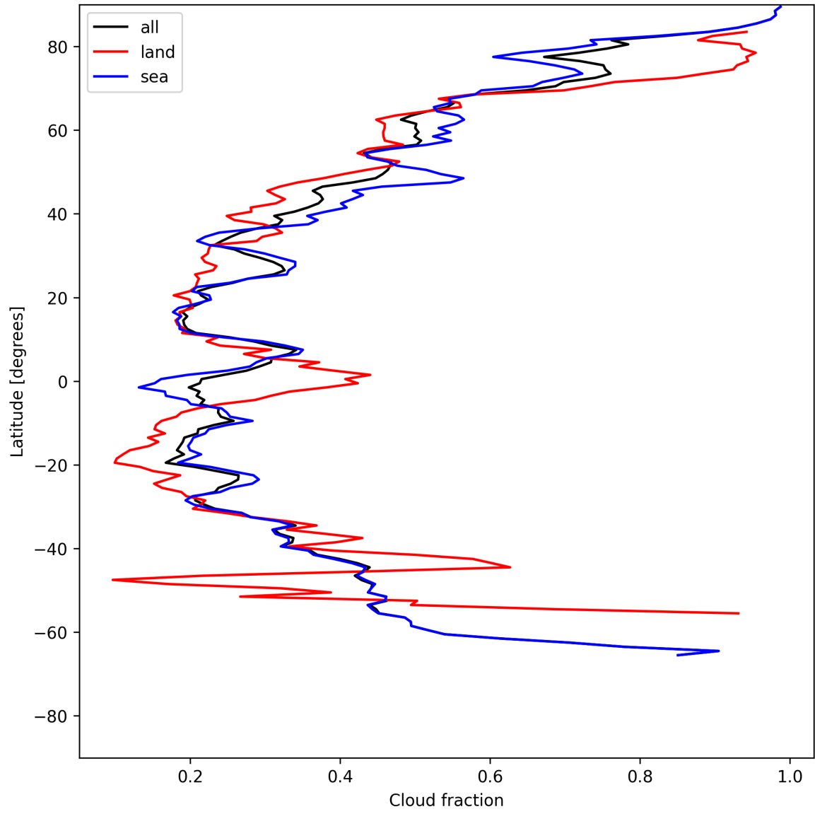
Figure 13: Zonal average of “Cloud fraction” for 2025-06-03 to 2025-06-04.
