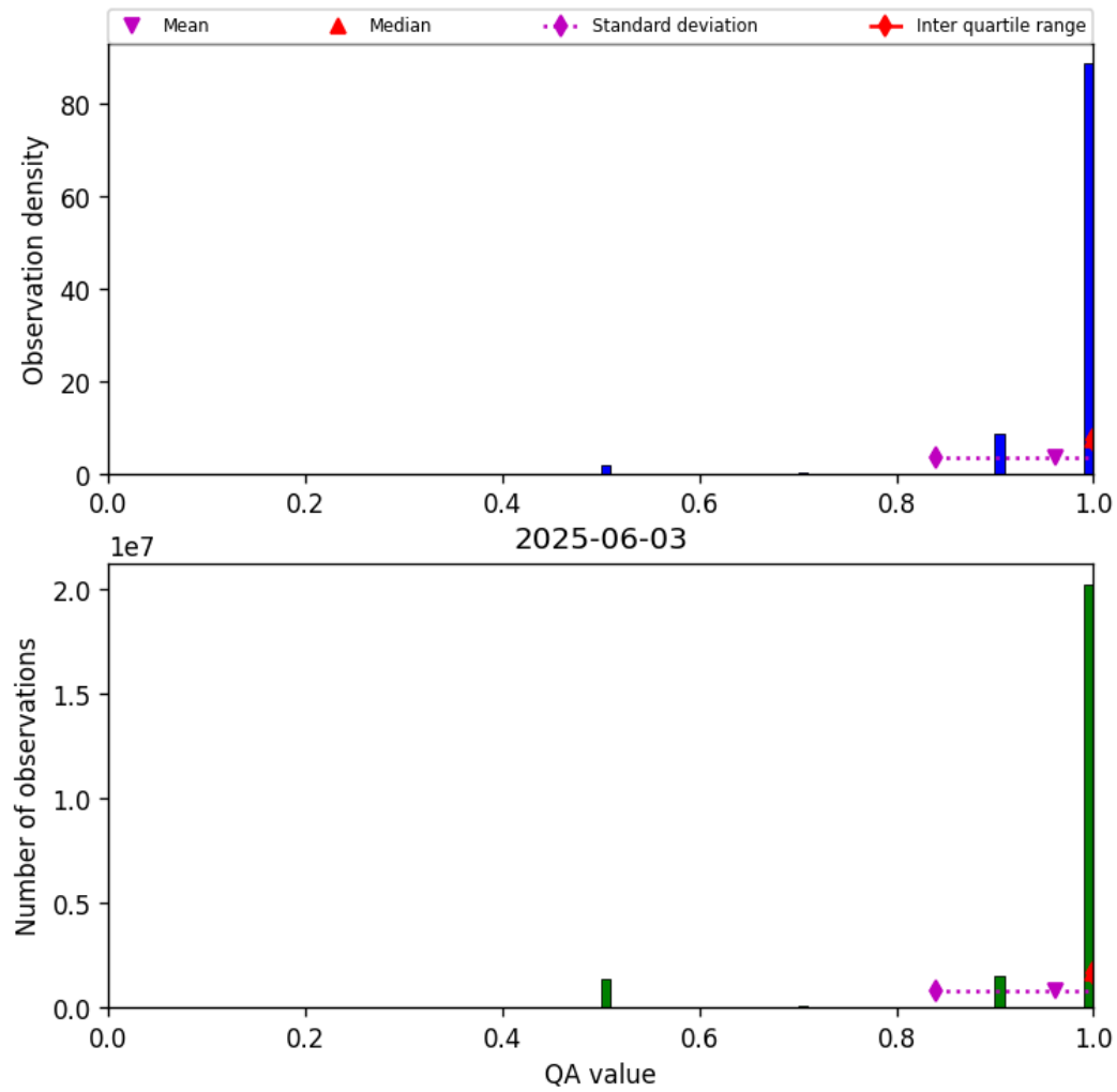
Figure 27: Histogram of “QA value” for 2025-06-03 to 2025-06-04
