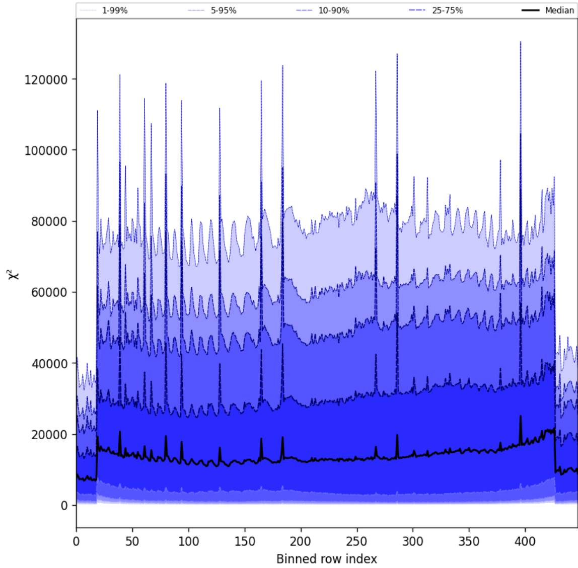
Figure 53: Along track statistics of “ \chi^2 ” for 2025-06-03 to 2025-06-04
