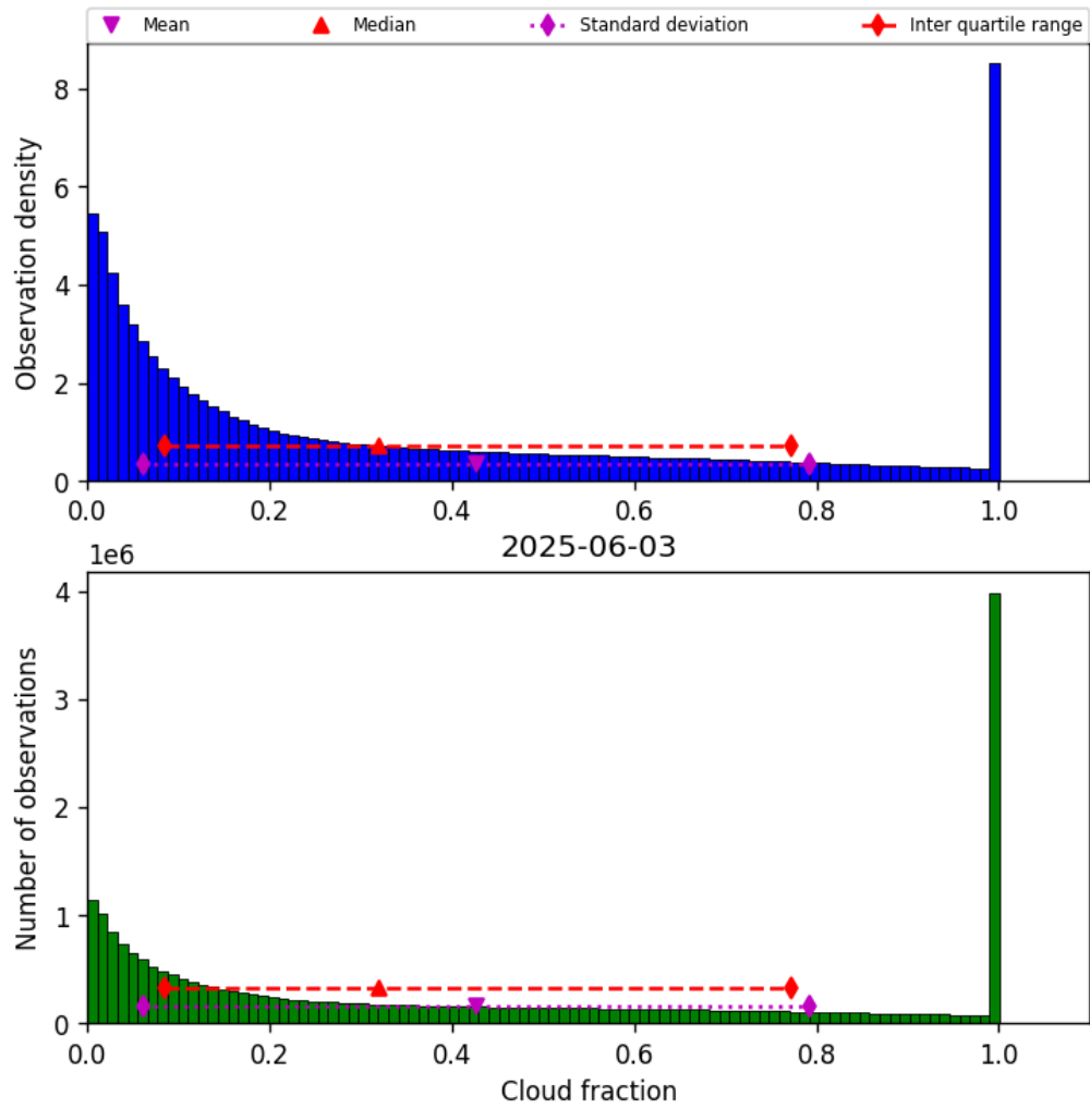
Figure 30: Histogram of “Cloud fraction” for 2025-06-03 to 2025-06-04
