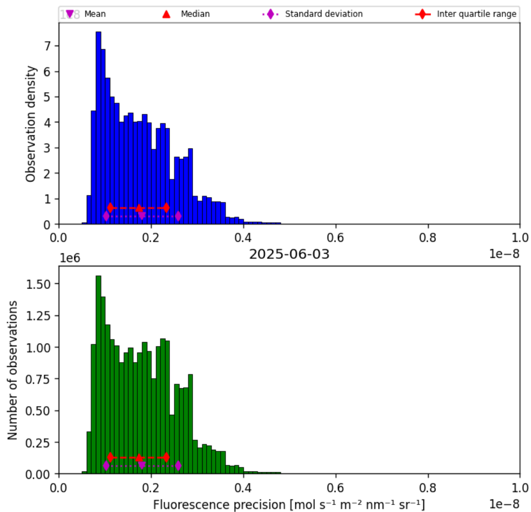
Figure 39: Histogram of “Fluorescence precision” for 2025-06-03 to 2025-06-04
