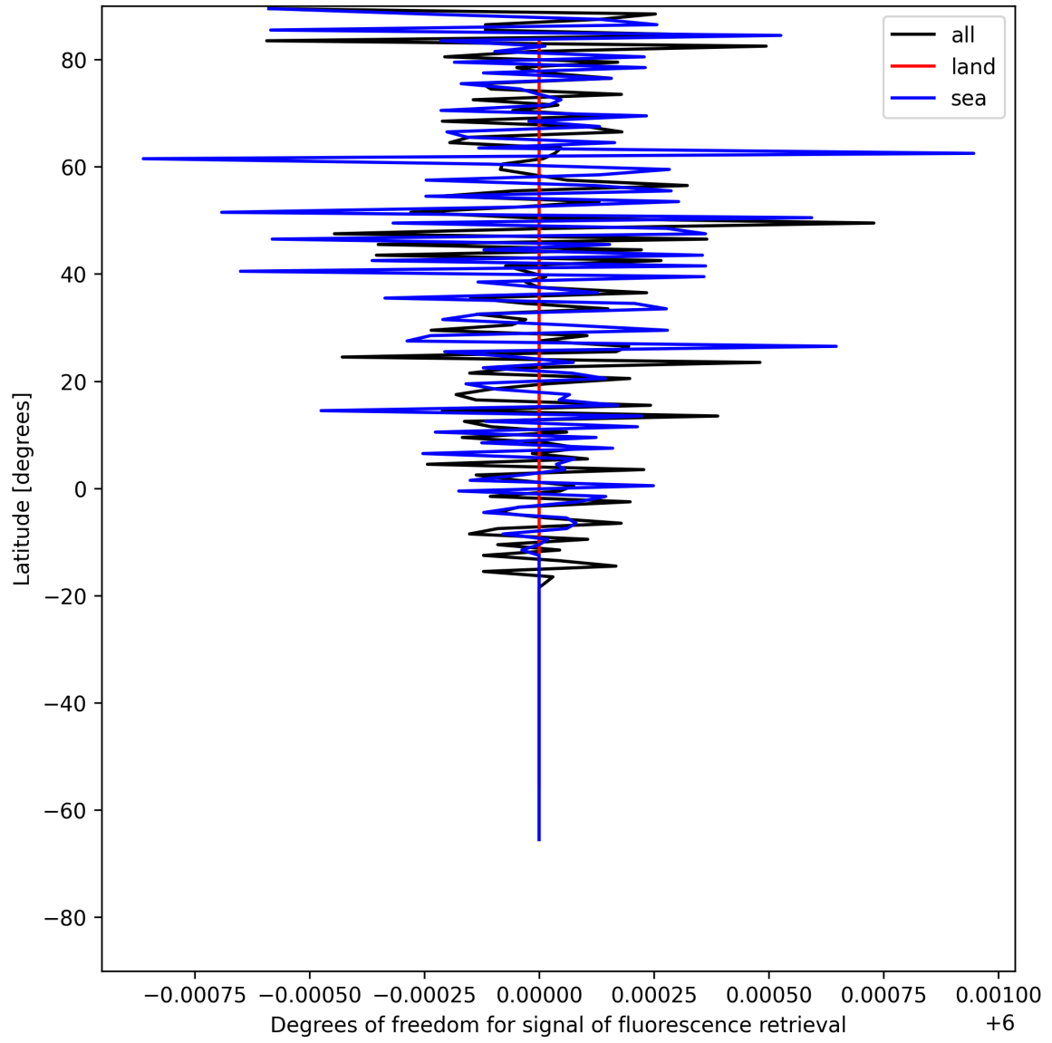
Figure 24: Zonal average of “Degrees of freedom for signal of fluorescence retrieval” for 2025-06-03 to 2025-06-04.
