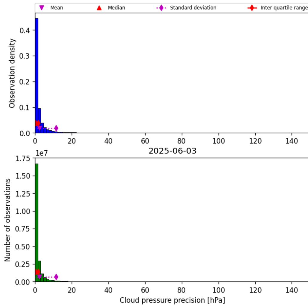
Figure 29: Histogram of “Cloud pressure precision” for 2025-06-03 to 2025-06-04
