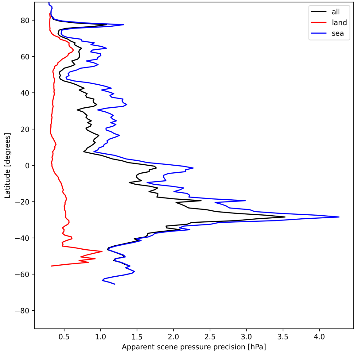
Figure 18: Zonal average of “Apparent scene pressure precision” for 2025-06-03 to 2025-06-04.
