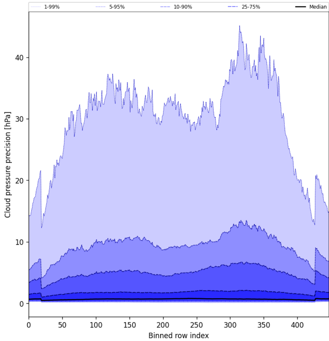
Figure 46: Along track statistics of “Cloud pressure precision” for 2025-06-03 to 2025-06-04
