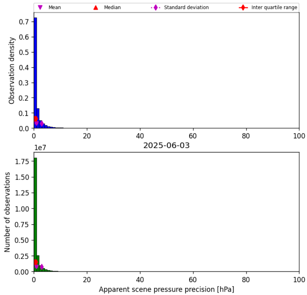
Figure 35: Histogram of “Apparent scene pressure precision” for 2025-06-03 to 2025-06-04
