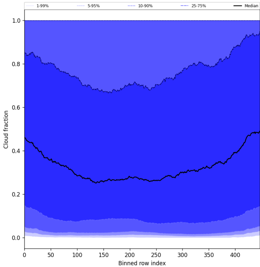
Figure 47: Along track statistics of “Cloud fraction” for 2025-06-03 to 2025-06-04
