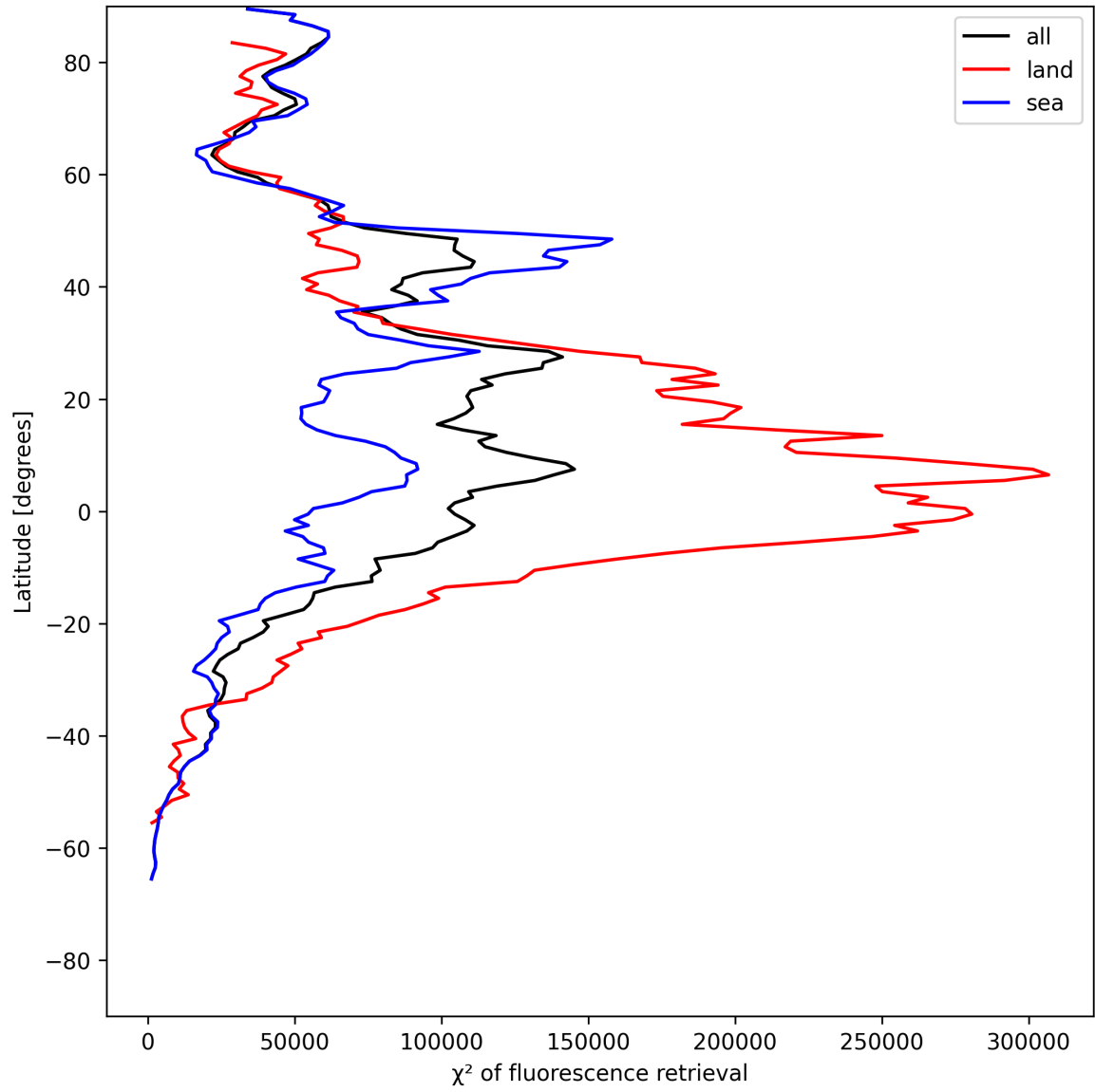
Figure 23: Zonal average of “ \chi^2 of fluorescence retrieval” for 2025-06-03 to 2025-06-04.
