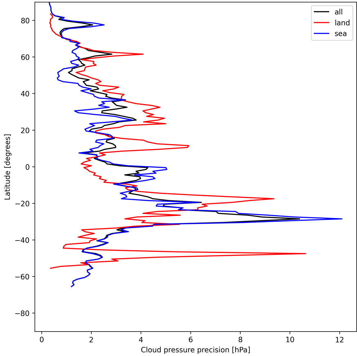
Figure 12: Zonal average of “Cloud pressure precision” for 2025-06-03 to 2025-06-04.
