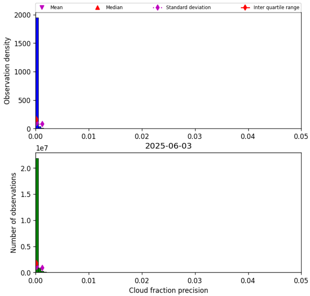
Figure 31: Histogram of “Cloud fraction precision” for 2025-06-03 to 2025-06-04
