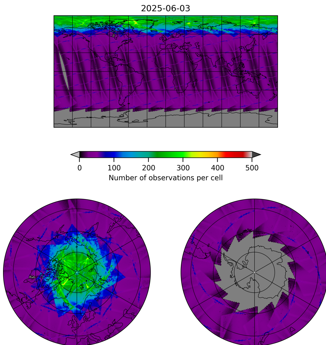
Figure 9: Map of the number of observations for 2025-06-03 to 2025-06-04
