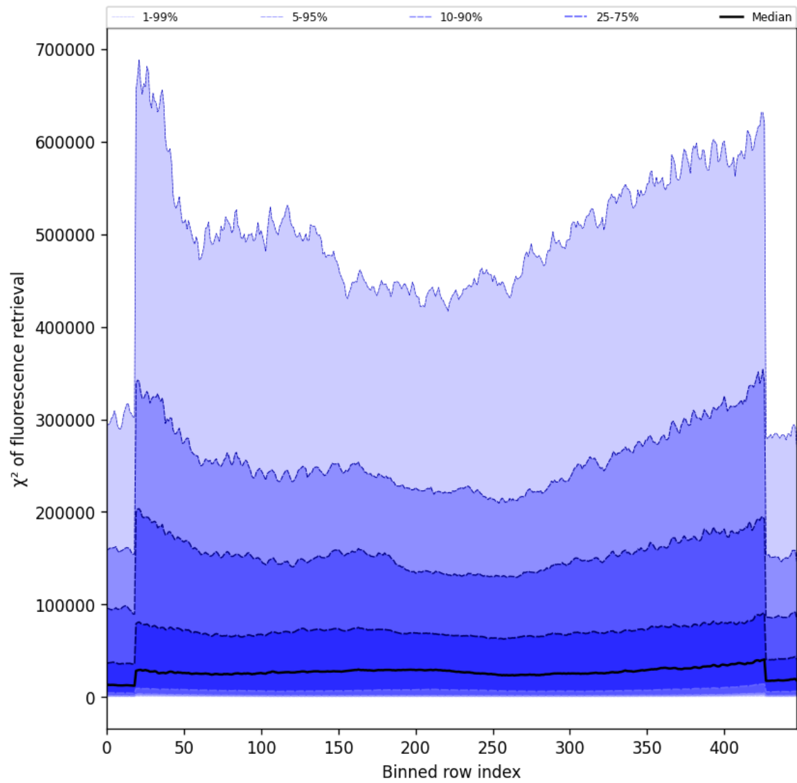
Figure 57: Along track statistics of “ \chi^2 of fluorescence retrieval” for 2025-06-03 to 2025-06-04
