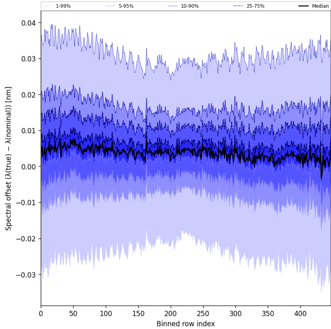
Figure 60: Along track statistics of “Spectral offset ( \lambda_{\text{true}} - \lambda_{\text{nominal}} )” for 2025-06-03 to 2025-06-04
