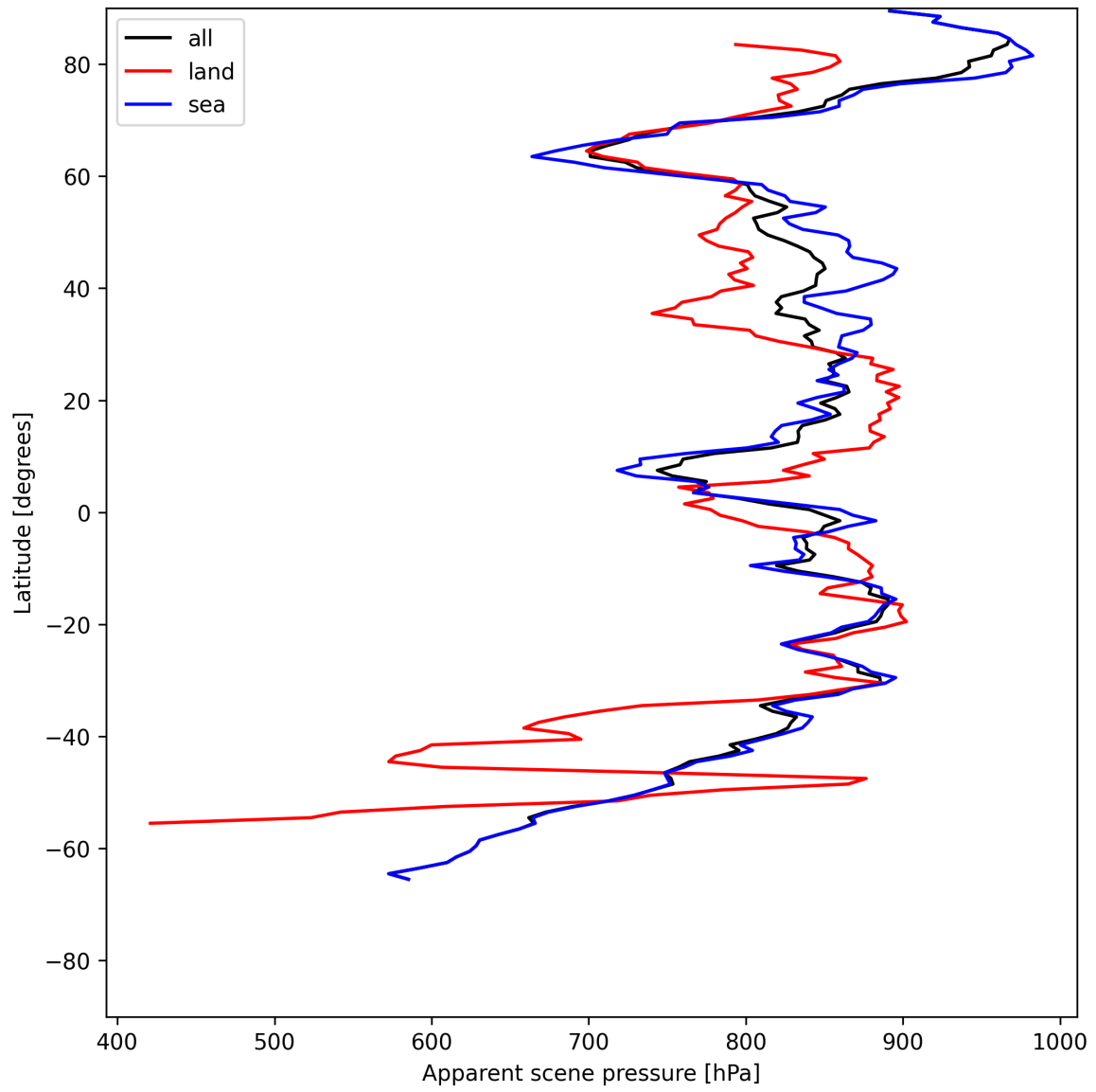
Figure 17: Zonal average of “Apparent scene pressure” for 2025-06-03 to 2025-06-04.
