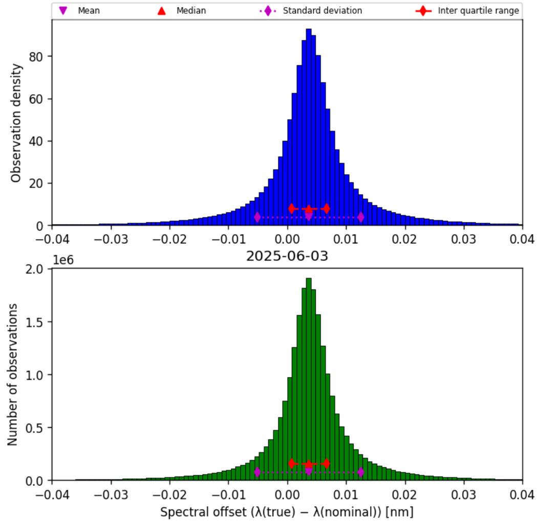
Figure 43: Histogram of “Spectral offset ( \lambda_{\text{true}} - \lambda_{\text{nominal}} )” for 2025-06-03 to 2025-06-04
