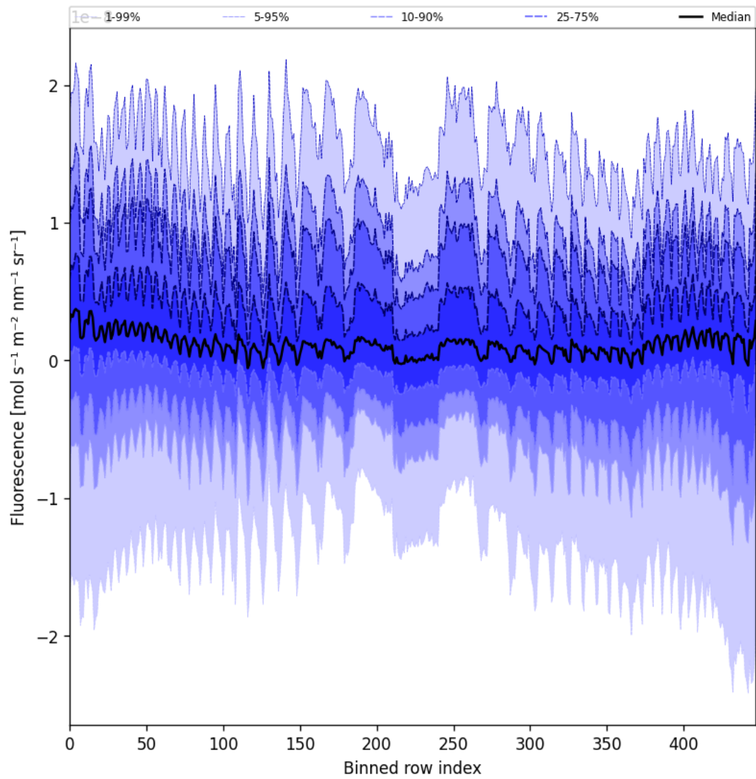
Figure 55: Along track statistics of “Fluorescence” for 2025-06-03 to 2025-06-04
