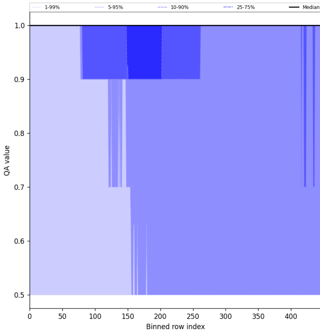
Figure 44: Along track statistics of "QA value" for 2025-06-03 to 2025-06-04
