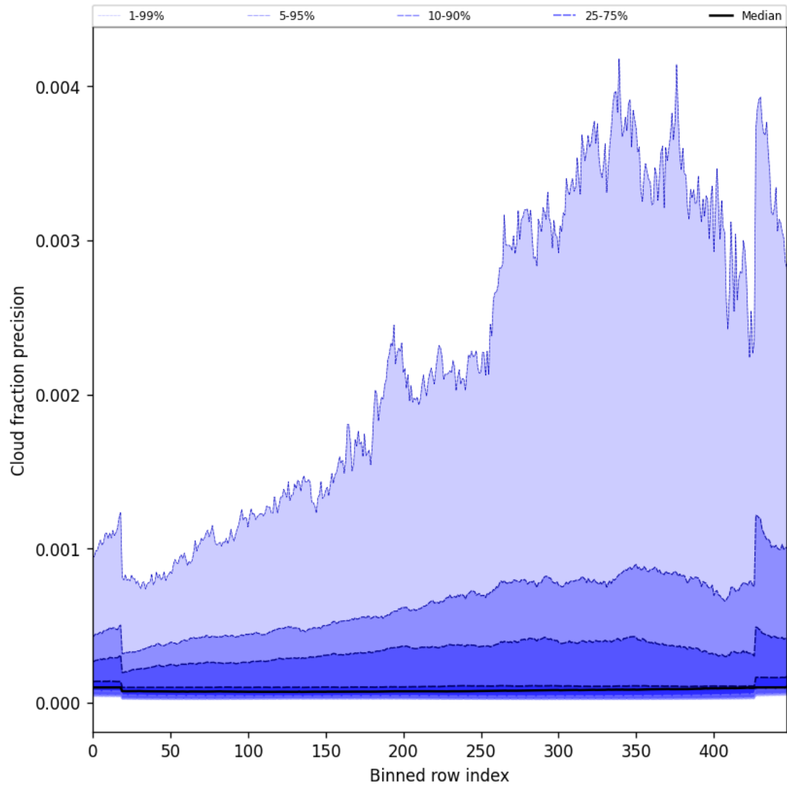
Figure 48: Along track statistics of “Cloud fraction precision” for 2025-06-03 to 2025-06-04
