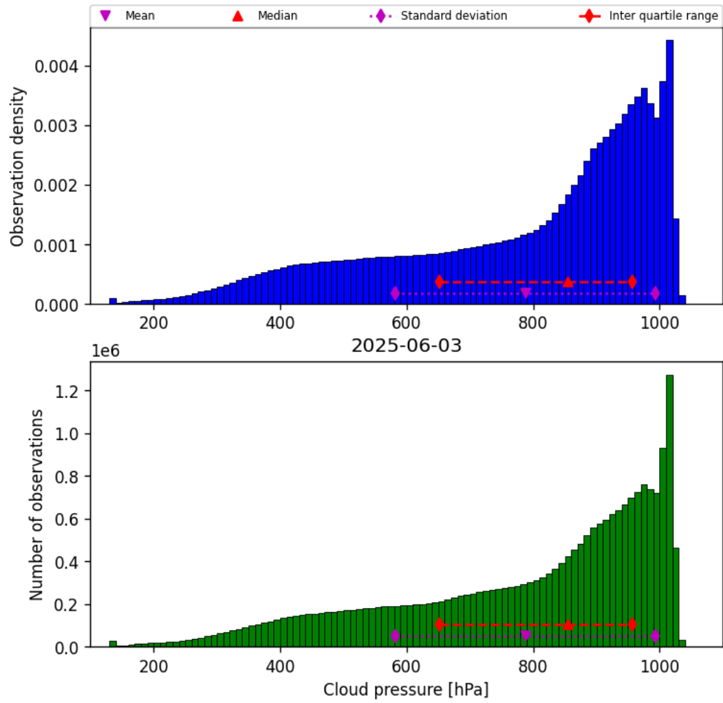
Figure 28: Histogram of “Cloud pressure” for 2025-06-03 to 2025-06-04
