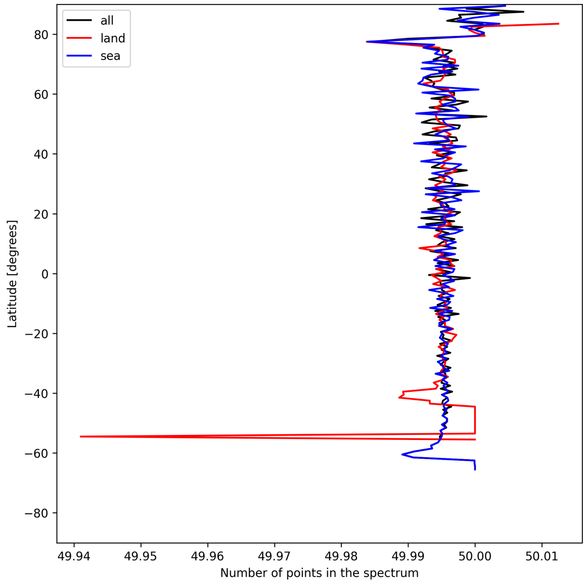
Figure 25: Zonal average of “Number of points in the spectrum” for 2025-06-03 to 2025-06-04.
