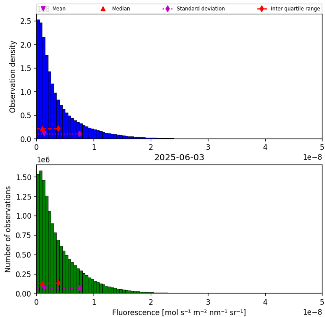
Figure 38: Histogram of “Fluorescence” for 2025-06-03 to 2025-06-04
