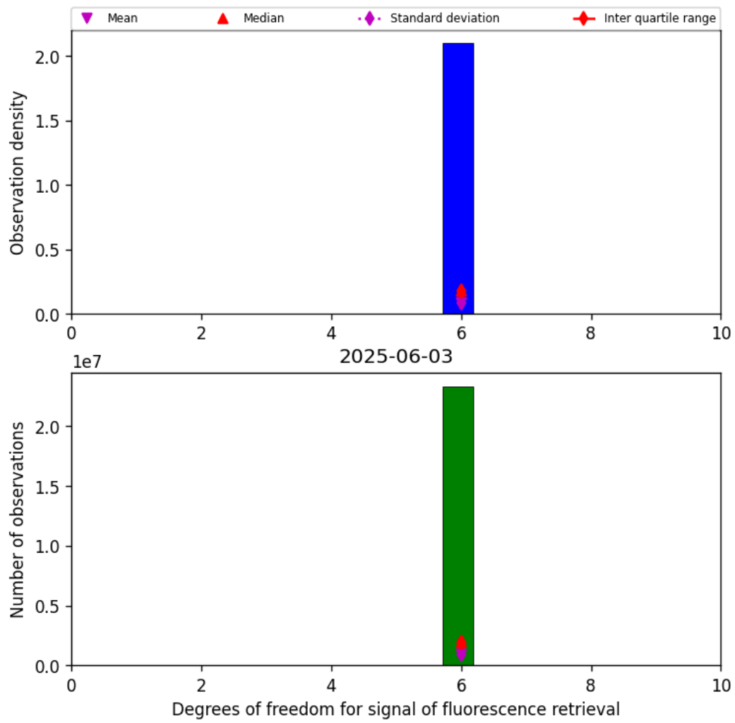
Figure 41: Histogram of “Degrees of freedom for signal of fluorescence retrieval” for 2025-06-03 to 2025-06-04
