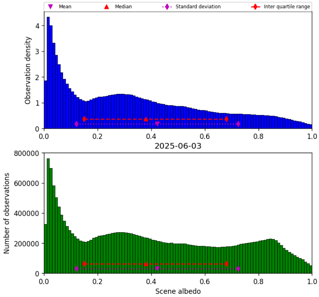
Figure 32: Histogram of “Scene albedo” for 2025-06-03 to 2025-06-04
