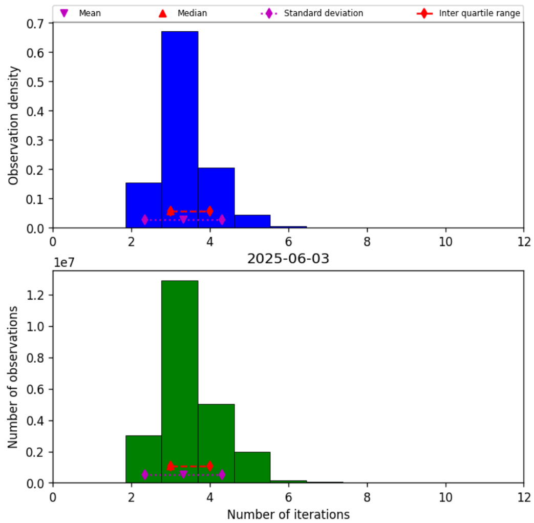
Figure 37: Histogram of “Number of iterations” for 2025-06-03 to 2025-06-04
