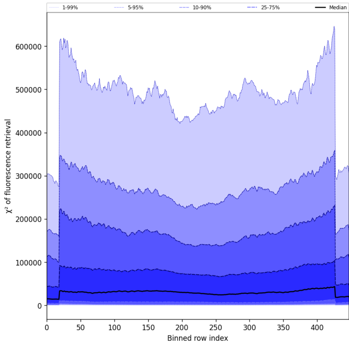
Figure 57: Along track statistics of “ \chi^2 of fluorescence retrieval” for 2025-06-07 to 2025-06-08
