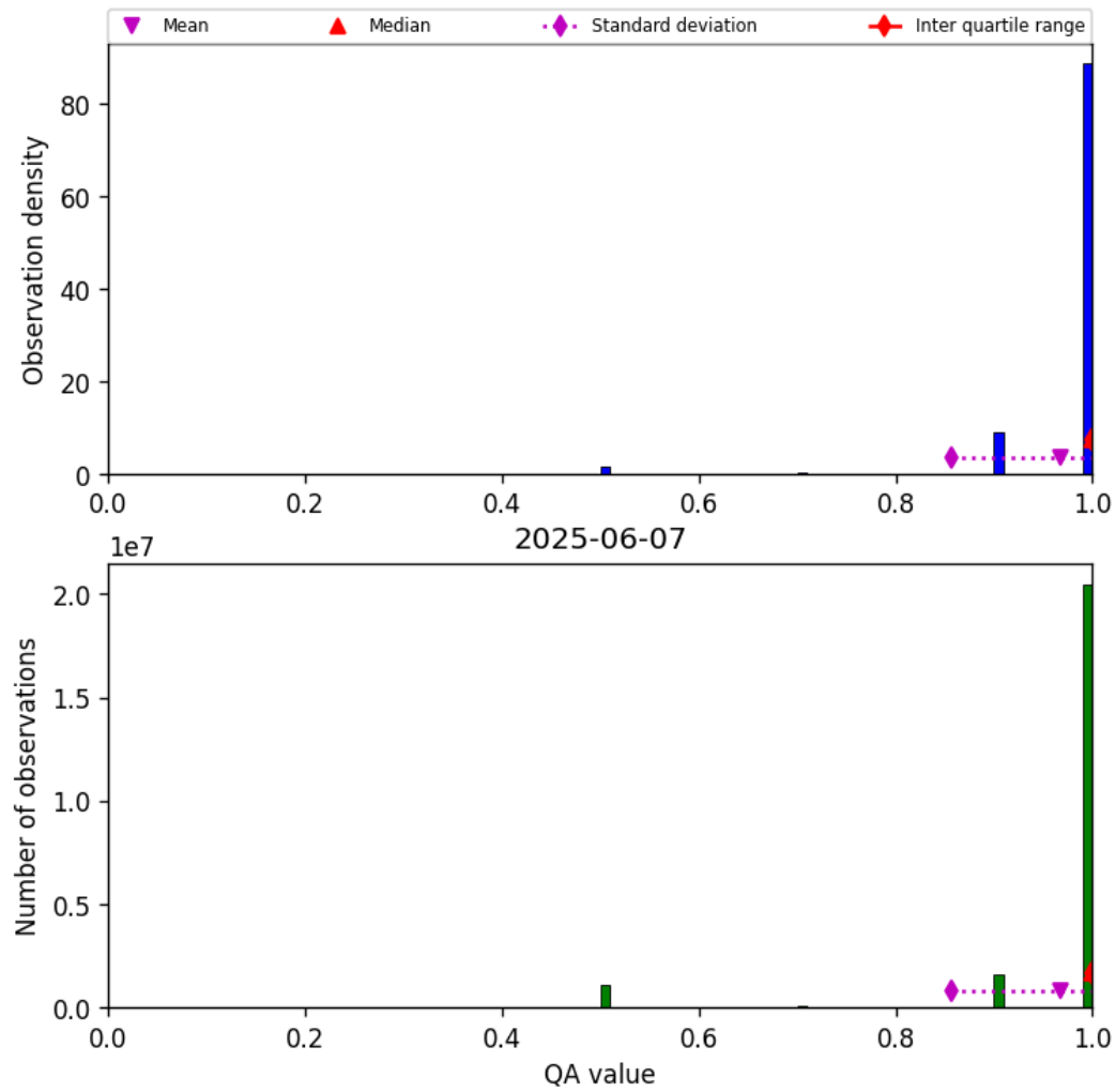
Figure 27: Histogram of “QA value” for 2025-06-07 to 2025-06-08
