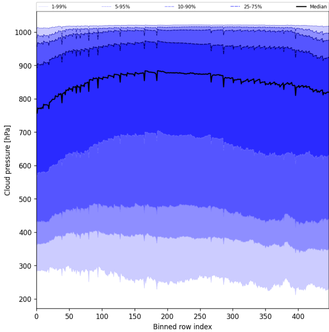
Figure 45: Along track statistics of “Cloud pressure” for 2025-06-07 to 2025-06-08
