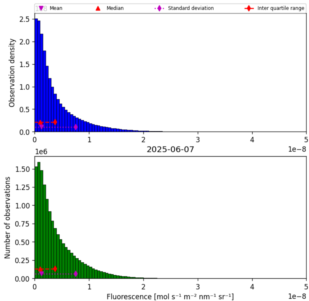
Figure 38: Histogram of “Fluorescence” for 2025-06-07 to 2025-06-08
