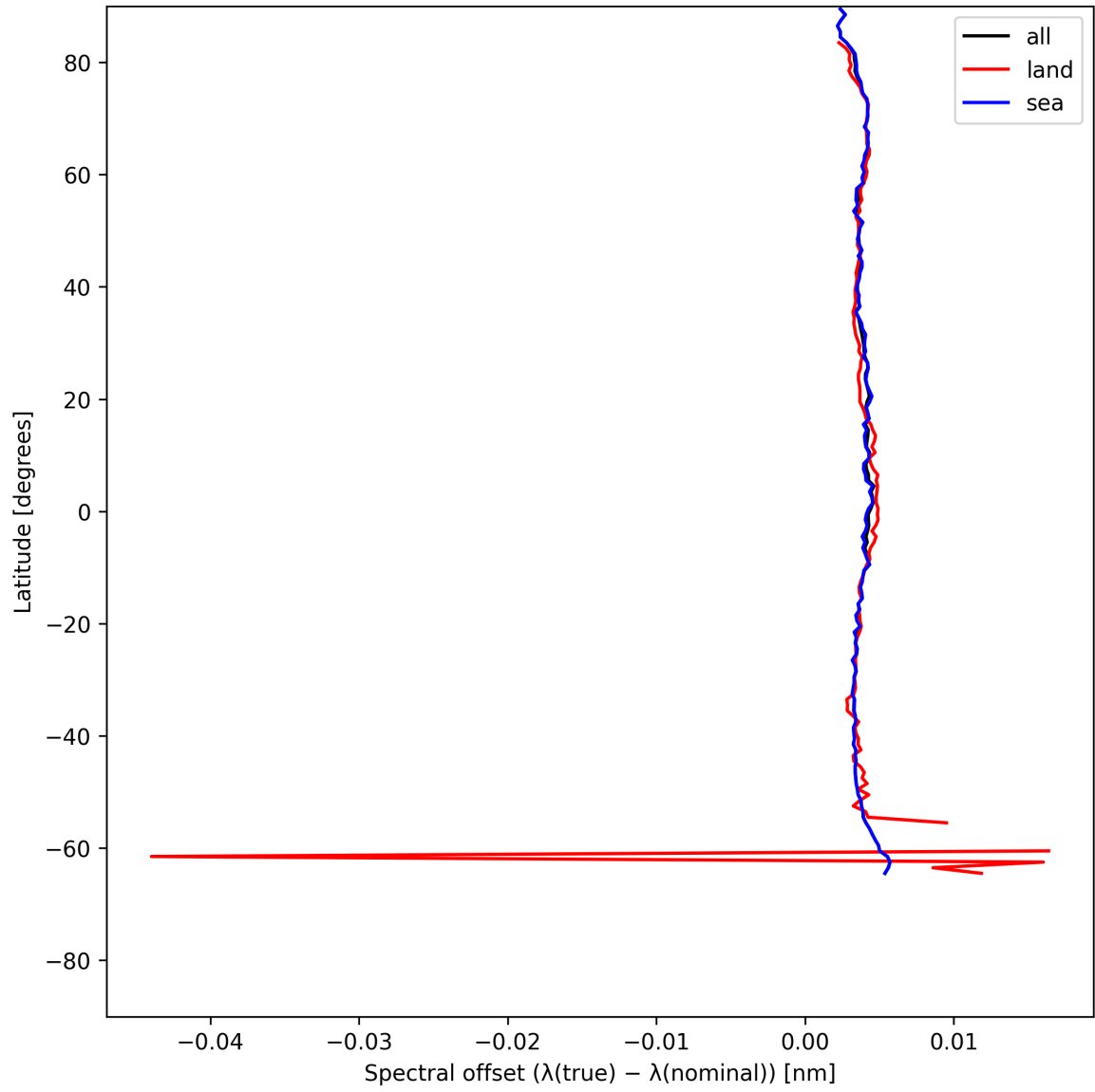
Figure 26: Zonal average of “Spectral offset ( \lambda_{\text{true}} - \lambda_{\text{nominal}} )” for 2025-06-07 to 2025-06-08.
