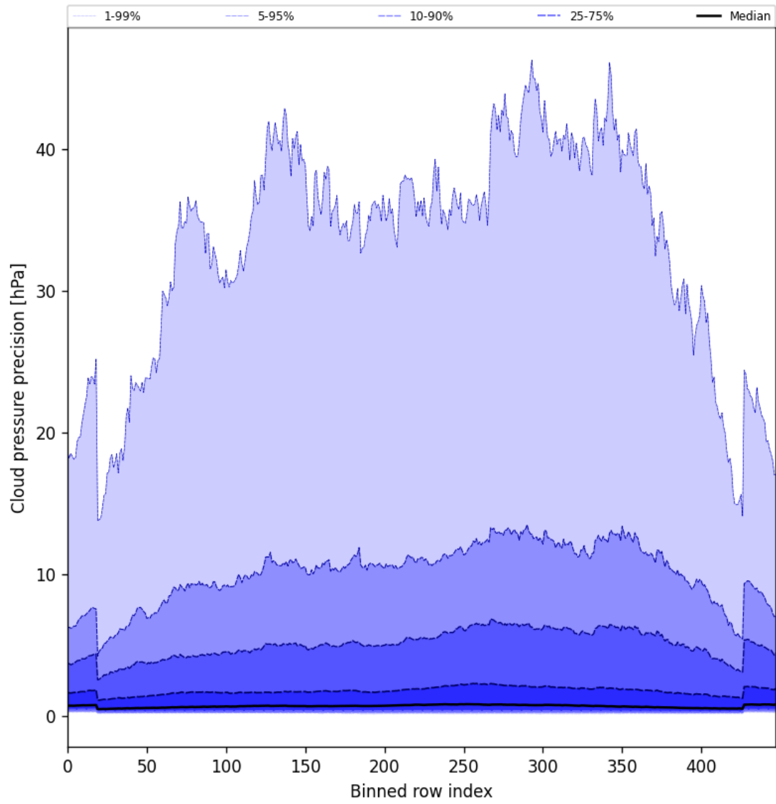
Figure 46: Along track statistics of “Cloud pressure precision” for 2025-06-07 to 2025-06-08
