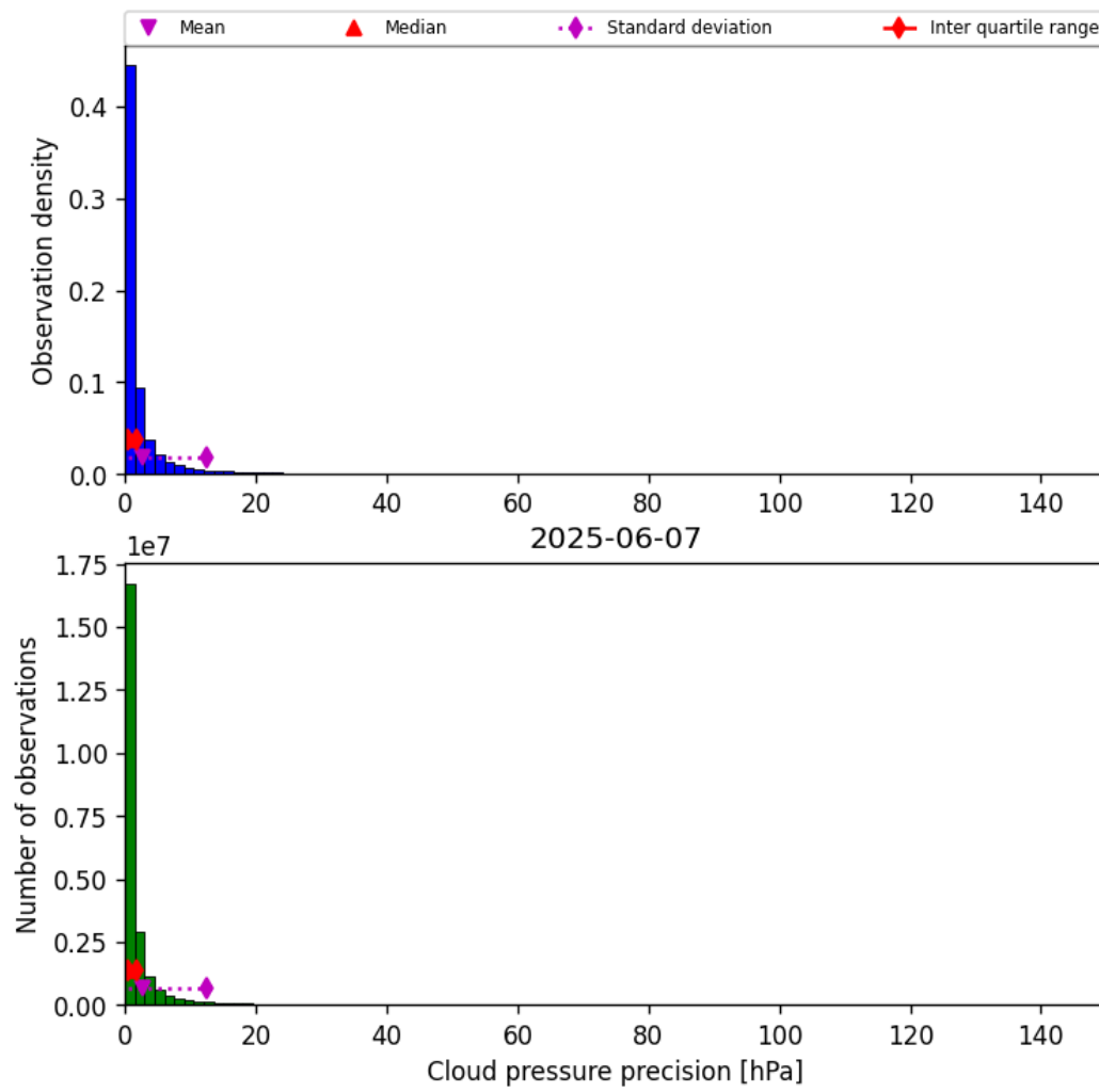
Figure 29: Histogram of “Cloud pressure precision” for 2025-06-07 to 2025-06-08
