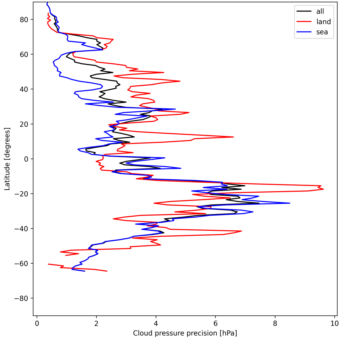
Figure 12: Zonal average of “Cloud pressure precision” for 2025-06-07 to 2025-06-08.
