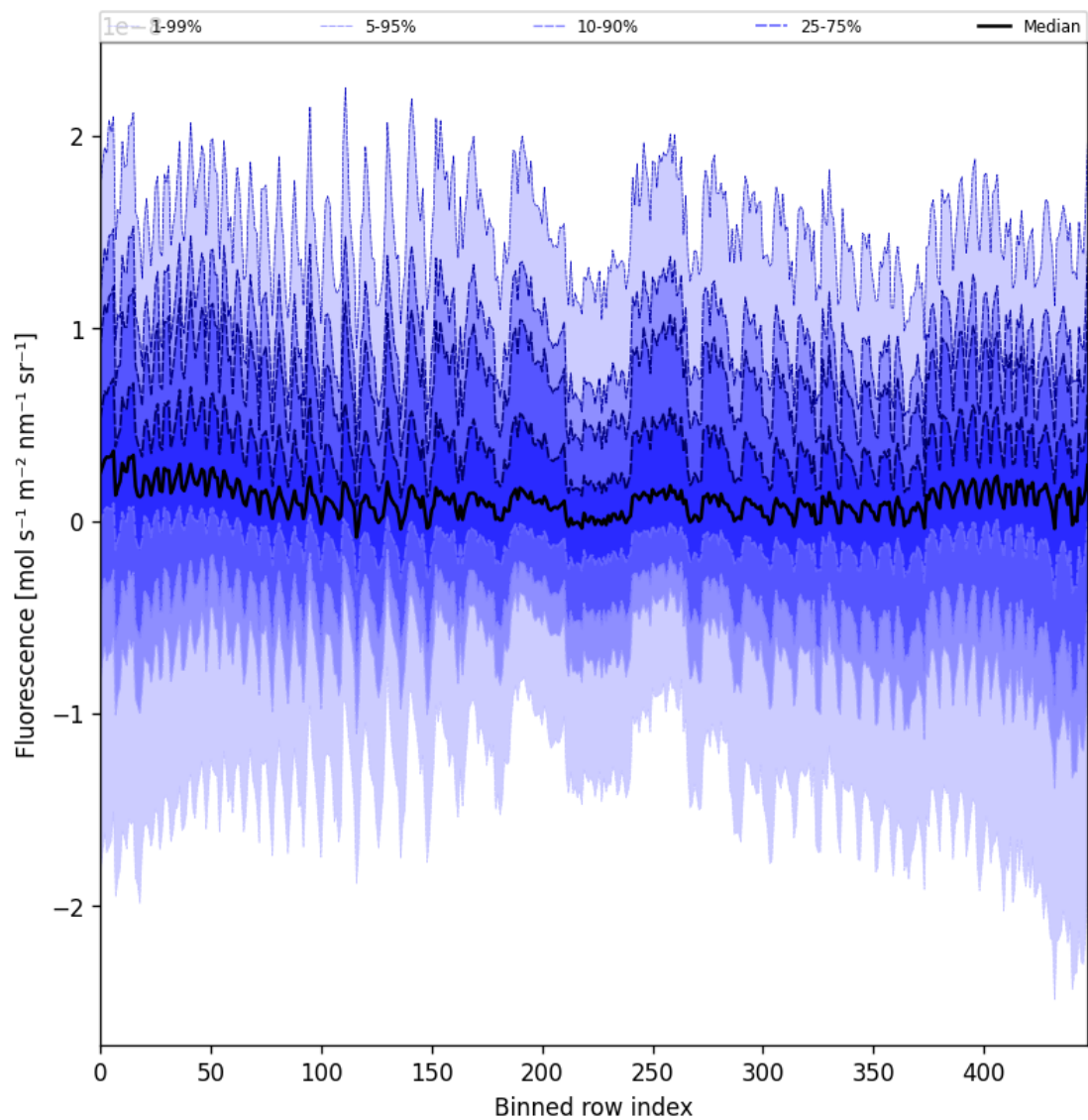
Figure 55: Along track statistics of “Fluorescence” for 2025-06-07 to 2025-06-08
