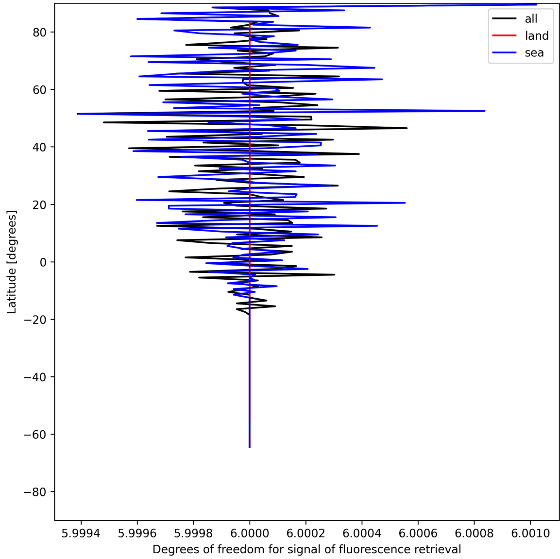
Figure 24: Zonal average of “Degrees of freedom for signal of fluorescence retrieval” for 2025-06-07 to 2025-06-08.
