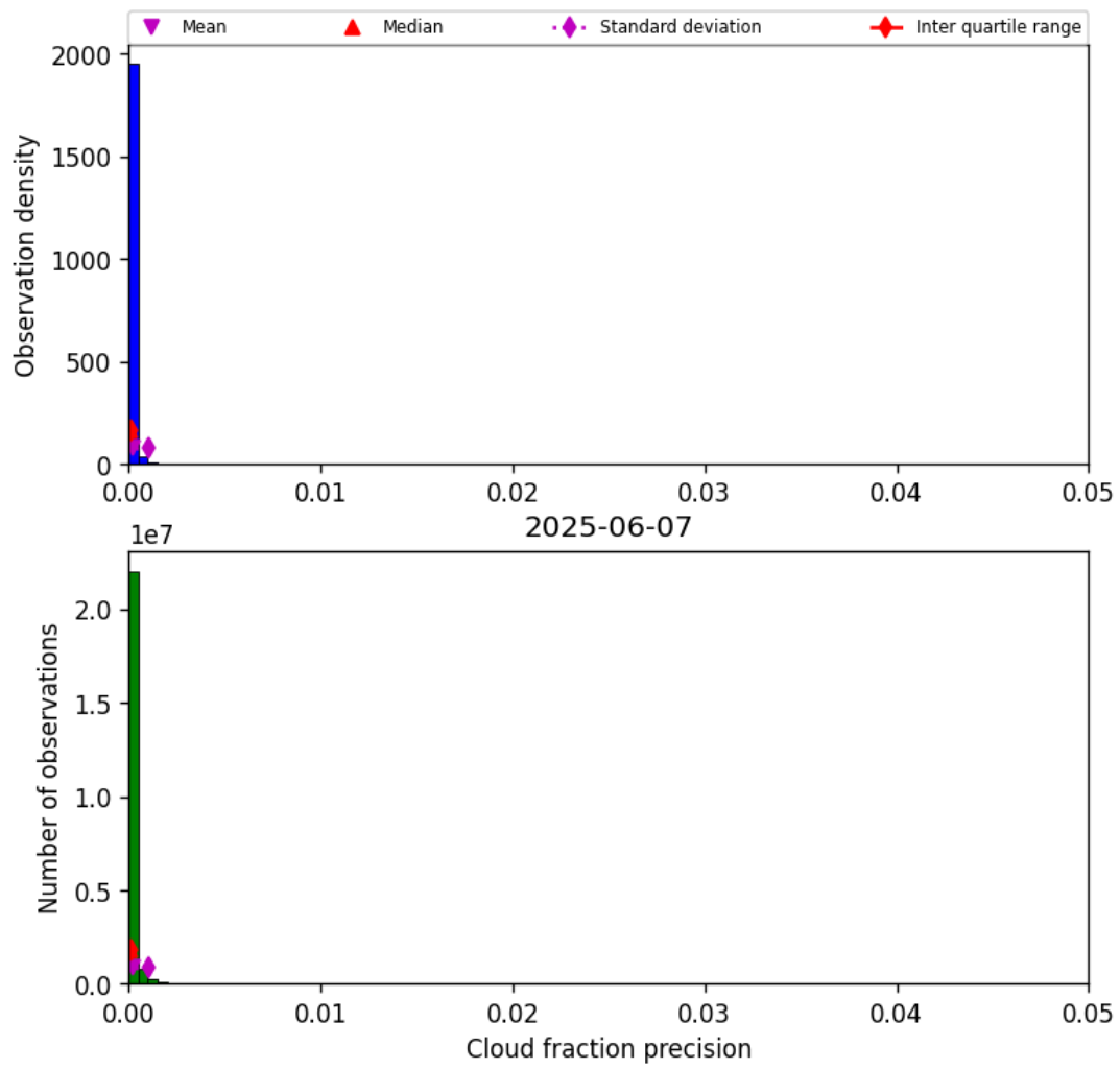
Figure 31: Histogram of “Cloud fraction precision” for 2025-06-07 to 2025-06-08
