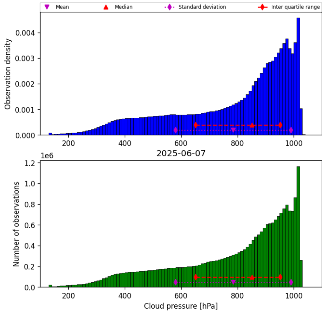
Figure 28: Histogram of “Cloud pressure” for 2025-06-07 to 2025-06-08
