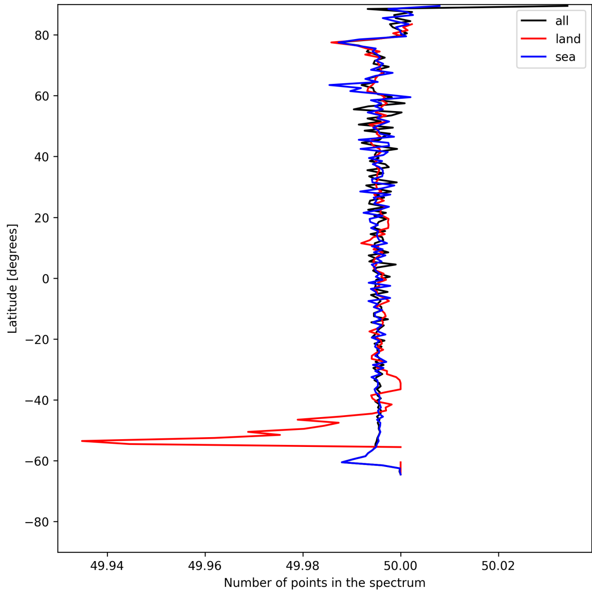
Figure 25: Zonal average of “Number of points in the spectrum” for 2025-06-07 to 2025-06-08.
