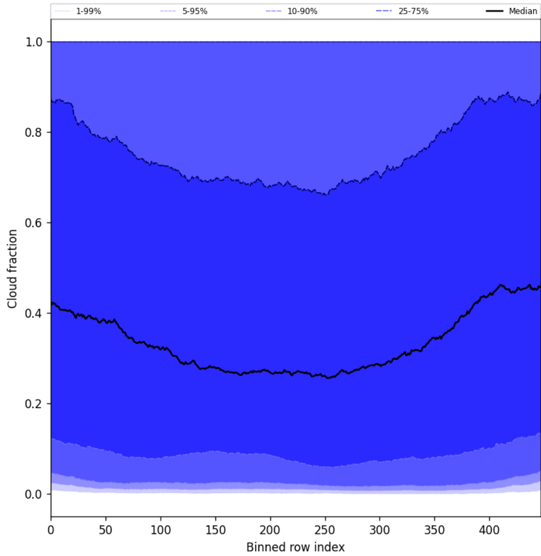
Figure 47: Along track statistics of “Cloud fraction” for 2025-06-07 to 2025-06-08
