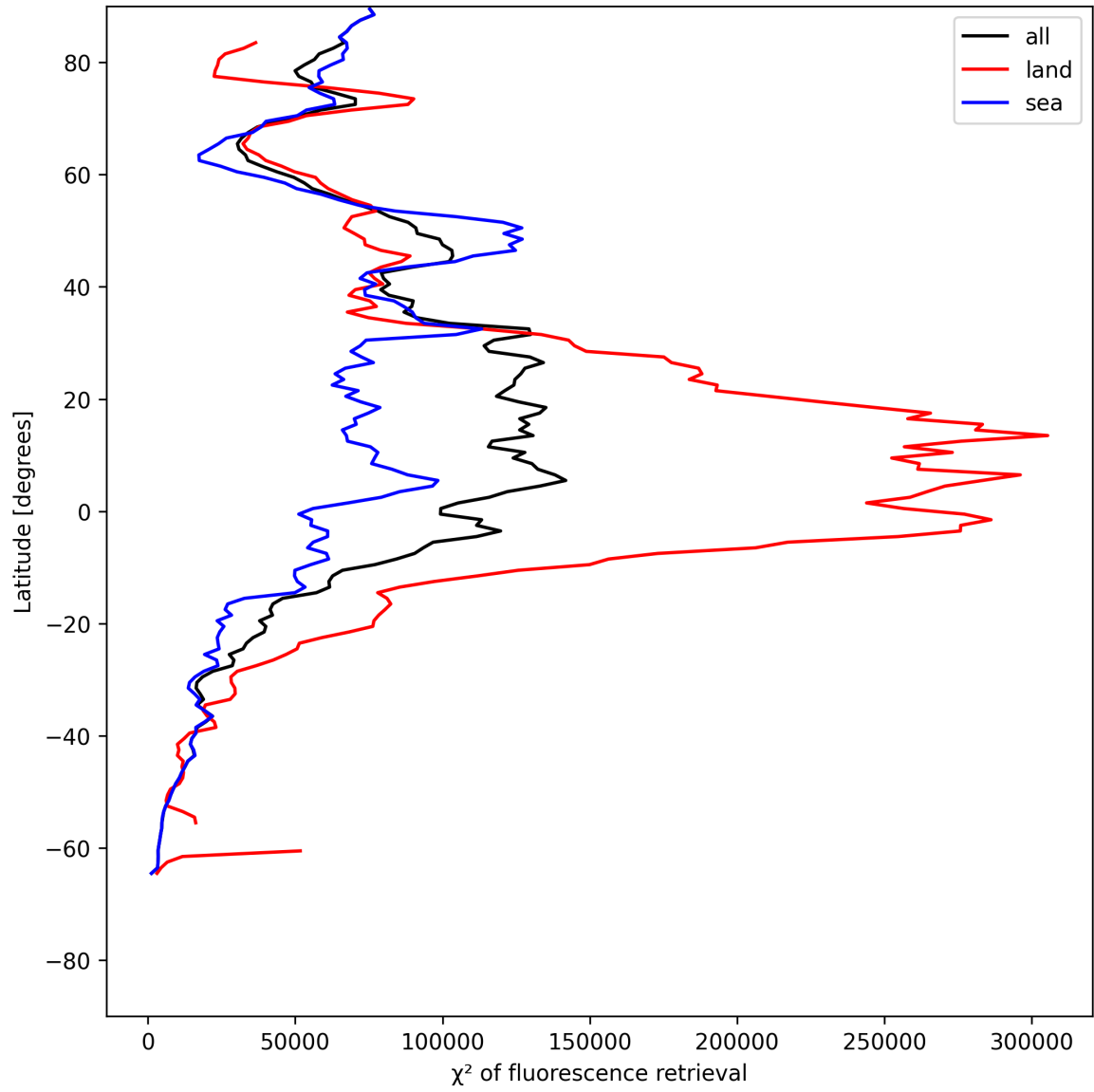
Figure 23: Zonal average of “ \chi^2 of fluorescence retrieval” for 2025-06-07 to 2025-06-08.
