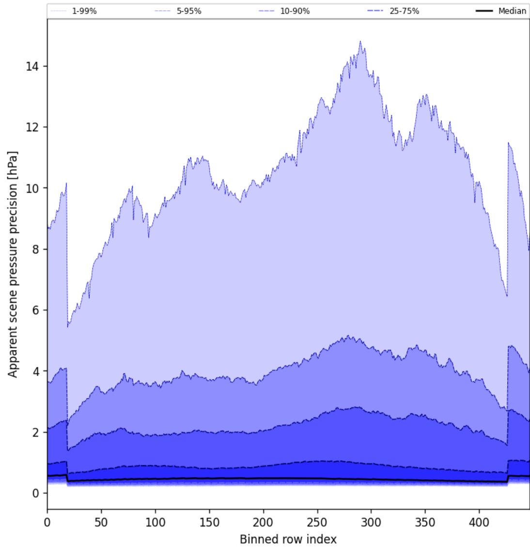
Figure 52: Along track statistics of “Apparent scene pressure precision” for 2025-06-07 to 2025-06-08
