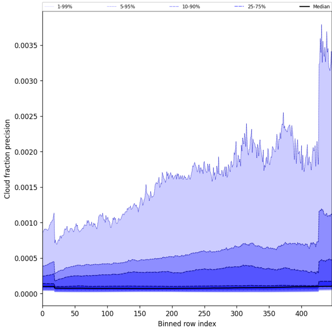
Figure 48: Along track statistics of “Cloud fraction precision” for 2025-06-07 to 2025-06-08
