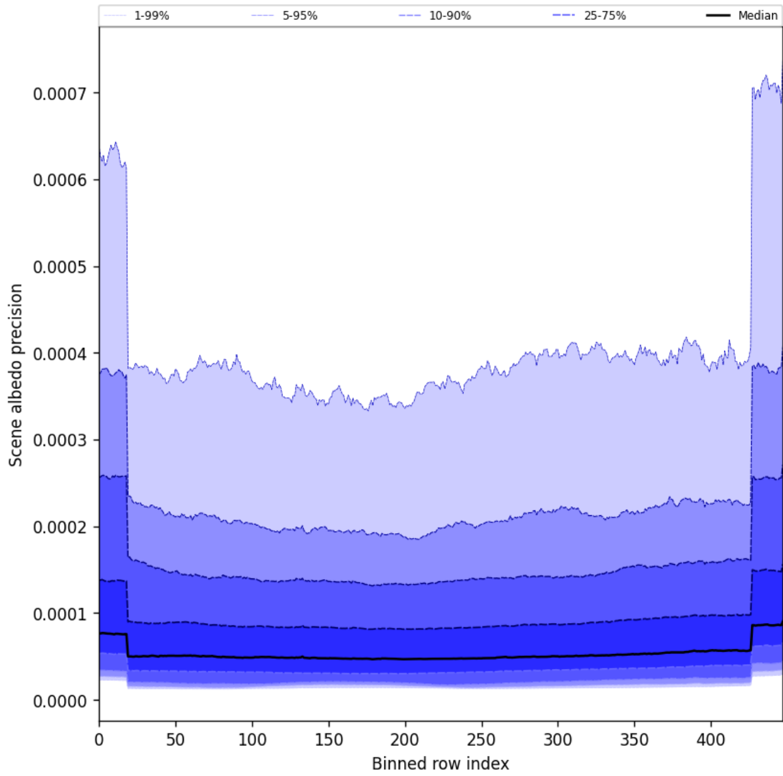
Figure 50: Along track statistics of “Scene albedo precision” for 2025-06-07 to 2025-06-08
