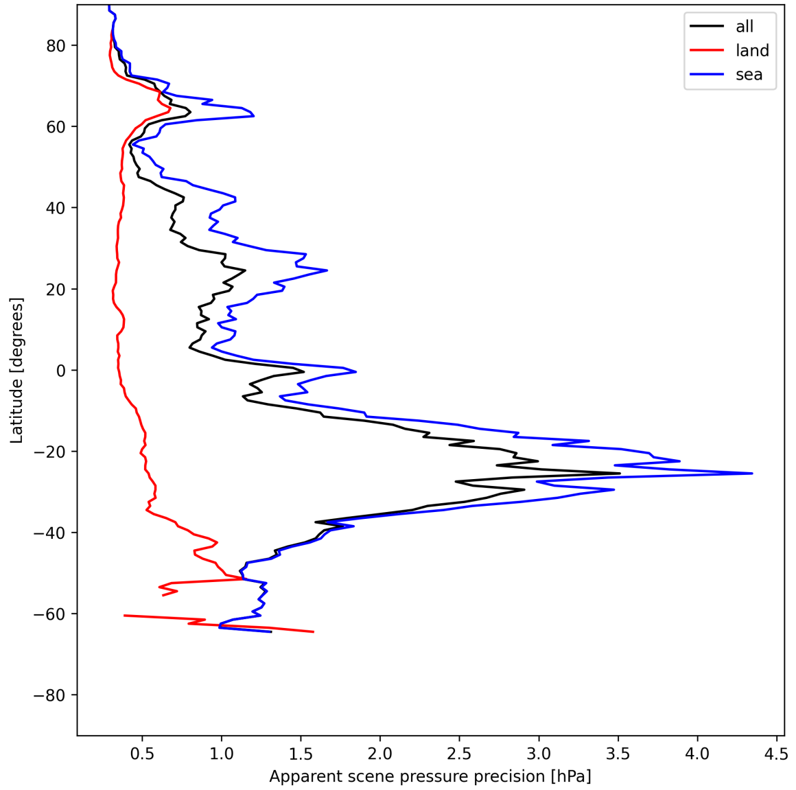
Figure 18: Zonal average of “Apparent scene pressure precision” for 2025-06-07 to 2025-06-08.
