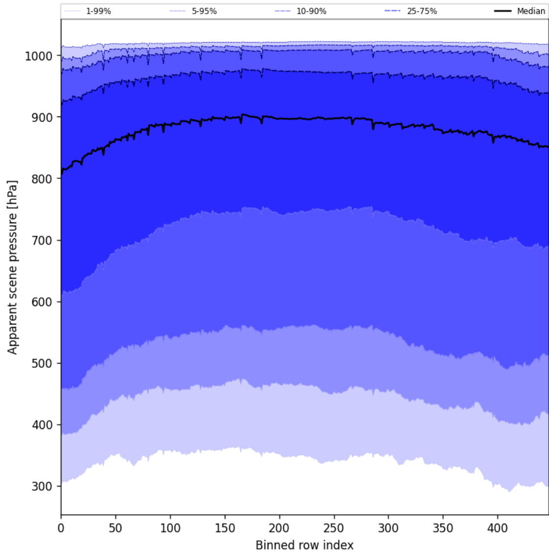
Figure 51: Along track statistics of “Apparent scene pressure” for 2025-06-07 to 2025-06-08
