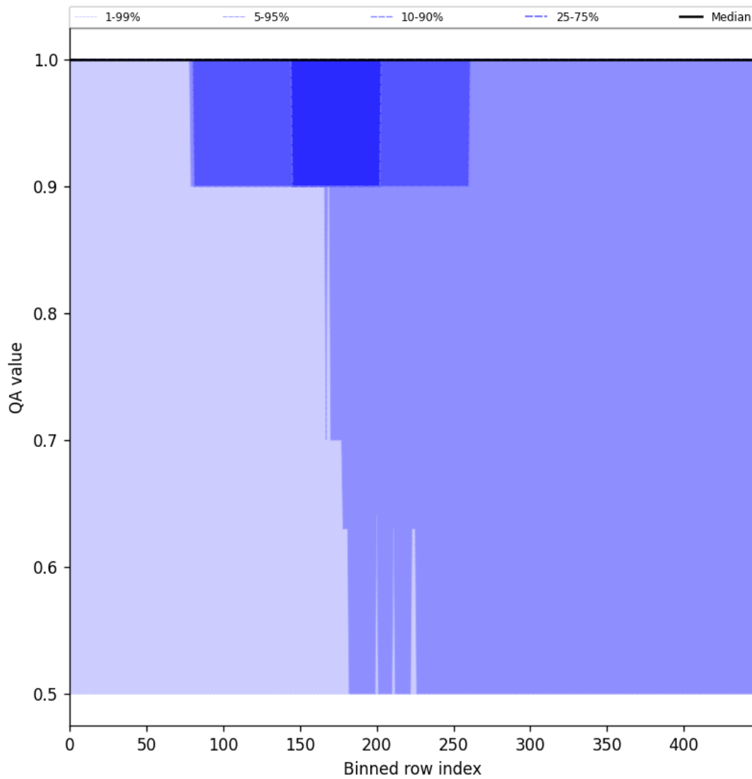
Figure 44: Along track statistics of “QA value” for 2025-06-07 to 2025-06-08
