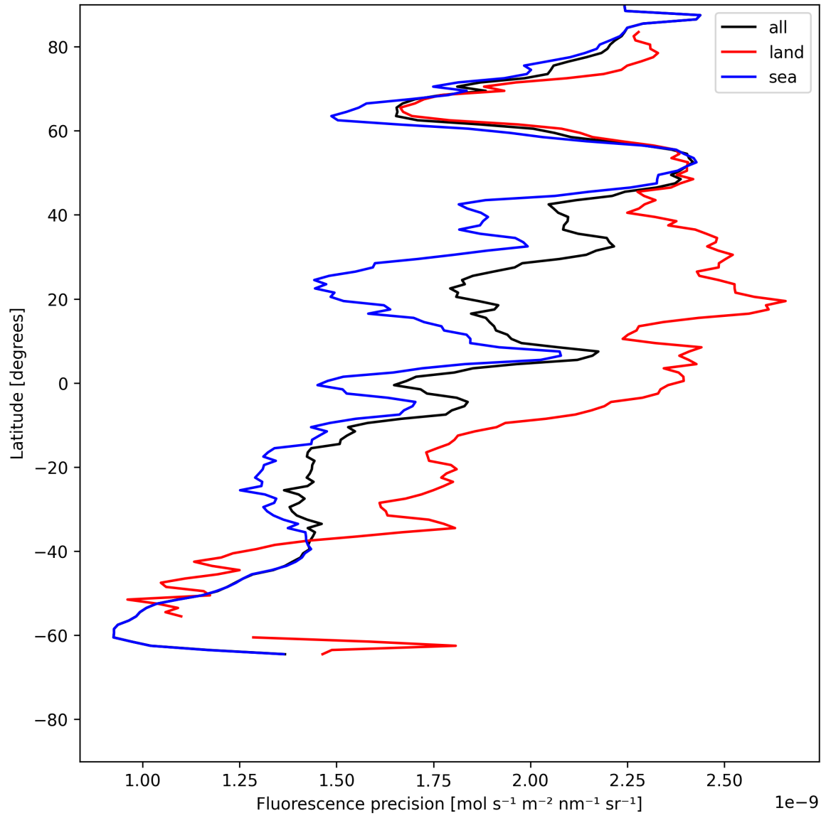
Figure 22: Zonal average of “Fluorescence precision” for 2025-06-07 to 2025-06-08.
