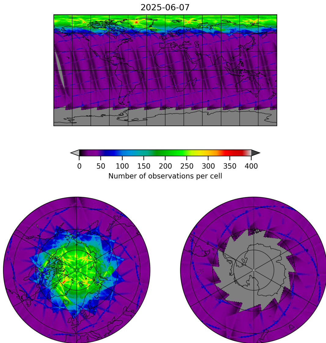
Figure 9: Map of the number of observations for 2025-06-07 to 2025-06-08
