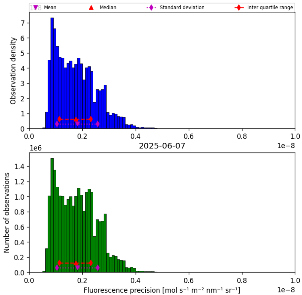
Figure 39: Histogram of “Fluorescence precision” for 2025-06-07 to 2025-06-08
