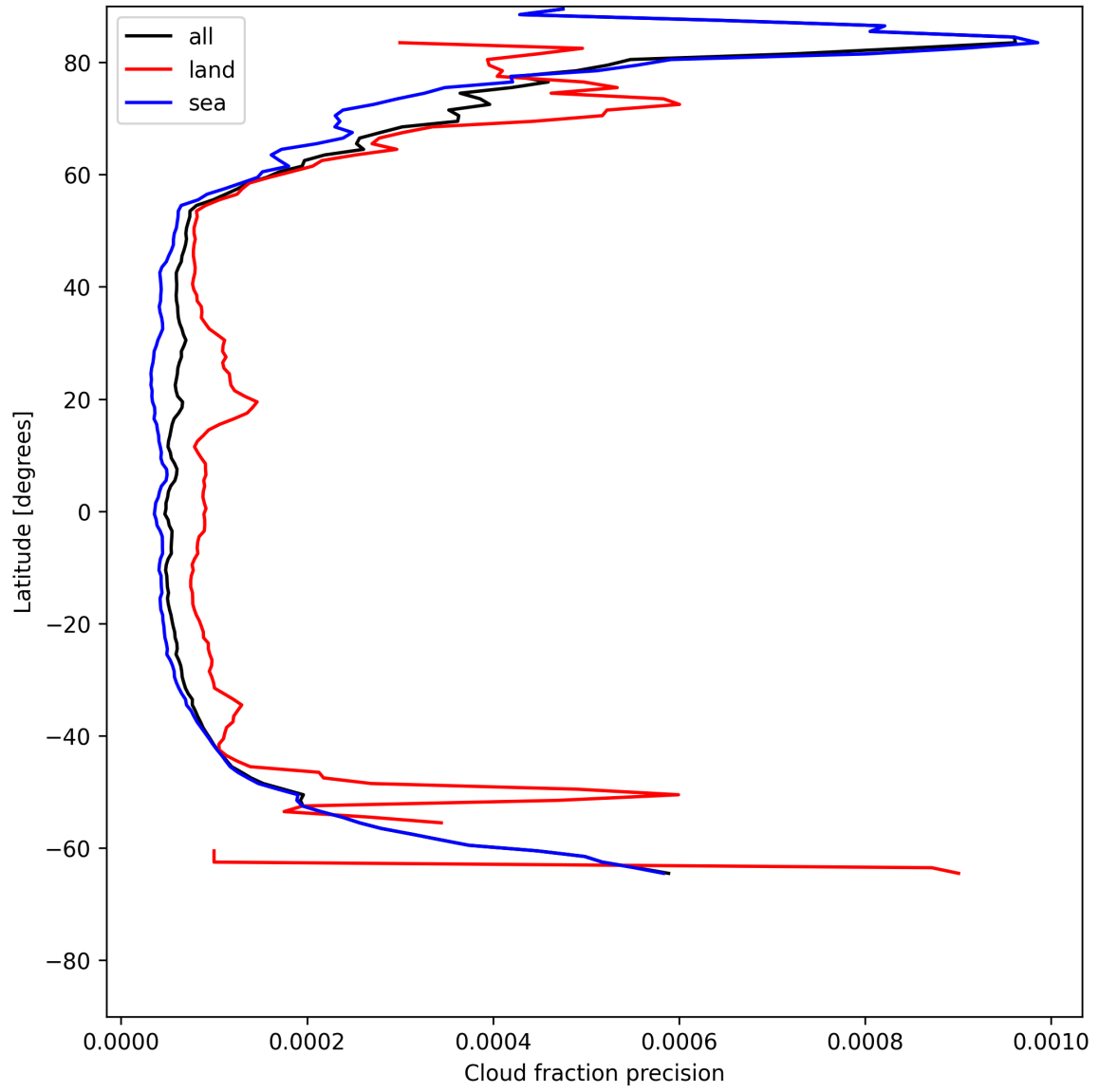
Figure 14: Zonal average of “Cloud fraction precision” for 2025-06-07 to 2025-06-08.
