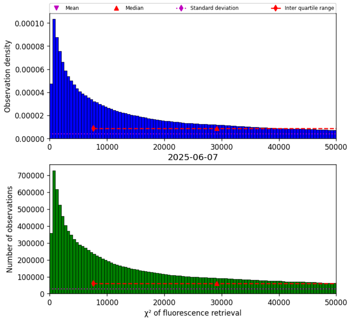
Figure 40: Histogram of “ \chi^2 of fluorescence retrieval” for 2025-06-07 to 2025-06-08
