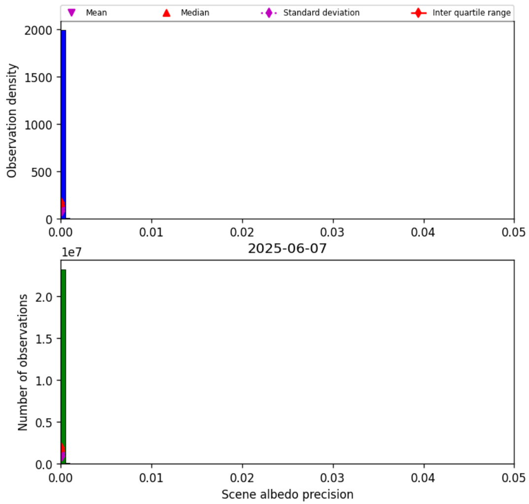
Figure 33: Histogram of “Scene albedo precision” for 2025-06-07 to 2025-06-08
