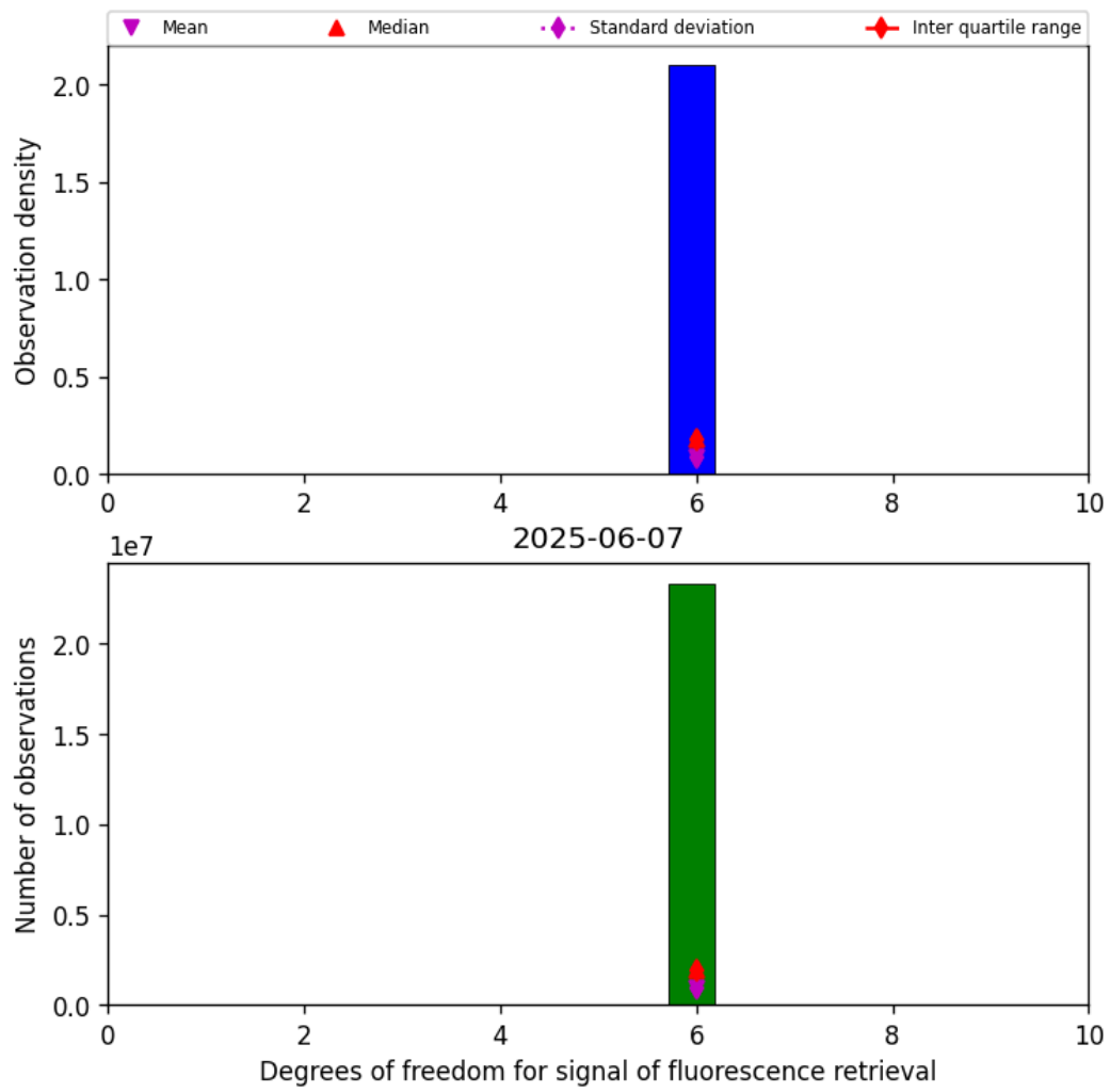
Figure 41: Histogram of “Degrees of freedom for signal of fluorescence retrieval” for 2025-06-07 to 2025-06-08
