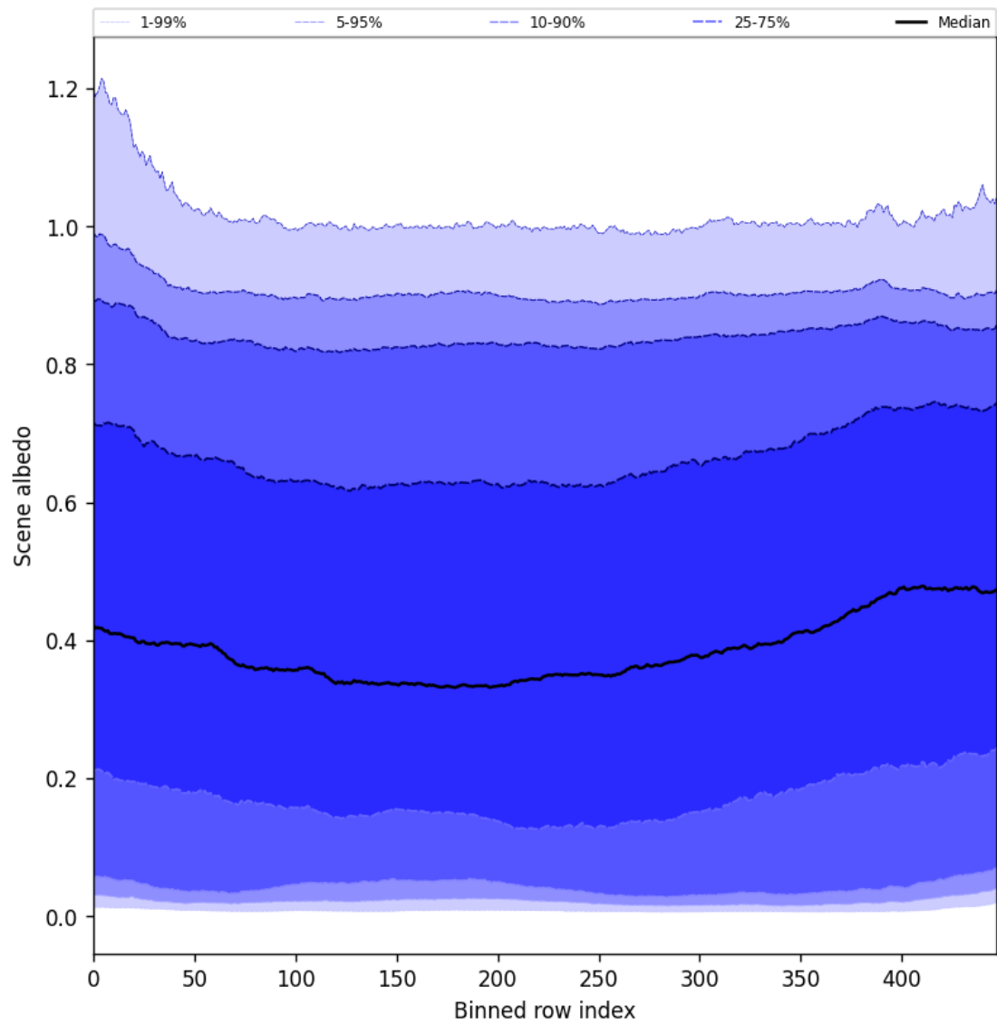
Figure 49: Along track statistics of “Scene albedo” for 2025-06-07 to 2025-06-08
