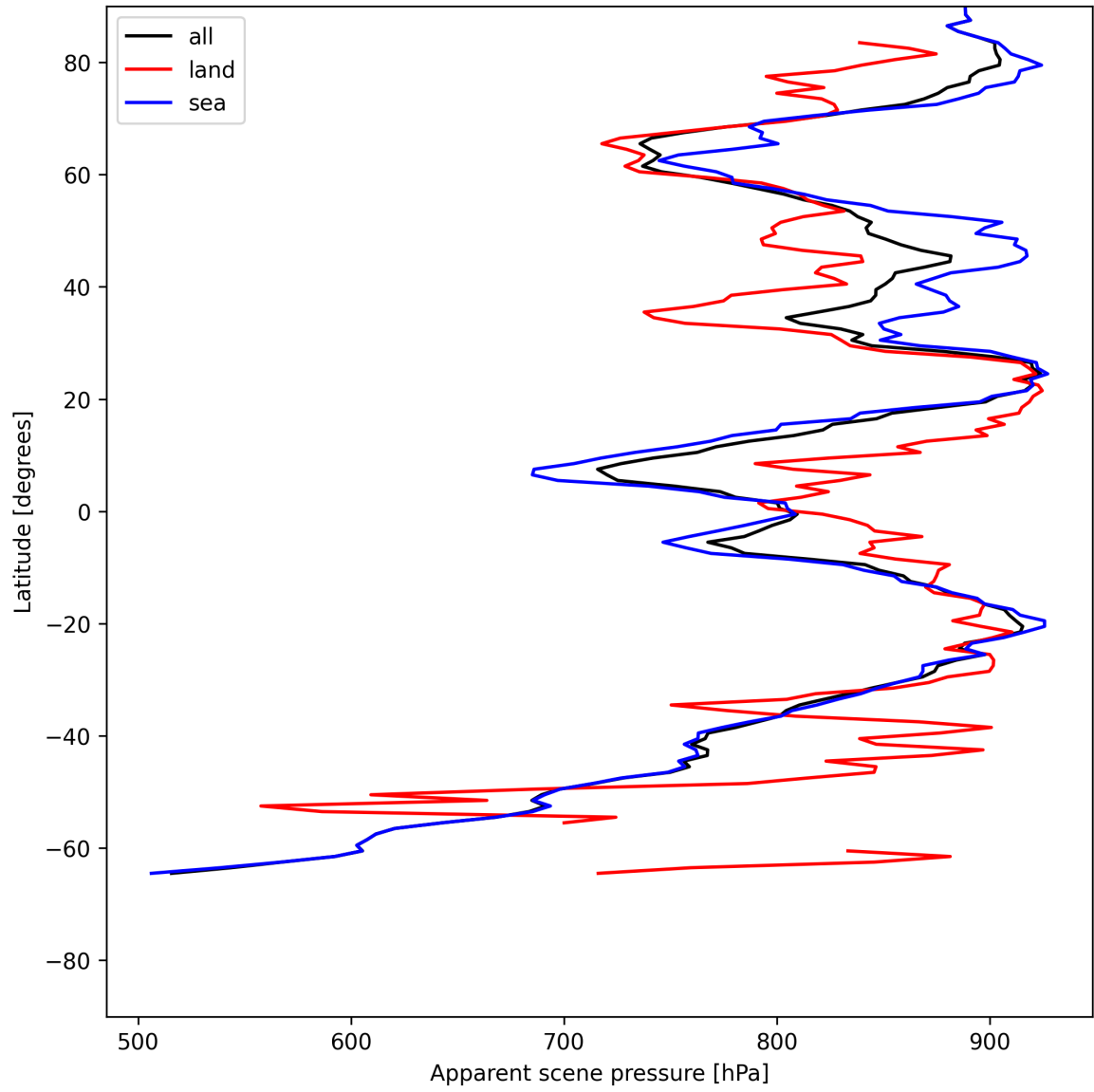
Figure 17: Zonal average of “Apparent scene pressure” for 2025-06-07 to 2025-06-08.
