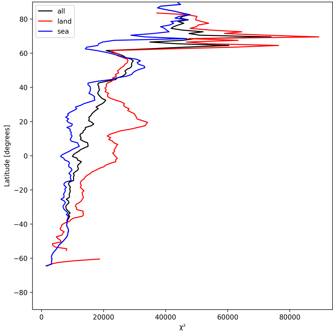
Figure 19: Zonal average of “ \chi^2 ” for 2025-06-07 to 2025-06-08.
