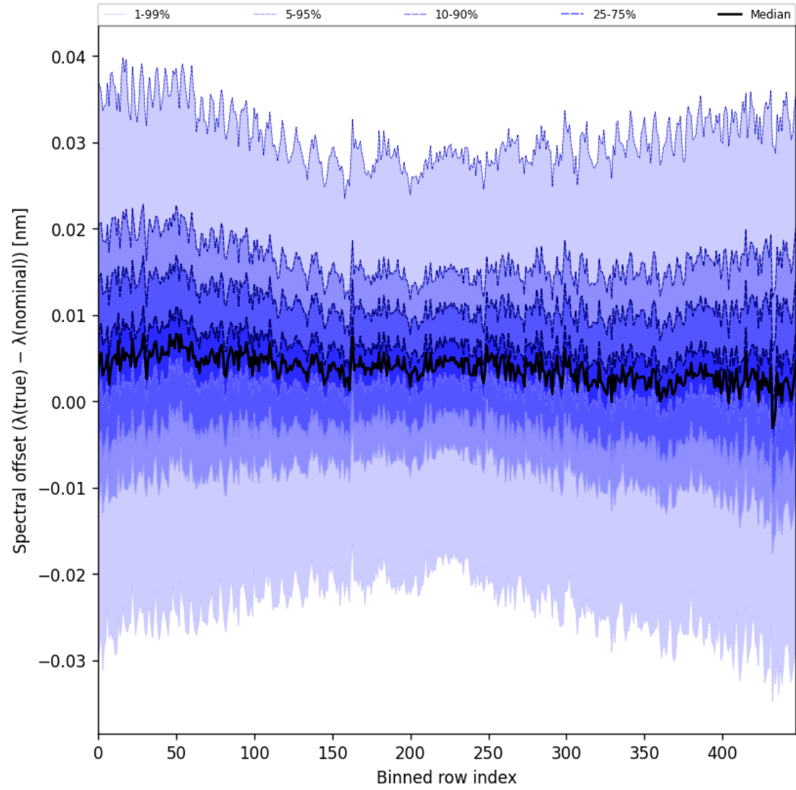
Figure 60: Along track statistics of “Spectral offset ( \lambda_{\text{true}} - \lambda_{\text{nominal}} )” for 2025-06-07 to 2025-06-08
