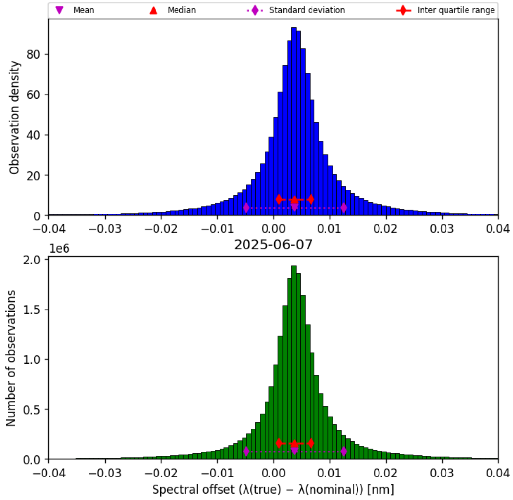
Figure 43: Histogram of “Spectral offset ( \lambda_{\text{true}} - \lambda_{\text{nominal}} )” for 2025-06-07 to 2025-06-08
