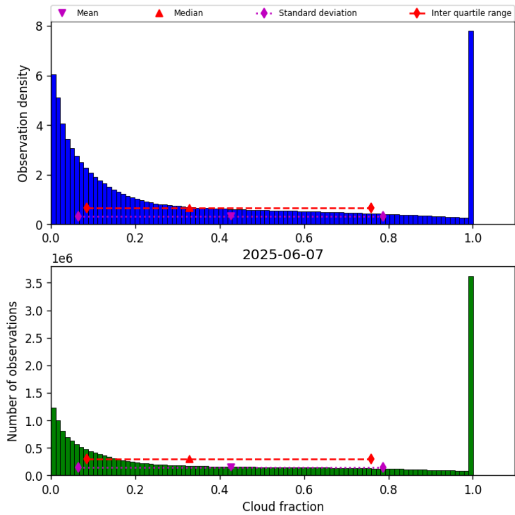
Figure 30: Histogram of “Cloud fraction” for 2025-06-07 to 2025-06-08
