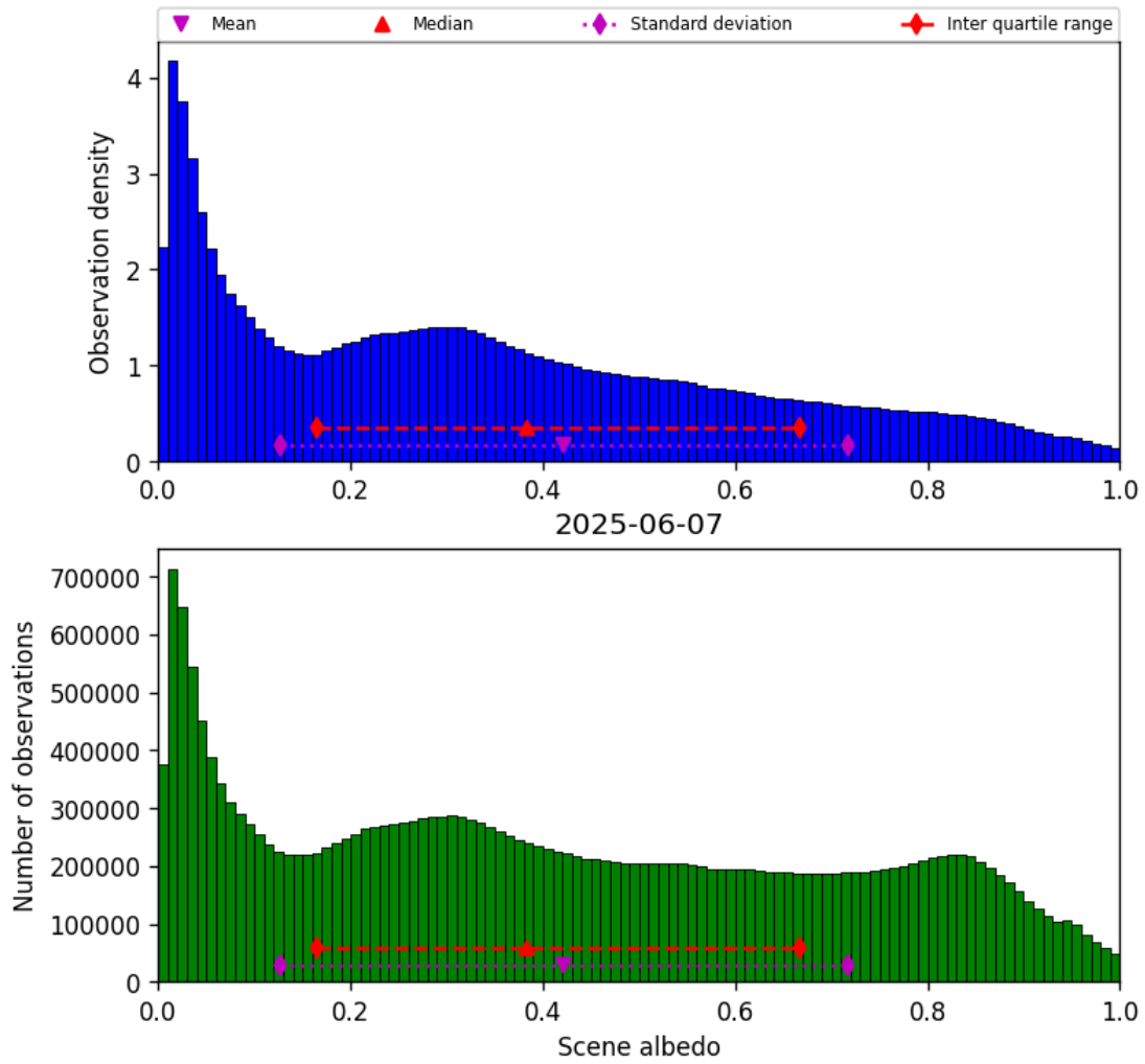
Figure 32: Histogram of “Scene albedo” for 2025-06-07 to 2025-06-08
