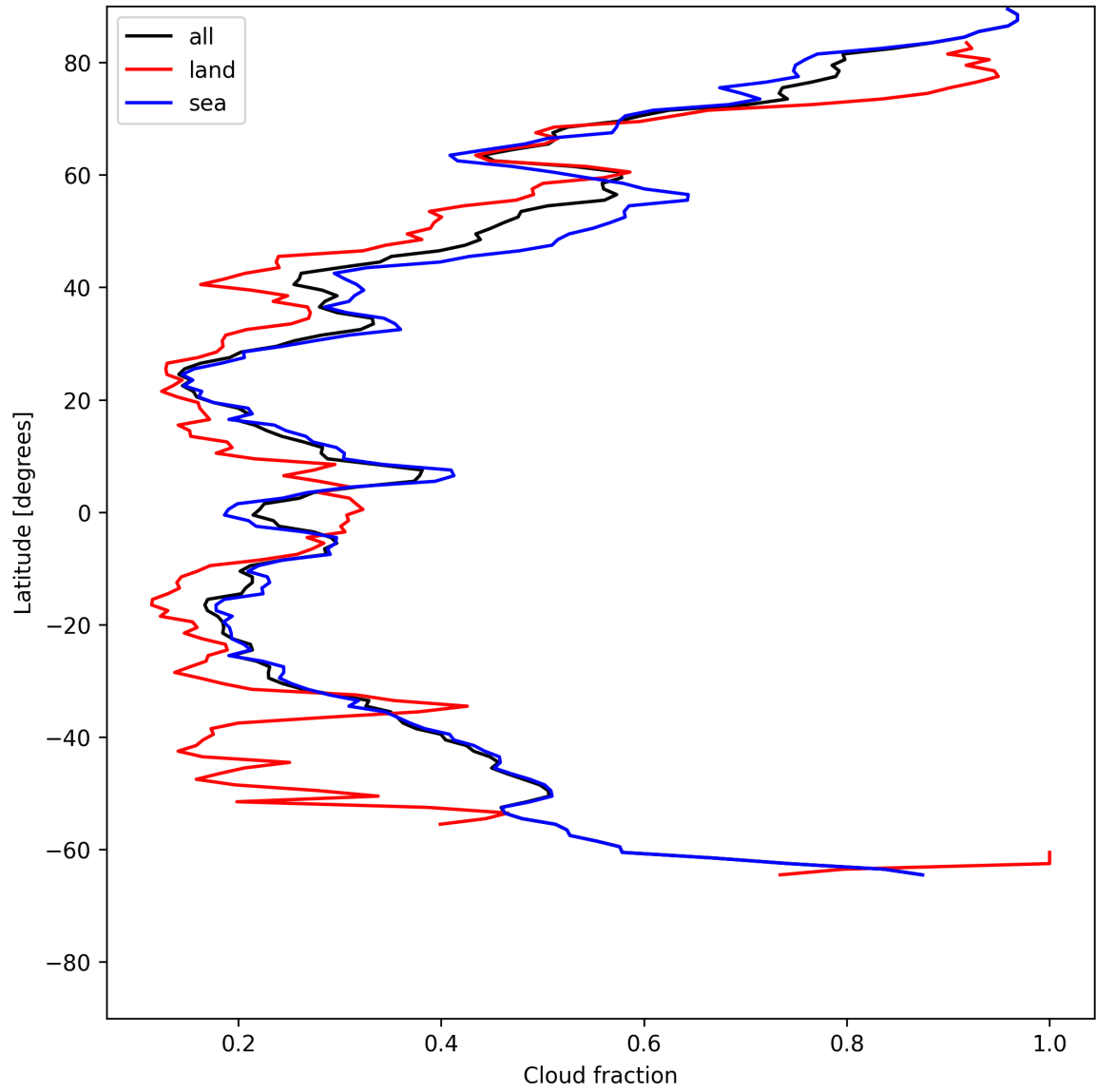
Figure 13: Zonal average of “Cloud fraction” for 2025-06-07 to 2025-06-08.
