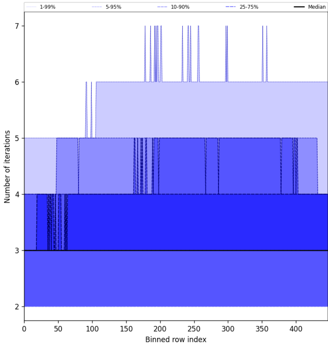
Figure 54: Along track statistics of “Number of iterations” for 2025-06-07 to 2025-06-08
