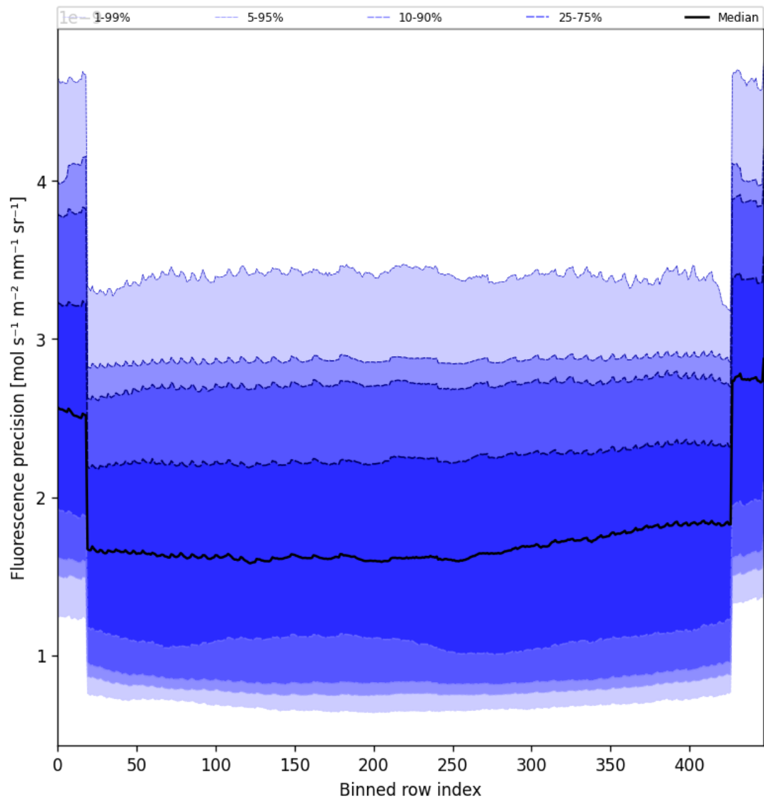
Figure 56: Along track statistics of “Fluorescence precision” for 2025-06-07 to 2025-06-08
