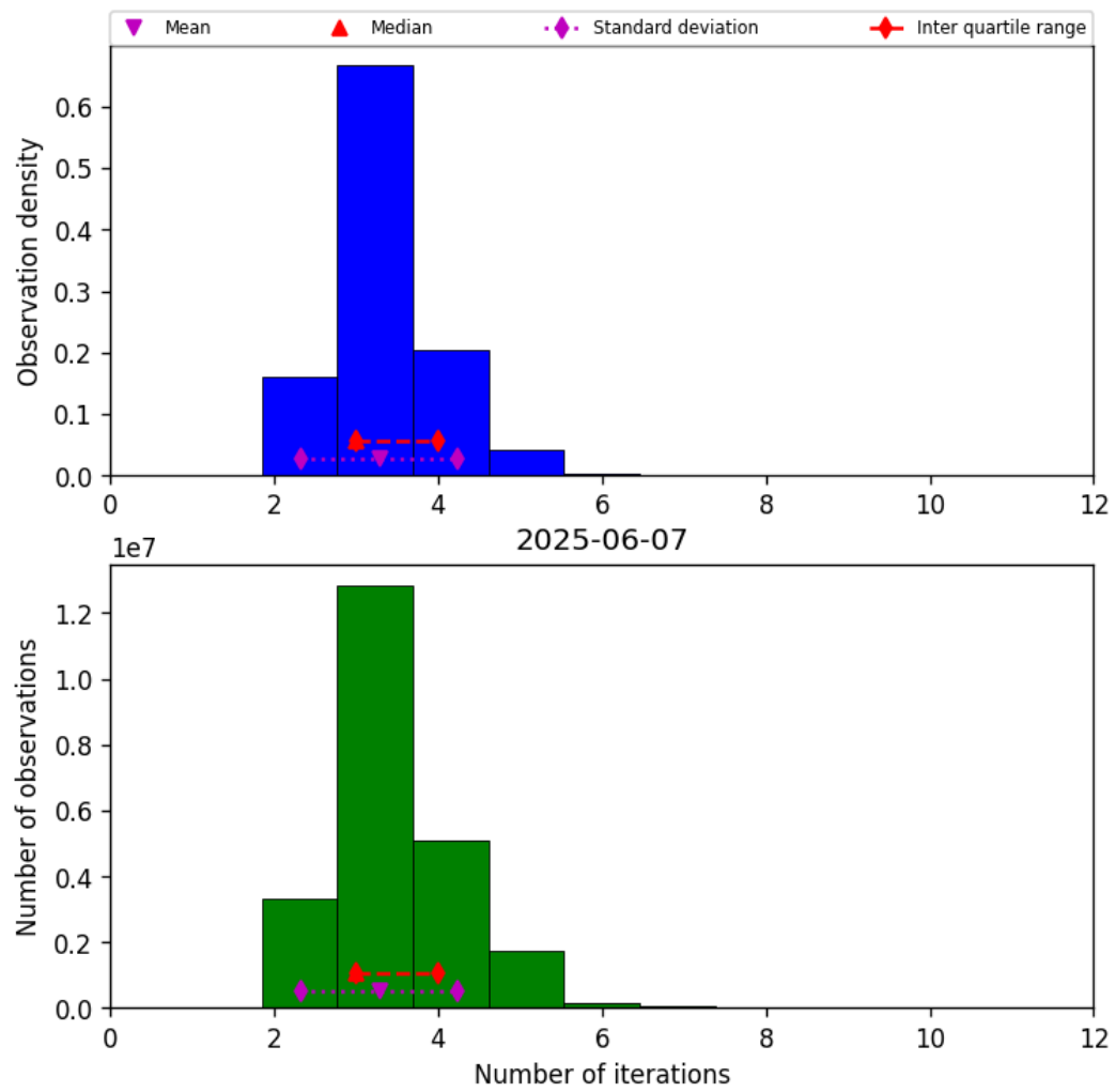
Figure 37: Histogram of “Number of iterations” for 2025-06-07 to 2025-06-08
