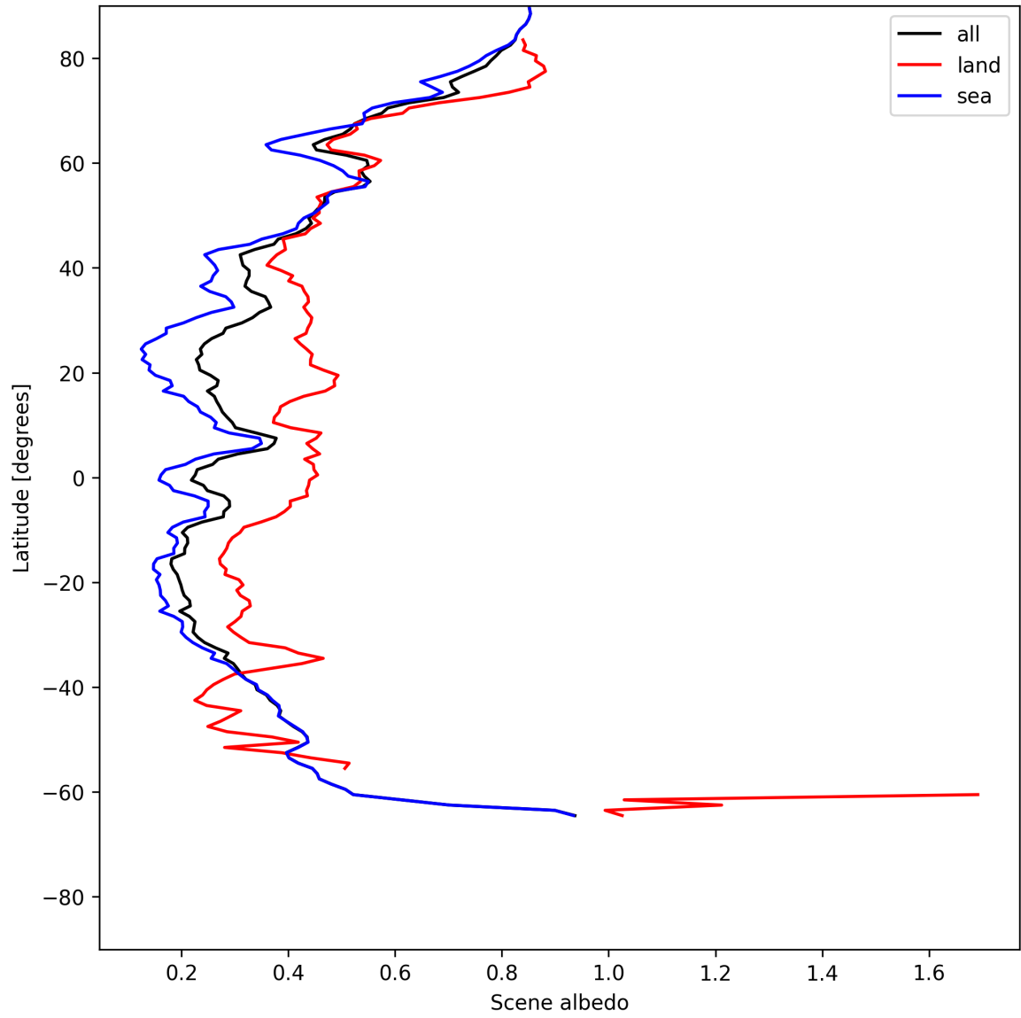
Figure 15: Zonal average of “Scene albedo” for 2025-06-07 to 2025-06-08.
