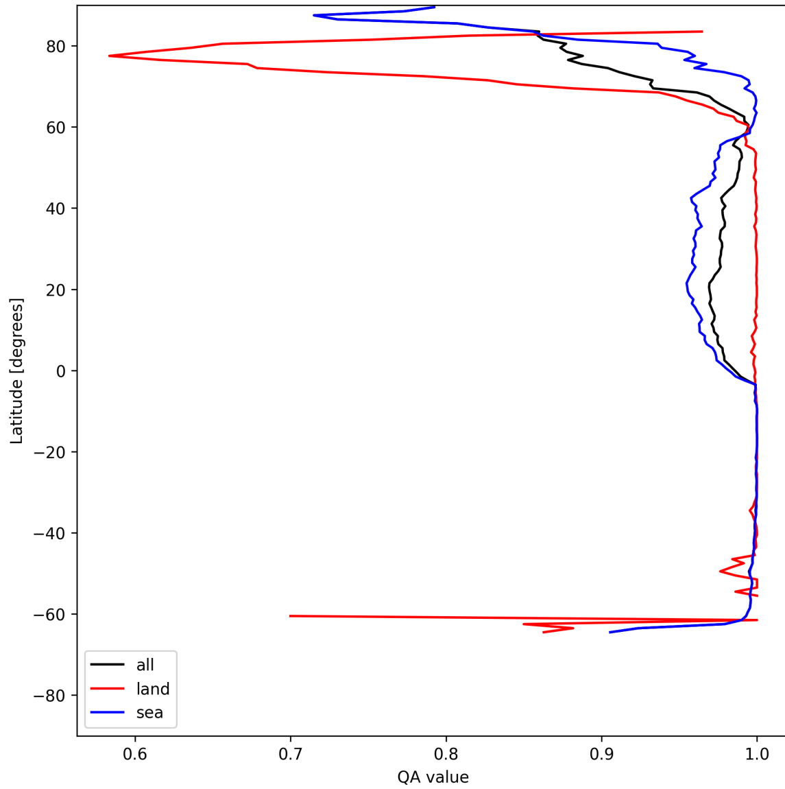
Figure 10: Zonal average of “QA value” for 2025-06-07 to 2025-06-08.
