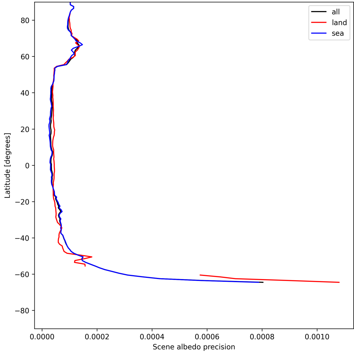
Figure 16: Zonal average of “Scene albedo precision” for 2025-06-07 to 2025-06-08.
