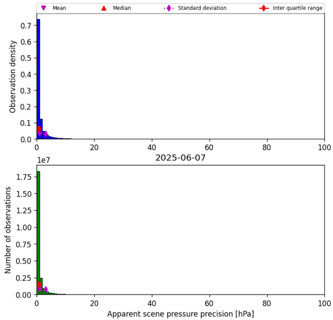
Figure 35: Histogram of “Apparent scene pressure precision” for 2025-06-07 to 2025-06-08
