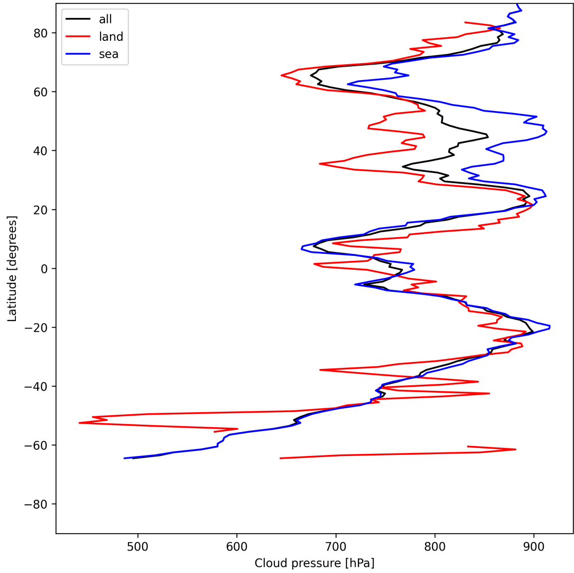
Figure 11: Zonal average of “Cloud pressure” for 2025-06-07 to 2025-06-08.
