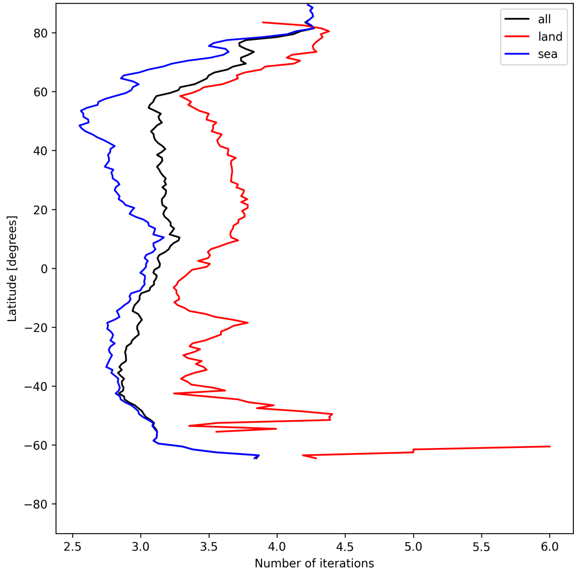
Figure 20: Zonal average of “Number of iterations” for 2025-06-07 to 2025-06-08.
