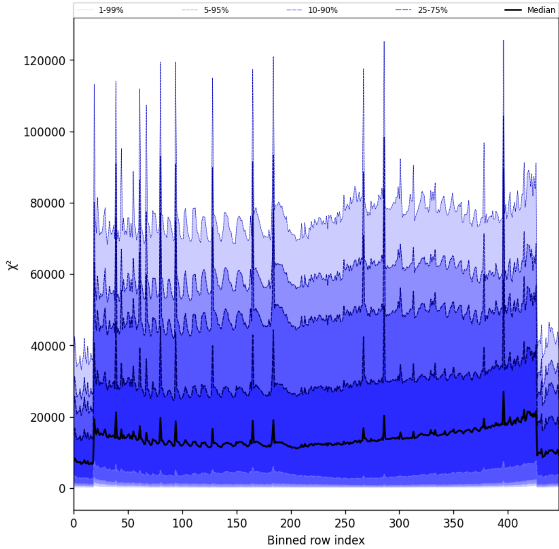
Figure 53: Along track statistics of “ \chi^2 ” for 2025-06-07 to 2025-06-08
