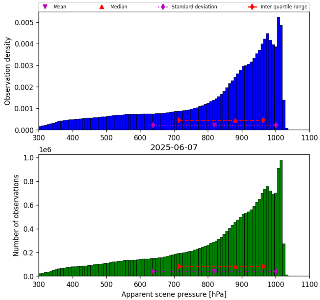
Figure 34: Histogram of “Apparent scene pressure” for 2025-06-07 to 2025-06-08
