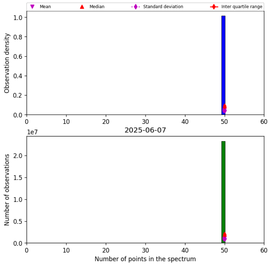
Figure 42: Histogram of “Number of points in the spectrum” for 2025-06-07 to 2025-06-08
