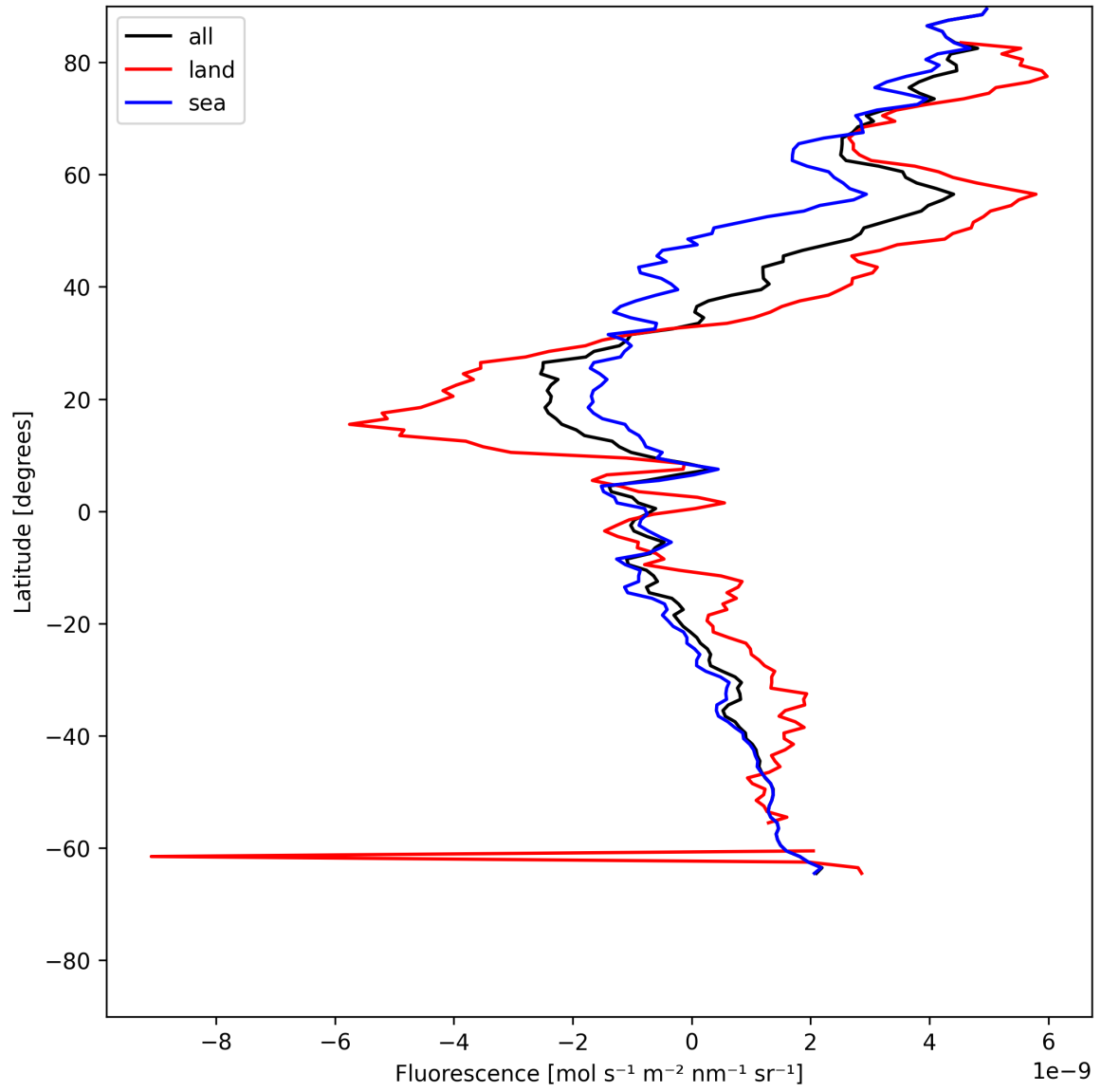
Figure 21: Zonal average of “Fluorescence” for 2025-06-07 to 2025-06-08.
