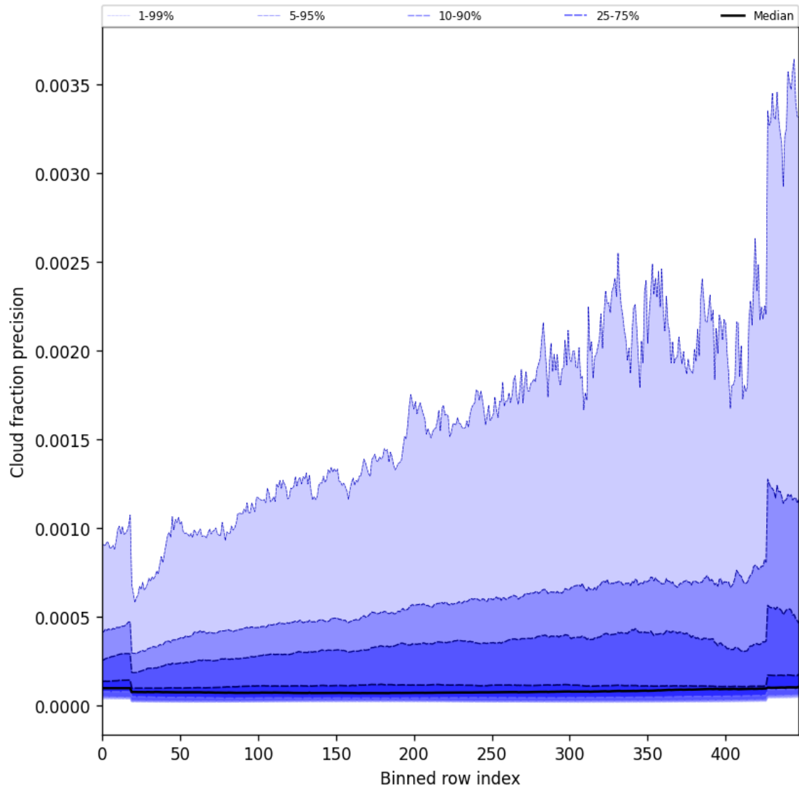
Figure 48: Along track statistics of “Cloud fraction precision” for 2025-06-08 to 2025-06-09
