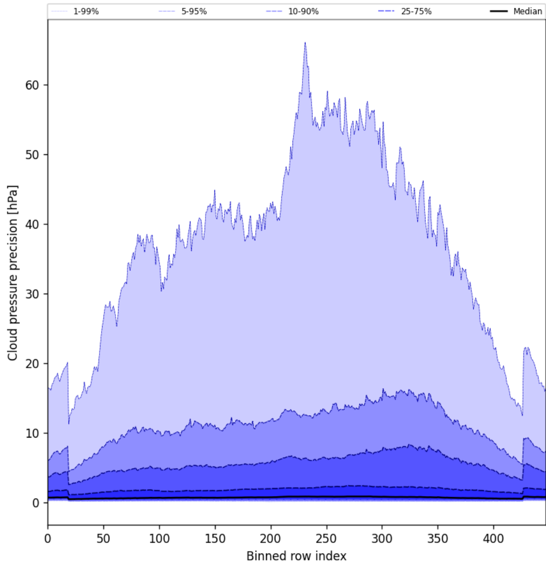
Figure 46: Along track statistics of “Cloud pressure precision” for 2025-06-08 to 2025-06-09
