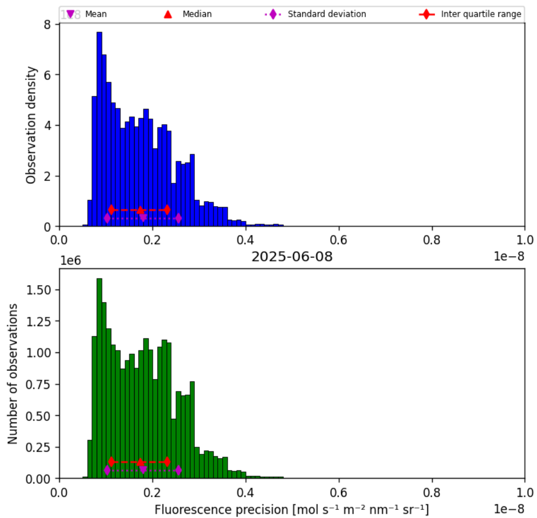
Figure 39: Histogram of “Fluorescence precision” for 2025-06-08 to 2025-06-09
