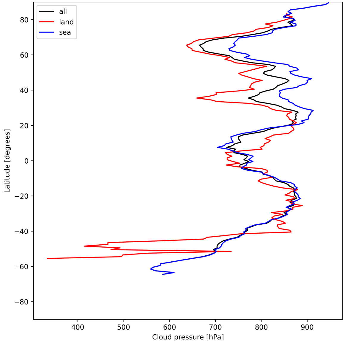
Figure 11: Zonal average of “Cloud pressure” for 2025-06-08 to 2025-06-09.
