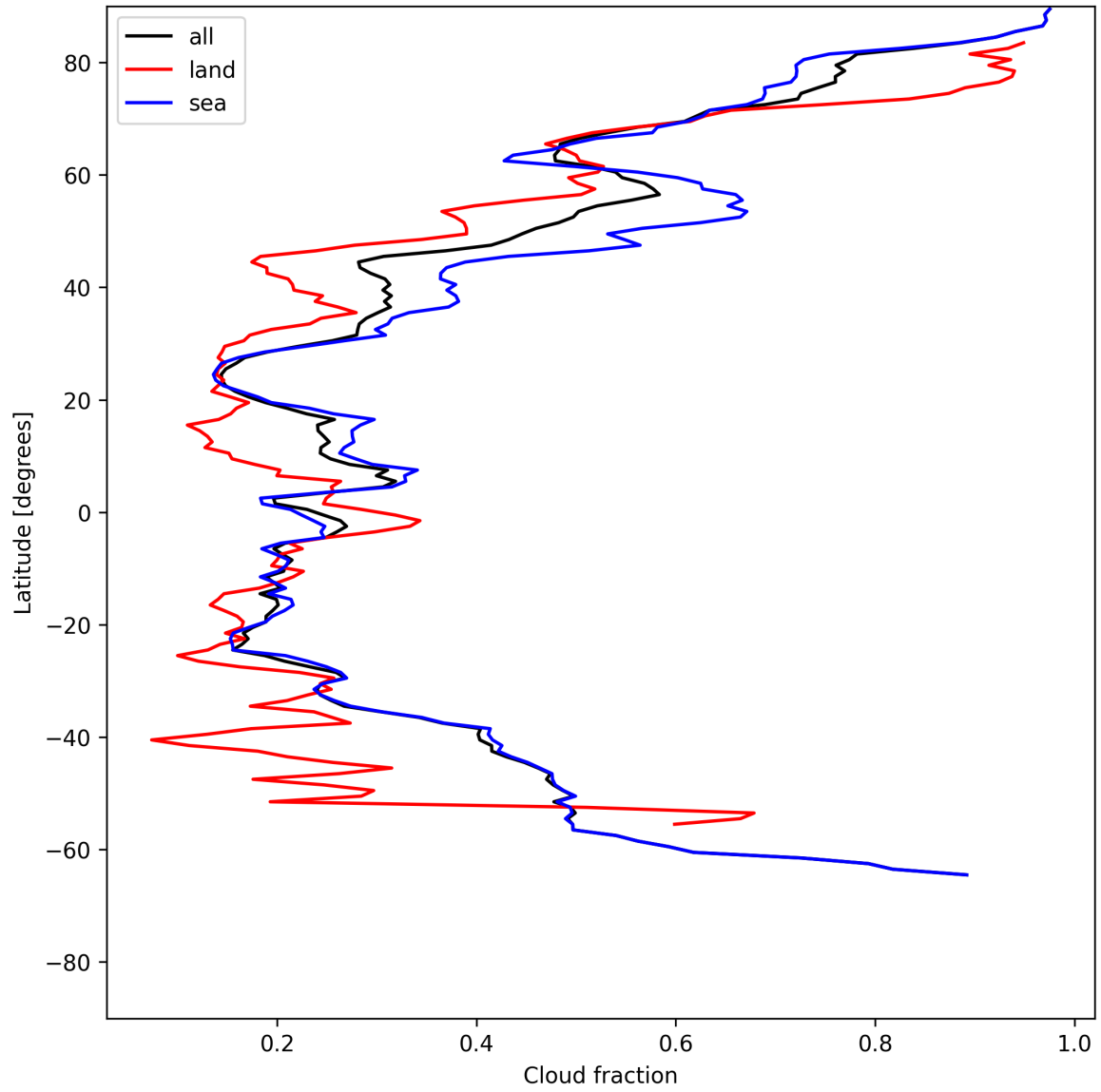
Figure 13: Zonal average of “Cloud fraction” for 2025-06-08 to 2025-06-09.
