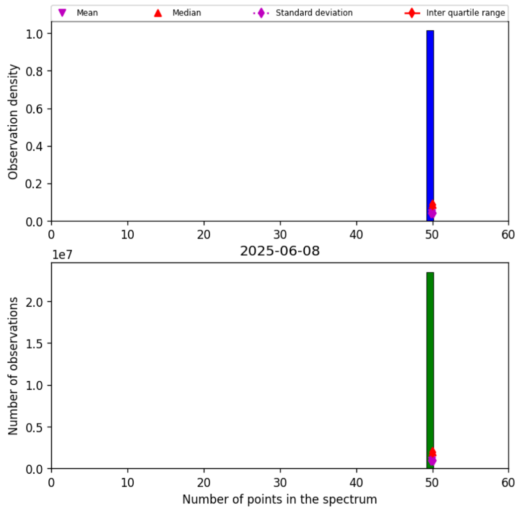
Figure 42: Histogram of “Number of points in the spectrum” for 2025-06-08 to 2025-06-09
