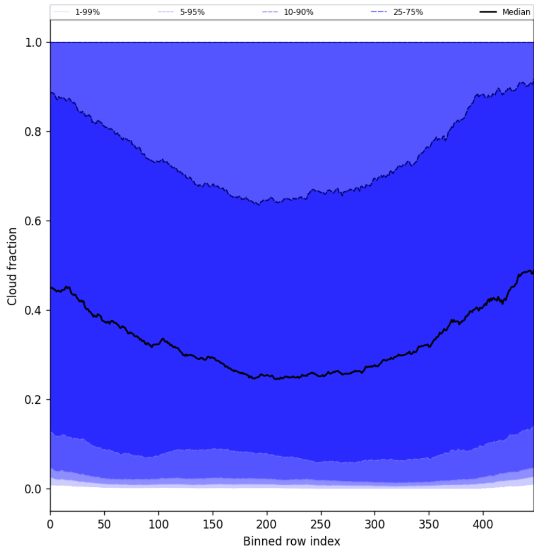
Figure 47: Along track statistics of “Cloud fraction” for 2025-06-08 to 2025-06-09
