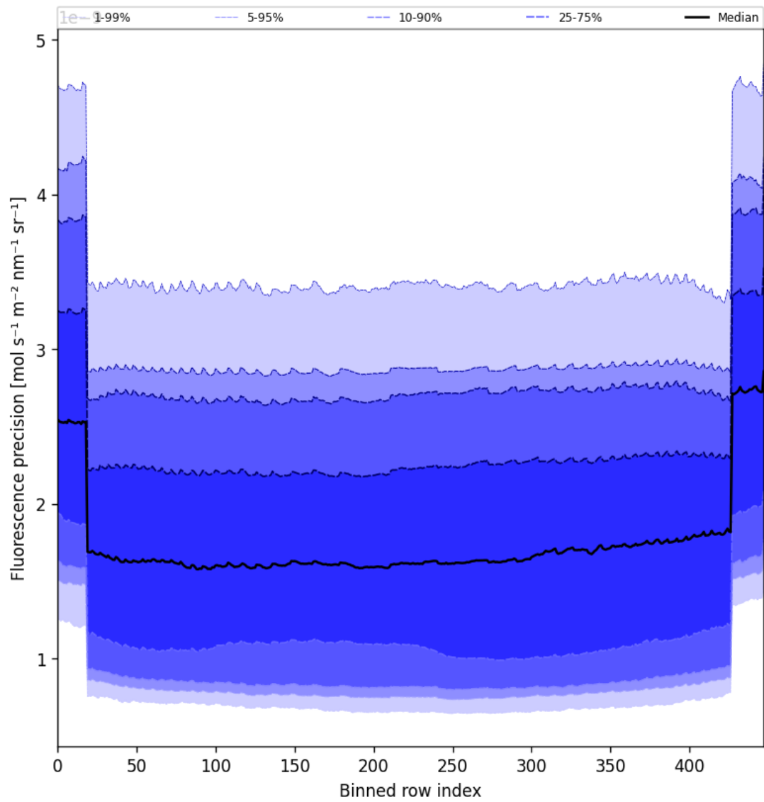
Figure 56: Along track statistics of “Fluorescence precision” for 2025-06-08 to 2025-06-09
