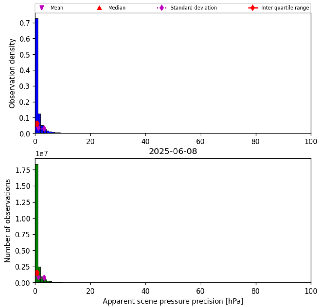
Figure 35: Histogram of “Apparent scene pressure precision” for 2025-06-08 to 2025-06-09
