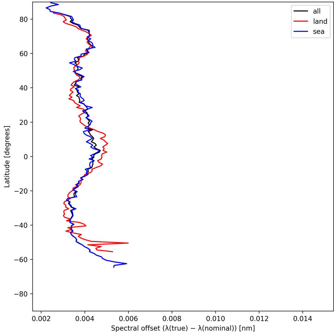
Figure 26: Zonal average of “Spectral offset ( \lambda_{\text{true}} - \lambda_{\text{nominal}} )” for 2025-06-08 to 2025-06-09.
