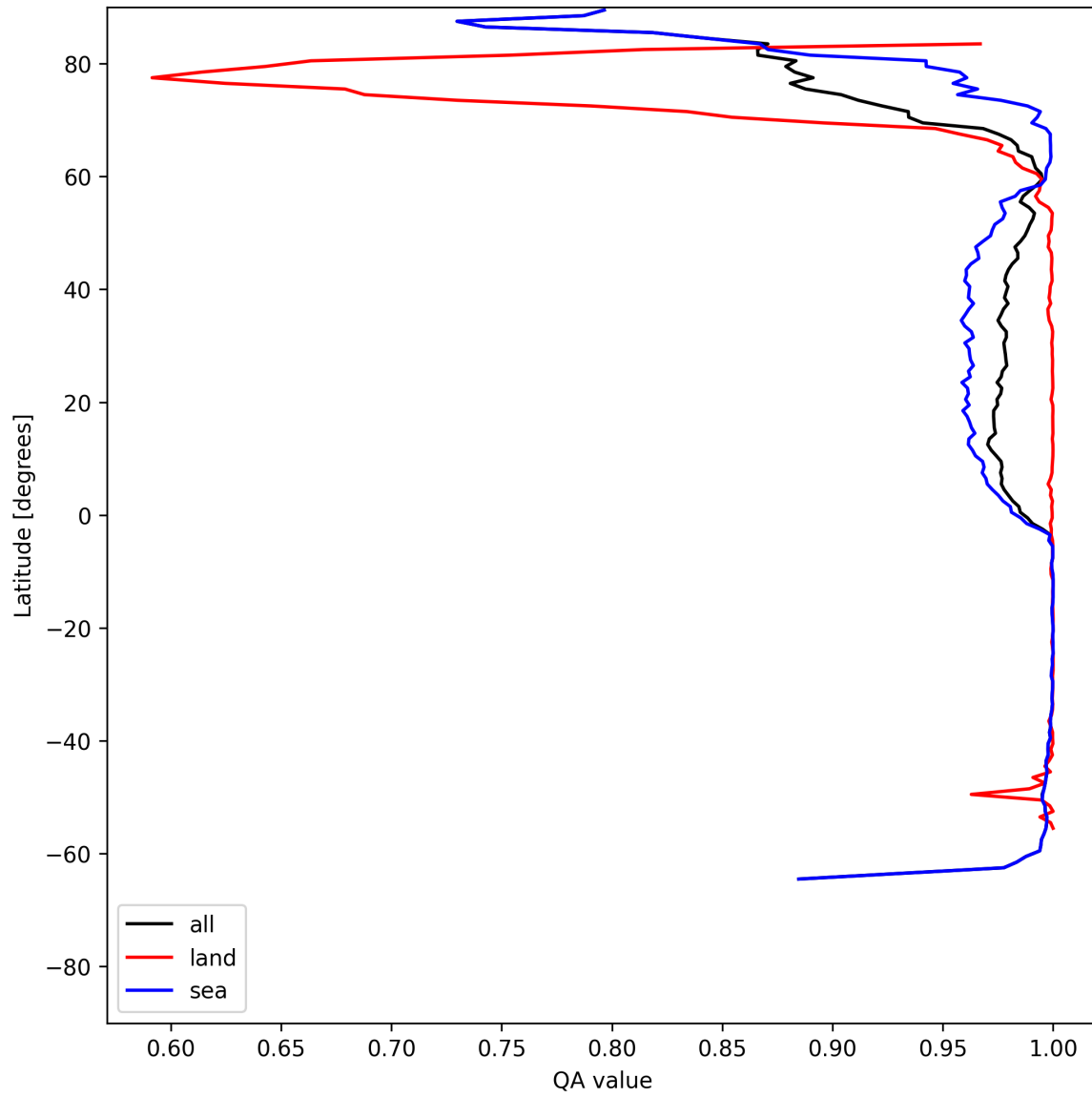
Figure 10: Zonal average of “QA value” for 2025-06-08 to 2025-06-09.
