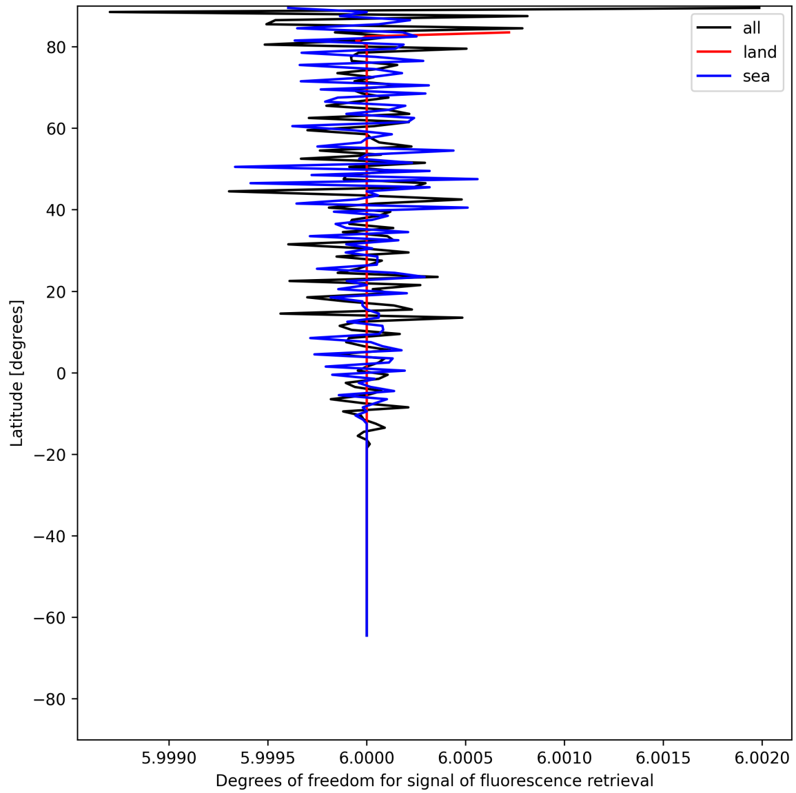
Figure 24: Zonal average of “Degrees of freedom for signal of fluorescence retrieval” for 2025-06-08 to 2025-06-09.
