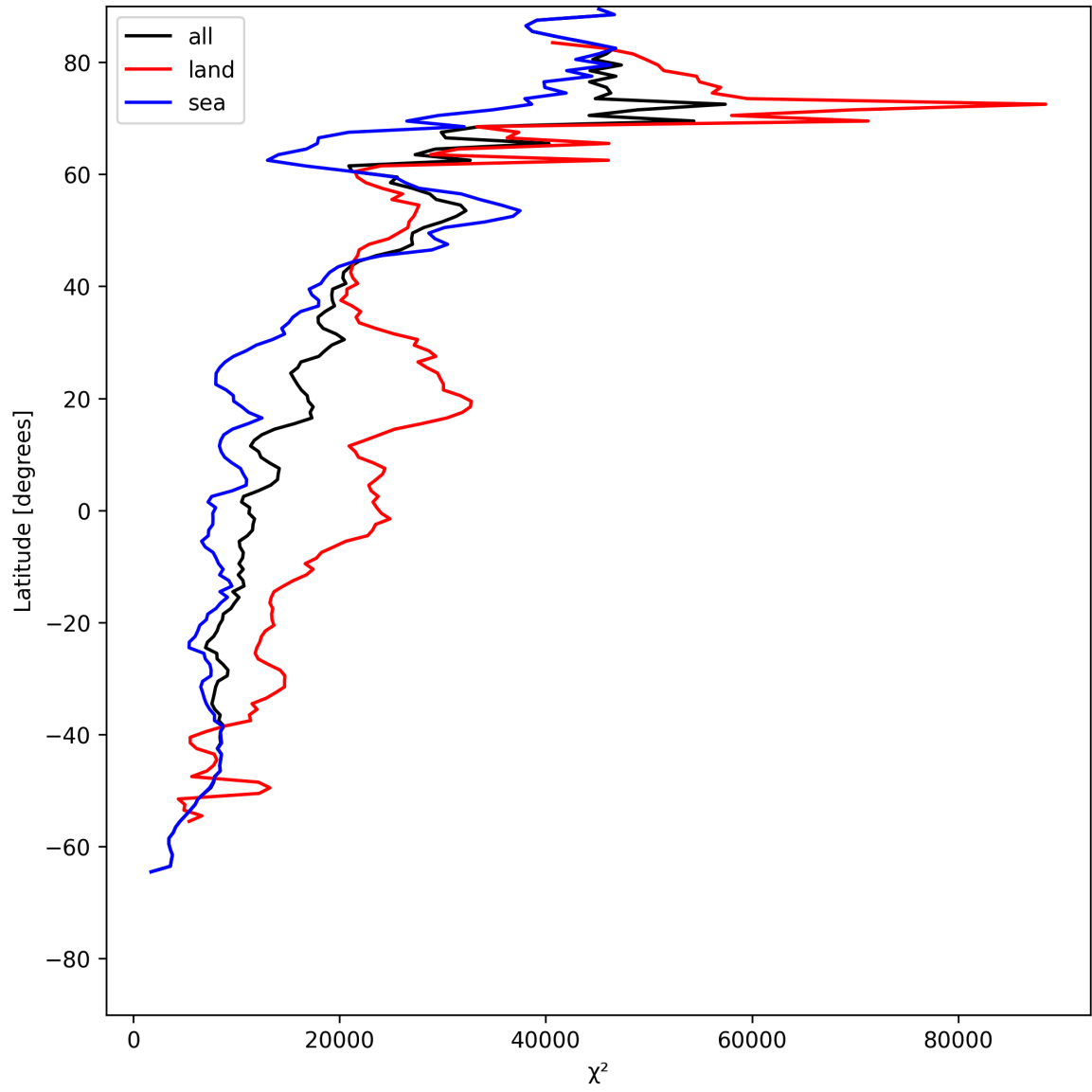
Figure 19: Zonal average of “ \chi^2 ” for 2025-06-08 to 2025-06-09.
