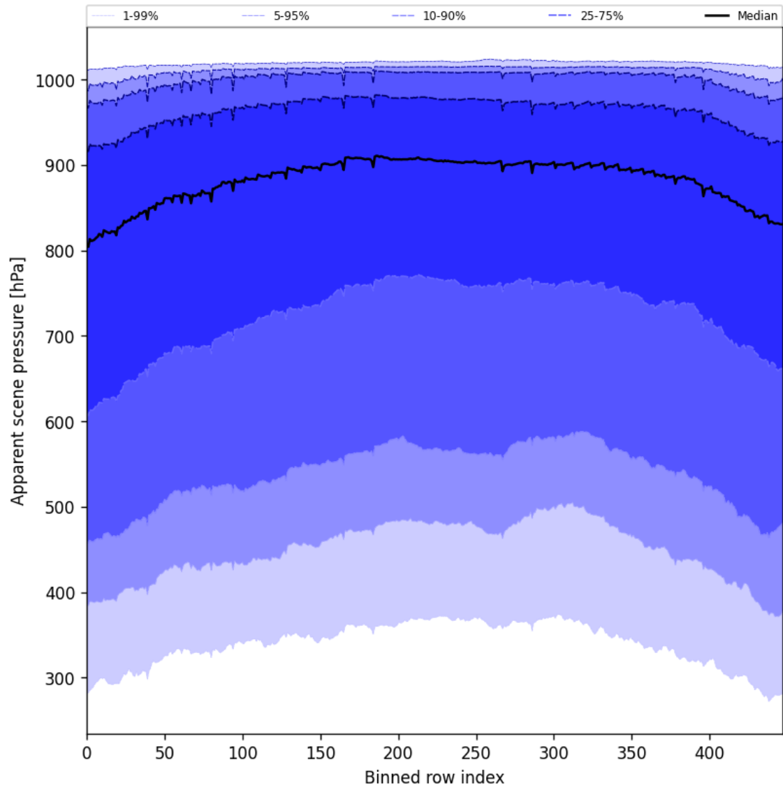
Figure 51: Along track statistics of “Apparent scene pressure” for 2025-06-08 to 2025-06-09
