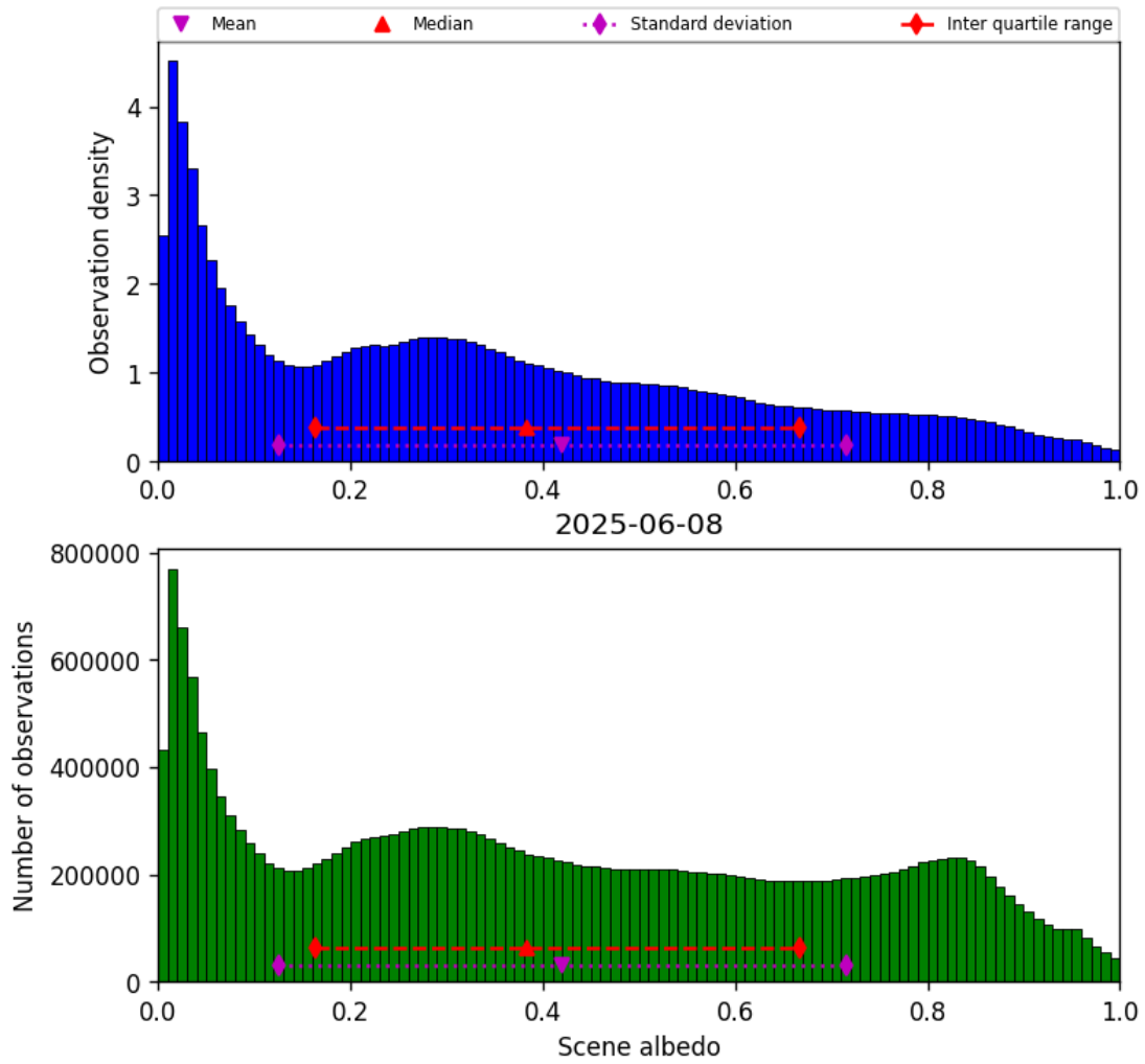
Figure 32: Histogram of “Scene albedo” for 2025-06-08 to 2025-06-09
