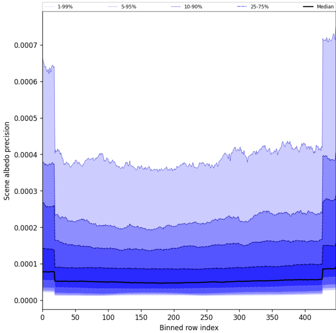
Figure 50: Along track statistics of “Scene albedo precision” for 2025-06-08 to 2025-06-09
