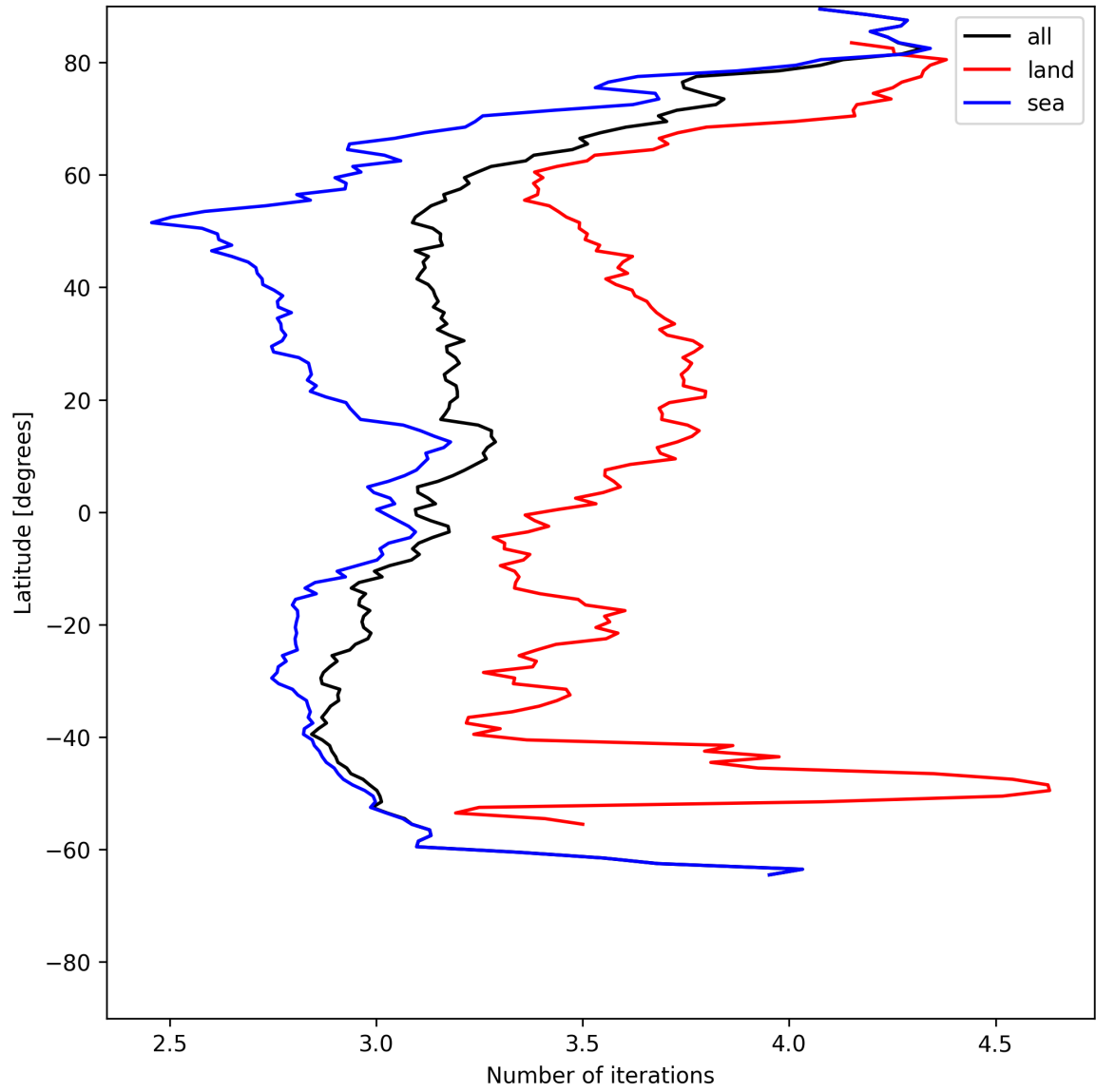
Figure 20: Zonal average of “Number of iterations” for 2025-06-08 to 2025-06-09.
