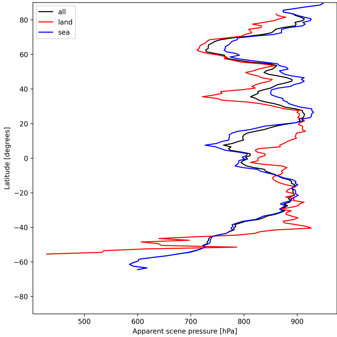
Figure 17: Zonal average of “Apparent scene pressure” for 2025-06-08 to 2025-06-09.
