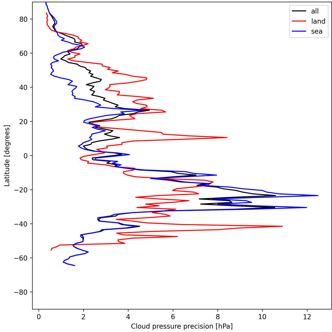
Figure 12: Zonal average of "Cloud pressure precision" for 2025-06-08 to 2025-06-09.
