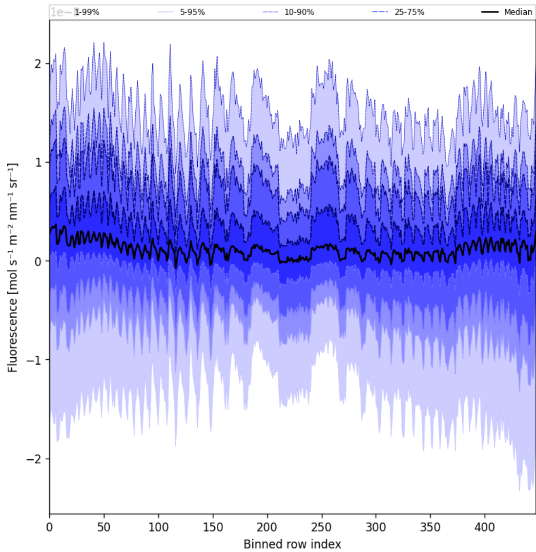
Figure 55: Along track statistics of “Fluorescence” for 2025-06-08 to 2025-06-09
