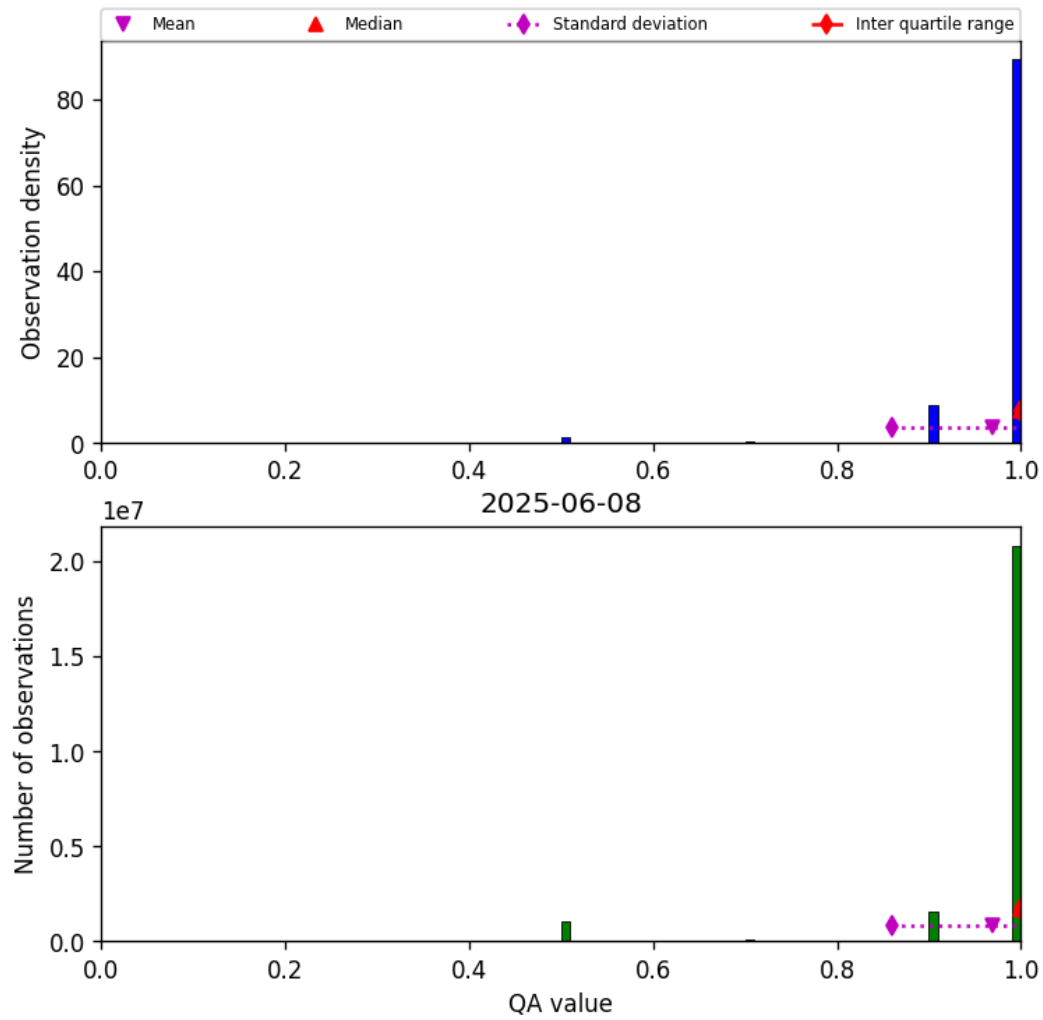
Figure 27: Histogram of “QA value” for 2025-06-08 to 2025-06-09
