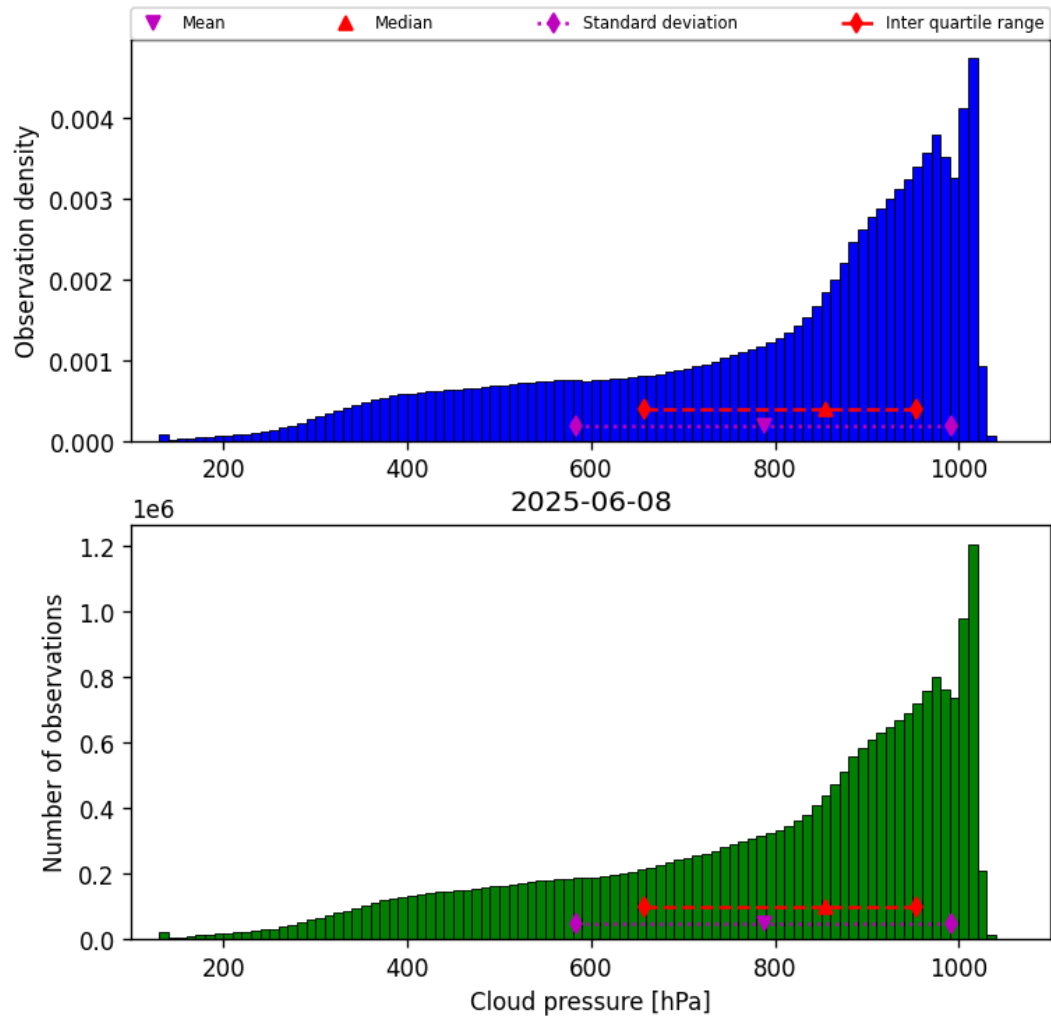
Figure 28: Histogram of “Cloud pressure” for 2025-06-08 to 2025-06-09
