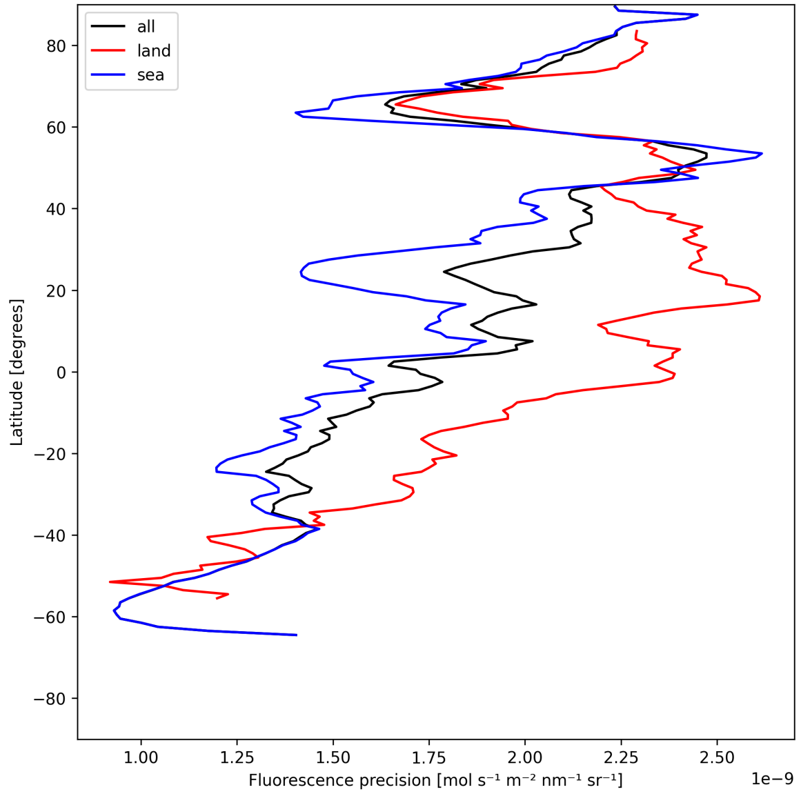
Figure 22: Zonal average of “Fluorescence precision” for 2025-06-08 to 2025-06-09.
