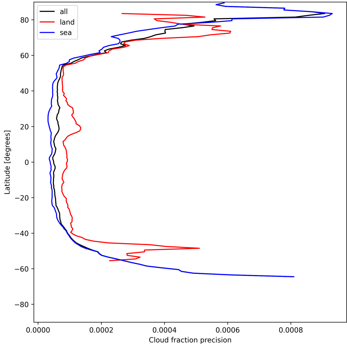
Figure 14: Zonal average of “Cloud fraction precision” for 2025-06-08 to 2025-06-09.
