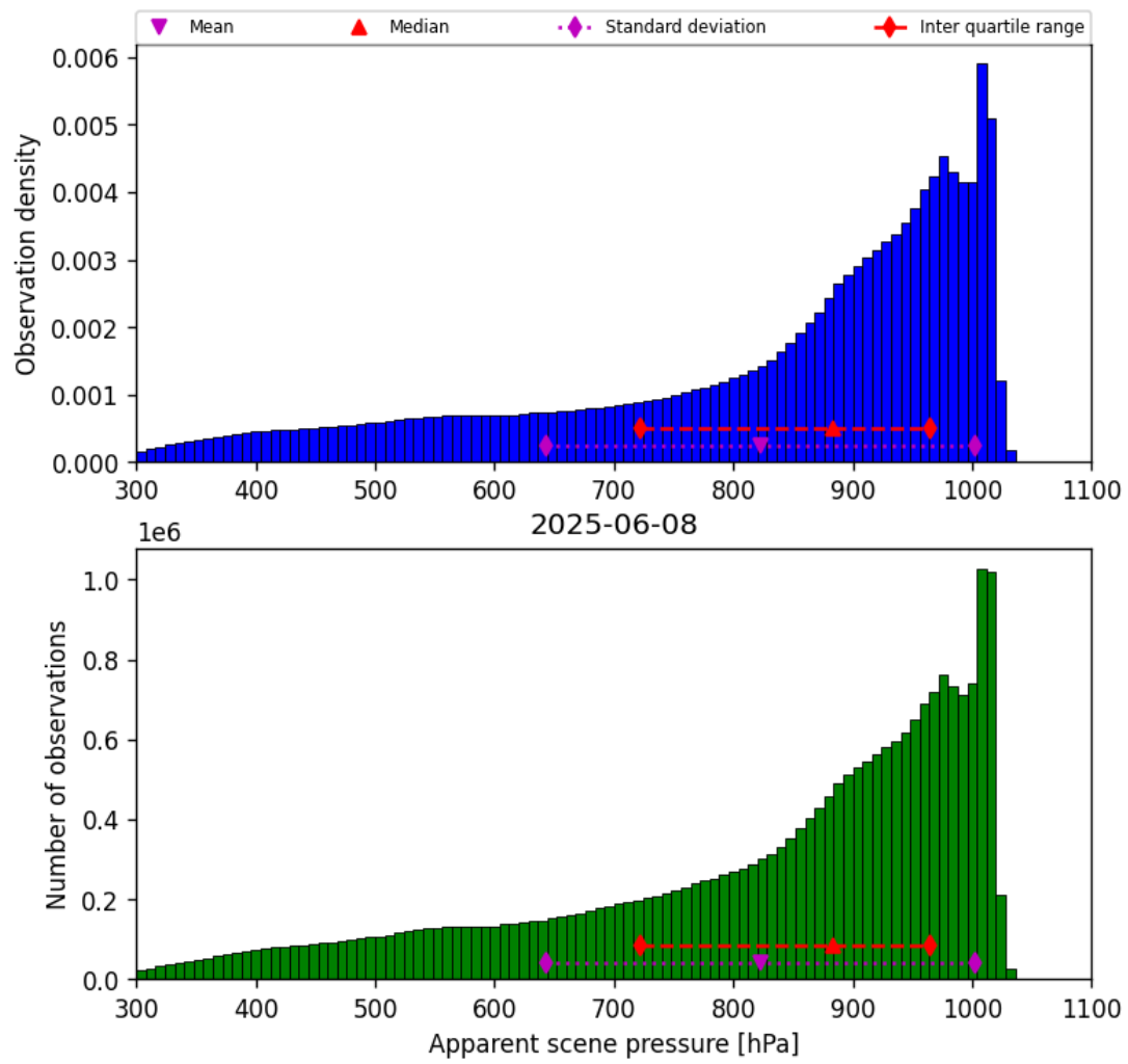
Figure 34: Histogram of “Apparent scene pressure” for 2025-06-08 to 2025-06-09
