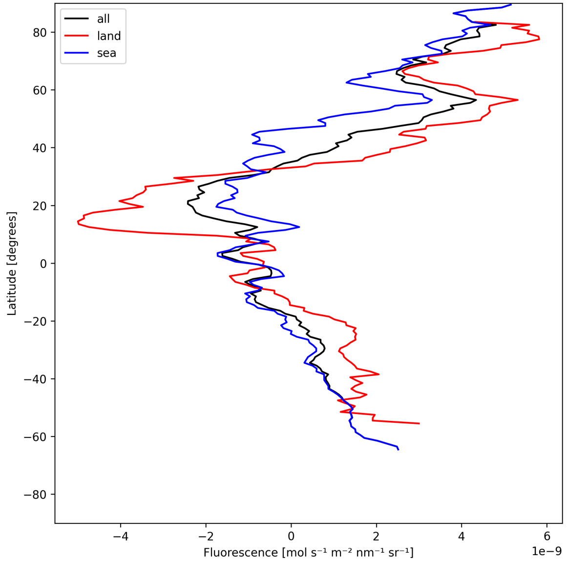
Figure 21: Zonal average of “Fluorescence” for 2025-06-08 to 2025-06-09.
