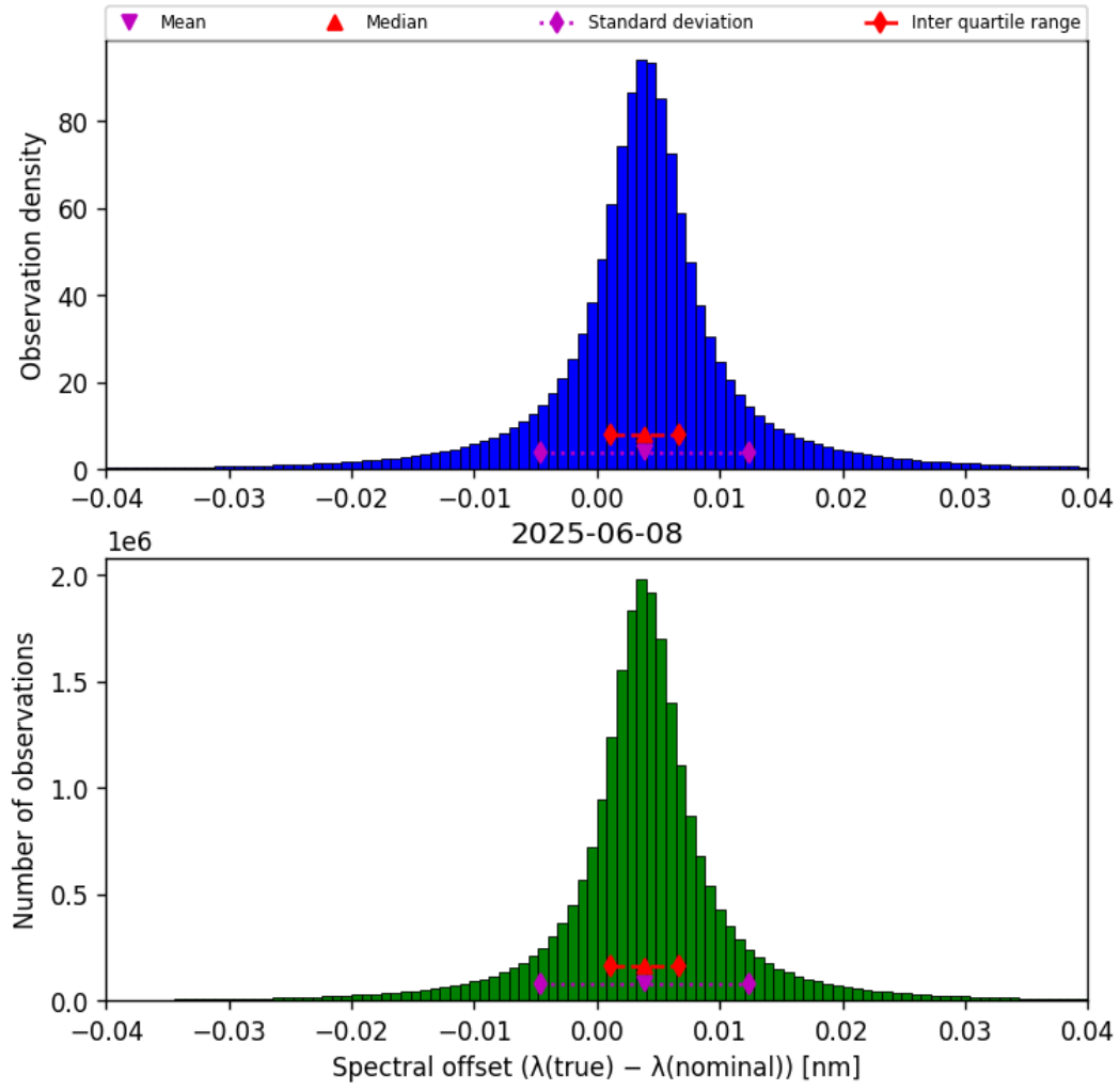
Figure 43: Histogram of “Spectral offset ( \lambda_{\text{true}} - \lambda_{\text{nominal}} )” for 2025-06-08 to 2025-06-09
