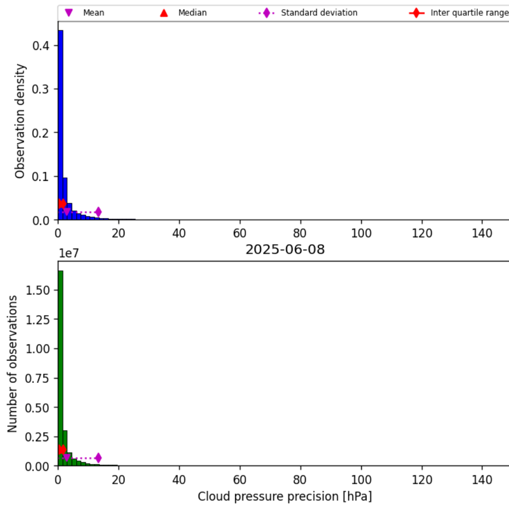
Figure 29: Histogram of “Cloud pressure precision” for 2025-06-08 to 2025-06-09
