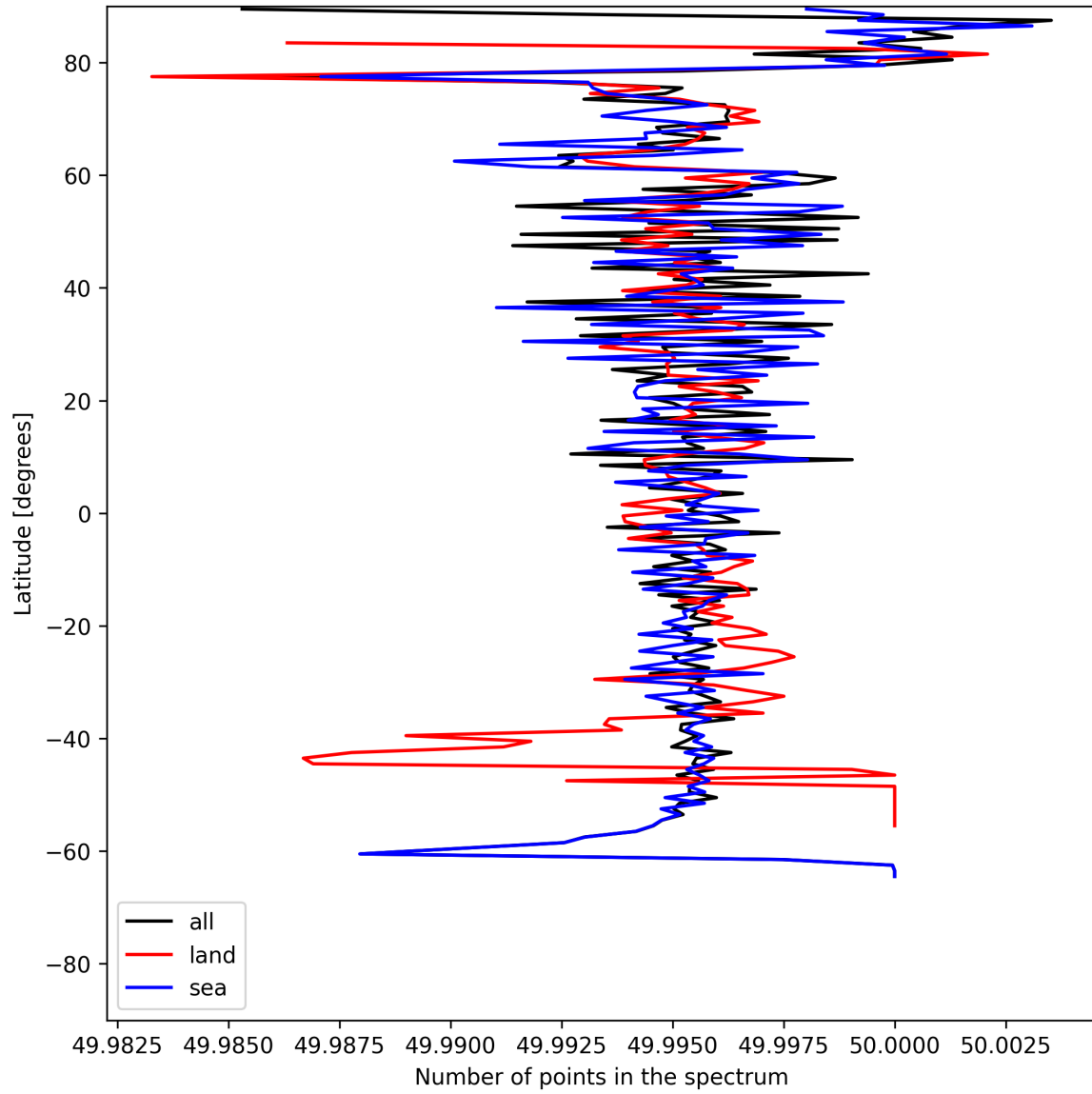
Figure 25: Zonal average of “Number of points in the spectrum” for 2025-06-08 to 2025-06-09.
