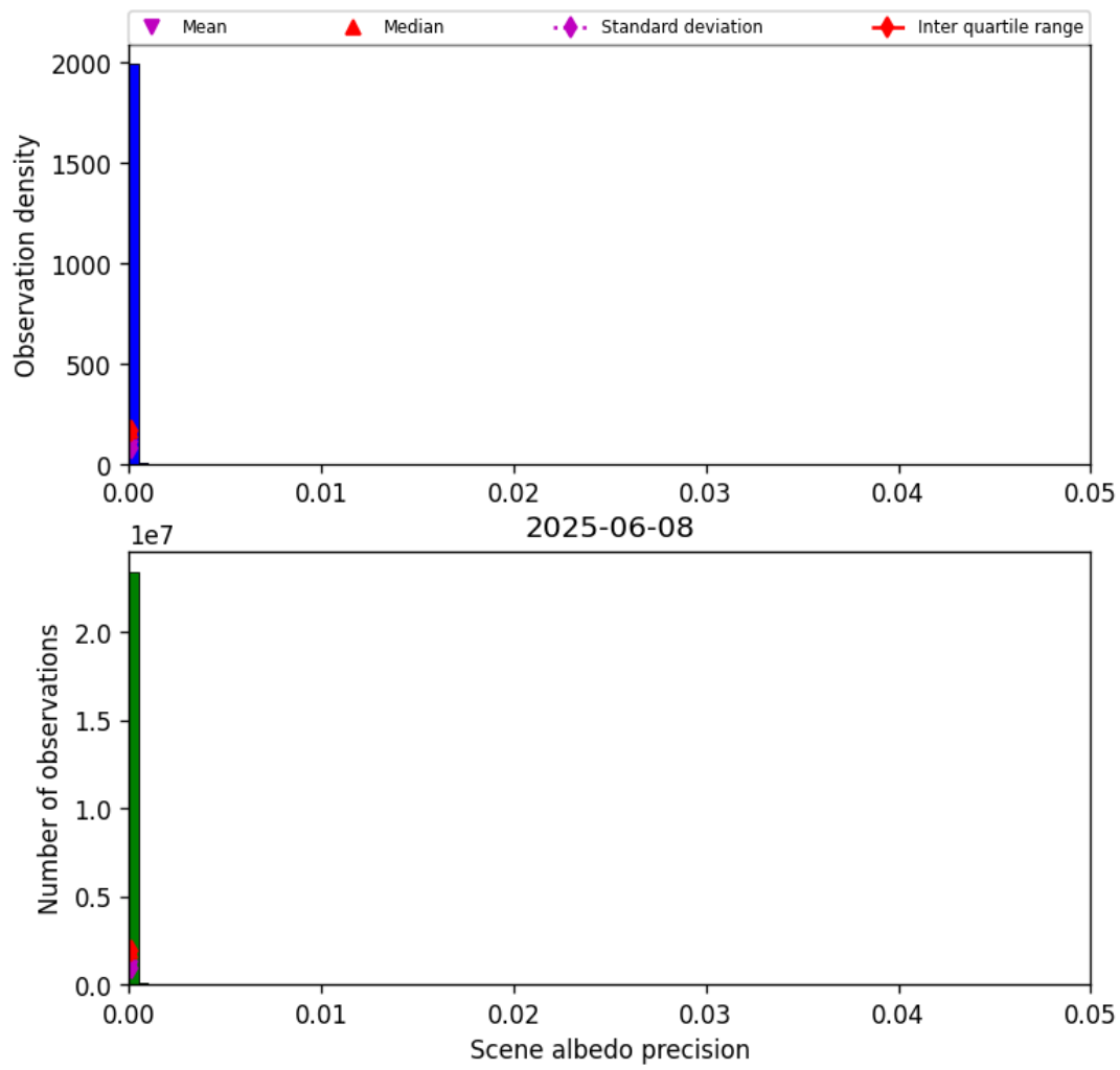
Figure 33: Histogram of “Scene albedo precision” for 2025-06-08 to 2025-06-09
