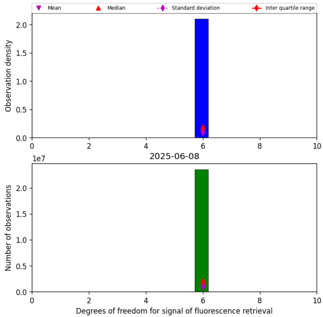
Figure 41: Histogram of “Degrees of freedom for signal of fluorescence retrieval” for 2025-06-08 to 2025-06-09
