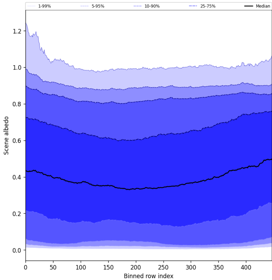
Figure 49: Along track statistics of “Scene albedo” for 2025-06-08 to 2025-06-09
