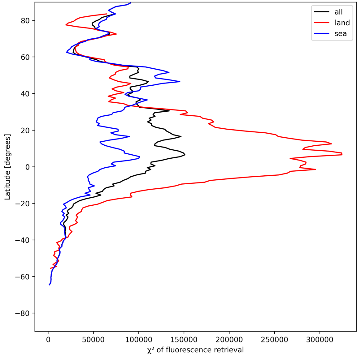
Figure 23: Zonal average of “ \chi^2 of fluorescence retrieval” for 2025-06-08 to 2025-06-09.
