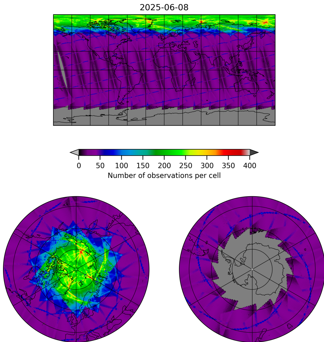
Figure 9: Map of the number of observations for 2025-06-08 to 2025-06-09
