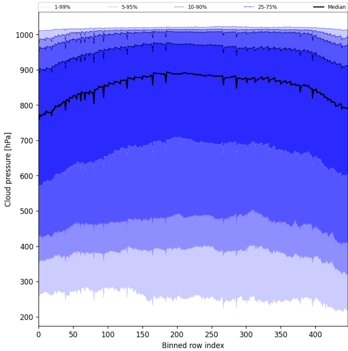
Figure 45: Along track statistics of “Cloud pressure” for 2025-06-08 to 2025-06-09
