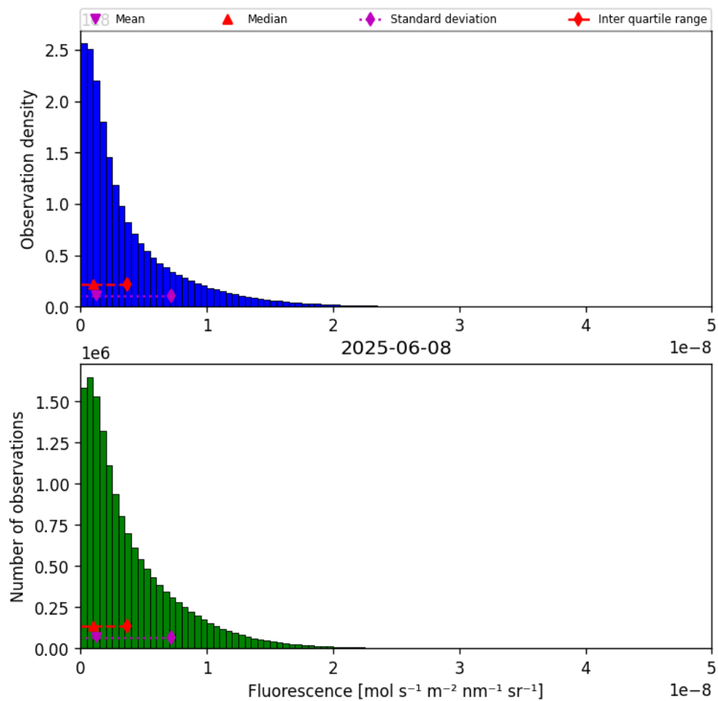
Figure 38: Histogram of “Fluorescence” for 2025-06-08 to 2025-06-09
