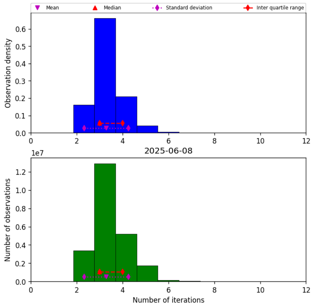
Figure 37: Histogram of “Number of iterations” for 2025-06-08 to 2025-06-09
