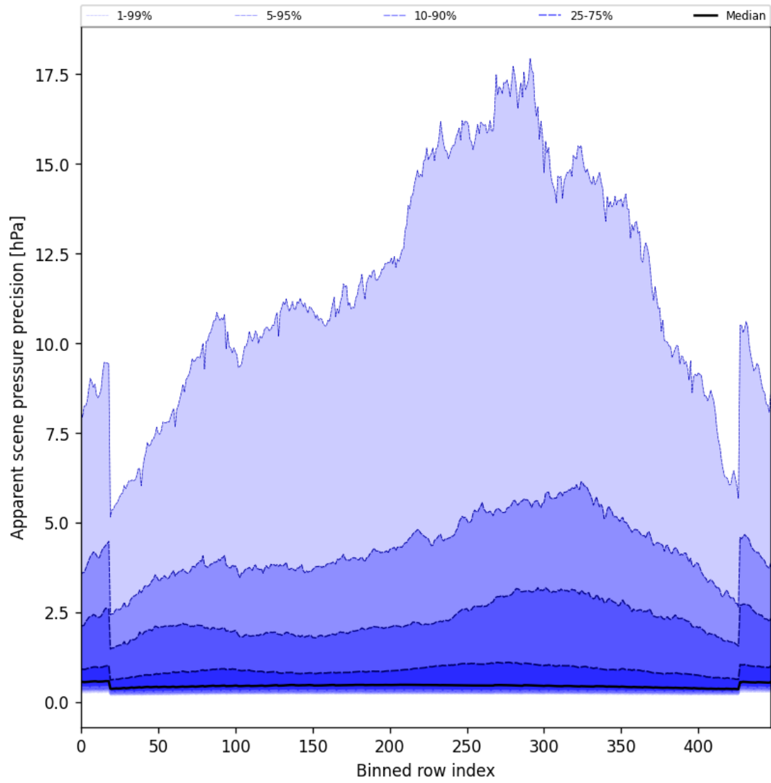
Figure 52: Along track statistics of “Apparent scene pressure precision” for 2025-06-08 to 2025-06-09
