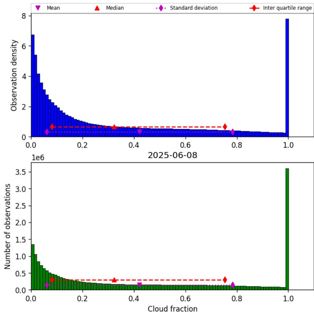
Figure 30: Histogram of “Cloud fraction” for 2025-06-08 to 2025-06-09
