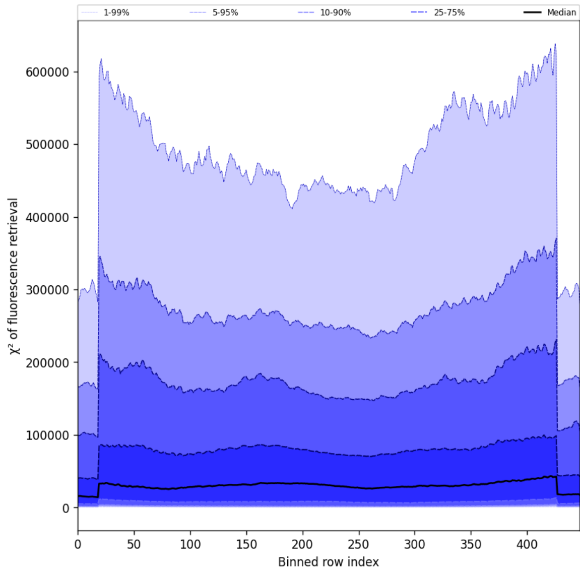
Figure 57: Along track statistics of “ \chi^2 of fluorescence retrieval” for 2025-06-08 to 2025-06-09
