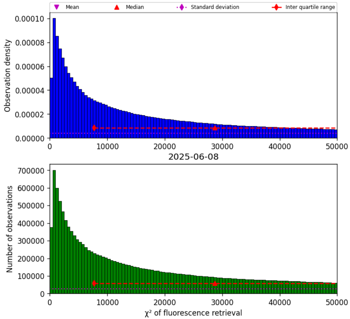
Figure 40: Histogram of “ \chi^2 of fluorescence retrieval” for 2025-06-08 to 2025-06-09
