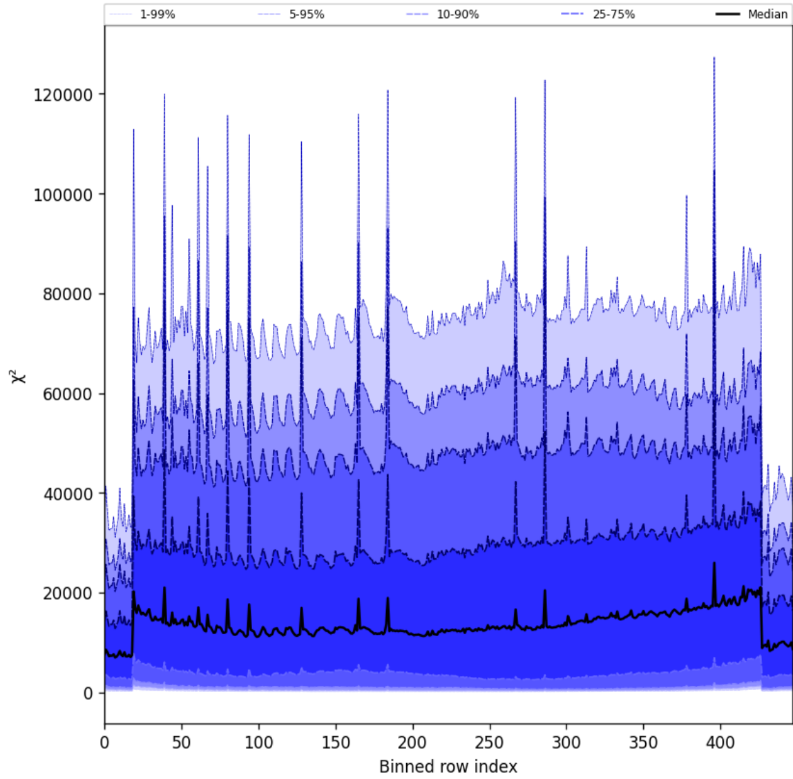
Figure 53: Along track statistics of “ \chi^2 ” for 2025-06-08 to 2025-06-09
