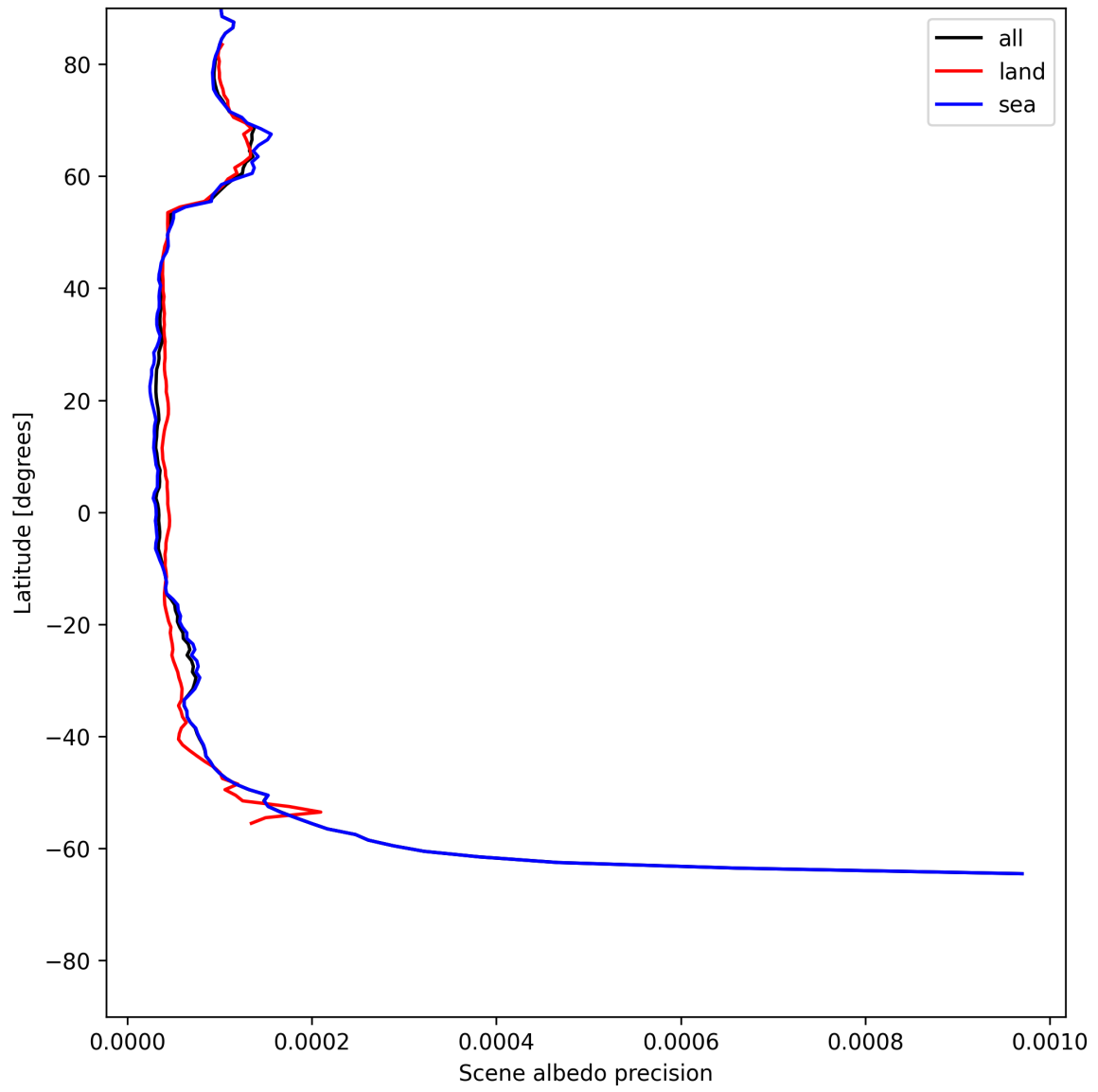
Figure 16: Zonal average of “Scene albedo precision” for 2025-06-08 to 2025-06-09.
