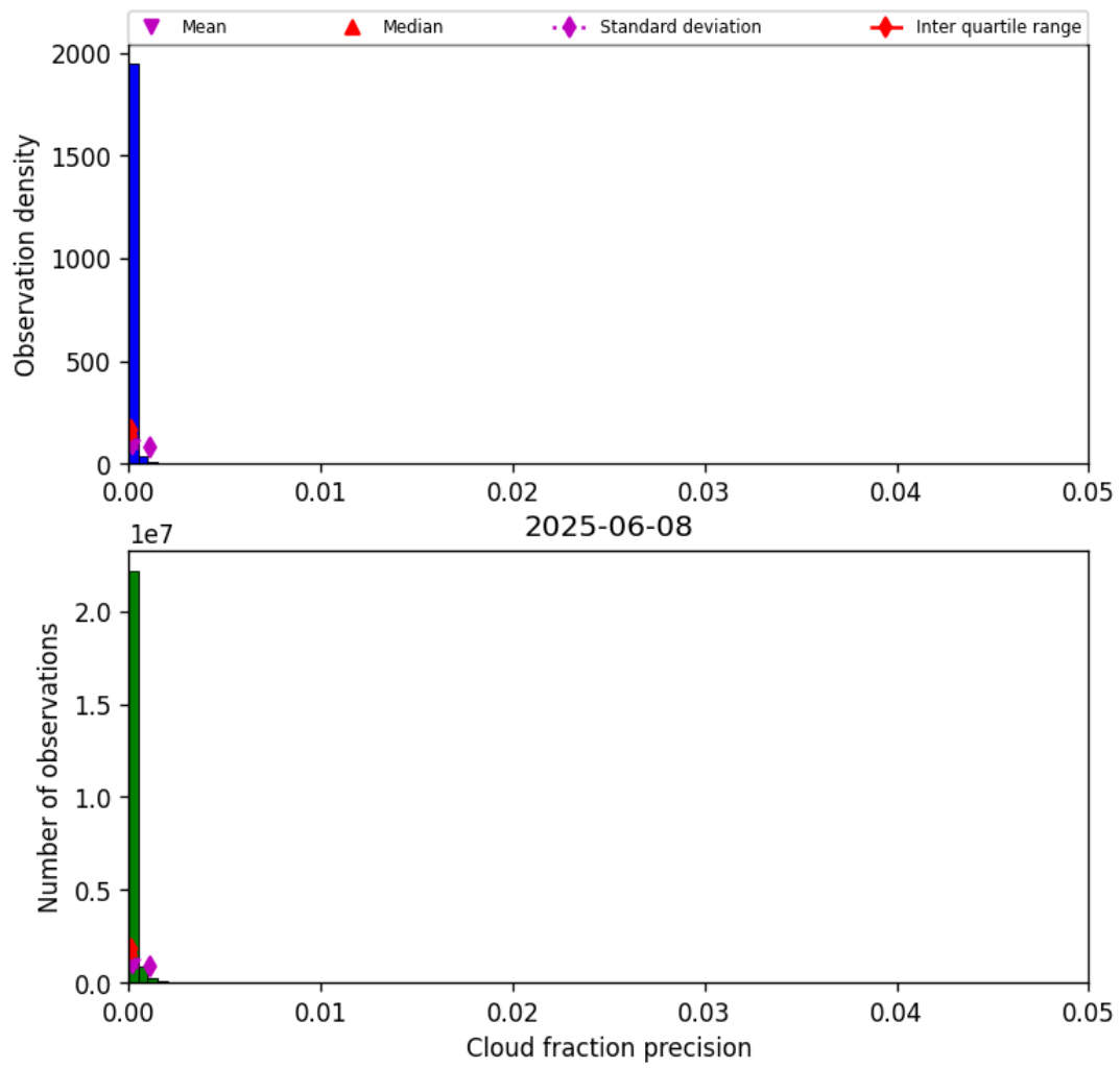
Figure 31: Histogram of “Cloud fraction precision” for 2025-06-08 to 2025-06-09
