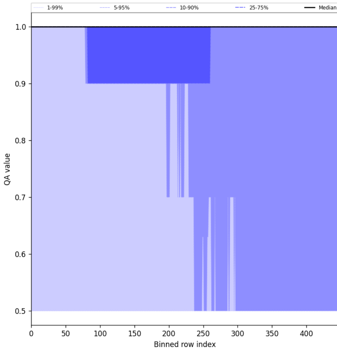
Figure 44: Along track statistics of “QA value” for 2025-06-08 to 2025-06-09
