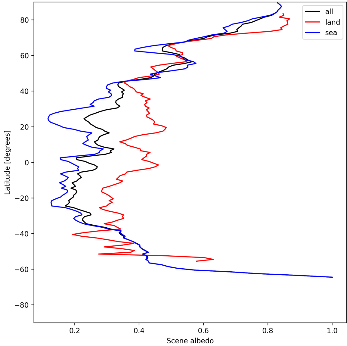
Figure 15: Zonal average of “Scene albedo” for 2025-06-08 to 2025-06-09.
