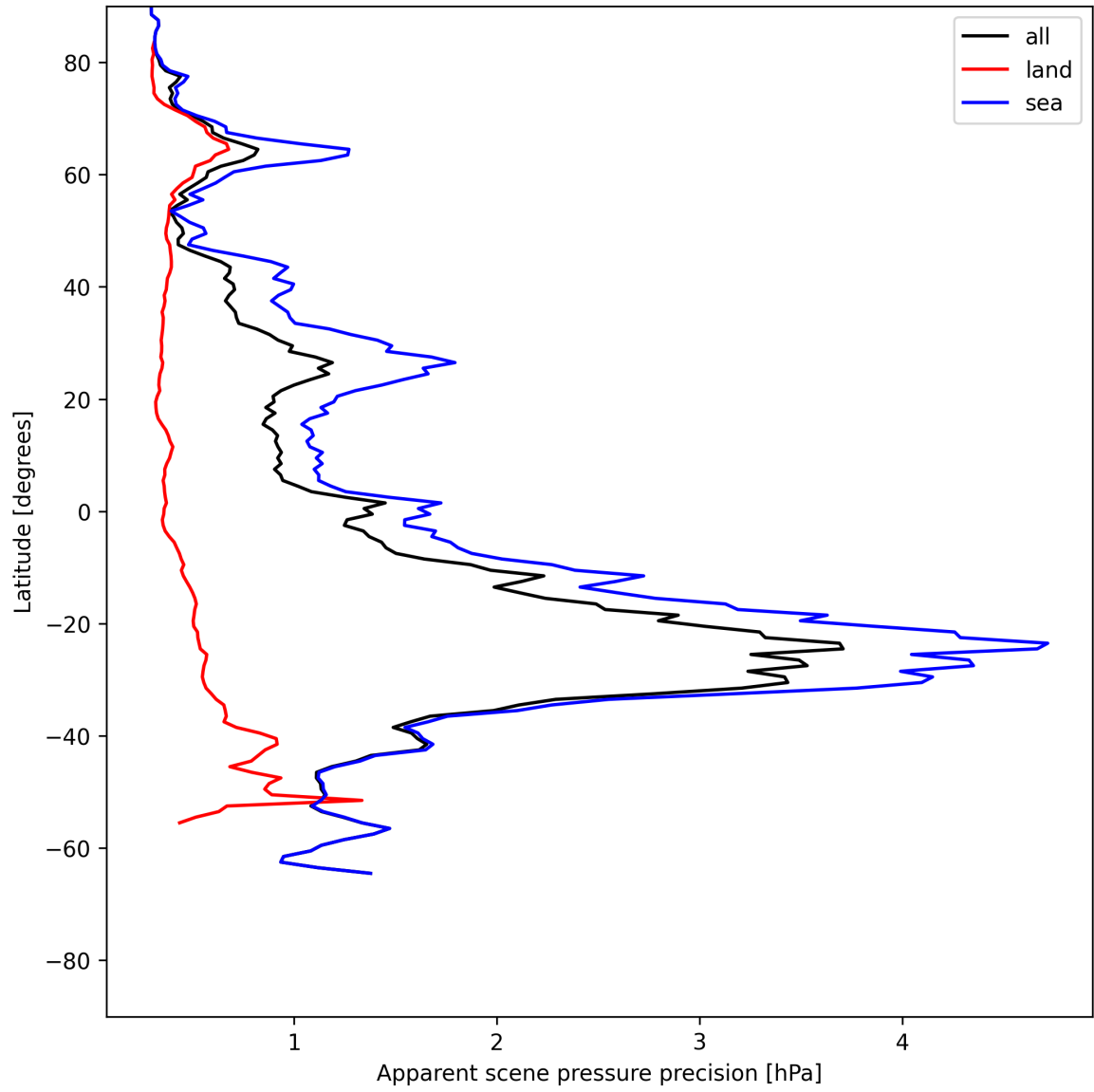
Figure 18: Zonal average of “Apparent scene pressure precision” for 2025-06-08 to 2025-06-09.
