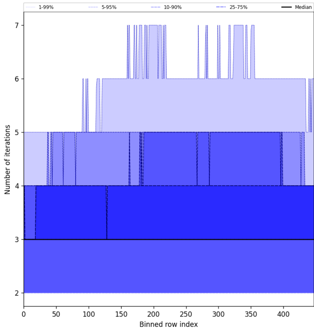
Figure 54: Along track statistics of “Number of iterations” for 2025-06-08 to 2025-06-09
