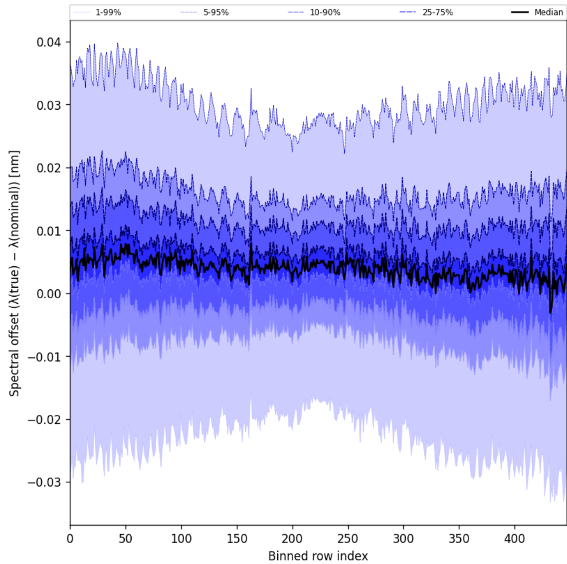
Figure 60: Along track statistics of “Spectral offset ( \lambda_{\text{true}} - \lambda_{\text{nominal}} )” for 2025-06-08 to 2025-06-09
