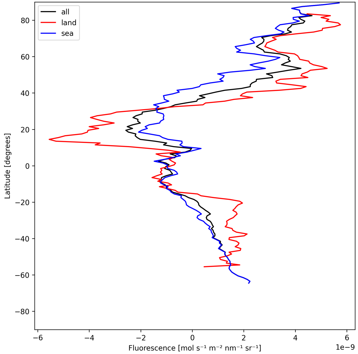
Figure 21: Zonal average of “Fluorescence” for 2025-06-09 to 2025-06-09.
