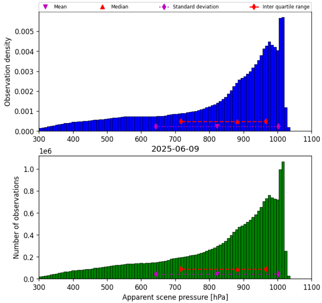
Figure 34: Histogram of “Apparent scene pressure” for 2025-06-09 to 2025-06-09
