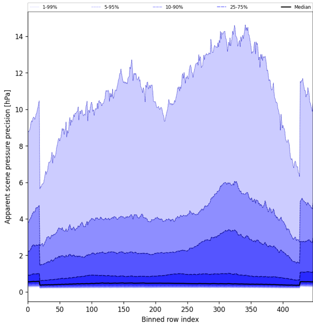
Figure 52: Along track statistics of “Apparent scene pressure precision” for 2025-06-09 to 2025-06-09
