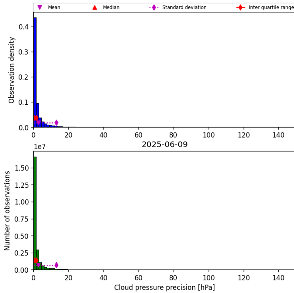
Figure 29: Histogram of “Cloud pressure precision” for 2025-06-09 to 2025-06-09
