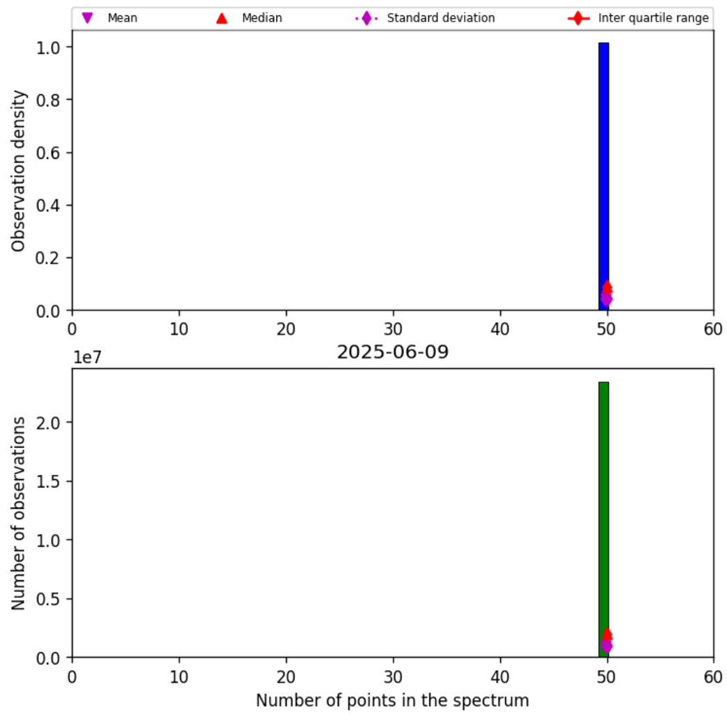
Figure 42: Histogram of "Number of points in the spectrum" for 2025-06-09 to 2025-06-09
