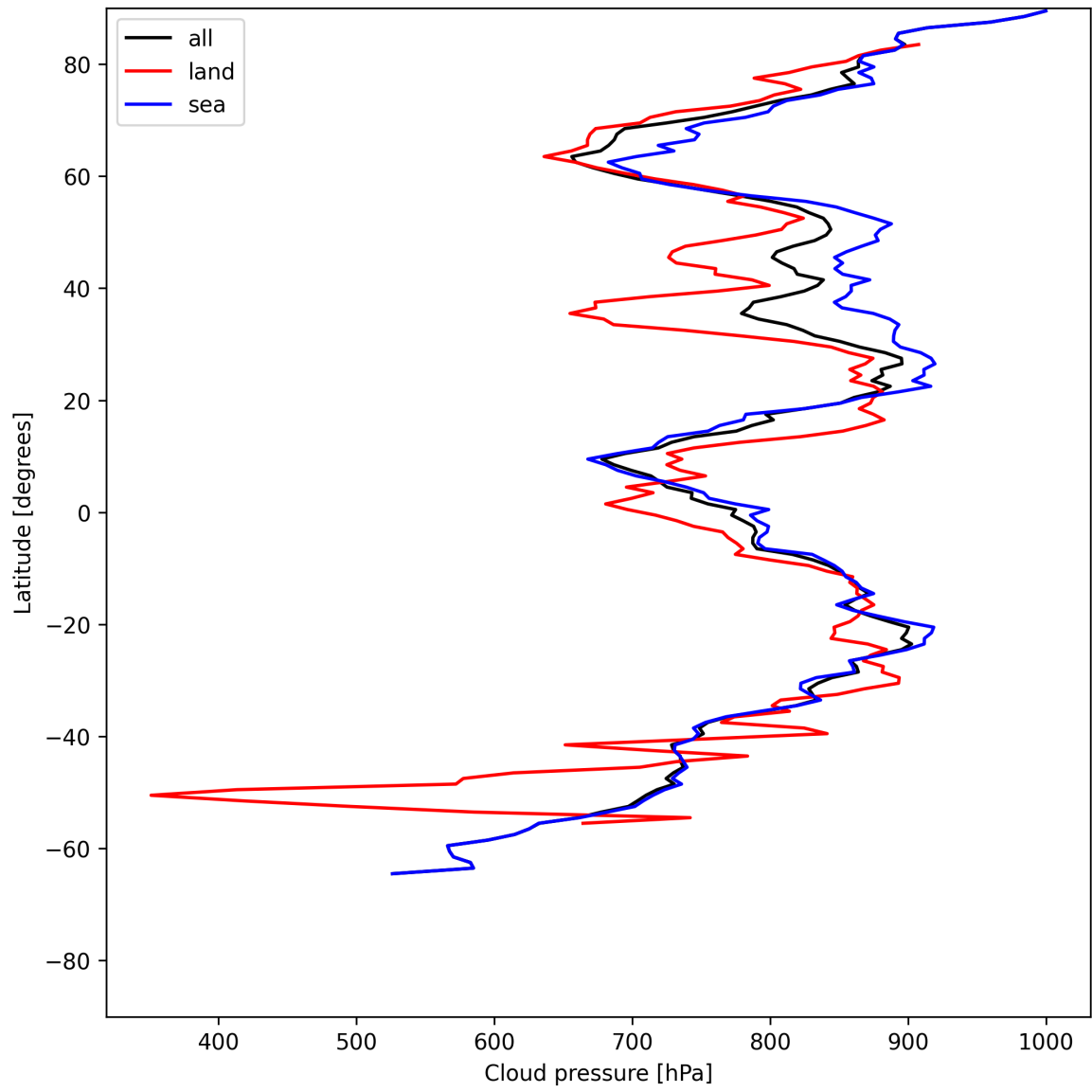
Figure 11: Zonal average of “Cloud pressure” for 2025-06-09 to 2025-06-09.
