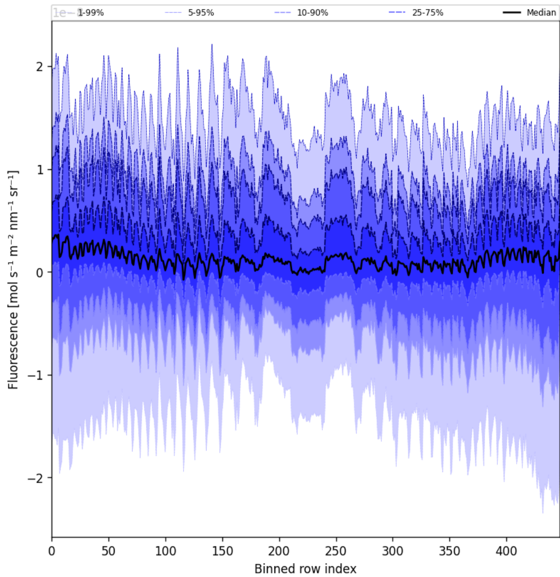
Figure 55: Along track statistics of “Fluorescence” for 2025-06-09 to 2025-06-09
