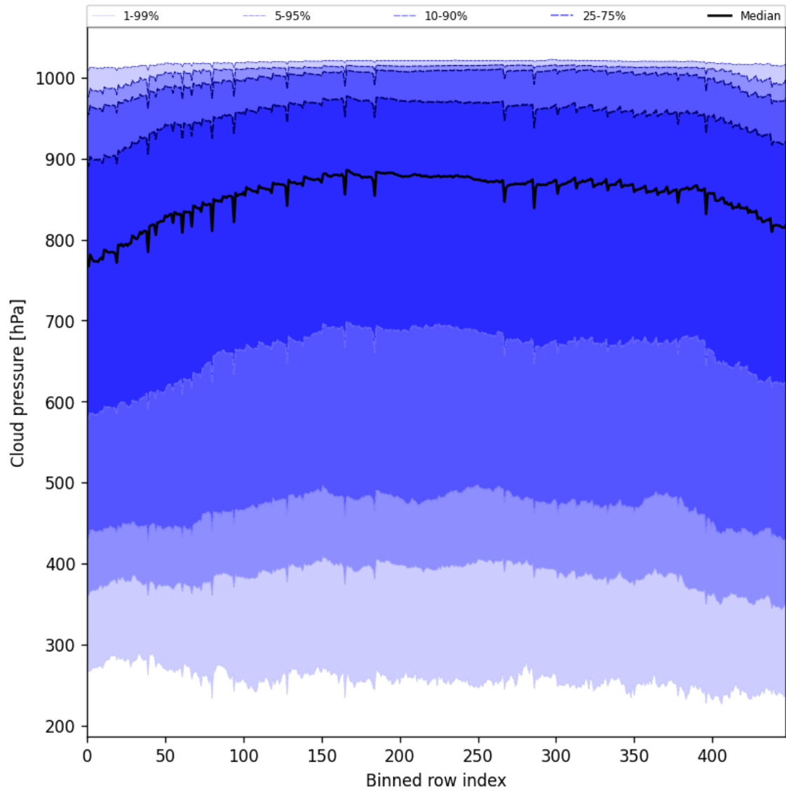
Figure 45: Along track statistics of “Cloud pressure” for 2025-06-09 to 2025-06-09
