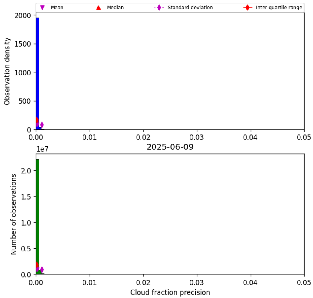
Figure 31: Histogram of “Cloud fraction precision” for 2025-06-09 to 2025-06-09
