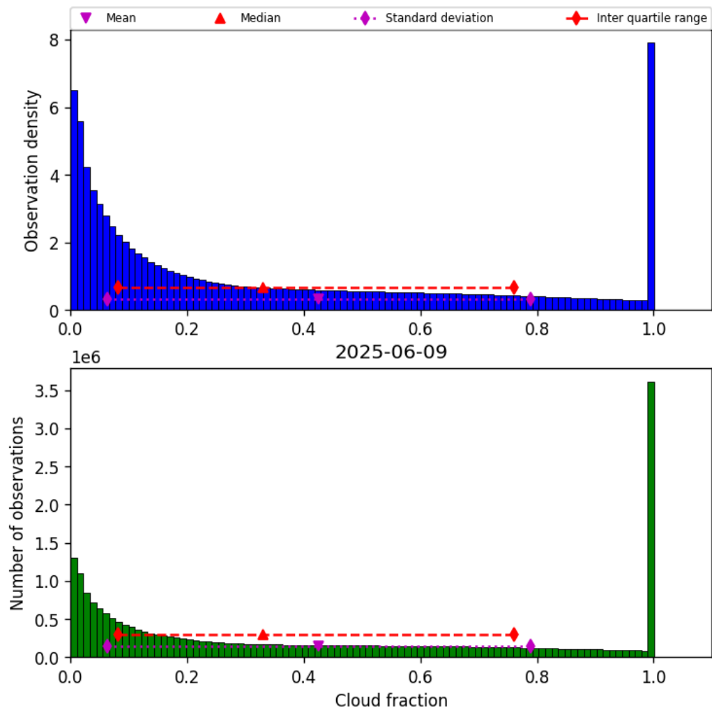
Figure 30: Histogram of “Cloud fraction” for 2025-06-09 to 2025-06-09
