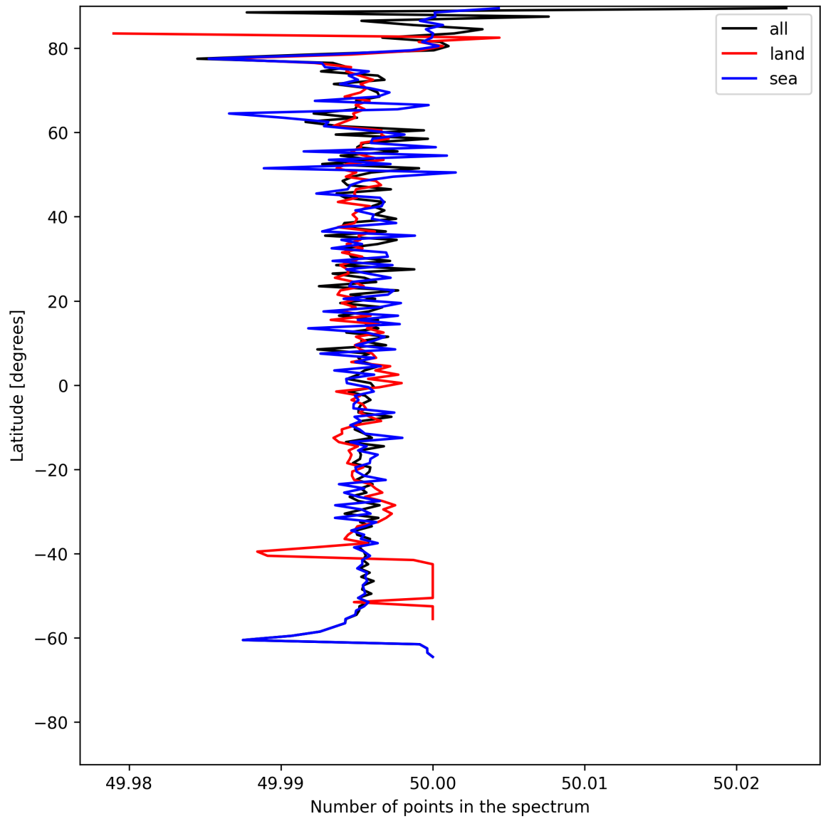
Figure 25: Zonal average of “Number of points in the spectrum” for 2025-06-09 to 2025-06-09.
