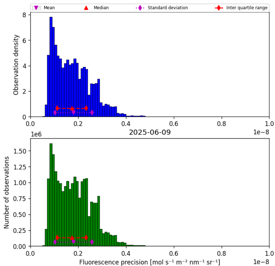
Figure 39: Histogram of “Fluorescence precision” for 2025-06-09 to 2025-06-09
