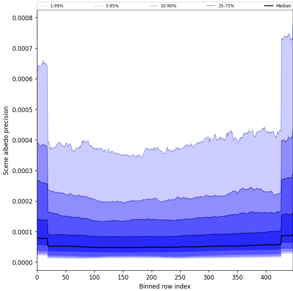
Figure 50: Along track statistics of “Scene albedo precision” for 2025-06-09 to 2025-06-09
