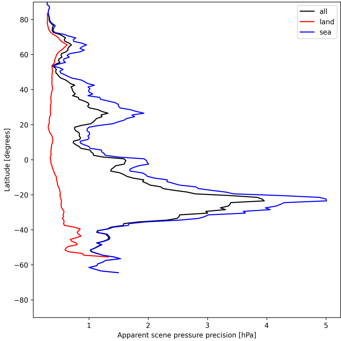
Figure 18: Zonal average of “Apparent scene pressure precision” for 2025-06-09 to 2025-06-09.
