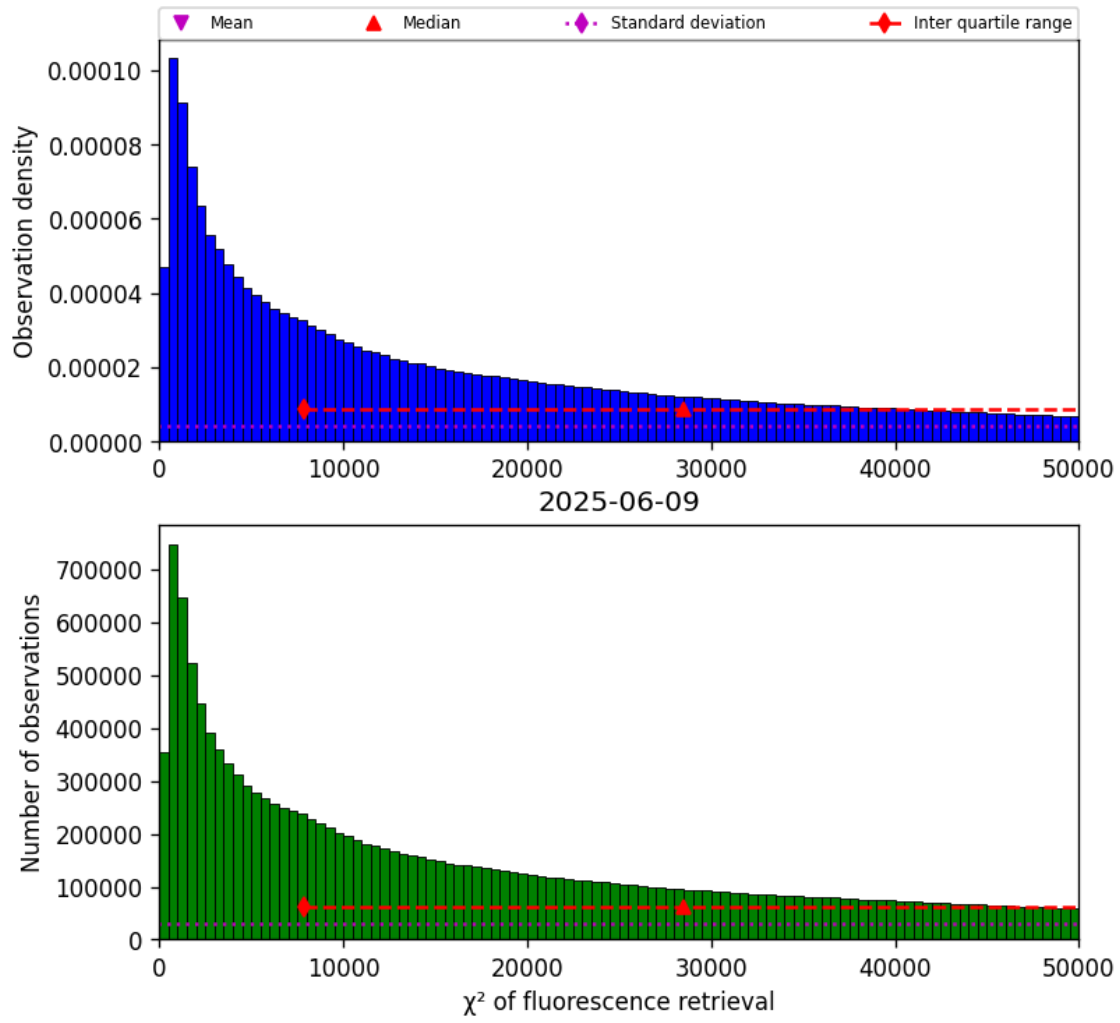
Figure 40: Histogram of “ \chi^2 of fluorescence retrieval” for 2025-06-09 to 2025-06-09
