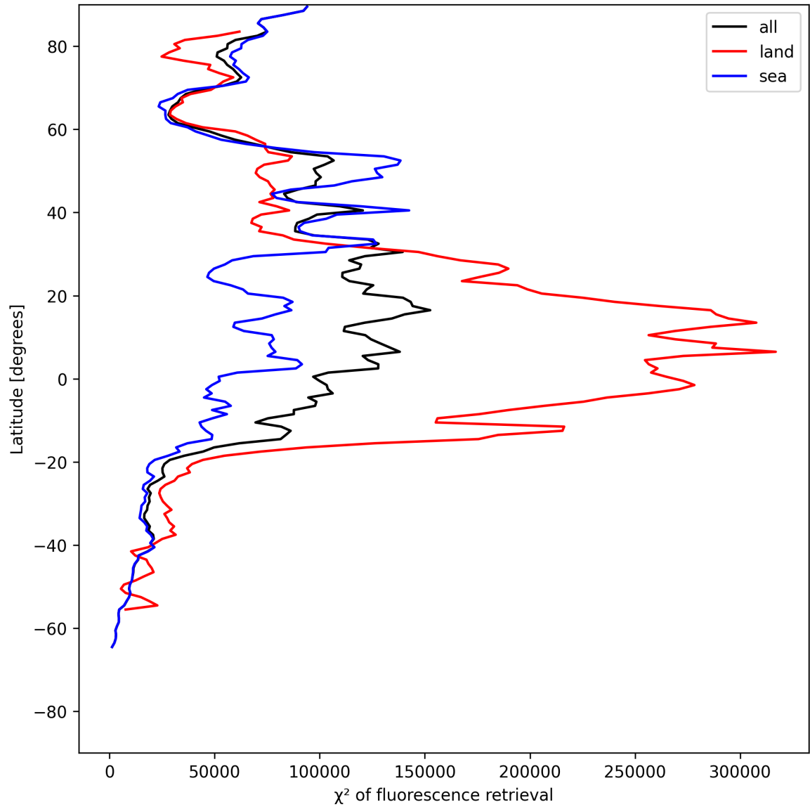
Figure 23: Zonal average of “ \chi^2 of fluorescence retrieval” for 2025-06-09 to 2025-06-09.
