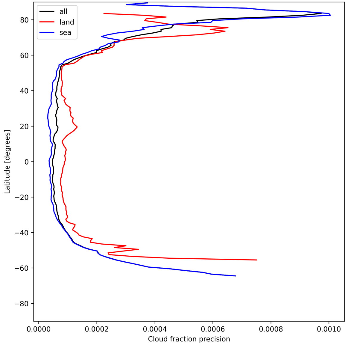
Figure 14: Zonal average of “Cloud fraction precision” for 2025-06-09 to 2025-06-09.
