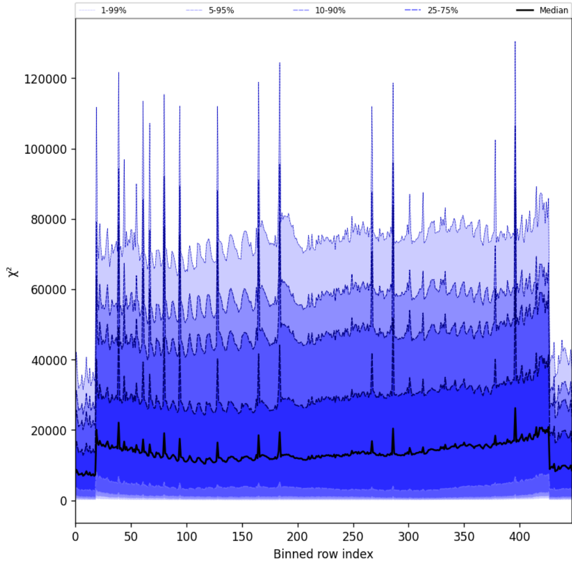
Figure 53: Along track statistics of “ \chi^2 ” for 2025-06-09 to 2025-06-09
