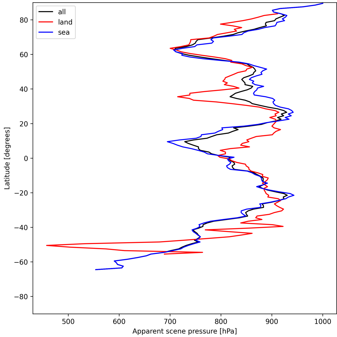
Figure 17: Zonal average of “Apparent scene pressure” for 2025-06-09 to 2025-06-09.
