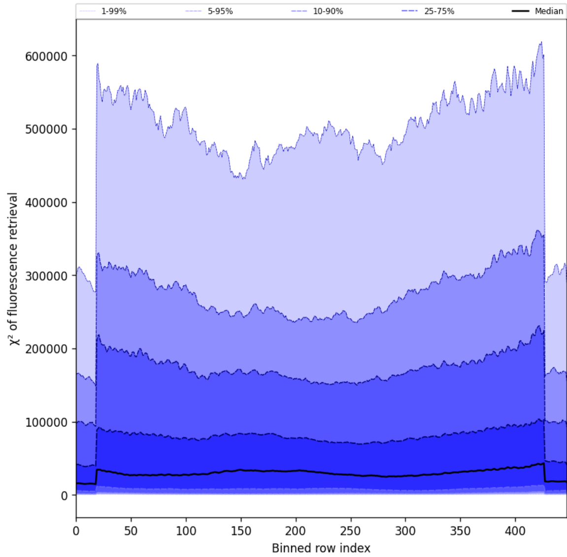
Figure 57: Along track statistics of “ \chi^2 of fluorescence retrieval” for 2025-06-09 to 2025-06-09
