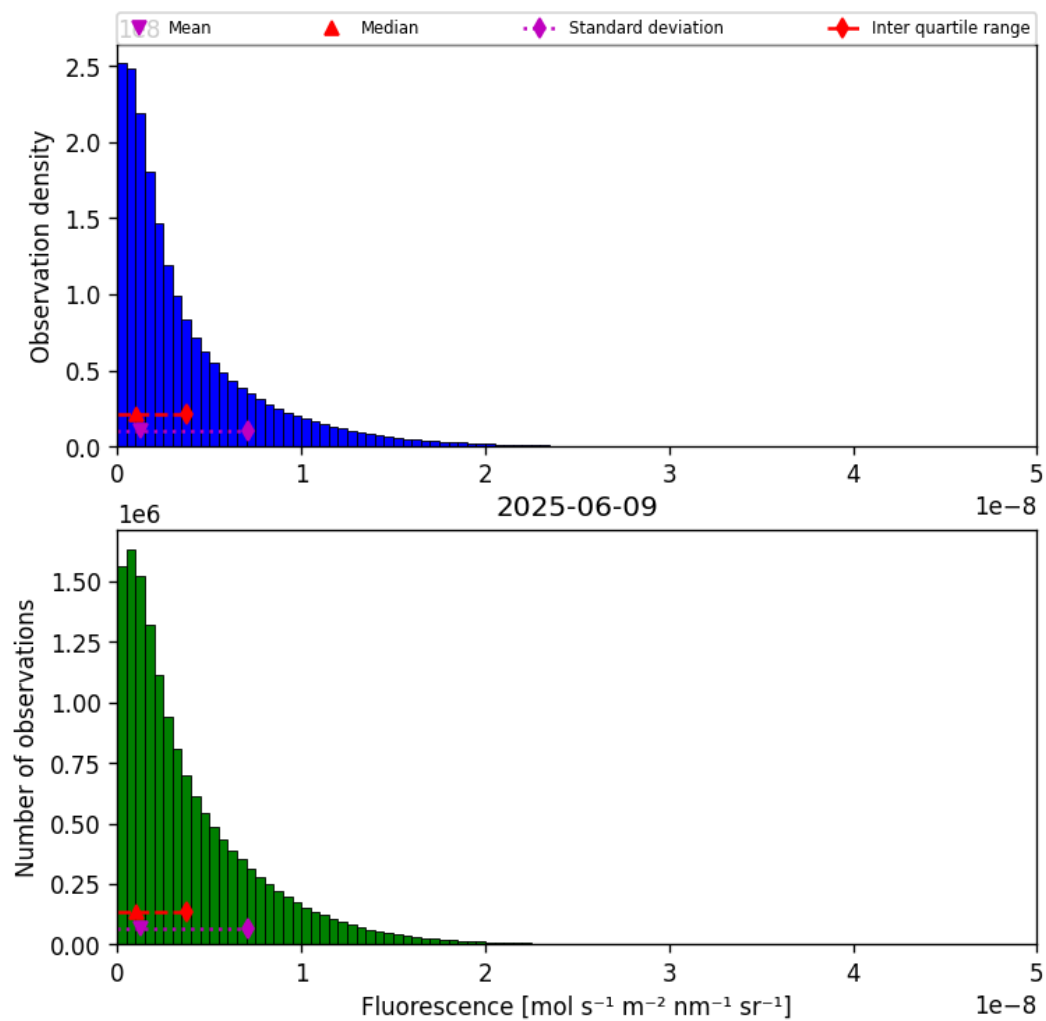
Figure 38: Histogram of “Fluorescence” for 2025-06-09 to 2025-06-09
