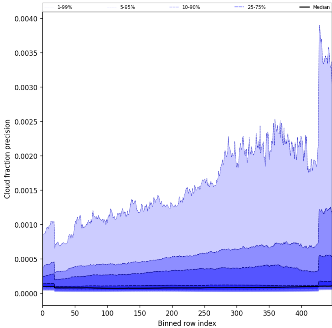
Figure 48: Along track statistics of “Cloud fraction precision” for 2025-06-09 to 2025-06-09
