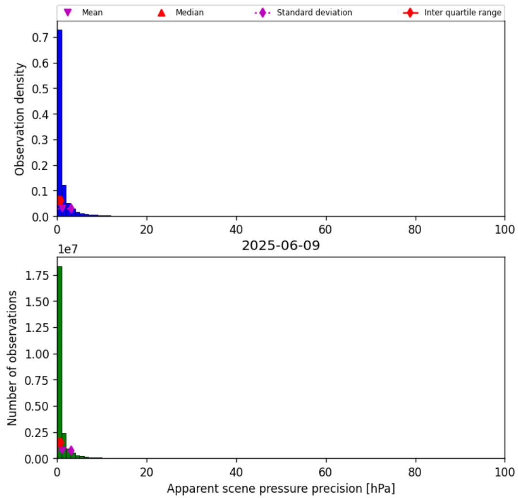
Figure 35: Histogram of “Apparent scene pressure precision” for 2025-06-09 to 2025-06-09
