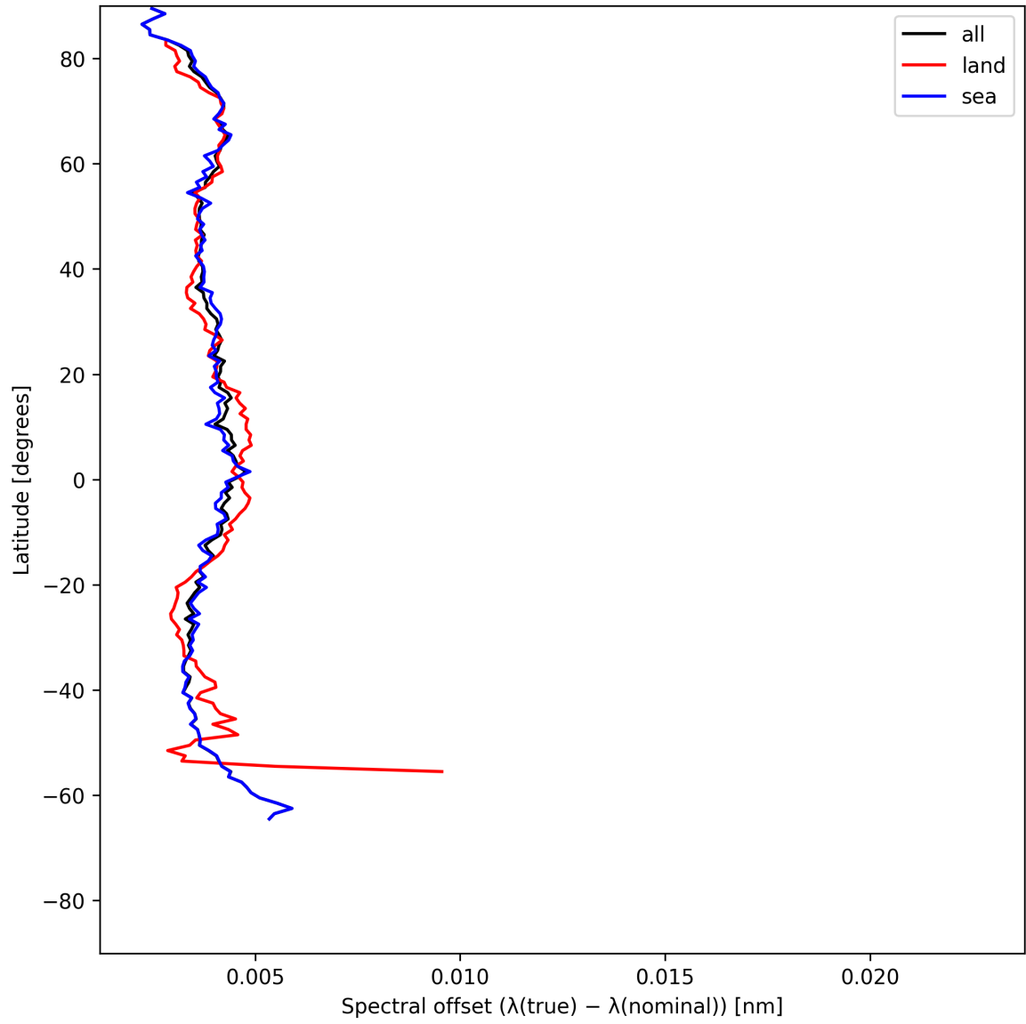
Figure 26: Zonal average of “Spectral offset ( \lambda_{\text{true}} - \lambda_{\text{nominal}} )” for 2025-06-09 to 2025-06-09.
