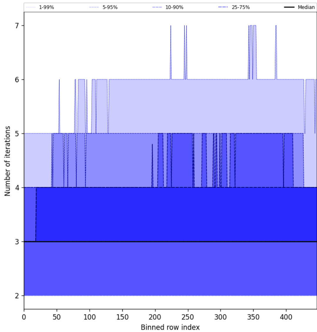
Figure 54: Along track statistics of "Number of iterations" for 2025-06-09 to 2025-06-09
