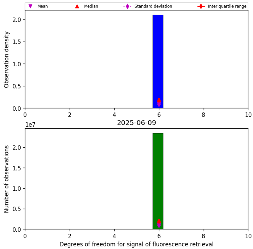
Figure 41: Histogram of “Degrees of freedom for signal of fluorescence retrieval” for 2025-06-09 to 2025-06-09
