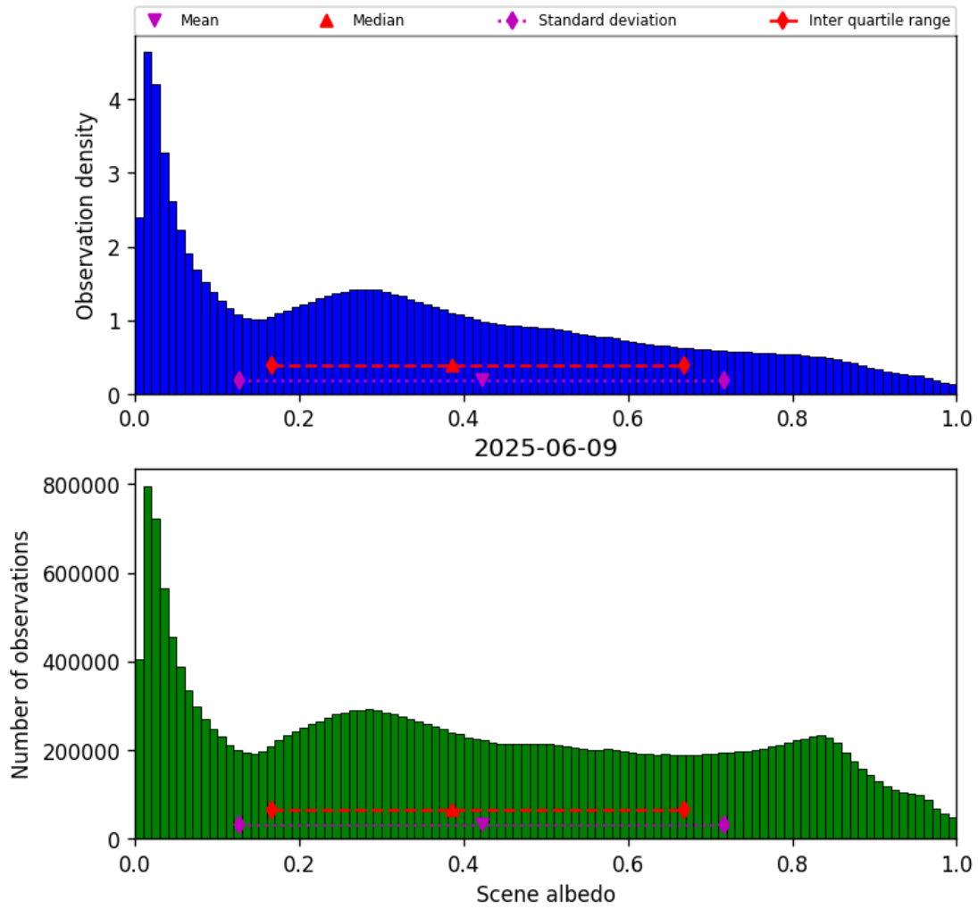
Figure 32: Histogram of “Scene albedo” for 2025-06-09 to 2025-06-09
