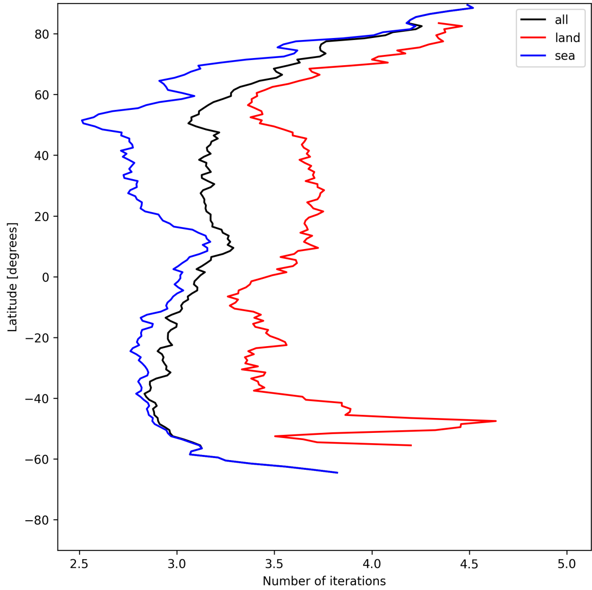
Figure 20: Zonal average of “Number of iterations” for 2025-06-09 to 2025-06-09.
