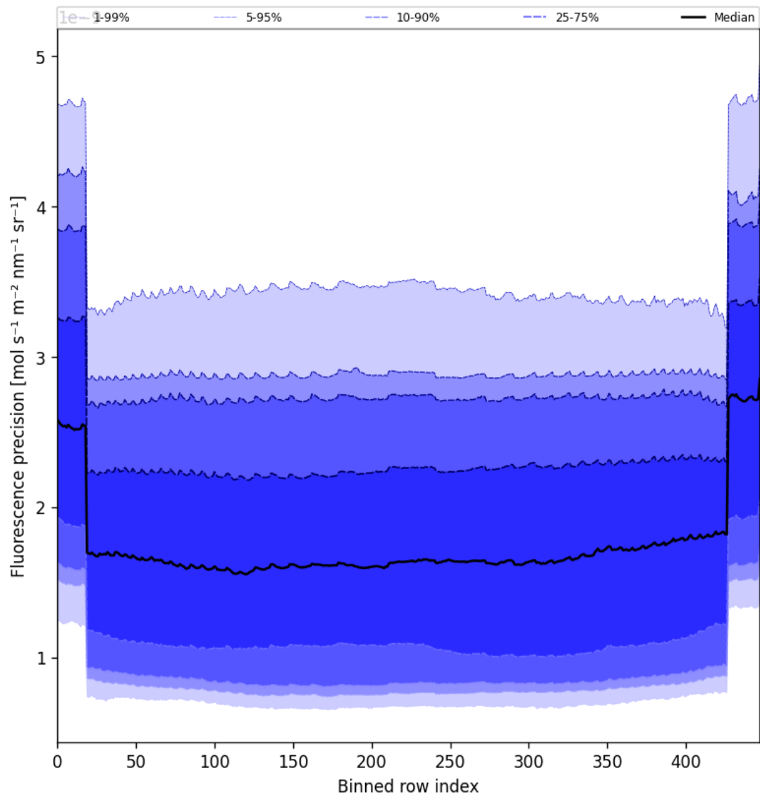
Figure 56: Along track statistics of “Fluorescence precision” for 2025-06-09 to 2025-06-09
