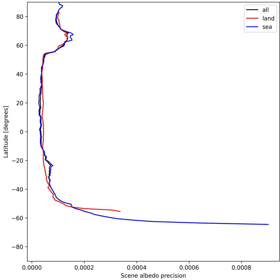
Figure 16: Zonal average of “Scene albedo precision” for 2025-06-09 to 2025-06-09.
