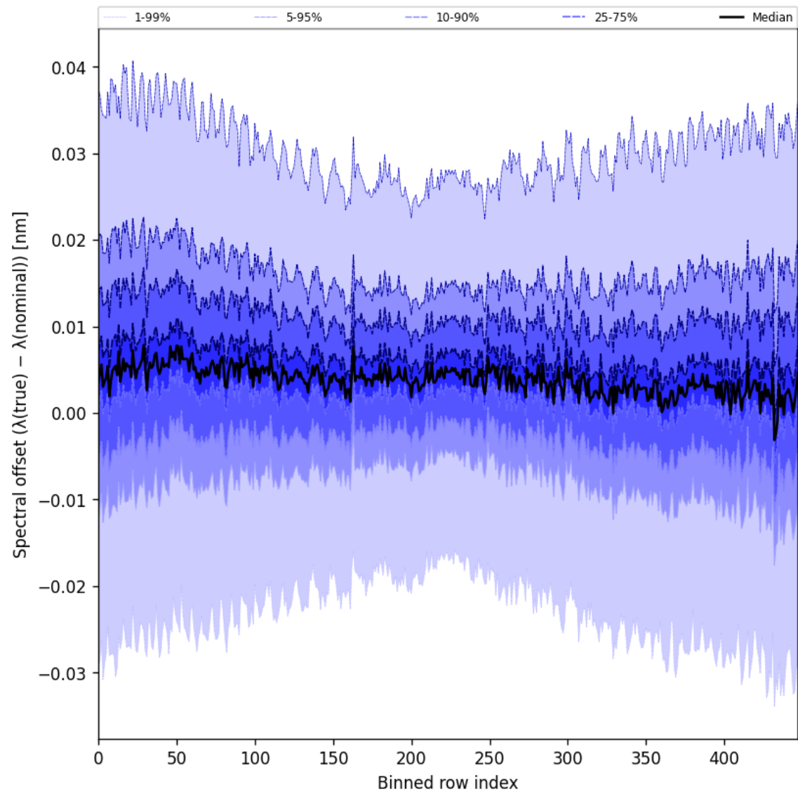
Figure 60: Along track statistics of “Spectral offset ( \lambda_{\text{true}} - \lambda_{\text{nominal}} )” for 2025-06-09 to 2025-06-09
