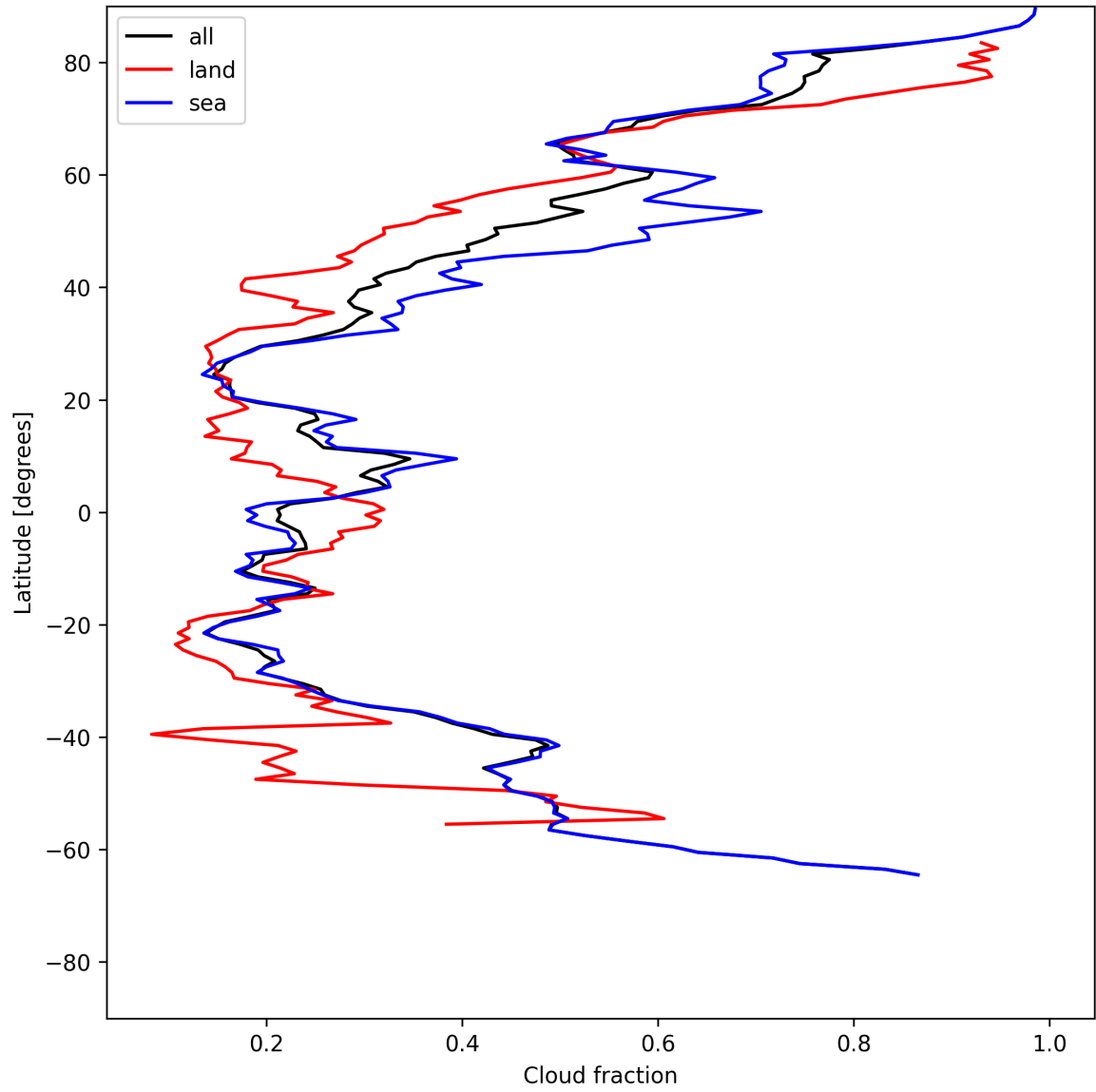
Figure 13: Zonal average of “Cloud fraction” for 2025-06-09 to 2025-06-09.
