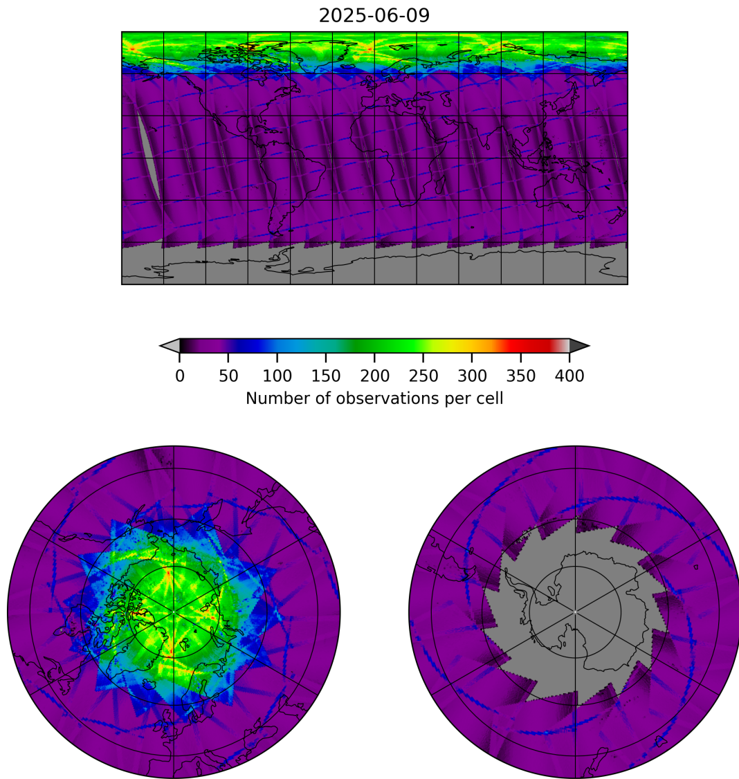
Figure 9: Map of the number of observations for 2025-06-09 to 2025-06-09
