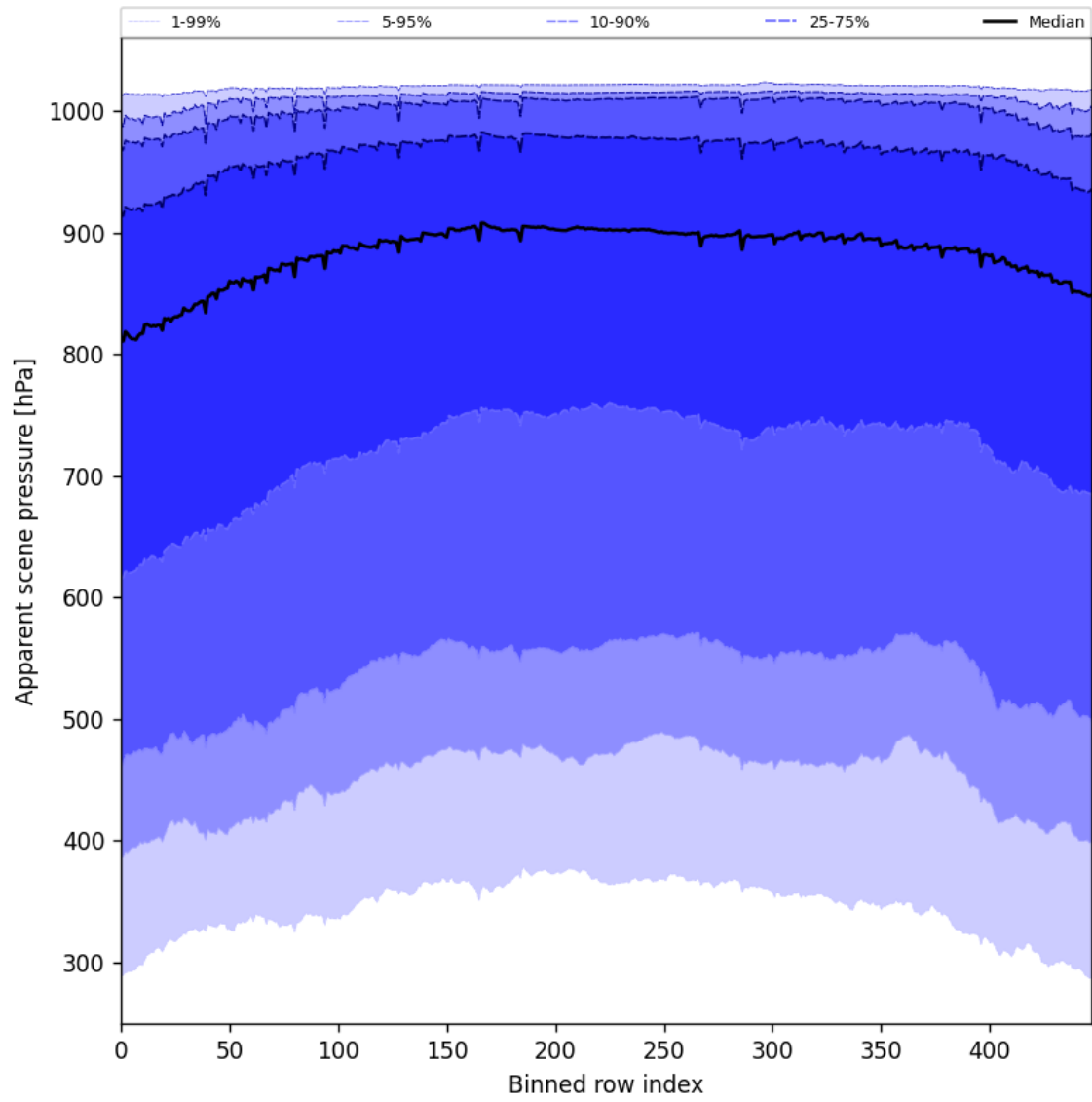
Figure 51: Along track statistics of “Apparent scene pressure” for 2025-06-09 to 2025-06-09
