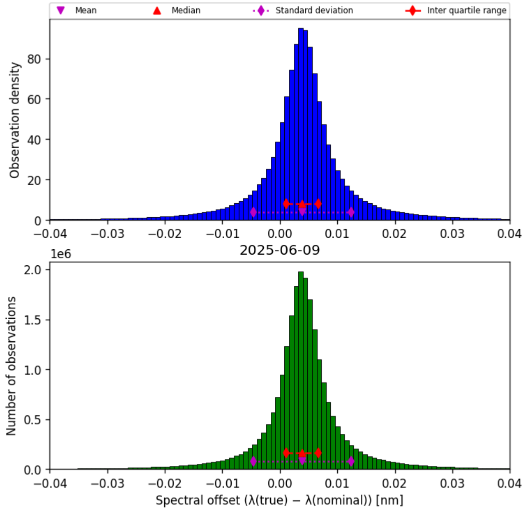
Figure 43: Histogram of “Spectral offset ( \lambda_{\text{true}} - \lambda_{\text{nominal}} )” for 2025-06-09 to 2025-06-09
