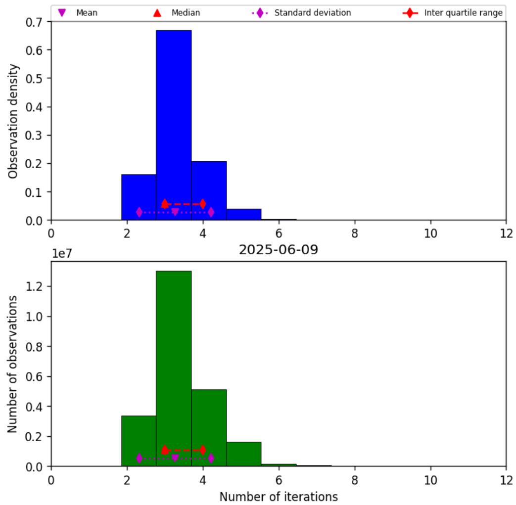
Figure 37: Histogram of “Number of iterations” for 2025-06-09 to 2025-06-09
