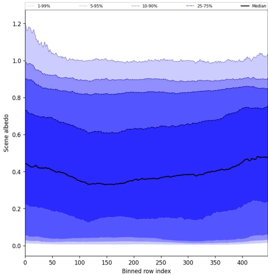
Figure 49: Along track statistics of “Scene albedo” for 2025-06-09 to 2025-06-09
