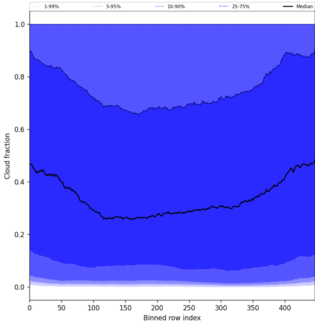
Figure 47: Along track statistics of “Cloud fraction” for 2025-06-09 to 2025-06-09
