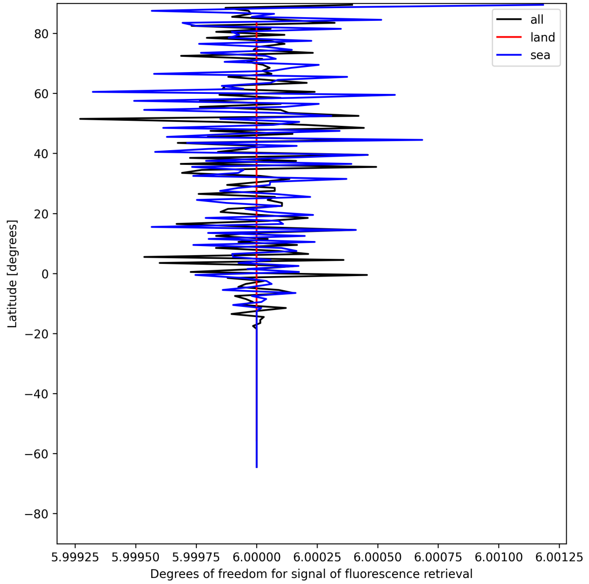
Figure 24: Zonal average of “Degrees of freedom for signal of fluorescence retrieval” for 2025-06-09 to 2025-06-09.
