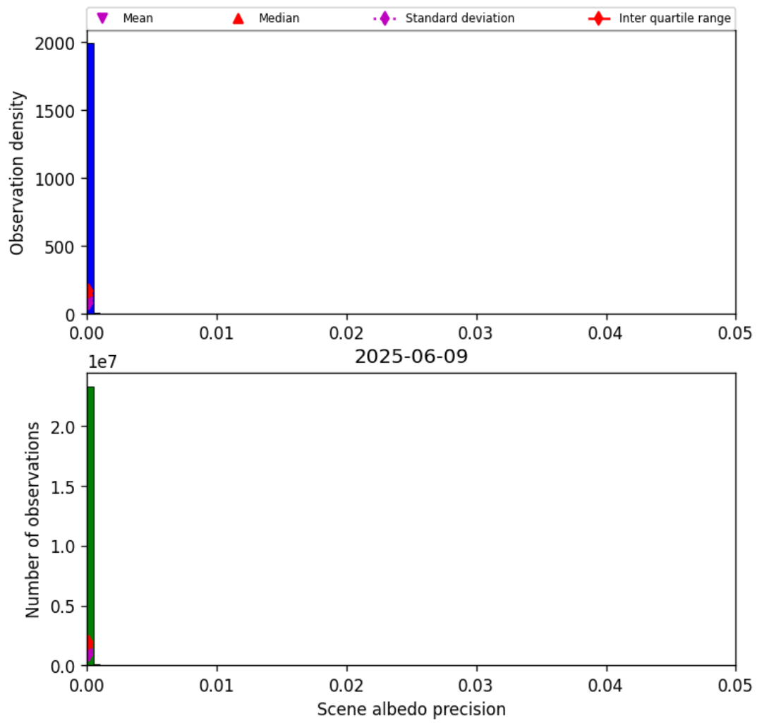
Figure 33: Histogram of “Scene albedo precision” for 2025-06-09 to 2025-06-09
