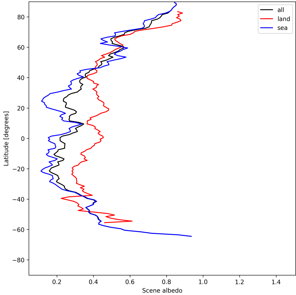
Figure 15: Zonal average of “Scene albedo” for 2025-06-09 to 2025-06-09.
