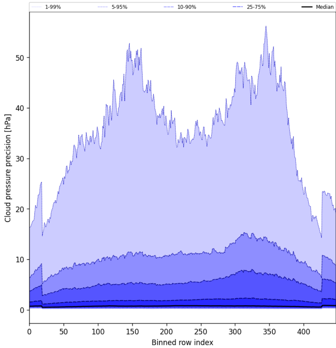
Figure 46: Along track statistics of “Cloud pressure precision” for 2025-06-09 to 2025-06-09
