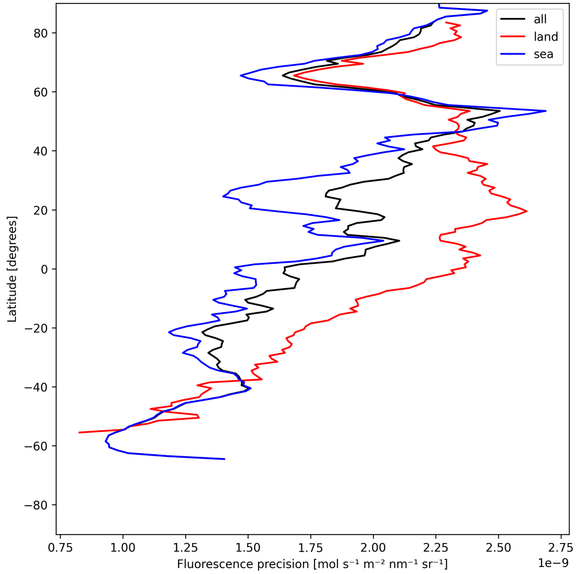
Figure 22: Zonal average of “Fluorescence precision” for 2025-06-09 to 2025-06-09.
