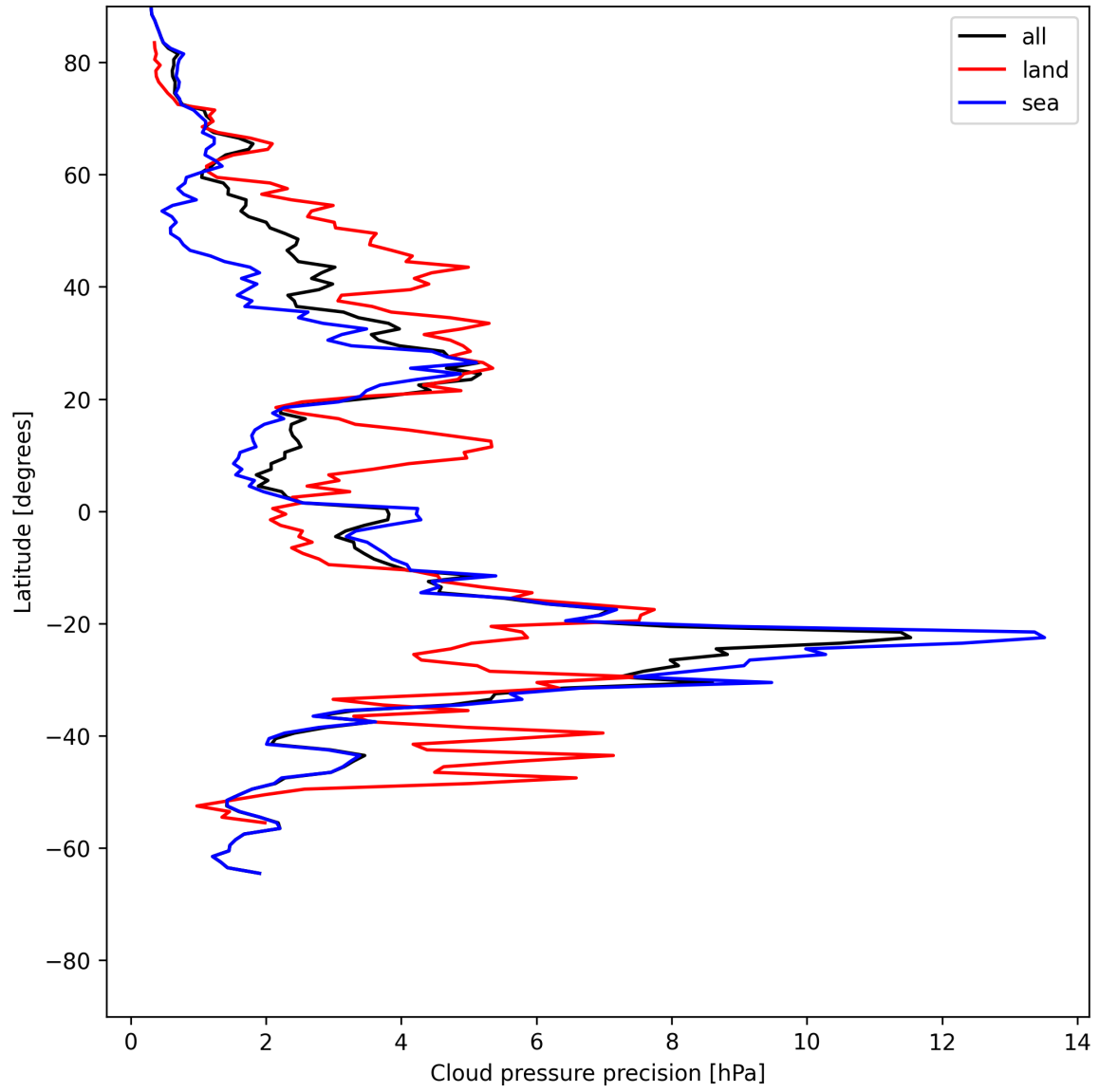
Figure 12: Zonal average of “Cloud pressure precision” for 2025-06-09 to 2025-06-09.
