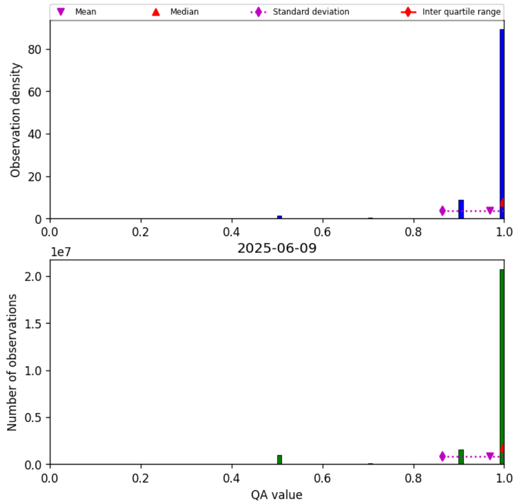
Figure 27: Histogram of “QA value” for 2025-06-09 to 2025-06-09
