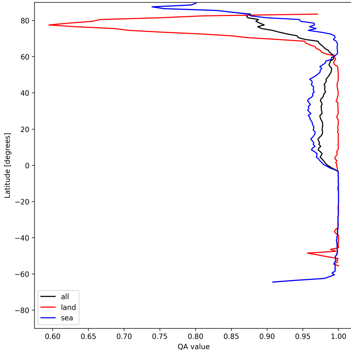
Figure 10: Zonal average of “QA value” for 2025-06-09 to 2025-06-09.
