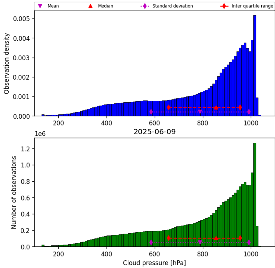
Figure 28: Histogram of “Cloud pressure” for 2025-06-09 to 2025-06-09
