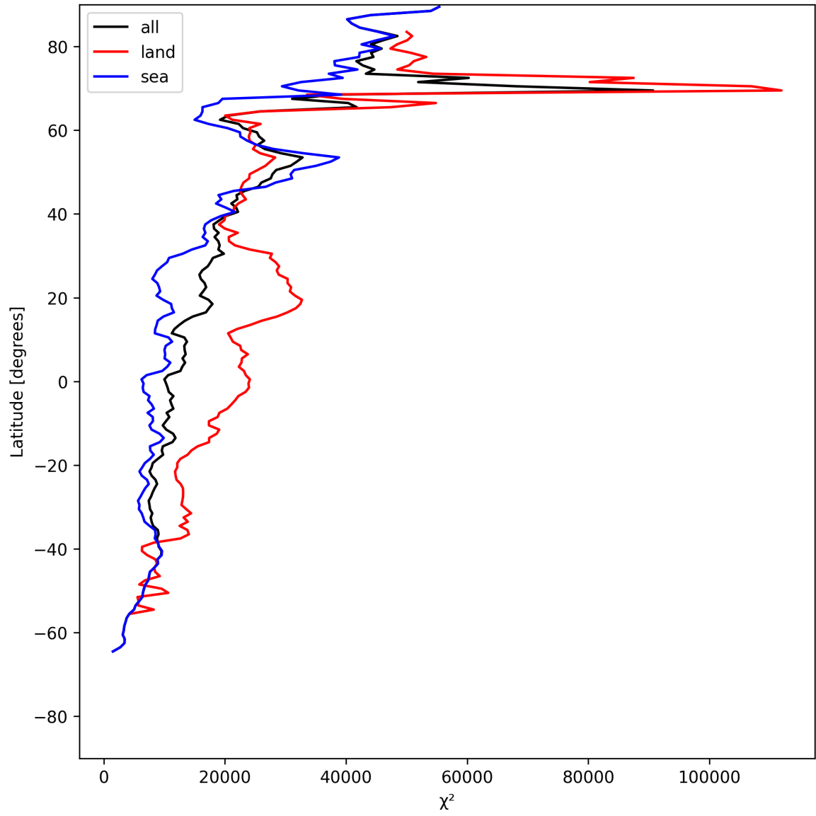
Figure 19: Zonal average of “ \chi^2 ” for 2025-06-09 to 2025-06-09.
