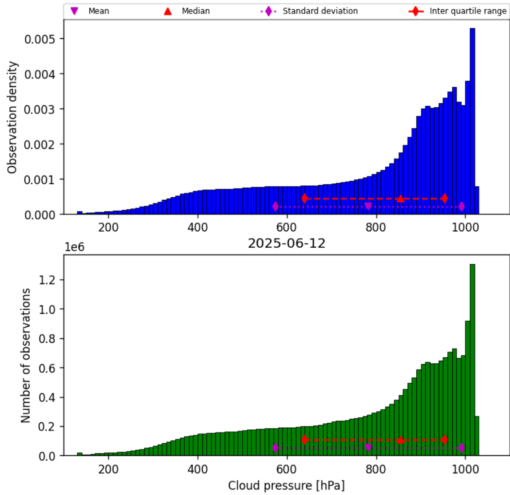
Figure 28: Histogram of “Cloud pressure” for 2025-06-12 to 2025-06-13
