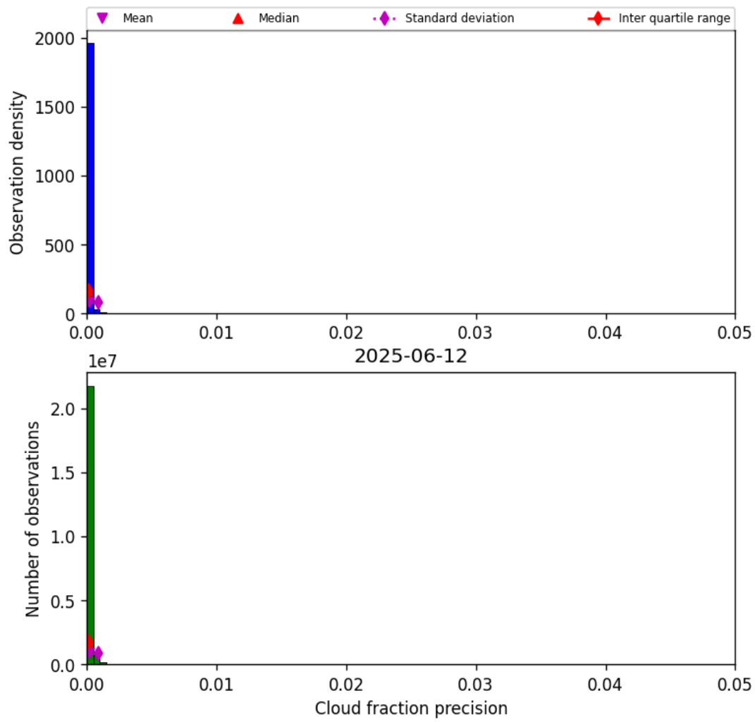
Figure 31: Histogram of “Cloud fraction precision” for 2025-06-12 to 2025-06-13
