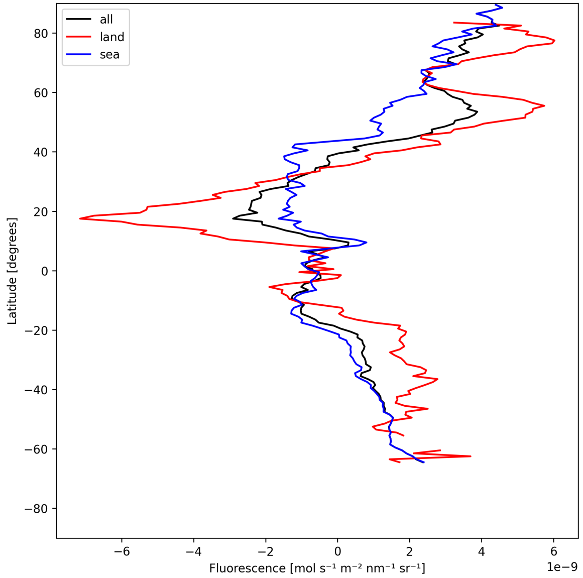
Figure 21: Zonal average of “Fluorescence” for 2025-06-12 to 2025-06-13.
