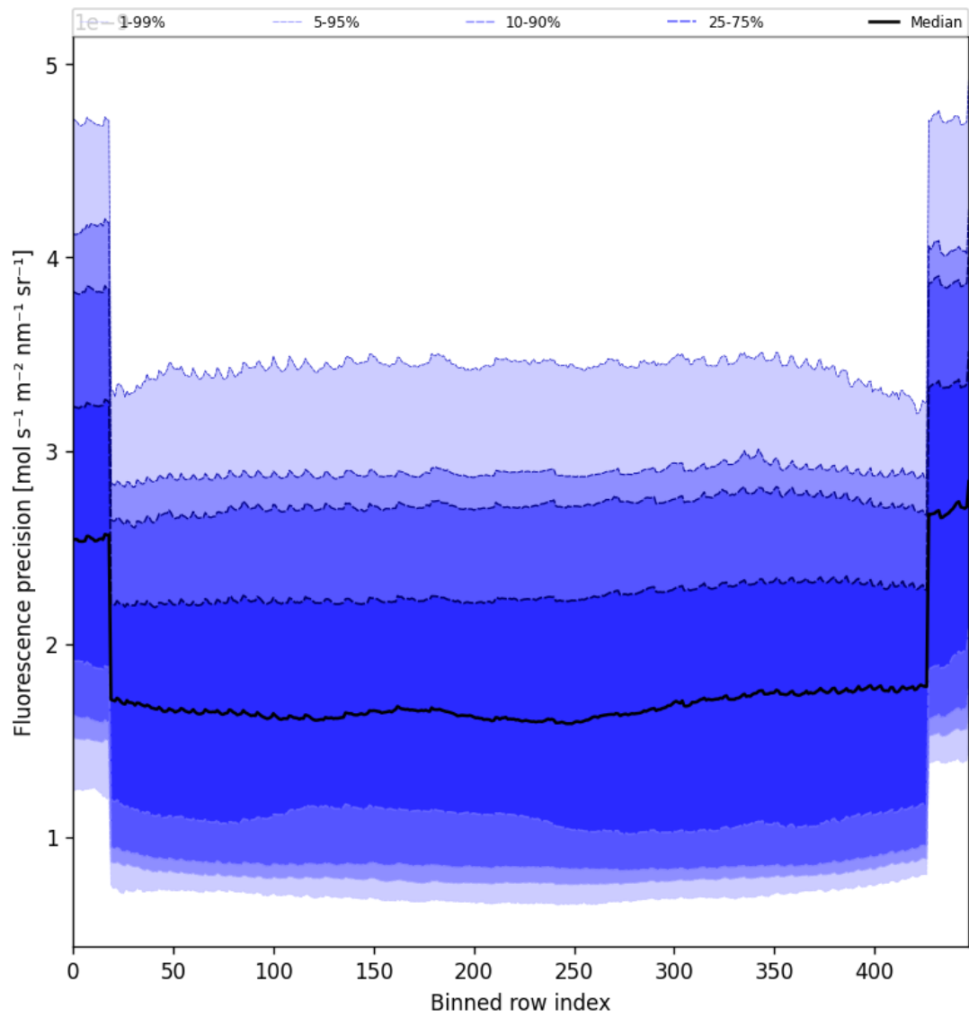
Figure 56: Along track statistics of “Fluorescence precision” for 2025-06-12 to 2025-06-13
