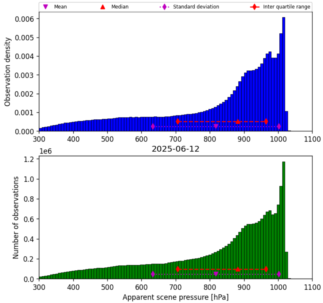
Figure 34: Histogram of “Apparent scene pressure” for 2025-06-12 to 2025-06-13
