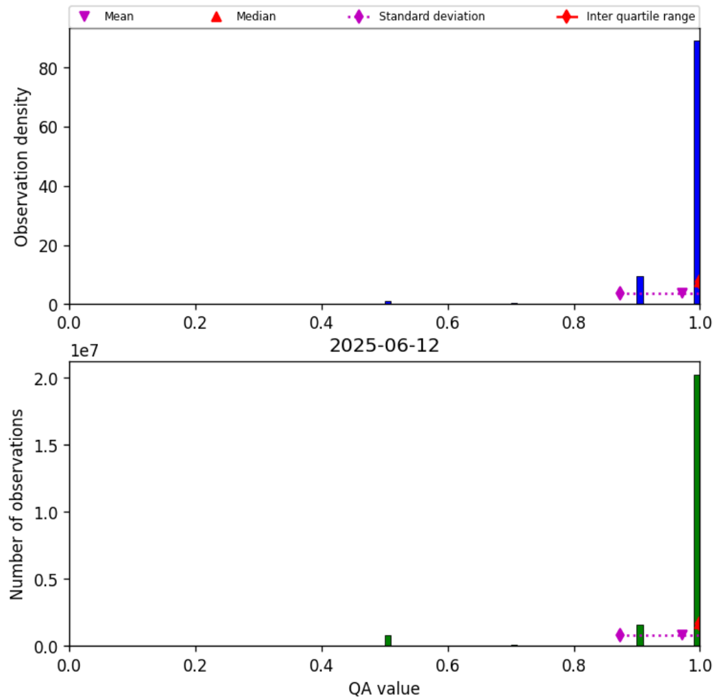
Figure 27: Histogram of “QA value” for 2025-06-12 to 2025-06-13
