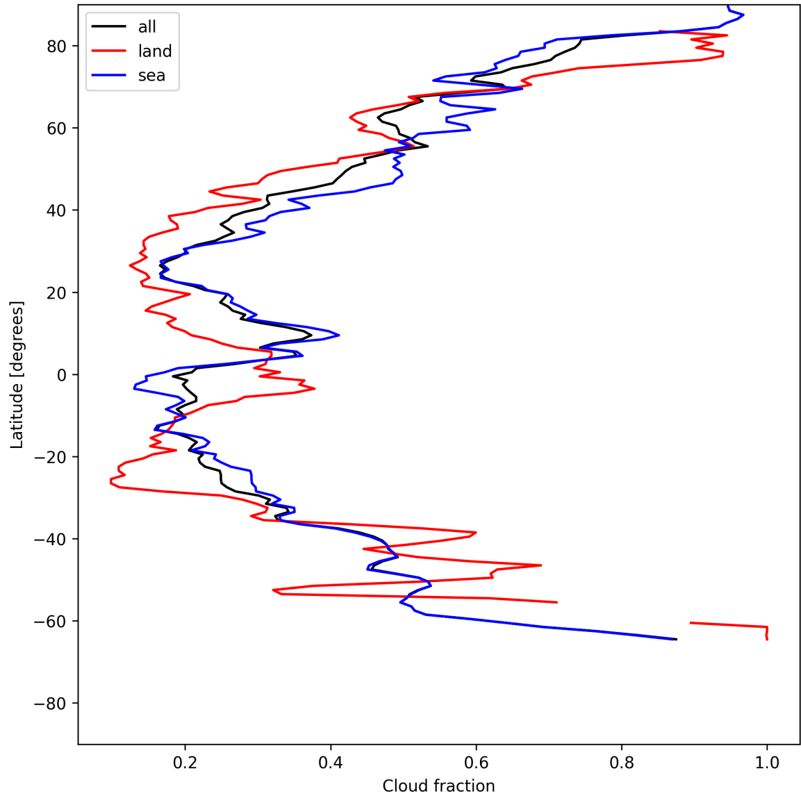
Figure 13: Zonal average of “Cloud fraction” for 2025-06-12 to 2025-06-13.
