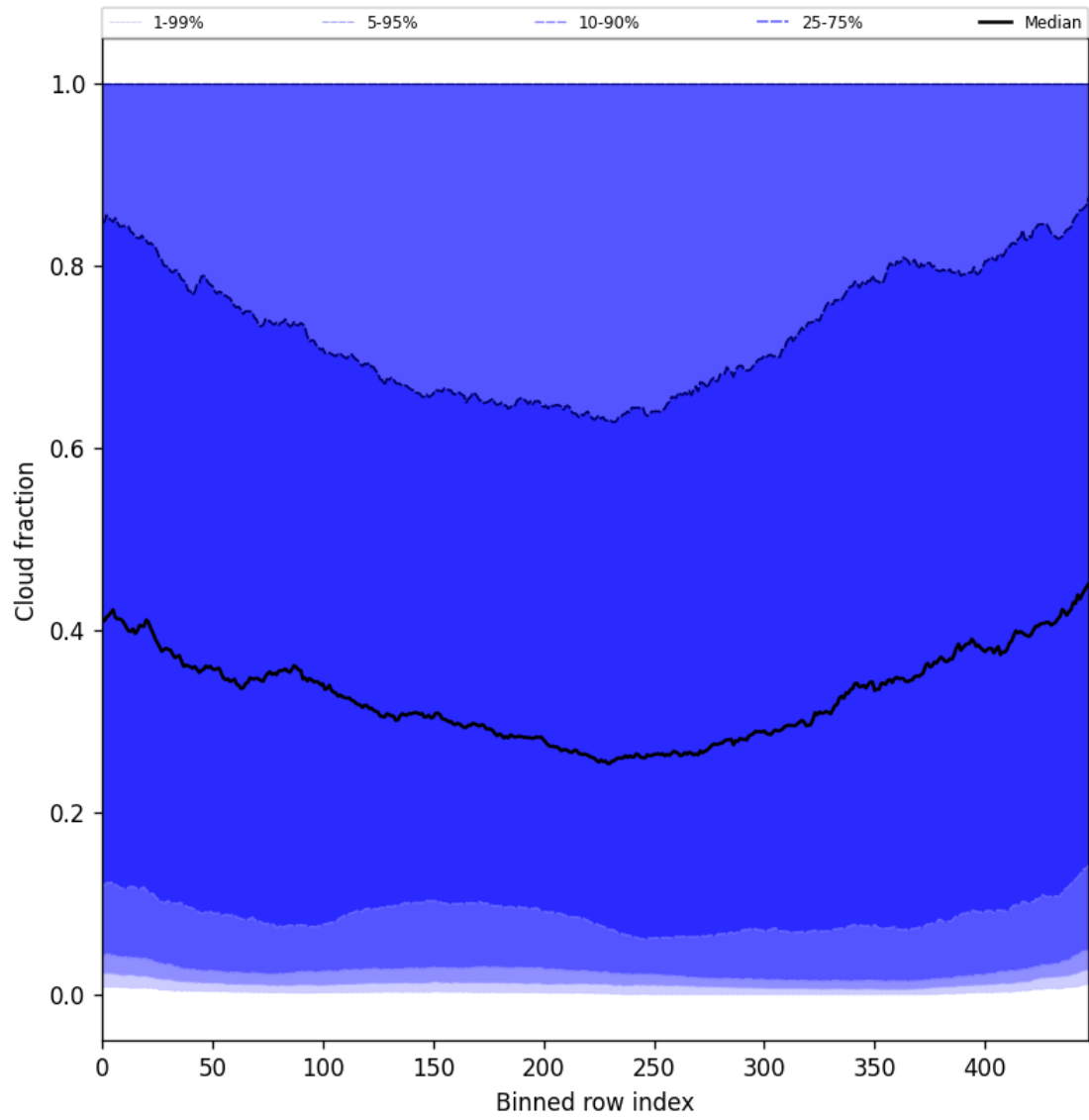
Figure 47: Along track statistics of “Cloud fraction” for 2025-06-12 to 2025-06-13
