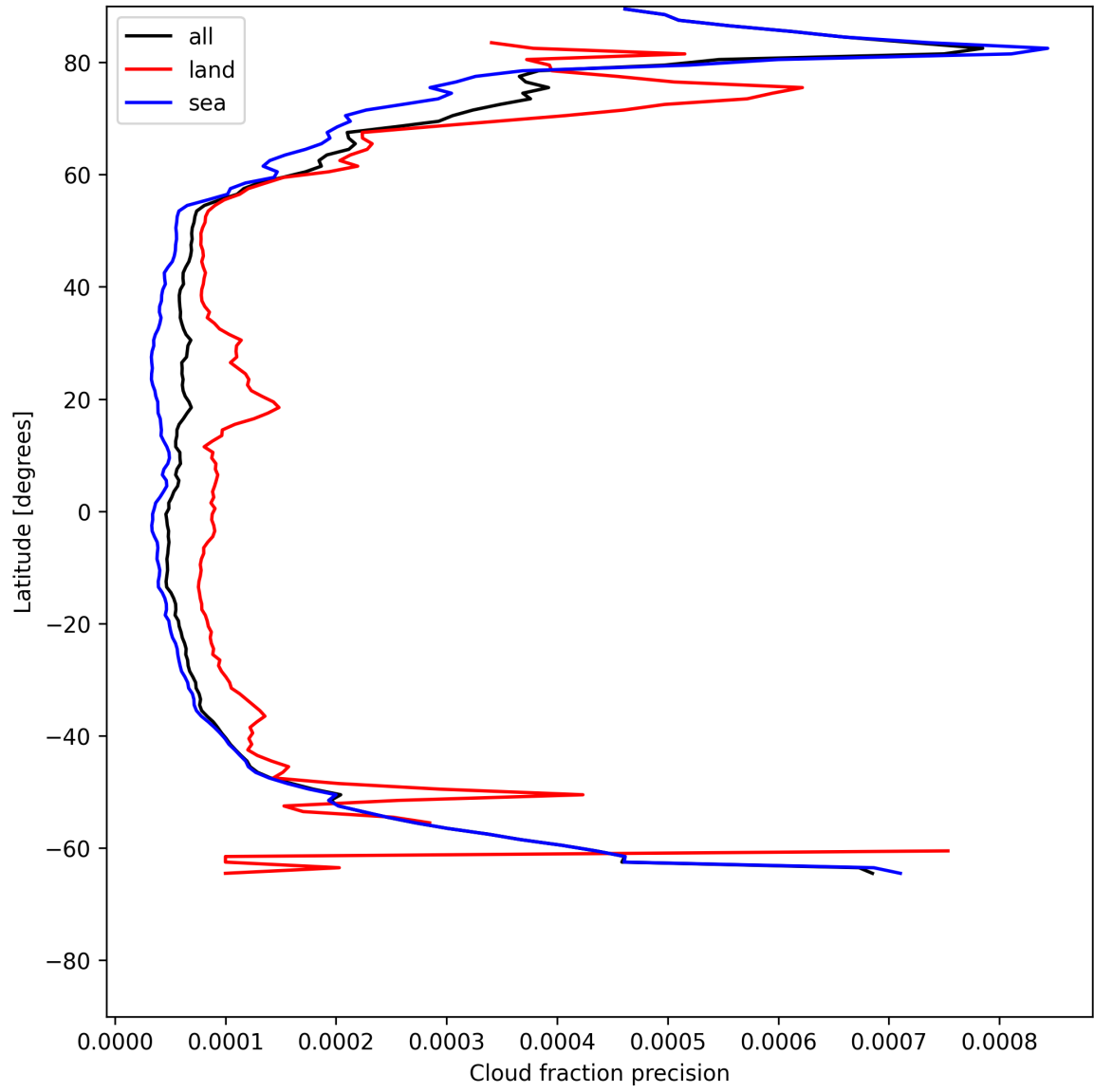
Figure 14: Zonal average of “Cloud fraction precision” for 2025-06-12 to 2025-06-13.
