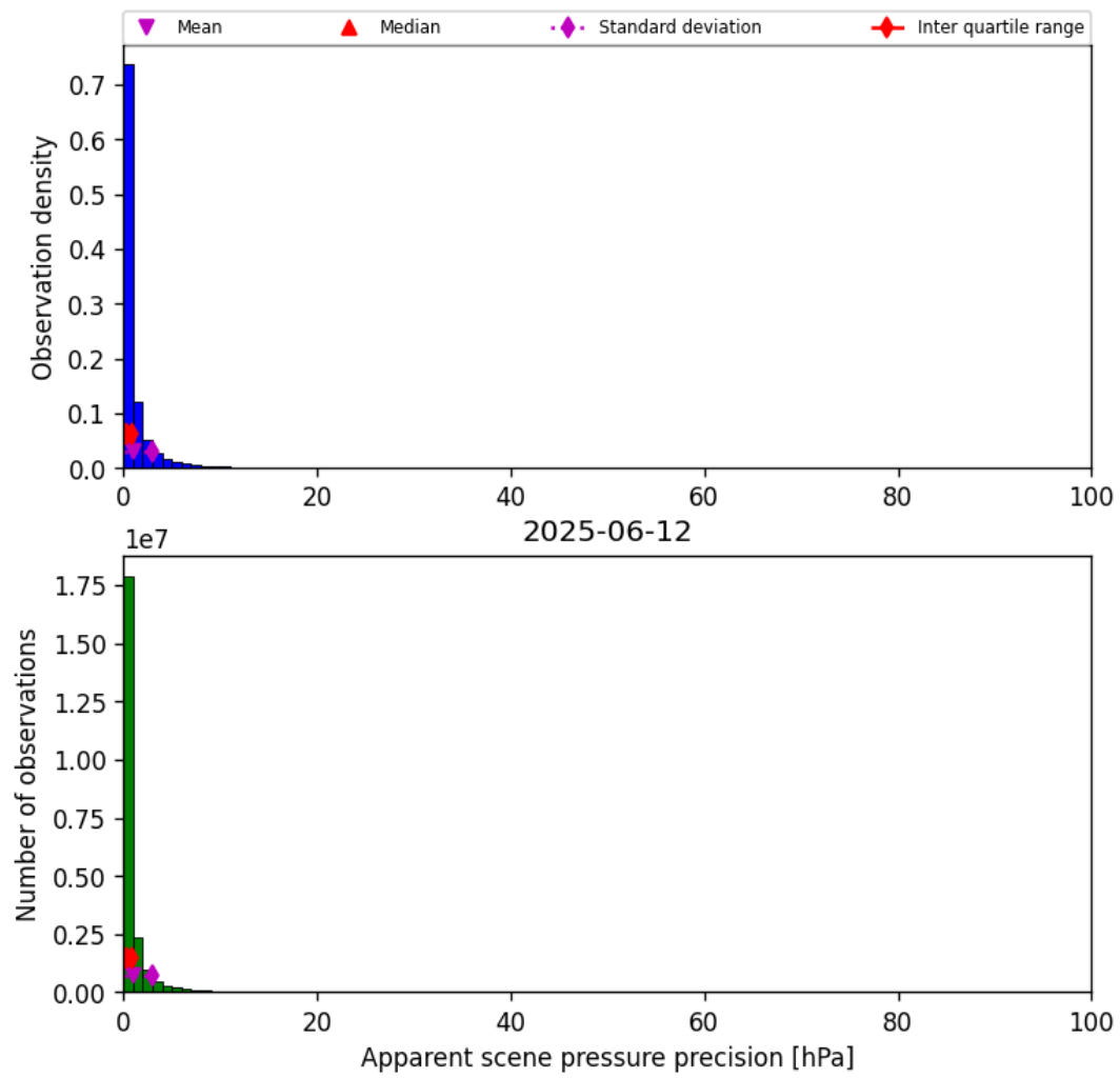
Figure 35: Histogram of “Apparent scene pressure precision” for 2025-06-12 to 2025-06-13
