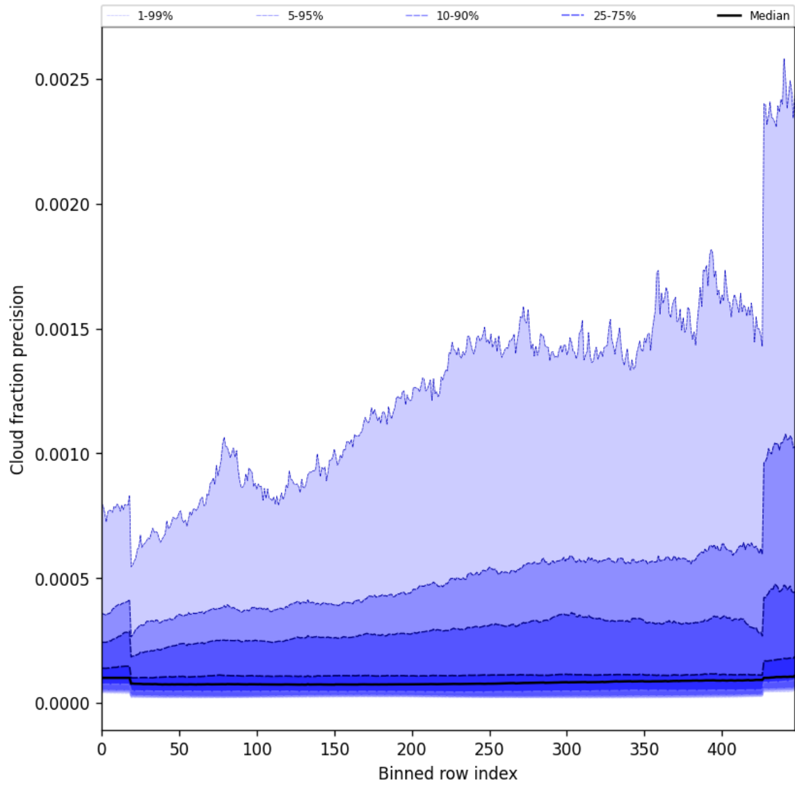
Figure 48: Along track statistics of “Cloud fraction precision” for 2025-06-12 to 2025-06-13
