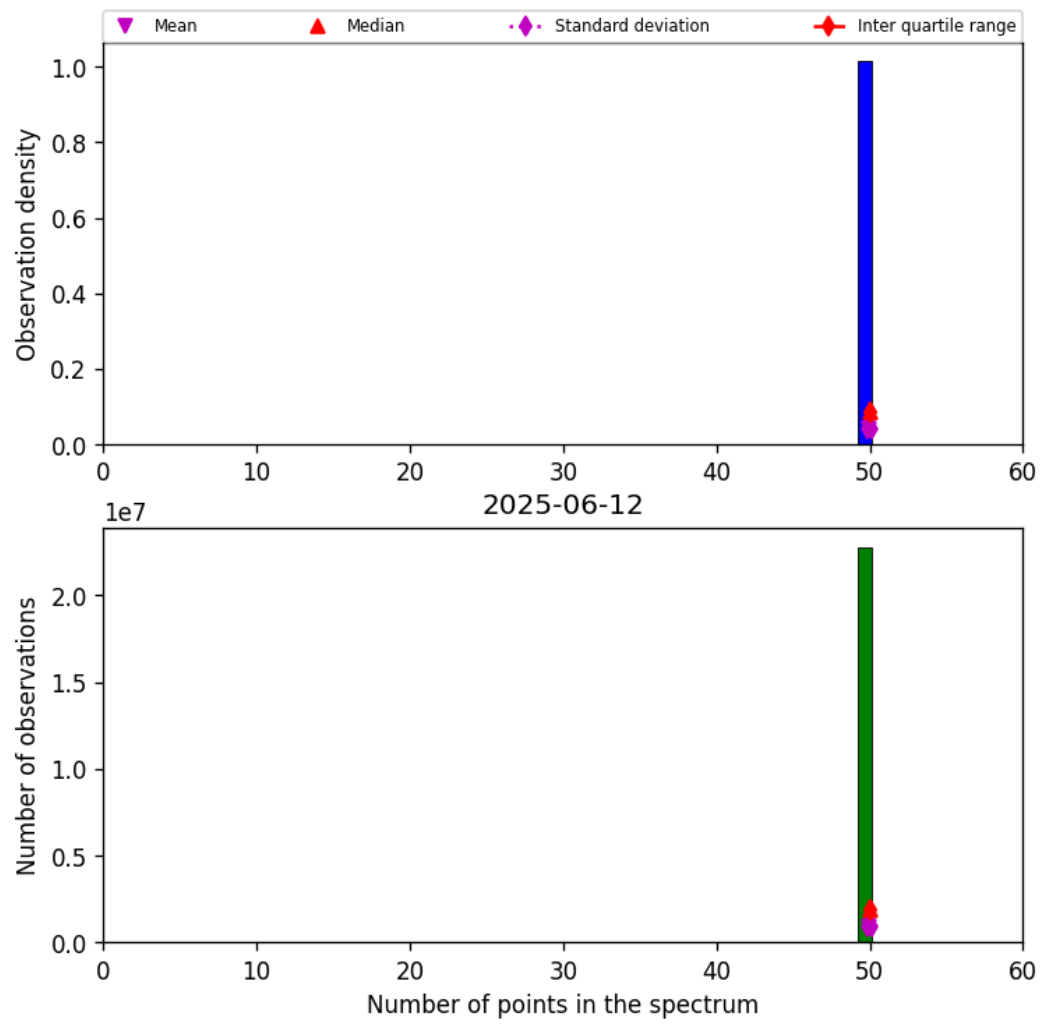
Figure 42: Histogram of “Number of points in the spectrum” for 2025-06-12 to 2025-06-13
