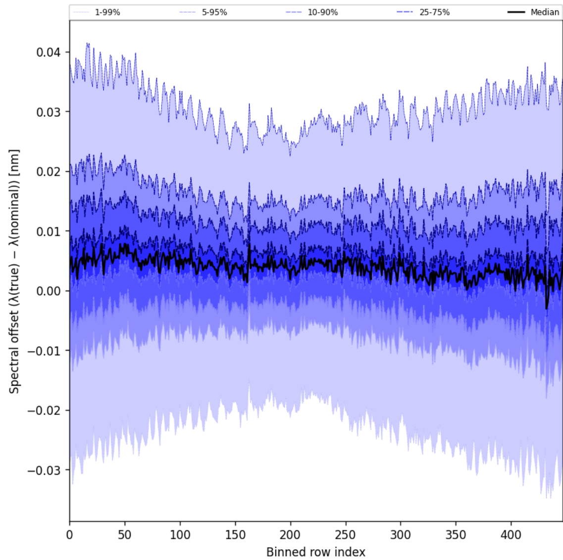
Figure 60: Along track statistics of “Spectral offset ( \lambda_{\text{true}} - \lambda_{\text{nominal}} )” for 2025-06-12 to 2025-06-13
