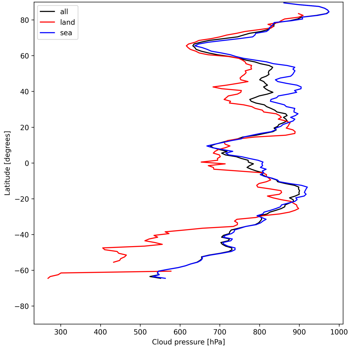
Figure 11: Zonal average of “Cloud pressure” for 2025-06-12 to 2025-06-13.
