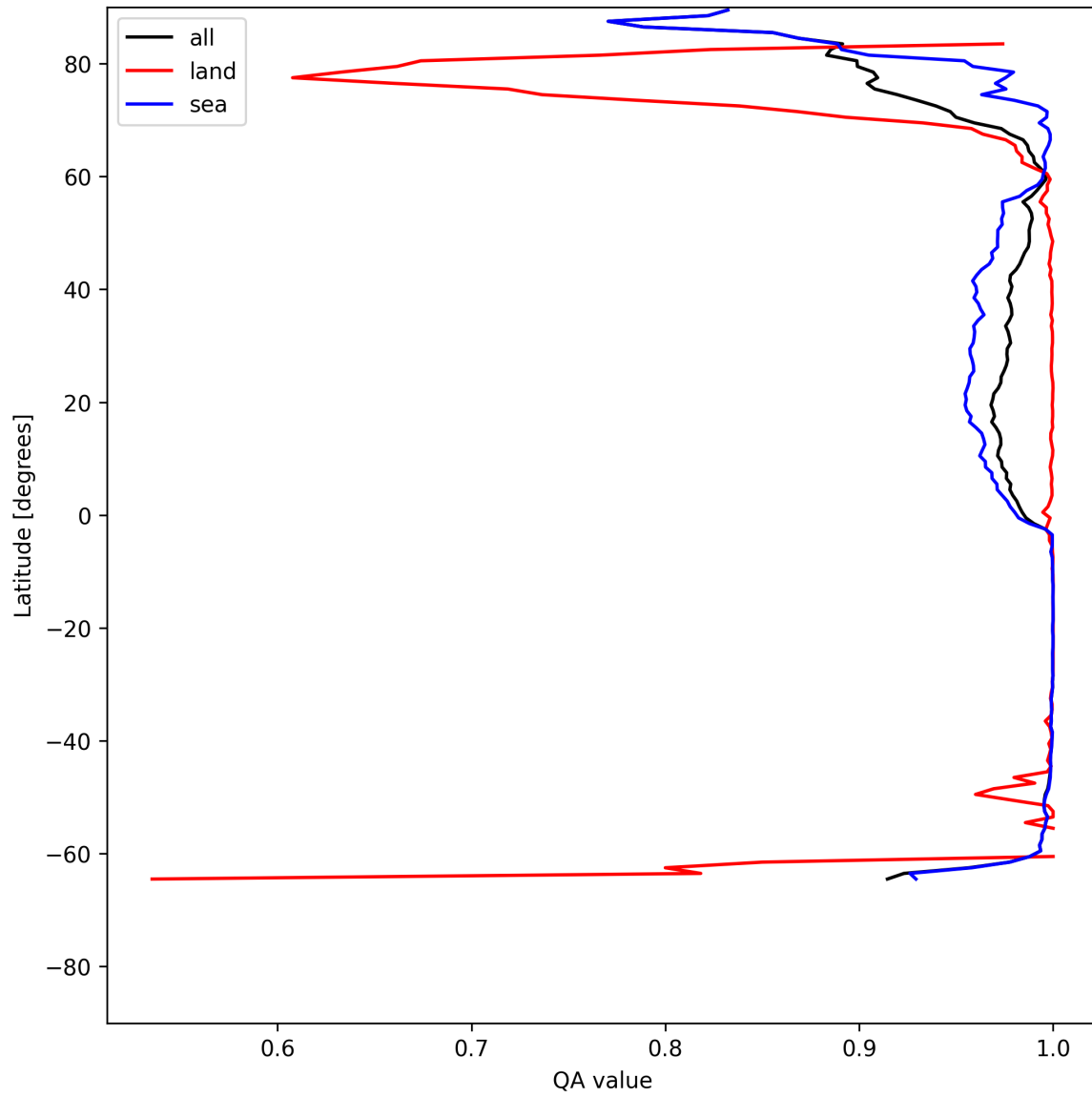
Figure 10: Zonal average of “QA value” for 2025-06-12 to 2025-06-13.
