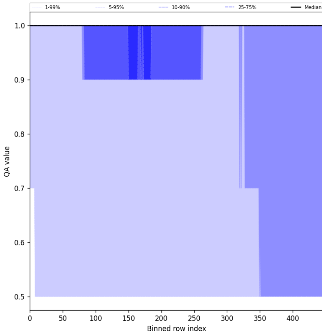
Figure 44: Along track statistics of “QA value” for 2025-06-12 to 2025-06-13
