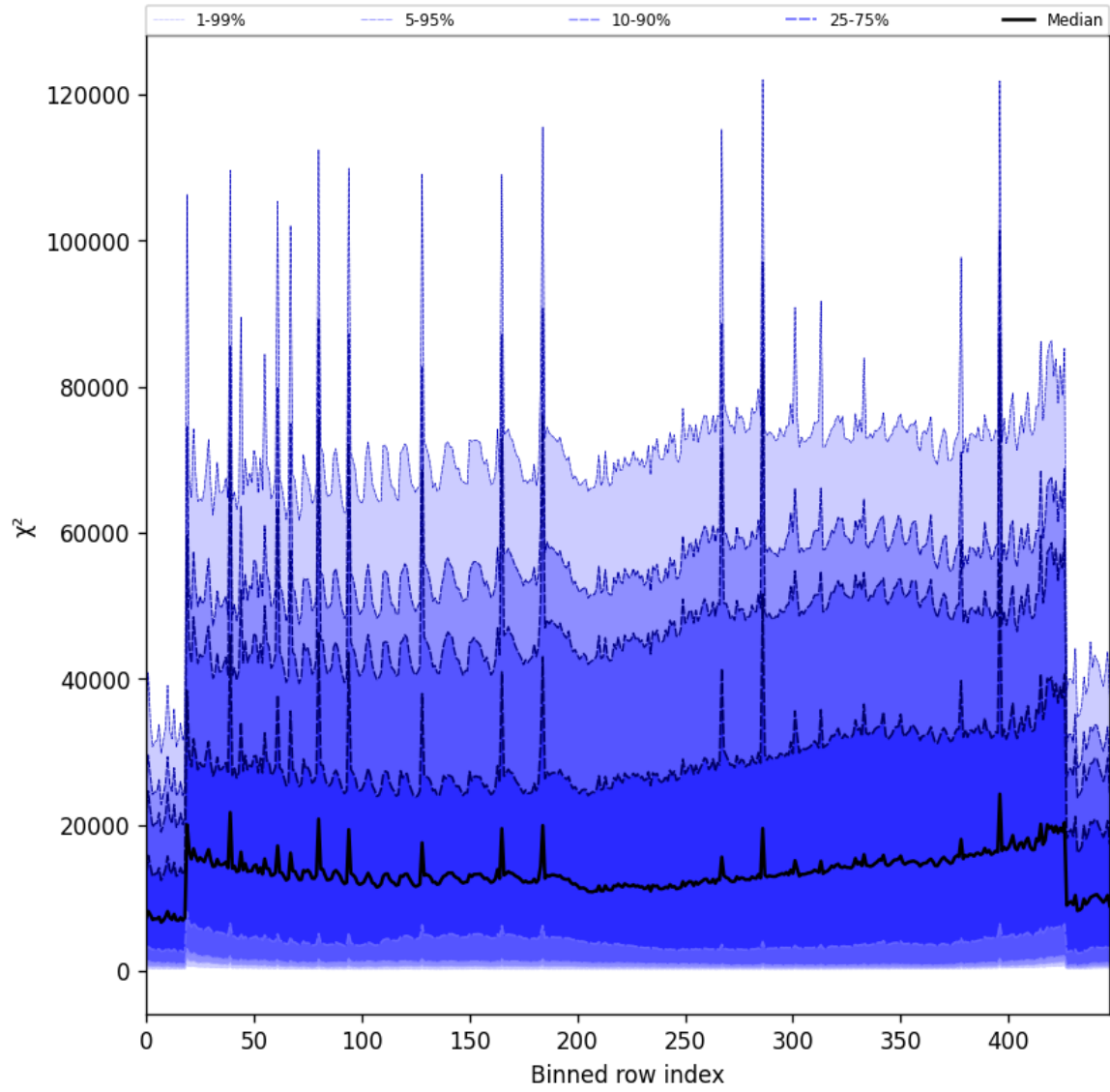
Figure 53: Along track statistics of “ \chi^2 ” for 2025-06-12 to 2025-06-13
