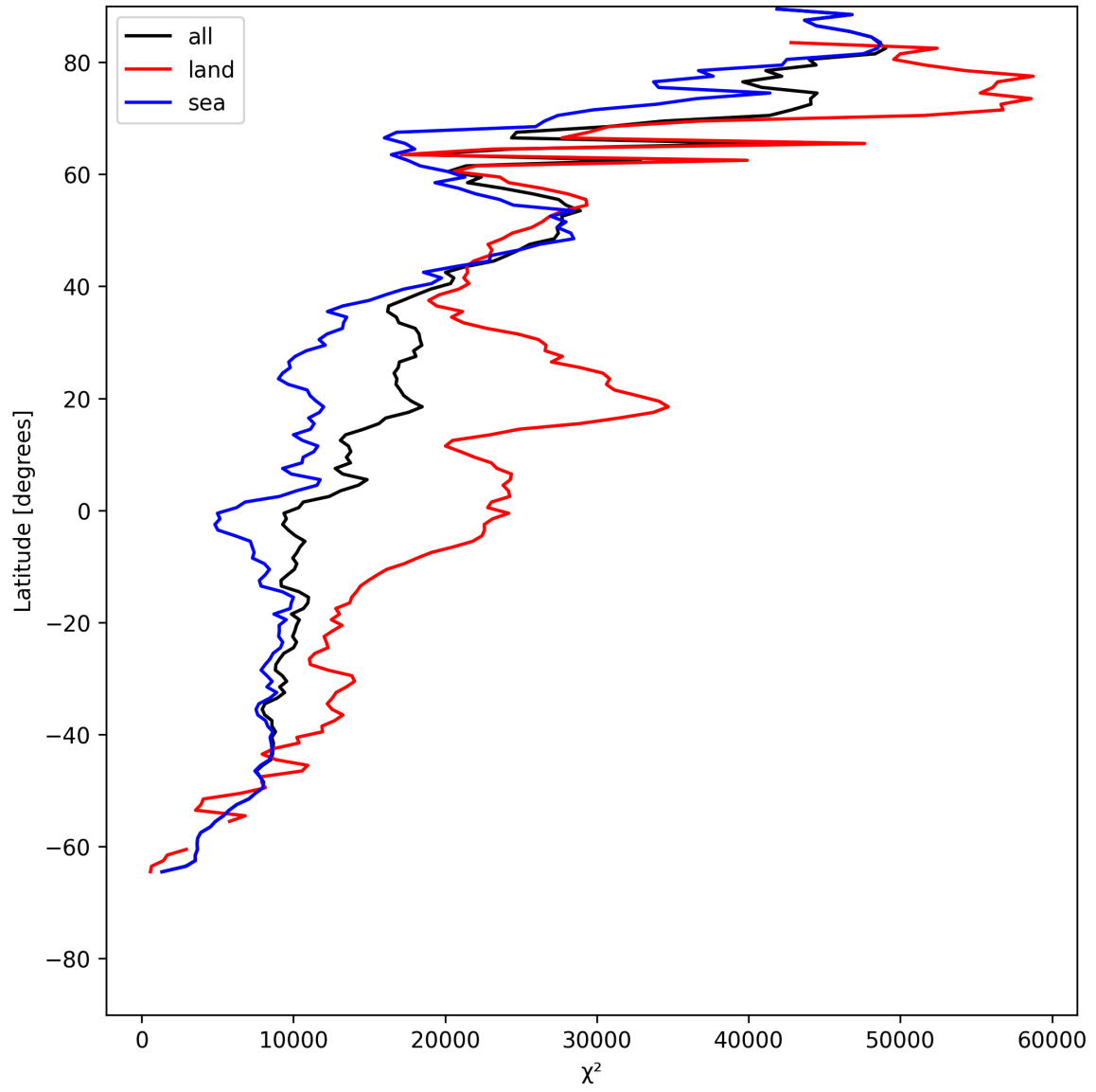
Figure 19: Zonal average of “ \chi^2 ” for 2025-06-12 to 2025-06-13.
