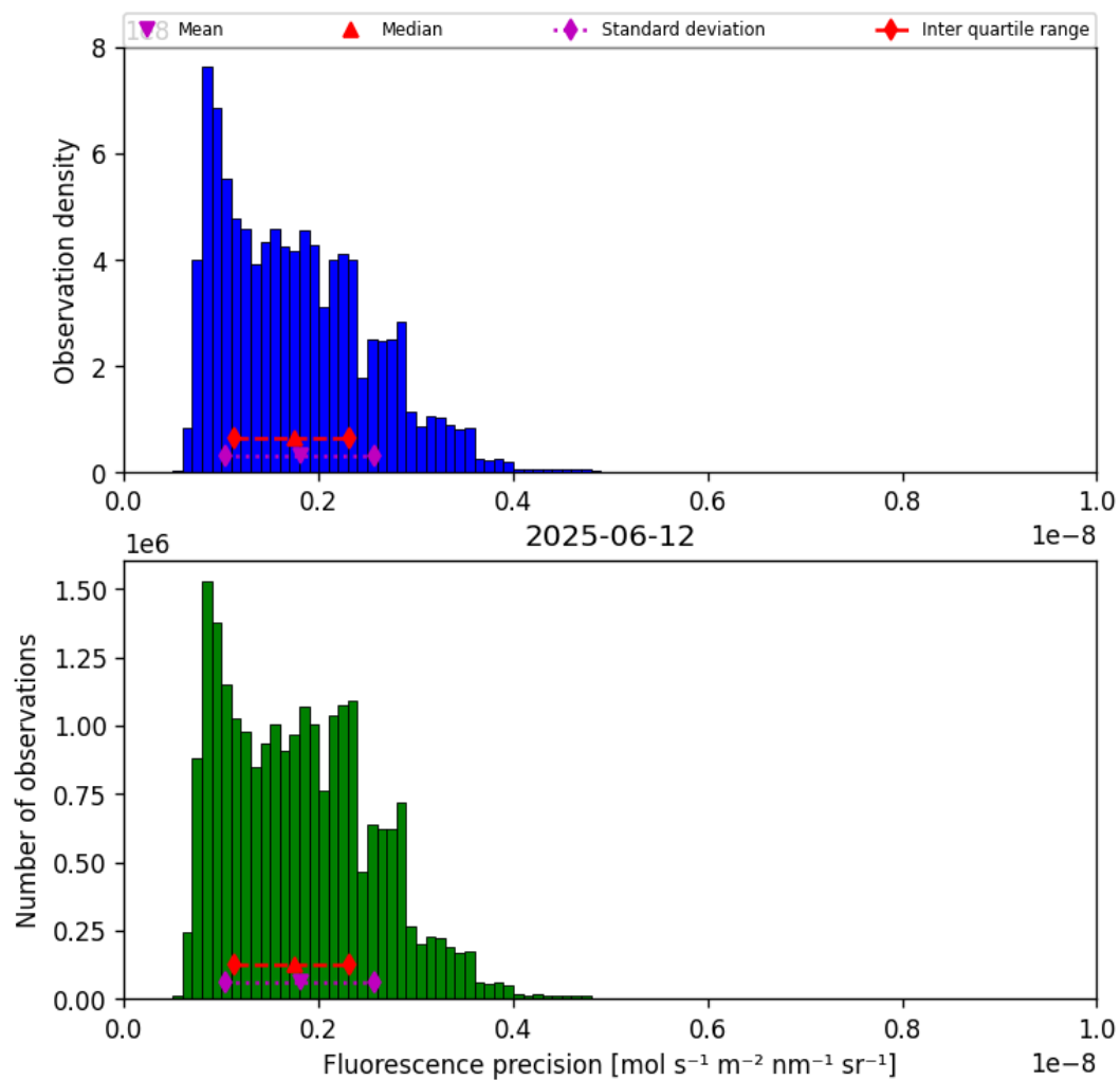
Figure 39: Histogram of “Fluorescence precision” for 2025-06-12 to 2025-06-13
