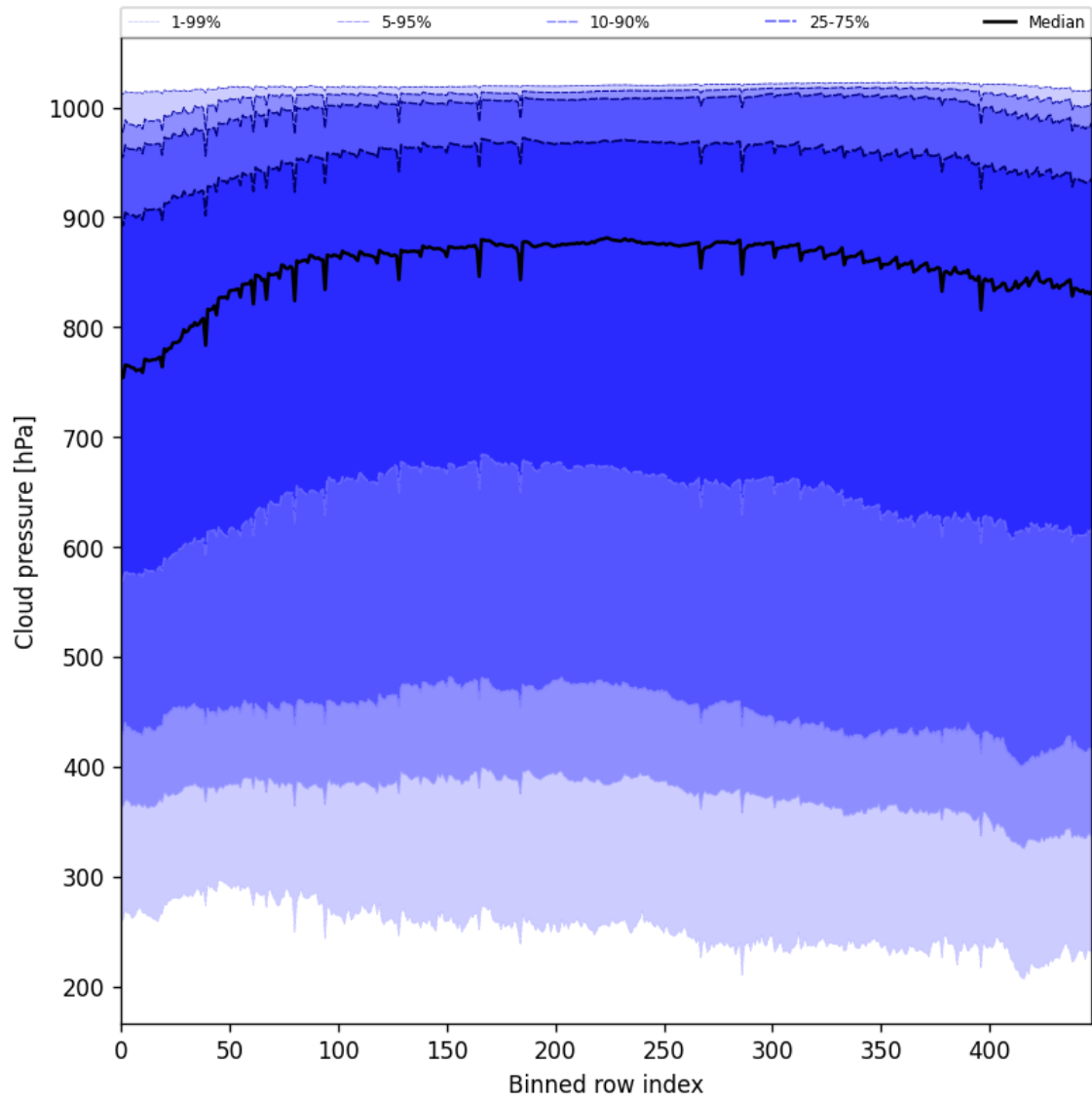
Figure 45: Along track statistics of “Cloud pressure” for 2025-06-12 to 2025-06-13
