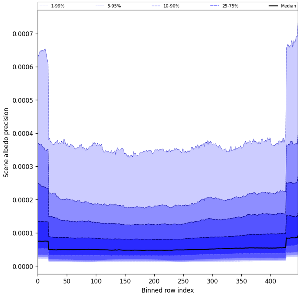
Figure 50: Along track statistics of “Scene albedo precision” for 2025-06-12 to 2025-06-13
