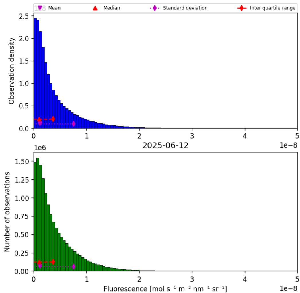
Figure 38: Histogram of “Fluorescence” for 2025-06-12 to 2025-06-13
