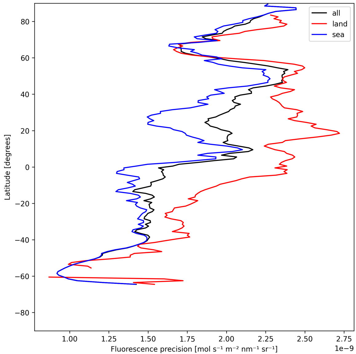
Figure 22: Zonal average of “Fluorescence precision” for 2025-06-12 to 2025-06-13.
