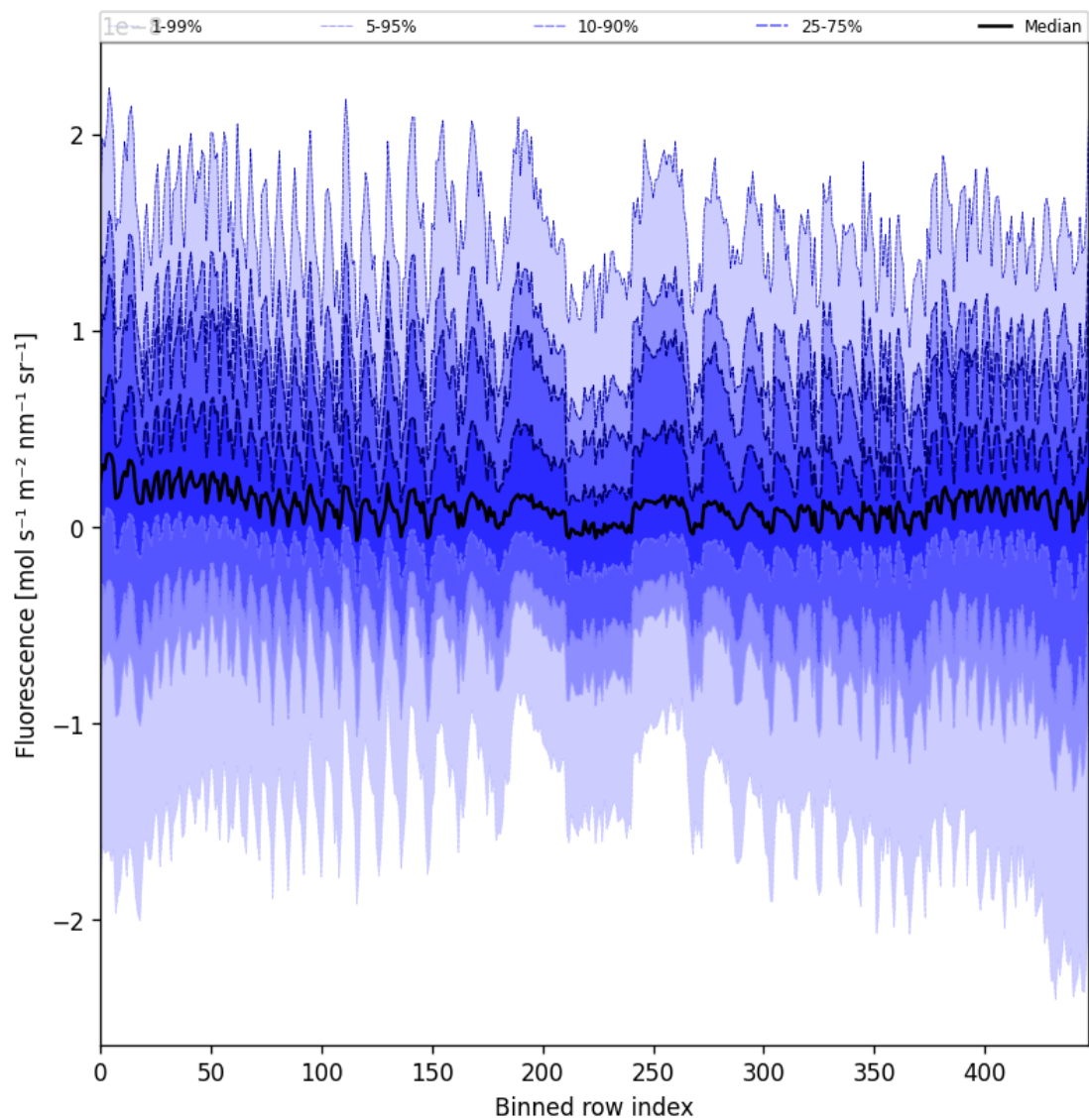
Figure 55: Along track statistics of "Fluorescence" for 2025-06-12 to 2025-06-13
