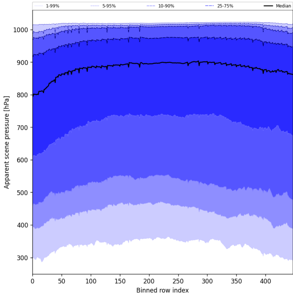
Figure 51: Along track statistics of “Apparent scene pressure” for 2025-06-12 to 2025-06-13
