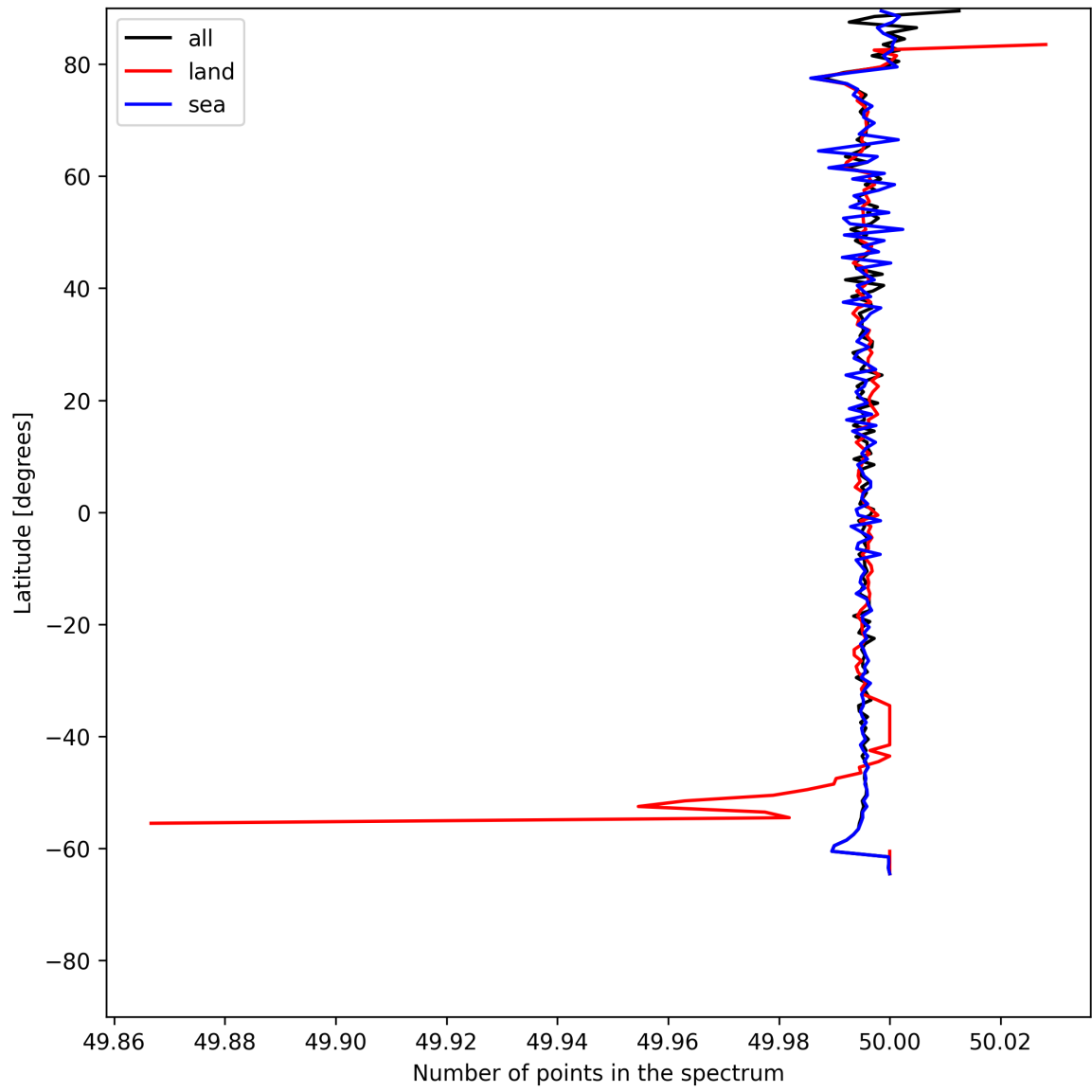
Figure 25: Zonal average of “Number of points in the spectrum” for 2025-06-12 to 2025-06-13.
