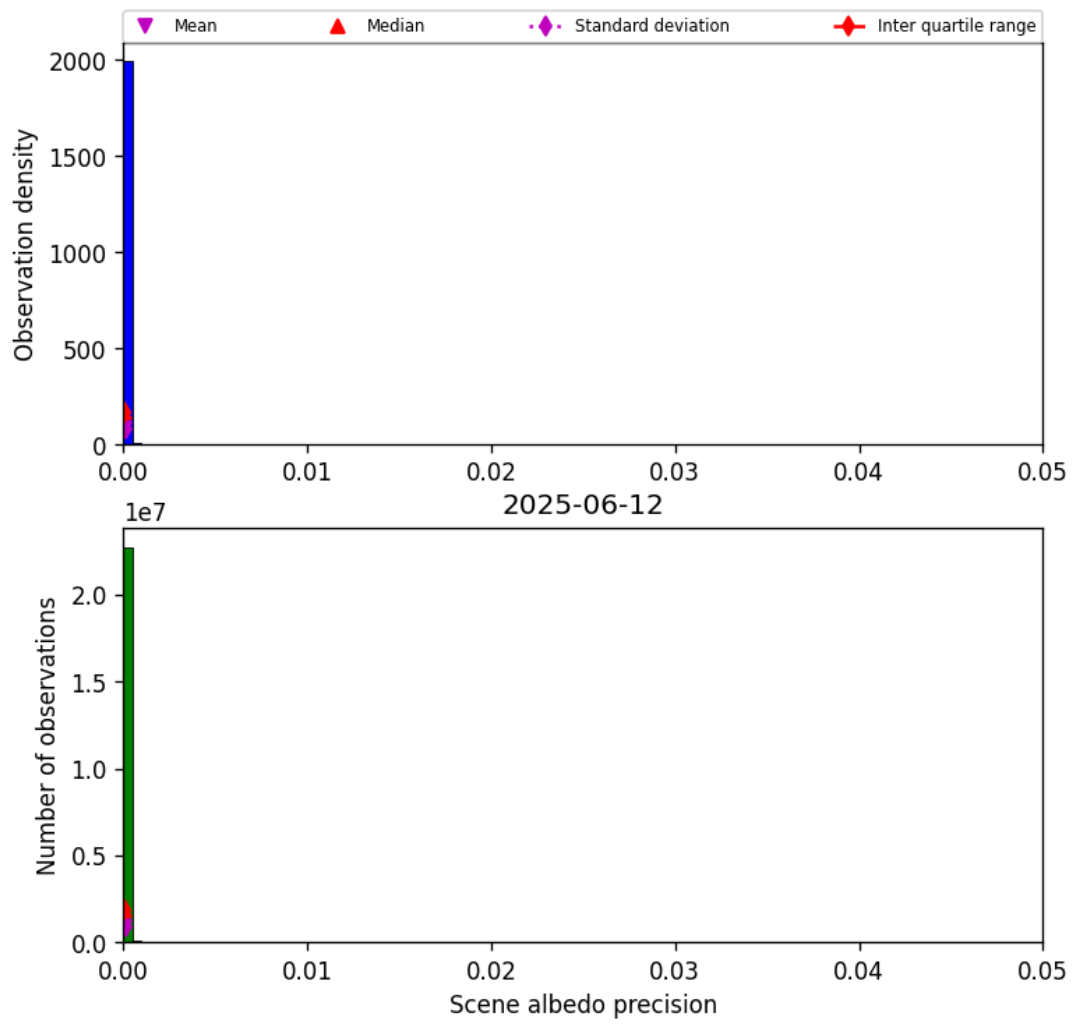
Figure 33: Histogram of “Scene albedo precision” for 2025-06-12 to 2025-06-13
