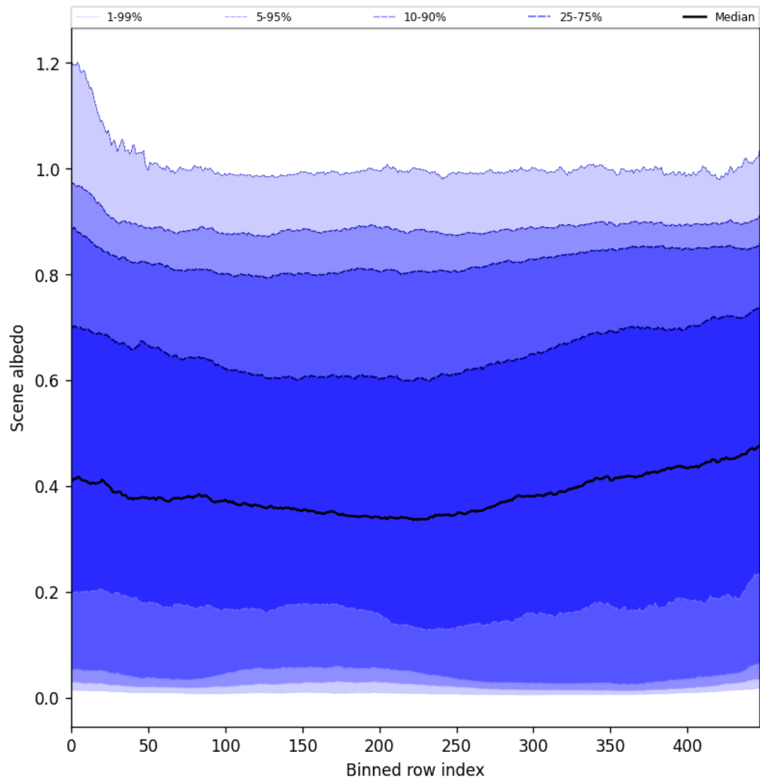
Figure 49: Along track statistics of “Scene albedo” for 2025-06-12 to 2025-06-13
