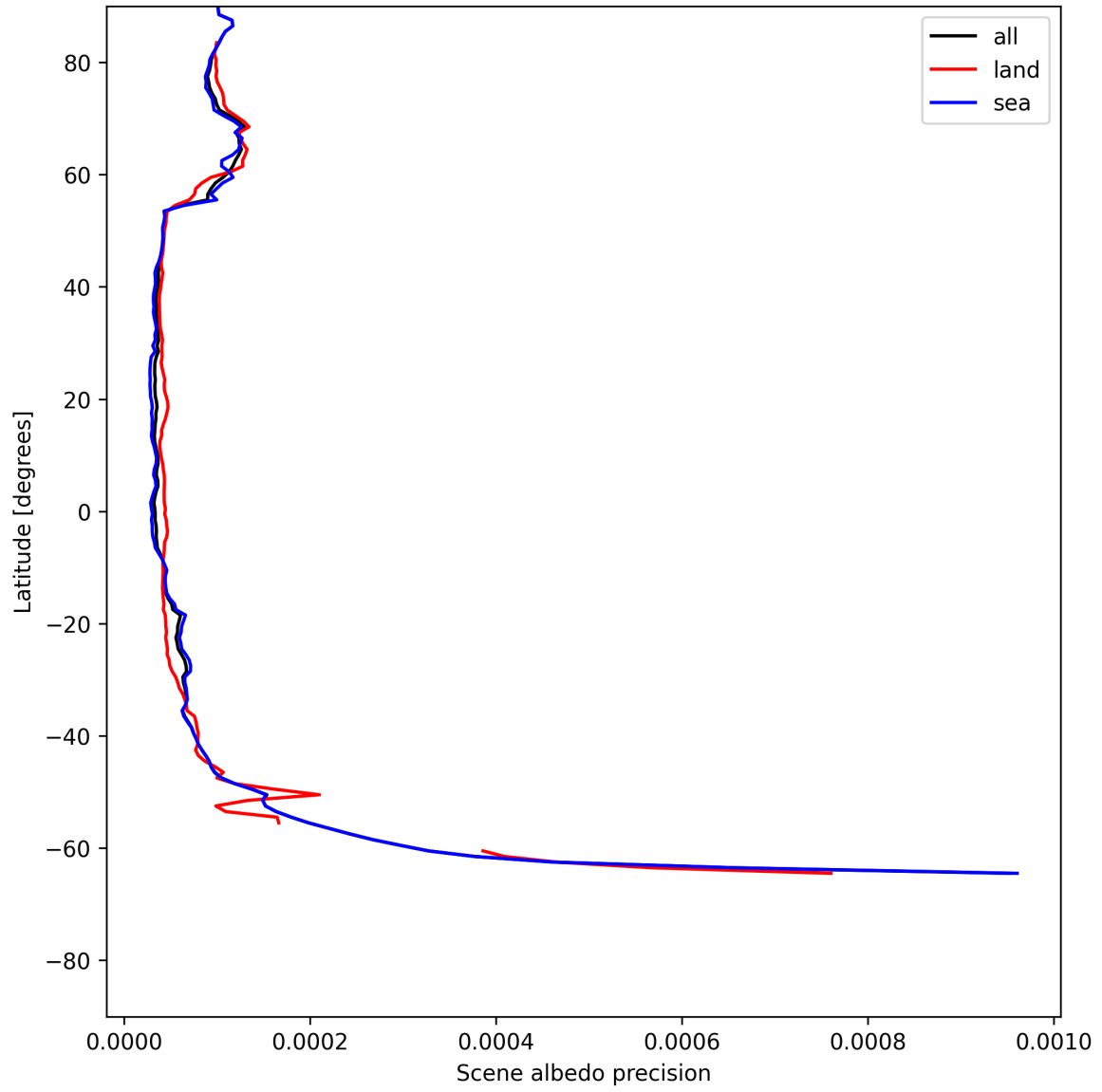
Figure 16: Zonal average of “Scene albedo precision” for 2025-06-12 to 2025-06-13.
