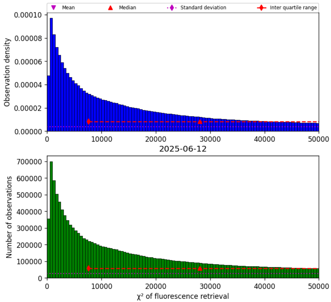
Figure 40: Histogram of “ \chi^2 of fluorescence retrieval” for 2025-06-12 to 2025-06-13
