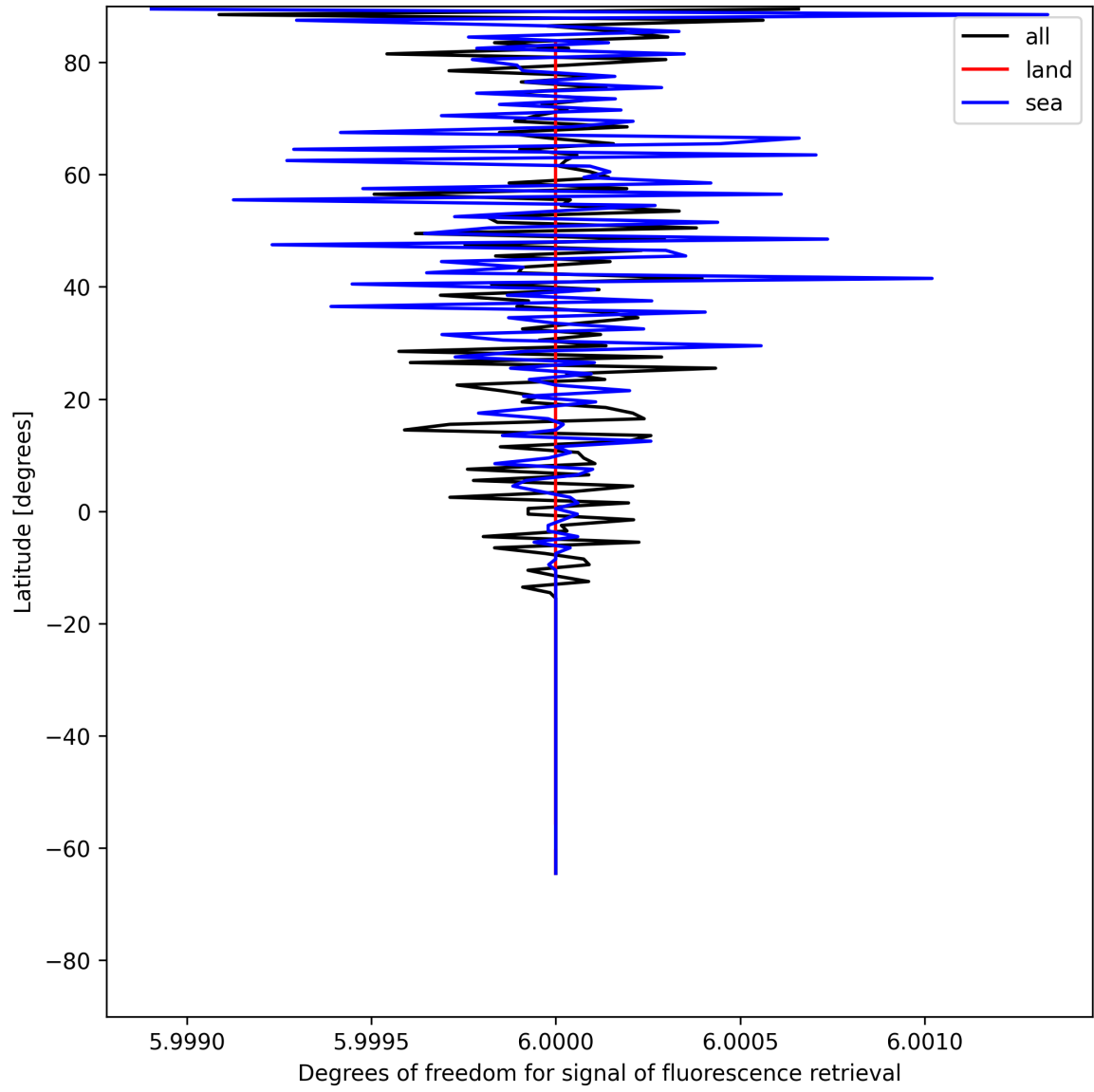
Figure 24: Zonal average of “Degrees of freedom for signal of fluorescence retrieval” for 2025-06-12 to 2025-06-13.
