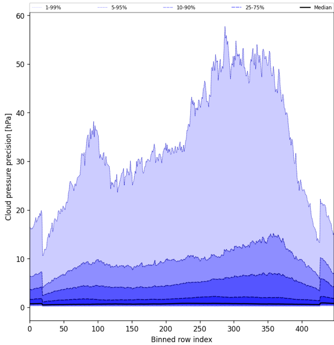
Figure 46: Along track statistics of “Cloud pressure precision” for 2025-06-12 to 2025-06-13
