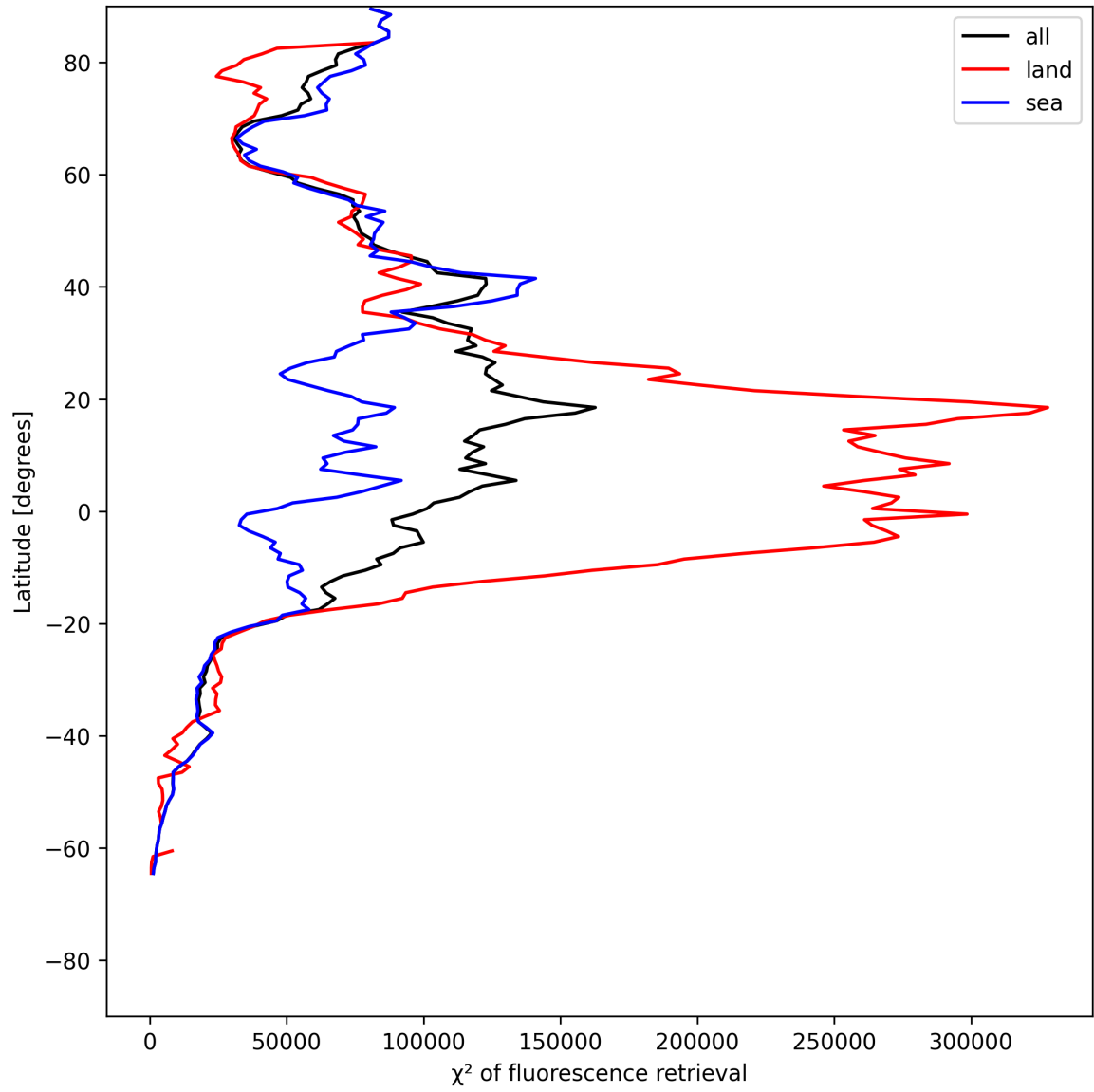
Figure 23: Zonal average of “ \chi^2 of fluorescence retrieval” for 2025-06-12 to 2025-06-13.
