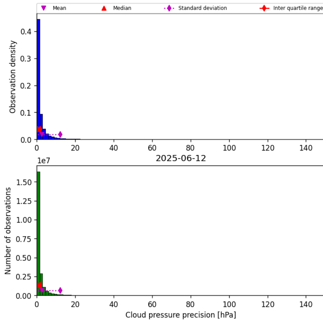
Figure 29: Histogram of “Cloud pressure precision” for 2025-06-12 to 2025-06-13
