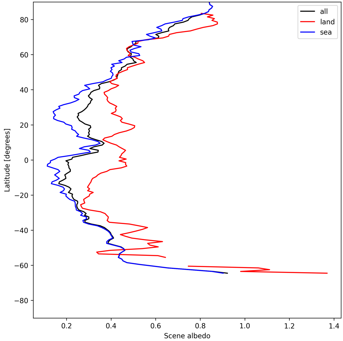
Figure 15: Zonal average of “Scene albedo” for 2025-06-12 to 2025-06-13.
