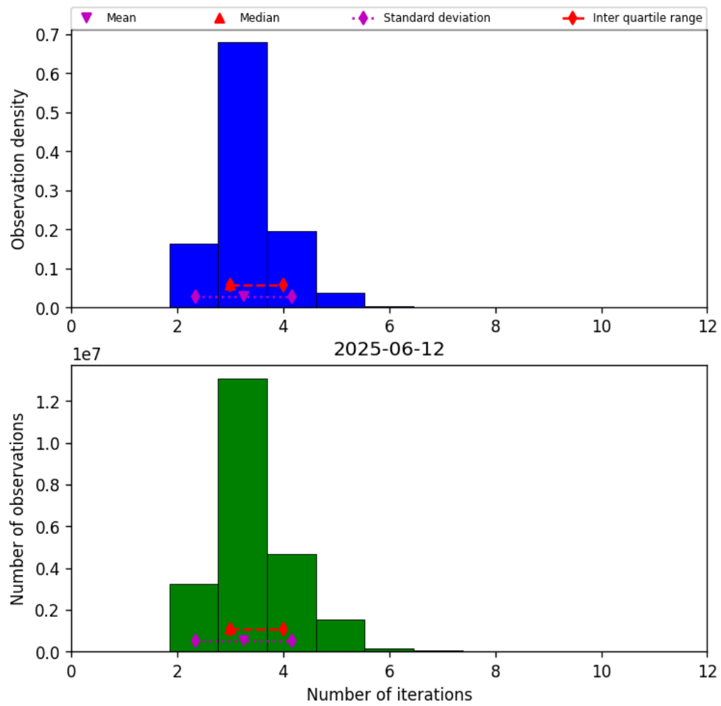
Figure 37: Histogram of “Number of iterations” for 2025-06-12 to 2025-06-13
