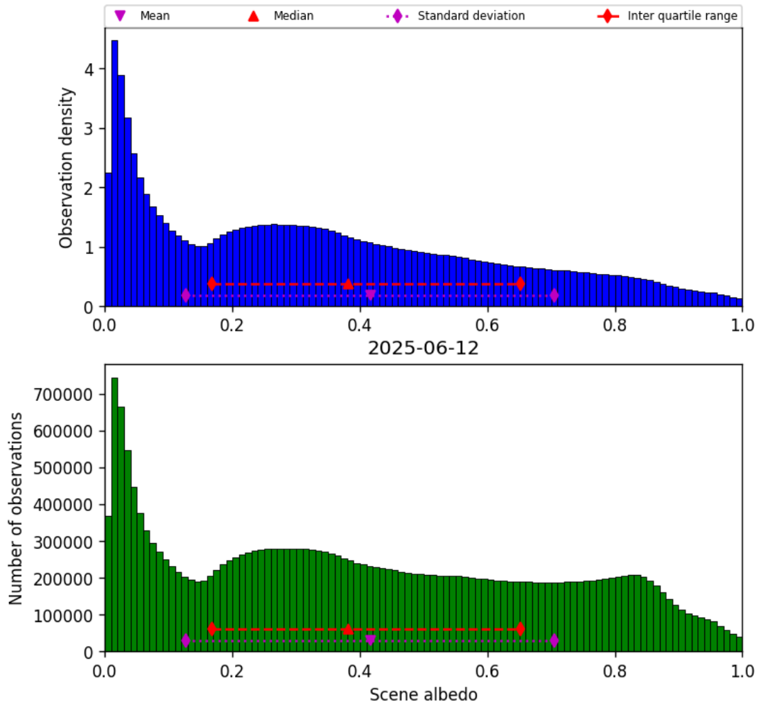
Figure 32: Histogram of “Scene albedo” for 2025-06-12 to 2025-06-13
