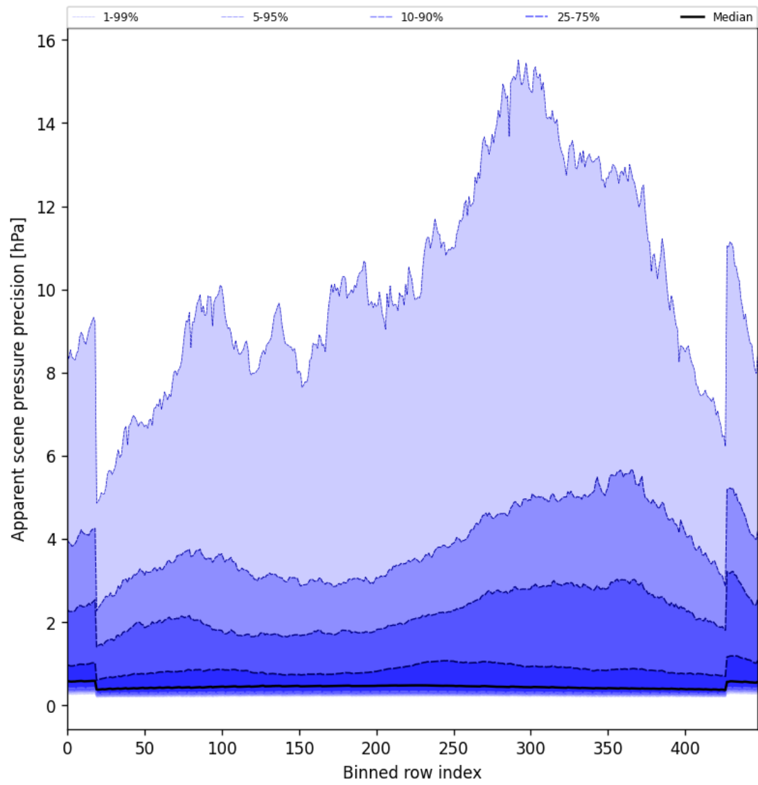
Figure 52: Along track statistics of “Apparent scene pressure precision” for 2025-06-12 to 2025-06-13
