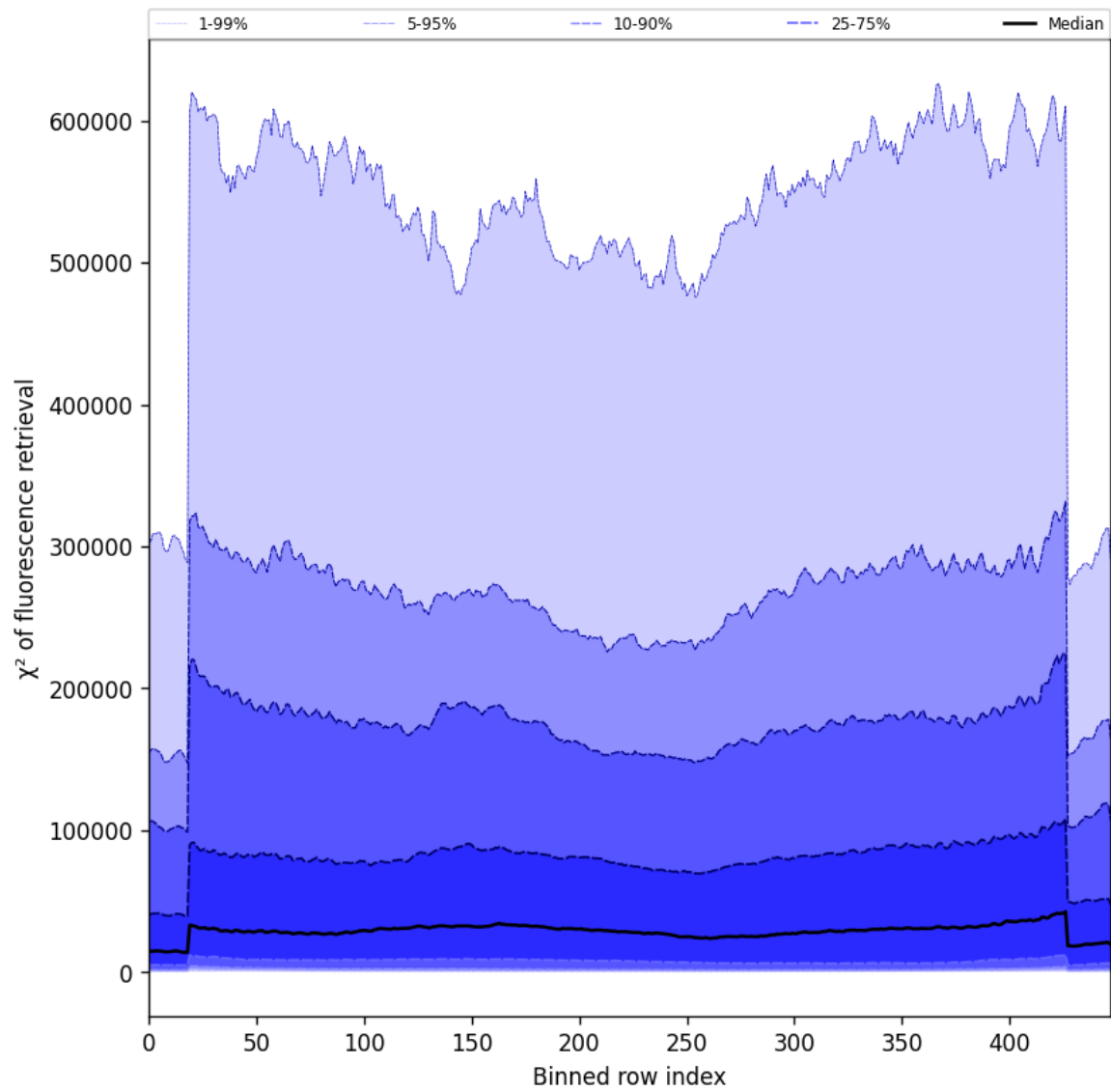
Figure 57: Along track statistics of “ \chi^2 of fluorescence retrieval” for 2025-06-12 to 2025-06-13
