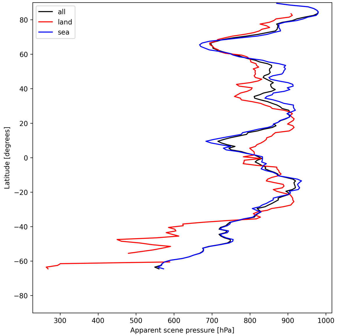
Figure 17: Zonal average of “Apparent scene pressure” for 2025-06-12 to 2025-06-13.
