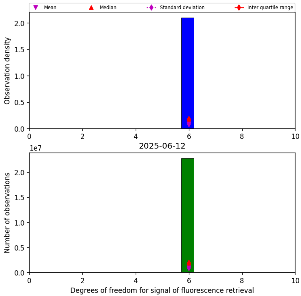
Figure 41: Histogram of “Degrees of freedom for signal of fluorescence retrieval” for 2025-06-12 to 2025-06-13
