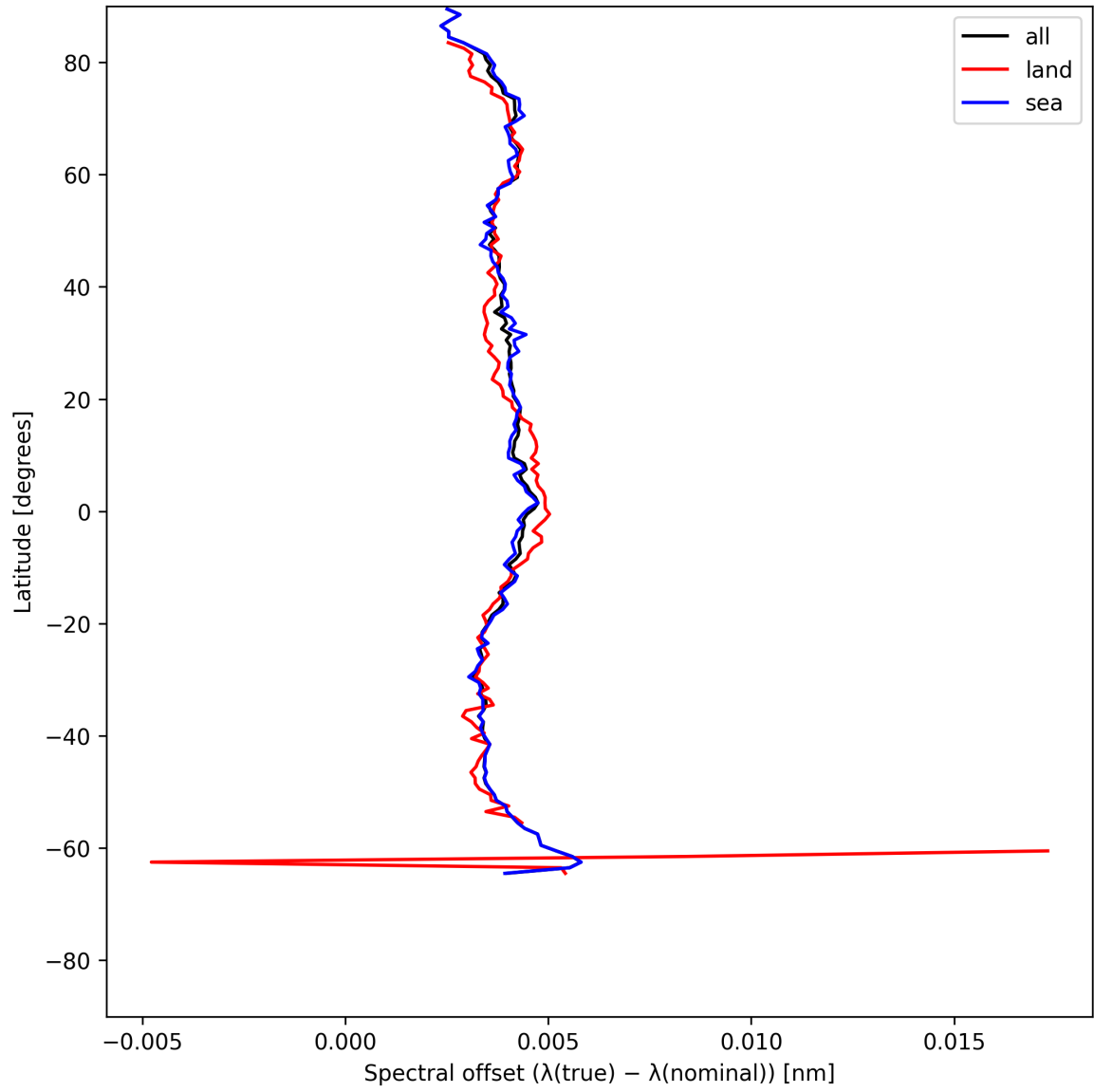
Figure 26: Zonal average of “Spectral offset ( \lambda_{\text{true}} - \lambda_{\text{nominal}} )” for 2025-06-12 to 2025-06-13.
