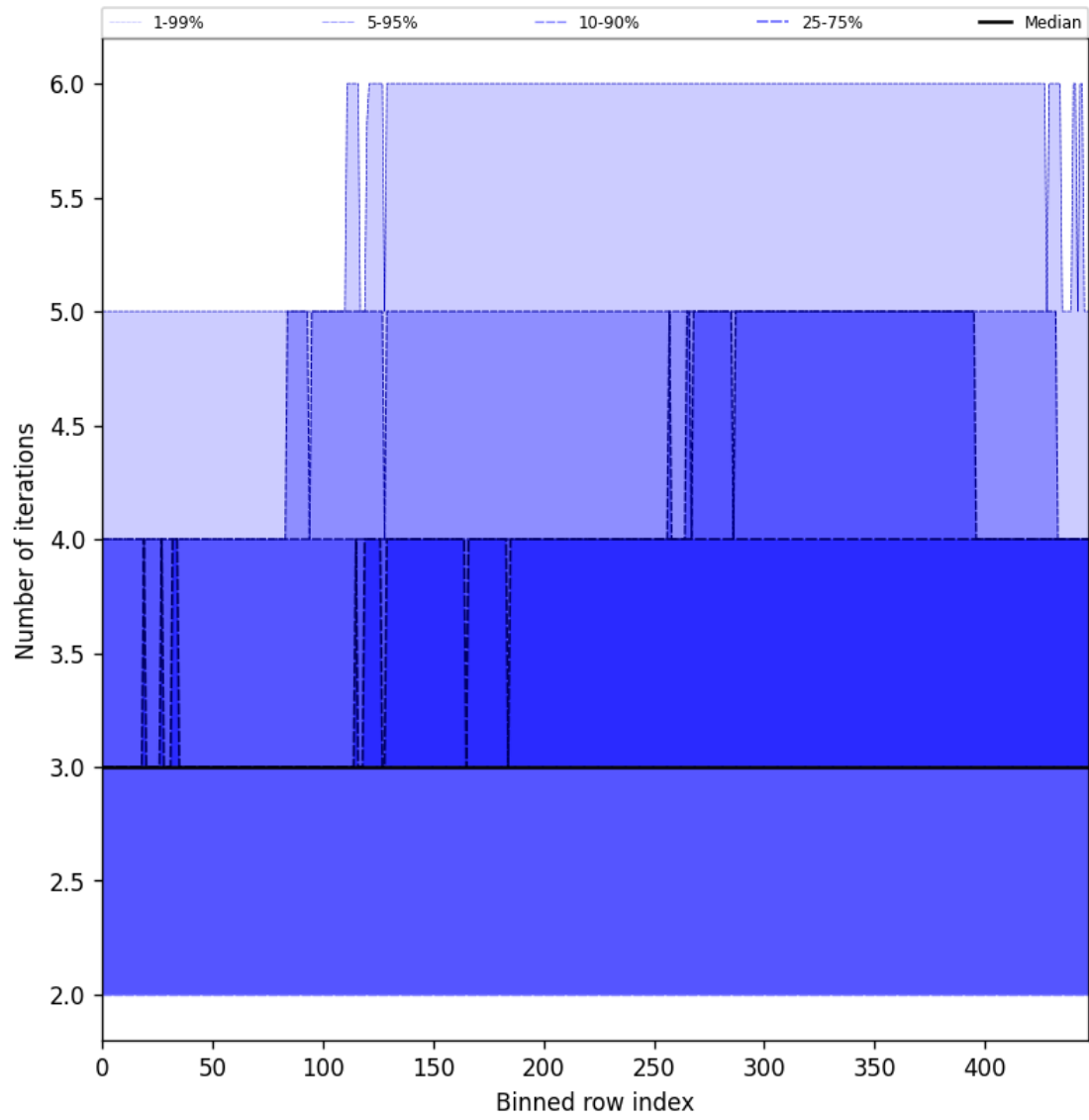
Figure 54: Along track statistics of “Number of iterations” for 2025-06-12 to 2025-06-13
