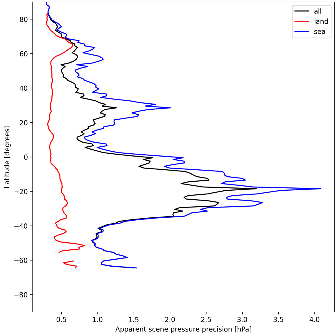
Figure 18: Zonal average of “Apparent scene pressure precision” for 2025-06-12 to 2025-06-13.
