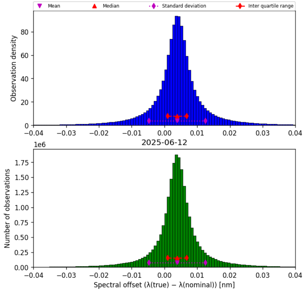
Figure 43: Histogram of “Spectral offset ( \lambda_{\text{true}} - \lambda_{\text{nominal}} )” for 2025-06-12 to 2025-06-13
