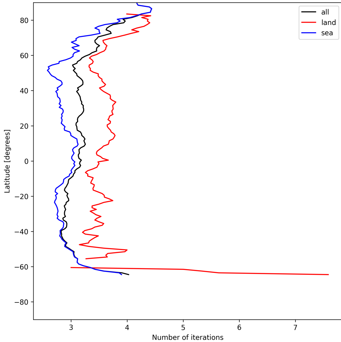
Figure 20: Zonal average of “Number of iterations” for 2025-06-12 to 2025-06-13.
