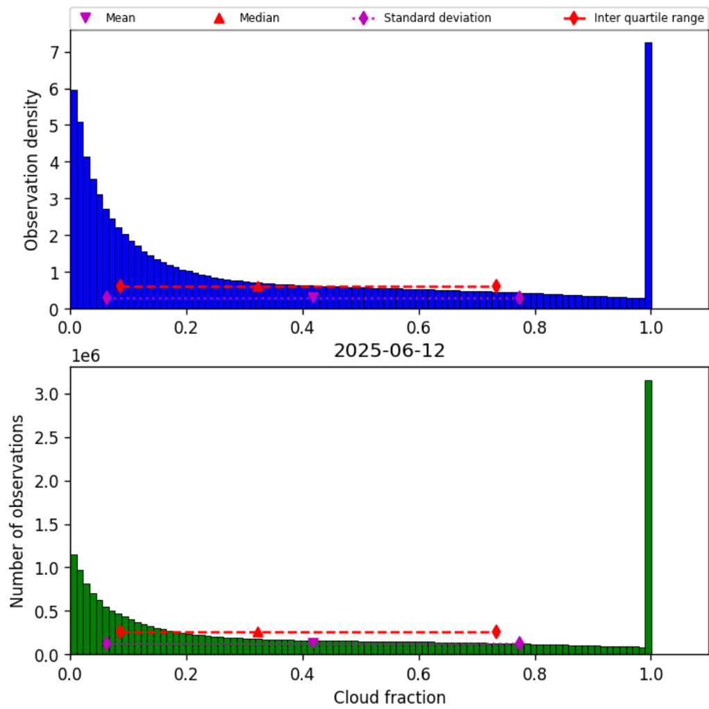
Figure 30: Histogram of “Cloud fraction” for 2025-06-12 to 2025-06-13
