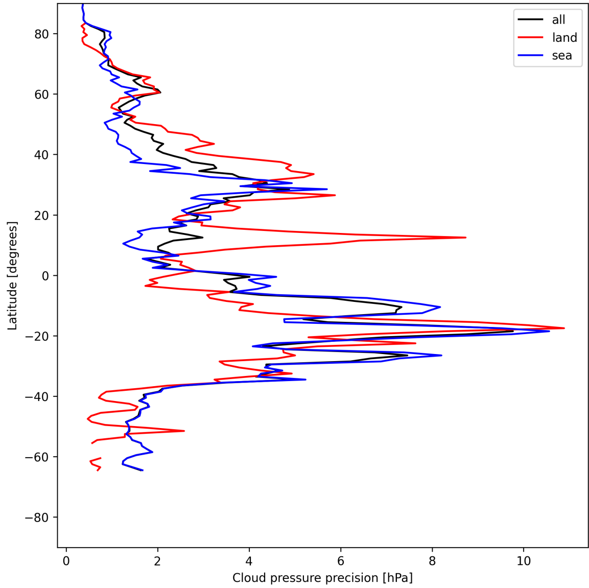
Figure 12: Zonal average of “Cloud pressure precision” for 2025-06-12 to 2025-06-13.
