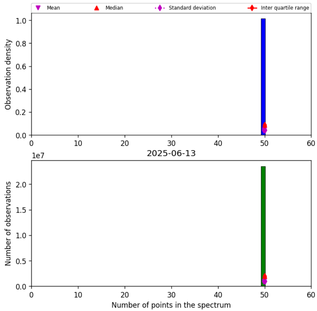
Figure 42: Histogram of “Number of points in the spectrum” for 2025-06-13 to 2025-06-14
