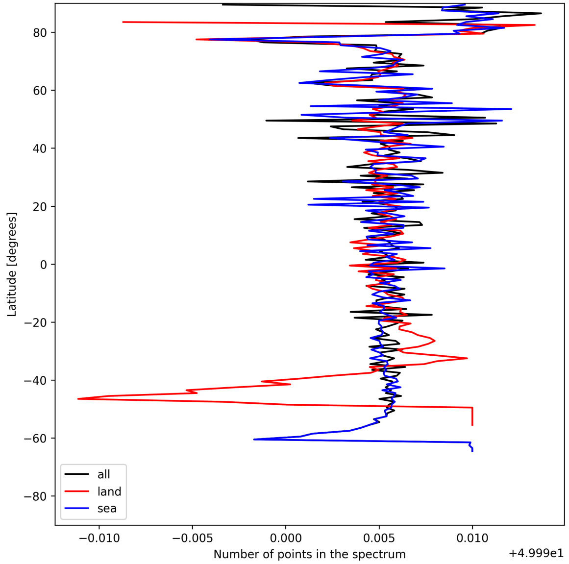
Figure 25: Zonal average of “Number of points in the spectrum” for 2025-06-13 to 2025-06-14.
