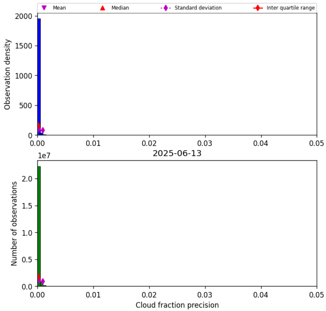
Figure 31: Histogram of “Cloud fraction precision” for 2025-06-13 to 2025-06-14
