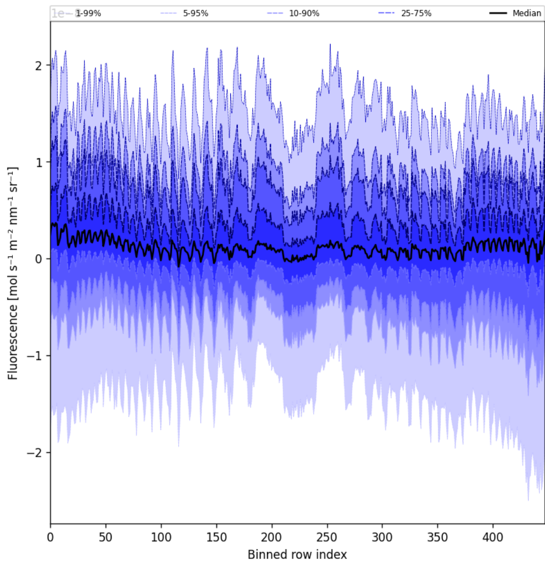
Figure 55: Along track statistics of “Fluorescence” for 2025-06-13 to 2025-06-14
