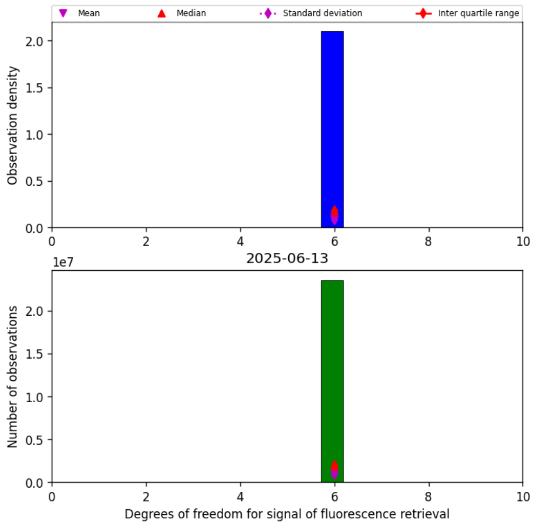
Figure 41: Histogram of “Degrees of freedom for signal of fluorescence retrieval” for 2025-06-13 to 2025-06-14
