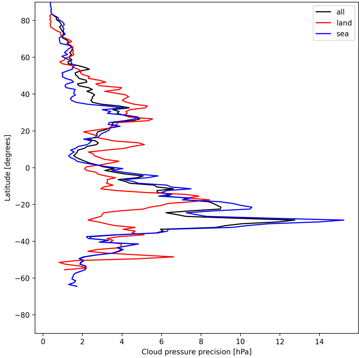
Figure 12: Zonal average of “Cloud pressure precision” for 2025-06-13 to 2025-06-14.
