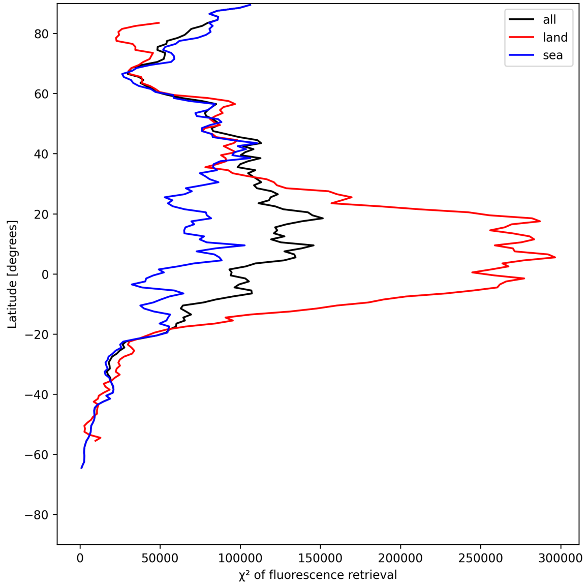
Figure 23: Zonal average of “ \chi^2 of fluorescence retrieval” for 2025-06-13 to 2025-06-14.
