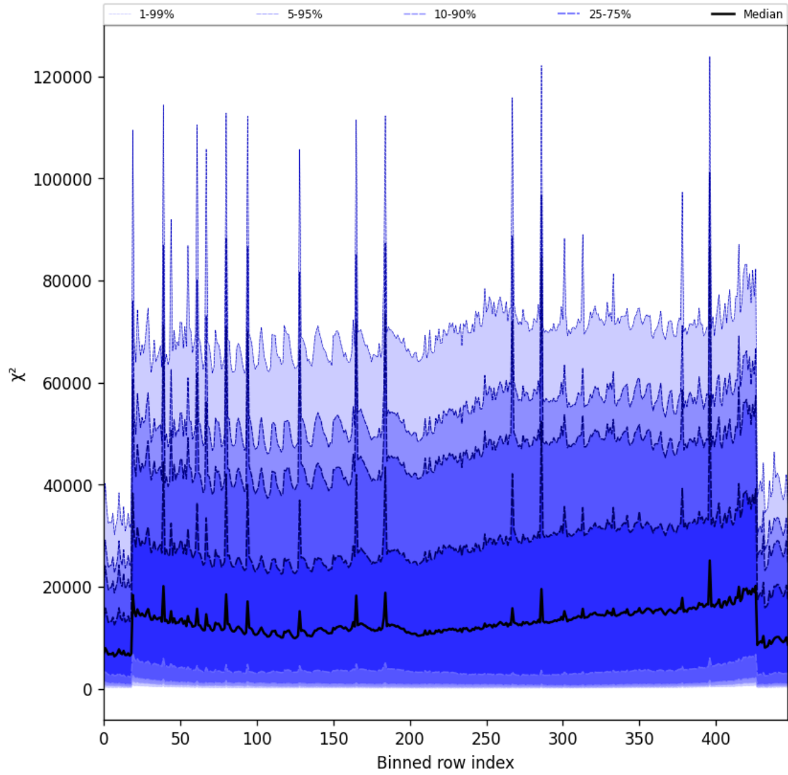
Figure 53: Along track statistics of “ \chi^2 ” for 2025-06-13 to 2025-06-14
