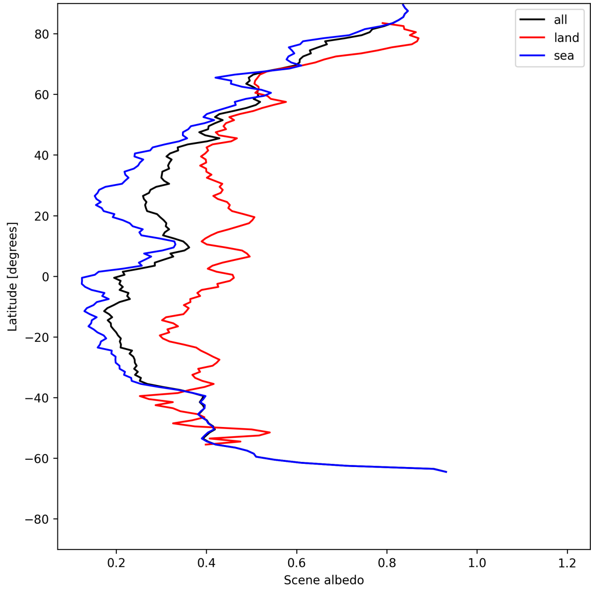
Figure 15: Zonal average of “Scene albedo” for 2025-06-13 to 2025-06-14.
