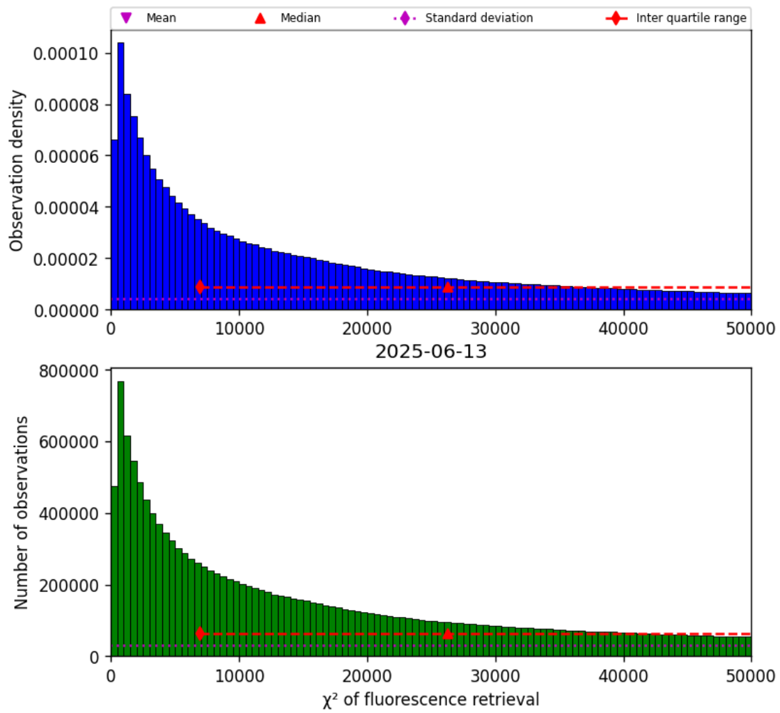
Figure 40: Histogram of “ \chi^2 of fluorescence retrieval” for 2025-06-13 to 2025-06-14
