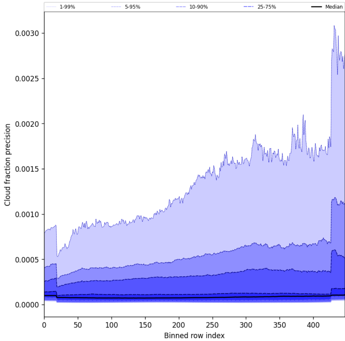
Figure 48: Along track statistics of “Cloud fraction precision” for 2025-06-13 to 2025-06-14
