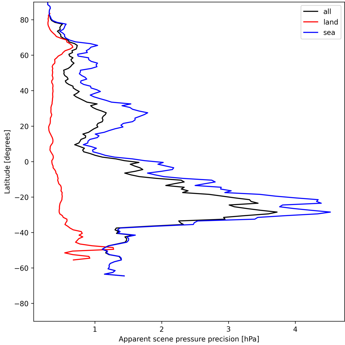
Figure 18: Zonal average of “Apparent scene pressure precision” for 2025-06-13 to 2025-06-14.
