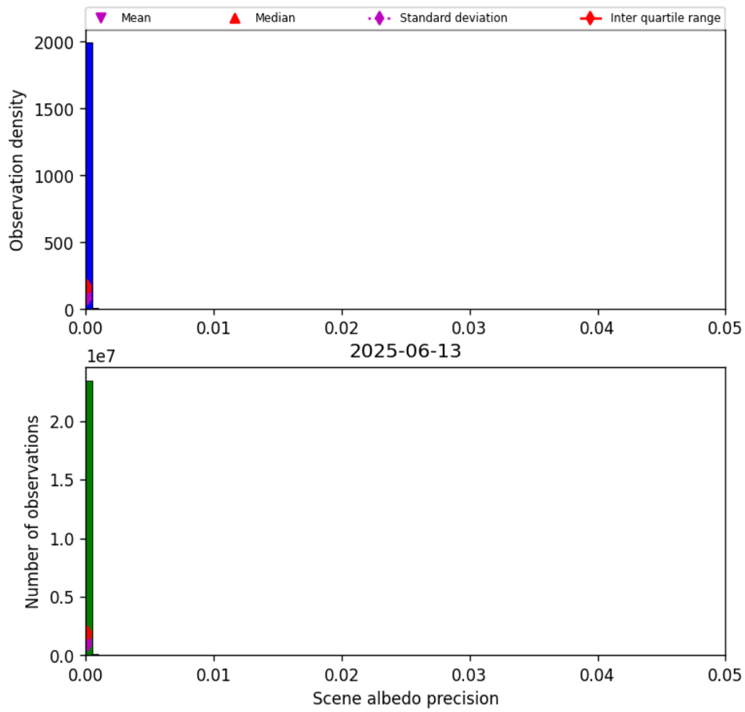
Figure 33: Histogram of “Scene albedo precision” for 2025-06-13 to 2025-06-14
