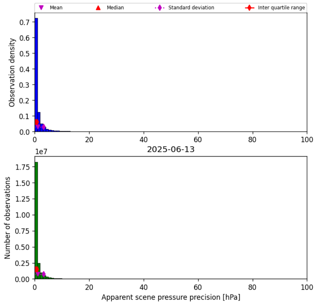
Figure 35: Histogram of “Apparent scene pressure precision” for 2025-06-13 to 2025-06-14
