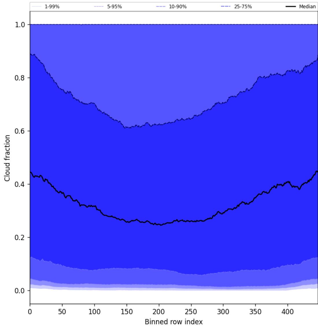
Figure 47: Along track statistics of “Cloud fraction” for 2025-06-13 to 2025-06-14
