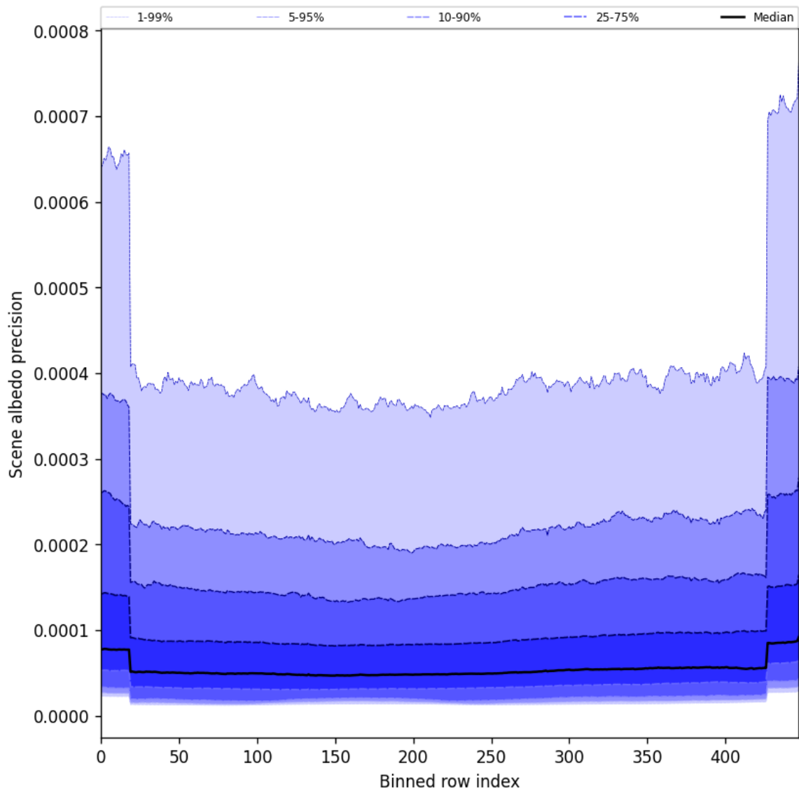
Figure 50: Along track statistics of “Scene albedo precision” for 2025-06-13 to 2025-06-14
