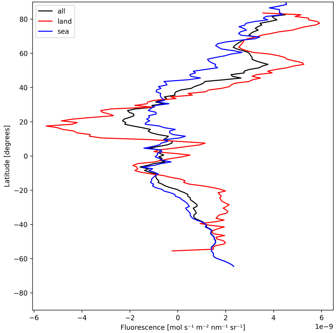
Figure 21: Zonal average of “Fluorescence” for 2025-06-13 to 2025-06-14.
