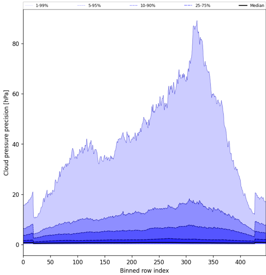
Figure 46: Along track statistics of “Cloud pressure precision” for 2025-06-13 to 2025-06-14
