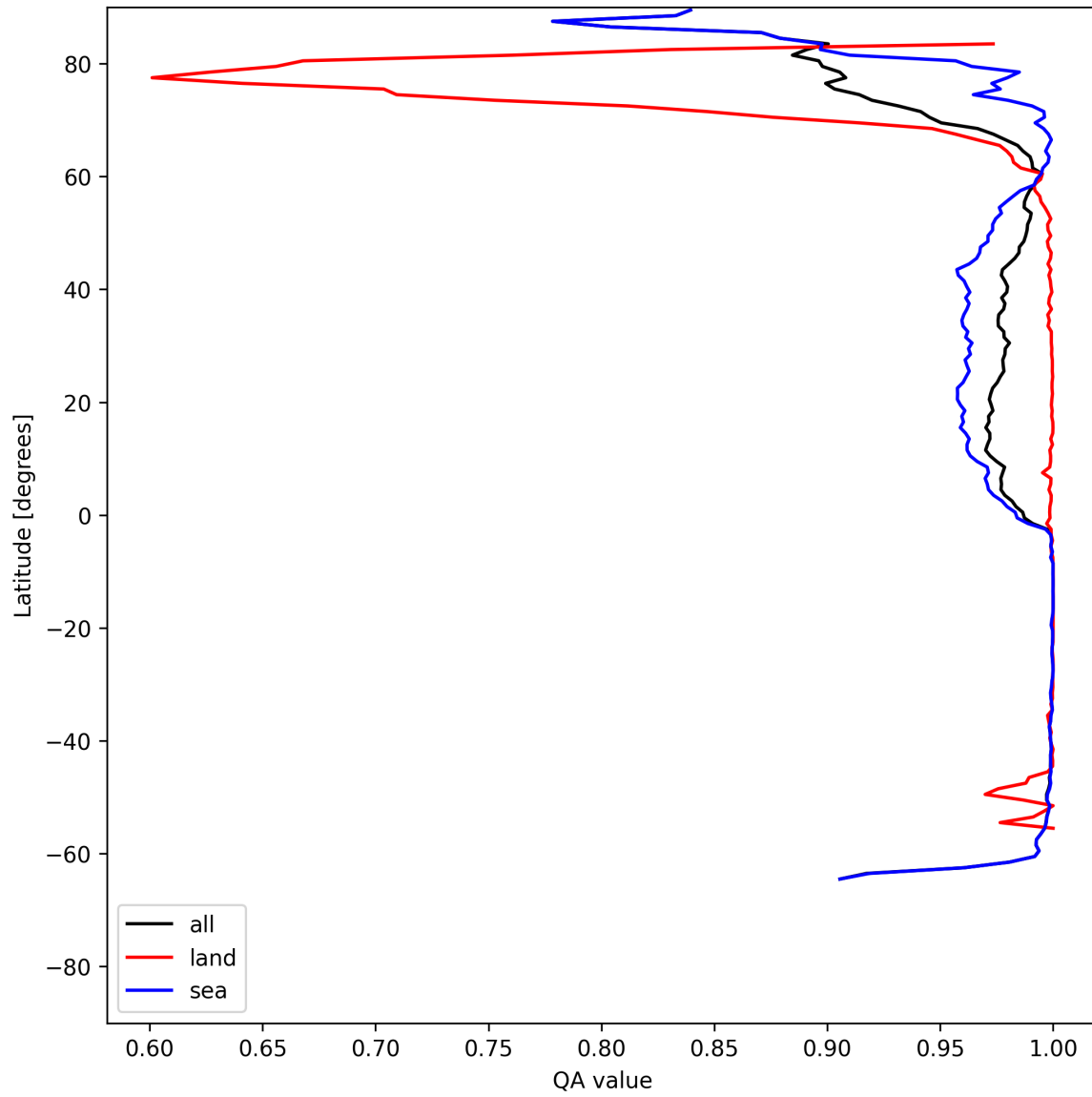
Figure 10: Zonal average of “QA value” for 2025-06-13 to 2025-06-14.
