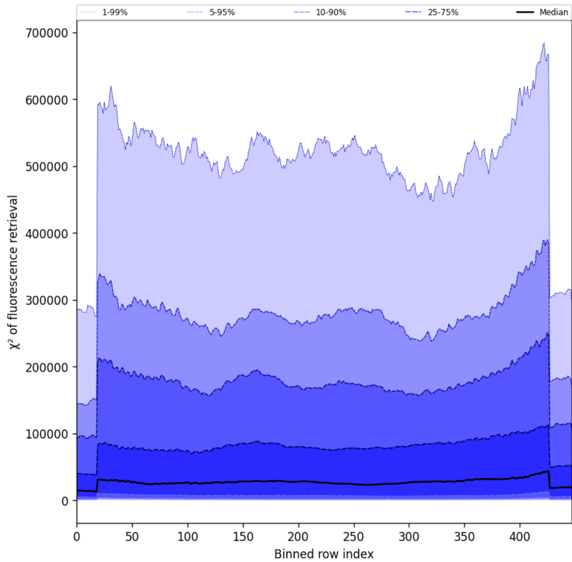
Figure 57: Along track statistics of “ \chi^2 of fluorescence retrieval” for 2025-06-13 to 2025-06-14
