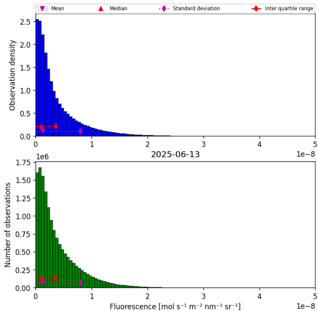
Figure 38: Histogram of “Fluorescence” for 2025-06-13 to 2025-06-14
