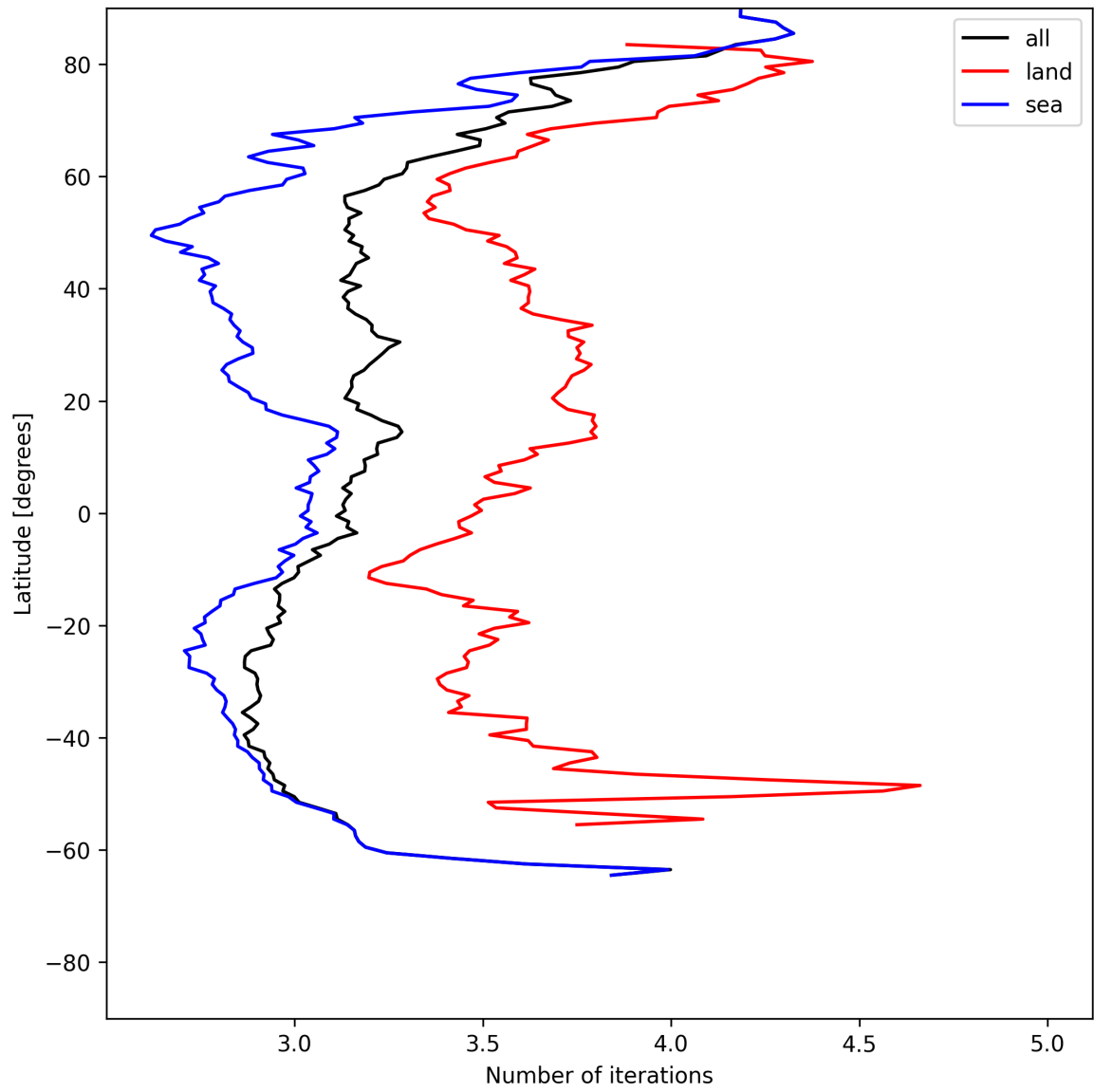
Figure 20: Zonal average of “Number of iterations” for 2025-06-13 to 2025-06-14.
