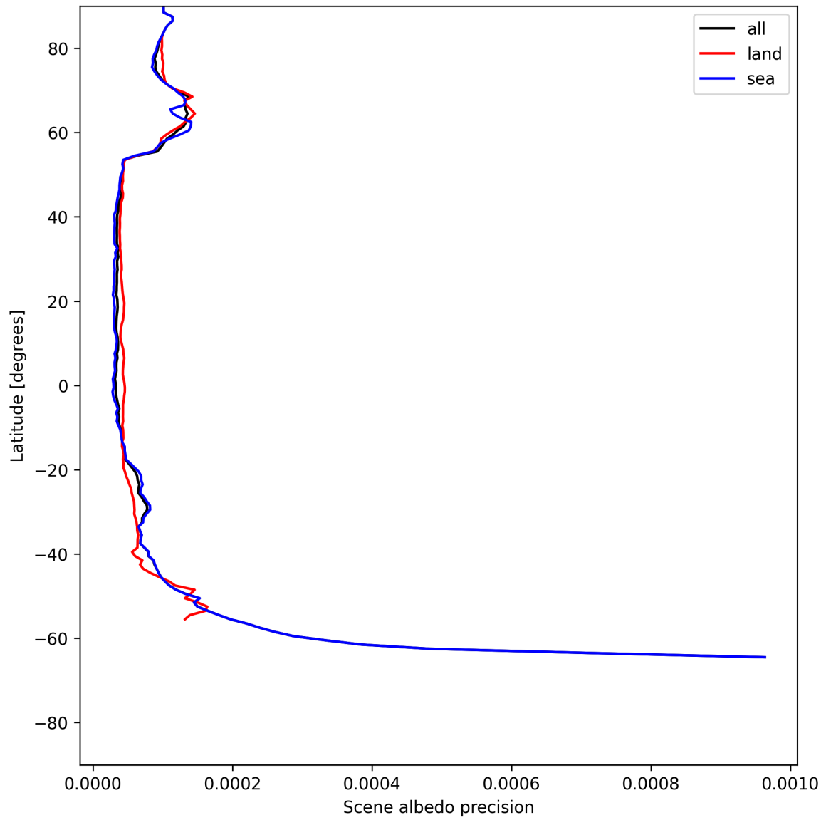
Figure 16: Zonal average of “Scene albedo precision” for 2025-06-13 to 2025-06-14.
