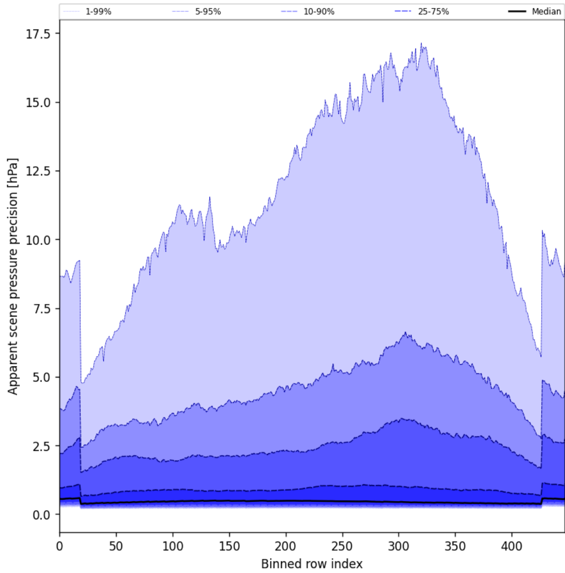
Figure 52: Along track statistics of “Apparent scene pressure precision” for 2025-06-13 to 2025-06-14
