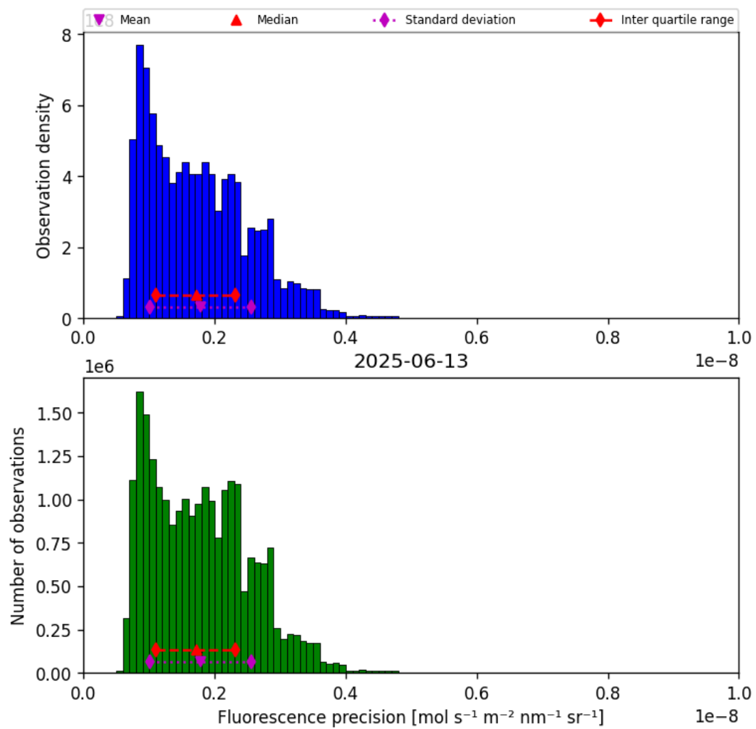
Figure 39: Histogram of “Fluorescence precision” for 2025-06-13 to 2025-06-14
