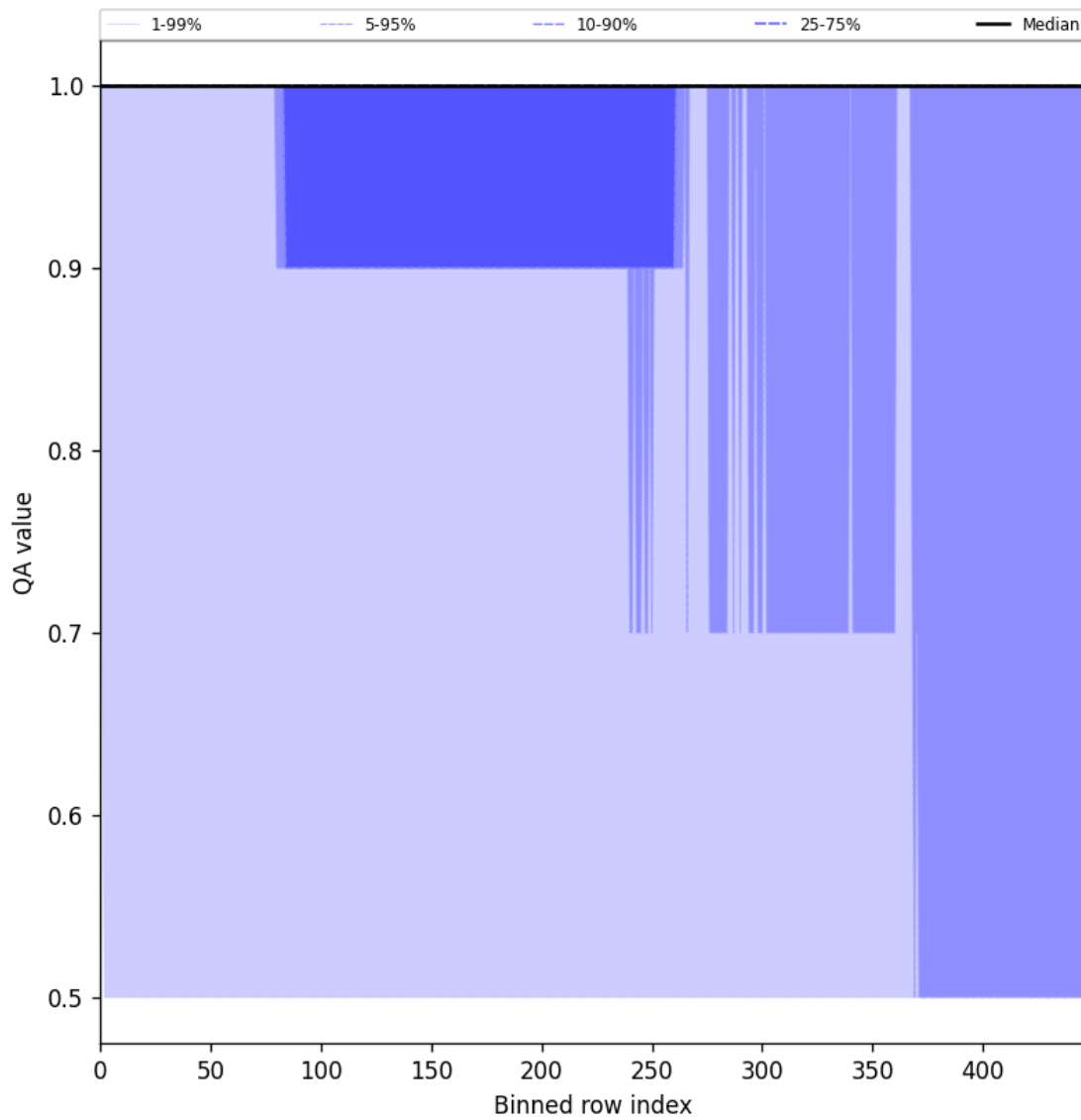
Figure 44: Along track statistics of “QA value” for 2025-06-13 to 2025-06-14
