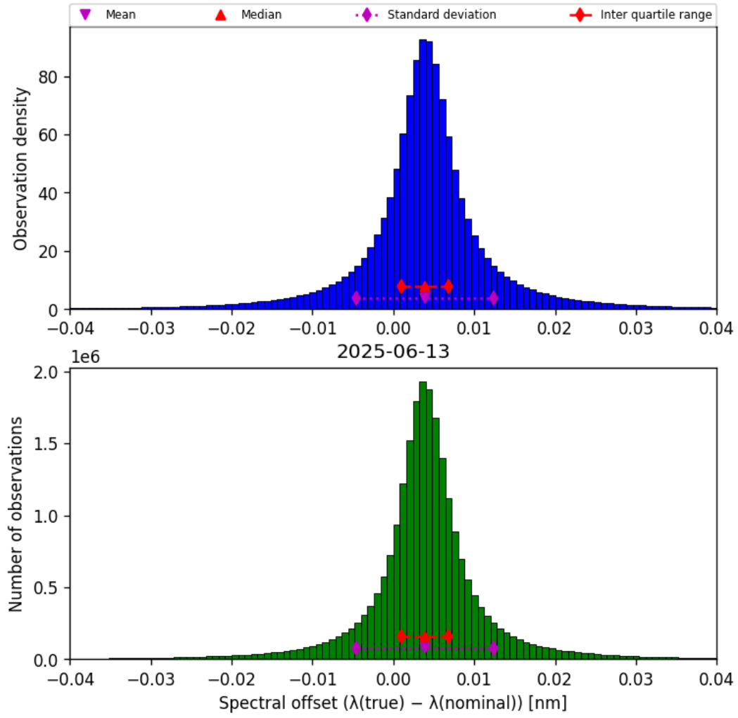
Figure 43: Histogram of “Spectral offset ( \lambda_{\text{true}} - \lambda_{\text{nominal}} )” for 2025-06-13 to 2025-06-14
