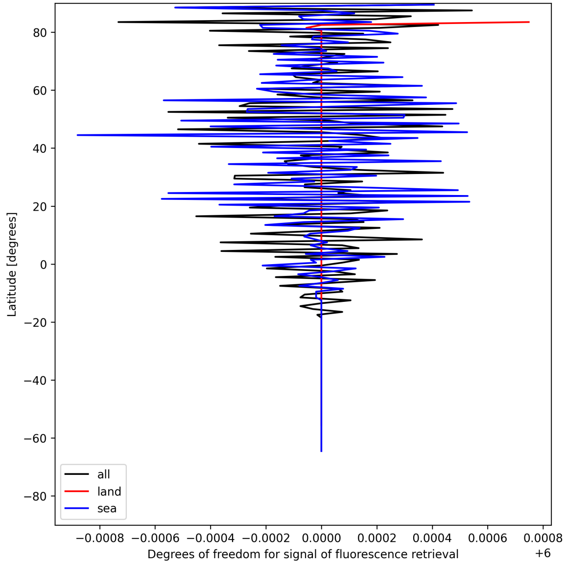
Figure 24: Zonal average of “Degrees of freedom for signal of fluorescence retrieval” for 2025-06-13 to 2025-06-14.
