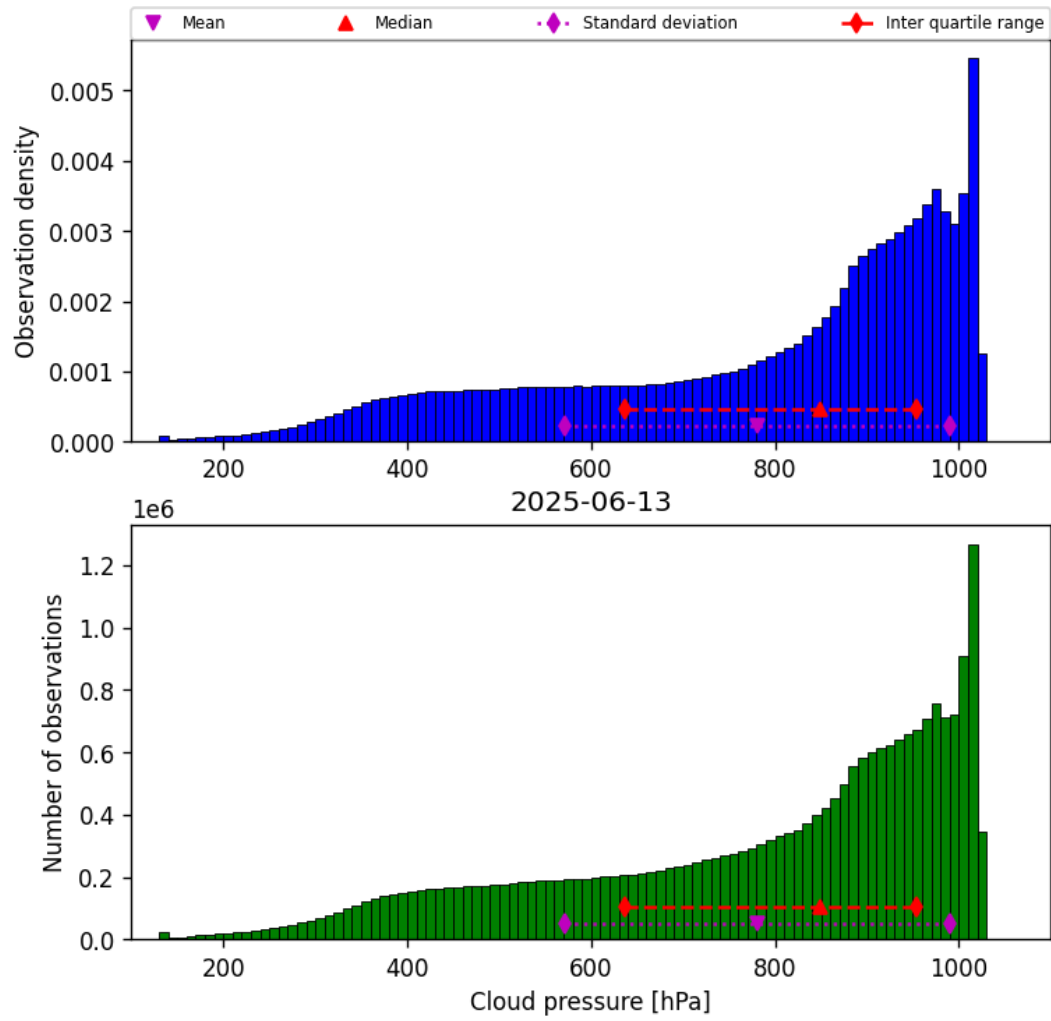
Figure 28: Histogram of “Cloud pressure” for 2025-06-13 to 2025-06-14
