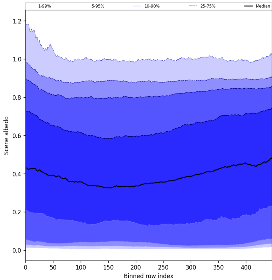
Figure 49: Along track statistics of “Scene albedo” for 2025-06-13 to 2025-06-14
