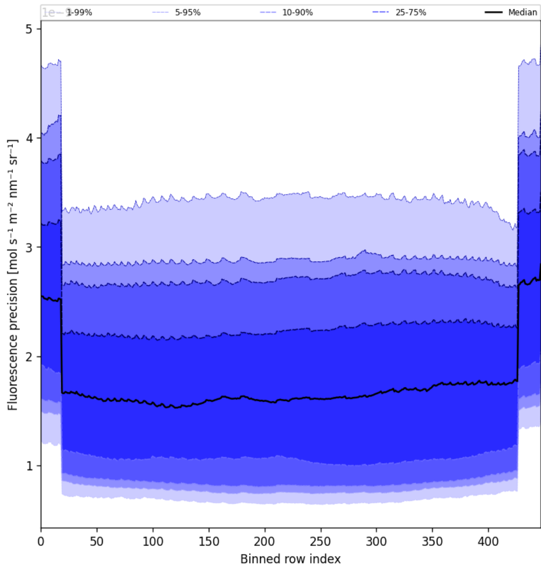
Figure 56: Along track statistics of “Fluorescence precision” for 2025-06-13 to 2025-06-14
