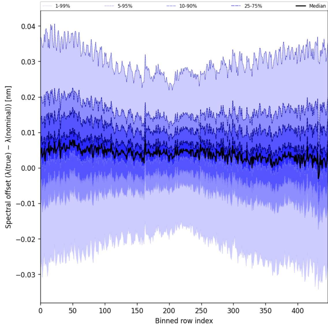
Figure 60: Along track statistics of “Spectral offset ( \lambda_{\text{true}} - \lambda_{\text{nominal}} )” for 2025-06-13 to 2025-06-14
