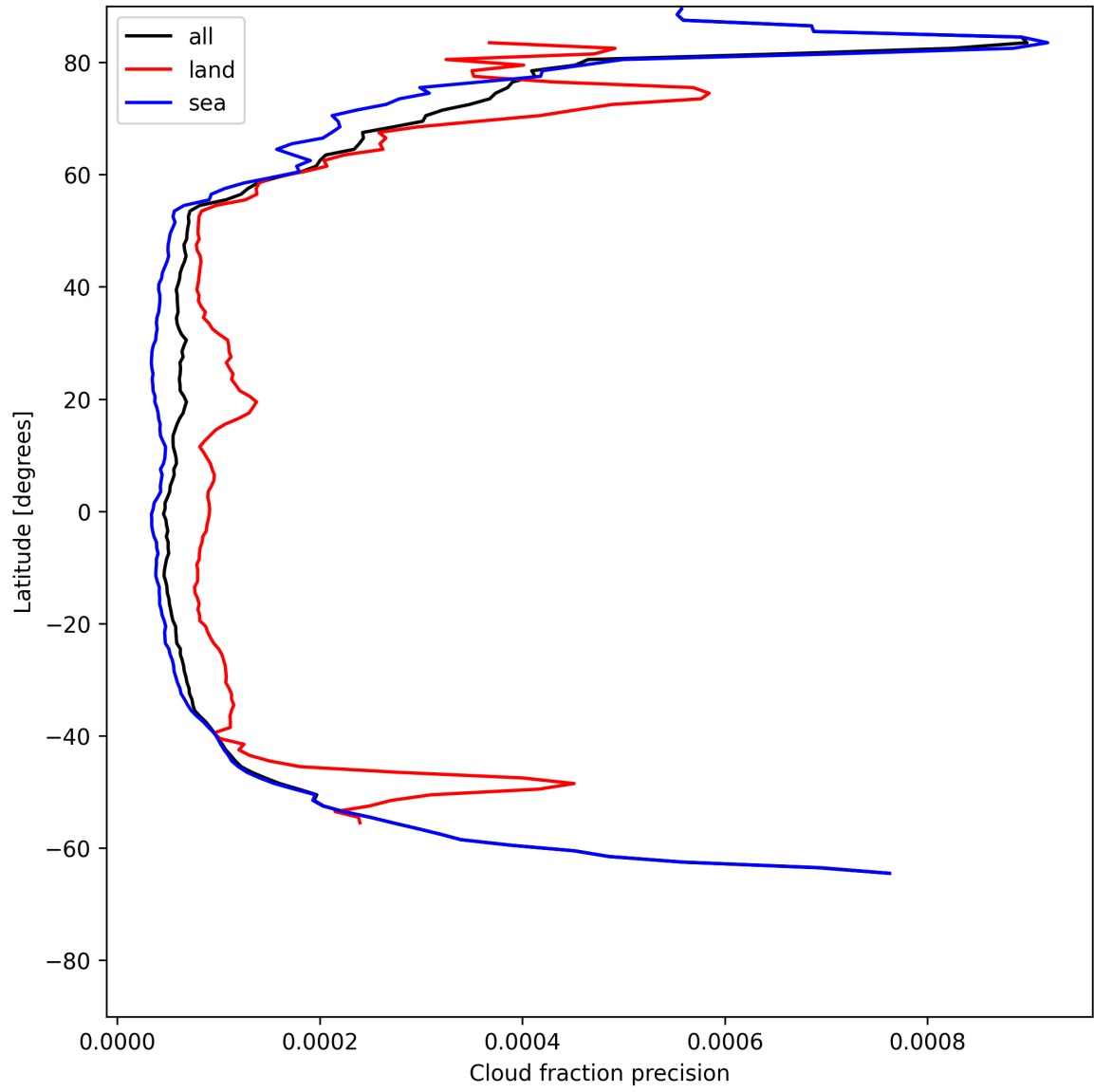
Figure 14: Zonal average of “Cloud fraction precision” for 2025-06-13 to 2025-06-14.
