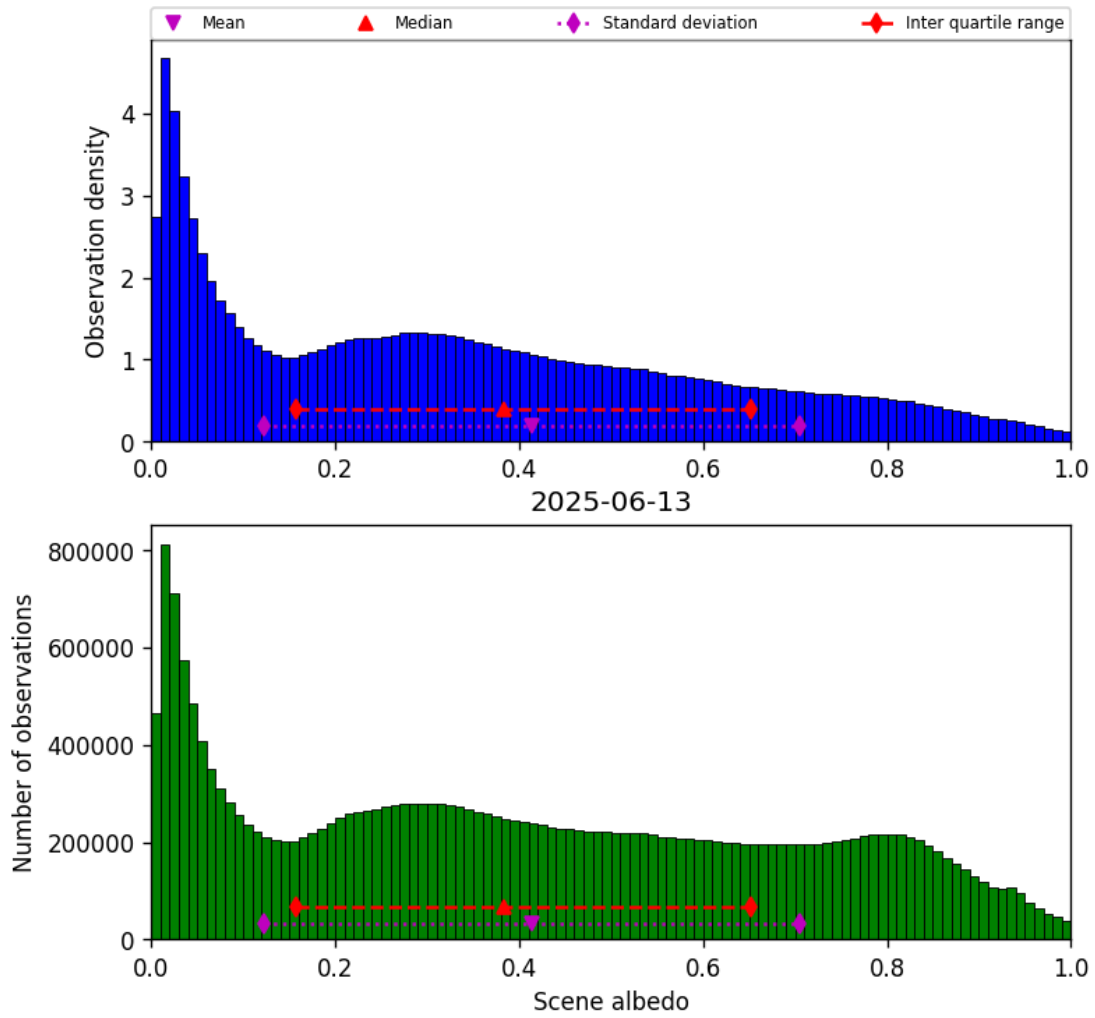
Figure 32: Histogram of “Scene albedo” for 2025-06-13 to 2025-06-14
