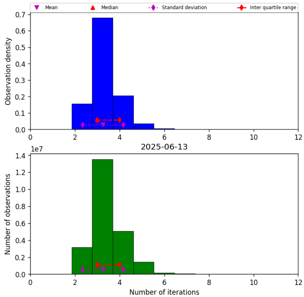
Figure 37: Histogram of “Number of iterations” for 2025-06-13 to 2025-06-14
