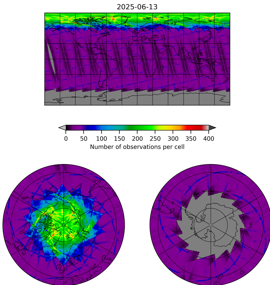
Figure 9: Map of the number of observations for 2025-06-13 to 2025-06-14
