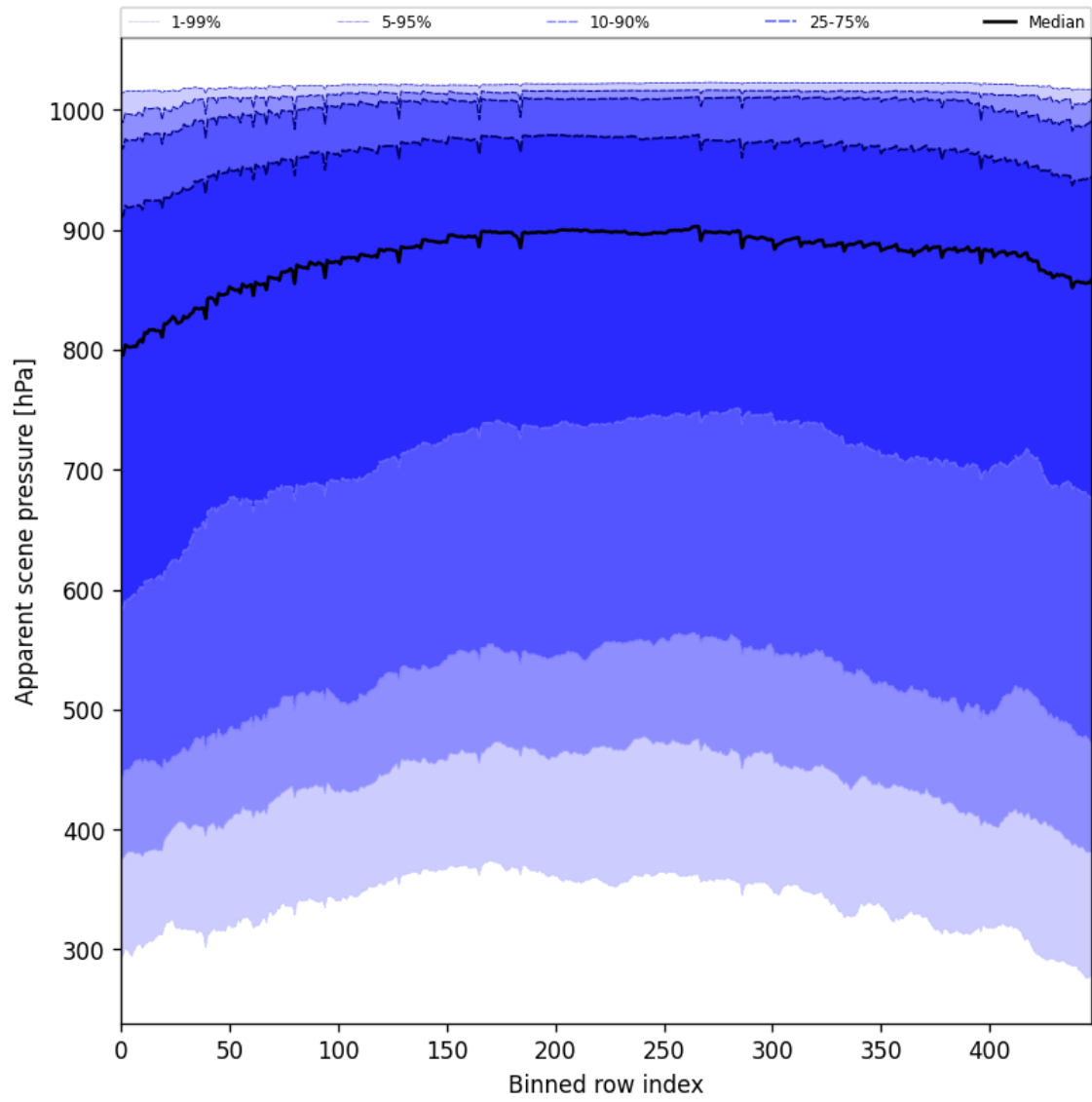
Figure 51: Along track statistics of “Apparent scene pressure” for 2025-06-13 to 2025-06-14
