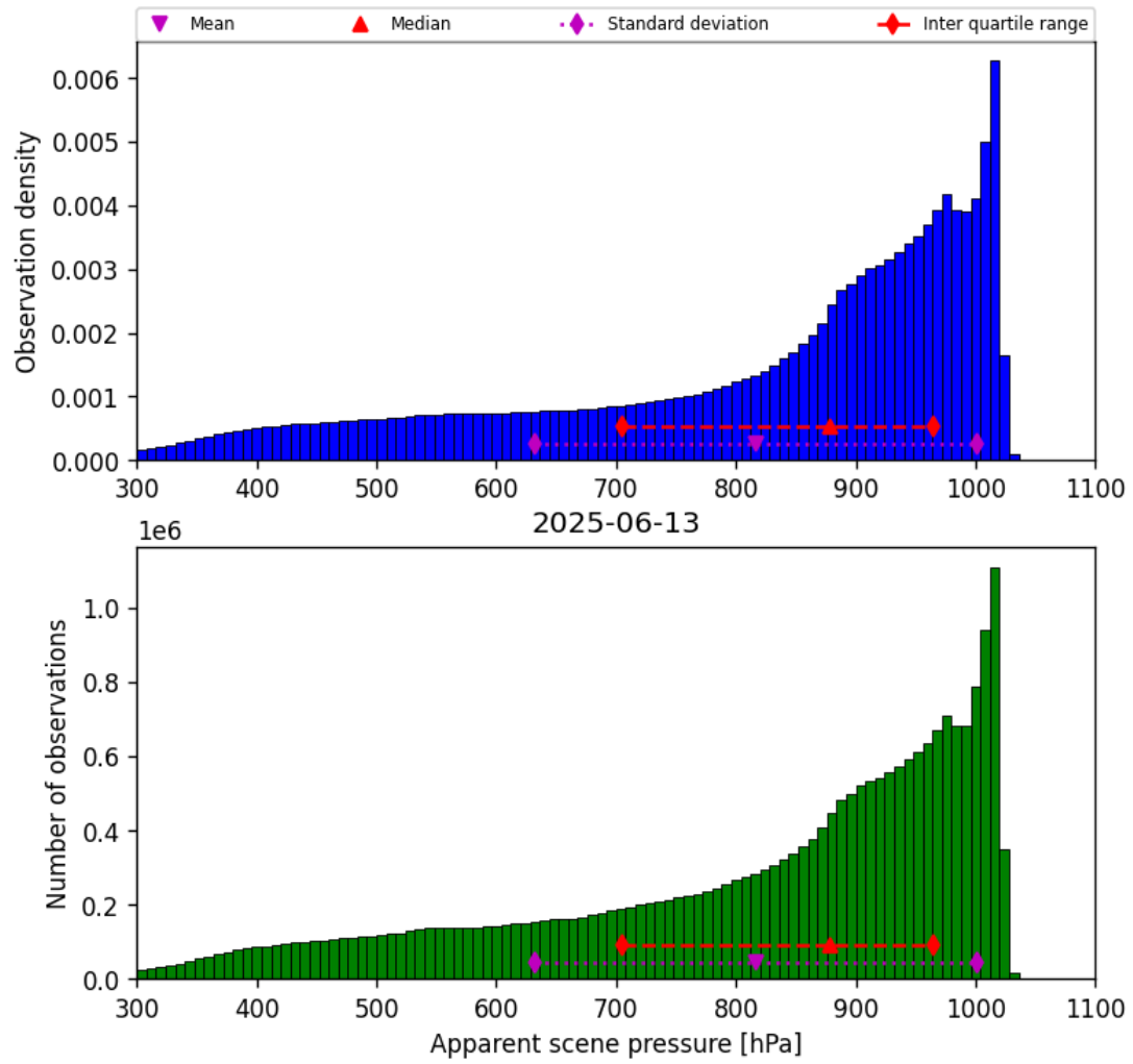
Figure 34: Histogram of “Apparent scene pressure” for 2025-06-13 to 2025-06-14
