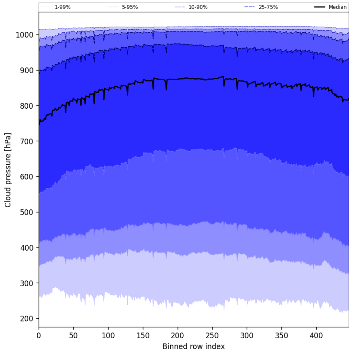
Figure 45: Along track statistics of “Cloud pressure” for 2025-06-13 to 2025-06-14
