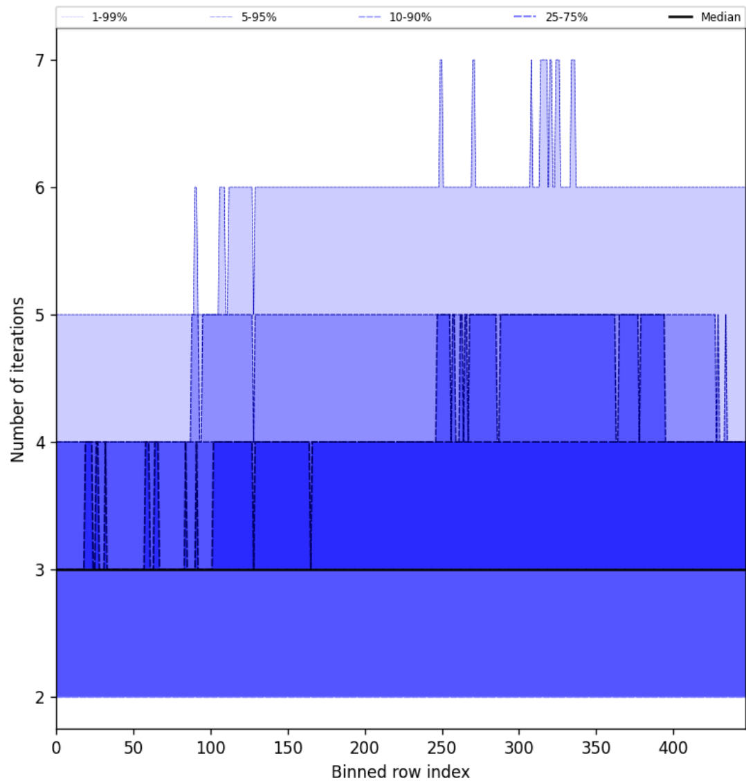
Figure 54: Along track statistics of “Number of iterations” for 2025-06-13 to 2025-06-14
