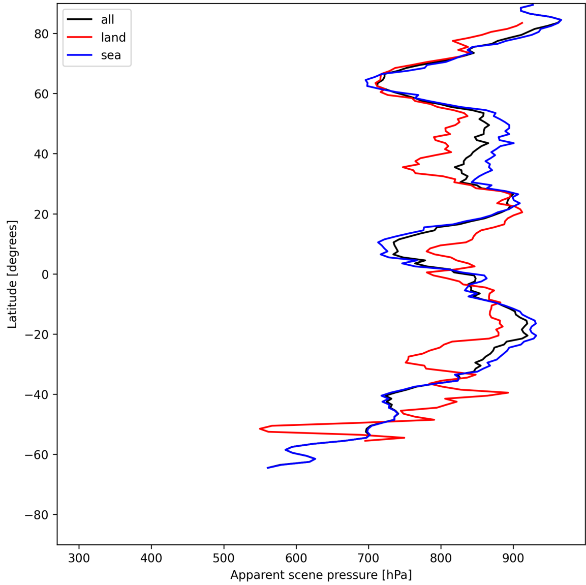
Figure 17: Zonal average of “Apparent scene pressure” for 2025-06-13 to 2025-06-14.
