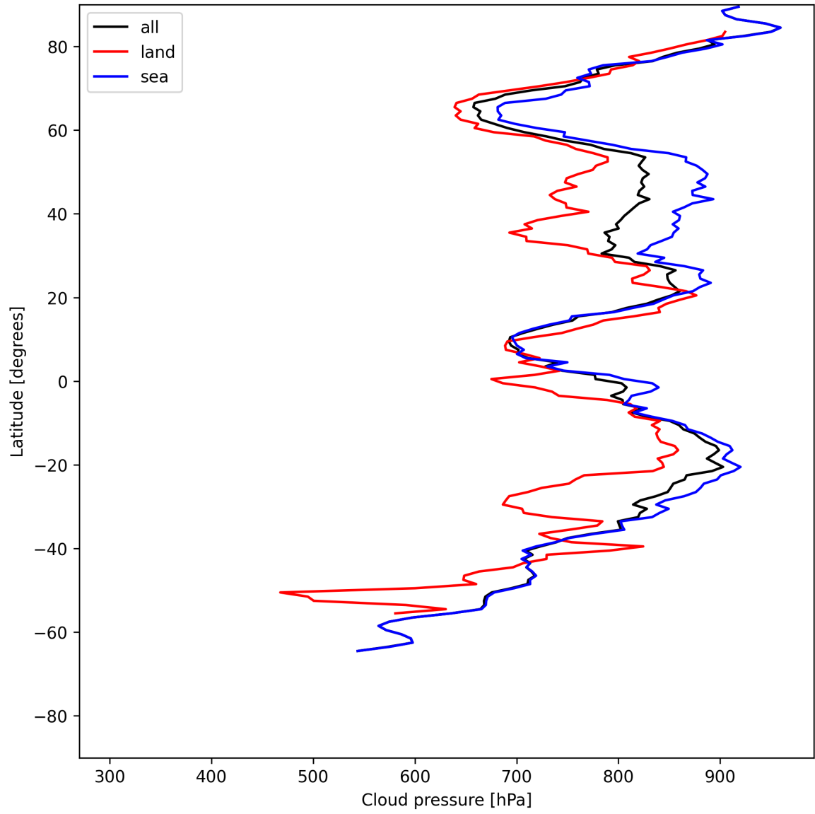
Figure 11: Zonal average of “Cloud pressure” for 2025-06-13 to 2025-06-14.
