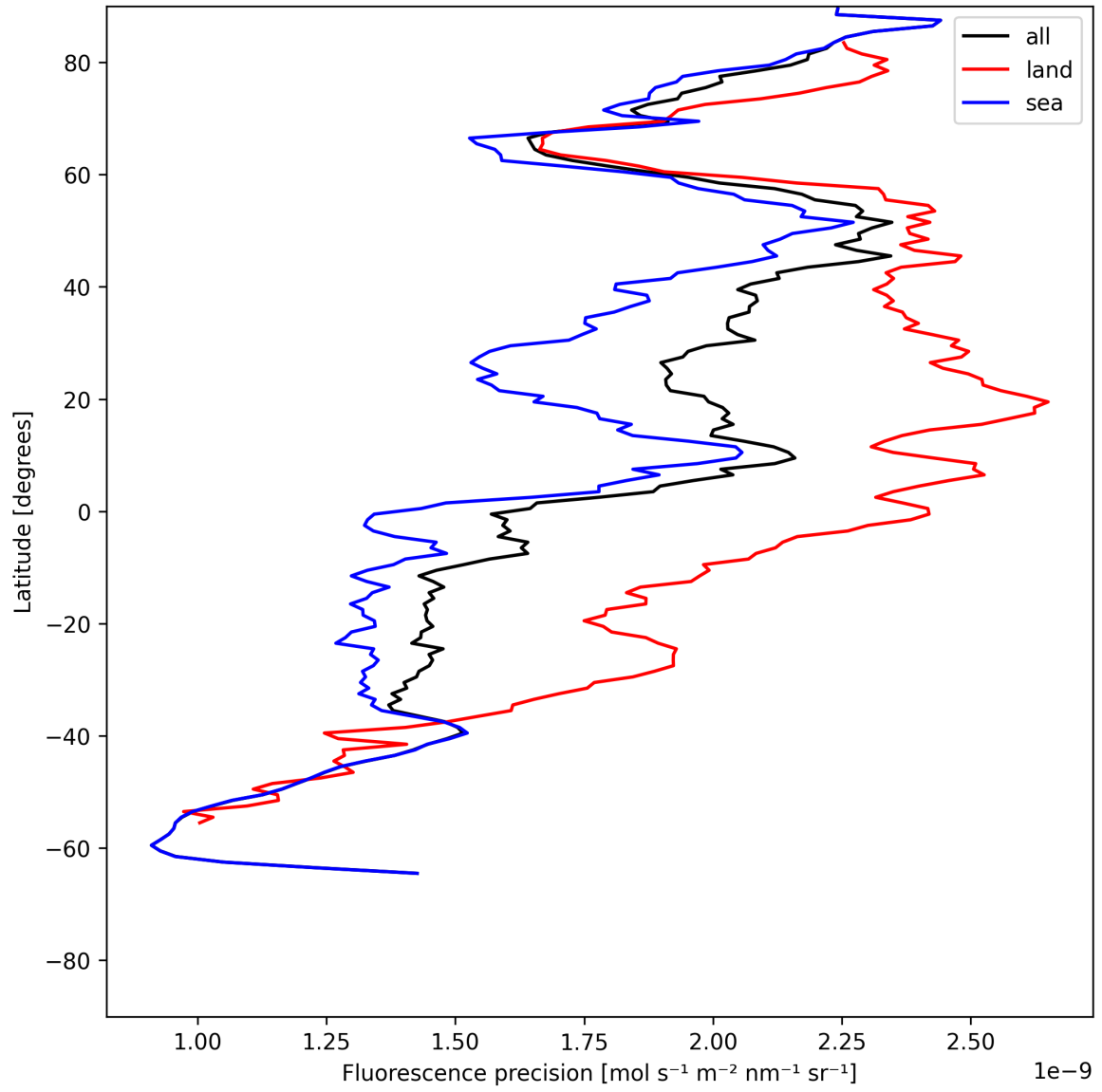
Figure 22: Zonal average of "Fluorescence precision" for 2025-06-13 to 2025-06-14.
