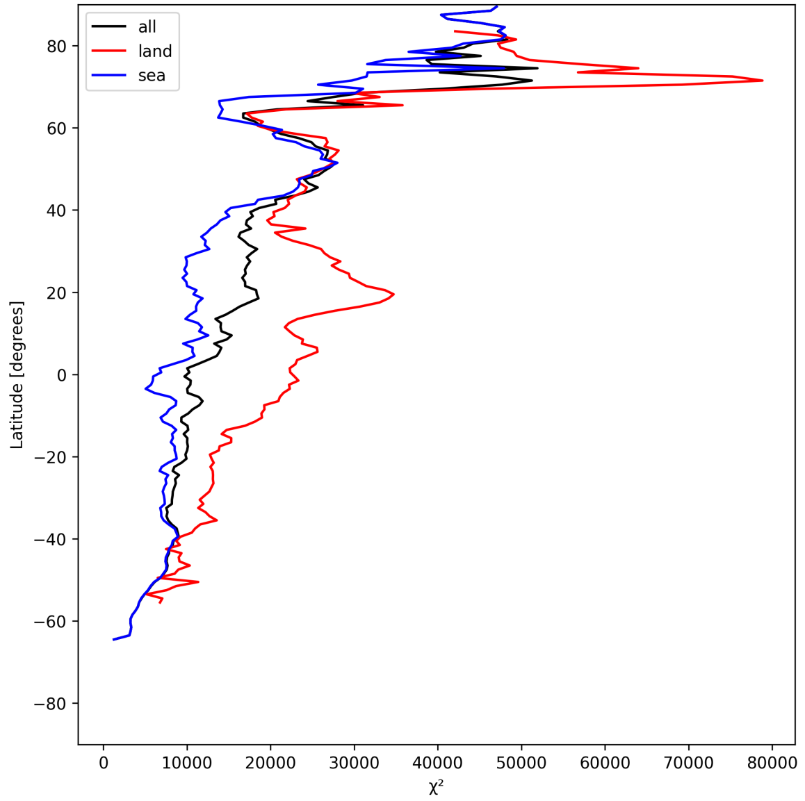
Figure 19: Zonal average of “ \chi^2 ” for 2025-06-13 to 2025-06-14.
