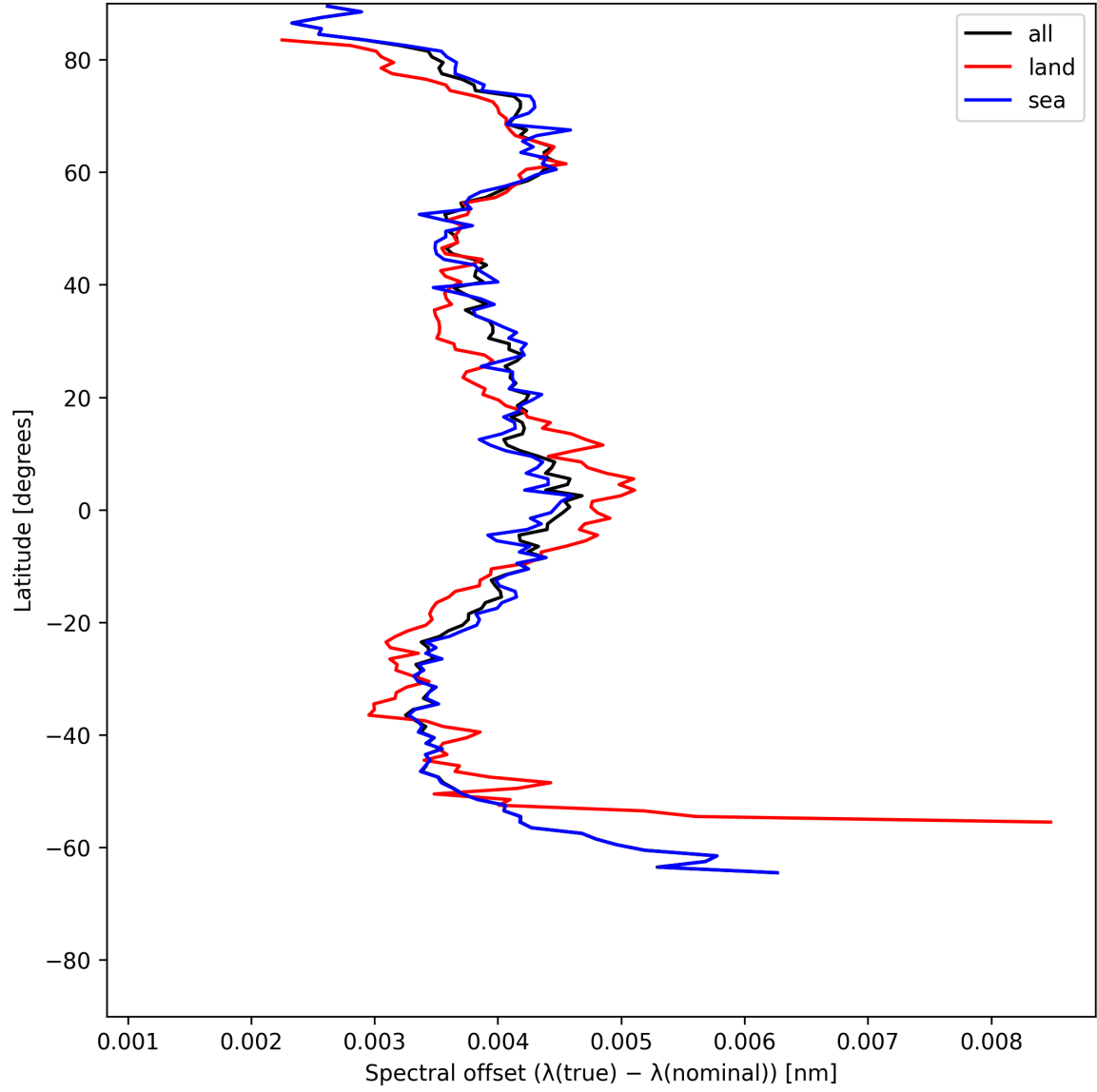
Figure 26: Zonal average of “Spectral offset ( \lambda_{\text{true}} - \lambda_{\text{nominal}} )” for 2025-06-13 to 2025-06-14.
