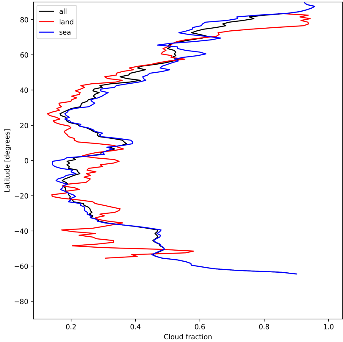
Figure 13: Zonal average of “Cloud fraction” for 2025-06-13 to 2025-06-14.
