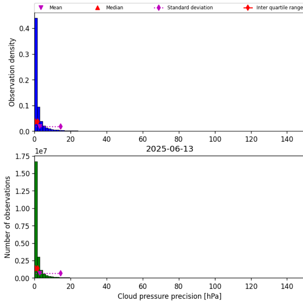
Figure 29: Histogram of “Cloud pressure precision” for 2025-06-13 to 2025-06-14
