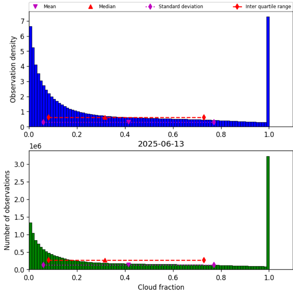
Figure 30: Histogram of “Cloud fraction” for 2025-06-13 to 2025-06-14
