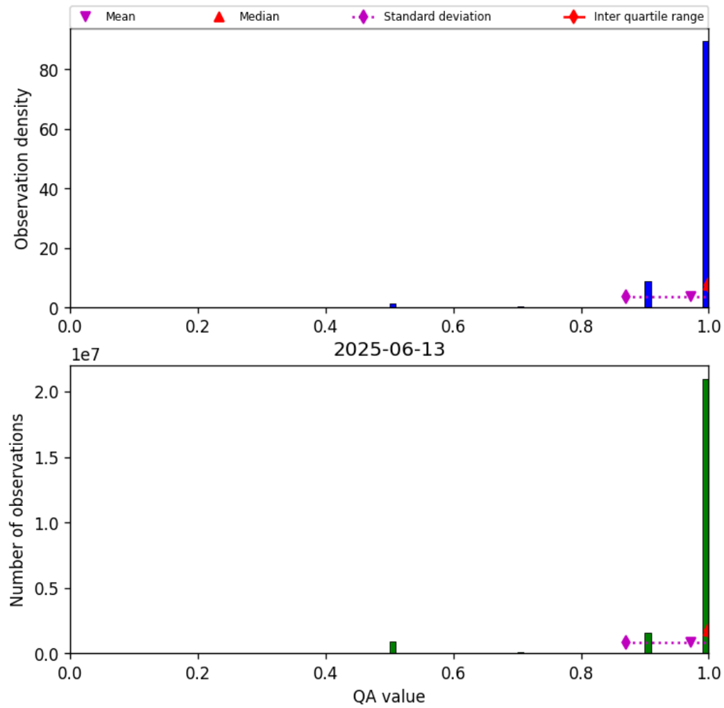
Figure 27: Histogram of “QA value” for 2025-06-13 to 2025-06-14
