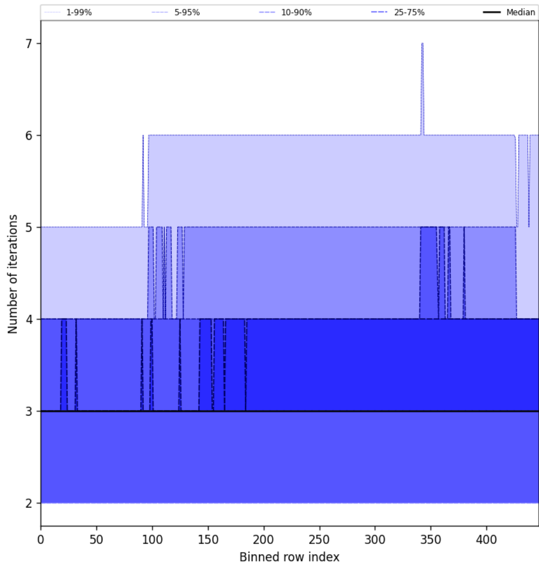
Figure 54: Along track statistics of “Number of iterations” for 2025-06-16 to 2025-06-17
