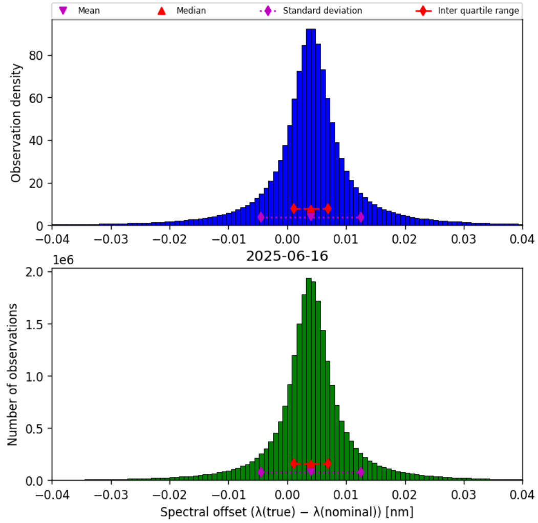
Figure 43: Histogram of “Spectral offset ( \lambda_{\text{true}} - \lambda_{\text{nominal}} )” for 2025-06-16 to 2025-06-17
