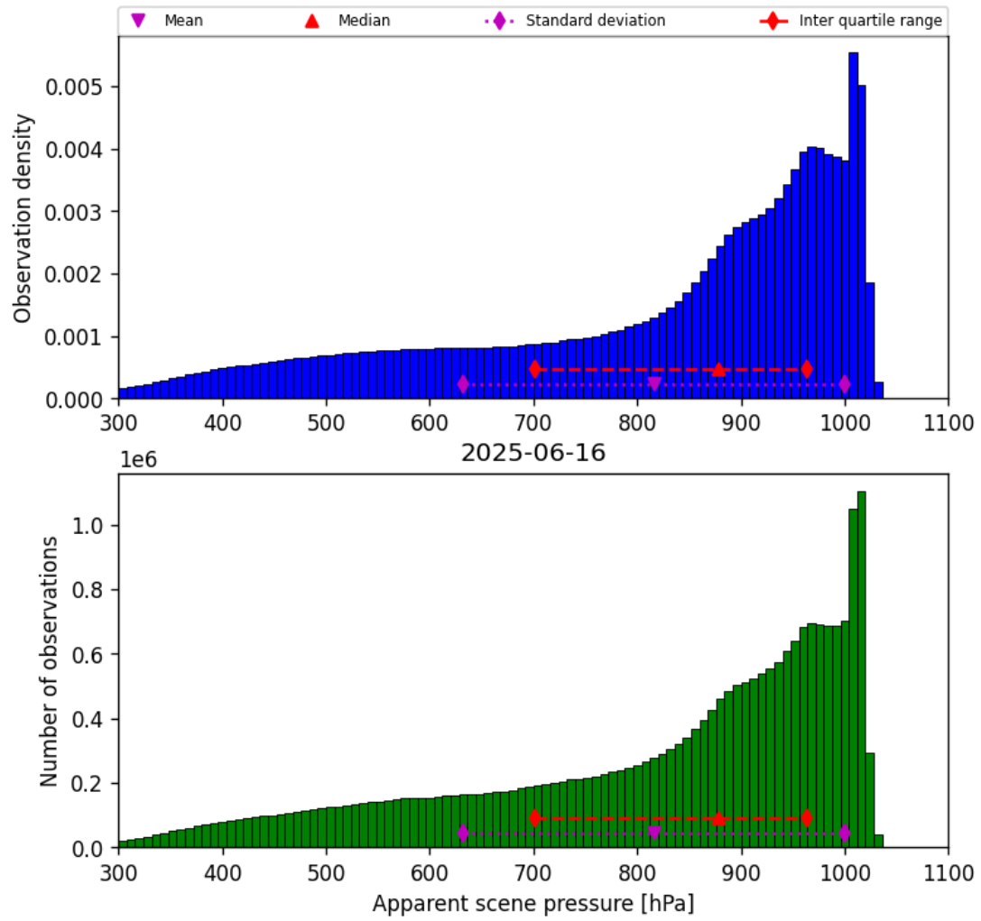
Figure 34: Histogram of “Apparent scene pressure” for 2025-06-16 to 2025-06-17
