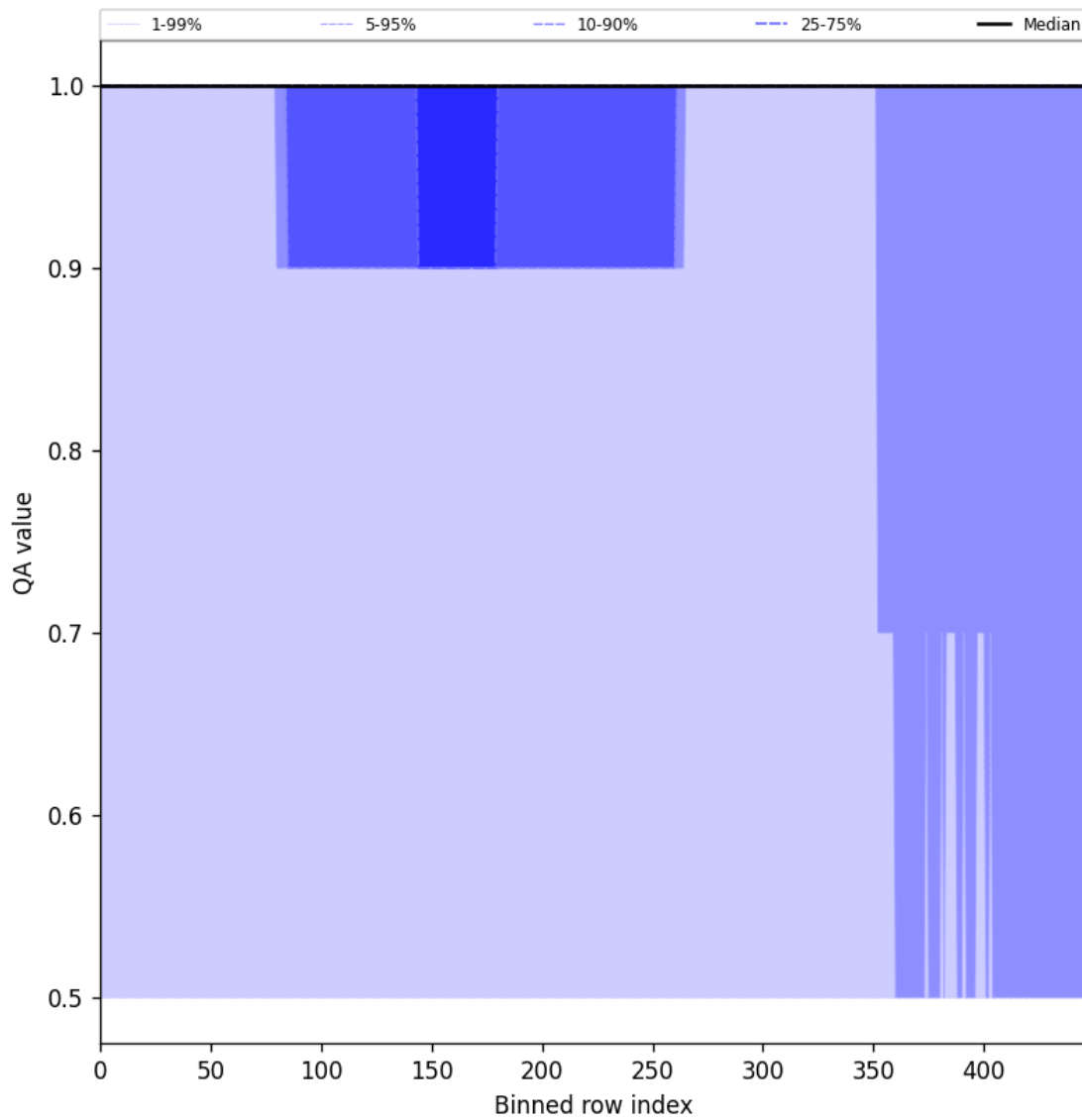
Figure 44: Along track statistics of “QA value” for 2025-06-16 to 2025-06-17
