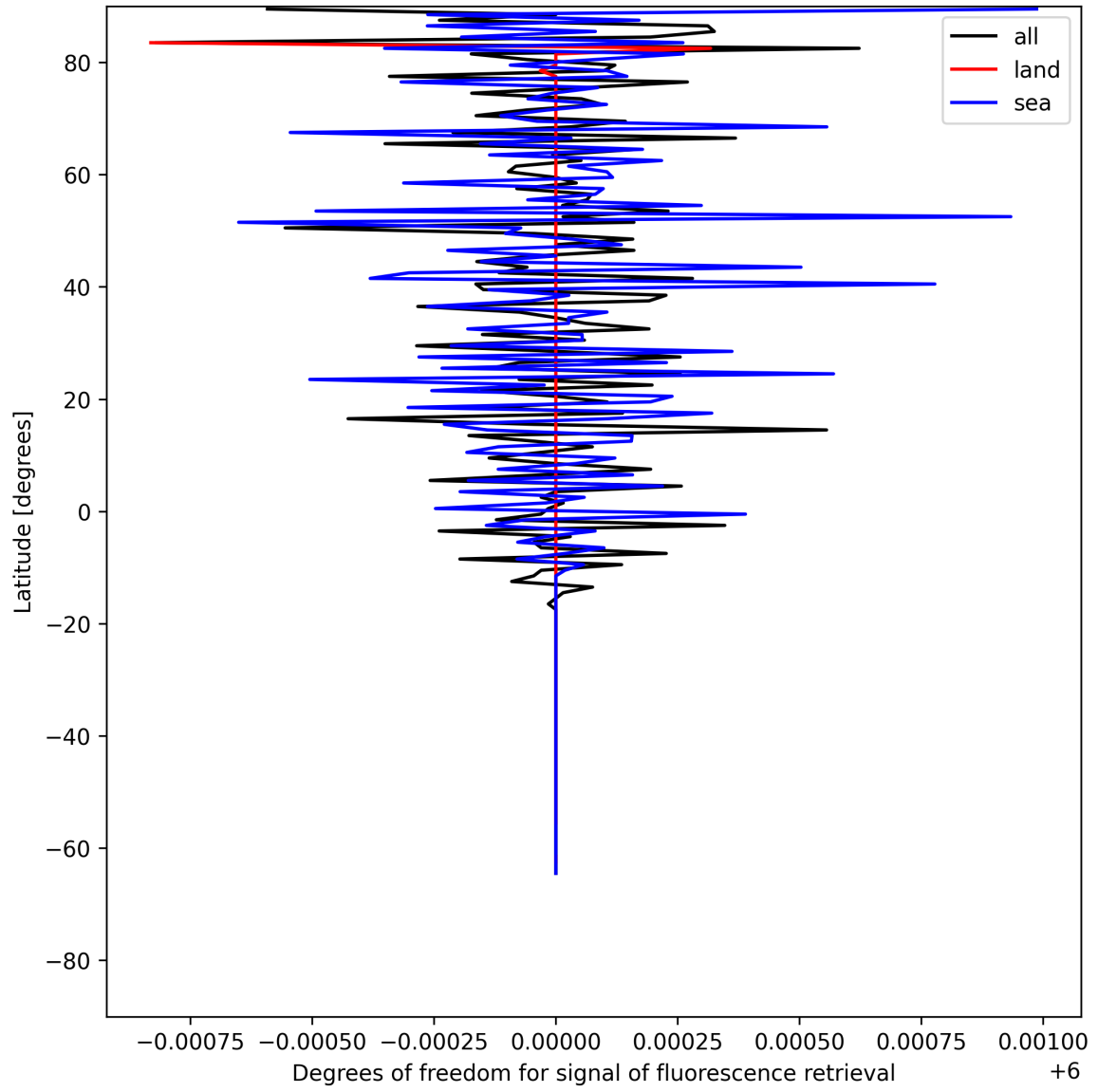
Figure 24: Zonal average of “Degrees of freedom for signal of fluorescence retrieval” for 2025-06-16 to 2025-06-17.
