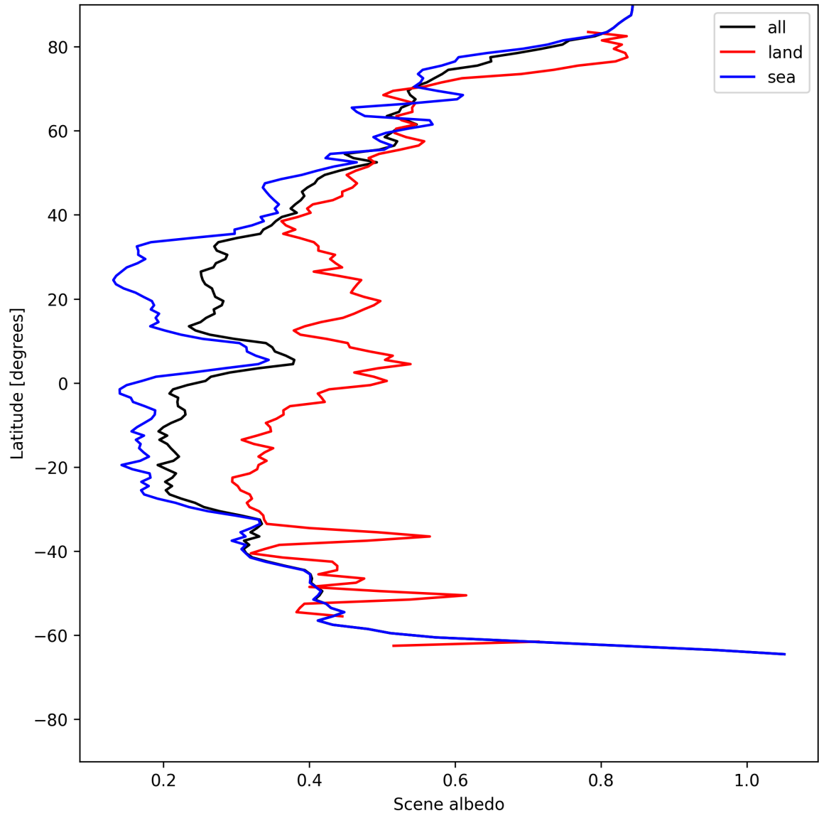
Figure 15: Zonal average of “Scene albedo” for 2025-06-16 to 2025-06-17.
