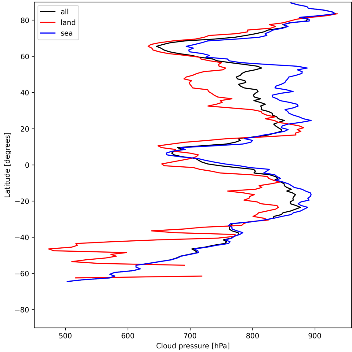
Figure 11: Zonal average of “Cloud pressure” for 2025-06-16 to 2025-06-17.
