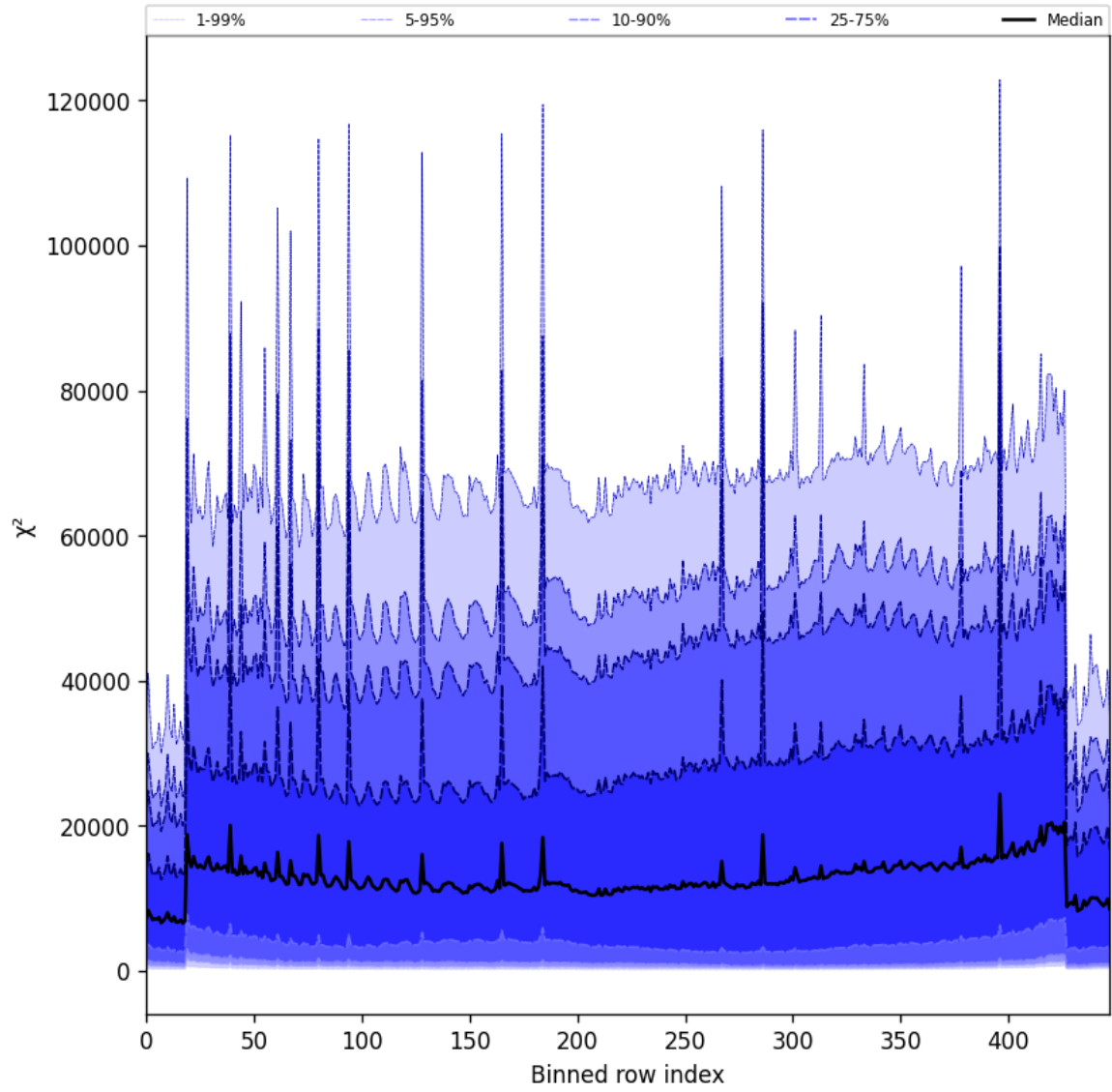
Figure 53: Along track statistics of “ \chi^2 ” for 2025-06-16 to 2025-06-17
