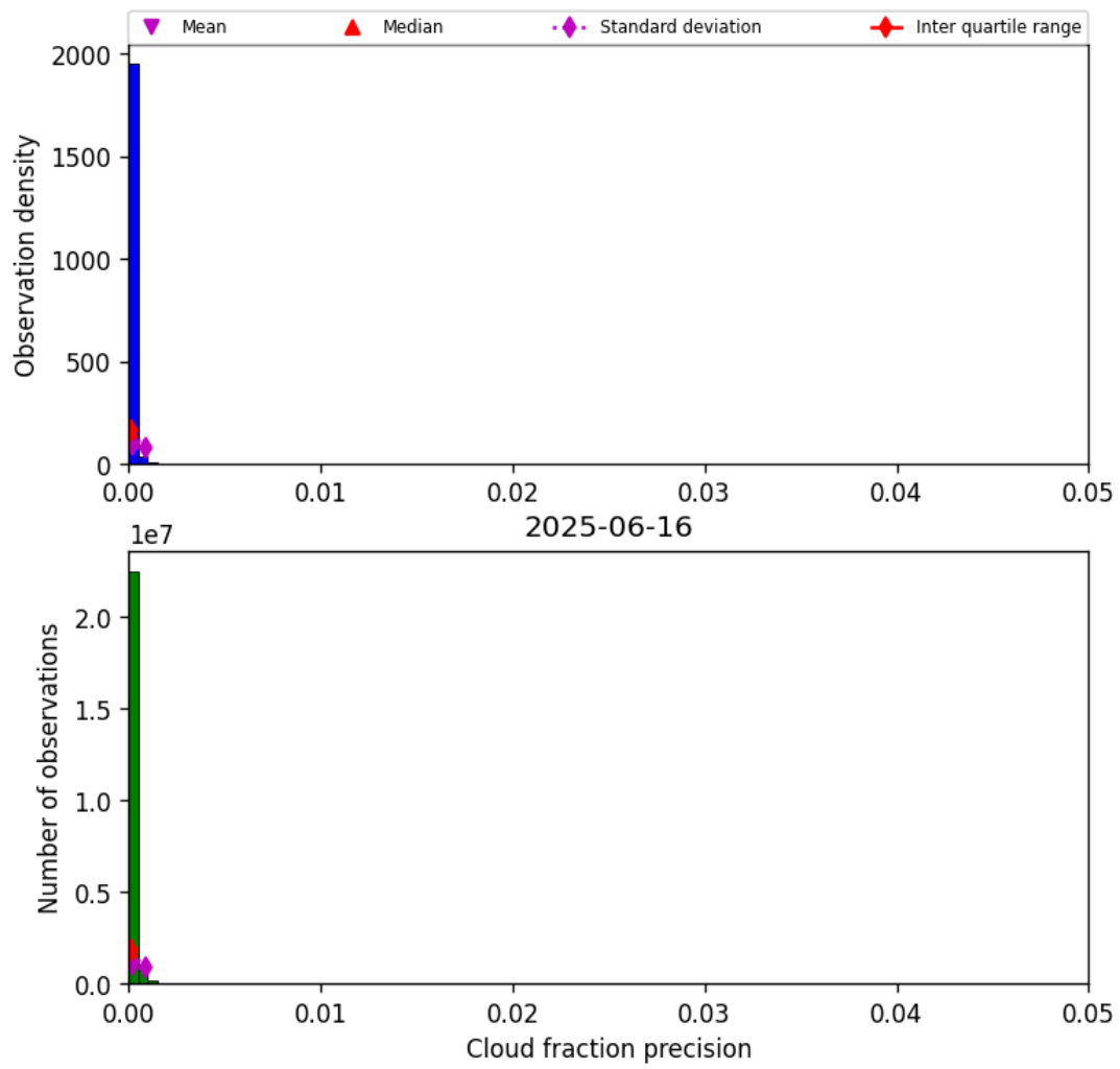
Figure 31: Histogram of “Cloud fraction precision” for 2025-06-16 to 2025-06-17
