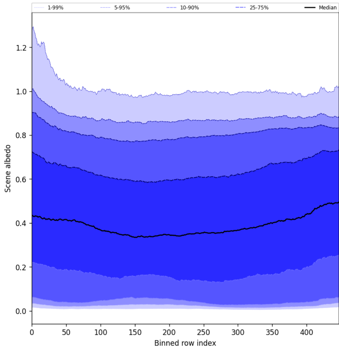
Figure 49: Along track statistics of “Scene albedo” for 2025-06-16 to 2025-06-17
