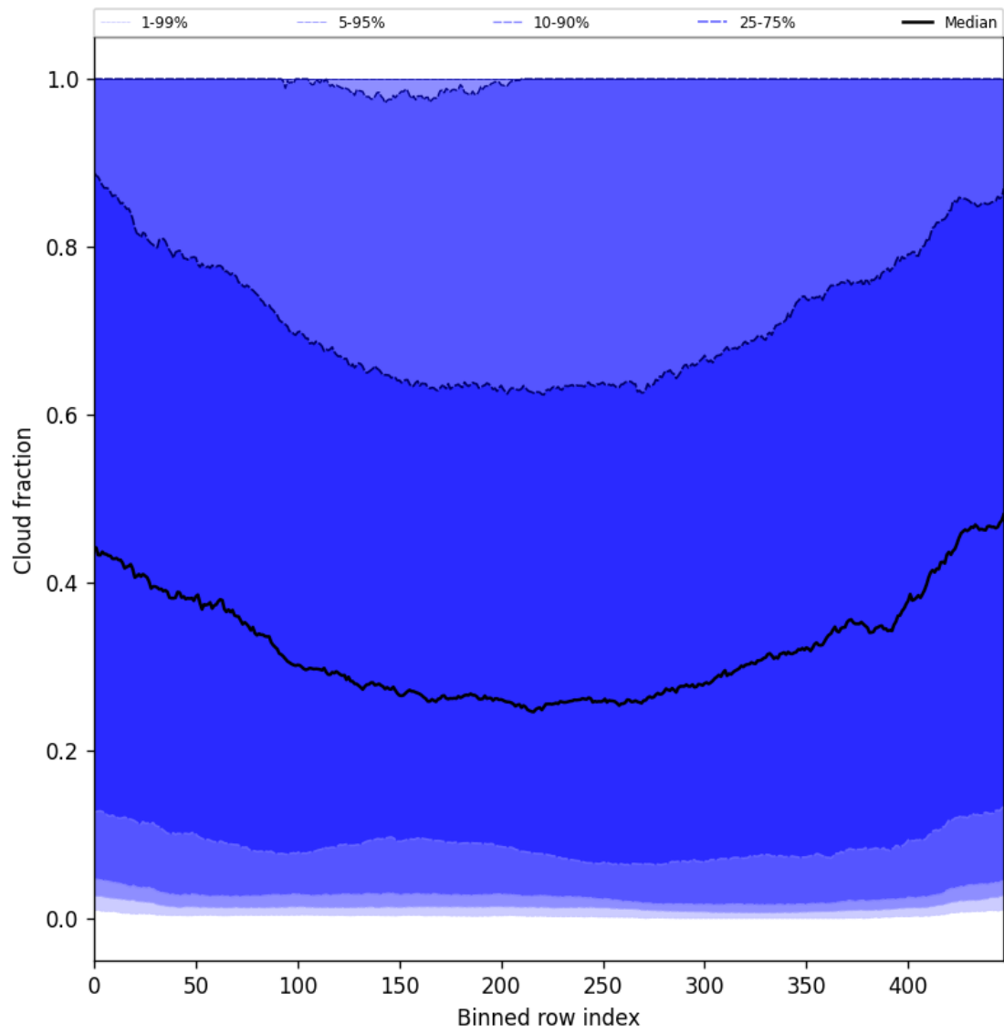
Figure 47: Along track statistics of “Cloud fraction” for 2025-06-16 to 2025-06-17
