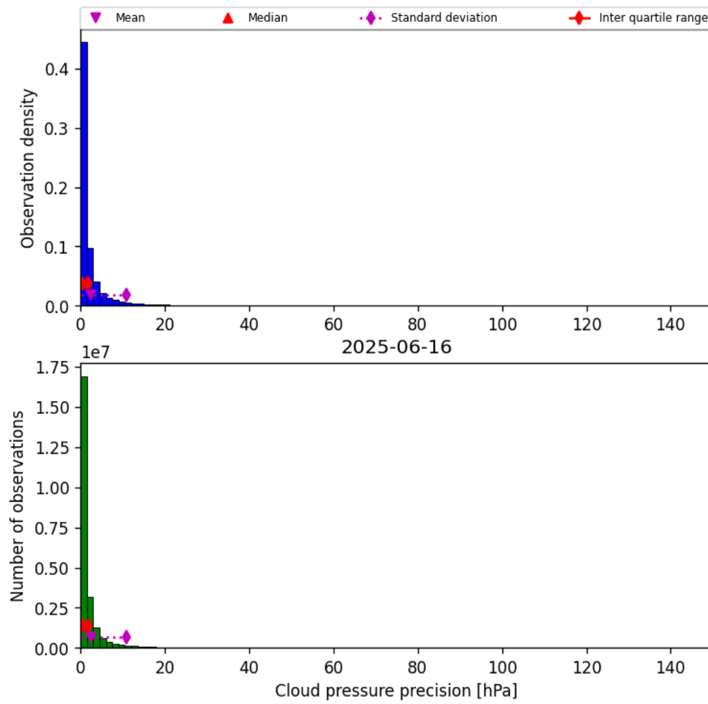
Figure 29: Histogram of “Cloud pressure precision” for 2025-06-16 to 2025-06-17
