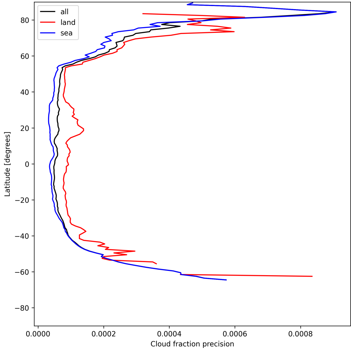
Figure 14: Zonal average of “Cloud fraction precision” for 2025-06-16 to 2025-06-17.
