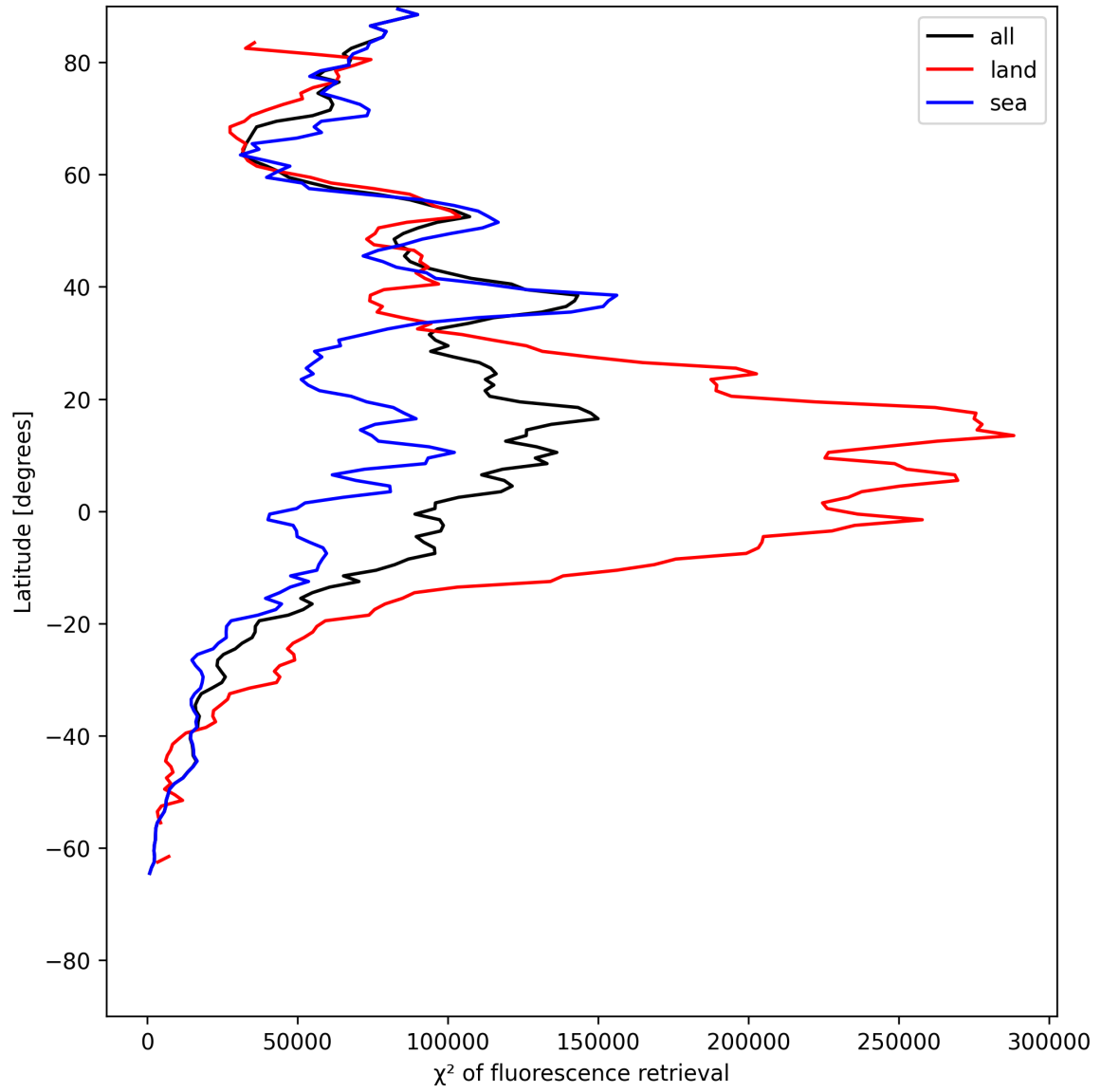
Figure 23: Zonal average of “ \chi^2 of fluorescence retrieval” for 2025-06-16 to 2025-06-17.
