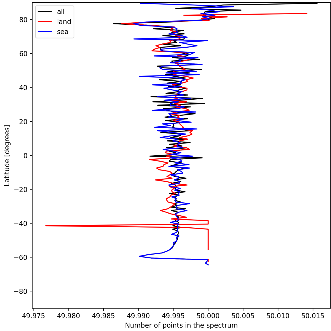
Figure 25: Zonal average of “Number of points in the spectrum” for 2025-06-16 to 2025-06-17.
