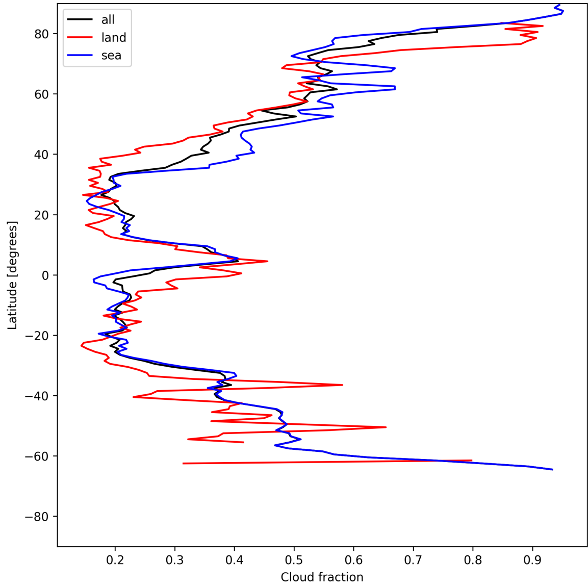
Figure 13: Zonal average of “Cloud fraction” for 2025-06-16 to 2025-06-17.
