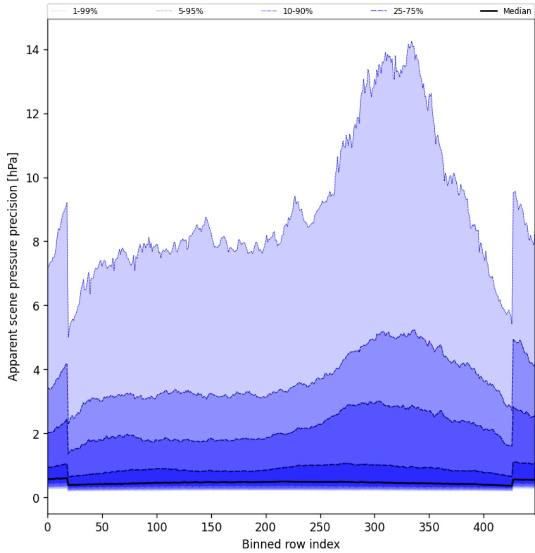
Figure 52: Along track statistics of “Apparent scene pressure precision” for 2025-06-16 to 2025-06-17
