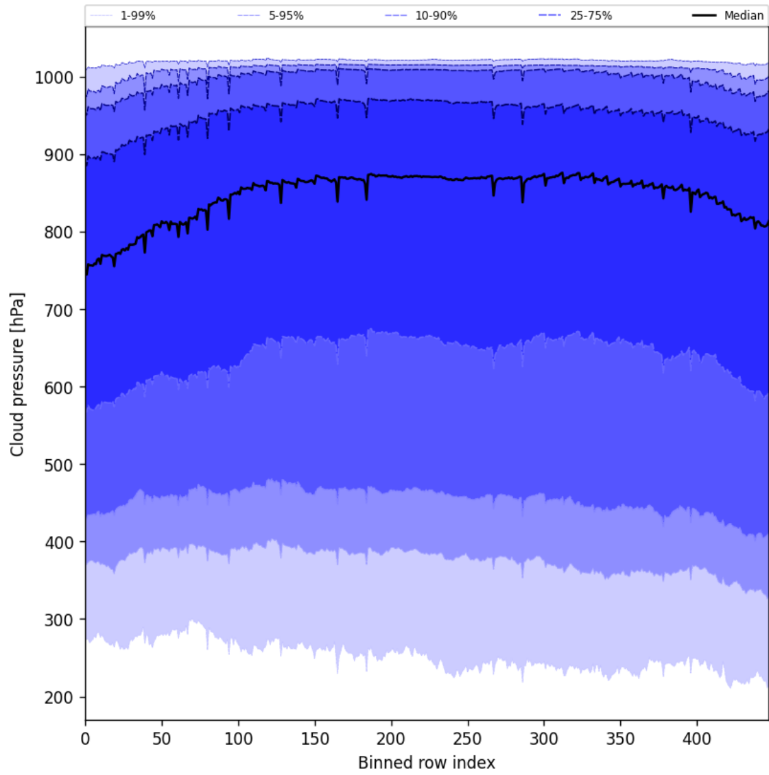
Figure 45: Along track statistics of “Cloud pressure” for 2025-06-16 to 2025-06-17
