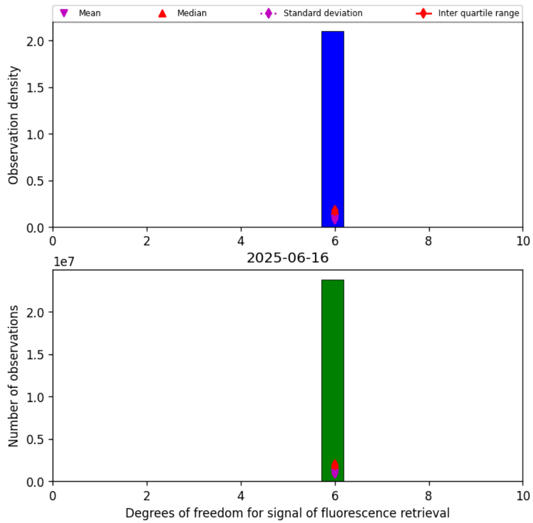
Figure 41: Histogram of “Degrees of freedom for signal of fluorescence retrieval” for 2025-06-16 to 2025-06-17
