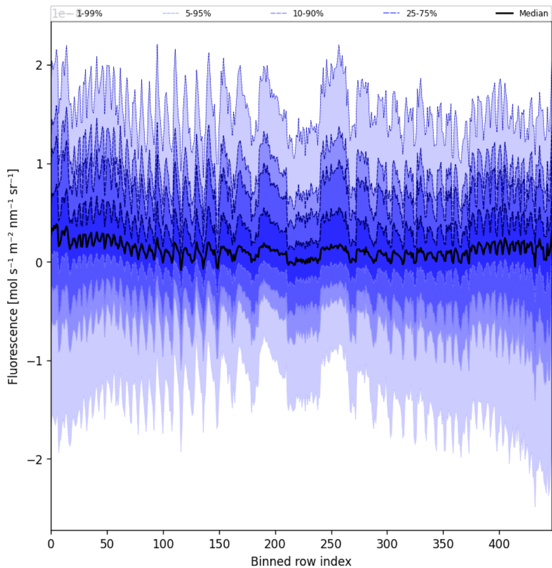
Figure 55: Along track statistics of “Fluorescence” for 2025-06-16 to 2025-06-17
