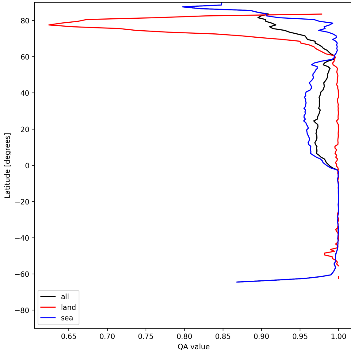
Figure 10: Zonal average of “QA value” for 2025-06-16 to 2025-06-17.
