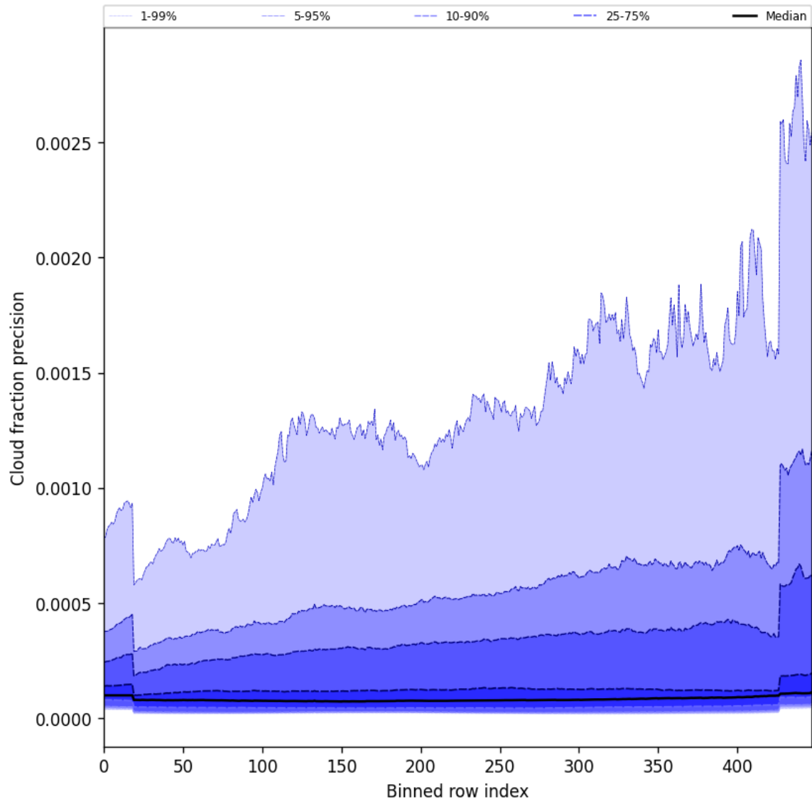
Figure 48: Along track statistics of “Cloud fraction precision” for 2025-06-16 to 2025-06-17
