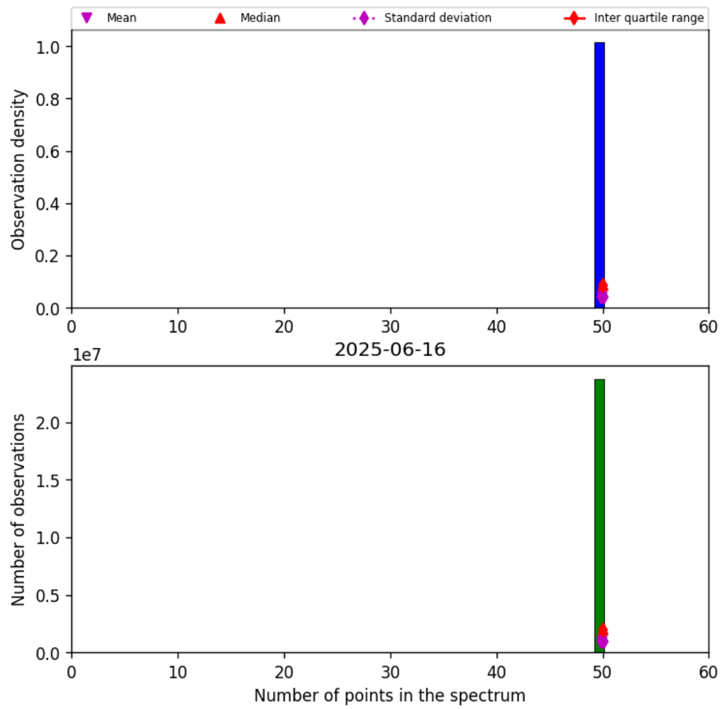
Figure 42: Histogram of “Number of points in the spectrum” for 2025-06-16 to 2025-06-17
