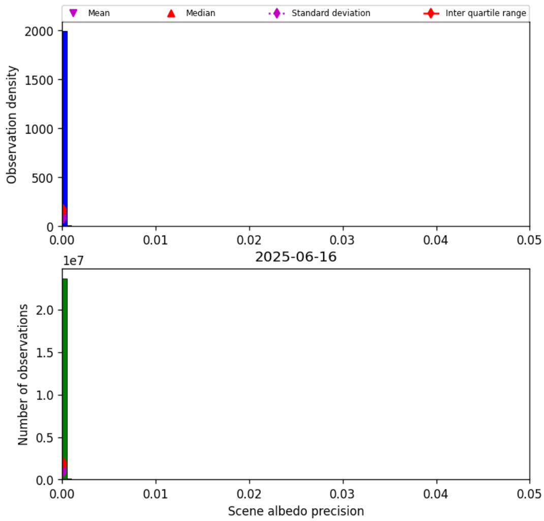
Figure 33: Histogram of “Scene albedo precision” for 2025-06-16 to 2025-06-17
