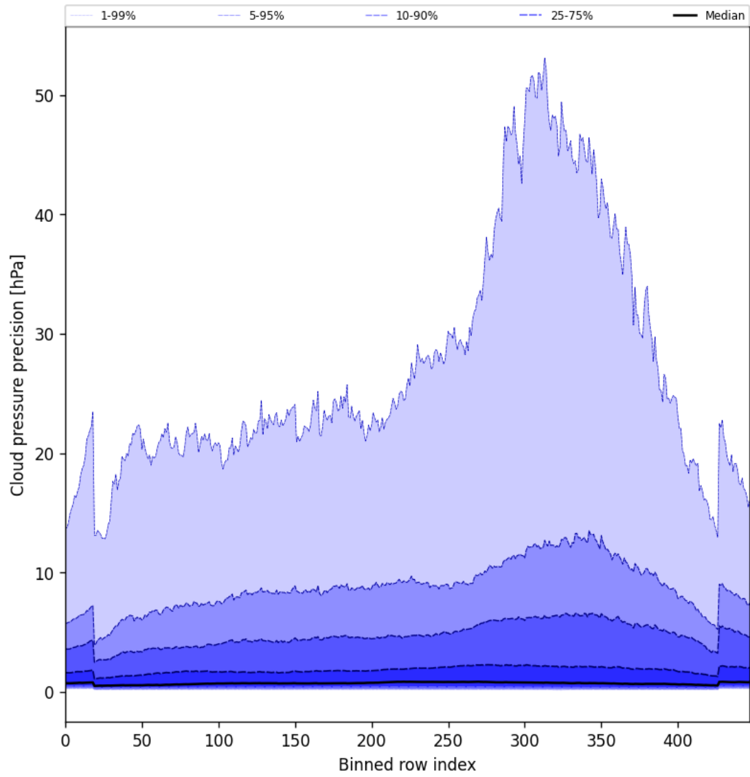
Figure 46: Along track statistics of “Cloud pressure precision” for 2025-06-16 to 2025-06-17
