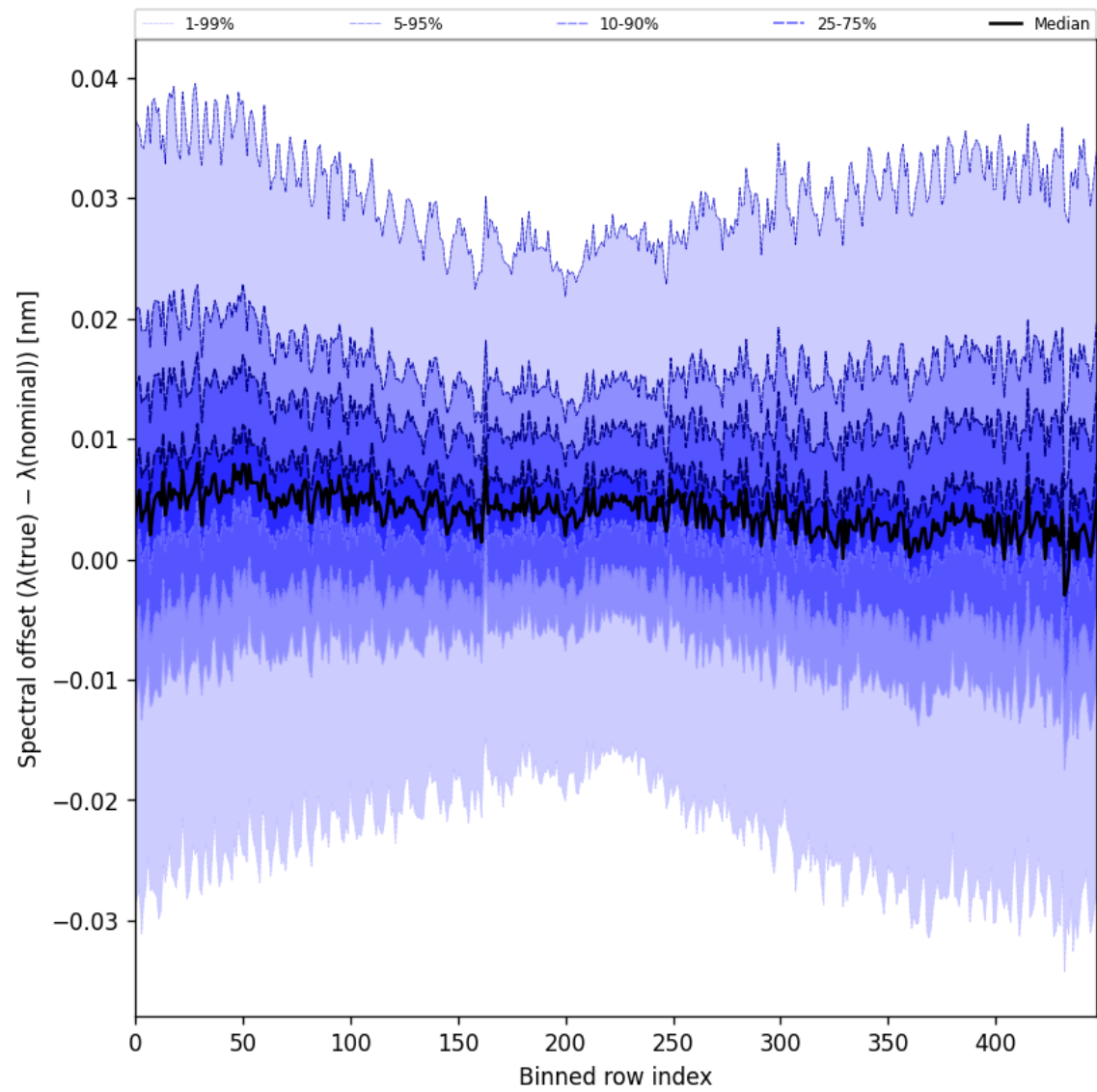
Figure 60: Along track statistics of “Spectral offset ( \lambda_{\text{true}} - \lambda_{\text{nominal}} )” for 2025-06-16 to 2025-06-17
