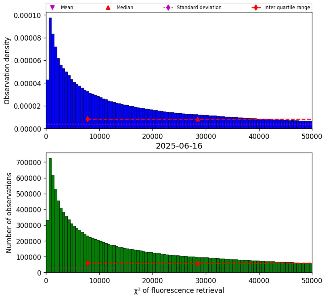
Figure 40: Histogram of “ \chi^2 of fluorescence retrieval” for 2025-06-16 to 2025-06-17
