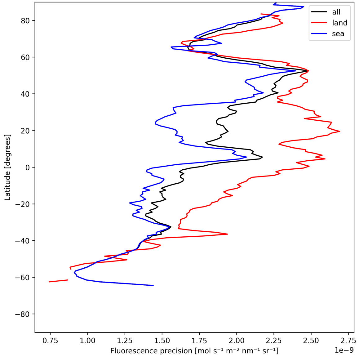
Figure 22: Zonal average of “Fluorescence precision” for 2025-06-16 to 2025-06-17.
