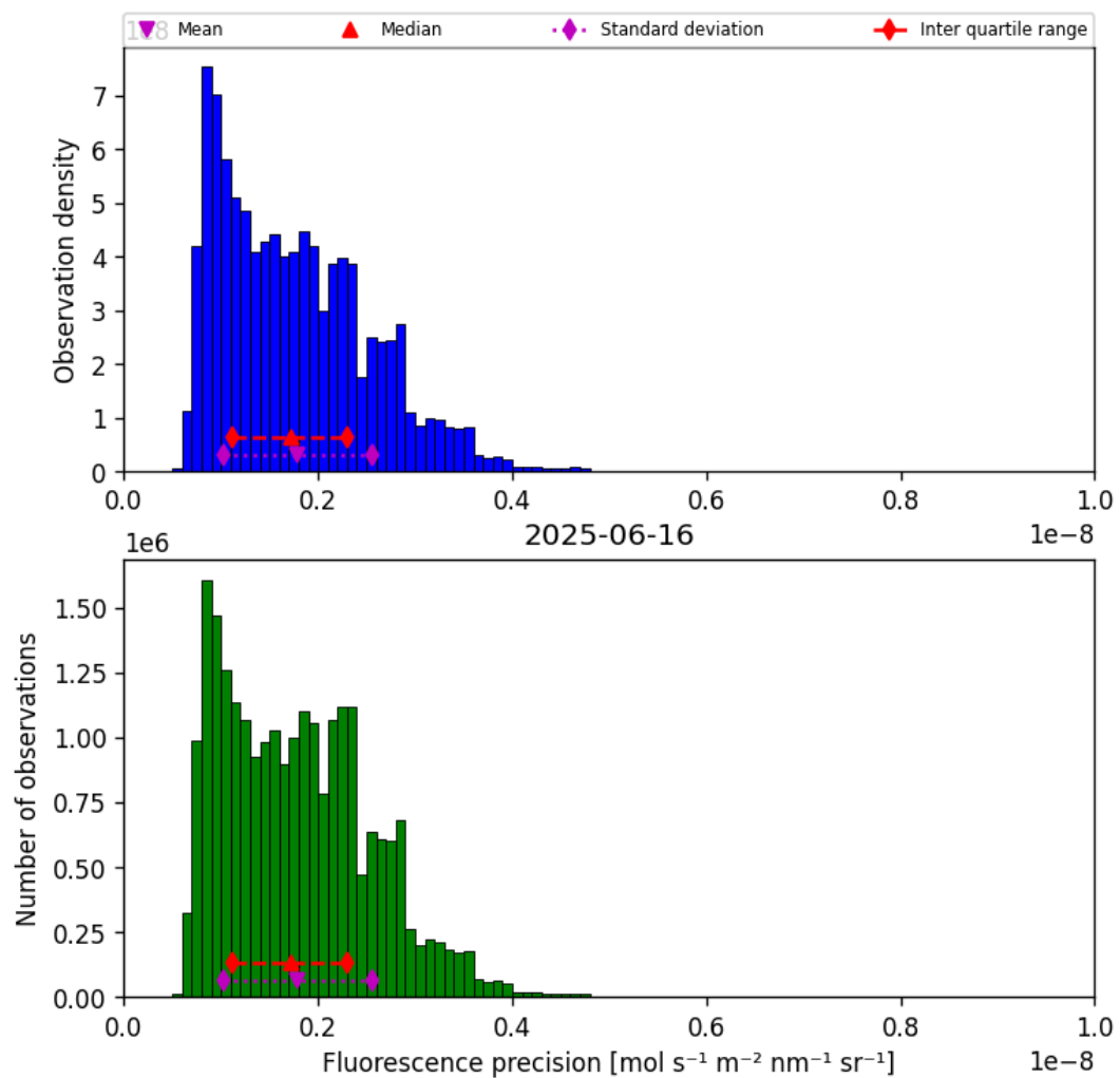
Figure 39: Histogram of “Fluorescence precision” for 2025-06-16 to 2025-06-17
