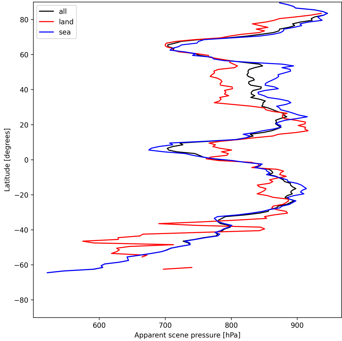
Figure 17: Zonal average of “Apparent scene pressure” for 2025-06-16 to 2025-06-17.
