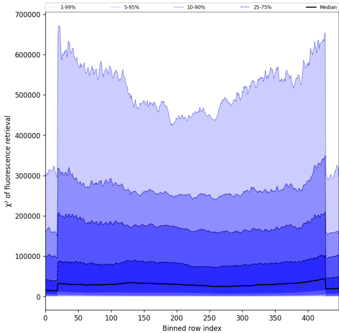
Figure 57: Along track statistics of “ \chi^2 of fluorescence retrieval” for 2025-06-16 to 2025-06-17
