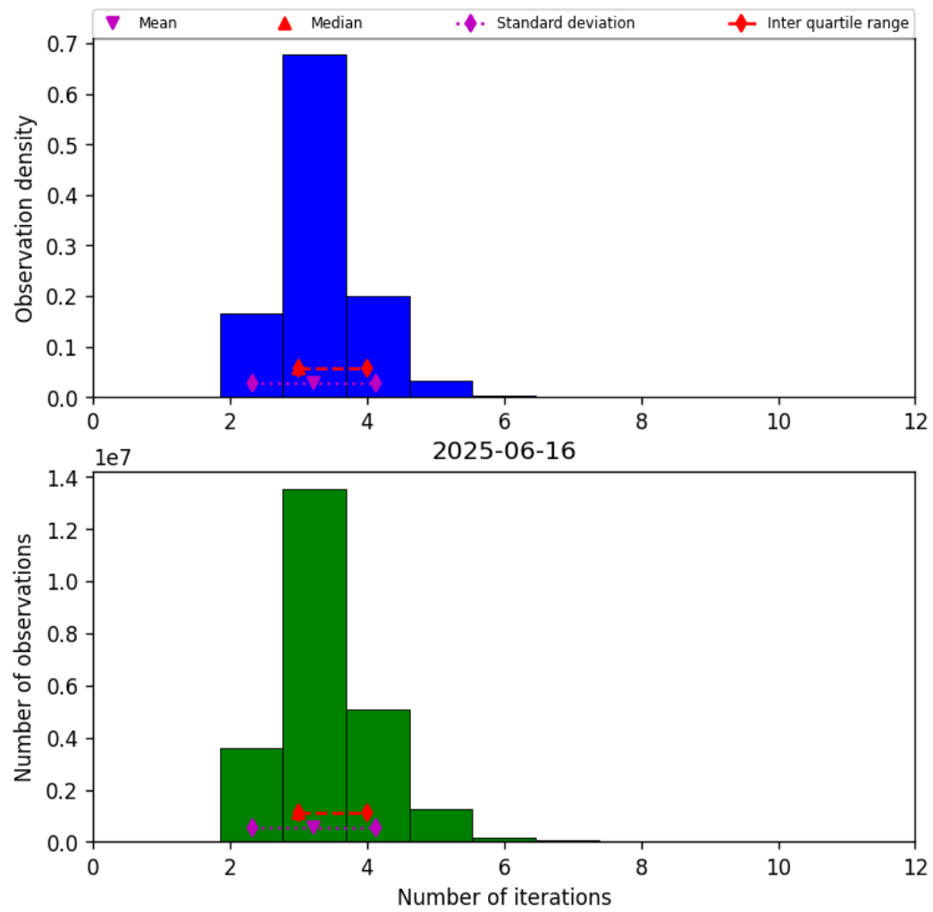
Figure 37: Histogram of “Number of iterations” for 2025-06-16 to 2025-06-17
