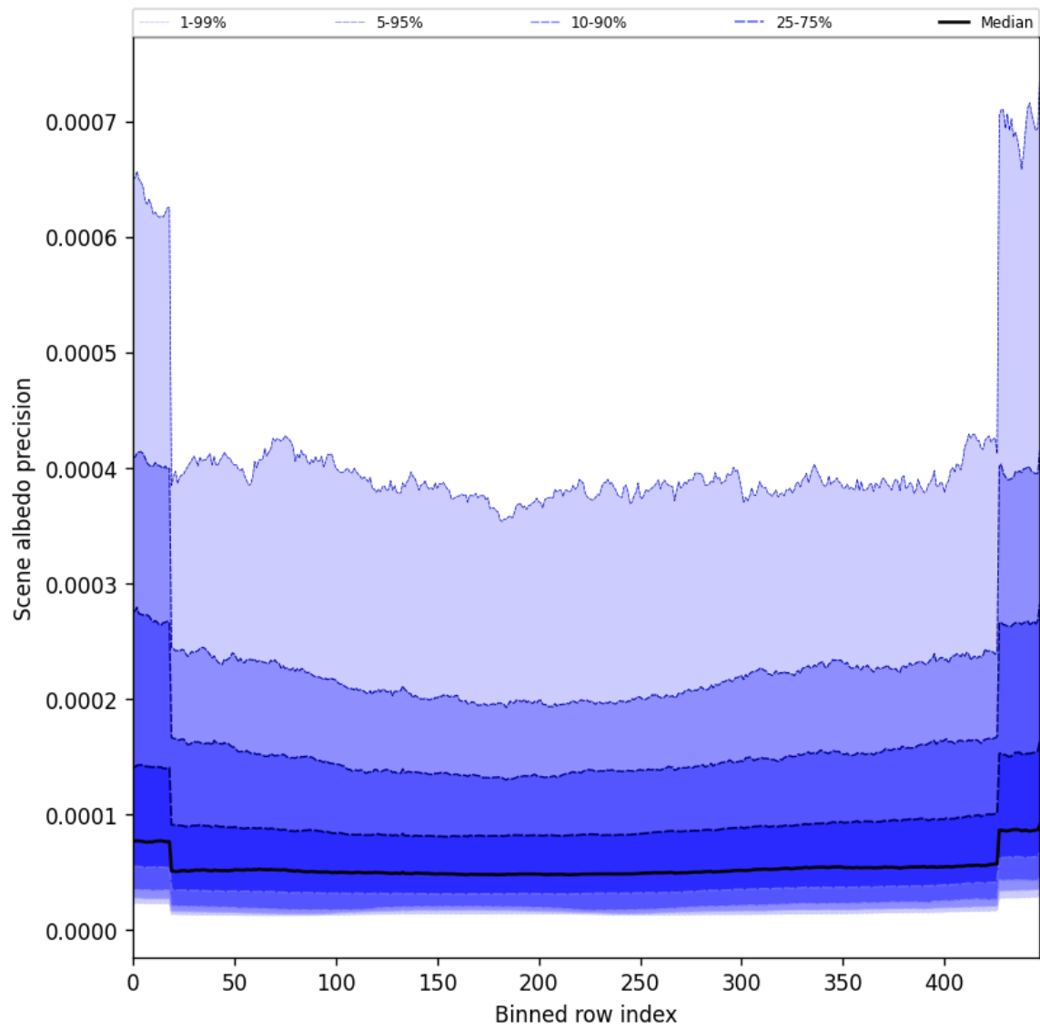
Figure 50: Along track statistics of “Scene albedo precision” for 2025-06-16 to 2025-06-17
