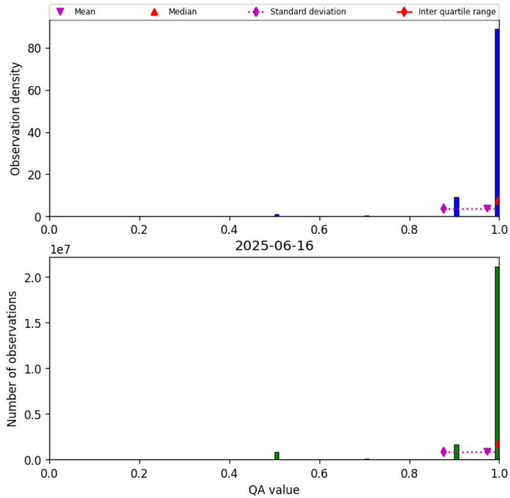
Figure 27: Histogram of “QA value” for 2025-06-16 to 2025-06-17
