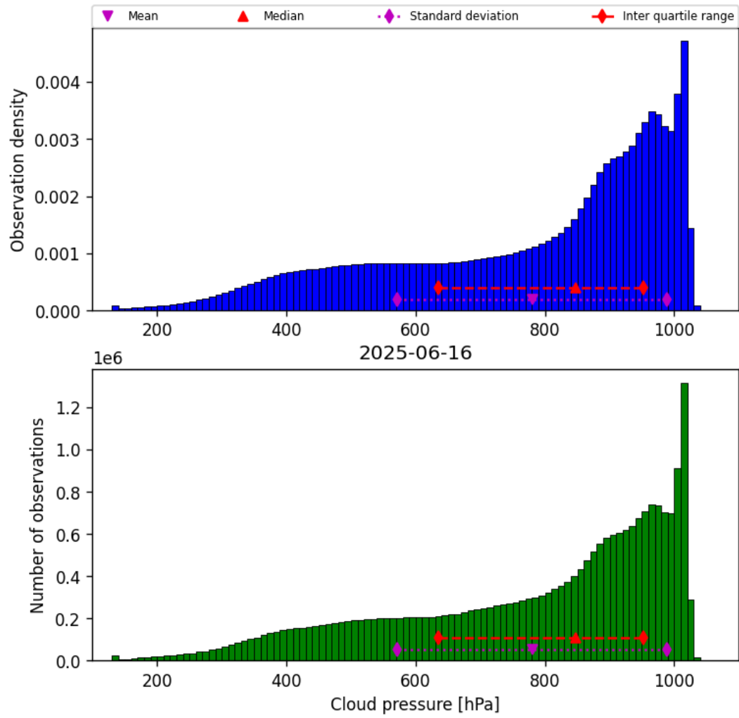
Figure 28: Histogram of “Cloud pressure” for 2025-06-16 to 2025-06-17
