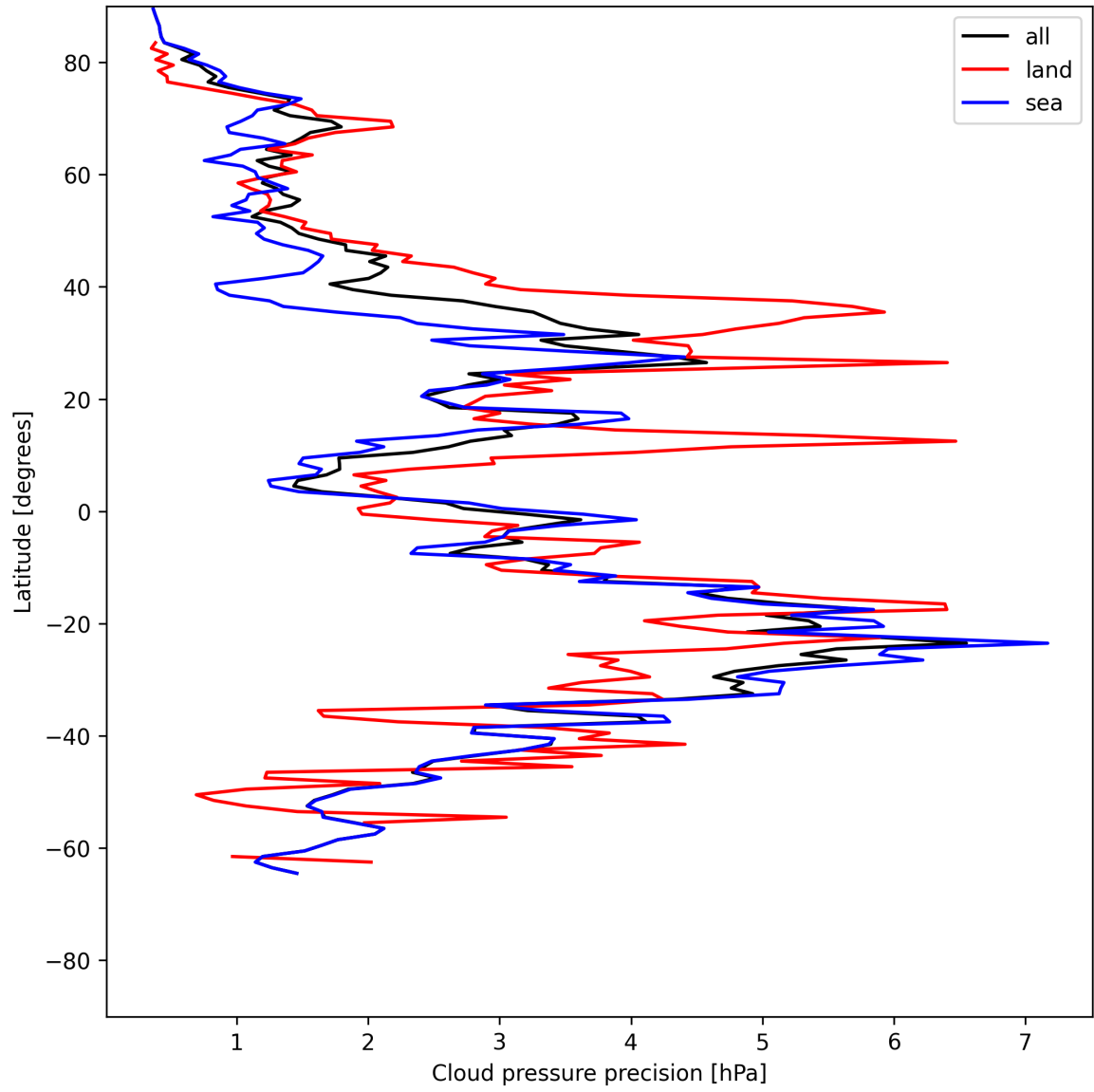
Figure 12: Zonal average of “Cloud pressure precision” for 2025-06-16 to 2025-06-17.
