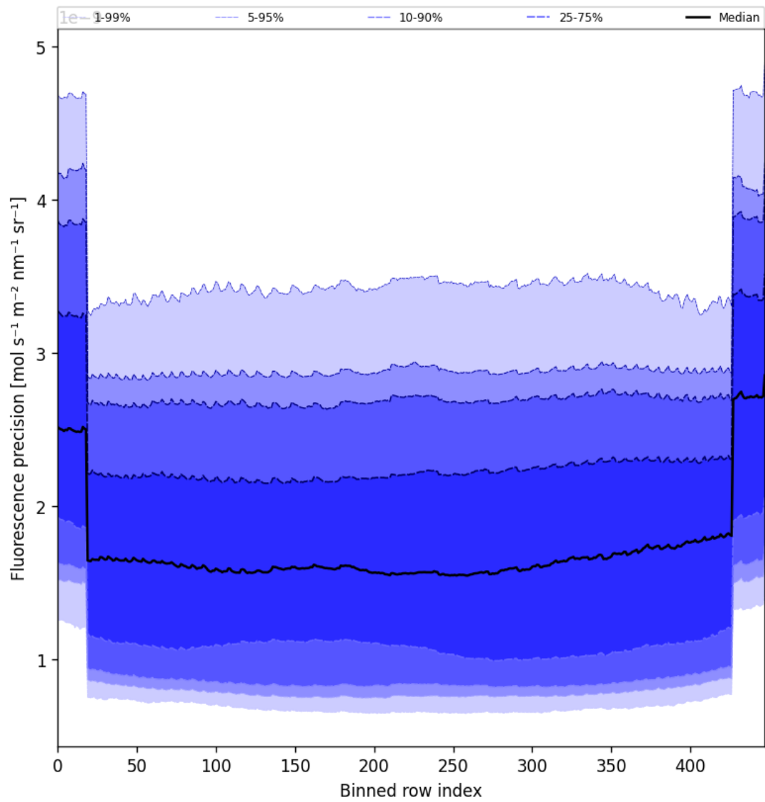
Figure 56: Along track statistics of “Fluorescence precision” for 2025-06-16 to 2025-06-17
