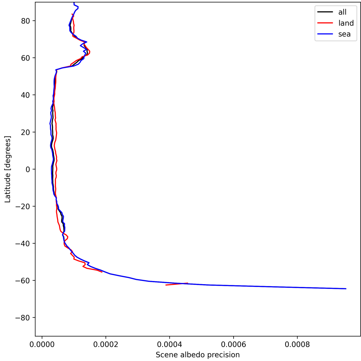
Figure 16: Zonal average of “Scene albedo precision” for 2025-06-16 to 2025-06-17.
