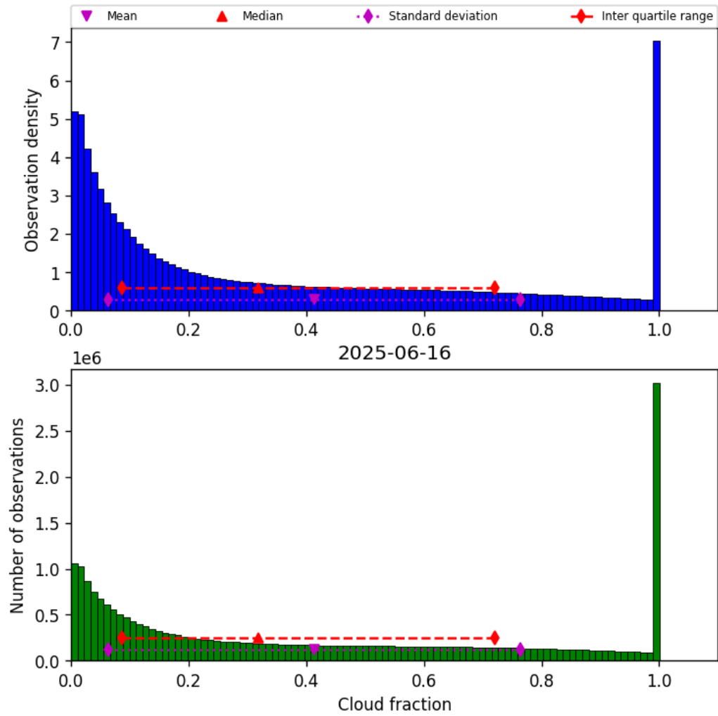
Figure 30: Histogram of “Cloud fraction” for 2025-06-16 to 2025-06-17
