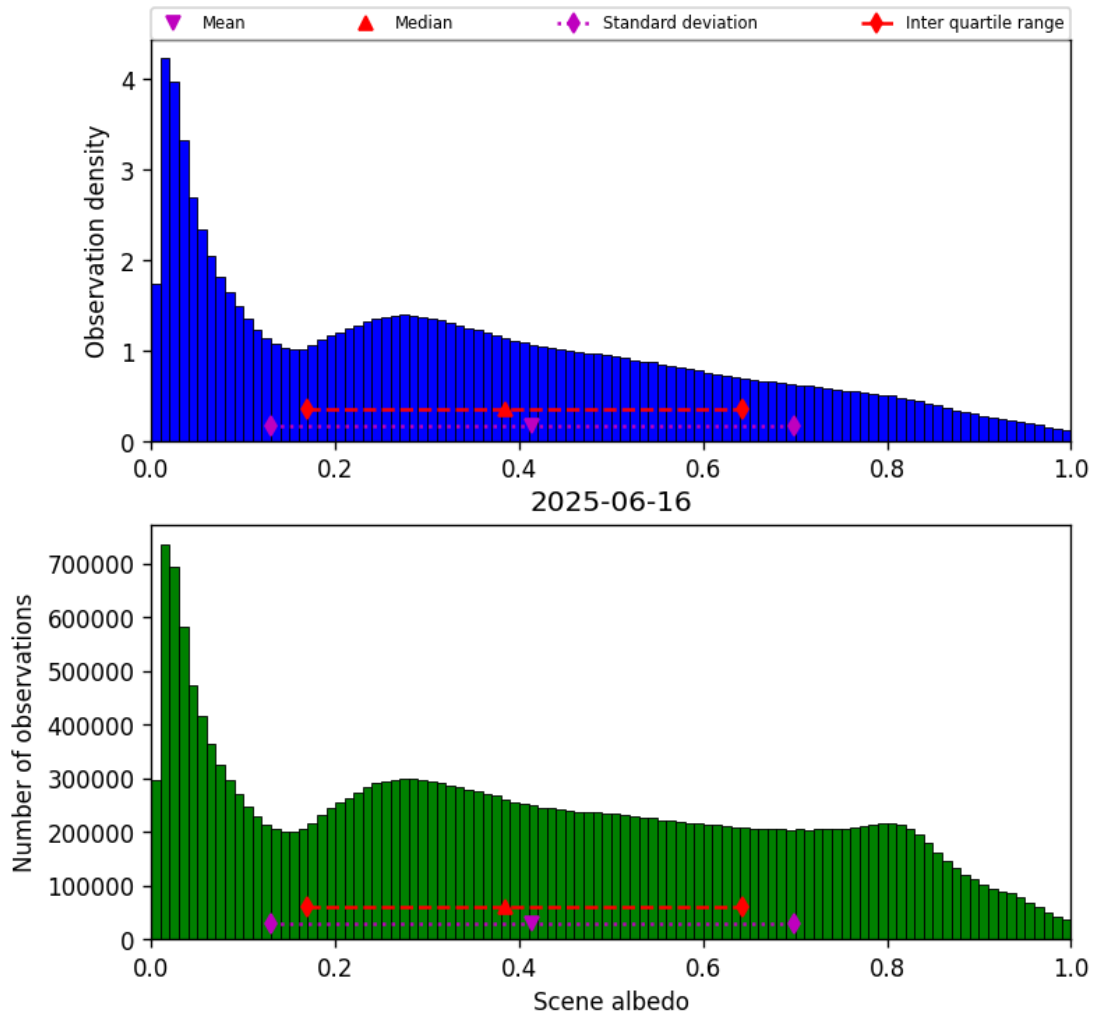
Figure 32: Histogram of “Scene albedo” for 2025-06-16 to 2025-06-17
