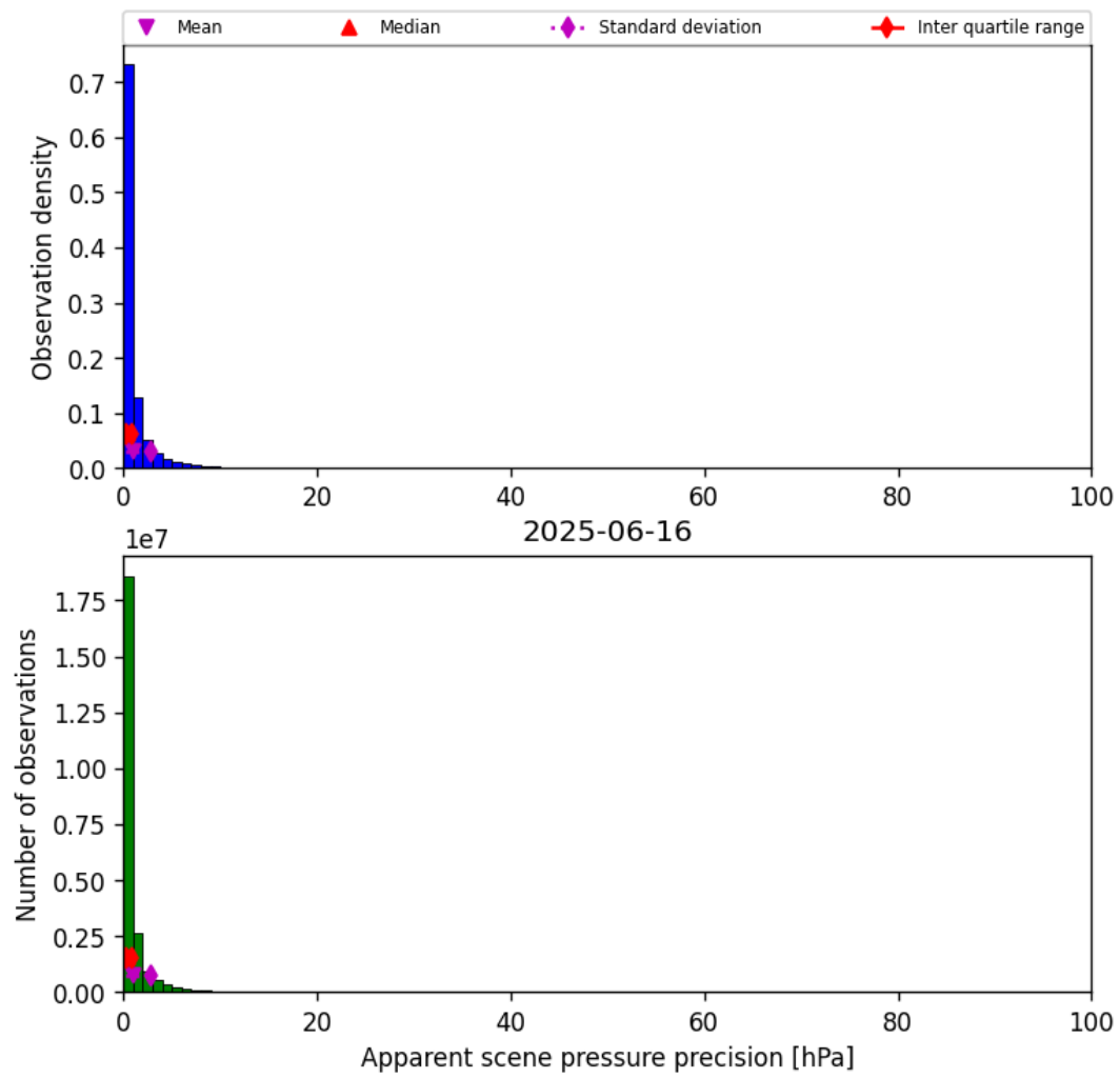
Figure 35: Histogram of “Apparent scene pressure precision” for 2025-06-16 to 2025-06-17
