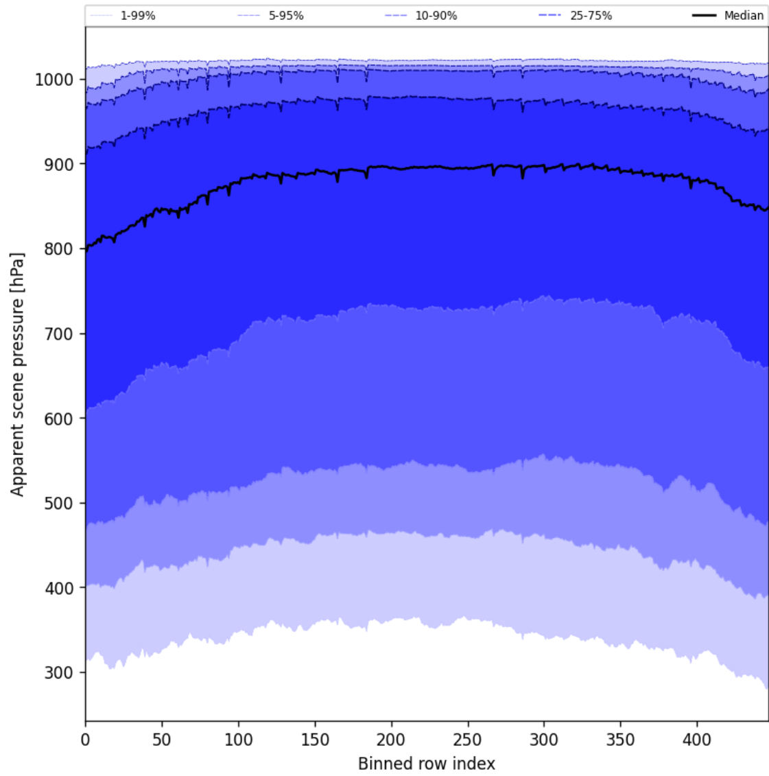
Figure 51: Along track statistics of “Apparent scene pressure” for 2025-06-16 to 2025-06-17
