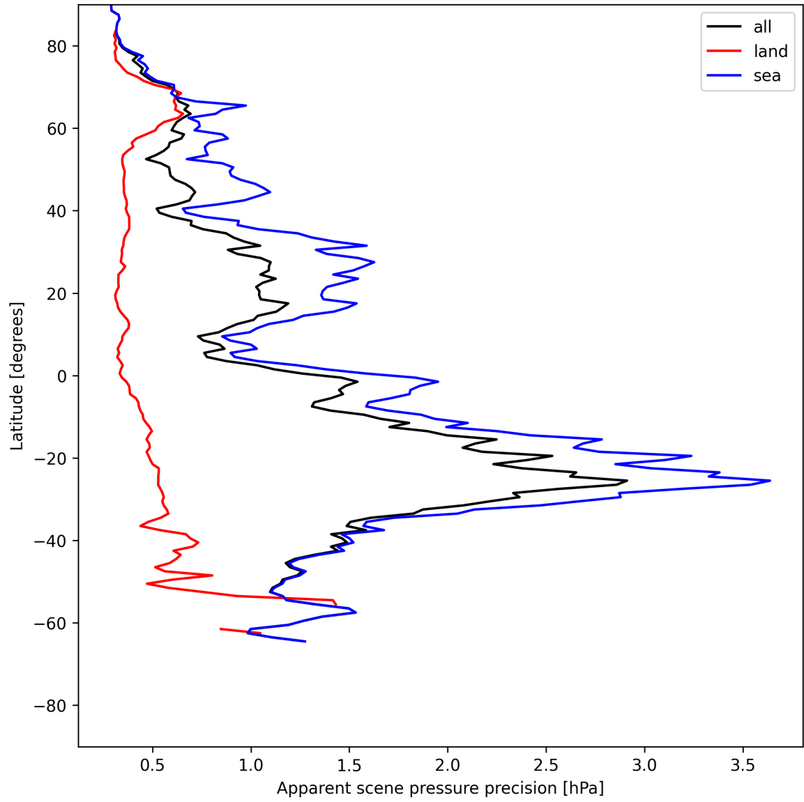
Figure 18: Zonal average of “Apparent scene pressure precision” for 2025-06-16 to 2025-06-17.
