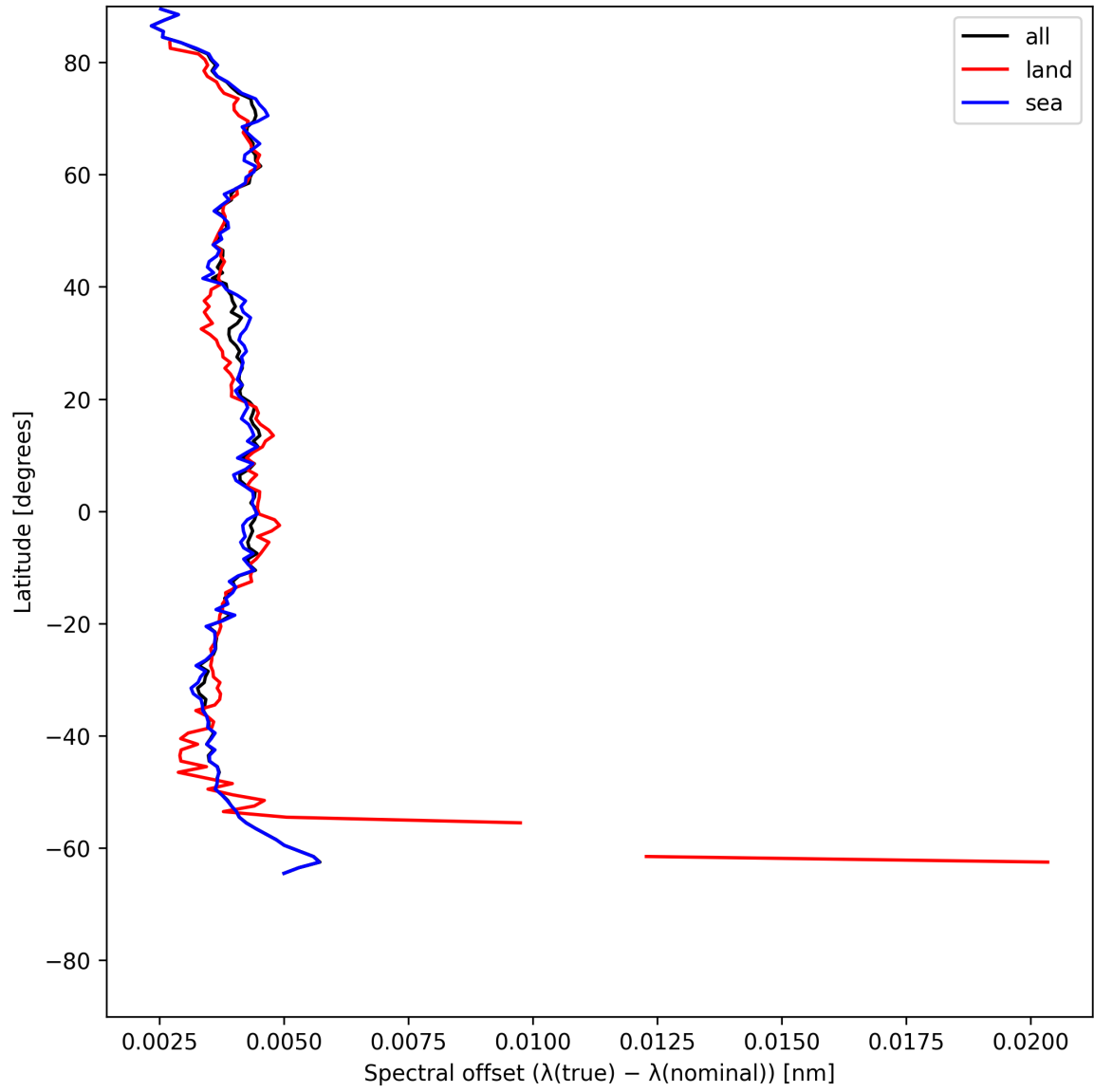
Figure 26: Zonal average of “Spectral offset ( \lambda_{\text{true}} - \lambda_{\text{nominal}} )” for 2025-06-16 to 2025-06-17.
