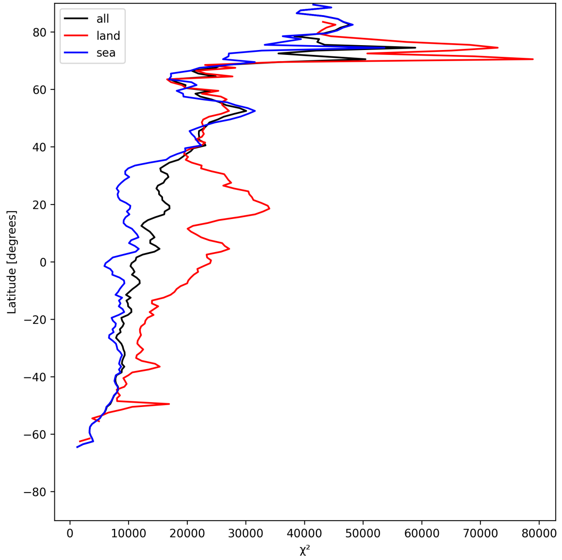
Figure 19: Zonal average of “ \chi^2 ” for 2025-06-16 to 2025-06-17.
