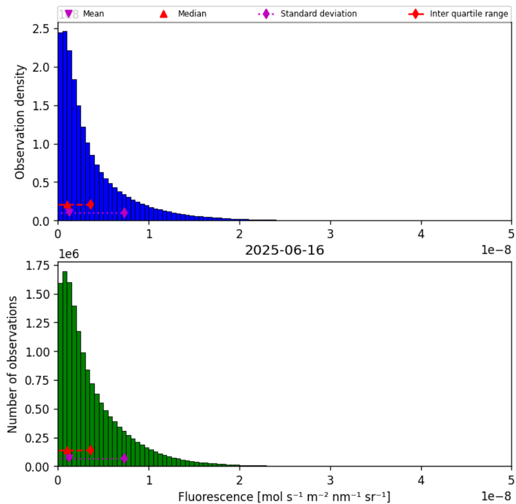
Figure 38: Histogram of “Fluorescence” for 2025-06-16 to 2025-06-17
