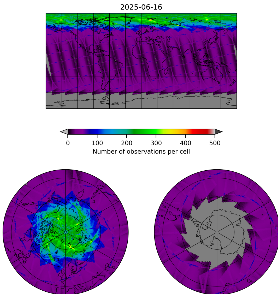
Figure 9: Map of the number of observations for 2025-06-16 to 2025-06-17
