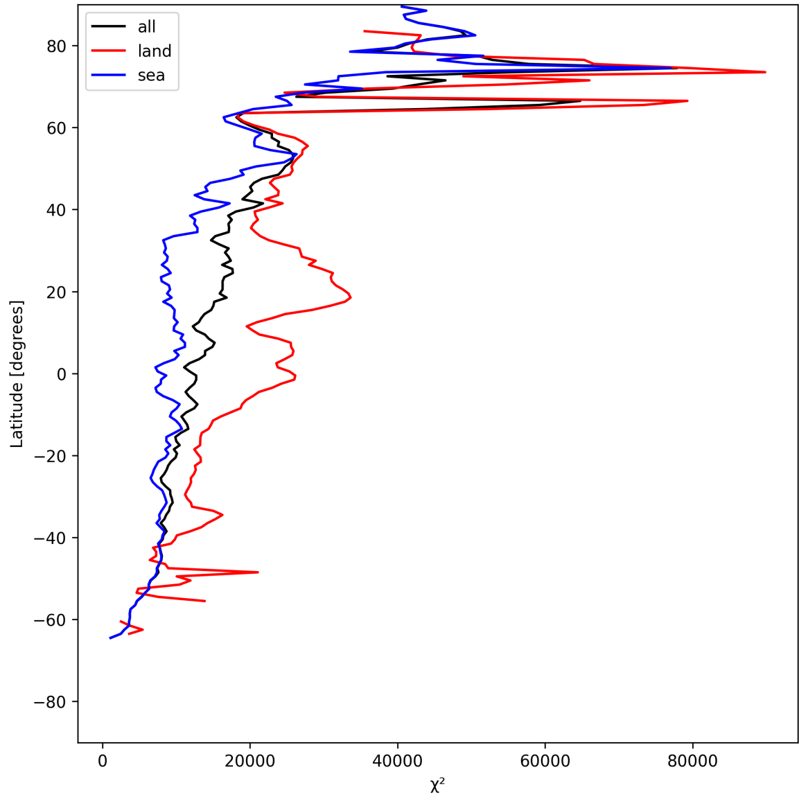
Figure 19: Zonal average of “ \chi^2 ” for 2025-06-17 to 2025-06-17.
