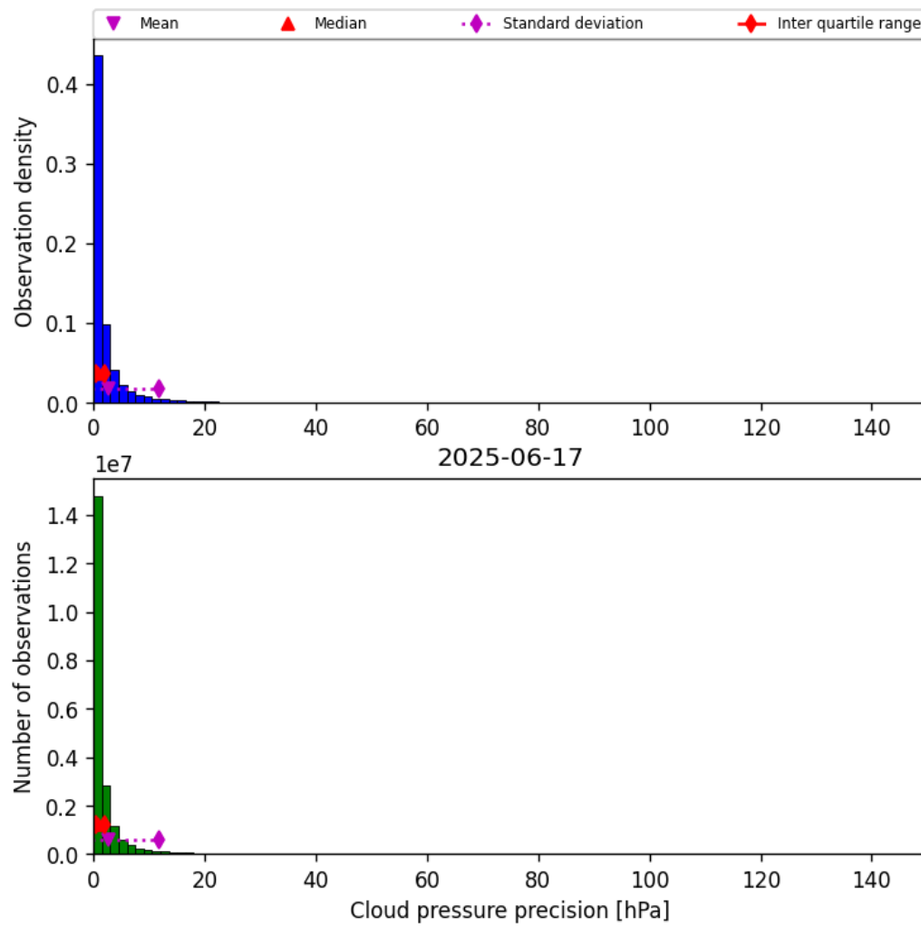
Figure 29: Histogram of “Cloud pressure precision” for 2025-06-17 to 2025-06-17
