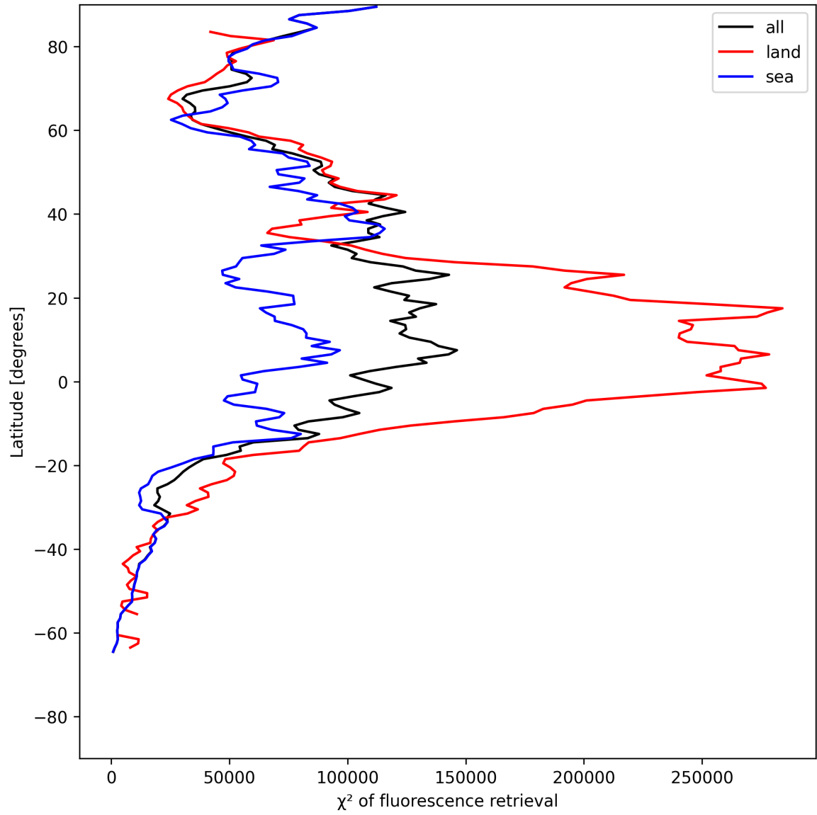
Figure 23: Zonal average of “ \chi^2 of fluorescence retrieval” for 2025-06-17 to 2025-06-17.
