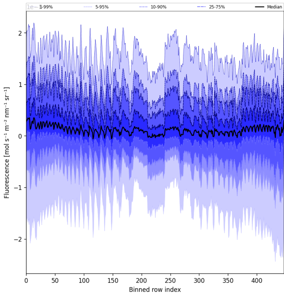
Figure 55: Along track statistics of “Fluorescence” for 2025-06-17 to 2025-06-17
