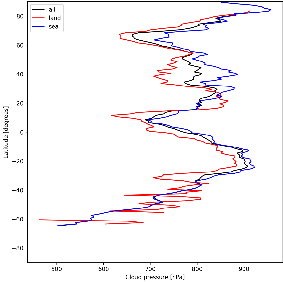
Figure 11: Zonal average of “Cloud pressure” for 2025-06-17 to 2025-06-17.
