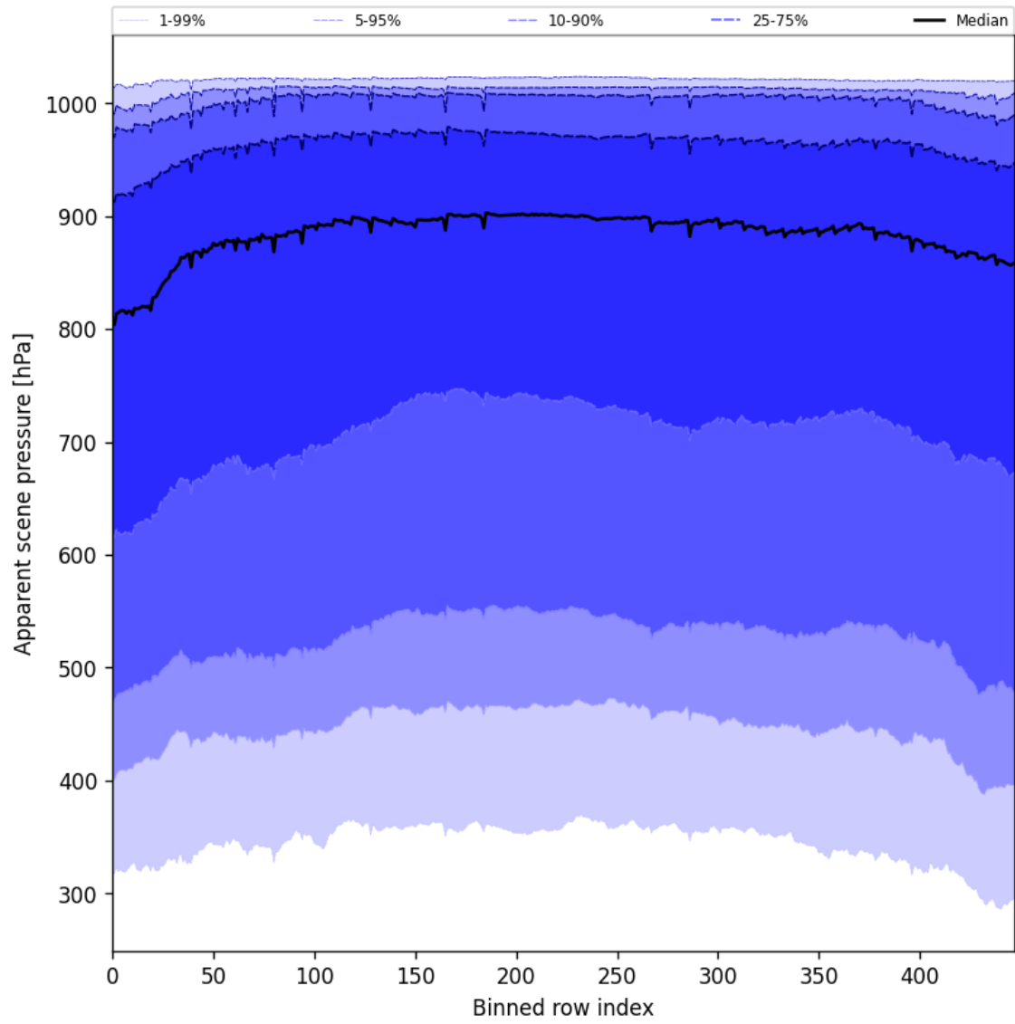
Figure 51: Along track statistics of “Apparent scene pressure” for 2025-06-17 to 2025-06-17
