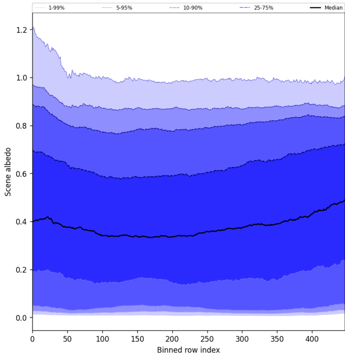
Figure 49: Along track statistics of "Scene albedo" for 2025-06-17 to 2025-06-17
