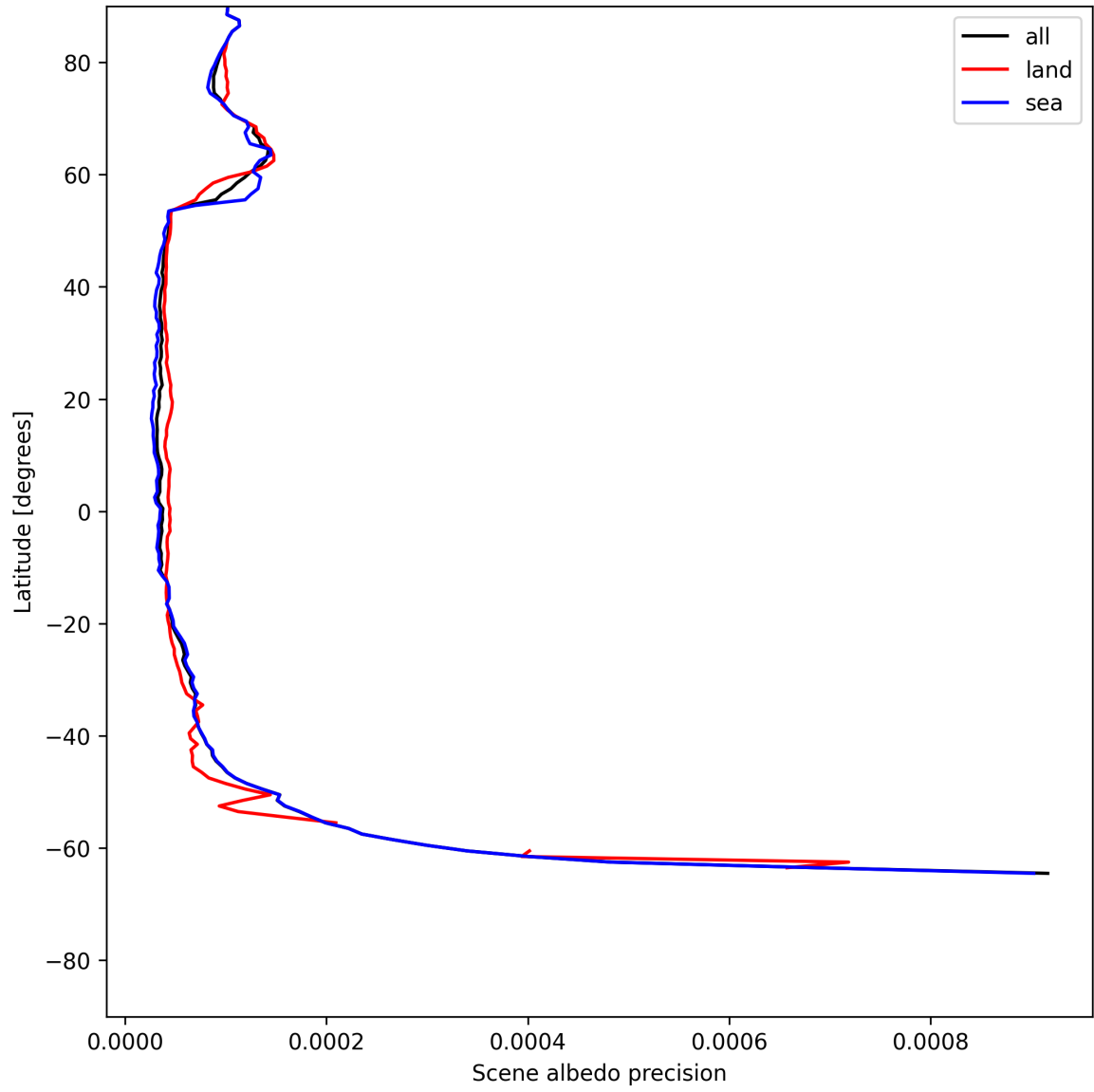
Figure 16: Zonal average of “Scene albedo precision” for 2025-06-17 to 2025-06-17.
