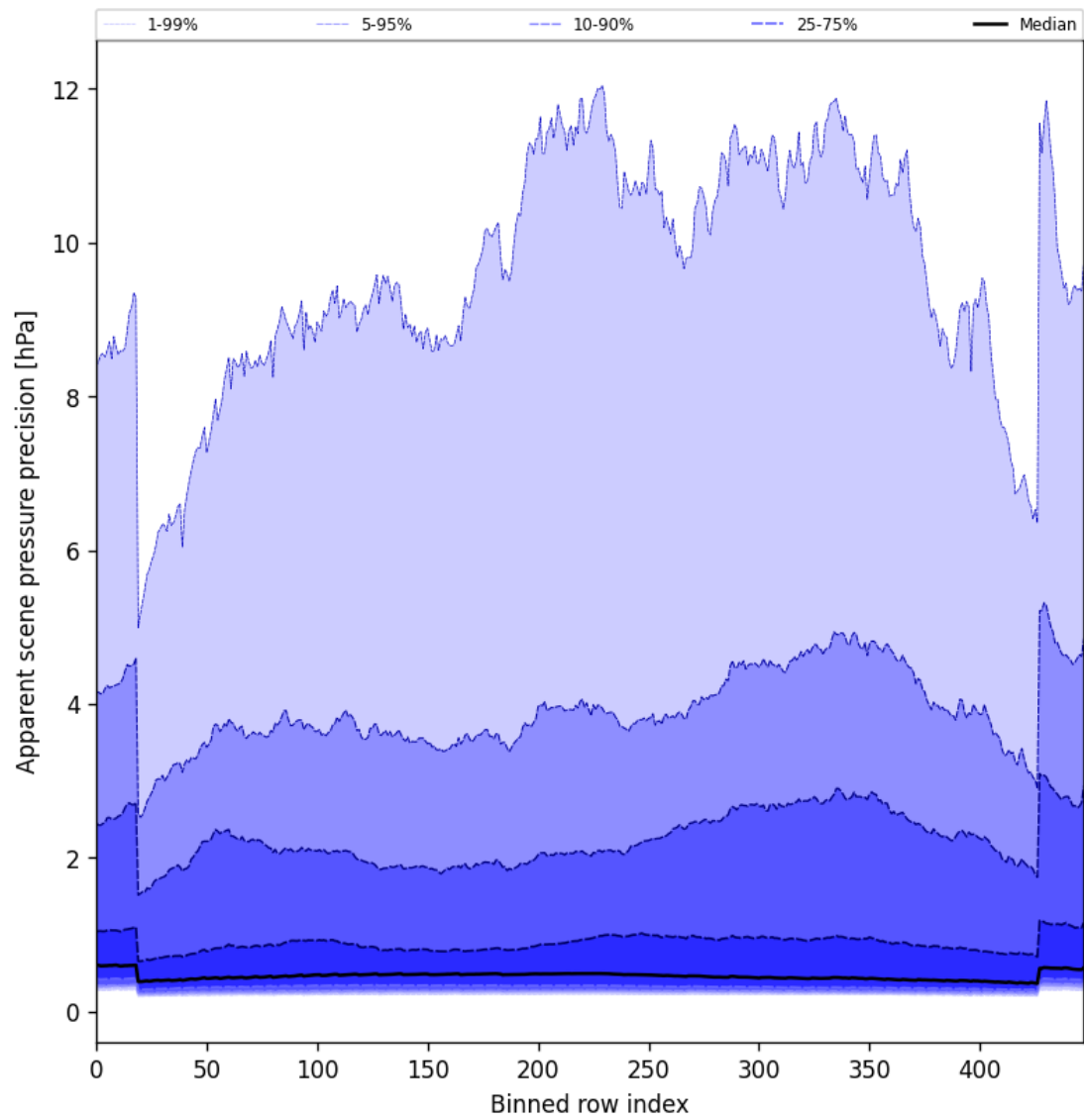
Figure 52: Along track statistics of “Apparent scene pressure precision” for 2025-06-17 to 2025-06-17
