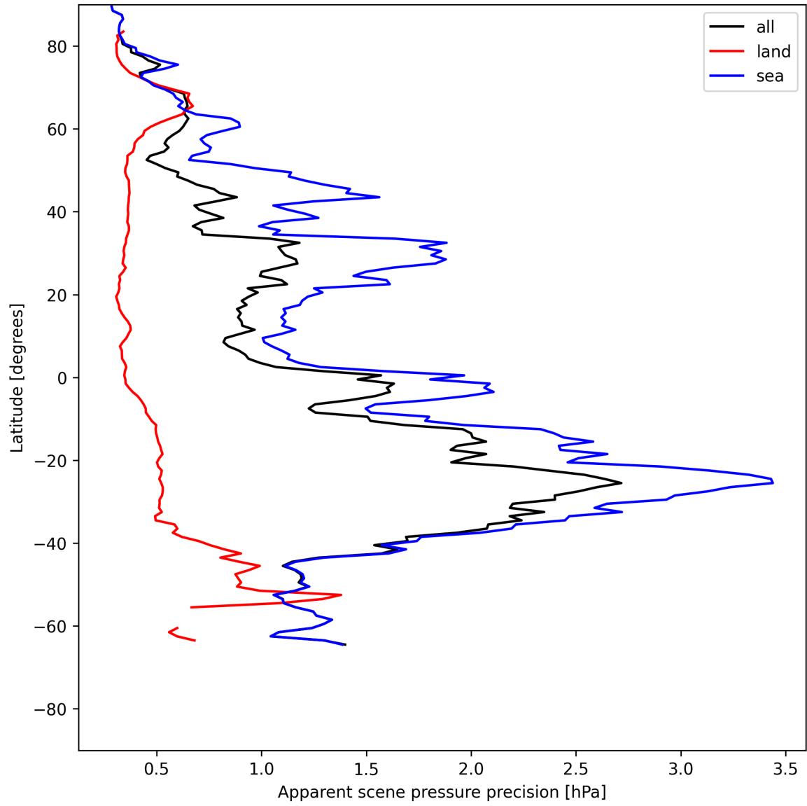
Figure 18: Zonal average of “Apparent scene pressure precision” for 2025-06-17 to 2025-06-17.
