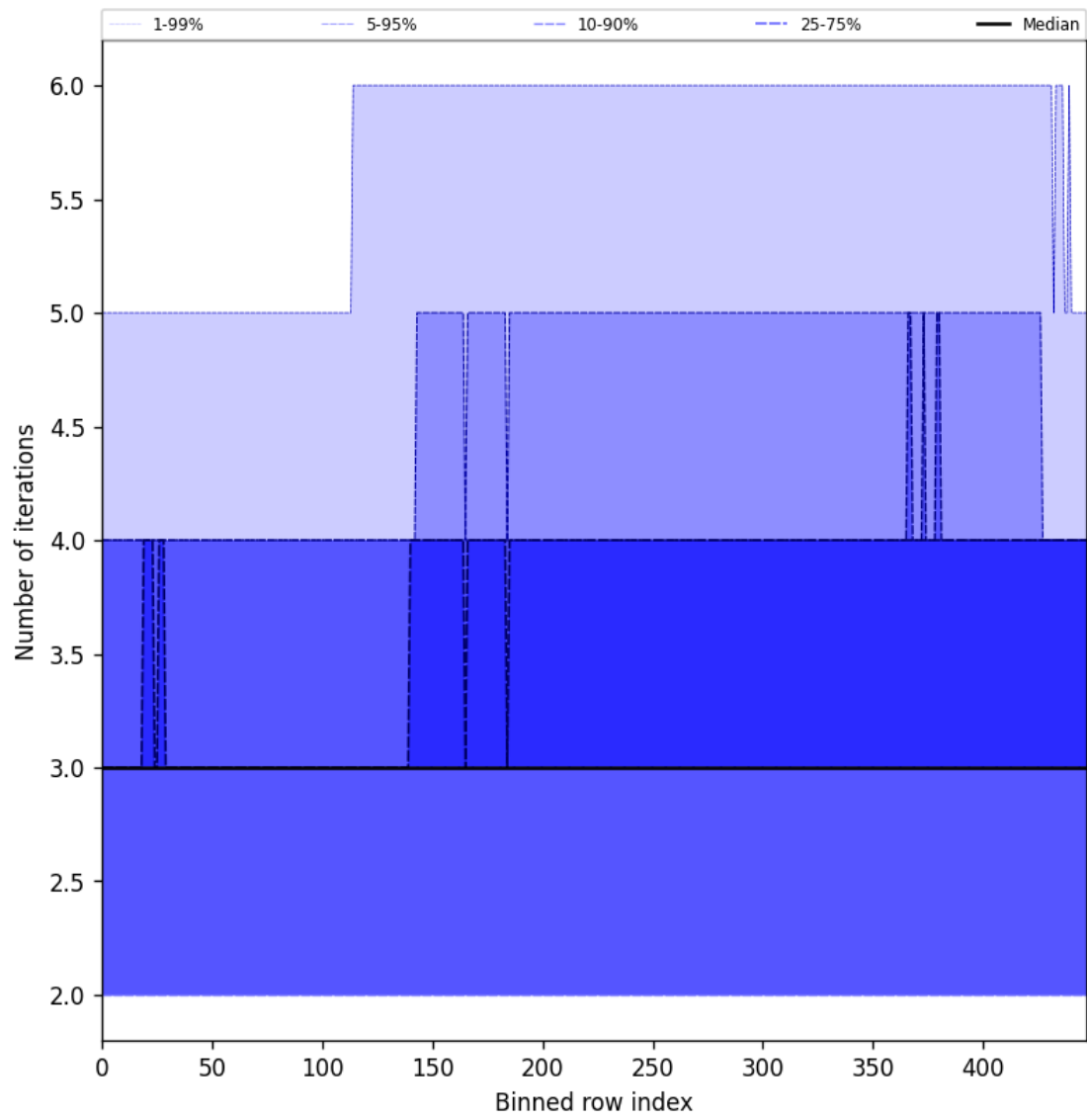
Figure 54: Along track statistics of “Number of iterations” for 2025-06-17 to 2025-06-17
