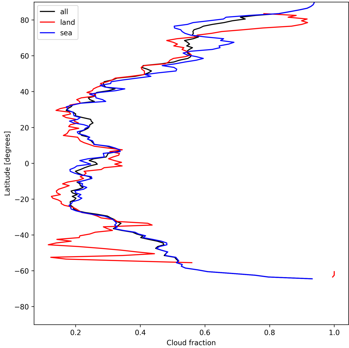
Figure 13: Zonal average of “Cloud fraction” for 2025-06-17 to 2025-06-17.
