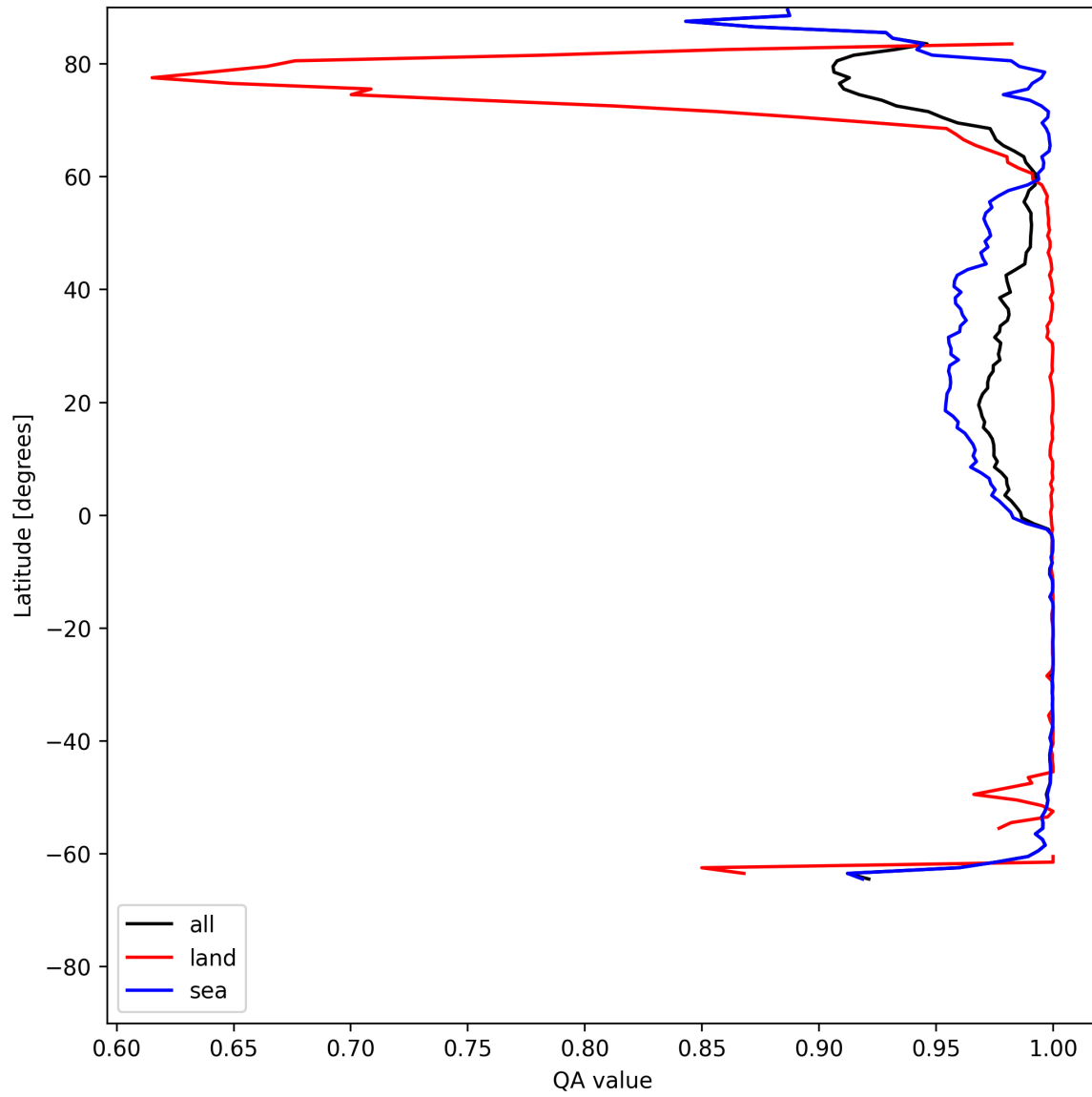
Figure 10: Zonal average of “QA value” for 2025-06-17 to 2025-06-17.
