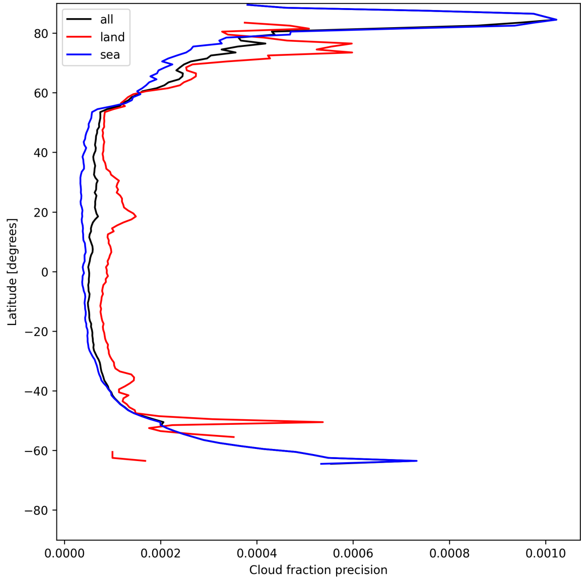
Figure 14: Zonal average of “Cloud fraction precision” for 2025-06-17 to 2025-06-17.
