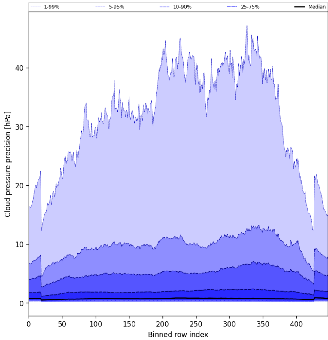
Figure 46: Along track statistics of “Cloud pressure precision” for 2025-06-17 to 2025-06-17
