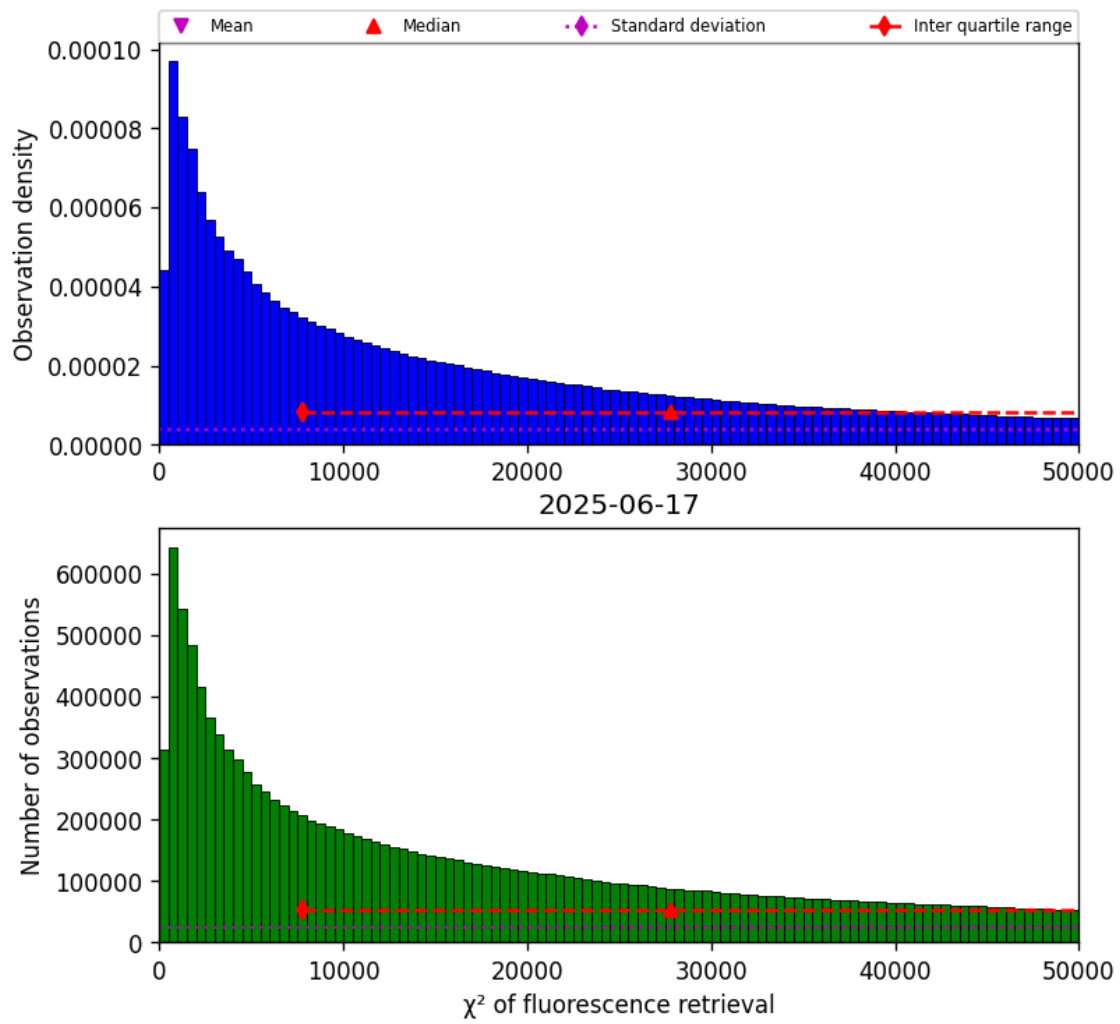
Figure 40: Histogram of " \chi^2 of fluorescence retrieval" for 2025-06-17 to 2025-06-17
