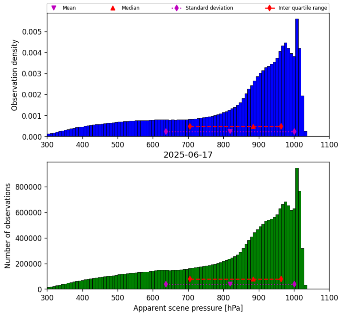
Figure 34: Histogram of "Apparent scene pressure" for 2025-06-17 to 2025-06-17
