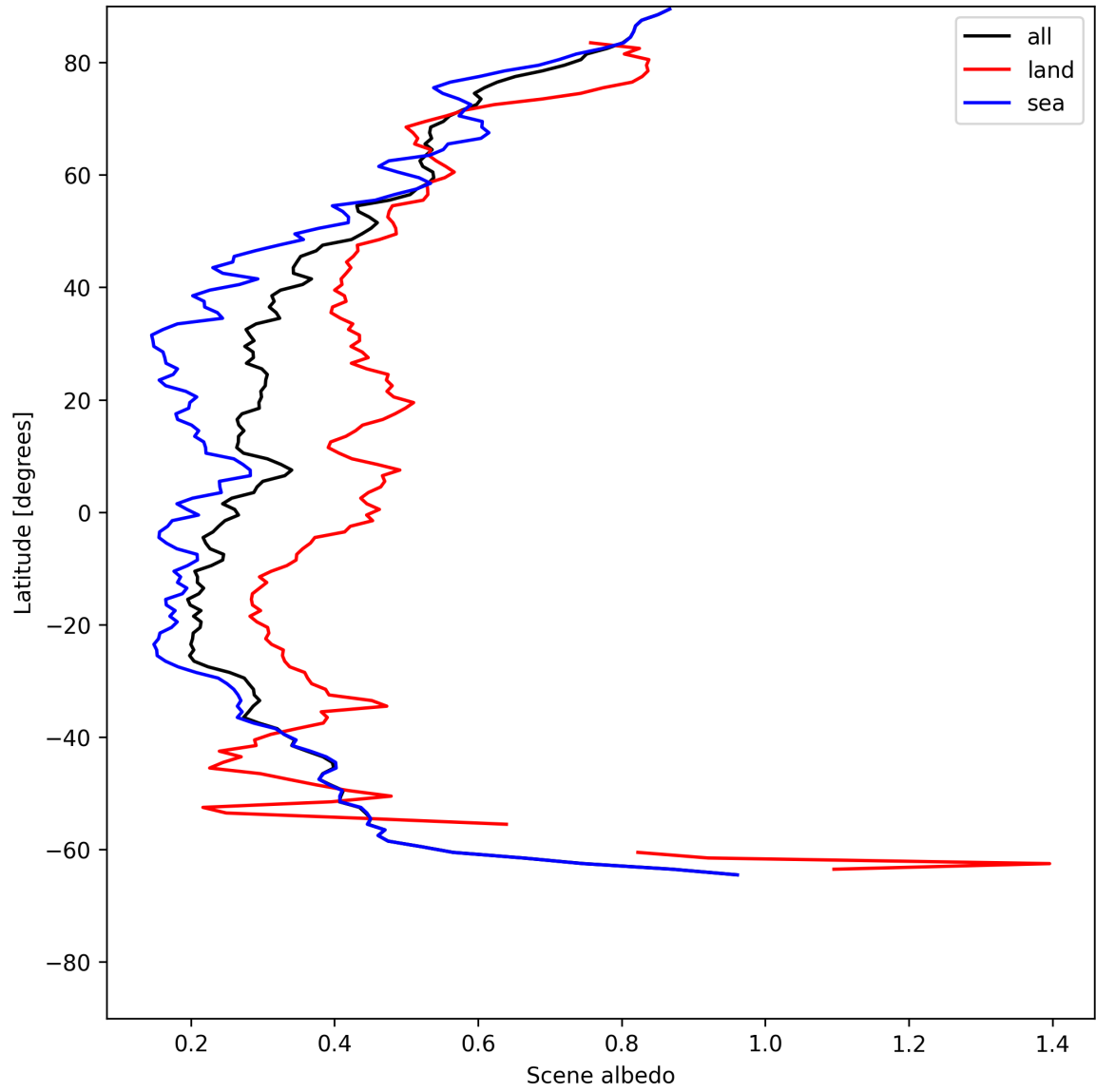
Figure 15: Zonal average of “Scene albedo” for 2025-06-17 to 2025-06-17.
