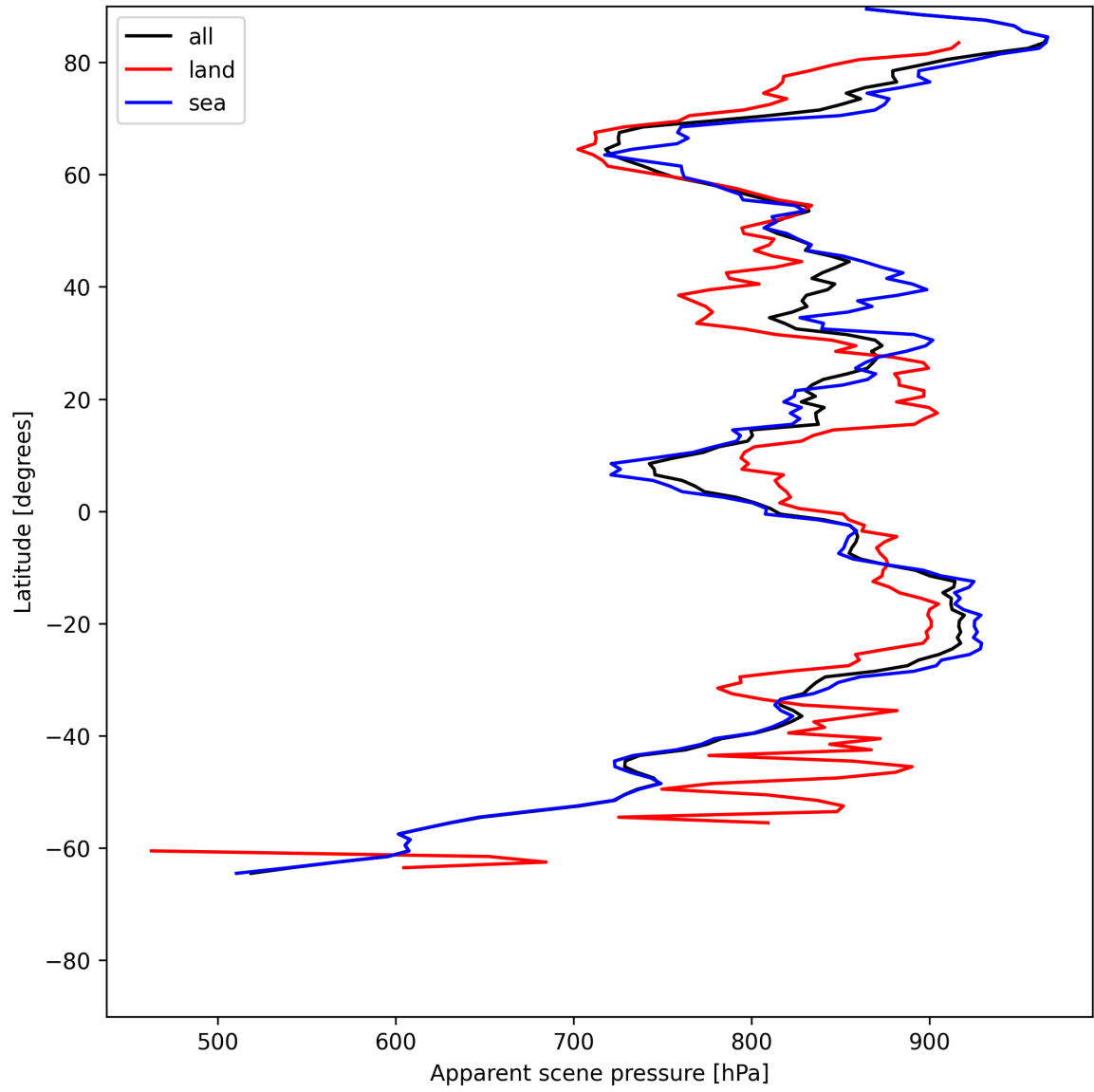
Figure 17: Zonal average of “Apparent scene pressure” for 2025-06-17 to 2025-06-17.
