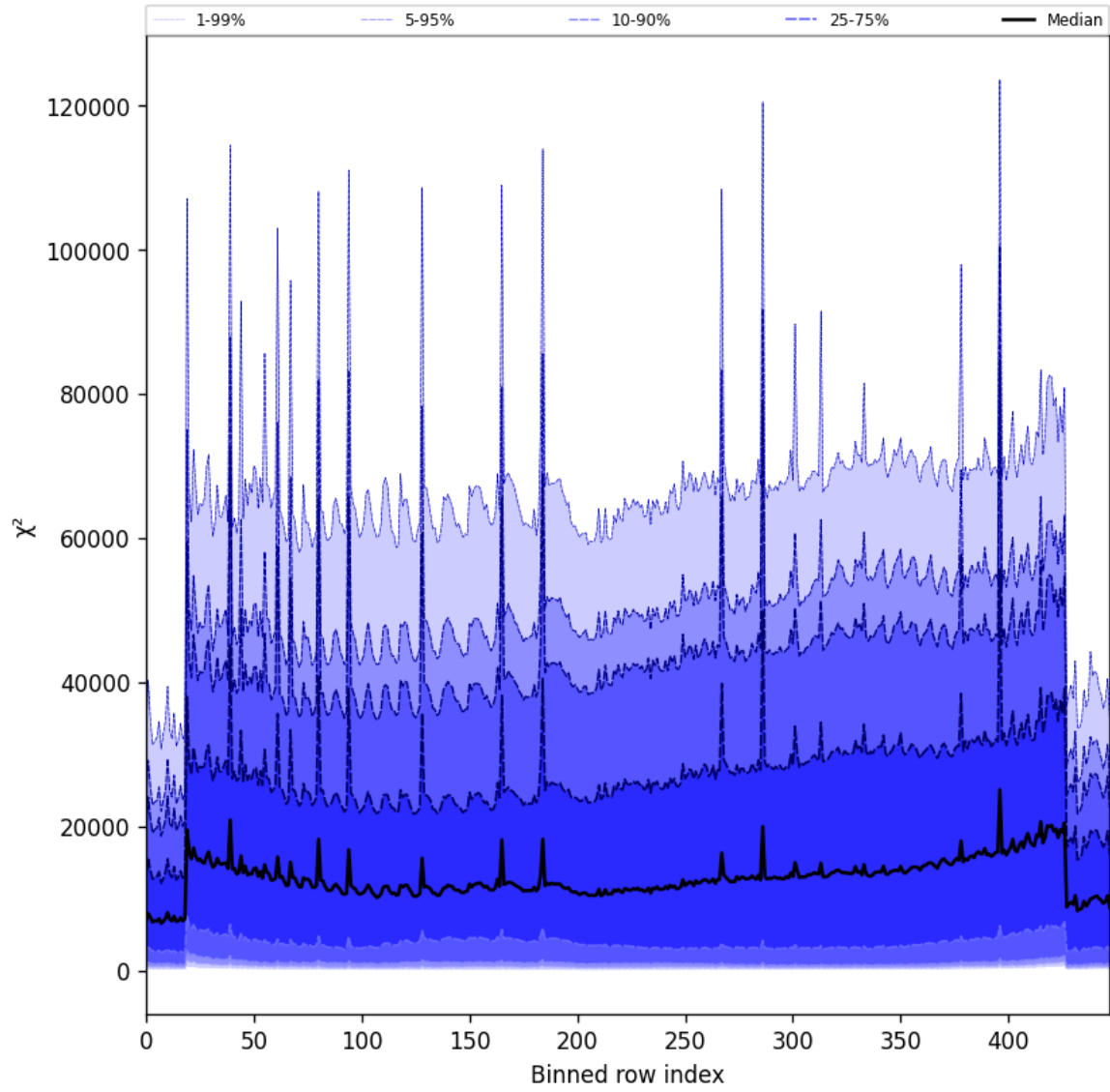
Figure 53: Along track statistics of “ \chi^2 ” for 2025-06-17 to 2025-06-17
