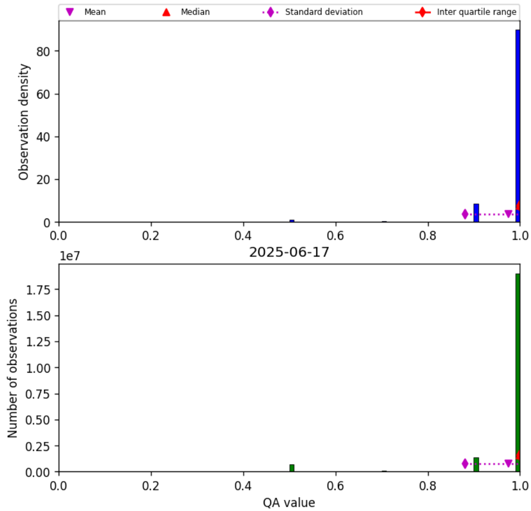
Figure 27: Histogram of “QA value” for 2025-06-17 to 2025-06-17
