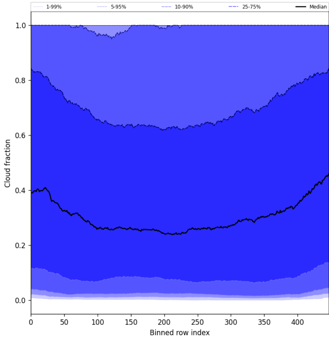
Figure 47: Along track statistics of “Cloud fraction” for 2025-06-17 to 2025-06-17
