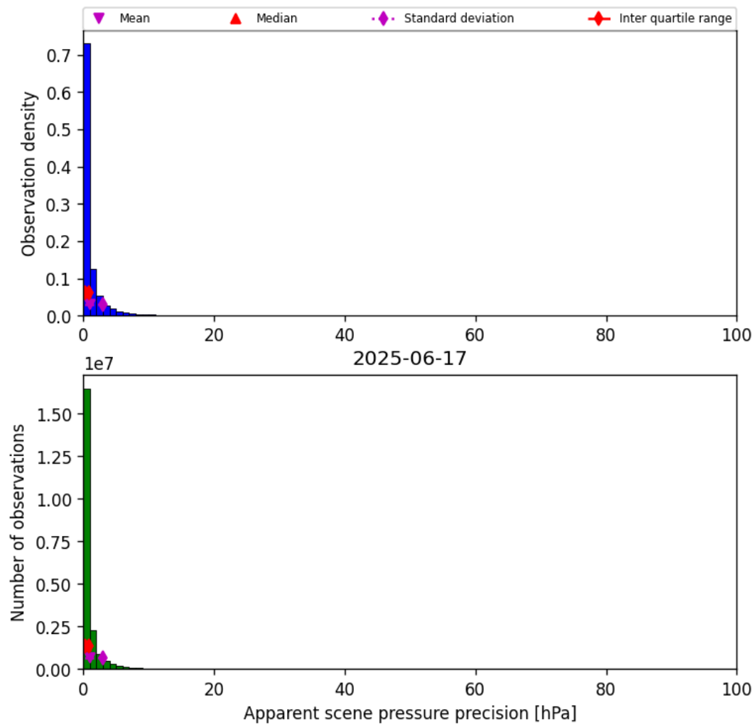
Figure 35: Histogram of “Apparent scene pressure precision” for 2025-06-17 to 2025-06-17
