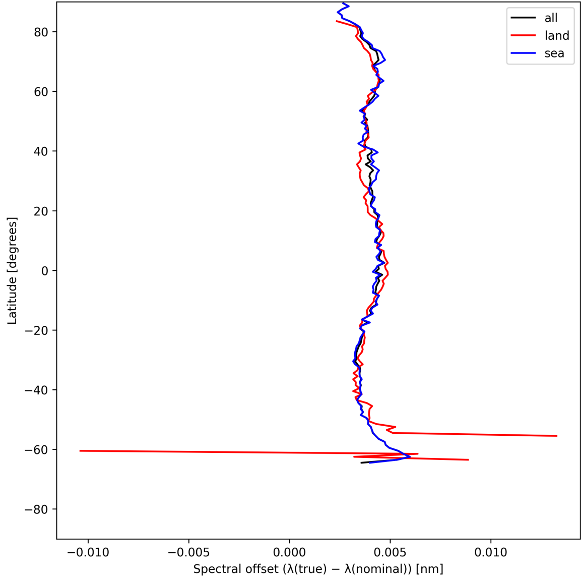
Figure 26: Zonal average of “Spectral offset ( \lambda_{\text{true}} - \lambda_{\text{nominal}} )” for 2025-06-17 to 2025-06-17.
