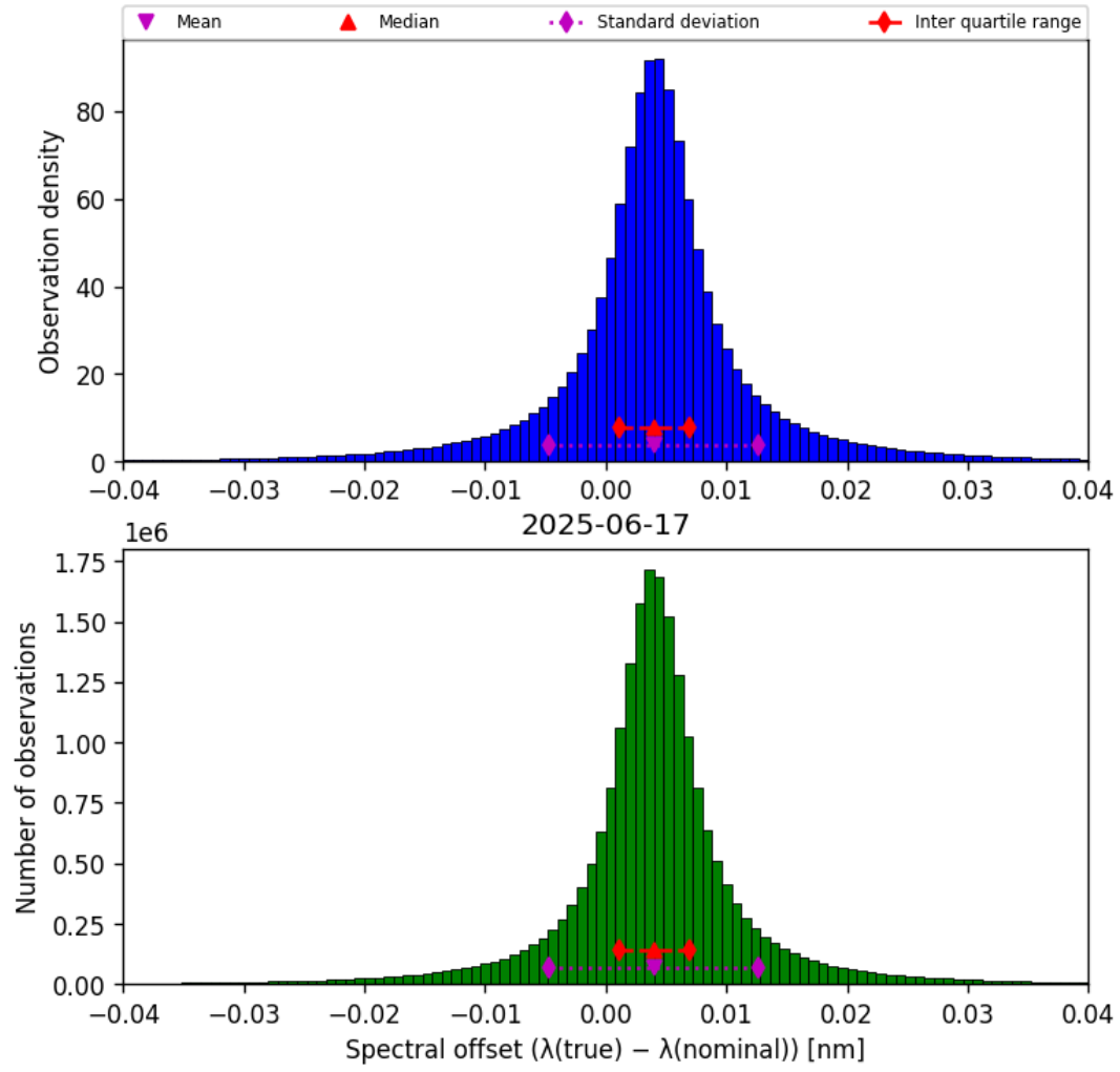
Figure 43: Histogram of “Spectral offset ( \lambda_{\text{true}} - \lambda_{\text{nominal}} )” for 2025-06-17 to 2025-06-17
