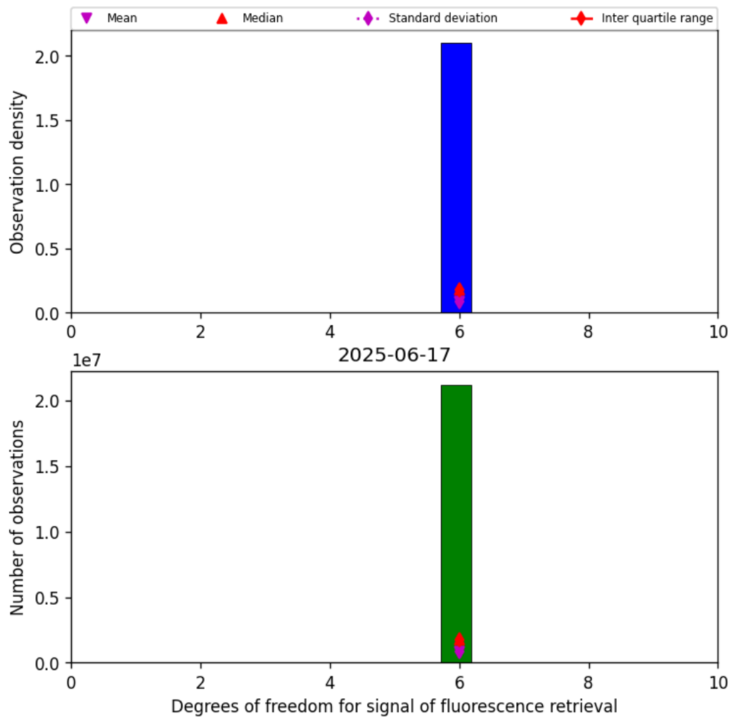
Figure 41: Histogram of “Degrees of freedom for signal of fluorescence retrieval” for 2025-06-17 to 2025-06-17
