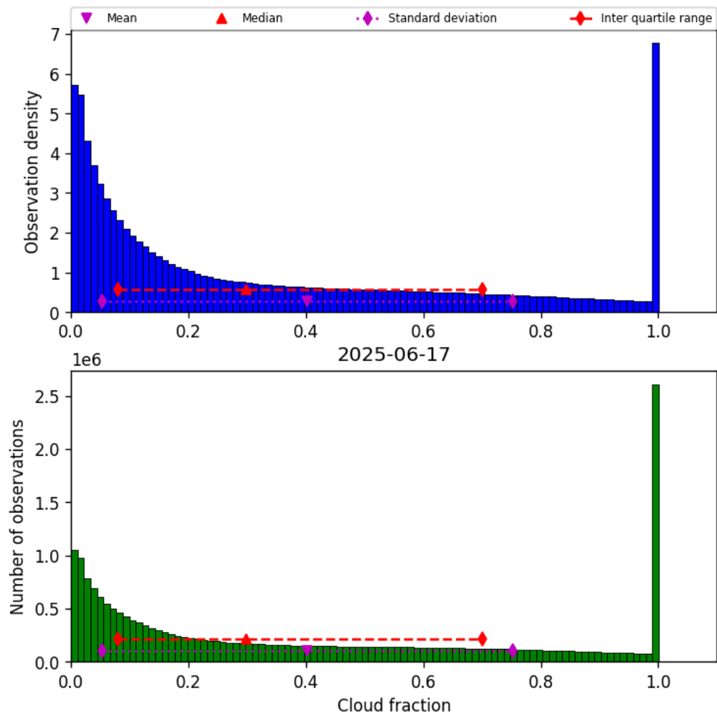
Figure 30: Histogram of “Cloud fraction” for 2025-06-17 to 2025-06-17
