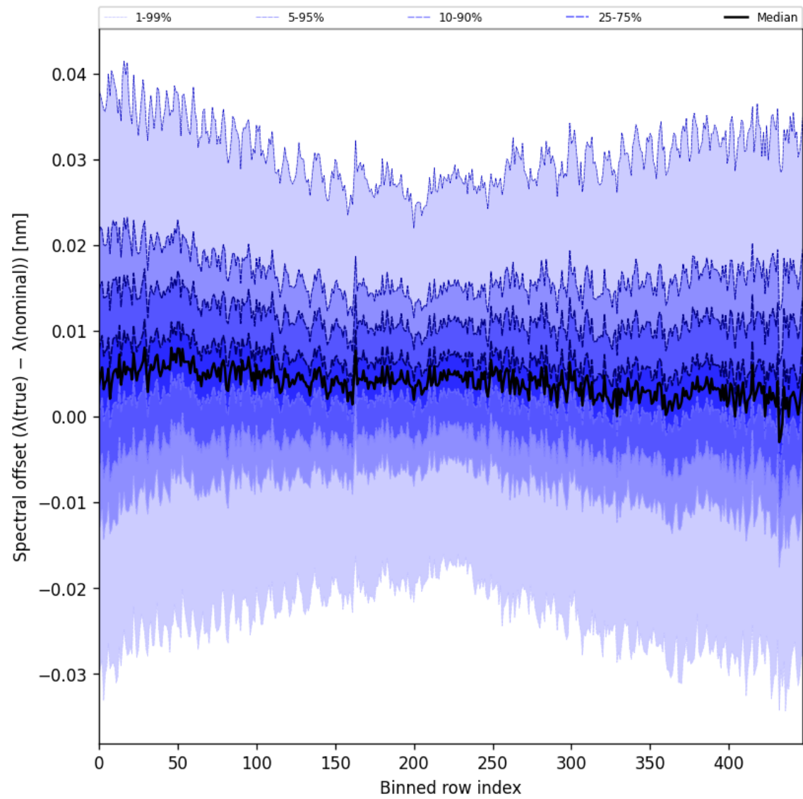
Figure 60: Along track statistics of “Spectral offset ( \lambda_{\text{true}} - \lambda_{\text{nominal}} )” for 2025-06-17 to 2025-06-17
