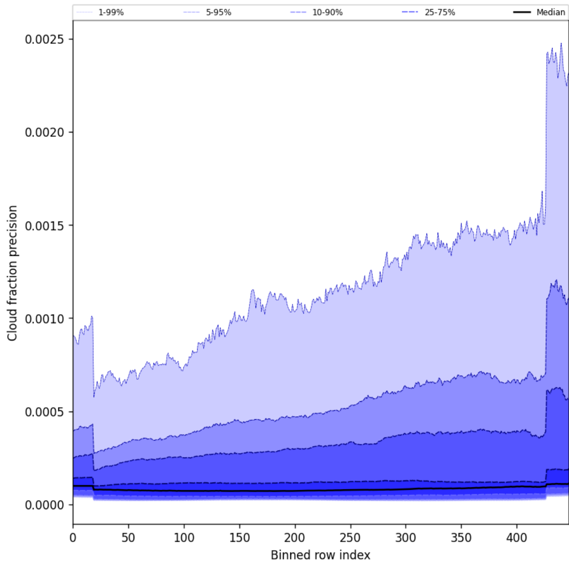
Figure 48: Along track statistics of “Cloud fraction precision” for 2025-06-17 to 2025-06-17
