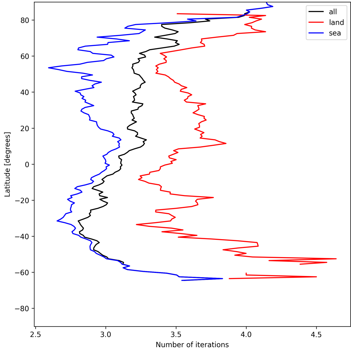
Figure 20: Zonal average of “Number of iterations” for 2025-06-17 to 2025-06-17.
