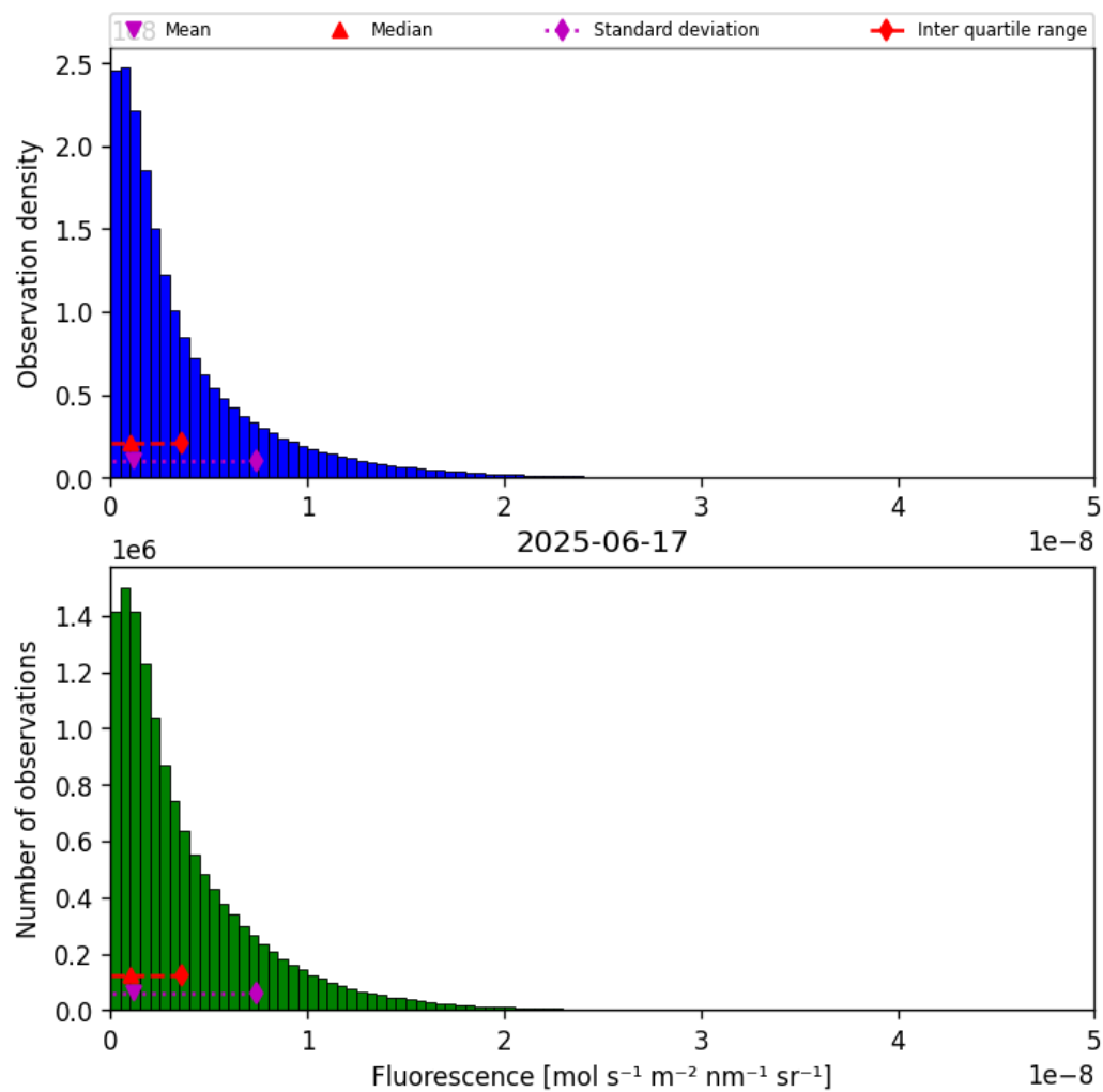
Figure 38: Histogram of “Fluorescence” for 2025-06-17 to 2025-06-17
