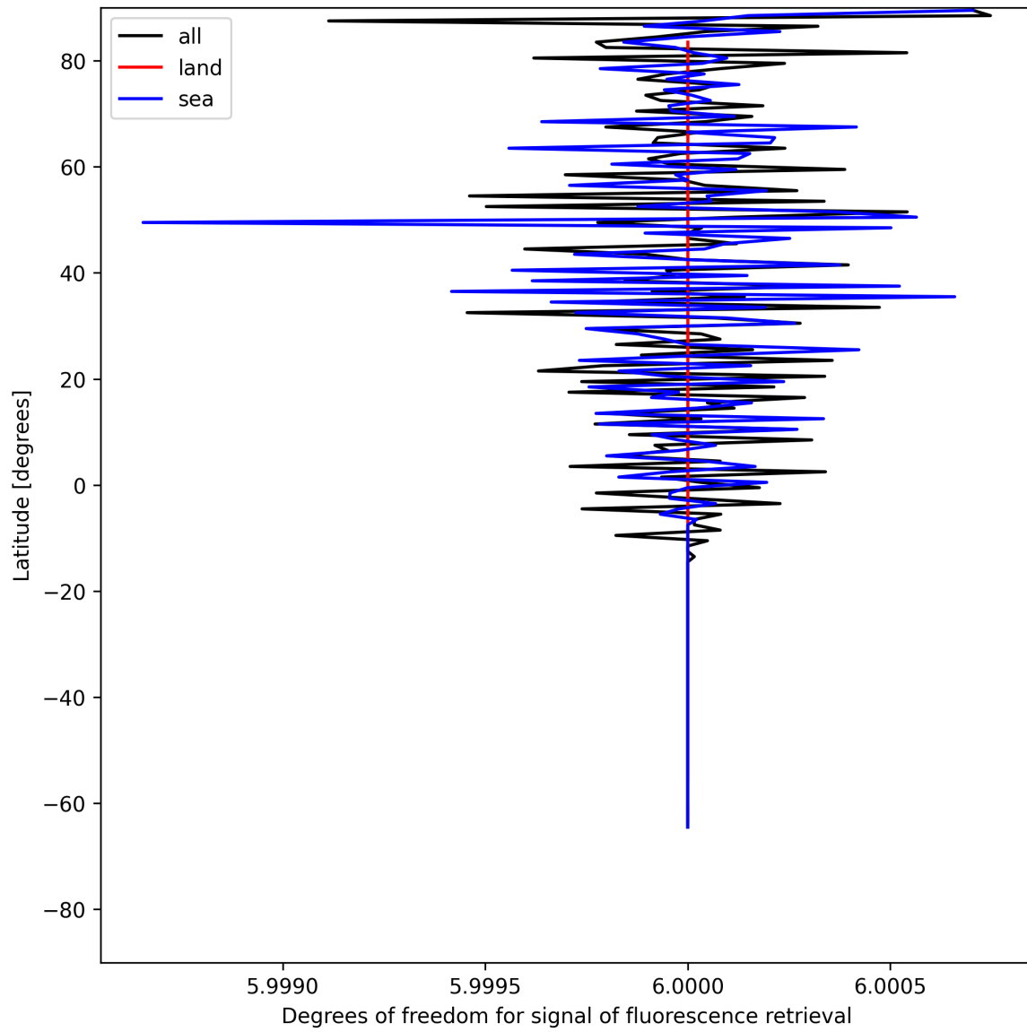
Figure 24: Zonal average of “Degrees of freedom for signal of fluorescence retrieval” for 2025-06-17 to 2025-06-17.
