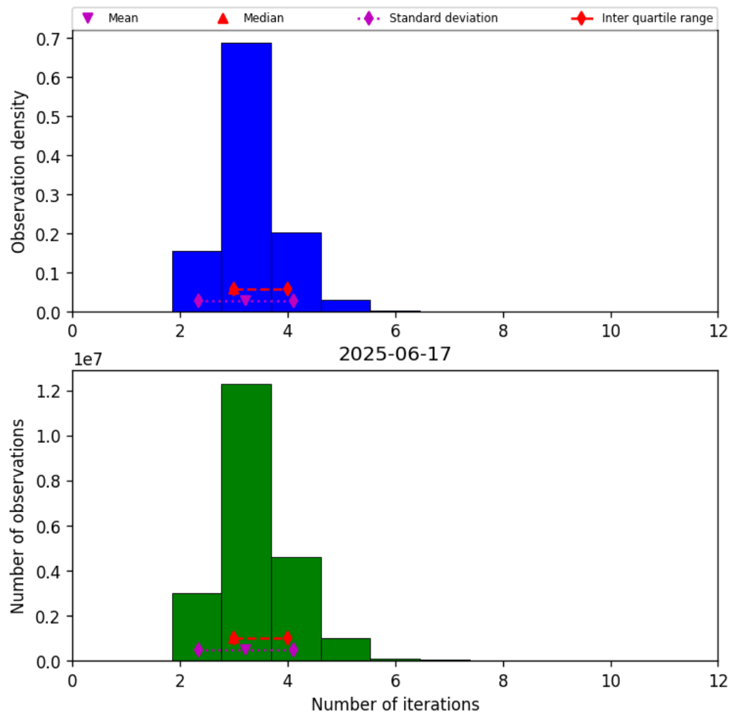
Figure 37: Histogram of “Number of iterations” for 2025-06-17 to 2025-06-17
