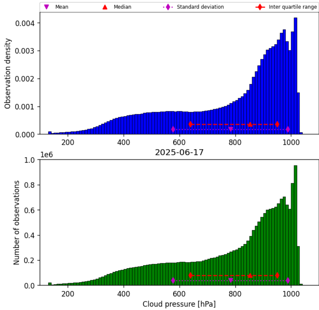
Figure 28: Histogram of “Cloud pressure” for 2025-06-17 to 2025-06-17
