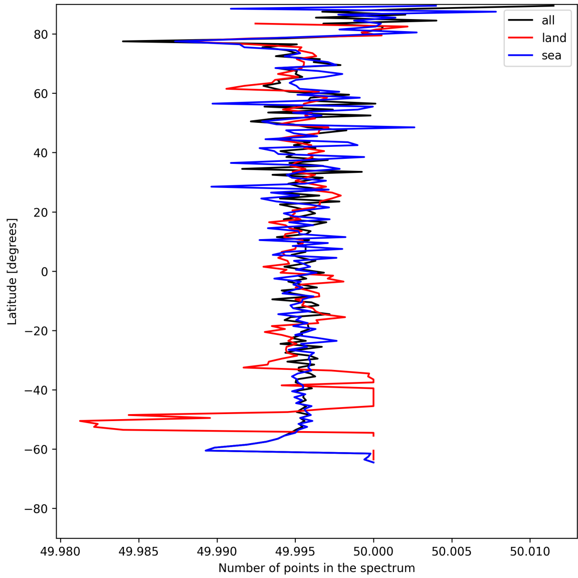
Figure 25: Zonal average of “Number of points in the spectrum” for 2025-06-17 to 2025-06-17.
