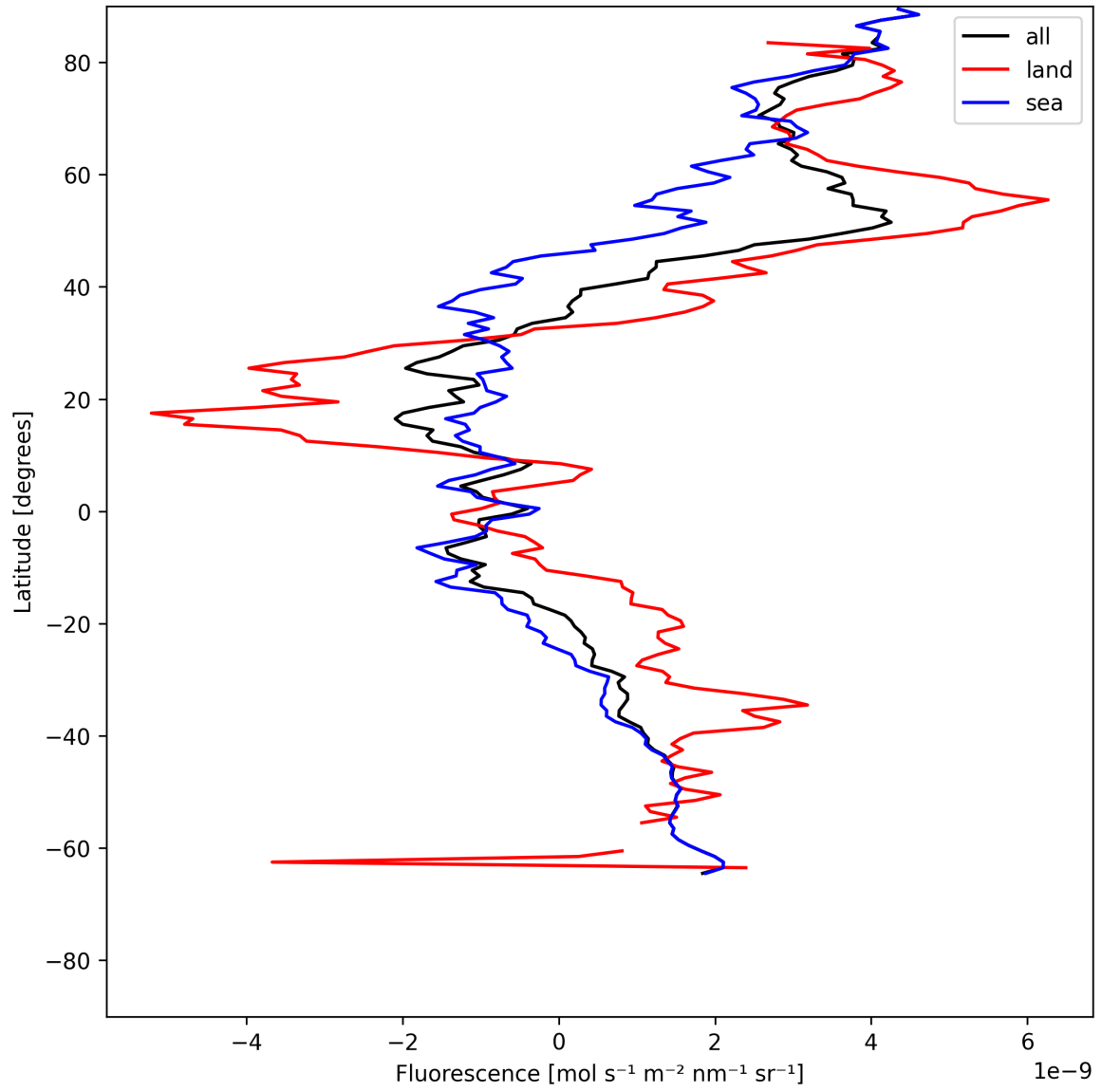
Figure 21: Zonal average of “Fluorescence” for 2025-06-17 to 2025-06-17.
