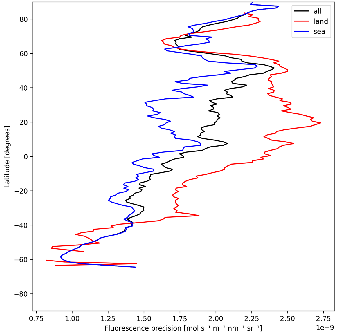
Figure 22: Zonal average of “Fluorescence precision” for 2025-06-17 to 2025-06-17.
