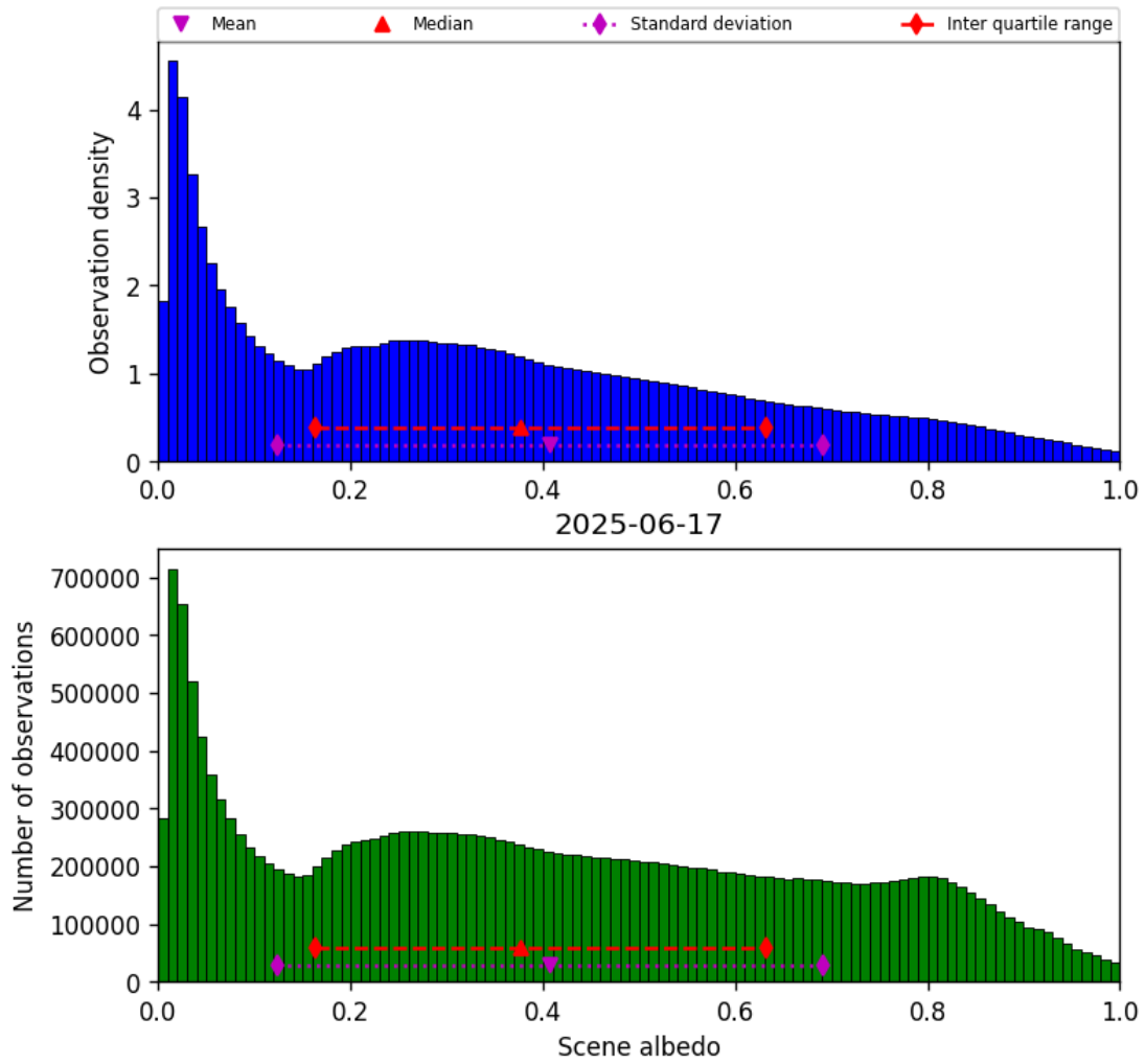
Figure 32: Histogram of “Scene albedo” for 2025-06-17 to 2025-06-17
