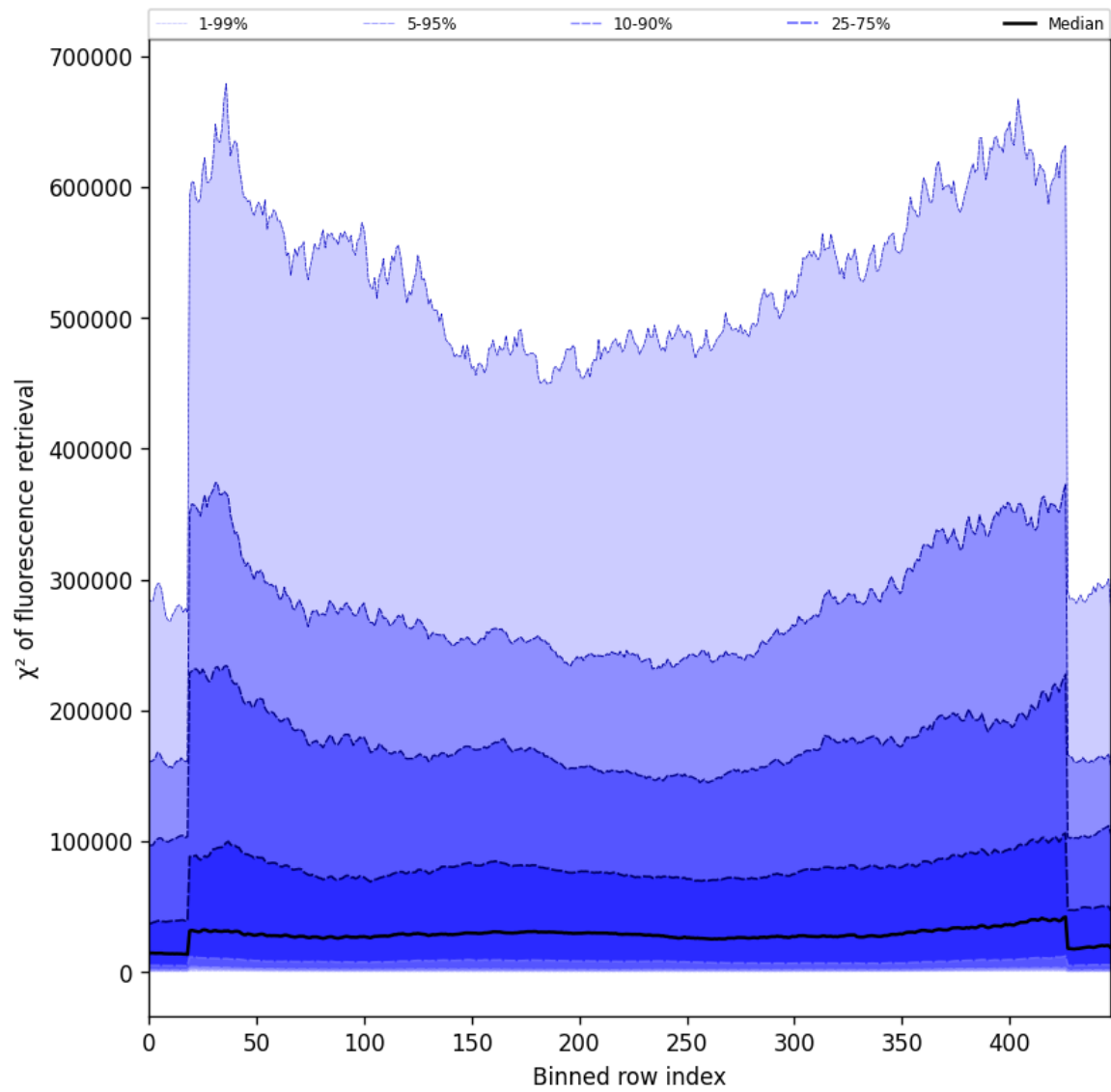
Figure 57: Along track statistics of “ \chi^2 of fluorescence retrieval” for 2025-06-17 to 2025-06-17
