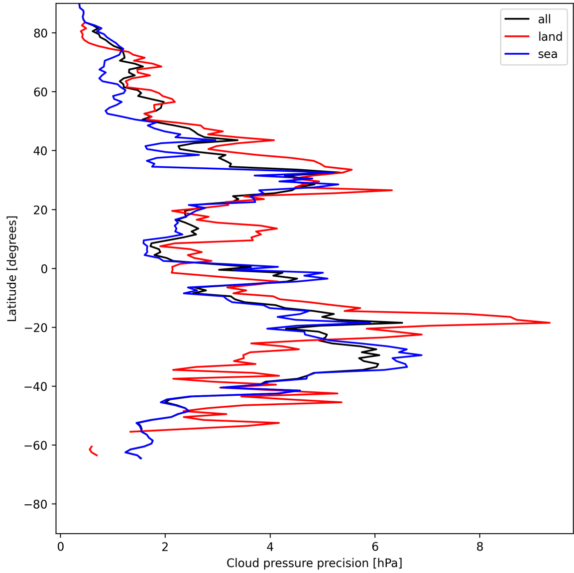
Figure 12: Zonal average of “Cloud pressure precision” for 2025-06-17 to 2025-06-17.
