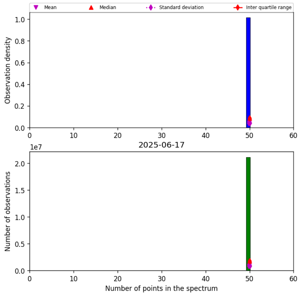
Figure 42: Histogram of “Number of points in the spectrum” for 2025-06-17 to 2025-06-17
