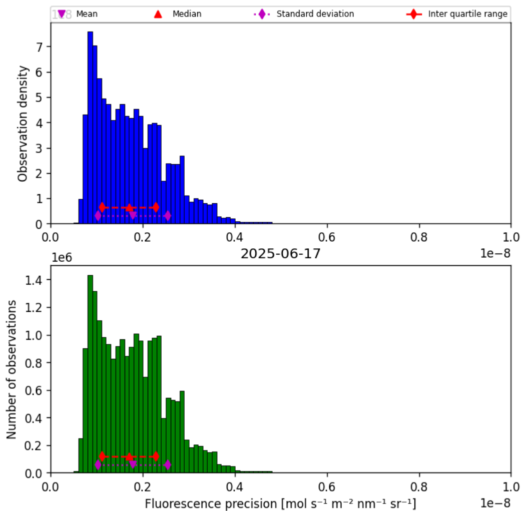
Figure 39: Histogram of “Fluorescence precision” for 2025-06-17 to 2025-06-17
