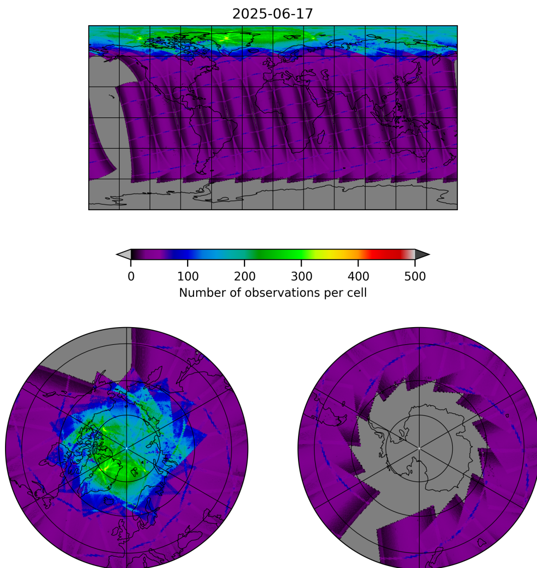
Figure 9: Map of the number of observations for 2025-06-17 to 2025-06-17
