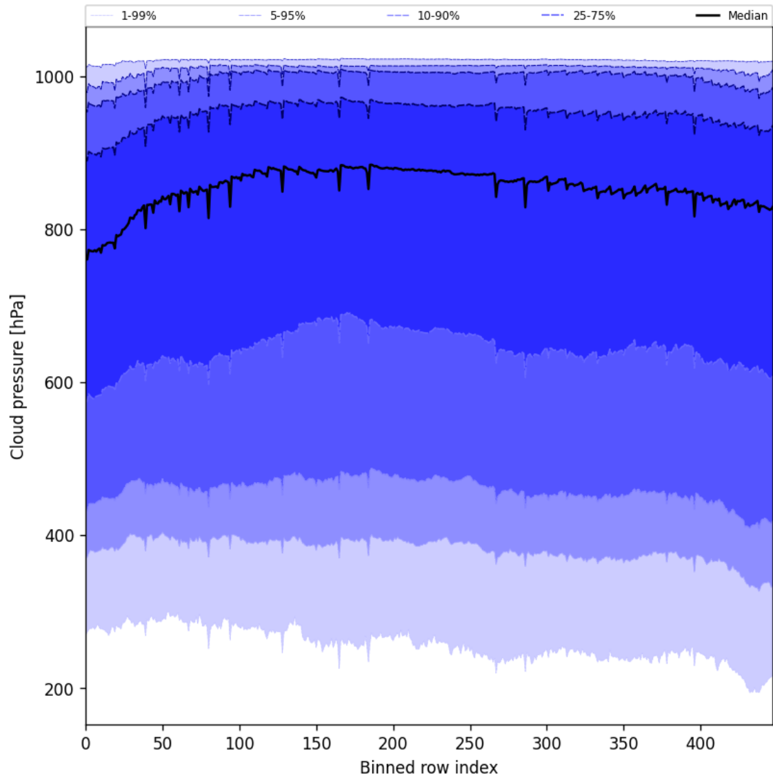
Figure 45: Along track statistics of “Cloud pressure” for 2025-06-17 to 2025-06-17
