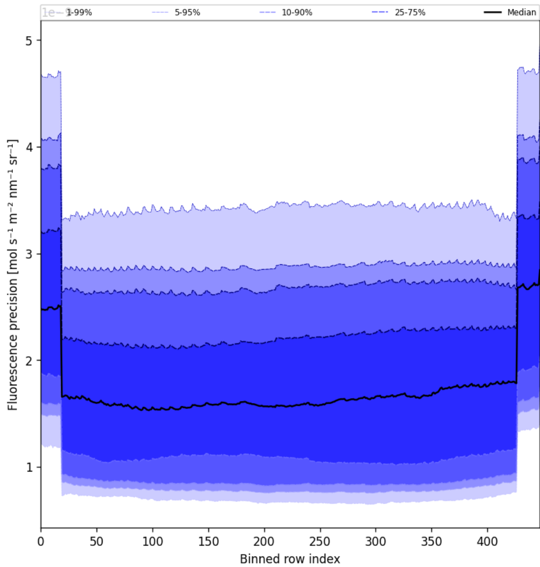
Figure 56: Along track statistics of “Fluorescence precision” for 2025-06-17 to 2025-06-17
