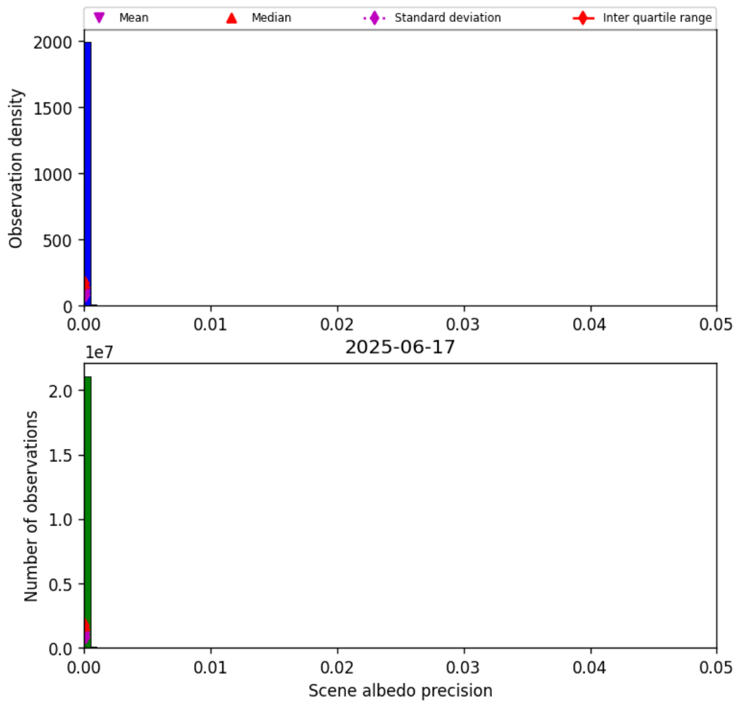
Figure 33: Histogram of “Scene albedo precision” for 2025-06-17 to 2025-06-17
