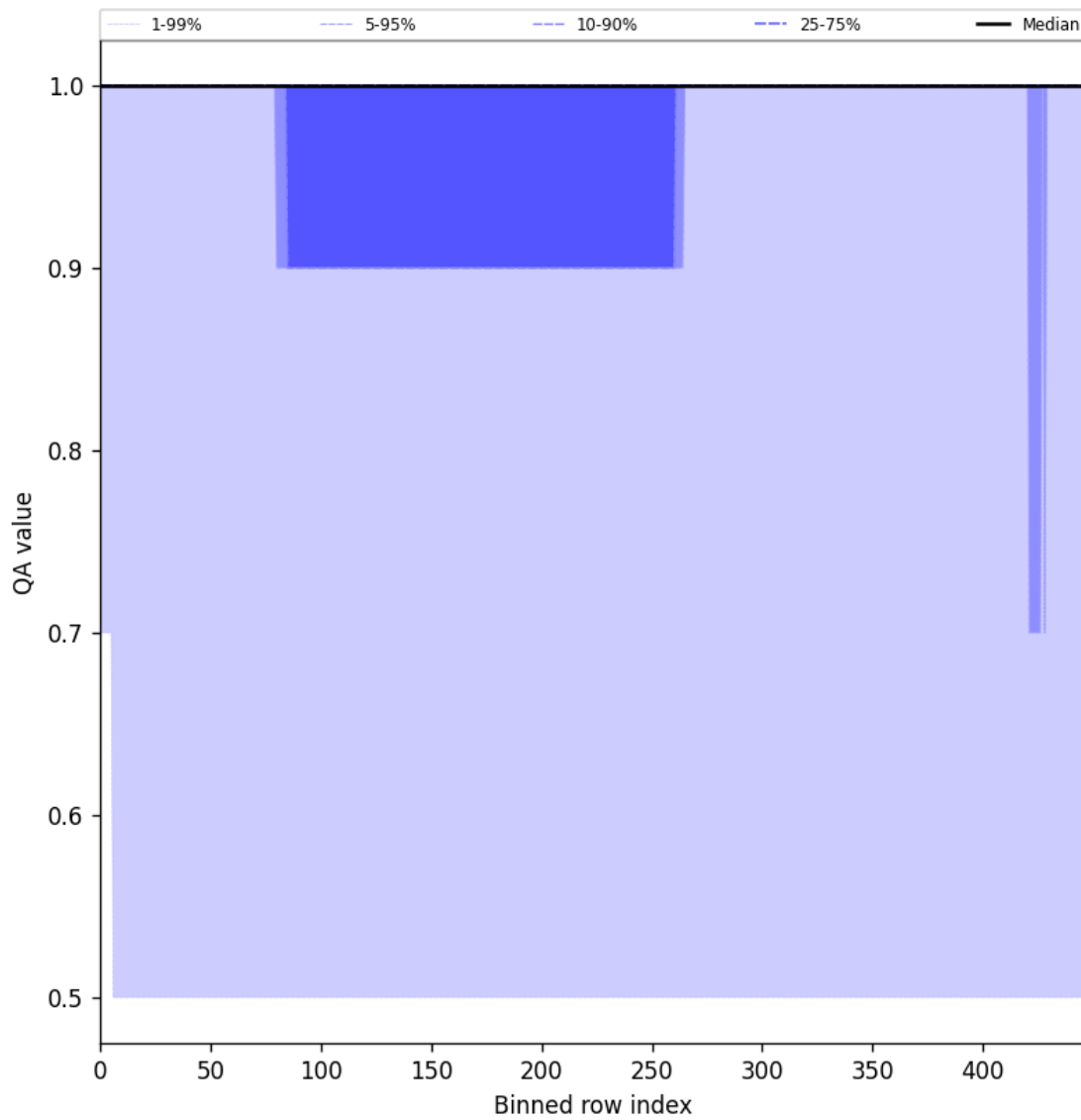
Figure 44: Along track statistics of “QA value” for 2025-06-17 to 2025-06-17
