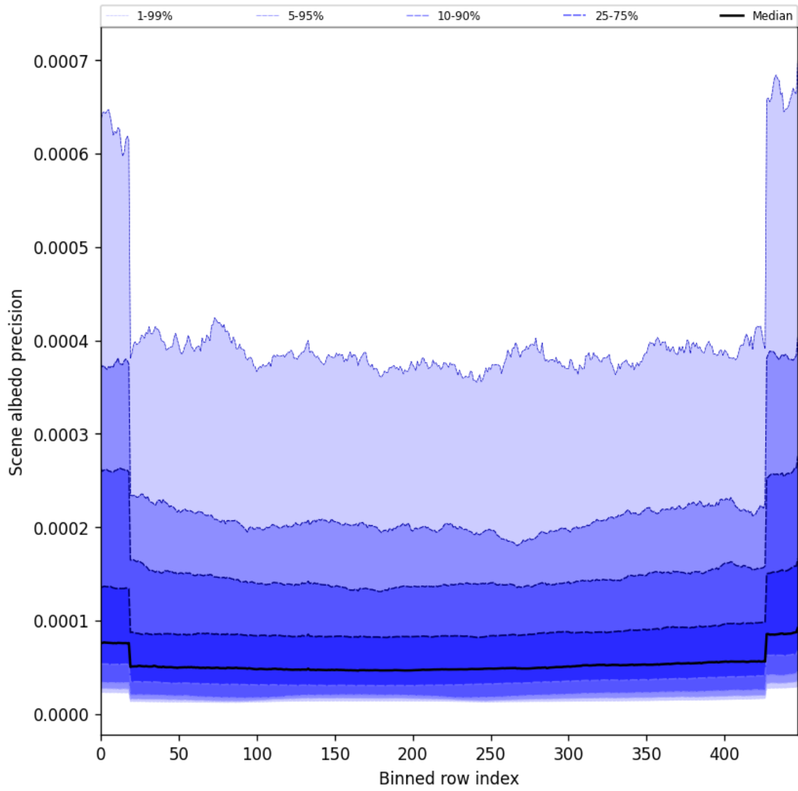
Figure 50: Along track statistics of “Scene albedo precision” for 2025-06-17 to 2025-06-17
