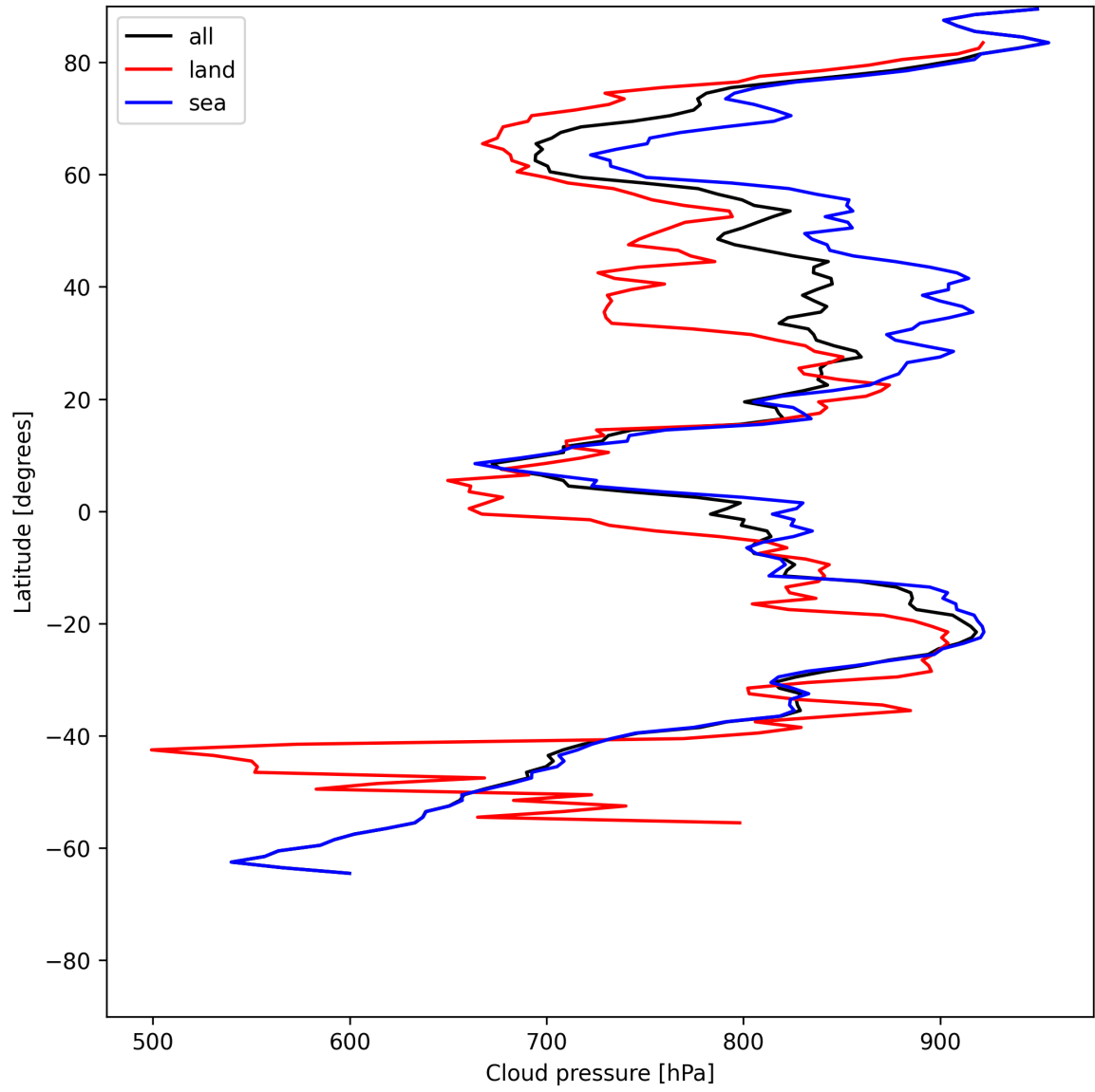
Figure 11: Zonal average of “Cloud pressure” for 2025-06-19 to 2025-06-20.
