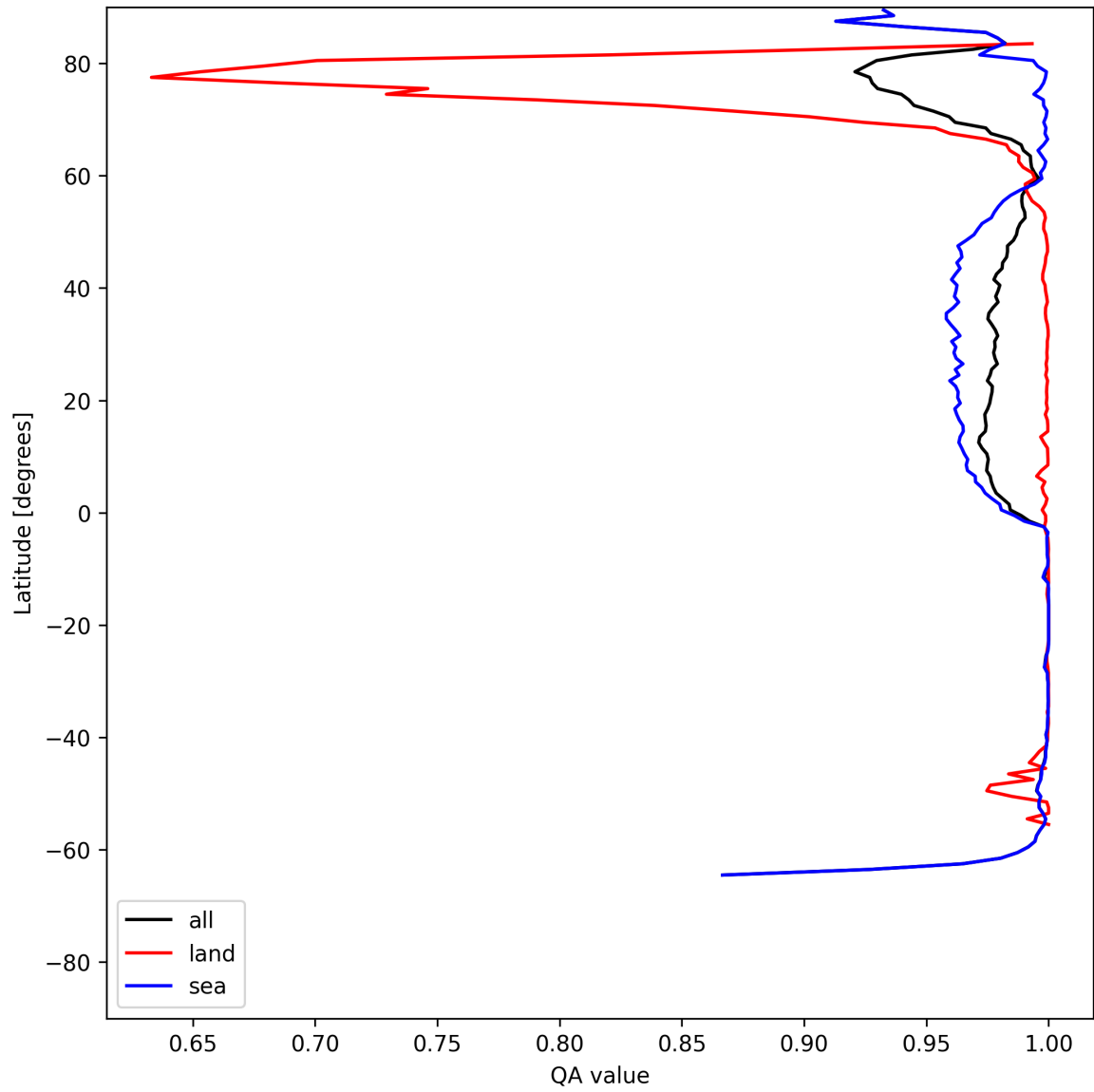
Figure 10: Zonal average of “QA value” for 2025-06-19 to 2025-06-20.
