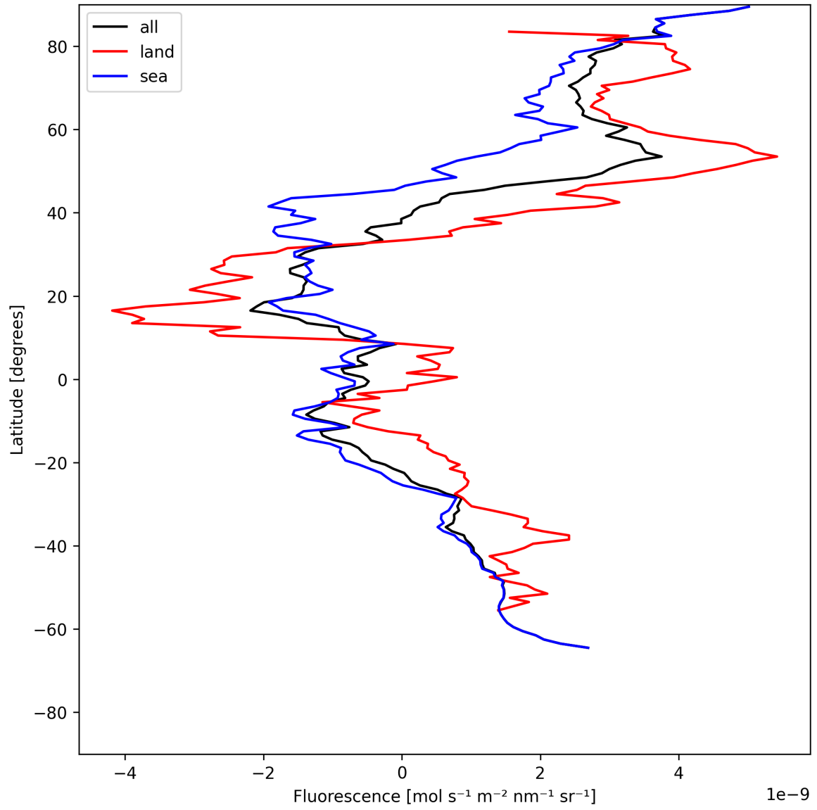
Figure 21: Zonal average of “Fluorescence” for 2025-06-19 to 2025-06-20.
