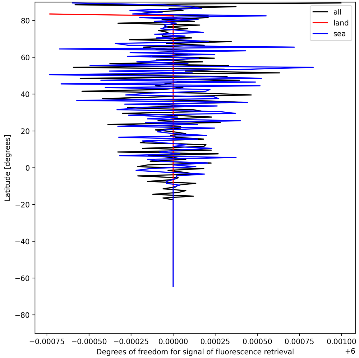
Figure 24: Zonal average of "Degrees of freedom for signal of fluorescence retrieval" for 2025-06-19 to 2025-06-20.
