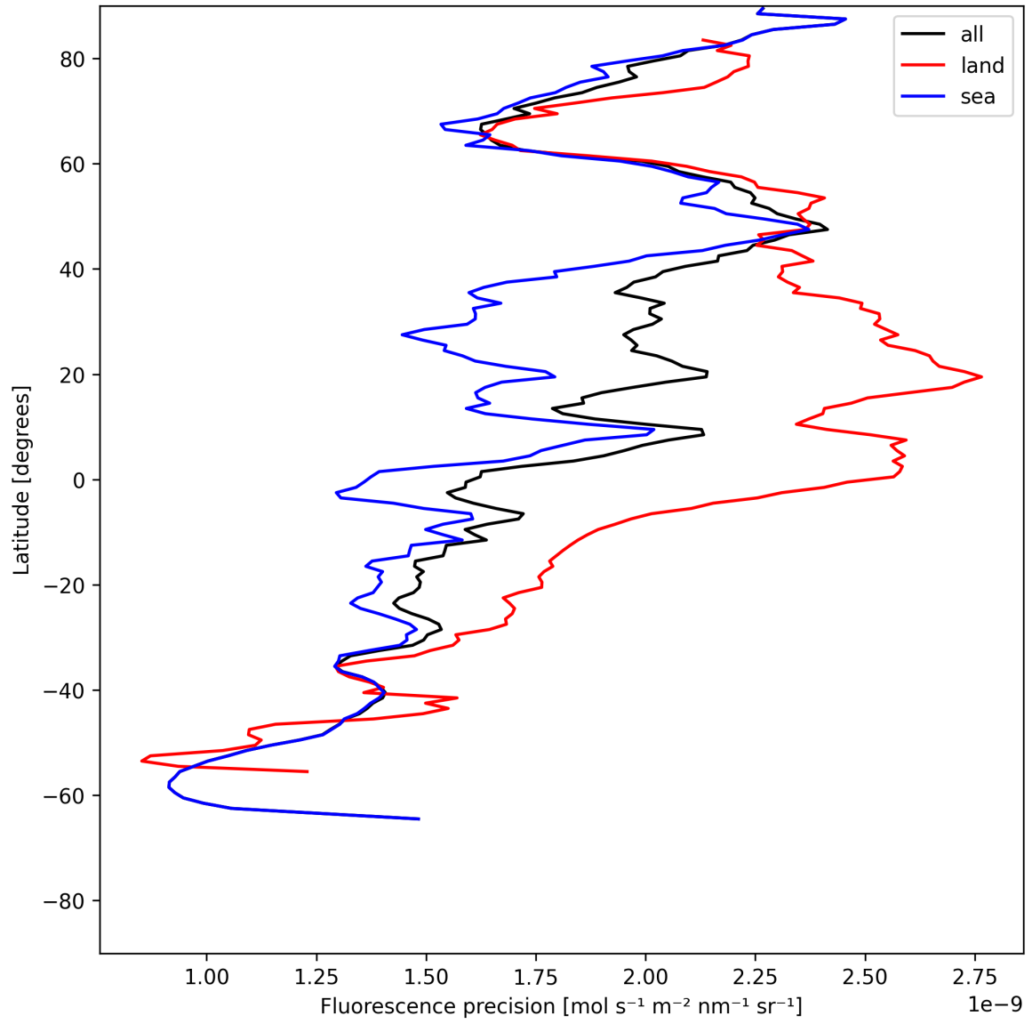
Figure 22: Zonal average of “Fluorescence precision” for 2025-06-19 to 2025-06-20.
