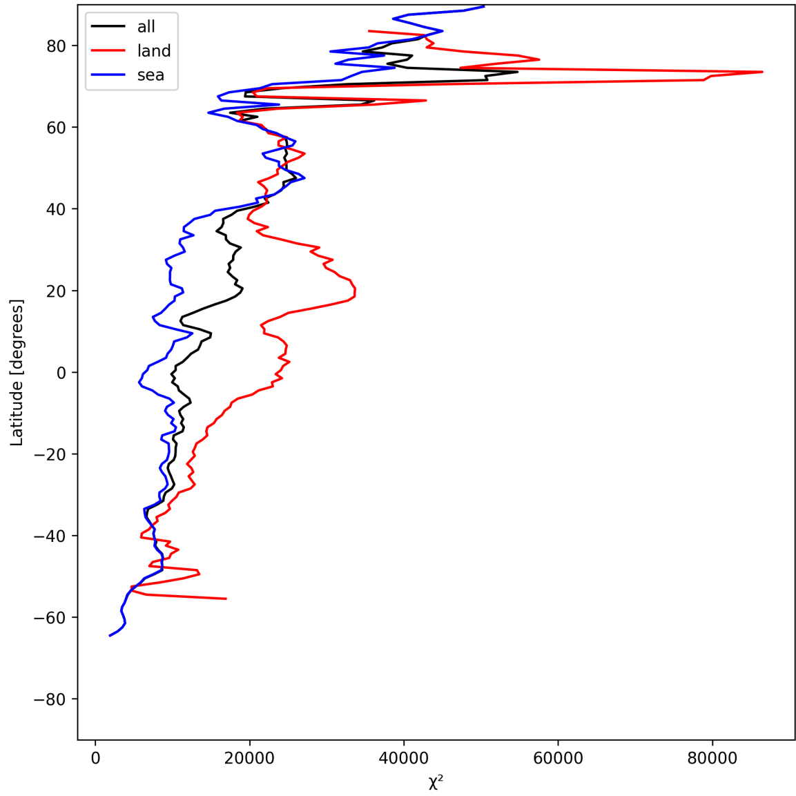
Figure 19: Zonal average of “ \chi^2 ” for 2025-06-19 to 2025-06-20.
