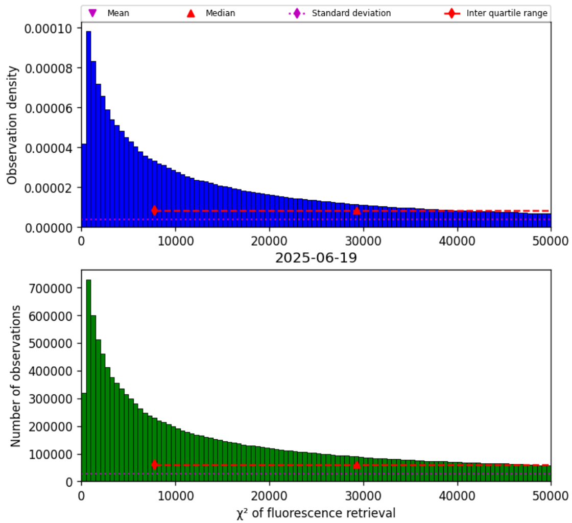
Figure 40: Histogram of “ \chi^2 of fluorescence retrieval” for 2025-06-19 to 2025-06-20
