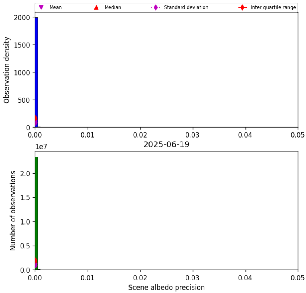
Figure 33: Histogram of “Scene albedo precision” for 2025-06-19 to 2025-06-20
