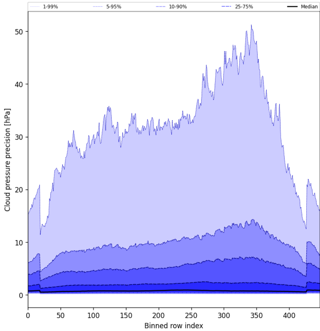
Figure 46: Along track statistics of “Cloud pressure precision” for 2025-06-19 to 2025-06-20
