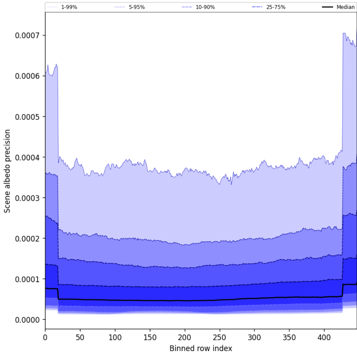
Figure 50: Along track statistics of “Scene albedo precision” for 2025-06-19 to 2025-06-20
