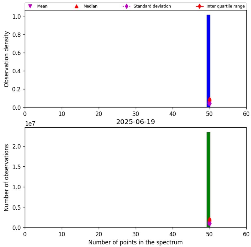
Figure 42: Histogram of “Number of points in the spectrum” for 2025-06-19 to 2025-06-20
