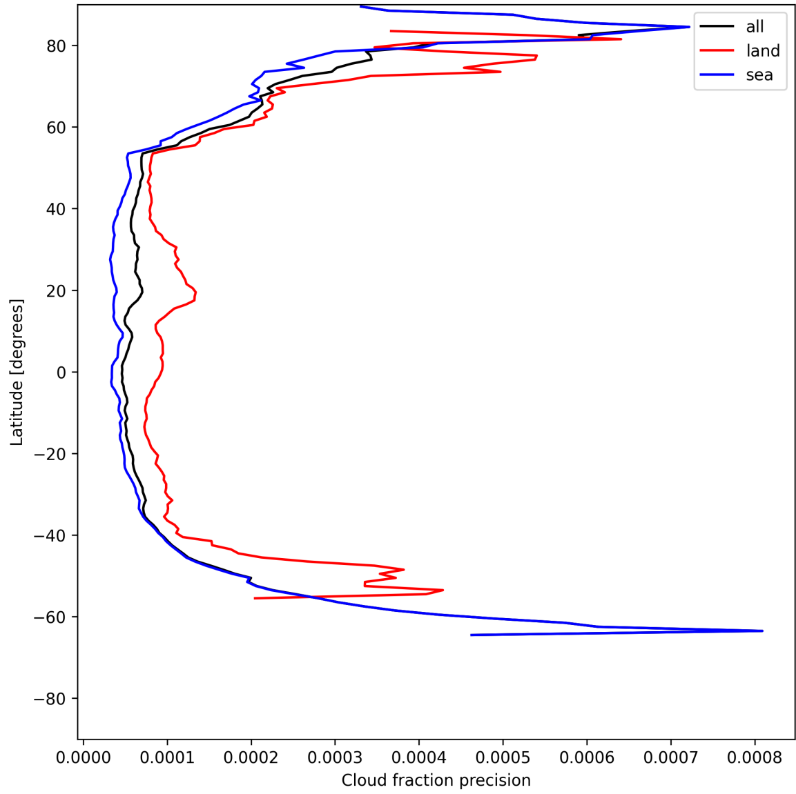
Figure 14: Zonal average of “Cloud fraction precision” for 2025-06-19 to 2025-06-20.
