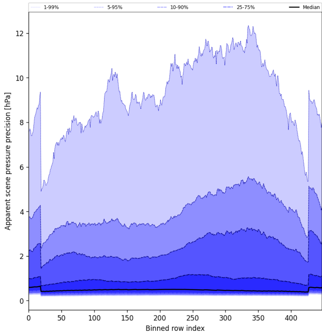
Figure 52: Along track statistics of “Apparent scene pressure precision” for 2025-06-19 to 2025-06-20
