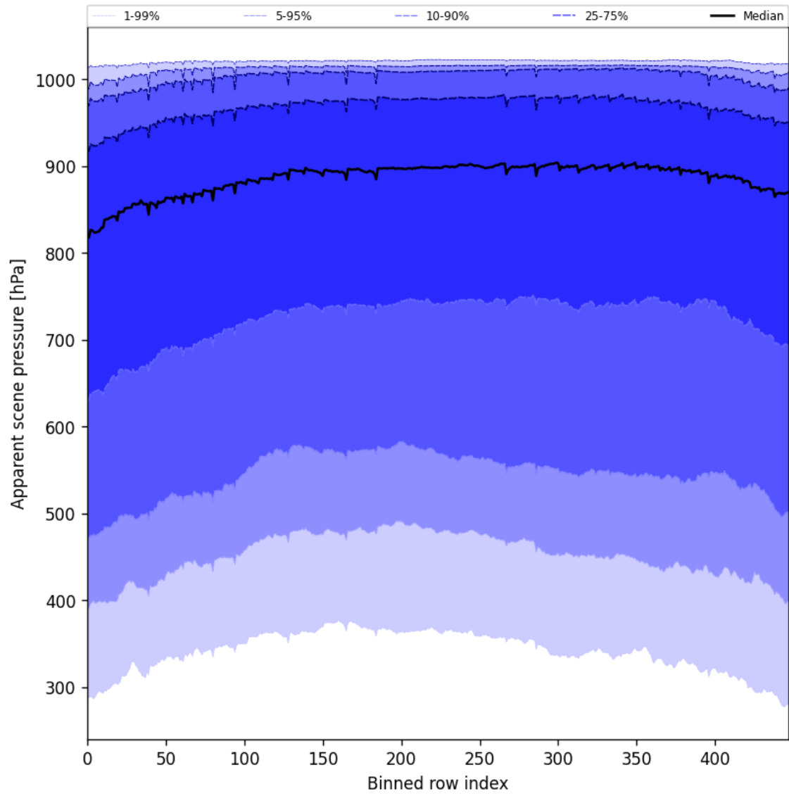
Figure 51: Along track statistics of “Apparent scene pressure” for 2025-06-19 to 2025-06-20
