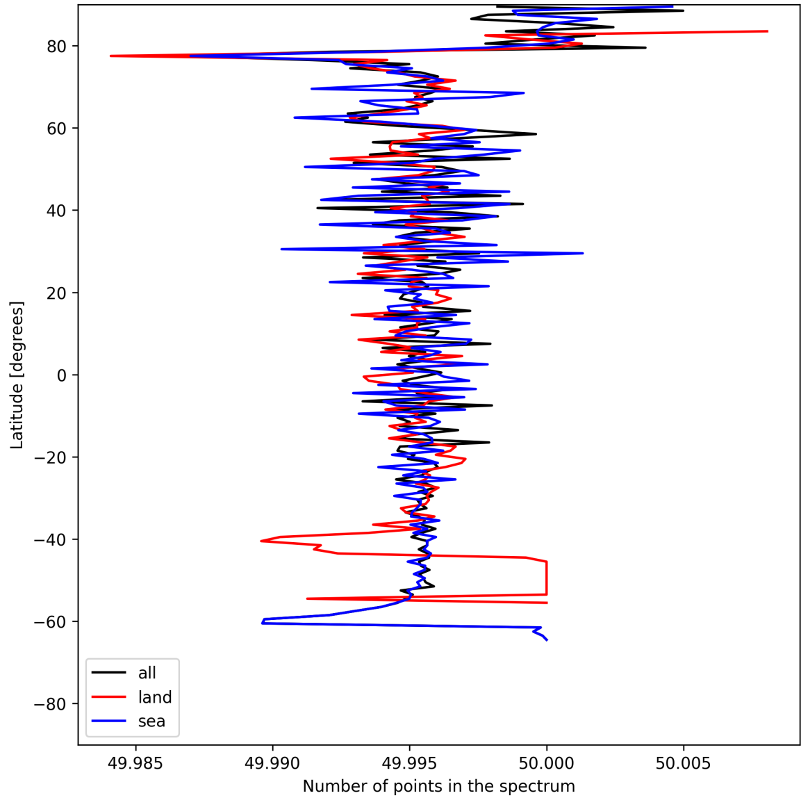
Figure 25: Zonal average of “Number of points in the spectrum” for 2025-06-19 to 2025-06-20.
