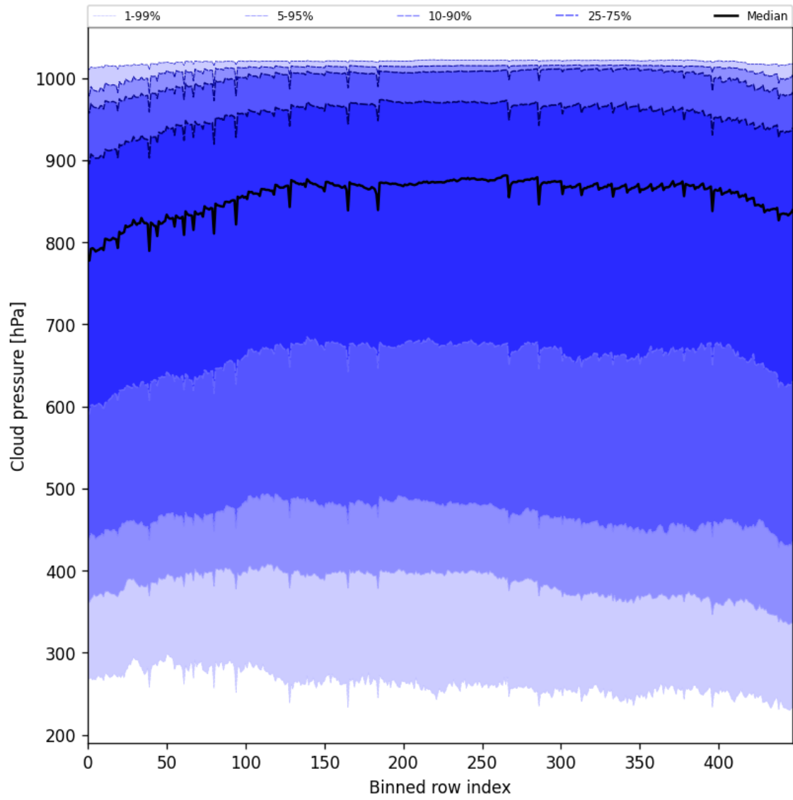
Figure 45: Along track statistics of “Cloud pressure” for 2025-06-19 to 2025-06-20
