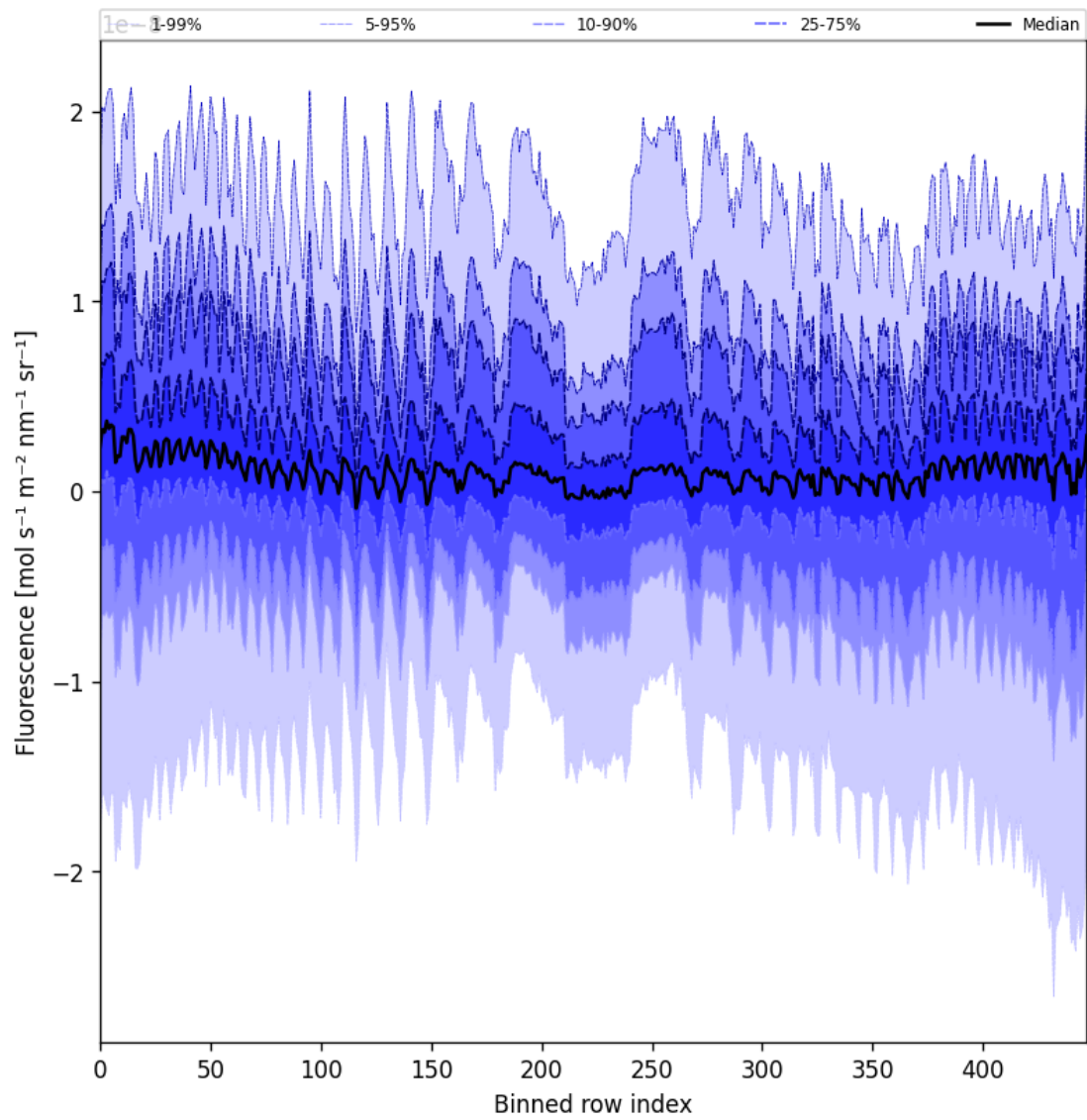
Figure 55: Along track statistics of “Fluorescence” for 2025-06-19 to 2025-06-20
