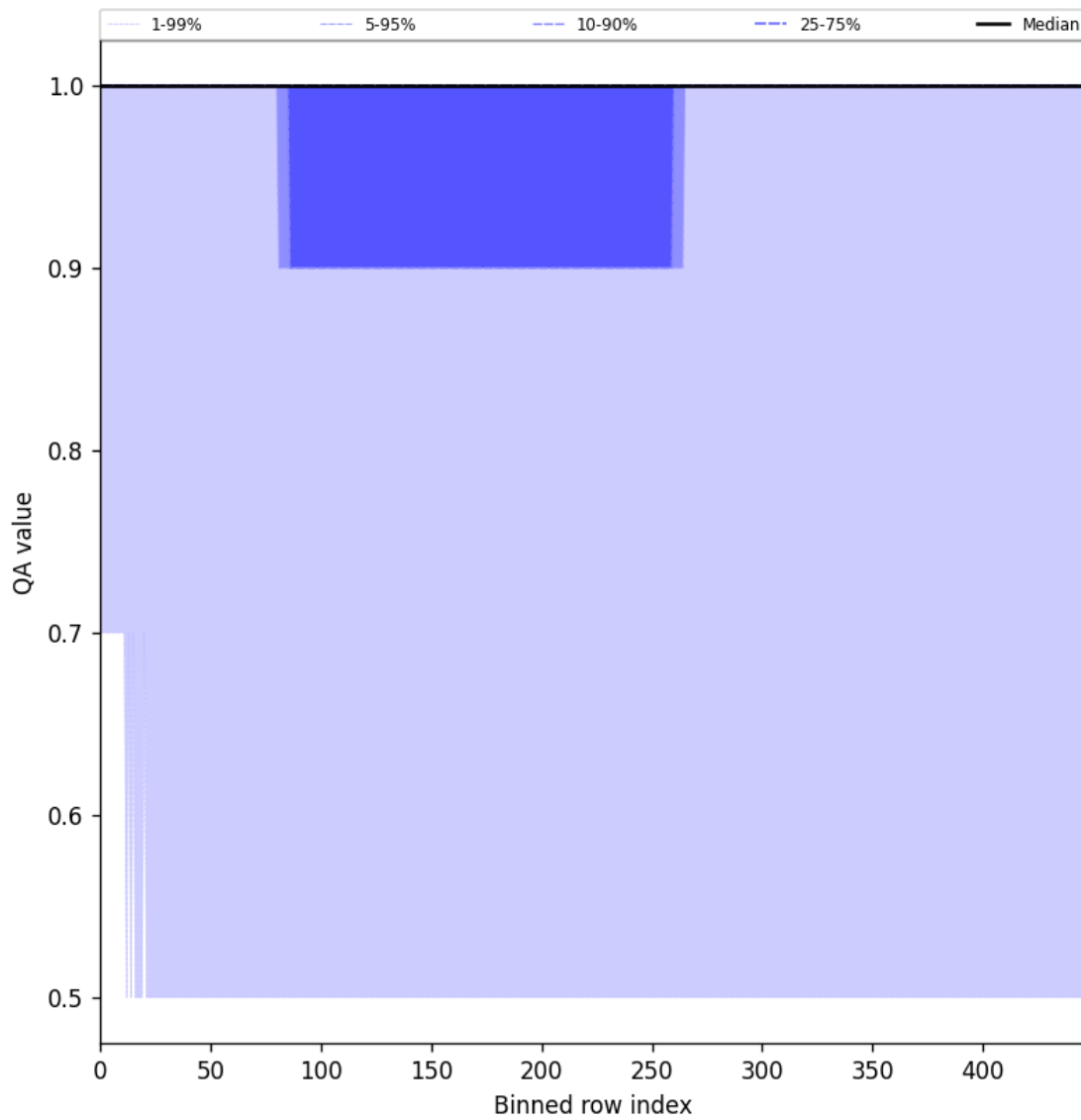
Figure 44: Along track statistics of “QA value” for 2025-06-19 to 2025-06-20
