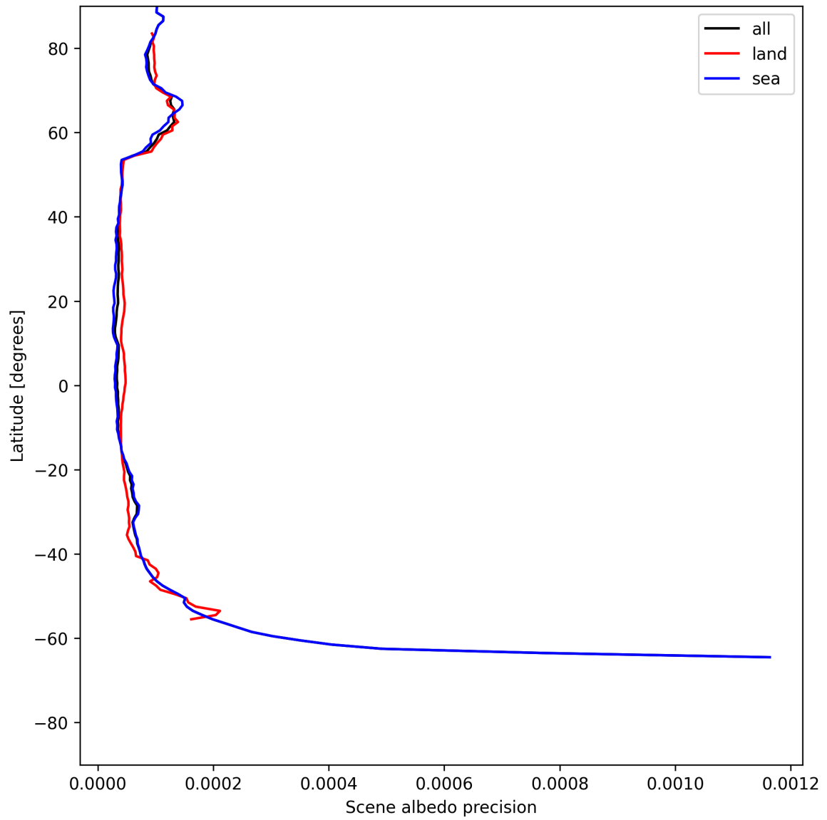
Figure 16: Zonal average of “Scene albedo precision” for 2025-06-19 to 2025-06-20.
