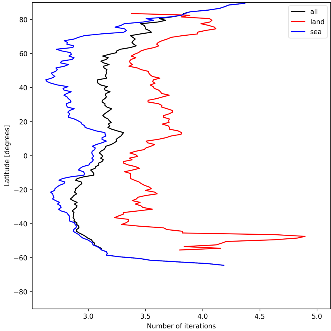
Figure 20: Zonal average of “Number of iterations” for 2025-06-19 to 2025-06-20.
