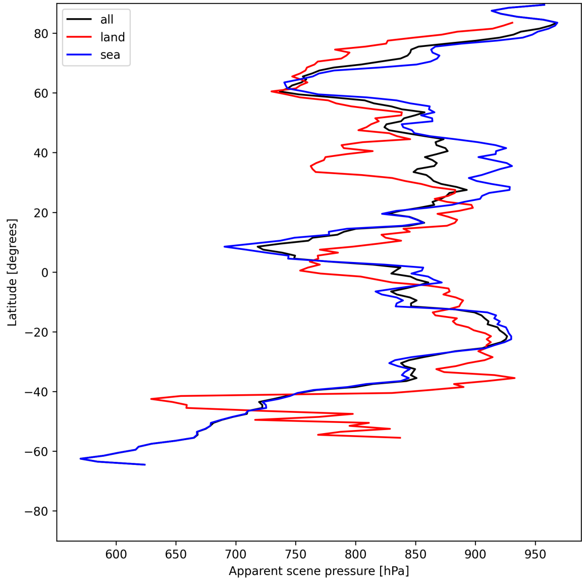
Figure 17: Zonal average of “Apparent scene pressure” for 2025-06-19 to 2025-06-20.
