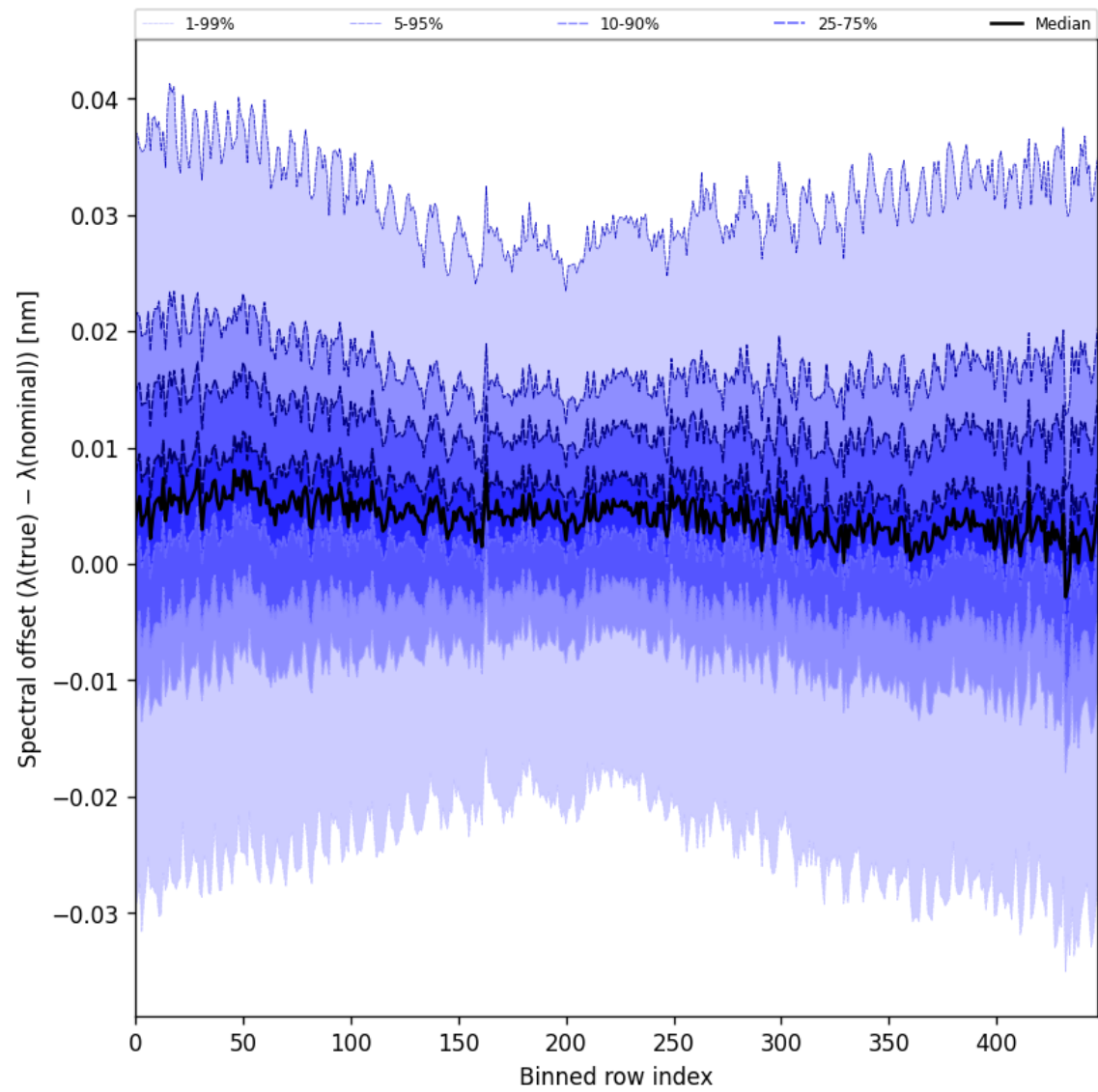
Figure 60: Along track statistics of “Spectral offset ( \lambda_{\text{true}} - \lambda_{\text{nominal}} )” for 2025-06-19 to 2025-06-20
