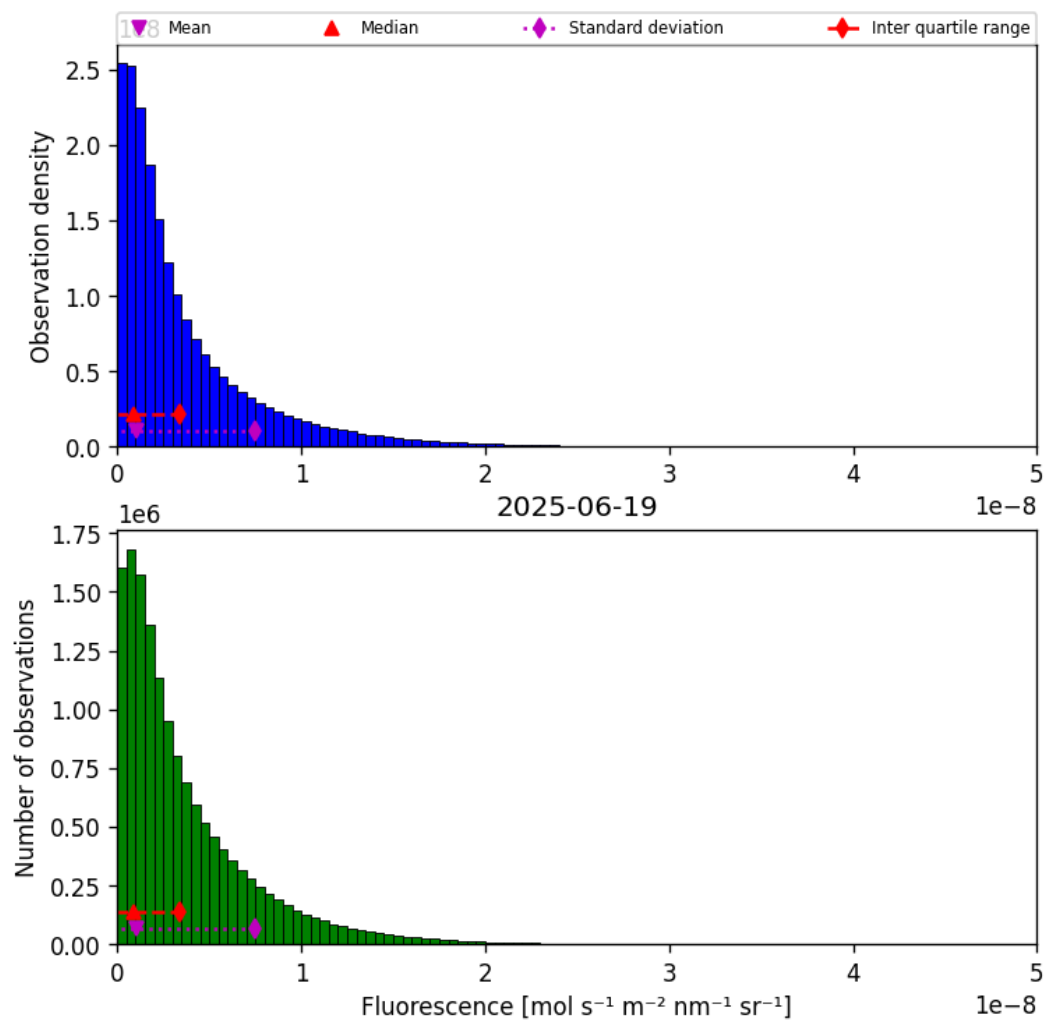
Figure 38: Histogram of “Fluorescence” for 2025-06-19 to 2025-06-20
