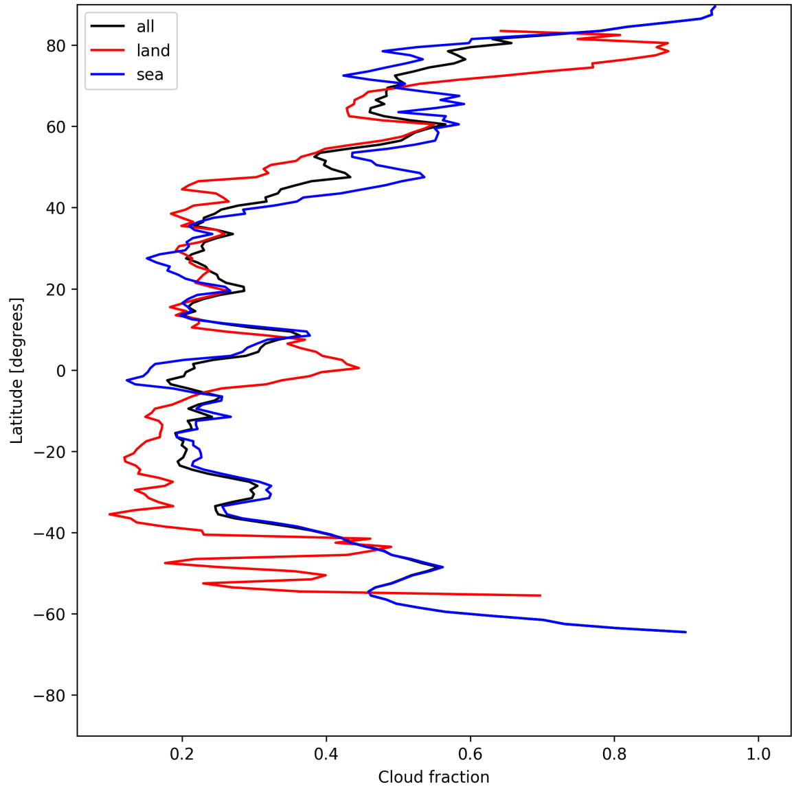
Figure 13: Zonal average of “Cloud fraction” for 2025-06-19 to 2025-06-20.
