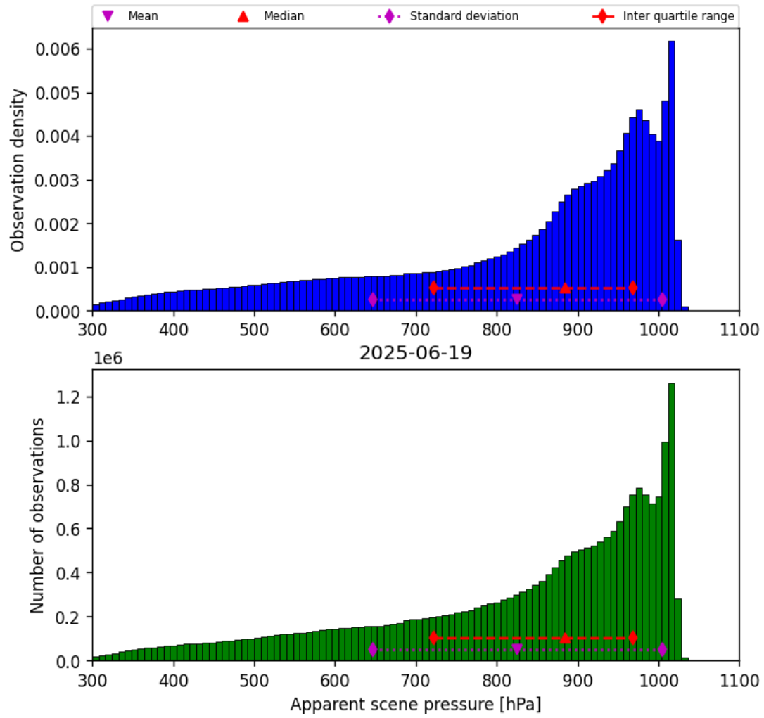
Figure 34: Histogram of “Apparent scene pressure” for 2025-06-19 to 2025-06-20
