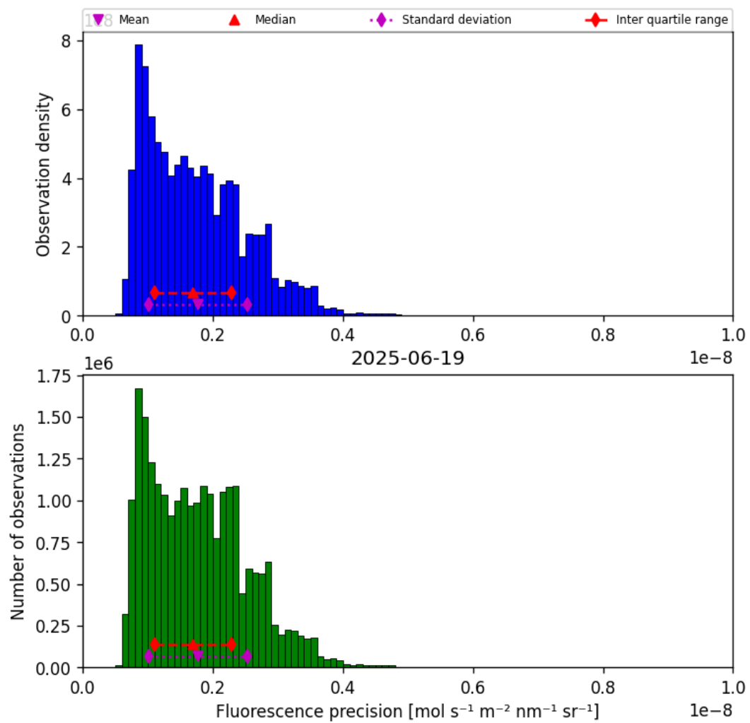
Figure 39: Histogram of “Fluorescence precision” for 2025-06-19 to 2025-06-20
