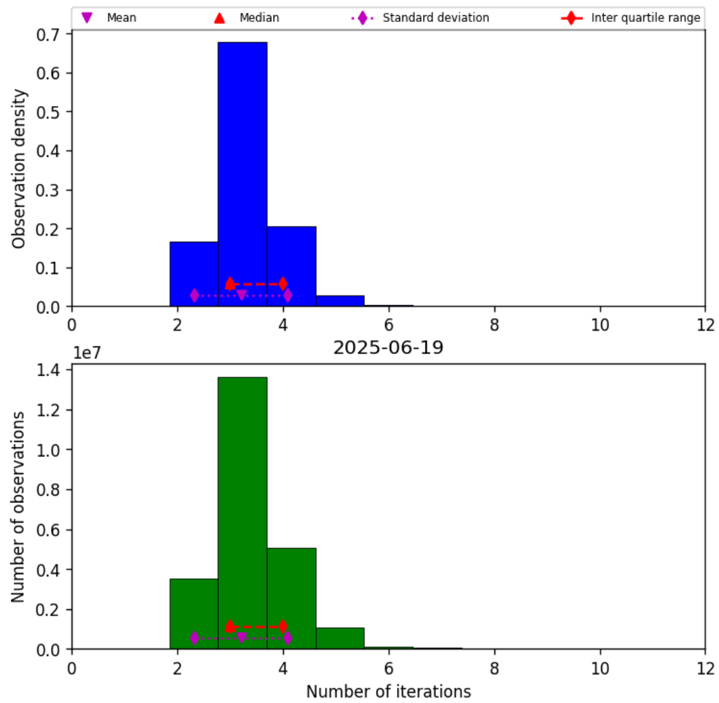
Figure 37: Histogram of “Number of iterations” for 2025-06-19 to 2025-06-20
