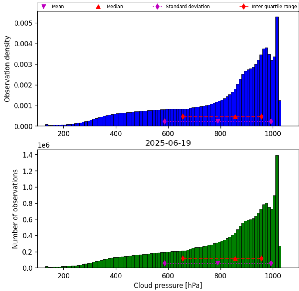
Figure 28: Histogram of “Cloud pressure” for 2025-06-19 to 2025-06-20
