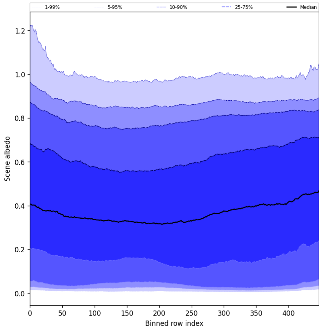
Figure 49: Along track statistics of “Scene albedo” for 2025-06-19 to 2025-06-20
