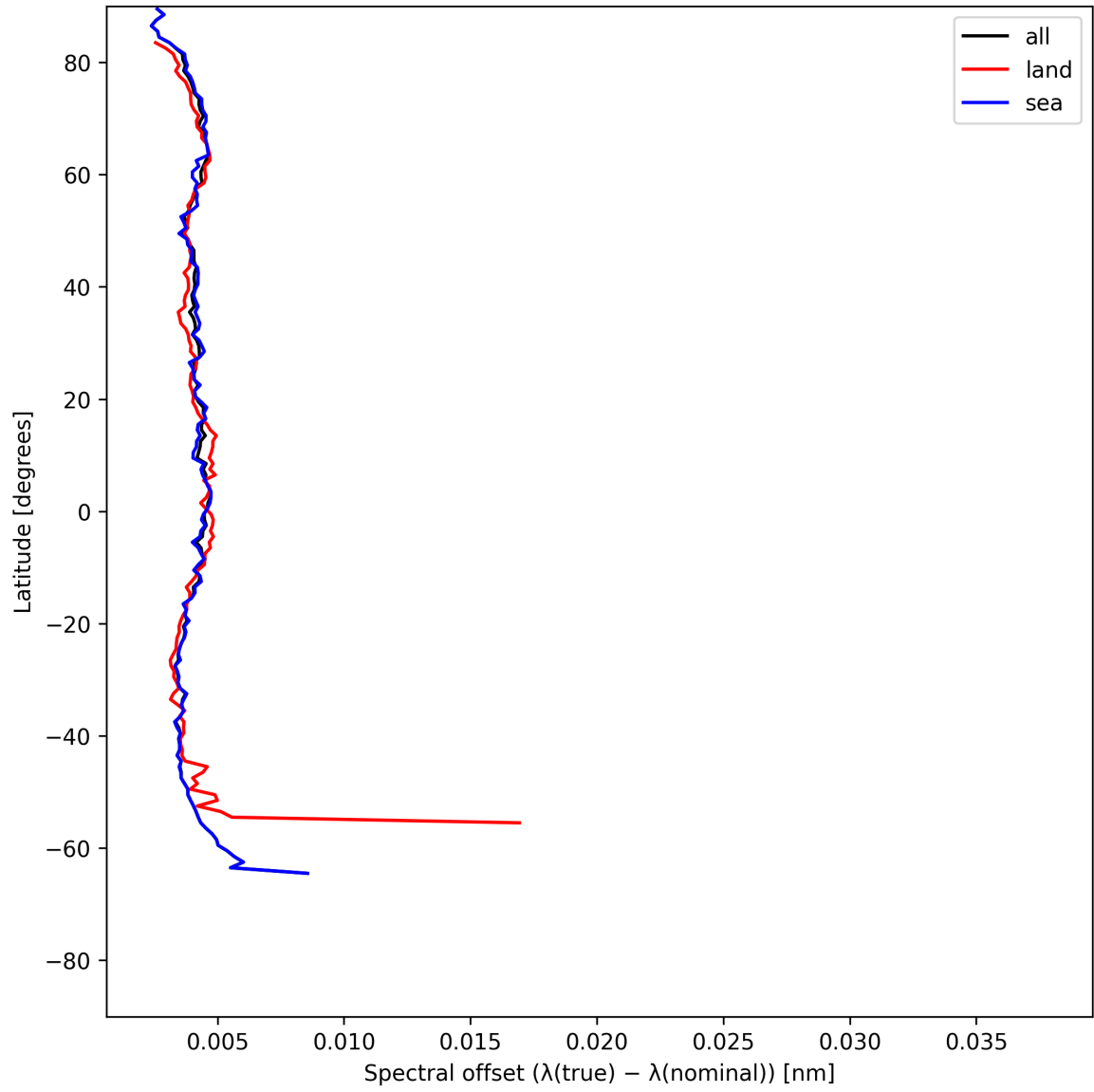
Figure 26: Zonal average of “Spectral offset ( \lambda_{\text{true}} - \lambda_{\text{nominal}} )” for 2025-06-19 to 2025-06-20.
