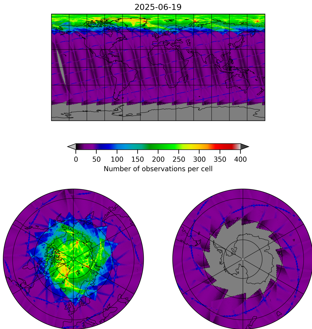
Figure 9: Map of the number of observations for 2025-06-19 to 2025-06-20
