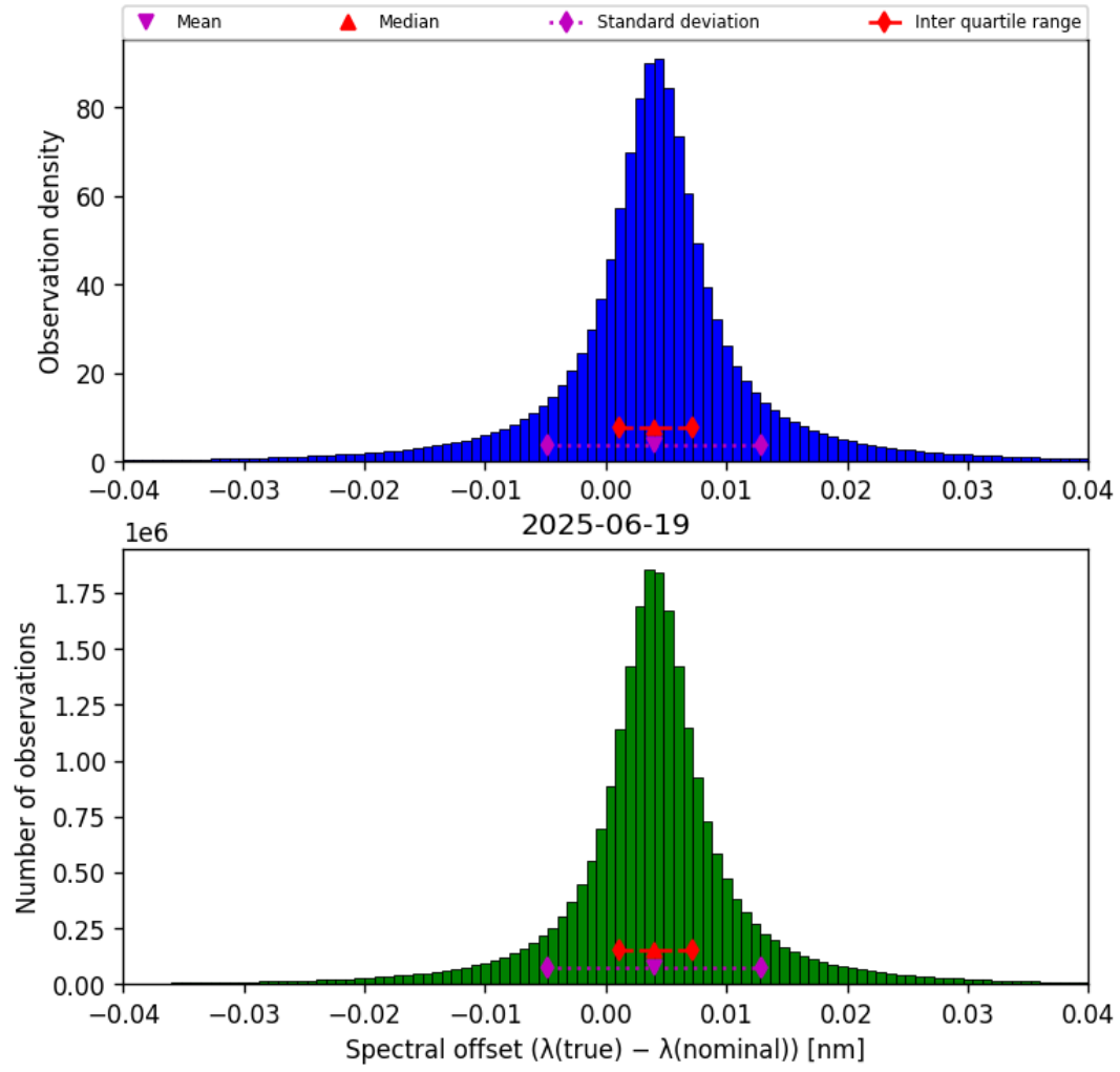
Figure 43: Histogram of “Spectral offset ( \lambda_{\text{true}} - \lambda_{\text{nominal}} )” for 2025-06-19 to 2025-06-20
