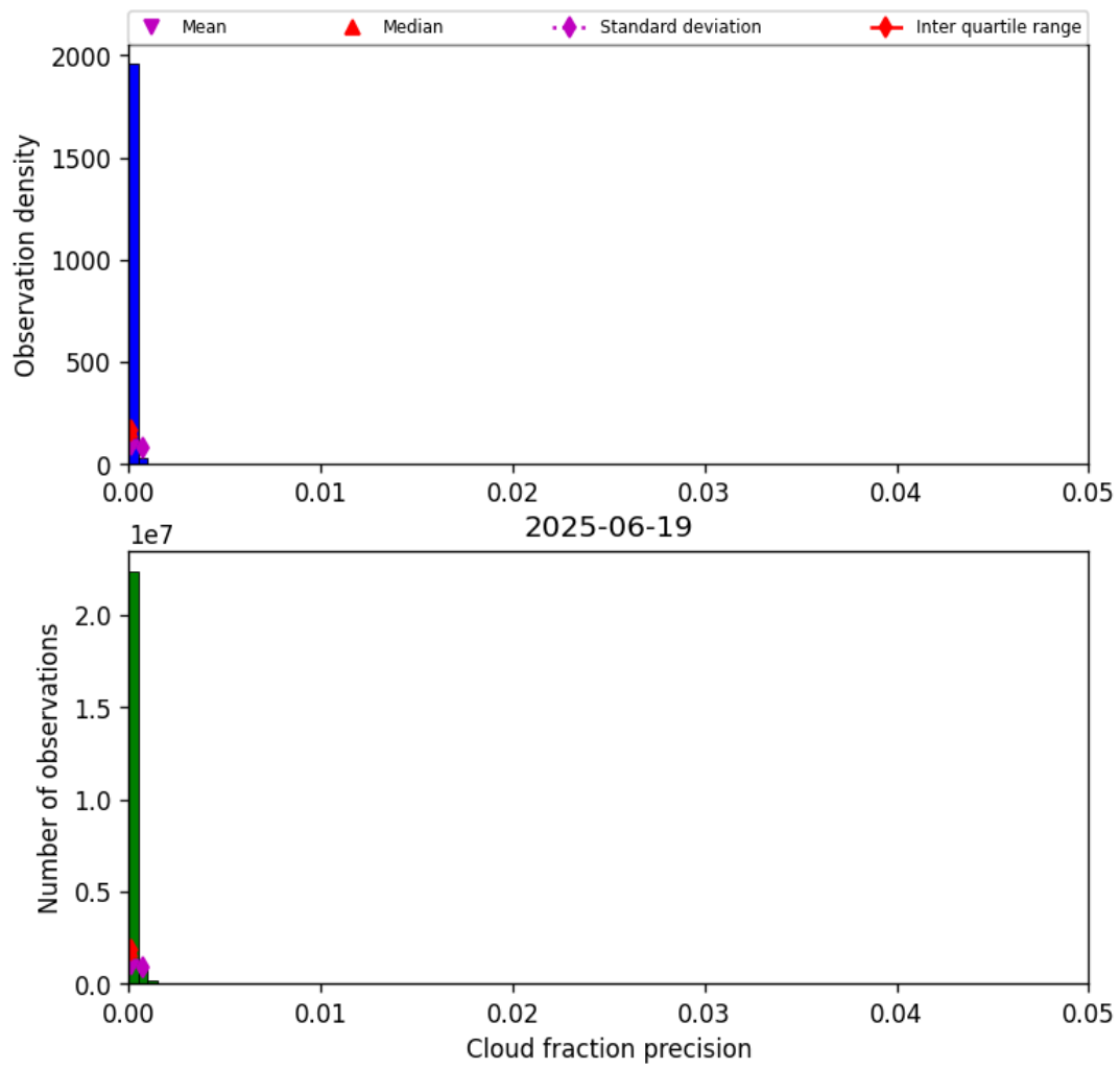
Figure 31: Histogram of “Cloud fraction precision” for 2025-06-19 to 2025-06-20
