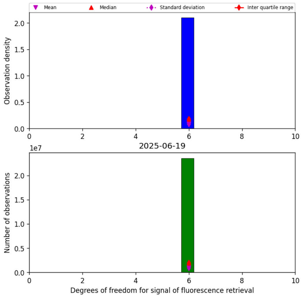
Figure 41: Histogram of “Degrees of freedom for signal of fluorescence retrieval” for 2025-06-19 to 2025-06-20
