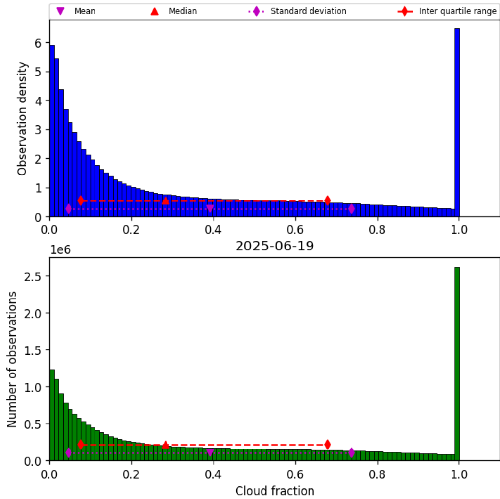
Figure 30: Histogram of “Cloud fraction” for 2025-06-19 to 2025-06-20
