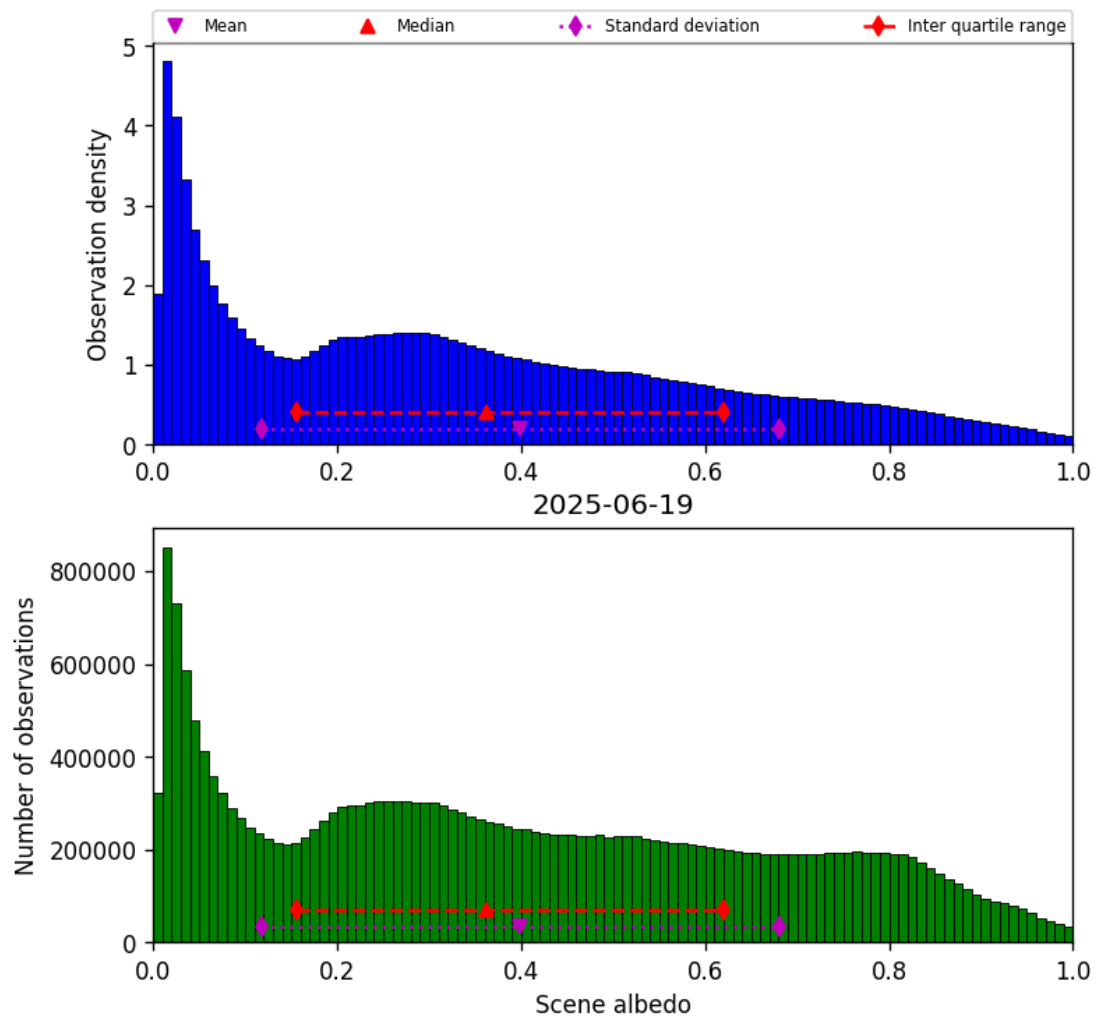
Figure 32: Histogram of “Scene albedo” for 2025-06-19 to 2025-06-20
