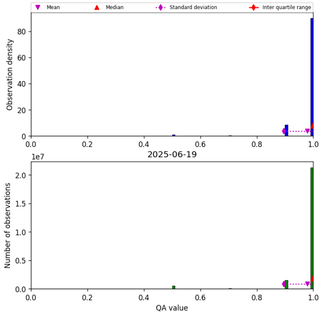
Figure 27: Histogram of “QA value” for 2025-06-19 to 2025-06-20
