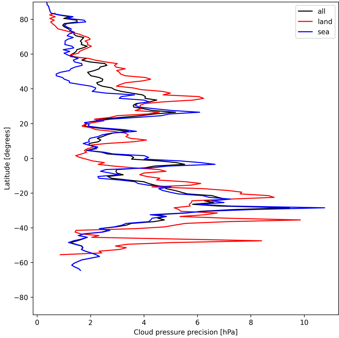
Figure 12: Zonal average of “Cloud pressure precision” for 2025-06-19 to 2025-06-20.
