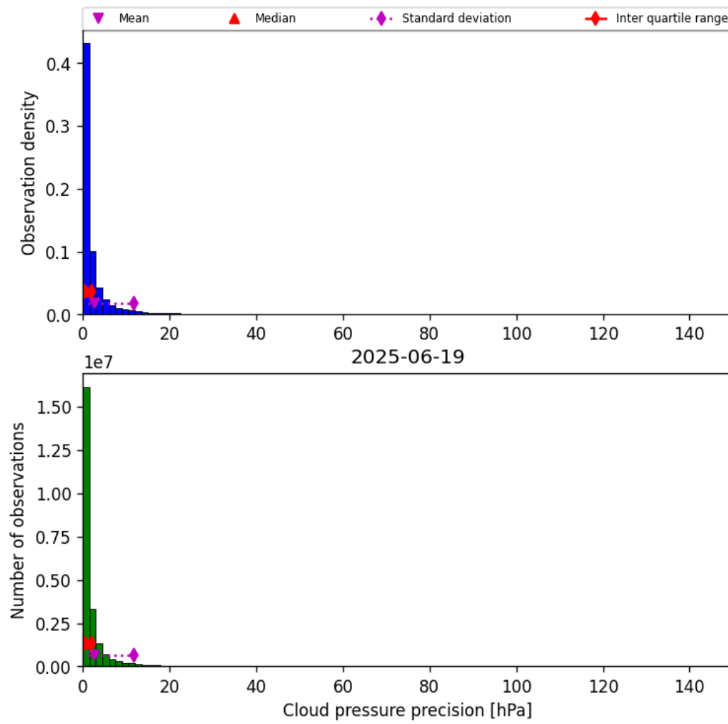
Figure 29: Histogram of “Cloud pressure precision” for 2025-06-19 to 2025-06-20
