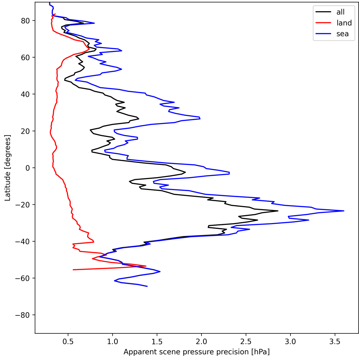
Figure 18: Zonal average of “Apparent scene pressure precision” for 2025-06-19 to 2025-06-20.
