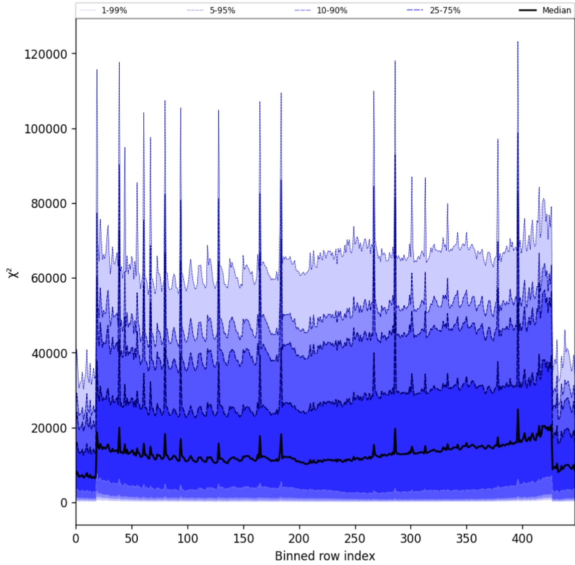
Figure 53: Along track statistics of “ \chi^2 ” for 2025-06-19 to 2025-06-20
