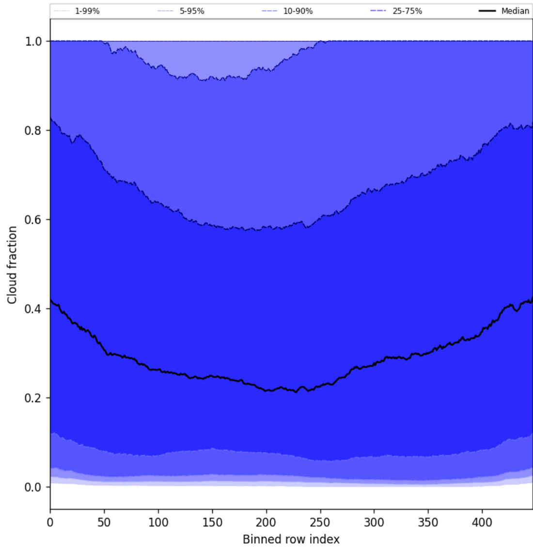
Figure 47: Along track statistics of “Cloud fraction” for 2025-06-19 to 2025-06-20
