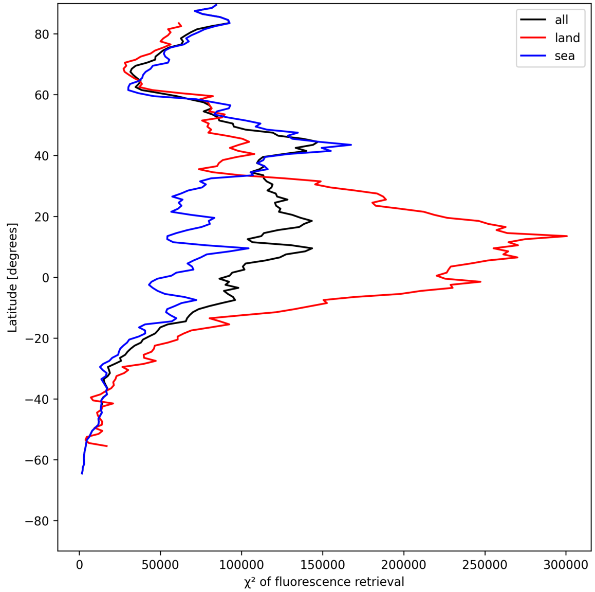
Figure 23: Zonal average of “ \chi^2 of fluorescence retrieval” for 2025-06-19 to 2025-06-20.
