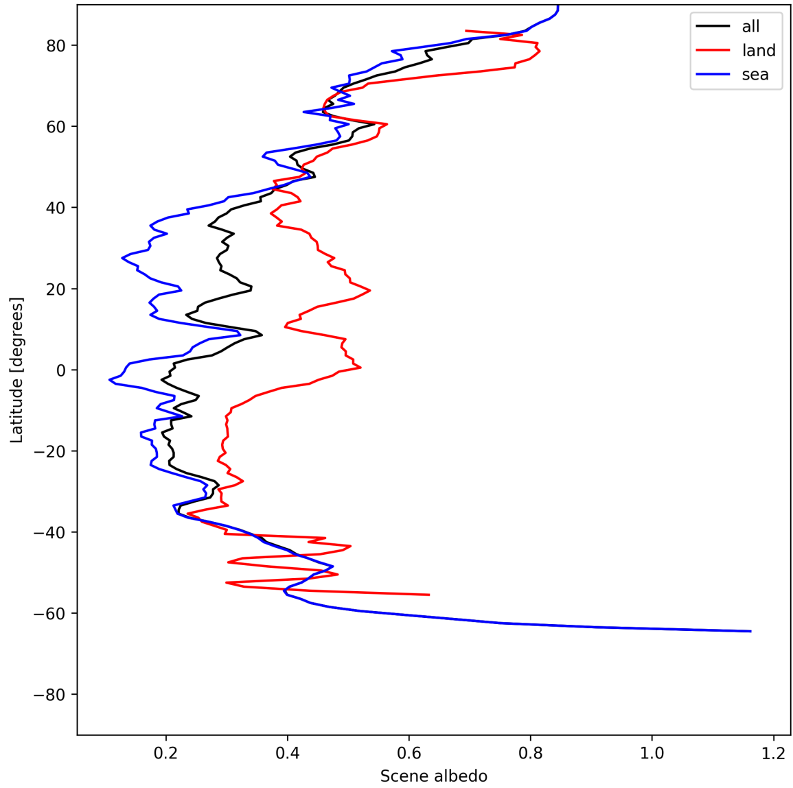
Figure 15: Zonal average of “Scene albedo” for 2025-06-19 to 2025-06-20.
