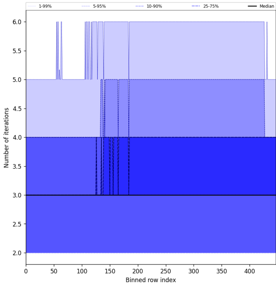
Figure 54: Along track statistics of “Number of iterations” for 2025-06-19 to 2025-06-20
