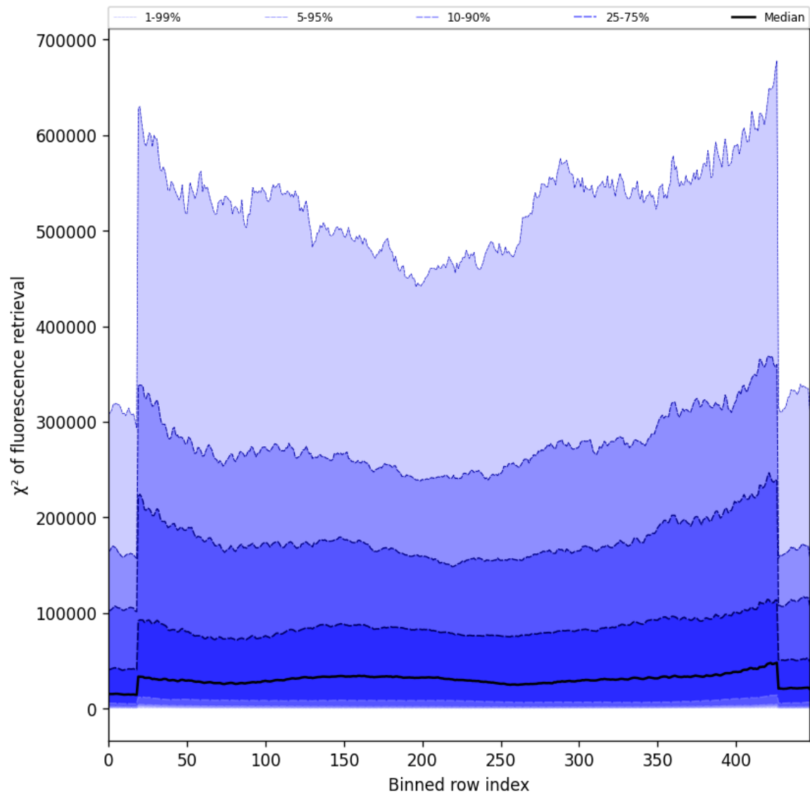
Figure 57: Along track statistics of “ \chi^2 of fluorescence retrieval” for 2025-06-19 to 2025-06-20
