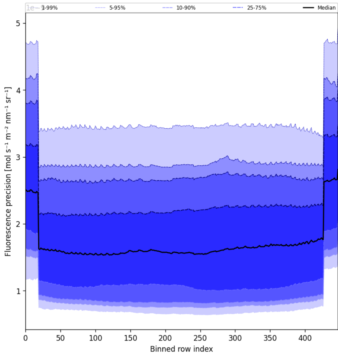
Figure 56: Along track statistics of “Fluorescence precision” for 2025-06-19 to 2025-06-20
