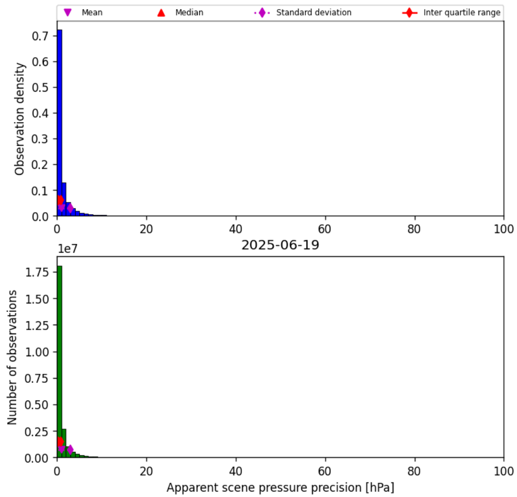
Figure 35: Histogram of “Apparent scene pressure precision” for 2025-06-19 to 2025-06-20
