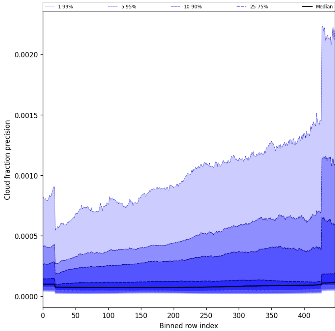
Figure 48: Along track statistics of “Cloud fraction precision” for 2025-06-19 to 2025-06-20
