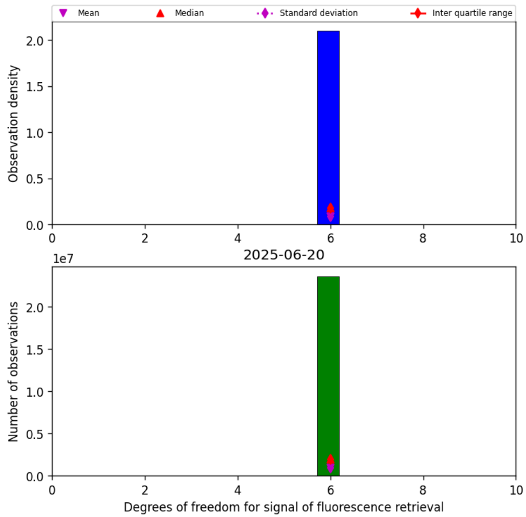
Figure 41: Histogram of “Degrees of freedom for signal of fluorescence retrieval” for 2025-06-20 to 2025-06-20
