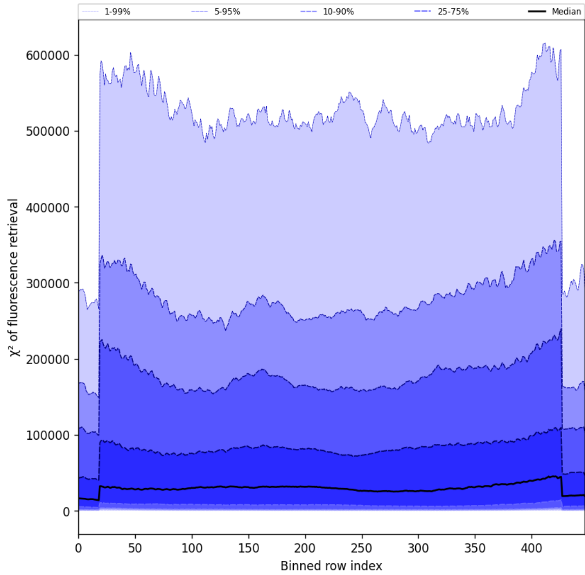
Figure 57: Along track statistics of “ \chi^2 of fluorescence retrieval” for 2025-06-20 to 2025-06-20
