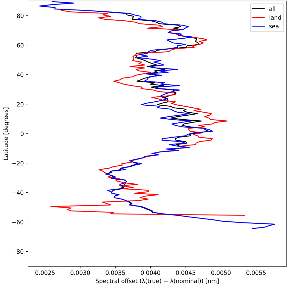
Figure 26: Zonal average of “Spectral offset ( \lambda_{\text{true}} - \lambda_{\text{nominal}} )” for 2025-06-20 to 2025-06-20.
