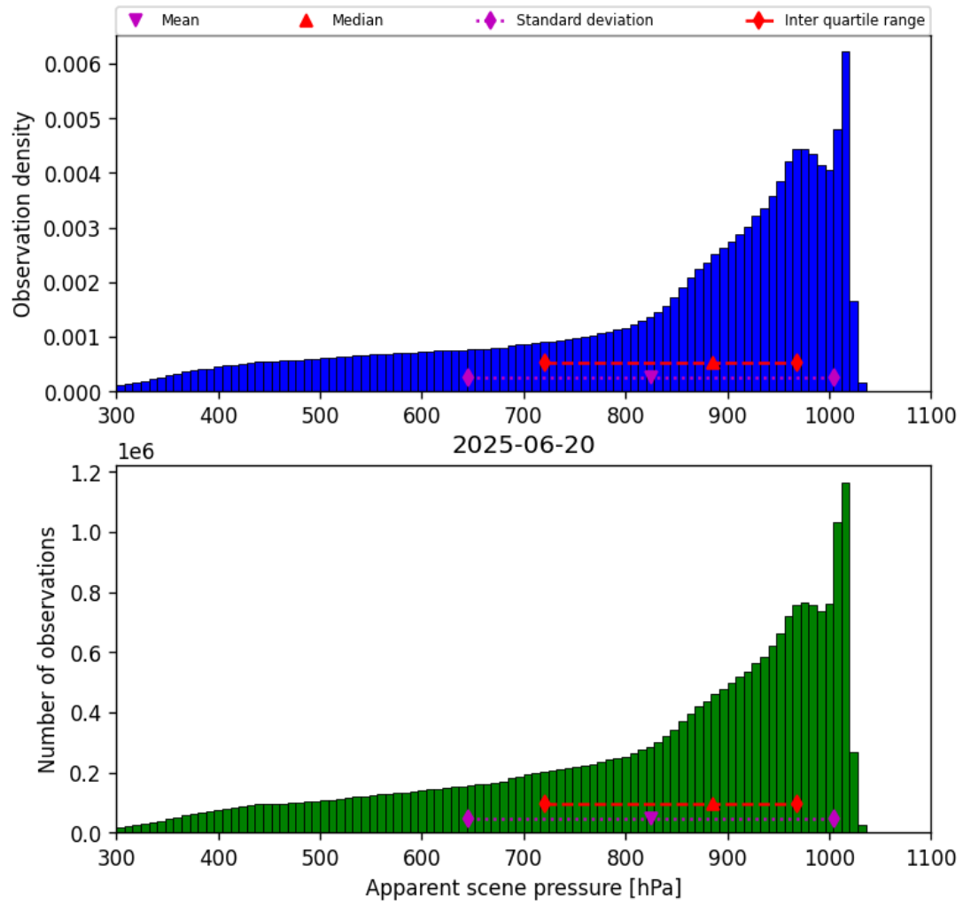
Figure 34: Histogram of “Apparent scene pressure” for 2025-06-20 to 2025-06-20
