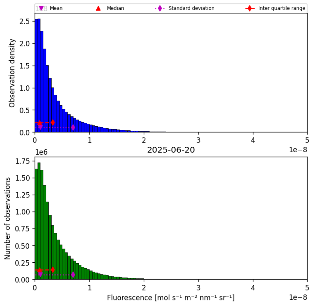
Figure 38: Histogram of “Fluorescence” for 2025-06-20 to 2025-06-20
