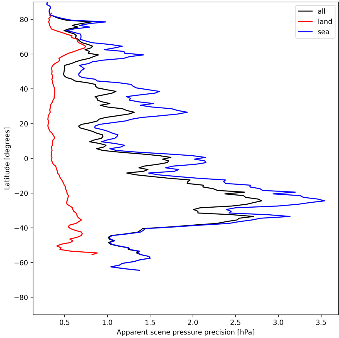
Figure 18: Zonal average of “Apparent scene pressure precision” for 2025-06-20 to 2025-06-20.
