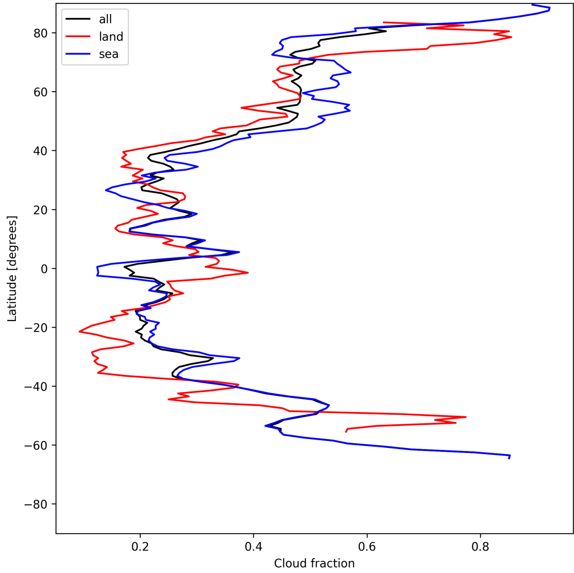
Figure 13: Zonal average of “Cloud fraction” for 2025-06-20 to 2025-06-20.
