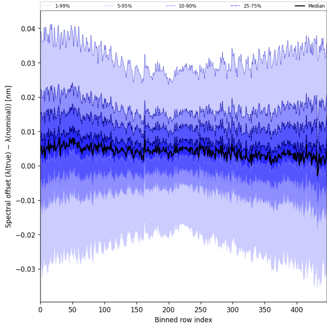
Figure 60: Along track statistics of “Spectral offset ( \lambda_{\text{true}} - \lambda_{\text{nominal}} )” for 2025-06-20 to 2025-06-20
