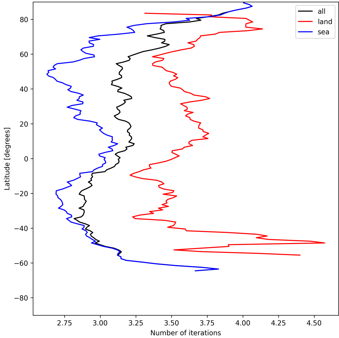
Figure 20: Zonal average of “Number of iterations” for 2025-06-20 to 2025-06-20.
