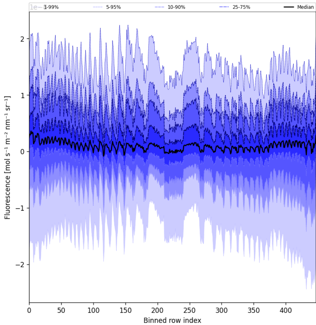
Figure 55: Along track statistics of “Fluorescence” for 2025-06-20 to 2025-06-20
