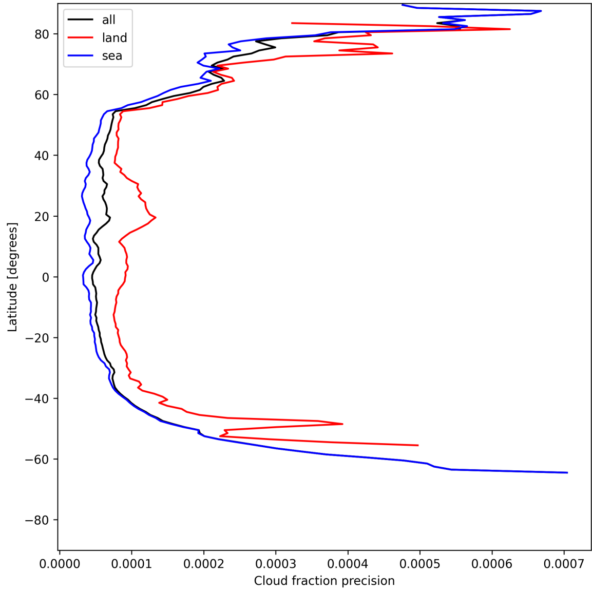
Figure 14: Zonal average of “Cloud fraction precision” for 2025-06-20 to 2025-06-20.
