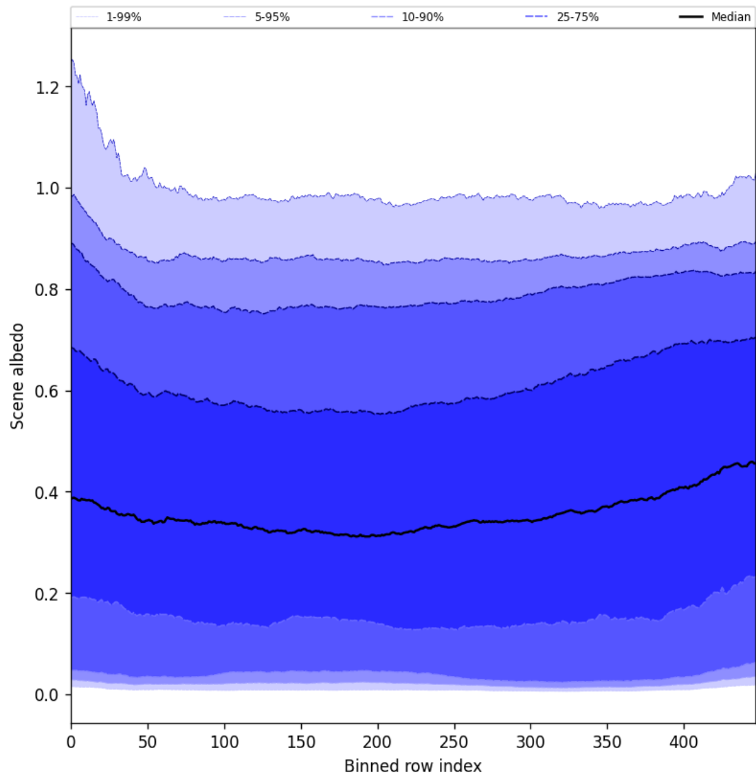
Figure 49: Along track statistics of “Scene albedo” for 2025-06-20 to 2025-06-20
