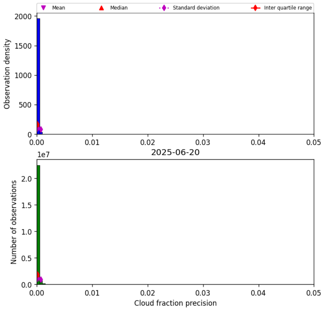
Figure 31: Histogram of “Cloud fraction precision” for 2025-06-20 to 2025-06-20
