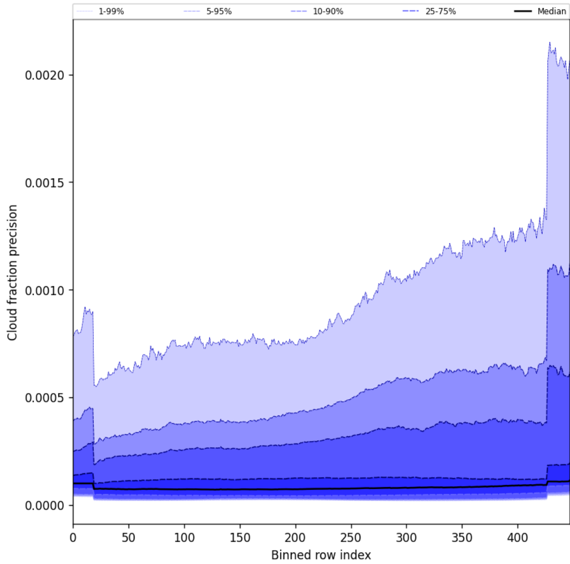
Figure 48: Along track statistics of “Cloud fraction precision” for 2025-06-20 to 2025-06-20
