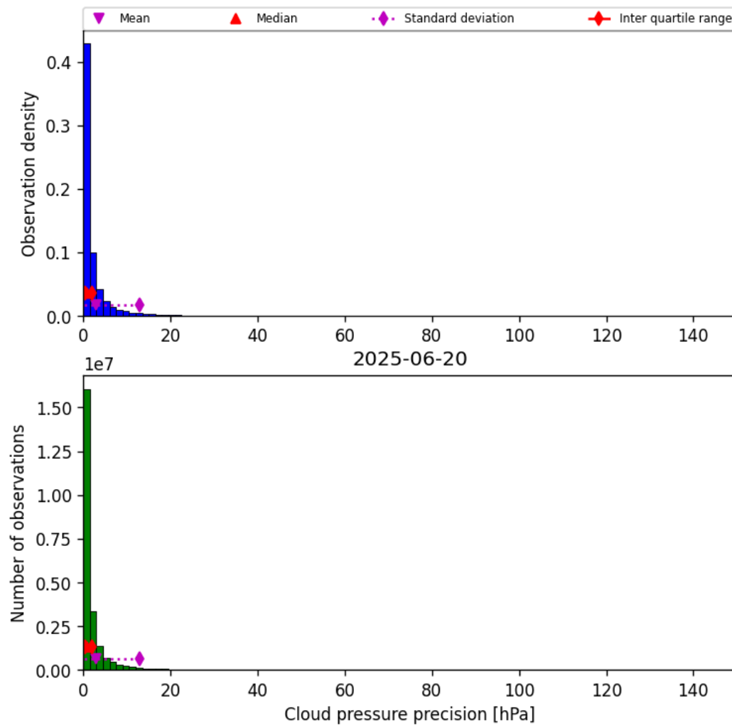
Figure 29: Histogram of “Cloud pressure precision” for 2025-06-20 to 2025-06-20
