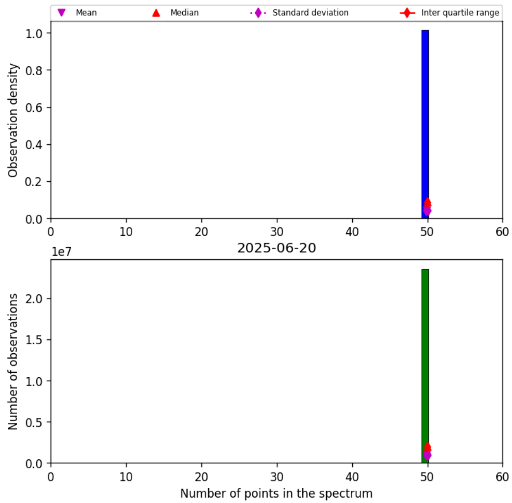
Figure 42: Histogram of “Number of points in the spectrum” for 2025-06-20 to 2025-06-20
