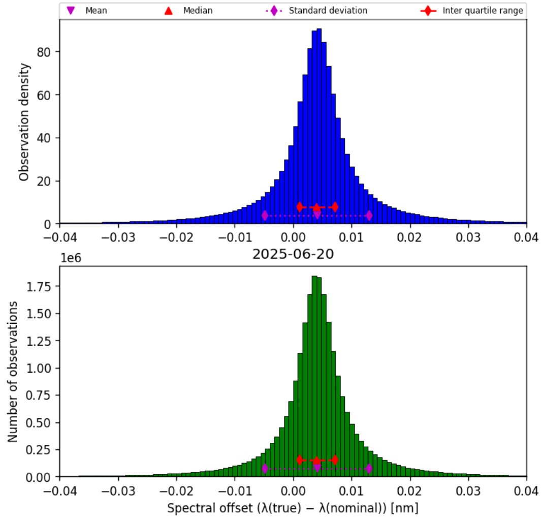
Figure 43: Histogram of “Spectral offset ( \lambda_{\text{true}} - \lambda_{\text{nominal}} )” for 2025-06-20 to 2025-06-20
