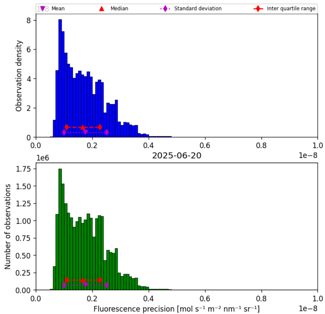
Figure 39: Histogram of “Fluorescence precision” for 2025-06-20 to 2025-06-20
