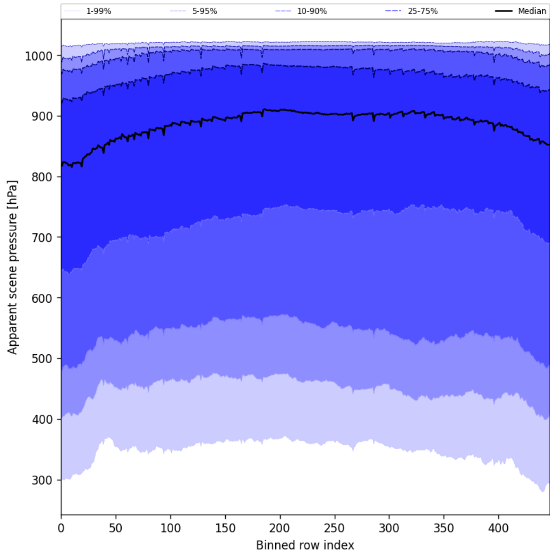
Figure 51: Along track statistics of “Apparent scene pressure” for 2025-06-20 to 2025-06-20
