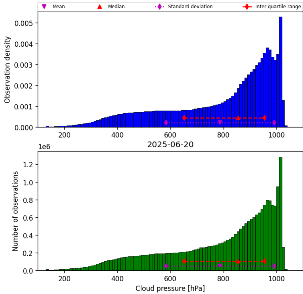
Figure 28: Histogram of “Cloud pressure” for 2025-06-20 to 2025-06-20
