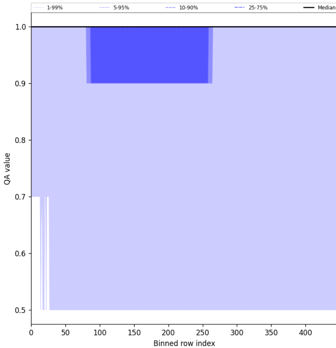
Figure 44: Along track statistics of “QA value” for 2025-06-20 to 2025-06-20
