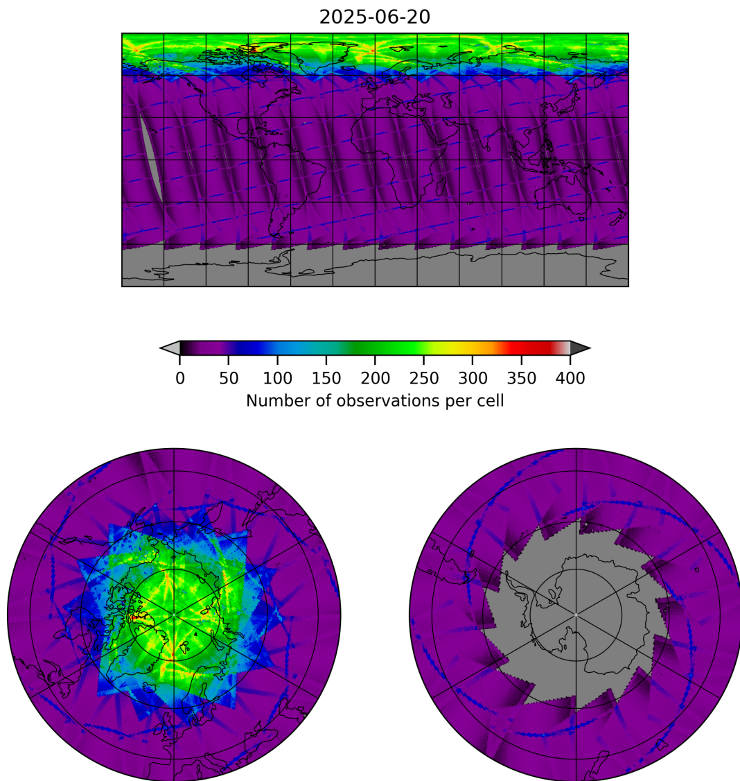
Figure 9: Map of the number of observations for 2025-06-20 to 2025-06-20
