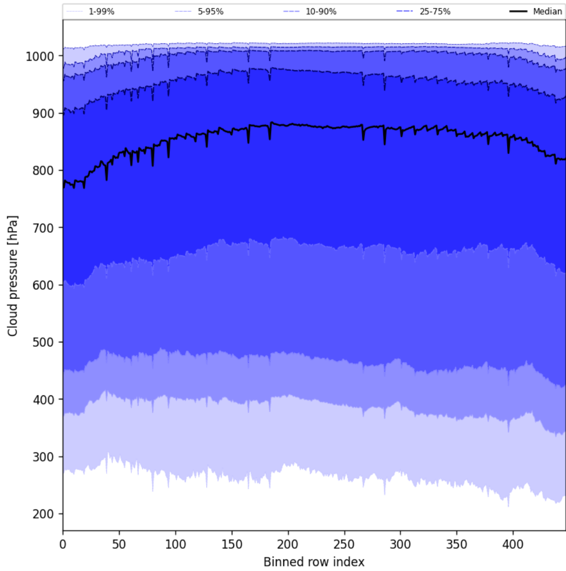
Figure 45: Along track statistics of “Cloud pressure” for 2025-06-20 to 2025-06-20
