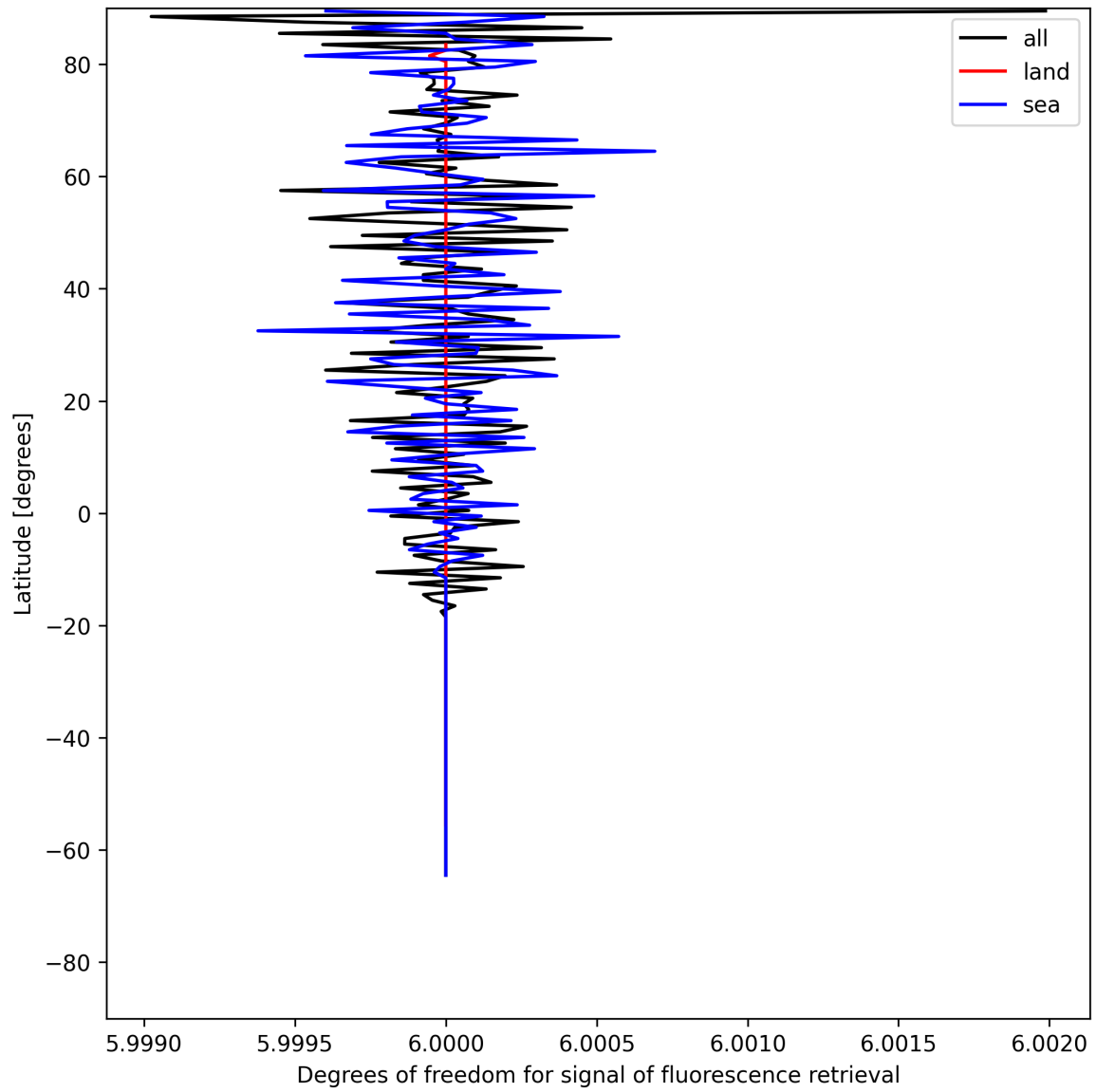
Figure 24: Zonal average of “Degrees of freedom for signal of fluorescence retrieval” for 2025-06-20 to 2025-06-20.
