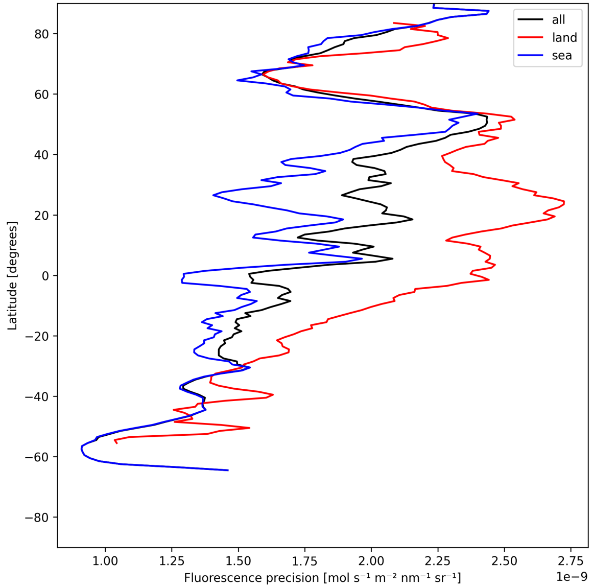
Figure 22: Zonal average of “Fluorescence precision” for 2025-06-20 to 2025-06-20.
