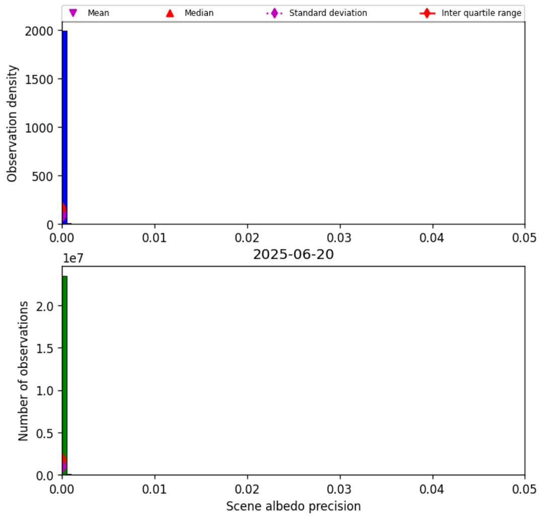
Figure 33: Histogram of “Scene albedo precision” for 2025-06-20 to 2025-06-20
