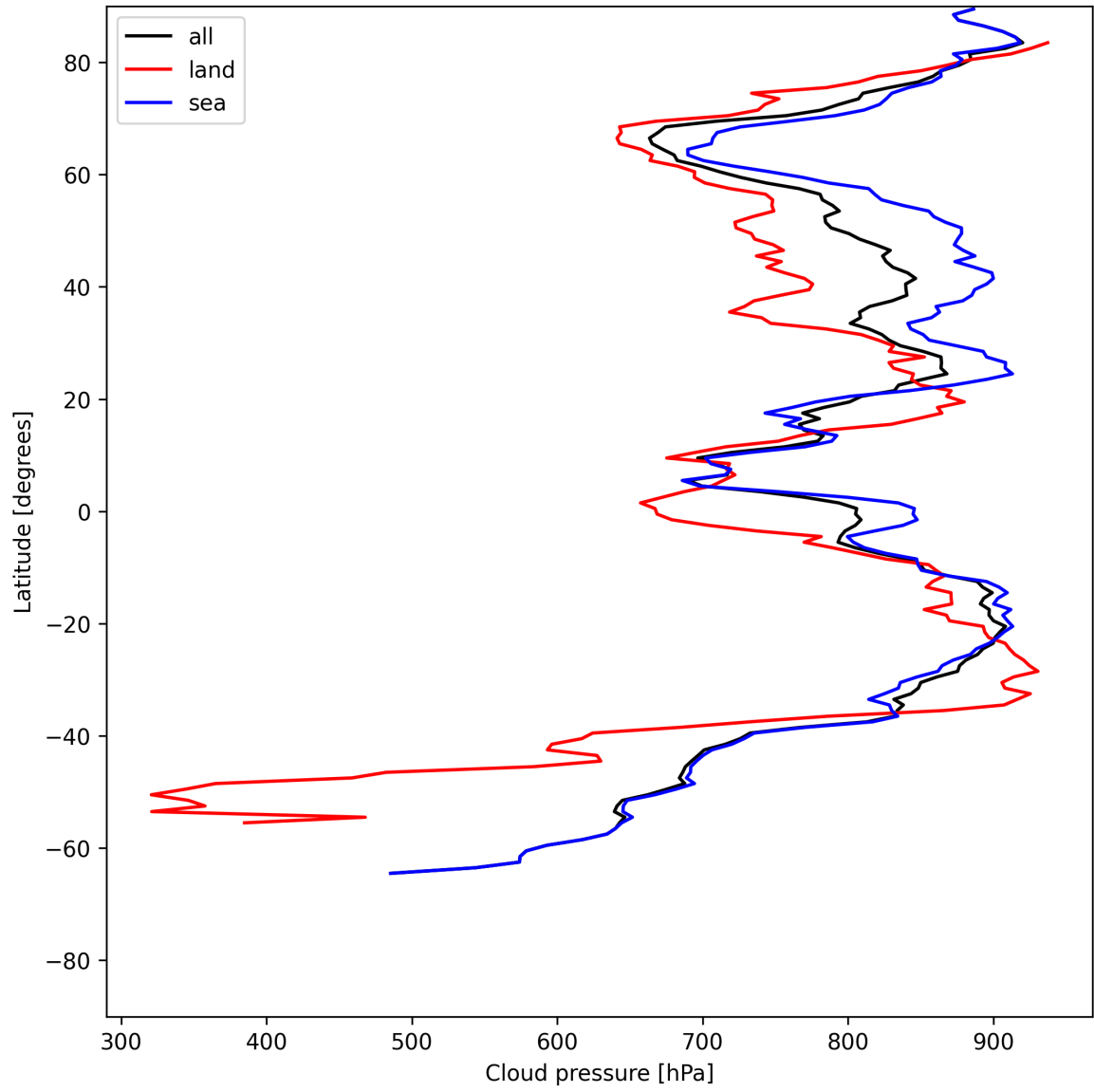
Figure 11: Zonal average of “Cloud pressure” for 2025-06-20 to 2025-06-20.
