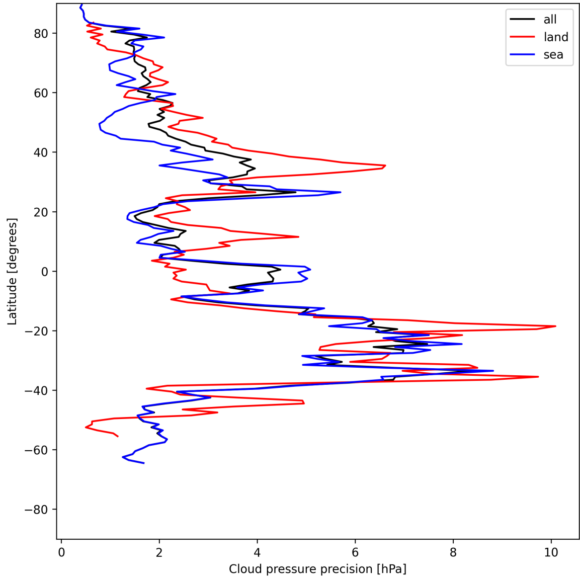
Figure 12: Zonal average of “Cloud pressure precision” for 2025-06-20 to 2025-06-20.
