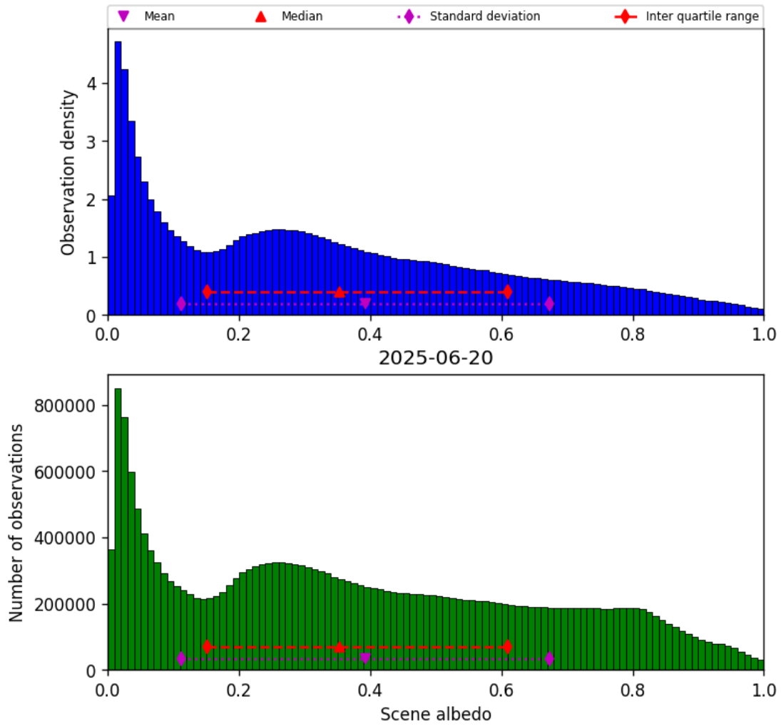
Figure 32: Histogram of “Scene albedo” for 2025-06-20 to 2025-06-20
