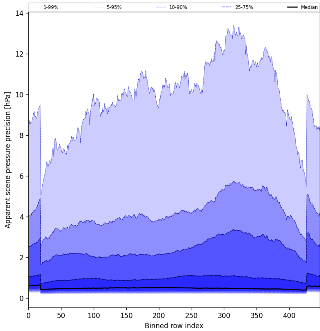
Figure 52: Along track statistics of “Apparent scene pressure precision” for 2025-06-20 to 2025-06-20
