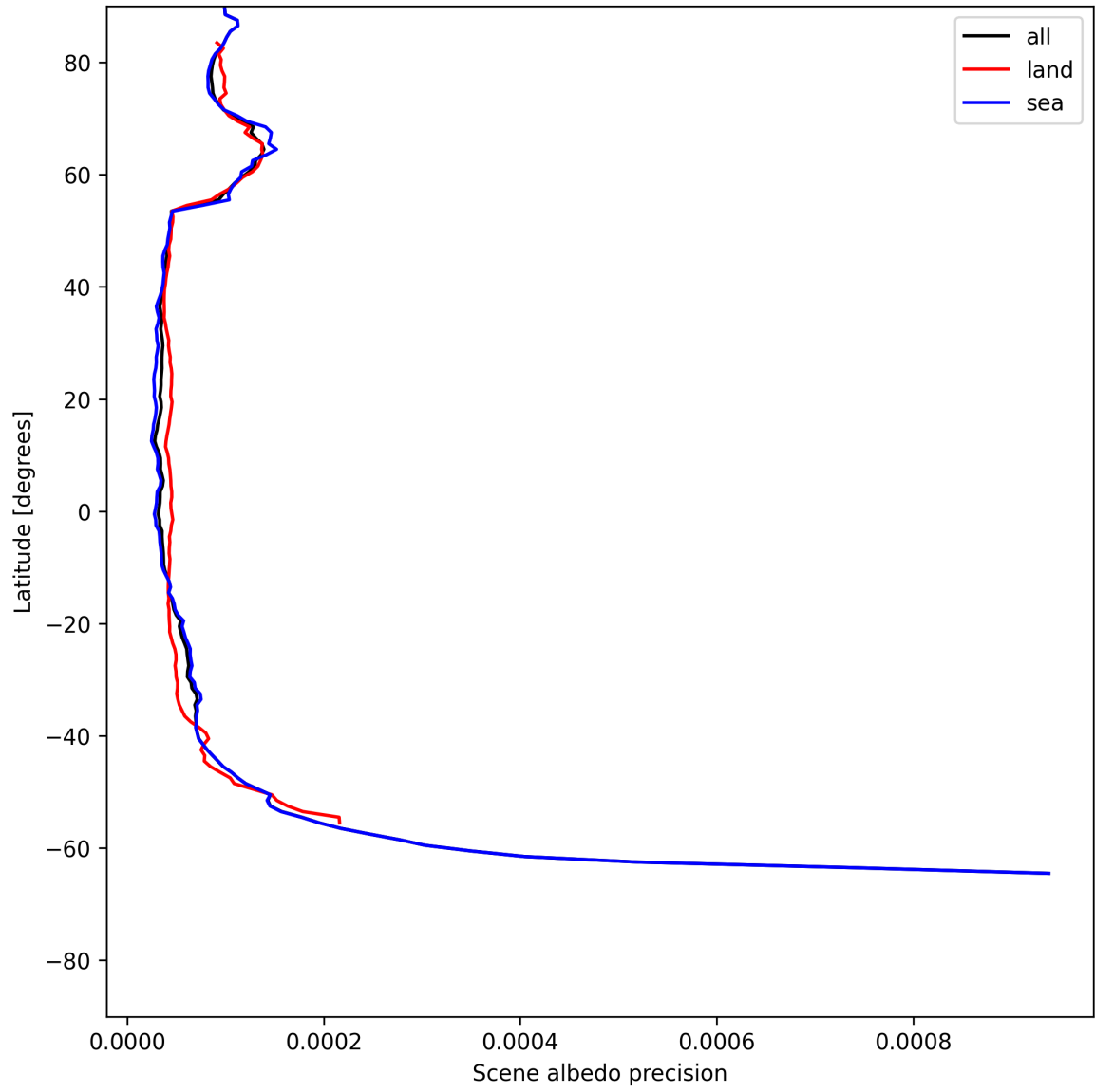
Figure 16: Zonal average of “Scene albedo precision” for 2025-06-20 to 2025-06-20.
