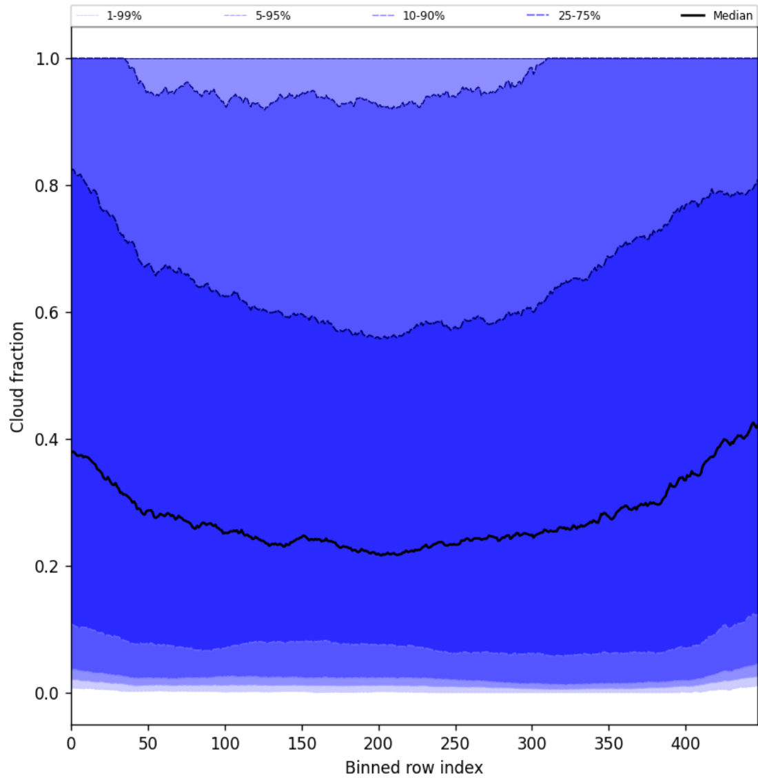
Figure 47: Along track statistics of “Cloud fraction” for 2025-06-20 to 2025-06-20
