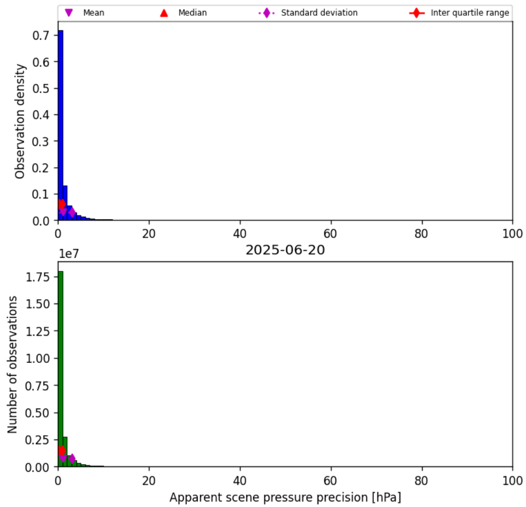
Figure 35: Histogram of “Apparent scene pressure precision” for 2025-06-20 to 2025-06-20
