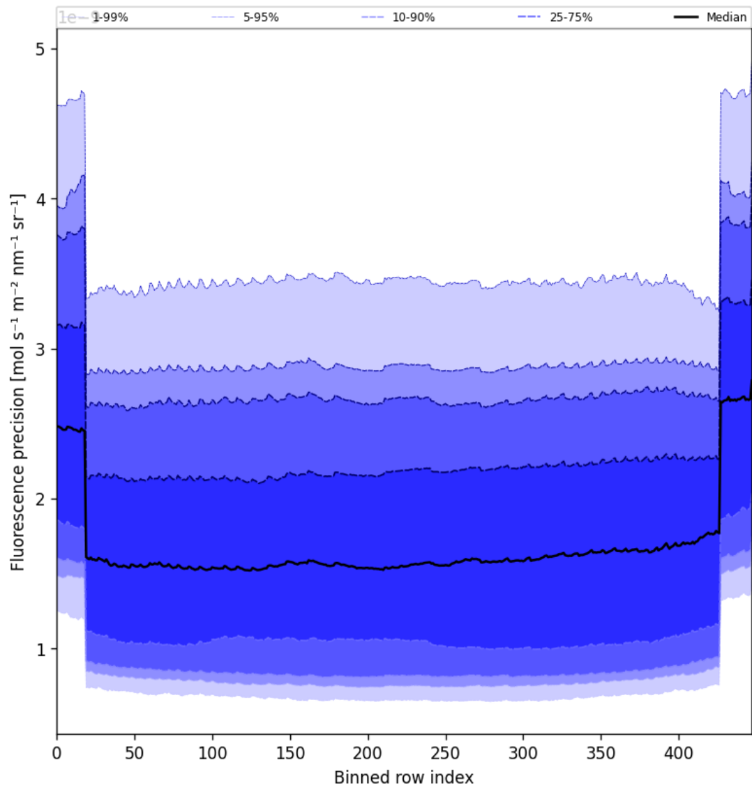
Figure 56: Along track statistics of “Fluorescence precision” for 2025-06-20 to 2025-06-20
