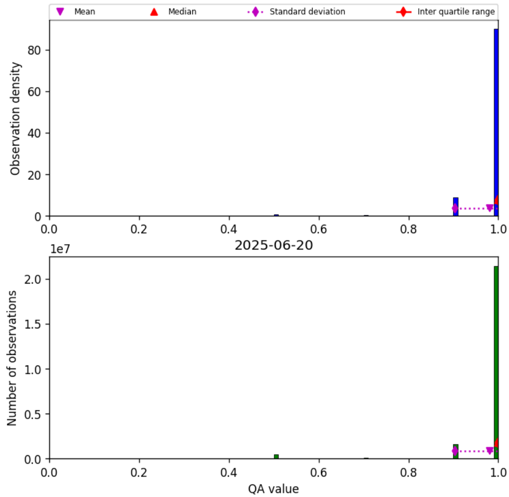
Figure 27: Histogram of “QA value” for 2025-06-20 to 2025-06-20
