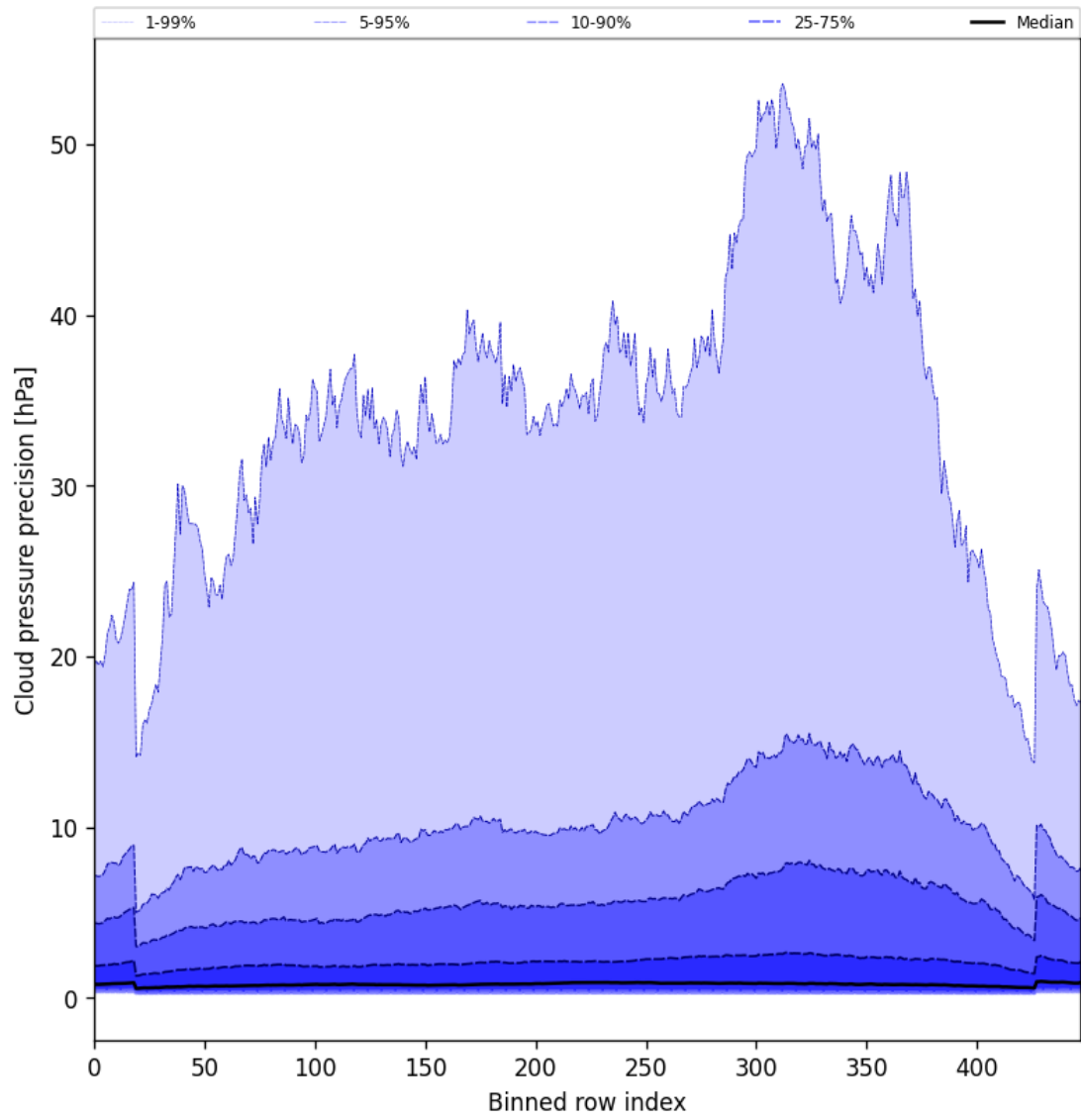
Figure 46: Along track statistics of “Cloud pressure precision” for 2025-06-20 to 2025-06-20
