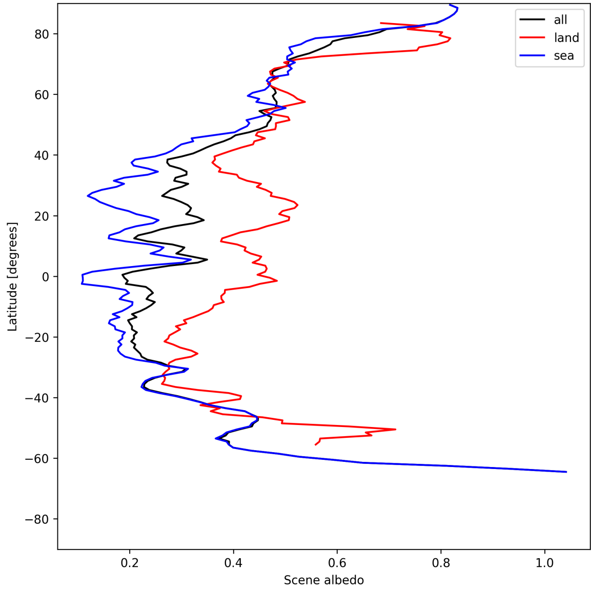
Figure 15: Zonal average of “Scene albedo” for 2025-06-20 to 2025-06-20.
