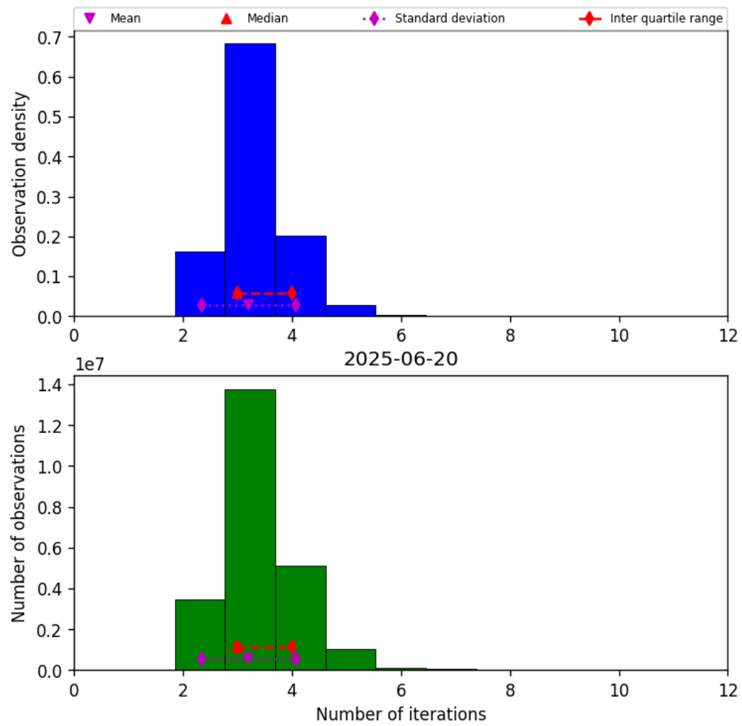
Figure 37: Histogram of “Number of iterations” for 2025-06-20 to 2025-06-20
