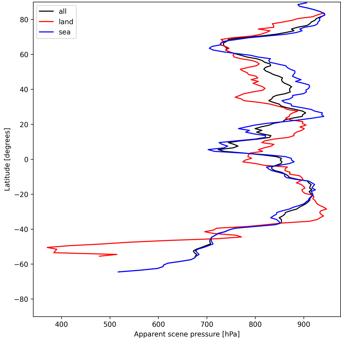
Figure 17: Zonal average of “Apparent scene pressure” for 2025-06-20 to 2025-06-20.
