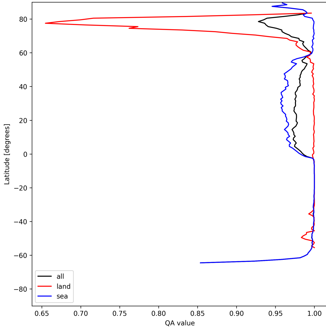
Figure 10: Zonal average of “QA value” for 2025-06-20 to 2025-06-20.
