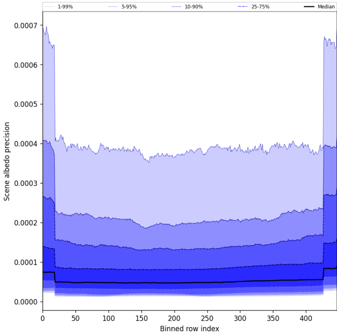
Figure 50: Along track statistics of “Scene albedo precision” for 2025-06-20 to 2025-06-20
