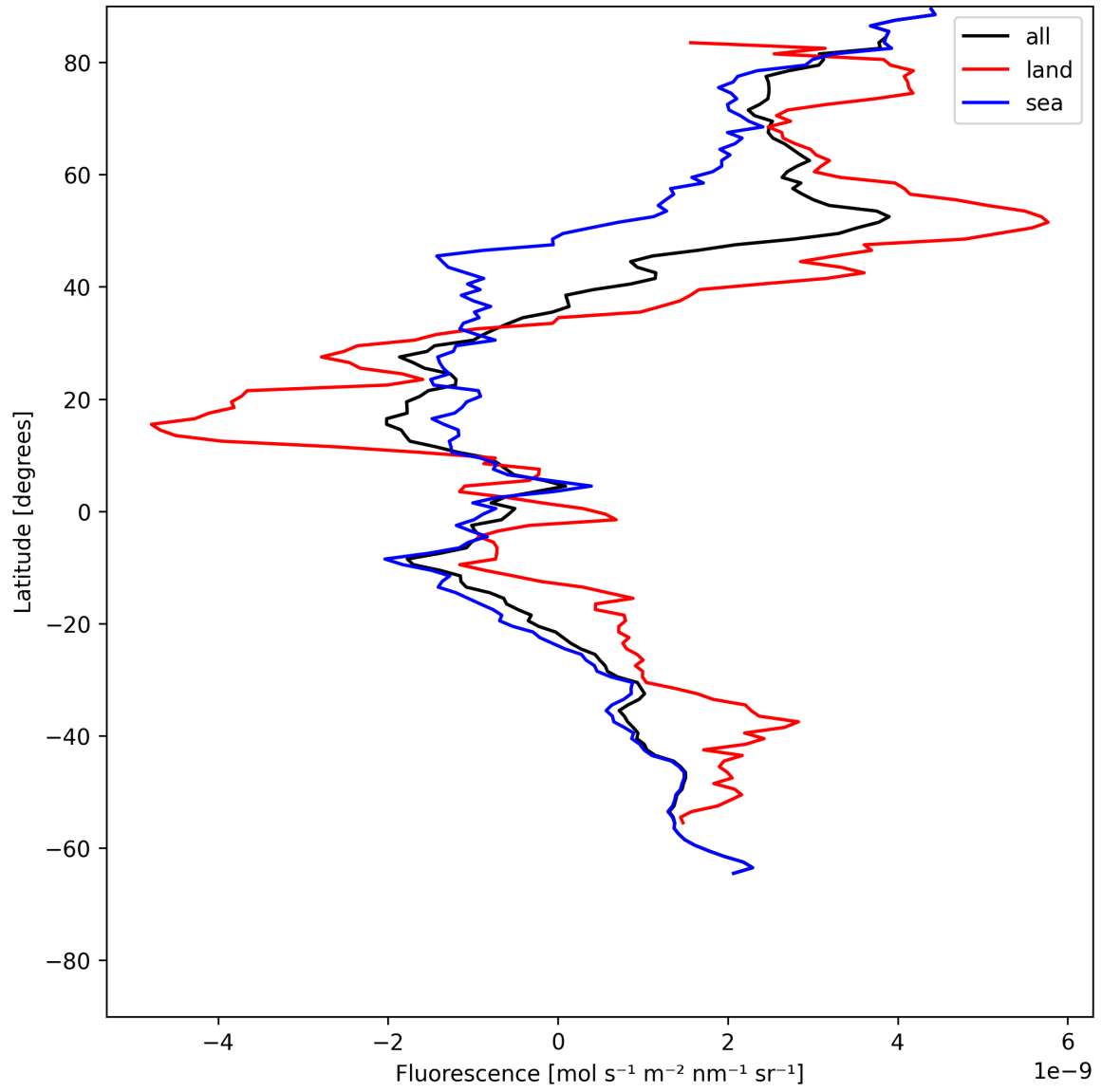
Figure 21: Zonal average of “Fluorescence” for 2025-06-20 to 2025-06-20.
