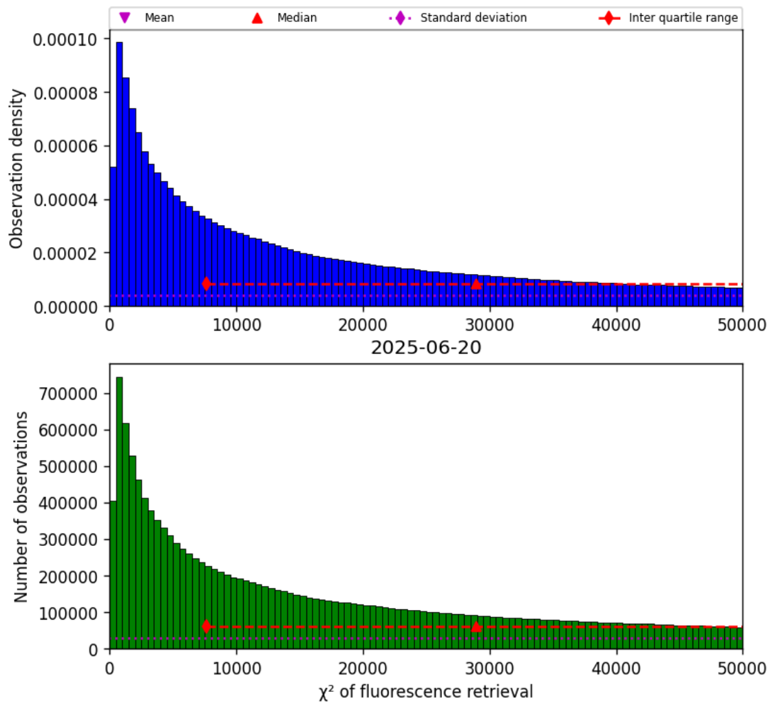
Figure 40: Histogram of “ \chi^2 of fluorescence retrieval” for 2025-06-20 to 2025-06-20
