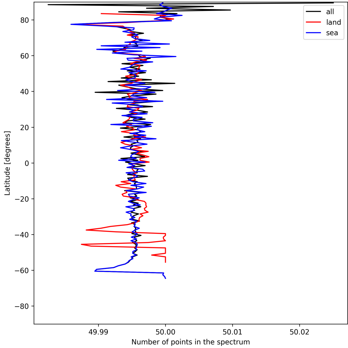
Figure 25: Zonal average of “Number of points in the spectrum” for 2025-06-20 to 2025-06-20.
