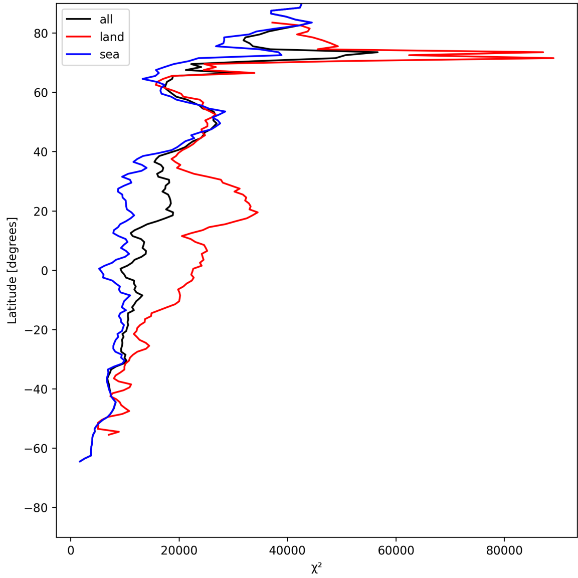
Figure 19: Zonal average of “ \chi^2 ” for 2025-06-20 to 2025-06-20.
