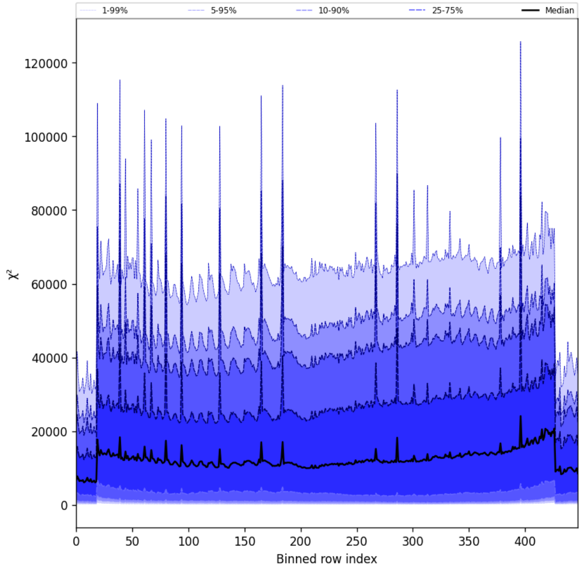
Figure 53: Along track statistics of “ \chi^2 ” for 2025-06-20 to 2025-06-20
