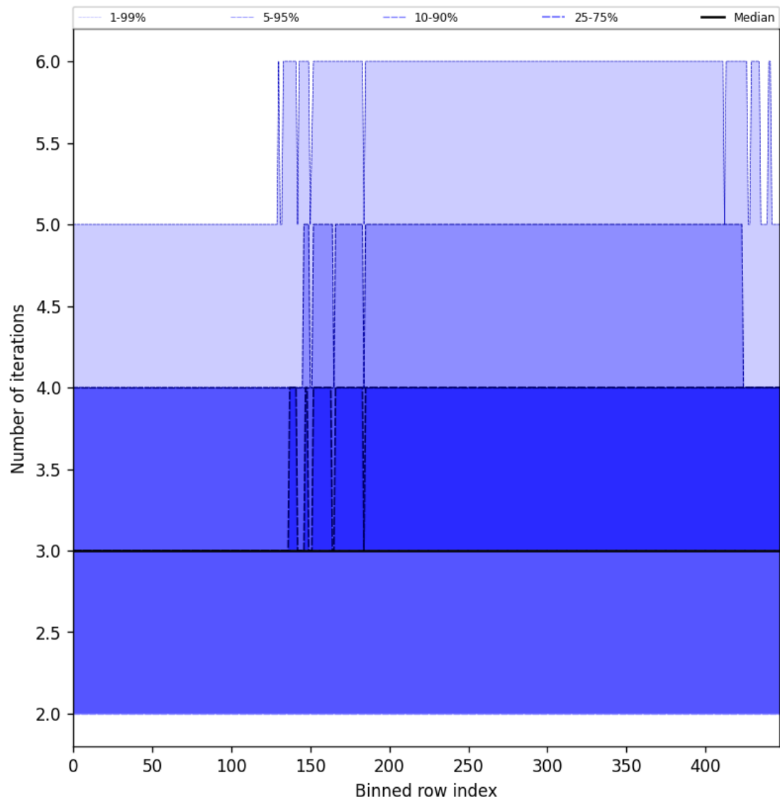
Figure 54: Along track statistics of “Number of iterations” for 2025-06-20 to 2025-06-20
