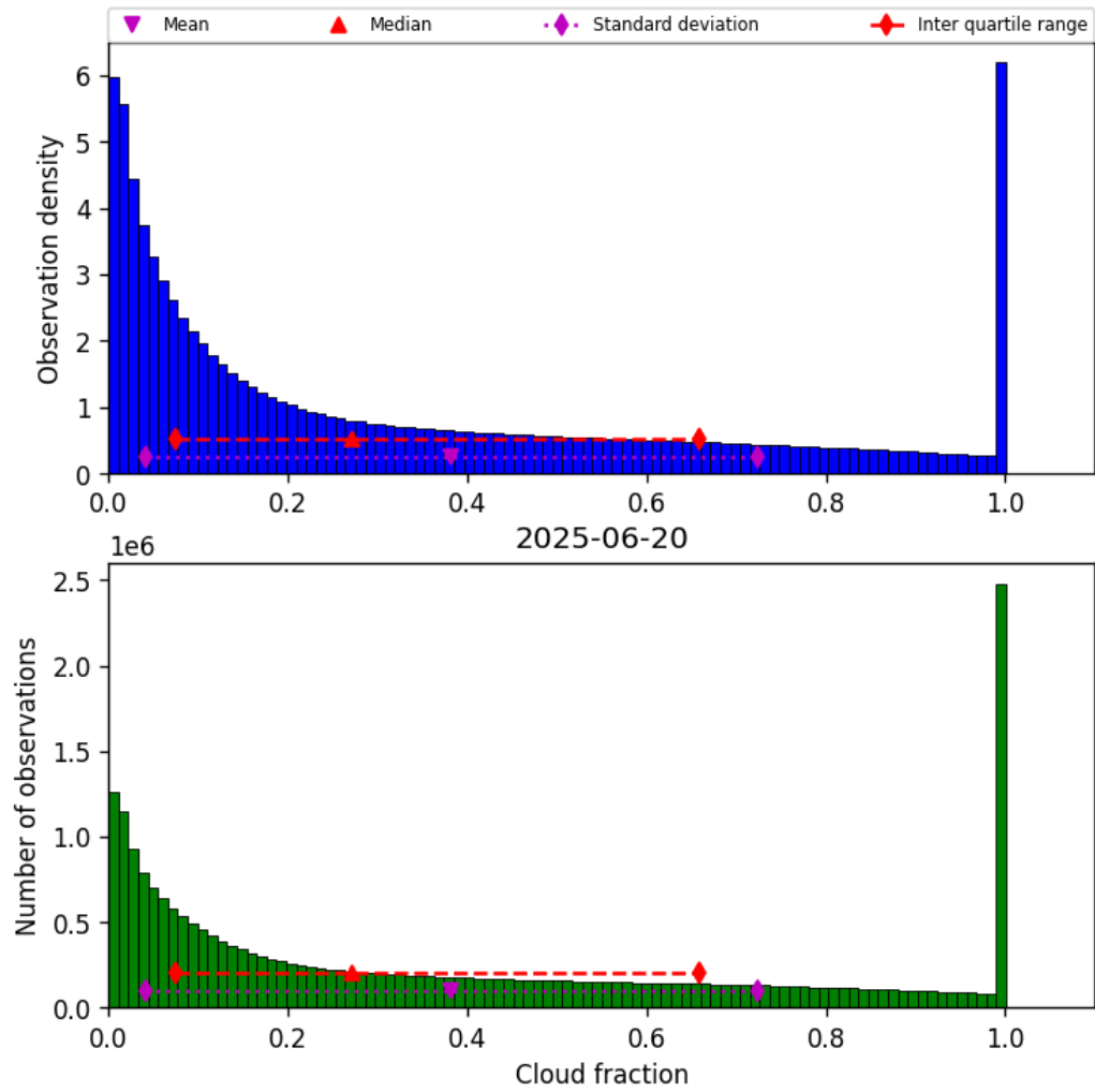
Figure 30: Histogram of “Cloud fraction” for 2025-06-20 to 2025-06-20
