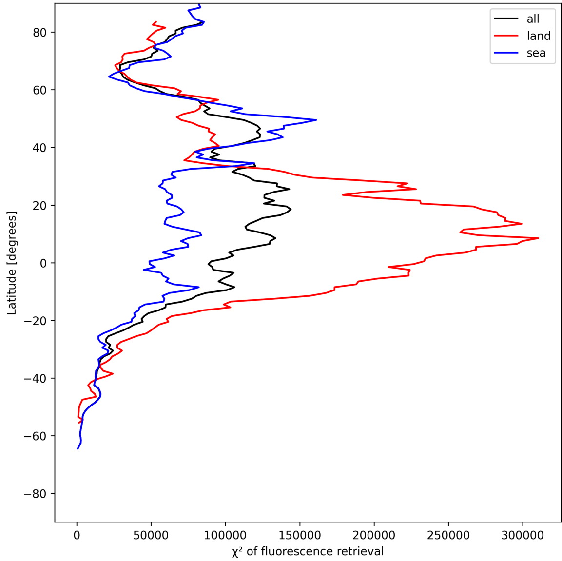
Figure 23: Zonal average of “ \chi^2 of fluorescence retrieval” for 2025-06-20 to 2025-06-20.
