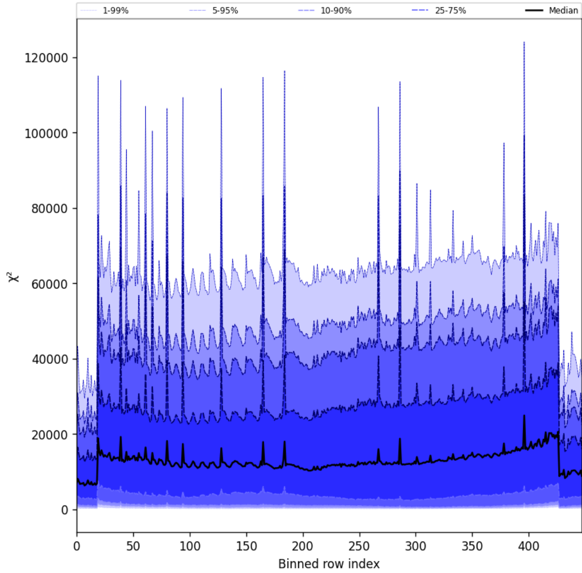
Figure 53: Along track statistics of “ \chi^2 ” for 2025-06-21 to 2025-06-22
