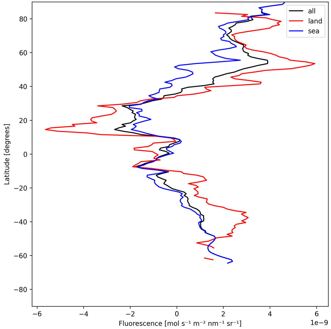
Figure 21: Zonal average of “Fluorescence” for 2025-06-21 to 2025-06-22.
