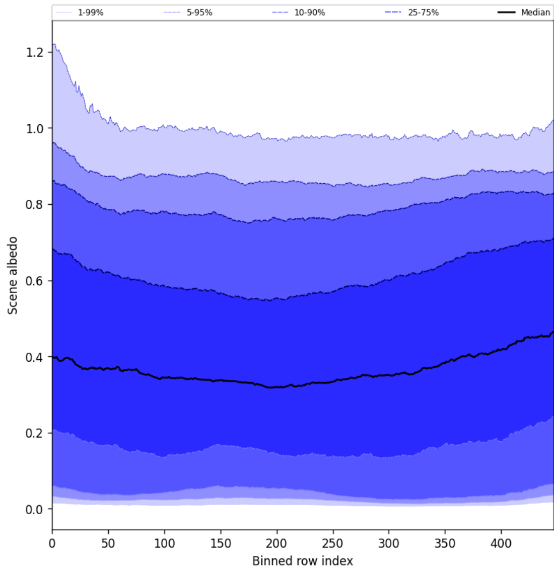
Figure 49: Along track statistics of “Scene albedo” for 2025-06-21 to 2025-06-22
