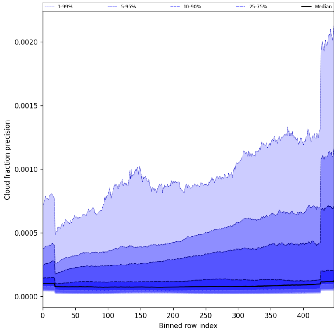
Figure 48: Along track statistics of “Cloud fraction precision” for 2025-06-21 to 2025-06-22
