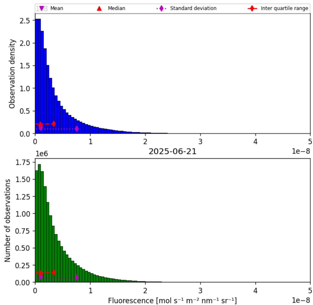
Figure 38: Histogram of “Fluorescence” for 2025-06-21 to 2025-06-22
