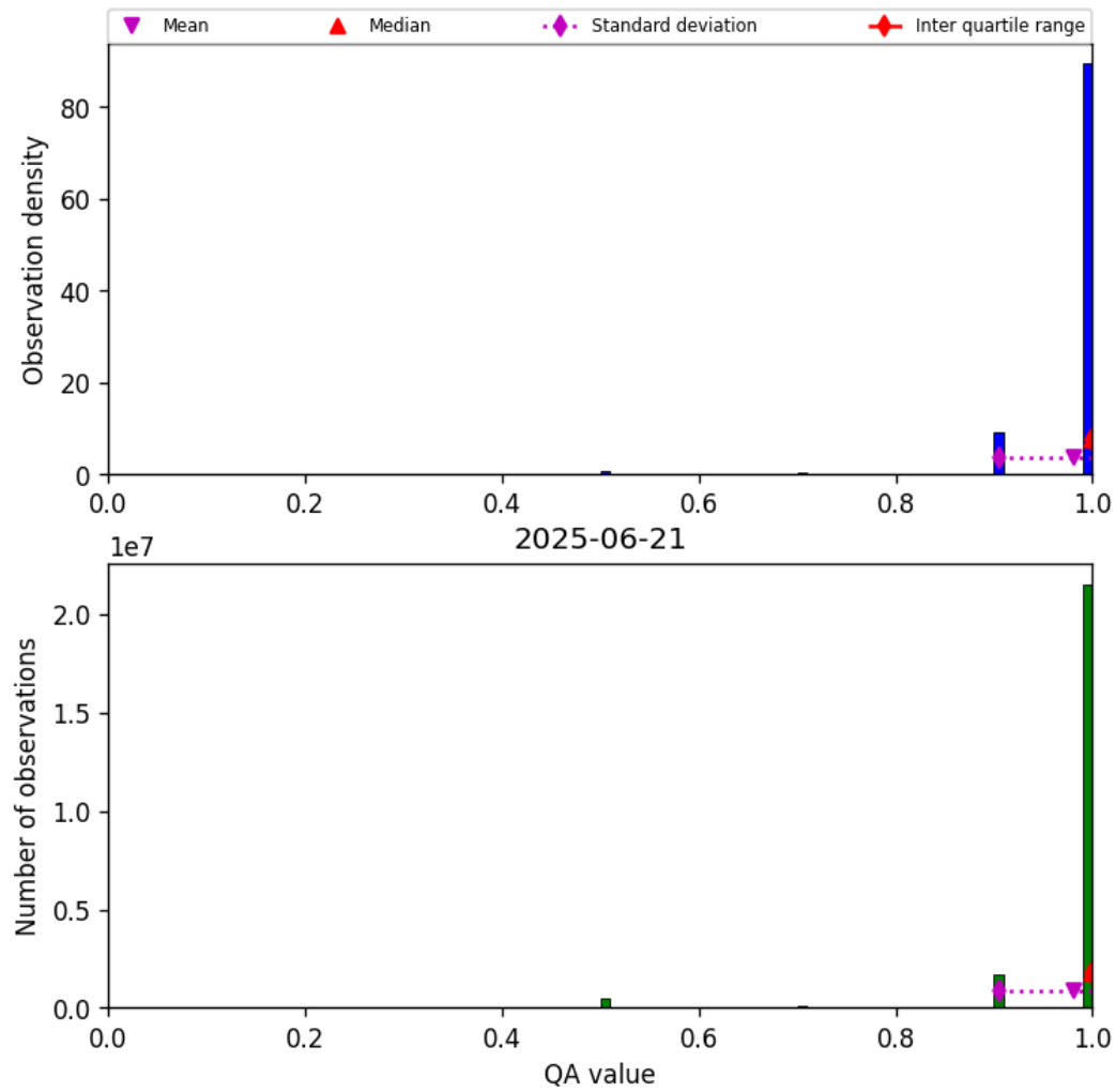
Figure 27: Histogram of “QA value” for 2025-06-21 to 2025-06-22
