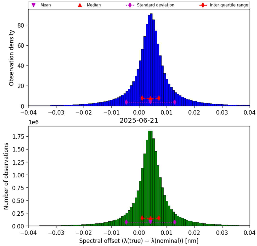
Figure 43: Histogram of “Spectral offset ( \lambda_{\text{true}} - \lambda_{\text{nominal}} )” for 2025-06-21 to 2025-06-22
