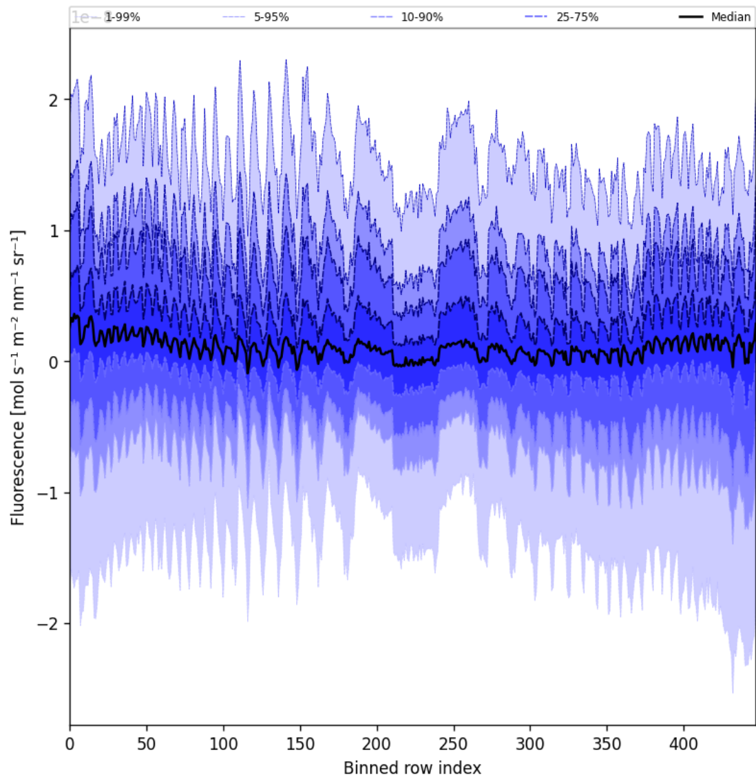
Figure 55: Along track statistics of “Fluorescence” for 2025-06-21 to 2025-06-22
