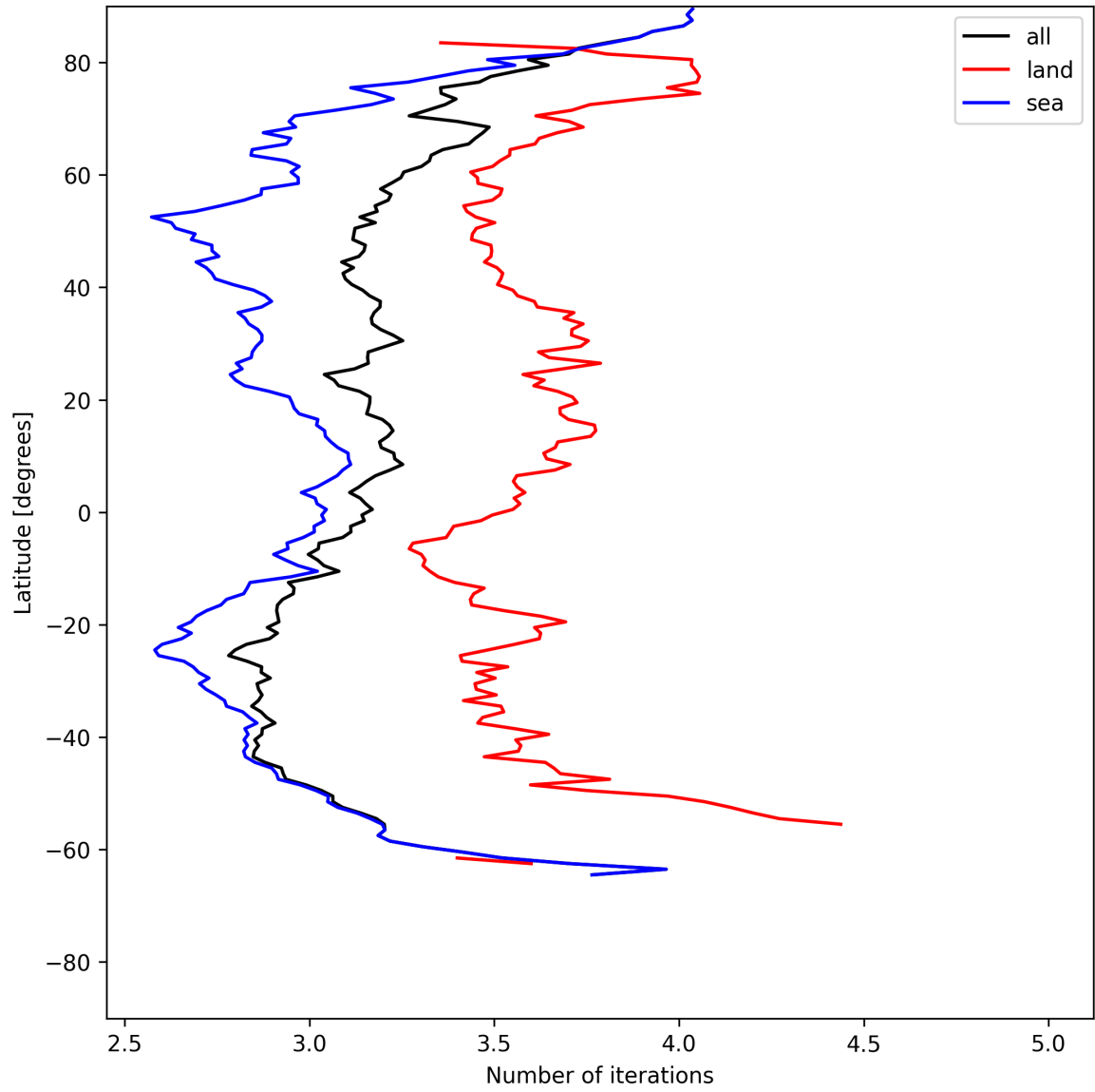
Figure 20: Zonal average of “Number of iterations” for 2025-06-21 to 2025-06-22.
