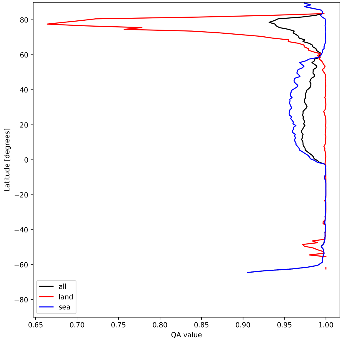
Figure 10: Zonal average of “QA value” for 2025-06-21 to 2025-06-22.
