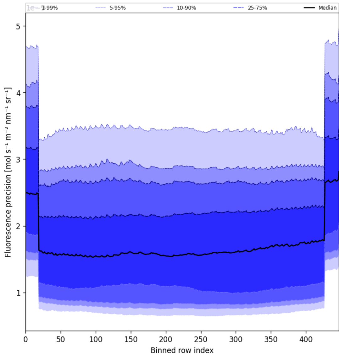
Figure 56: Along track statistics of “Fluorescence precision” for 2025-06-21 to 2025-06-22
