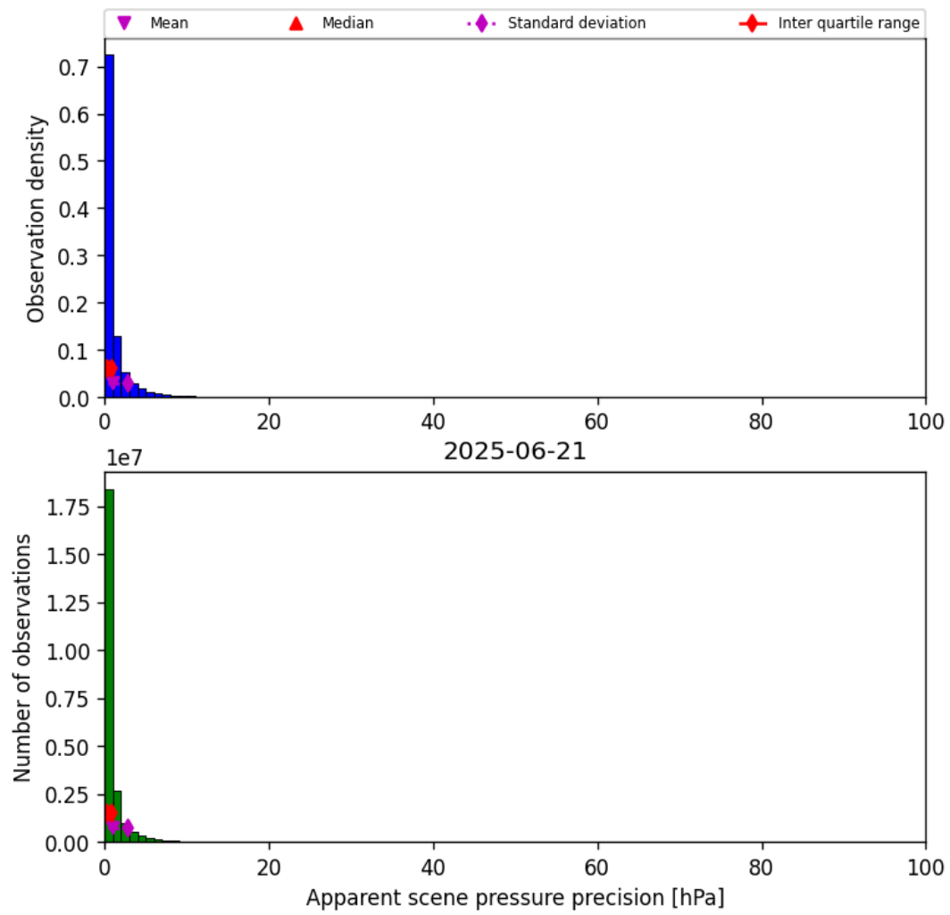
Figure 35: Histogram of “Apparent scene pressure precision” for 2025-06-21 to 2025-06-22
