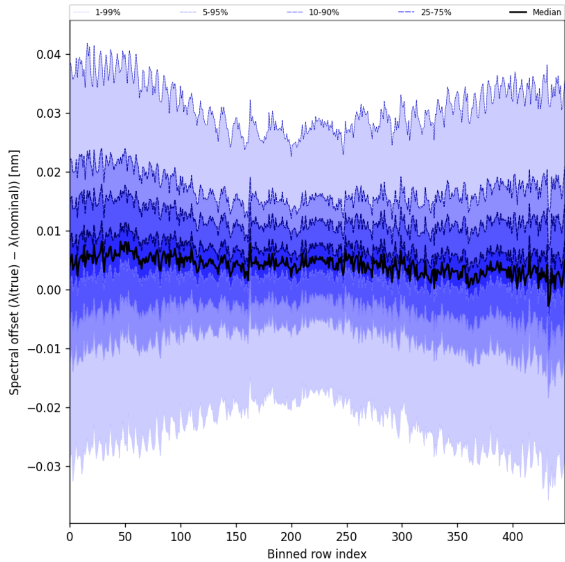
Figure 60: Along track statistics of “Spectral offset ( \lambda_{\text{true}} - \lambda_{\text{nominal}} )” for 2025-06-21 to 2025-06-22
