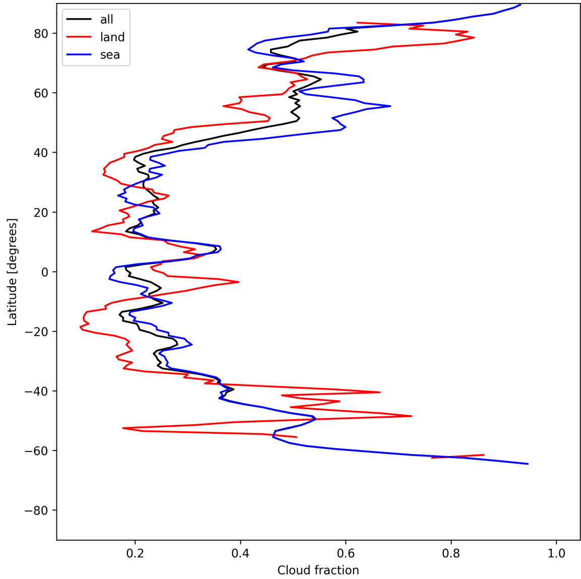
Figure 13: Zonal average of “Cloud fraction” for 2025-06-21 to 2025-06-22.
