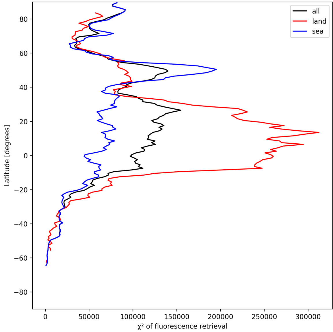
Figure 23: Zonal average of “ \chi^2 of fluorescence retrieval” for 2025-06-21 to 2025-06-22.
