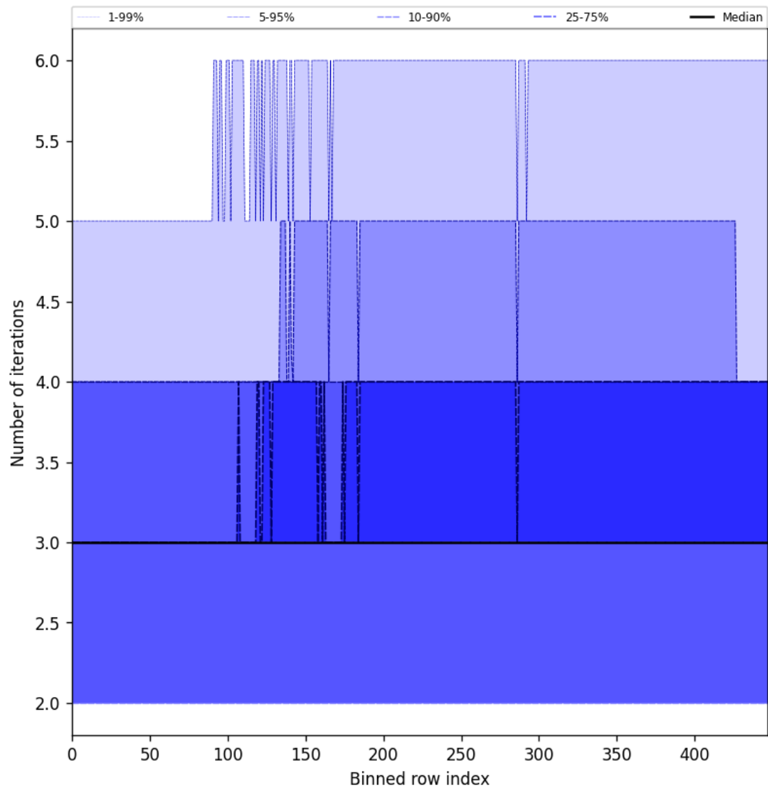
Figure 54: Along track statistics of “Number of iterations” for 2025-06-21 to 2025-06-22
