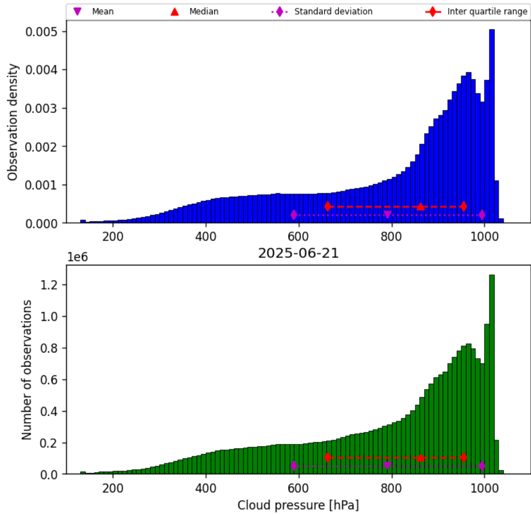
Figure 28: Histogram of “Cloud pressure” for 2025-06-21 to 2025-06-22
