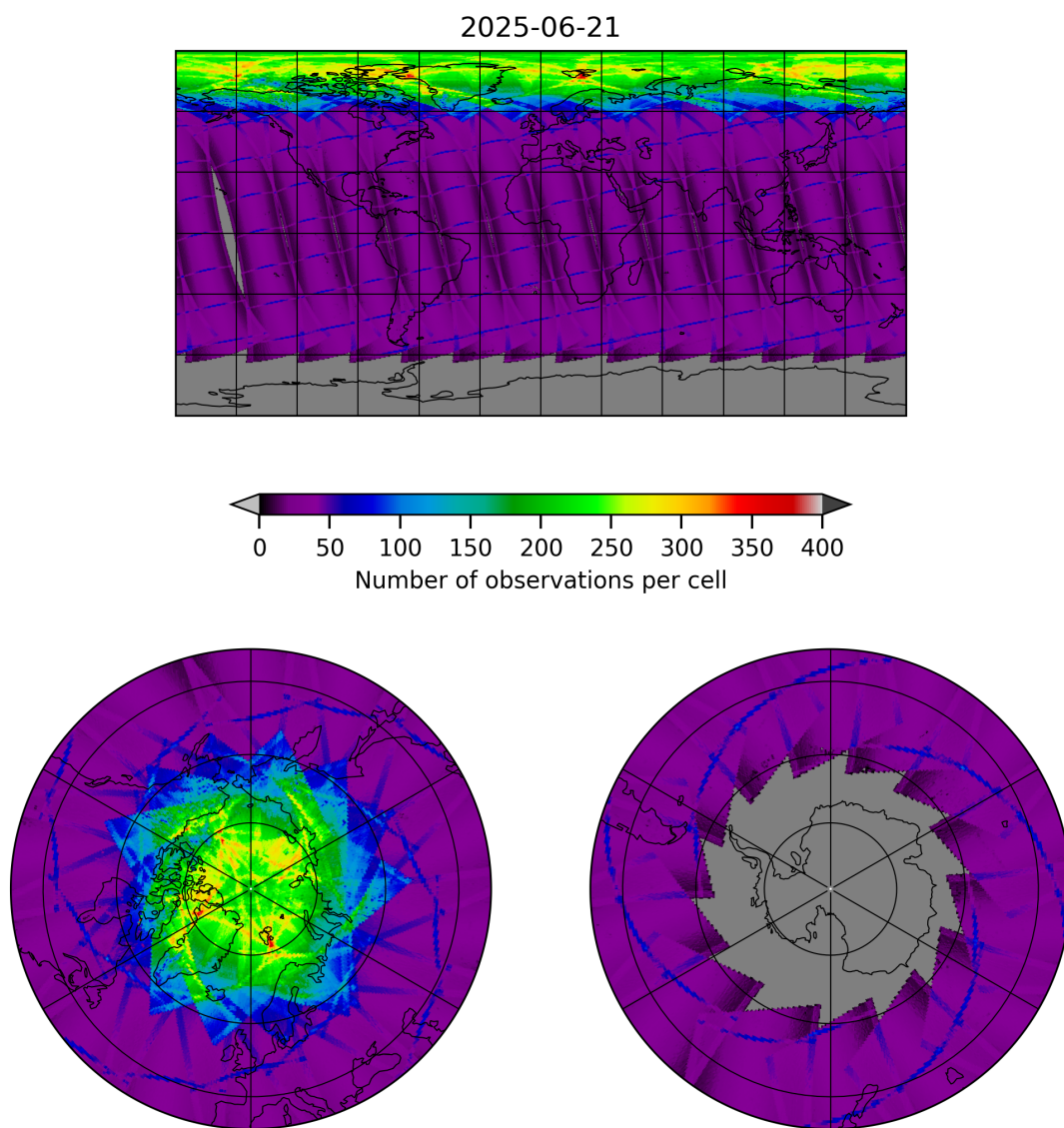
Figure 9: Map of the number of observations for 2025-06-21 to 2025-06-22
