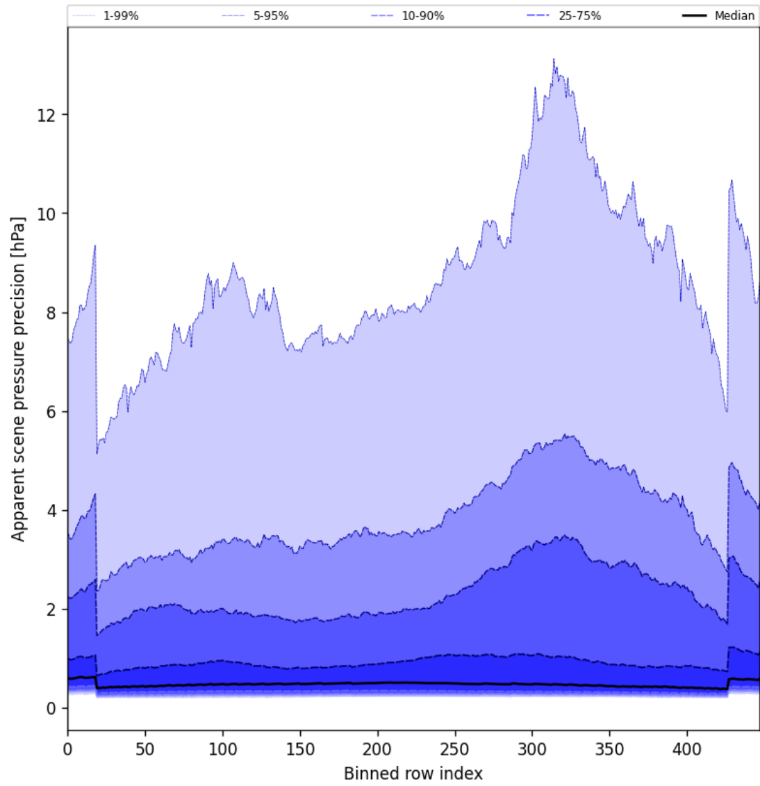
Figure 52: Along track statistics of “Apparent scene pressure precision” for 2025-06-21 to 2025-06-22
