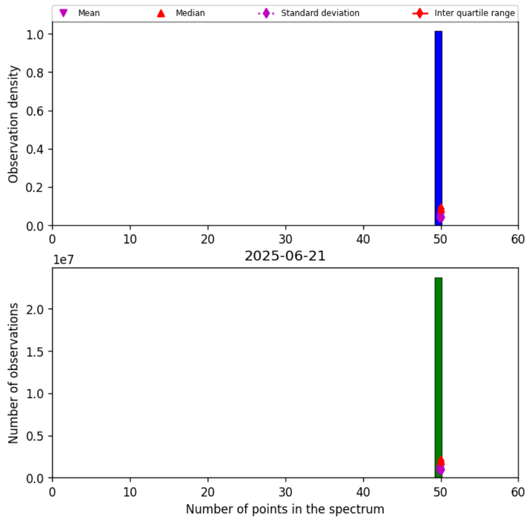
Figure 42: Histogram of “Number of points in the spectrum” for 2025-06-21 to 2025-06-22
