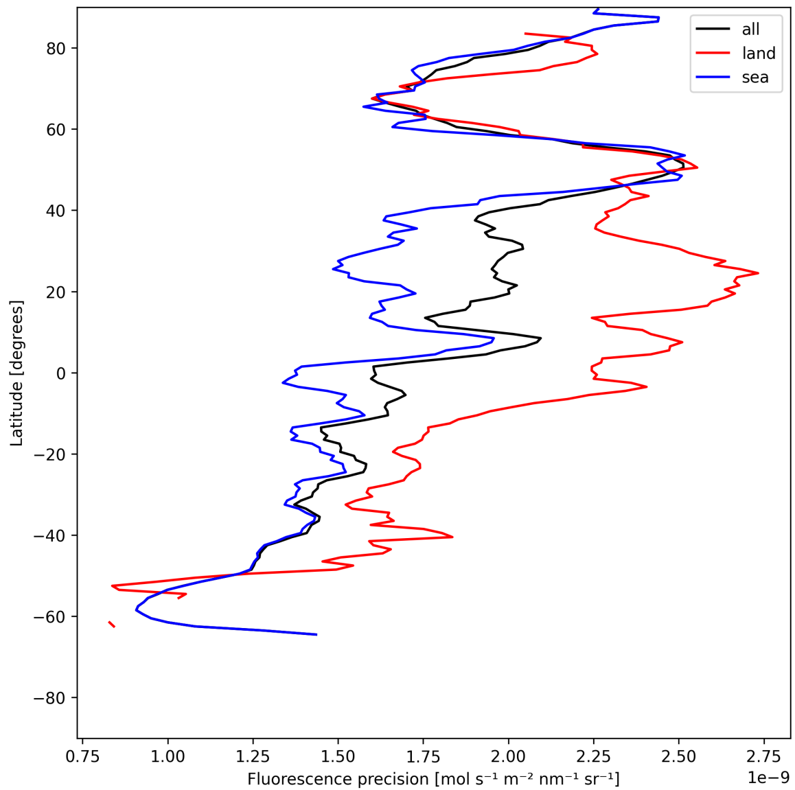
Figure 22: Zonal average of “Fluorescence precision” for 2025-06-21 to 2025-06-22.
