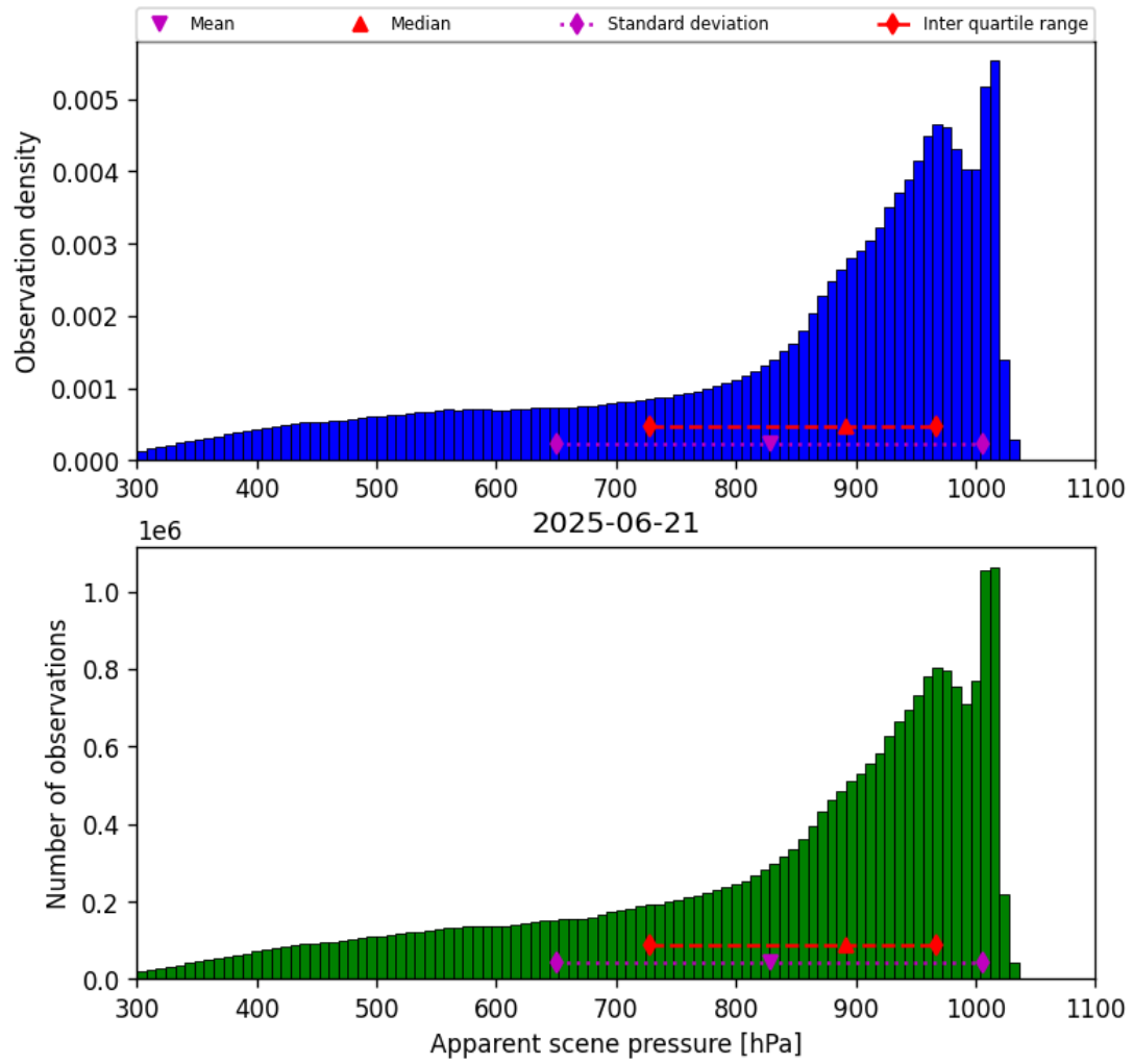
Figure 34: Histogram of “Apparent scene pressure” for 2025-06-21 to 2025-06-22
