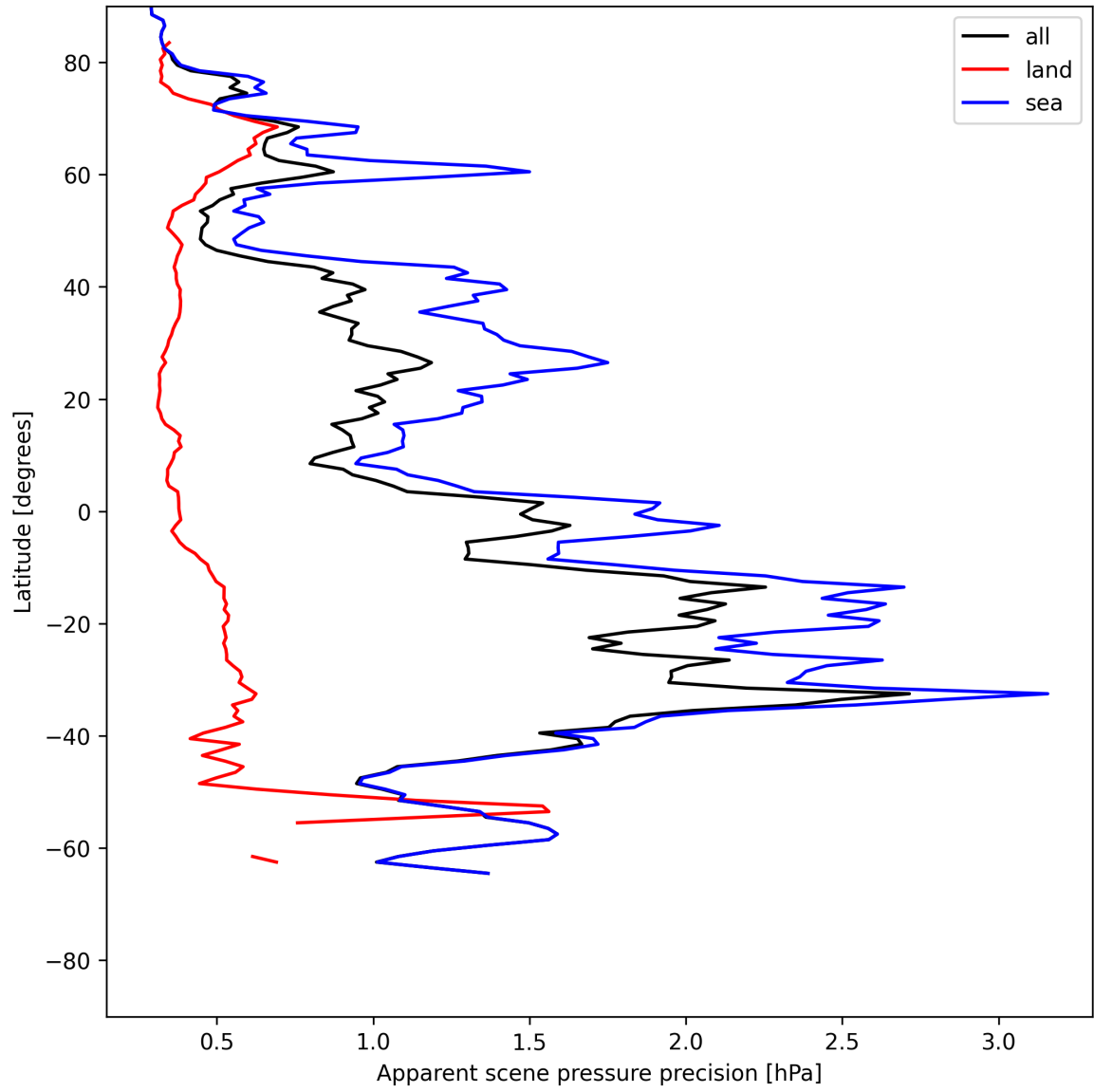
Figure 18: Zonal average of “Apparent scene pressure precision” for 2025-06-21 to 2025-06-22.
