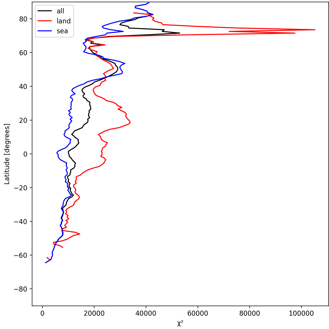
Figure 19: Zonal average of “ \chi^2 ” for 2025-06-21 to 2025-06-22.
