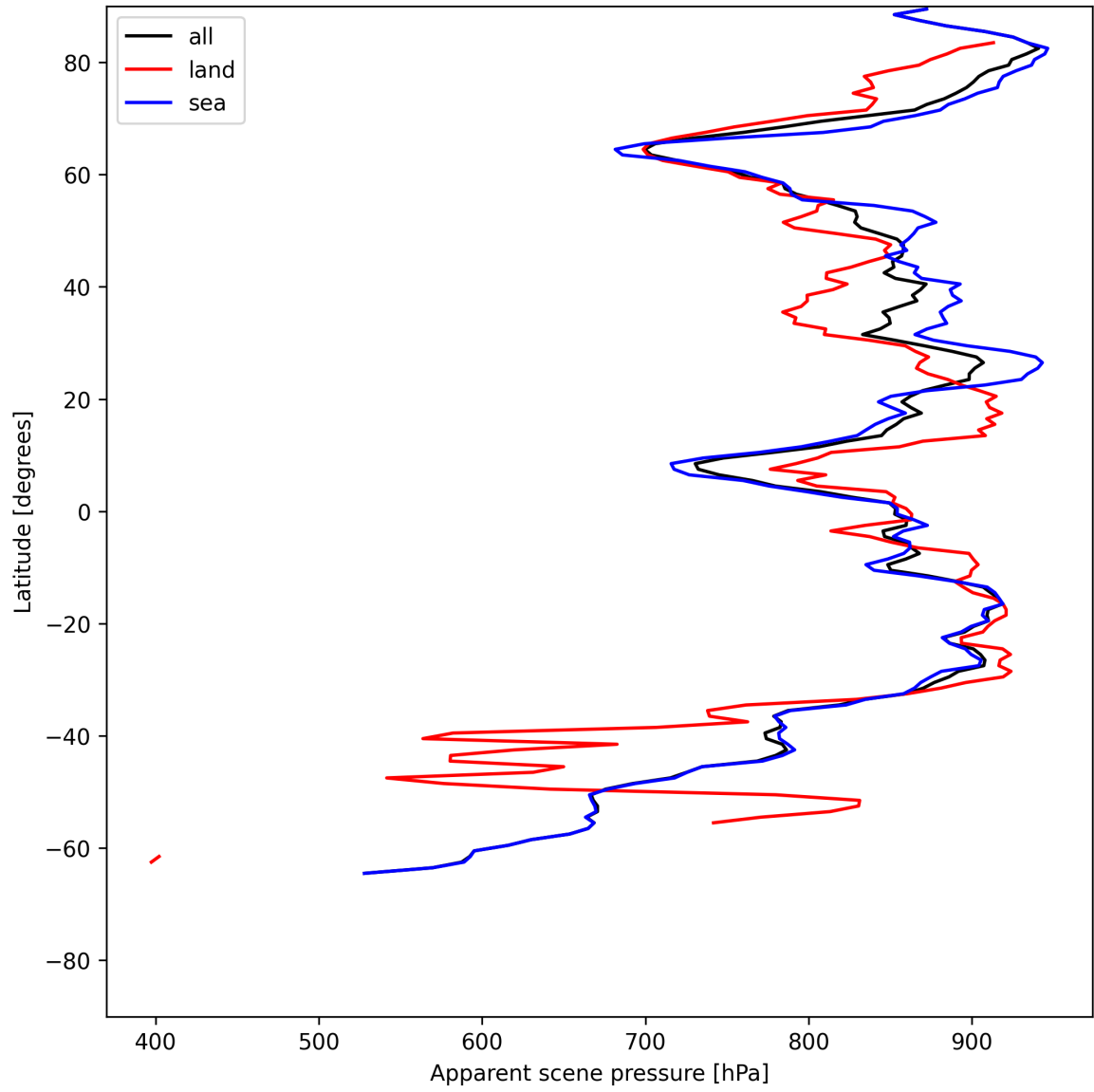
Figure 17: Zonal average of “Apparent scene pressure” for 2025-06-21 to 2025-06-22.
