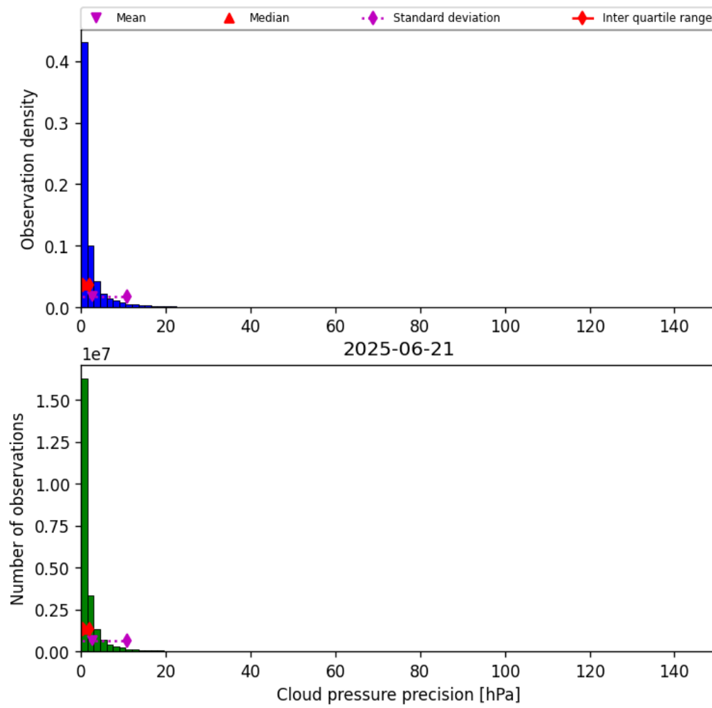
Figure 29: Histogram of “Cloud pressure precision” for 2025-06-21 to 2025-06-22
