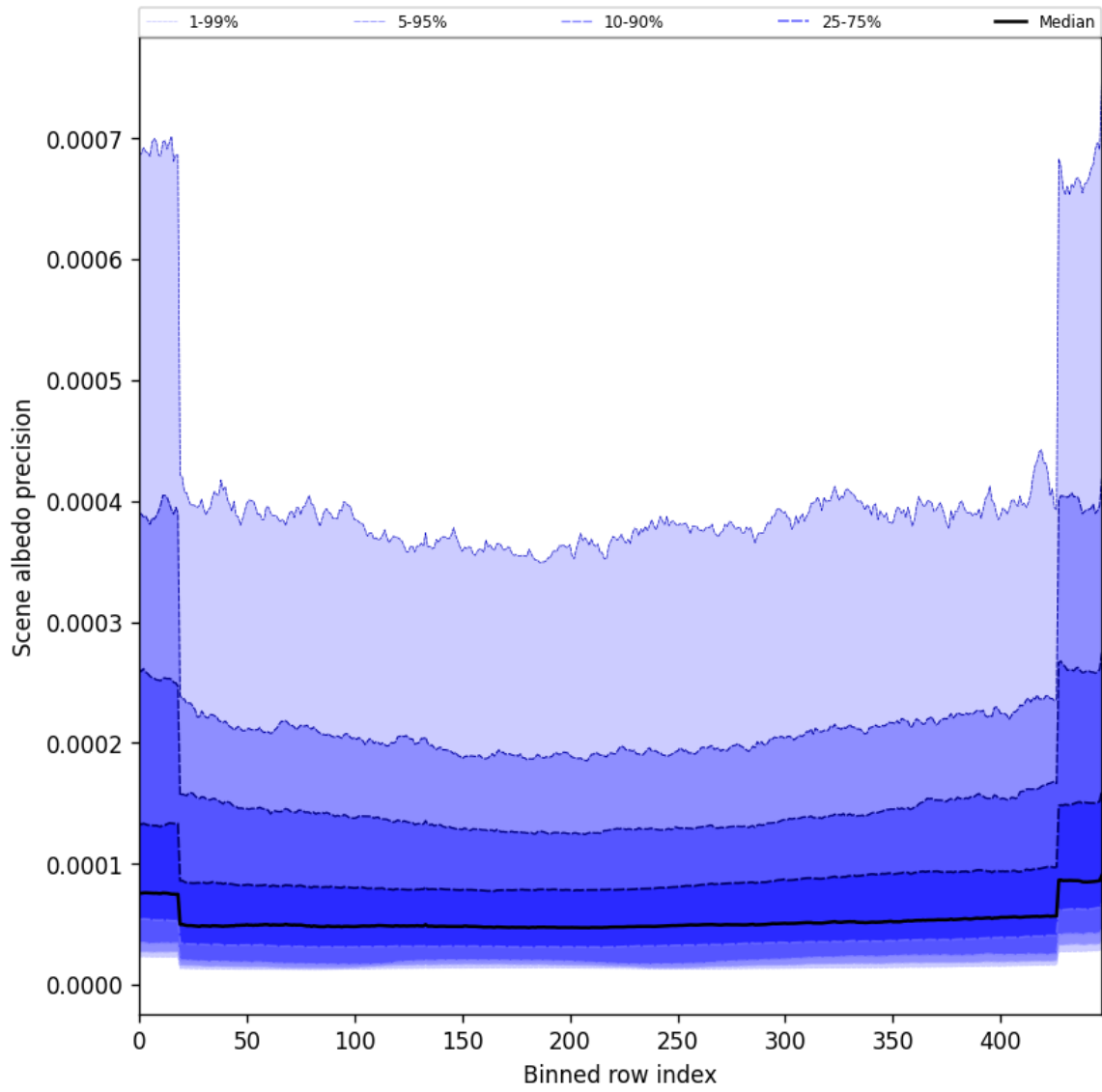
Figure 50: Along track statistics of “Scene albedo precision” for 2025-06-21 to 2025-06-22
