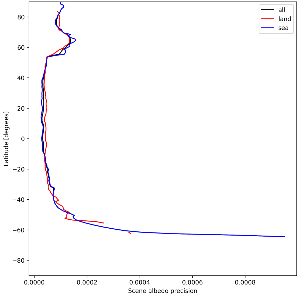
Figure 16: Zonal average of “Scene albedo precision” for 2025-06-21 to 2025-06-22.
