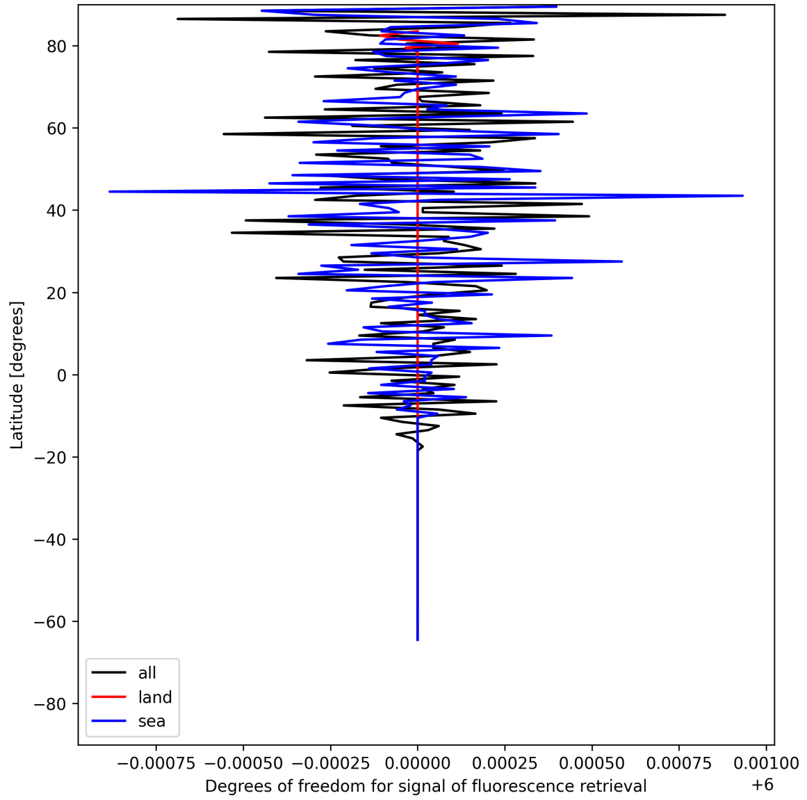
Figure 24: Zonal average of “Degrees of freedom for signal of fluorescence retrieval” for 2025-06-21 to 2025-06-22.
