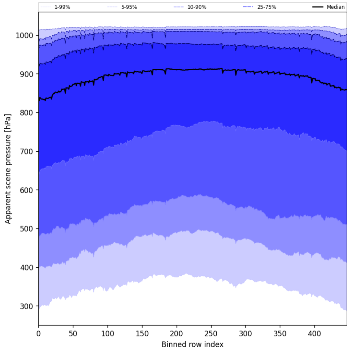
Figure 51: Along track statistics of “Apparent scene pressure” for 2025-06-21 to 2025-06-22
