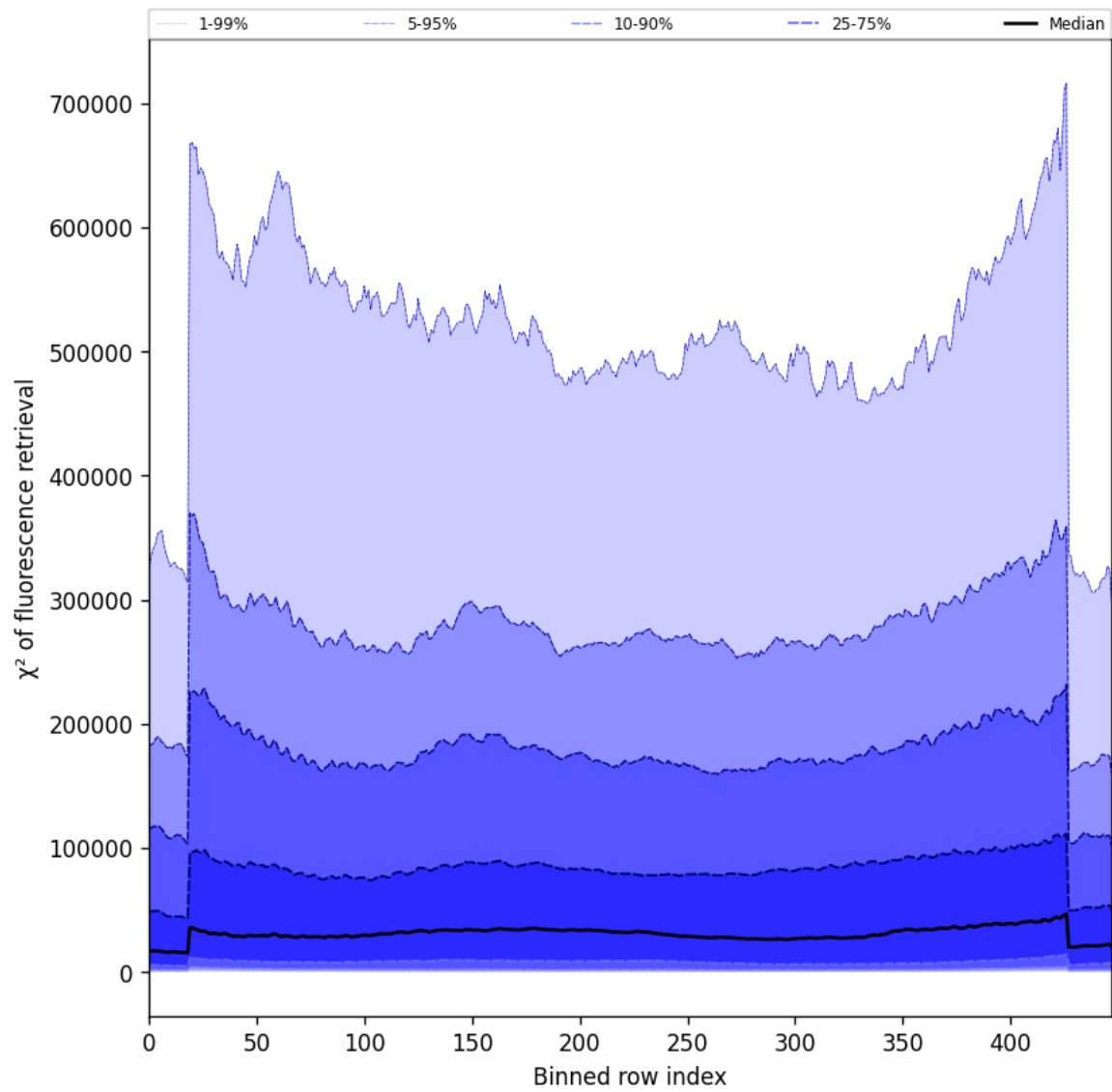
Figure 57: Along track statistics of “ \chi^2 of fluorescence retrieval” for 2025-06-21 to 2025-06-22
