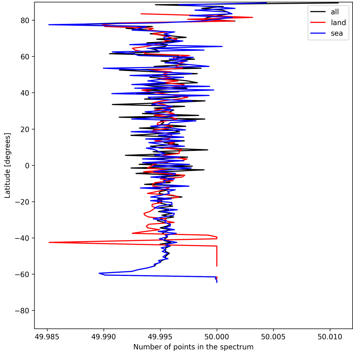
Figure 25: Zonal average of “Number of points in the spectrum” for 2025-06-21 to 2025-06-22.
