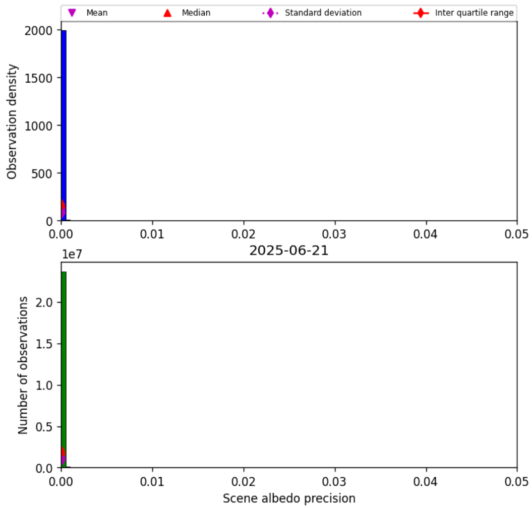
Figure 33: Histogram of “Scene albedo precision” for 2025-06-21 to 2025-06-22
