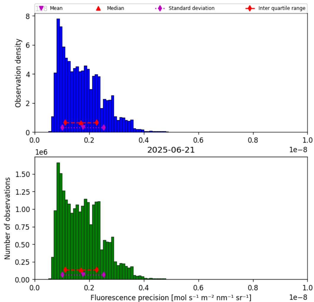
Figure 39: Histogram of “Fluorescence precision” for 2025-06-21 to 2025-06-22
