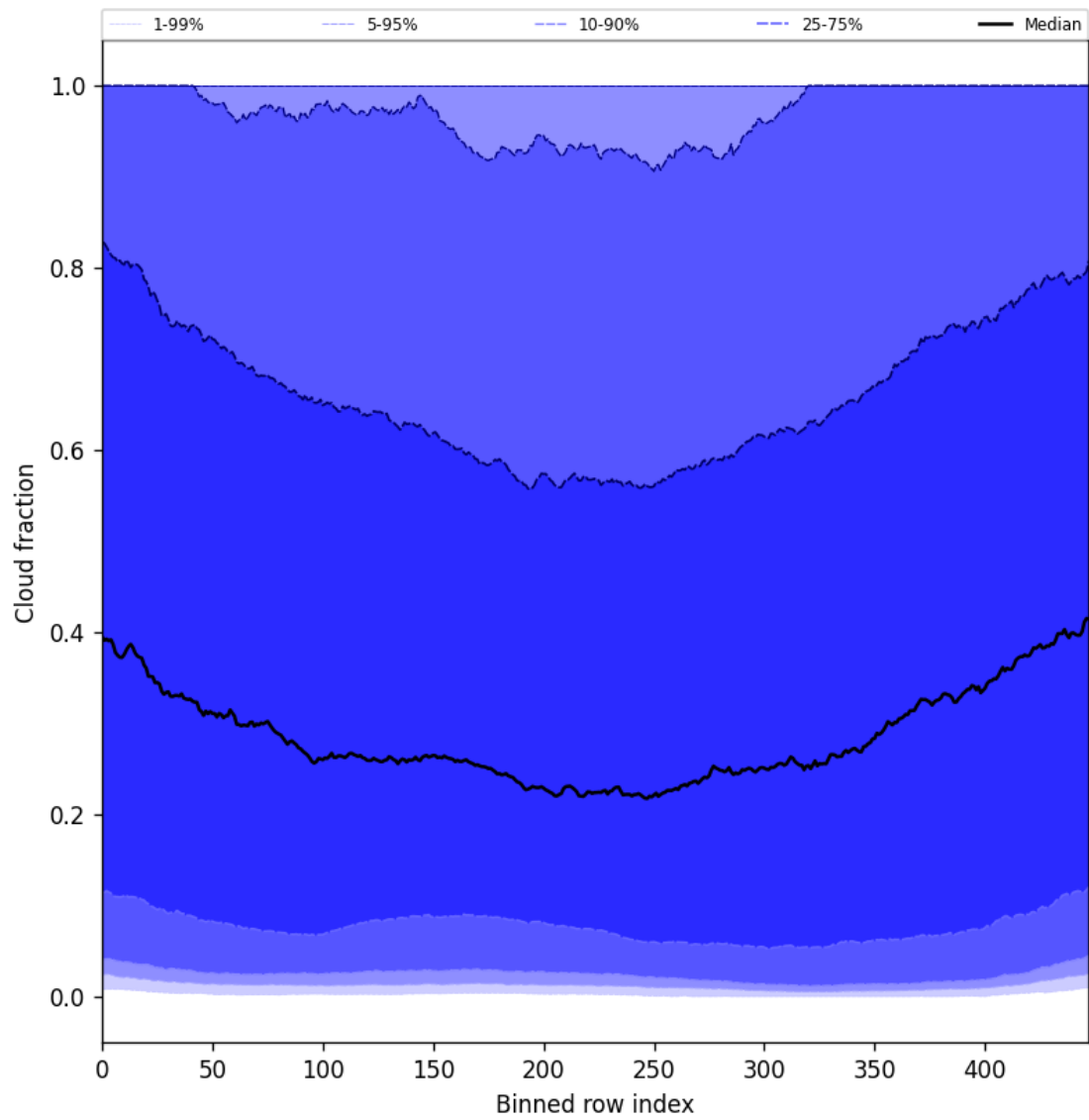
Figure 47: Along track statistics of “Cloud fraction” for 2025-06-21 to 2025-06-22
