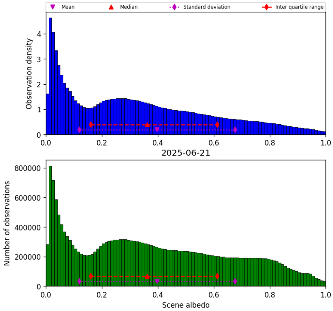
Figure 32: Histogram of “Scene albedo” for 2025-06-21 to 2025-06-22
