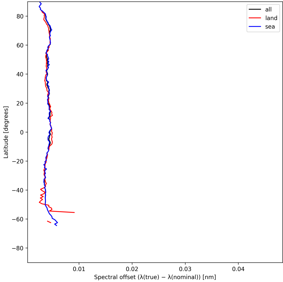
Figure 26: Zonal average of “Spectral offset ( \lambda_{\text{true}} - \lambda_{\text{nominal}} )” for 2025-06-21 to 2025-06-22.
