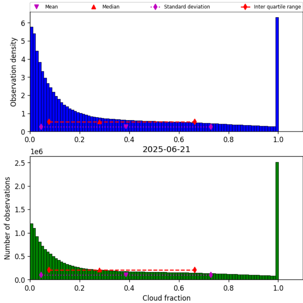
Figure 30: Histogram of “Cloud fraction” for 2025-06-21 to 2025-06-22
