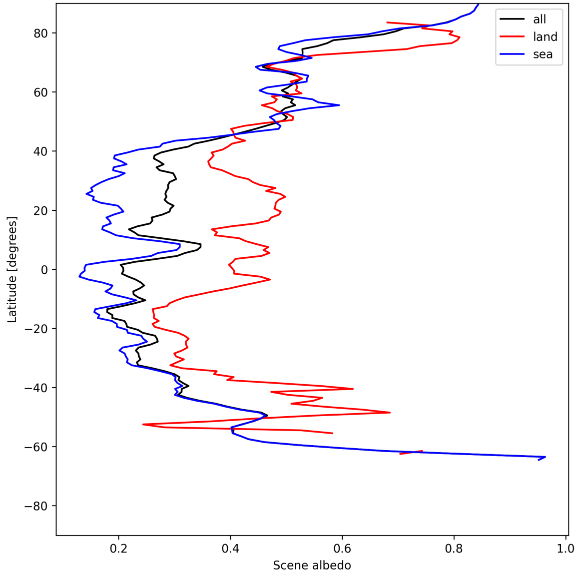
Figure 15: Zonal average of “Scene albedo” for 2025-06-21 to 2025-06-22.
