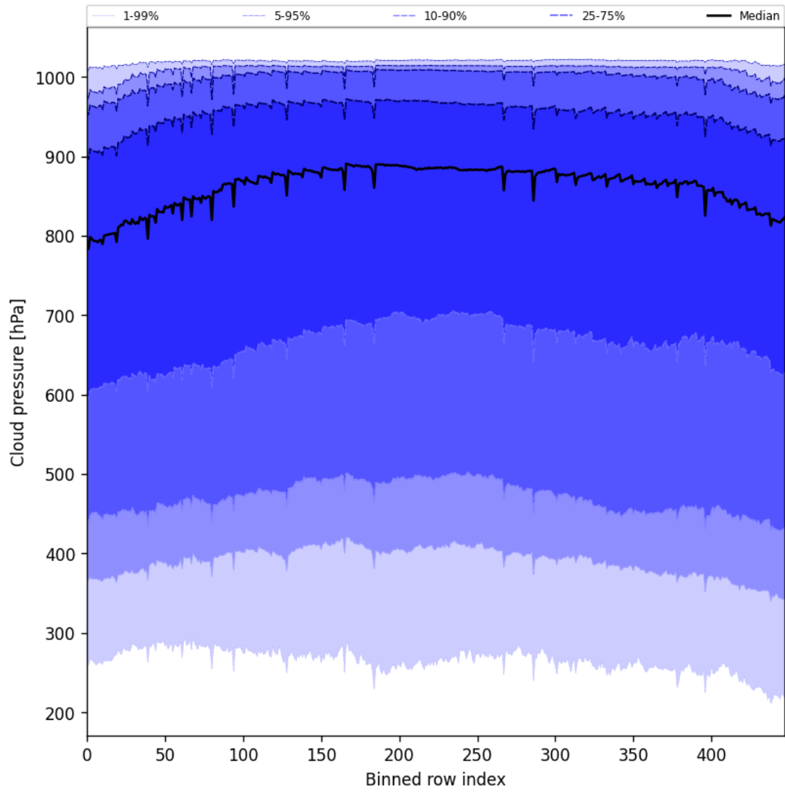
Figure 45: Along track statistics of “Cloud pressure” for 2025-06-21 to 2025-06-22
