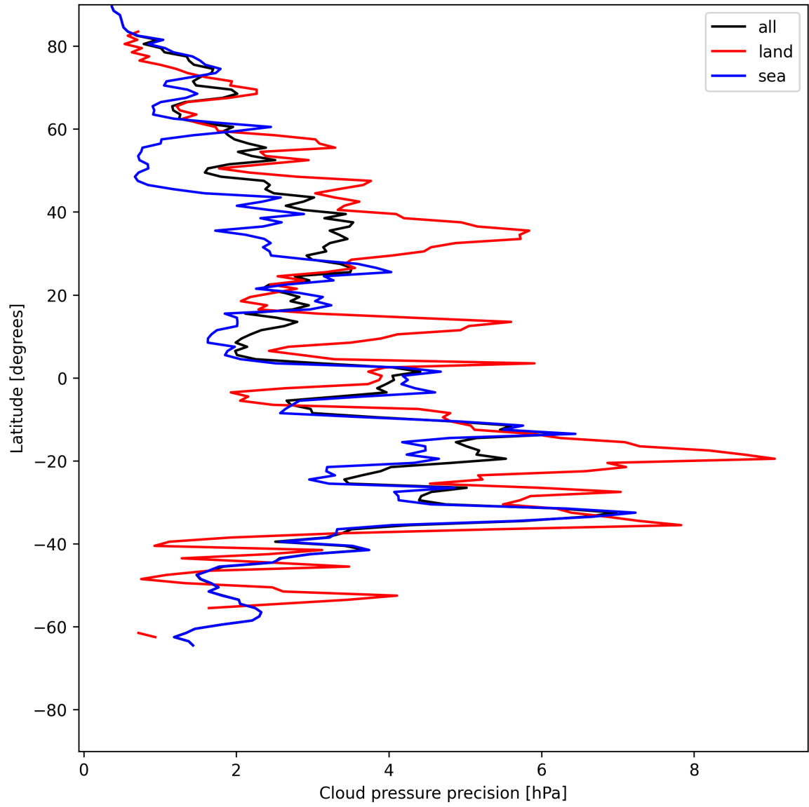
Figure 12: Zonal average of “Cloud pressure precision” for 2025-06-21 to 2025-06-22.
