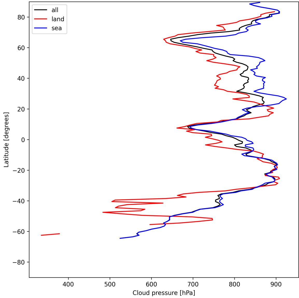
Figure 11: Zonal average of “Cloud pressure” for 2025-06-21 to 2025-06-22.
