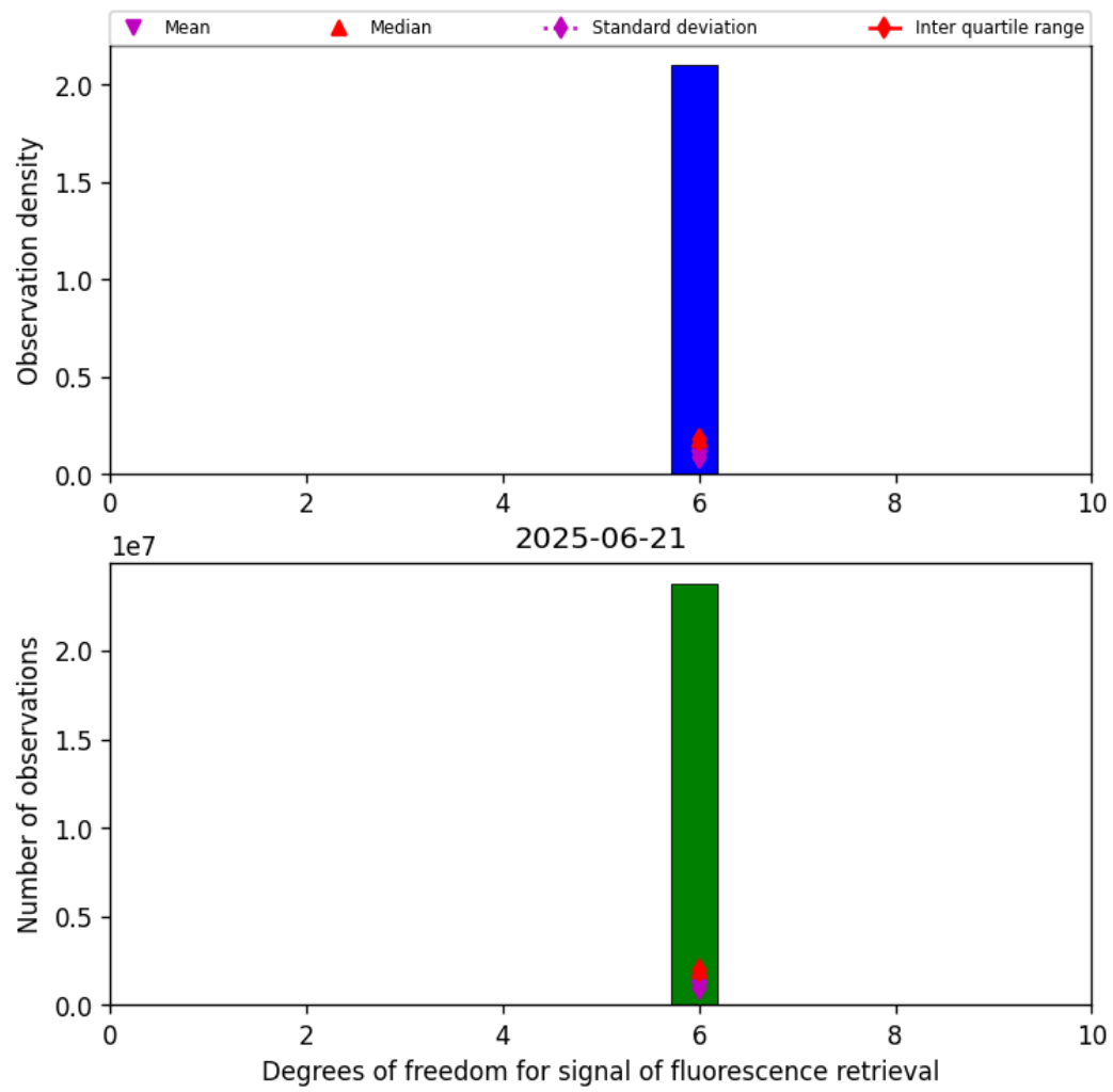
Figure 41: Histogram of “Degrees of freedom for signal of fluorescence retrieval” for 2025-06-21 to 2025-06-22
