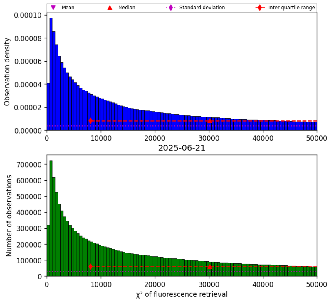
Figure 40: Histogram of “ \chi^2 of fluorescence retrieval” for 2025-06-21 to 2025-06-22
