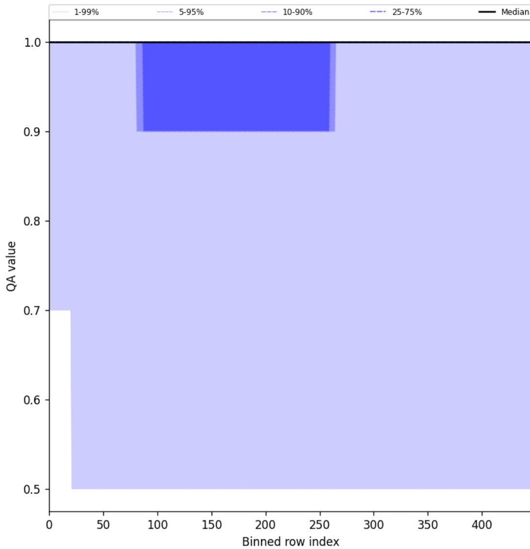
Figure 44: Along track statistics of “QA value” for 2025-06-21 to 2025-06-22
