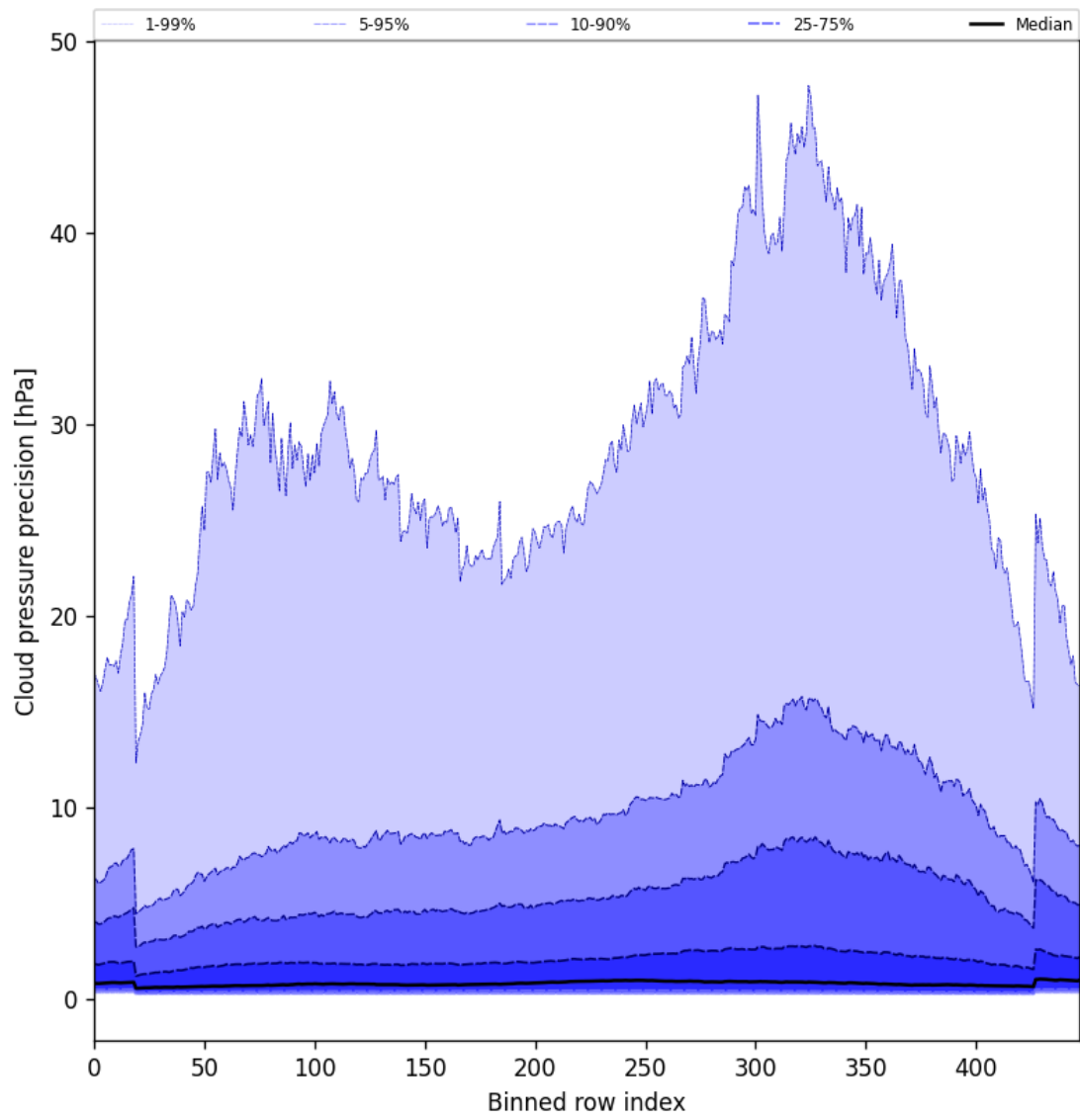
Figure 46: Along track statistics of “Cloud pressure precision” for 2025-06-21 to 2025-06-22
