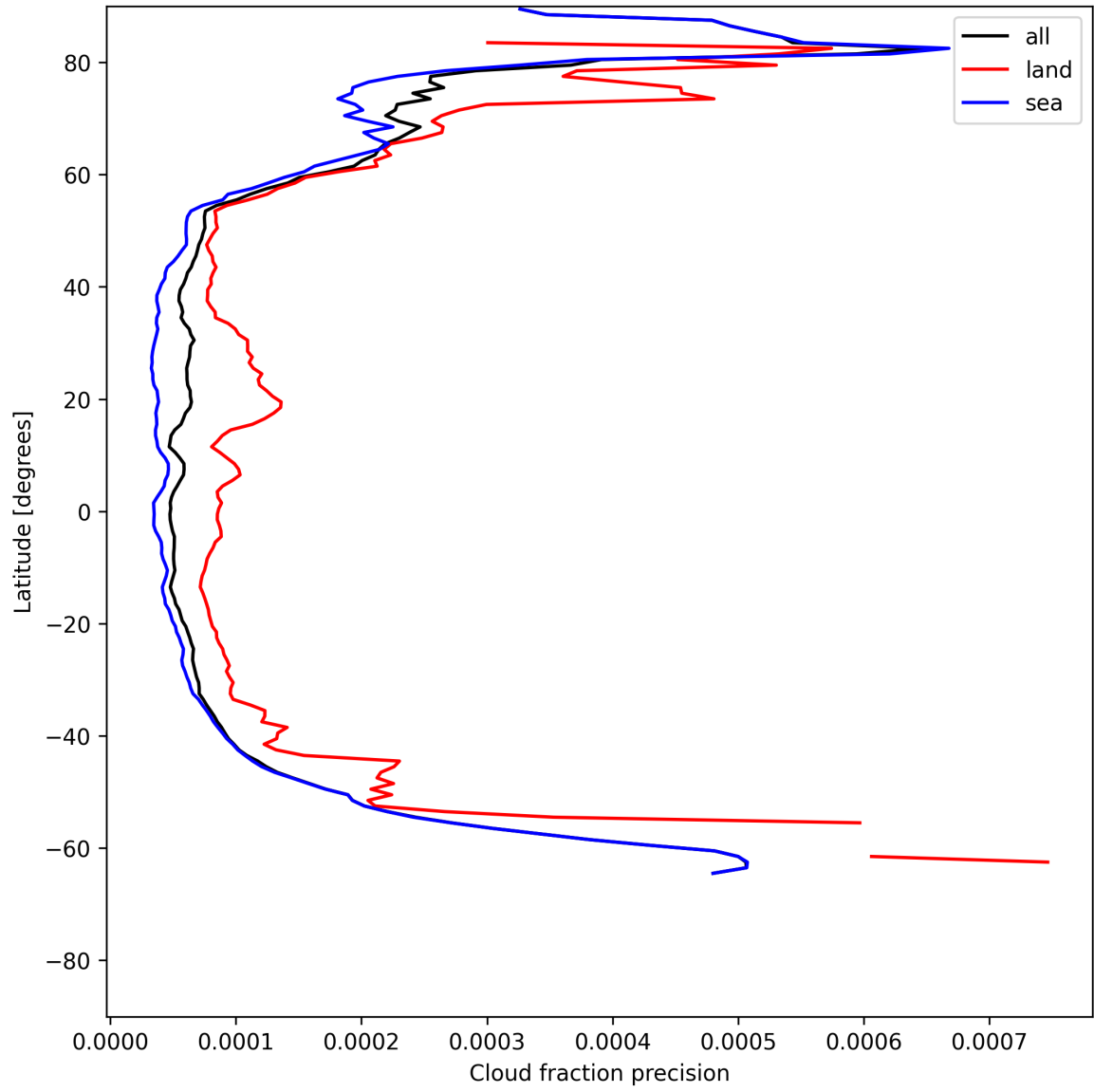
Figure 14: Zonal average of “Cloud fraction precision” for 2025-06-21 to 2025-06-22.
