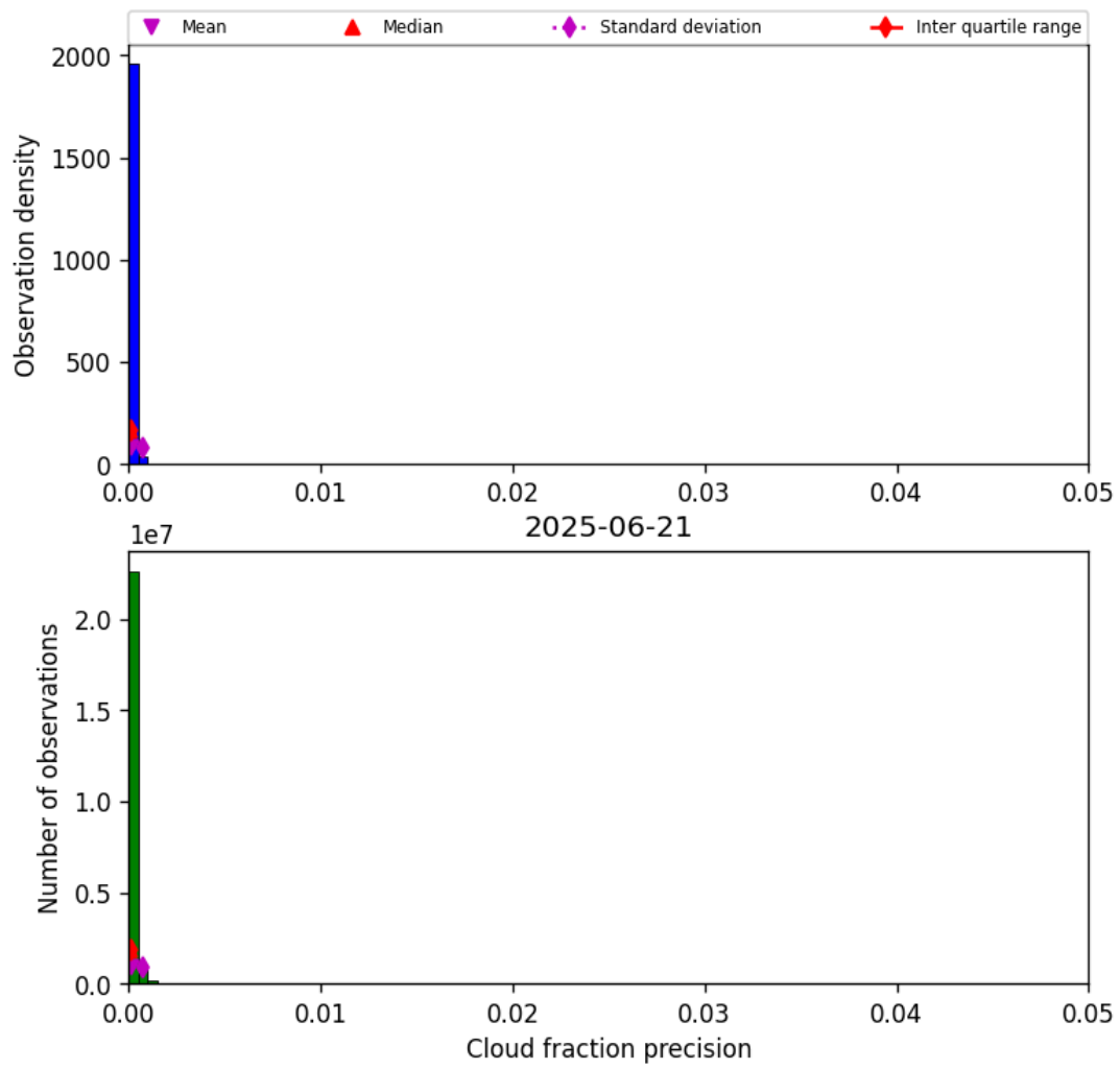
Figure 31: Histogram of “Cloud fraction precision” for 2025-06-21 to 2025-06-22
