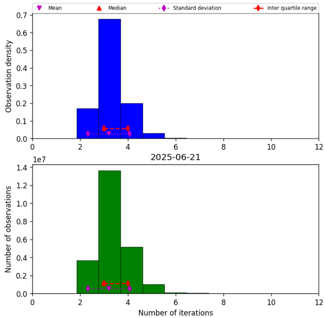
Figure 37: Histogram of “Number of iterations” for 2025-06-21 to 2025-06-22
