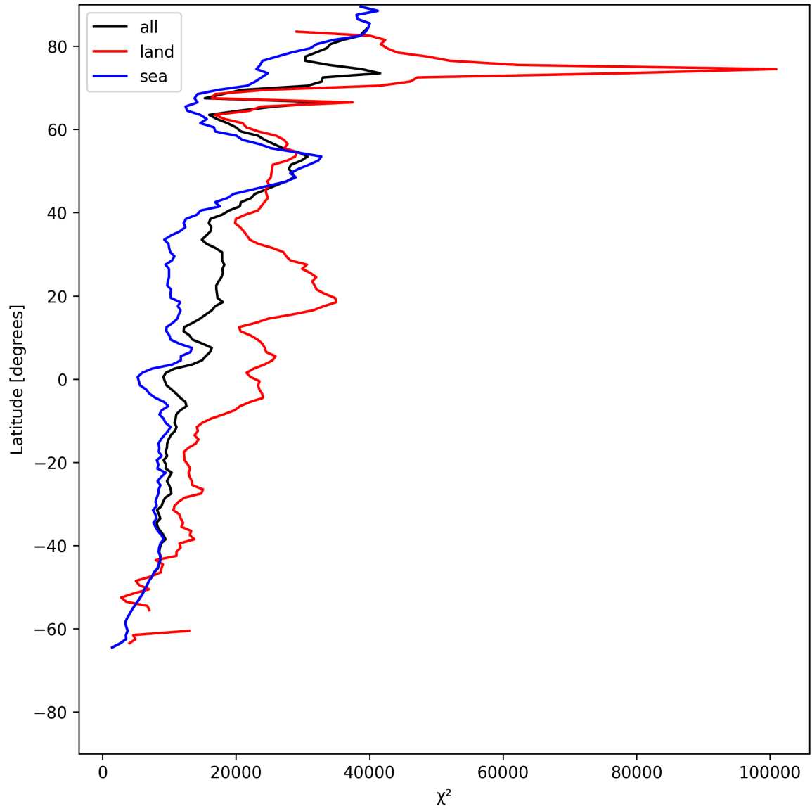
Figure 19: Zonal average of “ \chi^2 ” for 2025-06-22 to 2025-06-23.
