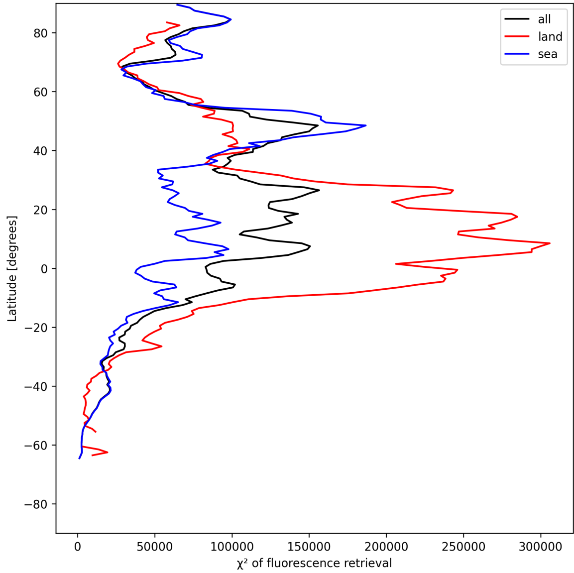
Figure 23: Zonal average of “ \chi^2 of fluorescence retrieval” for 2025-06-22 to 2025-06-23.
