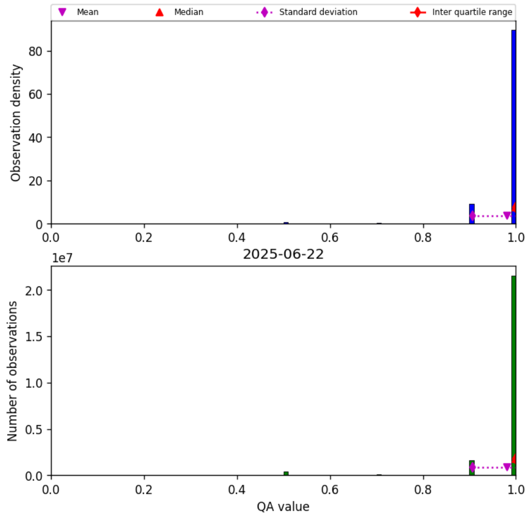
Figure 27: Histogram of “QA value” for 2025-06-22 to 2025-06-23
