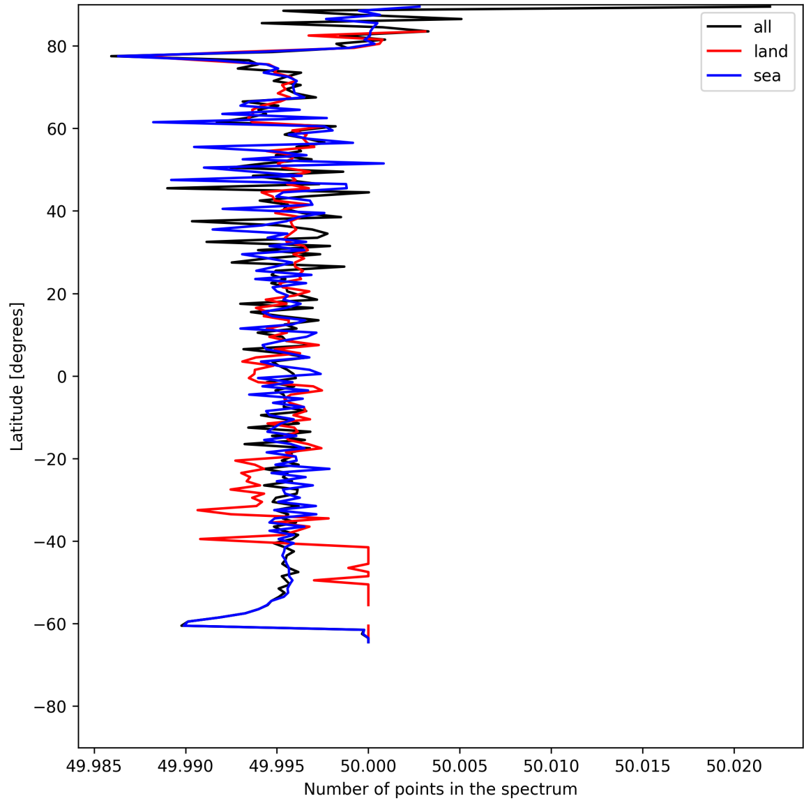
Figure 25: Zonal average of “Number of points in the spectrum” for 2025-06-22 to 2025-06-23.
