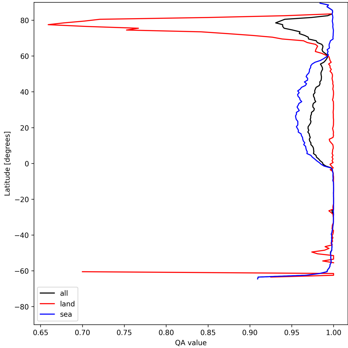
Figure 10: Zonal average of “QA value” for 2025-06-22 to 2025-06-23.
