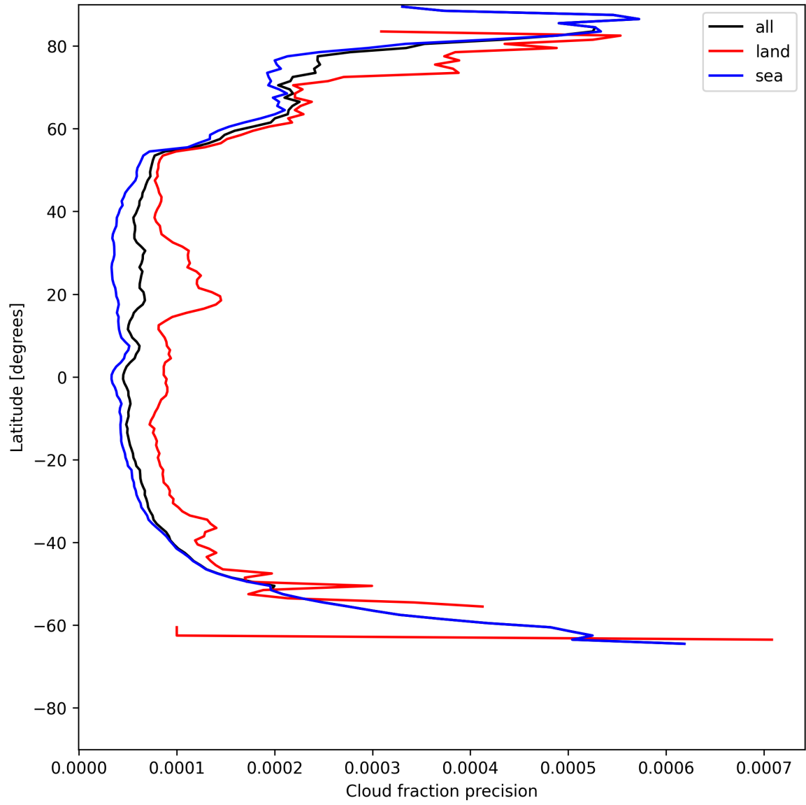
Figure 14: Zonal average of “Cloud fraction precision” for 2025-06-22 to 2025-06-23.
