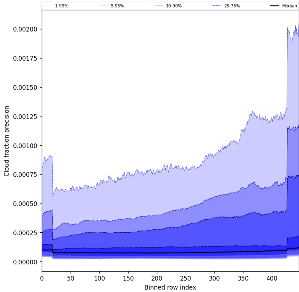
Figure 48: Along track statistics of “Cloud fraction precision” for 2025-06-22 to 2025-06-23
