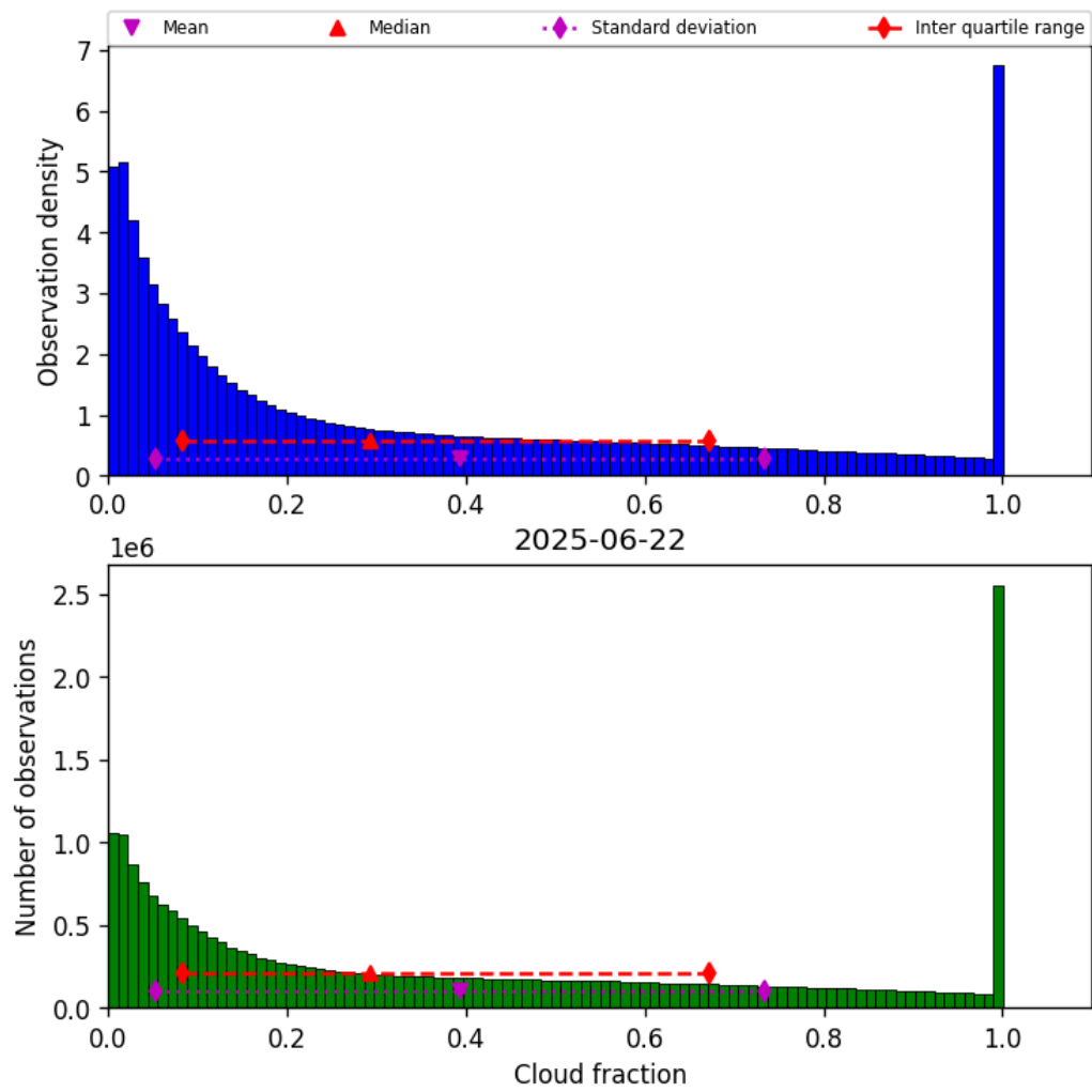
Figure 30: Histogram of “Cloud fraction” for 2025-06-22 to 2025-06-23
