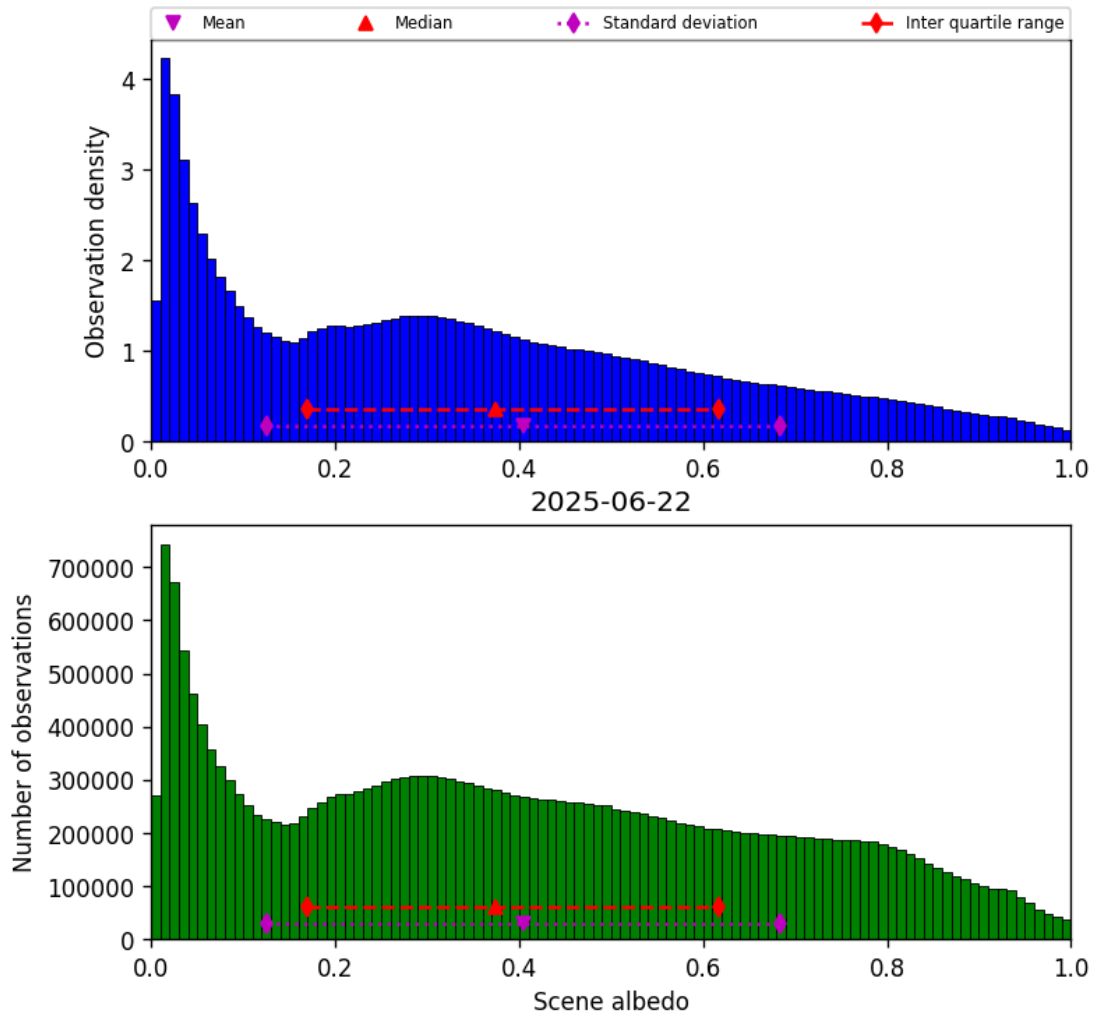
Figure 32: Histogram of “Scene albedo” for 2025-06-22 to 2025-06-23
