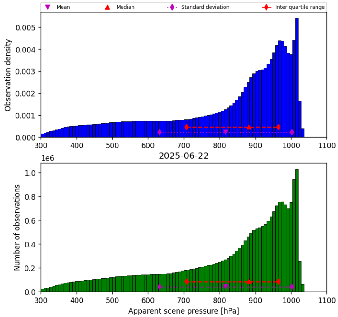
Figure 34: Histogram of “Apparent scene pressure” for 2025-06-22 to 2025-06-23
