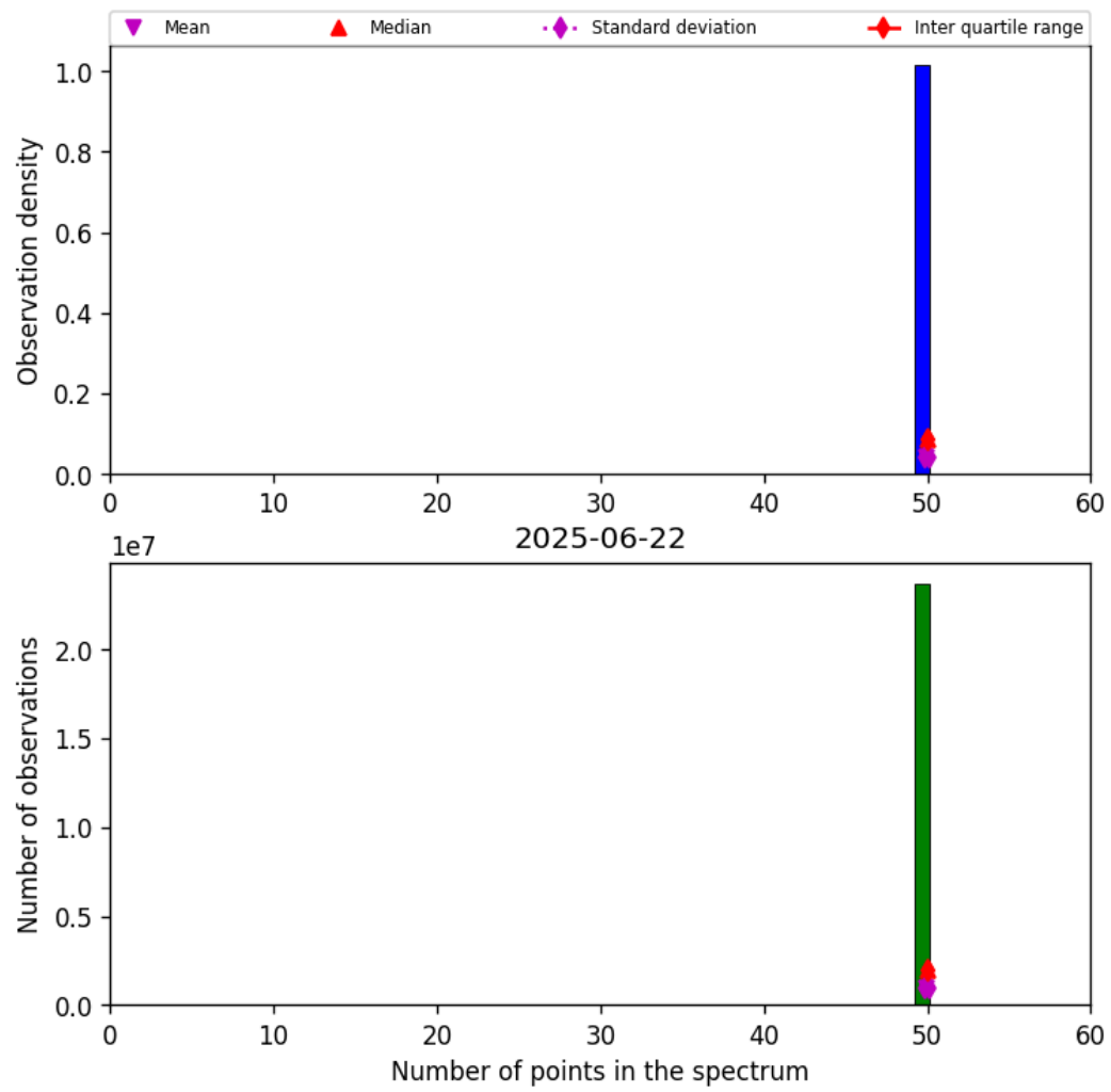
Figure 42: Histogram of “Number of points in the spectrum” for 2025-06-22 to 2025-06-23
