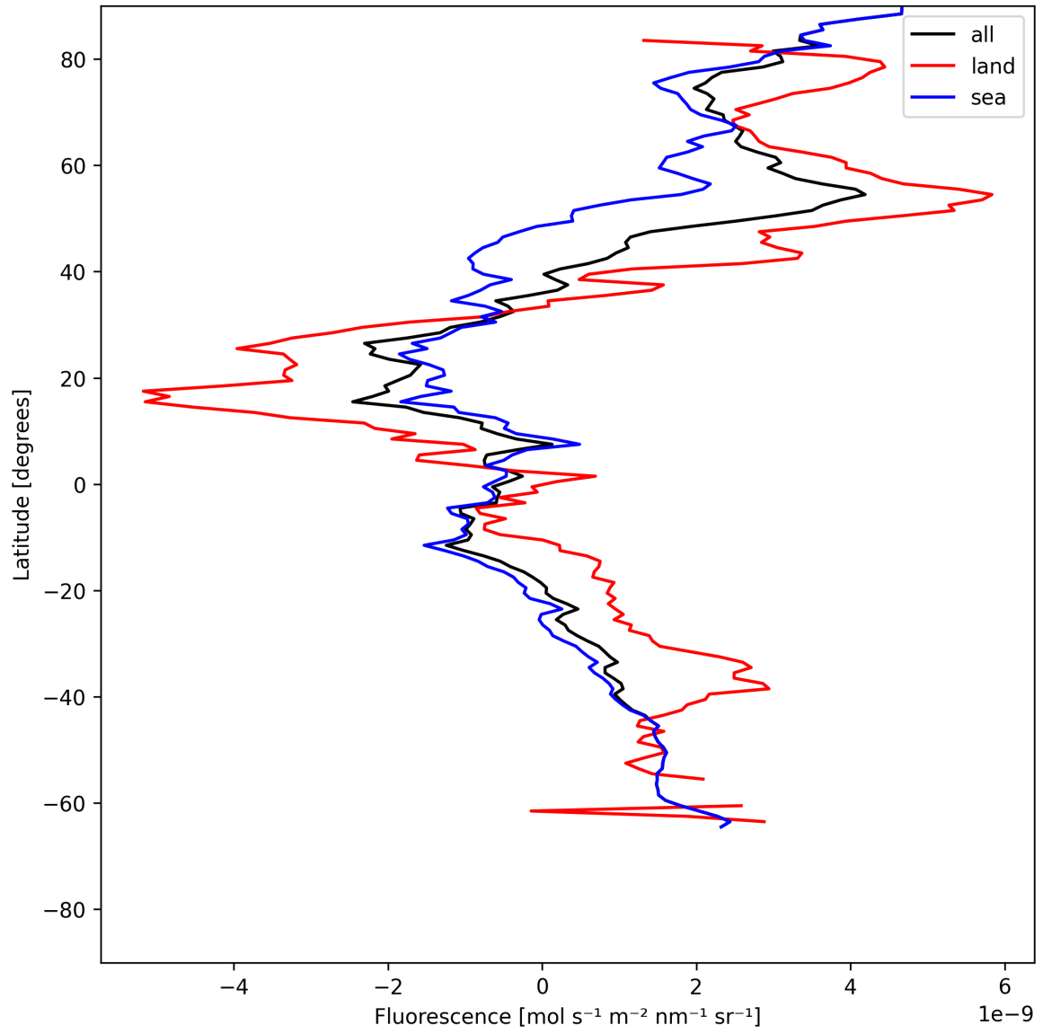
Figure 21: Zonal average of “Fluorescence” for 2025-06-22 to 2025-06-23.
