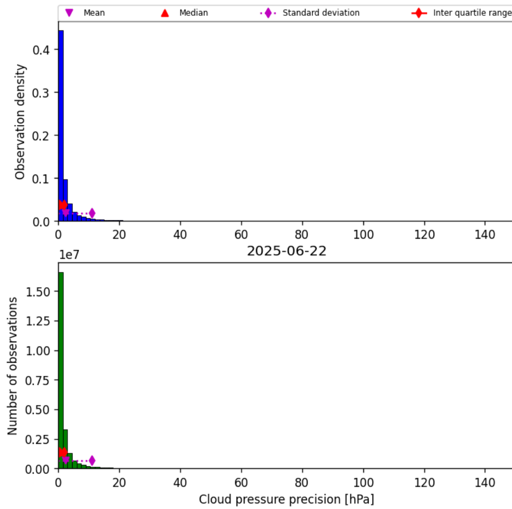
Figure 29: Histogram of “Cloud pressure precision” for 2025-06-22 to 2025-06-23
