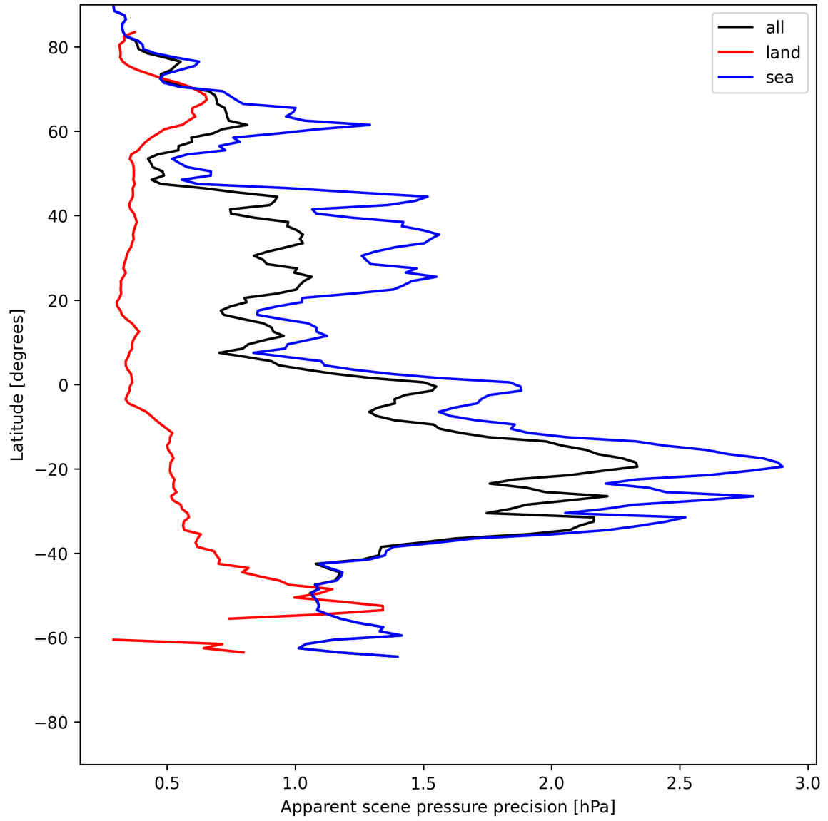
Figure 18: Zonal average of “Apparent scene pressure precision” for 2025-06-22 to 2025-06-23.
