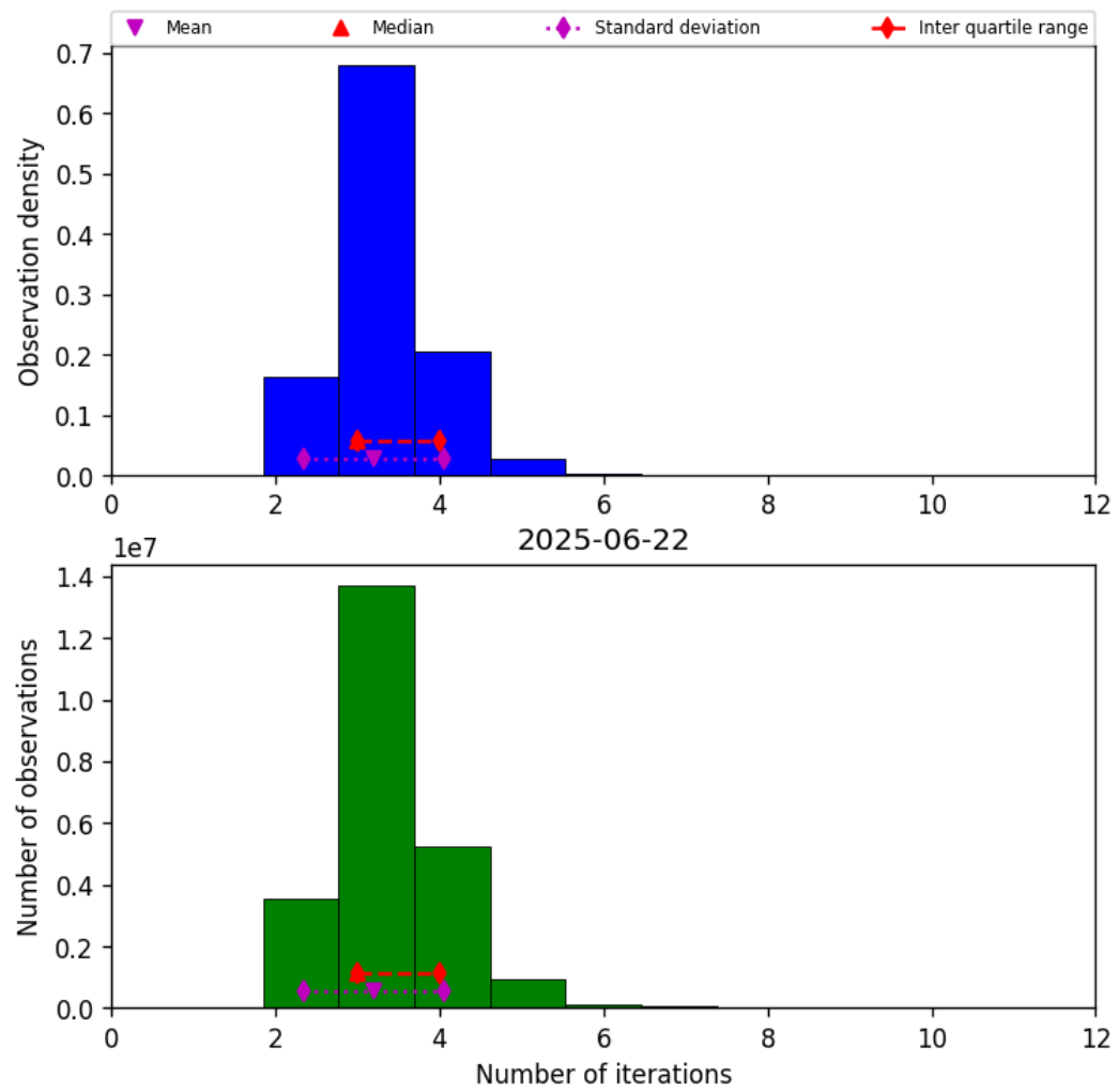
Figure 37: Histogram of “Number of iterations” for 2025-06-22 to 2025-06-23
