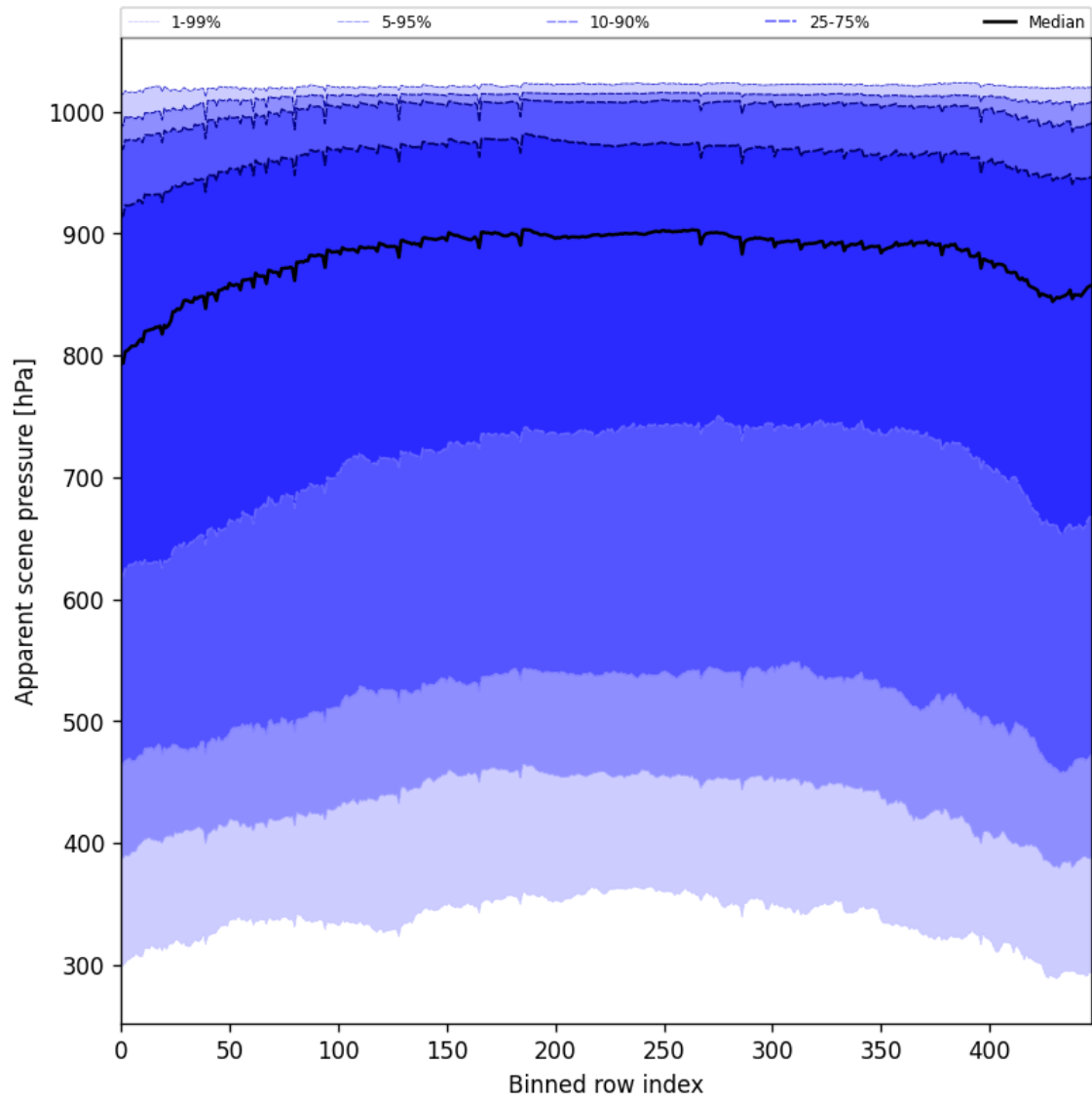
Figure 51: Along track statistics of “Apparent scene pressure” for 2025-06-22 to 2025-06-23
