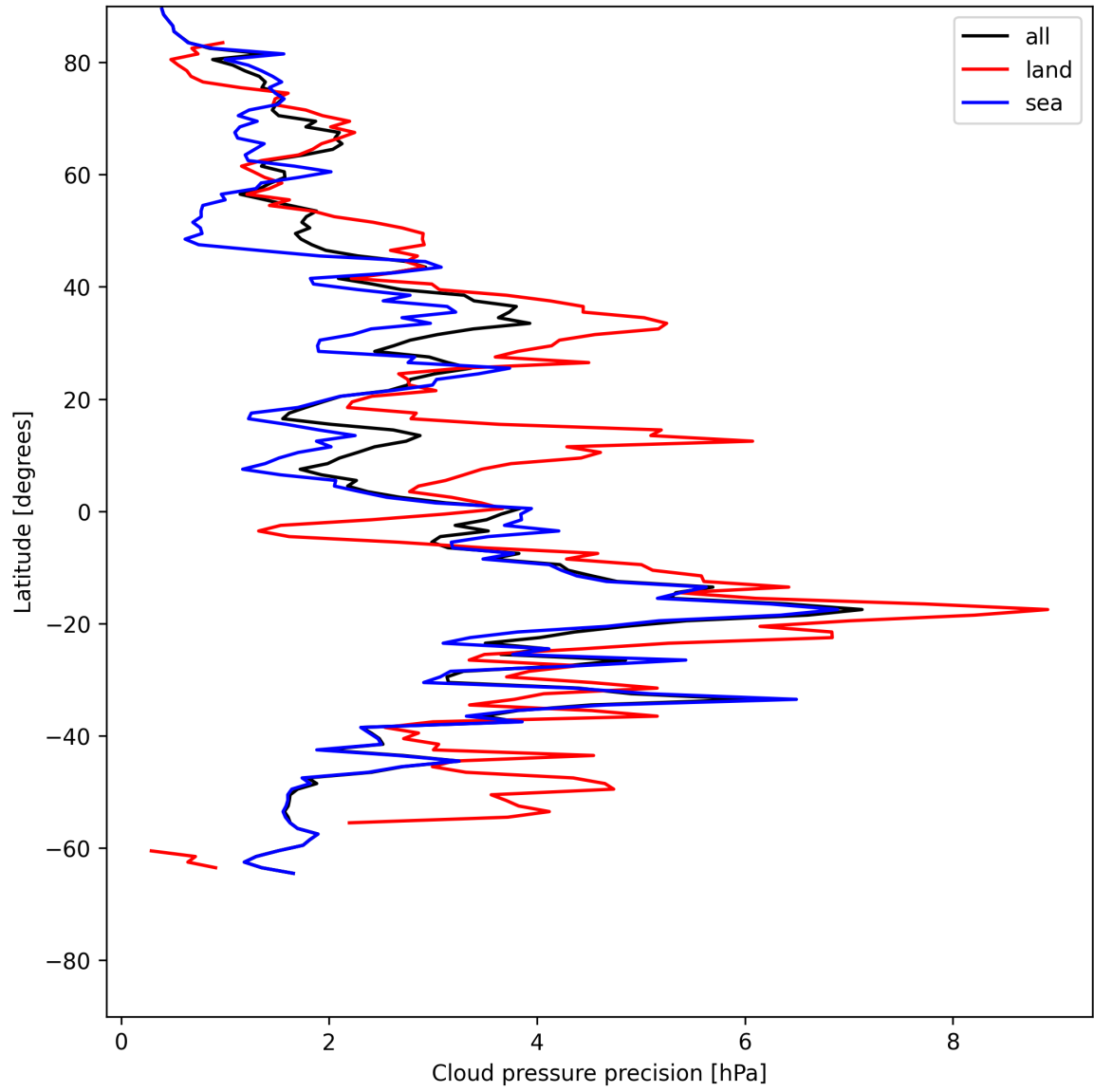
Figure 12: Zonal average of "Cloud pressure precision" for 2025-06-22 to 2025-06-23.
