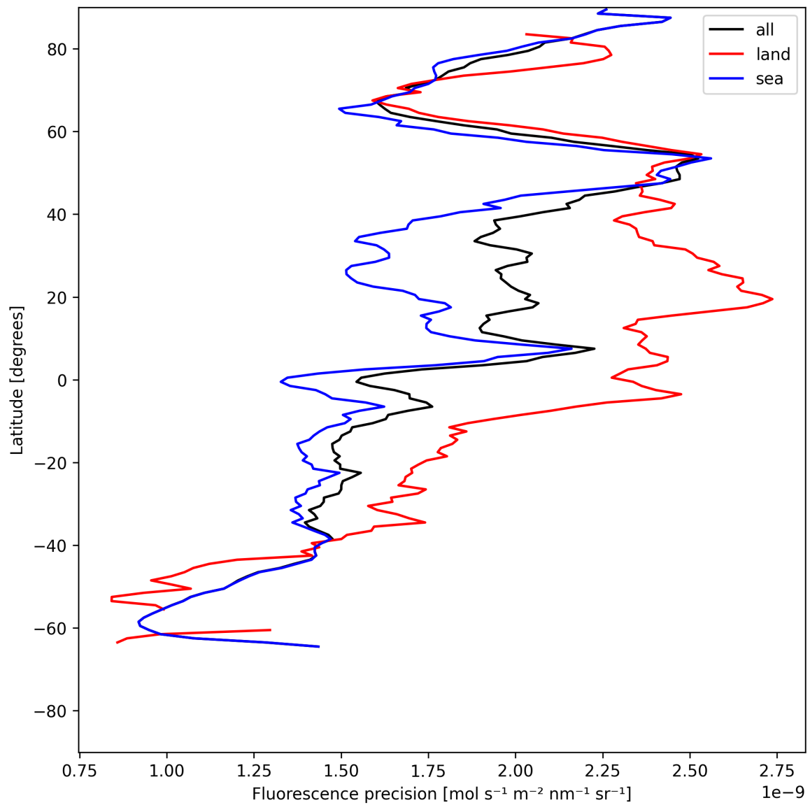
Figure 22: Zonal average of “Fluorescence precision” for 2025-06-22 to 2025-06-23.
