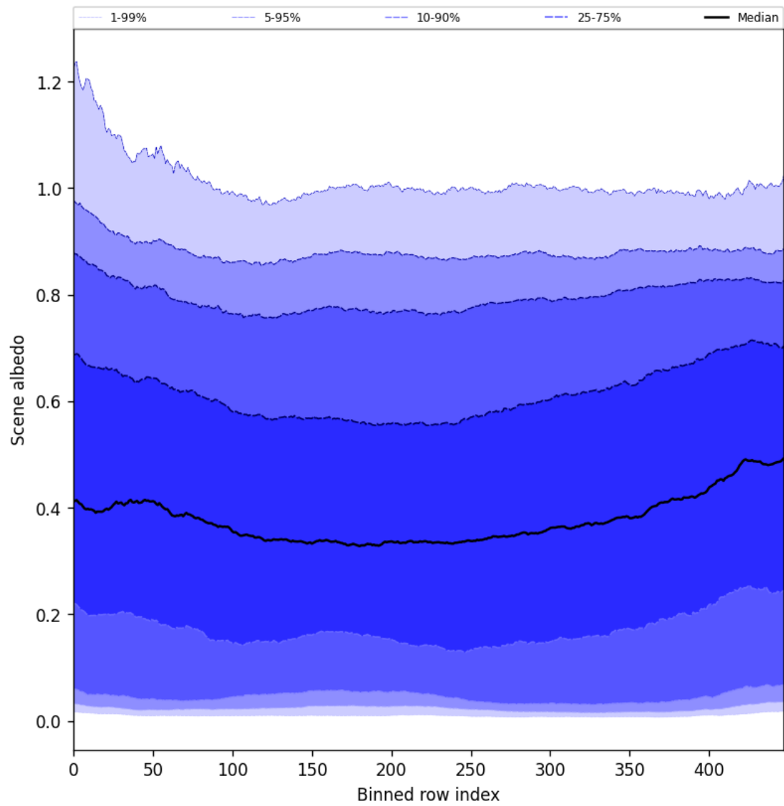
Figure 49: Along track statistics of “Scene albedo” for 2025-06-22 to 2025-06-23
