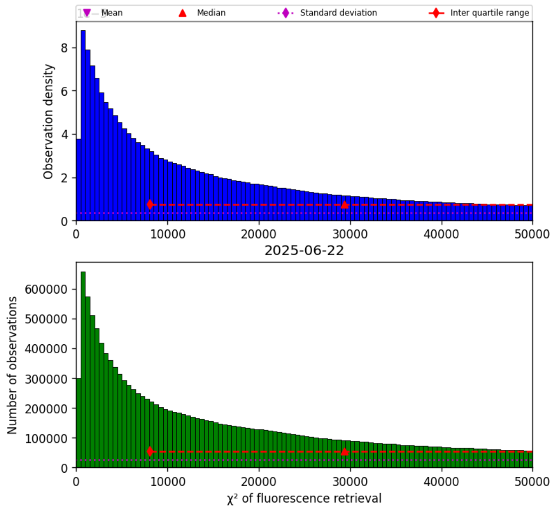
Figure 40: Histogram of “ \chi^2 of fluorescence retrieval” for 2025-06-22 to 2025-06-23
