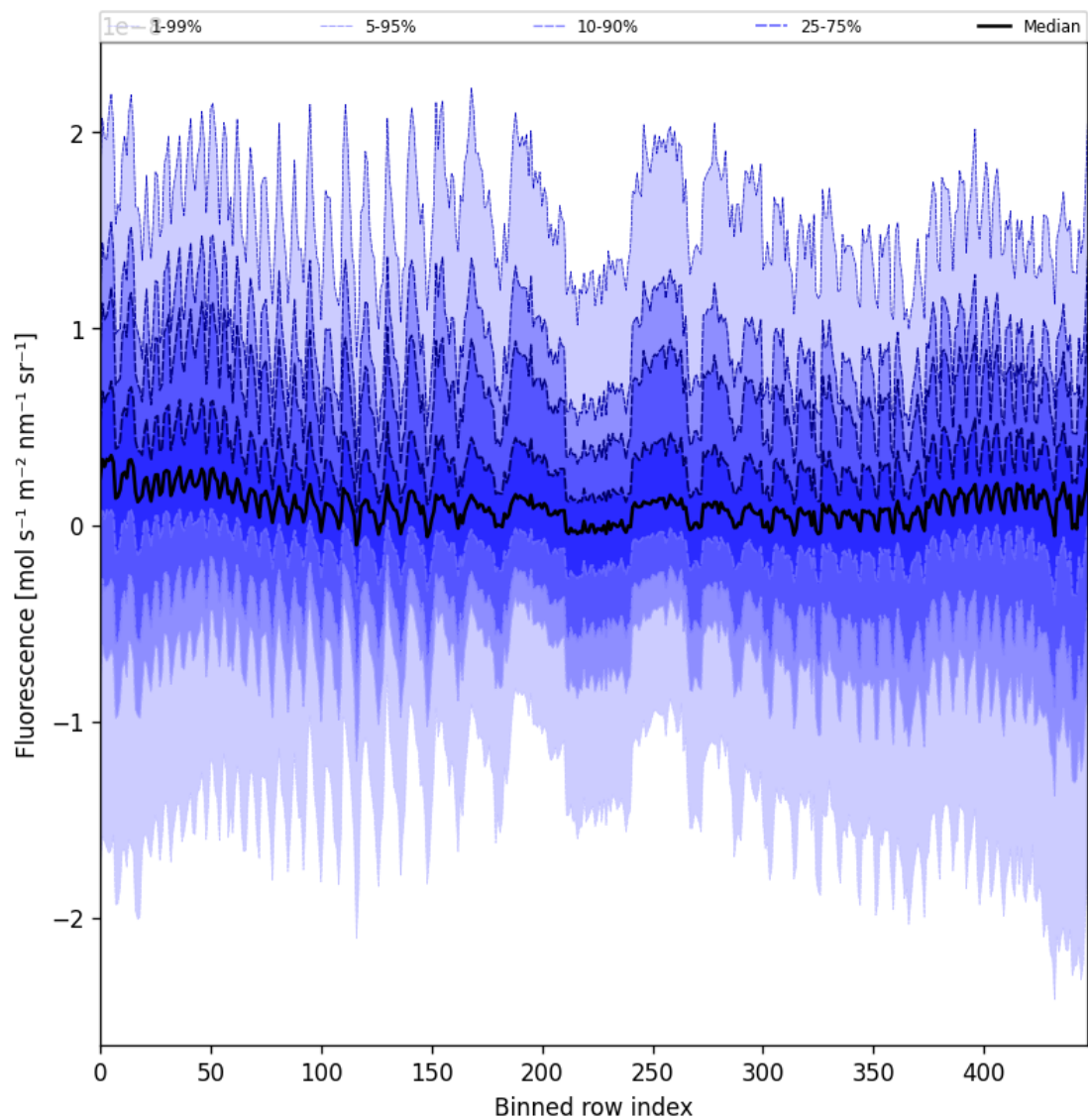
Figure 55: Along track statistics of "Fluorescence" for 2025-06-22 to 2025-06-23
