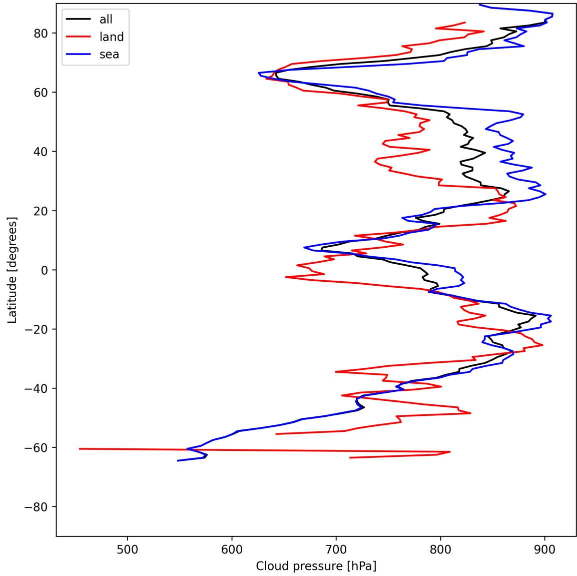
Figure 11: Zonal average of “Cloud pressure” for 2025-06-22 to 2025-06-23.
