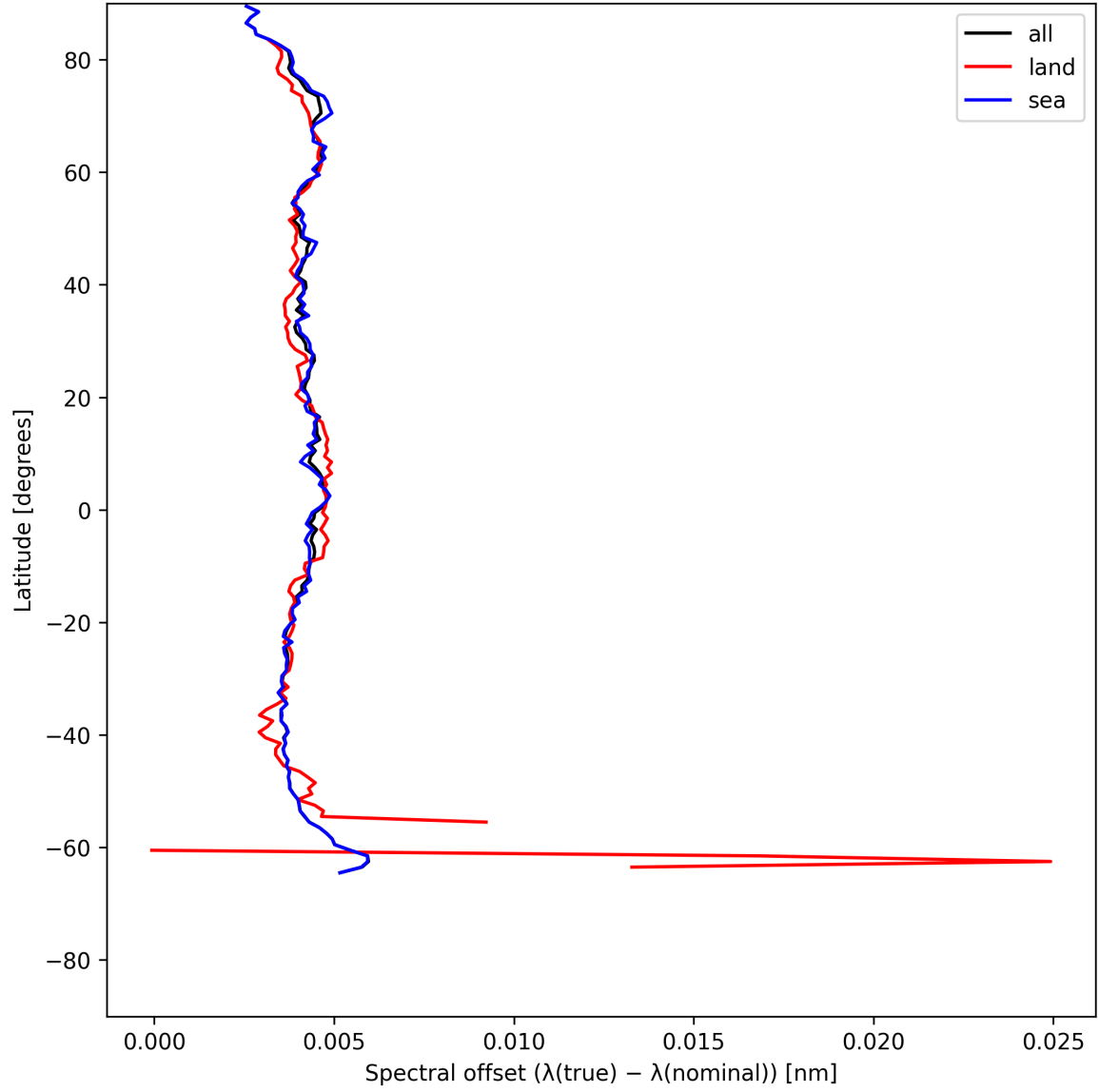
Figure 26: Zonal average of “Spectral offset ( \lambda_{\text{true}} - \lambda_{\text{nominal}} )” for 2025-06-22 to 2025-06-23.
