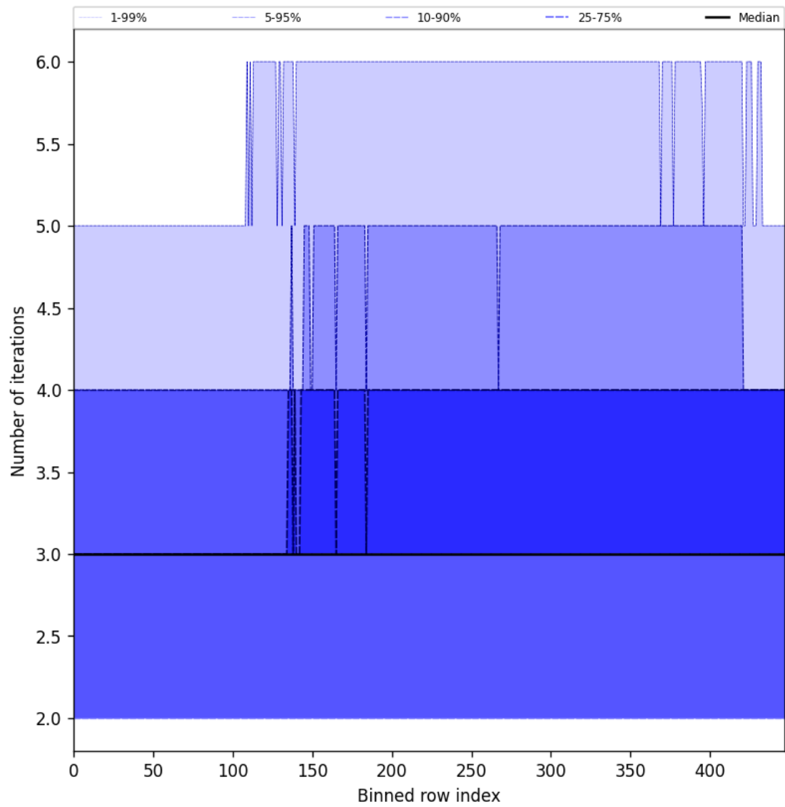
Figure 54: Along track statistics of “Number of iterations” for 2025-06-22 to 2025-06-23
