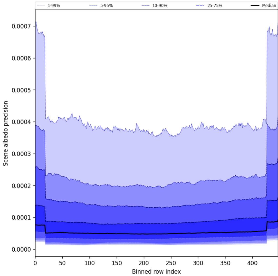
Figure 50: Along track statistics of “Scene albedo precision” for 2025-06-22 to 2025-06-23
