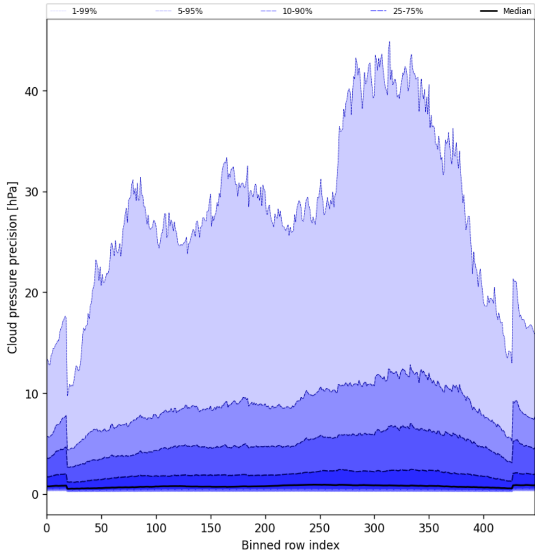
Figure 46: Along track statistics of “Cloud pressure precision” for 2025-06-22 to 2025-06-23
