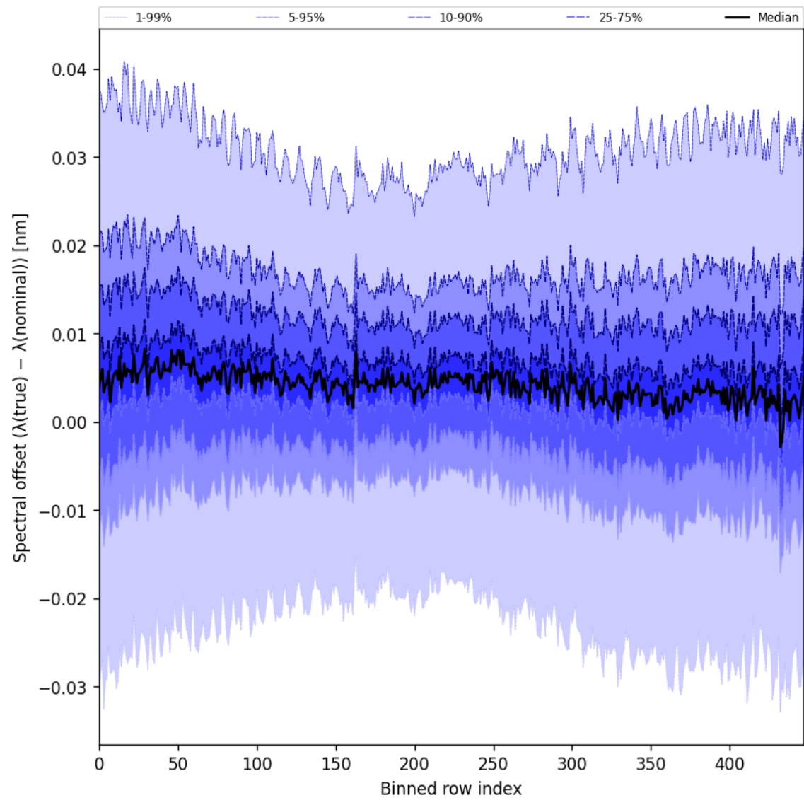
Figure 60: Along track statistics of “Spectral offset ( \lambda_{\text{true}} - \lambda_{\text{nominal}} )” for 2025-06-22 to 2025-06-23
