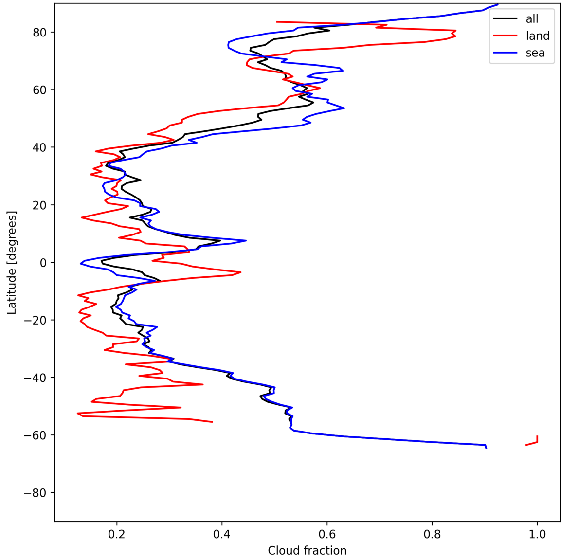
Figure 13: Zonal average of “Cloud fraction” for 2025-06-22 to 2025-06-23.
