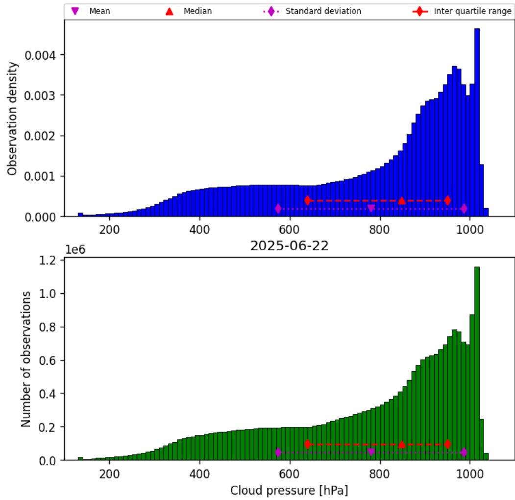
Figure 28: Histogram of “Cloud pressure” for 2025-06-22 to 2025-06-23
