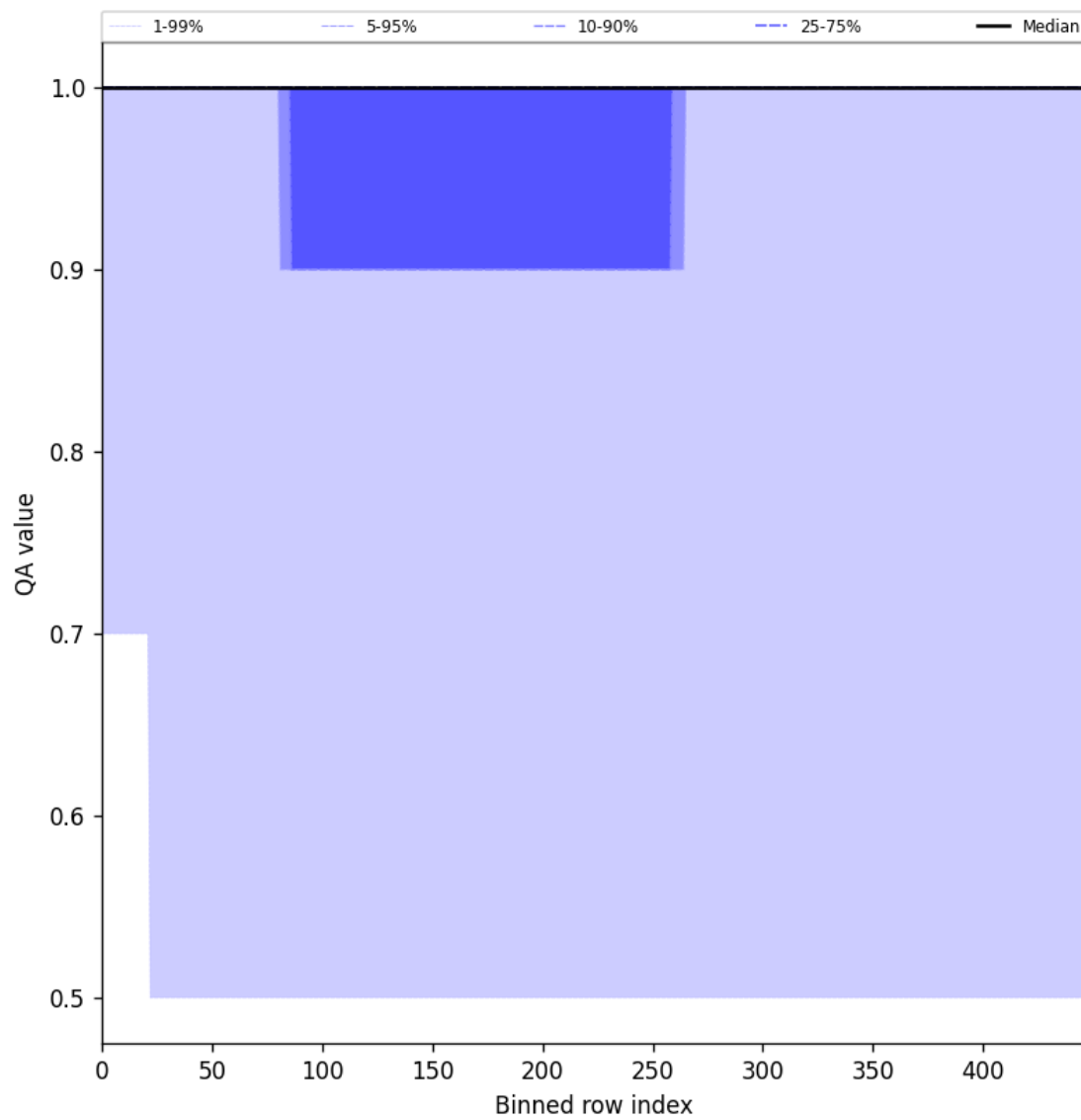
Figure 44: Along track statistics of “QA value” for 2025-06-22 to 2025-06-23
