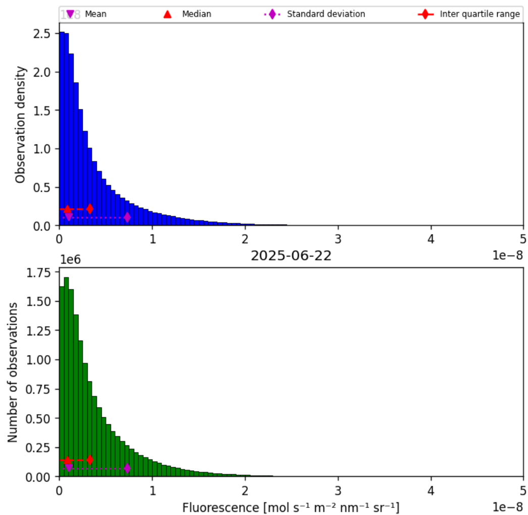
Figure 38: Histogram of “Fluorescence” for 2025-06-22 to 2025-06-23
