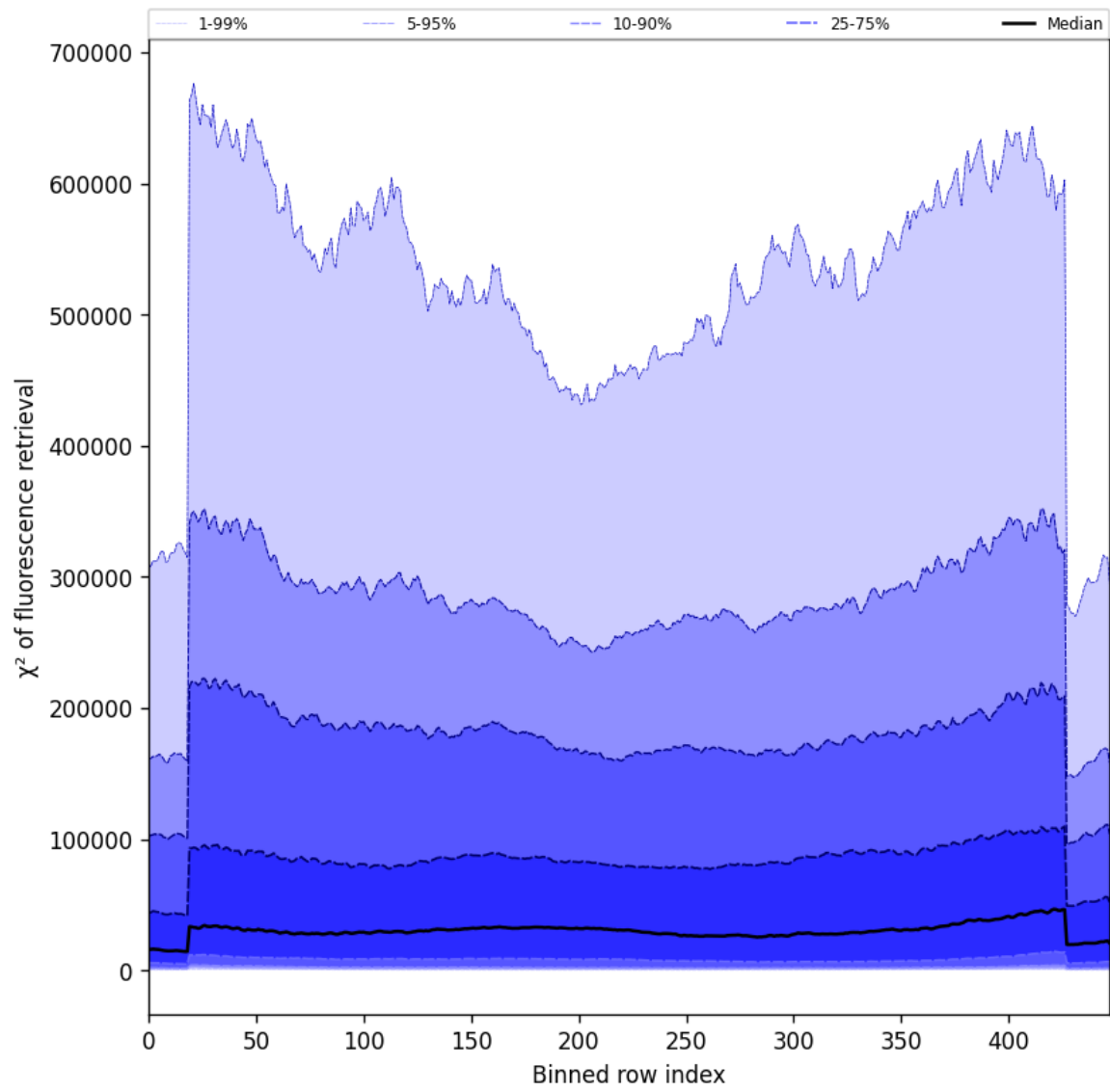
Figure 57: Along track statistics of “ \chi^2 of fluorescence retrieval” for 2025-06-22 to 2025-06-23
