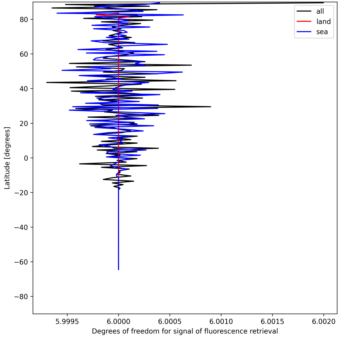
Figure 24: Zonal average of “Degrees of freedom for signal of fluorescence retrieval” for 2025-06-22 to 2025-06-23.
