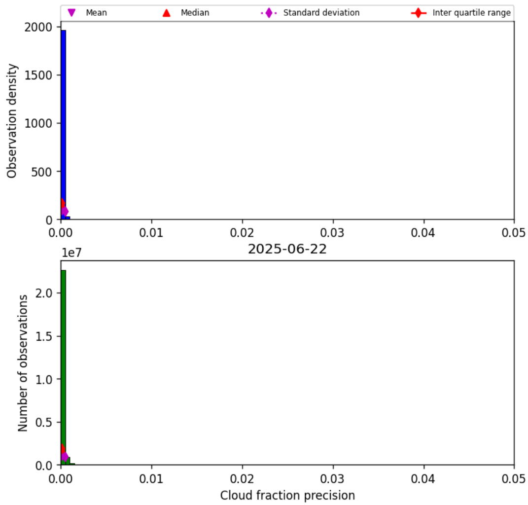
Figure 31: Histogram of “Cloud fraction precision” for 2025-06-22 to 2025-06-23
