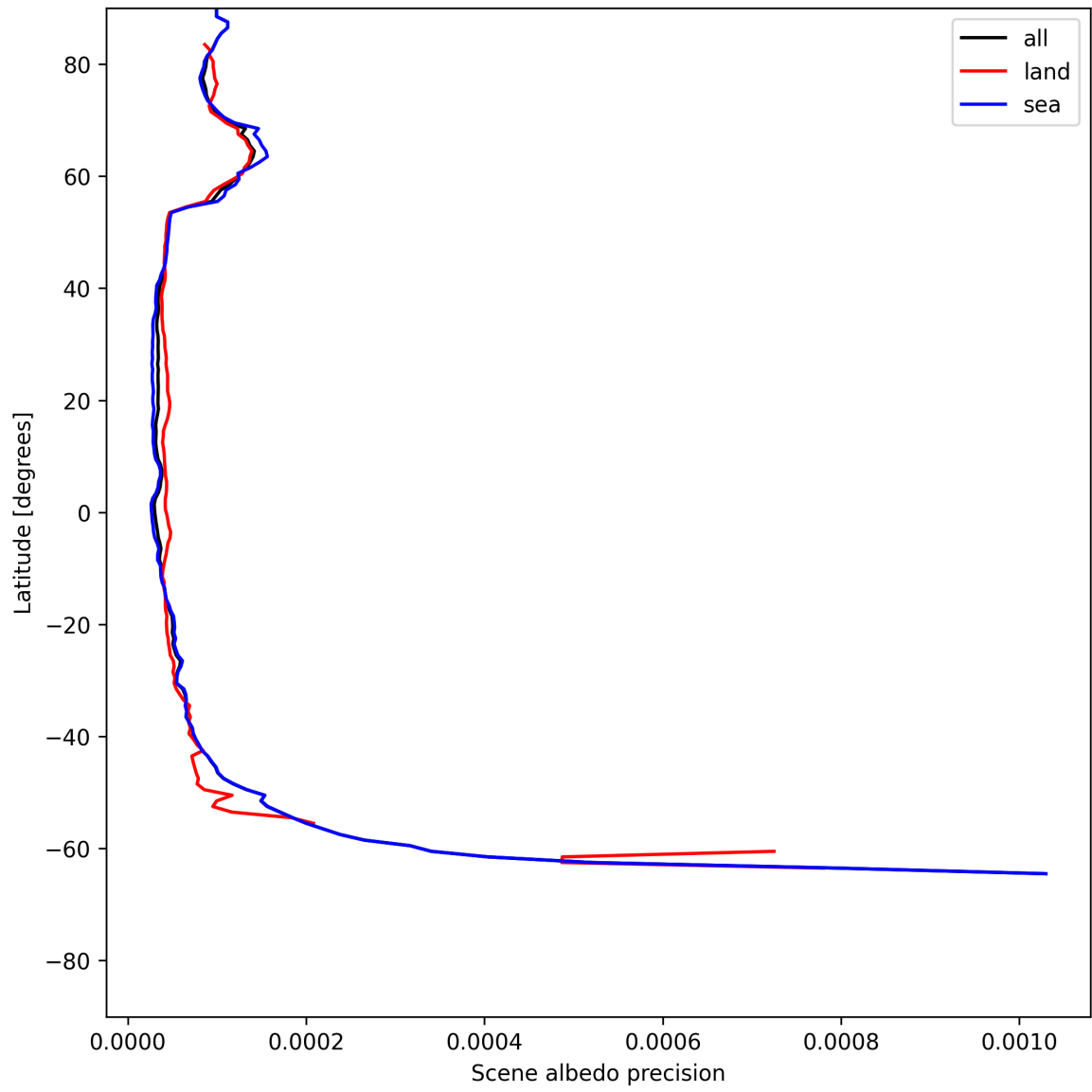
Figure 16: Zonal average of “Scene albedo precision” for 2025-06-22 to 2025-06-23.
