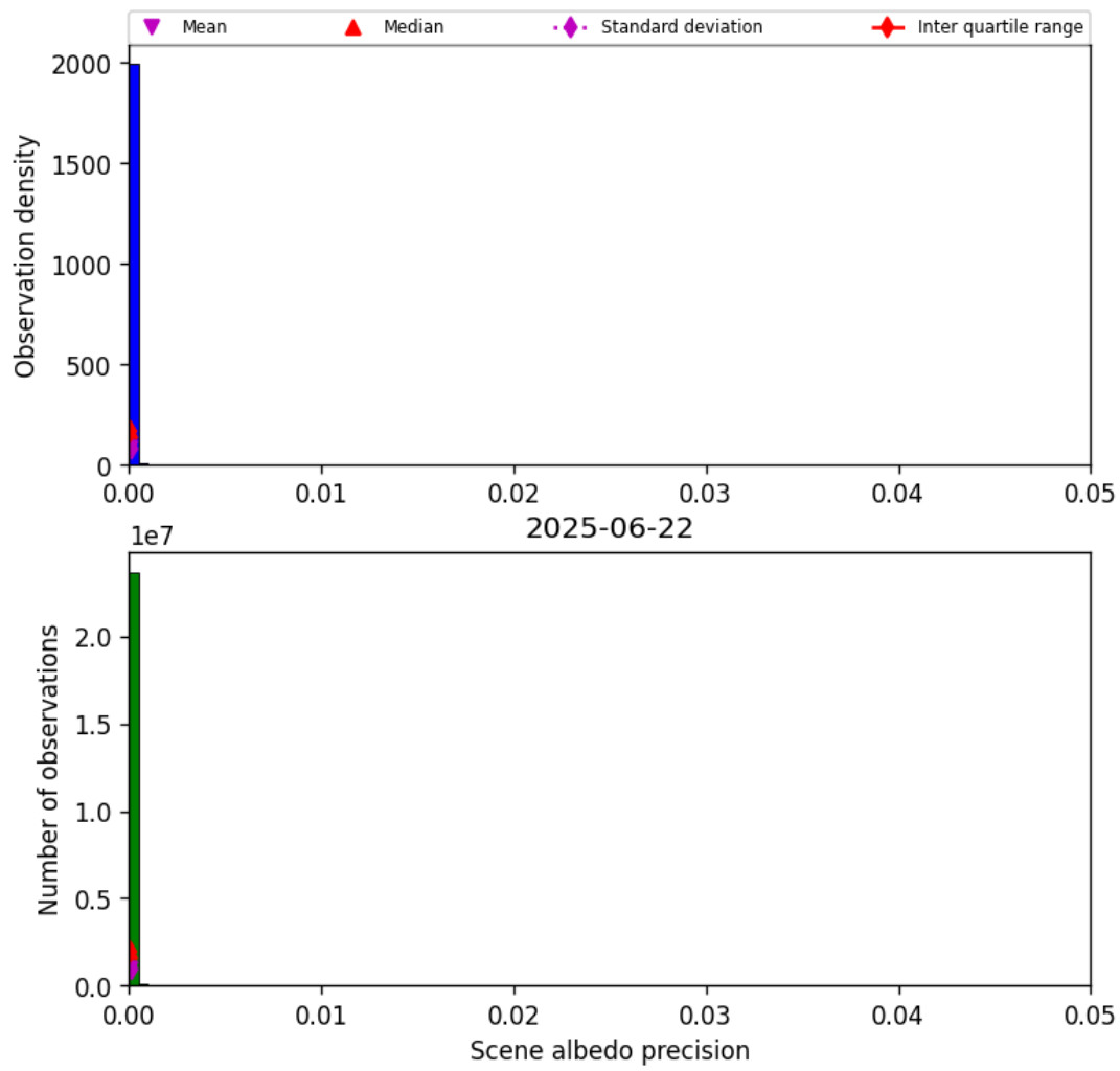
Figure 33: Histogram of “Scene albedo precision” for 2025-06-22 to 2025-06-23
