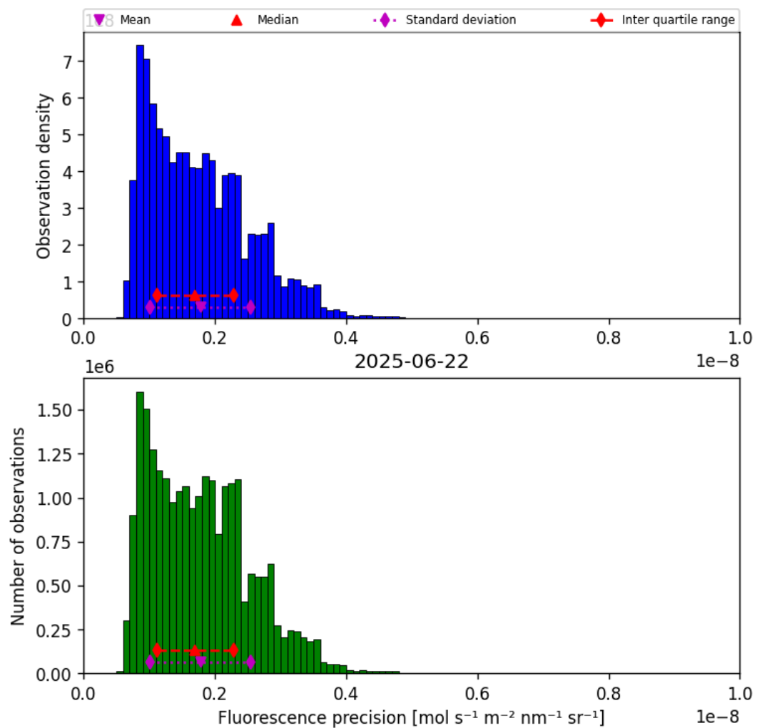
Figure 39: Histogram of “Fluorescence precision” for 2025-06-22 to 2025-06-23
