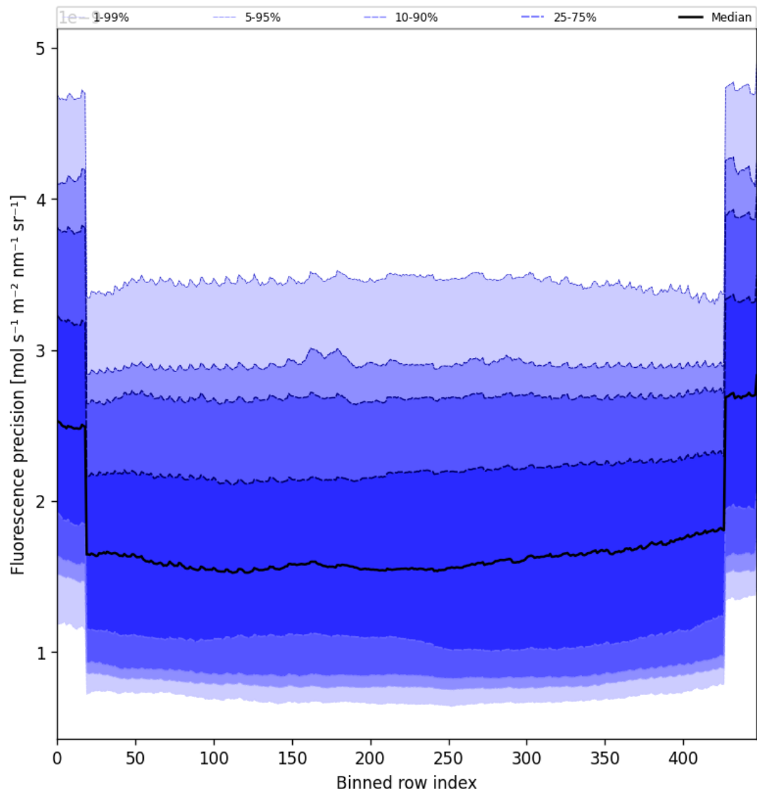
Figure 56: Along track statistics of "Fluorescence precision" for 2025-06-22 to 2025-06-23
