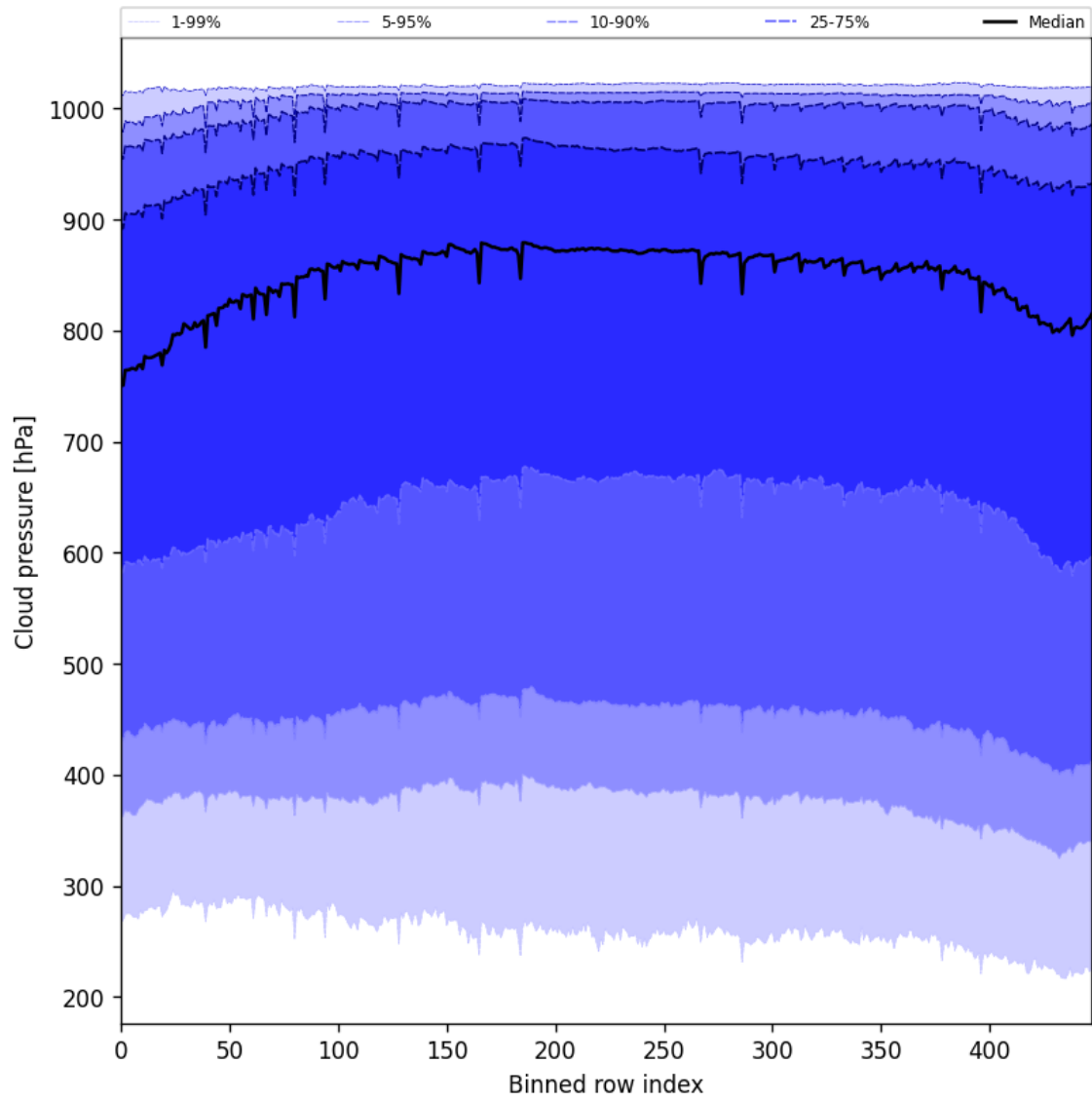
Figure 45: Along track statistics of “Cloud pressure” for 2025-06-22 to 2025-06-23
