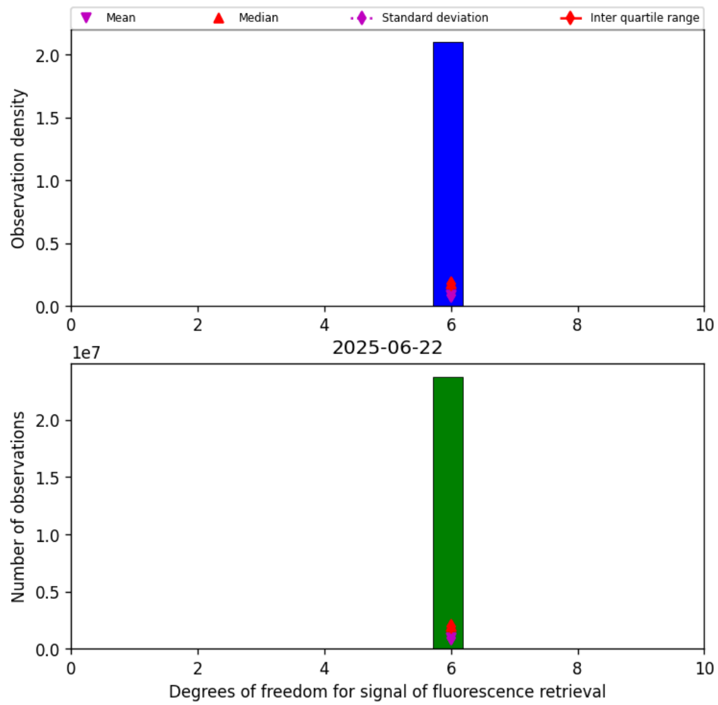
Figure 41: Histogram of “Degrees of freedom for signal of fluorescence retrieval” for 2025-06-22 to 2025-06-23
