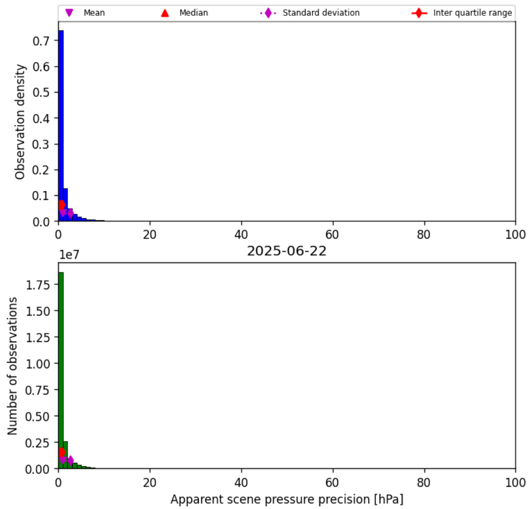
Figure 35: Histogram of “Apparent scene pressure precision” for 2025-06-22 to 2025-06-23
