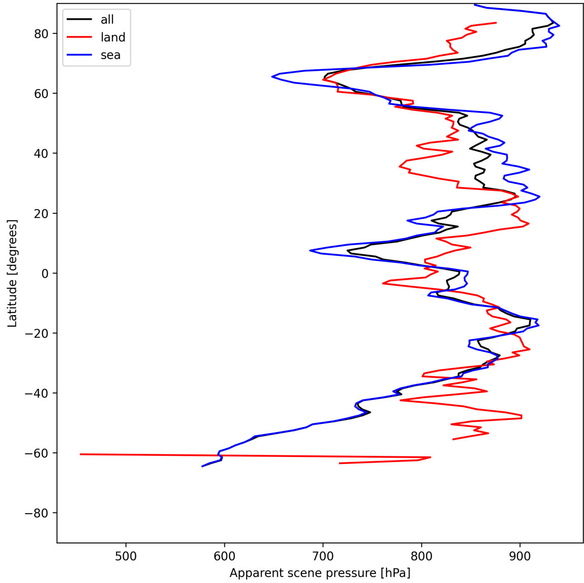
Figure 17: Zonal average of “Apparent scene pressure” for 2025-06-22 to 2025-06-23.
