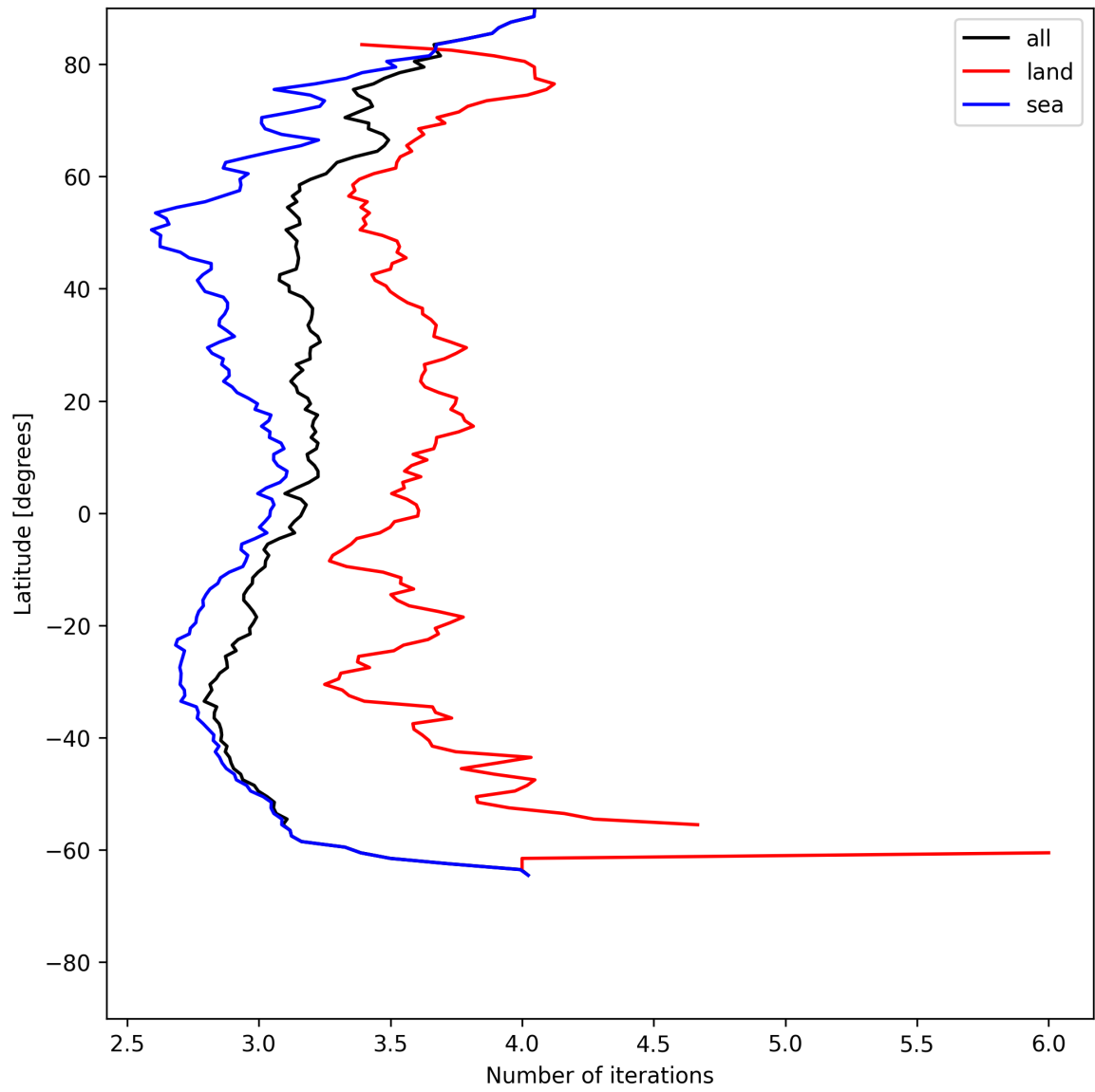
Figure 20: Zonal average of “Number of iterations” for 2025-06-22 to 2025-06-23.
