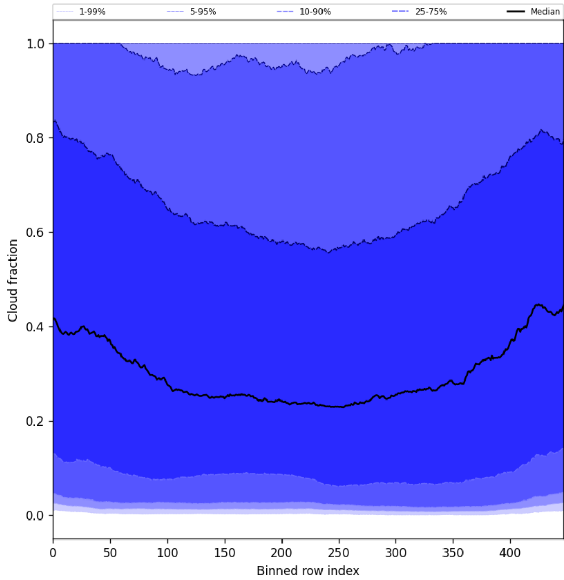
Figure 47: Along track statistics of “Cloud fraction” for 2025-06-22 to 2025-06-23
