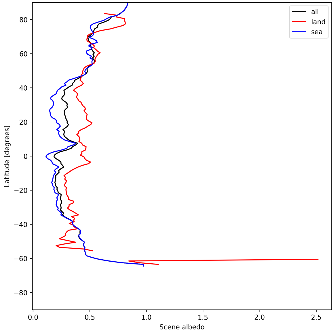
Figure 15: Zonal average of “Scene albedo” for 2025-06-22 to 2025-06-23.
