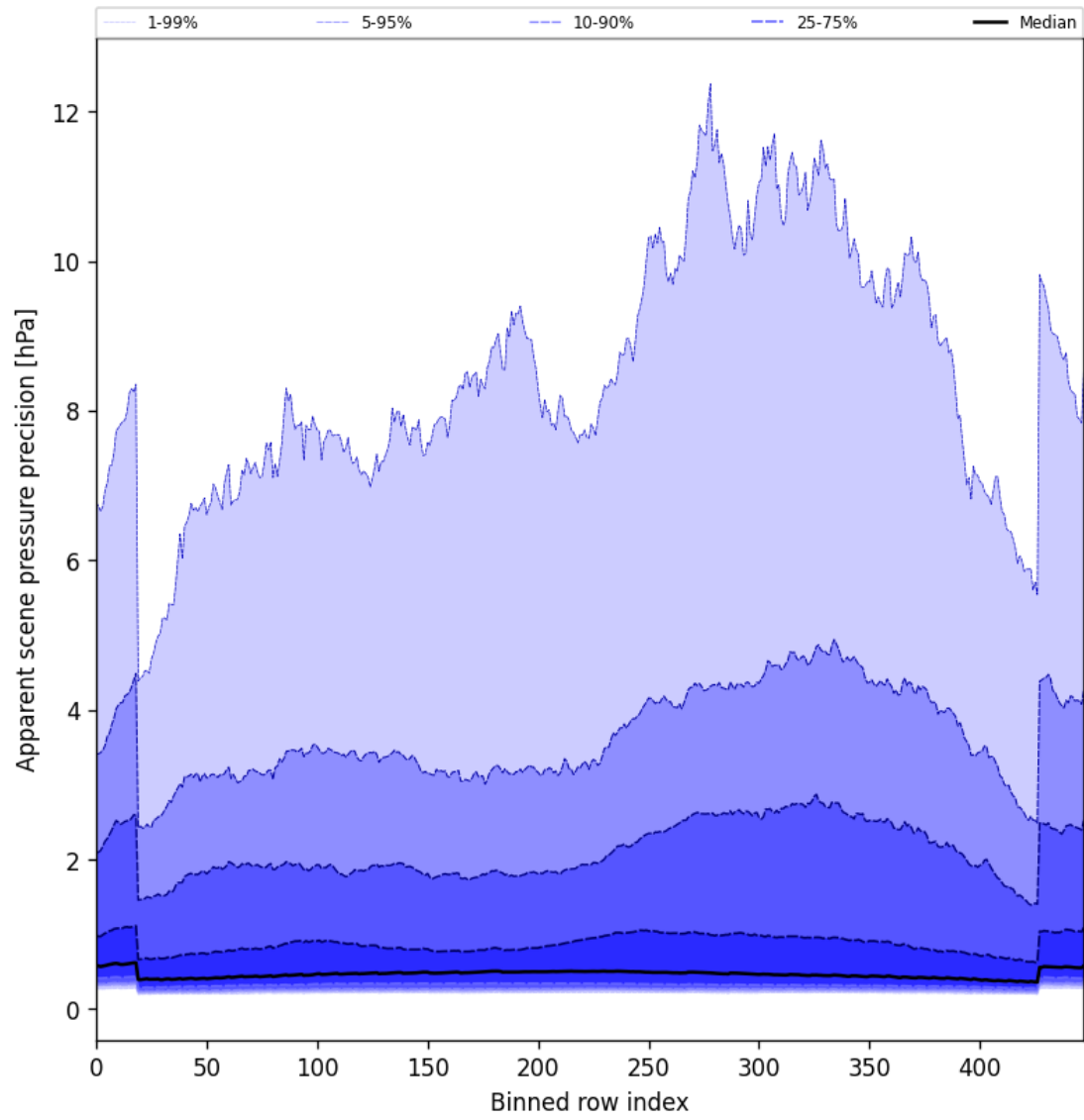
Figure 52: Along track statistics of “Apparent scene pressure precision” for 2025-06-22 to 2025-06-23
