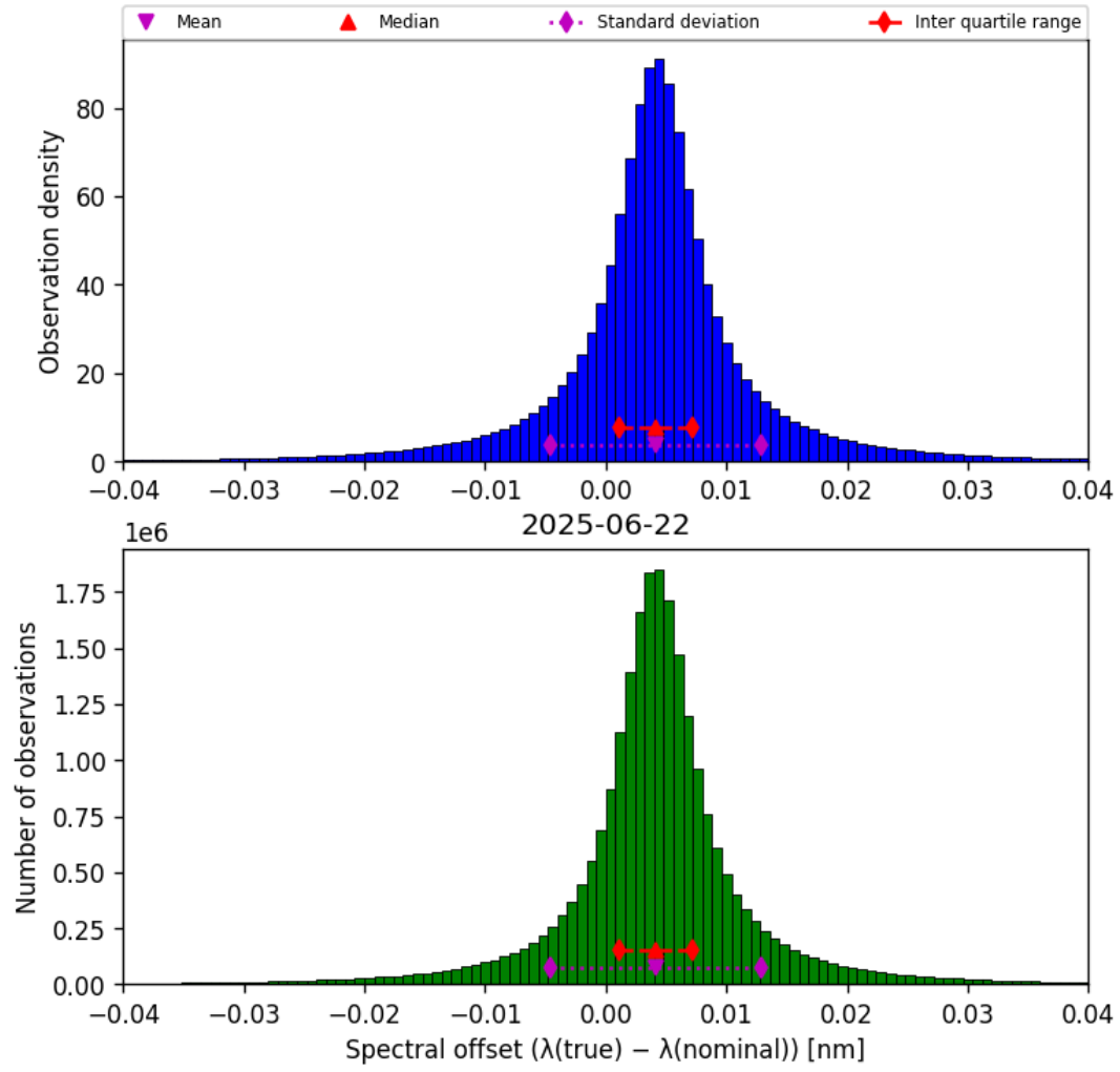
Figure 43: Histogram of “Spectral offset ( \lambda_{\text{true}} - \lambda_{\text{nominal}} )” for 2025-06-22 to 2025-06-23
