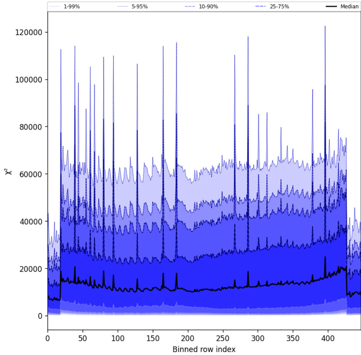
Figure 53: Along track statistics of “ \chi^2 ” for 2025-06-22 to 2025-06-23
