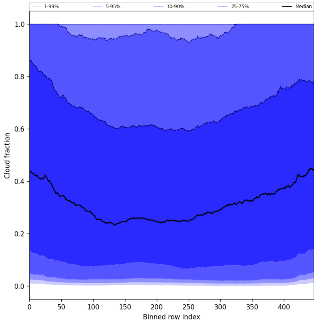
Figure 47: Along track statistics of “Cloud fraction” for 2025-06-23 to 2025-06-24
