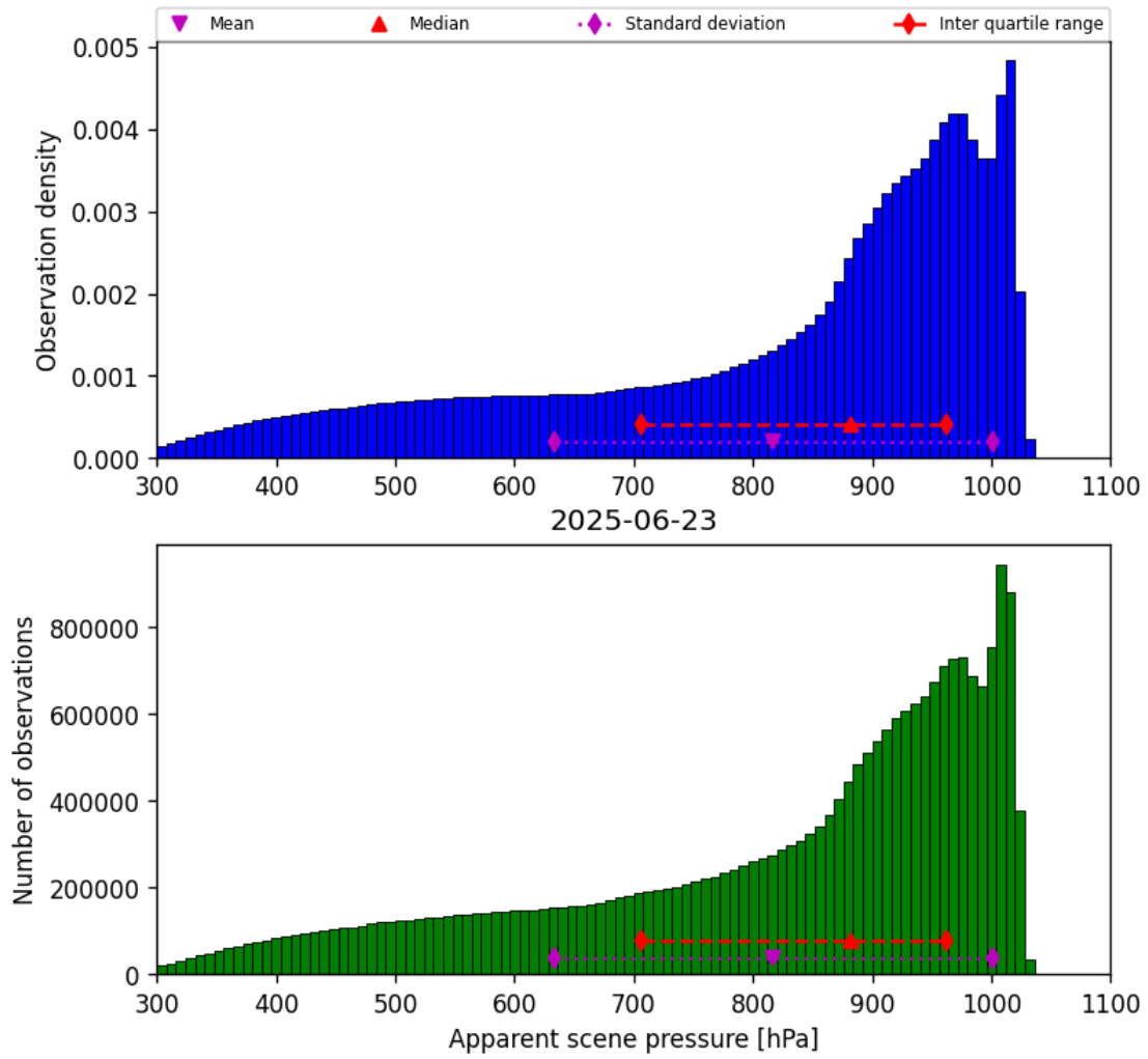
Figure 34: Histogram of “Apparent scene pressure” for 2025-06-23 to 2025-06-24
