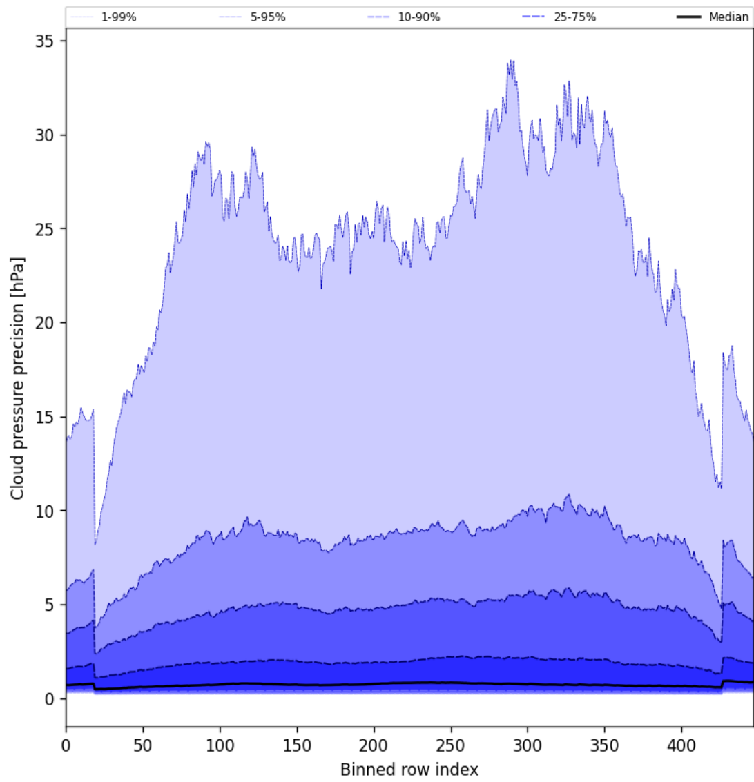
Figure 46: Along track statistics of “Cloud pressure precision” for 2025-06-23 to 2025-06-24
