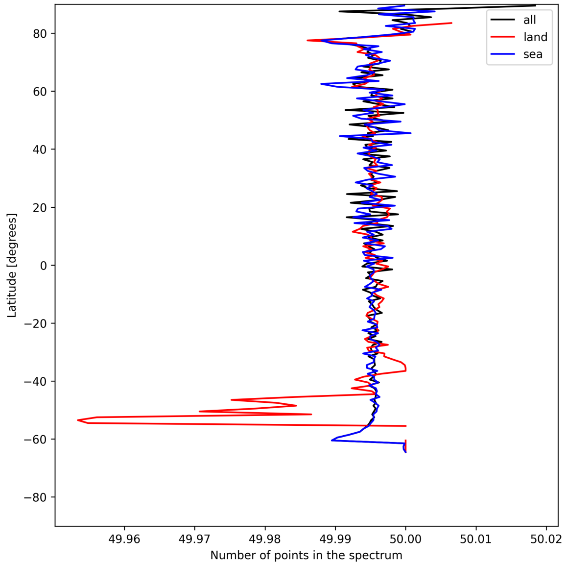
Figure 25: Zonal average of “Number of points in the spectrum” for 2025-06-23 to 2025-06-24.
