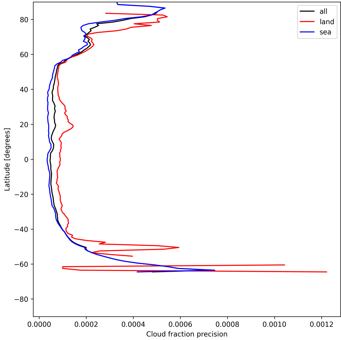
Figure 14: Zonal average of “Cloud fraction precision” for 2025-06-23 to 2025-06-24.
