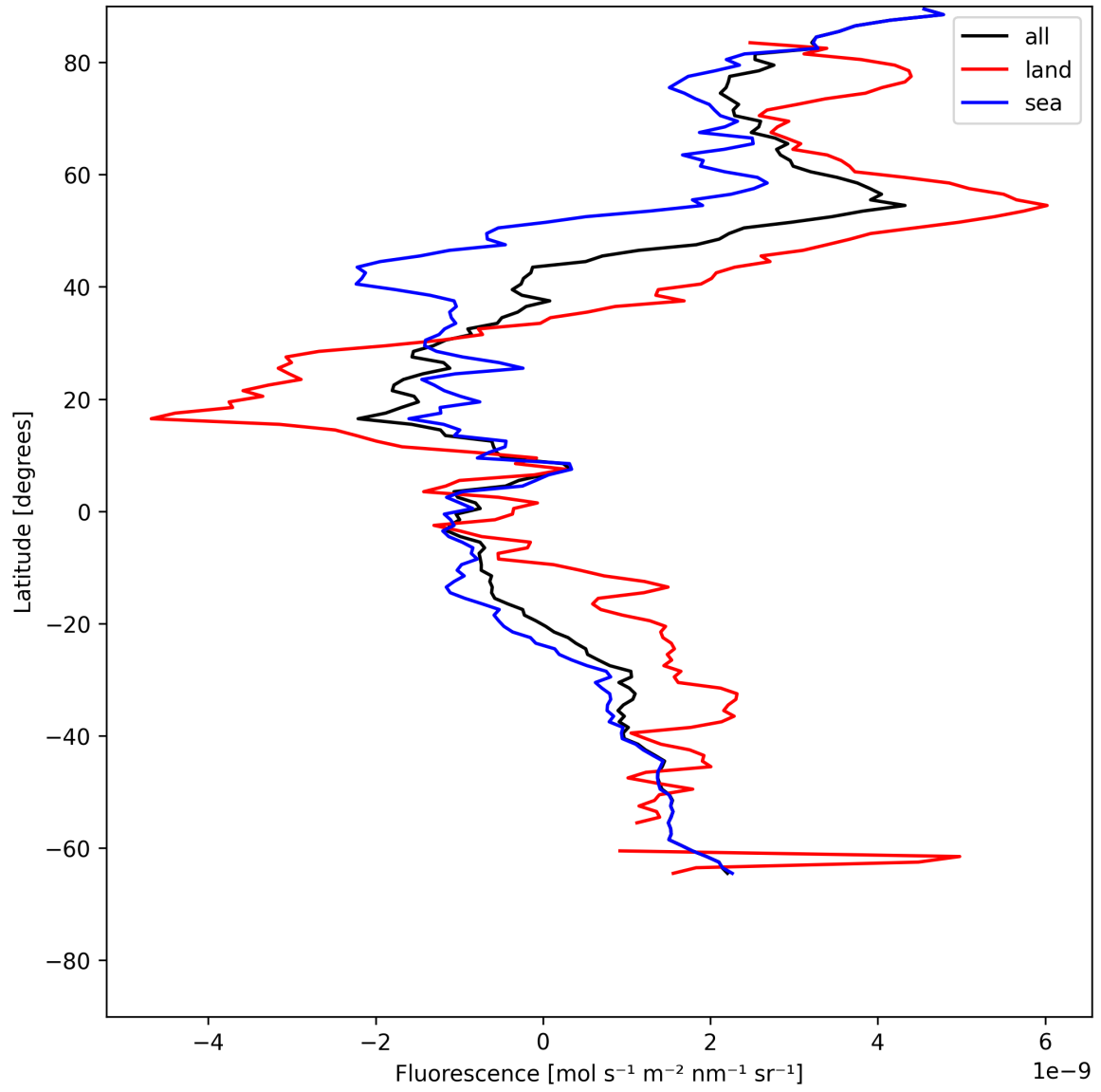
Figure 21: Zonal average of “Fluorescence” for 2025-06-23 to 2025-06-24.
