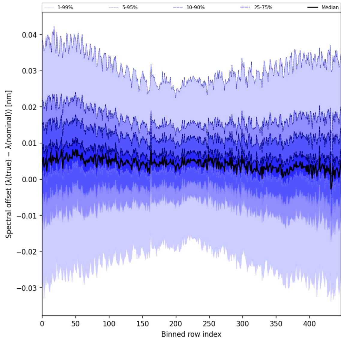
Figure 60: Along track statistics of “Spectral offset ( \lambda_{\text{true}} - \lambda_{\text{nominal}} )” for 2025-06-23 to 2025-06-24
