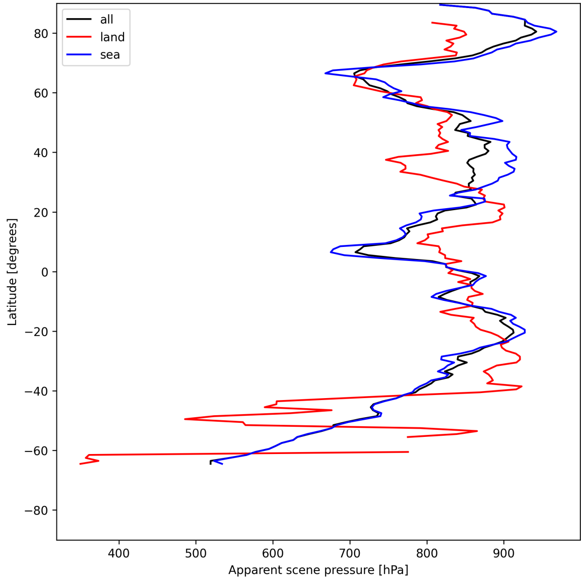
Figure 17: Zonal average of “Apparent scene pressure” for 2025-06-23 to 2025-06-24.
