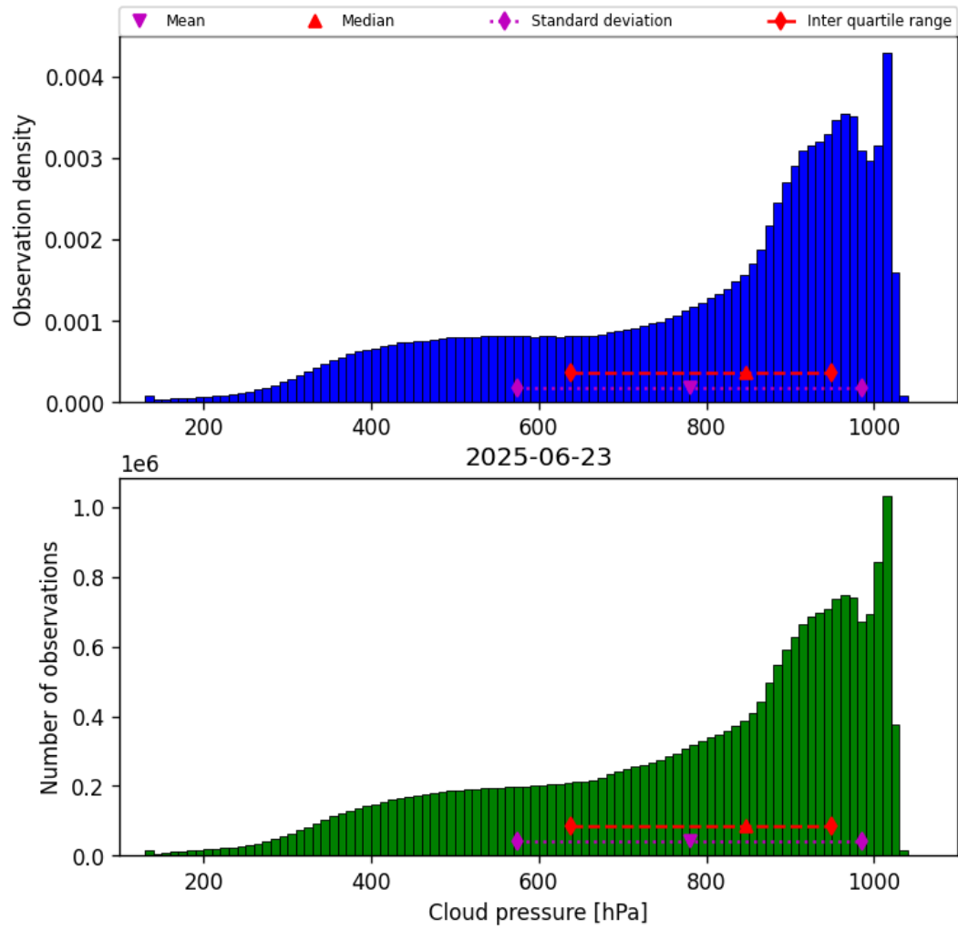
Figure 28: Histogram of “Cloud pressure” for 2025-06-23 to 2025-06-24
