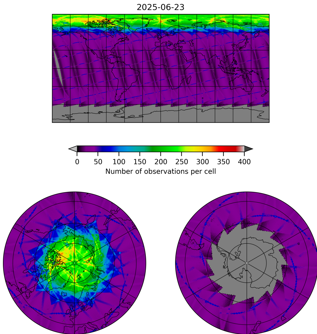
Figure 9: Map of the number of observations for 2025-06-23 to 2025-06-24
