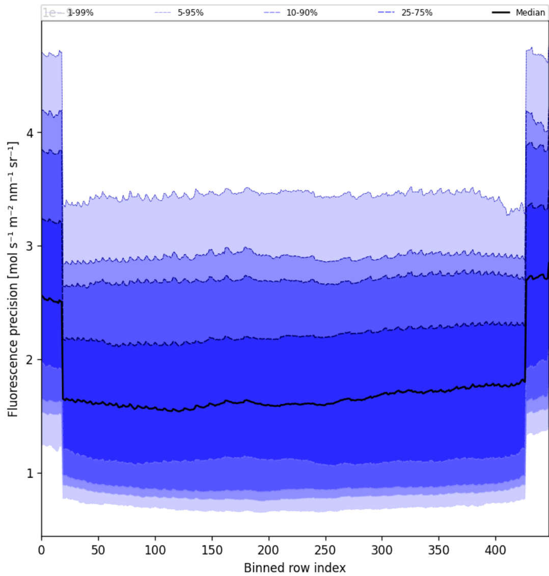
Figure 56: Along track statistics of “Fluorescence precision” for 2025-06-23 to 2025-06-24
