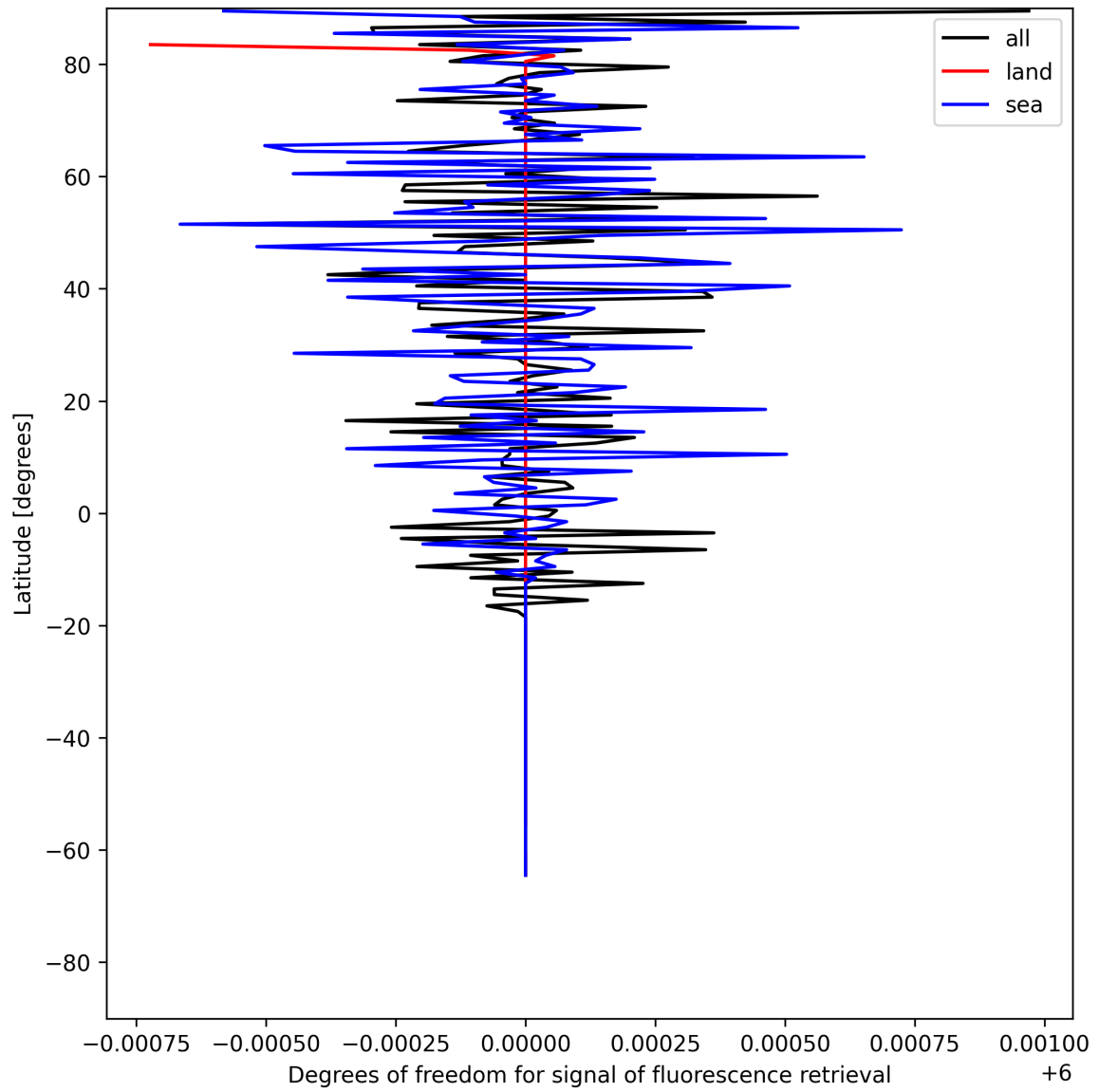
Figure 24: Zonal average of “Degrees of freedom for signal of fluorescence retrieval” for 2025-06-23 to 2025-06-24.
