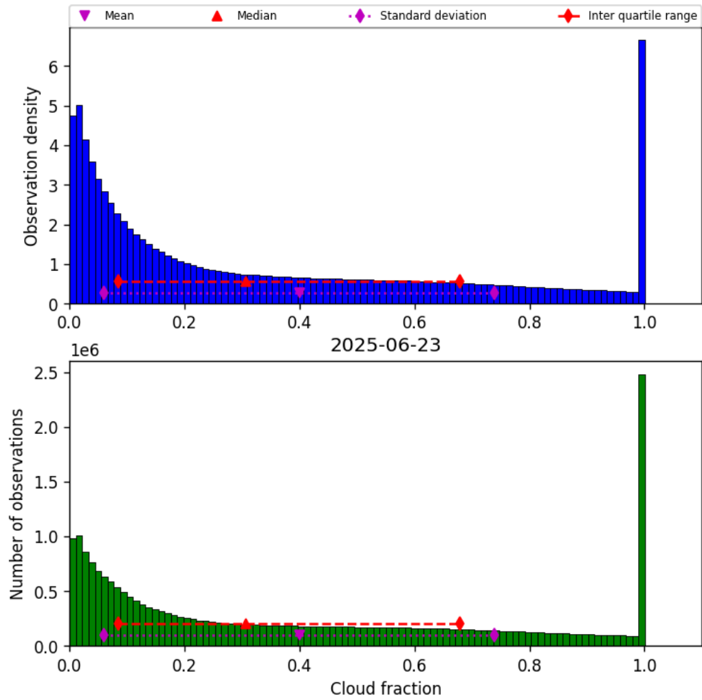
Figure 30: Histogram of “Cloud fraction” for 2025-06-23 to 2025-06-24
