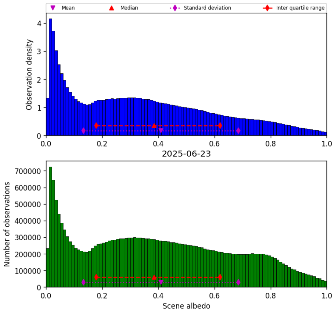
Figure 32: Histogram of “Scene albedo” for 2025-06-23 to 2025-06-24
