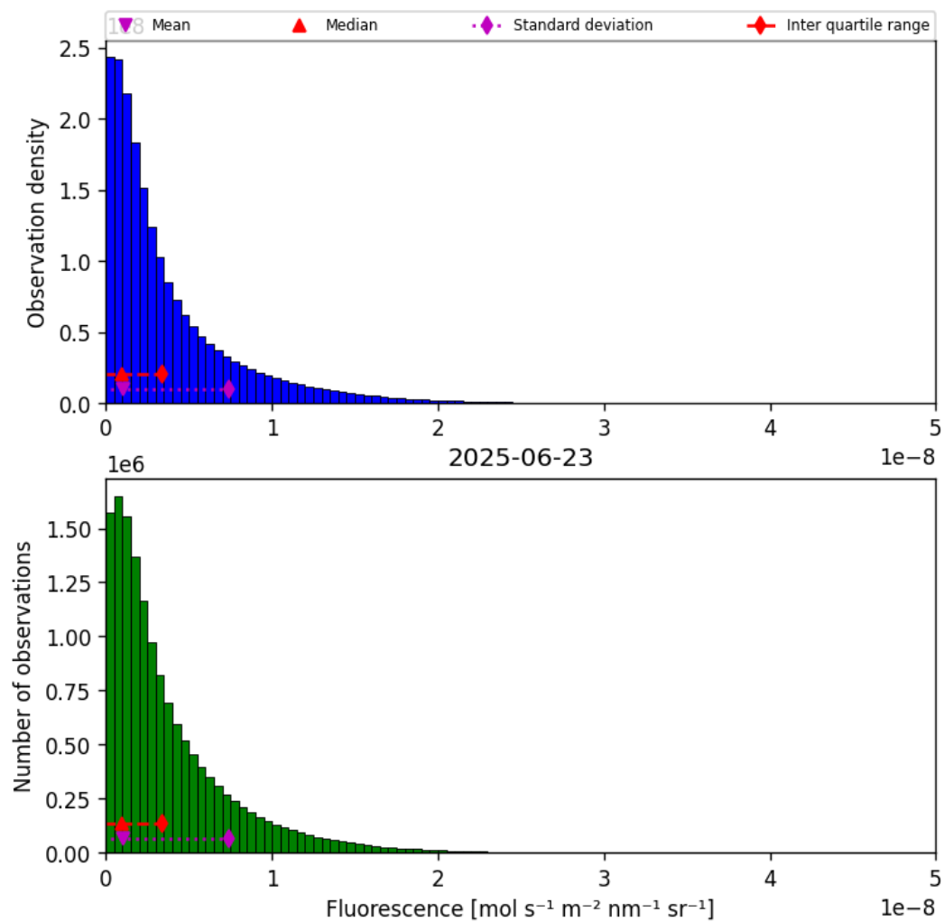
Figure 38: Histogram of “Fluorescence” for 2025-06-23 to 2025-06-24
