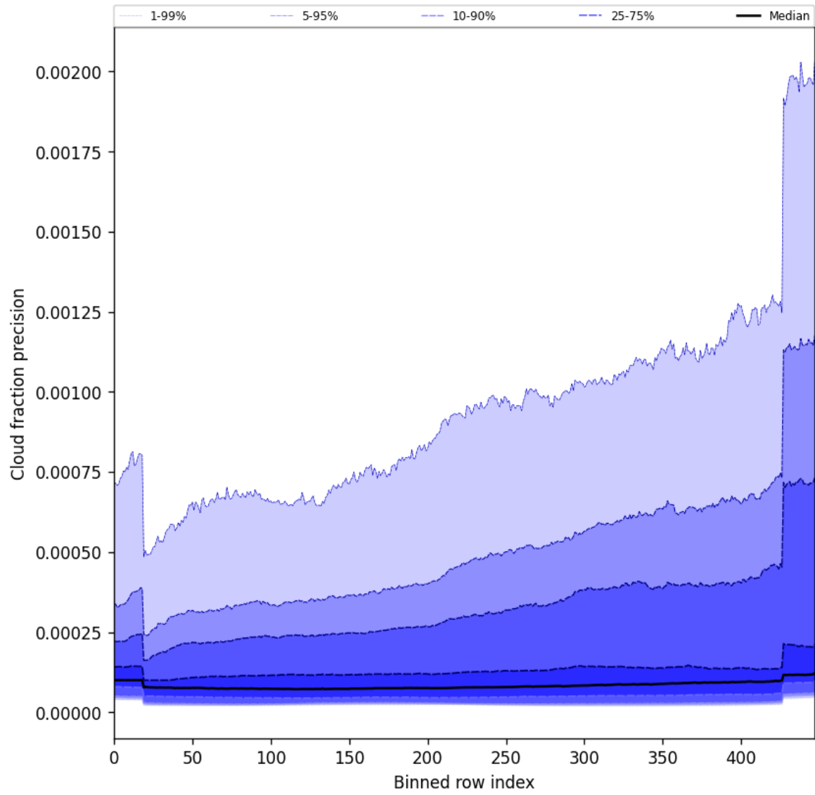
Figure 48: Along track statistics of “Cloud fraction precision” for 2025-06-23 to 2025-06-24
