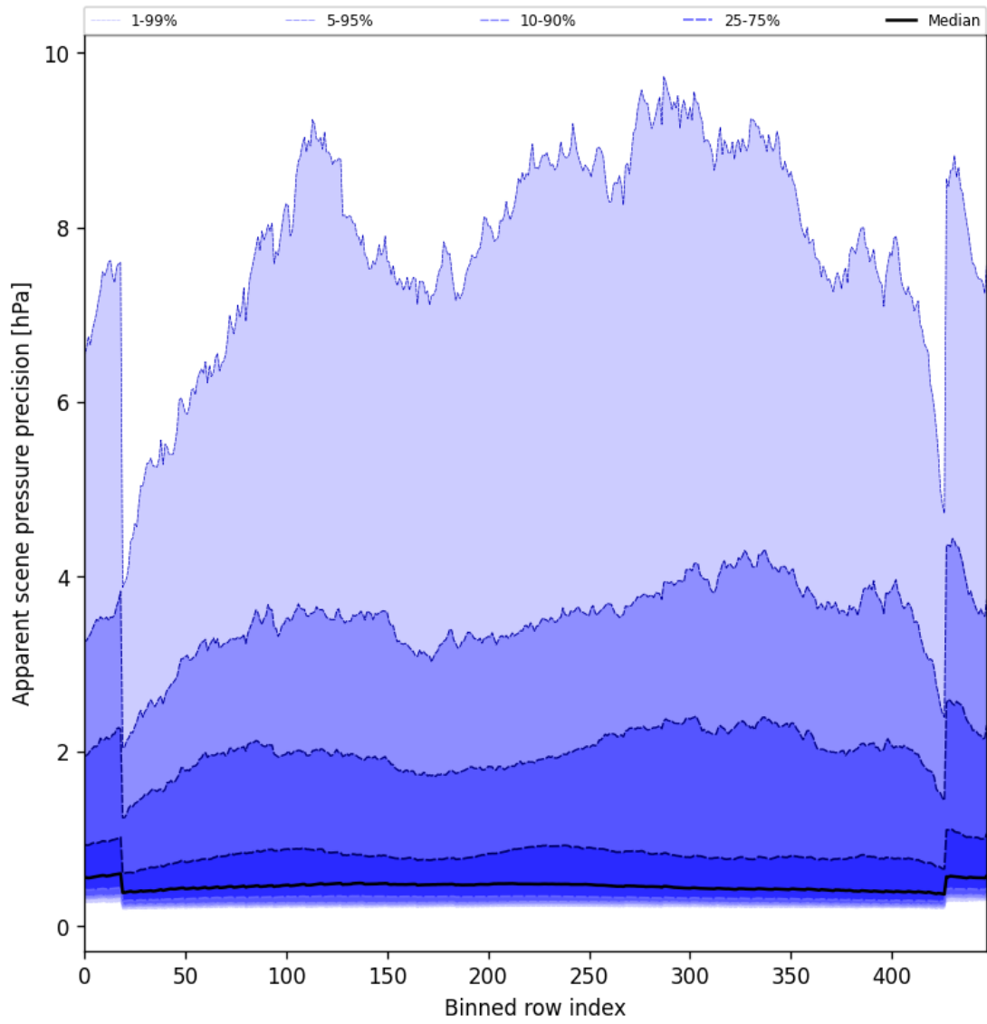
Figure 52: Along track statistics of “Apparent scene pressure precision” for 2025-06-23 to 2025-06-24
