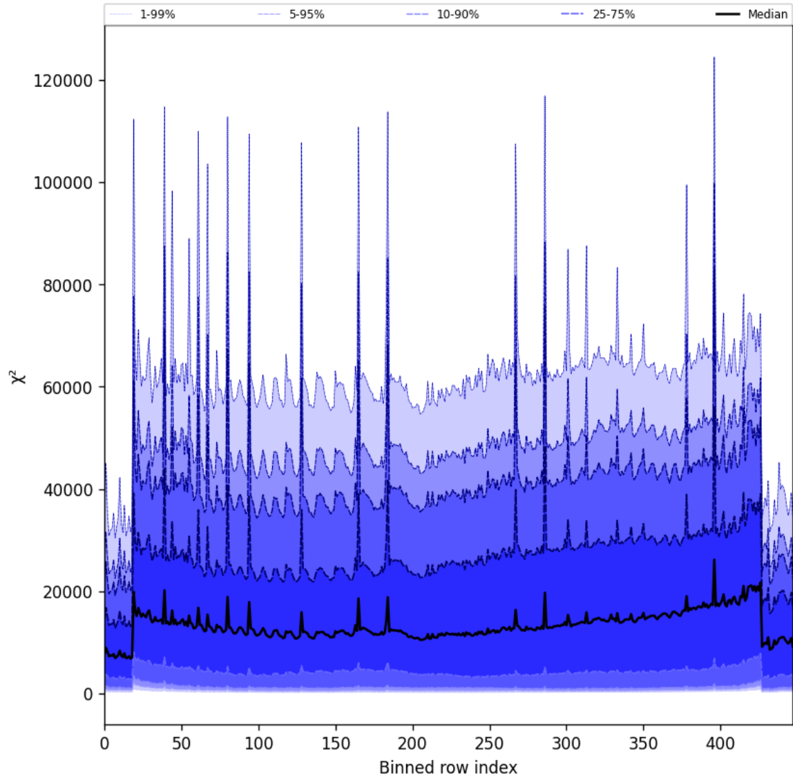
Figure 53: Along track statistics of “ \chi^2 ” for 2025-06-23 to 2025-06-24
