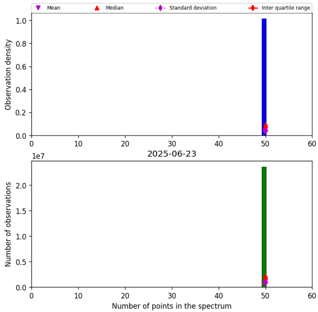
Figure 42: Histogram of “Number of points in the spectrum” for 2025-06-23 to 2025-06-24
