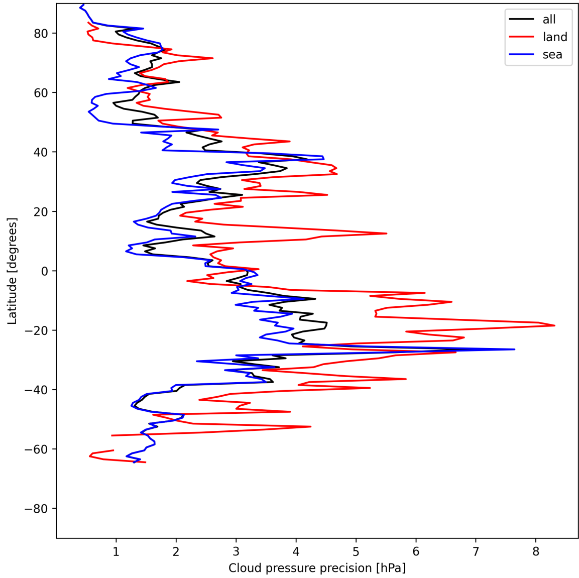
Figure 12: Zonal average of “Cloud pressure precision” for 2025-06-23 to 2025-06-24.
