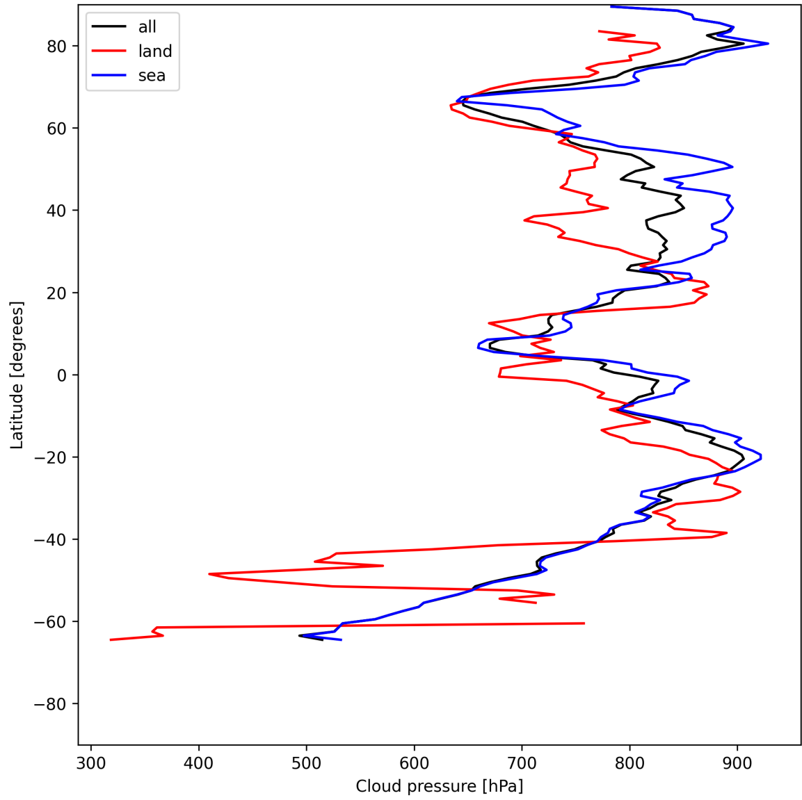
Figure 11: Zonal average of “Cloud pressure” for 2025-06-23 to 2025-06-24.
