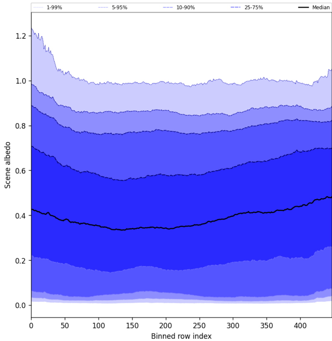
Figure 49: Along track statistics of “Scene albedo” for 2025-06-23 to 2025-06-24
