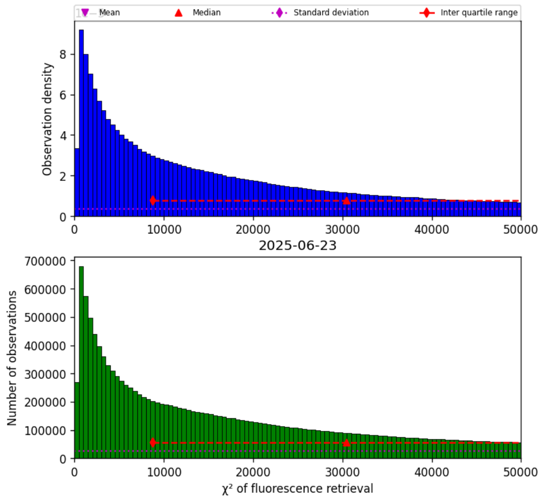
Figure 40: Histogram of “ \chi^2 of fluorescence retrieval” for 2025-06-23 to 2025-06-24
