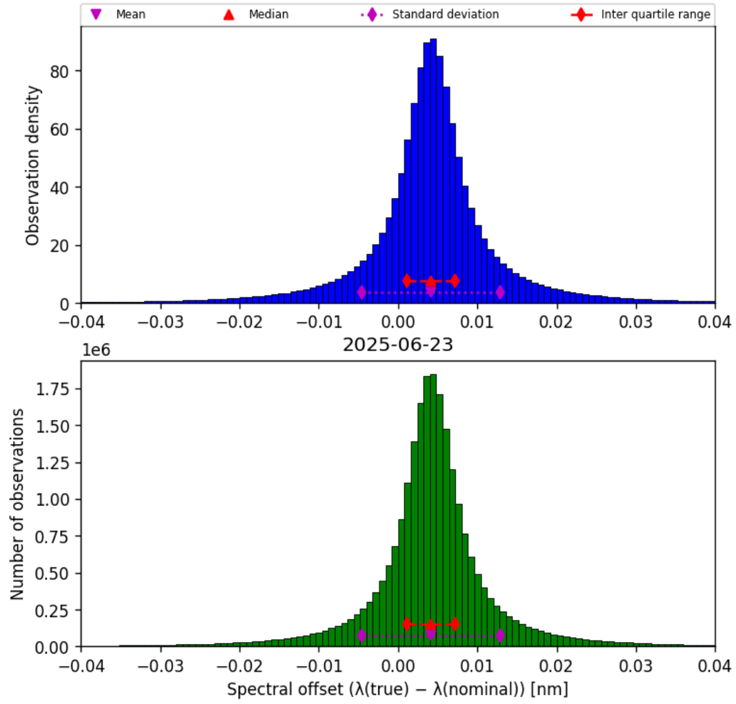
Figure 43: Histogram of “Spectral offset ( \lambda_{\text{true}} - \lambda_{\text{nominal}} )” for 2025-06-23 to 2025-06-24
