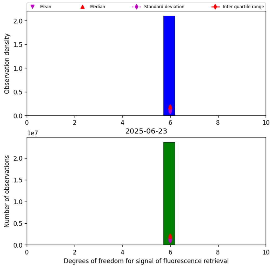
Figure 41: Histogram of “Degrees of freedom for signal of fluorescence retrieval” for 2025-06-23 to 2025-06-24
