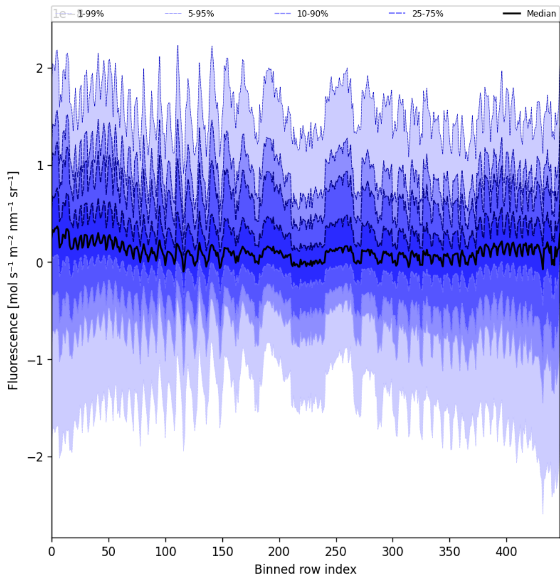
Figure 55: Along track statistics of “Fluorescence” for 2025-06-23 to 2025-06-24
