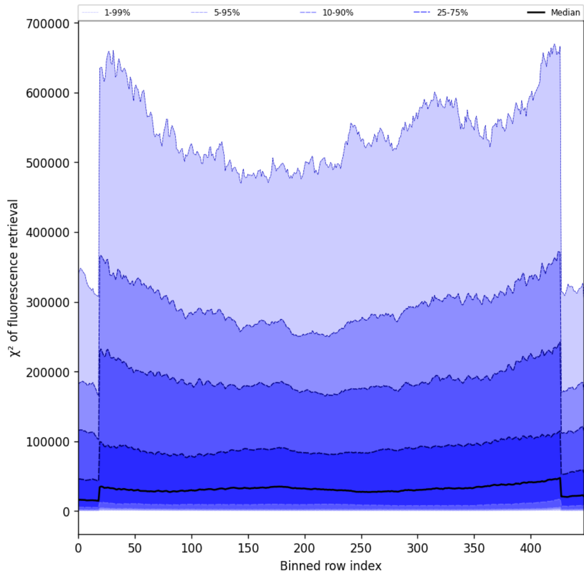
Figure 57: Along track statistics of “ \chi^2 of fluorescence retrieval” for 2025-06-23 to 2025-06-24
