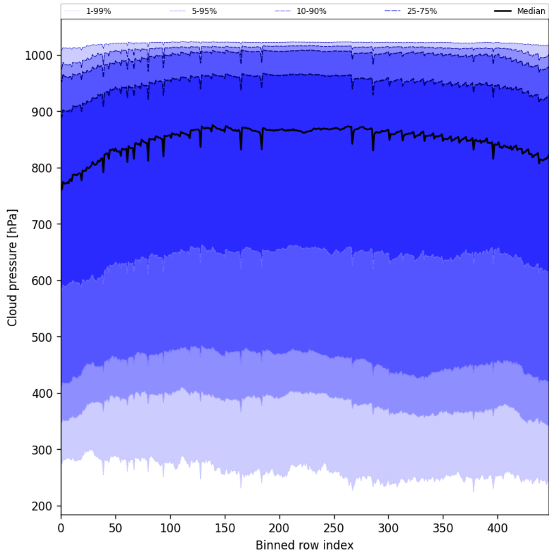
Figure 45: Along track statistics of “Cloud pressure” for 2025-06-23 to 2025-06-24
