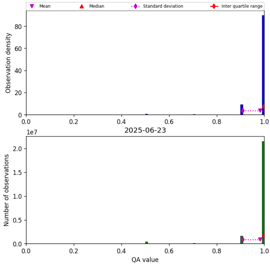
Figure 27: Histogram of “QA value” for 2025-06-23 to 2025-06-24
