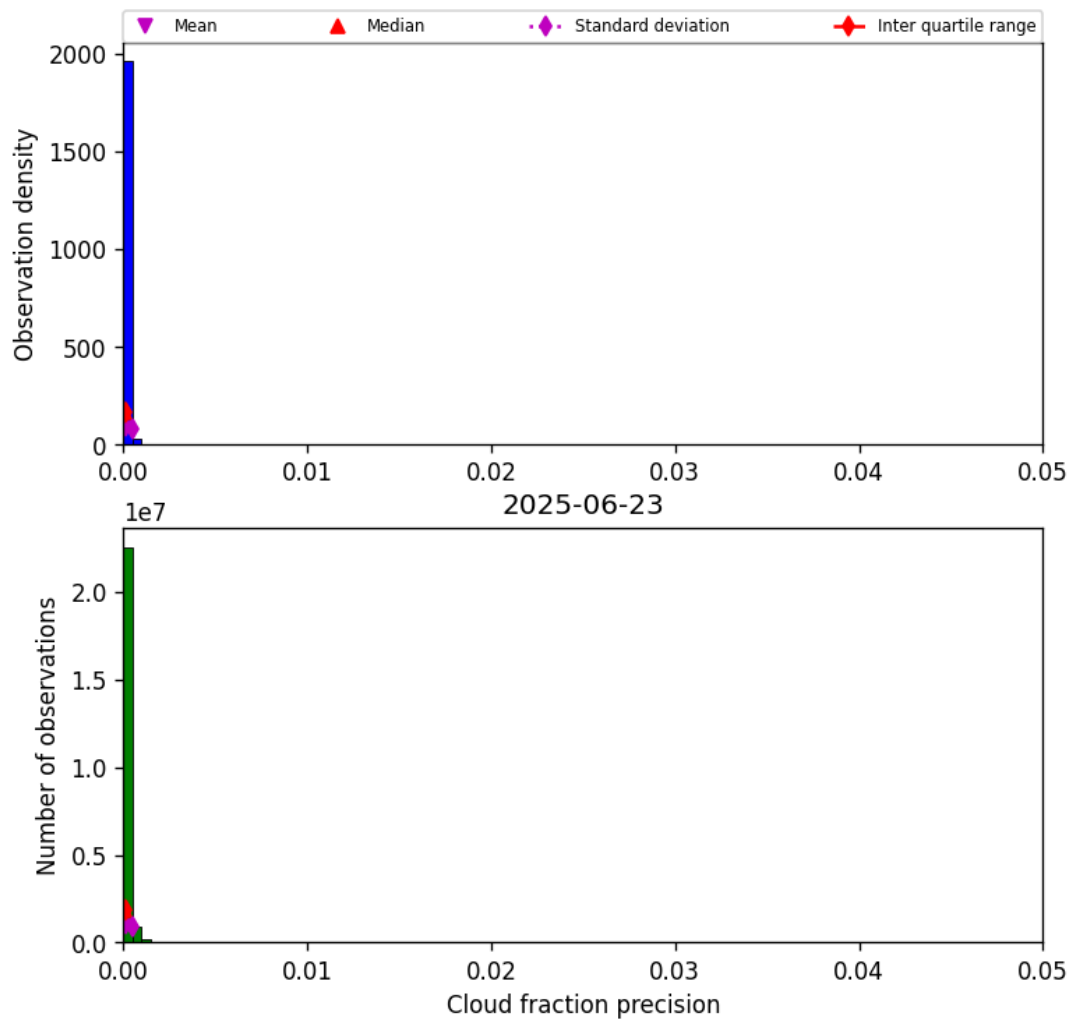
Figure 31: Histogram of “Cloud fraction precision” for 2025-06-23 to 2025-06-24
