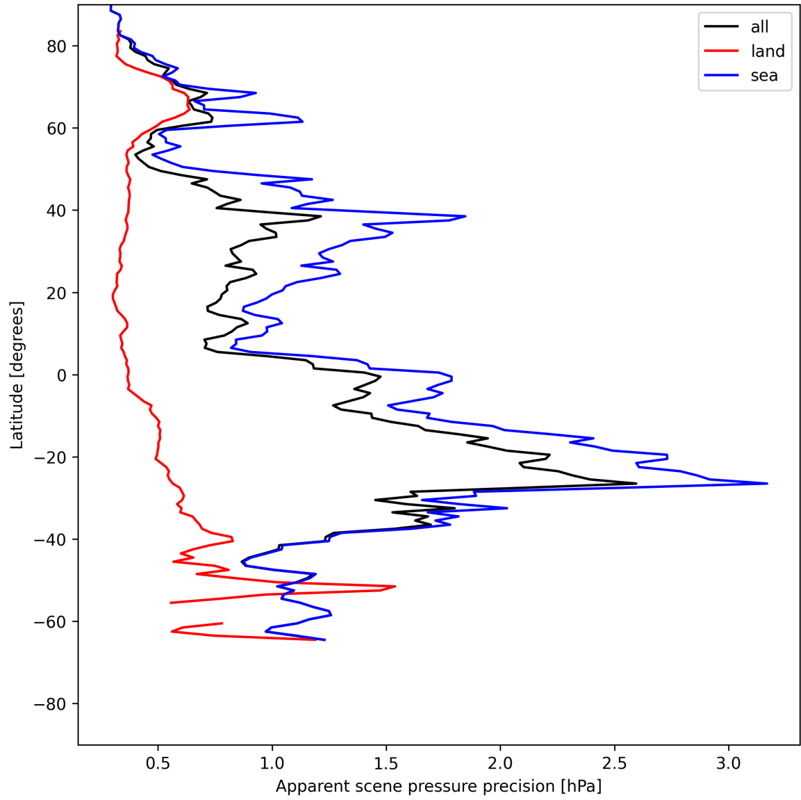
Figure 18: Zonal average of “Apparent scene pressure precision” for 2025-06-23 to 2025-06-24.
