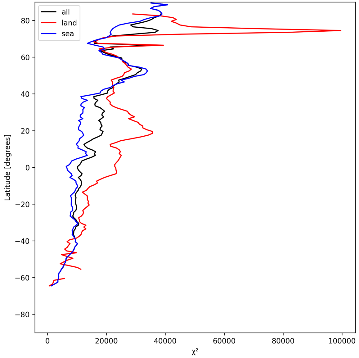
Figure 19: Zonal average of “ \chi^2 ” for 2025-06-23 to 2025-06-24.
