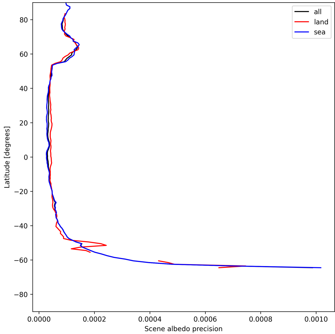
Figure 16: Zonal average of “Scene albedo precision” for 2025-06-23 to 2025-06-24.
