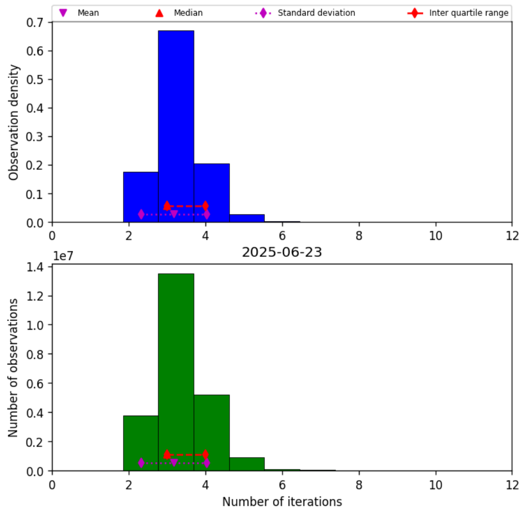
Figure 37: Histogram of “Number of iterations” for 2025-06-23 to 2025-06-24
