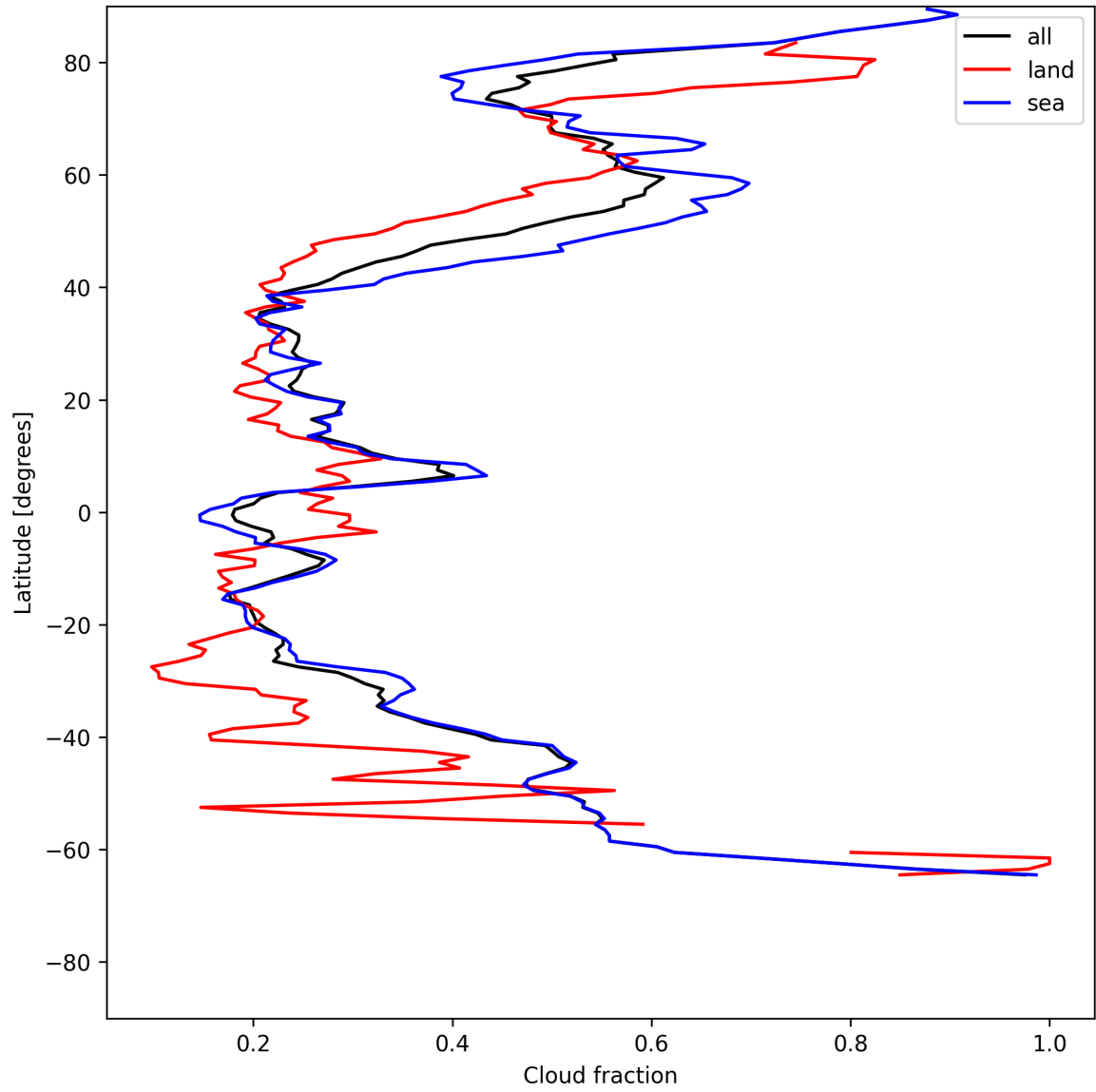
Figure 13: Zonal average of “Cloud fraction” for 2025-06-23 to 2025-06-24.
