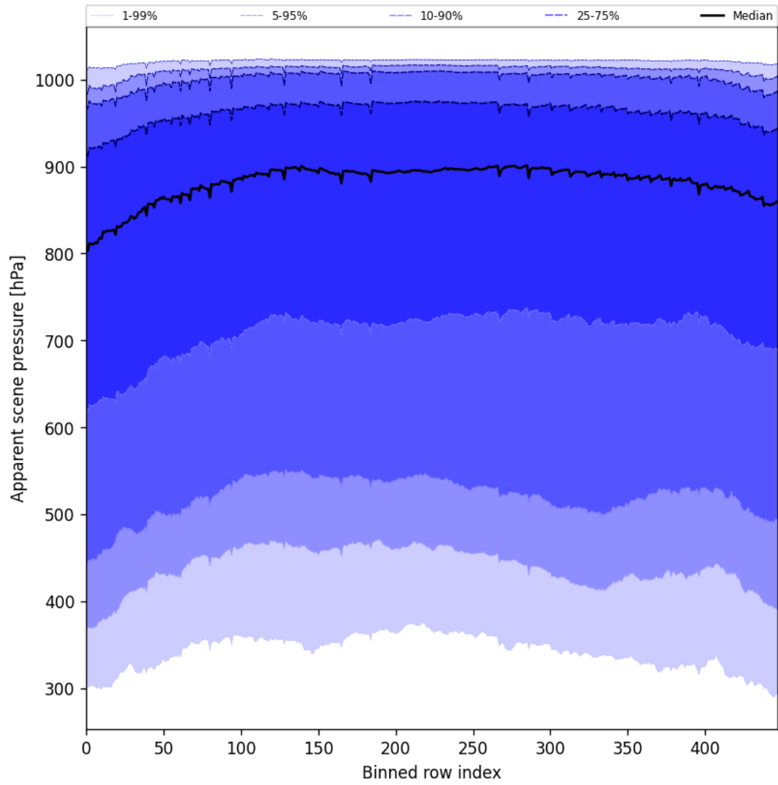
Figure 51: Along track statistics of “Apparent scene pressure” for 2025-06-23 to 2025-06-24
