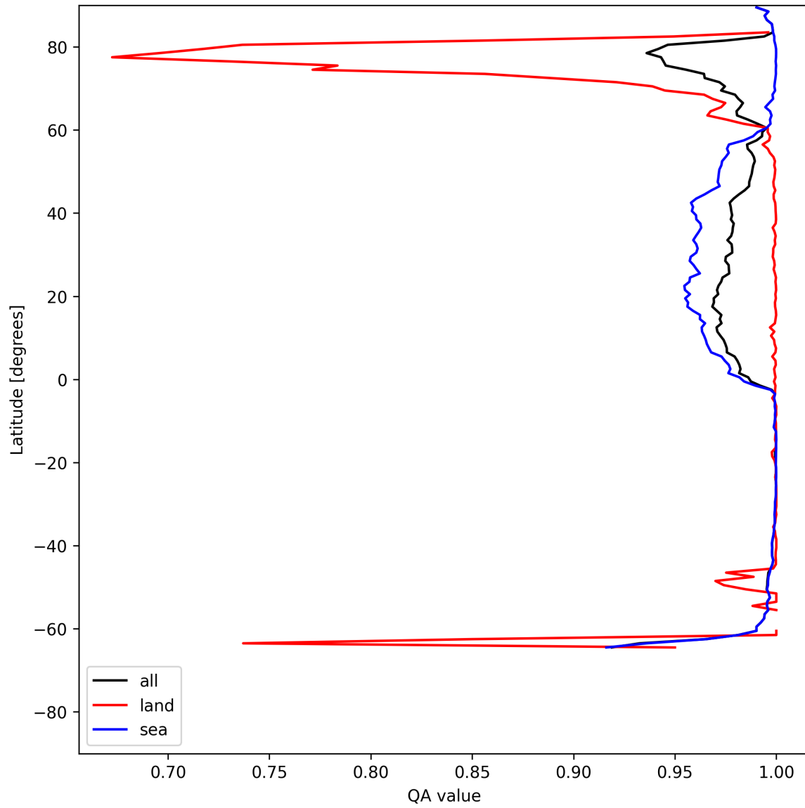
Figure 10: Zonal average of “QA value” for 2025-06-23 to 2025-06-24.
