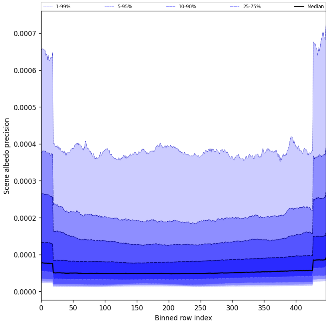
Figure 50: Along track statistics of “Scene albedo precision” for 2025-06-23 to 2025-06-24
