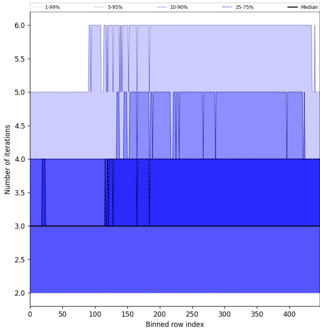
Figure 54: Along track statistics of “Number of iterations” for 2025-06-23 to 2025-06-24
