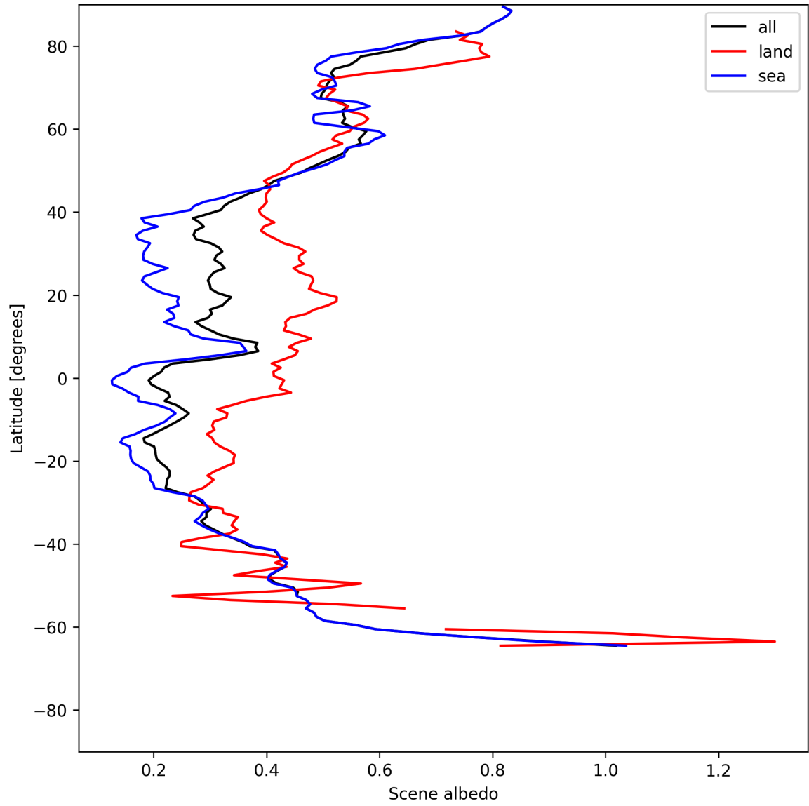
Figure 15: Zonal average of “Scene albedo” for 2025-06-23 to 2025-06-24.
