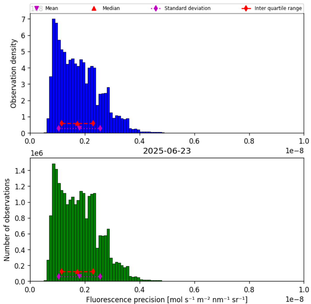
Figure 39: Histogram of “Fluorescence precision” for 2025-06-23 to 2025-06-24
