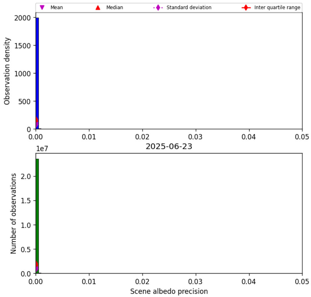
Figure 33: Histogram of “Scene albedo precision” for 2025-06-23 to 2025-06-24
