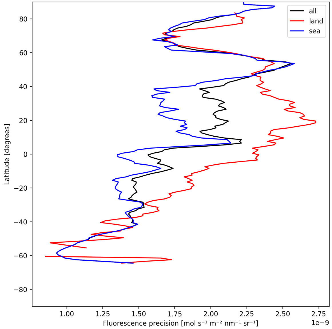
Figure 22: Zonal average of “Fluorescence precision” for 2025-06-23 to 2025-06-24.
