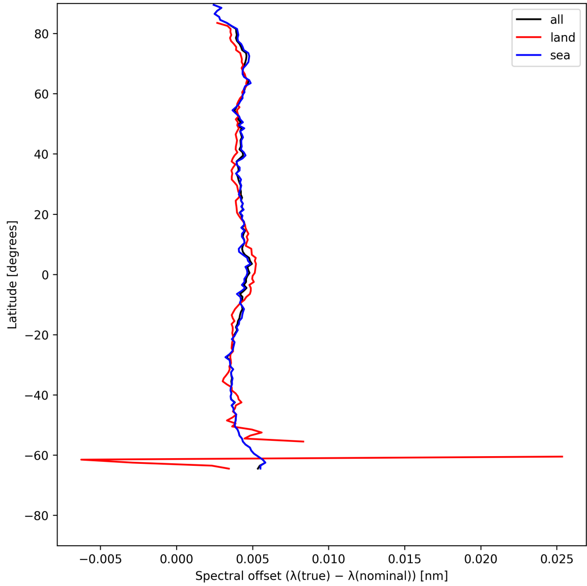
Figure 26: Zonal average of “Spectral offset ( \lambda_{\text{true}} - \lambda_{\text{nominal}} )” for 2025-06-23 to 2025-06-24.
