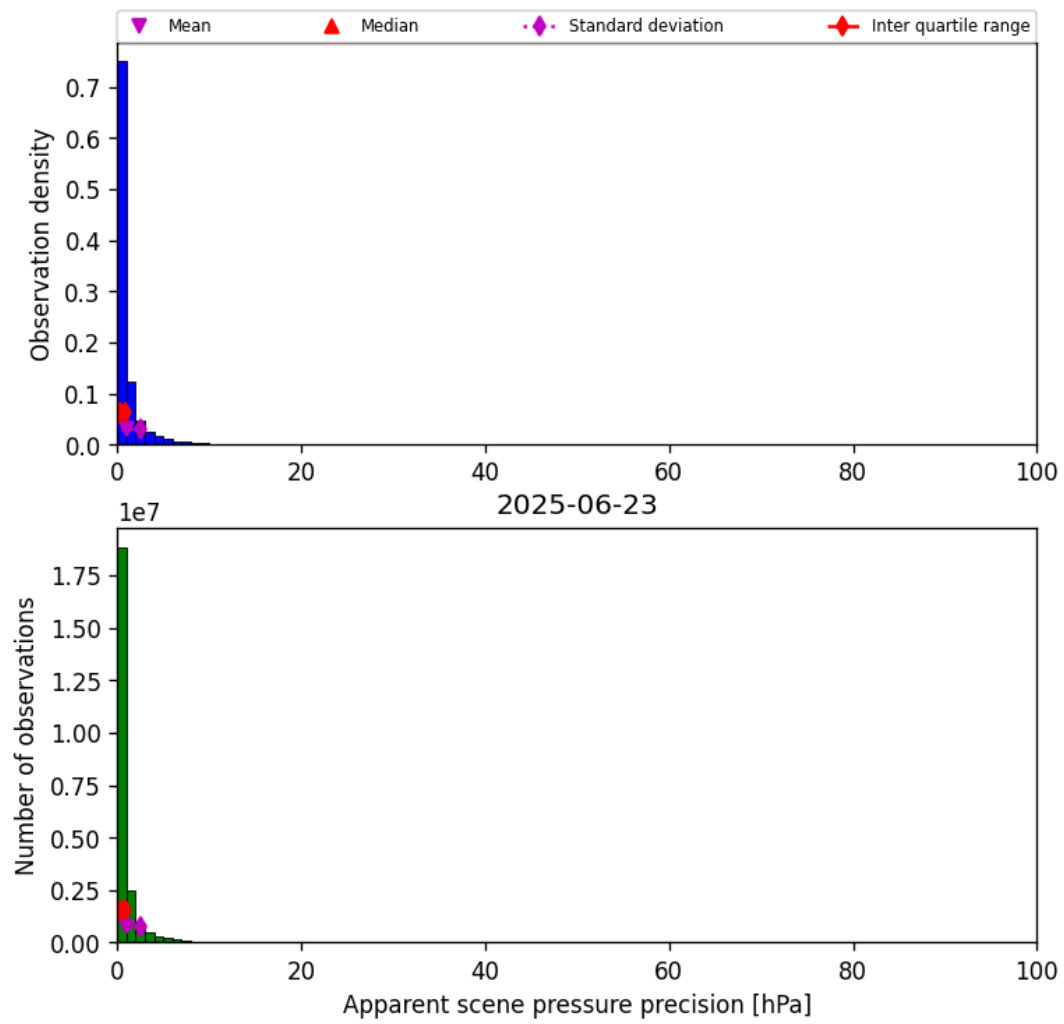
Figure 35: Histogram of “Apparent scene pressure precision” for 2025-06-23 to 2025-06-24
