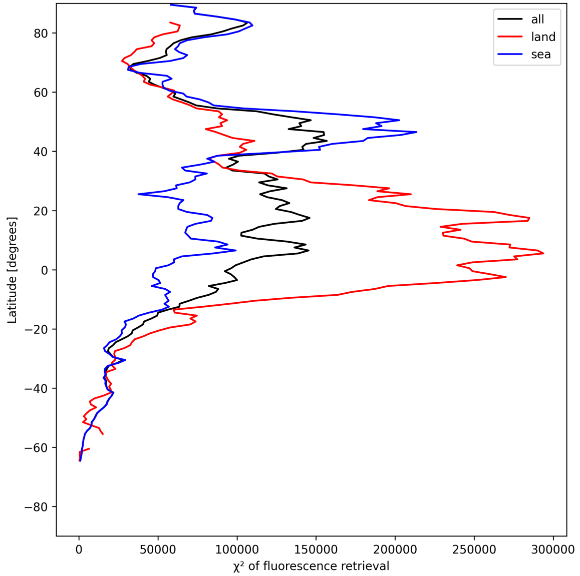
Figure 23: Zonal average of “ \chi^2 of fluorescence retrieval” for 2025-06-23 to 2025-06-24.
