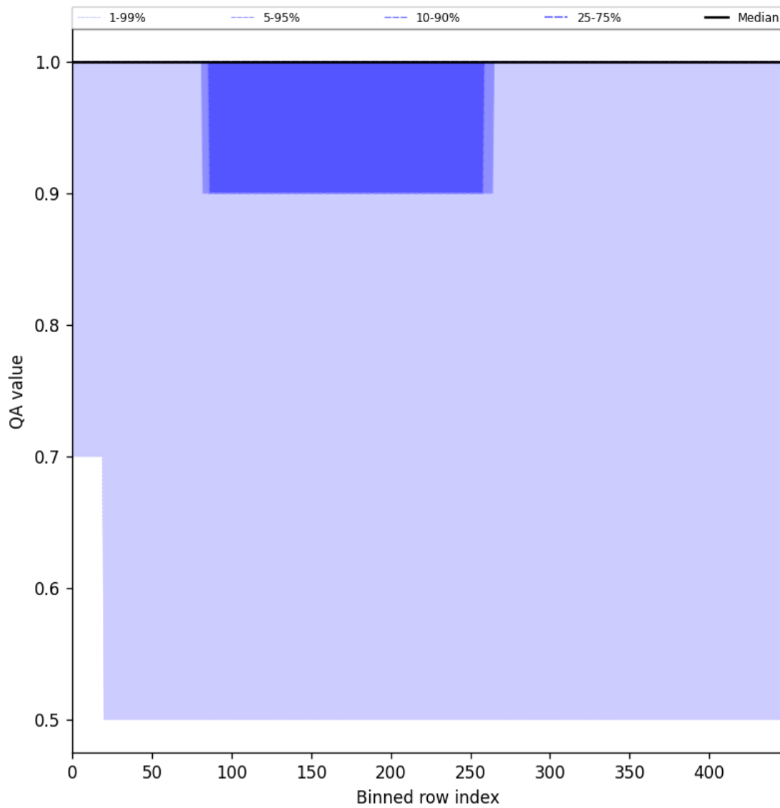
Figure 44: Along track statistics of “QA value” for 2025-06-23 to 2025-06-24
