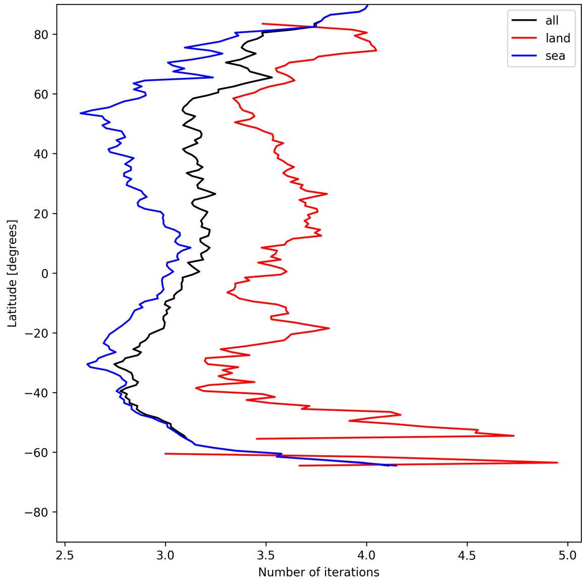
Figure 20: Zonal average of “Number of iterations” for 2025-06-23 to 2025-06-24.
