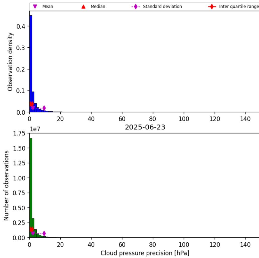
Figure 29: Histogram of “Cloud pressure precision” for 2025-06-23 to 2025-06-24
