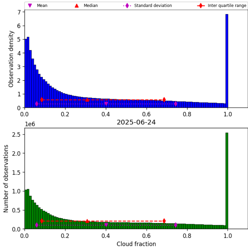
Figure 30: Histogram of “Cloud fraction” for 2025-06-24 to 2025-06-25
