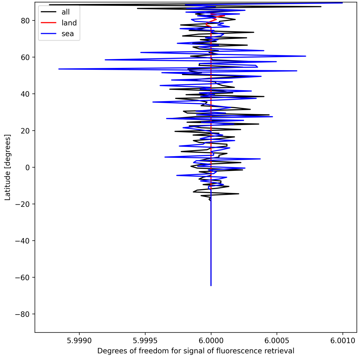
Figure 24: Zonal average of “Degrees of freedom for signal of fluorescence retrieval” for 2025-06-24 to 2025-06-25.
