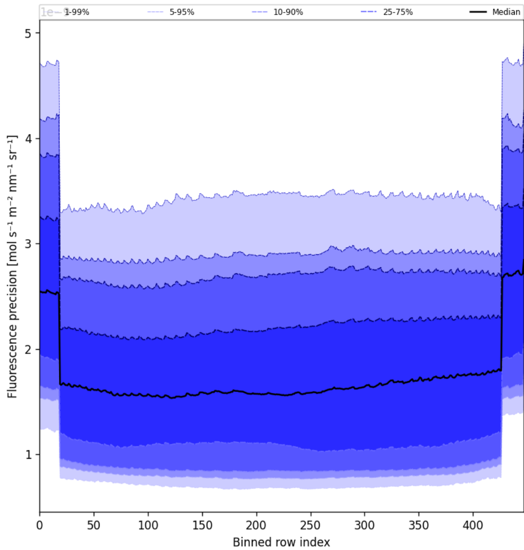
Figure 56: Along track statistics of “Fluorescence precision” for 2025-06-24 to 2025-06-25
