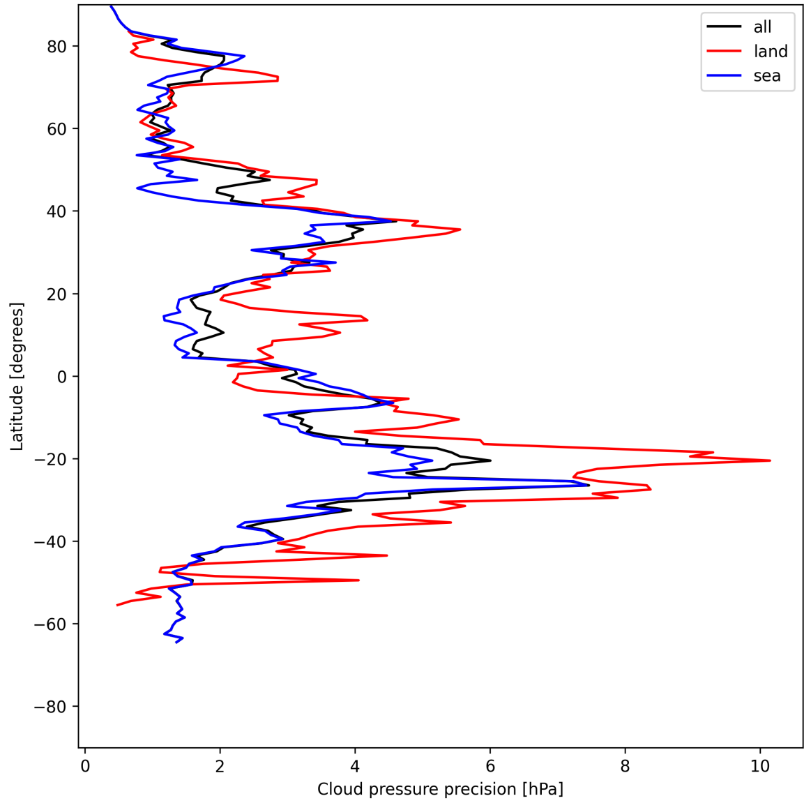
Figure 12: Zonal average of "Cloud pressure precision" for 2025-06-24 to 2025-06-25.
