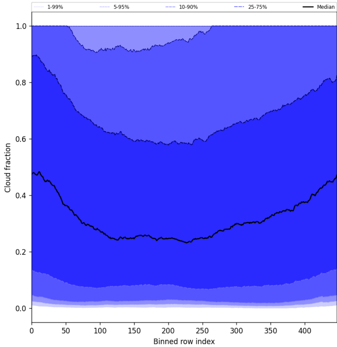
Figure 47: Along track statistics of “Cloud fraction” for 2025-06-24 to 2025-06-25
