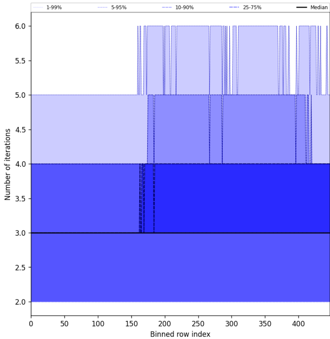
Figure 54: Along track statistics of “Number of iterations” for 2025-06-24 to 2025-06-25
