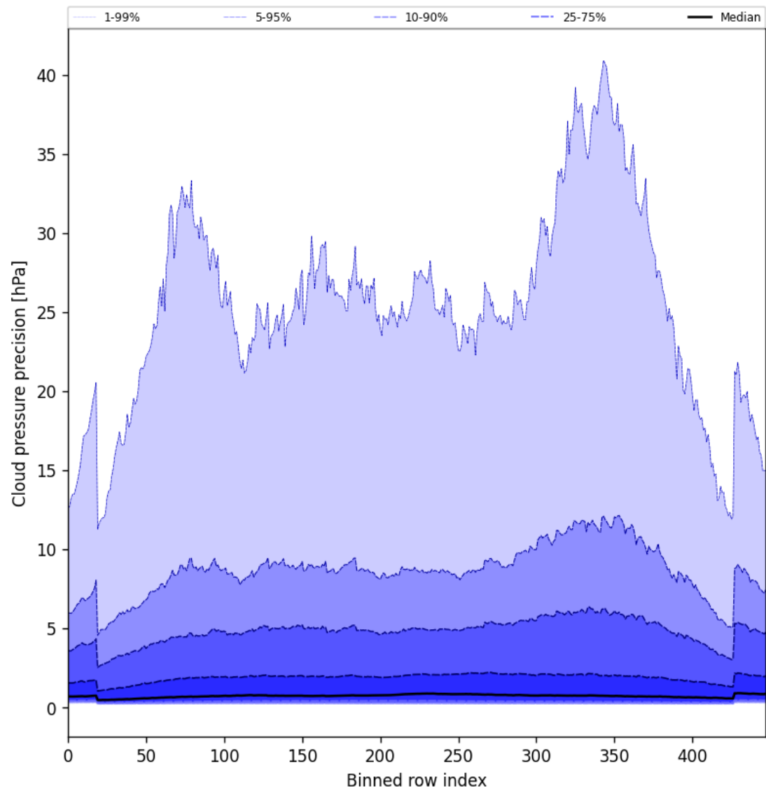
Figure 46: Along track statistics of “Cloud pressure precision” for 2025-06-24 to 2025-06-25
