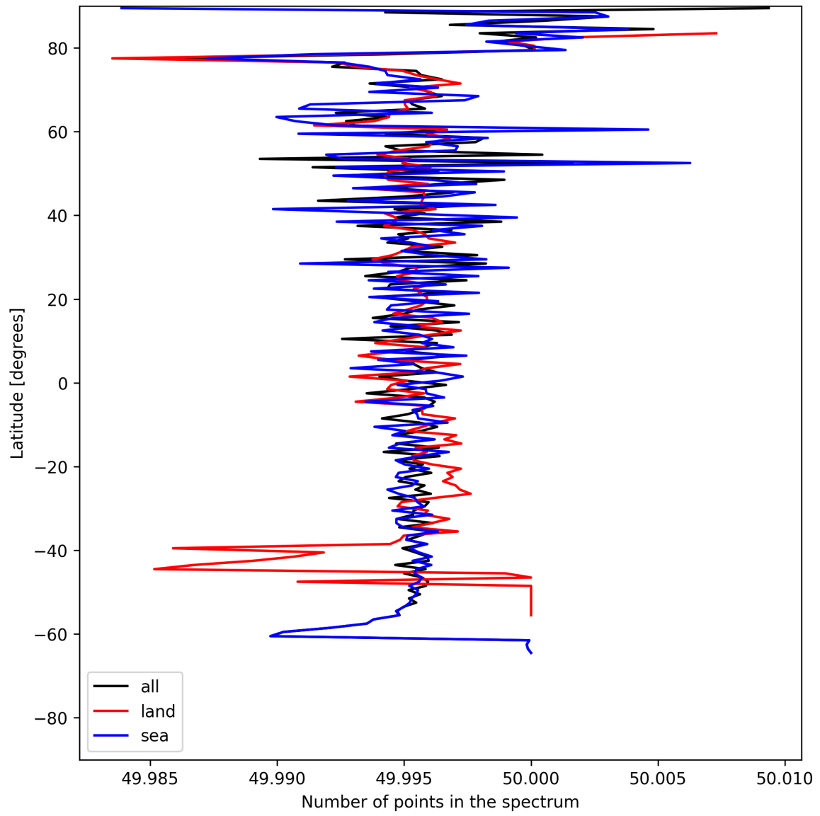
Figure 25: Zonal average of “Number of points in the spectrum” for 2025-06-24 to 2025-06-25.
