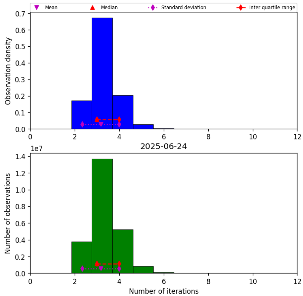
Figure 37: Histogram of “Number of iterations” for 2025-06-24 to 2025-06-25
