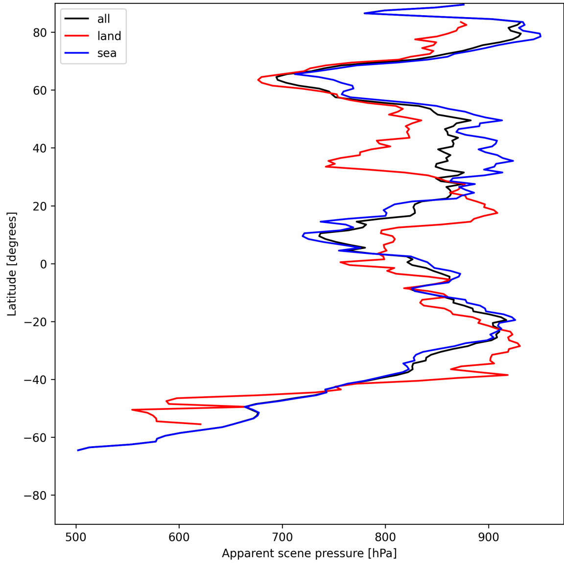
Figure 17: Zonal average of “Apparent scene pressure” for 2025-06-24 to 2025-06-25.
