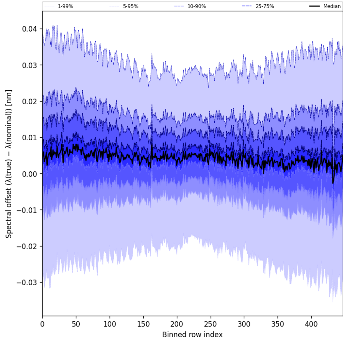
Figure 60: Along track statistics of “Spectral offset ( \lambda_{\text{true}} - \lambda_{\text{nominal}} )” for 2025-06-24 to 2025-06-25
