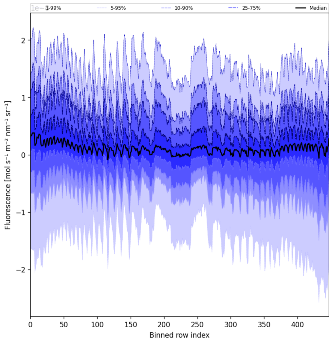
Figure 55: Along track statistics of “Fluorescence” for 2025-06-24 to 2025-06-25
