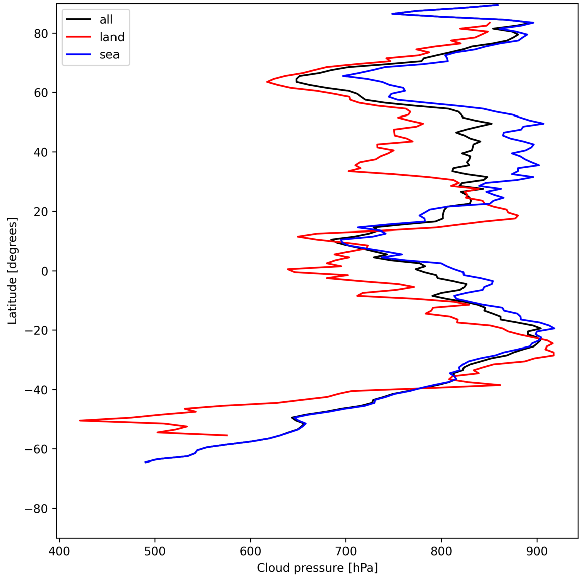
Figure 11: Zonal average of “Cloud pressure” for 2025-06-24 to 2025-06-25.
