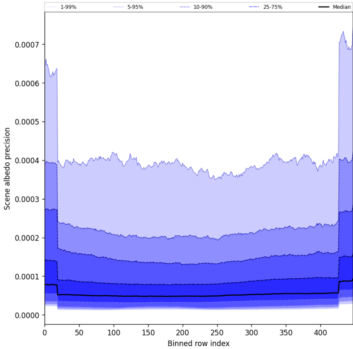
Figure 50: Along track statistics of “Scene albedo precision” for 2025-06-24 to 2025-06-25
