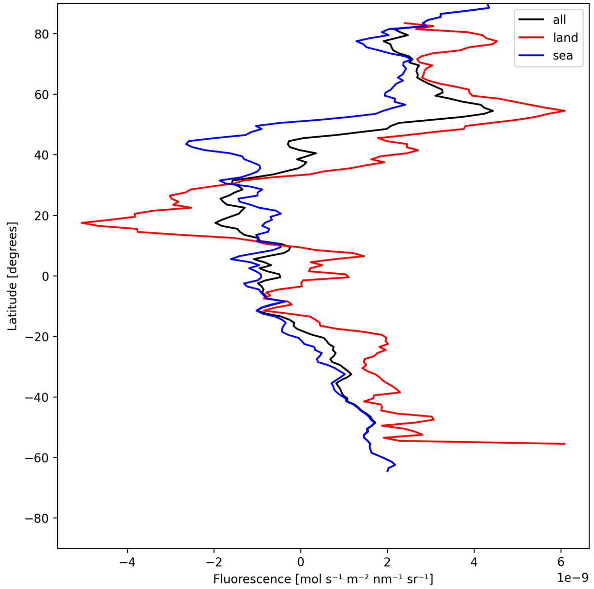
Figure 21: Zonal average of “Fluorescence” for 2025-06-24 to 2025-06-25.
