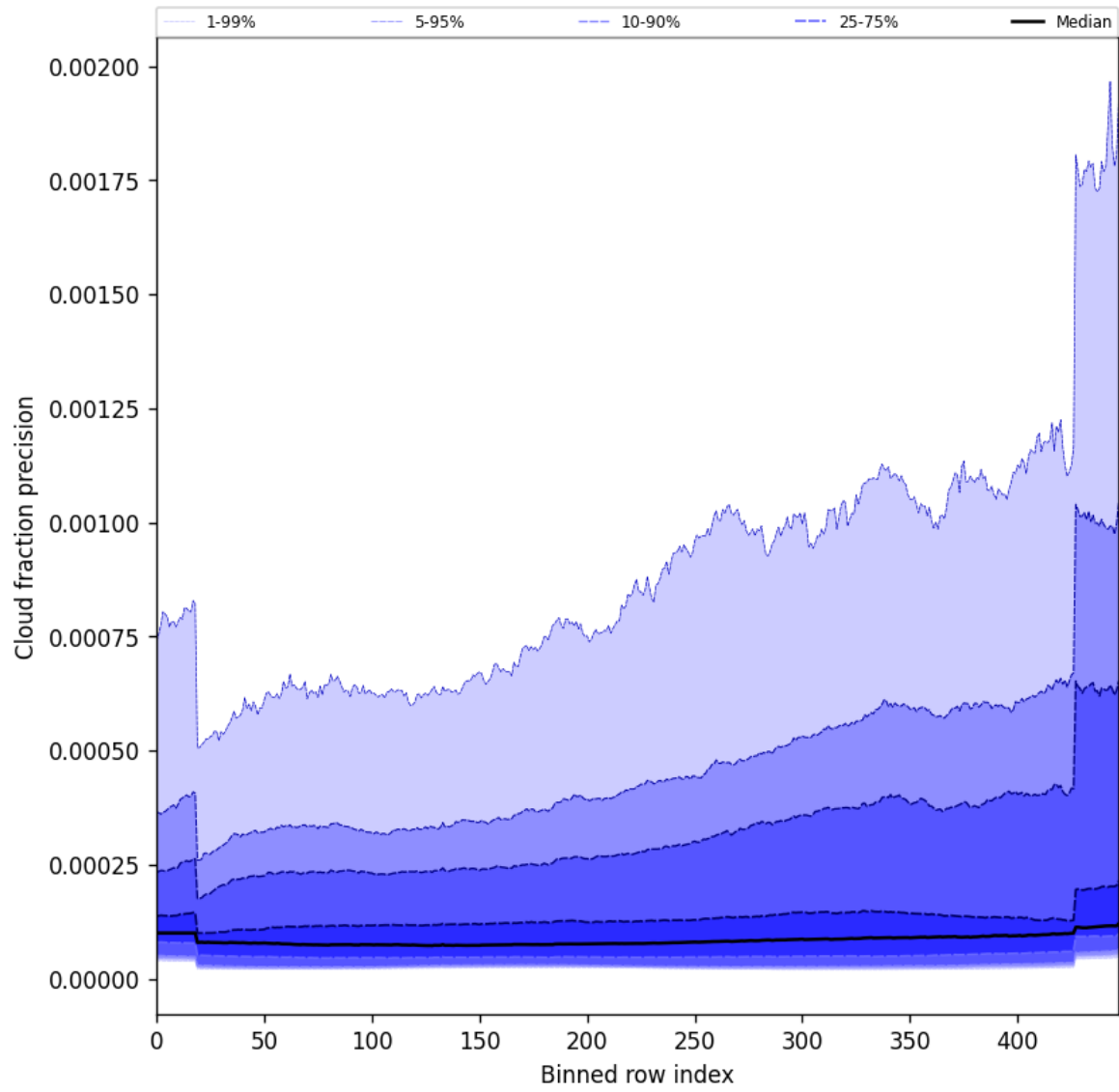
Figure 48: Along track statistics of “Cloud fraction precision” for 2025-06-24 to 2025-06-25
