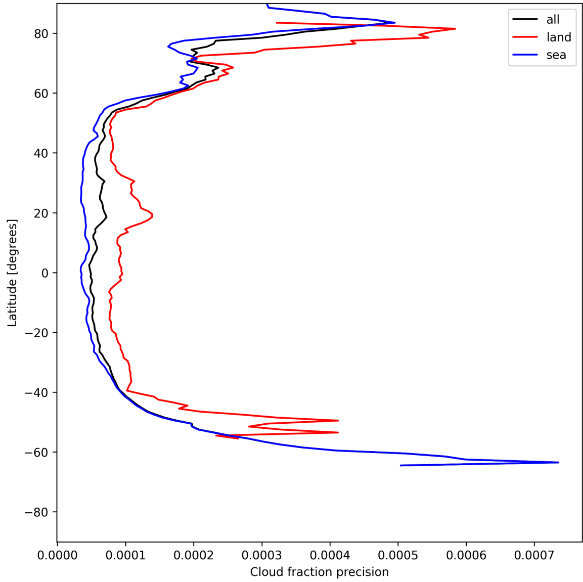
Figure 14: Zonal average of “Cloud fraction precision” for 2025-06-24 to 2025-06-25.
