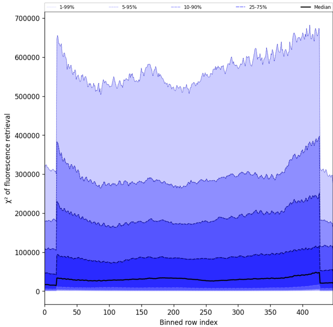
Figure 57: Along track statistics of “ \chi^2 of fluorescence retrieval” for 2025-06-24 to 2025-06-25
