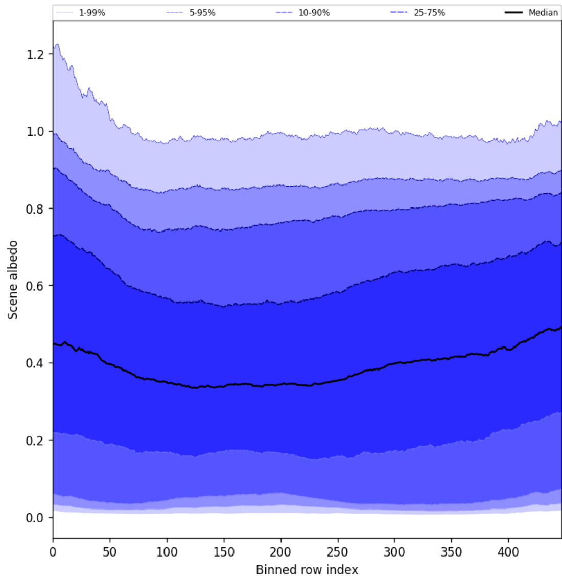
Figure 49: Along track statistics of “Scene albedo” for 2025-06-24 to 2025-06-25
