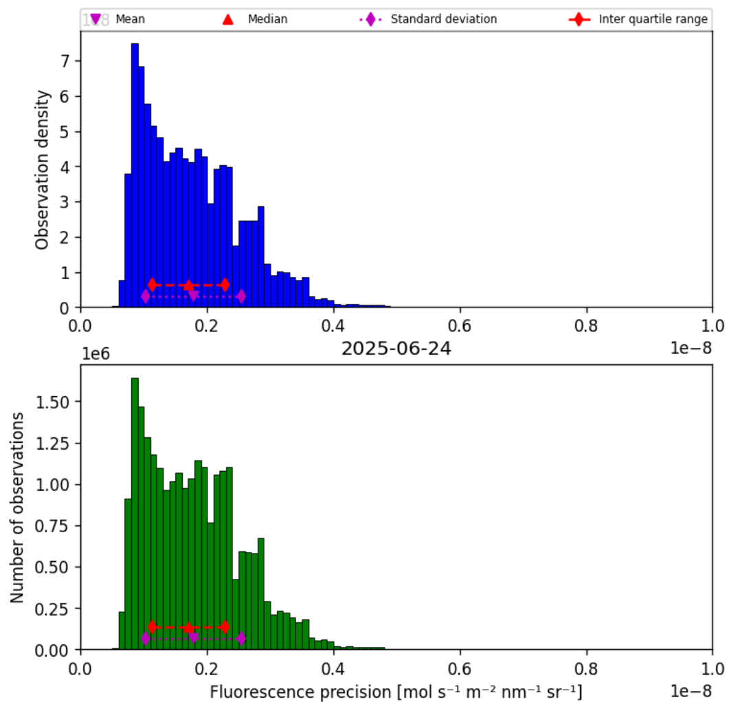
Figure 39: Histogram of “Fluorescence precision” for 2025-06-24 to 2025-06-25
