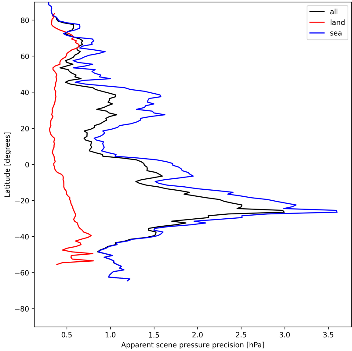
Figure 18: Zonal average of “Apparent scene pressure precision” for 2025-06-24 to 2025-06-25.
