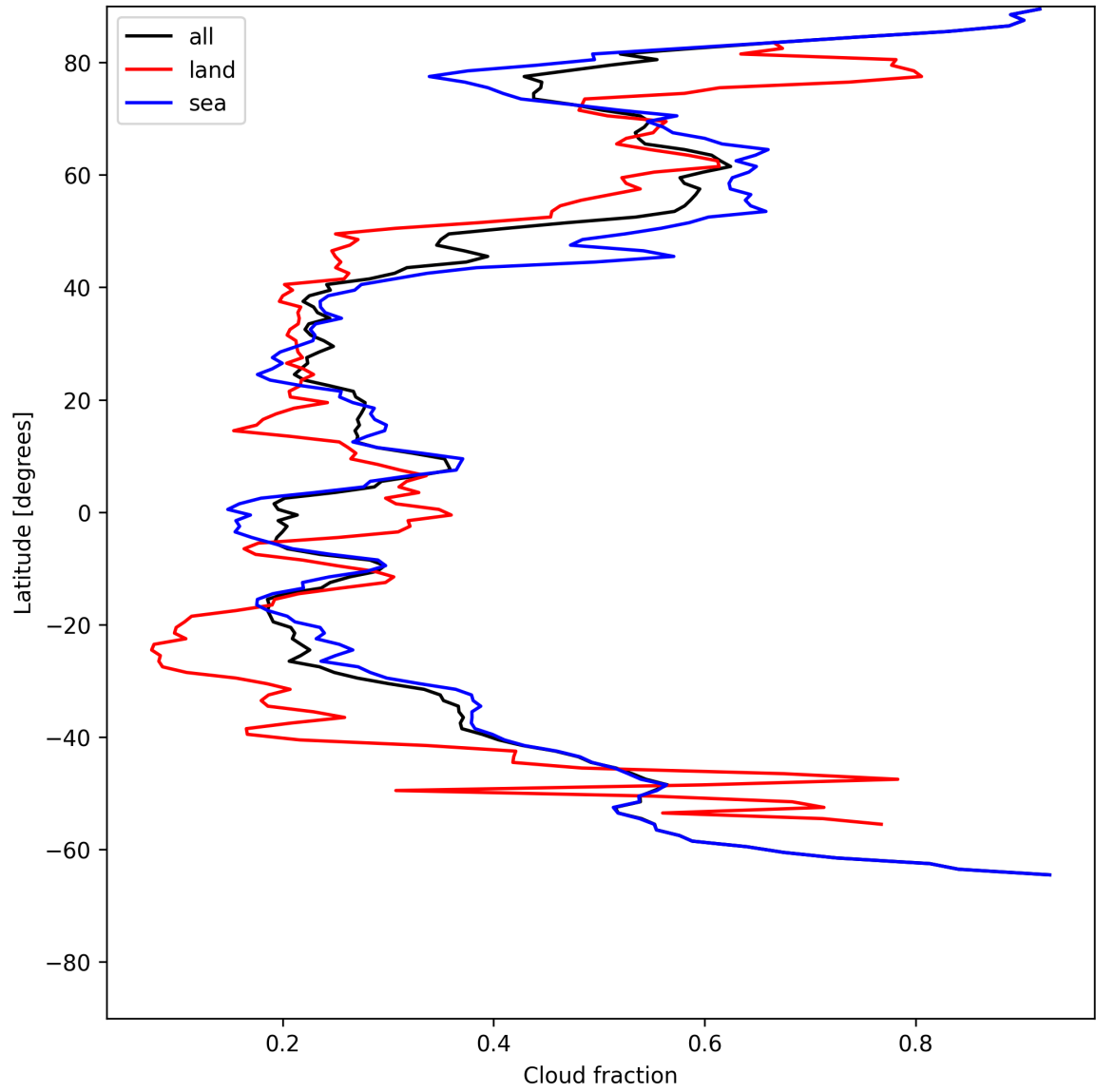
Figure 13: Zonal average of “Cloud fraction” for 2025-06-24 to 2025-06-25.
