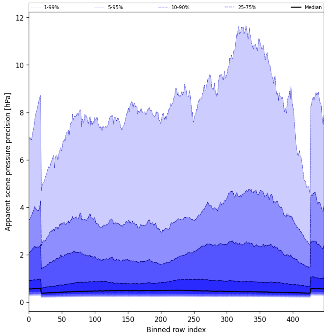
Figure 52: Along track statistics of “Apparent scene pressure precision” for 2025-06-24 to 2025-06-25
