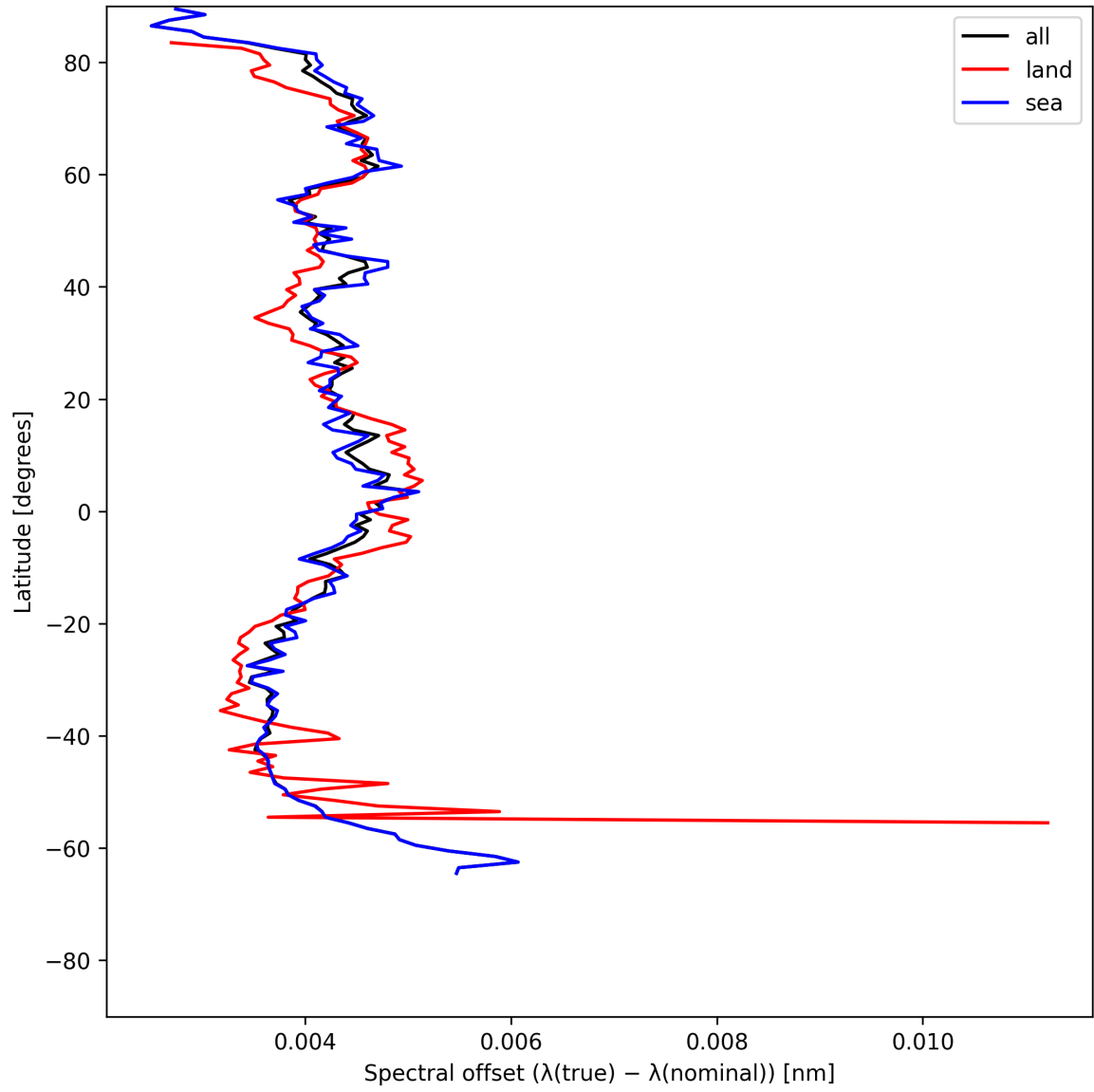
Figure 26: Zonal average of “Spectral offset ( \lambda_{\text{true}} - \lambda_{\text{nominal}} )” for 2025-06-24 to 2025-06-25.
