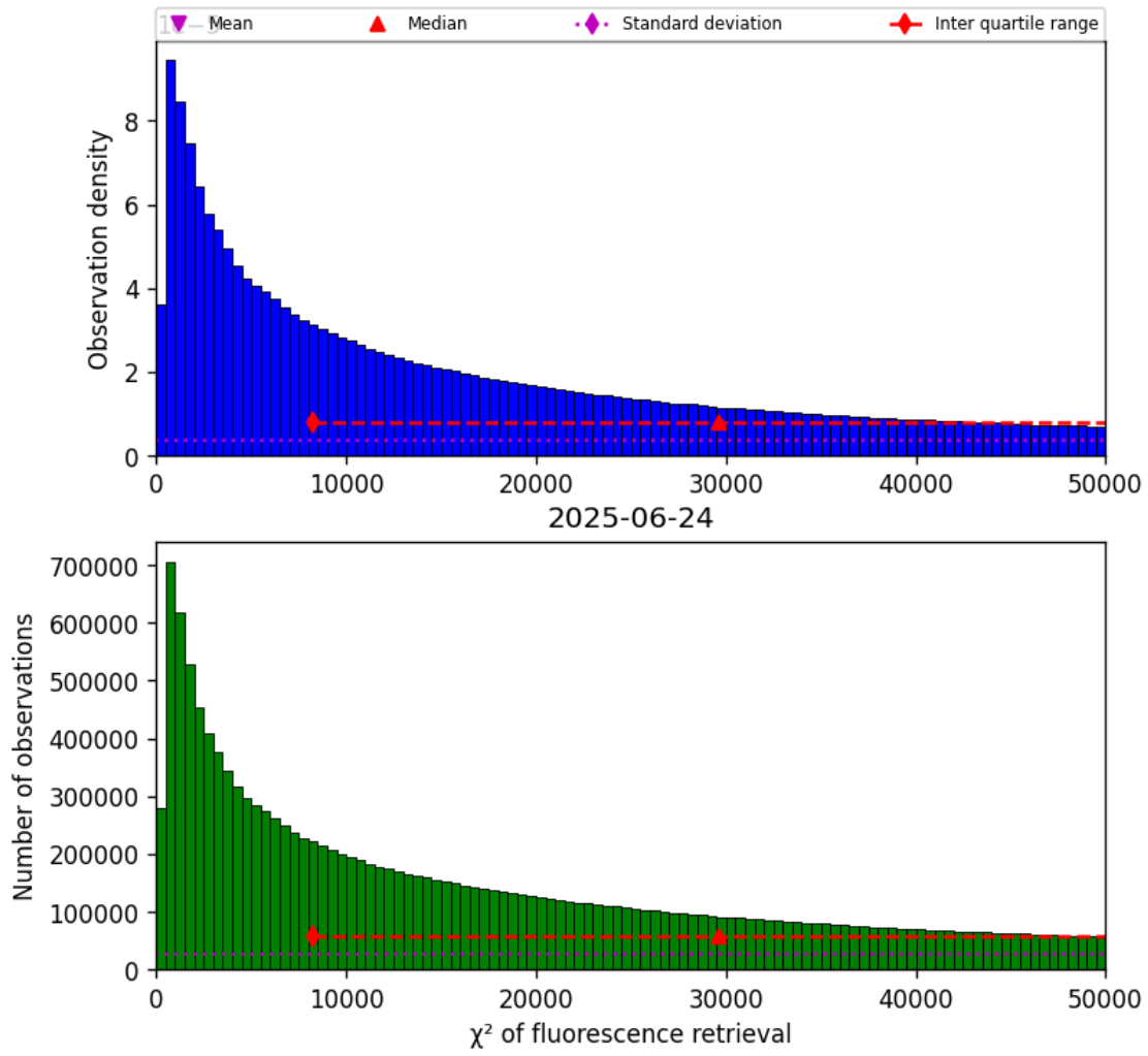
Figure 40: Histogram of “ \chi^2 of fluorescence retrieval” for 2025-06-24 to 2025-06-25
