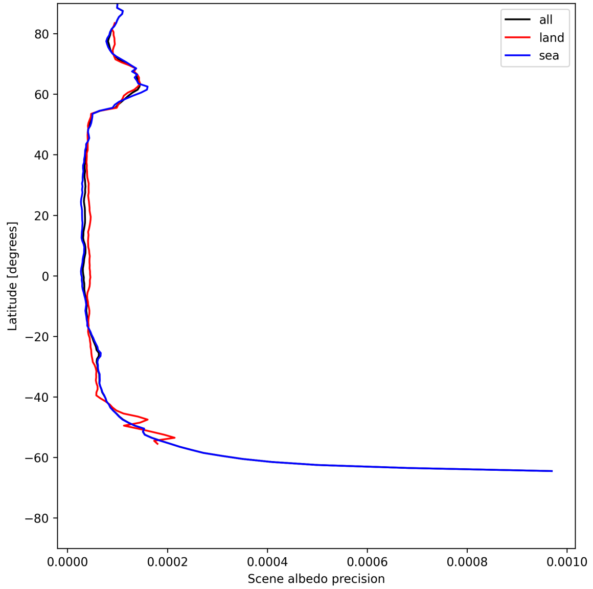
Figure 16: Zonal average of “Scene albedo precision” for 2025-06-24 to 2025-06-25.
