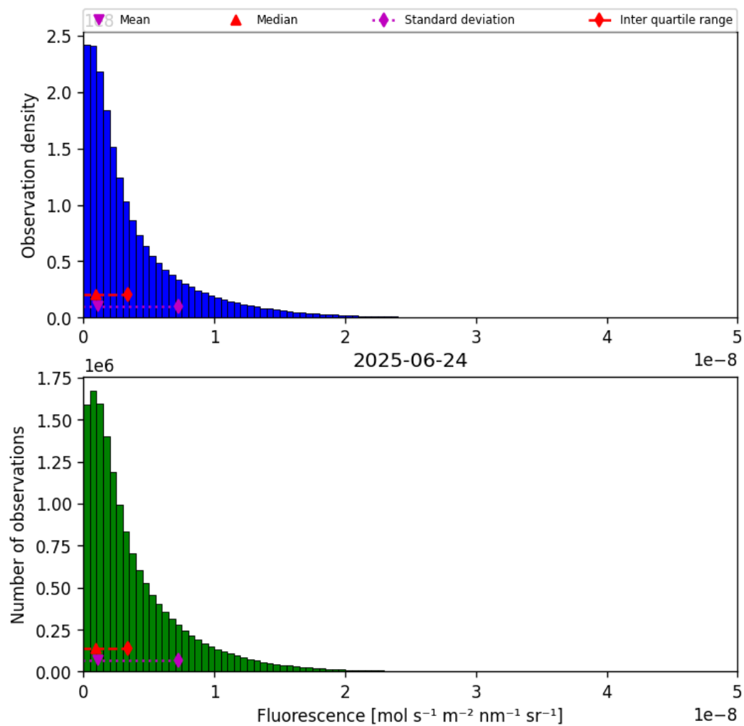
Figure 38: Histogram of “Fluorescence” for 2025-06-24 to 2025-06-25
