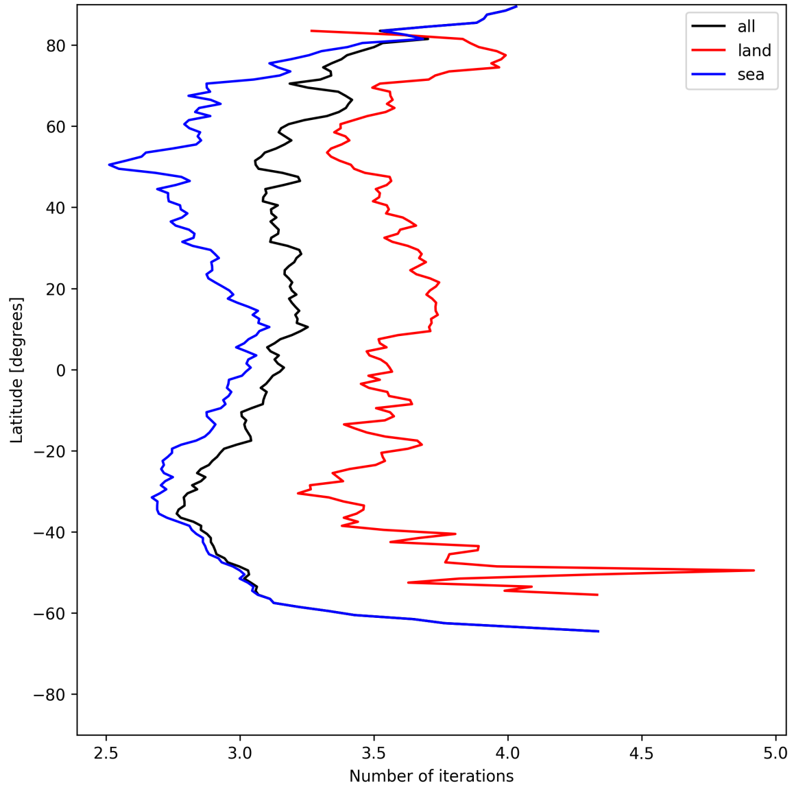
Figure 20: Zonal average of “Number of iterations” for 2025-06-24 to 2025-06-25.
