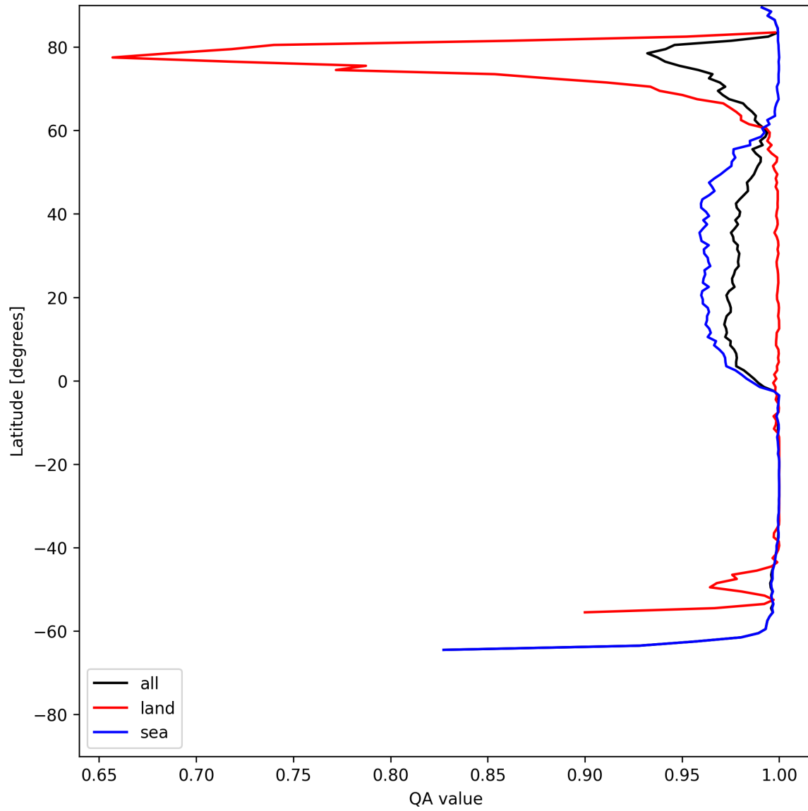
Figure 10: Zonal average of “QA value” for 2025-06-24 to 2025-06-25.
