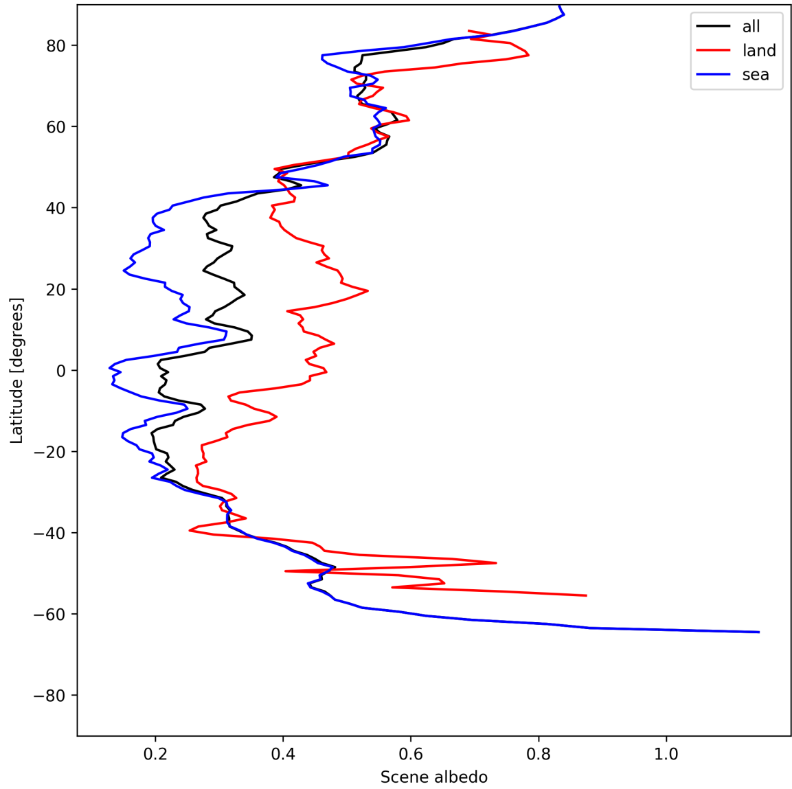
Figure 15: Zonal average of “Scene albedo” for 2025-06-24 to 2025-06-25.
