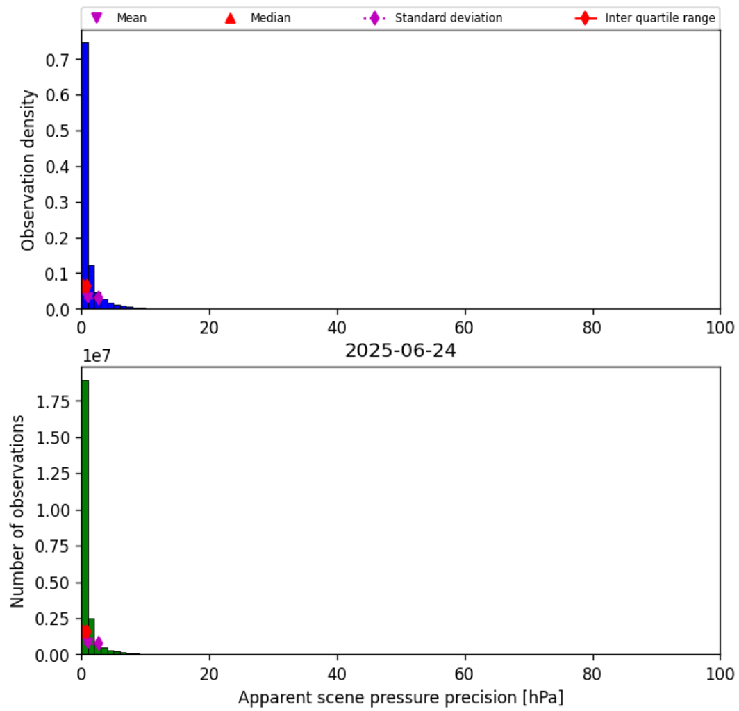
Figure 35: Histogram of “Apparent scene pressure precision” for 2025-06-24 to 2025-06-25
