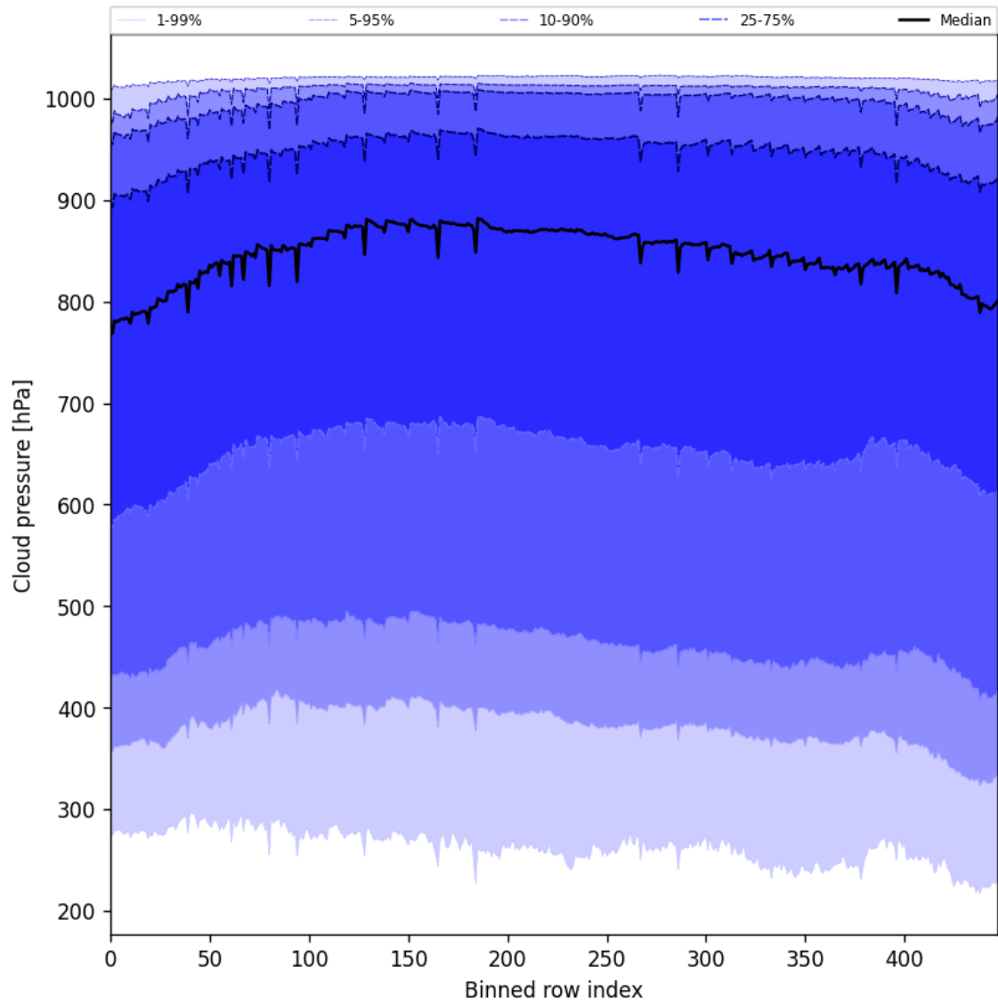
Figure 45: Along track statistics of “Cloud pressure” for 2025-06-24 to 2025-06-25
