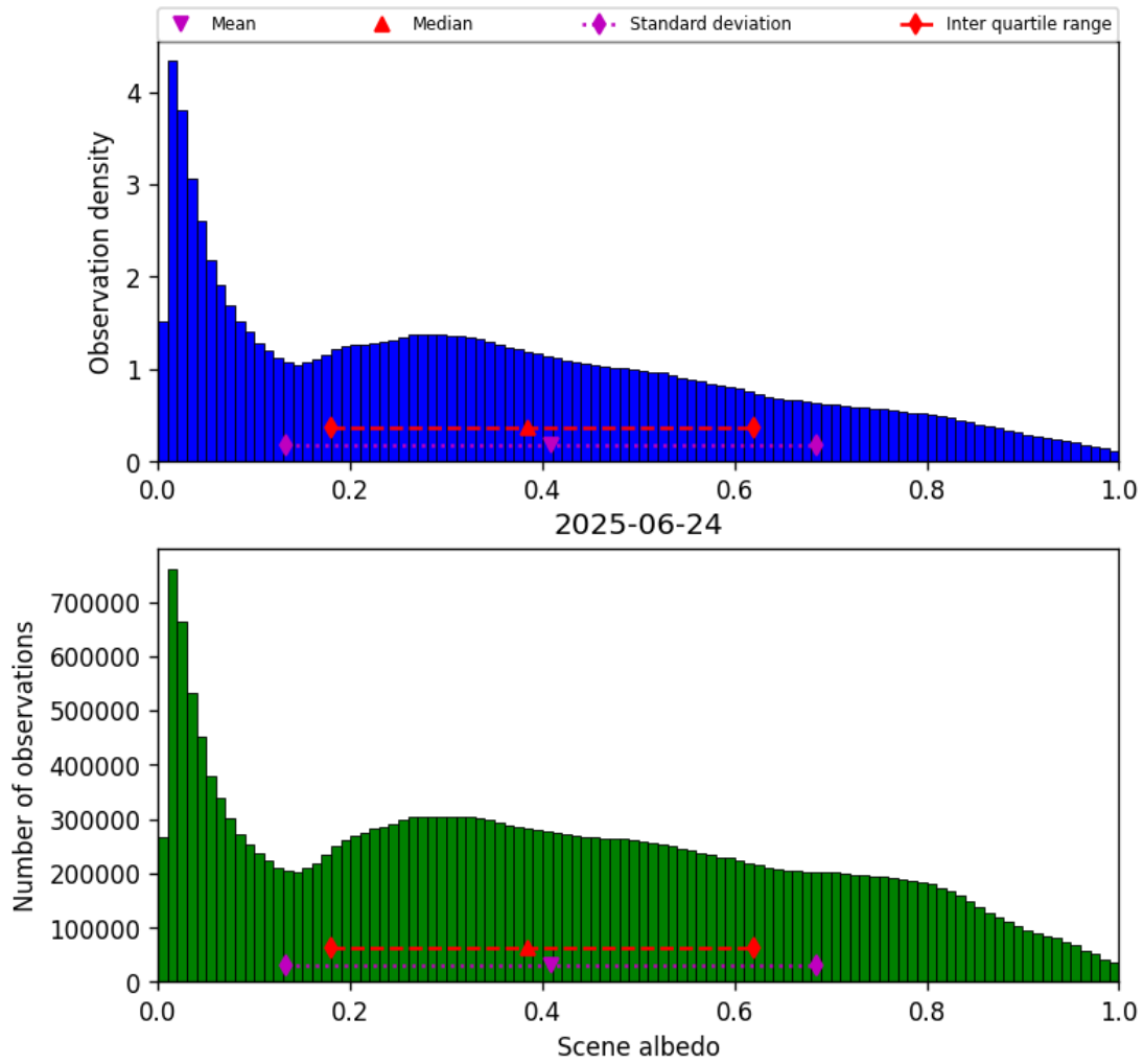
Figure 32: Histogram of “Scene albedo” for 2025-06-24 to 2025-06-25
