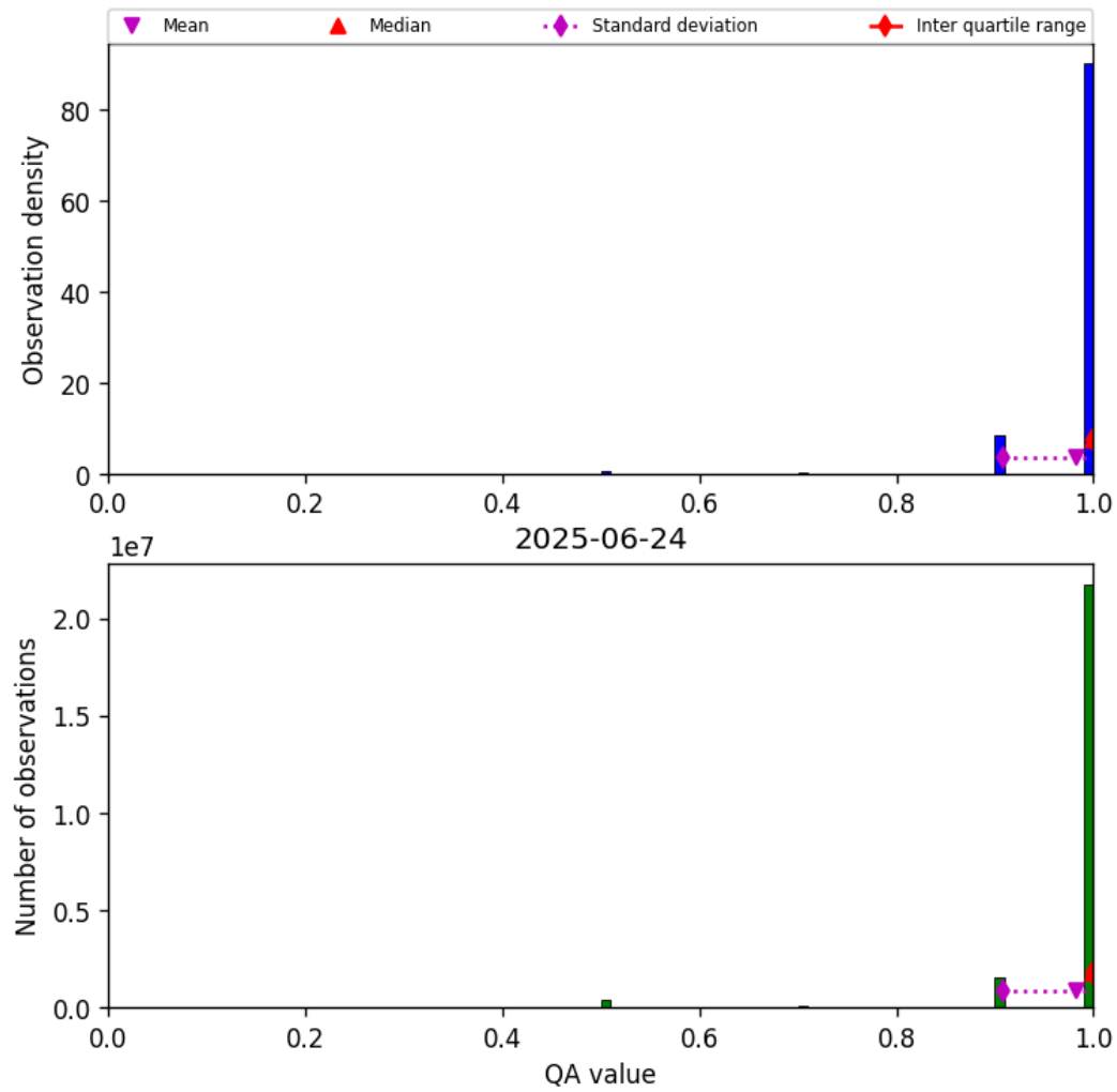
Figure 27: Histogram of “QA value” for 2025-06-24 to 2025-06-25
