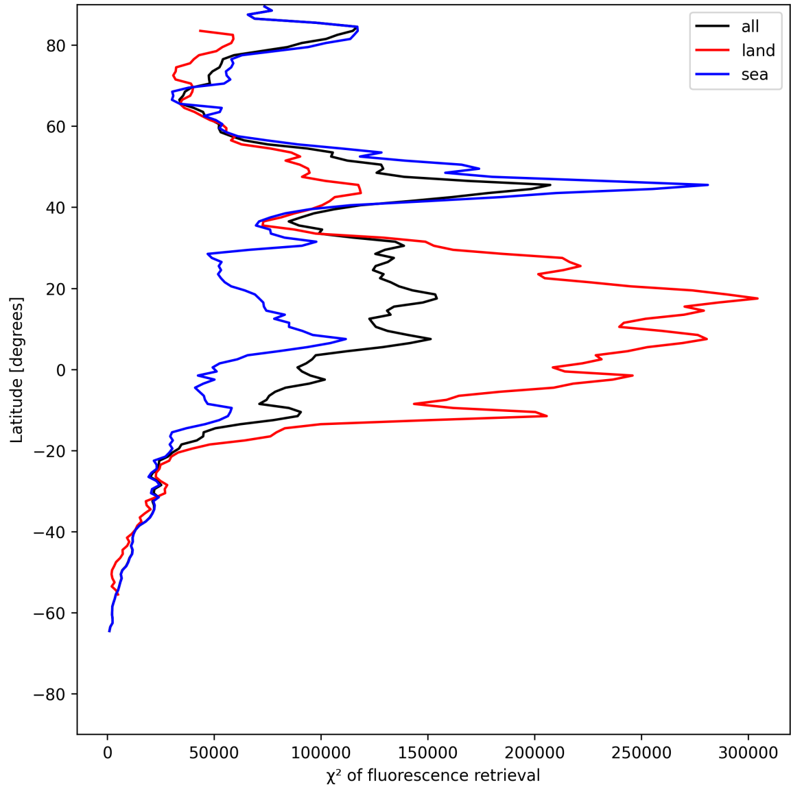
Figure 23: Zonal average of “ \chi^2 of fluorescence retrieval” for 2025-06-24 to 2025-06-25.
