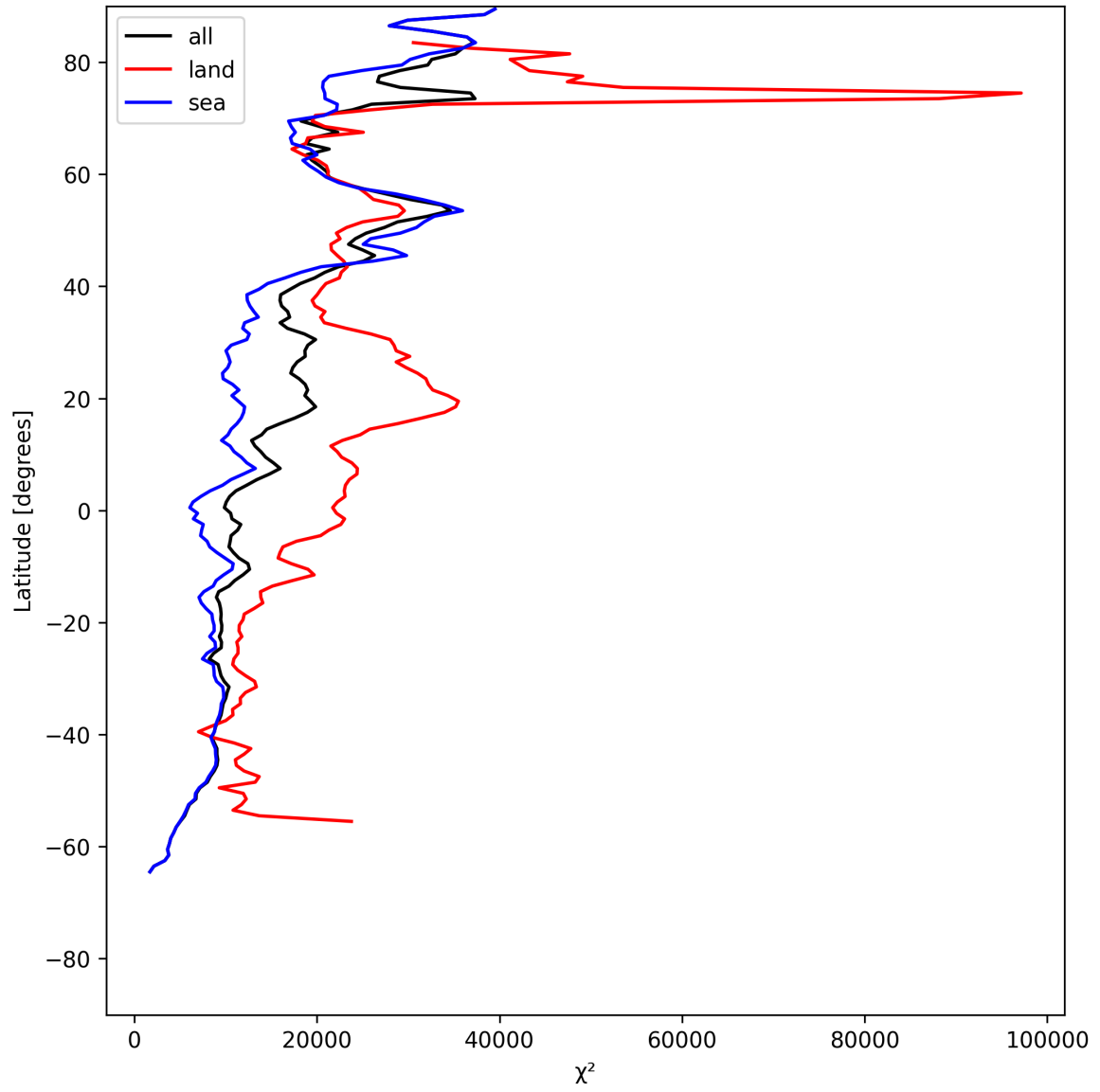
Figure 19: Zonal average of “ \chi^2 ” for 2025-06-24 to 2025-06-25.
