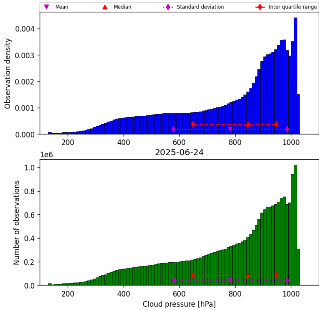
Figure 28: Histogram of “Cloud pressure” for 2025-06-24 to 2025-06-25
