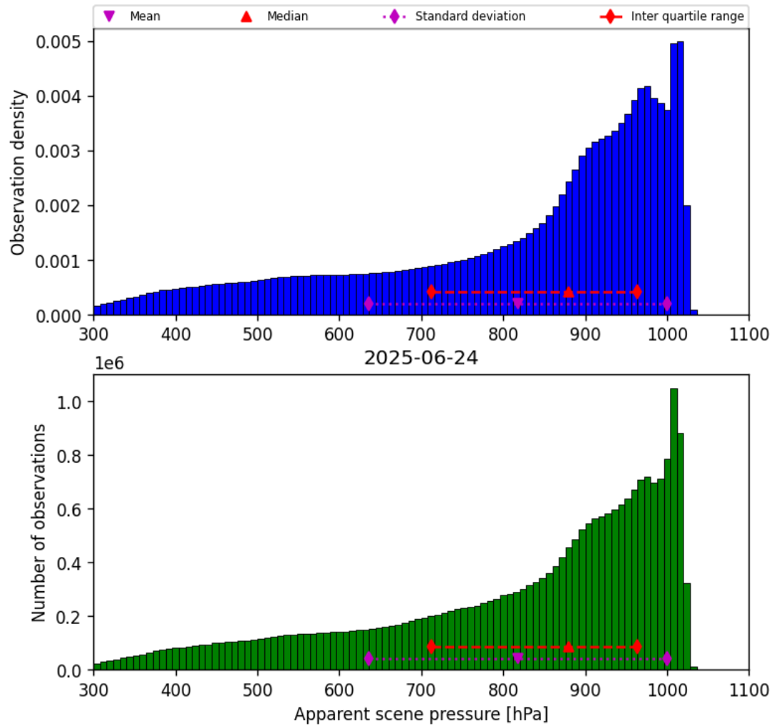
Figure 34: Histogram of “Apparent scene pressure” for 2025-06-24 to 2025-06-25
