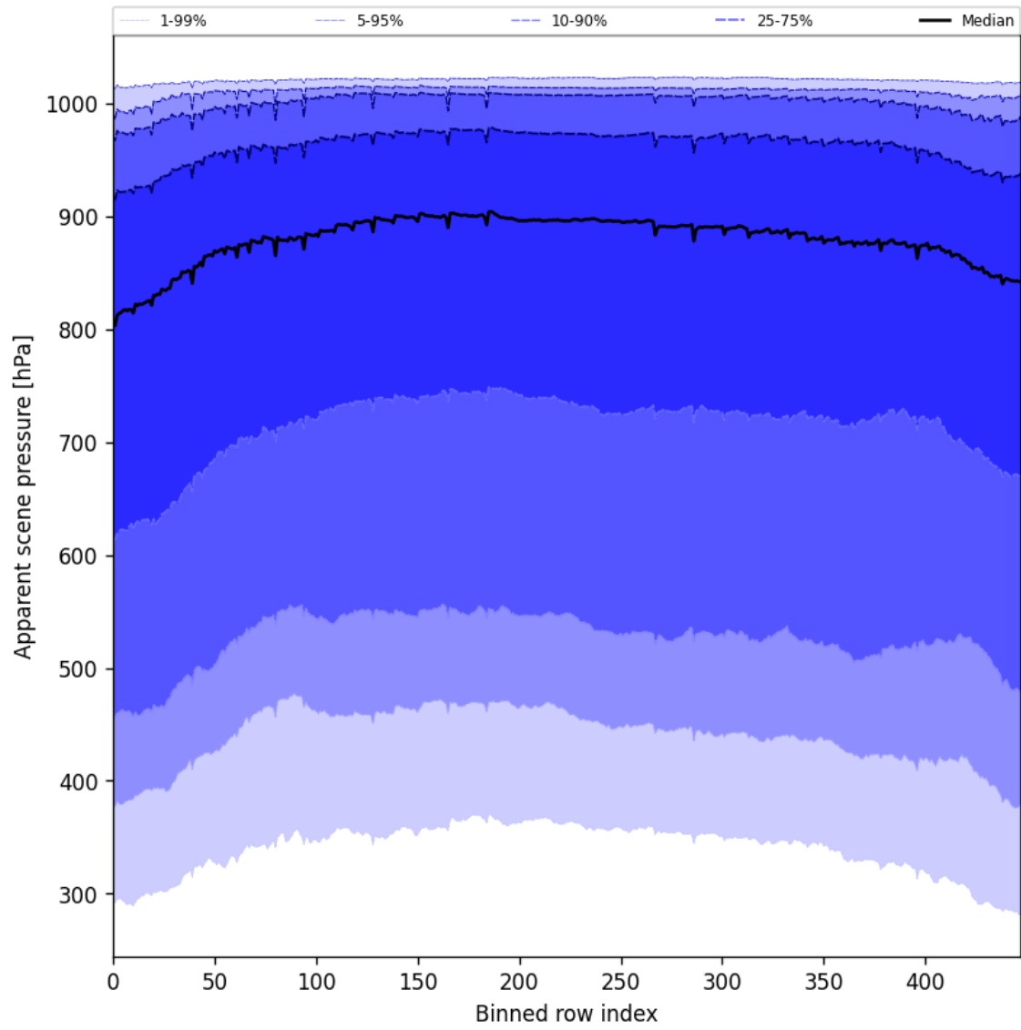
Figure 51: Along track statistics of “Apparent scene pressure” for 2025-06-24 to 2025-06-25
