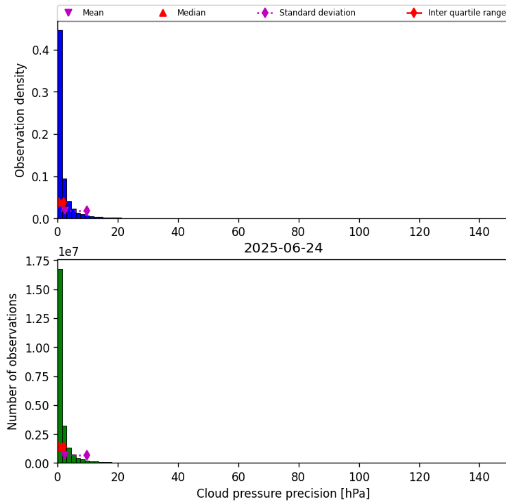
Figure 29: Histogram of “Cloud pressure precision” for 2025-06-24 to 2025-06-25
