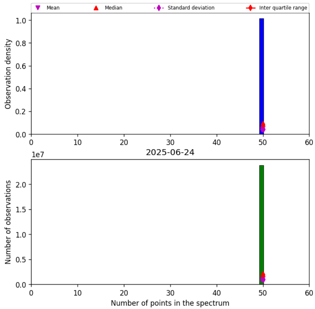
Figure 42: Histogram of “Number of points in the spectrum” for 2025-06-24 to 2025-06-25
