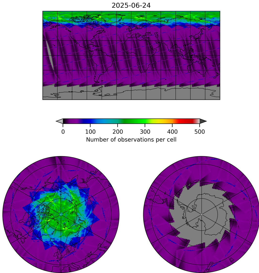
Figure 9: Map of the number of observations for 2025-06-24 to 2025-06-25
