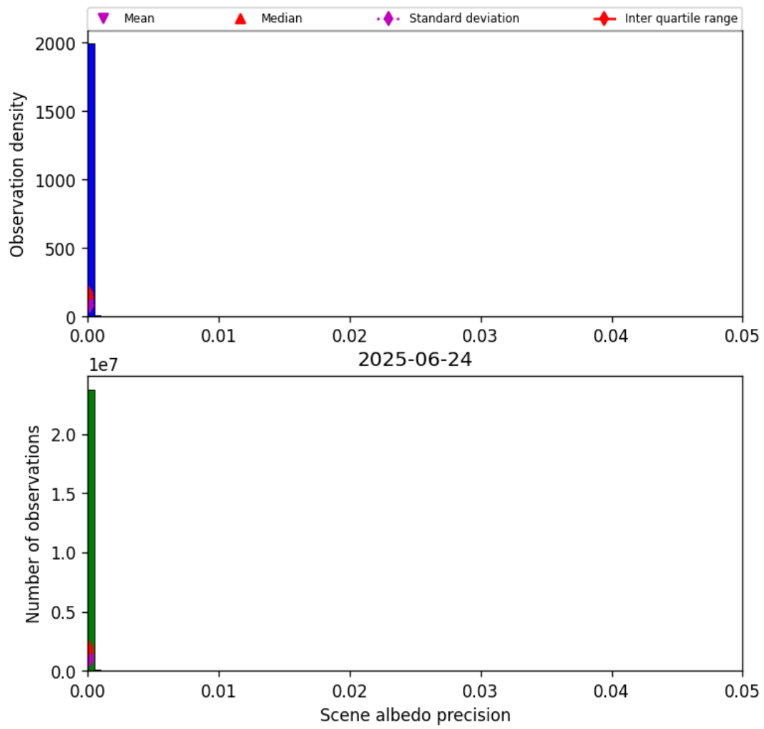
Figure 33: Histogram of “Scene albedo precision” for 2025-06-24 to 2025-06-25
