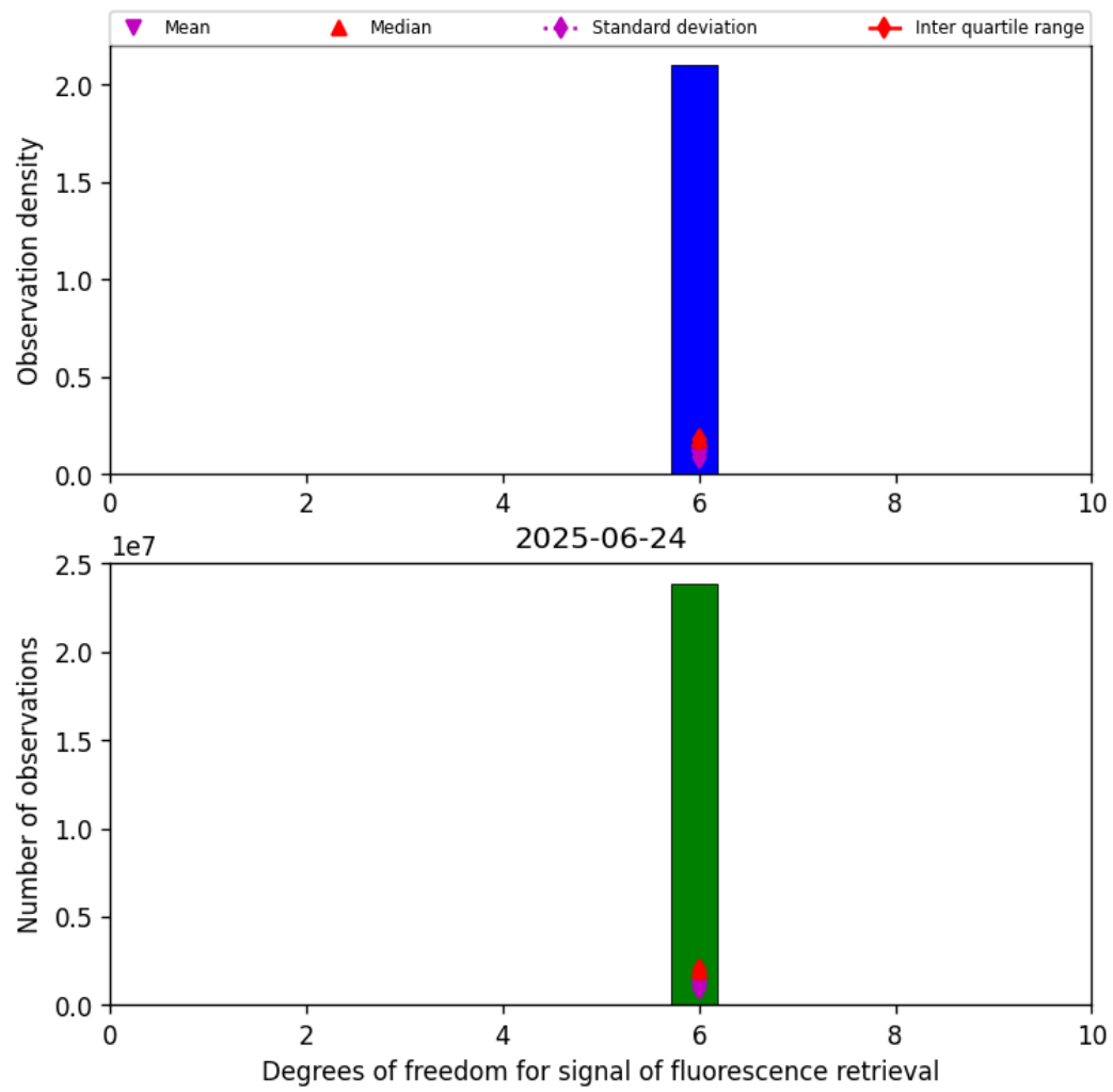
Figure 41: Histogram of “Degrees of freedom for signal of fluorescence retrieval” for 2025-06-24 to 2025-06-25
