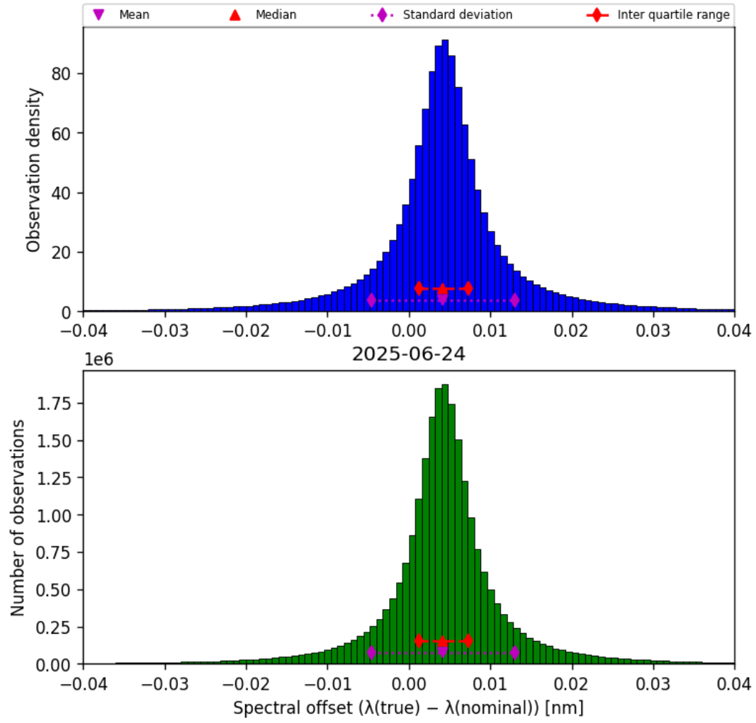
Figure 43: Histogram of “Spectral offset ( \lambda_{\text{true}} - \lambda_{\text{nominal}} )” for 2025-06-24 to 2025-06-25
