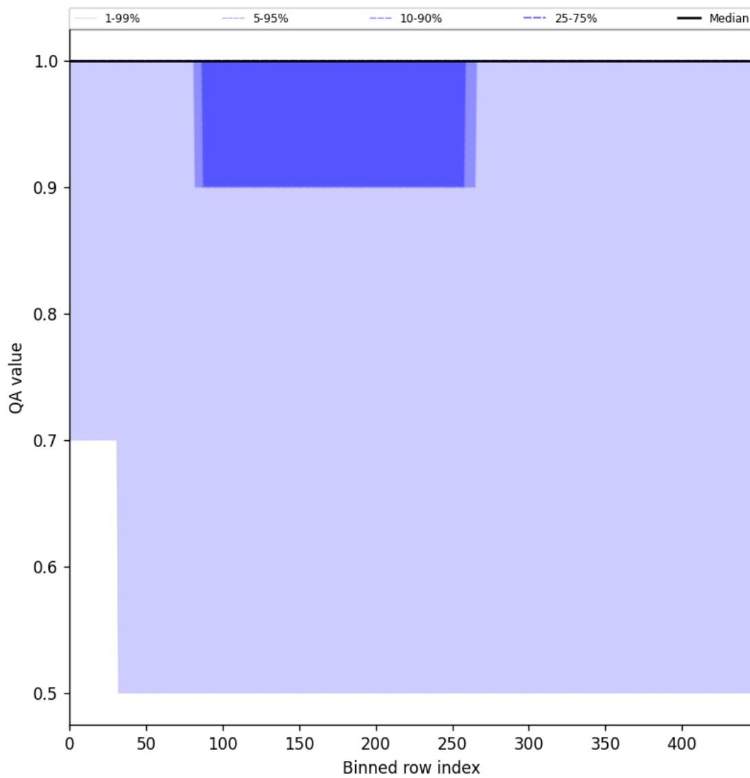
Figure 44: Along track statistics of “QA value” for 2025-06-24 to 2025-06-25
