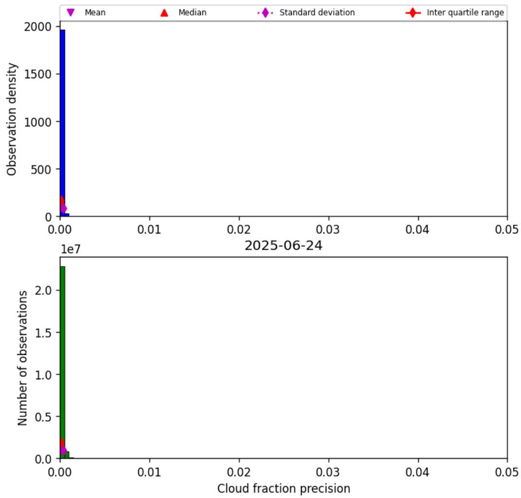
Figure 31: Histogram of “Cloud fraction precision” for 2025-06-24 to 2025-06-25
