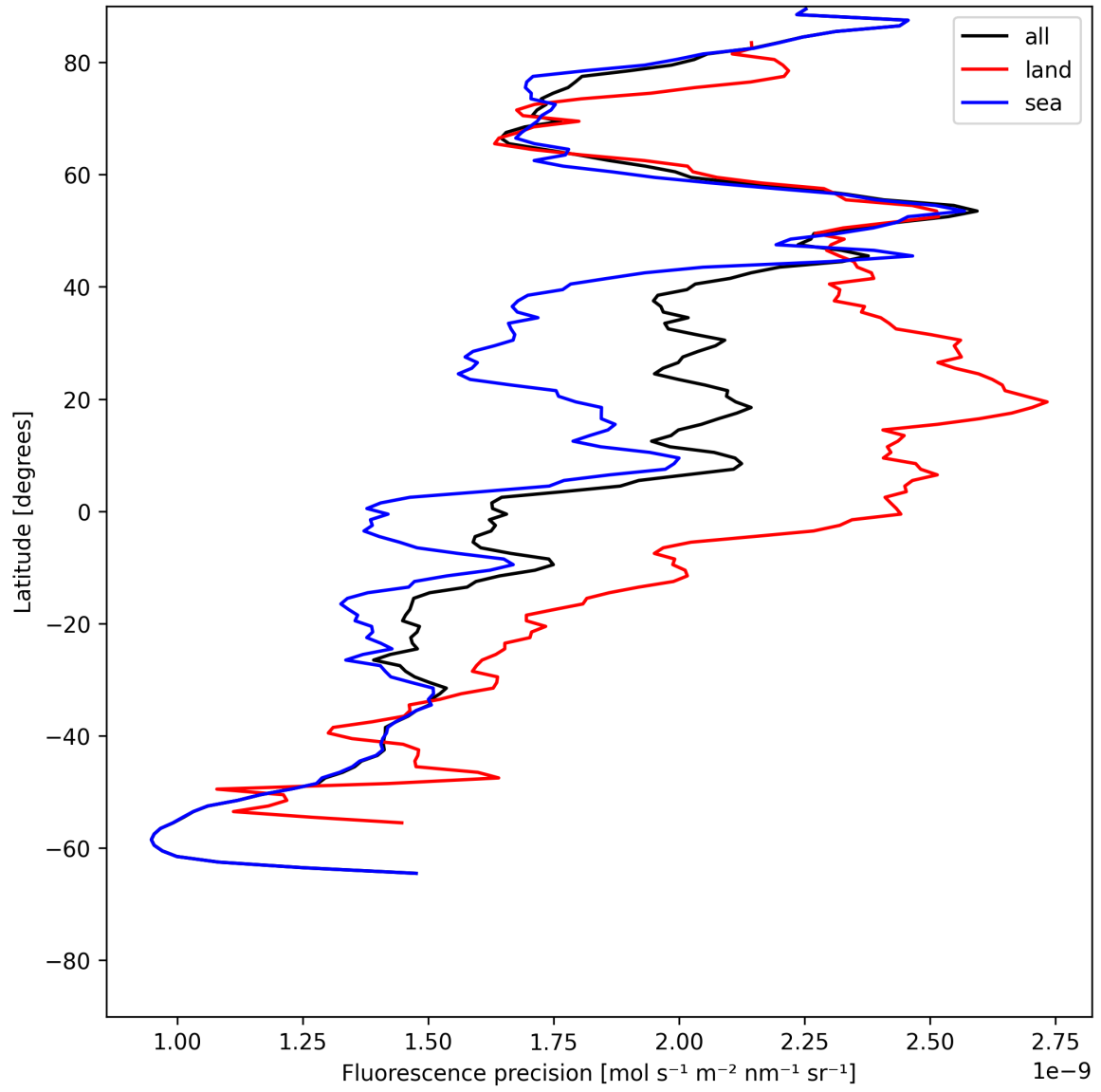
Figure 22: Zonal average of “Fluorescence precision” for 2025-06-24 to 2025-06-25.
