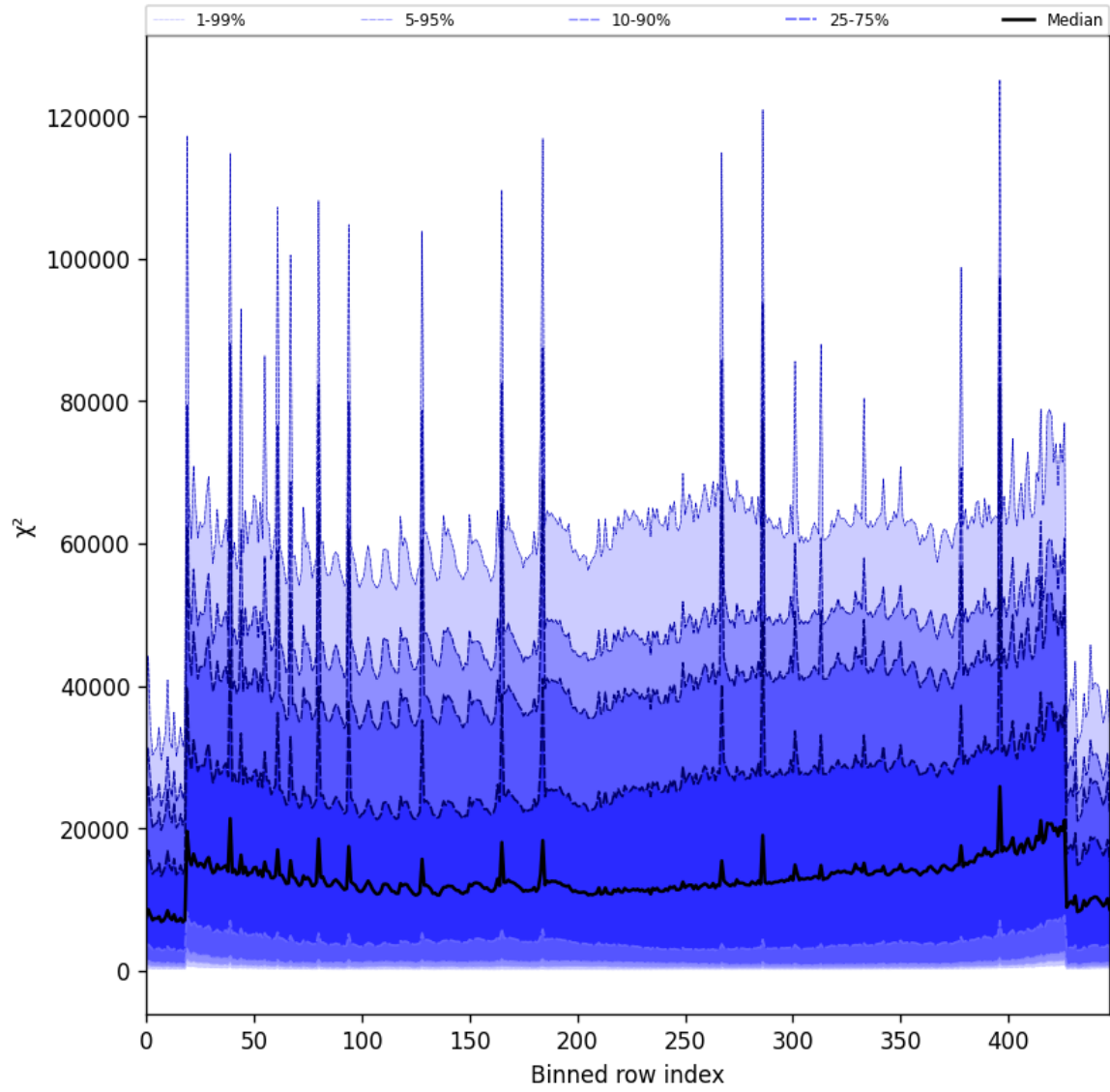
Figure 53: Along track statistics of “ \chi^2 ” for 2025-06-24 to 2025-06-25
