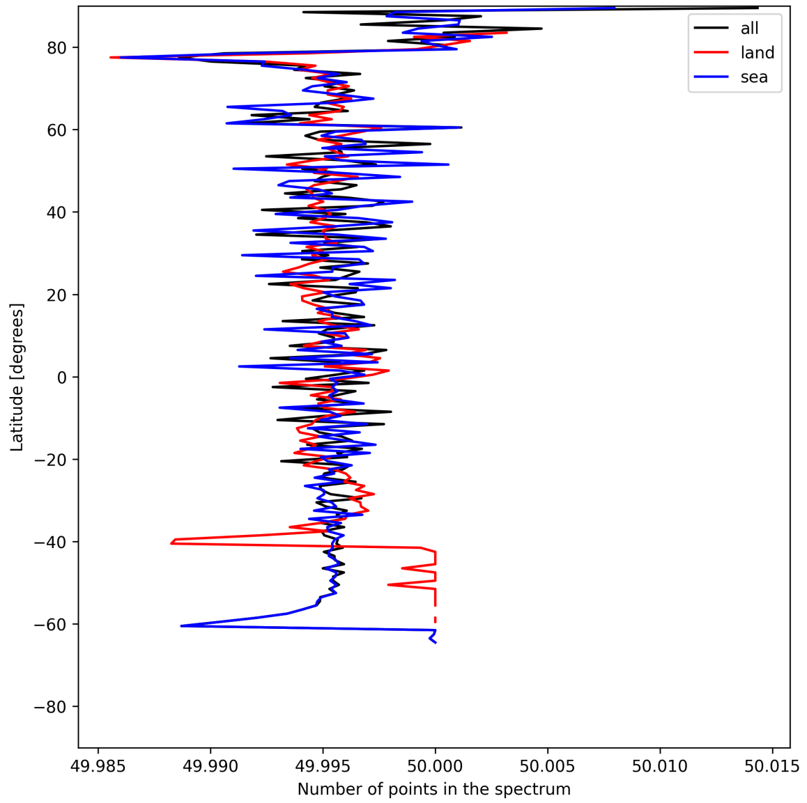
Figure 25: Zonal average of “Number of points in the spectrum” for 2025-06-25 to 2025-06-25.
