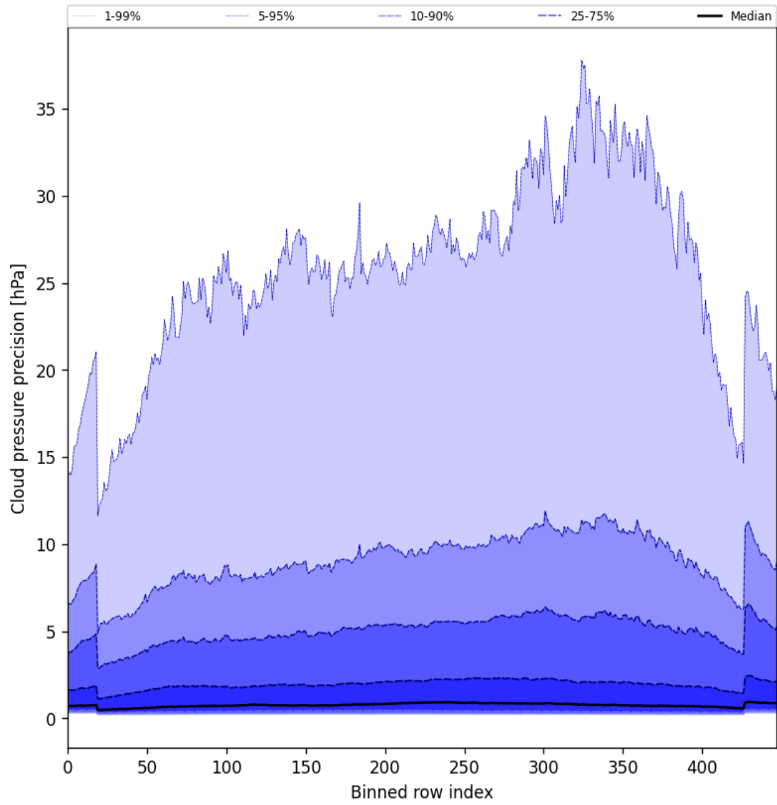
Figure 46: Along track statistics of “Cloud pressure precision” for 2025-06-25 to 2025-06-25
