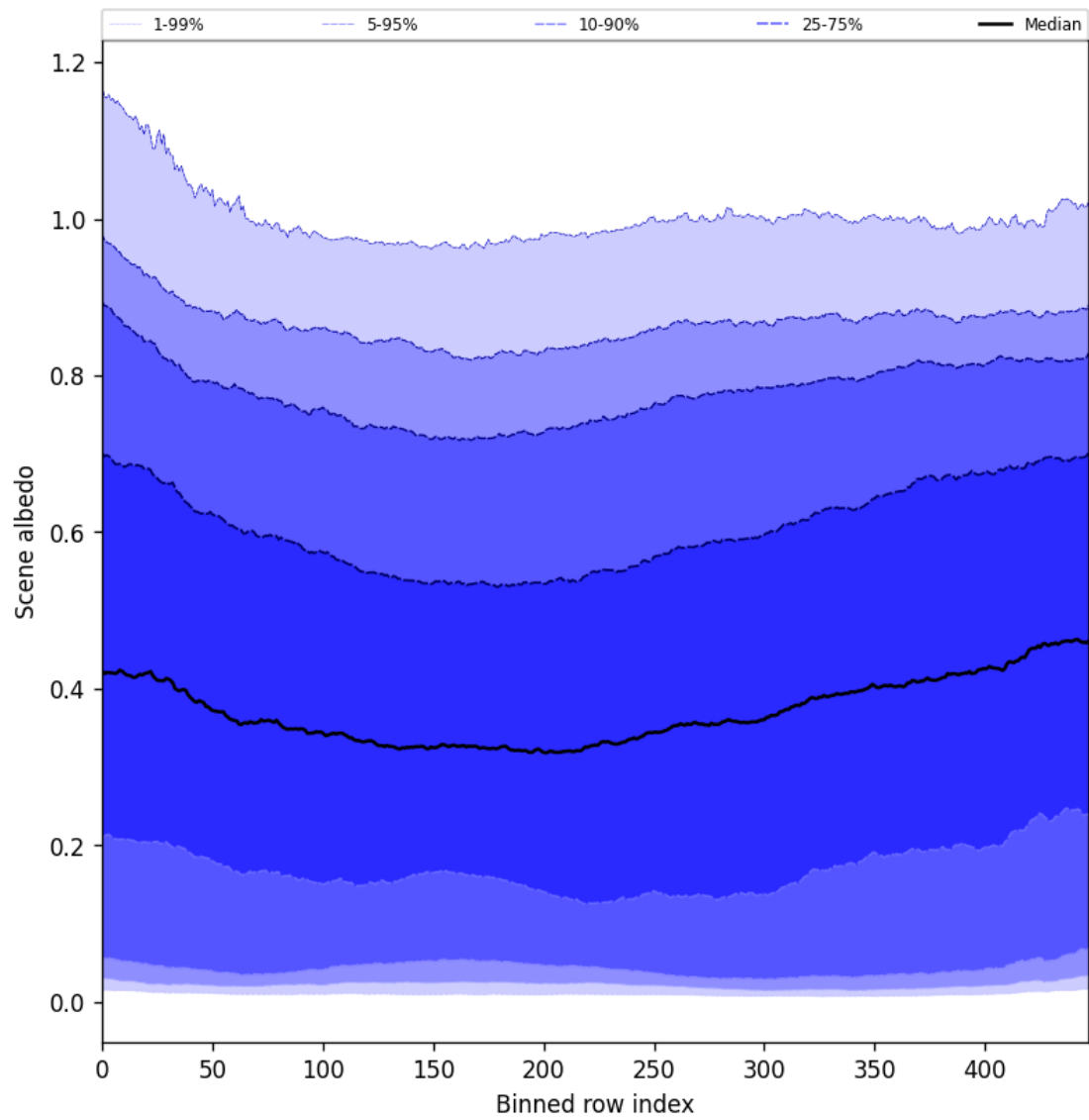
Figure 49: Along track statistics of “Scene albedo” for 2025-06-25 to 2025-06-25
