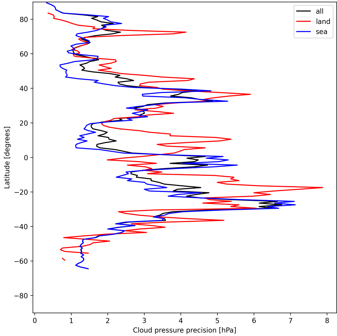
Figure 12: Zonal average of “Cloud pressure precision” for 2025-06-25 to 2025-06-25.
