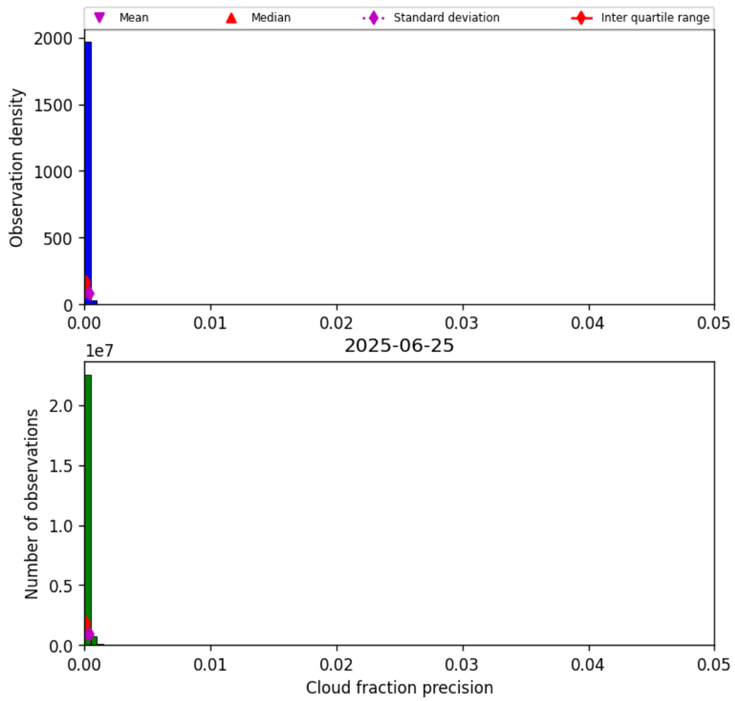
Figure 31: Histogram of “Cloud fraction precision” for 2025-06-25 to 2025-06-25
