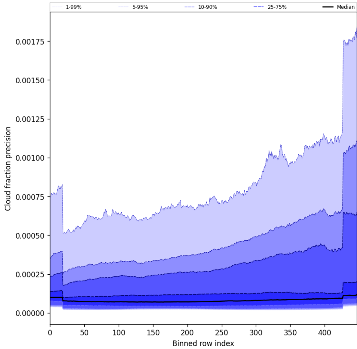
Figure 48: Along track statistics of “Cloud fraction precision” for 2025-06-25 to 2025-06-25
