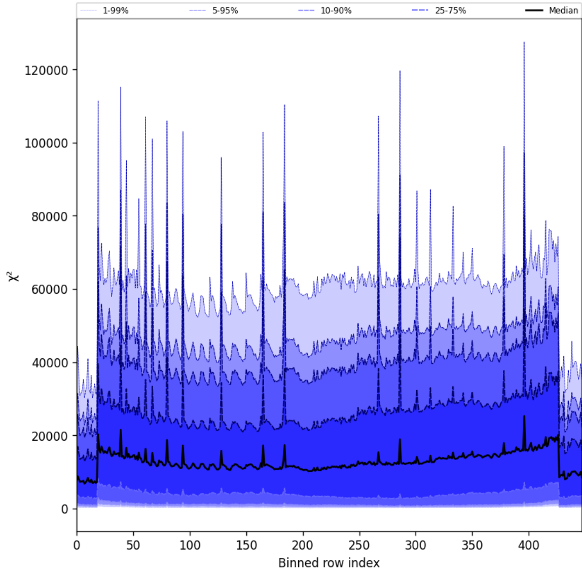
Figure 53: Along track statistics of “ \chi^2 ” for 2025-06-25 to 2025-06-25
