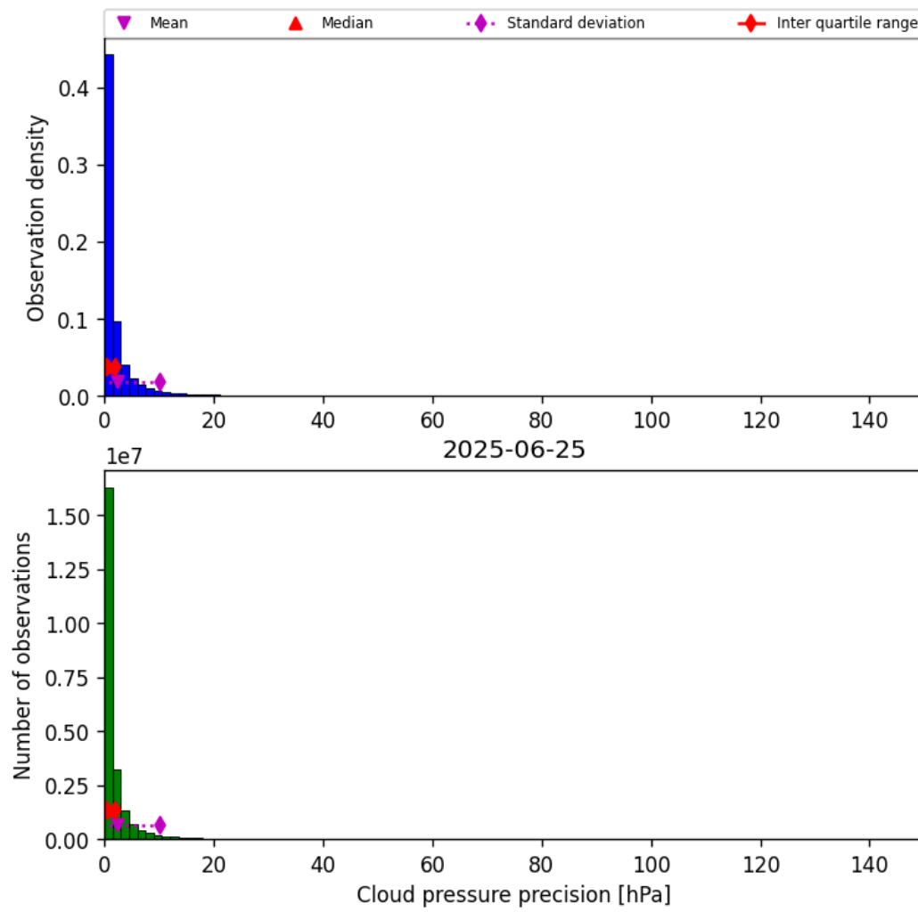
Figure 29: Histogram of “Cloud pressure precision” for 2025-06-25 to 2025-06-25
