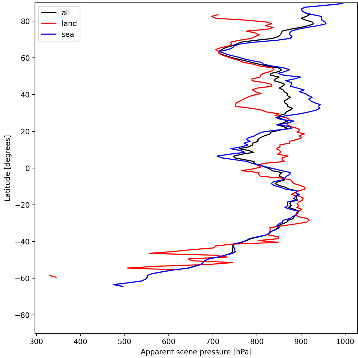
Figure 17: Zonal average of “Apparent scene pressure” for 2025-06-25 to 2025-06-25.
