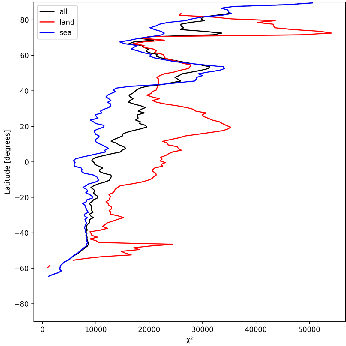
Figure 19: Zonal average of “ \chi^2 ” for 2025-06-25 to 2025-06-25.
