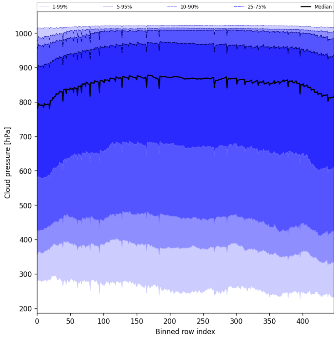
Figure 45: Along track statistics of “Cloud pressure” for 2025-06-25 to 2025-06-25
