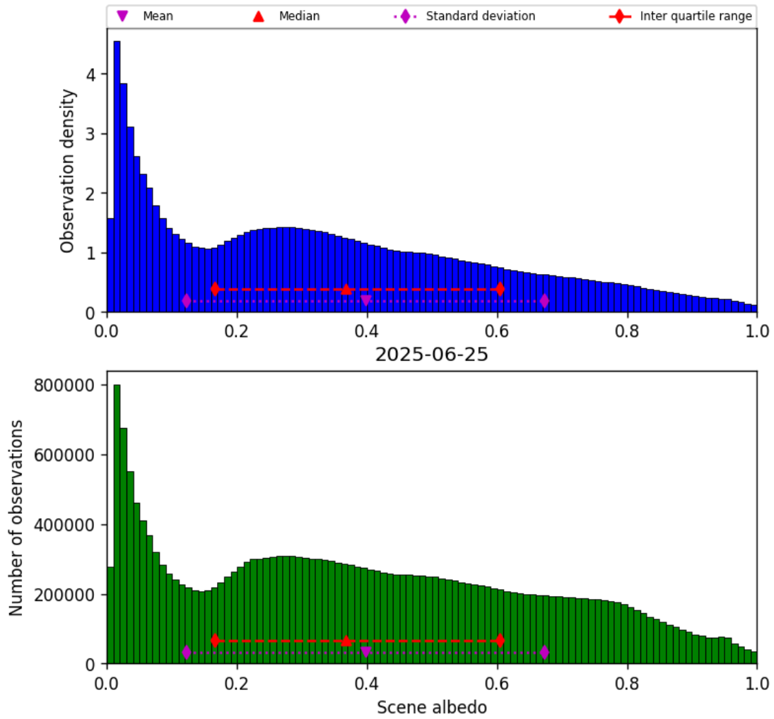
Figure 32: Histogram of “Scene albedo” for 2025-06-25 to 2025-06-25
