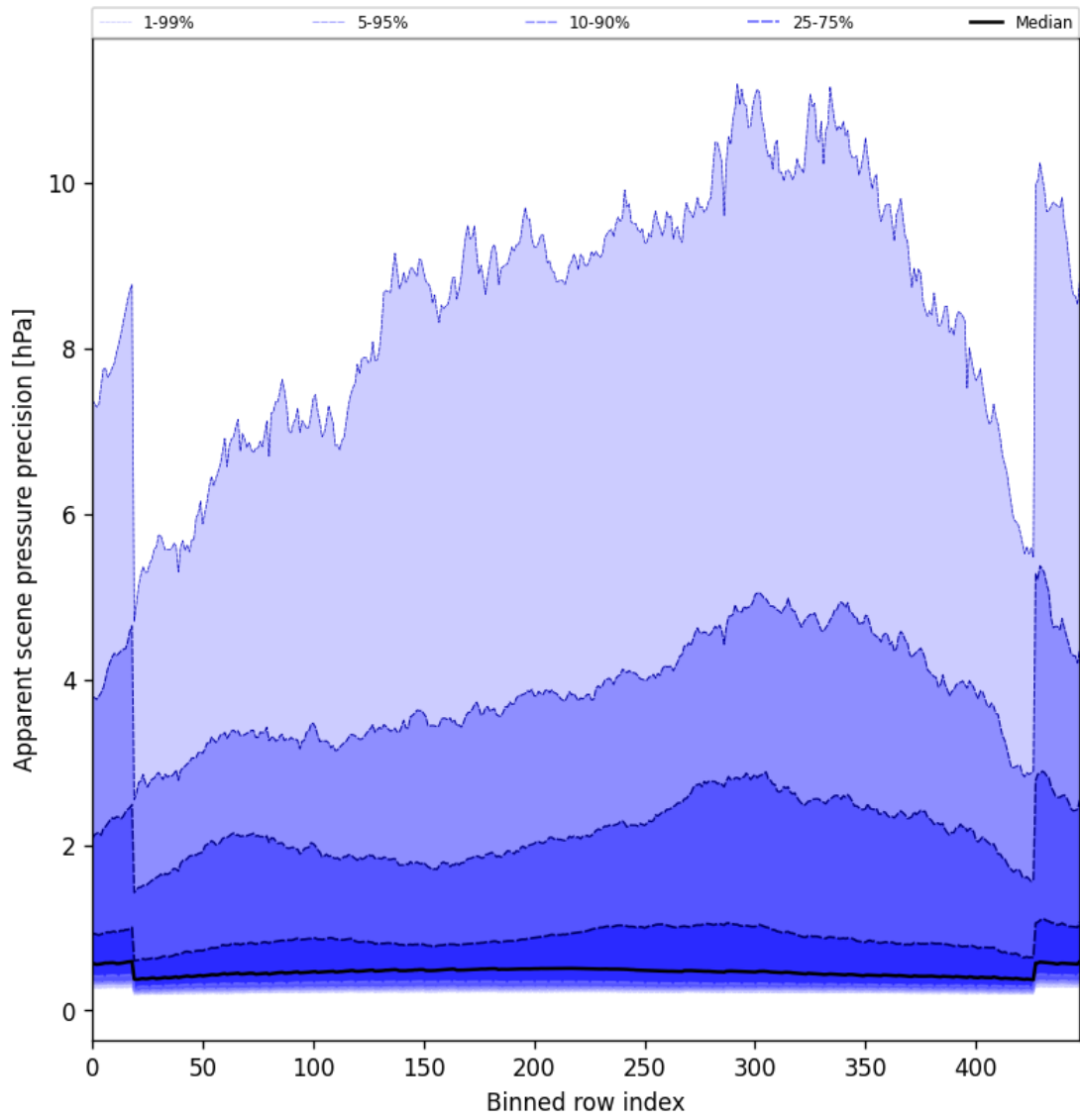
Figure 52: Along track statistics of “Apparent scene pressure precision” for 2025-06-25 to 2025-06-25
