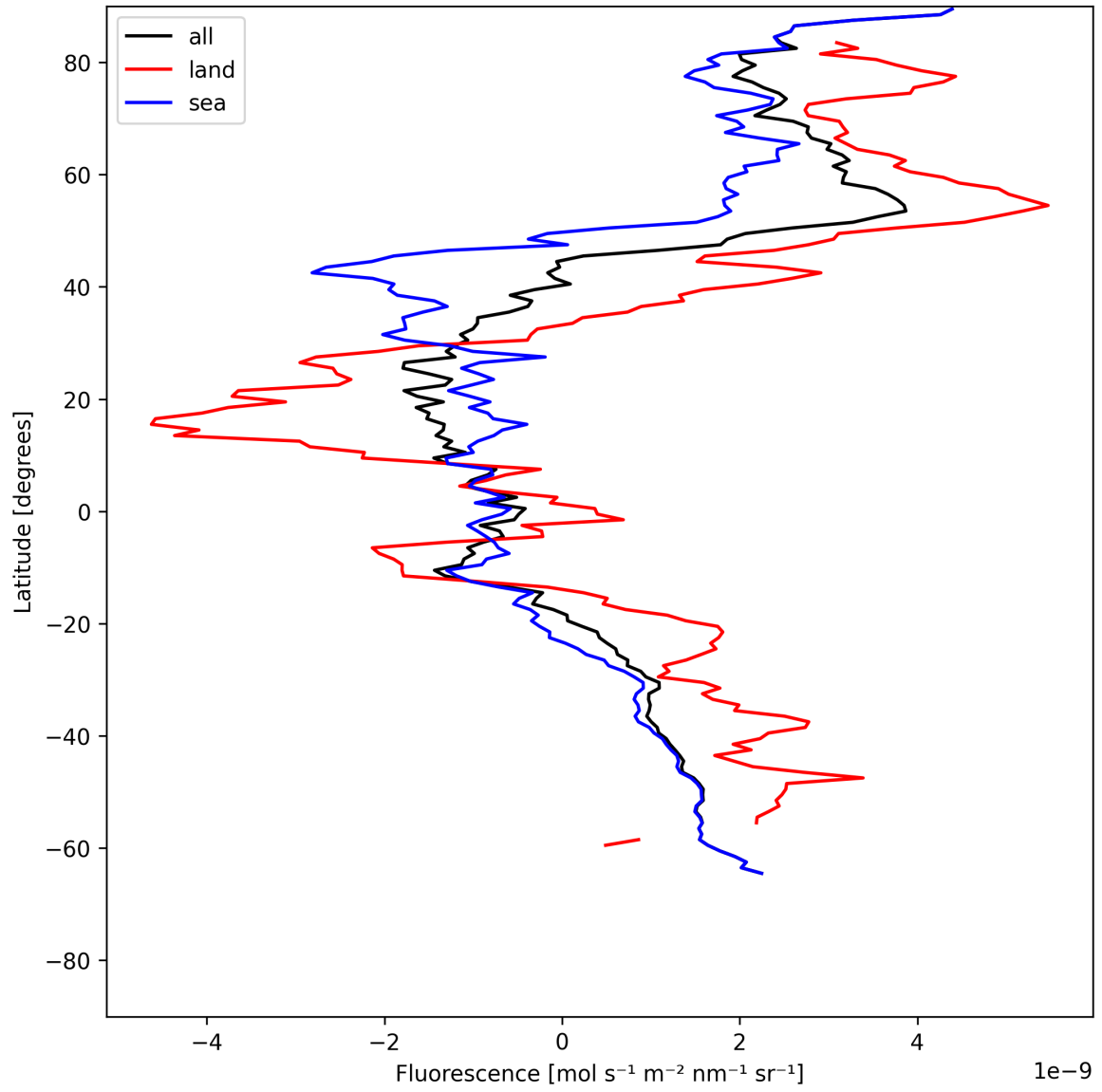
Figure 21: Zonal average of “Fluorescence” for 2025-06-25 to 2025-06-25.
