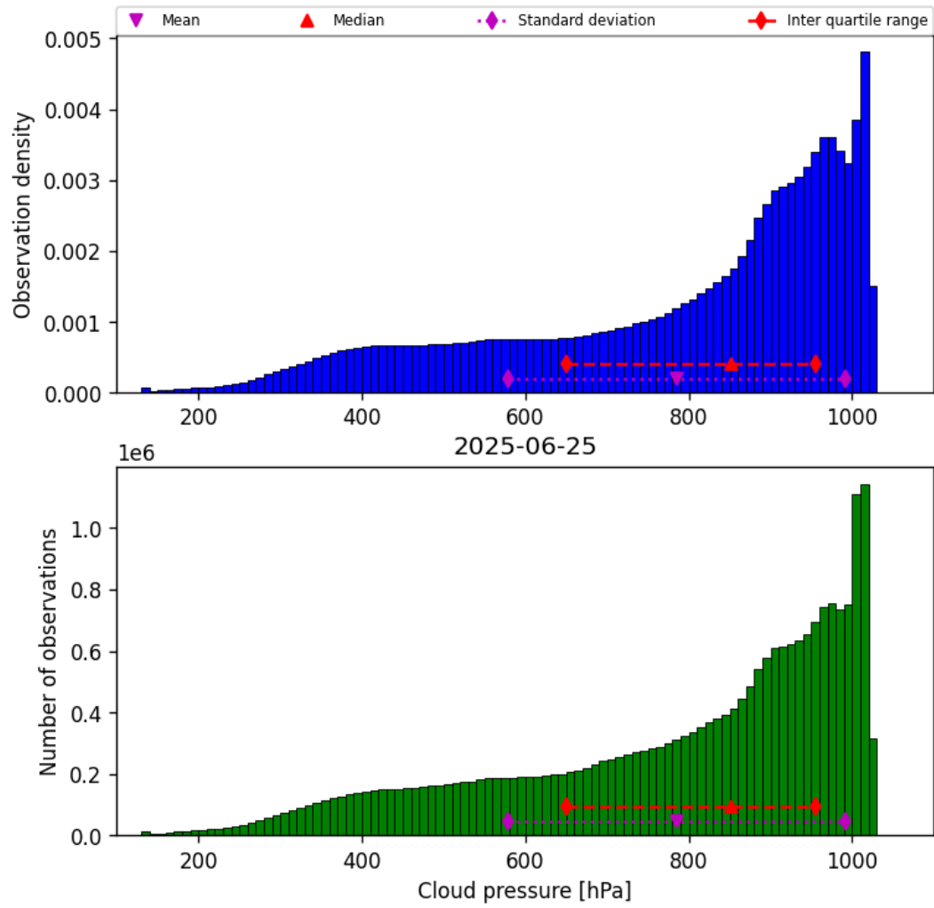
Figure 28: Histogram of “Cloud pressure” for 2025-06-25 to 2025-06-25
