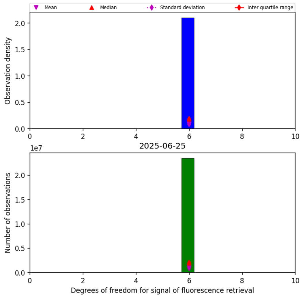
Figure 41: Histogram of “Degrees of freedom for signal of fluorescence retrieval” for 2025-06-25 to 2025-06-25
