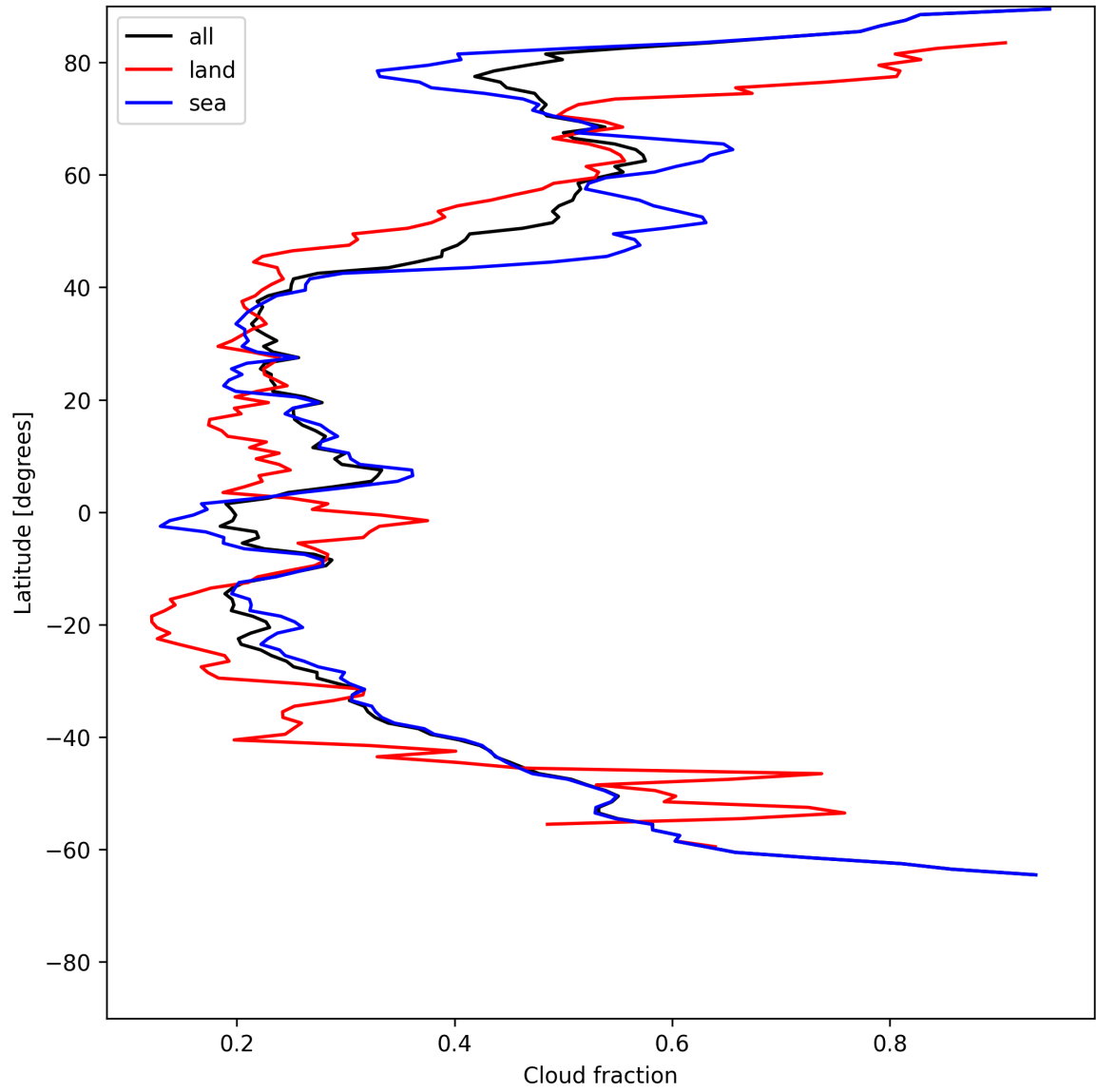
Figure 13: Zonal average of “Cloud fraction” for 2025-06-25 to 2025-06-25.
