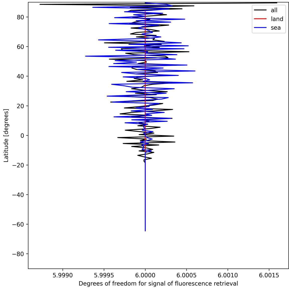
Figure 24: Zonal average of “Degrees of freedom for signal of fluorescence retrieval” for 2025-06-25 to 2025-06-25.
