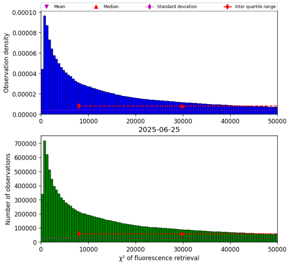
Figure 40: Histogram of “ \chi^2 of fluorescence retrieval” for 2025-06-25 to 2025-06-25
