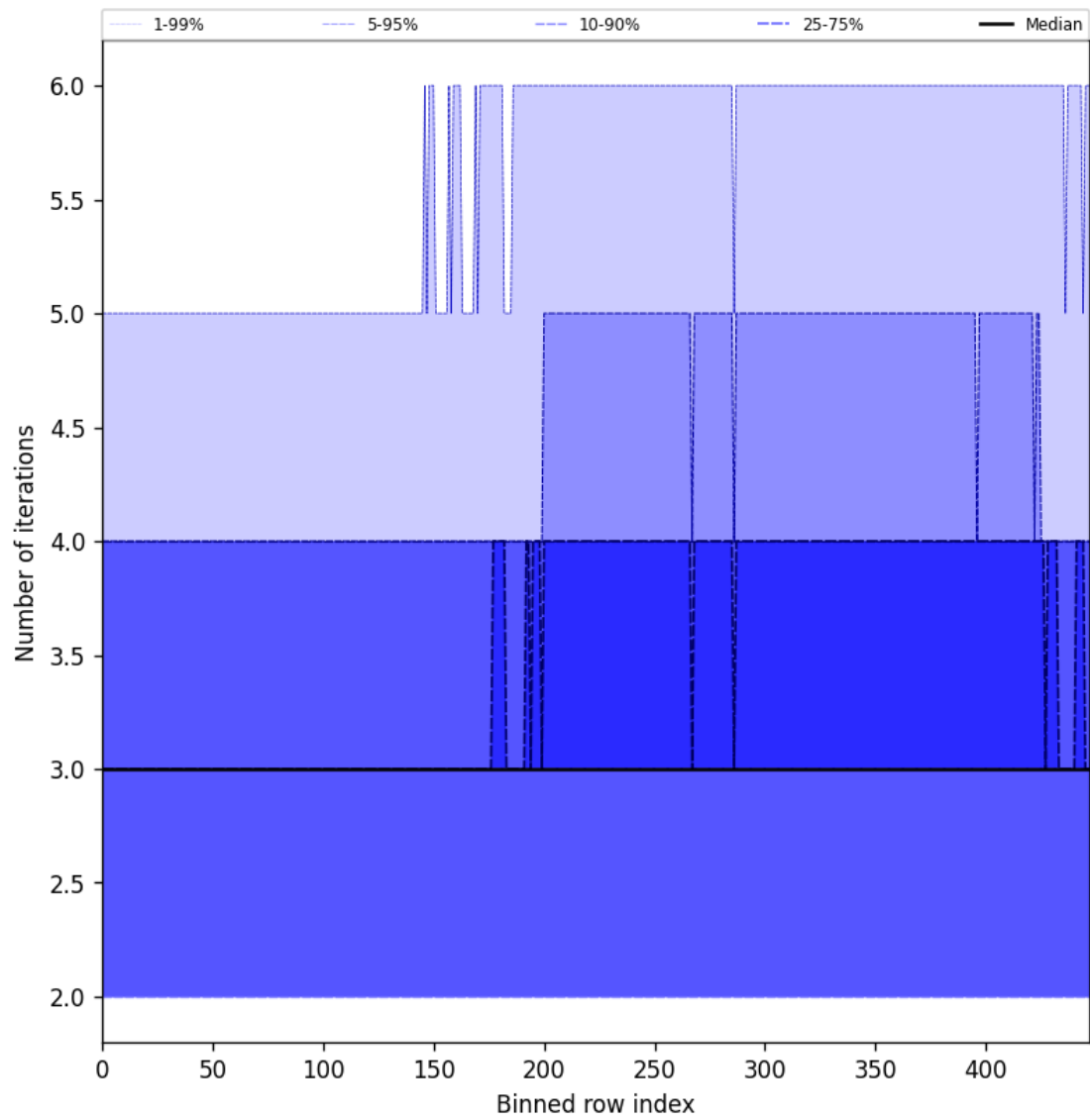
Figure 54: Along track statistics of “Number of iterations” for 2025-06-25 to 2025-06-25
