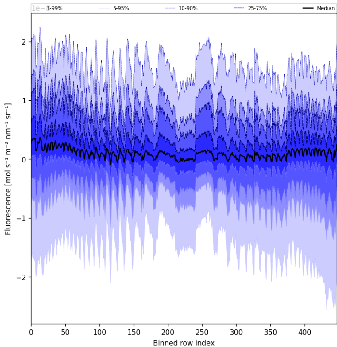
Figure 55: Along track statistics of “Fluorescence” for 2025-06-25 to 2025-06-25
