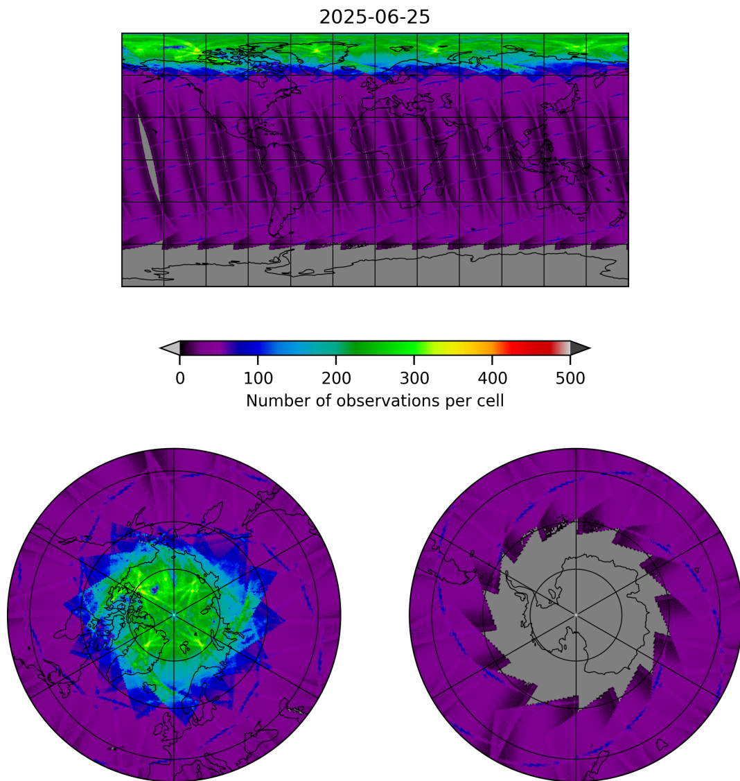
Figure 9: Map of the number of observations for 2025-06-25 to 2025-06-25
