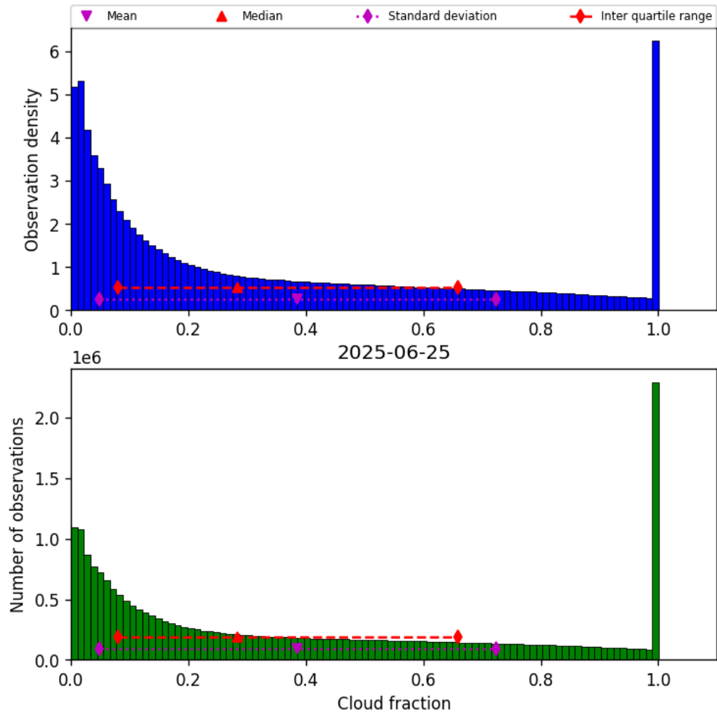
Figure 30: Histogram of “Cloud fraction” for 2025-06-25 to 2025-06-25
