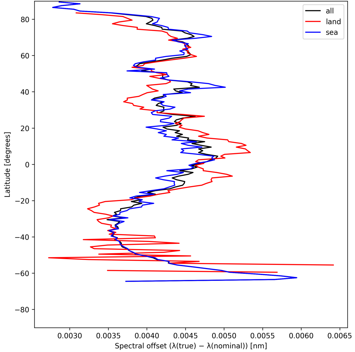
Figure 26: Zonal average of “Spectral offset ( \lambda_{\text{true}} - \lambda_{\text{nominal}} )” for 2025-06-25 to 2025-06-25.
