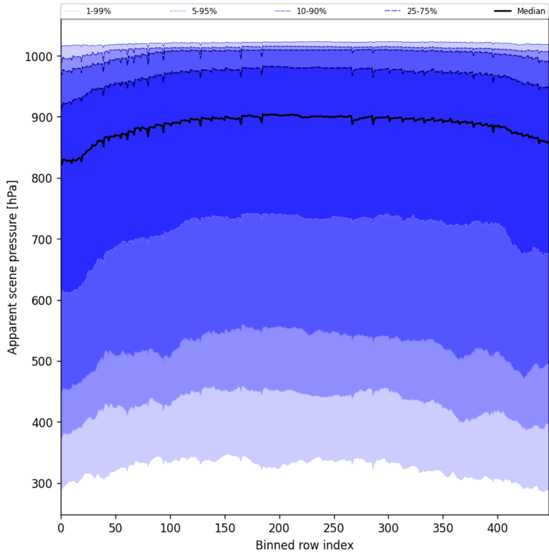
Figure 51: Along track statistics of “Apparent scene pressure” for 2025-06-25 to 2025-06-25
