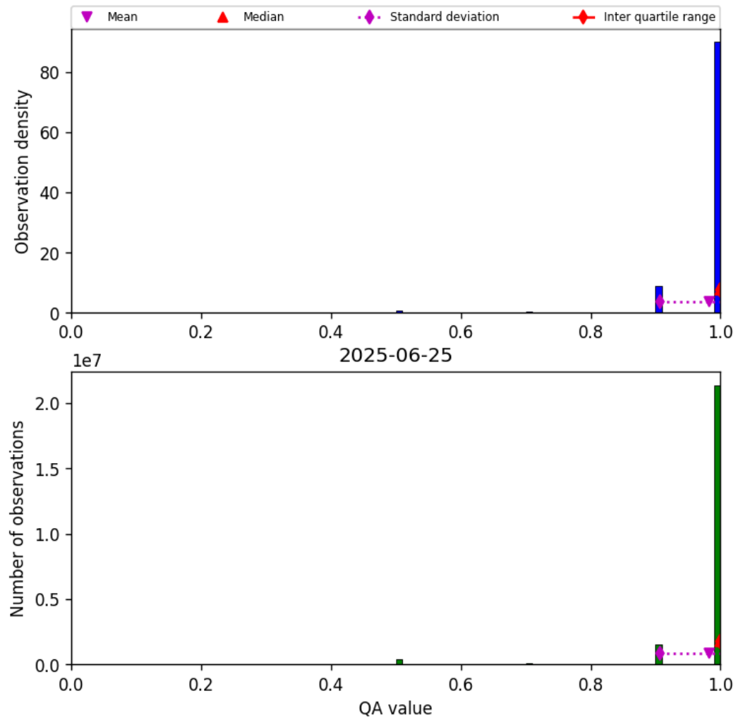
Figure 27: Histogram of “QA value” for 2025-06-25 to 2025-06-25
