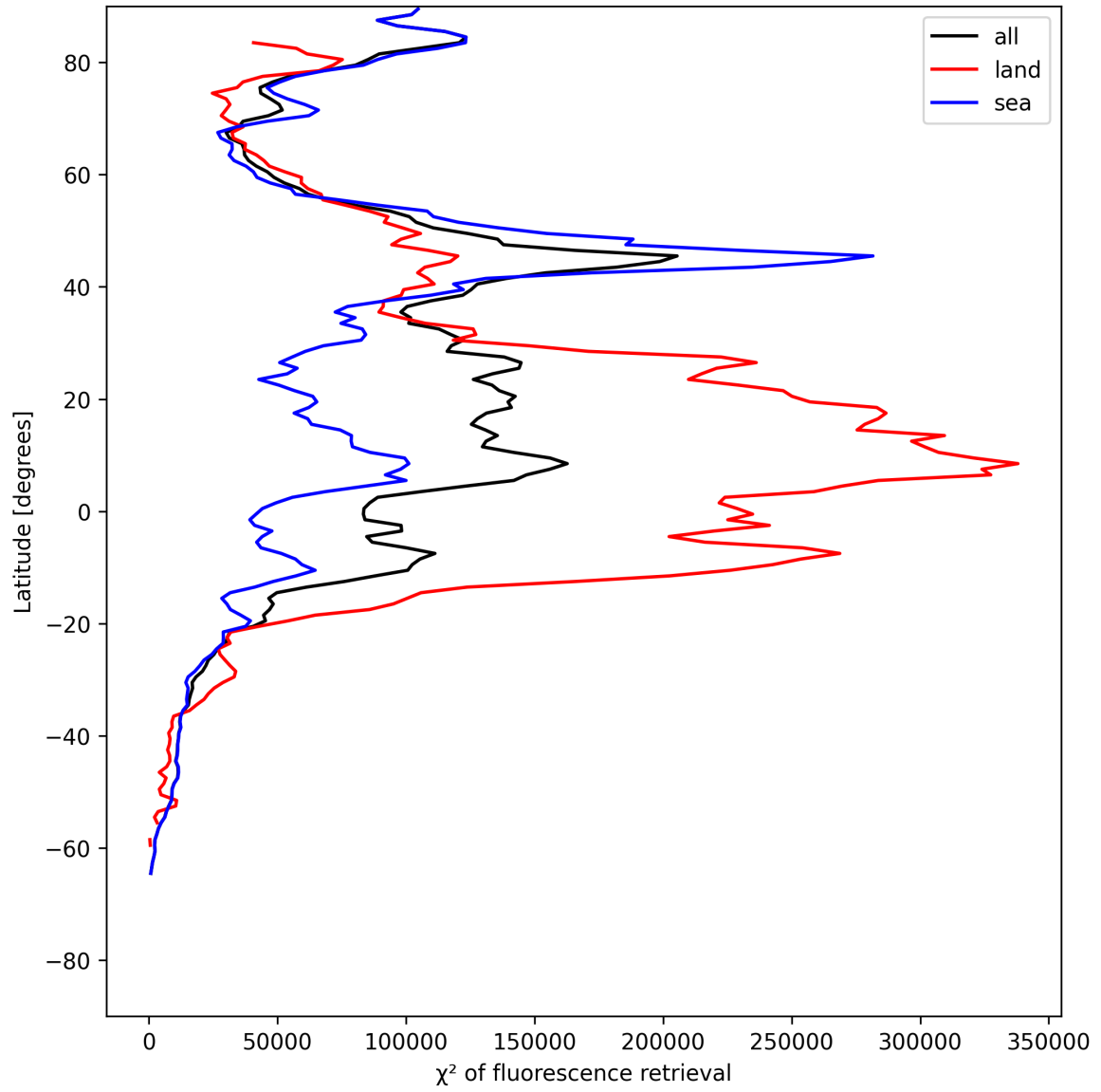
Figure 23: Zonal average of “ \chi^2 of fluorescence retrieval” for 2025-06-25 to 2025-06-25.
