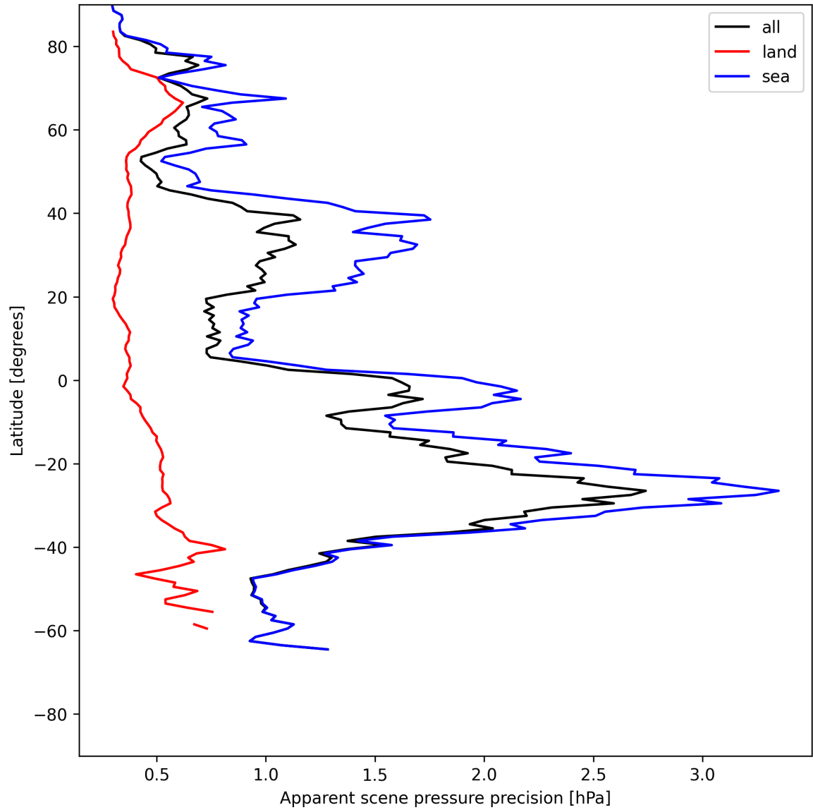
Figure 18: Zonal average of “Apparent scene pressure precision” for 2025-06-25 to 2025-06-25.
