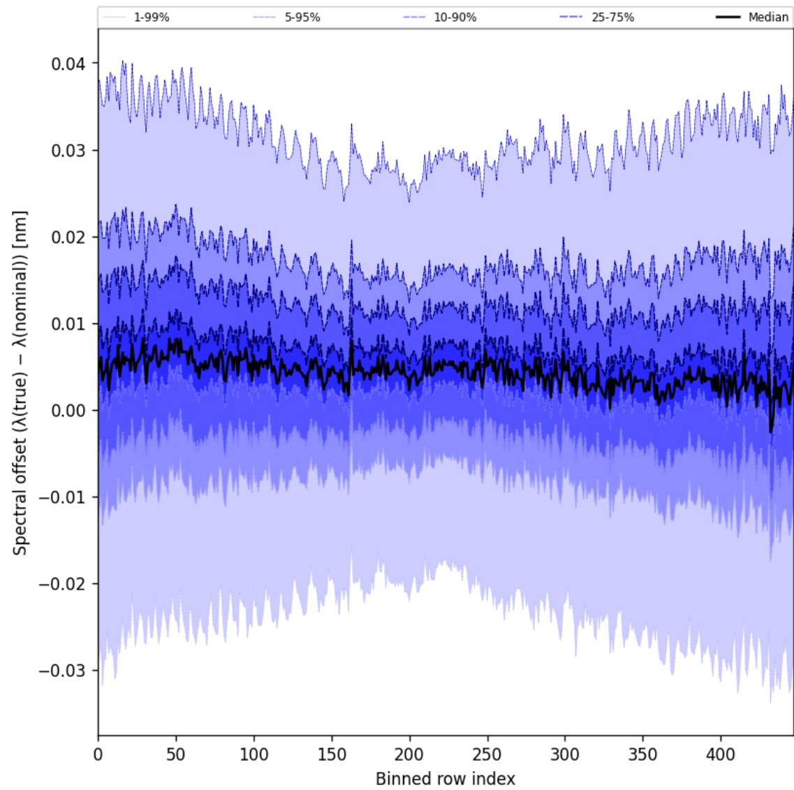
Figure 60: Along track statistics of “Spectral offset ( \lambda_{\text{true}} - \lambda_{\text{nominal}} )” for 2025-06-25 to 2025-06-25
