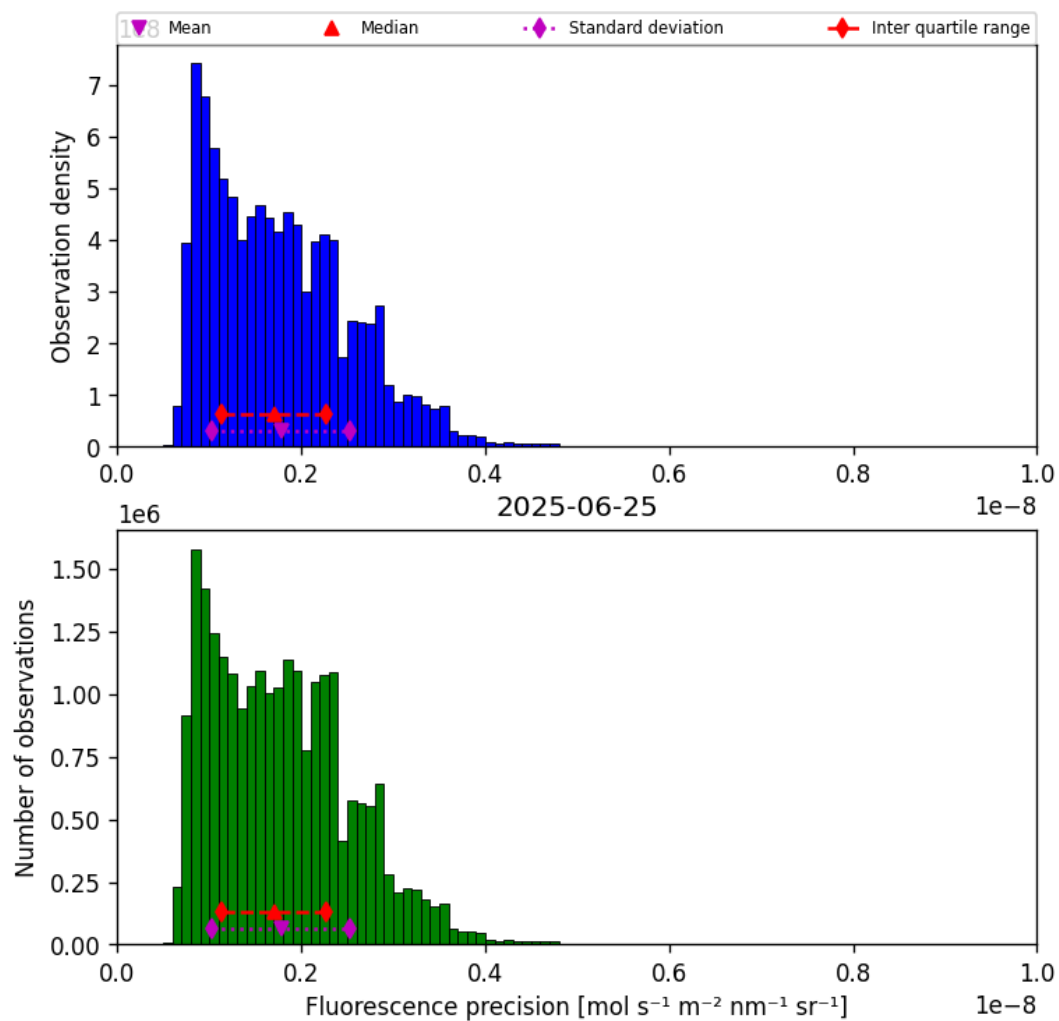
Figure 39: Histogram of “Fluorescence precision” for 2025-06-25 to 2025-06-25
