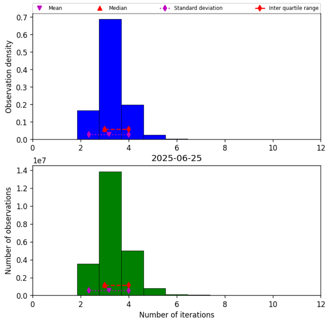
Figure 37: Histogram of “Number of iterations” for 2025-06-25 to 2025-06-25
