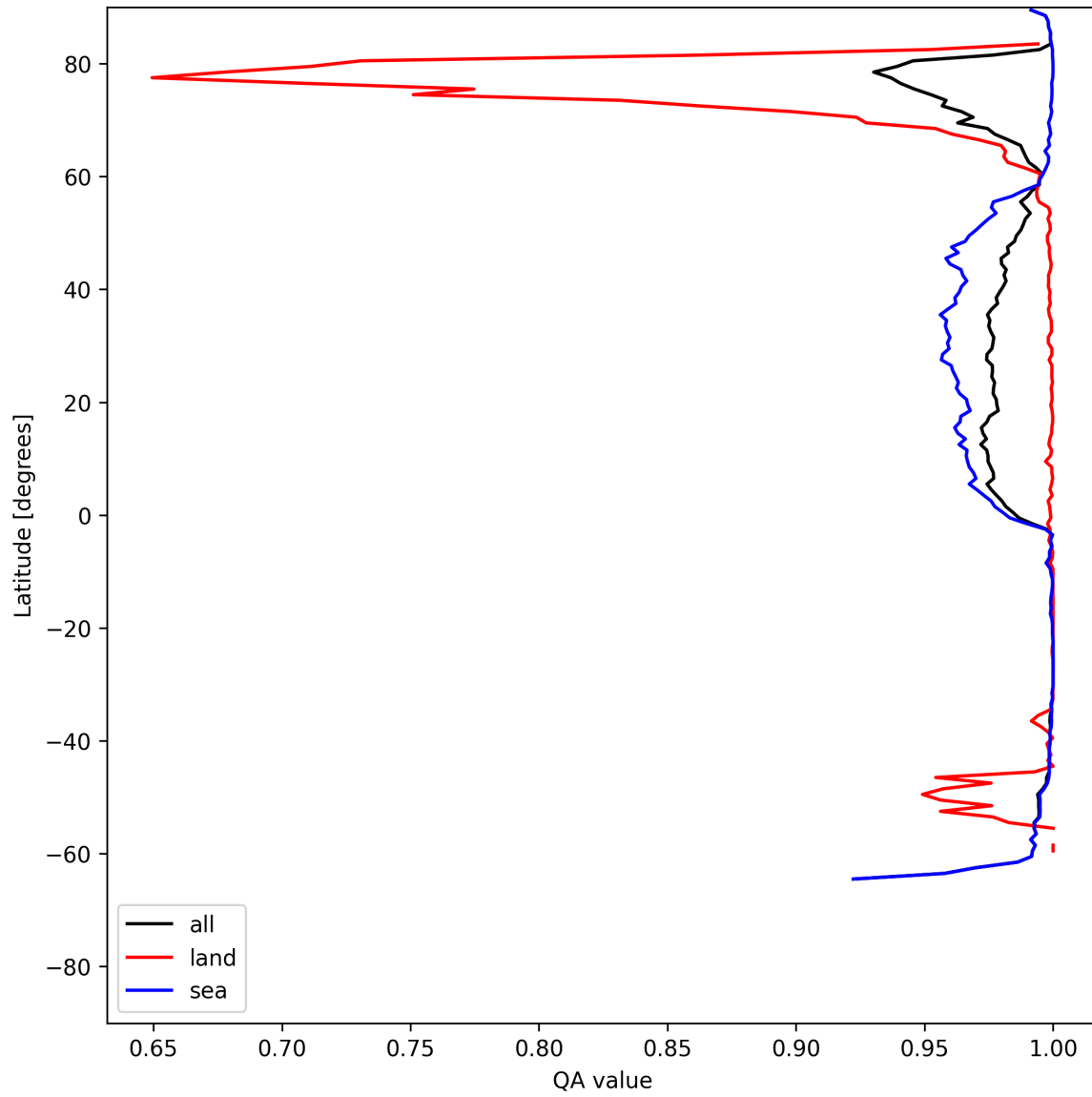
Figure 10: Zonal average of “QA value” for 2025-06-25 to 2025-06-25.
