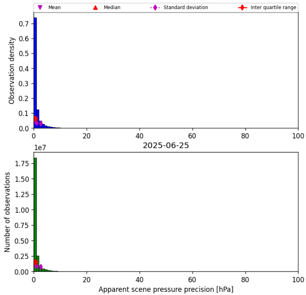
Figure 35: Histogram of “Apparent scene pressure precision” for 2025-06-25 to 2025-06-25
