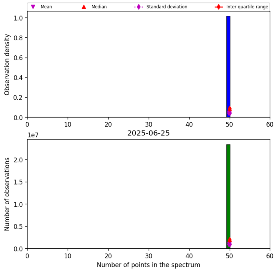
Figure 42: Histogram of "Number of points in the spectrum" for 2025-06-25 to 2025-06-25
