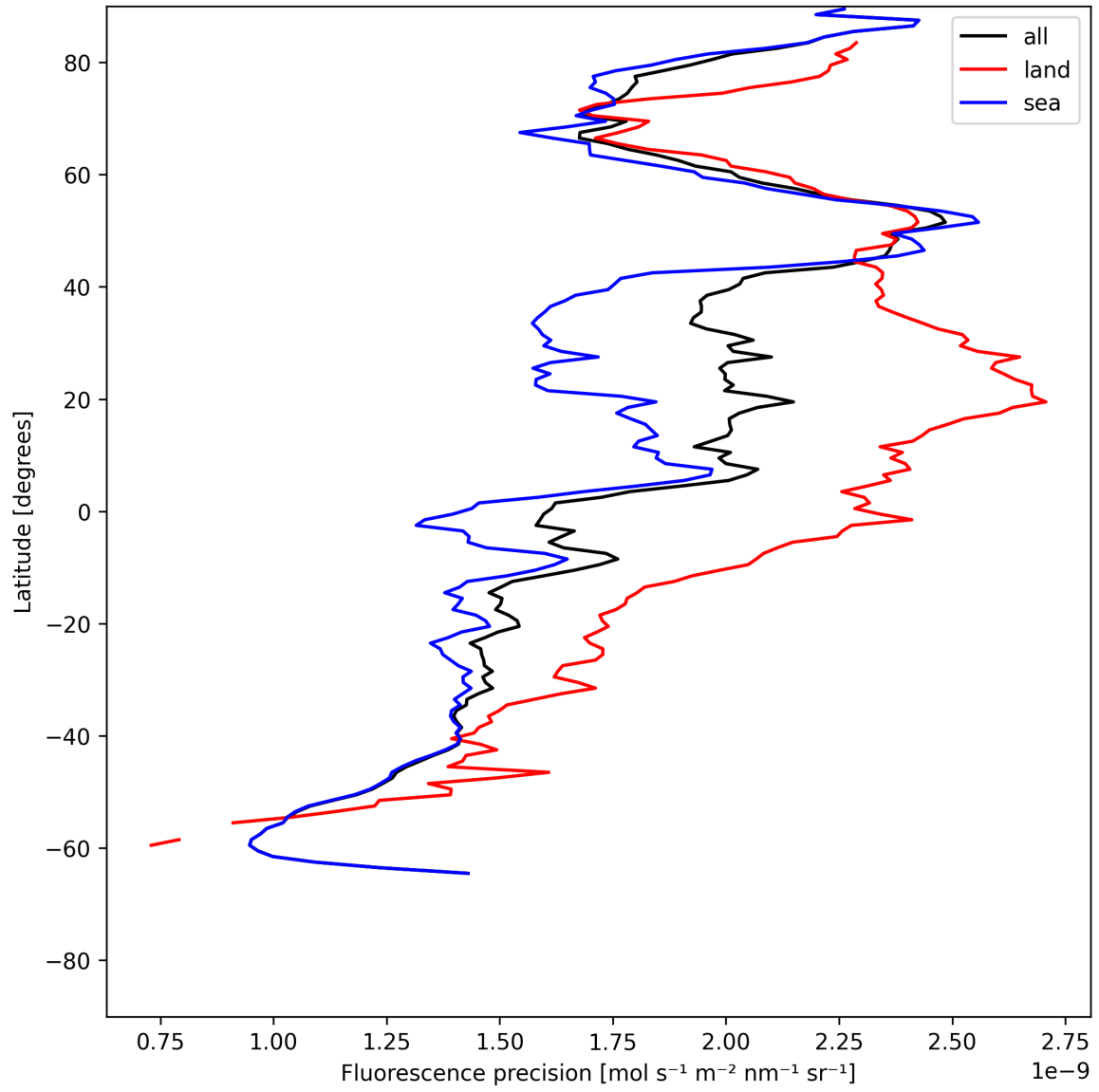
Figure 22: Zonal average of “Fluorescence precision” for 2025-06-25 to 2025-06-25.
