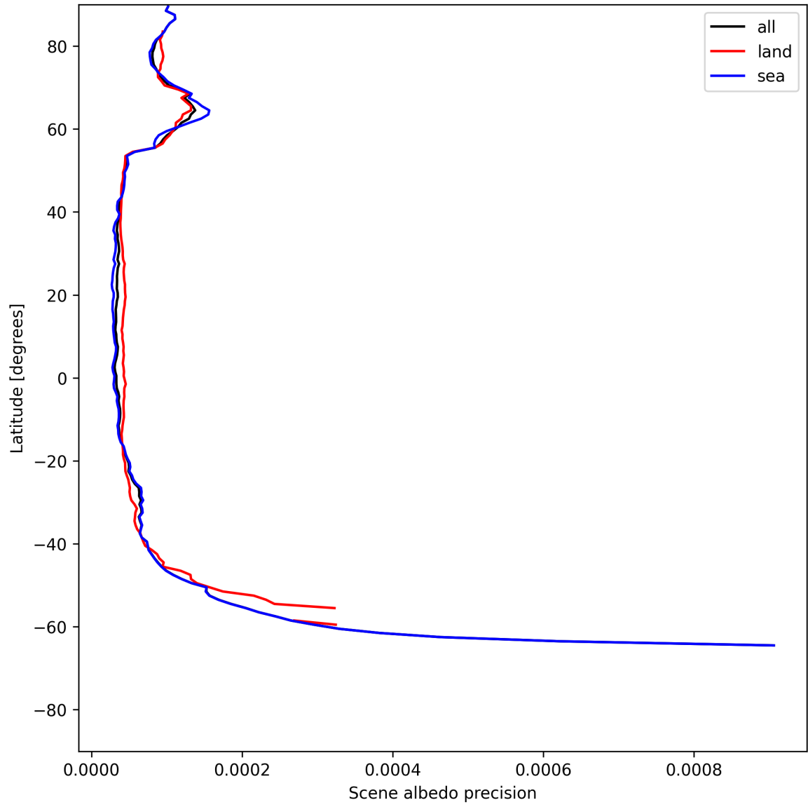
Figure 16: Zonal average of “Scene albedo precision” for 2025-06-25 to 2025-06-25.
