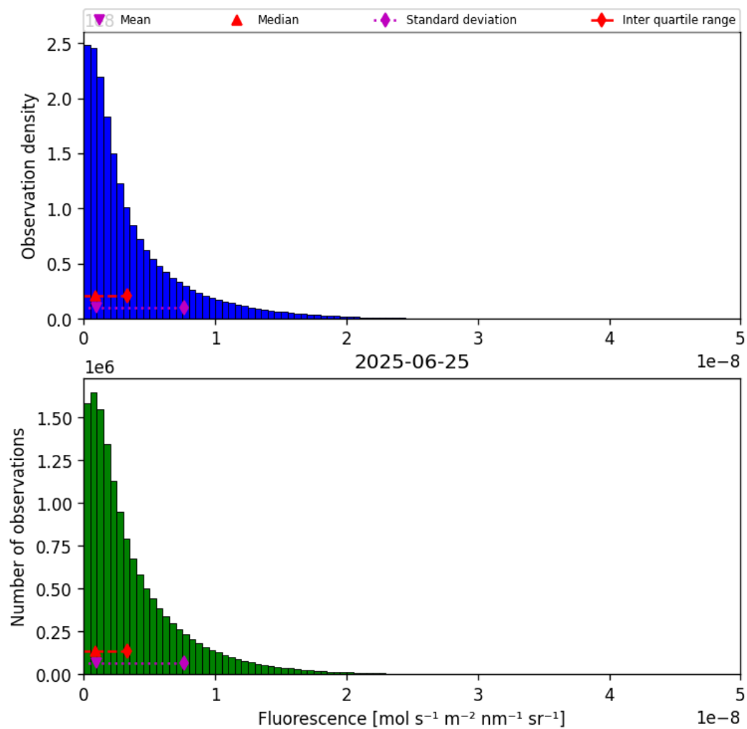
Figure 38: Histogram of “Fluorescence” for 2025-06-25 to 2025-06-25
