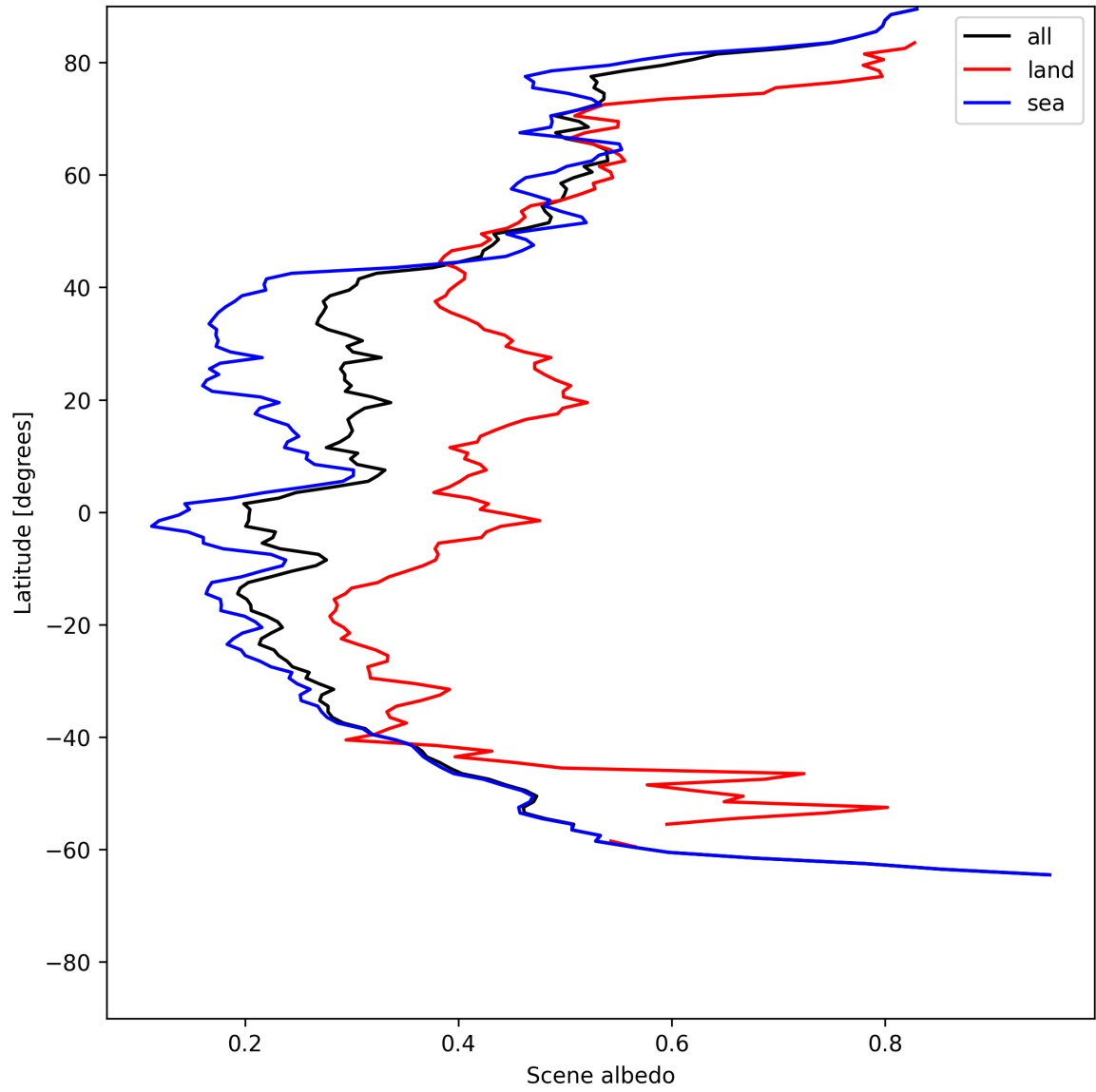
Figure 15: Zonal average of “Scene albedo” for 2025-06-25 to 2025-06-25.
