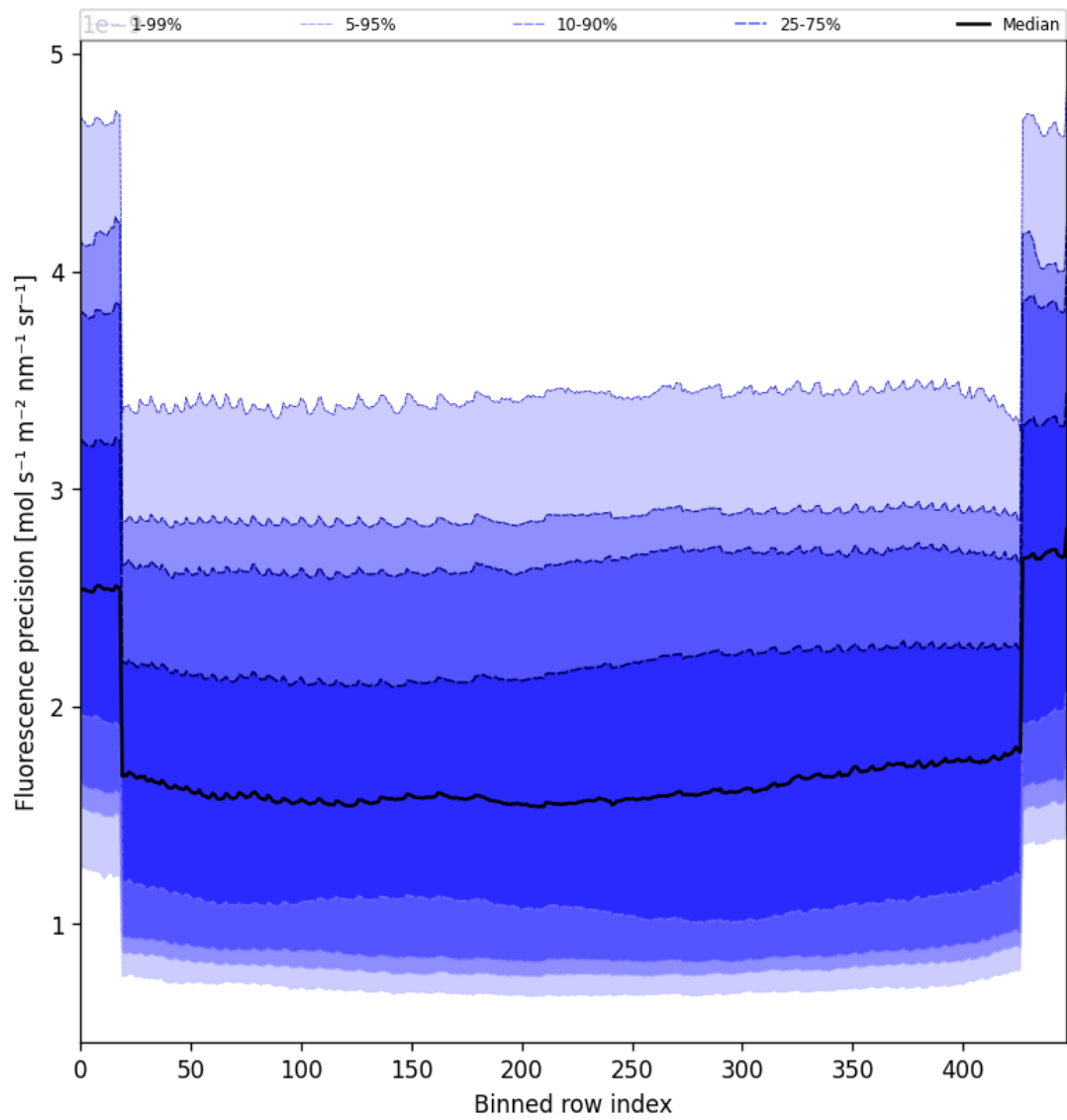
Figure 56: Along track statistics of “Fluorescence precision” for 2025-06-25 to 2025-06-25
