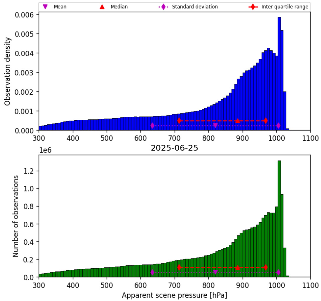
Figure 34: Histogram of “Apparent scene pressure” for 2025-06-25 to 2025-06-25
