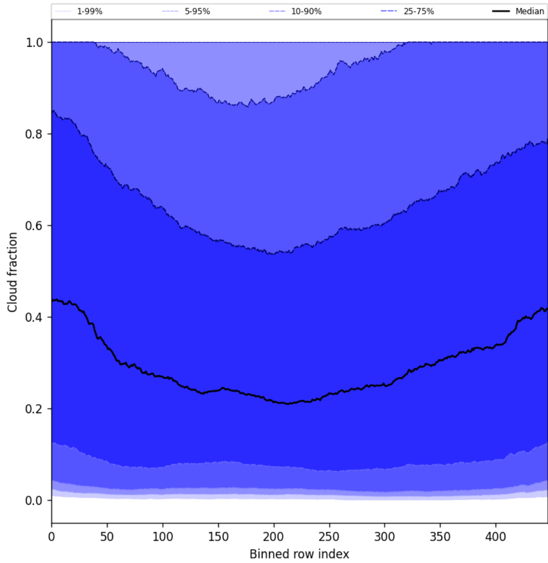
Figure 47: Along track statistics of “Cloud fraction” for 2025-06-25 to 2025-06-25
