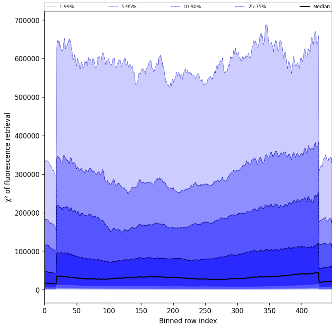
Figure 57: Along track statistics of “ \chi^2 of fluorescence retrieval” for 2025-06-25 to 2025-06-25
