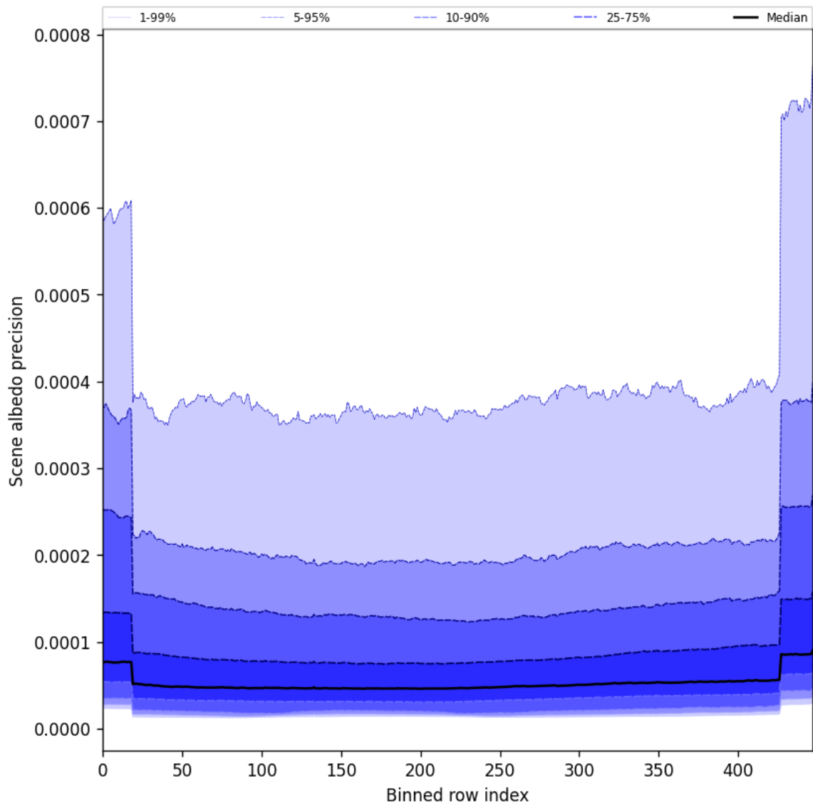
Figure 50: Along track statistics of “Scene albedo precision” for 2025-06-25 to 2025-06-25
