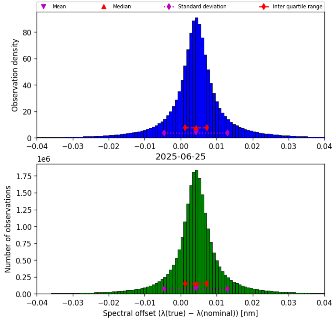
Figure 43: Histogram of “Spectral offset ( \lambda_{\text{true}} - \lambda_{\text{nominal}} )” for 2025-06-25 to 2025-06-25
