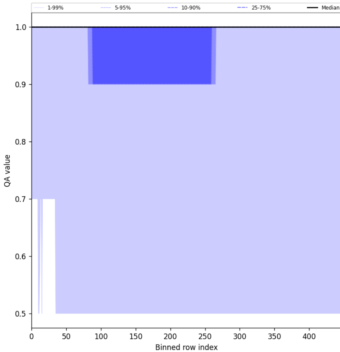
Figure 44: Along track statistics of “QA value” for 2025-06-25 to 2025-06-25
