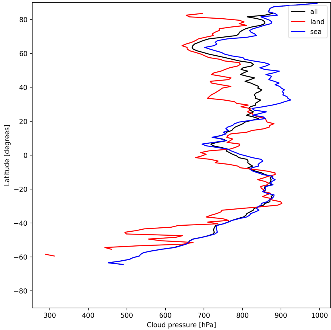
Figure 11: Zonal average of “Cloud pressure” for 2025-06-25 to 2025-06-25.
