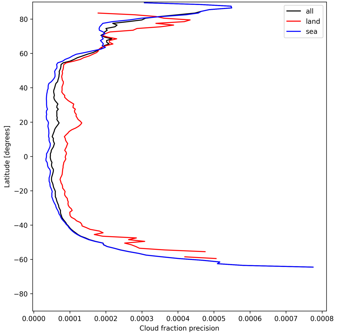
Figure 14: Zonal average of “Cloud fraction precision” for 2025-06-25 to 2025-06-25.
