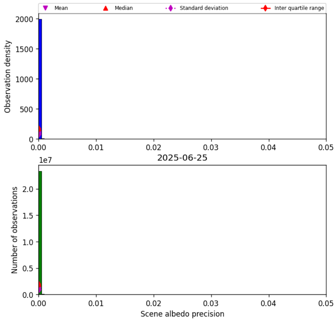
Figure 33: Histogram of “Scene albedo precision” for 2025-06-25 to 2025-06-25
