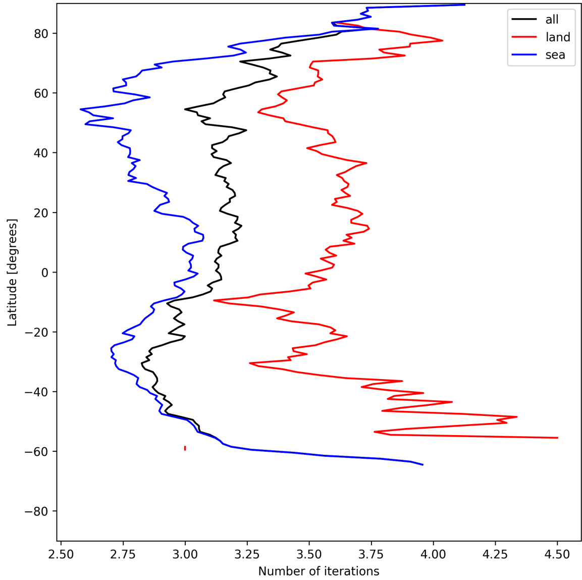
Figure 20: Zonal average of “Number of iterations” for 2025-06-25 to 2025-06-25.
